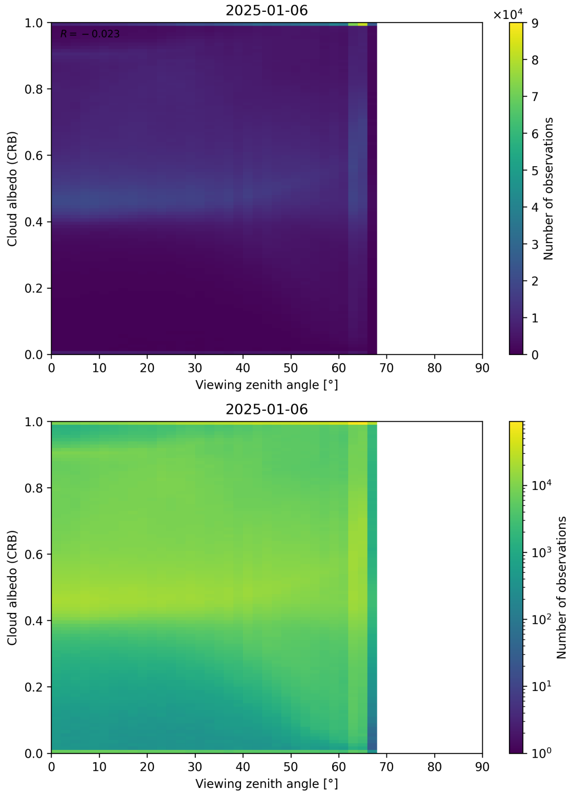
Figure 106: Scatter density plot of “Viewing zenith angle” against “Cloud albedo (CRB)” for 2025-01-05 to 2025-01-07.
