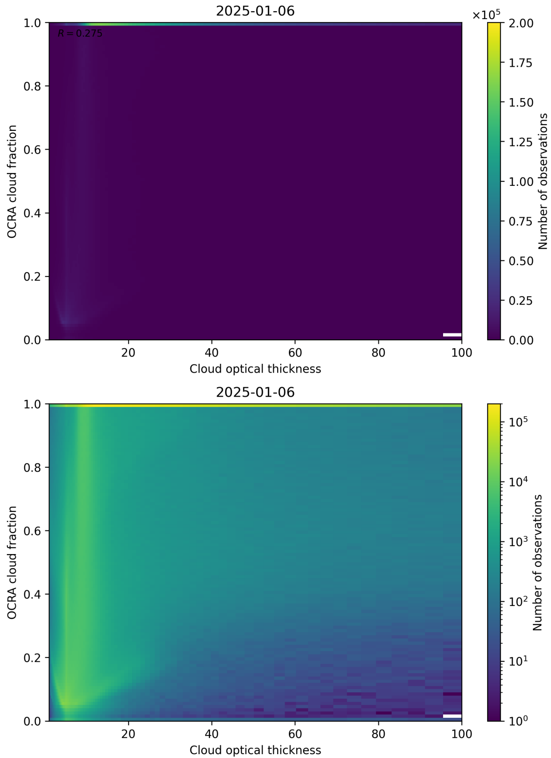
Figure 83: Scatter density plot of “Cloud optical thickness” against “OCRA cloud fraction” for 2025-01-05 to 2025-01-07.
