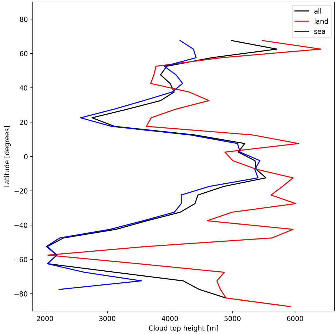
Figure 24: Zonal average of “Cloud top height” for 2025-01-05 to 2025-01-07.
