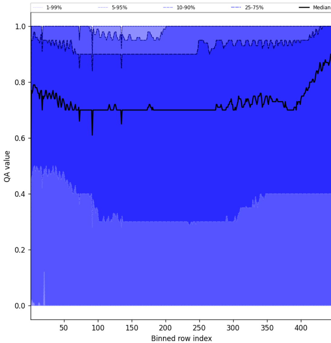
Figure 54: Along track statistics of “QA value” for 2025-01-05 to 2025-01-07
