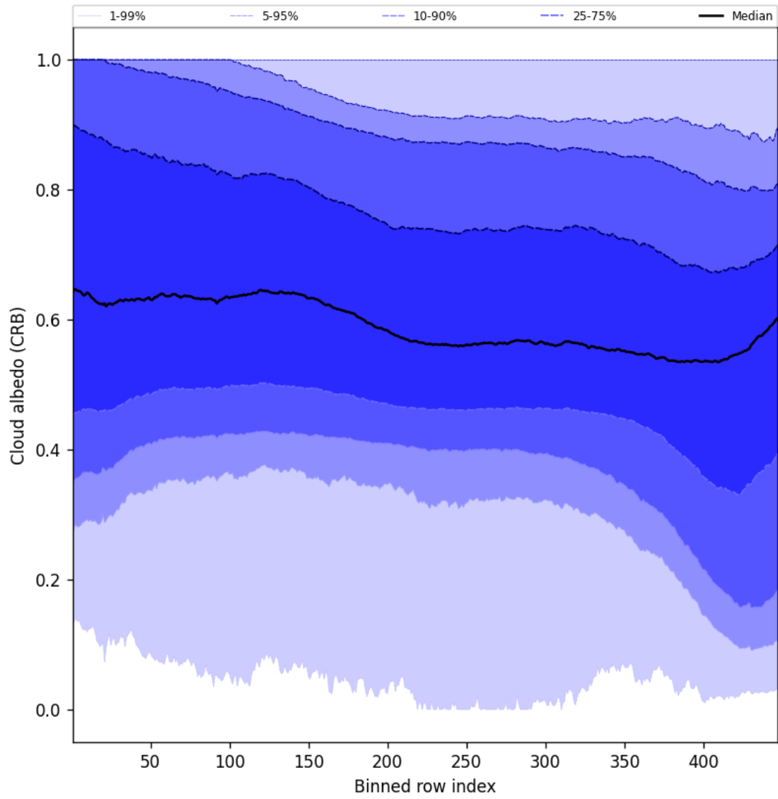
Figure 60: Along track statistics of “Cloud albedo (CRB)” for 2025-01-05 to 2025-01-07
