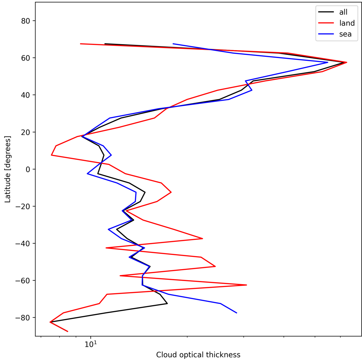
Figure 25: Zonal average of “Cloud optical thickness” for 2025-01-05 to 2025-01-07.
