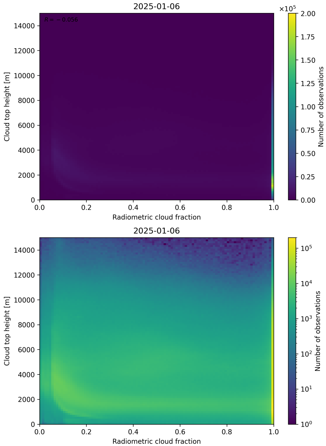
Figure 76: Scatter density plot of “Radiometric cloud fraction” against “Cloud top height” for 2025-01-05 to 2025-01-07.
