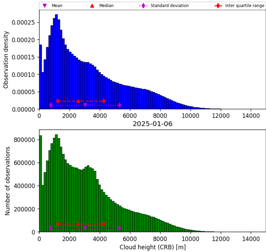
Figure 43: Histogram of “Cloud height (CRB)” for 2025-01-05 to 2025-01-07
