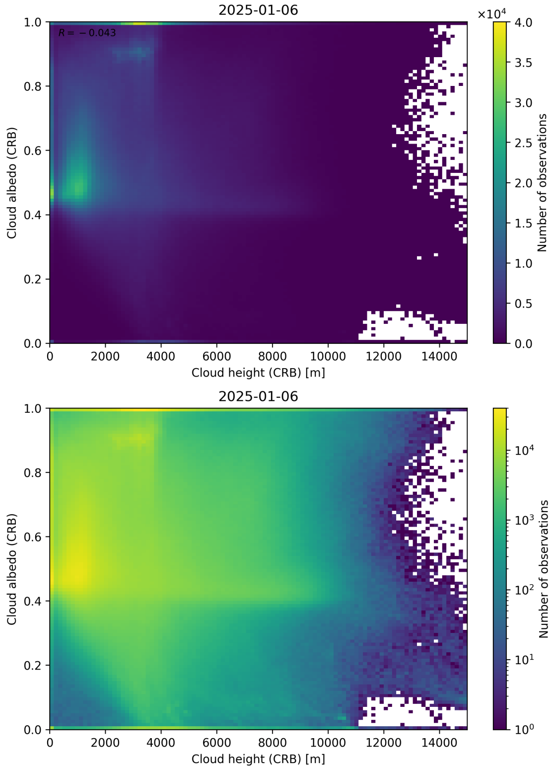
Figure 80: Scatter density plot of “Cloud height (CRB)” against “Cloud albedo (CRB)” for 2025-01-05 to 2025-01-07.
