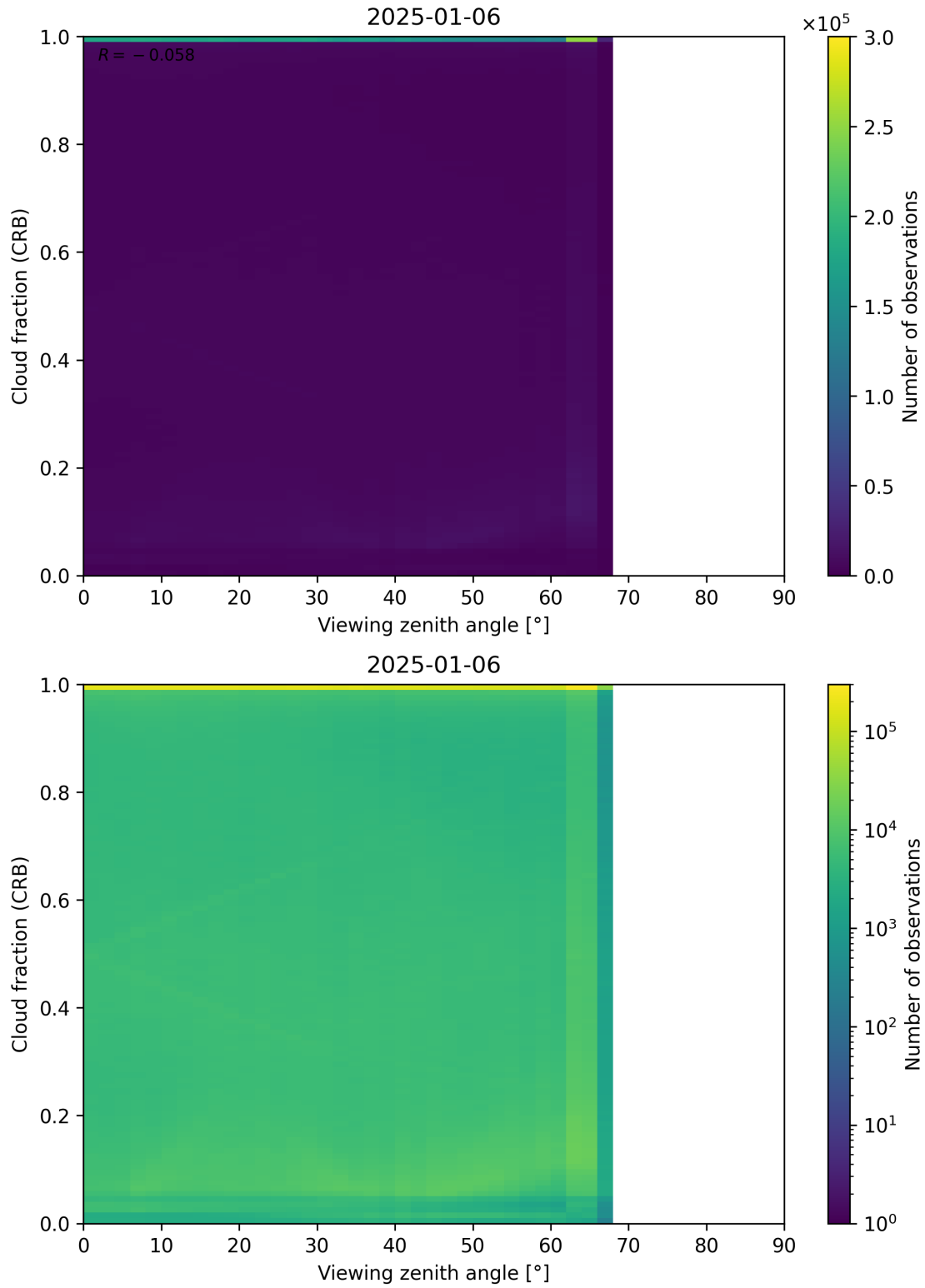
Figure 109: Scatter density plot of “Viewing zenith angle” against “Cloud fraction (CRB)” for 2025-01-05 to 2025-01-07.
