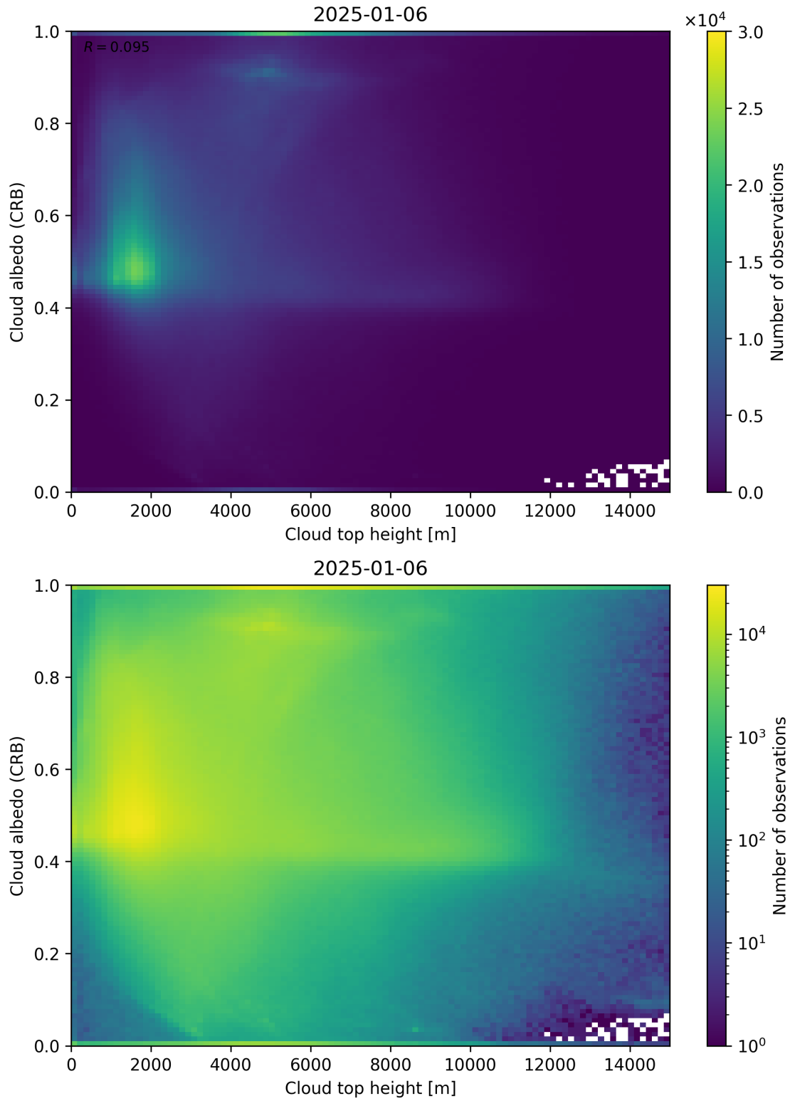
Figure 86: Scatter density plot of “Cloud top height” against “Cloud albedo (CRB)” for 2025-01-05 to 2025-01-07.
