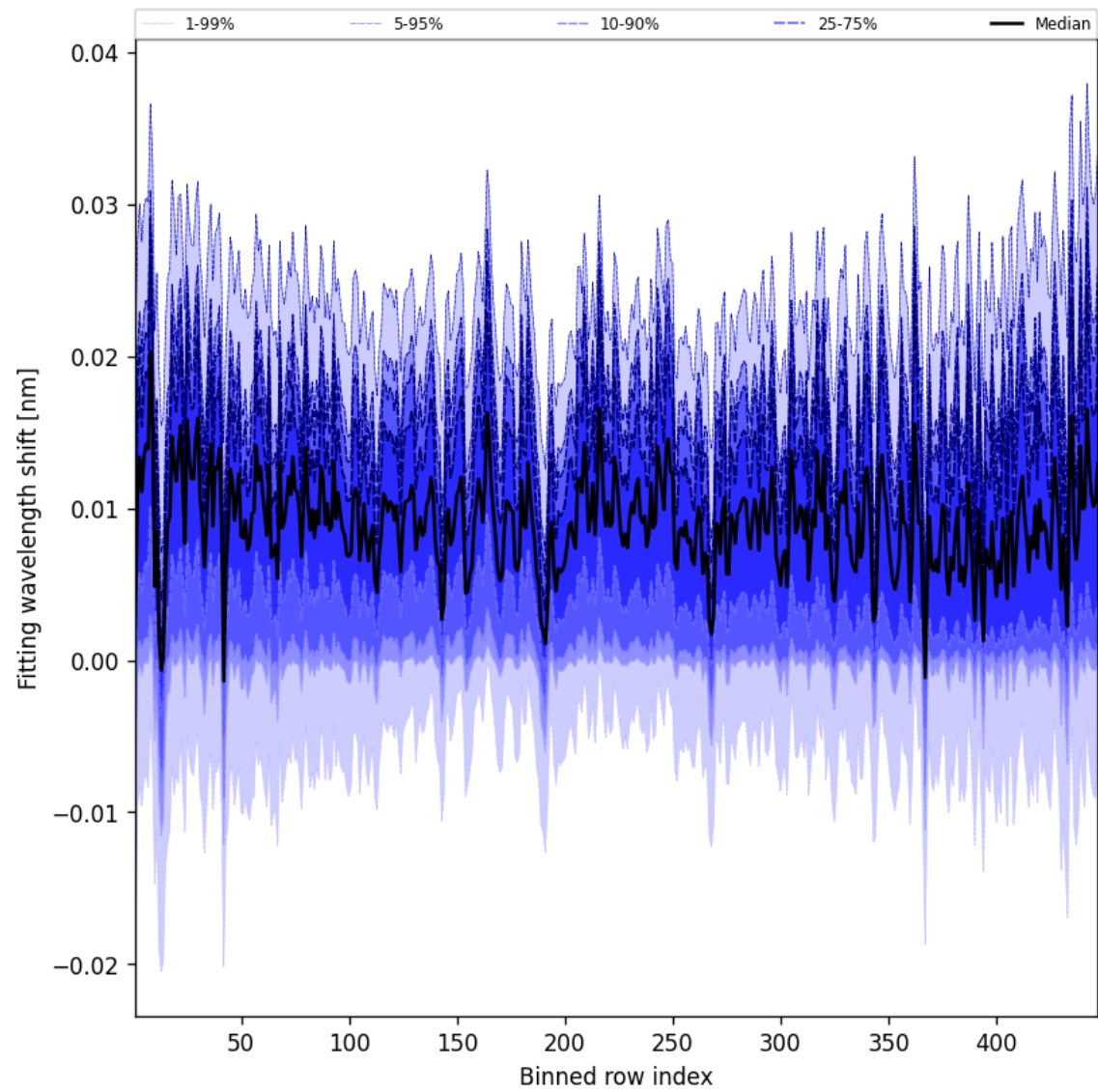
Figure 65: Along track statistics of “Fitting wavelength shift” for 2025-01-05 to 2025-01-07
