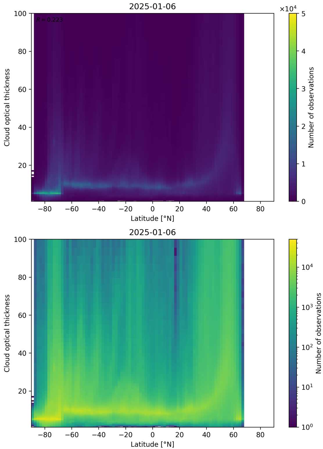
Figure 96: Scatter density plot of “Latitude” against “Cloud optical thickness” for 2025-01-05 to 2025-01-07.
