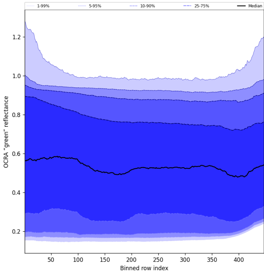
Figure 68: Along track statistics of “OCRA “green” reflectance” for 2025-01-05 to 2025-01-07
