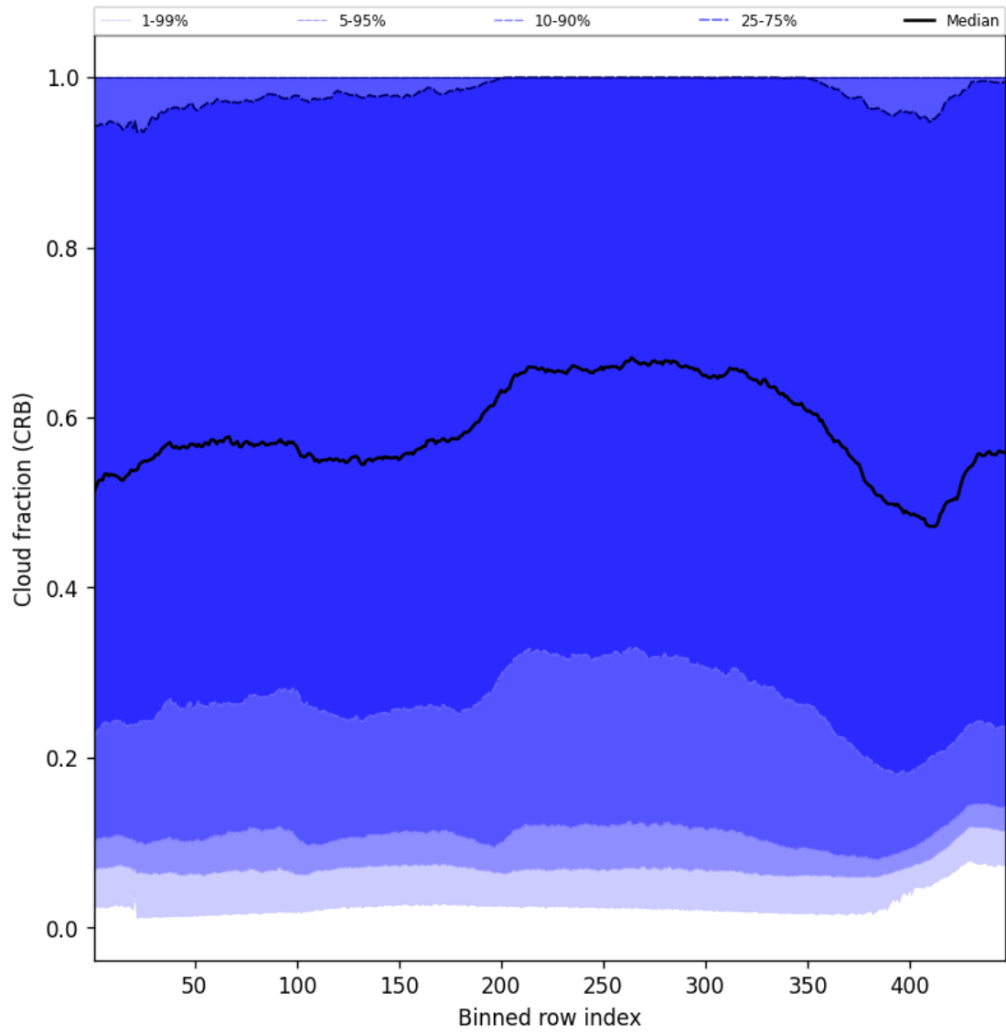
Figure 58: Along track statistics of “Cloud fraction (CRB)” for 2025-01-05 to 2025-01-07
