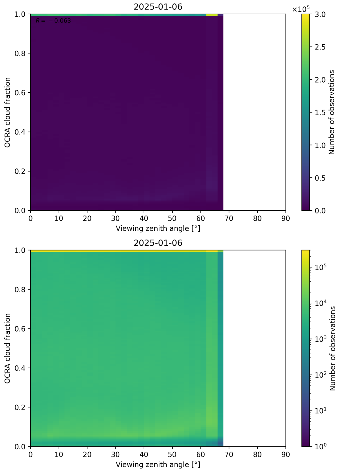
Figure 108: Scatter density plot of “Viewing zenith angle” against “OCRA cloud fraction” for 2025-01-05 to 2025-01-07.
