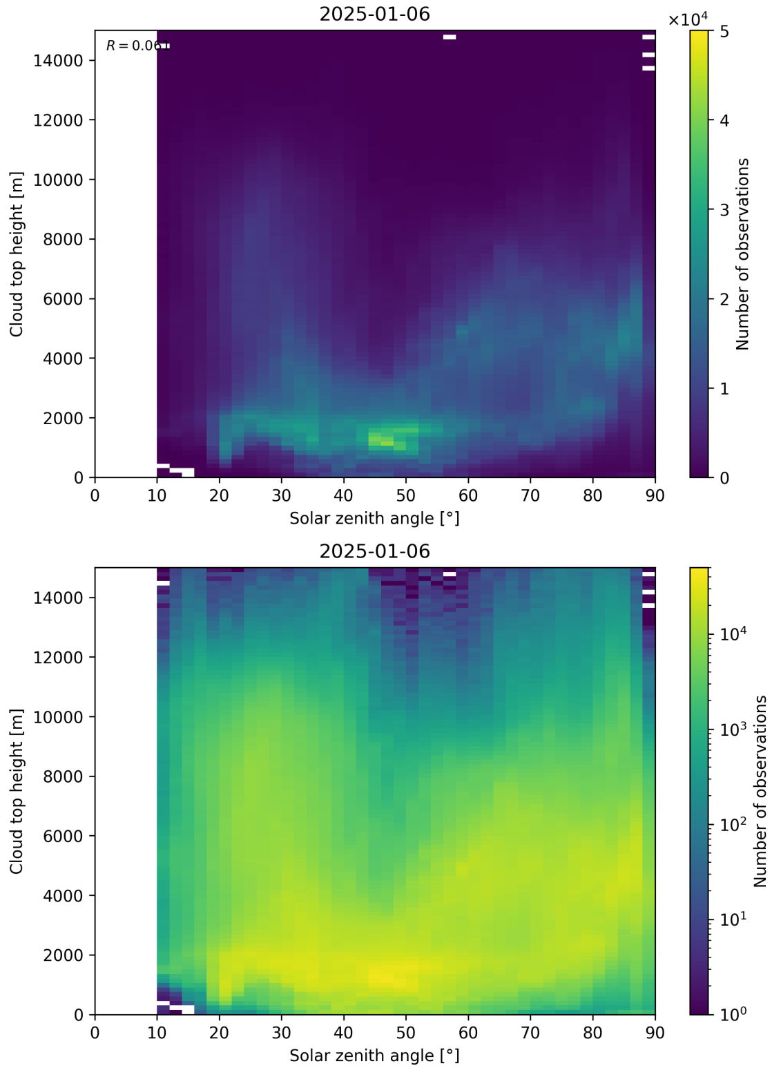
Figure 104: Scatter density plot of “Solar zenith angle” against “Cloud top height” for 2025-01-05 to 2025-01-07.
