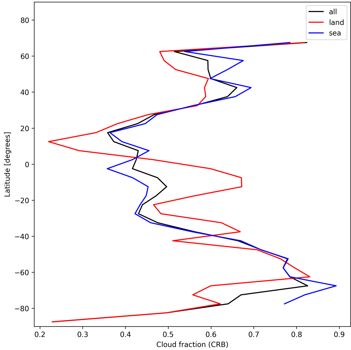
Figure 26: Zonal average of “Cloud fraction (CRB)” for 2025-01-05 to 2025-01-07.
