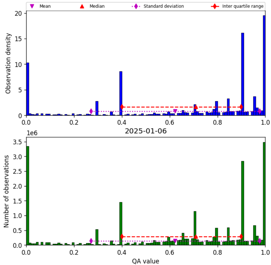
Figure 38: Histogram of “QA value” for 2025-01-05 to 2025-01-07
