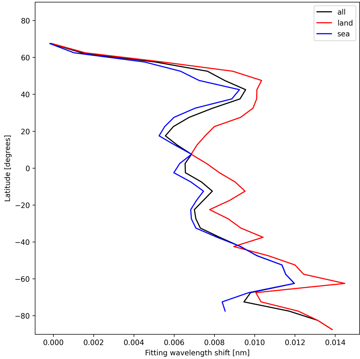
Figure 33: Zonal average of “Fitting wavelength shift” for 2025-01-05 to 2025-01-07.
