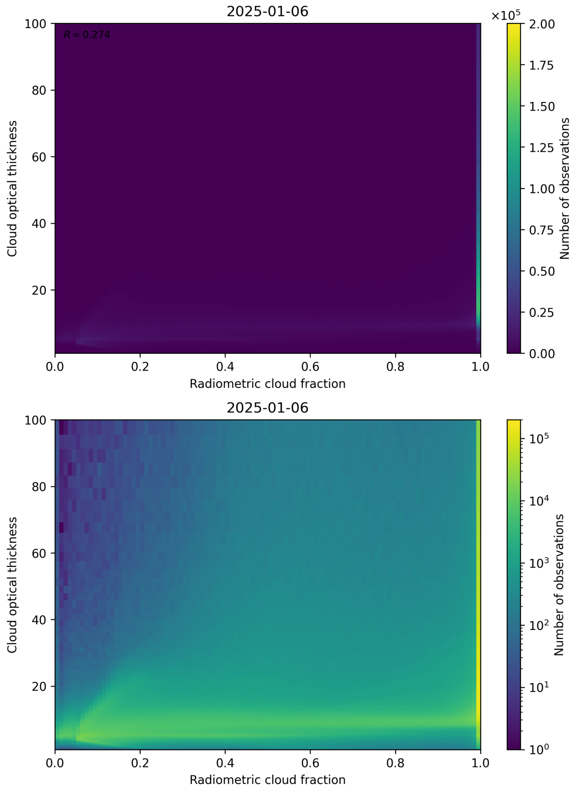
Figure 75: Scatter density plot of “Radiometric cloud fraction” against “Cloud optical thickness” for 2025-01-05 to 2025-01-07.
