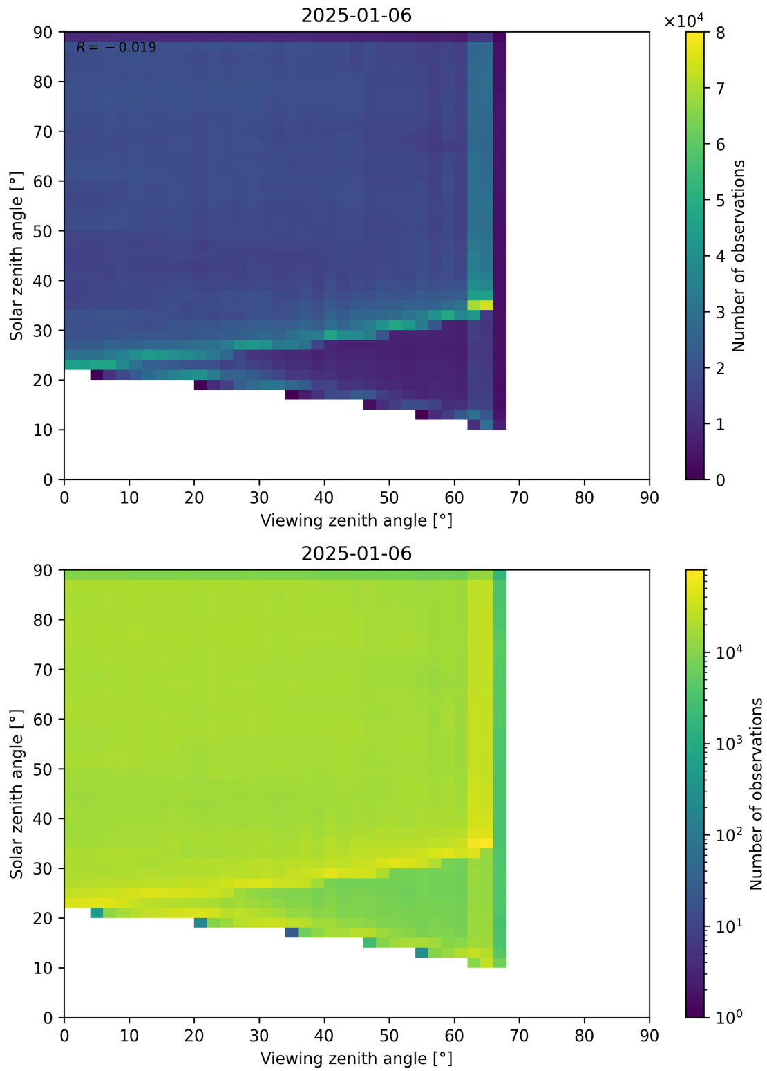
Figure 114: Scatter density plot of “Viewing zenith angle” against “Solar zenith angle” for 2025-01-05 to 2025-01-07.
