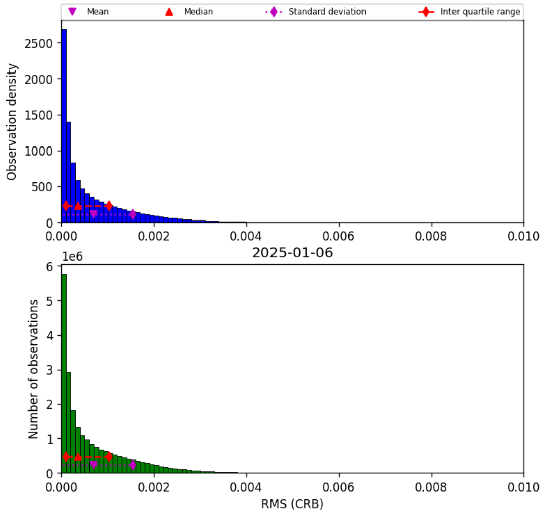
Figure 48: Histogram of “RMS (CRB)” for 2025-01-05 to 2025-01-07
