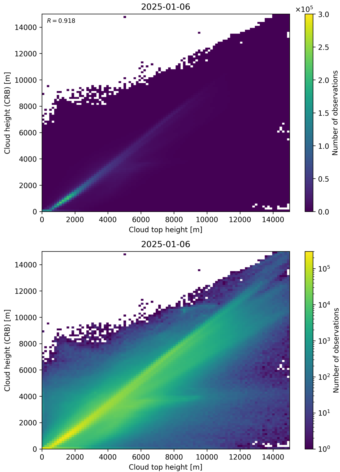
Figure 89: Scatter density plot of “Cloud top height” against “Cloud height (CRB)” for 2025-01-05 to 2025-01-07.
