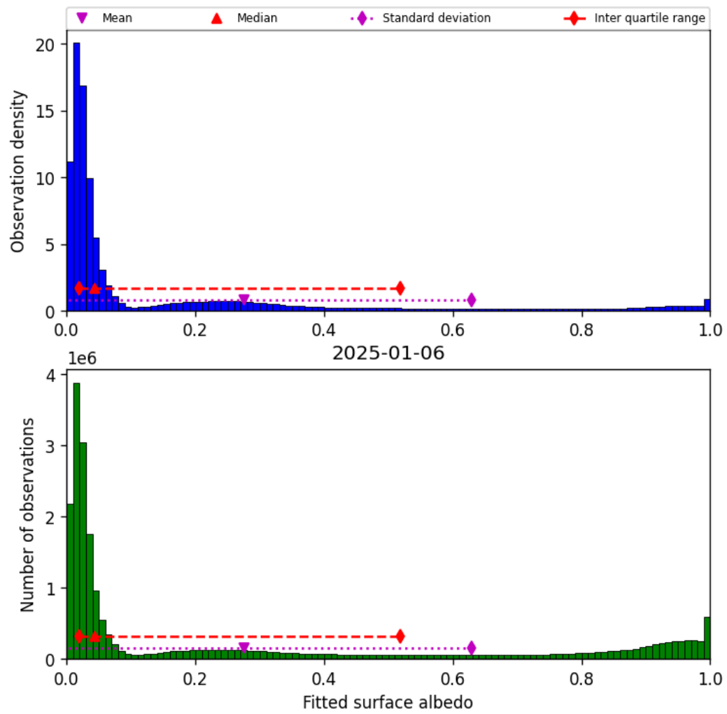
Figure 45: Histogram of “Fitted surface albedo” for 2025-01-05 to 2025-01-07
