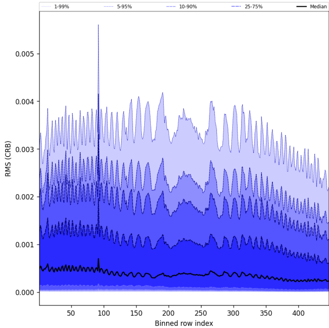
Figure 64: Along track statistics of “RMS (CRB)” for 2025-01-05 to 2025-01-07
