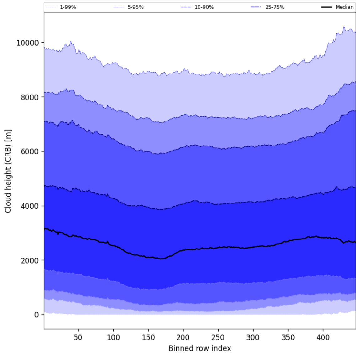
Figure 59: Along track statistics of “Cloud height (CRB)” for 2025-01-05 to 2025-01-07
