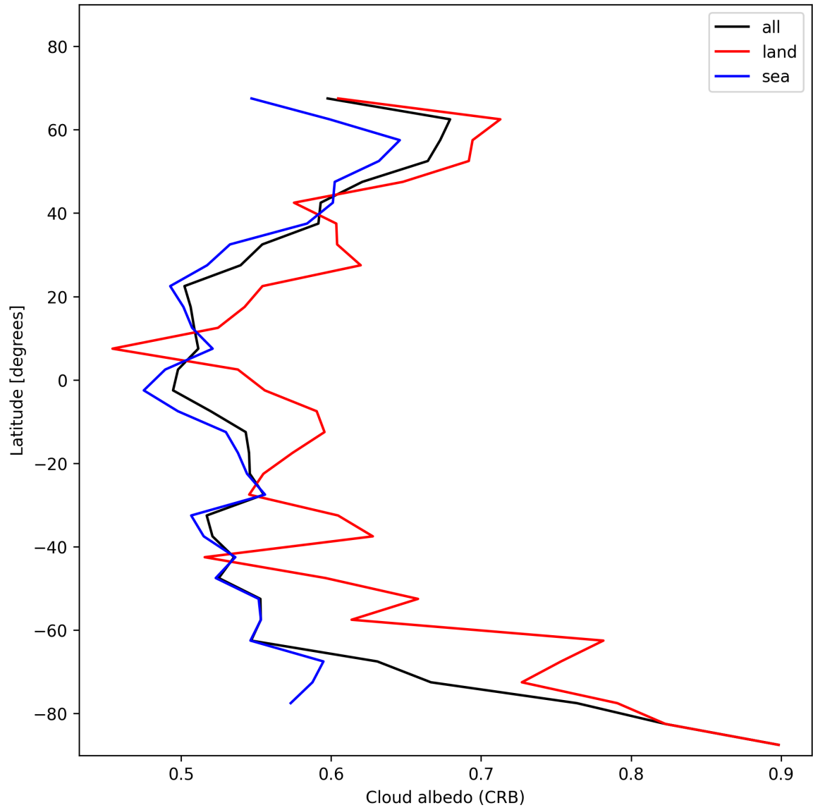
Figure 28: Zonal average of “Cloud albedo (CRB)” for 2025-01-05 to 2025-01-07.
