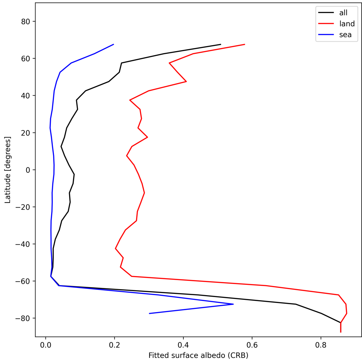
Figure 30: Zonal average of “Fitted surface albedo (CRB)” for 2025-01-05 to 2025-01-07.
