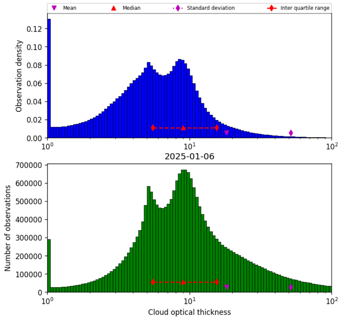
Figure 41: Histogram of “Cloud optical thickness” for 2025-01-05 to 2025-01-07
