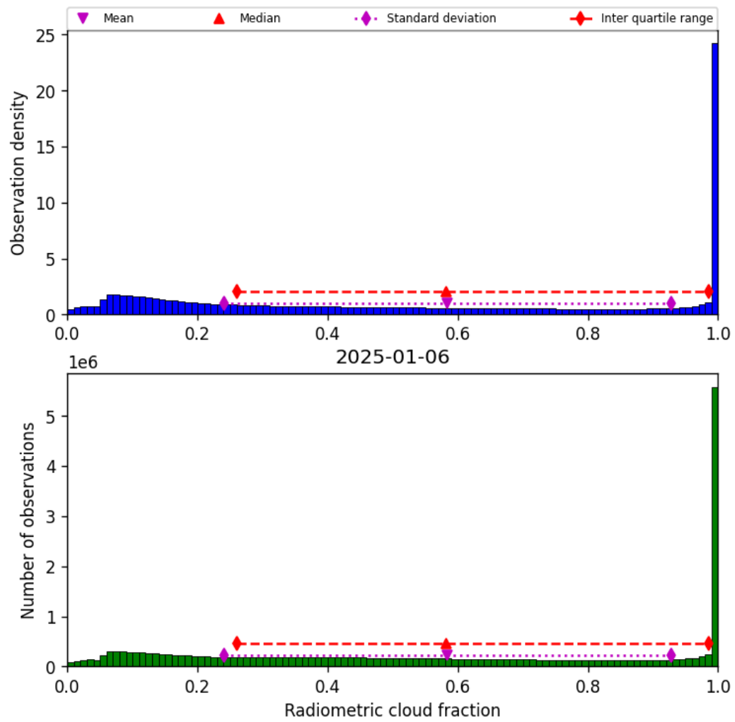
Figure 39: Histogram of “Radiometric cloud fraction” for 2025-01-05 to 2025-01-07
