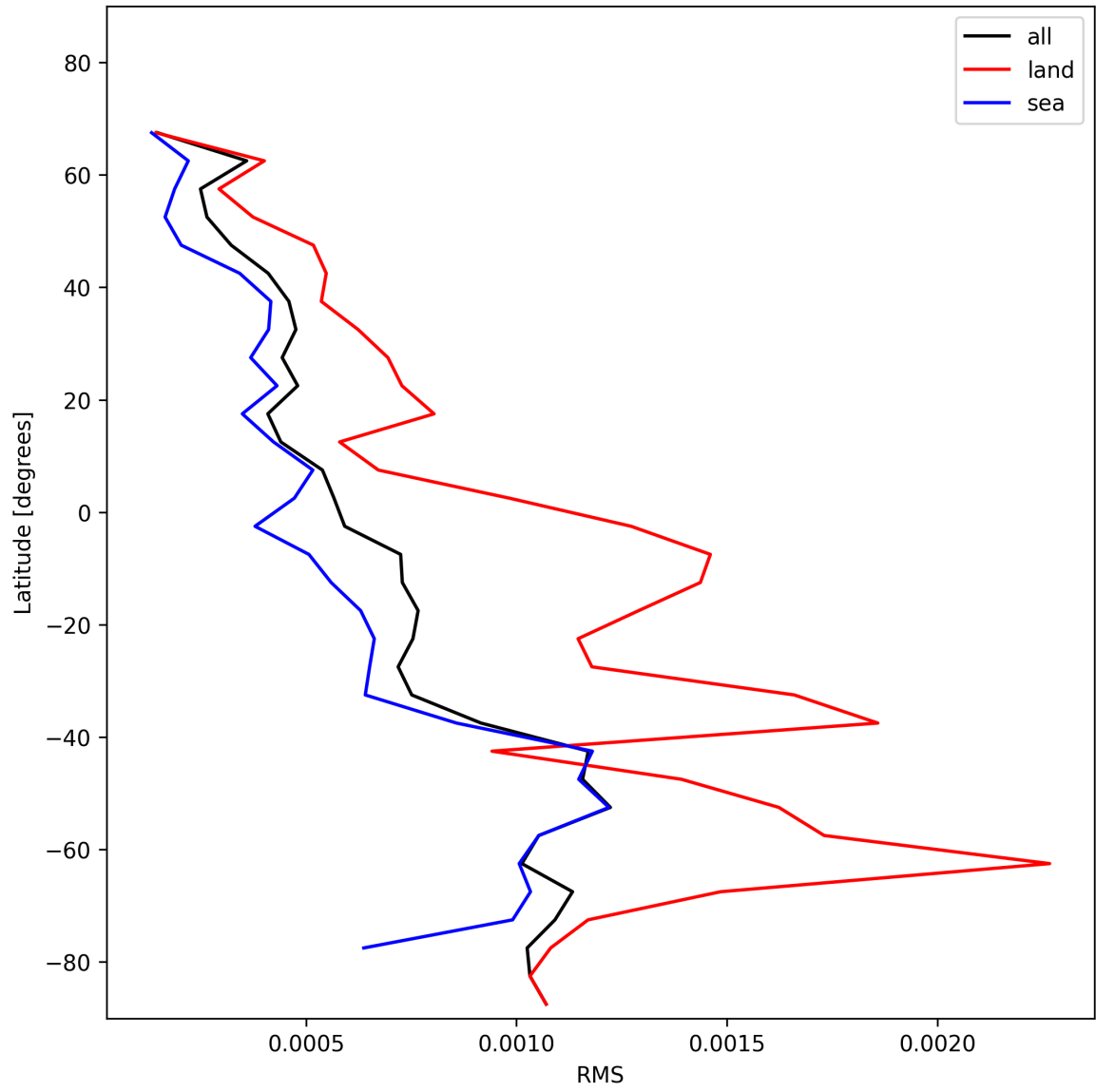
Figure 31: Zonal average of “RMS” for 2025-01-05 to 2025-01-07.
