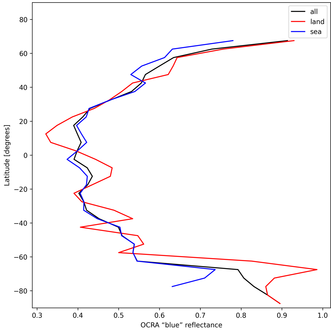
Figure 35: Zonal average of “OCRA “blue” reflectance” for 2025-01-05 to 2025-01-07.
