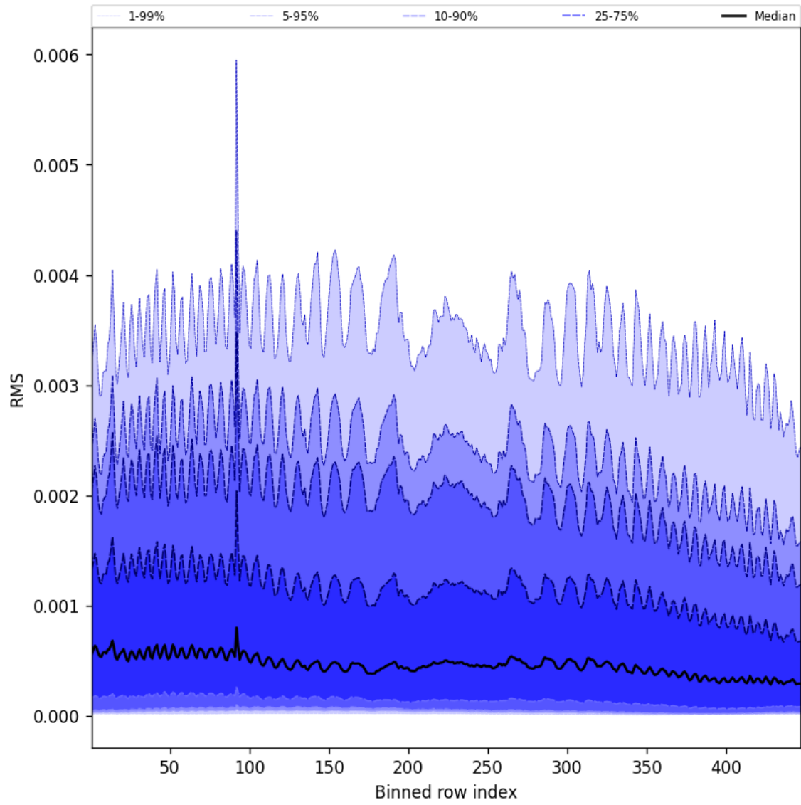
Figure 63: Along track statistics of “RMS” for 2025-01-05 to 2025-01-07
