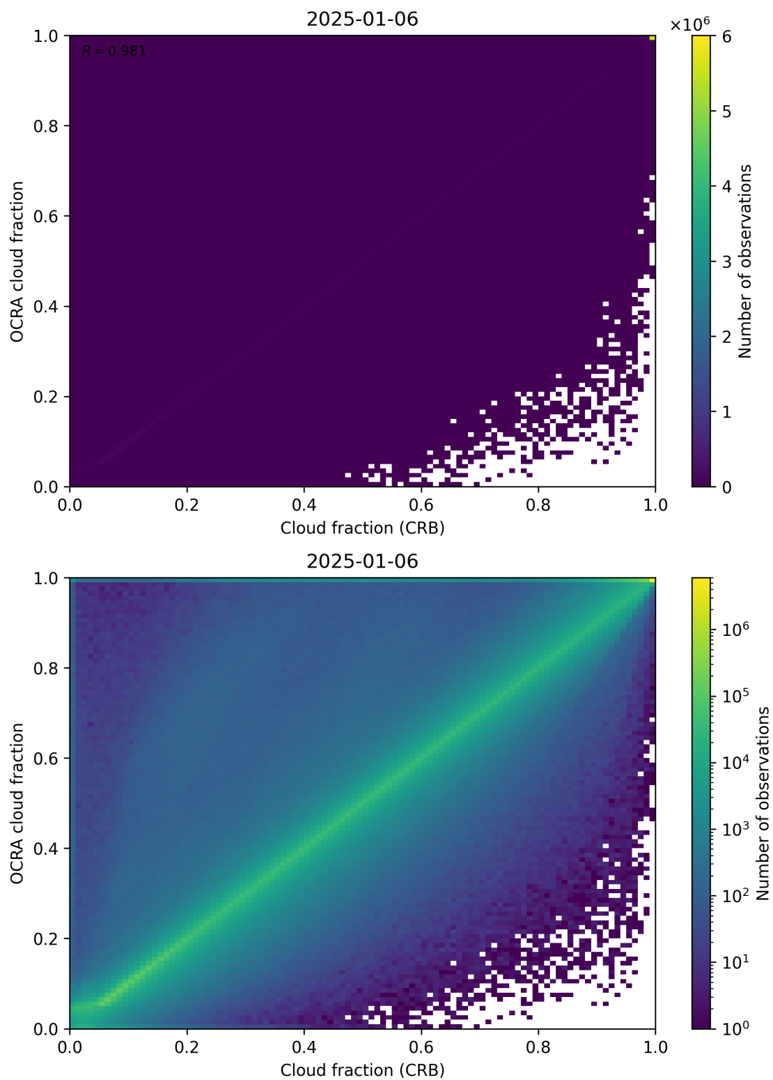
Figure 78: Scatter density plot of “Cloud fraction (CRB)” against “OCRA cloud fraction” for 2025-01-05 to 2025-01-07.
