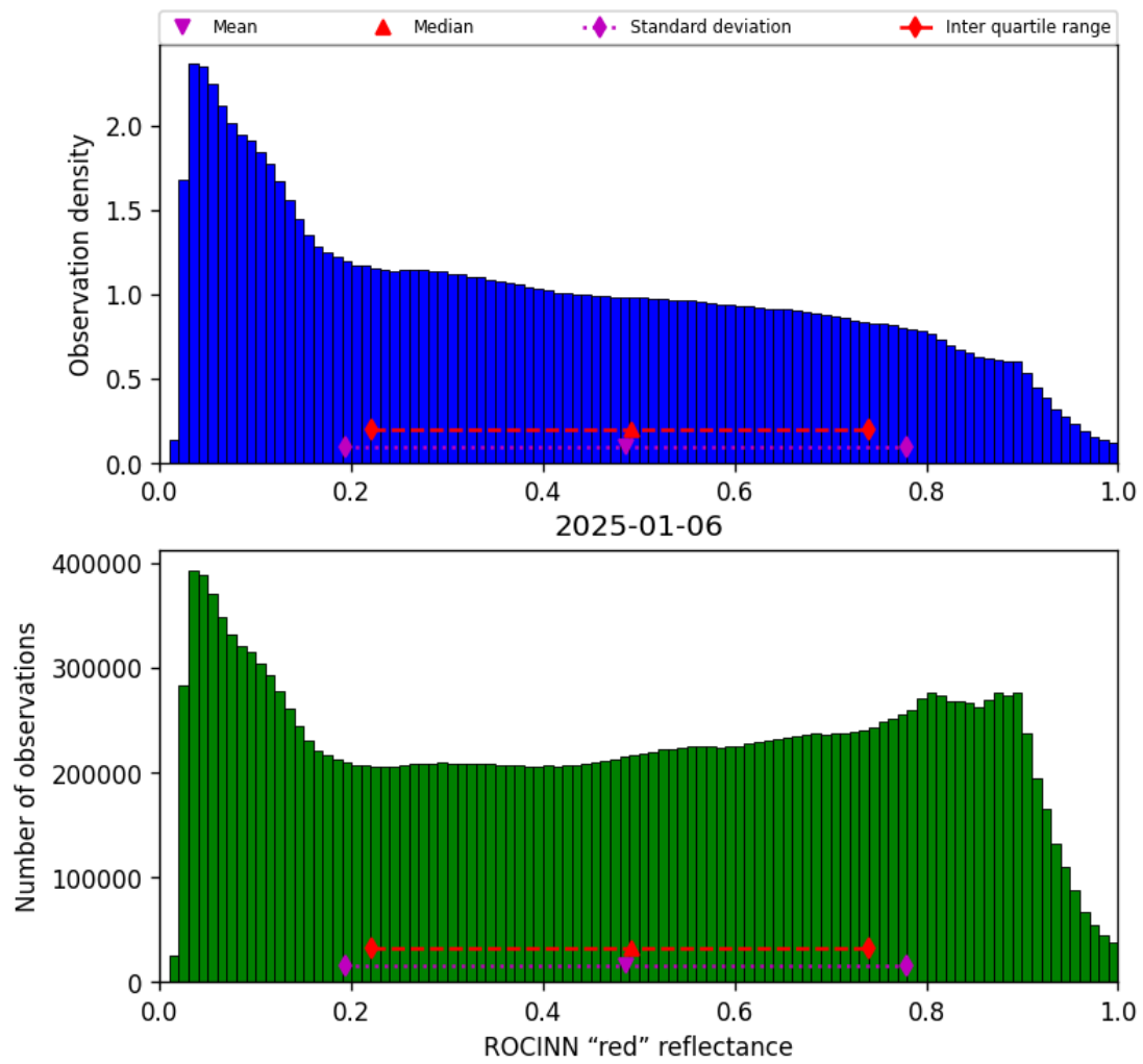
Figure 53: Histogram of “ROCINN “red” reflectance” for 2025-01-05 to 2025-01-07
