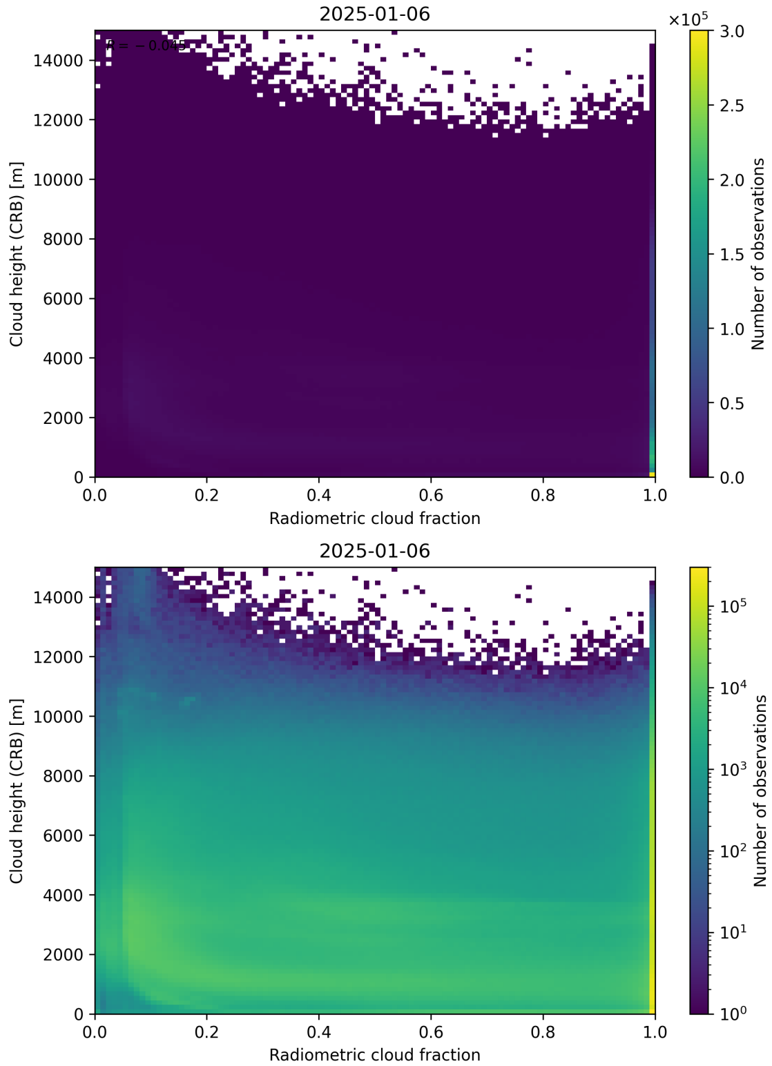
Figure 74: Scatter density plot of “Radiometric cloud fraction” against “Cloud height (CRB)” for 2025-01-05 to 2025-01-07.
