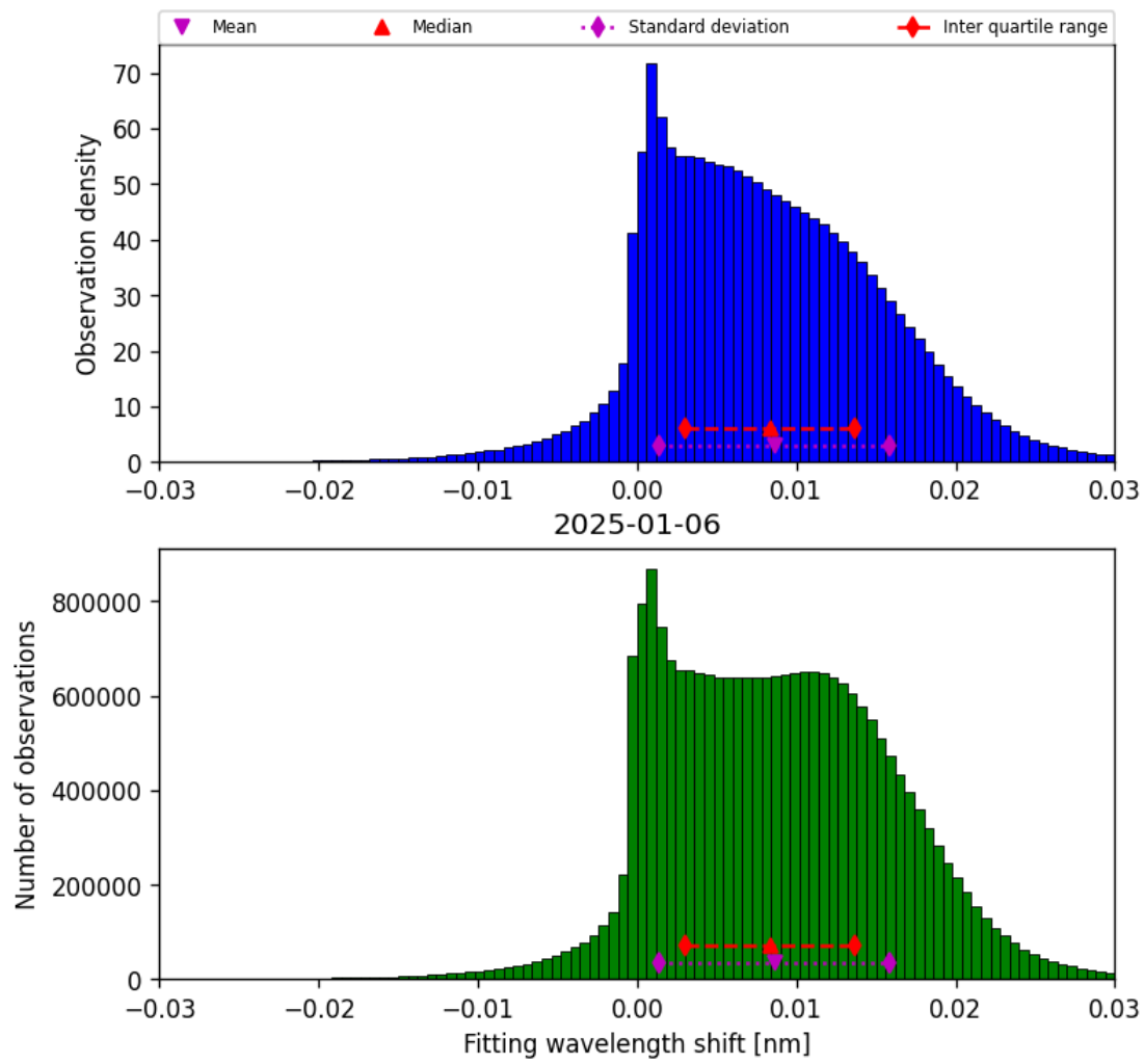
Figure 49: Histogram of “Fitting wavelength shift” for 2025-01-05 to 2025-01-07
