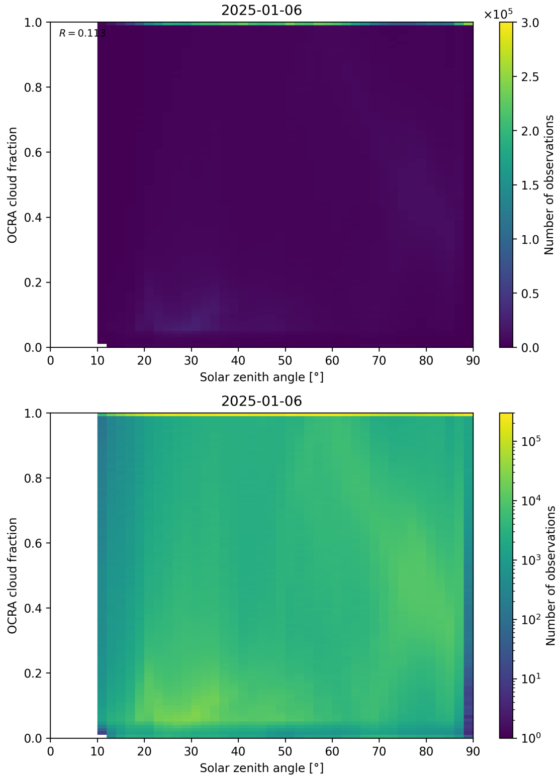
Figure 100: Scatter density plot of “Solar zenith angle” against “OCRA cloud fraction” for 2025-01-05 to 2025-01-07.
