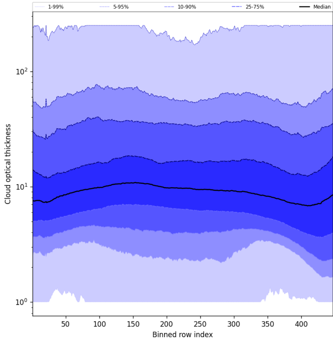
Figure 57: Along track statistics of “Cloud optical thickness” for 2025-01-05 to 2025-01-07
