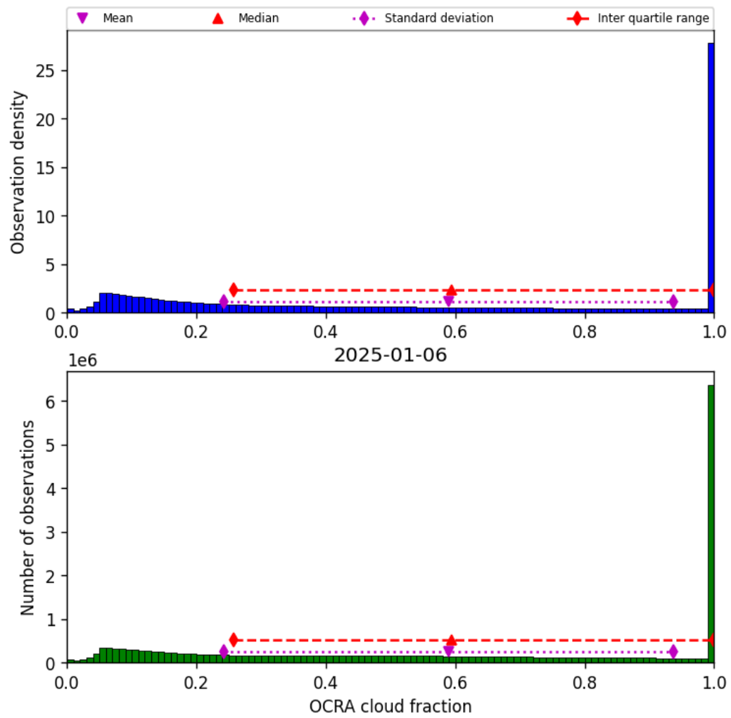
Figure 50: Histogram of “OCRA cloud fraction” for 2025-01-05 to 2025-01-07
