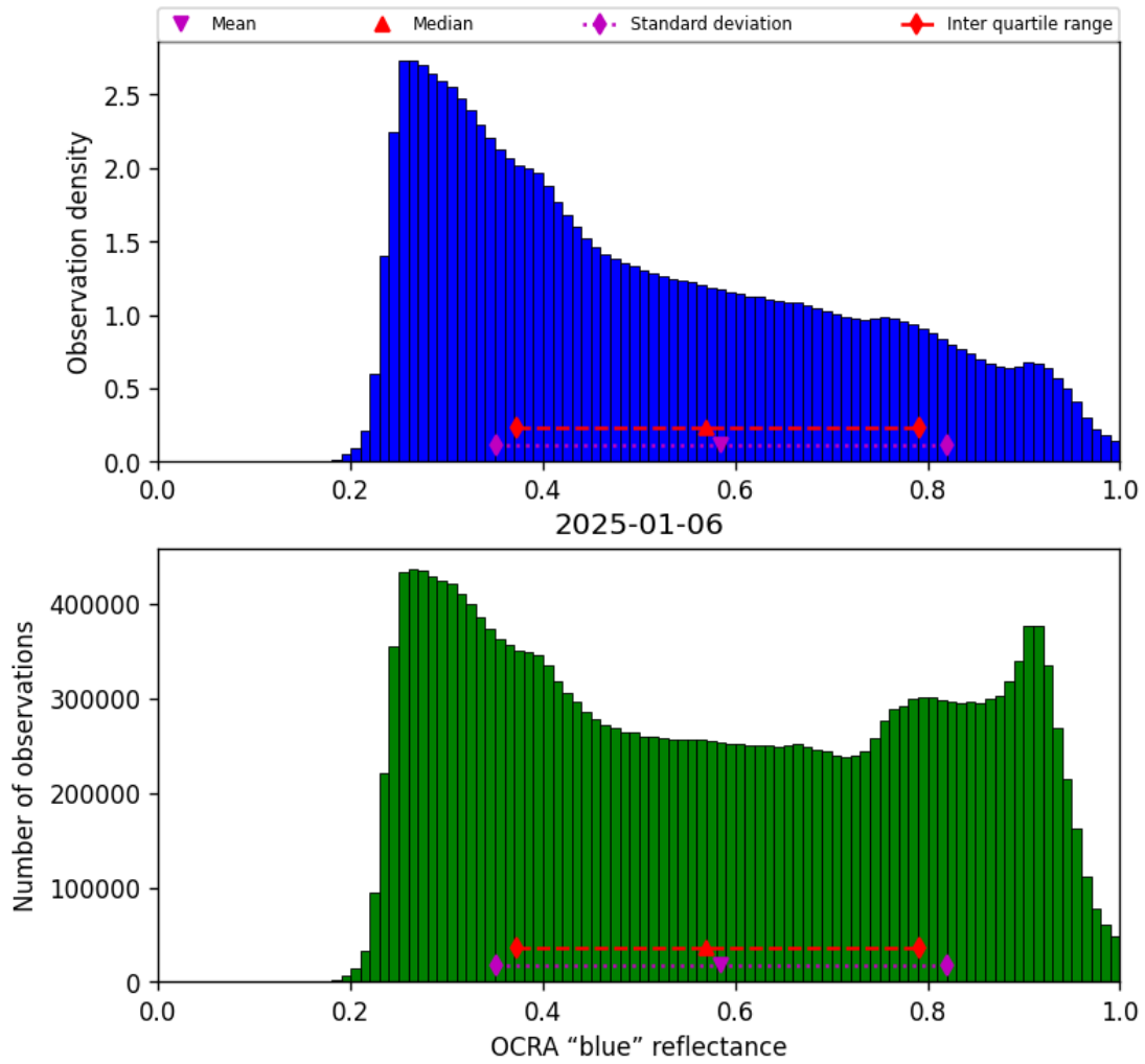
Figure 51: Histogram of “OCRA “blue” reflectance” for 2025-01-05 to 2025-01-07
