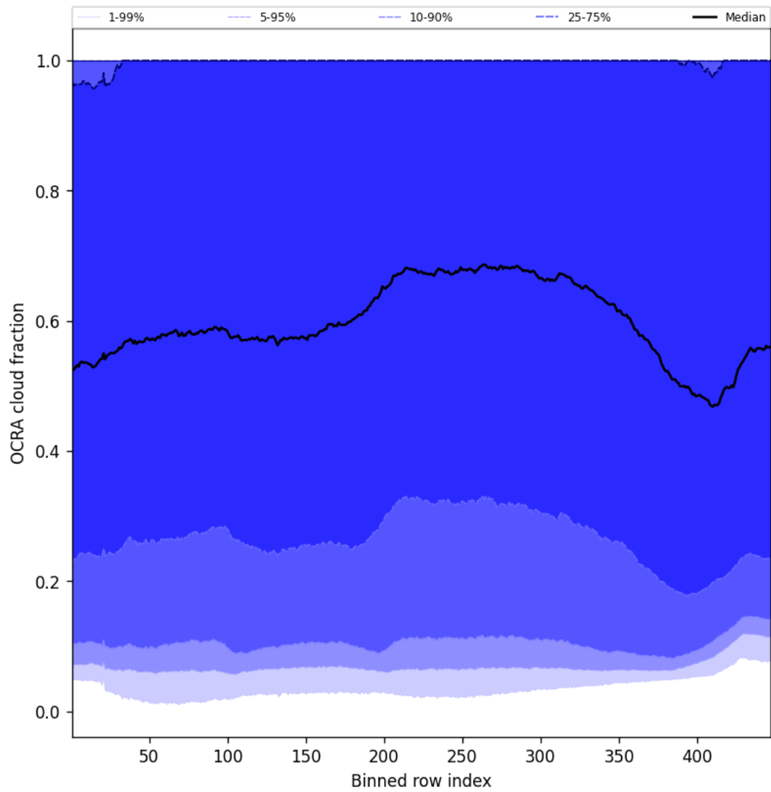
Figure 66: Along track statistics of “OCRA cloud fraction” for 2025-01-05 to 2025-01-07
