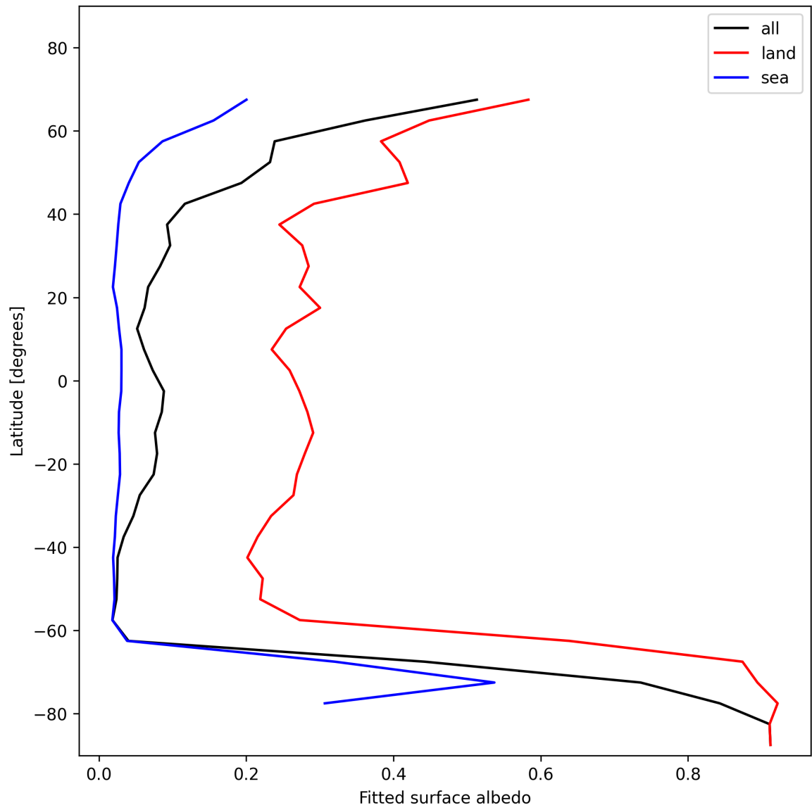
Figure 29: Zonal average of “Fitted surface albedo” for 2025-01-05 to 2025-01-07.
