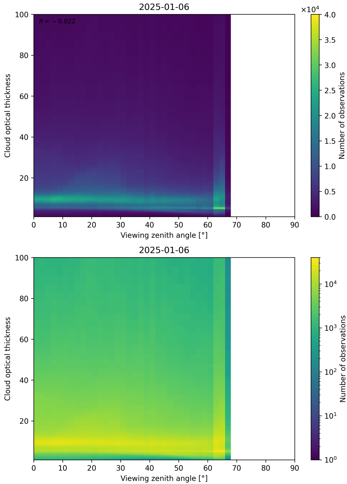
Figure 111: Scatter density plot of “Viewing zenith angle” against “Cloud optical thickness” for 2025-01-05 to 2025-01-07.
