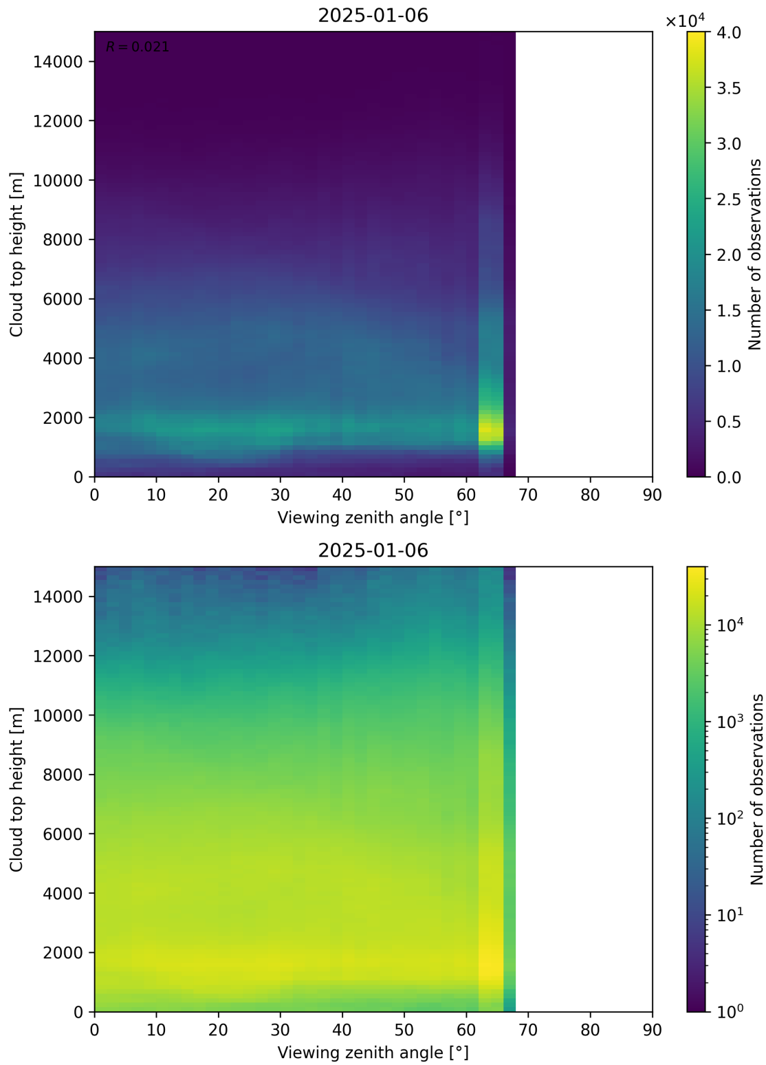
Figure 112: Scatter density plot of “Viewing zenith angle” against “Cloud top height” for 2025-01-05 to 2025-01-07.
