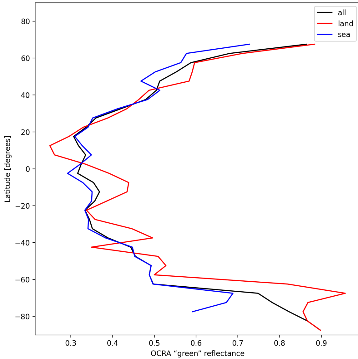
Figure 36: Zonal average of “OCRA “green” reflectance” for 2025-01-05 to 2025-01-07.
