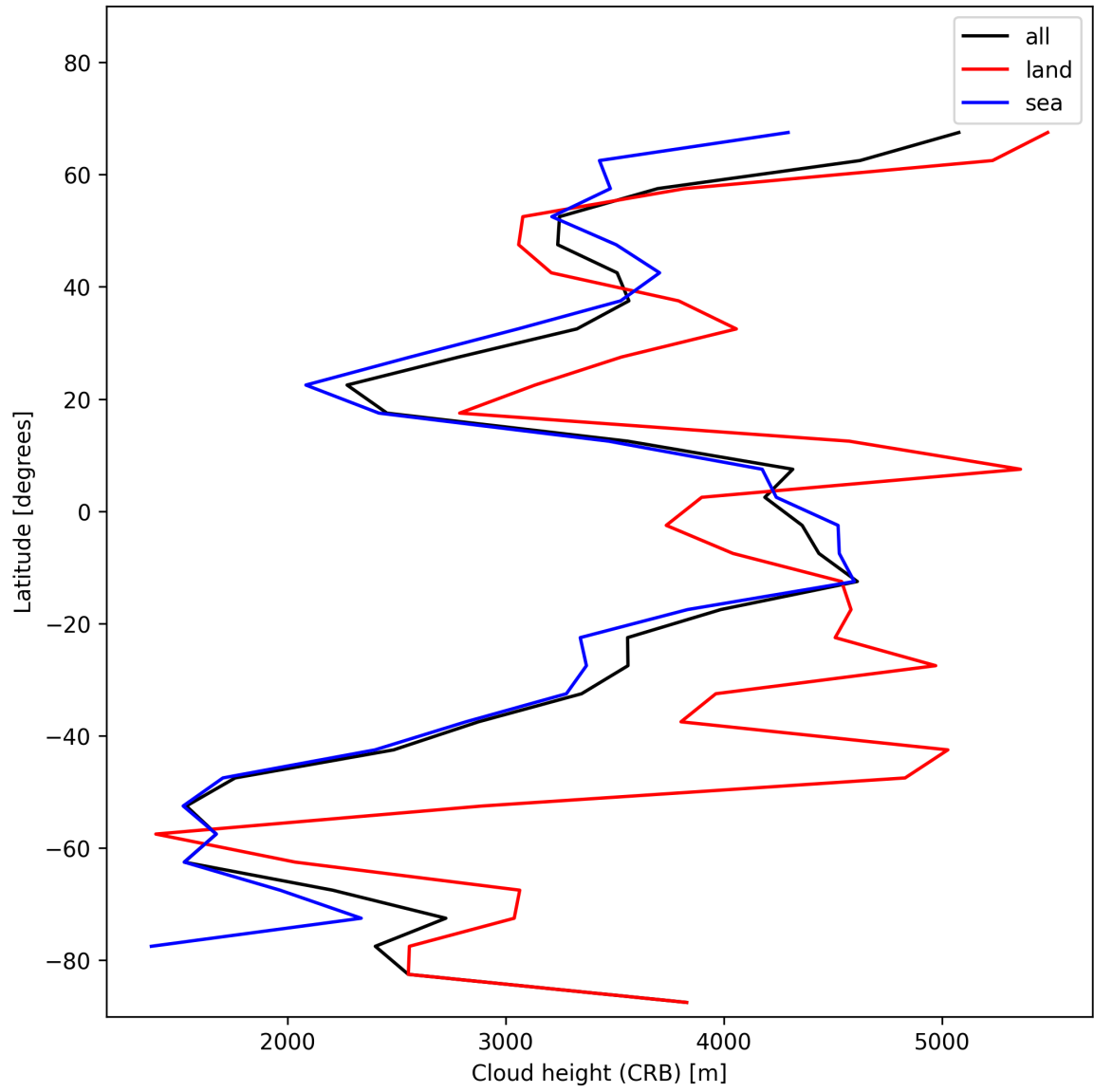
Figure 27: Zonal average of “Cloud height (CRB)” for 2025-01-05 to 2025-01-07.
