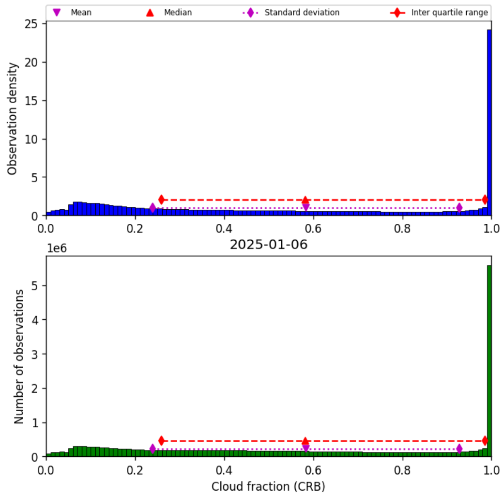
Figure 42: Histogram of “Cloud fraction (CRB)” for 2025-01-05 to 2025-01-07
