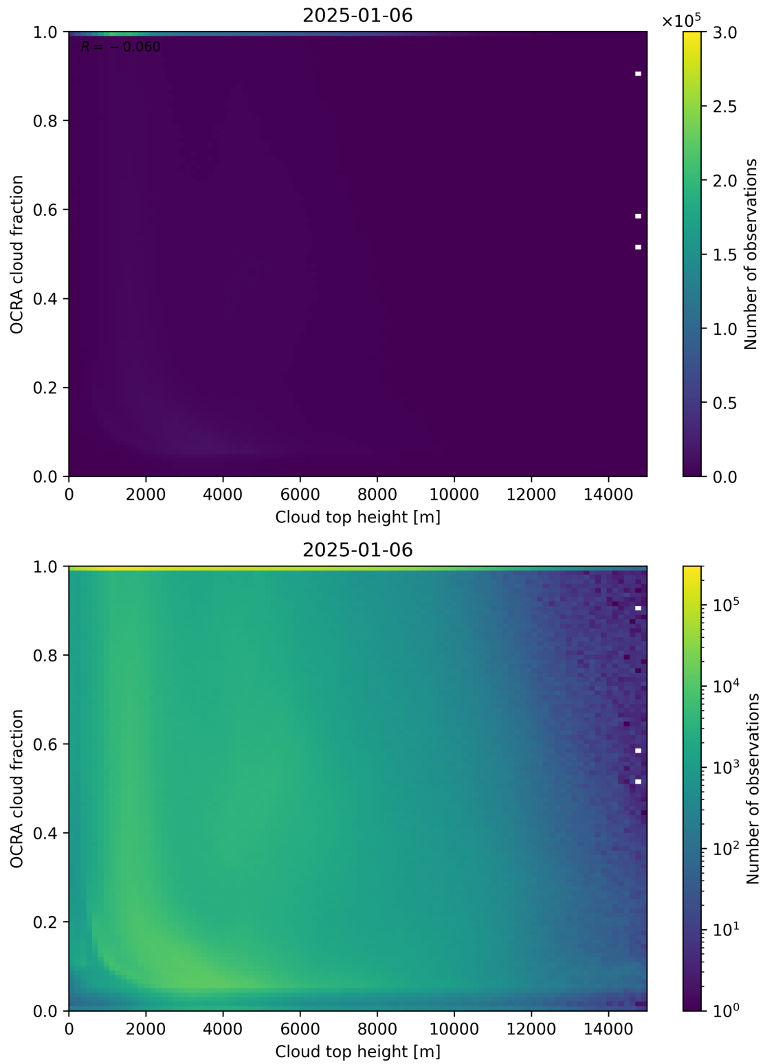
Figure 87: Scatter density plot of “Cloud top height” against “OCRA cloud fraction” for 2025-01-05 to 2025-01-07.
