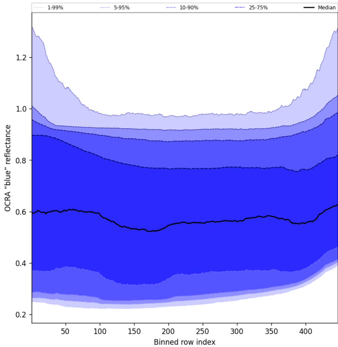
Figure 67: Along track statistics of “OCRA “blue” reflectance” for 2025-01-05 to 2025-01-07
