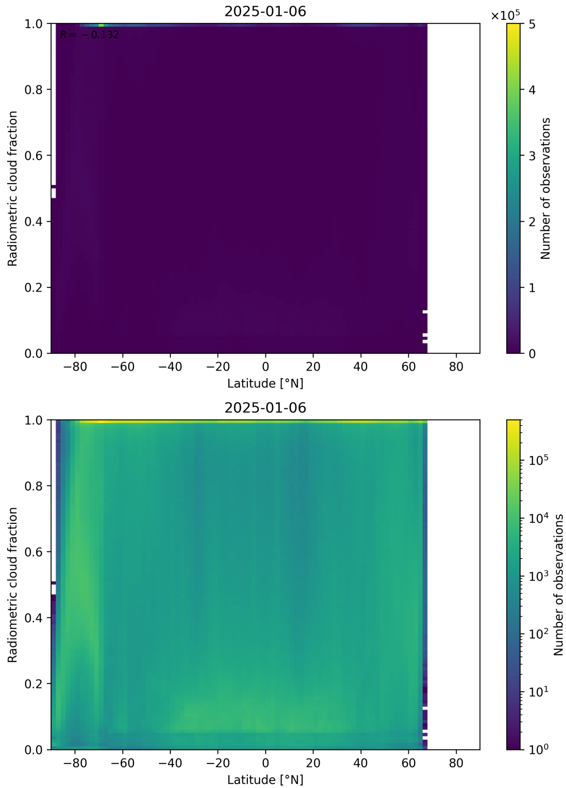
Figure 92: Scatter density plot of “Latitude” against “Radiometric cloud fraction” for 2025-01-05 to 2025-01-07.
