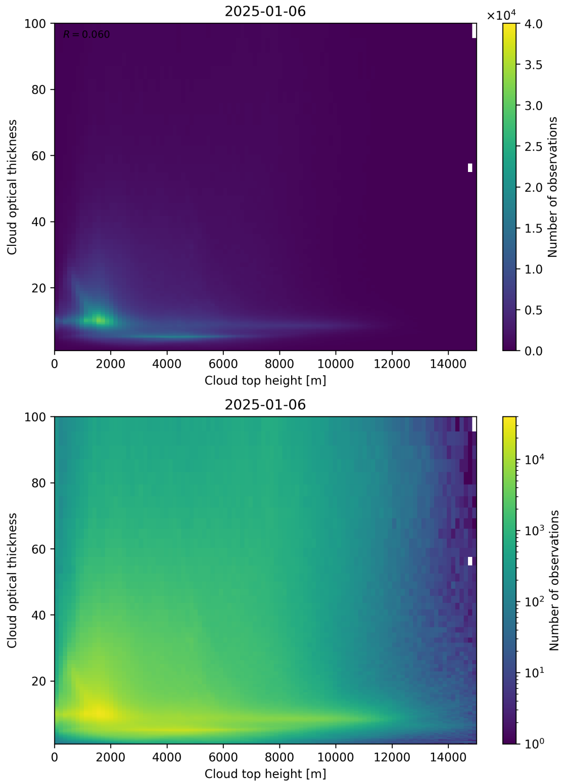
Figure 90: Scatter density plot of “Cloud top height” against “Cloud optical thickness” for 2025-01-05 to 2025-01-07.
