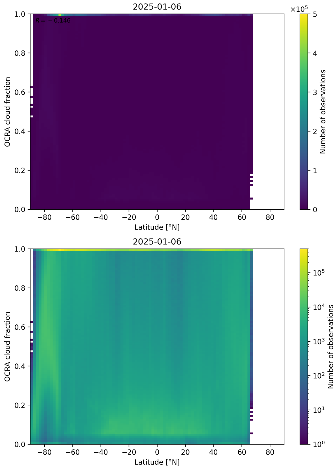
Figure 93: Scatter density plot of “Latitude” against “OCRA cloud fraction” for 2025-01-05 to 2025-01-07.
