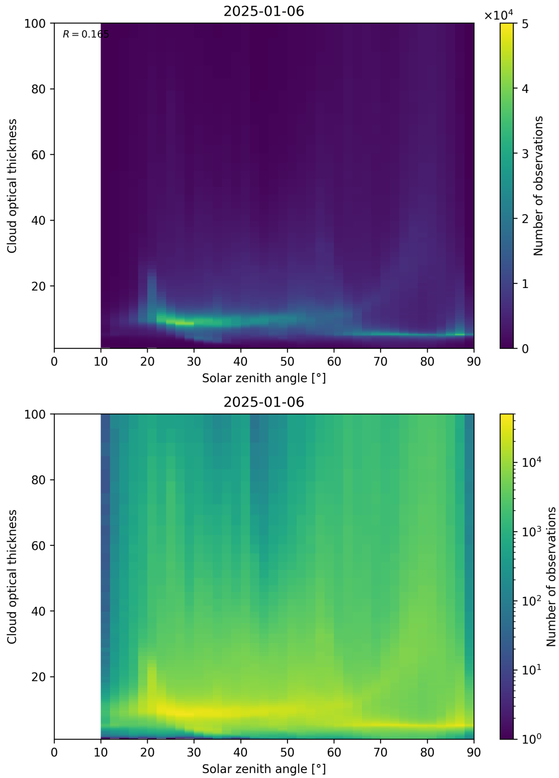
Figure 103: Scatter density plot of “Solar zenith angle” against “Cloud optical thickness” for 2025-01-05 to 2025-01-07.
