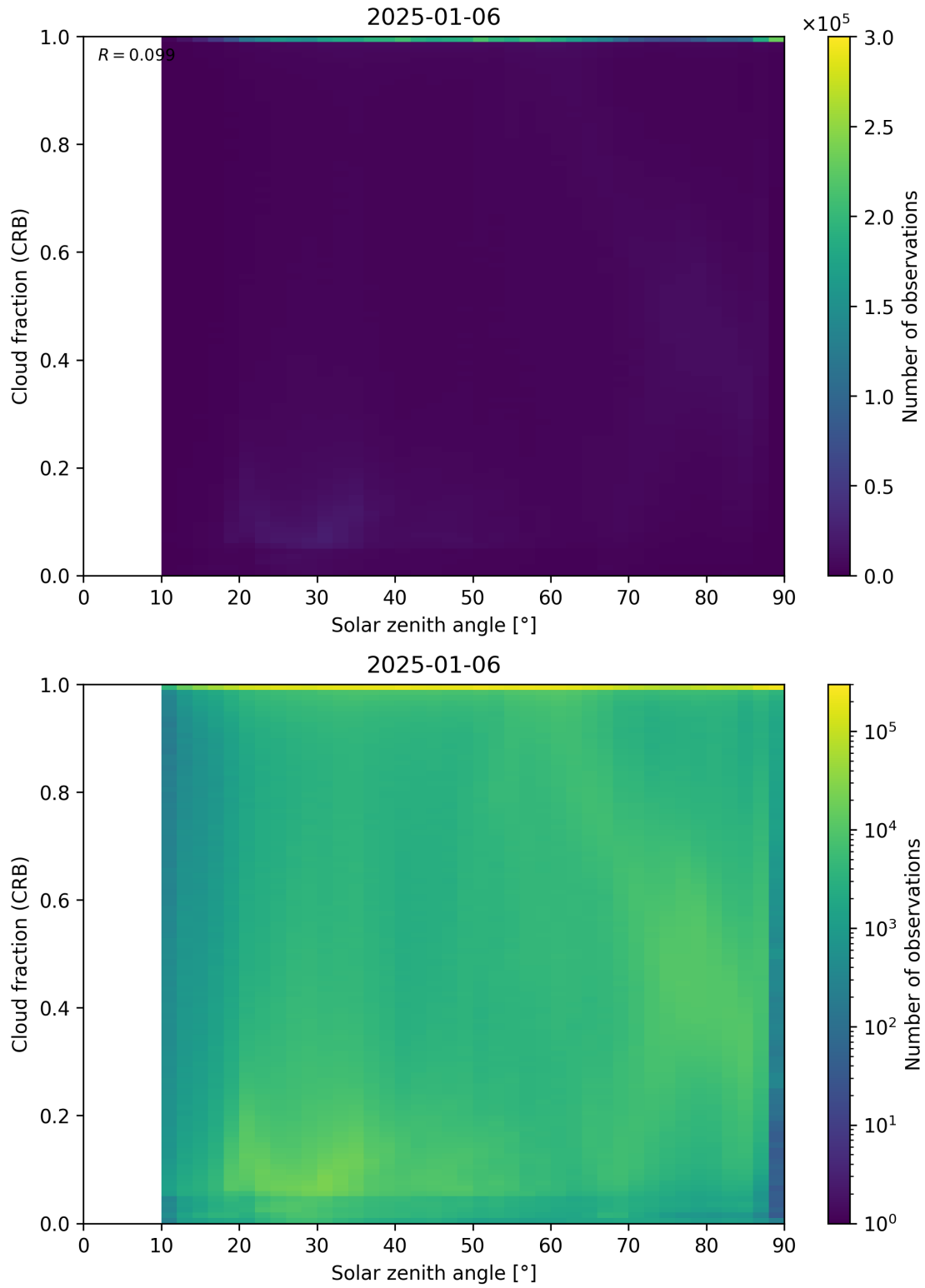
Figure 101: Scatter density plot of “Solar zenith angle” against “Cloud fraction (CRB)” for 2025-01-05 to 2025-01-07.
