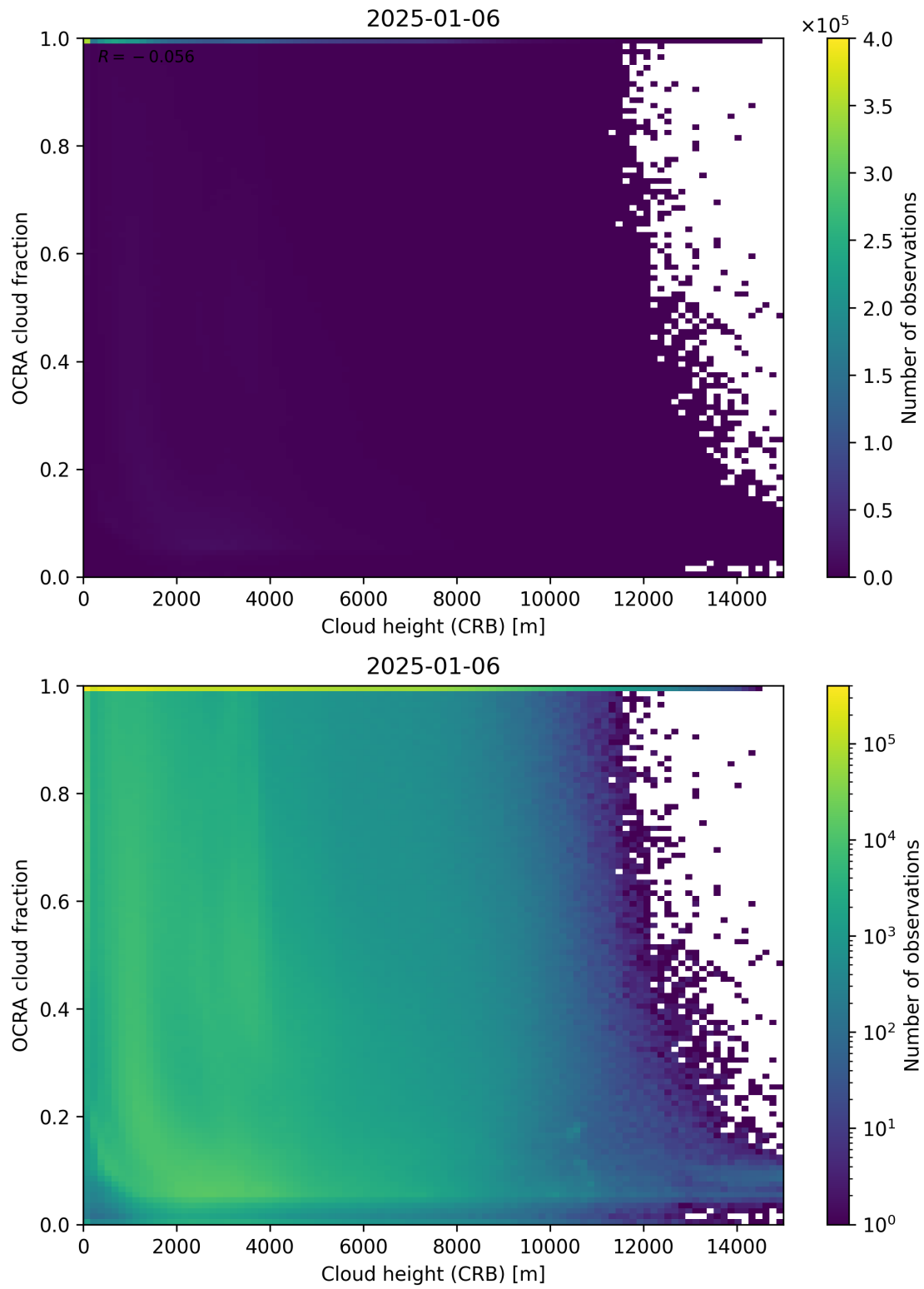
Figure 81: Scatter density plot of “Cloud height (CRB)” against “OCRA cloud fraction” for 2025-01-05 to 2025-01-07.
