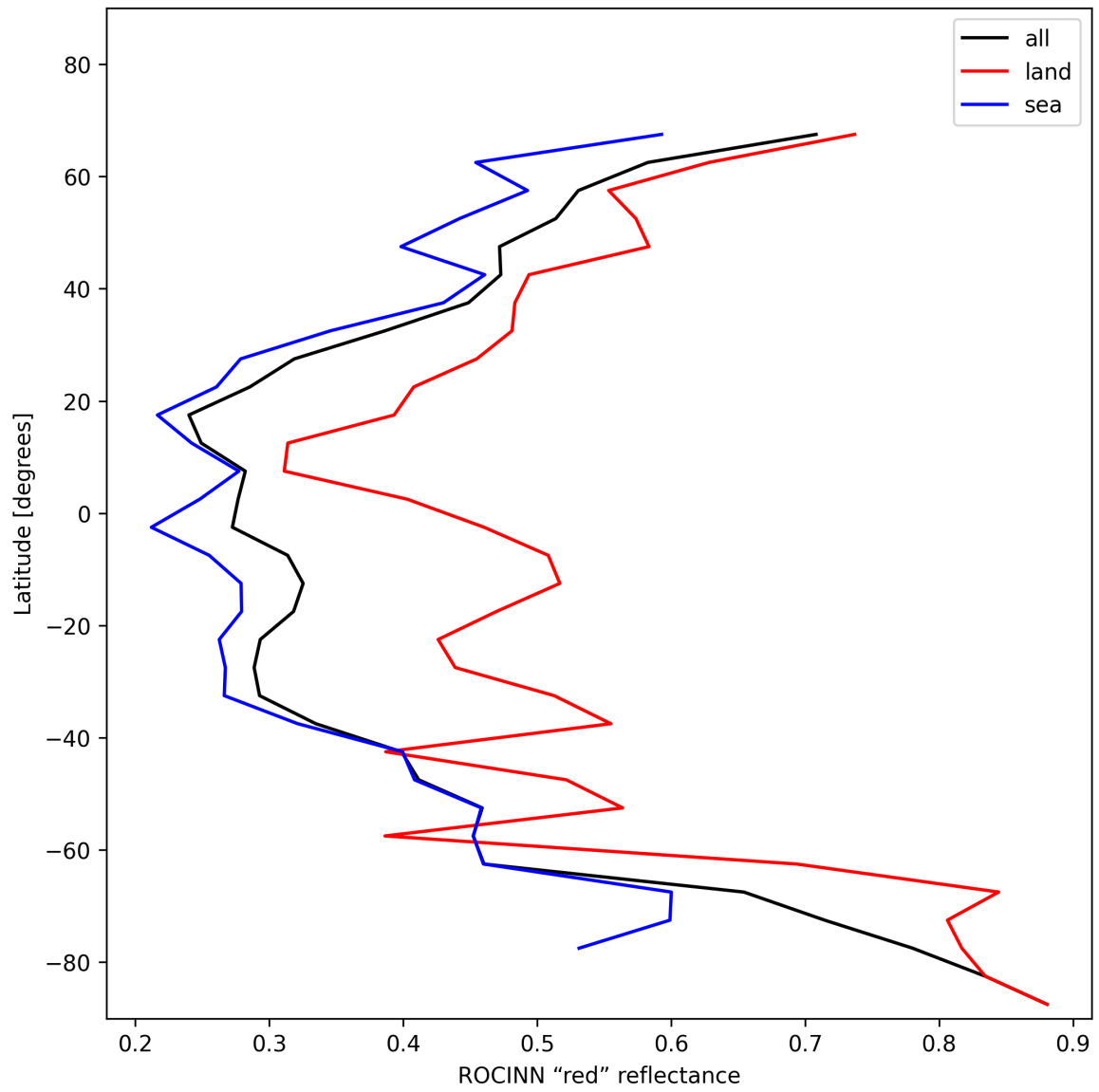
Figure 37: Zonal average of “ROCINN “red” reflectance” for 2025-01-05 to 2025-01-07.
