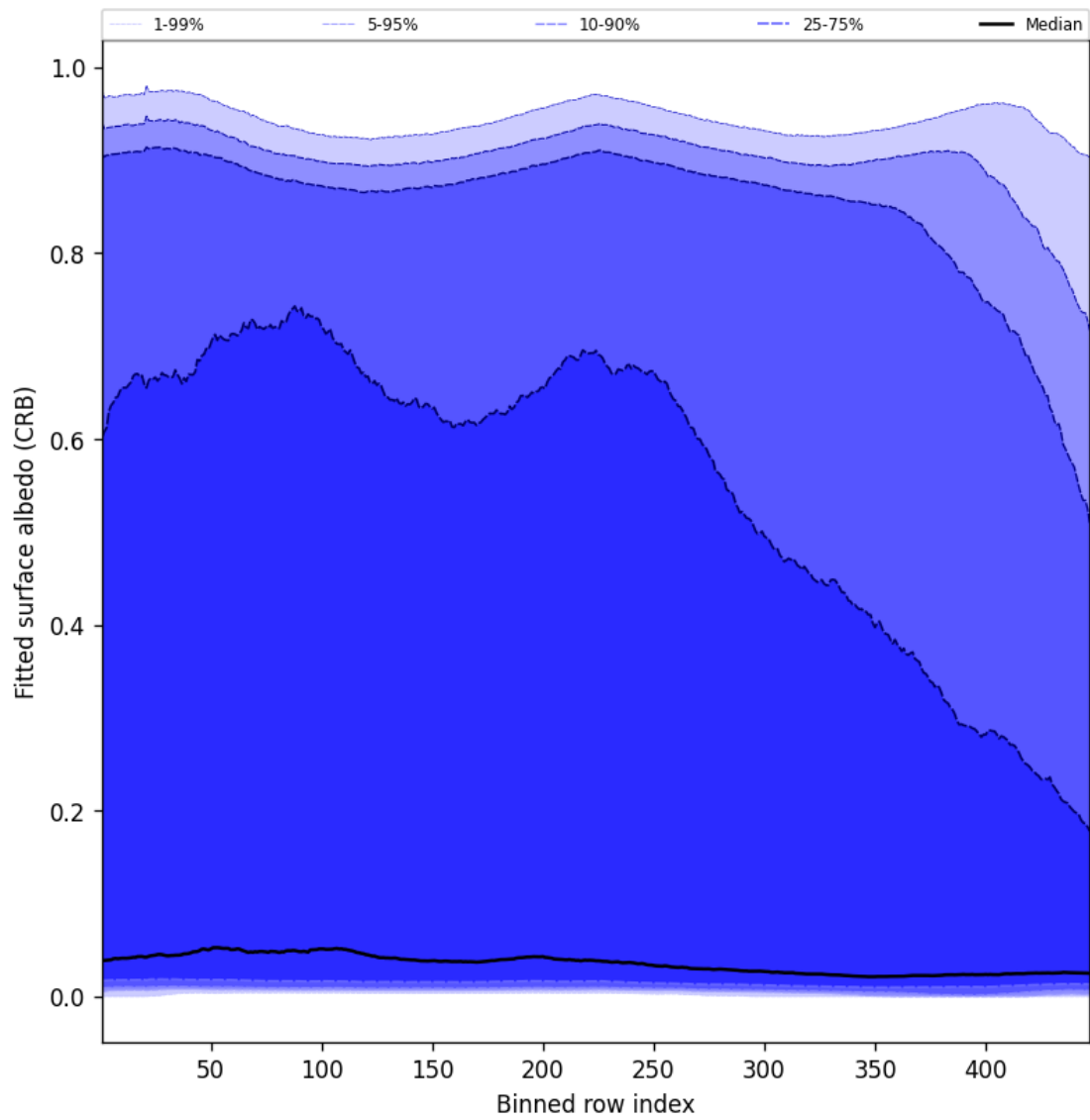
Figure 62: Along track statistics of “Fitted surface albedo (CRB)” for 2025-01-05 to 2025-01-07
