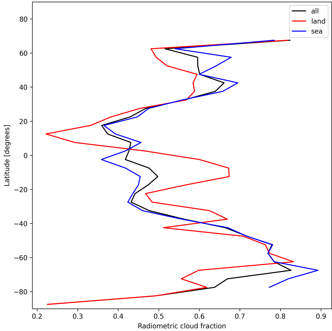
Figure 23: Zonal average of “Radiometric cloud fraction” for 2025-01-05 to 2025-01-07.
