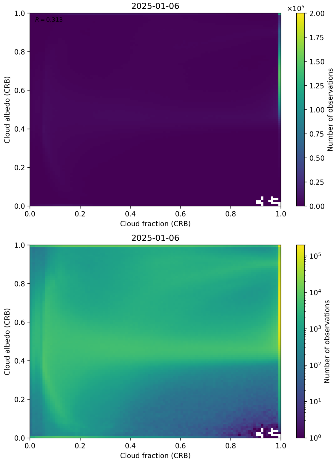
Figure 77: Scatter density plot of “Cloud fraction (CRB)” against “Cloud albedo (CRB)” for 2025-01-05 to 2025-01-07.
