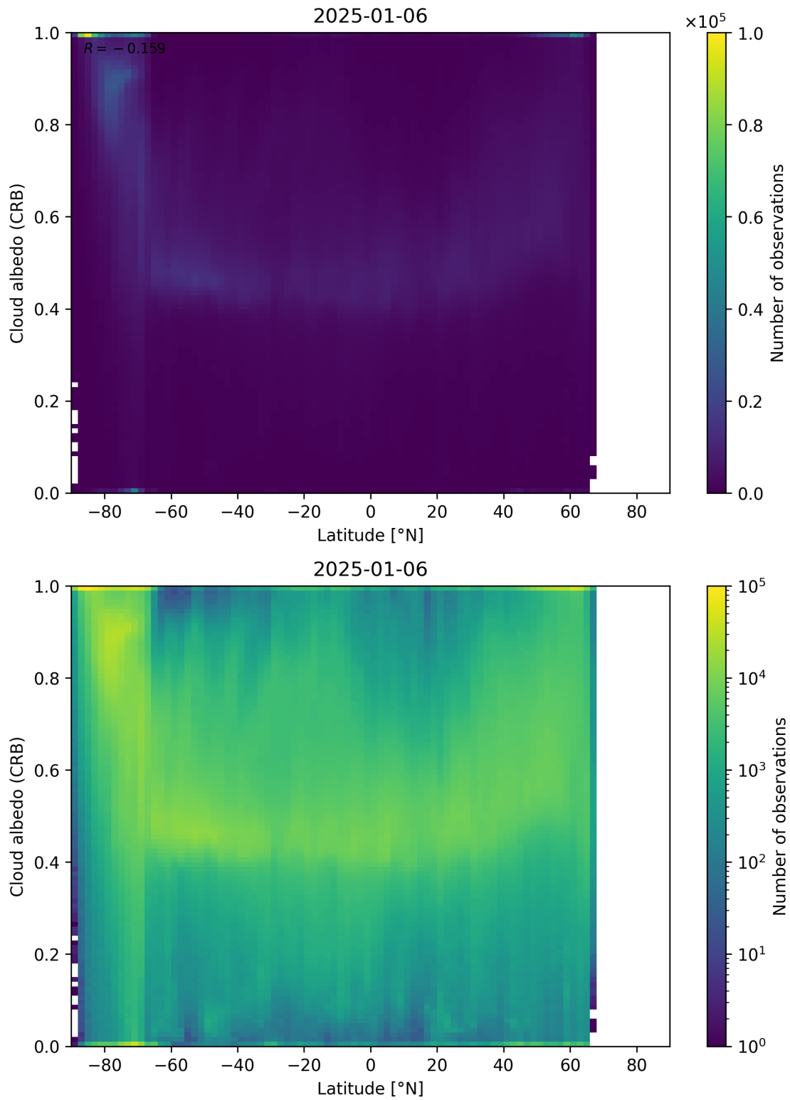
Figure 91: Scatter density plot of “Latitude” against “Cloud albedo (CRB)” for 2025-01-05 to 2025-01-07.
