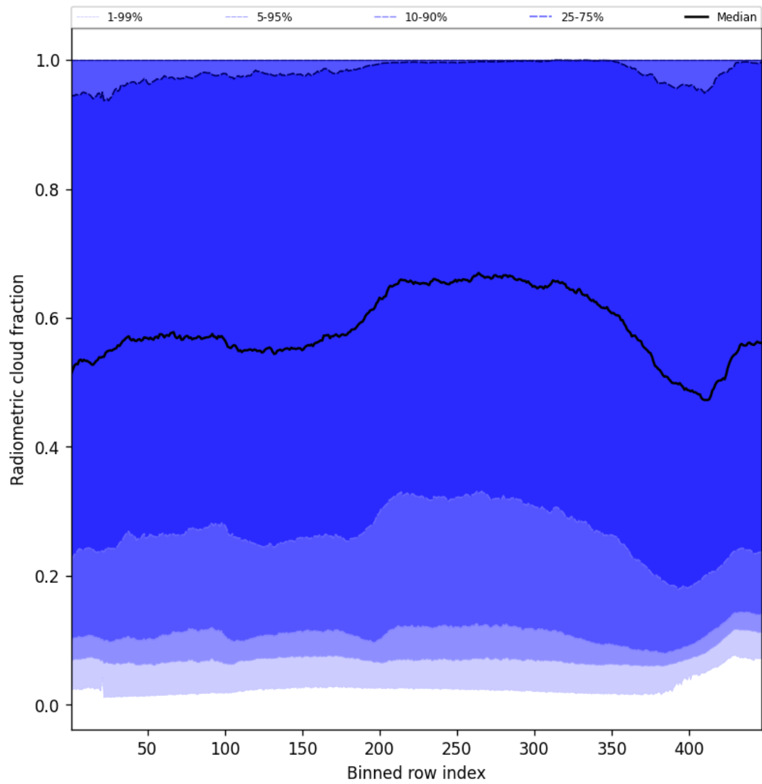
Figure 55: Along track statistics of “Radiometric cloud fraction” for 2025-01-05 to 2025-01-07
