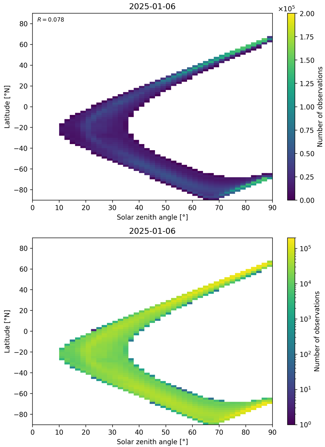
Figure 105: Scatter density plot of “Solar zenith angle” against “Latitude” for 2025-01-05 to 2025-01-07.
