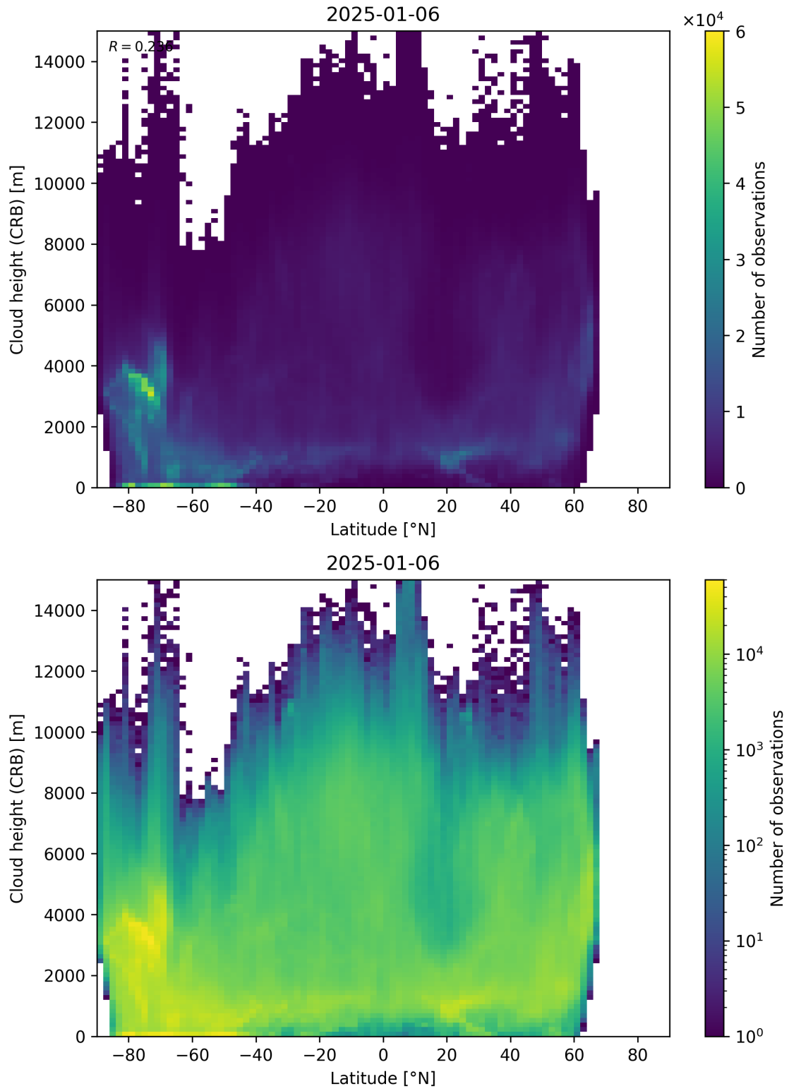
Figure 95: Scatter density plot of “Latitude” against “Cloud height (CRB)” for 2025-01-05 to 2025-01-07.
