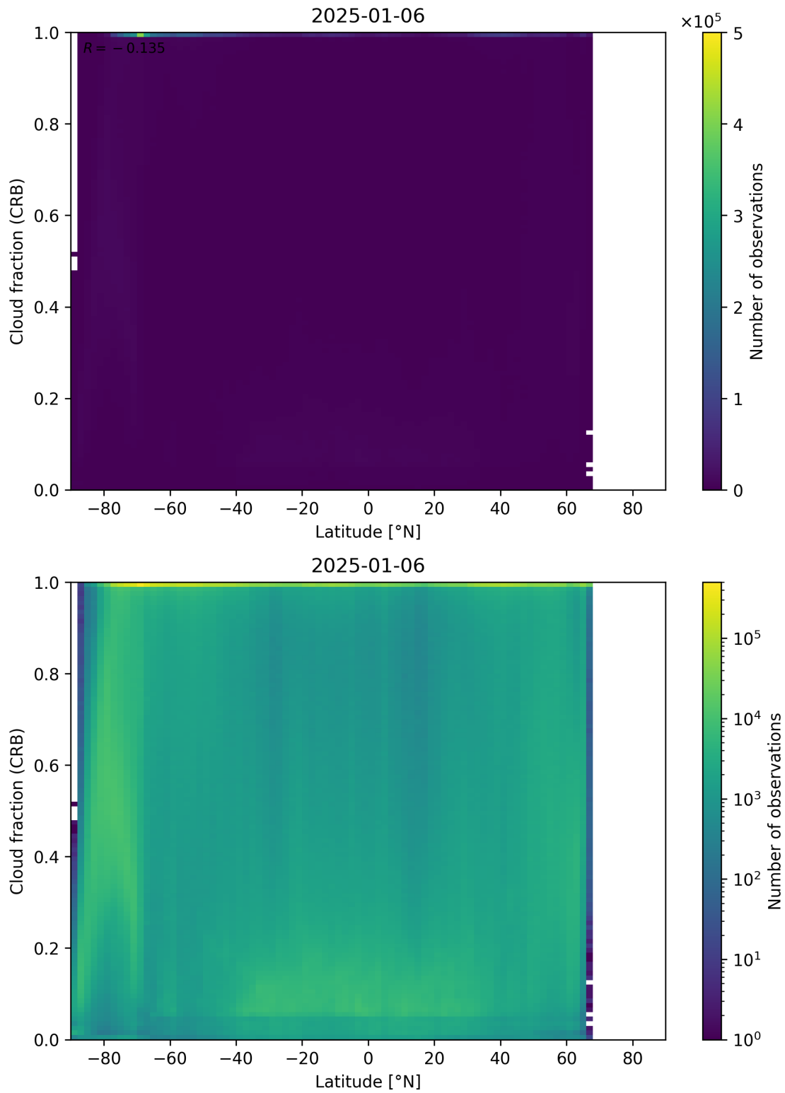
Figure 94: Scatter density plot of “Latitude” against “Cloud fraction (CRB)” for 2025-01-05 to 2025-01-07.
