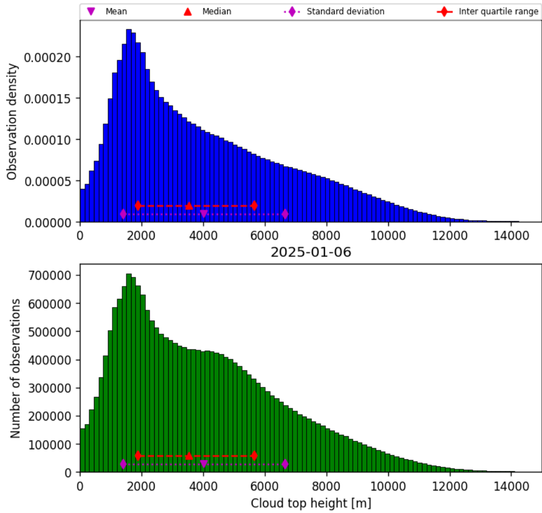
Figure 40: Histogram of “Cloud top height” for 2025-01-05 to 2025-01-07
