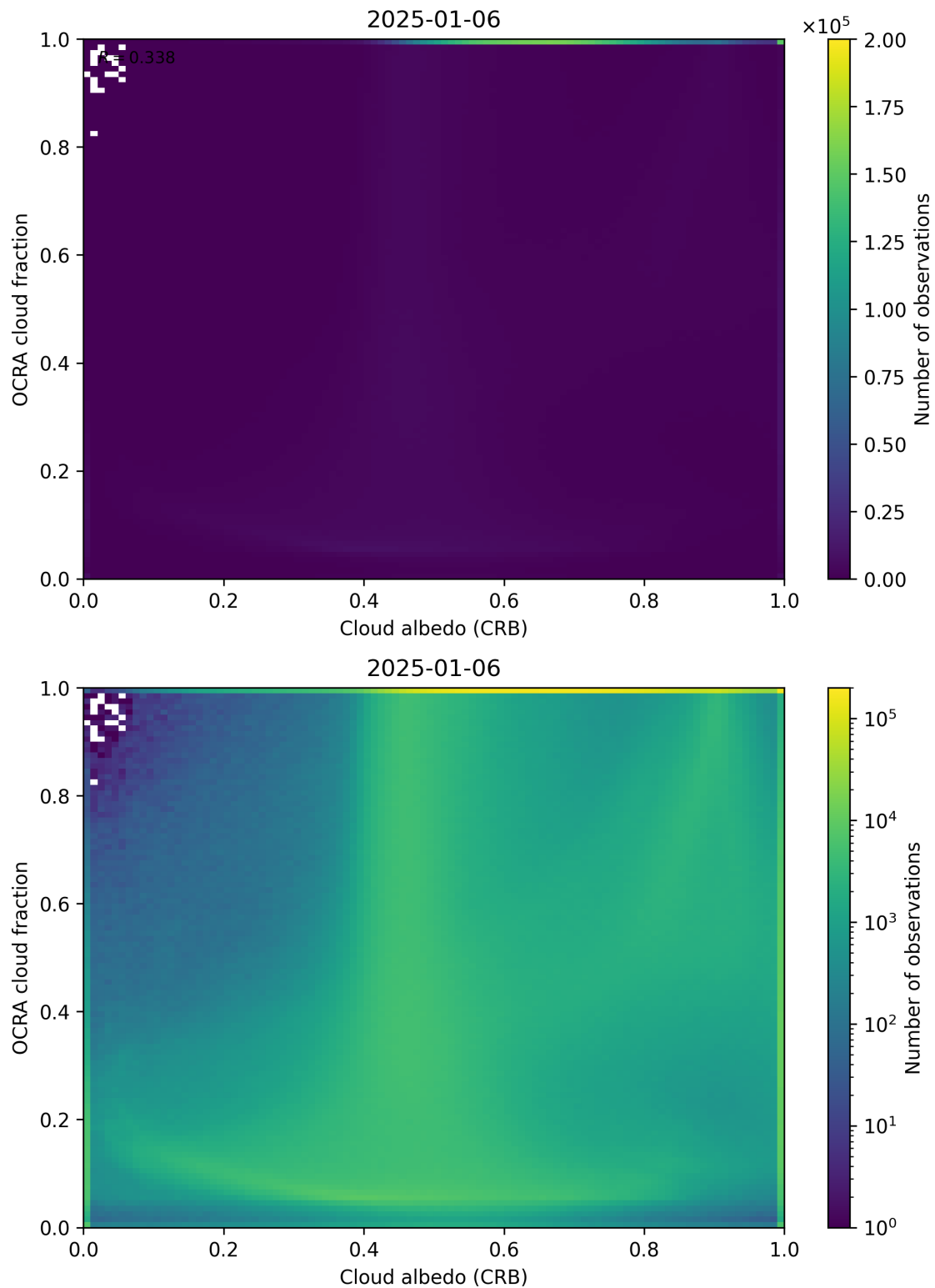
Figure 70: Scatter density plot of “Cloud albedo (CRB)” against “OCRA cloud fraction” for 2025-01-05 to 2025-01-07.
