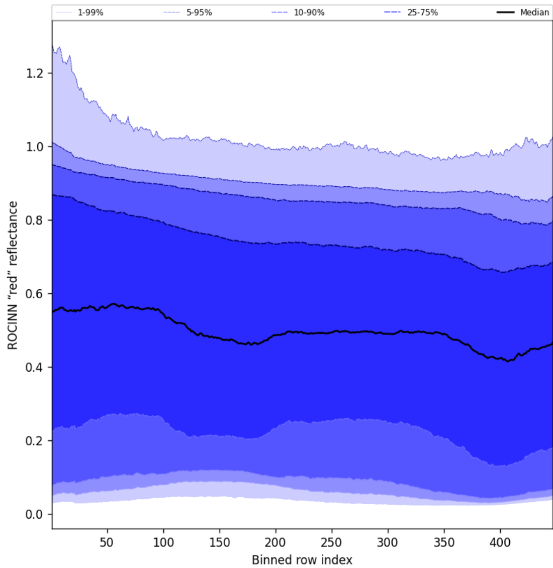
Figure 69: Along track statistics of “ROCINN “red” reflectance” for 2025-01-05 to 2025-01-07
