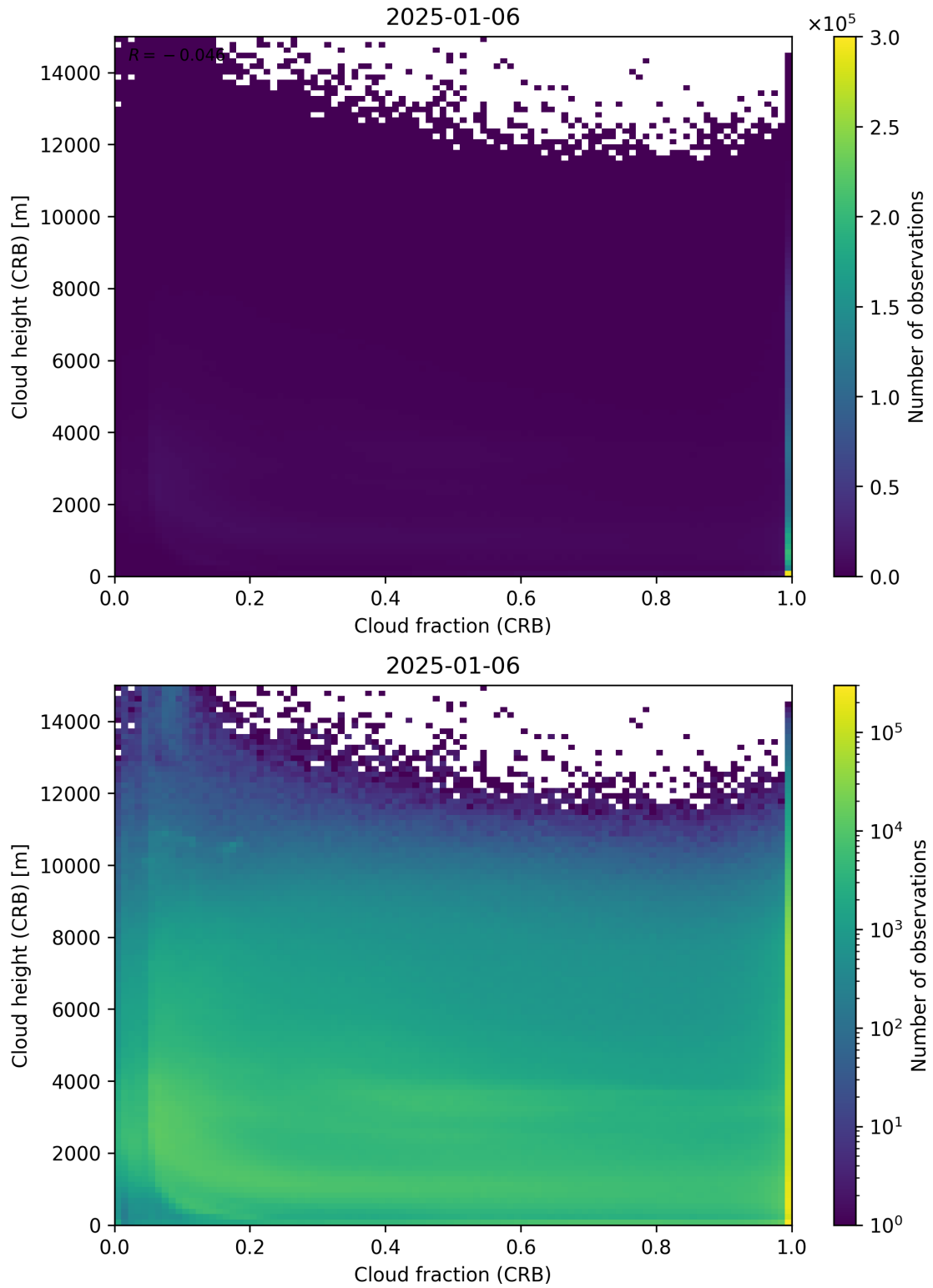
Figure 79: Scatter density plot of “Cloud fraction (CRB)” against “Cloud height (CRB)” for 2025-01-05 to 2025-01-07.
