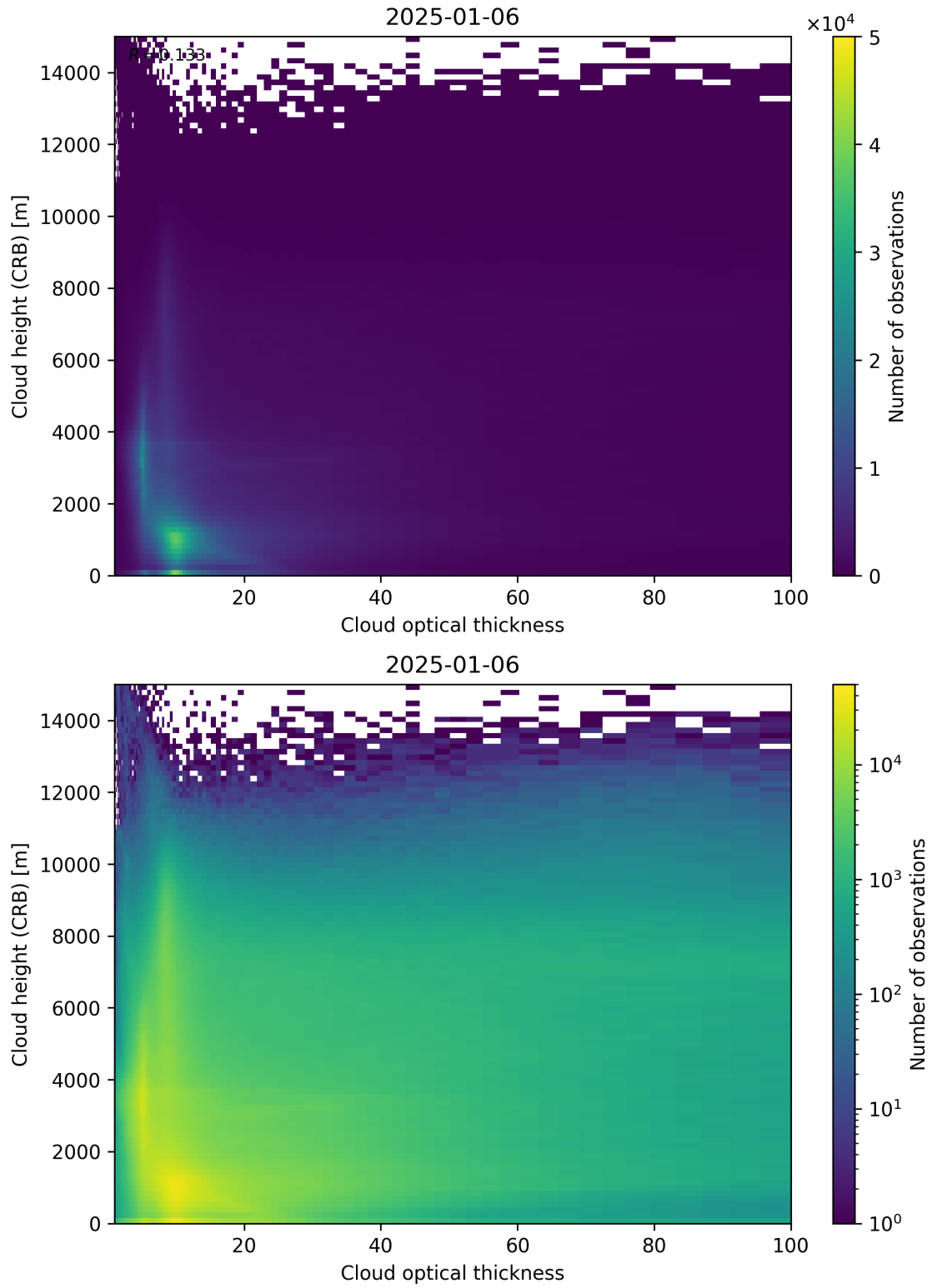
Figure 85: Scatter density plot of “Cloud optical thickness” against “Cloud height (CRB)” for 2025-01-05 to 2025-01-07.
