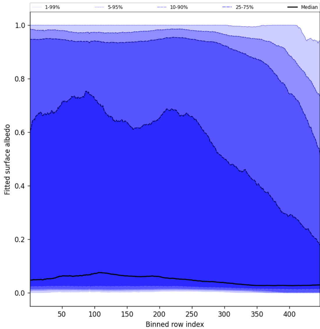
Figure 61: Along track statistics of “Fitted surface albedo” for 2025-01-05 to 2025-01-07
