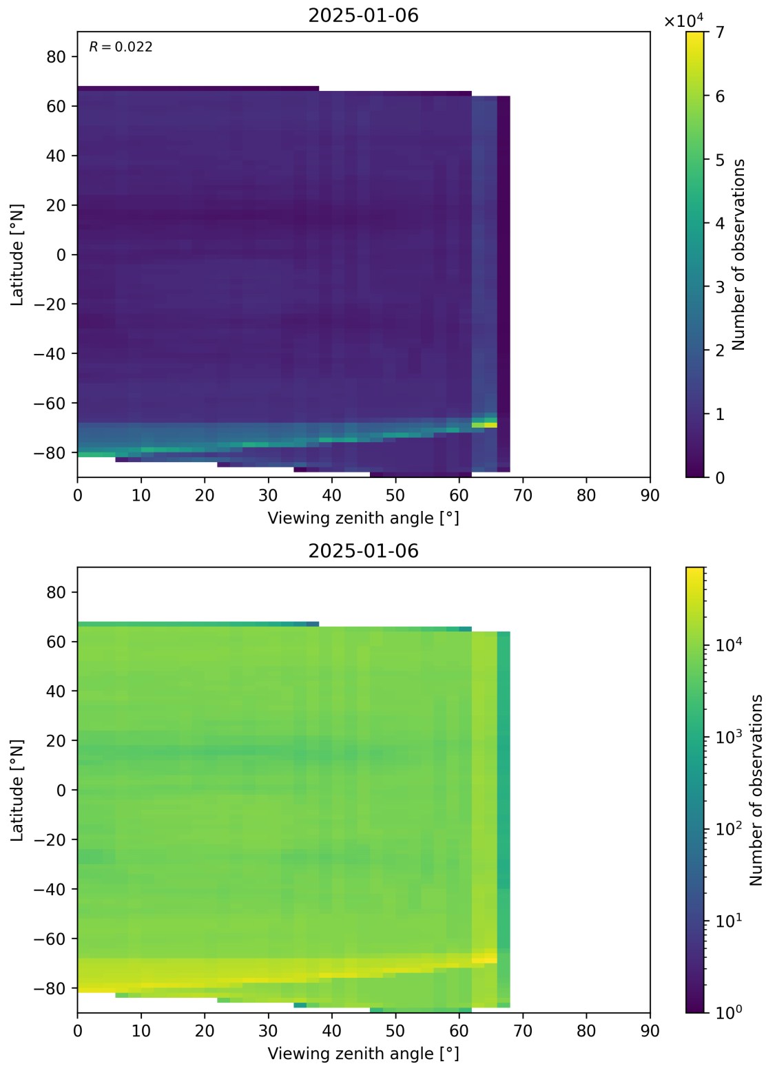
Figure 113: Scatter density plot of “Viewing zenith angle” against “Latitude” for 2025-01-05 to 2025-01-07.
