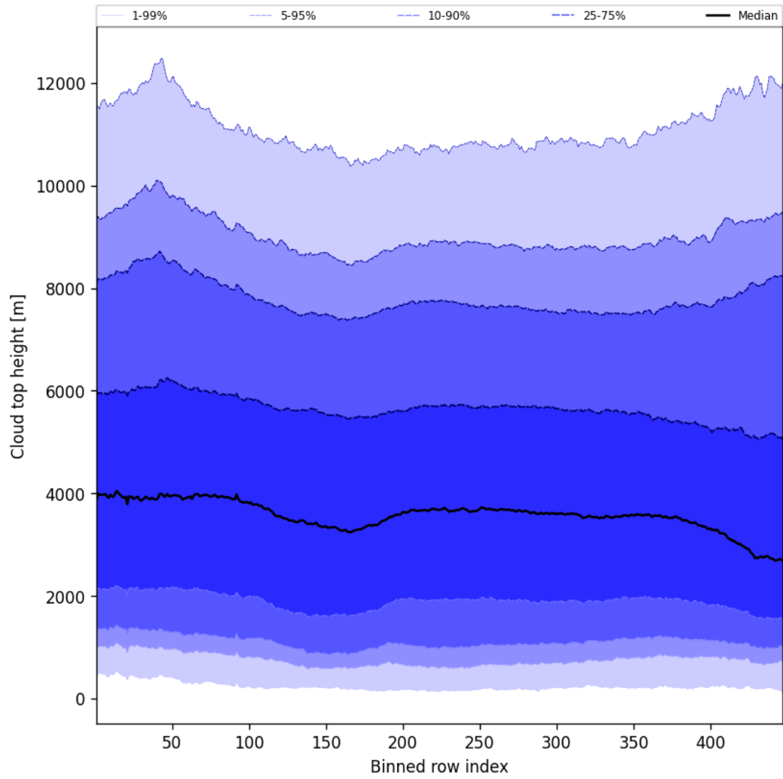
Figure 56: Along track statistics of “Cloud top height” for 2025-01-05 to 2025-01-07
