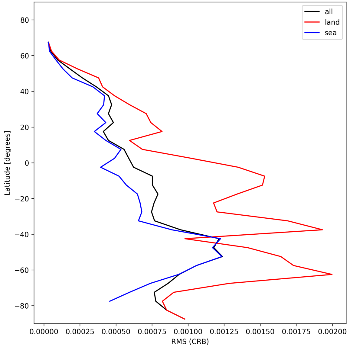
Figure 32: Zonal average of “RMS (CRB)” for 2025-01-05 to 2025-01-07.
