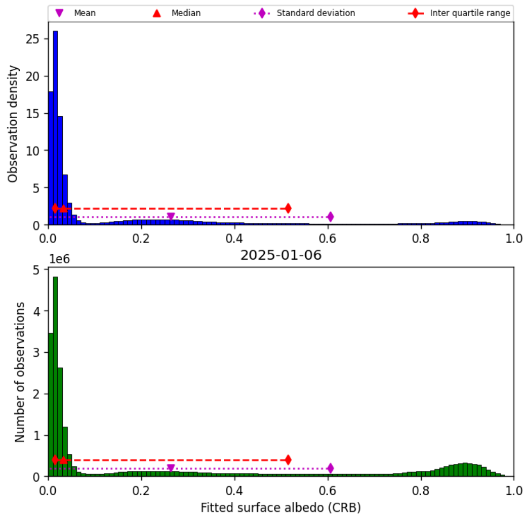
Figure 46: Histogram of “Fitted surface albedo (CRB)” for 2025-01-05 to 2025-01-07
