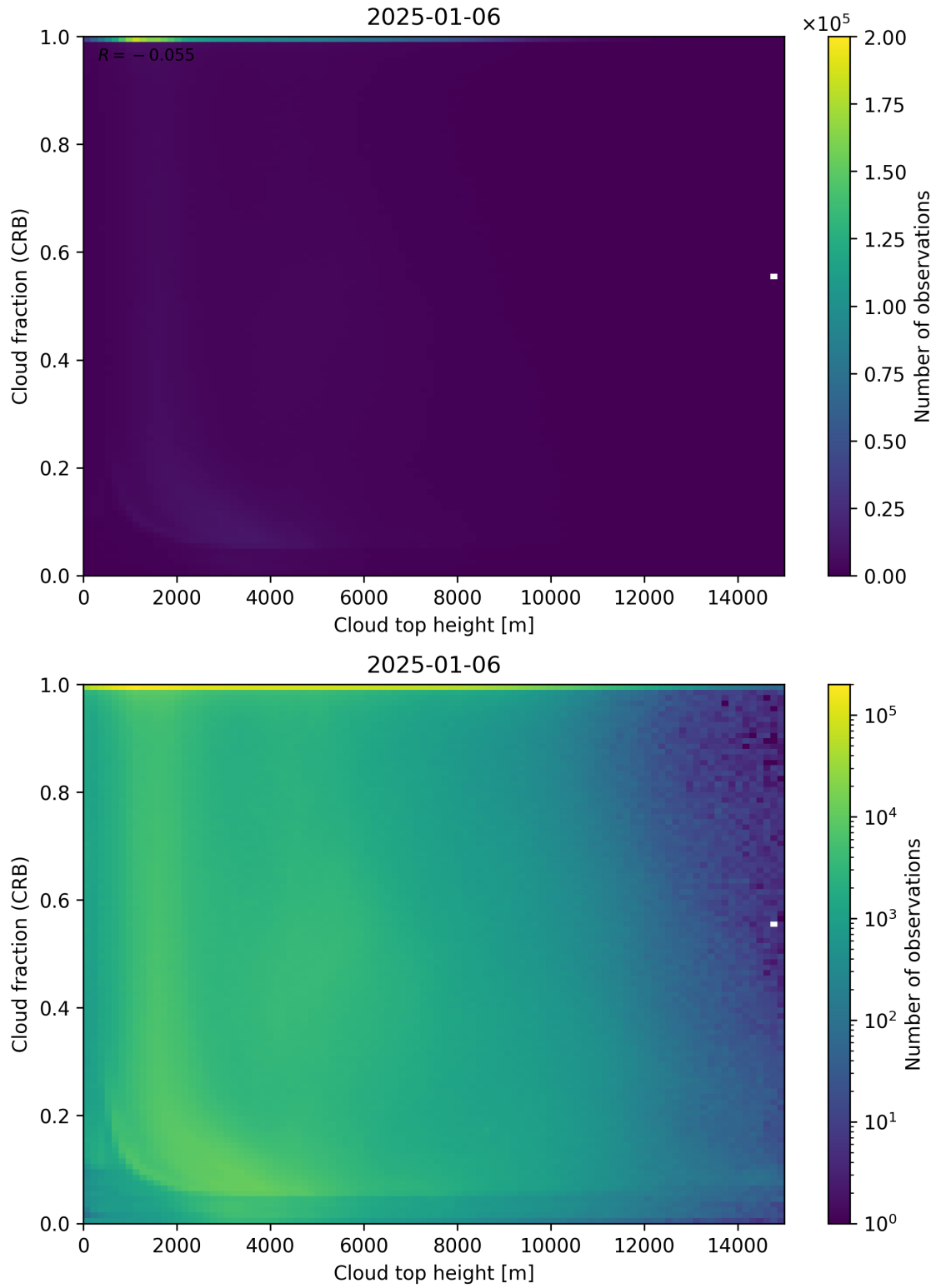
Figure 88: Scatter density plot of “Cloud top height” against “Cloud fraction (CRB)” for 2025-01-05 to 2025-01-07.
