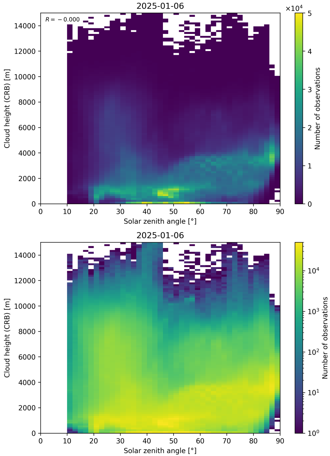
Figure 102: Scatter density plot of “Solar zenith angle” against “Cloud height (CRB)” for 2025-01-05 to 2025-01-07.
