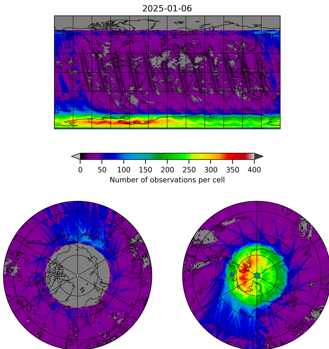
Figure 21: Map of the number of observations for 2025-01-05 to 2025-01-07
