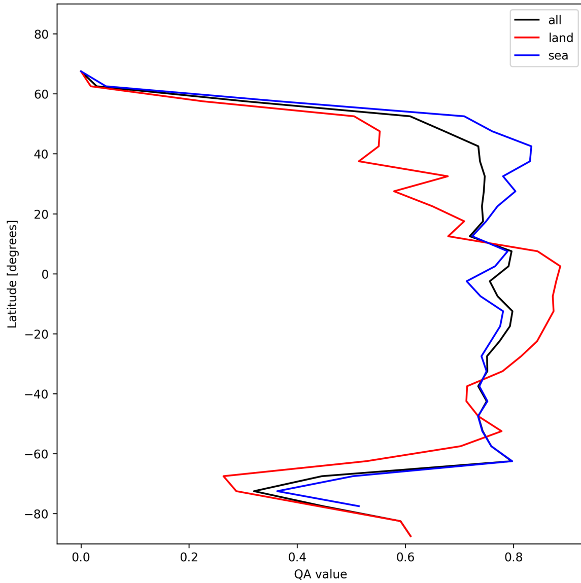
Figure 22: Zonal average of “QA value” for 2025-01-07 to 2025-01-08.
