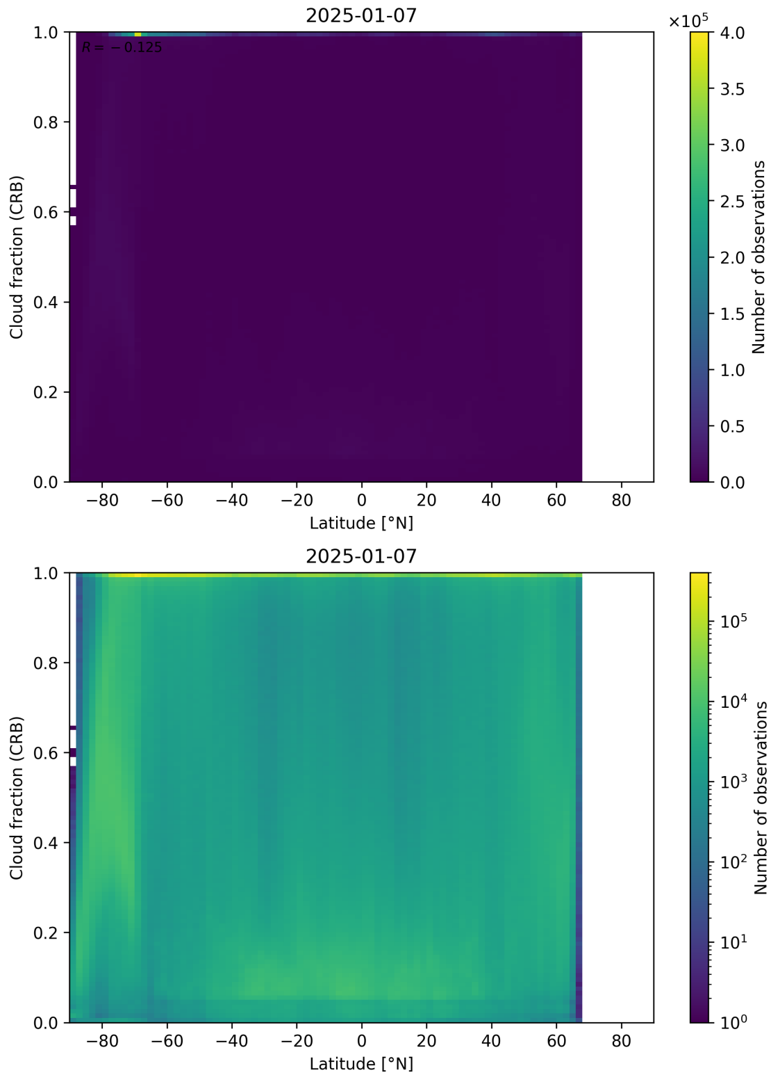
Figure 94: Scatter density plot of “Latitude” against “Cloud fraction (CRB)” for 2025-01-07 to 2025-01-08.
