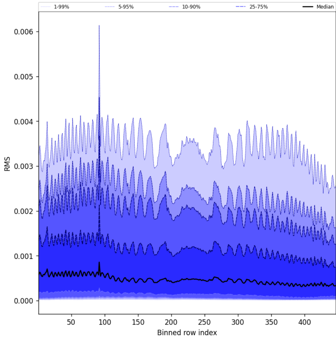
Figure 63: Along track statistics of “RMS” for 2025-01-07 to 2025-01-08
