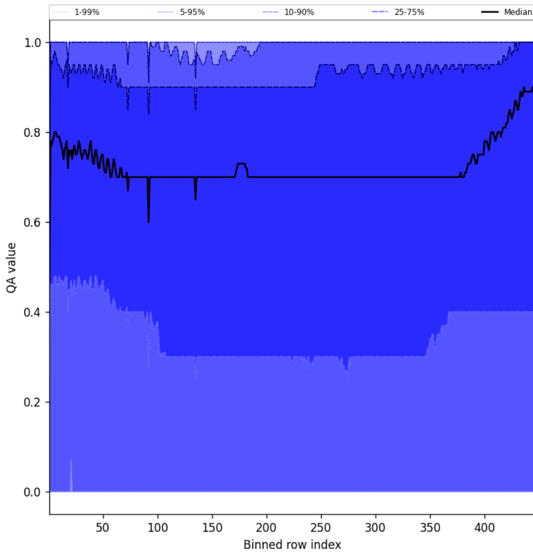
Figure 54: Along track statistics of “QA value” for 2025-01-07 to 2025-01-08
