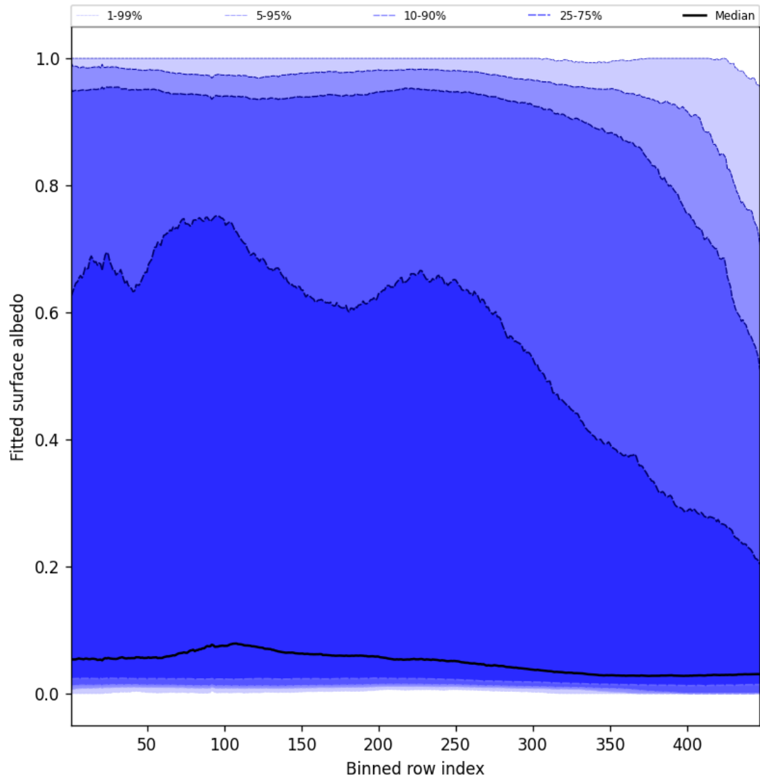
Figure 61: Along track statistics of “Fitted surface albedo” for 2025-01-07 to 2025-01-08
