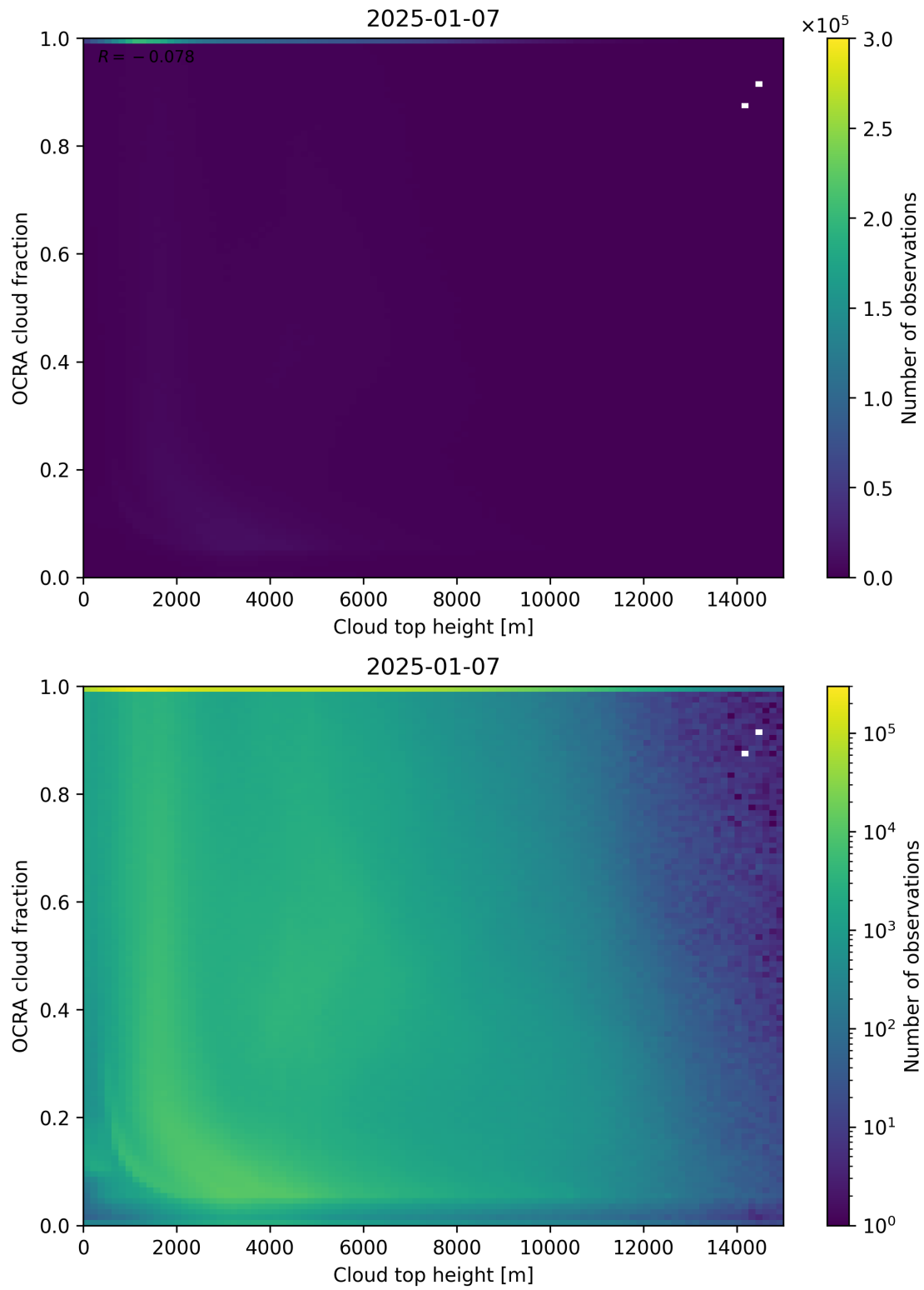
Figure 87: Scatter density plot of “Cloud top height” against “OCRA cloud fraction” for 2025-01-07 to 2025-01-08.
