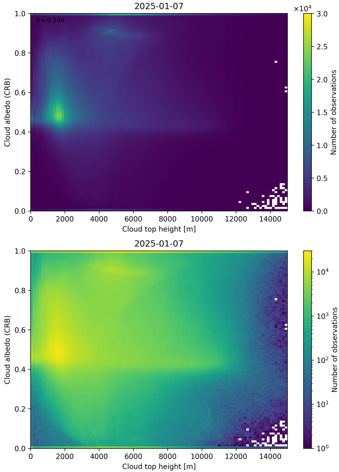
Figure 86: Scatter density plot of “Cloud top height” against “Cloud albedo (CRB)” for 2025-01-07 to 2025-01-08.
