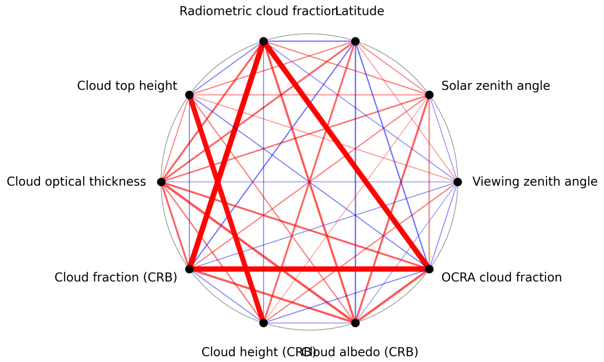
Figure 1: Map of correlation graph for 2025-01-07 to 2025-01-08.
