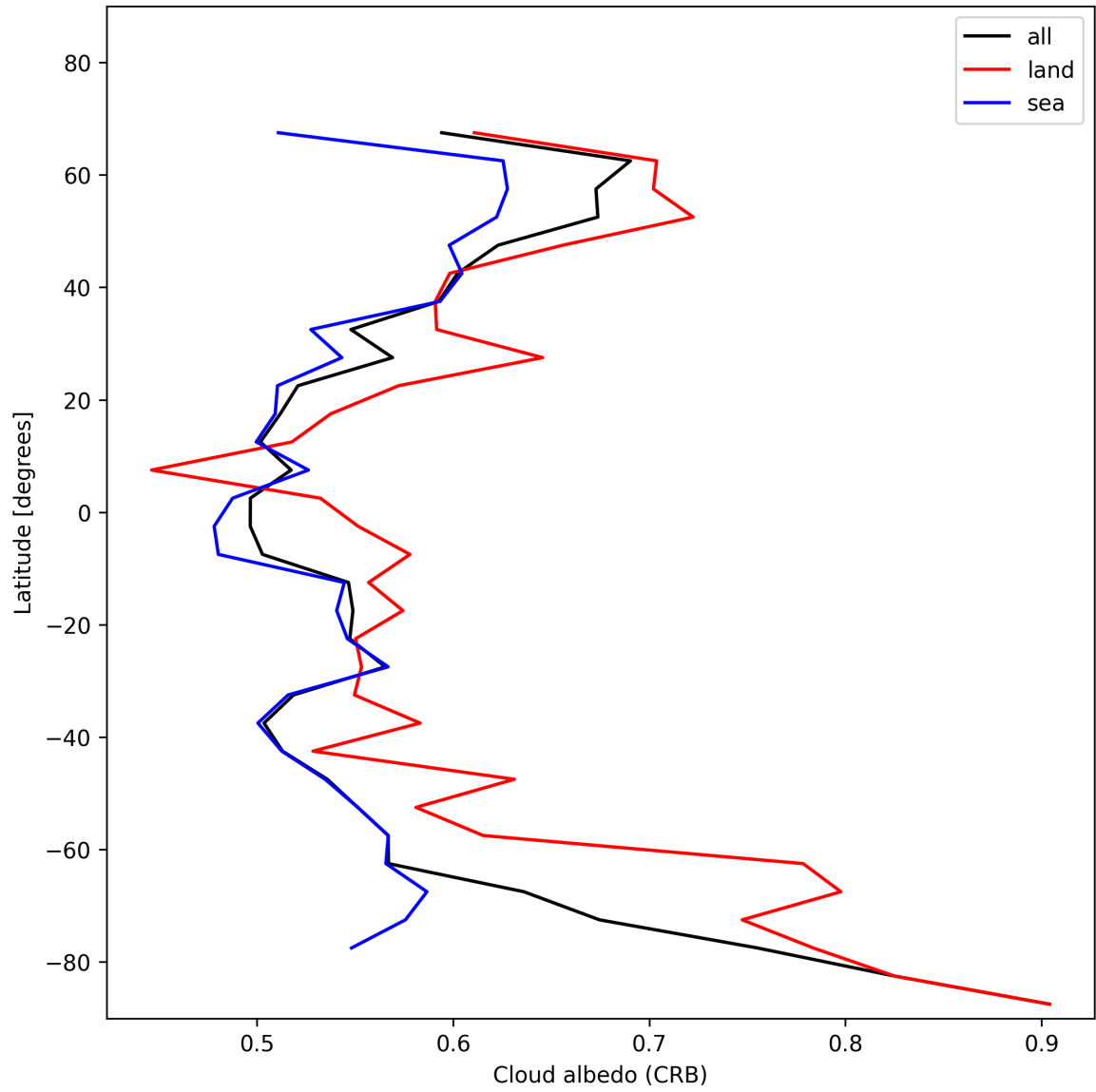
Figure 28: Zonal average of “Cloud albedo (CRB)” for 2025-01-07 to 2025-01-08.
