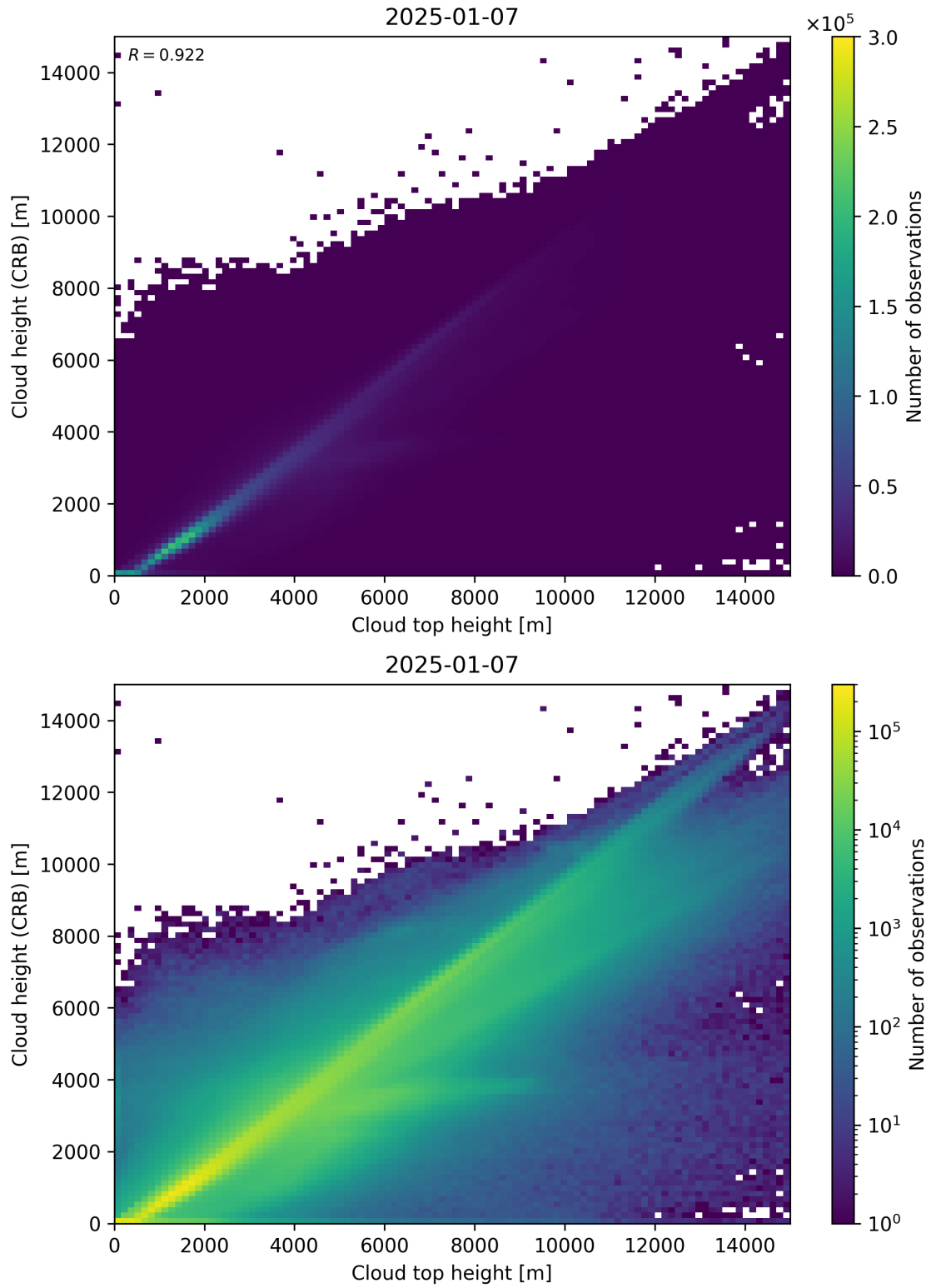
Figure 89: Scatter density plot of “Cloud top height” against “Cloud height (CRB)” for 2025-01-07 to 2025-01-08.
