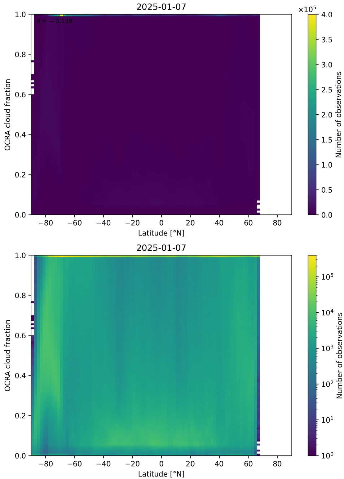
Figure 93: Scatter density plot of “Latitude” against “OCRA cloud fraction” for 2025-01-07 to 2025-01-08.
