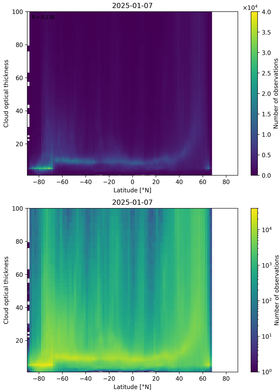
Figure 96: Scatter density plot of “Latitude” against “Cloud optical thickness” for 2025-01-07 to 2025-01-08.
