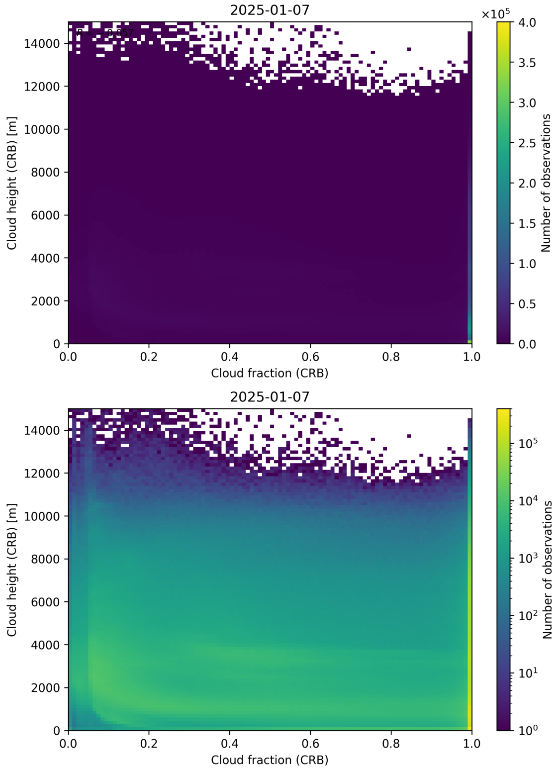
Figure 79: Scatter density plot of “Cloud fraction (CRB)” against “Cloud height (CRB)” for 2025-01-07 to 2025-01-08.
