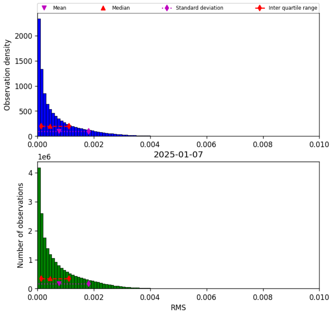
Figure 47: Histogram of “RMS” for 2025-01-07 to 2025-01-08
