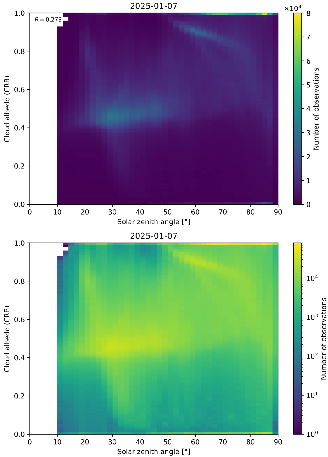
Figure 98: Scatter density plot of “Solar zenith angle” against “Cloud albedo (CRB)” for 2025-01-07 to 2025-01-08.
