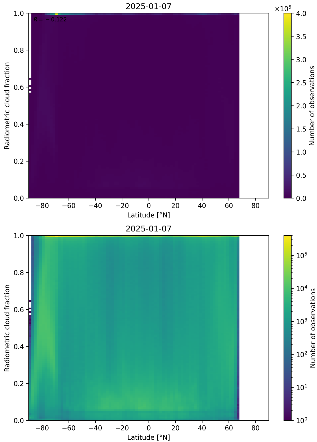
Figure 92: Scatter density plot of “Latitude” against “Radiometric cloud fraction” for 2025-01-07 to 2025-01-08.
