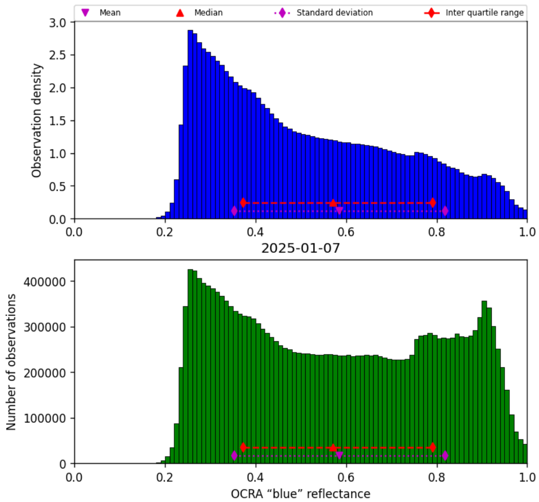
Figure 51: Histogram of “OCRA “blue” reflectance” for 2025-01-07 to 2025-01-08
