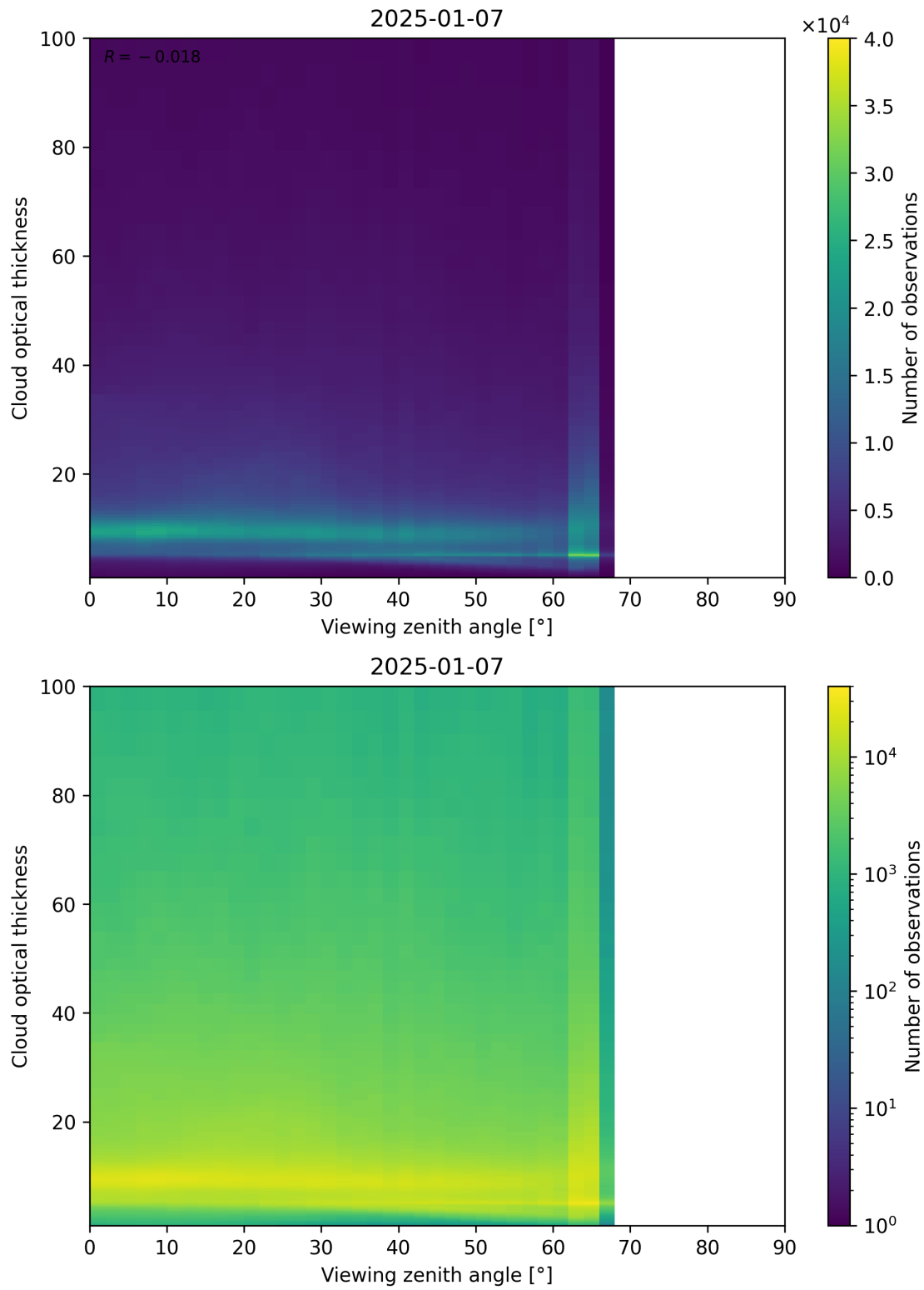
Figure 111: Scatter density plot of “Viewing zenith angle” against “Cloud optical thickness” for 2025-01-07 to 2025-01-08.
