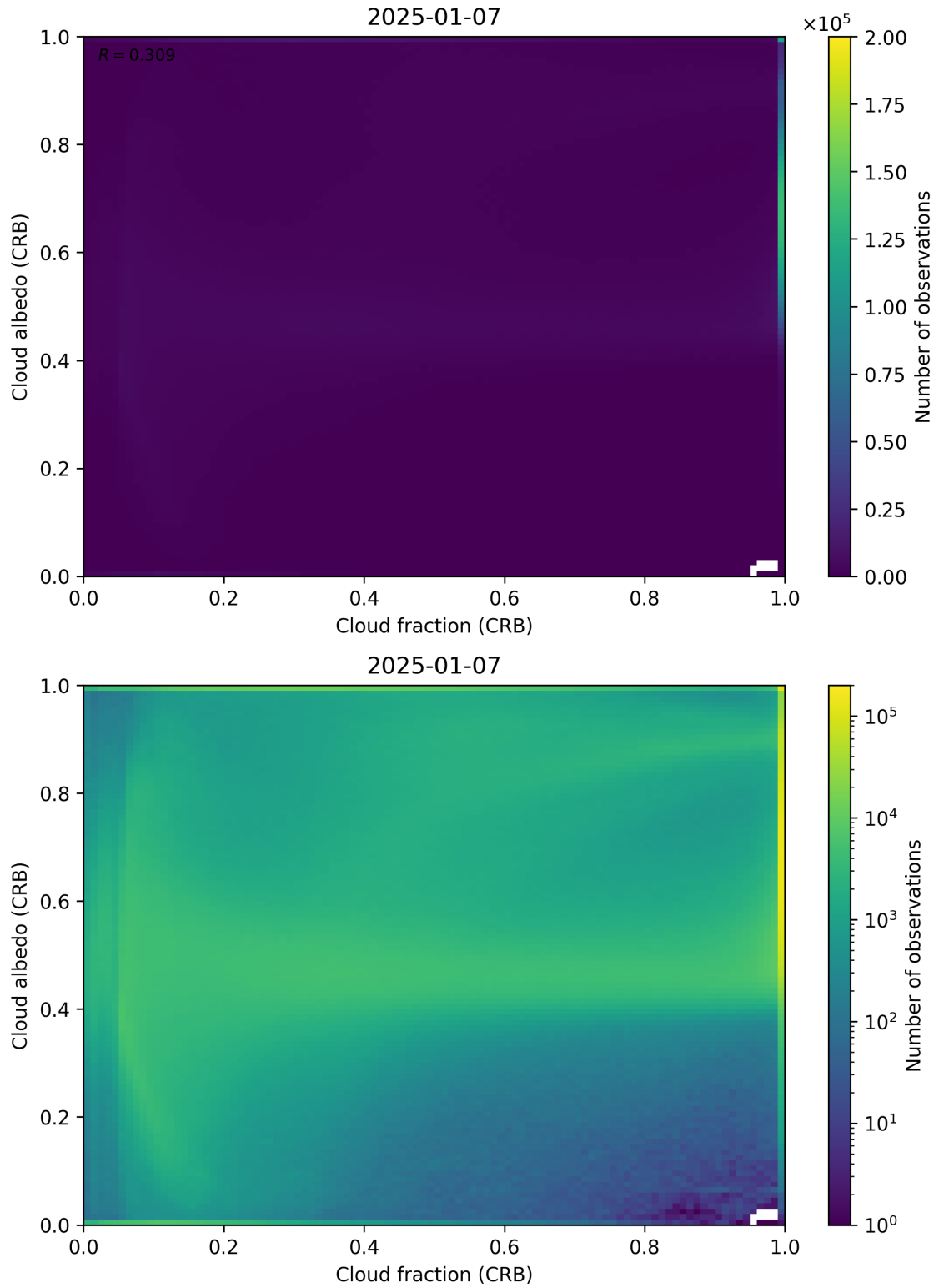
Figure 77: Scatter density plot of “Cloud fraction (CRB)” against “Cloud albedo (CRB)” for 2025-01-07 to 2025-01-08.
