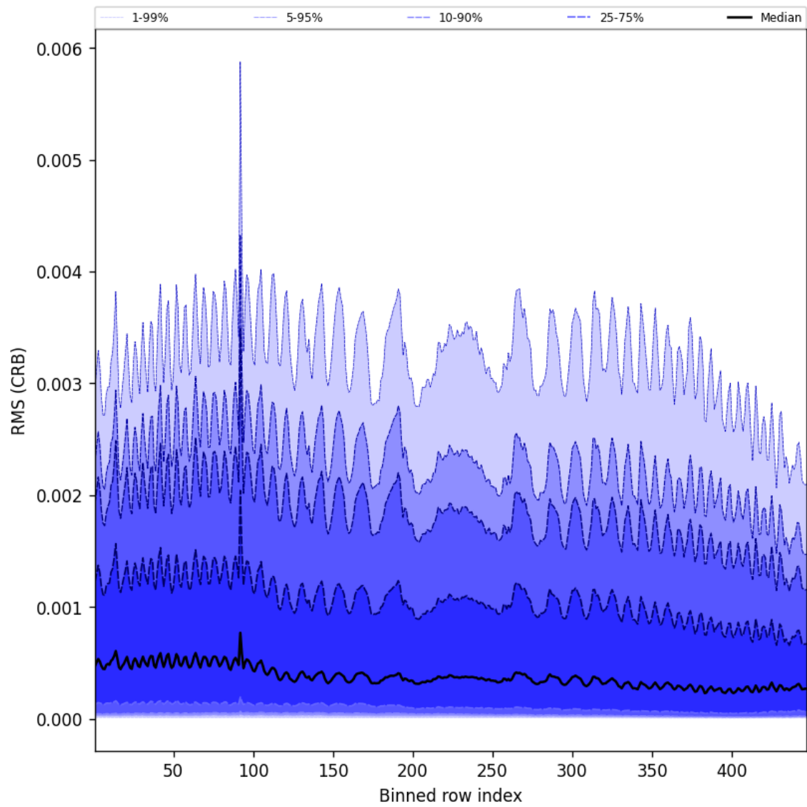
Figure 64: Along track statistics of “RMS (CRB)” for 2025-01-07 to 2025-01-08
