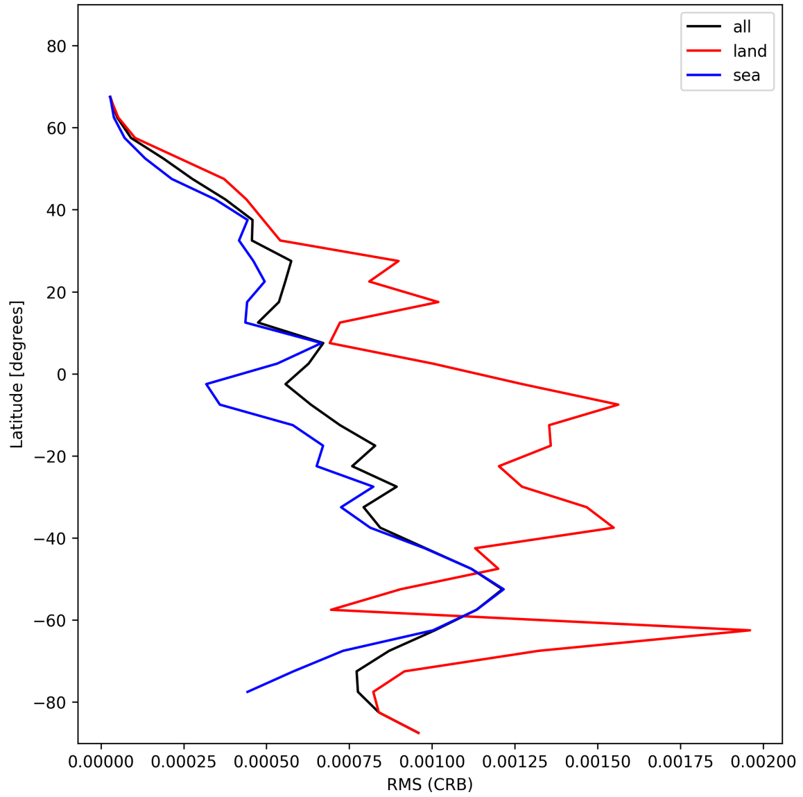
Figure 32: Zonal average of “RMS (CRB)” for 2025-01-07 to 2025-01-08.
