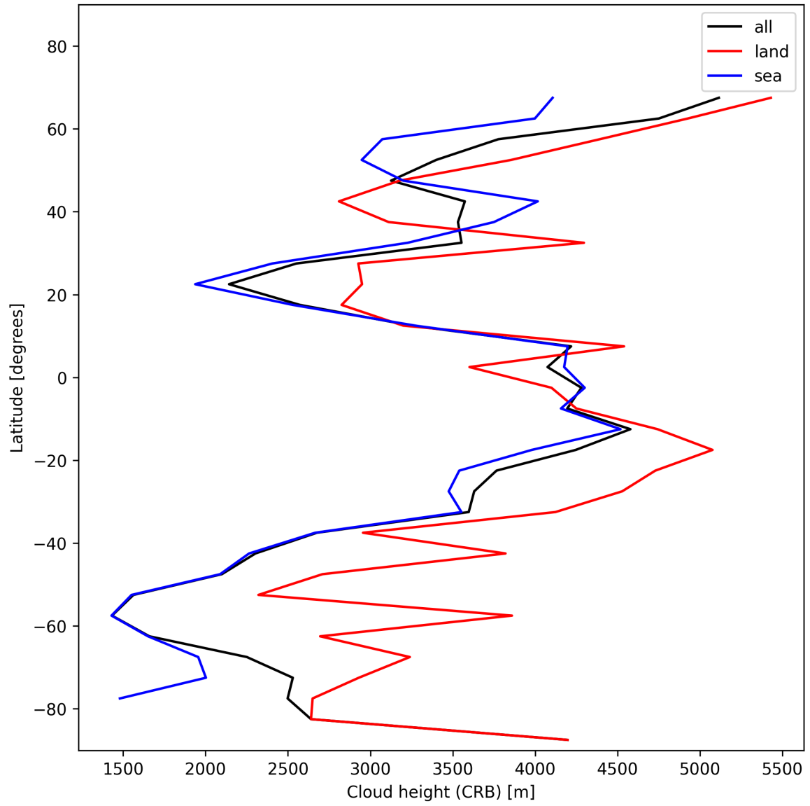
Figure 27: Zonal average of “Cloud height (CRB)” for 2025-01-07 to 2025-01-08.
