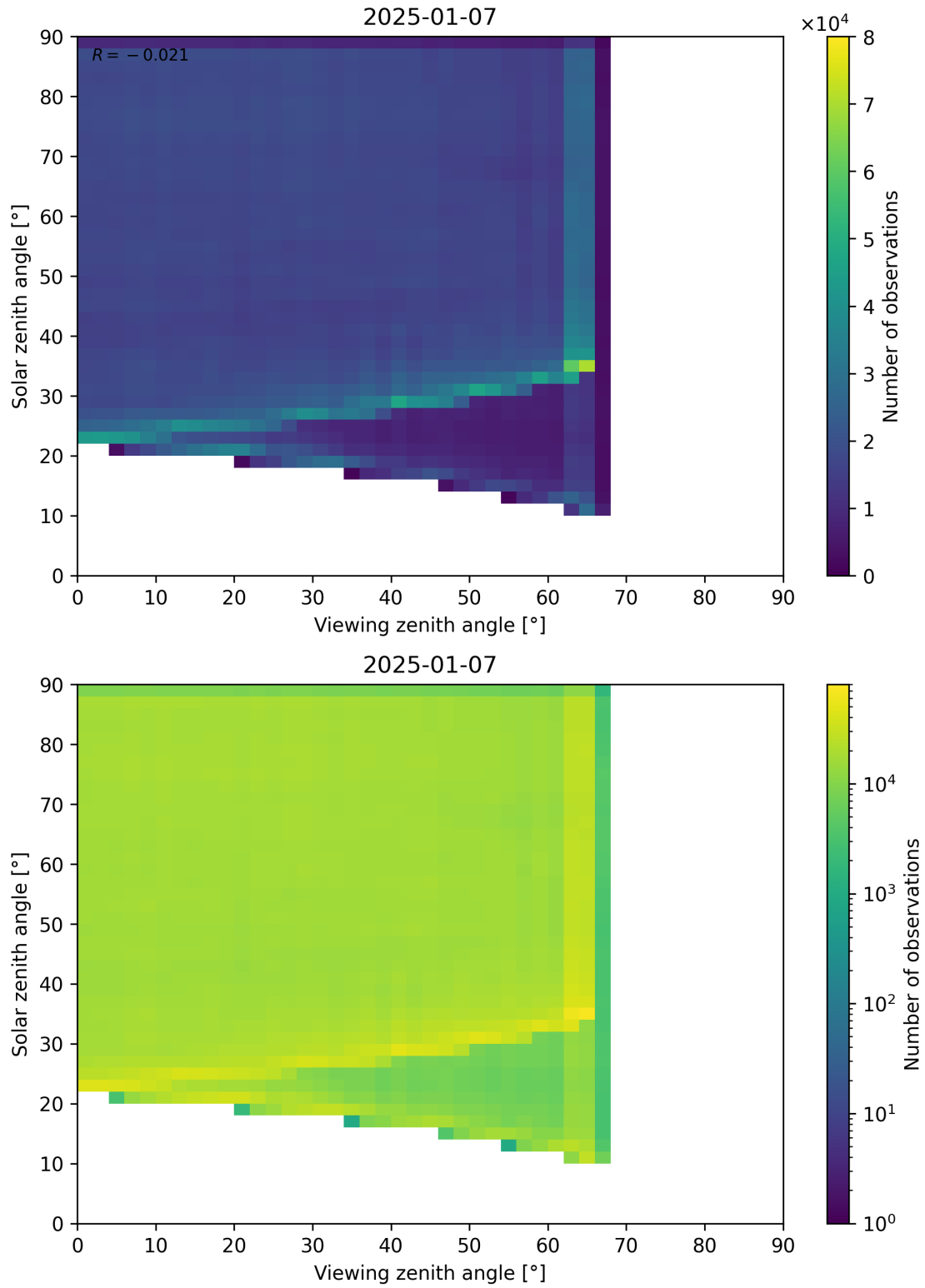
Figure 114: Scatter density plot of “Viewing zenith angle” against “Solar zenith angle” for 2025-01-07 to 2025-01-08.
