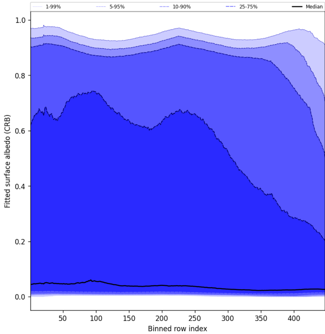
Figure 62: Along track statistics of “Fitted surface albedo (CRB)” for 2025-01-07 to 2025-01-08
