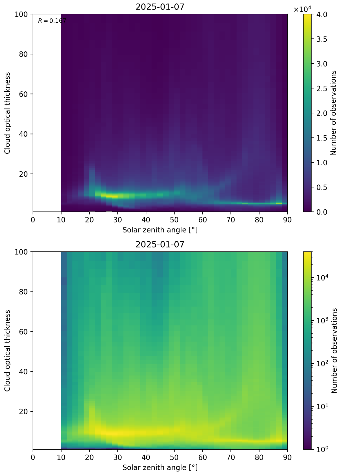
Figure 103: Scatter density plot of “Solar zenith angle” against “Cloud optical thickness” for 2025-01-07 to 2025-01-08.
