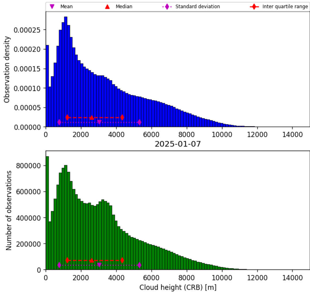
Figure 43: Histogram of “Cloud height (CRB)” for 2025-01-07 to 2025-01-08
