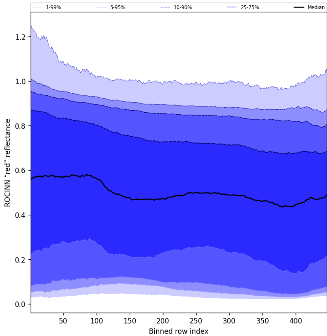
Figure 69: Along track statistics of "ROCINN "red" reflectance" for 2025-01-07 to 2025-01-08
