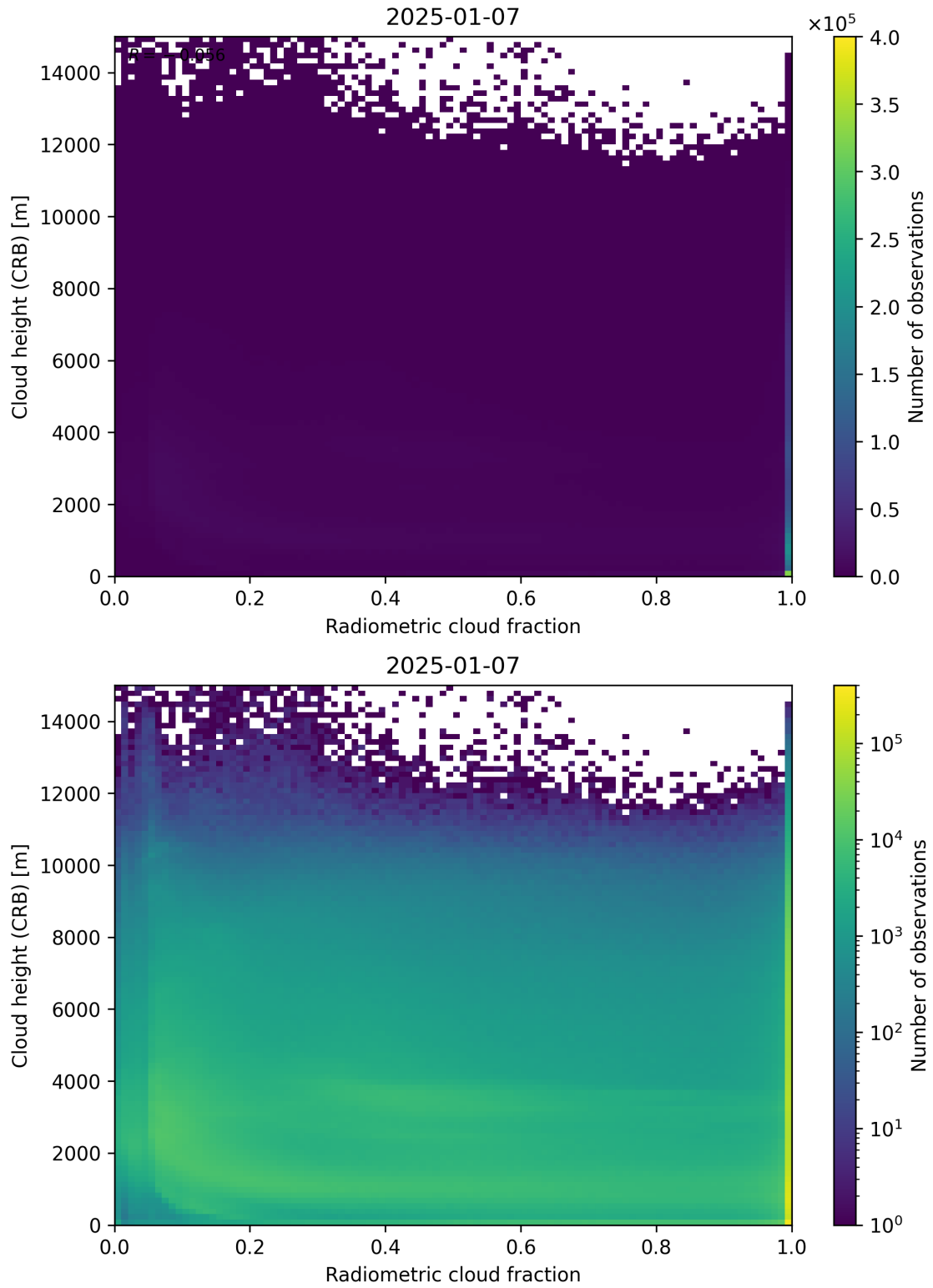
Figure 74: Scatter density plot of “Radiometric cloud fraction” against “Cloud height (CRB)” for 2025-01-07 to 2025-01-08.
