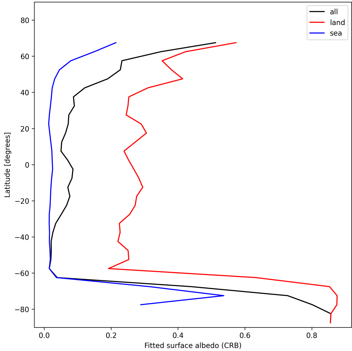
Figure 30: Zonal average of “Fitted surface albedo (CRB)” for 2025-01-07 to 2025-01-08.
