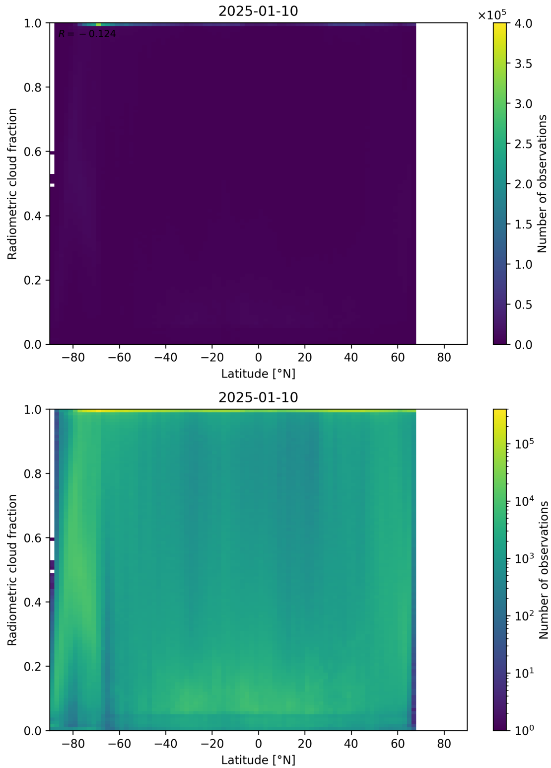
Figure 92: Scatter density plot of “Latitude” against “Radiometric cloud fraction” for 2025-01-09 to 2025-01-11.
