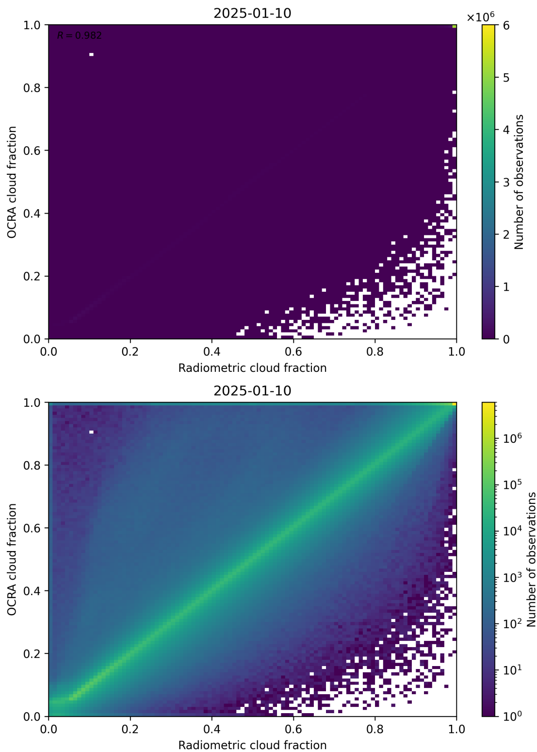
Figure 72: Scatter density plot of “Radiometric cloud fraction” against “OCRA cloud fraction” for 2025-01-09 to 2025-01-11.
