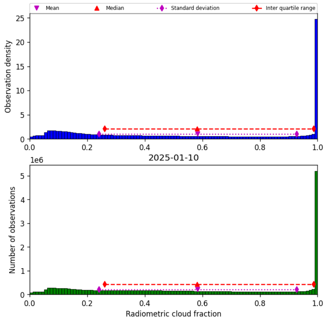
Figure 39: Histogram of “Radiometric cloud fraction” for 2025-01-09 to 2025-01-11
