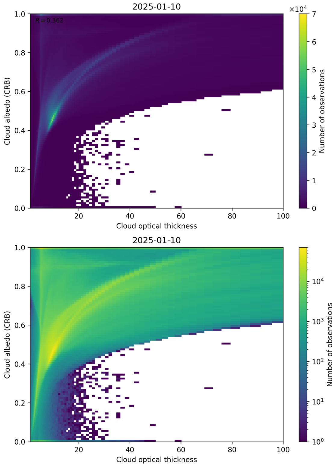
Figure 82: Scatter density plot of “Cloud optical thickness” against “Cloud albedo (CRB)” for 2025-01-09 to 2025-01-11.
