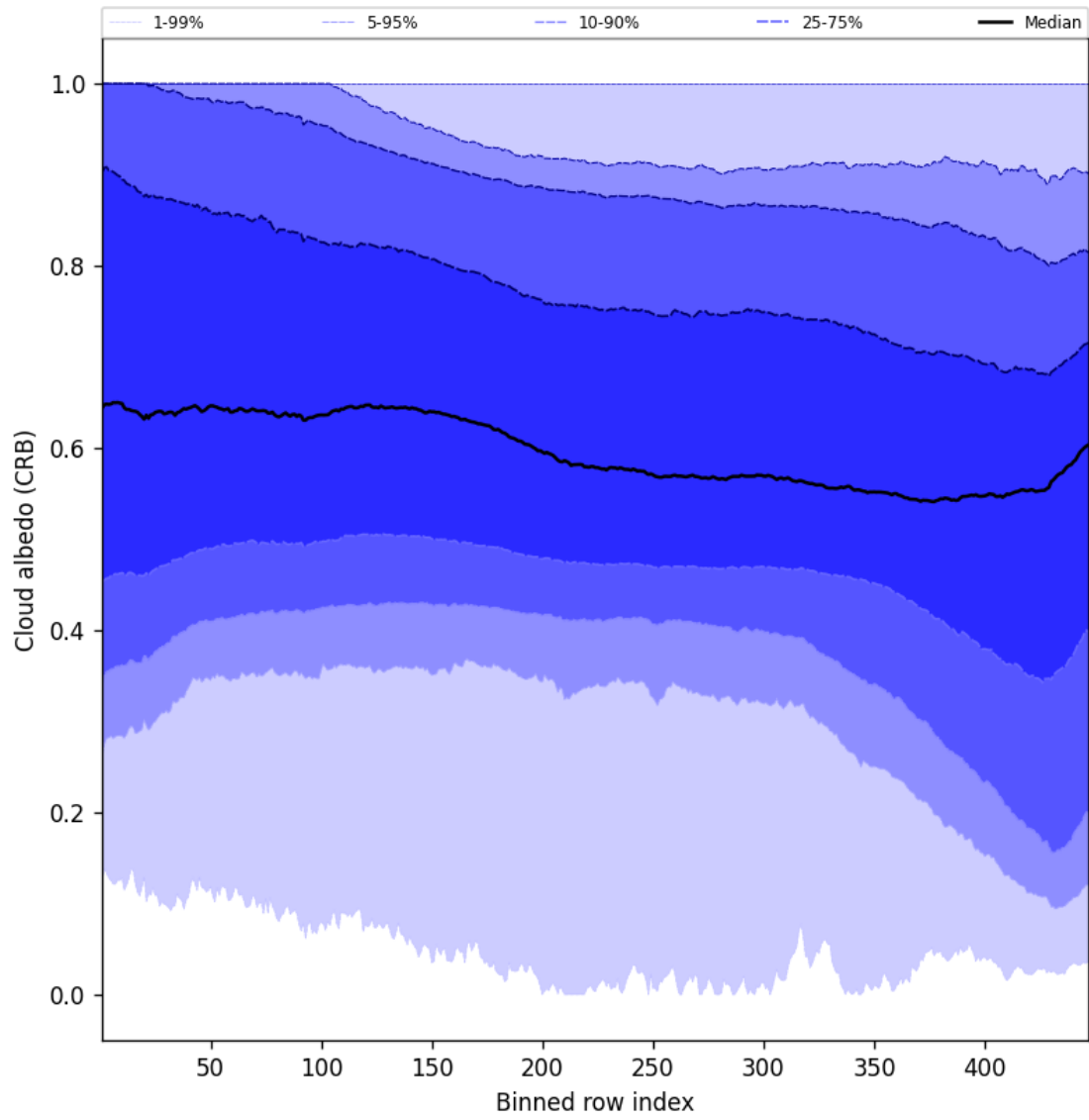
Figure 60: Along track statistics of “Cloud albedo (CRB)” for 2025-01-09 to 2025-01-11
