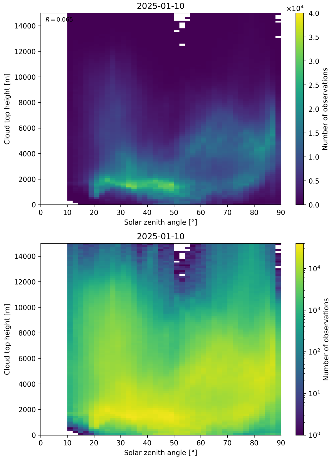
Figure 104: Scatter density plot of “Solar zenith angle” against “Cloud top height” for 2025-01-09 to 2025-01-11.
