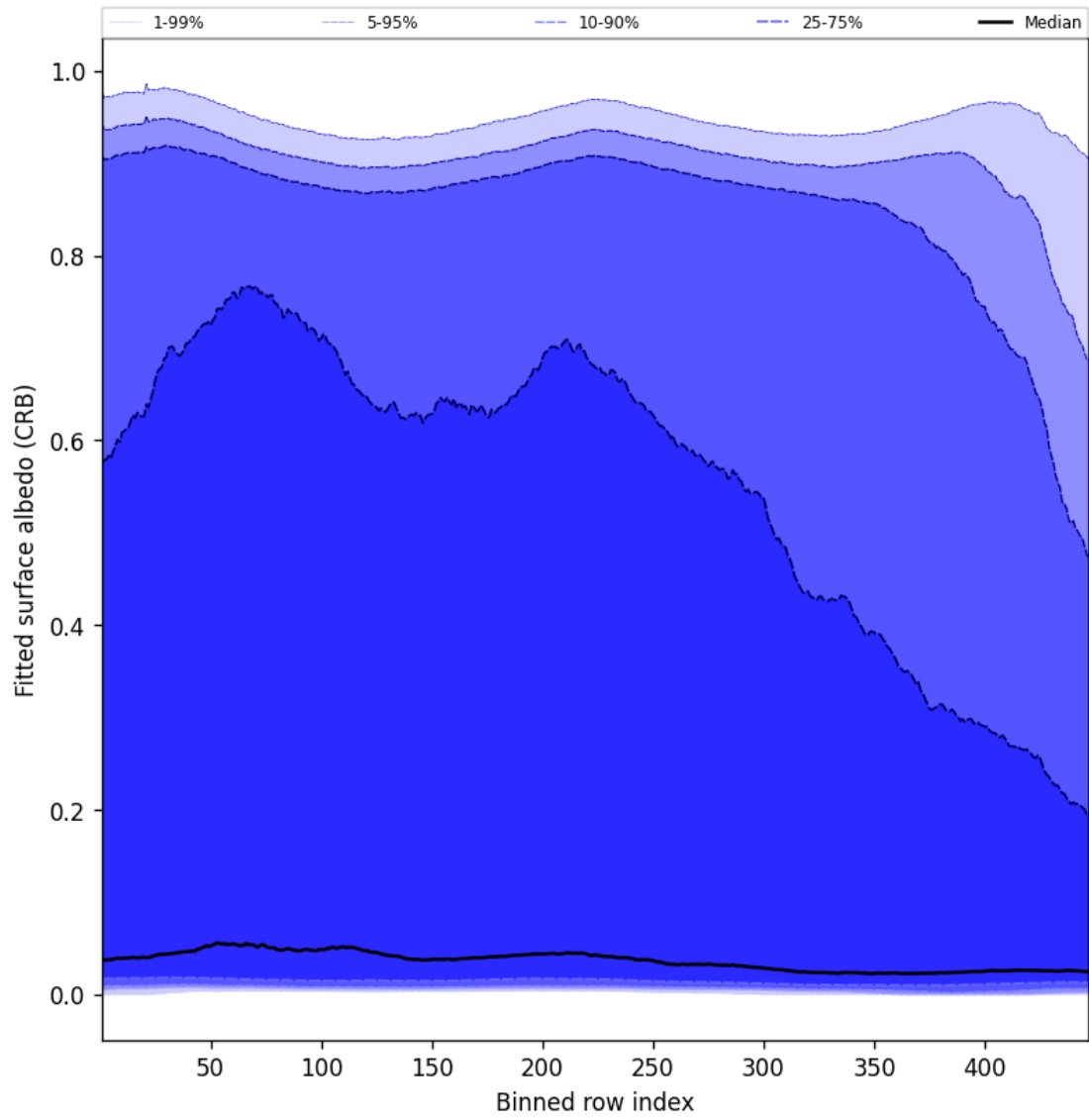
Figure 62: Along track statistics of “Fitted surface albedo (CRB)” for 2025-01-09 to 2025-01-11
