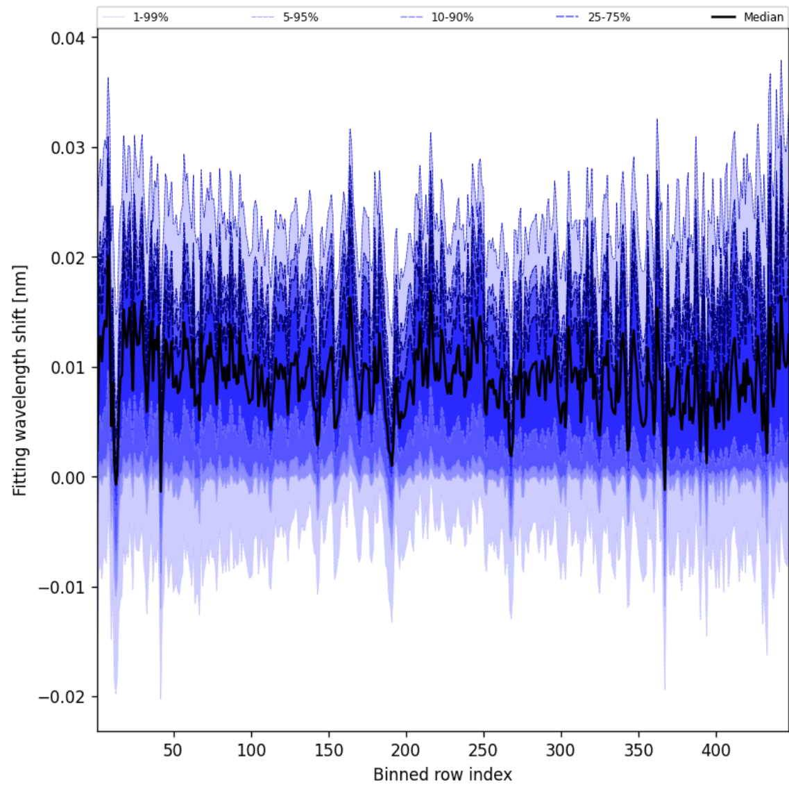
Figure 65: Along track statistics of “Fitting wavelength shift” for 2025-01-09 to 2025-01-11
