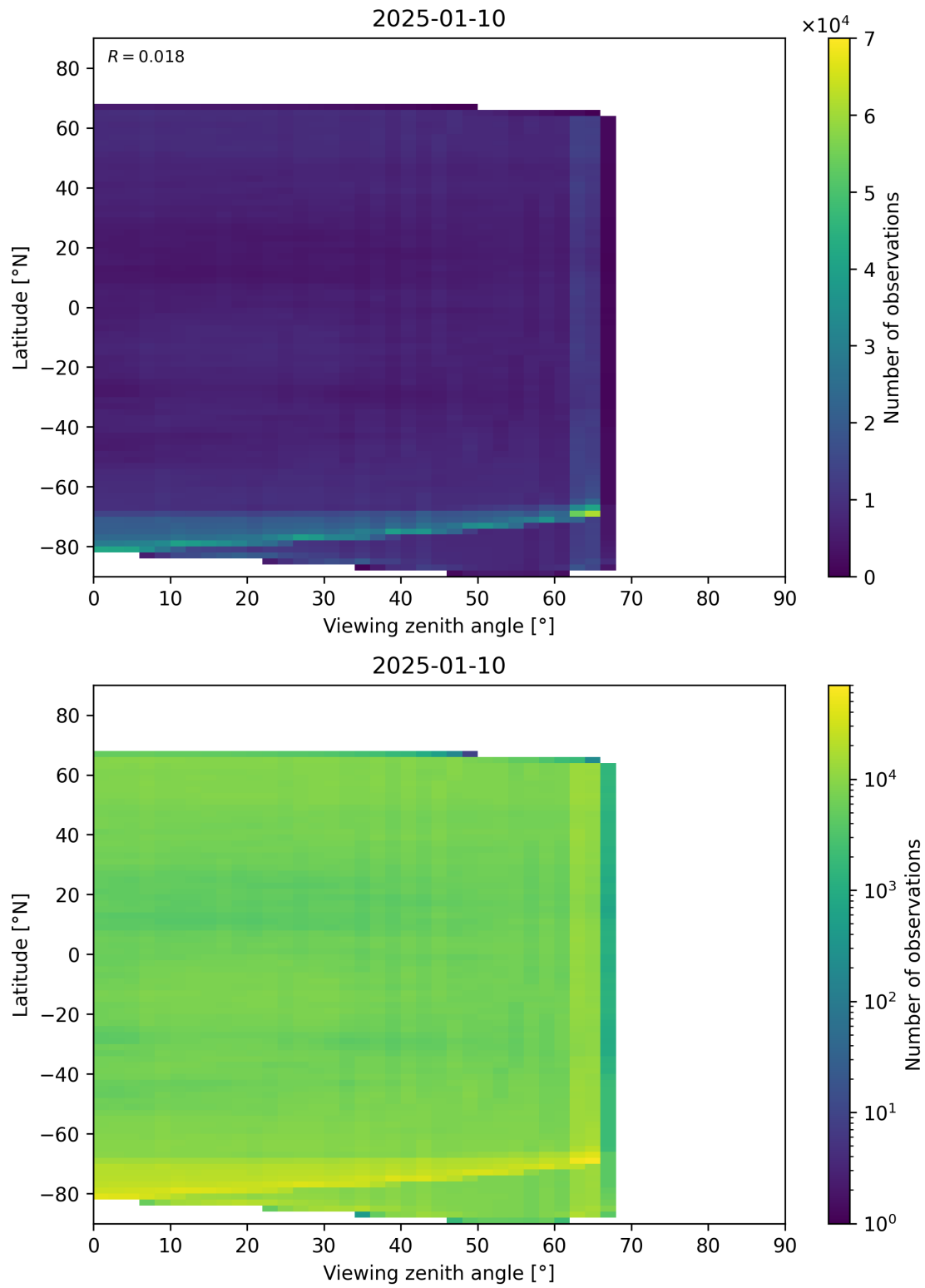
Figure 113: Scatter density plot of “Viewing zenith angle” against “Latitude” for 2025-01-09 to 2025-01-11.
