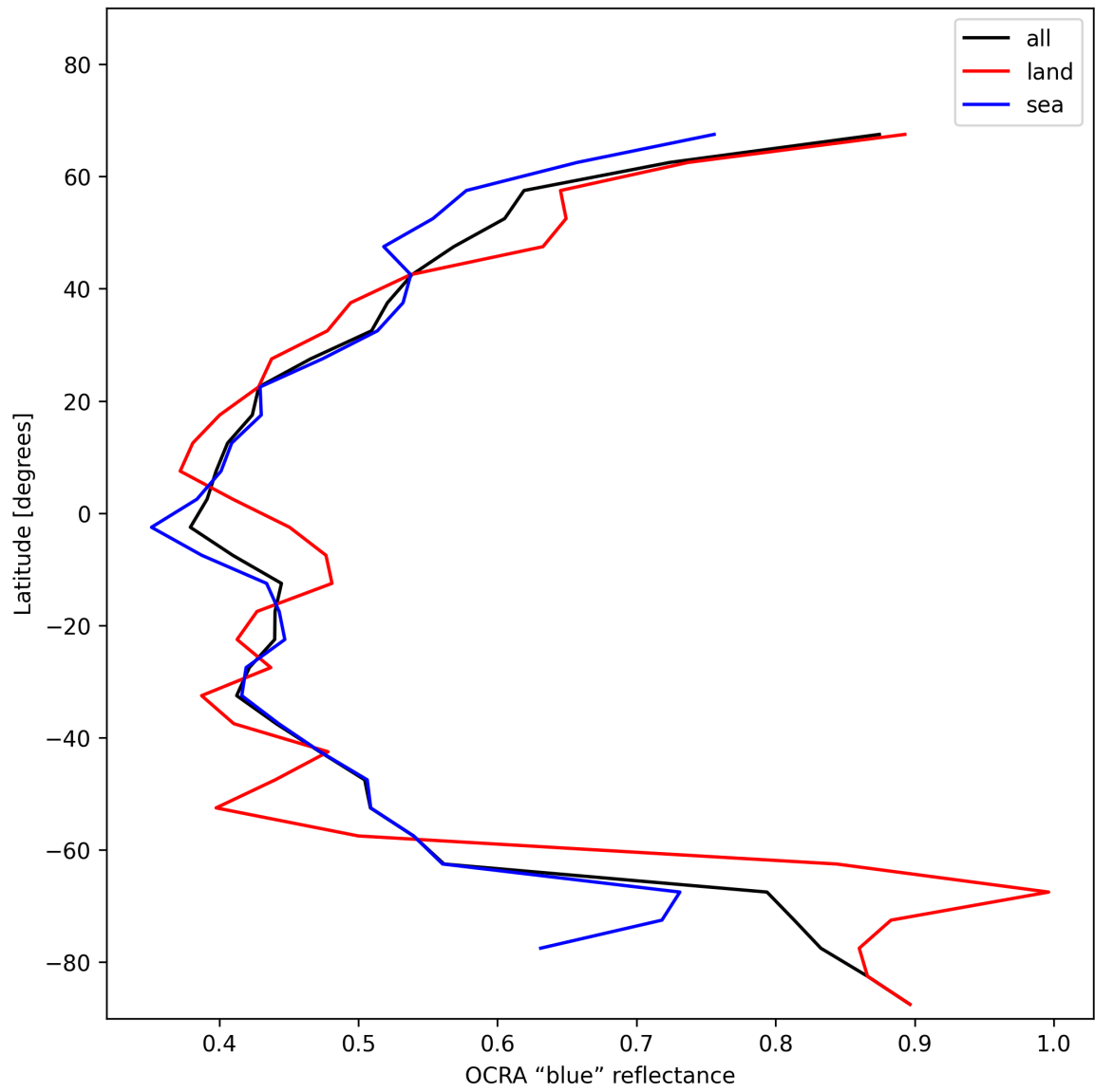
Figure 35: Zonal average of “OCRA “blue” reflectance” for 2025-01-09 to 2025-01-11.
