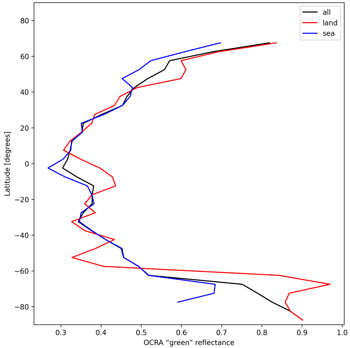
Figure 36: Zonal average of “OCRA “green” reflectance” for 2025-01-09 to 2025-01-11.
