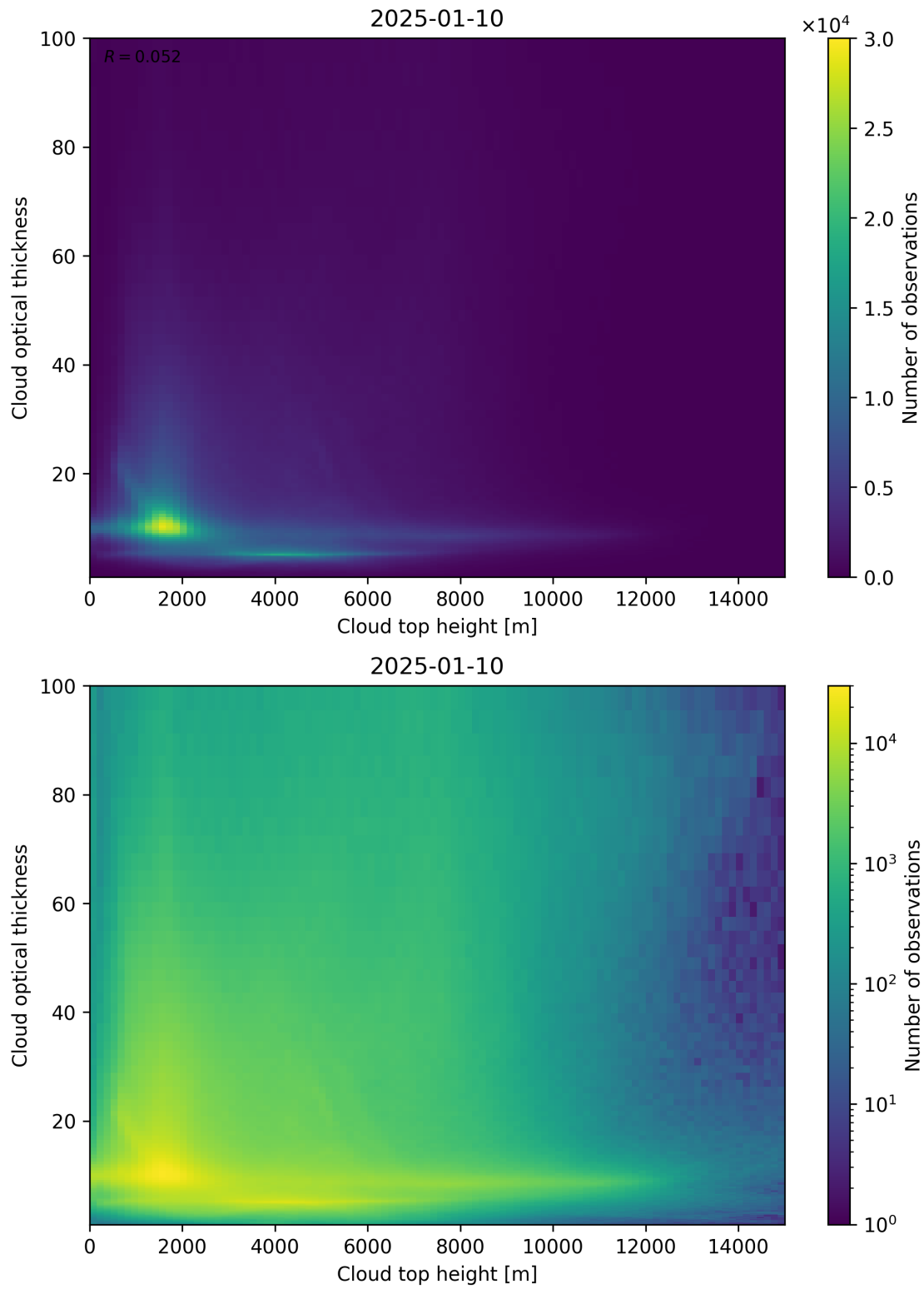
Figure 90: Scatter density plot of “Cloud top height” against “Cloud optical thickness” for 2025-01-09 to 2025-01-11.
