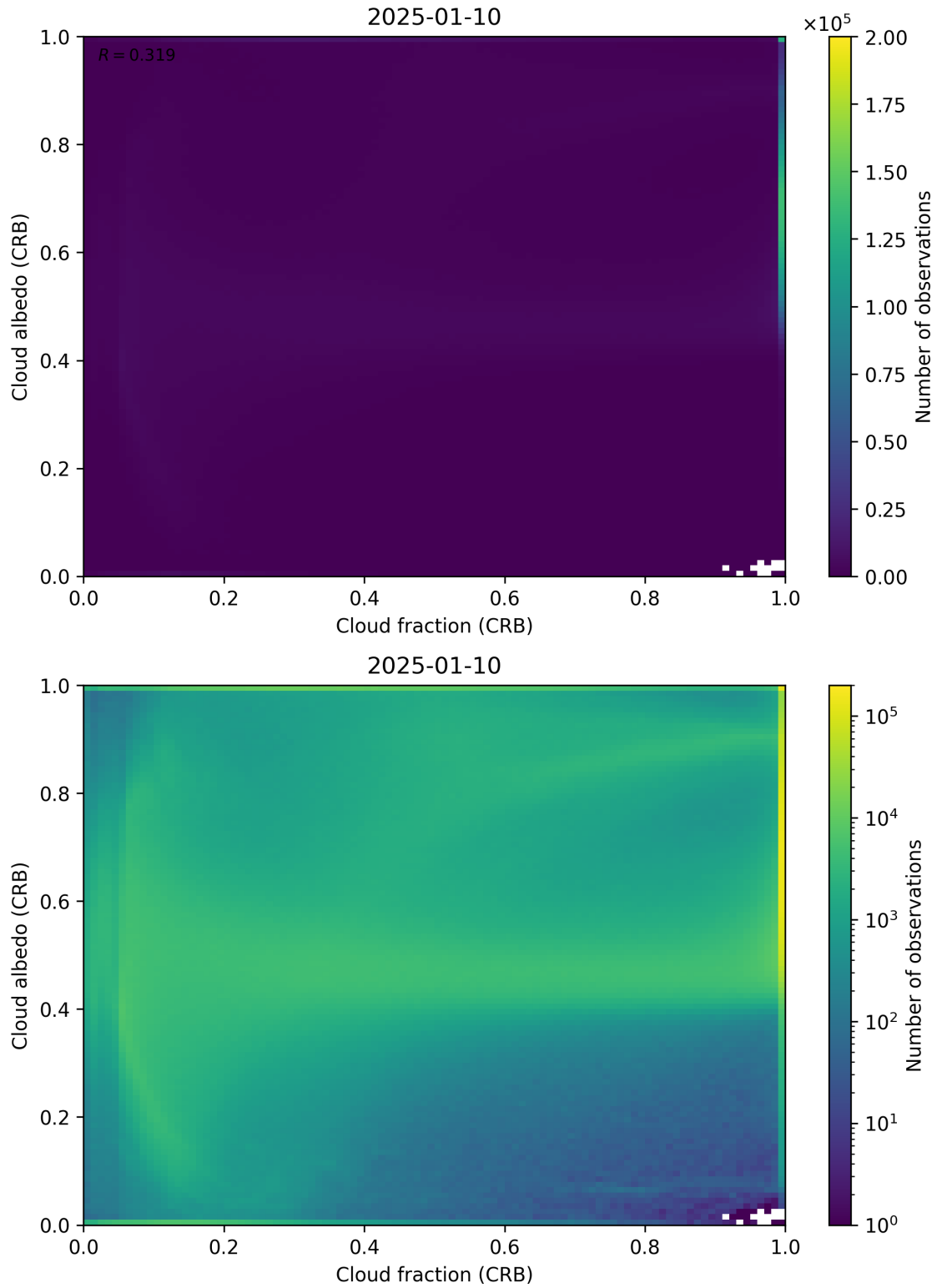
Figure 77: Scatter density plot of “Cloud fraction (CRB)” against “Cloud albedo (CRB)” for 2025-01-09 to 2025-01-11.
