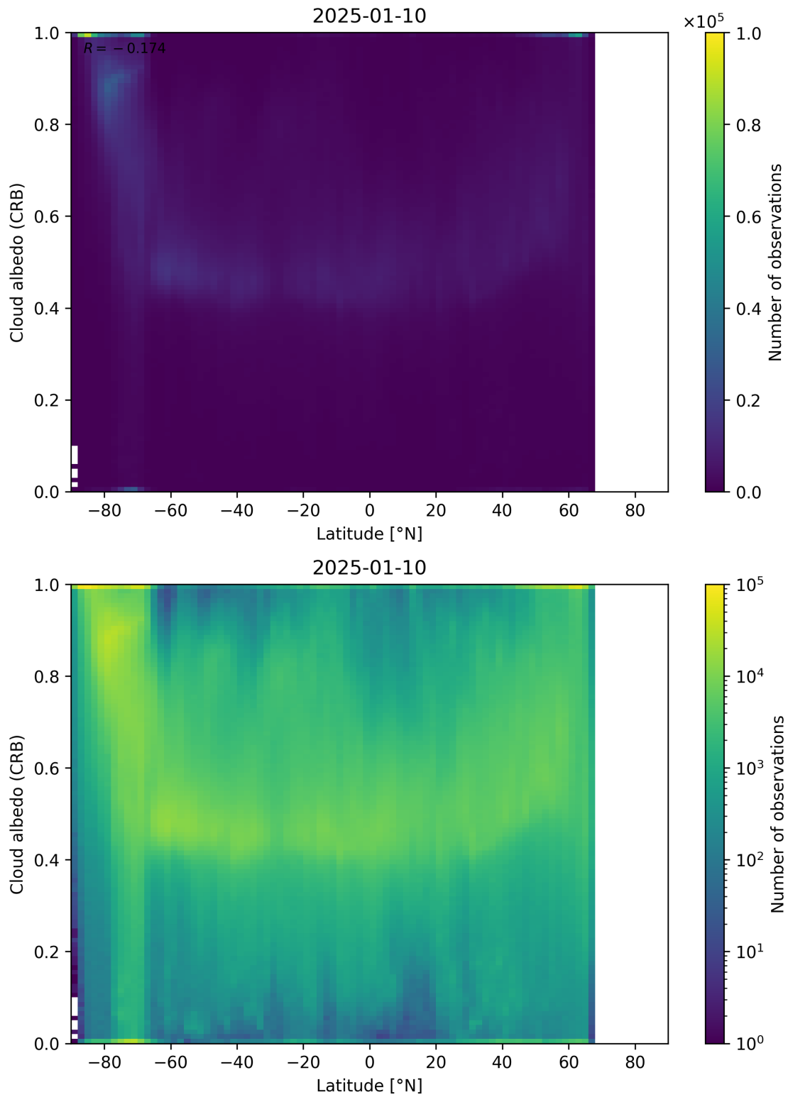
Figure 91: Scatter density plot of “Latitude” against “Cloud albedo (CRB)” for 2025-01-09 to 2025-01-11.
