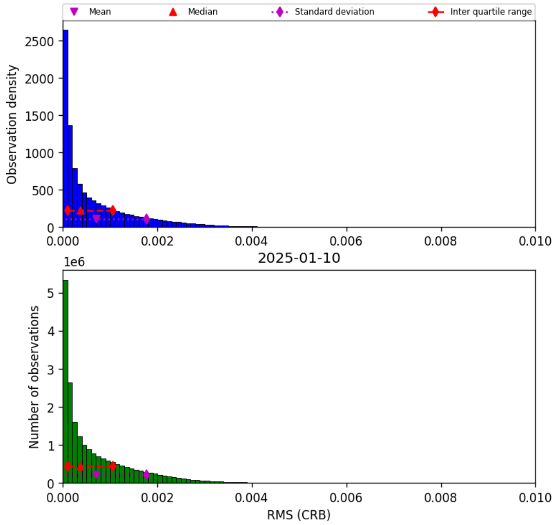
Figure 48: Histogram of “RMS (CRB)” for 2025-01-09 to 2025-01-11
