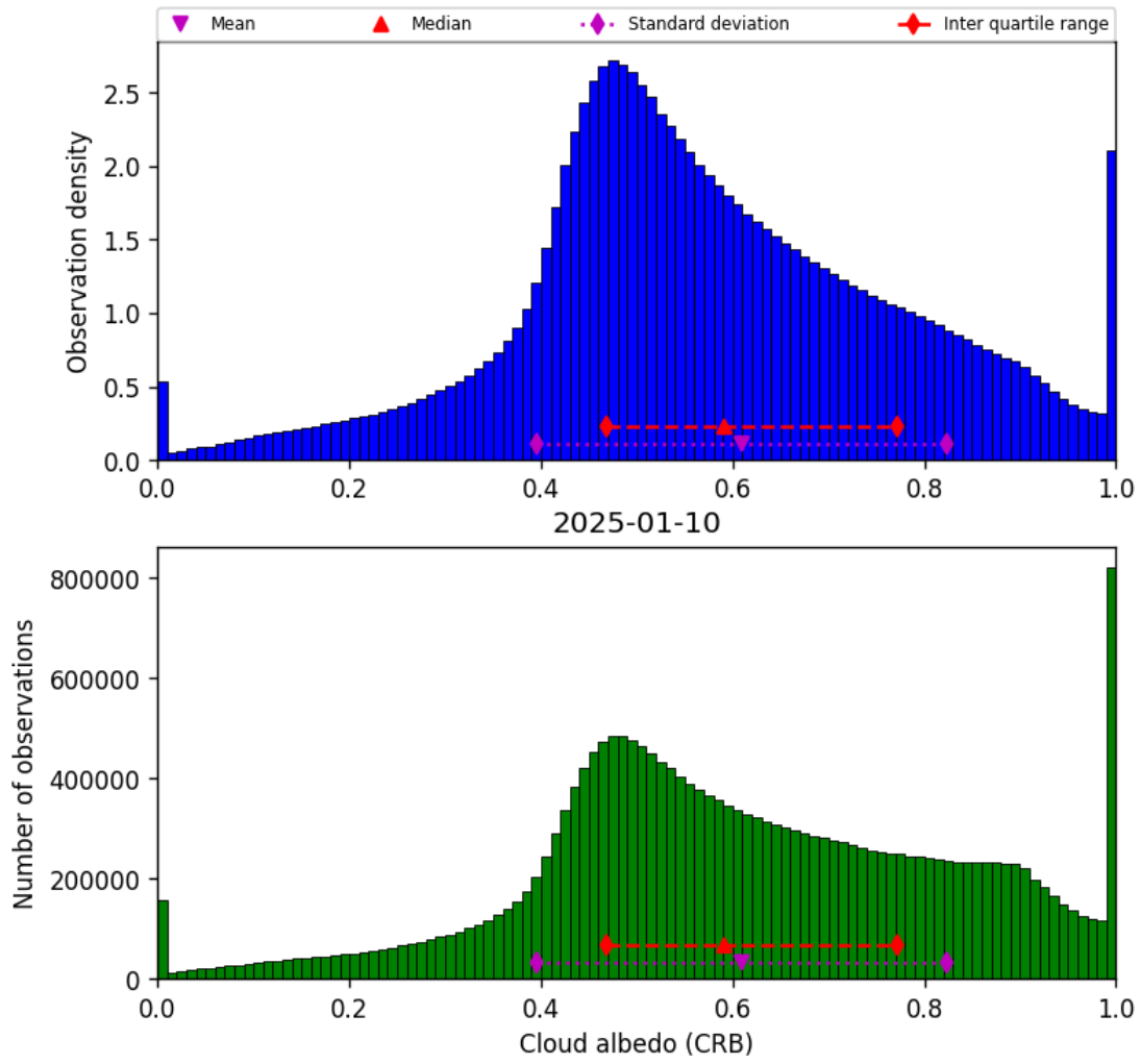
Figure 44: Histogram of “Cloud albedo (CRB)” for 2025-01-09 to 2025-01-11
