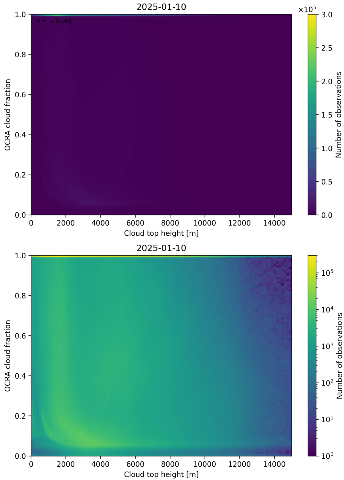
Figure 87: Scatter density plot of “Cloud top height” against “OCRA cloud fraction” for 2025-01-09 to 2025-01-11.
