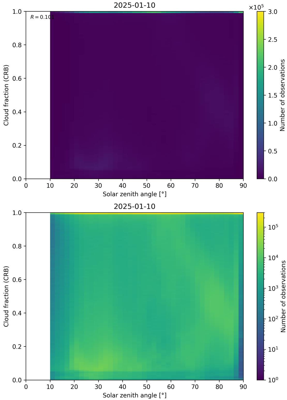
Figure 101: Scatter density plot of “Solar zenith angle” against “Cloud fraction (CRB)” for 2025-01-09 to 2025-01-11.
