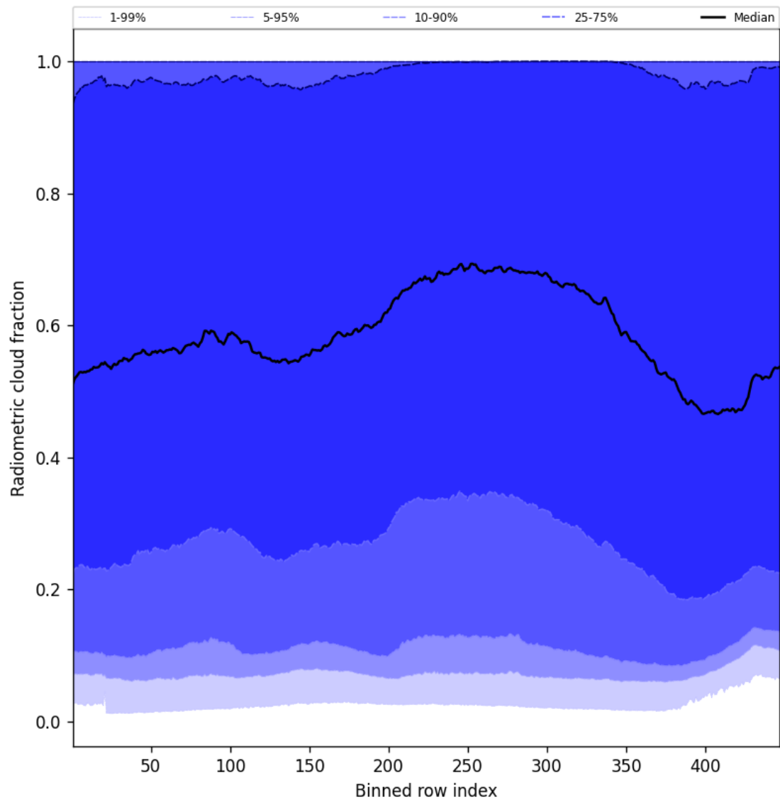
Figure 55: Along track statistics of “Radiometric cloud fraction” for 2025-01-09 to 2025-01-11
