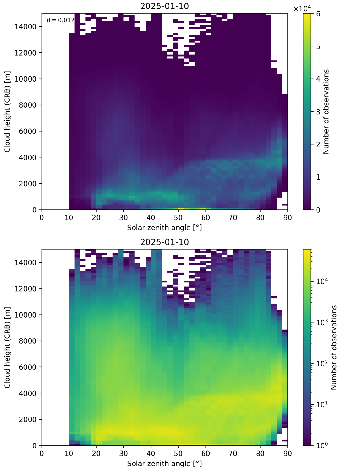
Figure 102: Scatter density plot of “Solar zenith angle” against “Cloud height (CRB)” for 2025-01-09 to 2025-01-11.
