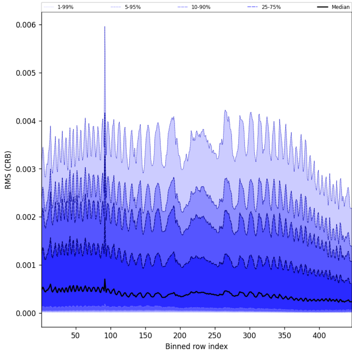
Figure 64: Along track statistics of “RMS (CRB)” for 2025-01-09 to 2025-01-11
