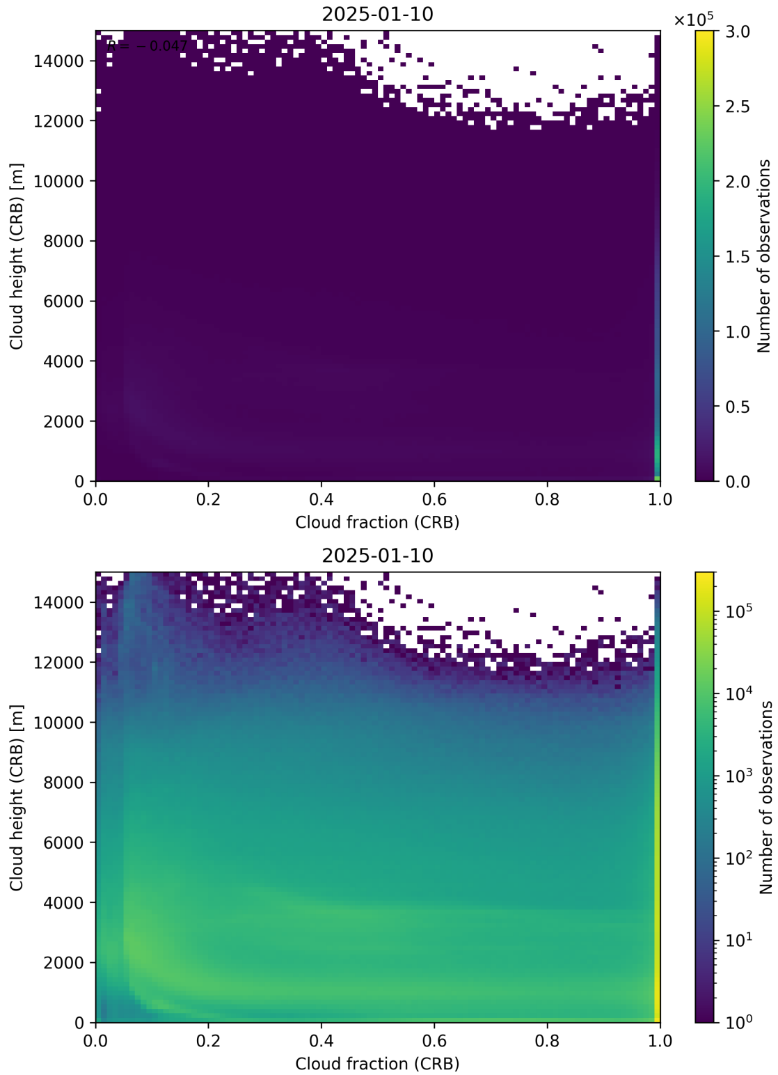
Figure 79: Scatter density plot of “Cloud fraction (CRB)” against “Cloud height (CRB)” for 2025-01-09 to 2025-01-11.
