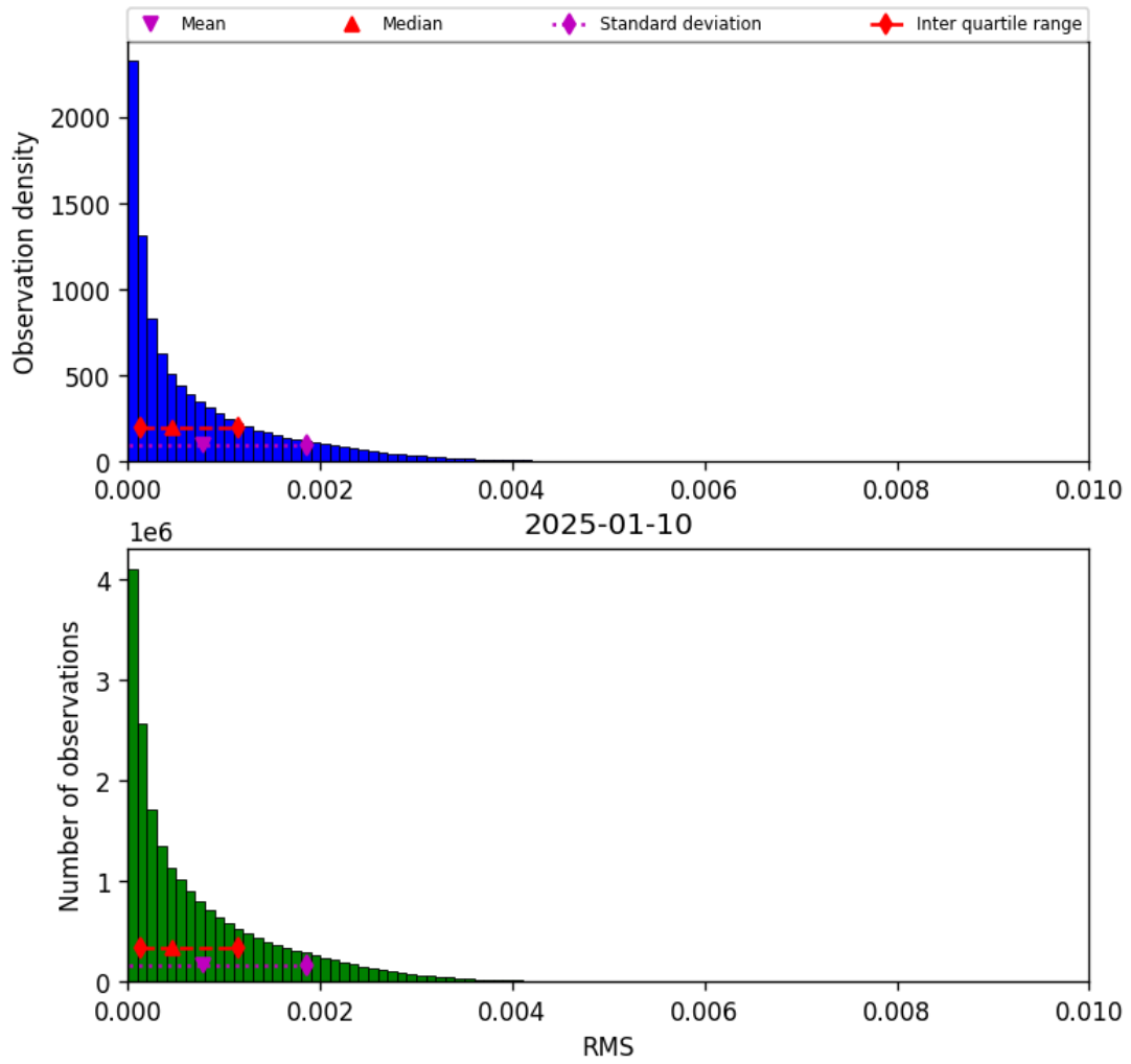
Figure 47: Histogram of “RMS” for 2025-01-09 to 2025-01-11
