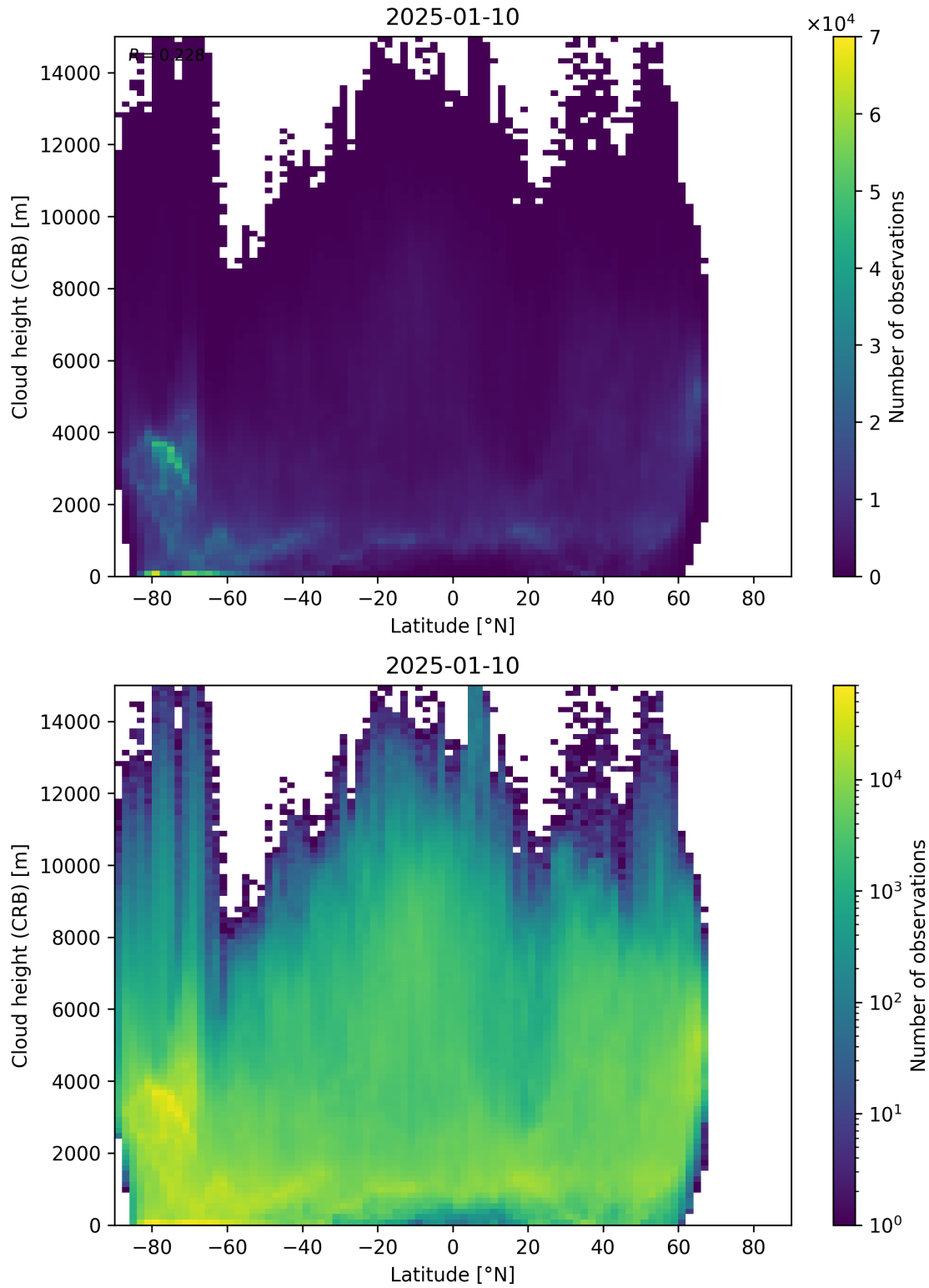
Figure 95: Scatter density plot of “Latitude” against “Cloud height (CRB)” for 2025-01-09 to 2025-01-11.
