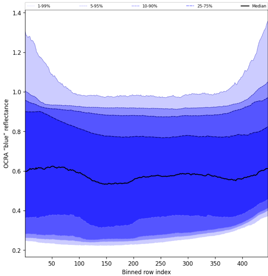
Figure 67: Along track statistics of “OCRA “blue” reflectance” for 2025-01-09 to 2025-01-11
