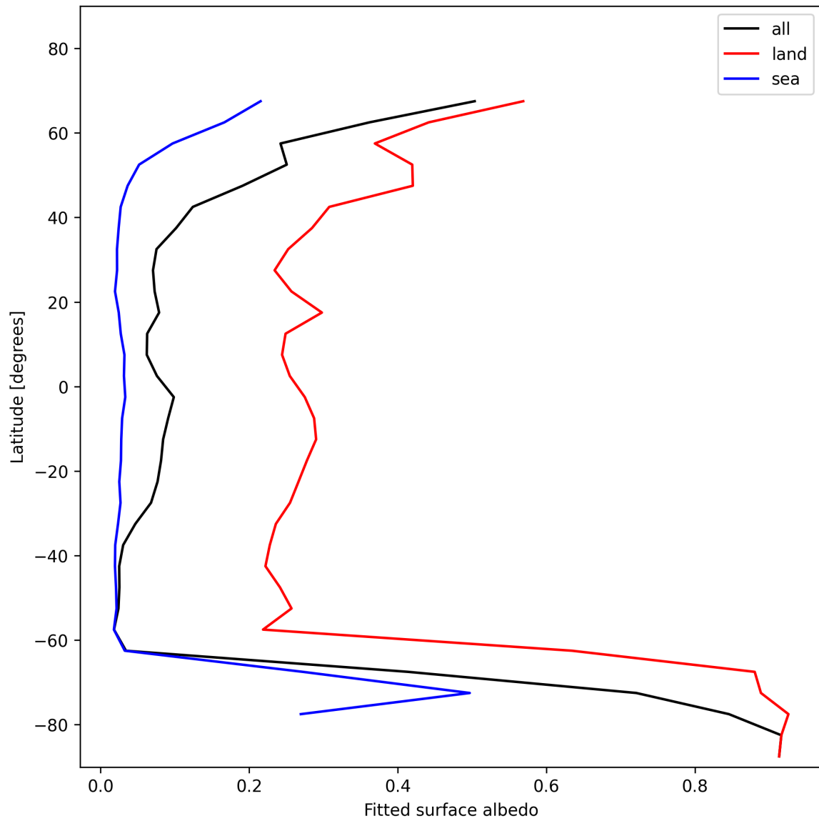
Figure 29: Zonal average of “Fitted surface albedo” for 2025-01-09 to 2025-01-11.
