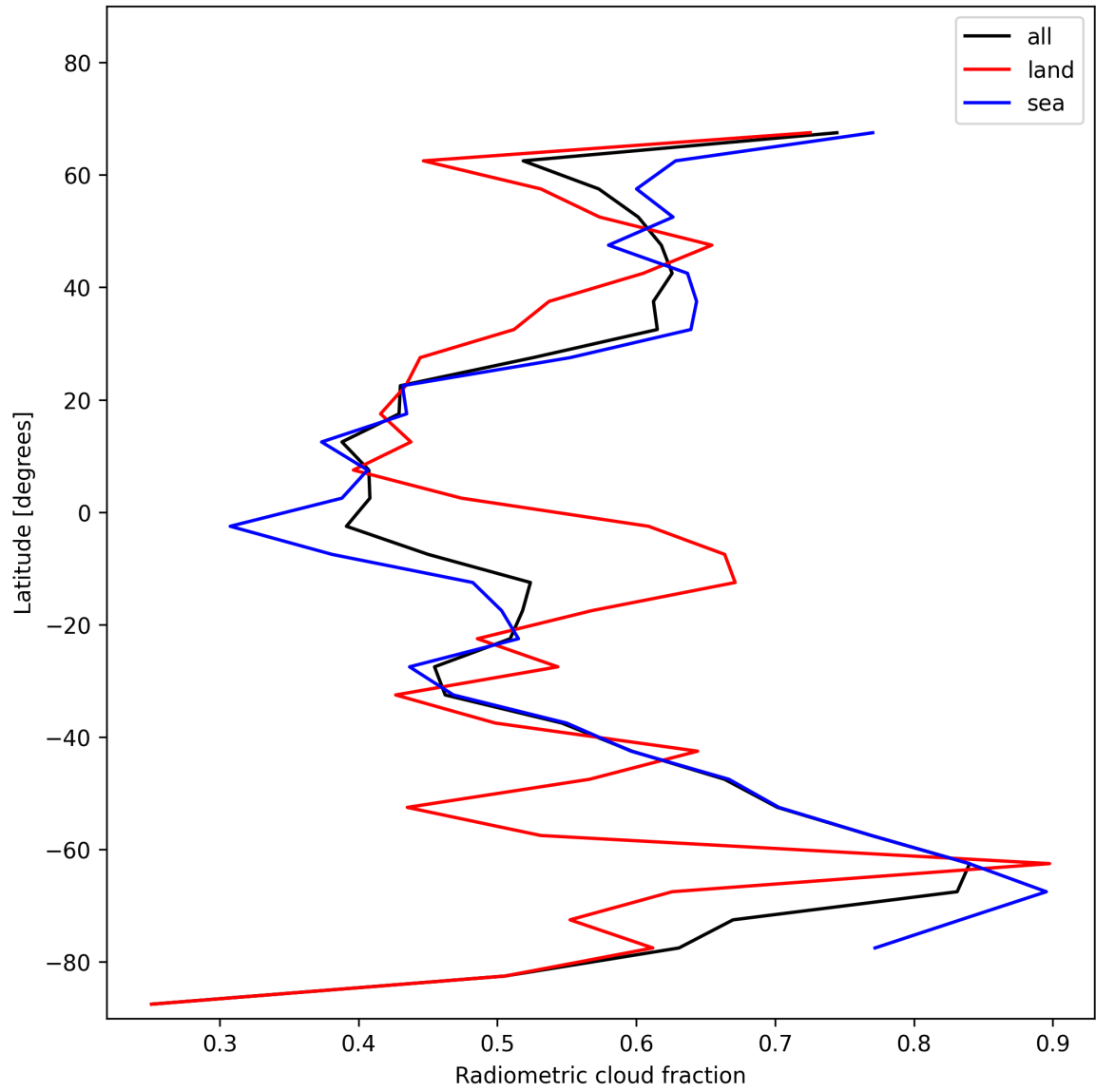
Figure 23: Zonal average of “Radiometric cloud fraction” for 2025-01-09 to 2025-01-11.
