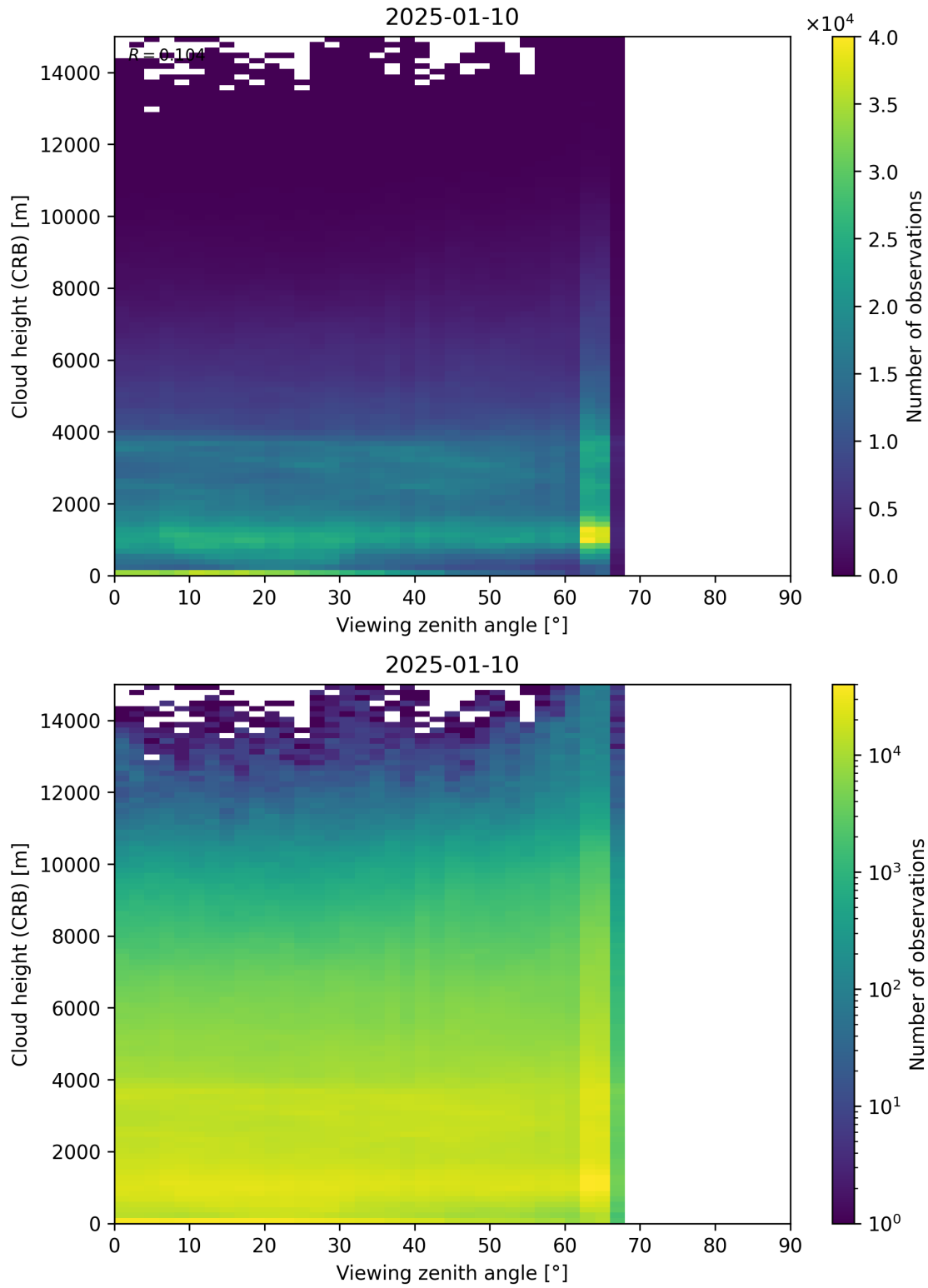
Figure 110: Scatter density plot of “Viewing zenith angle” against “Cloud height (CRB)” for 2025-01-09 to 2025-01-11.
