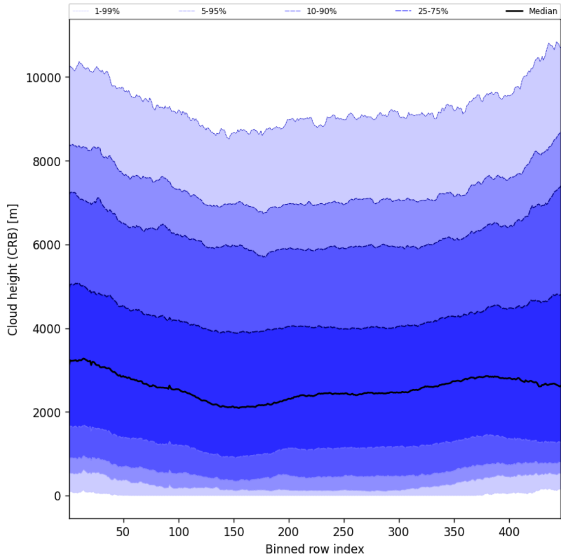
Figure 59: Along track statistics of “Cloud height (CRB)” for 2025-01-09 to 2025-01-11
