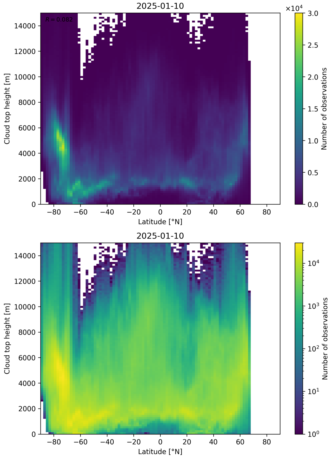
Figure 97: Scatter density plot of “Latitude” against “Cloud top height” for 2025-01-09 to 2025-01-11.
