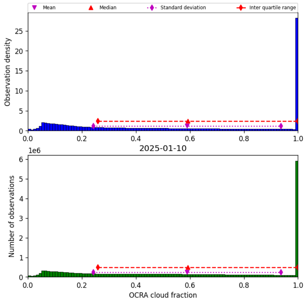
Figure 50: Histogram of “OCRA cloud fraction” for 2025-01-09 to 2025-01-11
