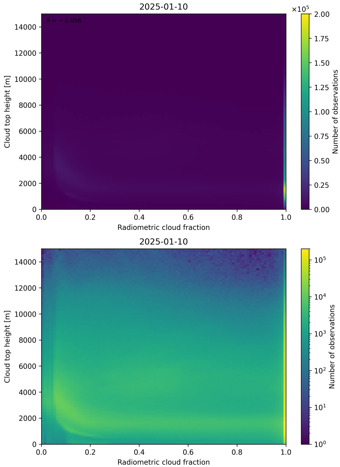
Figure 76: Scatter density plot of “Radiometric cloud fraction” against “Cloud top height” for 2025-01-09 to 2025-01-11.
