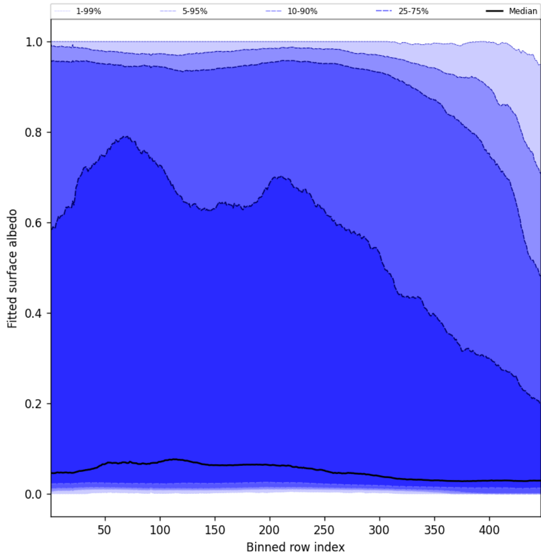
Figure 61: Along track statistics of “Fitted surface albedo” for 2025-01-09 to 2025-01-11
