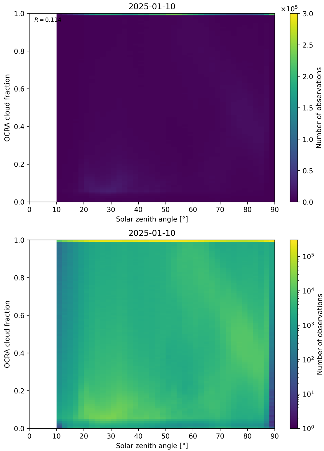
Figure 100: Scatter density plot of “Solar zenith angle” against “OCRA cloud fraction” for 2025-01-09 to 2025-01-11.
