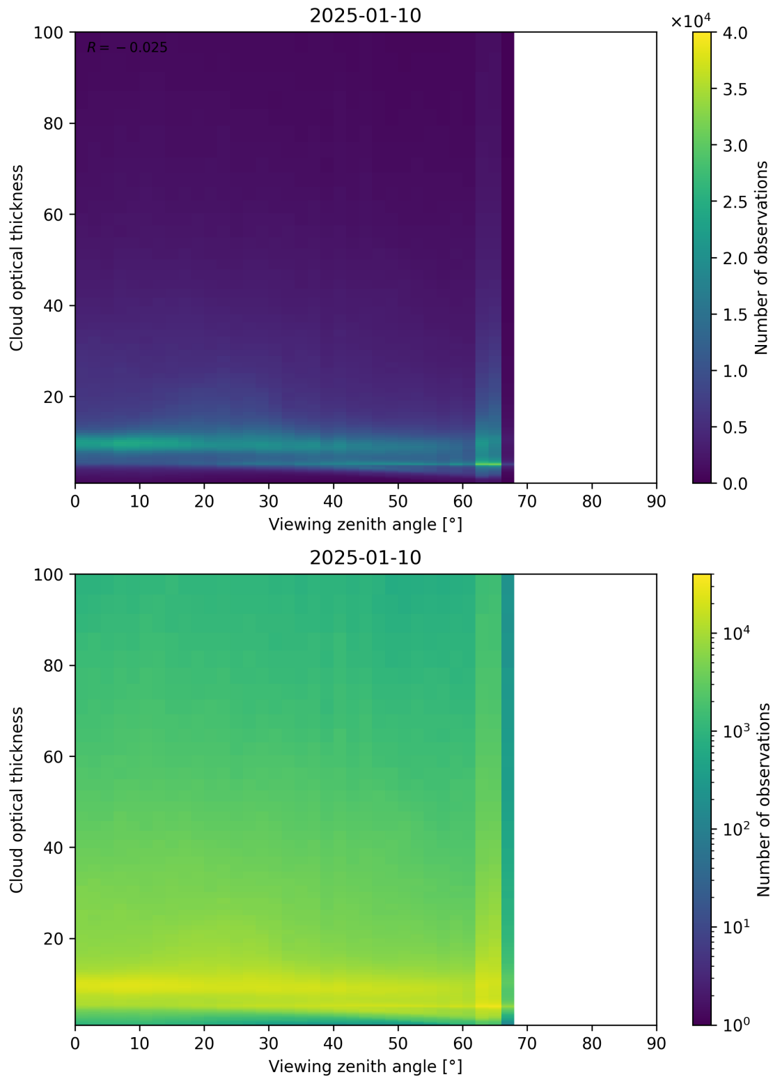
Figure 111: Scatter density plot of “Viewing zenith angle” against “Cloud optical thickness” for 2025-01-09 to 2025-01-11.
