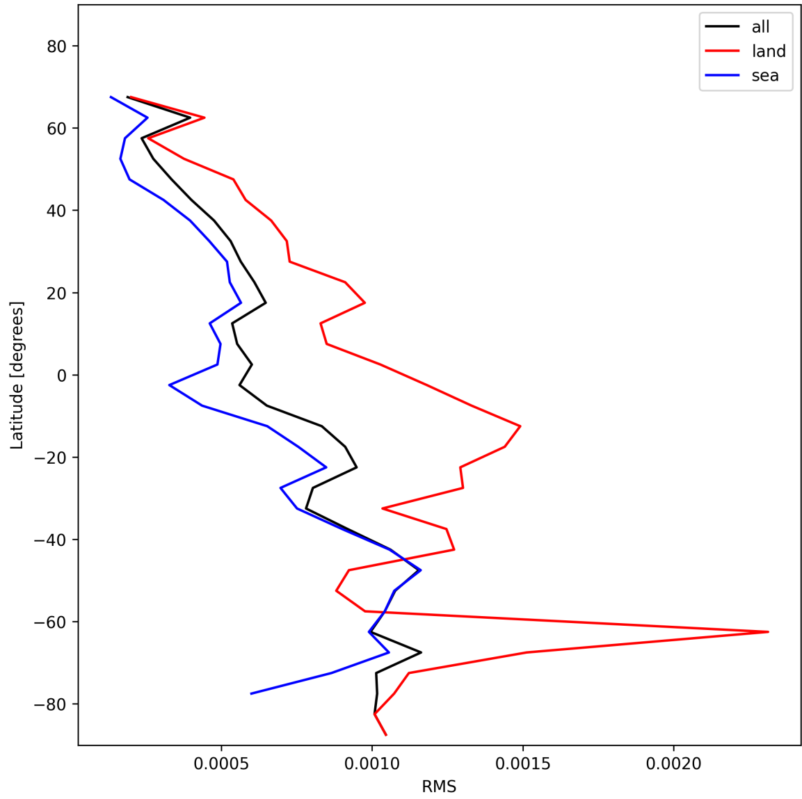
Figure 31: Zonal average of “RMS” for 2025-01-09 to 2025-01-11.
