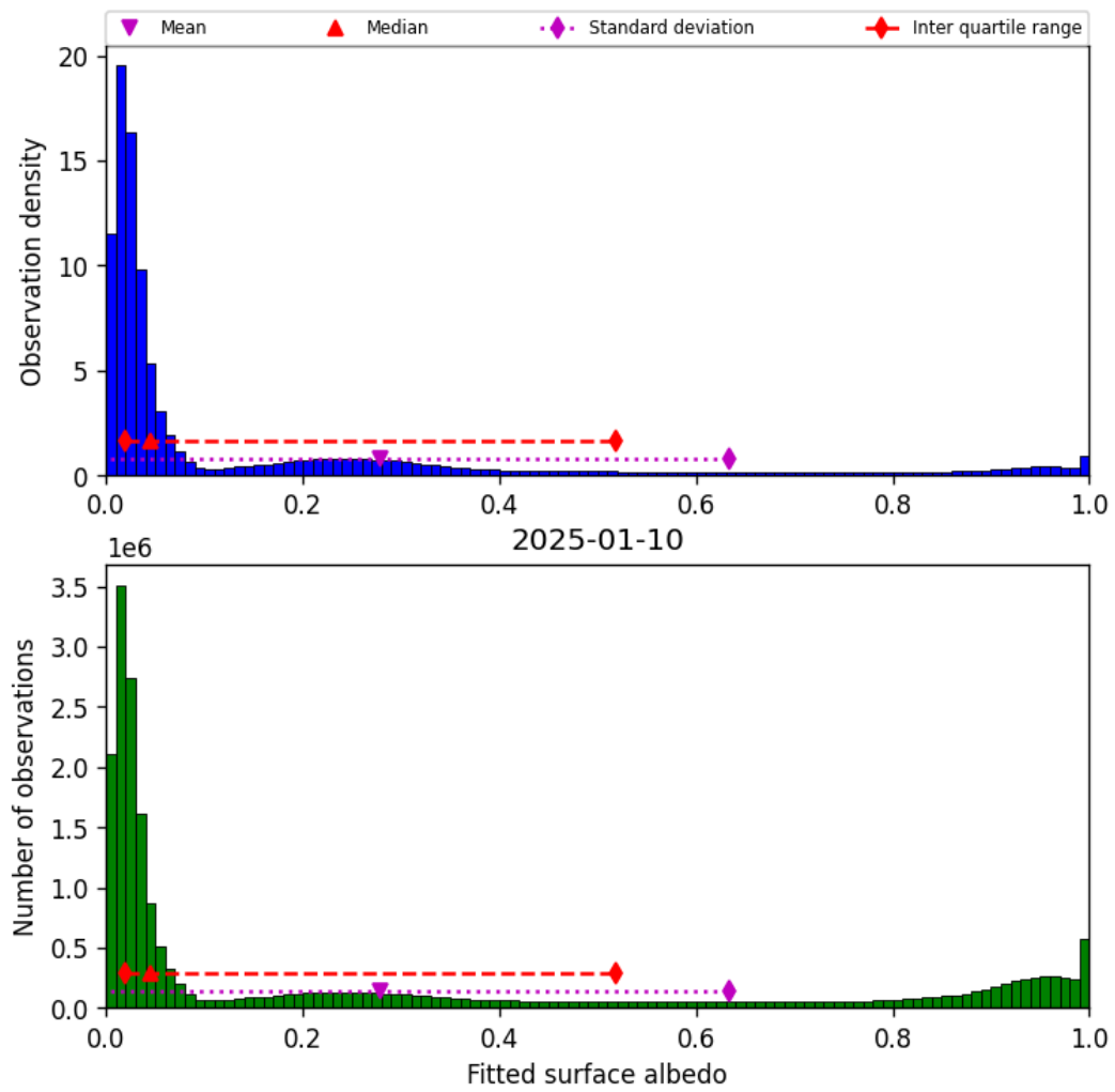
Figure 45: Histogram of “Fitted surface albedo” for 2025-01-09 to 2025-01-11
