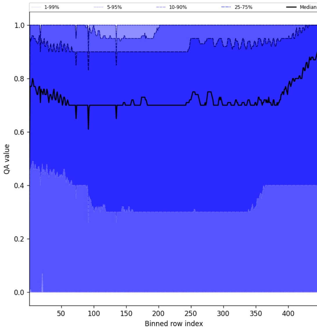
Figure 54: Along track statistics of “QA value” for 2025-01-09 to 2025-01-11
