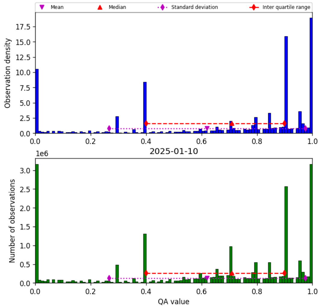
Figure 38: Histogram of “QA value” for 2025-01-09 to 2025-01-11
