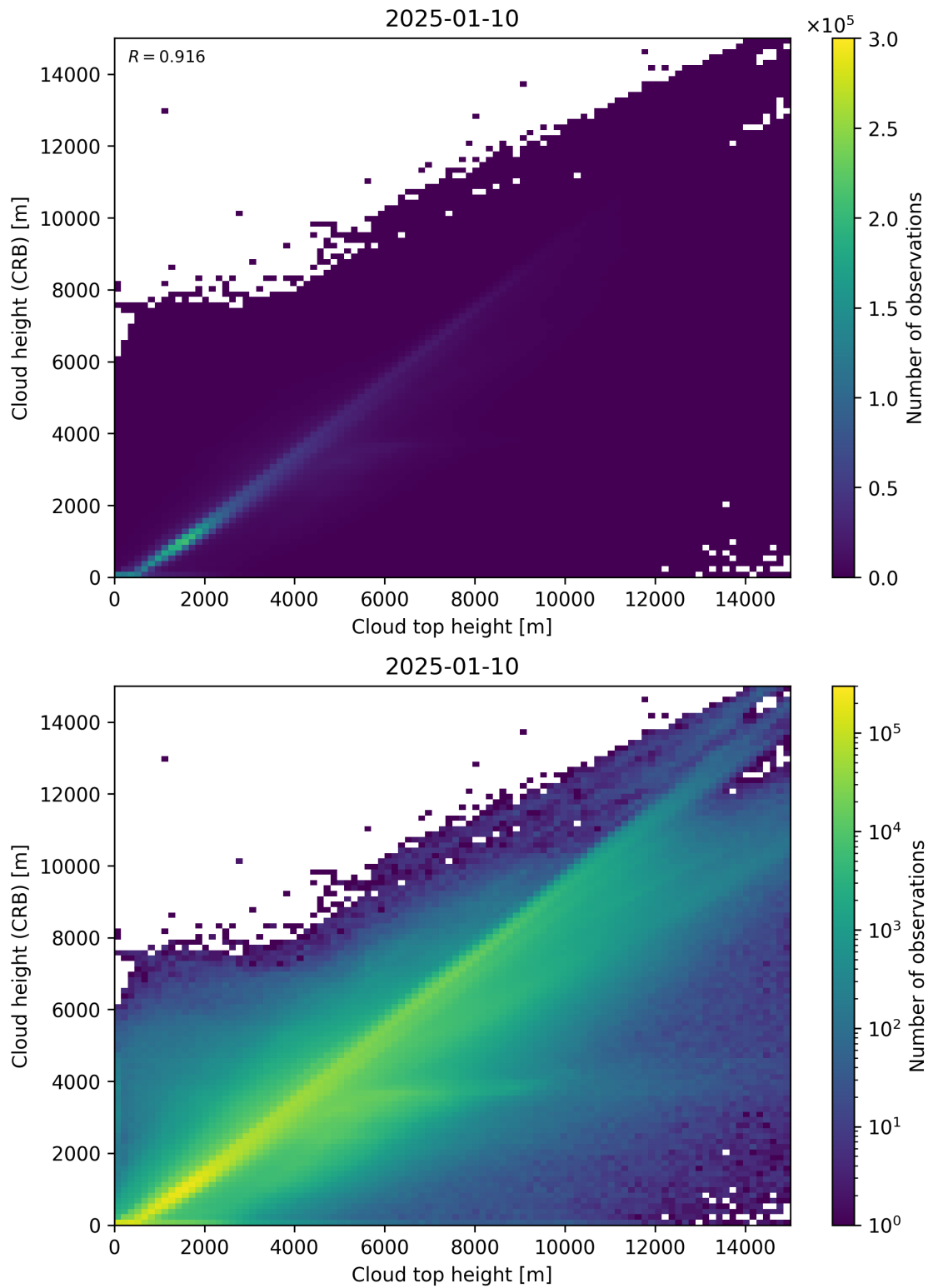
Figure 89: Scatter density plot of “Cloud top height” against “Cloud height (CRB)” for 2025-01-09 to 2025-01-11.
