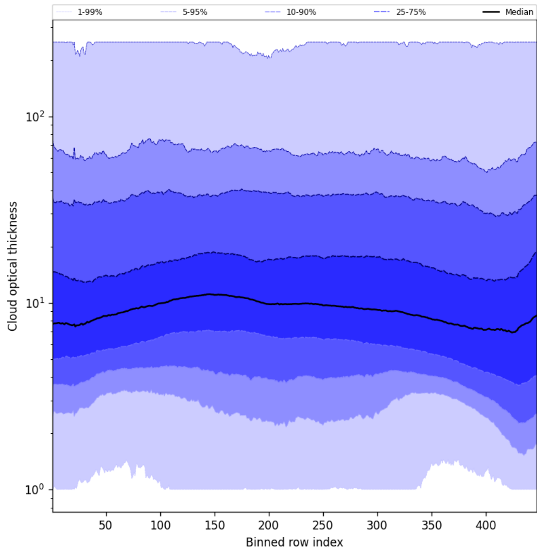
Figure 57: Along track statistics of “Cloud optical thickness” for 2025-01-09 to 2025-01-11
