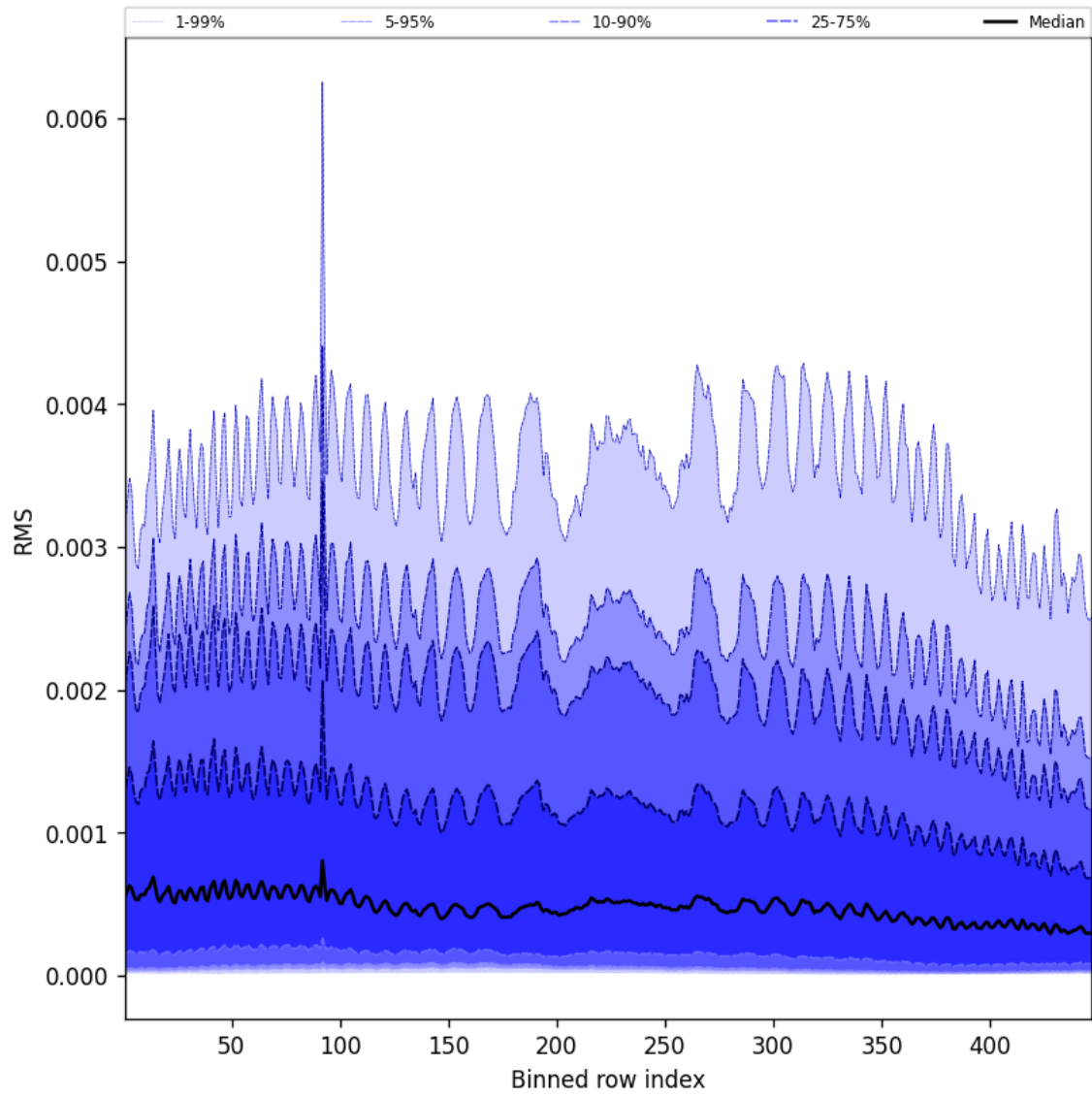
Figure 63: Along track statistics of “RMS” for 2025-01-09 to 2025-01-11
