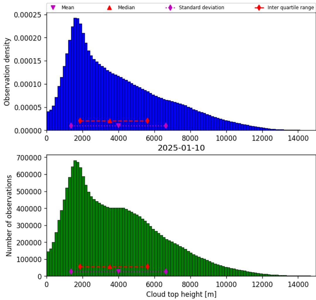
Figure 40: Histogram of “Cloud top height” for 2025-01-09 to 2025-01-11
