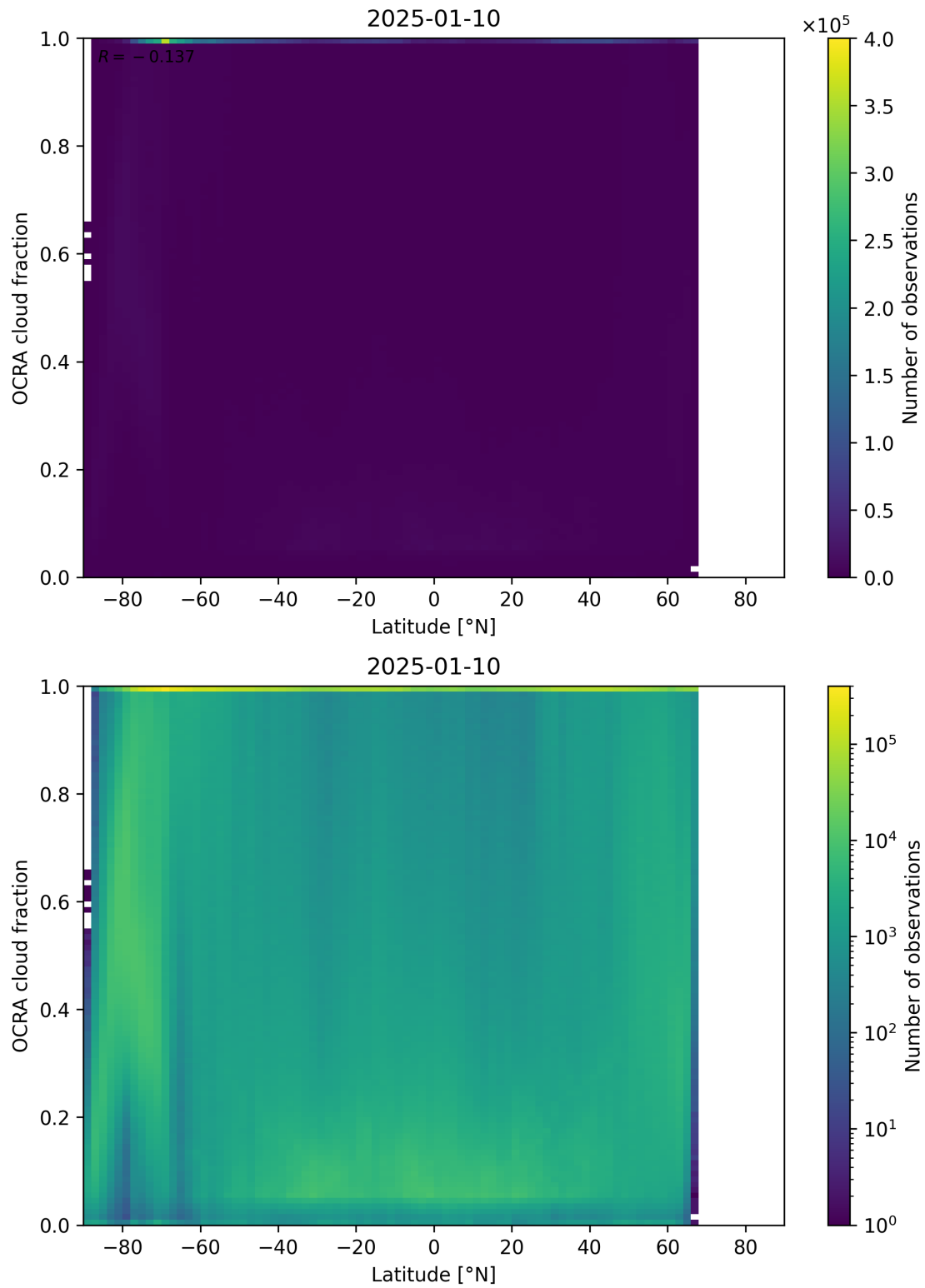
Figure 93: Scatter density plot of “Latitude” against “OCRA cloud fraction” for 2025-01-09 to 2025-01-11.
