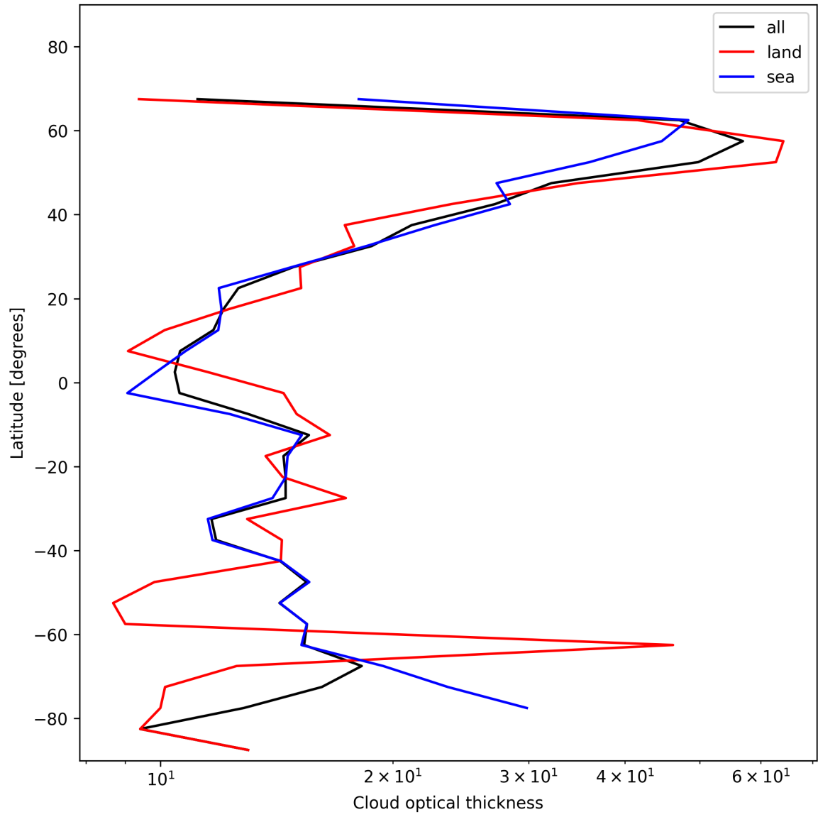
Figure 25: Zonal average of “Cloud optical thickness” for 2025-01-09 to 2025-01-11.
