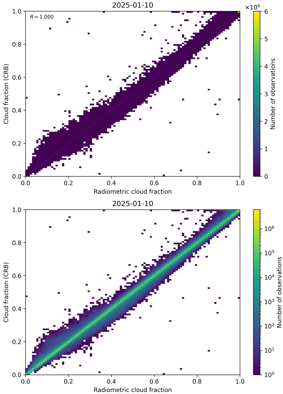
Figure 73: Scatter density plot of “Radiometric cloud fraction” against “Cloud fraction (CRB)” for 2025-01-09 to 2025-01-11.
