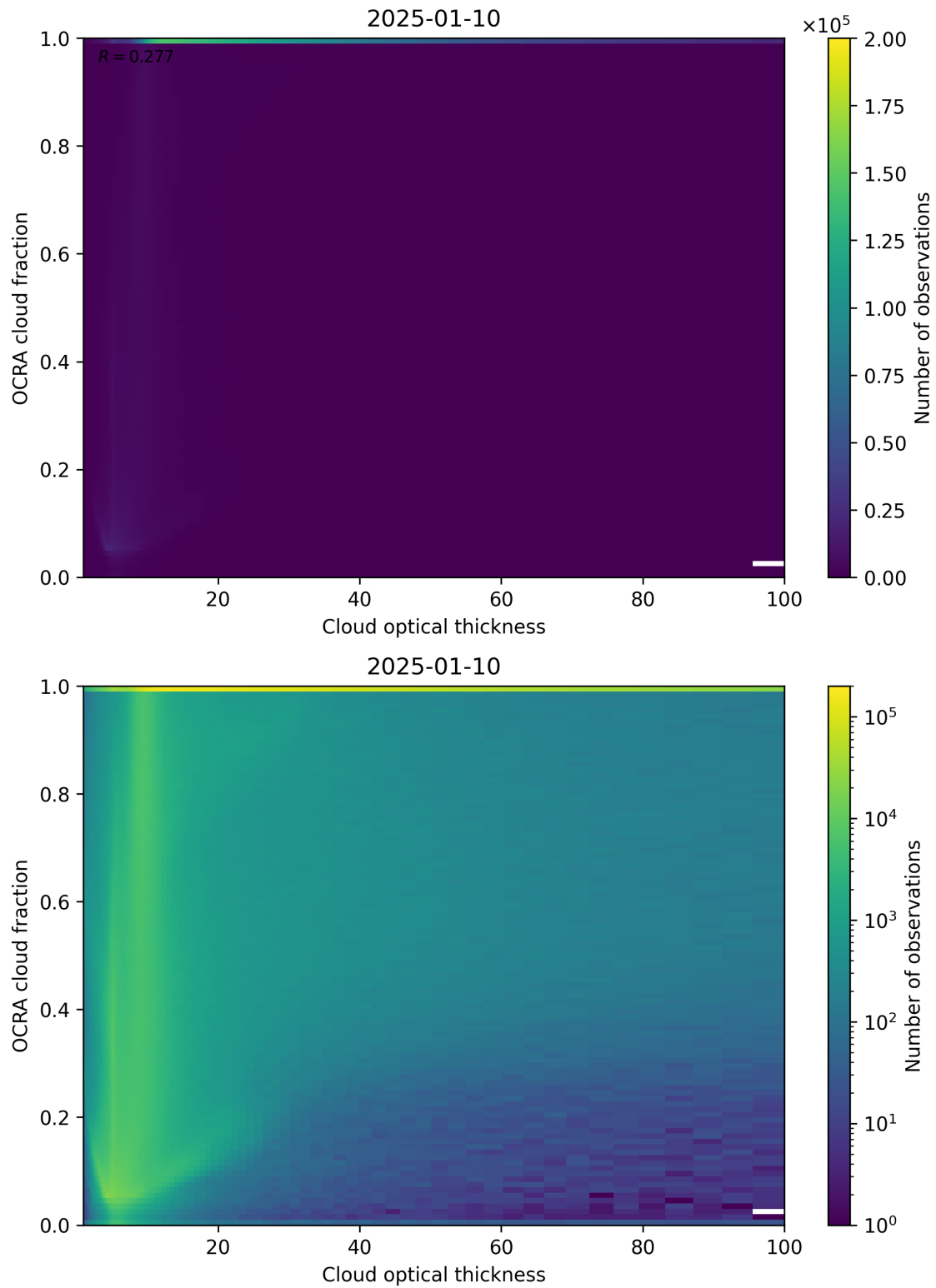
Figure 83: Scatter density plot of “Cloud optical thickness” against “OCRA cloud fraction” for 2025-01-09 to 2025-01-11.
