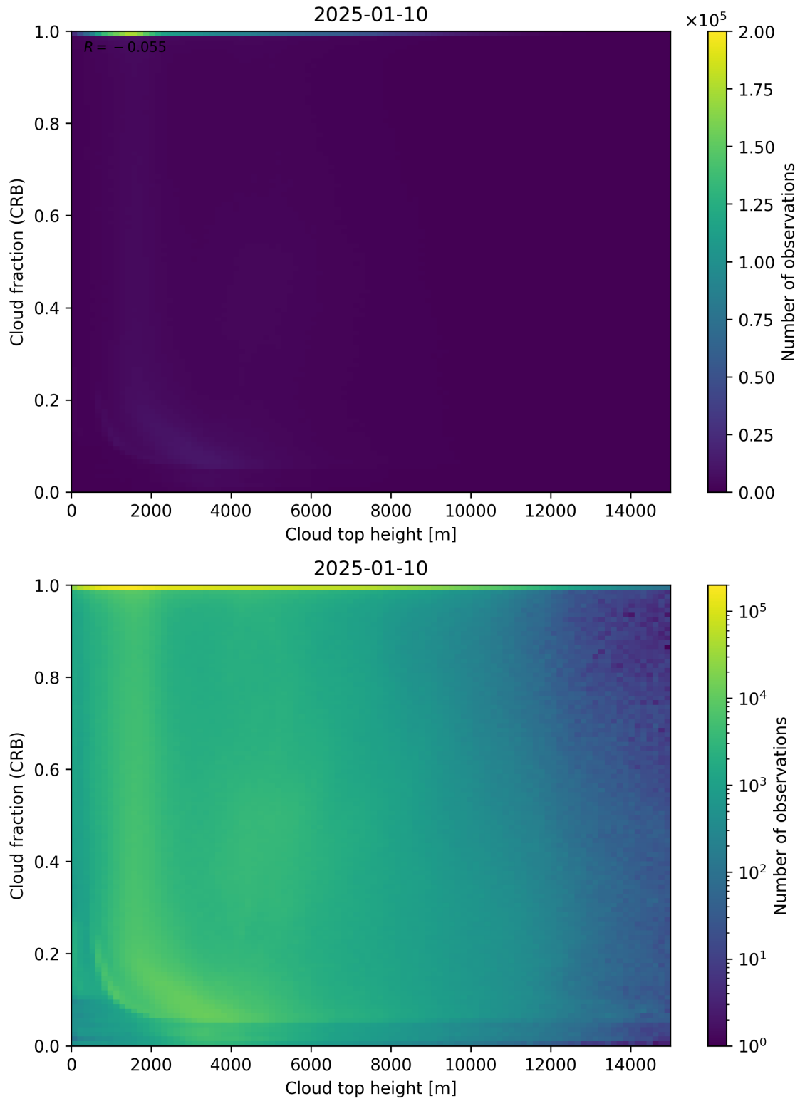
Figure 88: Scatter density plot of “Cloud top height” against “Cloud fraction (CRB)” for 2025-01-09 to 2025-01-11.
