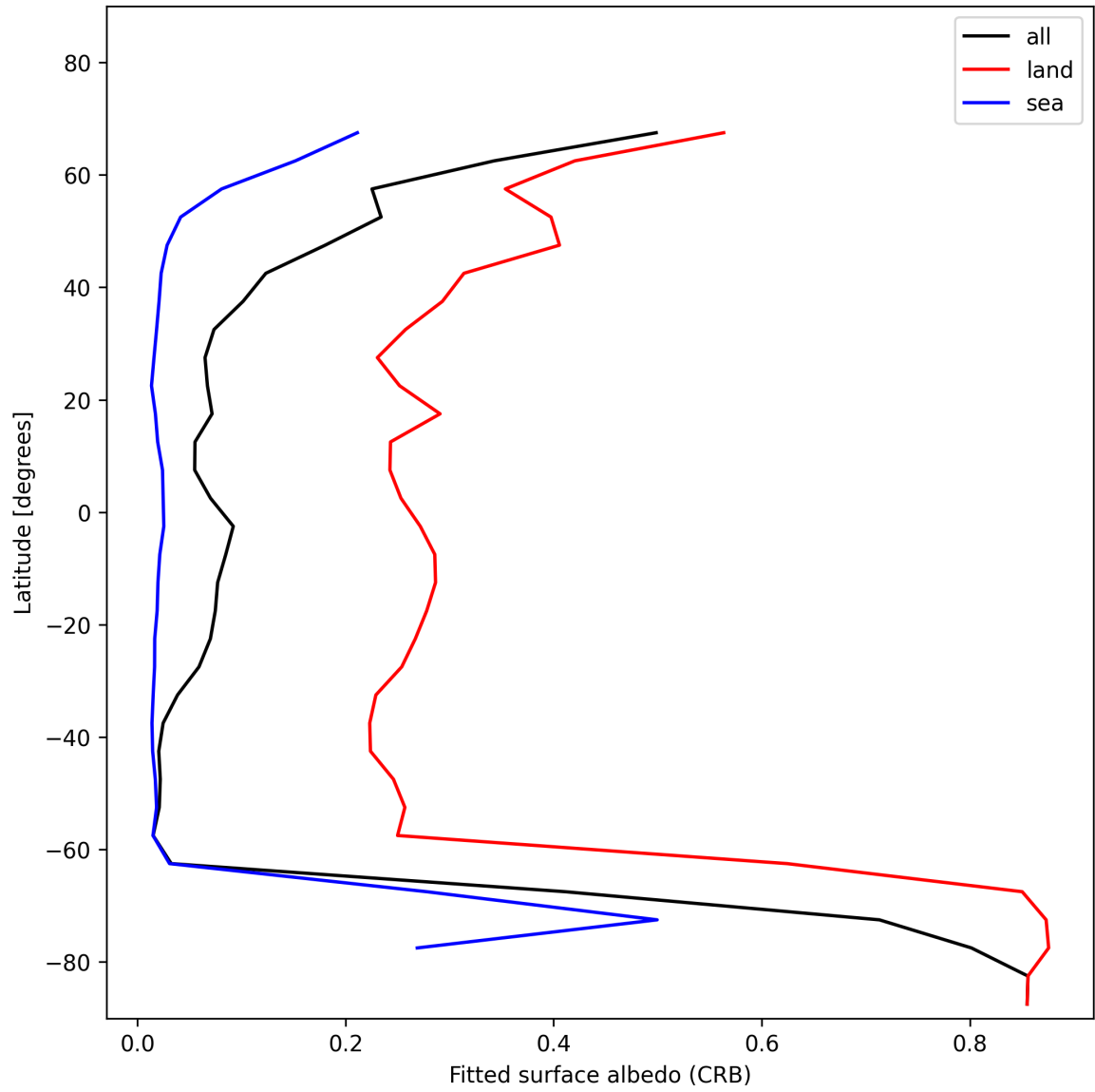
Figure 30: Zonal average of “Fitted surface albedo (CRB)” for 2025-01-09 to 2025-01-11.
