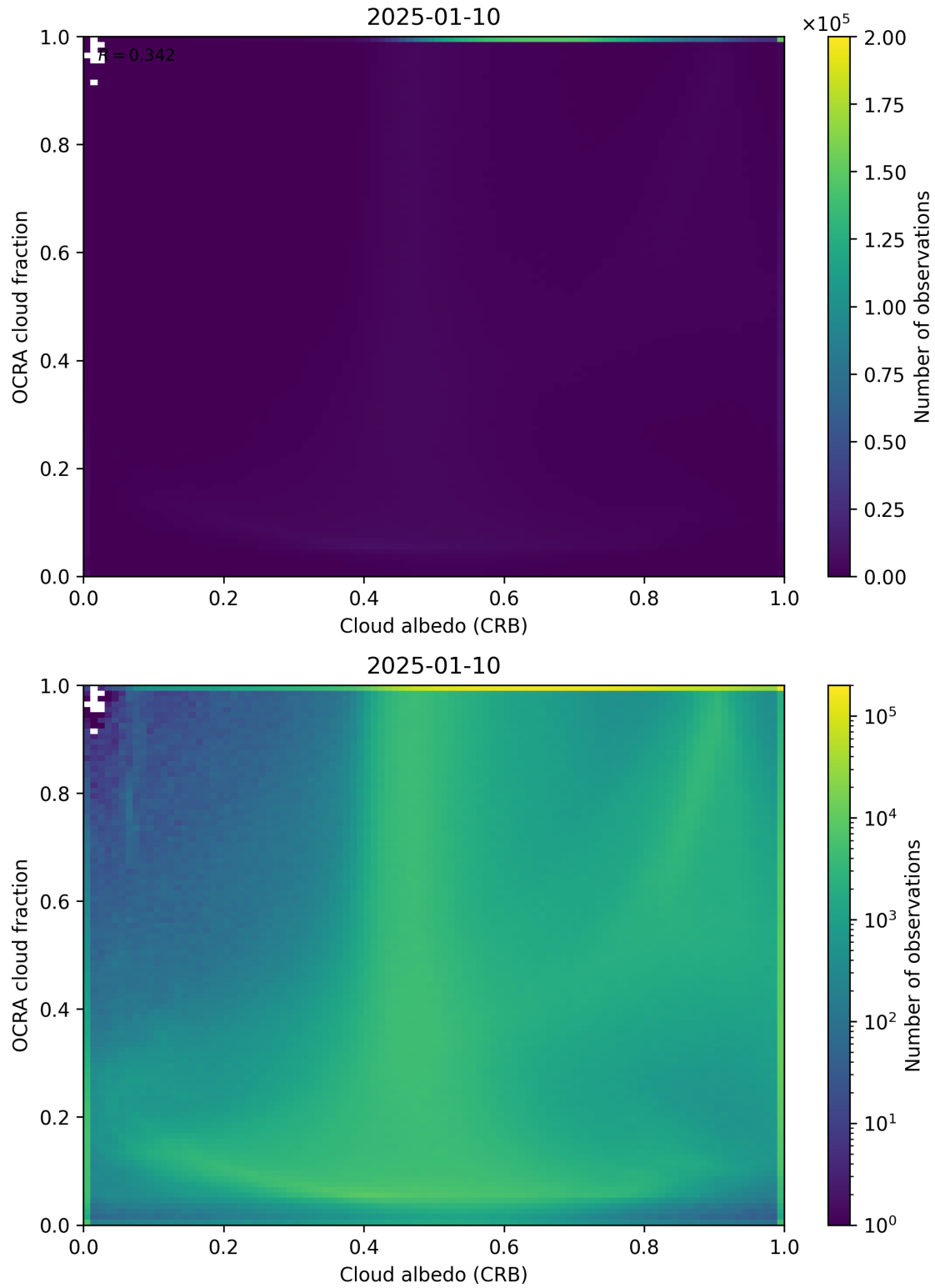
Figure 70: Scatter density plot of “Cloud albedo (CRB)” against “OCRA cloud fraction” for 2025-01-09 to 2025-01-11.
