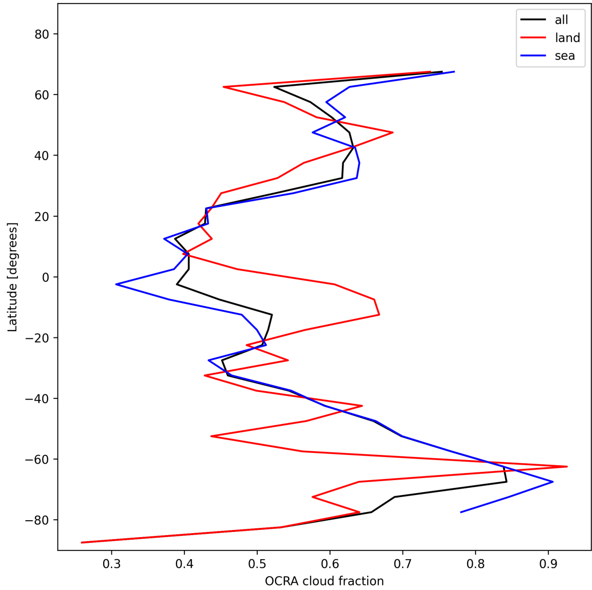
Figure 34: Zonal average of “OCRA cloud fraction” for 2025-01-09 to 2025-01-11.
