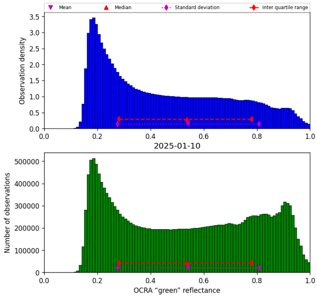
Figure 52: Histogram of “OCRA “green” reflectance” for 2025-01-09 to 2025-01-11
