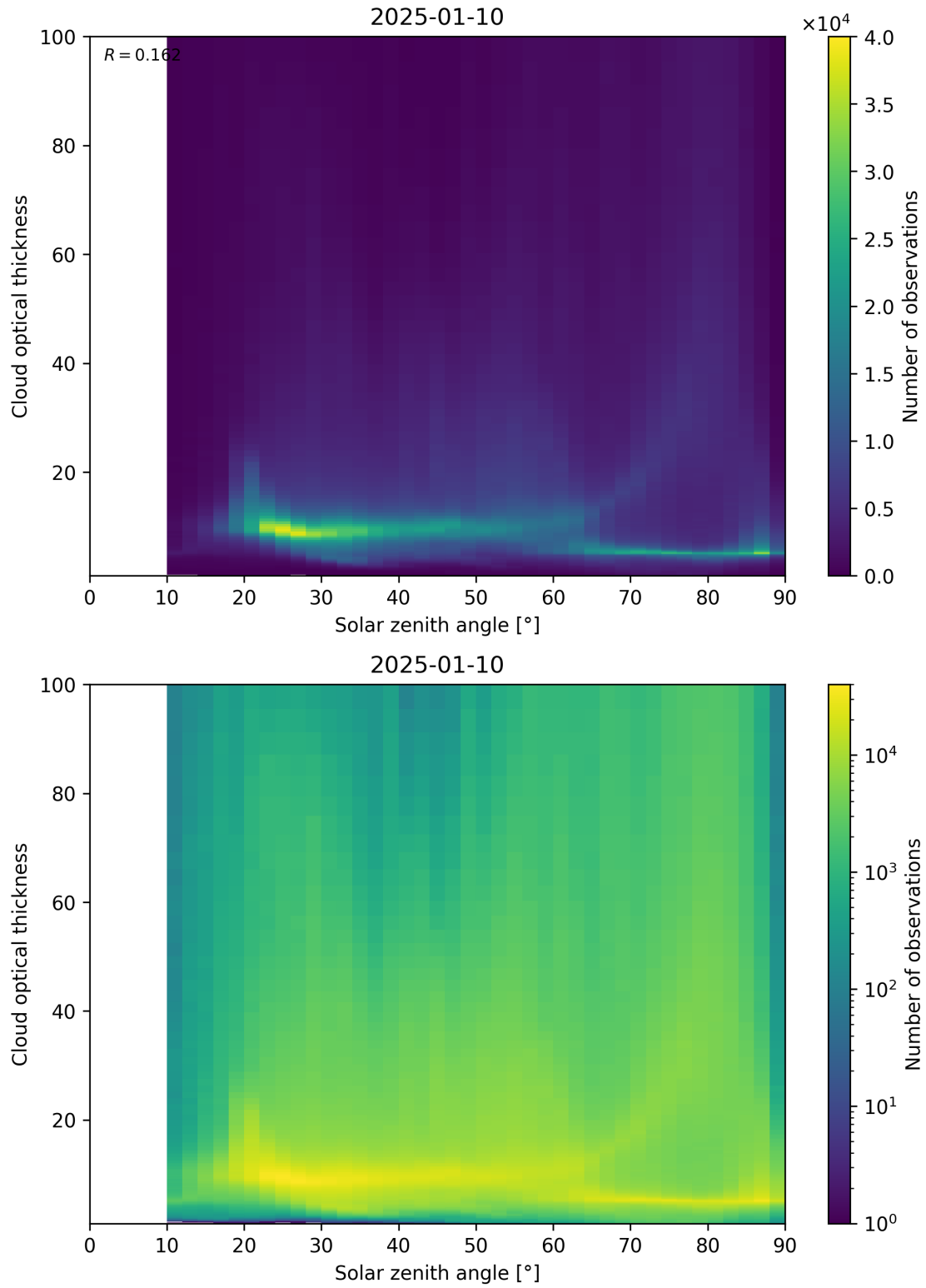
Figure 103: Scatter density plot of “Solar zenith angle” against “Cloud optical thickness” for 2025-01-09 to 2025-01-11.
