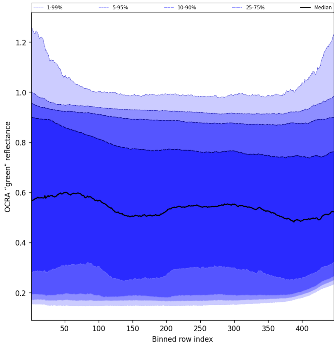
Figure 68: Along track statistics of "OCRA "green" reflectance" for 2025-01-09 to 2025-01-11
