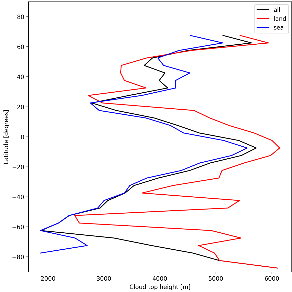
Figure 24: Zonal average of “Cloud top height” for 2025-01-09 to 2025-01-11.
