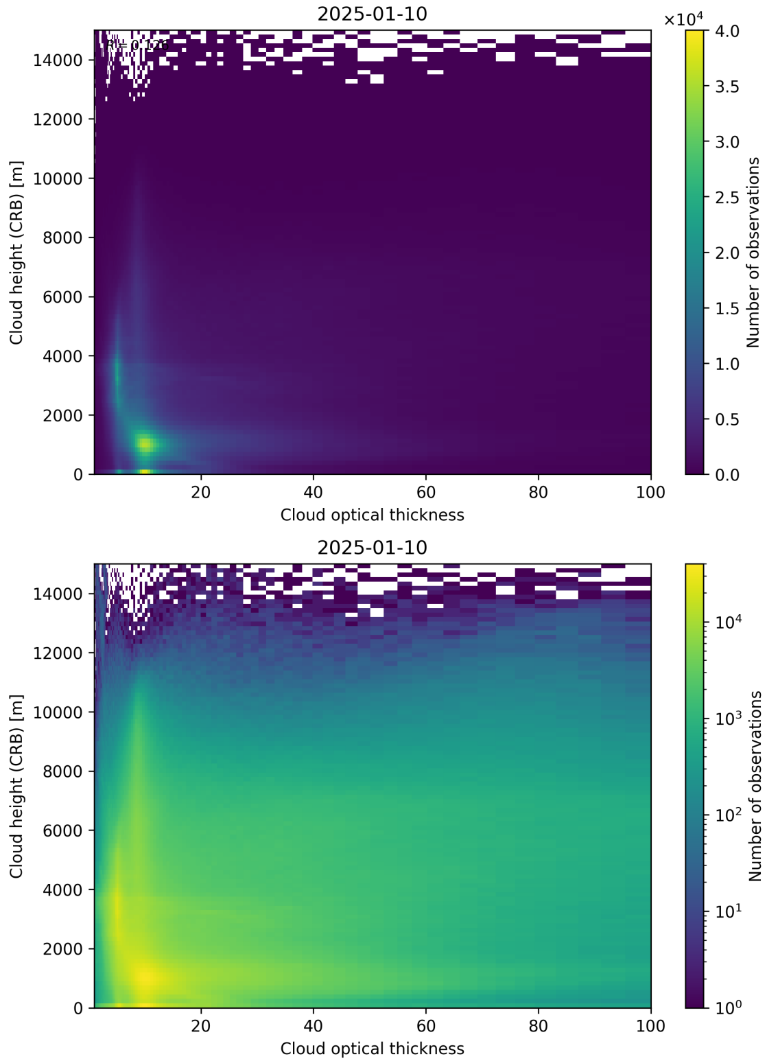
Figure 85: Scatter density plot of “Cloud optical thickness” against “Cloud height (CRB)” for 2025-01-09 to 2025-01-11.
