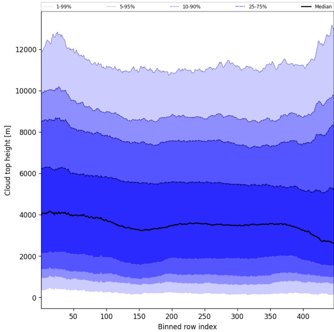
Figure 56: Along track statistics of “Cloud top height” for 2025-01-09 to 2025-01-11
