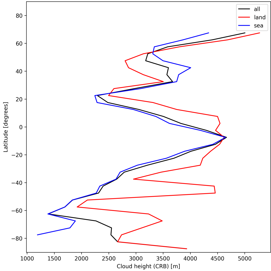
Figure 27: Zonal average of “Cloud height (CRB)” for 2025-01-09 to 2025-01-11.
