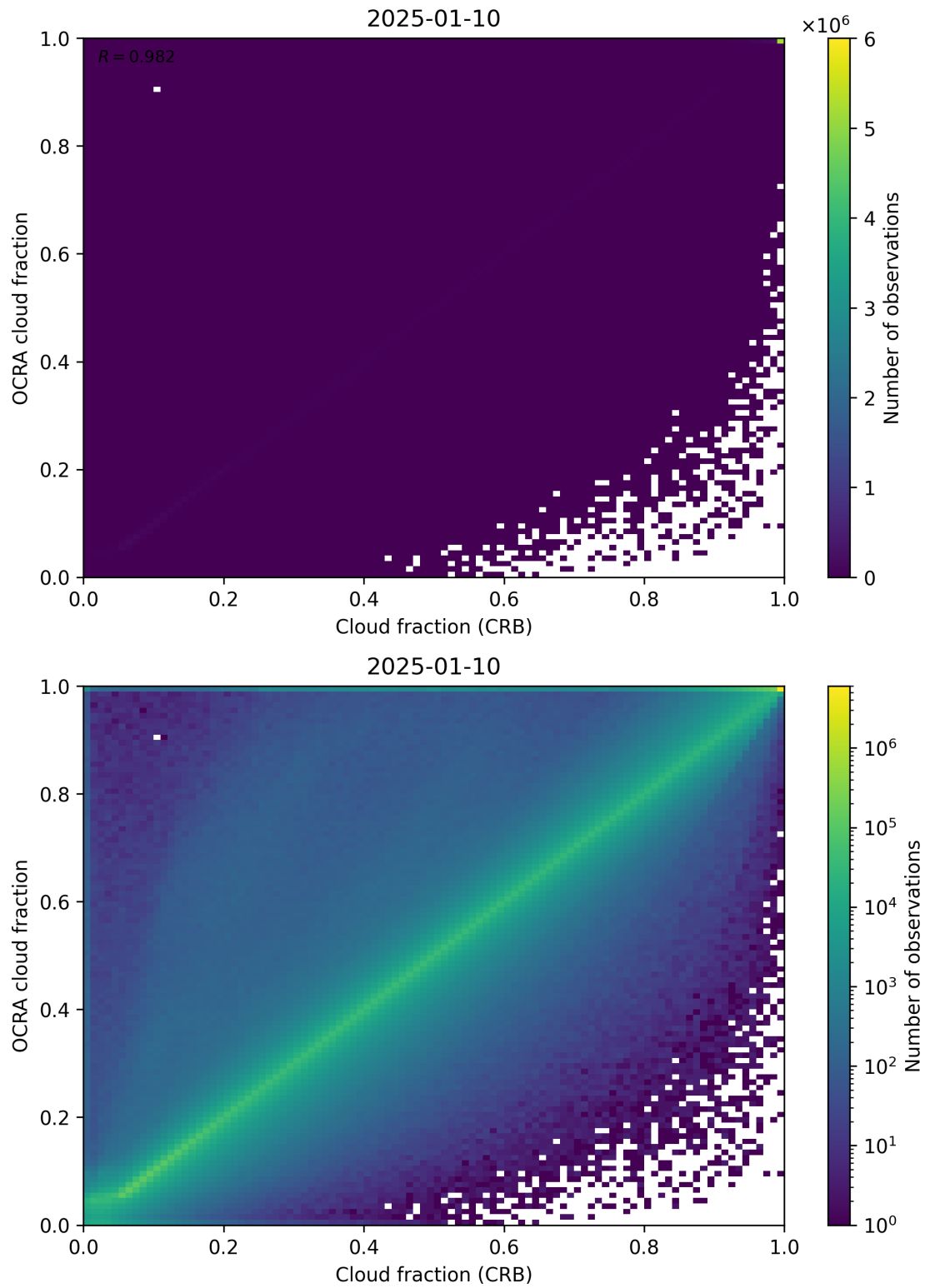
Figure 78: Scatter density plot of “Cloud fraction (CRB)” against “OCRA cloud fraction” for 2025-01-09 to 2025-01-11.
