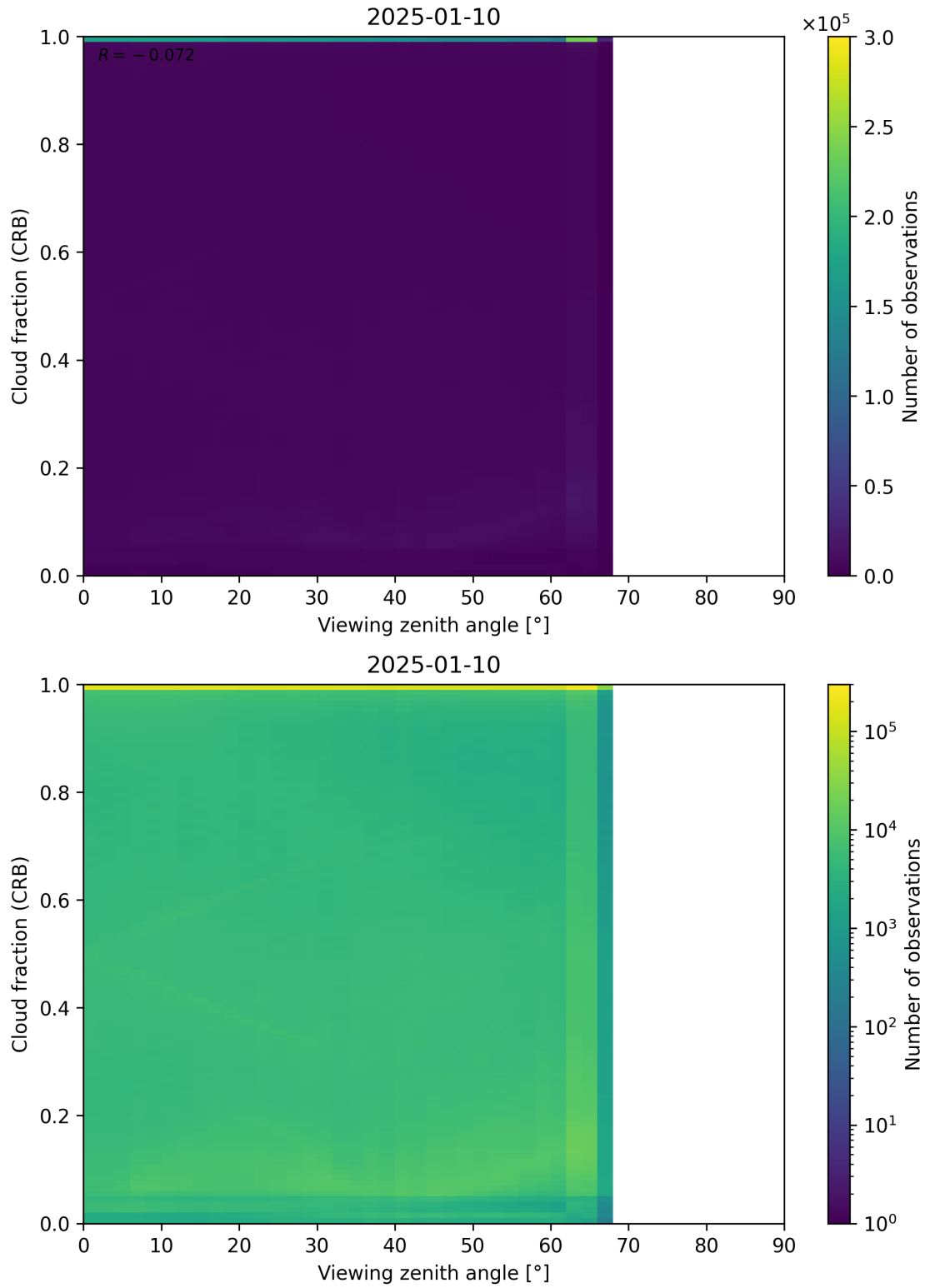
Figure 109: Scatter density plot of “Viewing zenith angle” against “Cloud fraction (CRB)” for 2025-01-09 to 2025-01-11.
