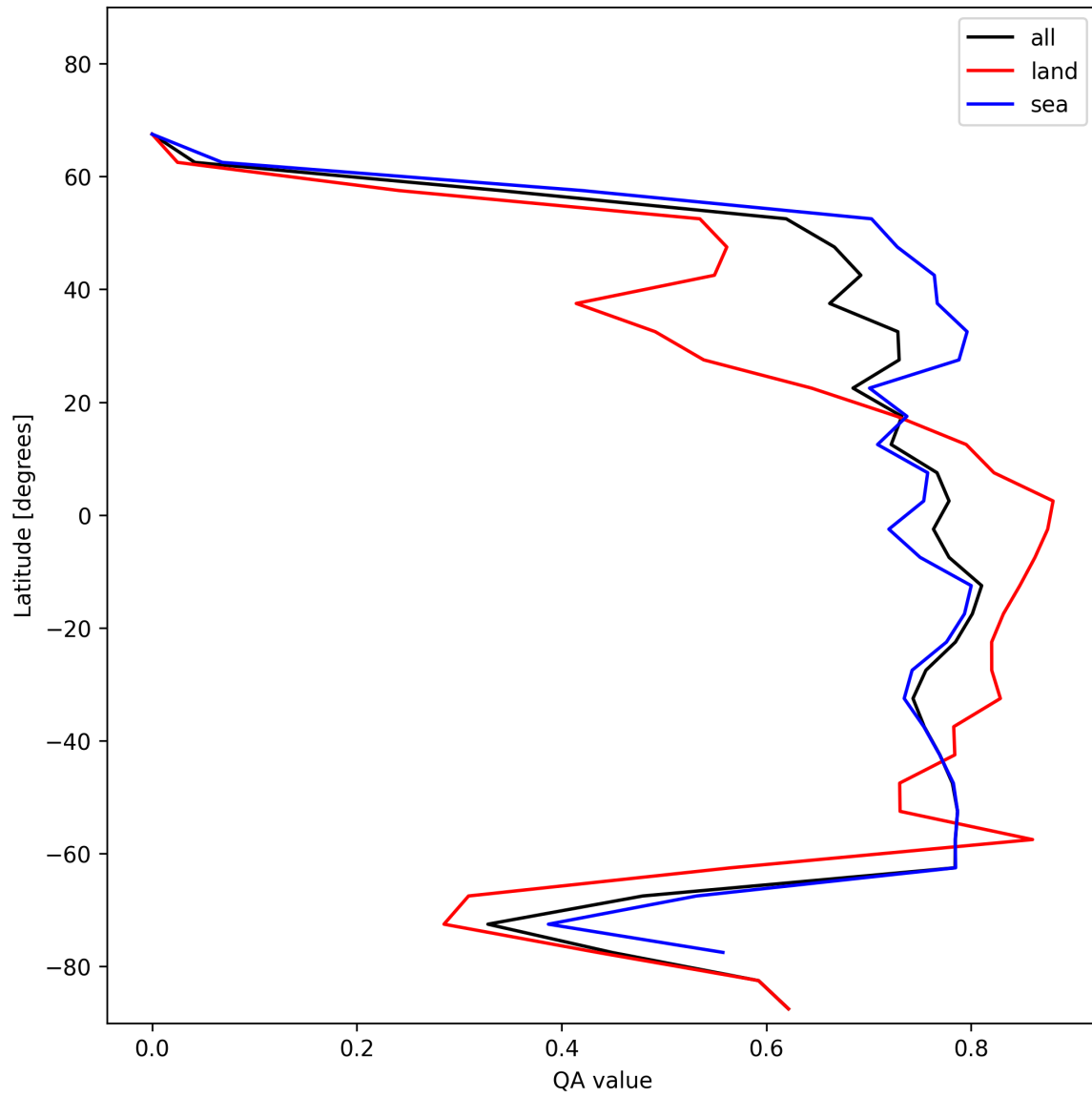
Figure 22: Zonal average of “QA value” for 2025-01-09 to 2025-01-11.
