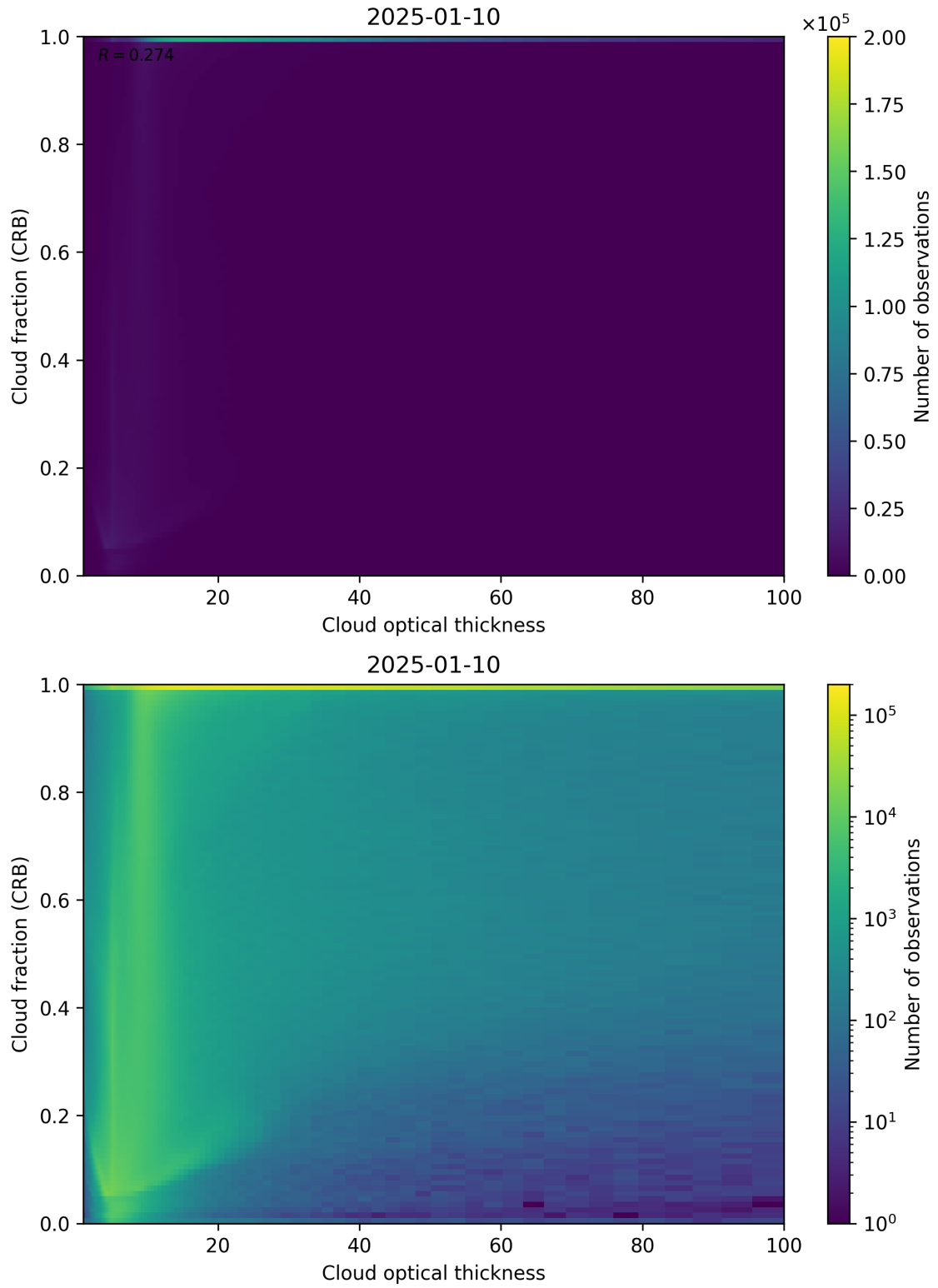
Figure 84: Scatter density plot of “Cloud optical thickness” against “Cloud fraction (CRB)” for 2025-01-09 to 2025-01-11.
