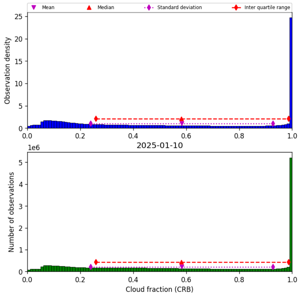
Figure 42: Histogram of “Cloud fraction (CRB)” for 2025-01-09 to 2025-01-11
