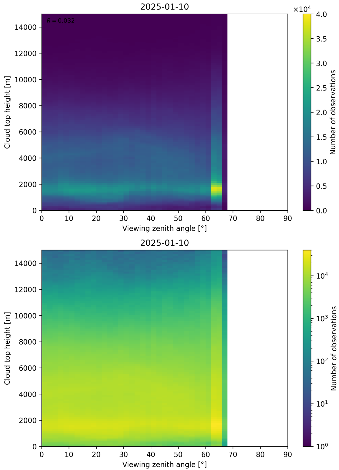
Figure 112: Scatter density plot of “Viewing zenith angle” against “Cloud top height” for 2025-01-09 to 2025-01-11.
