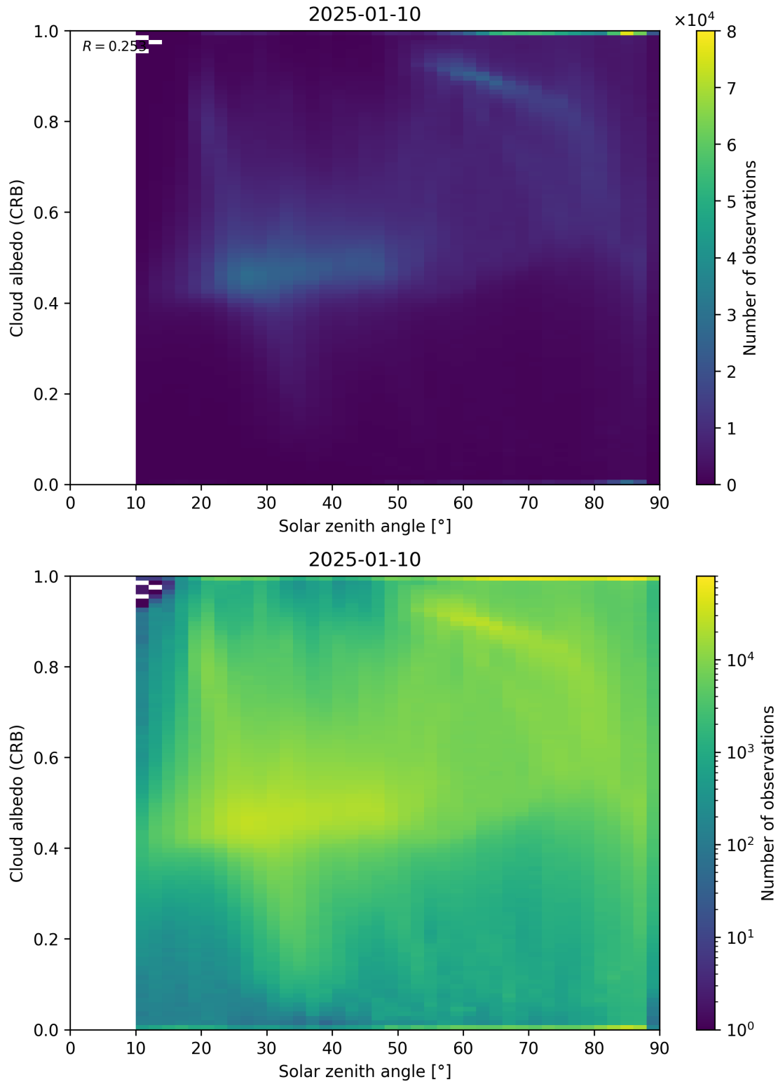
Figure 98: Scatter density plot of “Solar zenith angle” against “Cloud albedo (CRB)” for 2025-01-09 to 2025-01-11.
