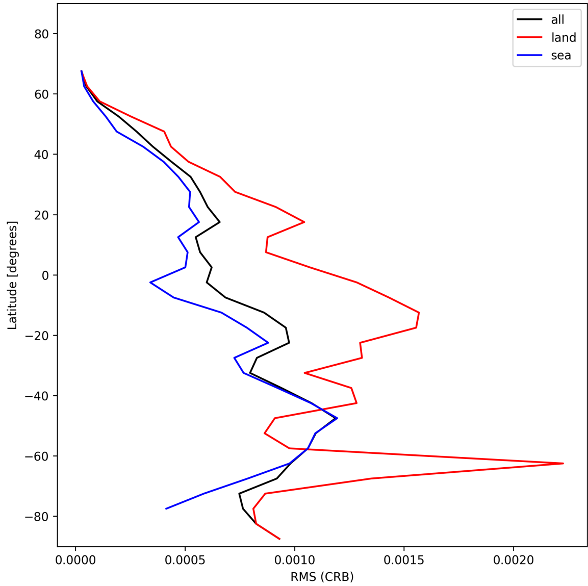
Figure 32: Zonal average of “RMS (CRB)” for 2025-01-09 to 2025-01-11.
