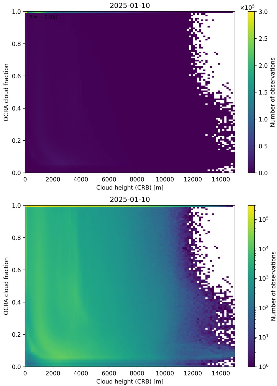
Figure 81: Scatter density plot of “Cloud height (CRB)” against “OCRA cloud fraction” for 2025-01-09 to 2025-01-11.
