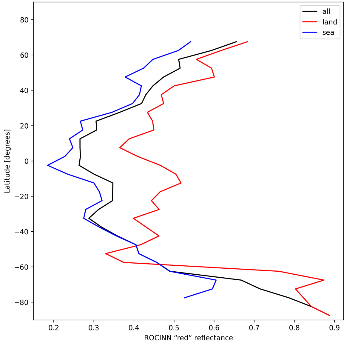
Figure 37: Zonal average of “ROCINN “red” reflectance” for 2025-01-09 to 2025-01-11.
