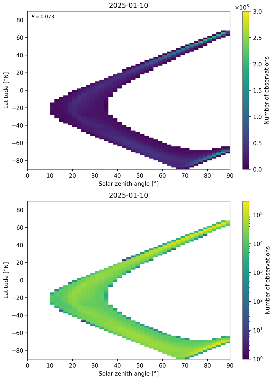
Figure 105: Scatter density plot of “Solar zenith angle” against “Latitude” for 2025-01-09 to 2025-01-11.
