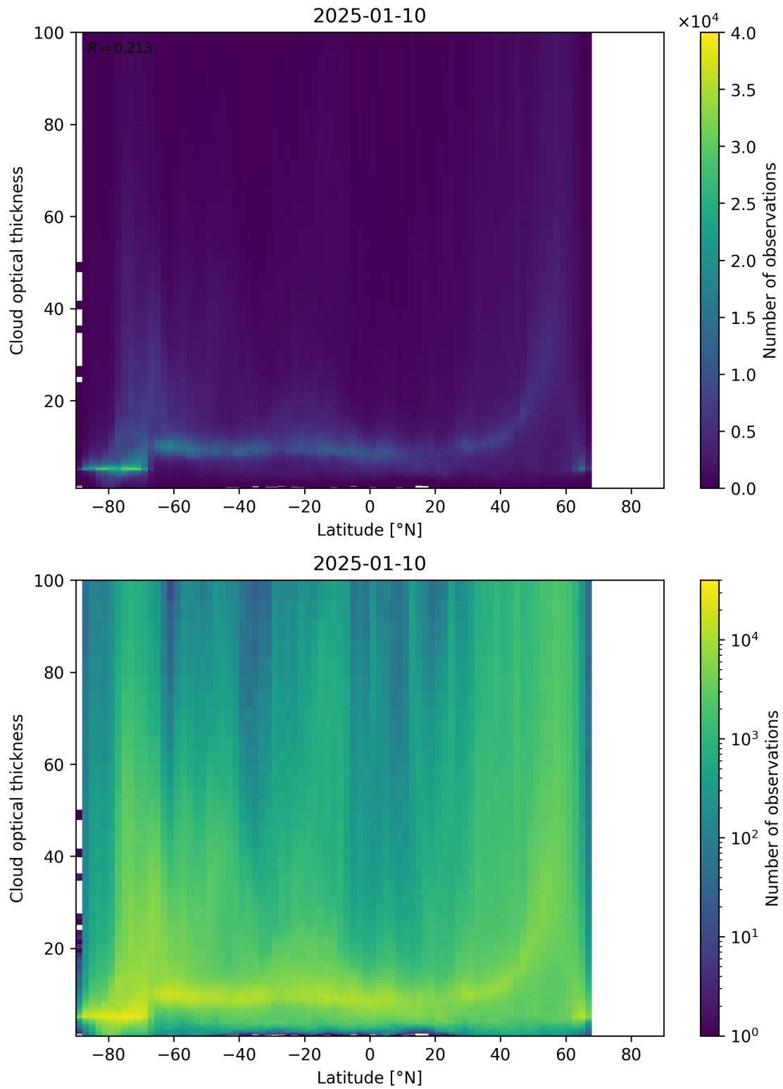
Figure 96: Scatter density plot of “Latitude” against “Cloud optical thickness” for 2025-01-09 to 2025-01-11.
