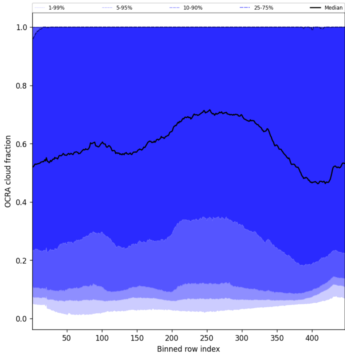
Figure 66: Along track statistics of “OCRA cloud fraction” for 2025-01-09 to 2025-01-11
