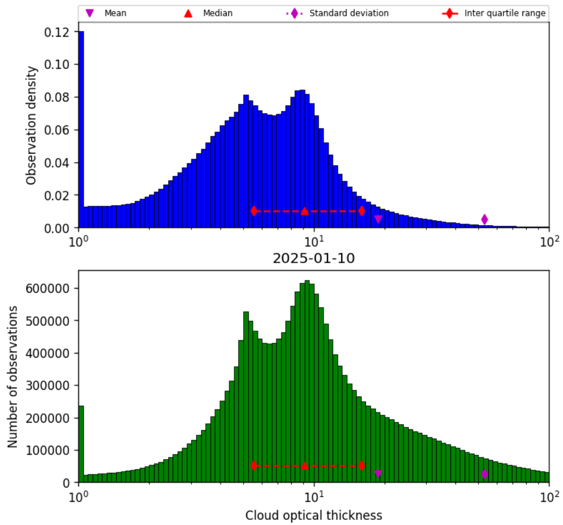
Figure 41: Histogram of “Cloud optical thickness” for 2025-01-09 to 2025-01-11
