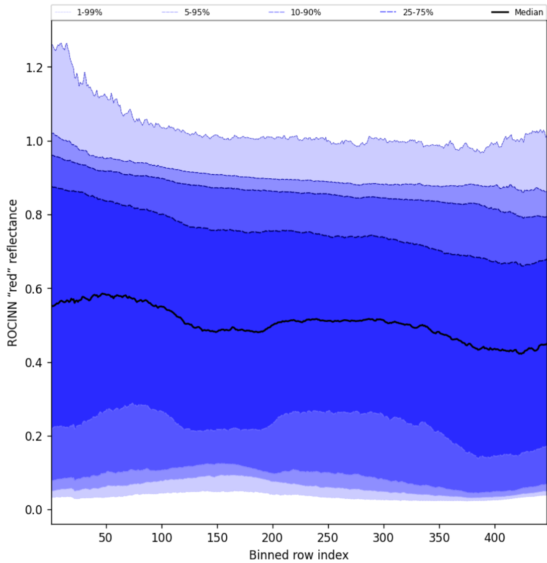
Figure 69: Along track statistics of "ROCINN "red" reflectance" for 2025-01-09 to 2025-01-11
