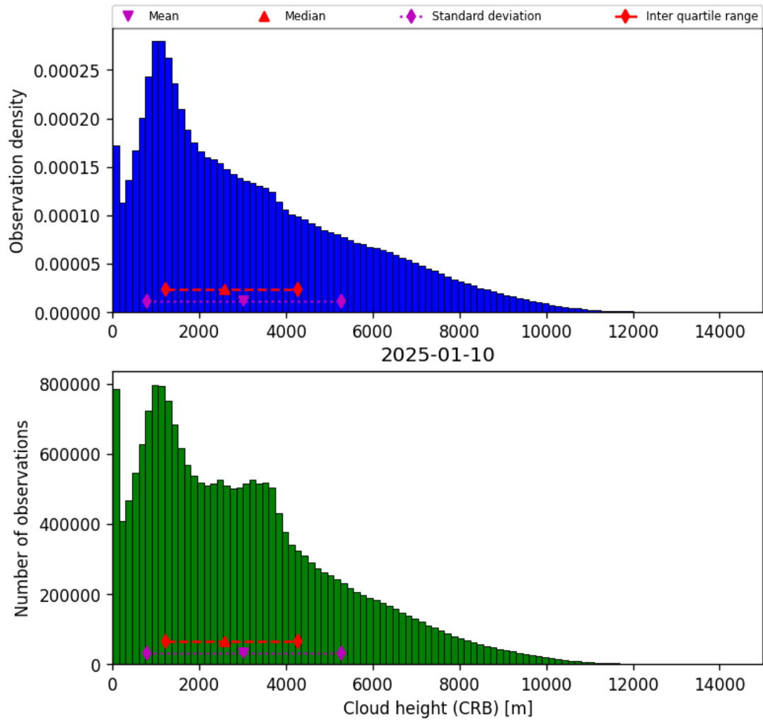
Figure 43: Histogram of “Cloud height (CRB)” for 2025-01-09 to 2025-01-11
