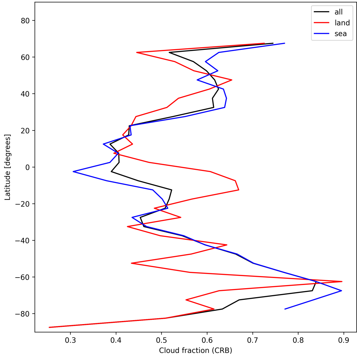
Figure 26: Zonal average of “Cloud fraction (CRB)” for 2025-01-09 to 2025-01-11.
