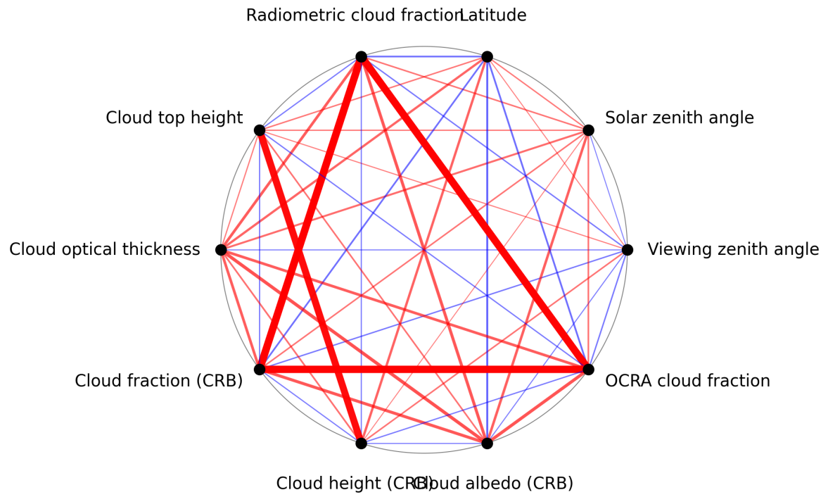
Figure 1: Map of correlation graph for 2025-01-09 to 2025-01-11.
