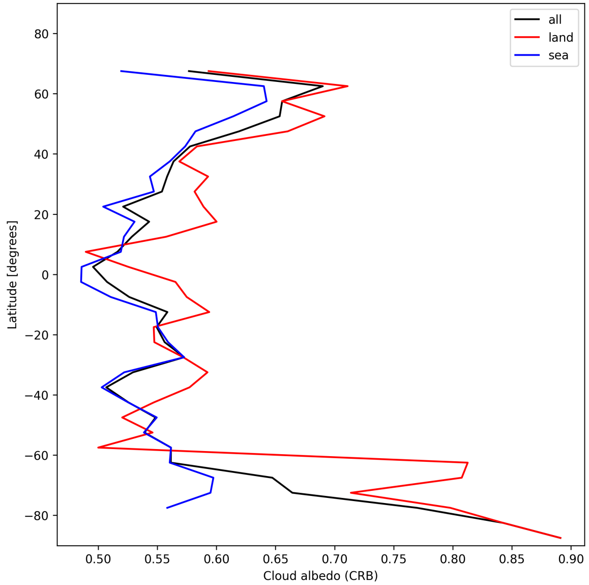
Figure 28: Zonal average of “Cloud albedo (CRB)” for 2025-01-09 to 2025-01-11.
