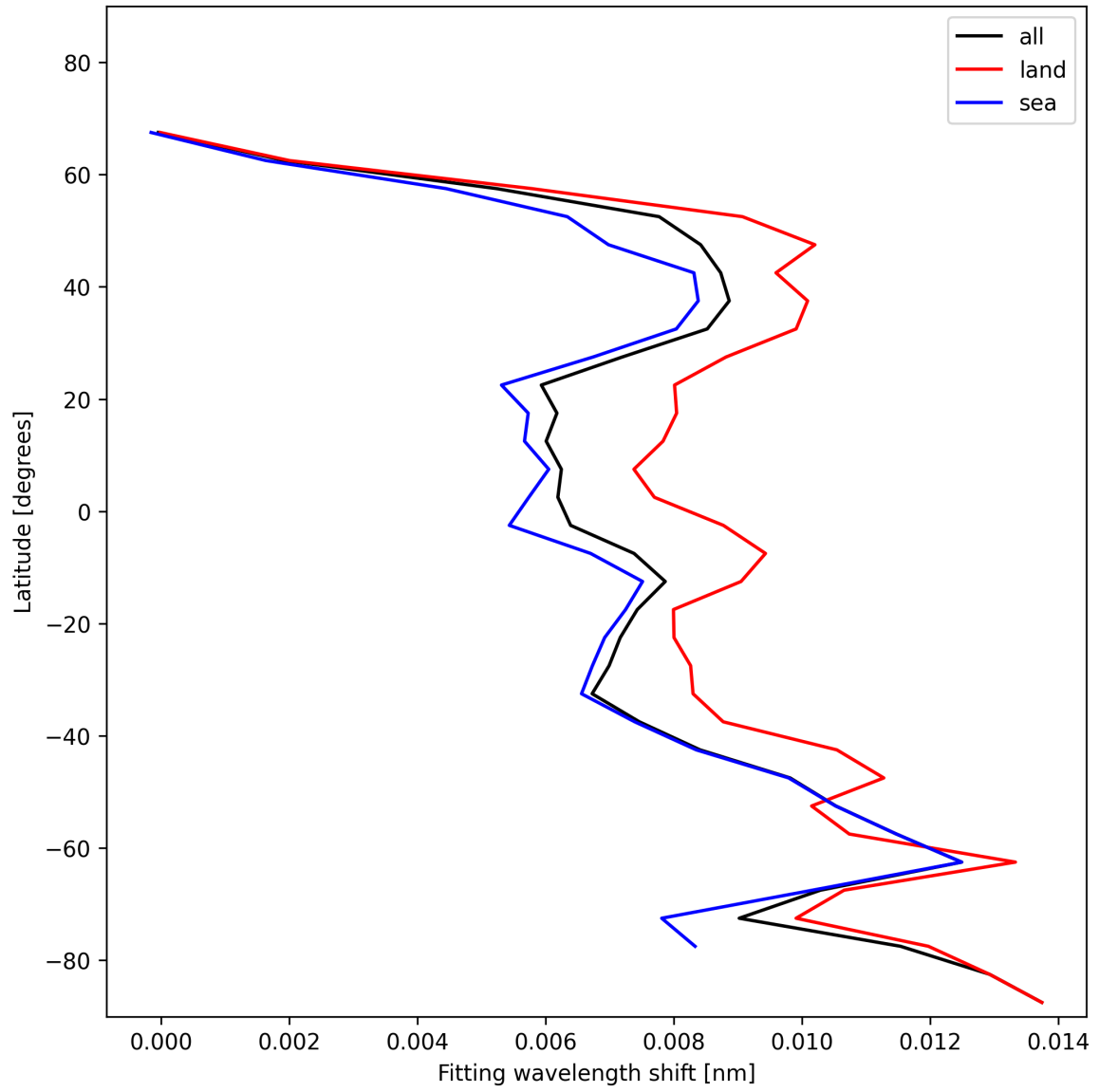
Figure 33: Zonal average of “Fitting wavelength shift” for 2025-01-09 to 2025-01-11.
