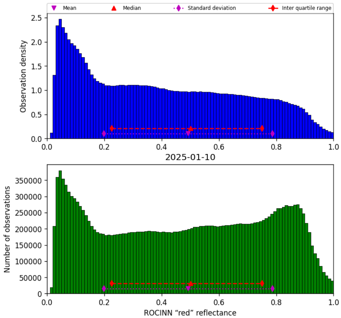
Figure 53: Histogram of “ROCINN “red” reflectance” for 2025-01-09 to 2025-01-11
