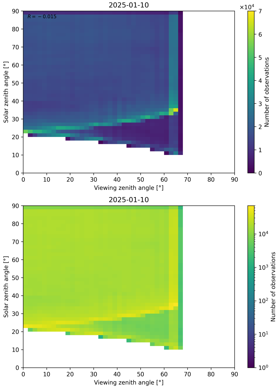
Figure 114: Scatter density plot of “Viewing zenith angle” against “Solar zenith angle” for 2025-01-09 to 2025-01-11.
