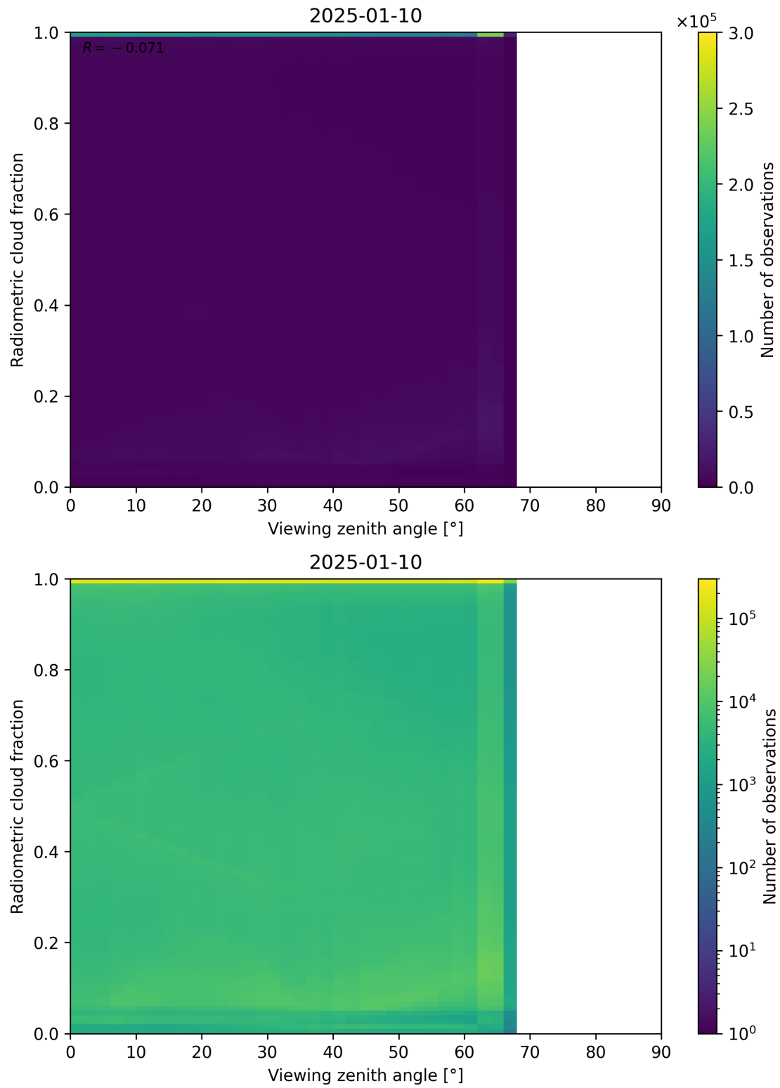
Figure 107: Scatter density plot of “Viewing zenith angle” against “Radiometric cloud fraction” for 2025-01-09 to 2025-01-11.
