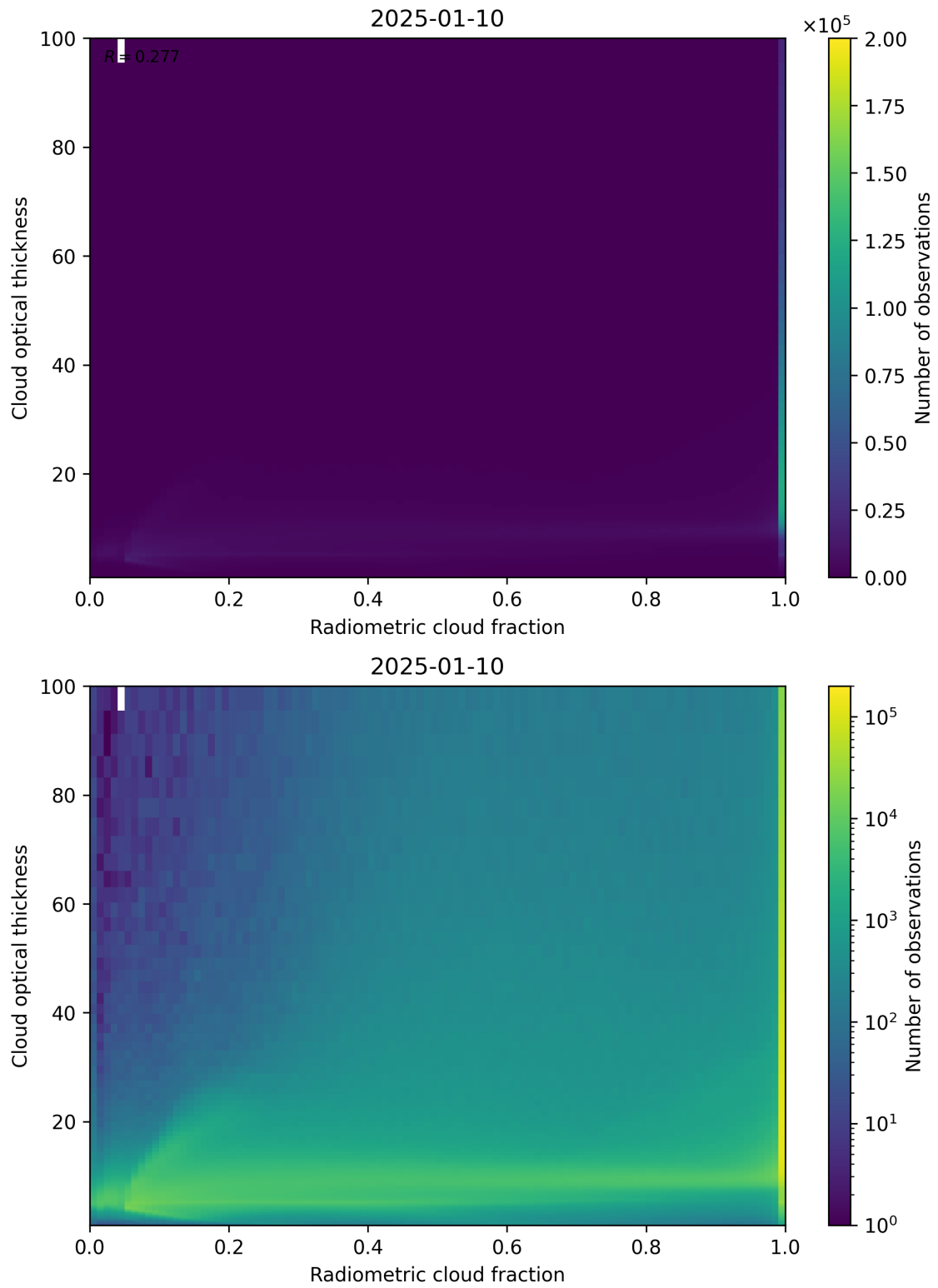
Figure 75: Scatter density plot of “Radiometric cloud fraction” against “Cloud optical thickness” for 2025-01-09 to 2025-01-11.
