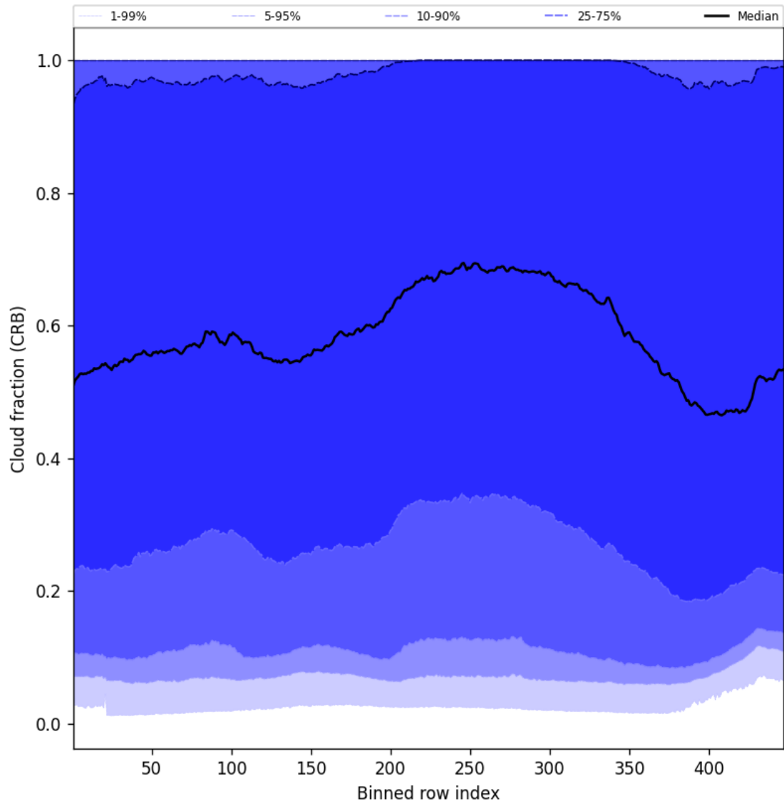
Figure 58: Along track statistics of “Cloud fraction (CRB)” for 2025-01-09 to 2025-01-11
