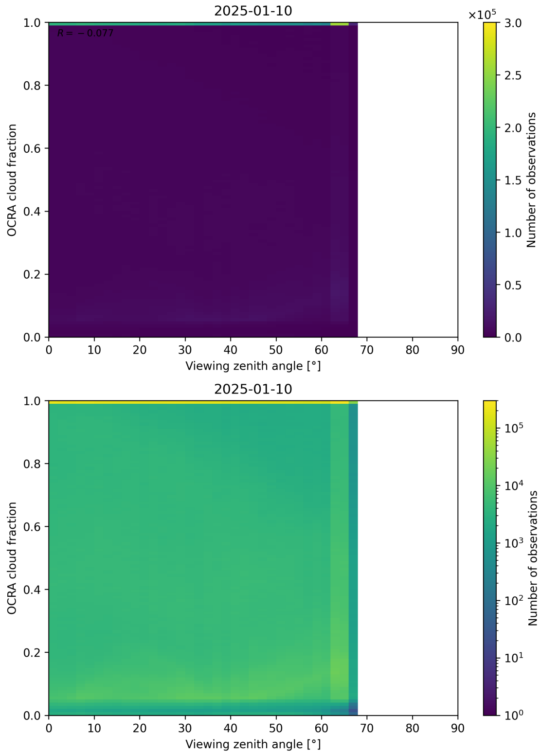
Figure 108: Scatter density plot of “Viewing zenith angle” against “OCRA cloud fraction” for 2025-01-09 to 2025-01-11.
