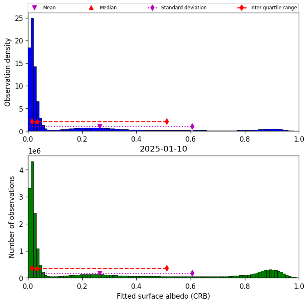
Figure 46: Histogram of “Fitted surface albedo (CRB)” for 2025-01-09 to 2025-01-11
