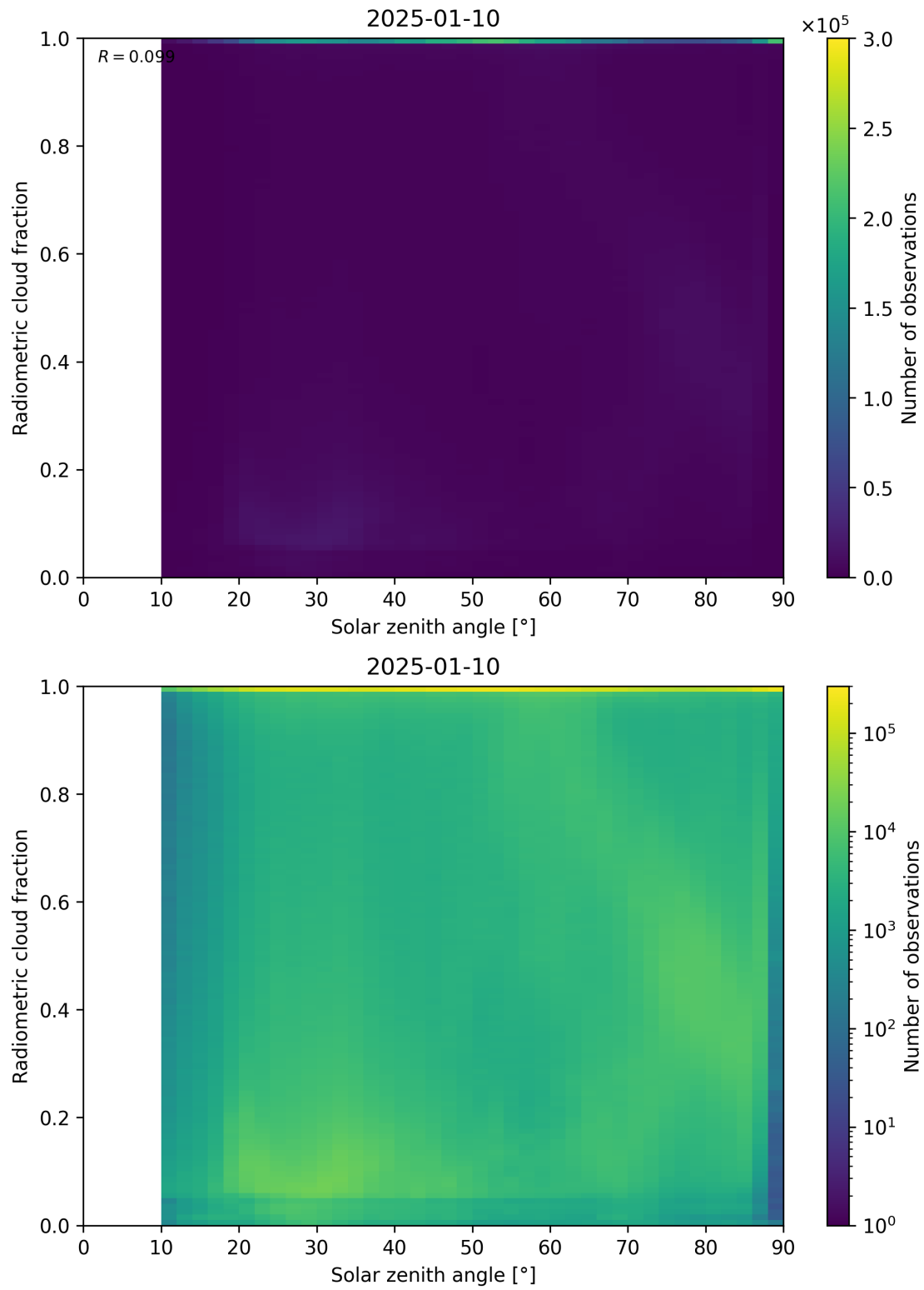
Figure 99: Scatter density plot of “Solar zenith angle” against “Radiometric cloud fraction” for 2025-01-09 to 2025-01-11.
