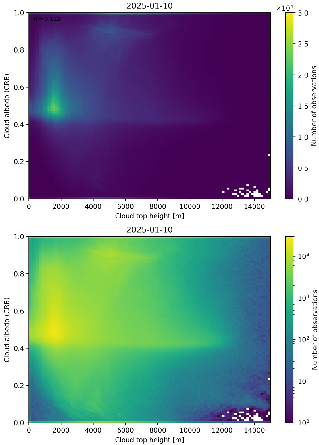
Figure 86: Scatter density plot of “Cloud top height” against “Cloud albedo (CRB)” for 2025-01-09 to 2025-01-11.
