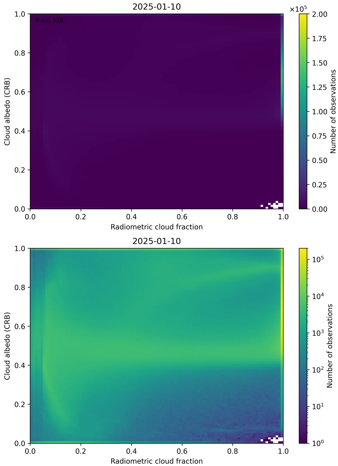
Figure 71: Scatter density plot of “Radiometric cloud fraction” against “Cloud albedo (CRB)” for 2025-01-09 to 2025-01-11.
