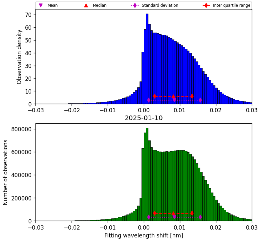
Figure 49: Histogram of “Fitting wavelength shift” for 2025-01-09 to 2025-01-11
