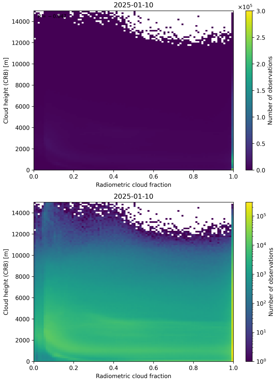
Figure 74: Scatter density plot of “Radiometric cloud fraction” against “Cloud height (CRB)” for 2025-01-09 to 2025-01-11.
