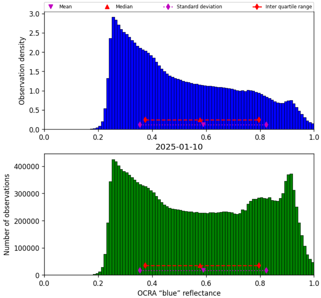
Figure 51: Histogram of “OCRA “blue” reflectance” for 2025-01-09 to 2025-01-11
