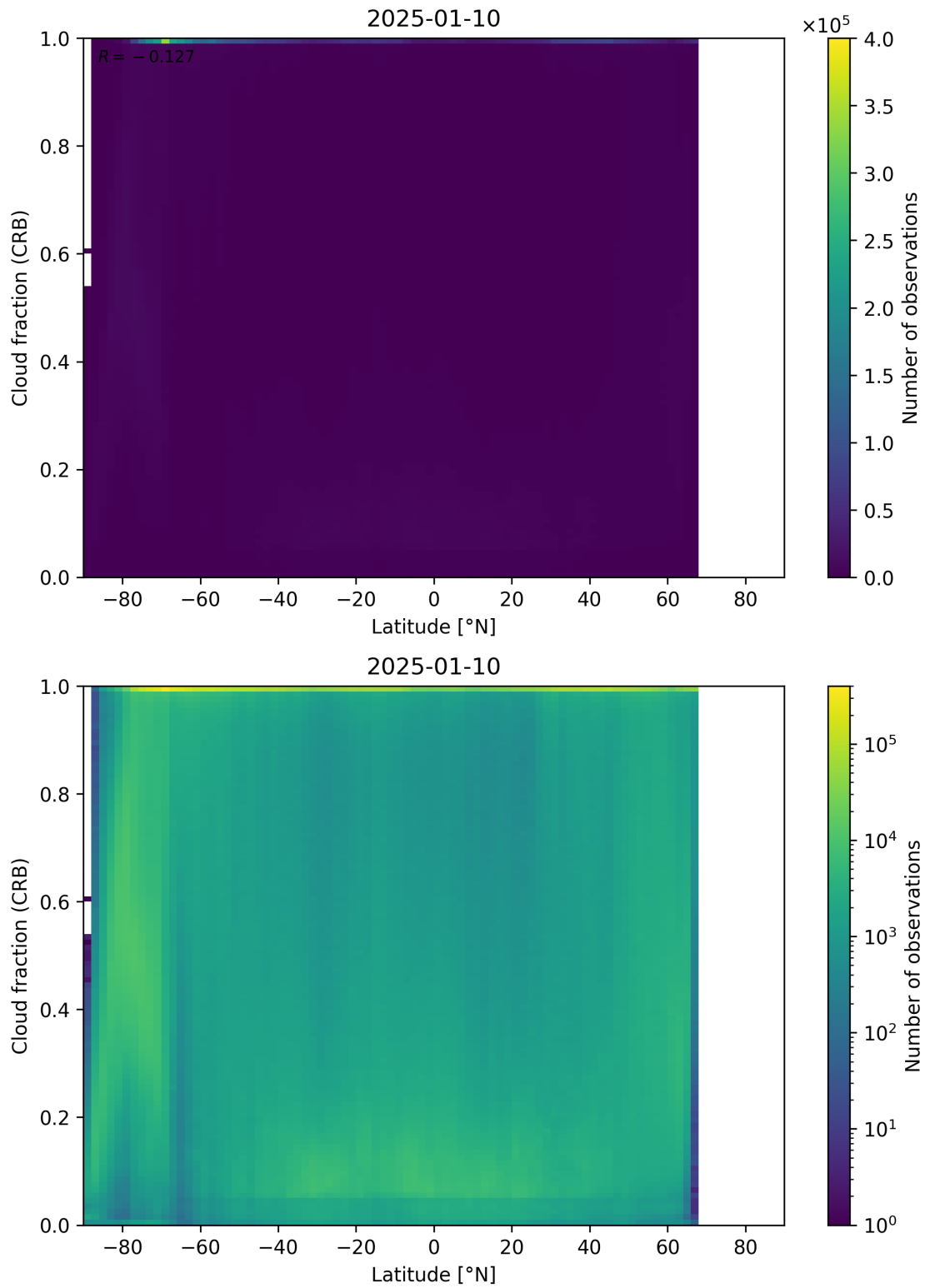
Figure 94: Scatter density plot of “Latitude” against “Cloud fraction (CRB)” for 2025-01-09 to 2025-01-11.
