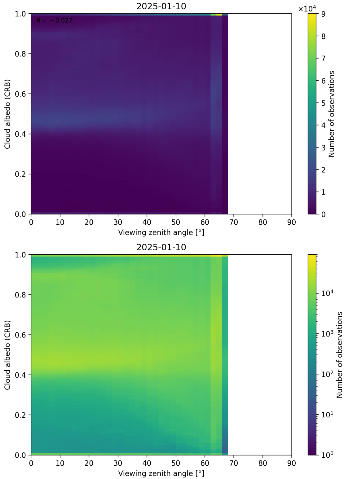
Figure 106: Scatter density plot of “Viewing zenith angle” against “Cloud albedo (CRB)” for 2025-01-09 to 2025-01-11.
