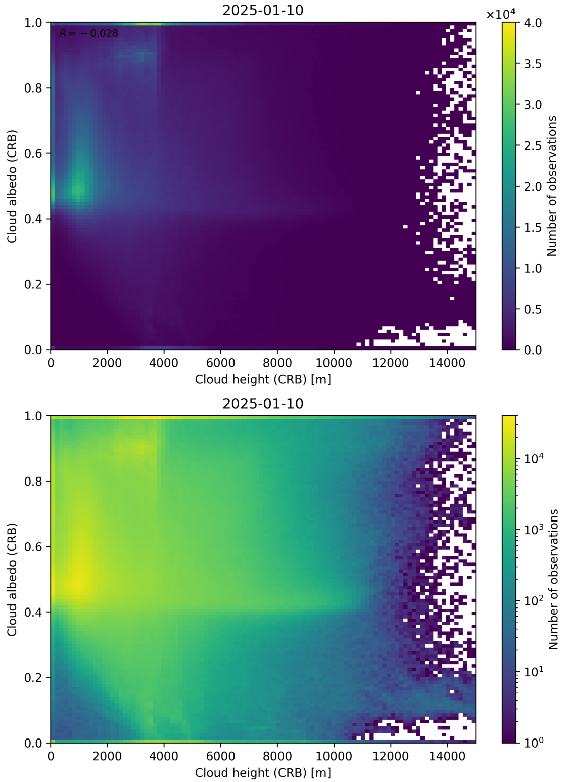
Figure 80: Scatter density plot of “Cloud height (CRB)” against “Cloud albedo (CRB)” for 2025-01-09 to 2025-01-11.
