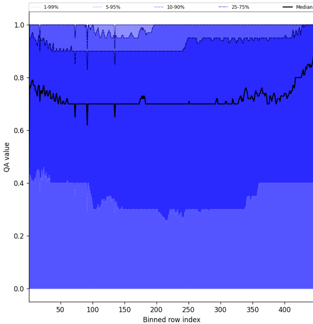
Figure 54: Along track statistics of “QA value” for 2025-01-12 to 2025-01-13
