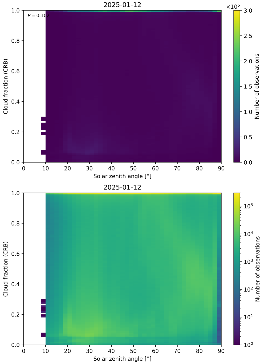
Figure 101: Scatter density plot of “Solar zenith angle” against “Cloud fraction (CRB)” for 2025-01-12 to 2025-01-13.
