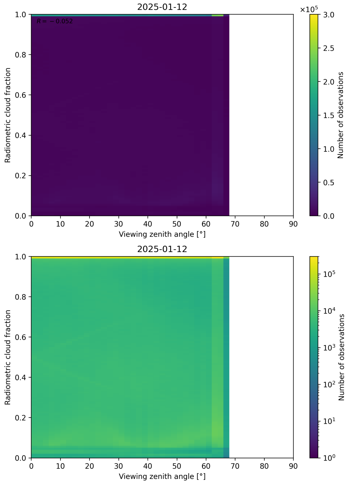
Figure 107: Scatter density plot of “Viewing zenith angle” against “Radiometric cloud fraction” for 2025-01-12 to 2025-01-13.
