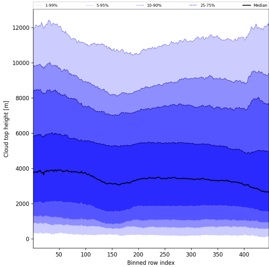
Figure 56: Along track statistics of “Cloud top height” for 2025-01-12 to 2025-01-13
