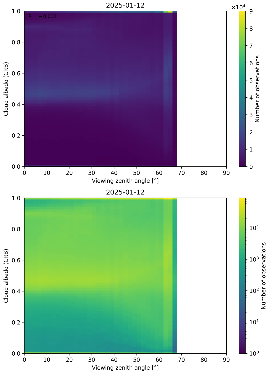
Figure 106: Scatter density plot of “Viewing zenith angle” against “Cloud albedo (CRB)” for 2025-01-12 to 2025-01-13.
