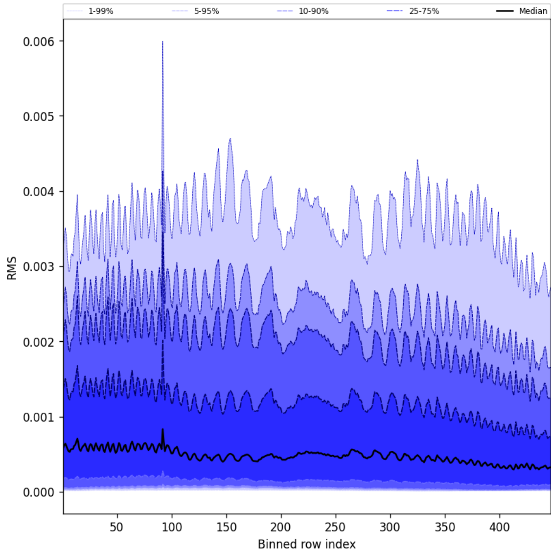
Figure 63: Along track statistics of “RMS” for 2025-01-12 to 2025-01-13
