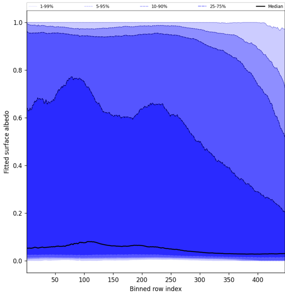
Figure 61: Along track statistics of “Fitted surface albedo” for 2025-01-12 to 2025-01-13
