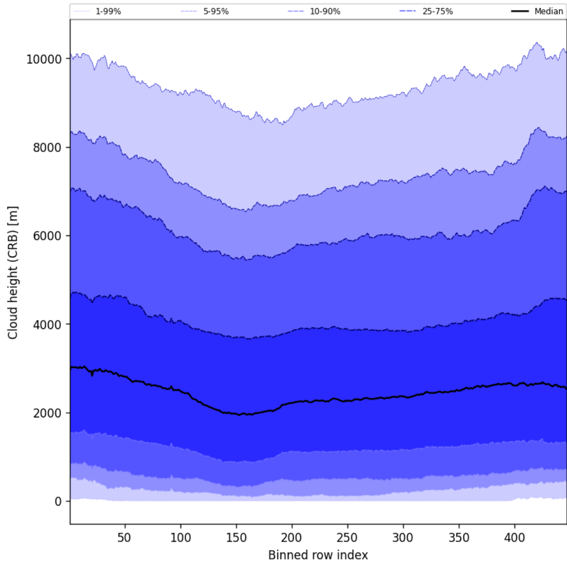
Figure 59: Along track statistics of “Cloud height (CRB)” for 2025-01-12 to 2025-01-13
