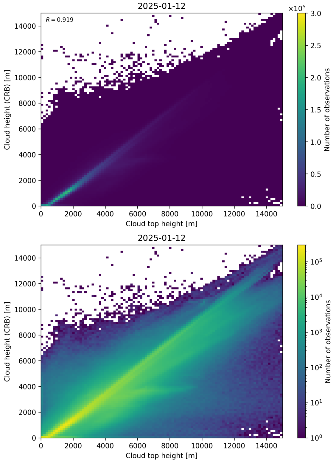
Figure 89: Scatter density plot of “Cloud top height” against “Cloud height (CRB)” for 2025-01-12 to 2025-01-13.
