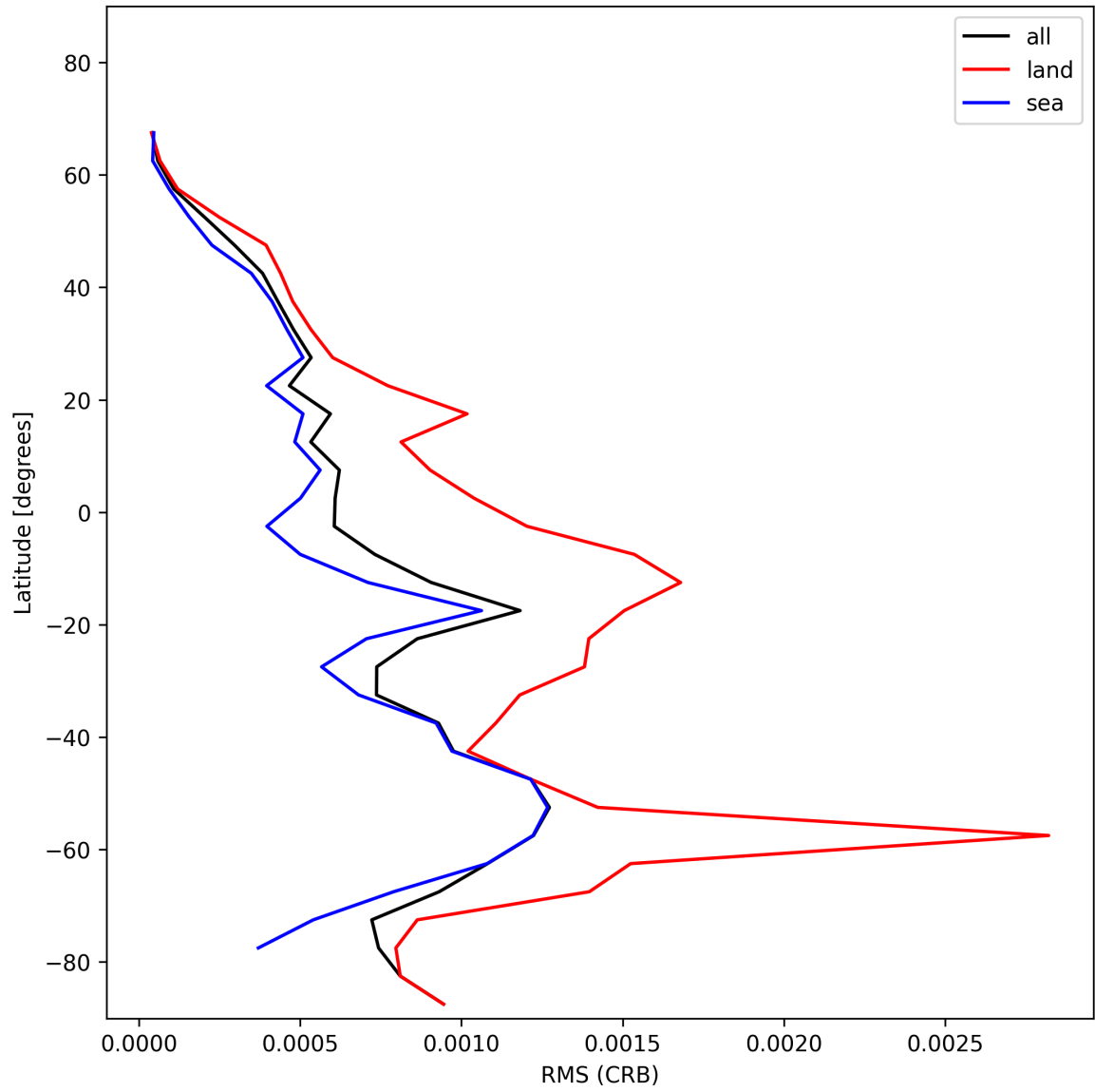
Figure 32: Zonal average of “RMS (CRB)” for 2025-01-12 to 2025-01-13.
