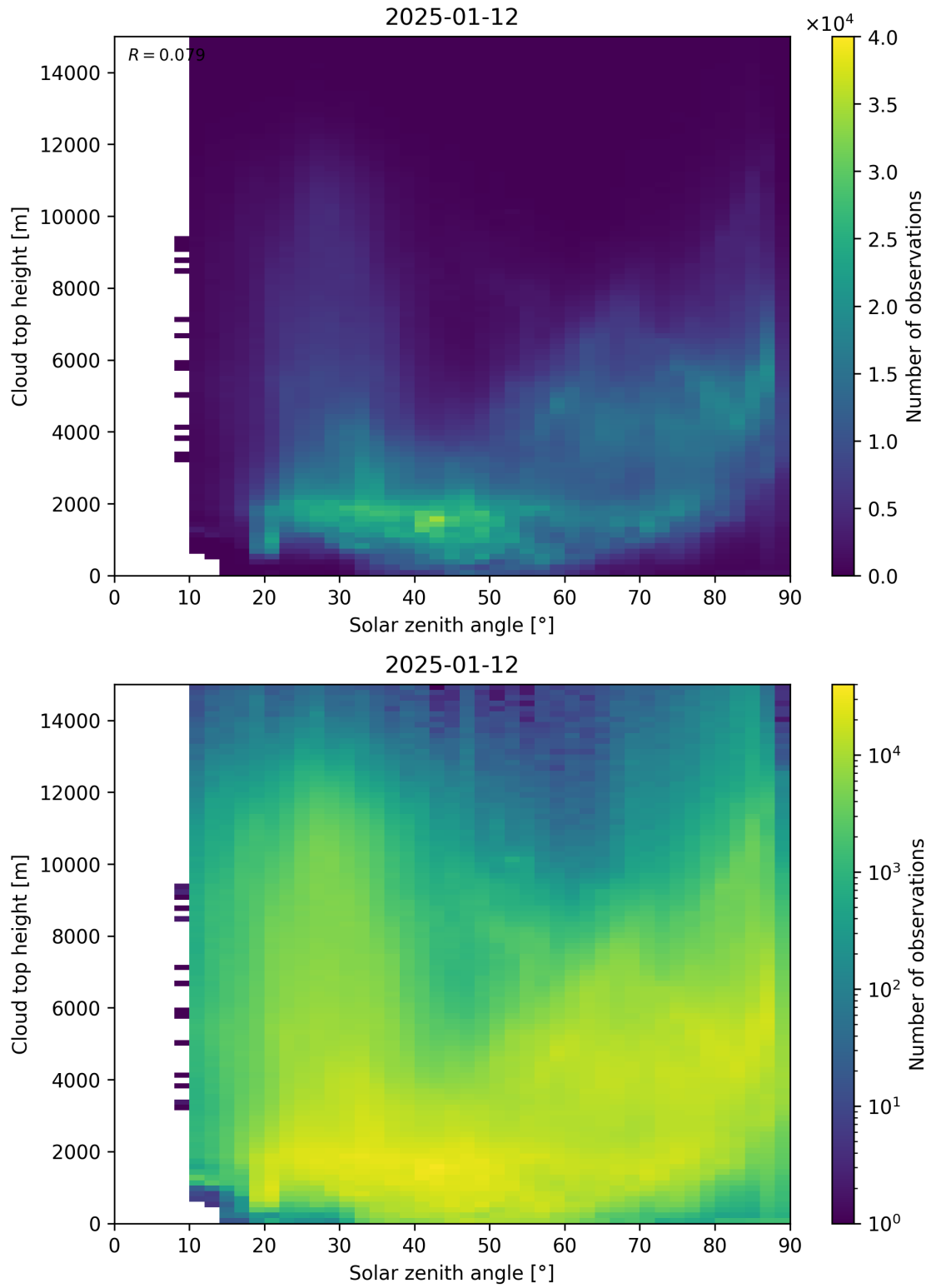
Figure 104: Scatter density plot of “Solar zenith angle” against “Cloud top height” for 2025-01-12 to 2025-01-13.
