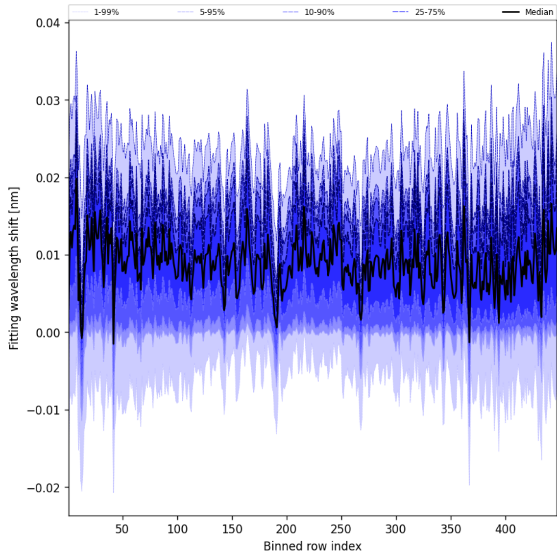
Figure 65: Along track statistics of “Fitting wavelength shift” for 2025-01-12 to 2025-01-13
