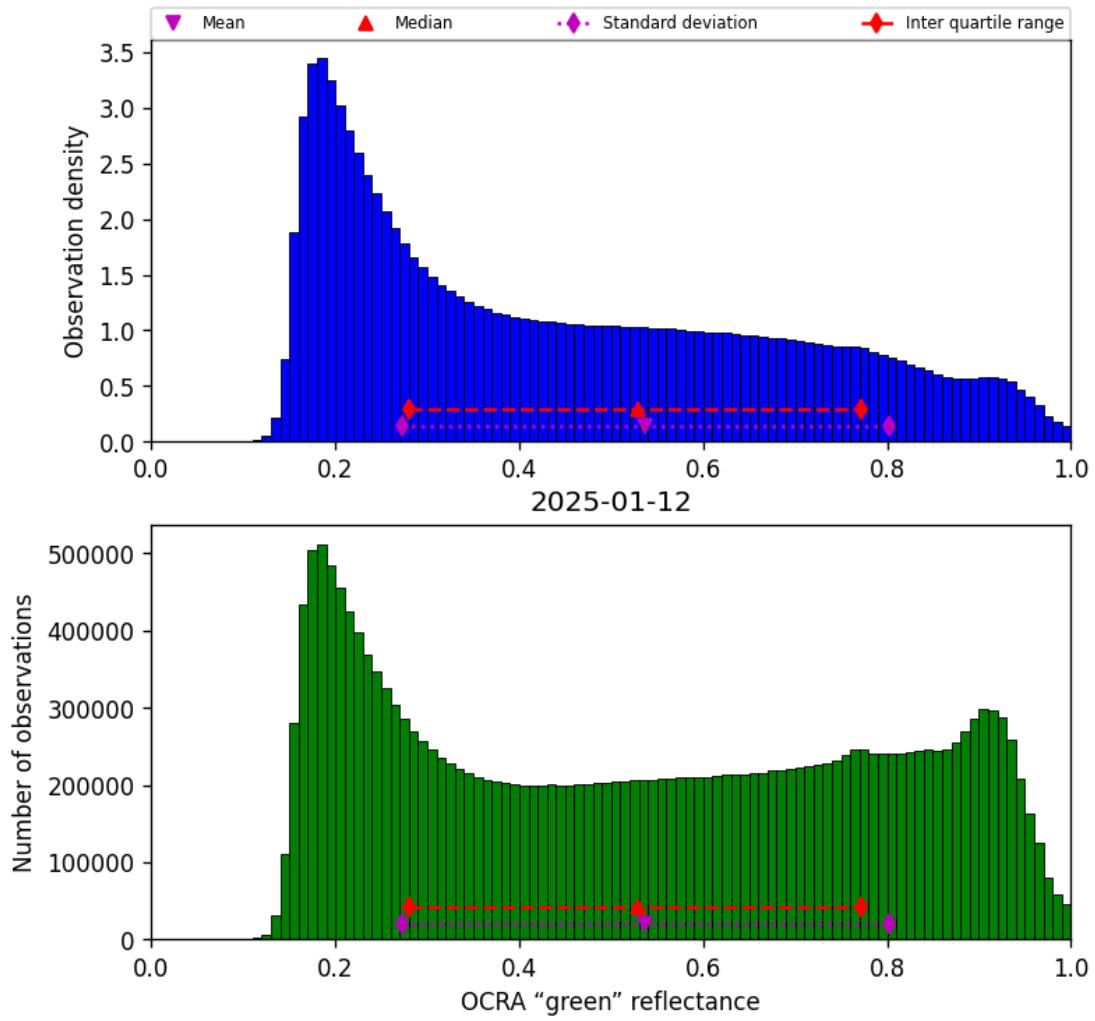
Figure 52: Histogram of “OCRA “green” reflectance” for 2025-01-12 to 2025-01-13
