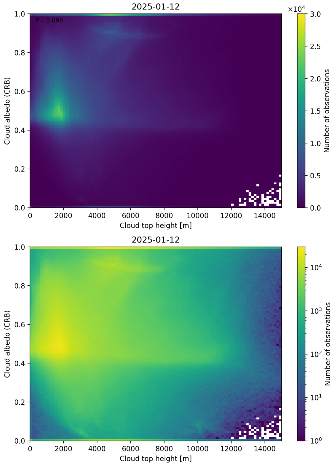
Figure 86: Scatter density plot of “Cloud top height” against “Cloud albedo (CRB)” for 2025-01-12 to 2025-01-13.
