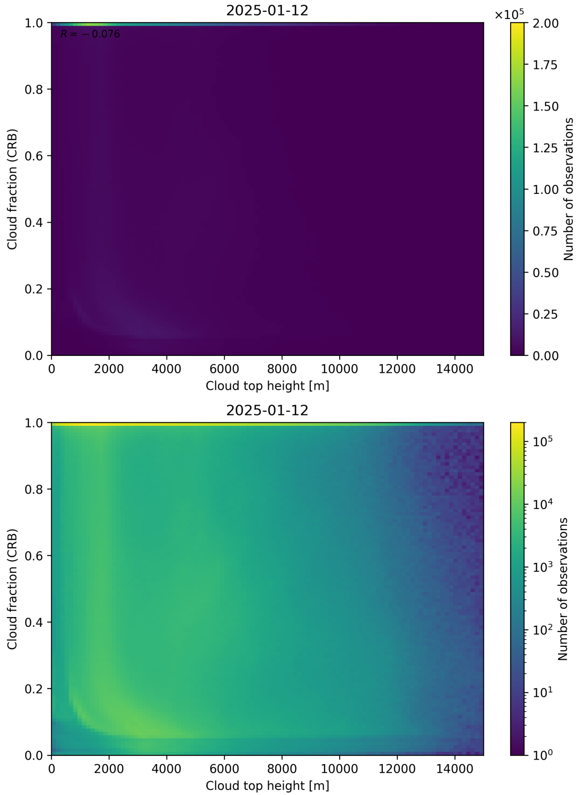
Figure 88: Scatter density plot of “Cloud top height” against “Cloud fraction (CRB)” for 2025-01-12 to 2025-01-13.
