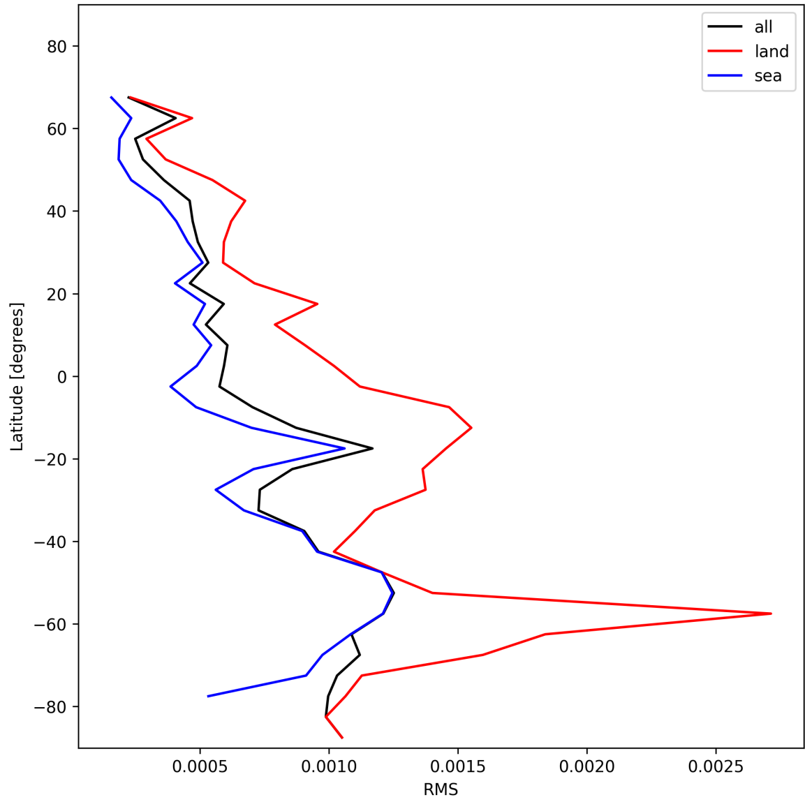
Figure 31: Zonal average of “RMS” for 2025-01-12 to 2025-01-13.
