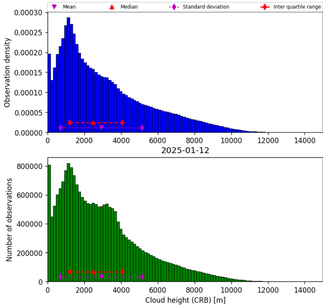
Figure 43: Histogram of “Cloud height (CRB)” for 2025-01-12 to 2025-01-13
