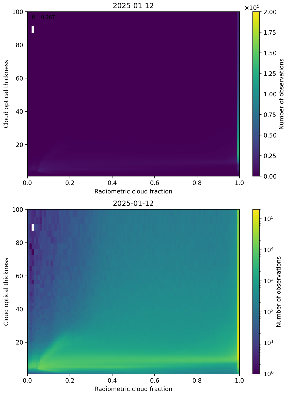
Figure 75: Scatter density plot of “Radiometric cloud fraction” against “Cloud optical thickness” for 2025-01-12 to 2025-01-13.
