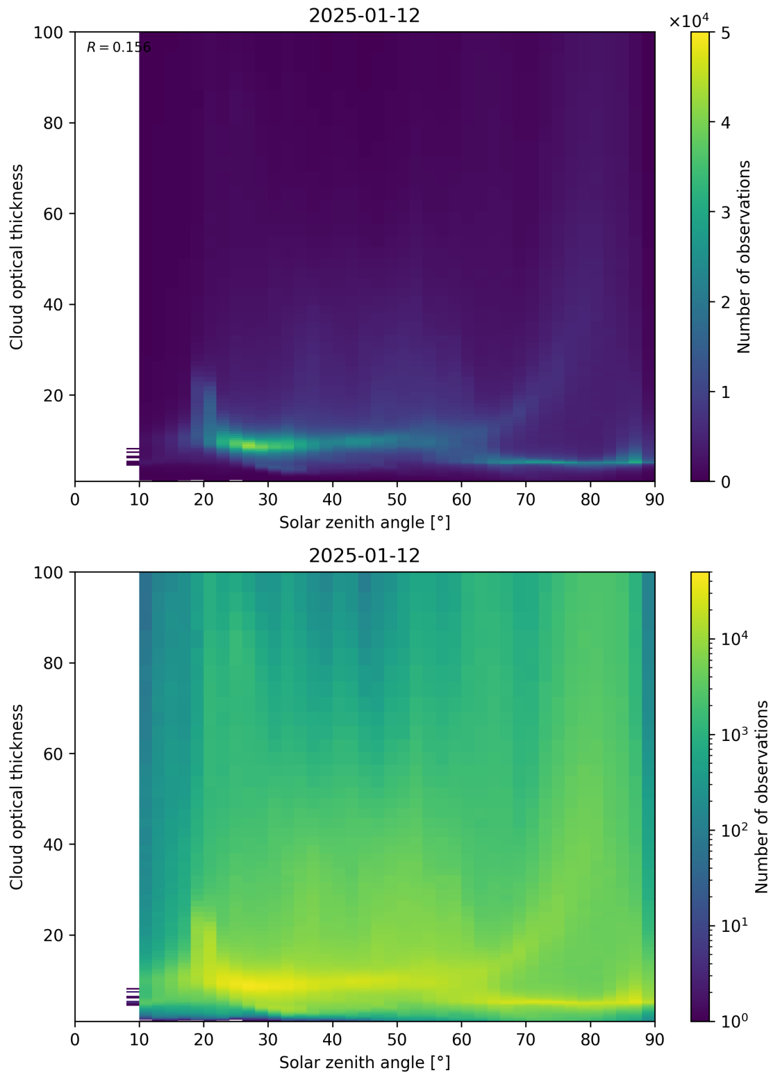
Figure 103: Scatter density plot of “Solar zenith angle” against “Cloud optical thickness” for 2025-01-12 to 2025-01-13.
