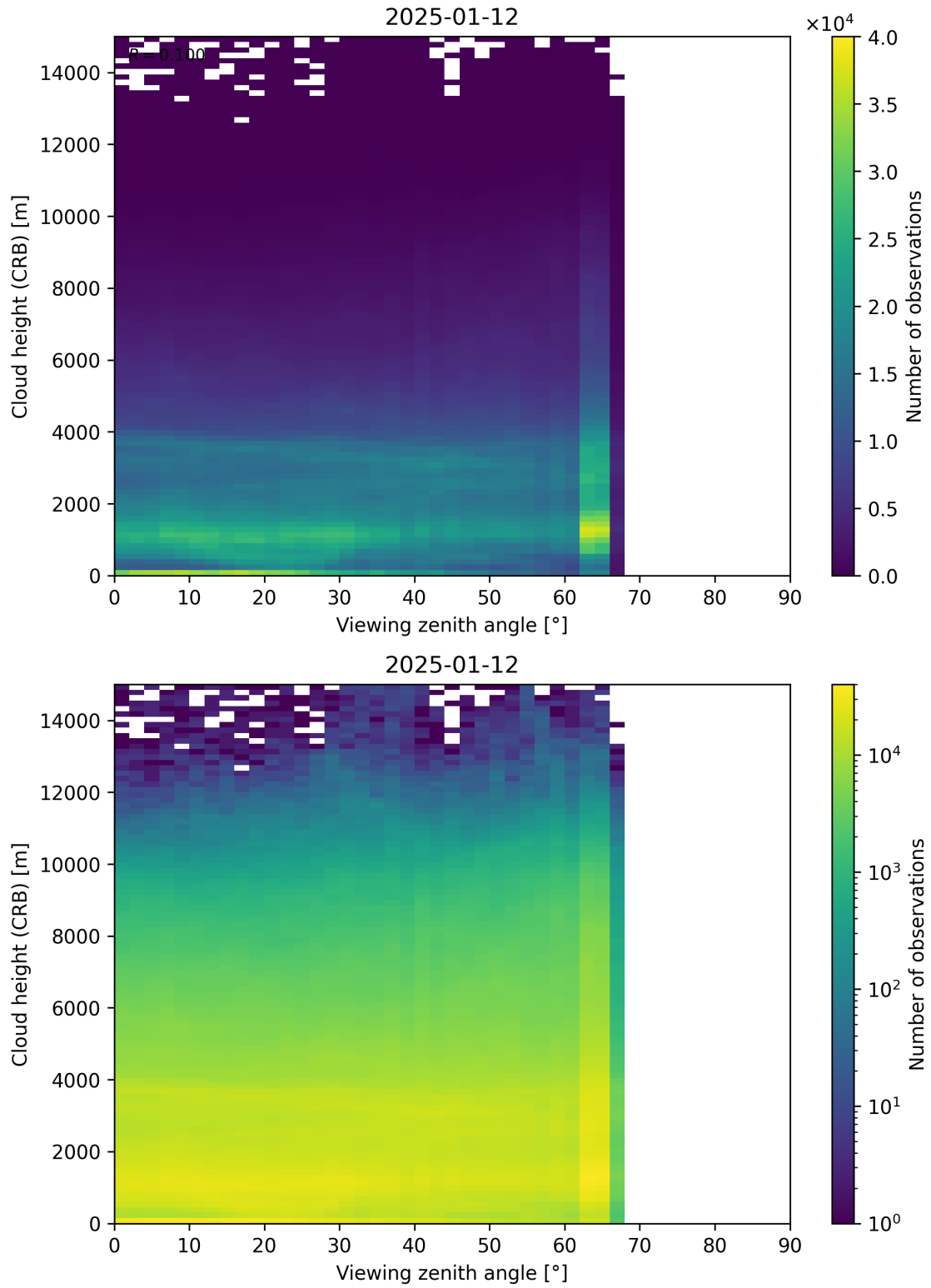
Figure 110: Scatter density plot of “Viewing zenith angle” against “Cloud height (CRB)” for 2025-01-12 to 2025-01-13.
