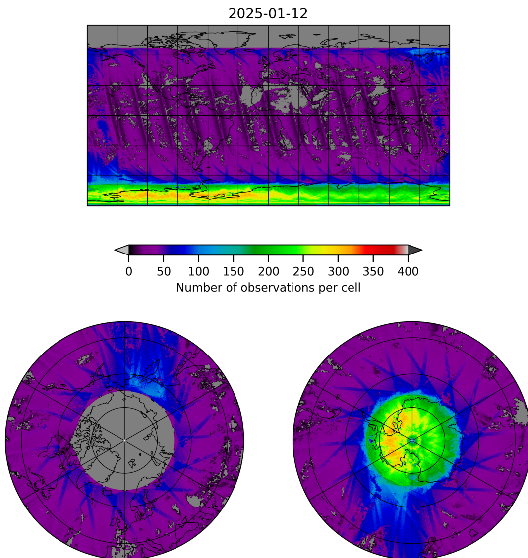
Figure 21: Map of the number of observations for 2025-01-12 to 2025-01-13
