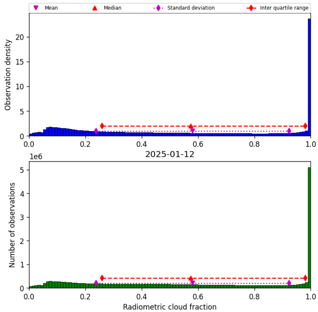
Figure 39: Histogram of “Radiometric cloud fraction” for 2025-01-12 to 2025-01-13
