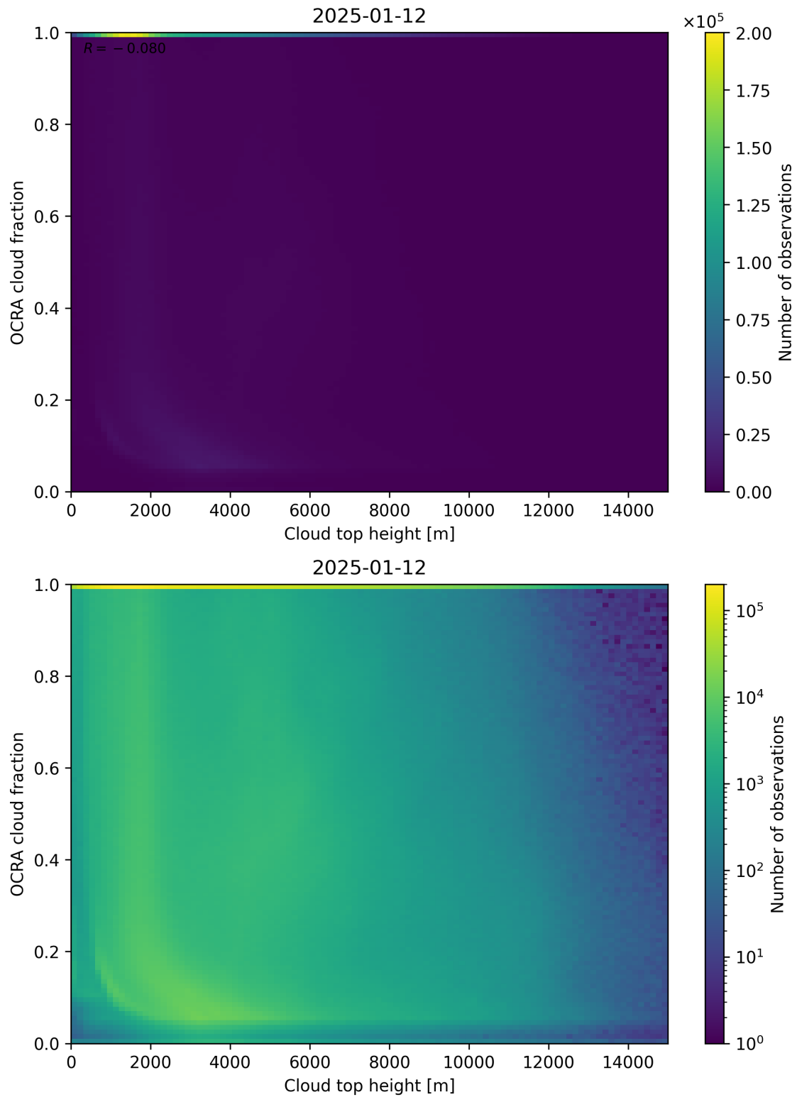
Figure 87: Scatter density plot of “Cloud top height” against “OCRA cloud fraction” for 2025-01-12 to 2025-01-13.
