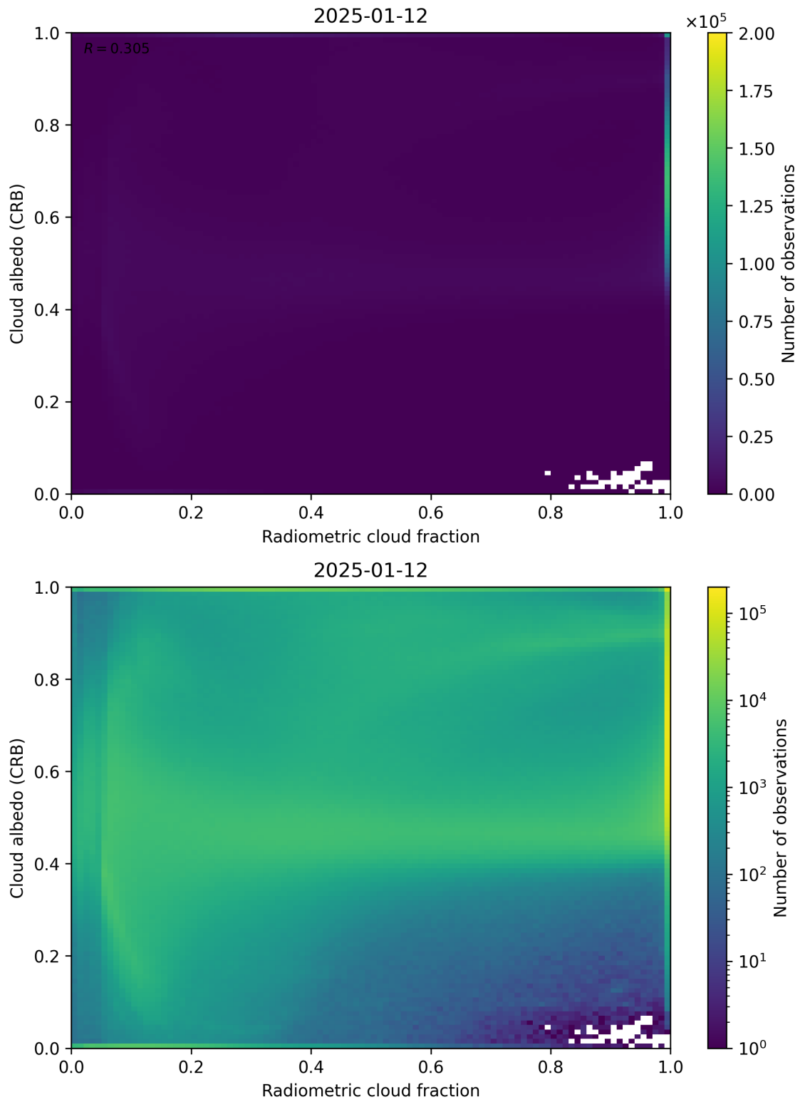
Figure 71: Scatter density plot of “Radiometric cloud fraction” against “Cloud albedo (CRB)” for 2025-01-12 to 2025-01-13.
