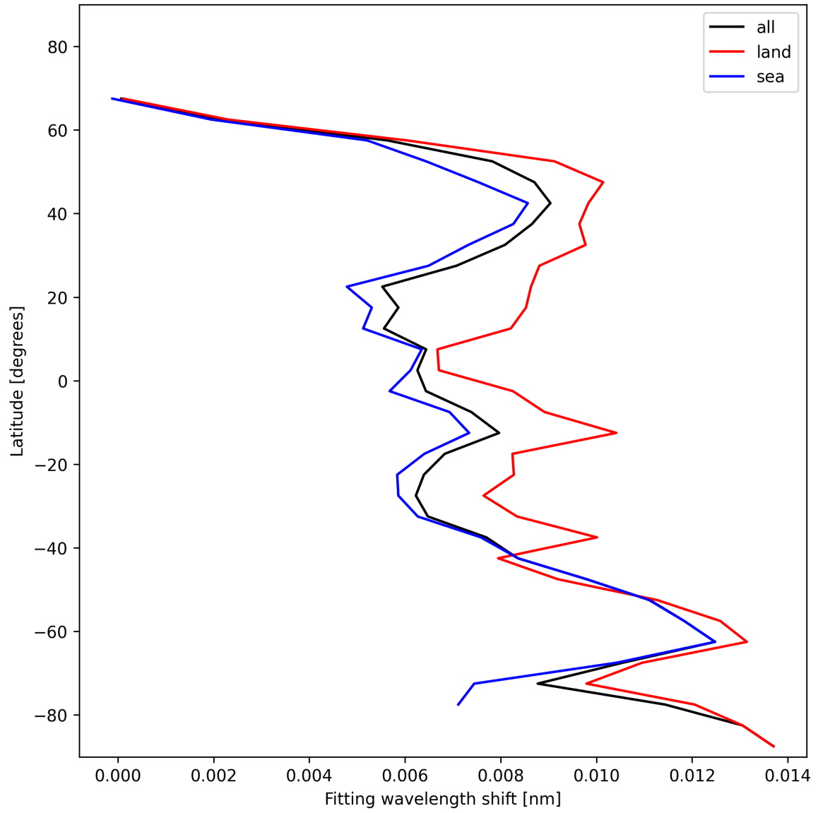
Figure 33: Zonal average of “Fitting wavelength shift” for 2025-01-12 to 2025-01-13.
