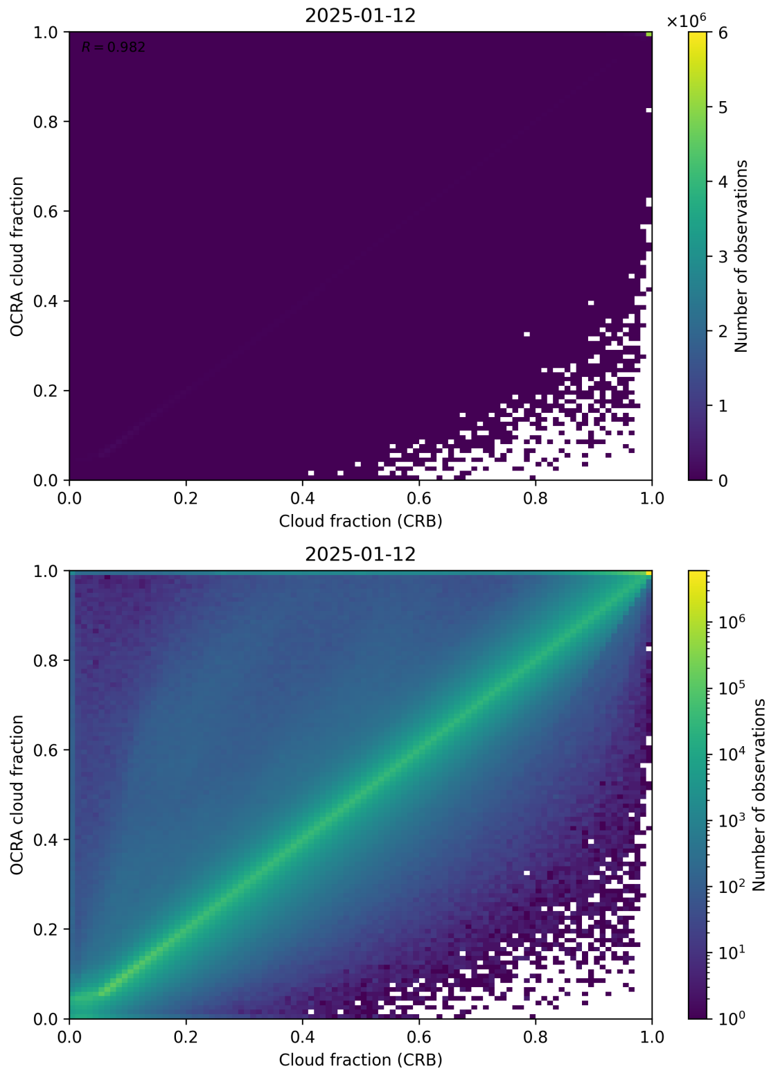
Figure 78: Scatter density plot of “Cloud fraction (CRB)” against “OCRA cloud fraction” for 2025-01-12 to 2025-01-13.
