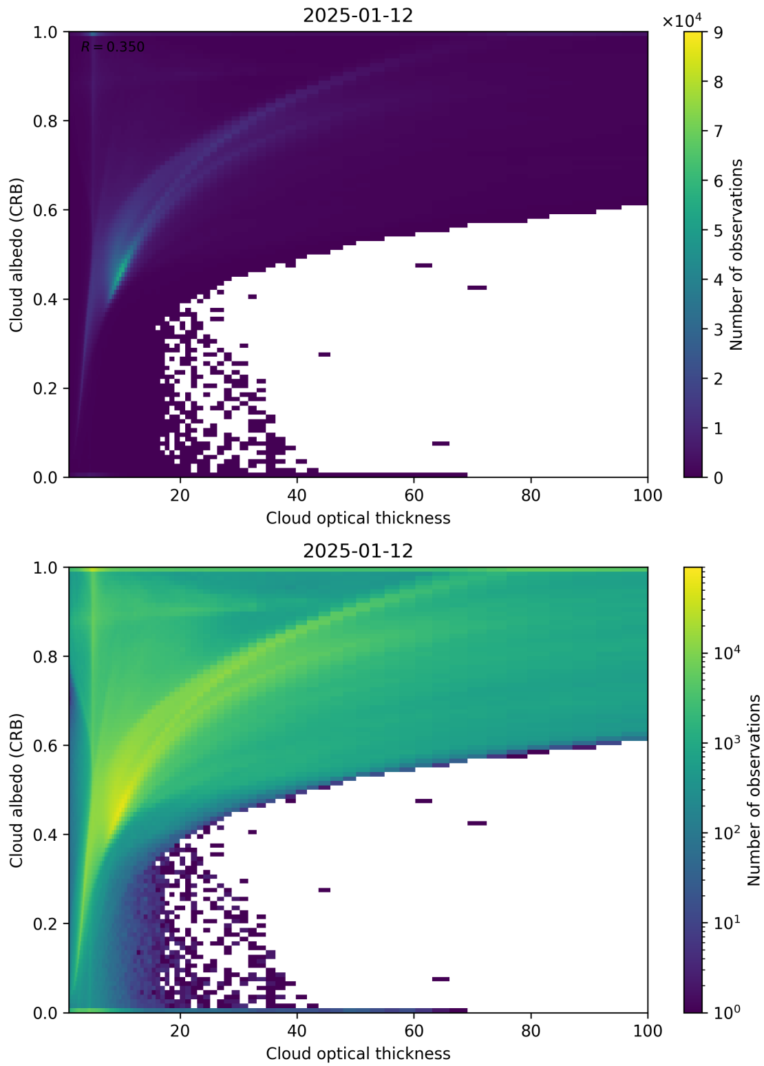
Figure 82: Scatter density plot of “Cloud optical thickness” against “Cloud albedo (CRB)” for 2025-01-12 to 2025-01-13.
