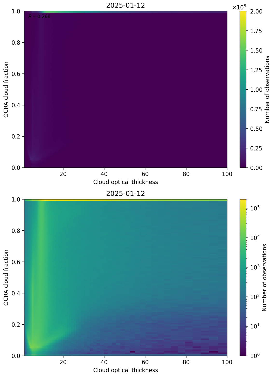
Figure 83: Scatter density plot of “Cloud optical thickness” against “OCRA cloud fraction” for 2025-01-12 to 2025-01-13.
