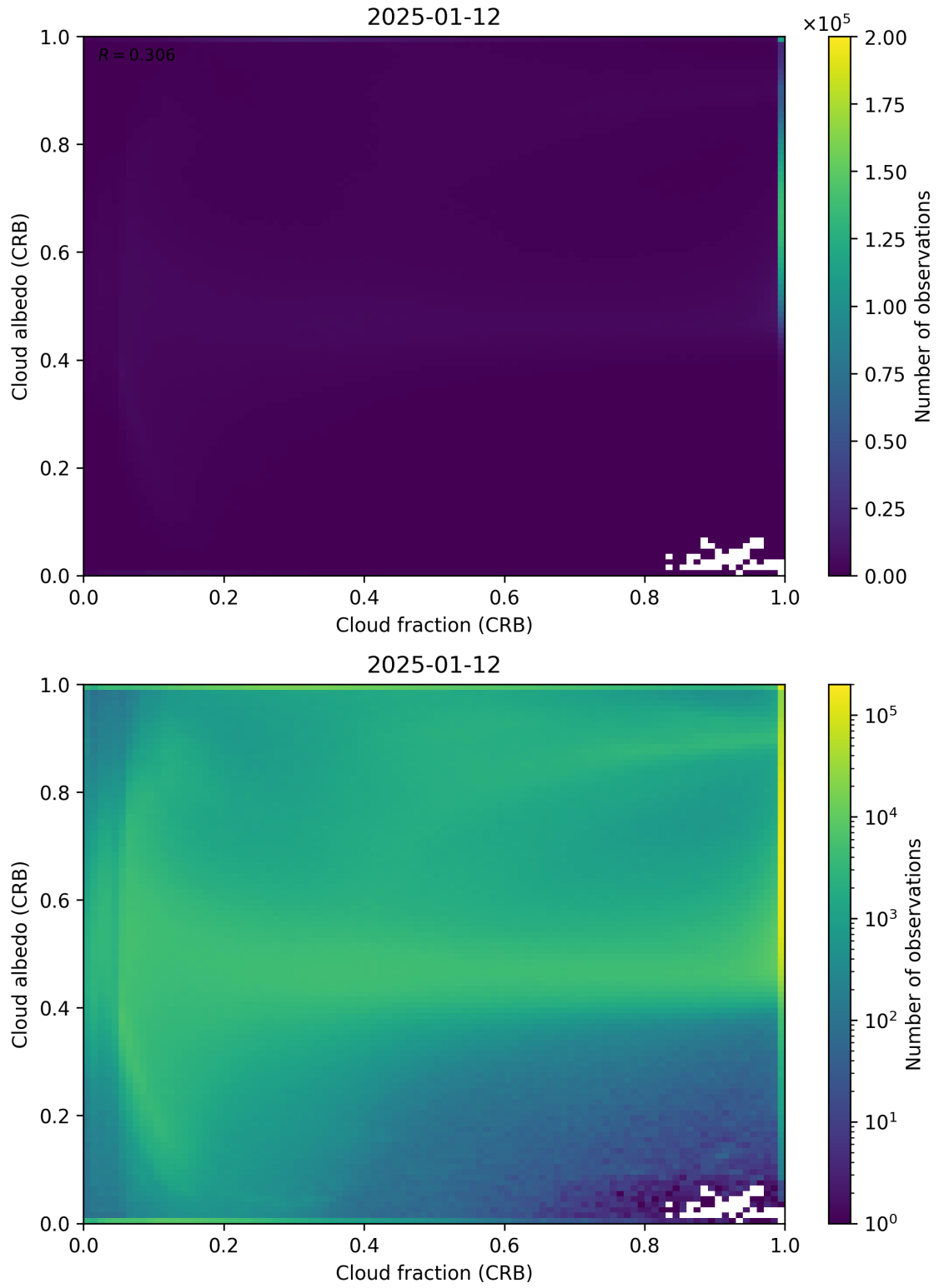
Figure 77: Scatter density plot of “Cloud fraction (CRB)” against “Cloud albedo (CRB)” for 2025-01-12 to 2025-01-13.
