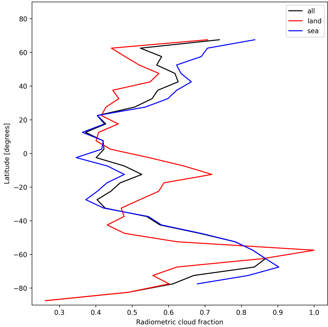
Figure 23: Zonal average of “Radiometric cloud fraction” for 2025-01-12 to 2025-01-13.
