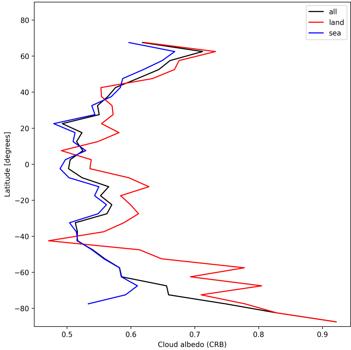
Figure 28: Zonal average of “Cloud albedo (CRB)” for 2025-01-12 to 2025-01-13.
