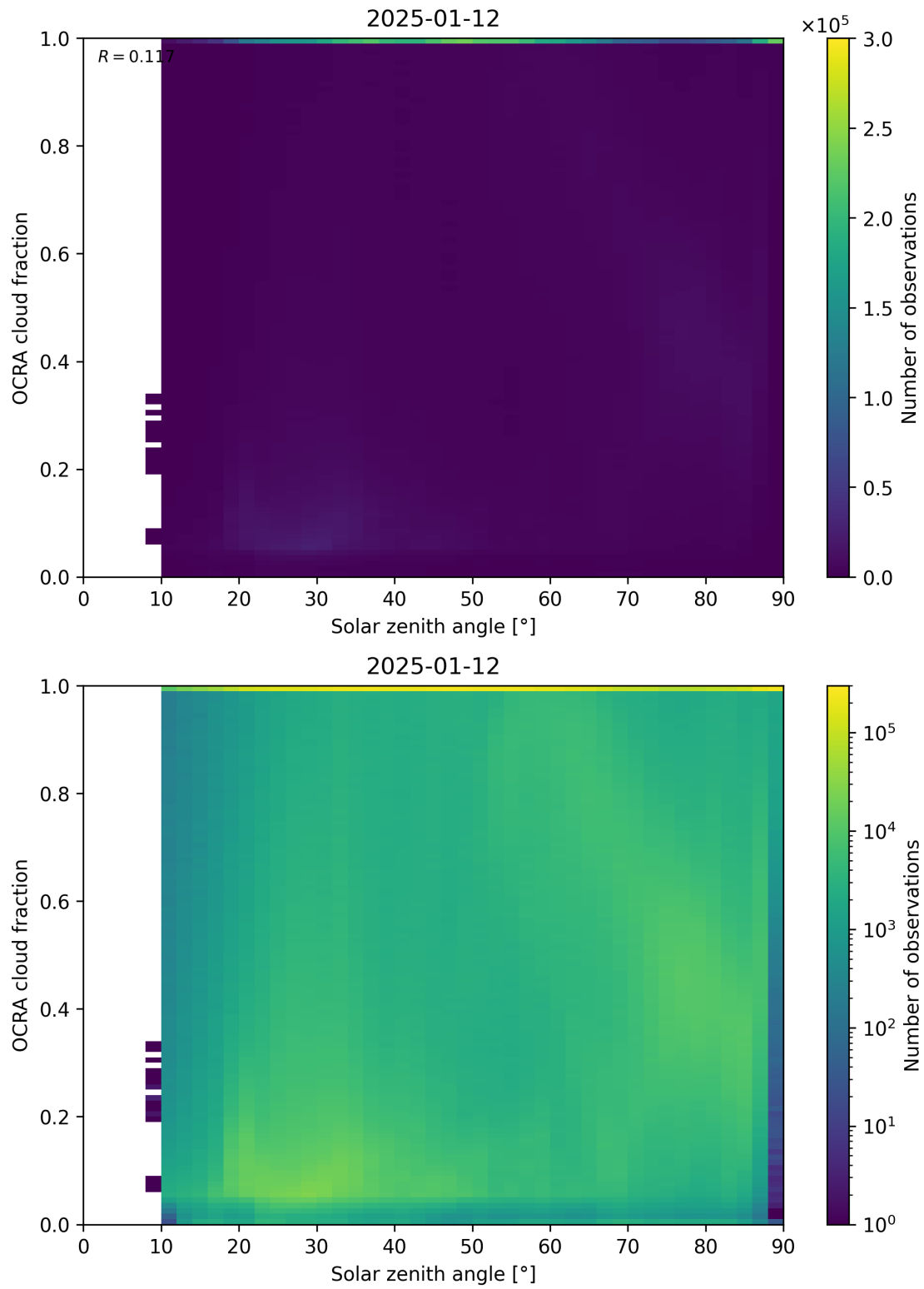
Figure 100: Scatter density plot of “Solar zenith angle” against “OCRA cloud fraction” for 2025-01-12 to 2025-01-13.
