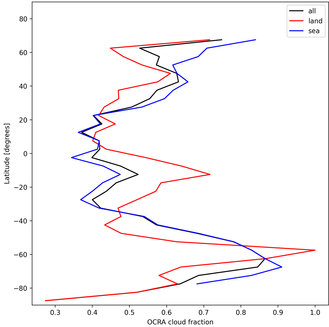
Figure 34: Zonal average of “OCRA cloud fraction” for 2025-01-12 to 2025-01-13.
