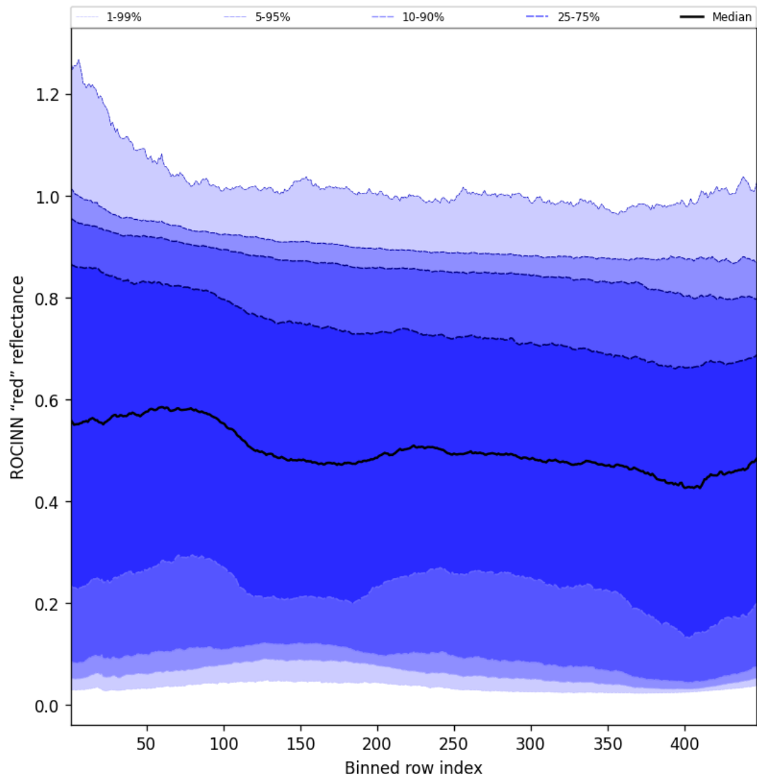
Figure 69: Along track statistics of “ROCINN “red” reflectance” for 2025-01-12 to 2025-01-13
