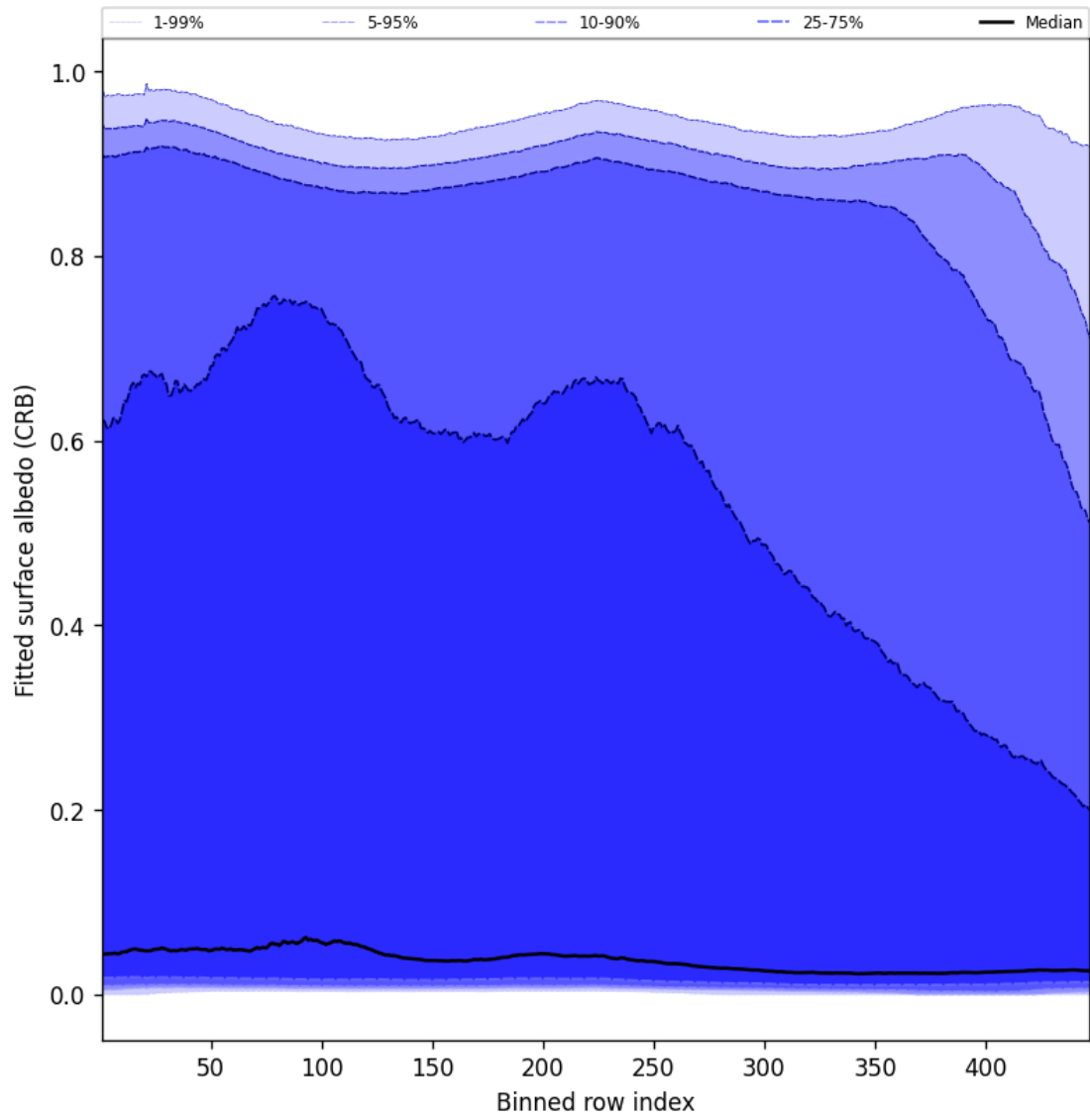
Figure 62: Along track statistics of “Fitted surface albedo (CRB)” for 2025-01-12 to 2025-01-13
