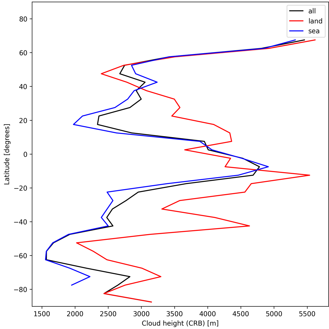
Figure 27: Zonal average of “Cloud height (CRB)” for 2025-01-12 to 2025-01-13.
