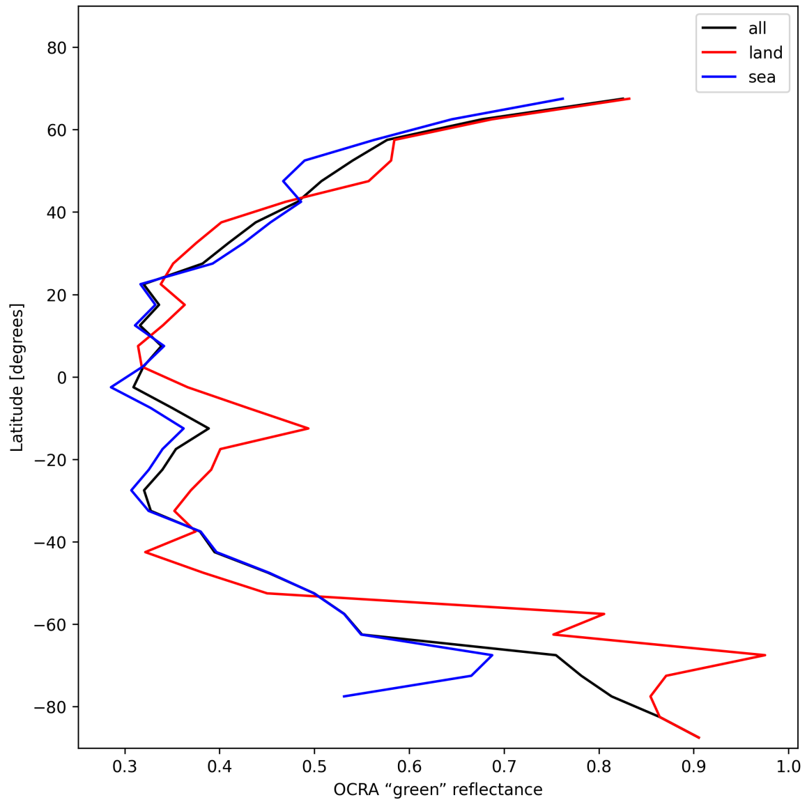
Figure 36: Zonal average of “OCRA “green” reflectance” for 2025-01-12 to 2025-01-13.
