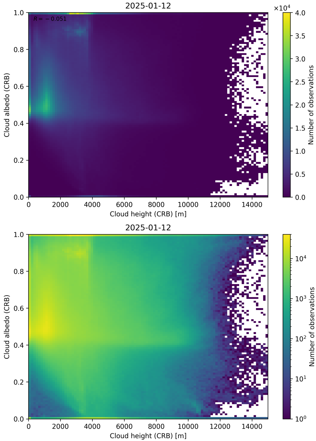
Figure 80: Scatter density plot of “Cloud height (CRB)” against “Cloud albedo (CRB)” for 2025-01-12 to 2025-01-13.
