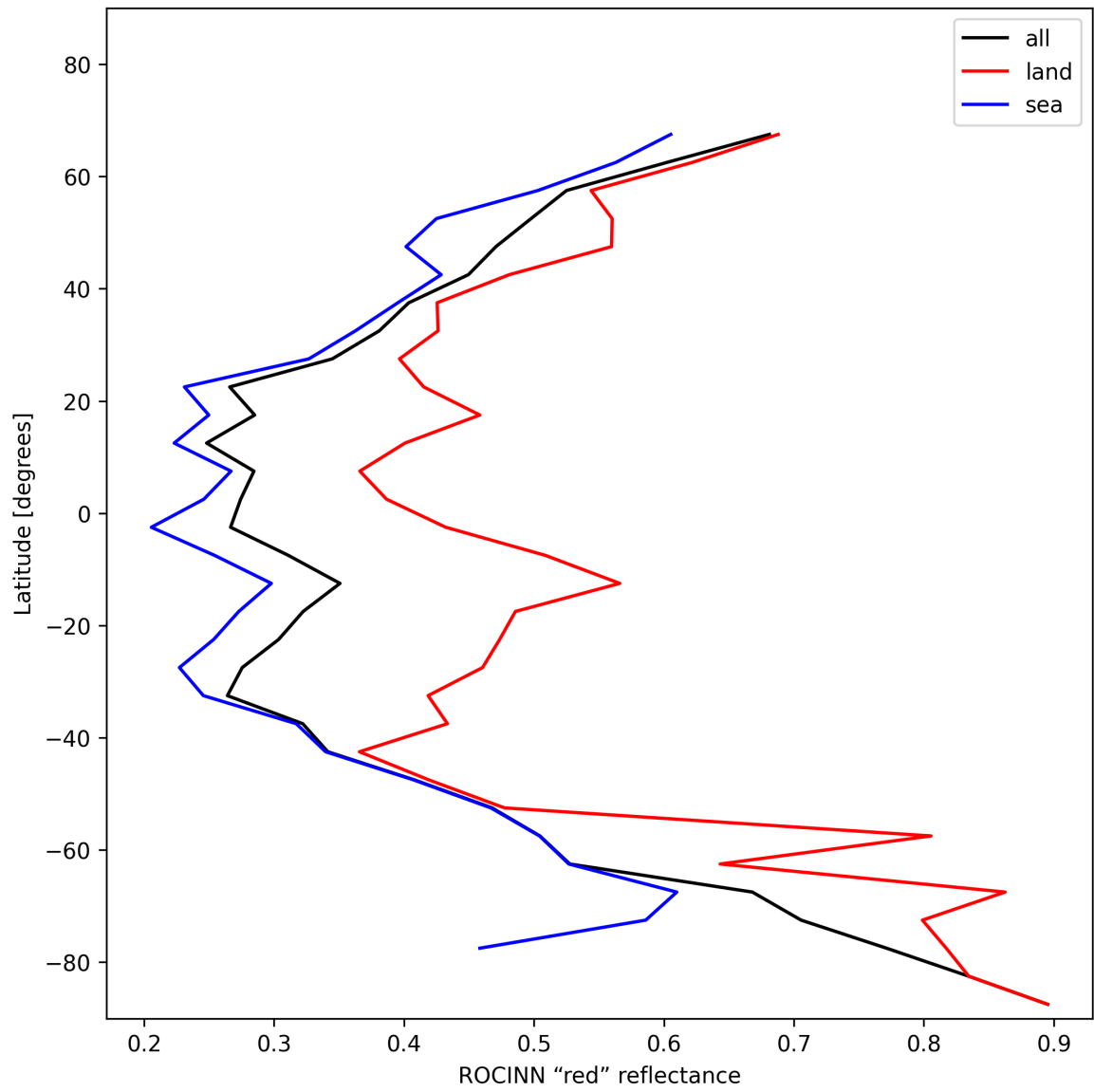
Figure 37: Zonal average of “ROCINN “red” reflectance” for 2025-01-12 to 2025-01-13.
