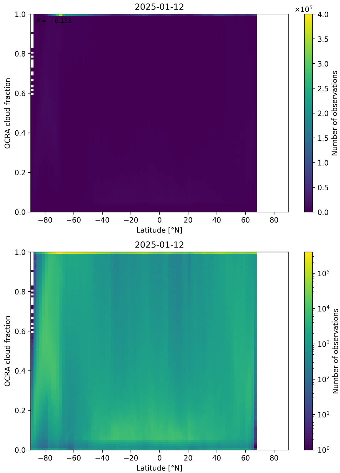
Figure 93: Scatter density plot of “Latitude” against “OCRA cloud fraction” for 2025-01-12 to 2025-01-13.
