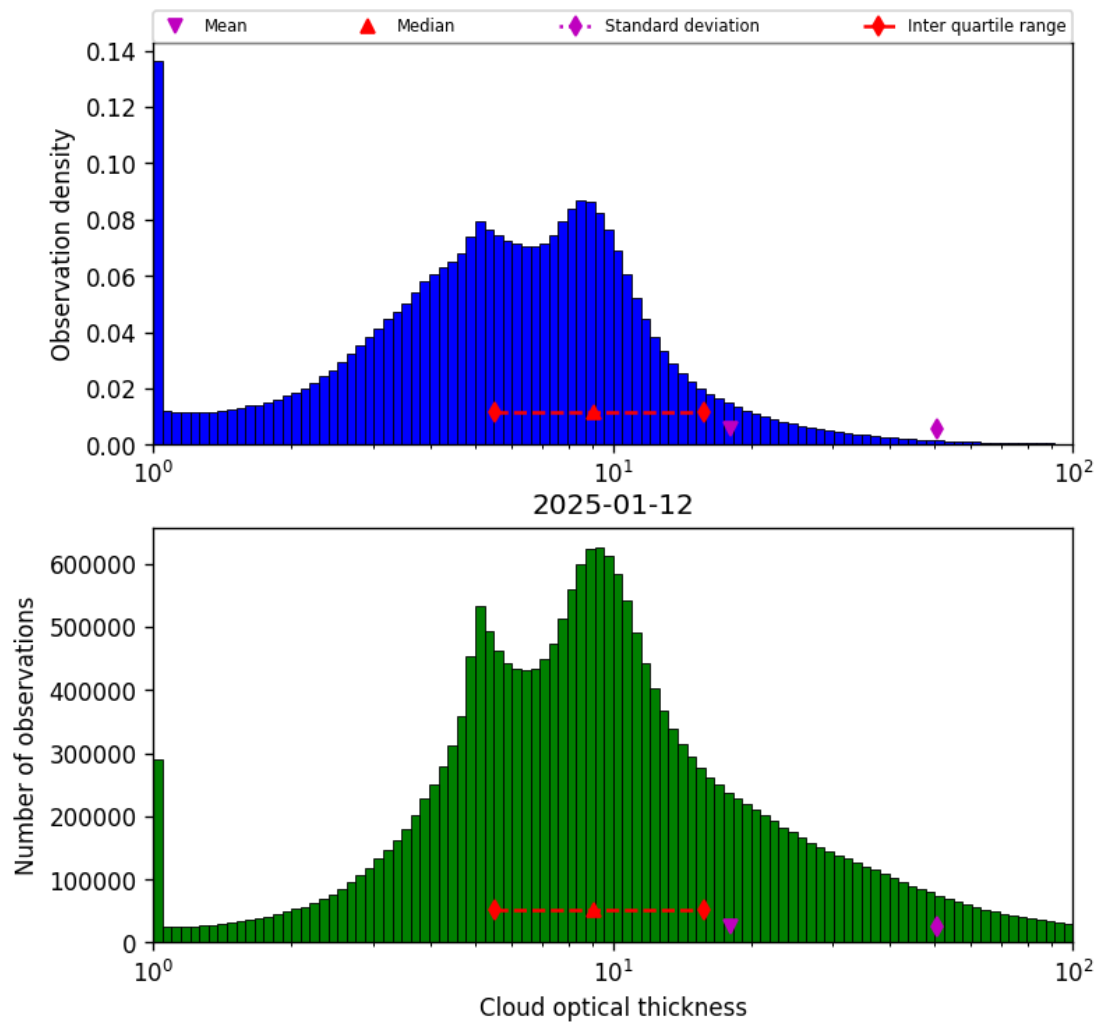
Figure 41: Histogram of “Cloud optical thickness” for 2025-01-12 to 2025-01-13
