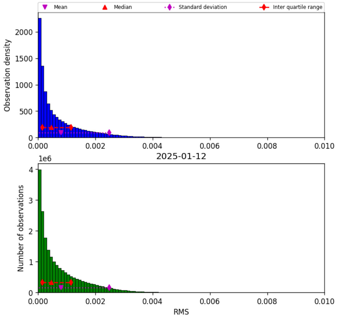
Figure 47: Histogram of “RMS” for 2025-01-12 to 2025-01-13
