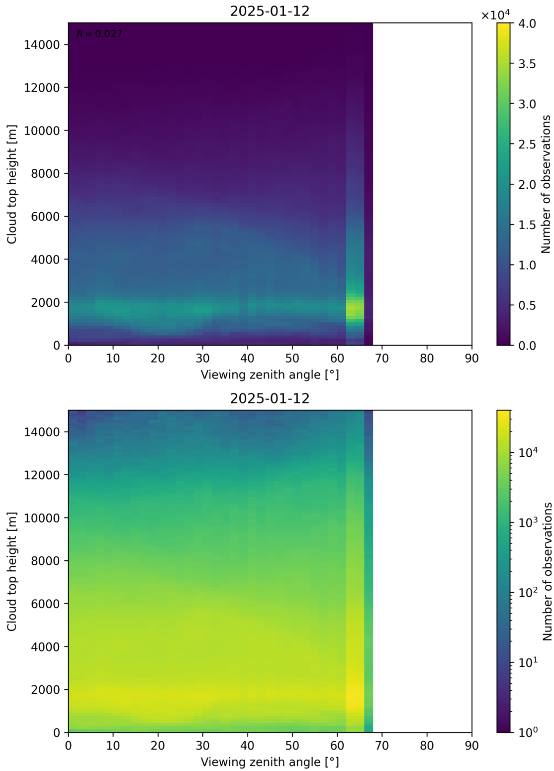
Figure 112: Scatter density plot of “Viewing zenith angle” against “Cloud top height” for 2025-01-12 to 2025-01-13.
