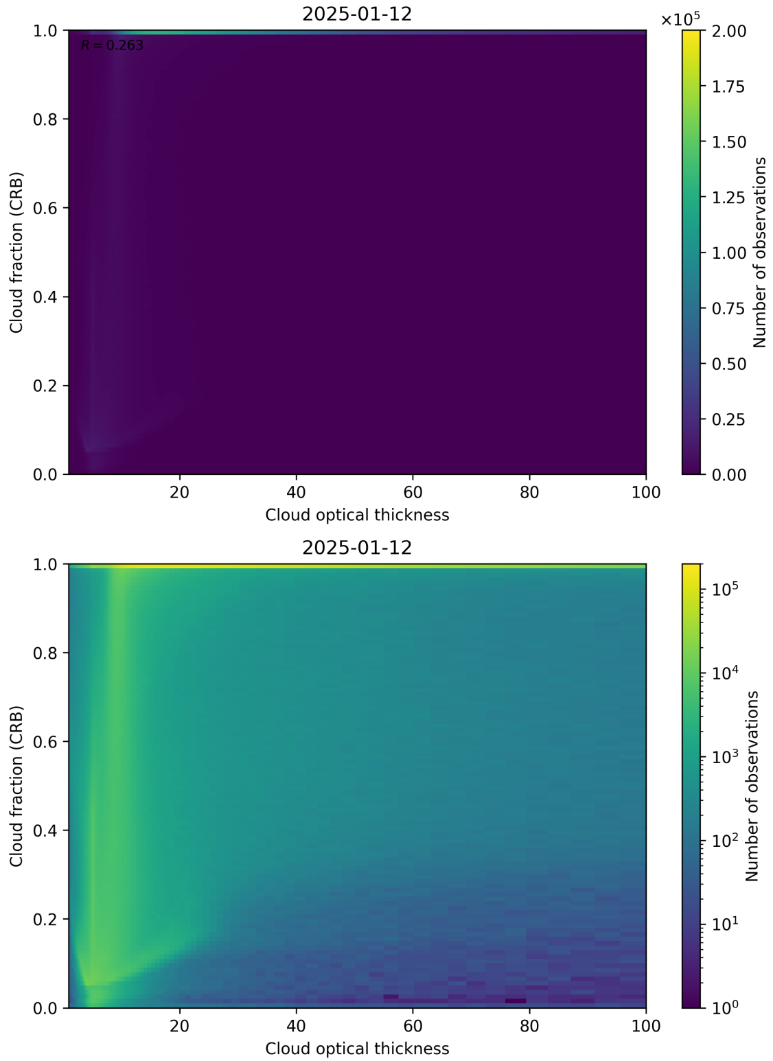
Figure 84: Scatter density plot of “Cloud optical thickness” against “Cloud fraction (CRB)” for 2025-01-12 to 2025-01-13.
