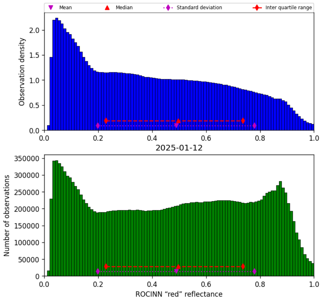
Figure 53: Histogram of “ROCINN “red” reflectance” for 2025-01-12 to 2025-01-13
