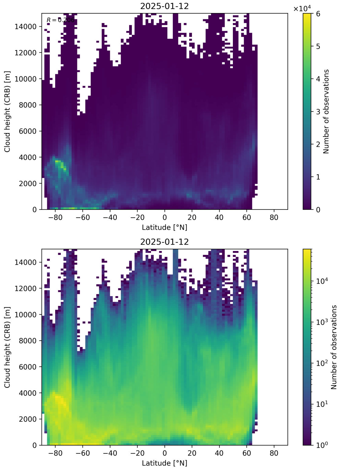
Figure 95: Scatter density plot of “Latitude” against “Cloud height (CRB)” for 2025-01-12 to 2025-01-13.
