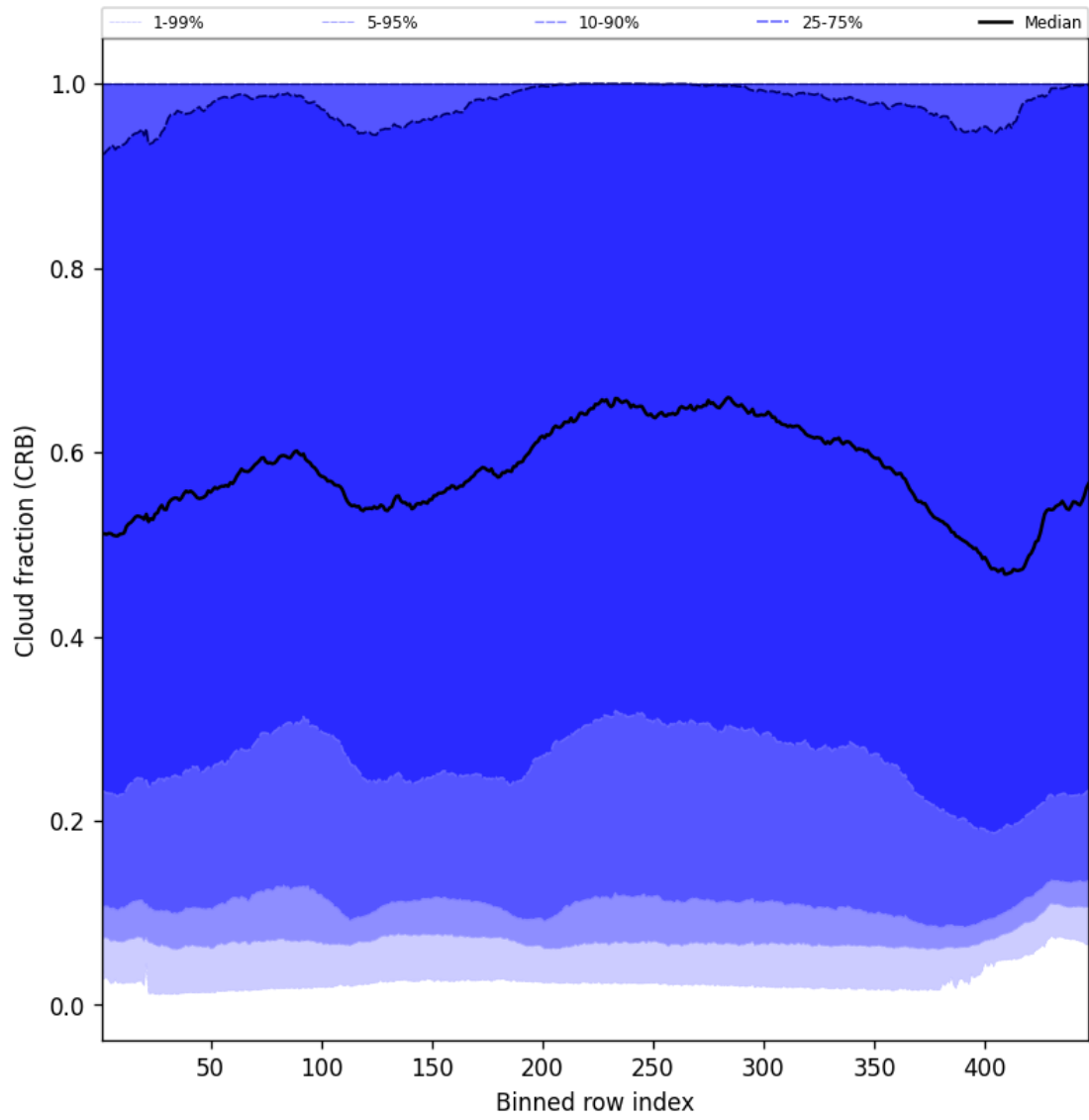
Figure 58: Along track statistics of “Cloud fraction (CRB)” for 2025-01-12 to 2025-01-13
