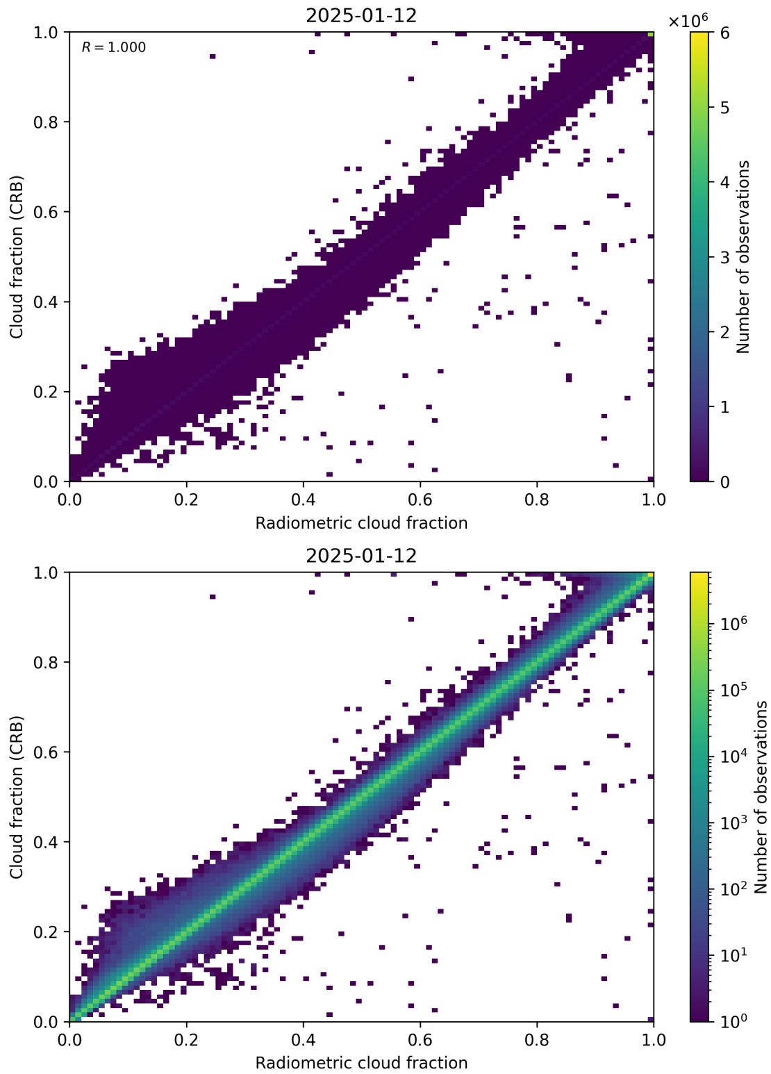
Figure 73: Scatter density plot of “Radiometric cloud fraction” against “Cloud fraction (CRB)” for 2025-01-12 to 2025-01-13.
