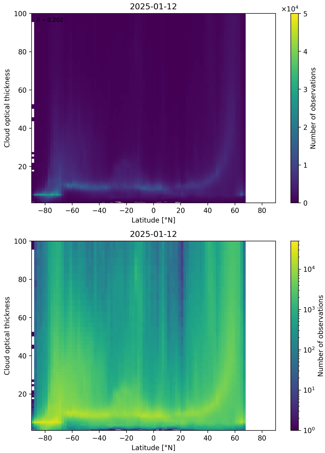
Figure 96: Scatter density plot of “Latitude” against “Cloud optical thickness” for 2025-01-12 to 2025-01-13.
