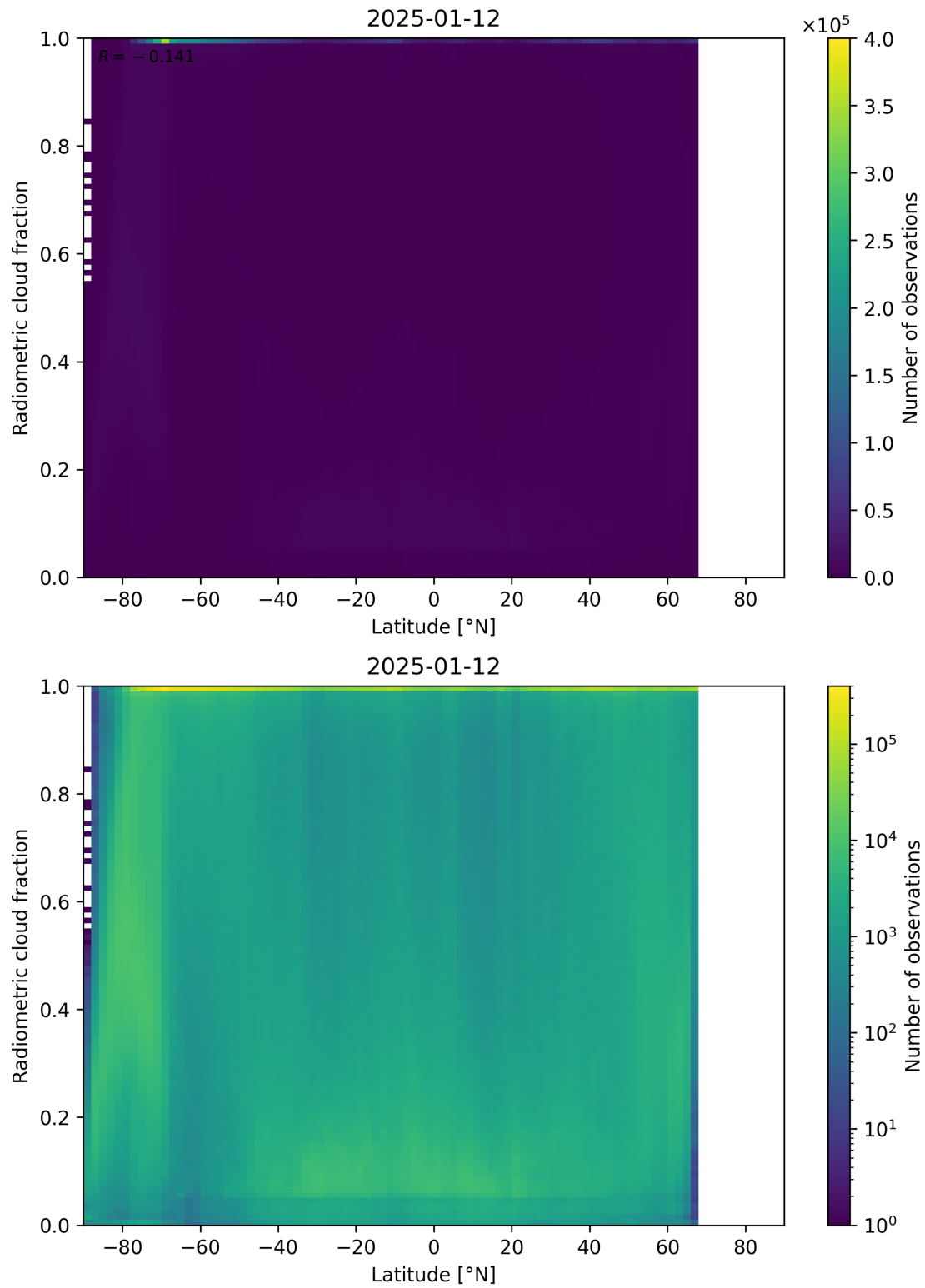
Figure 92: Scatter density plot of “Latitude” against “Radiometric cloud fraction” for 2025-01-12 to 2025-01-13.
