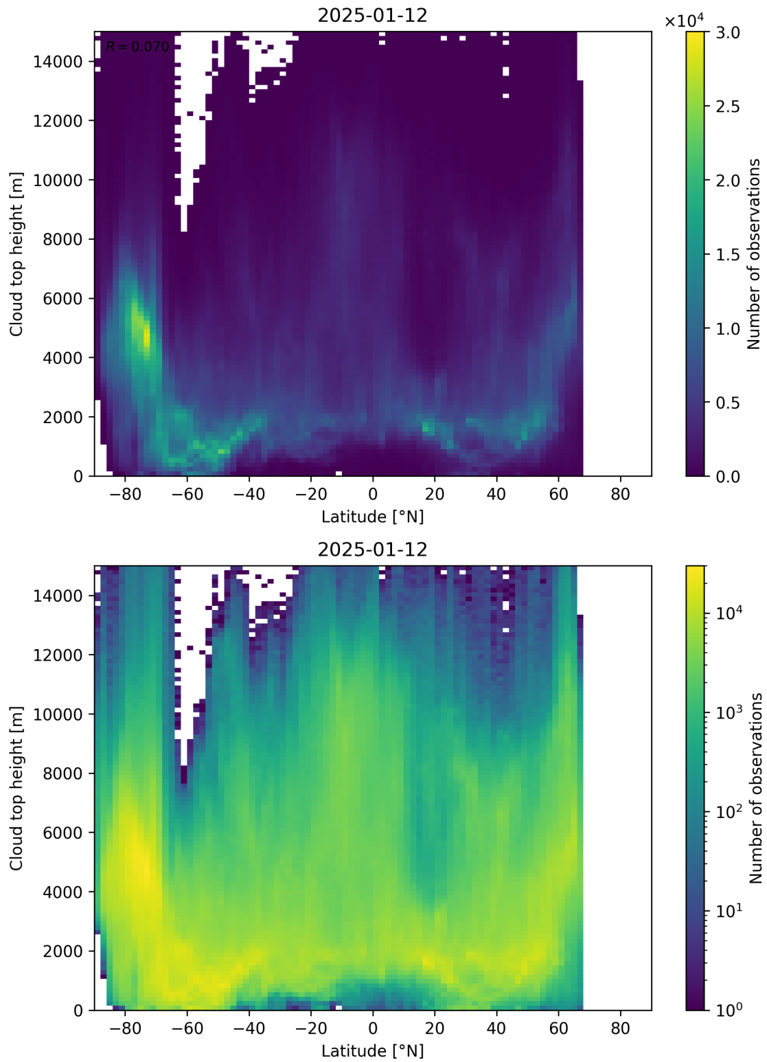
Figure 97: Scatter density plot of “Latitude” against “Cloud top height” for 2025-01-12 to 2025-01-13.
