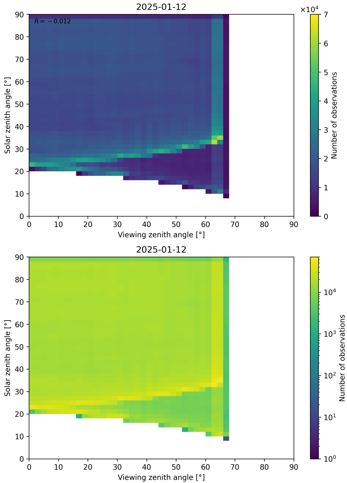
Figure 114: Scatter density plot of “Viewing zenith angle” against “Solar zenith angle” for 2025-01-12 to 2025-01-13.
