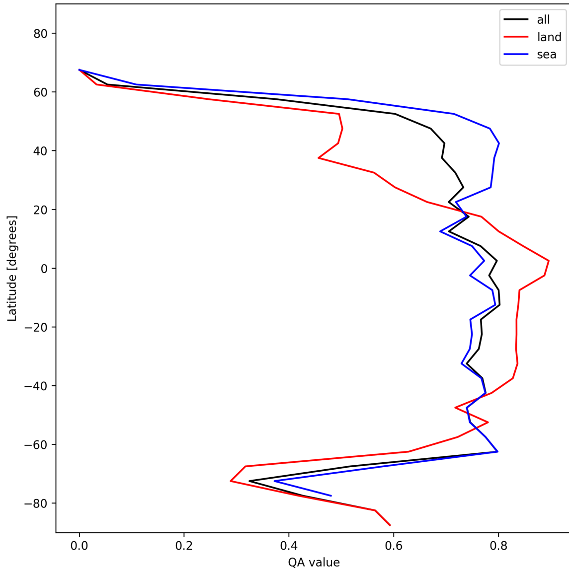
Figure 22: Zonal average of “QA value” for 2025-01-12 to 2025-01-13.
