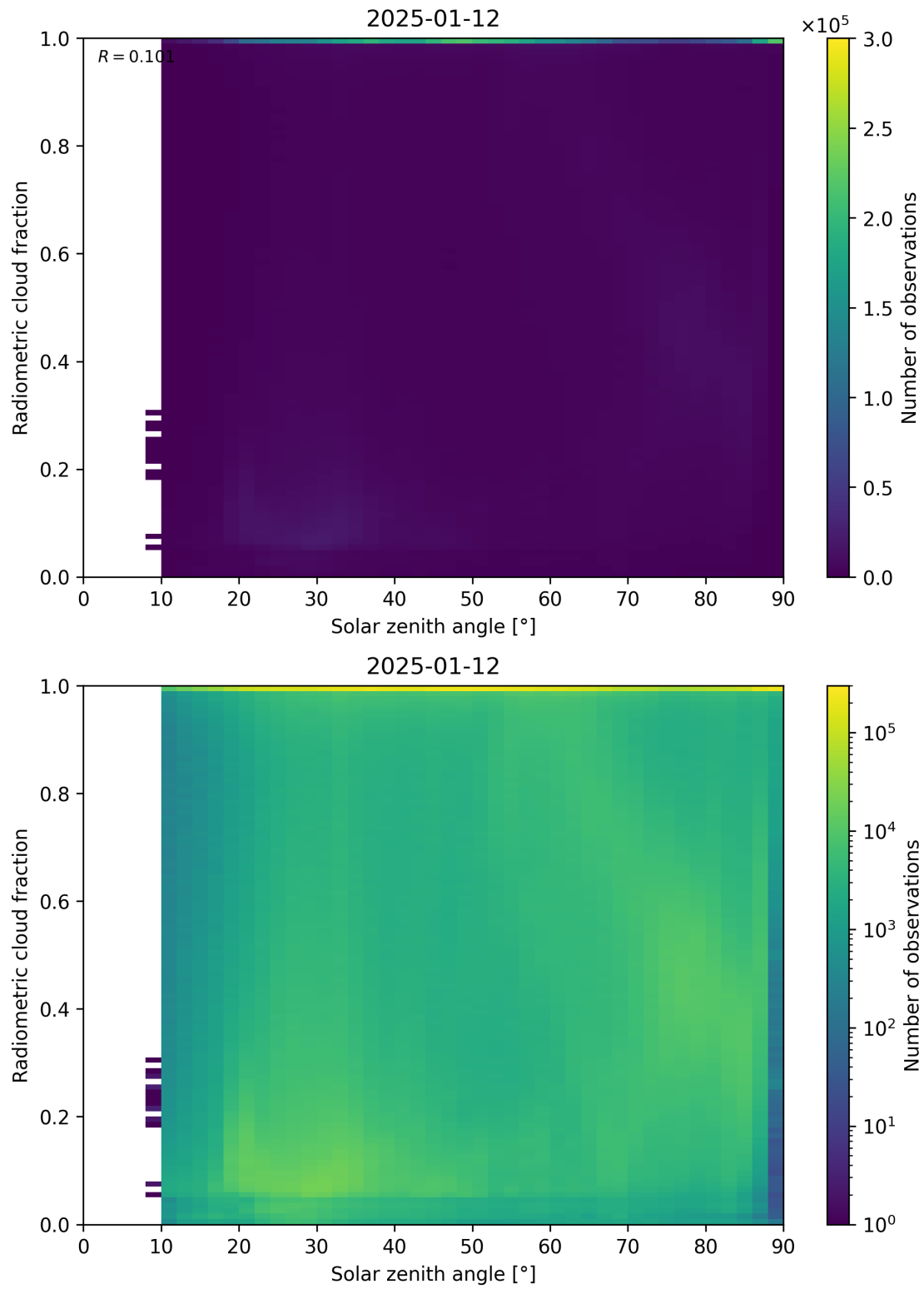
Figure 99: Scatter density plot of “Solar zenith angle” against “Radiometric cloud fraction” for 2025-01-12 to 2025-01-13.
