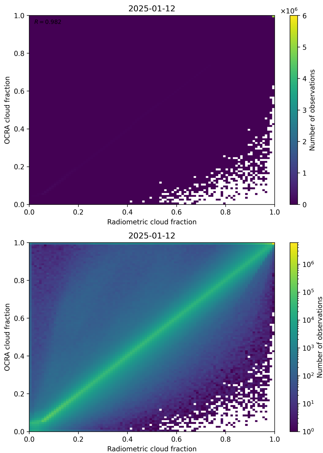
Figure 72: Scatter density plot of “Radiometric cloud fraction” against “OCRA cloud fraction” for 2025-01-12 to 2025-01-13.
