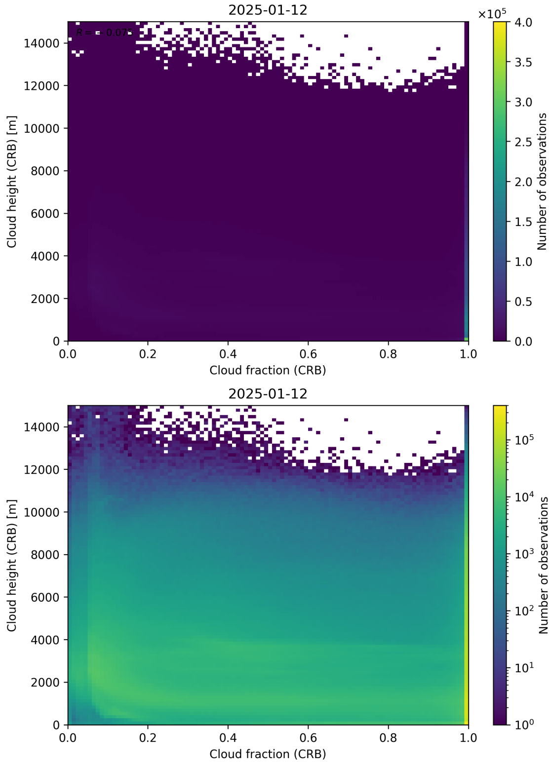
Figure 79: Scatter density plot of “Cloud fraction (CRB)” against “Cloud height (CRB)” for 2025-01-12 to 2025-01-13.
