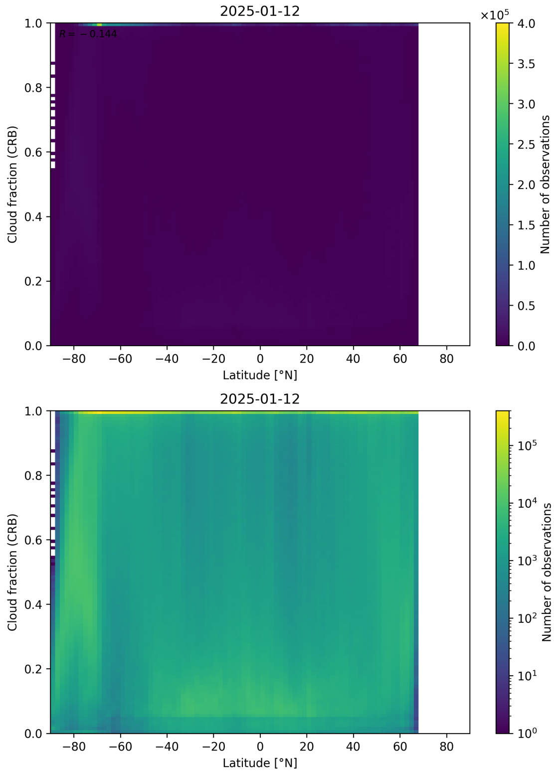
Figure 94: Scatter density plot of “Latitude” against “Cloud fraction (CRB)” for 2025-01-12 to 2025-01-13.
