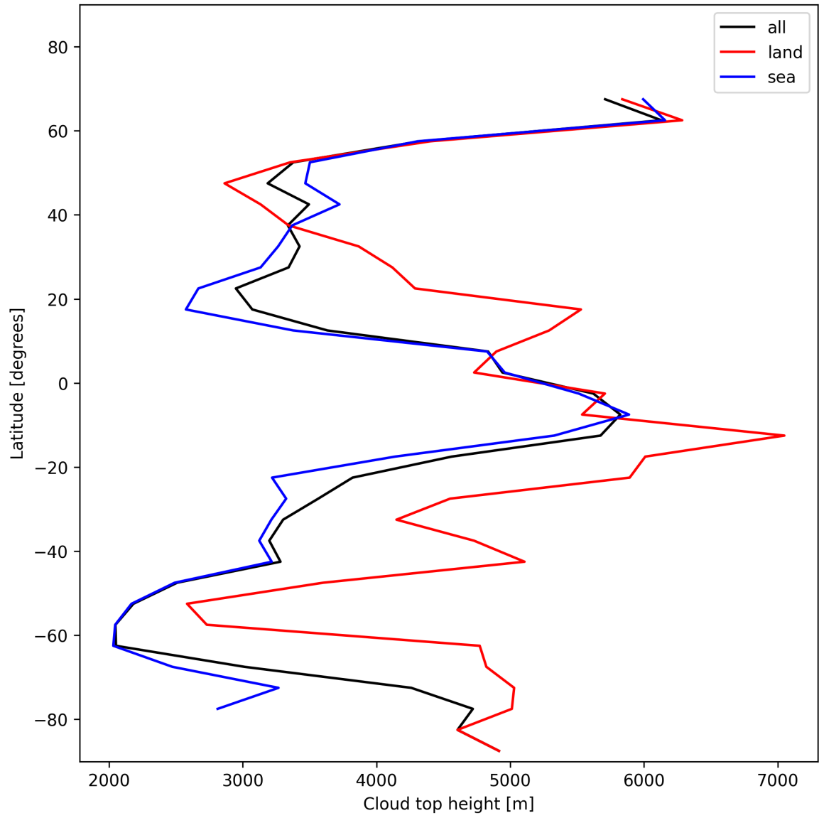
Figure 24: Zonal average of “Cloud top height” for 2025-01-12 to 2025-01-13.
