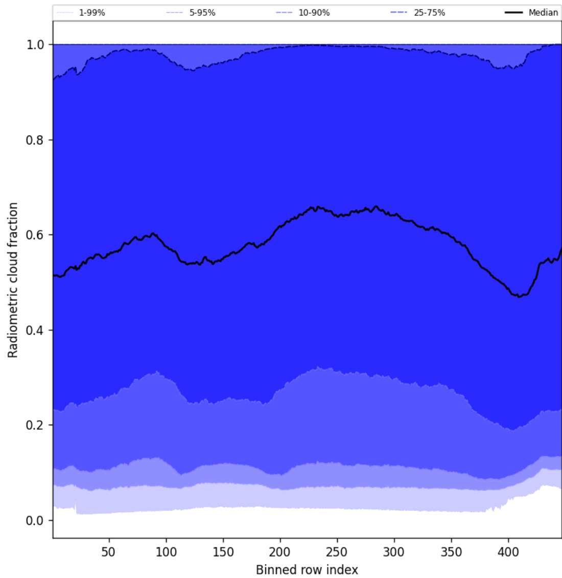
Figure 55: Along track statistics of “Radiometric cloud fraction” for 2025-01-12 to 2025-01-13
