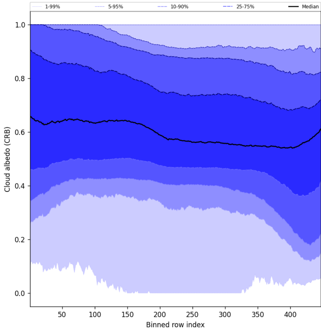
Figure 60: Along track statistics of “Cloud albedo (CRB)” for 2025-01-12 to 2025-01-13
