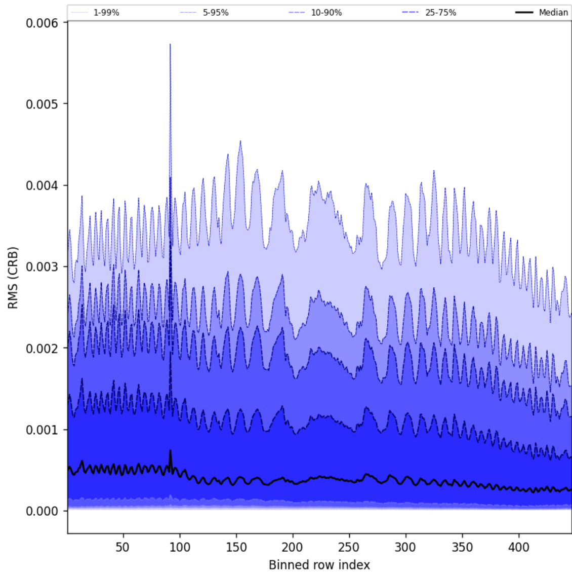
Figure 64: Along track statistics of “RMS (CRB)” for 2025-01-12 to 2025-01-13
