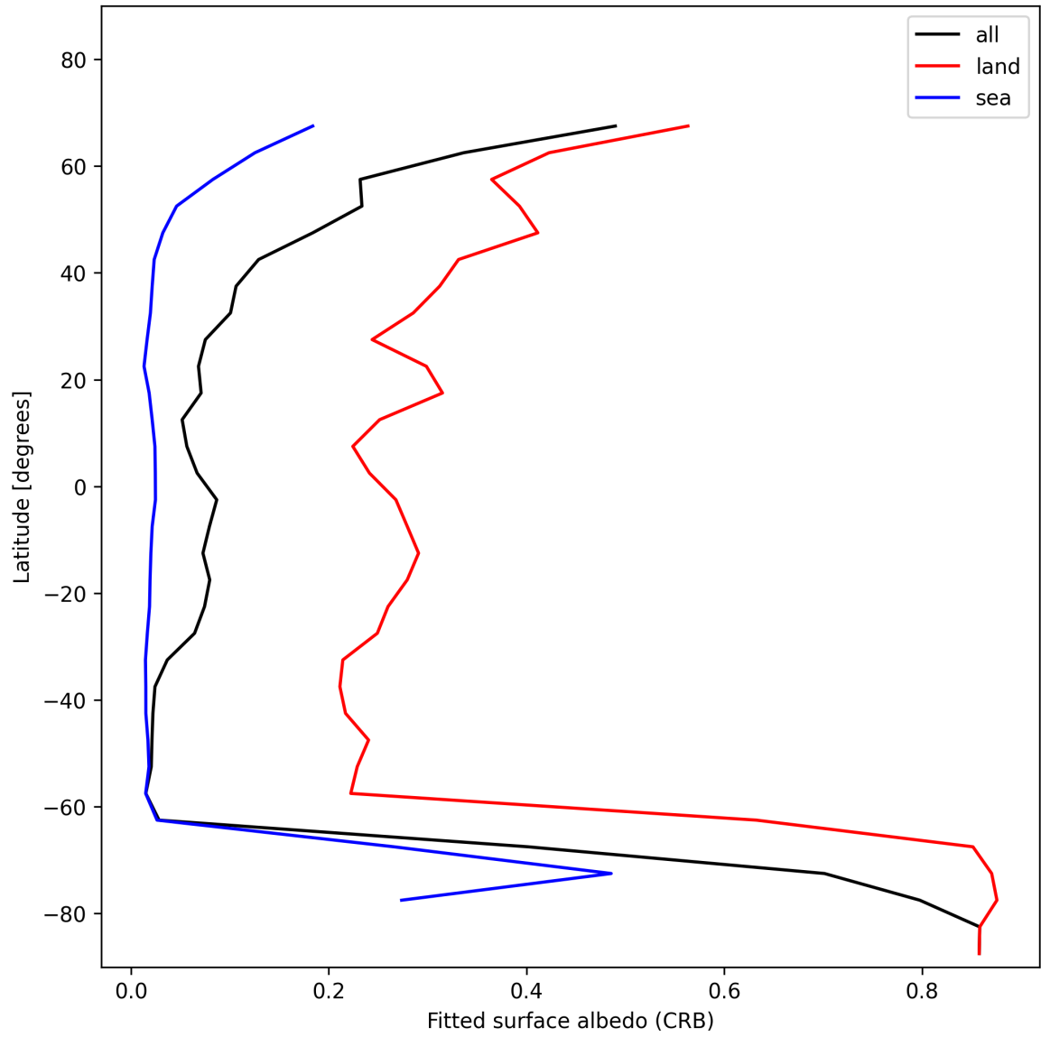
Figure 30: Zonal average of “Fitted surface albedo (CRB)” for 2025-01-12 to 2025-01-13.
