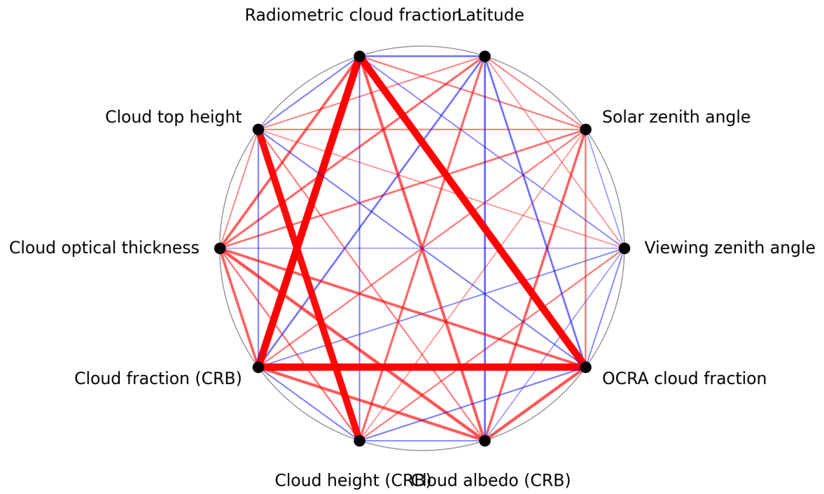
Figure 1: Map of correlation graph for 2025-01-12 to 2025-01-13.
