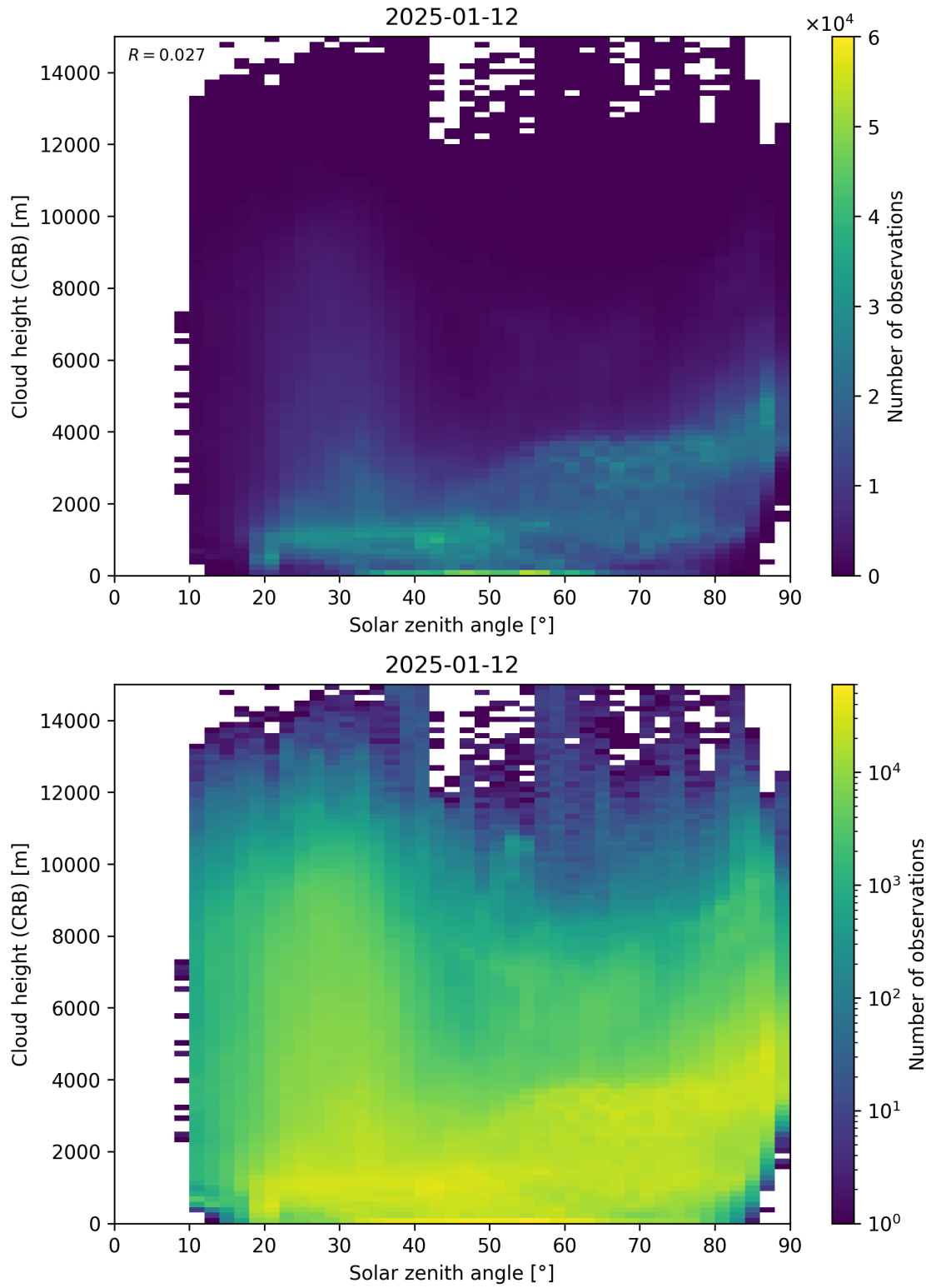
Figure 102: Scatter density plot of “Solar zenith angle” against “Cloud height (CRB)” for 2025-01-12 to 2025-01-13.
