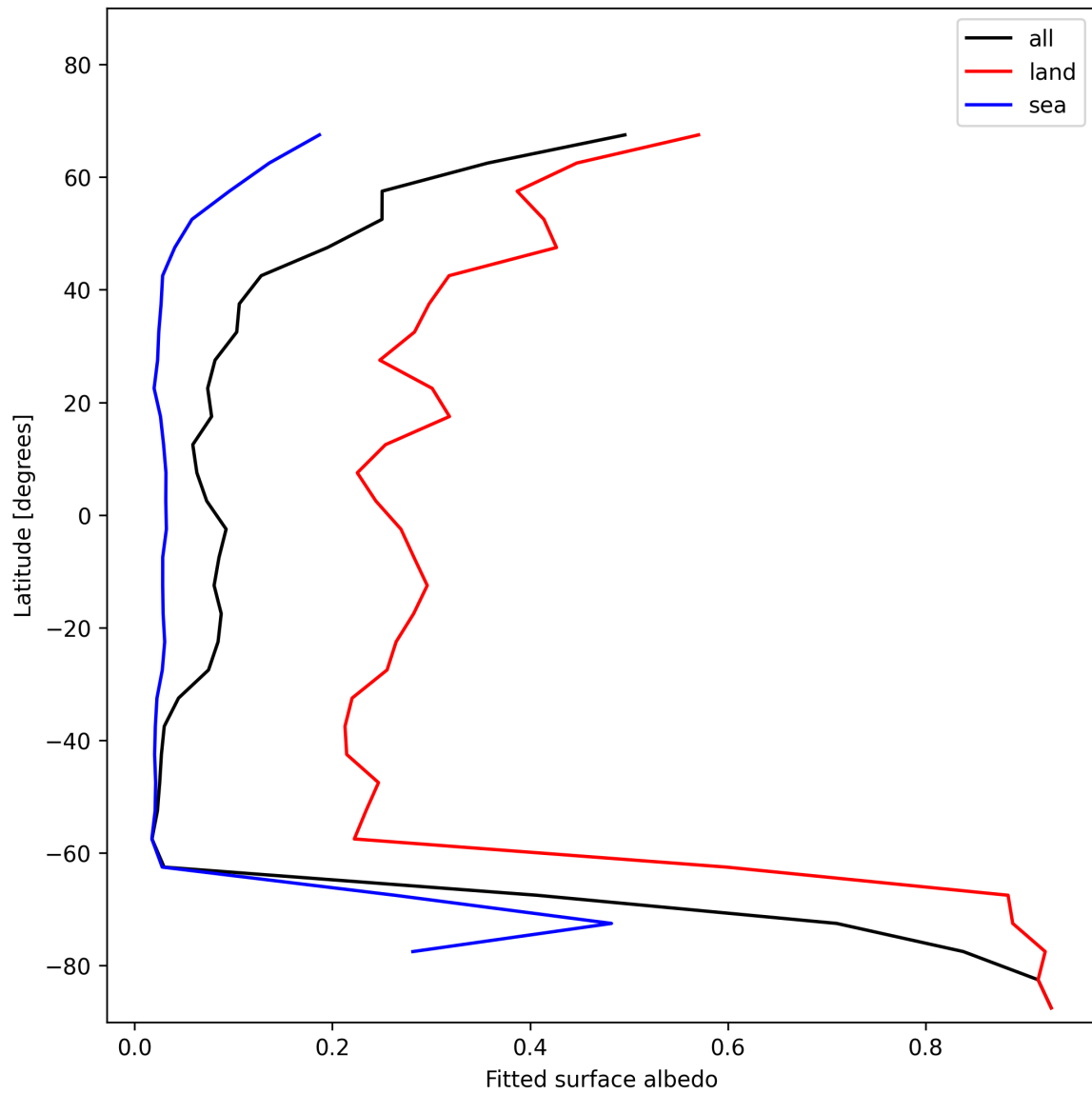
Figure 29: Zonal average of “Fitted surface albedo” for 2025-01-12 to 2025-01-13.
