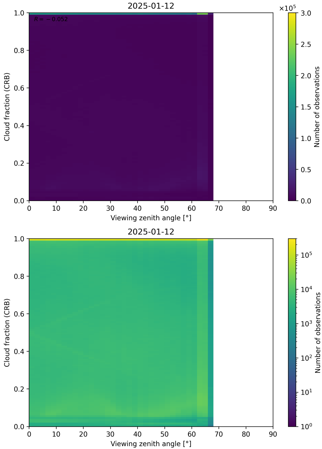
Figure 109: Scatter density plot of “Viewing zenith angle” against “Cloud fraction (CRB)” for 2025-01-12 to 2025-01-13.
