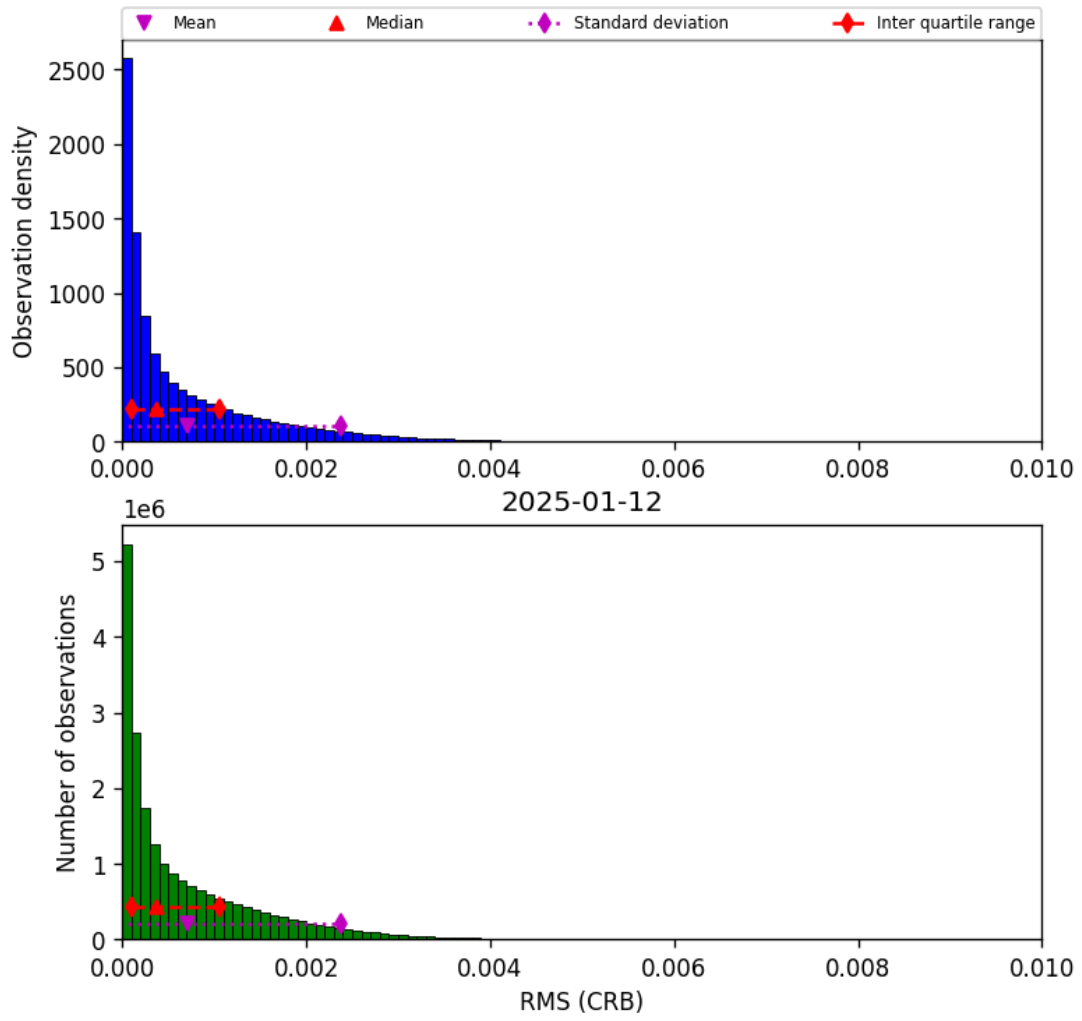
Figure 48: Histogram of “RMS (CRB)” for 2025-01-12 to 2025-01-13
