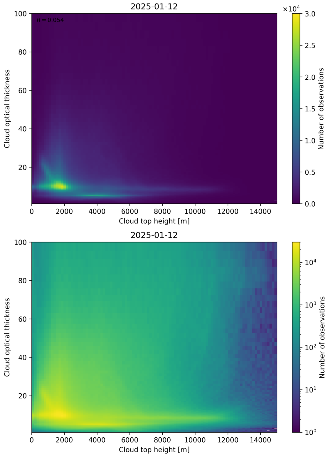
Figure 90: Scatter density plot of “Cloud top height” against “Cloud optical thickness” for 2025-01-12 to 2025-01-13.
