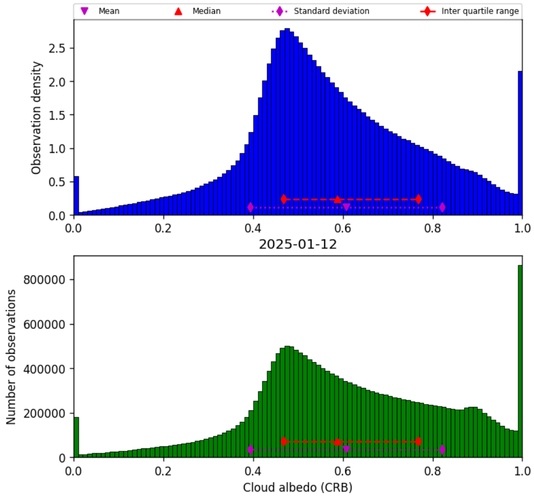
Figure 44: Histogram of “Cloud albedo (CRB)” for 2025-01-12 to 2025-01-13
