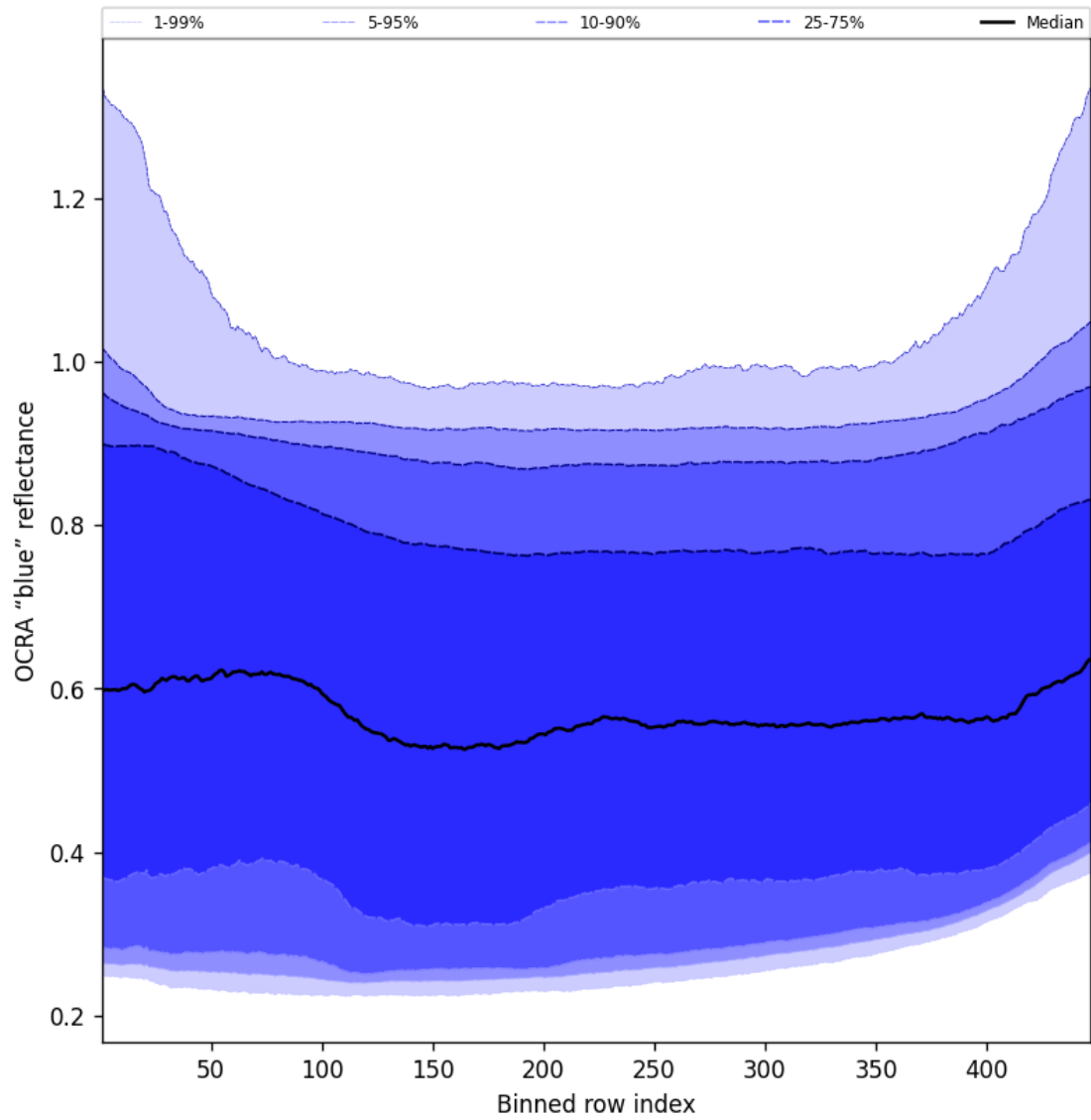
Figure 67: Along track statistics of “OCRA “blue” reflectance” for 2025-01-12 to 2025-01-13
