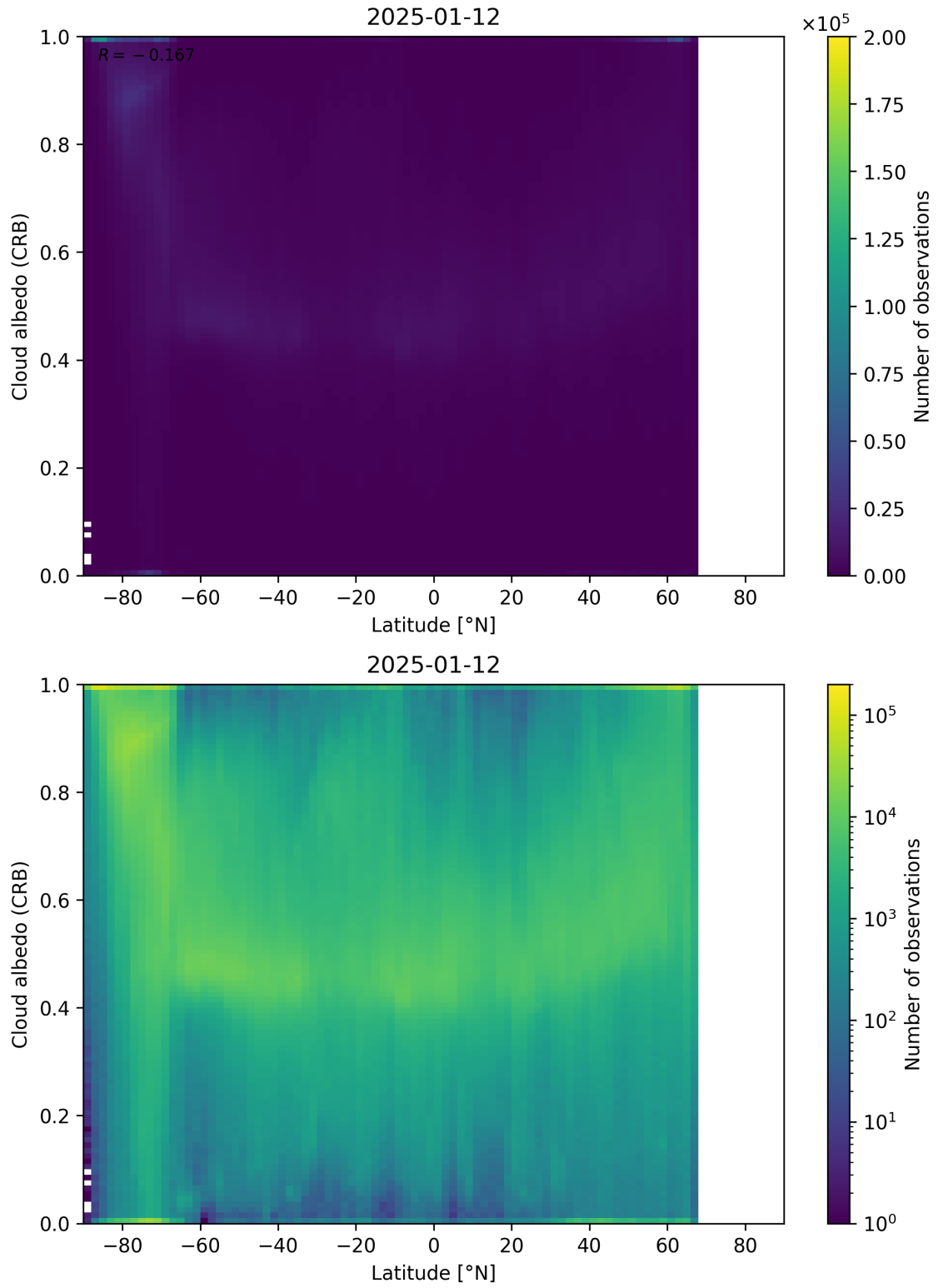
Figure 91: Scatter density plot of “Latitude” against “Cloud albedo (CRB)” for 2025-01-12 to 2025-01-13.
