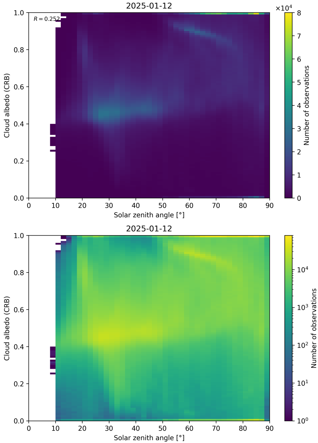
Figure 98: Scatter density plot of “Solar zenith angle” against “Cloud albedo (CRB)” for 2025-01-12 to 2025-01-13.
