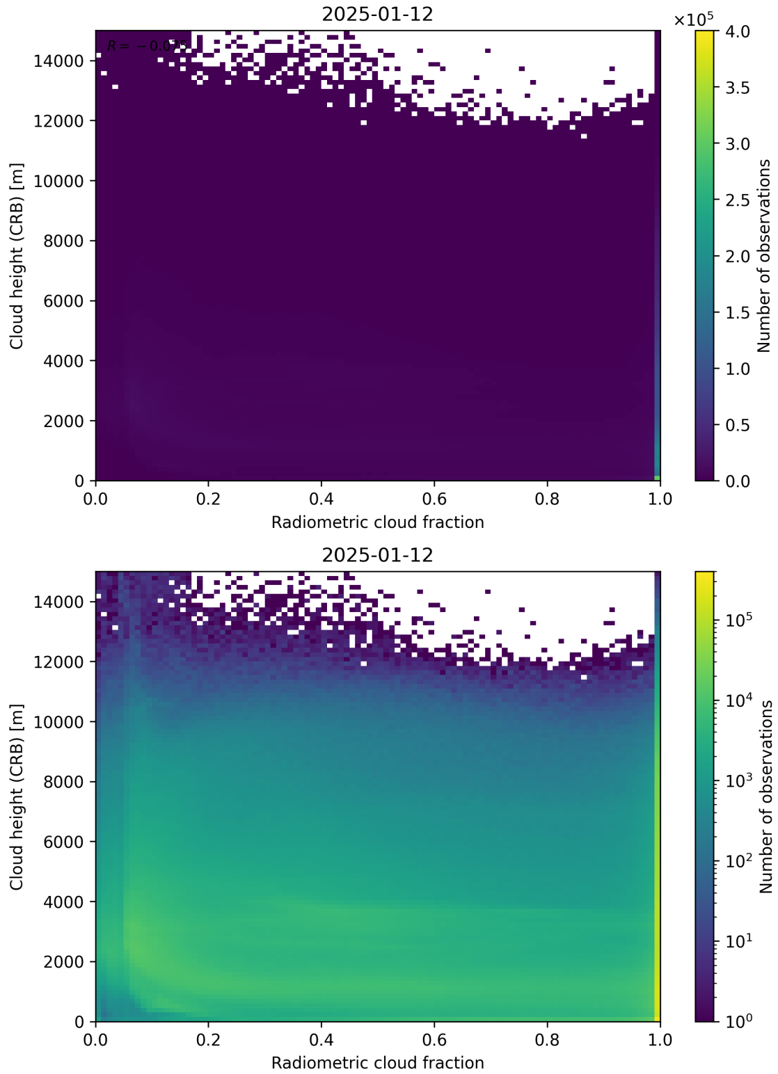
Figure 74: Scatter density plot of “Radiometric cloud fraction” against “Cloud height (CRB)” for 2025-01-12 to 2025-01-13.
