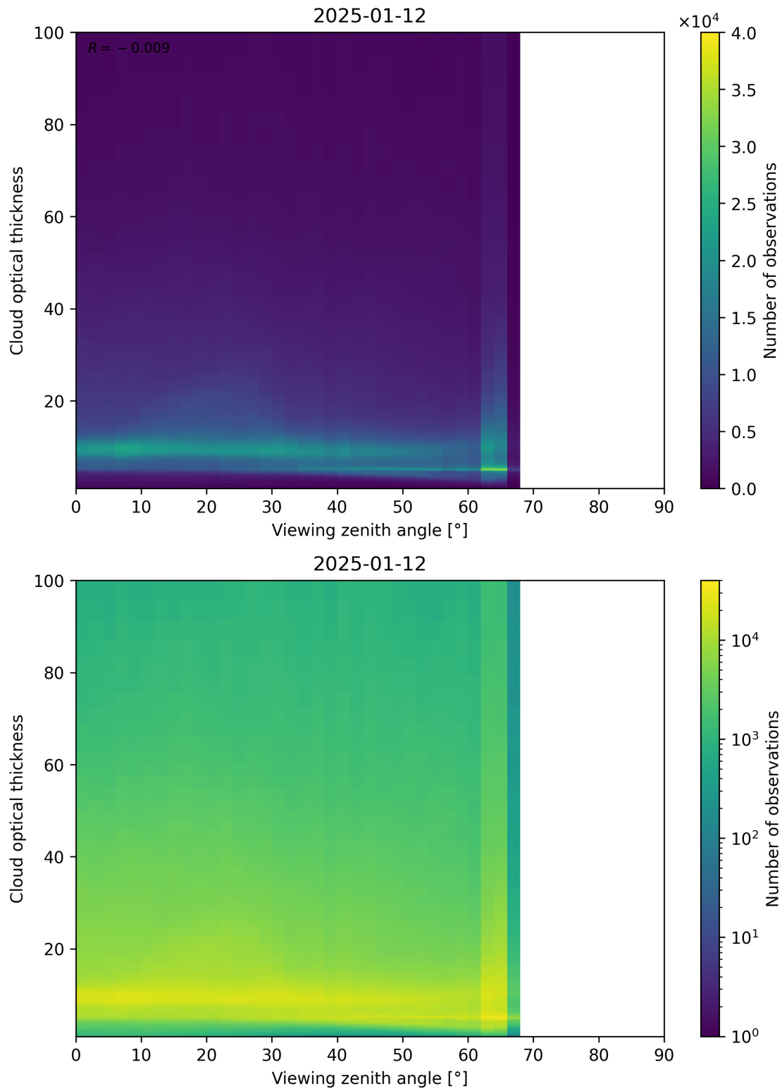
Figure 111: Scatter density plot of “Viewing zenith angle” against “Cloud optical thickness” for 2025-01-12 to 2025-01-13.
