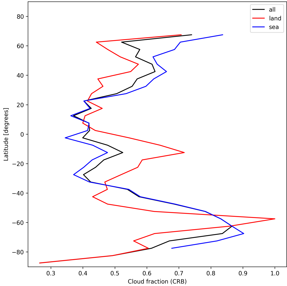
Figure 26: Zonal average of “Cloud fraction (CRB)” for 2025-01-12 to 2025-01-13.
