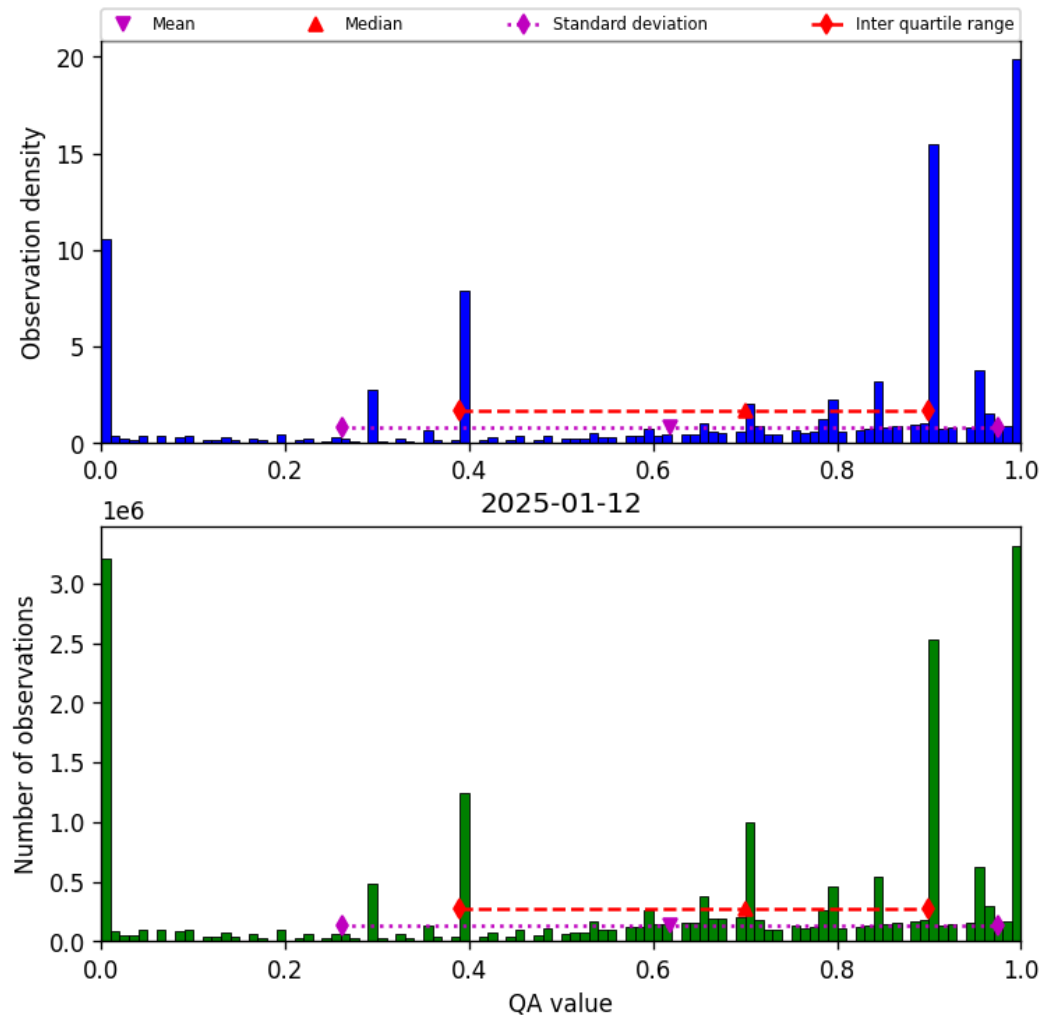
Figure 38: Histogram of “QA value” for 2025-01-12 to 2025-01-13
