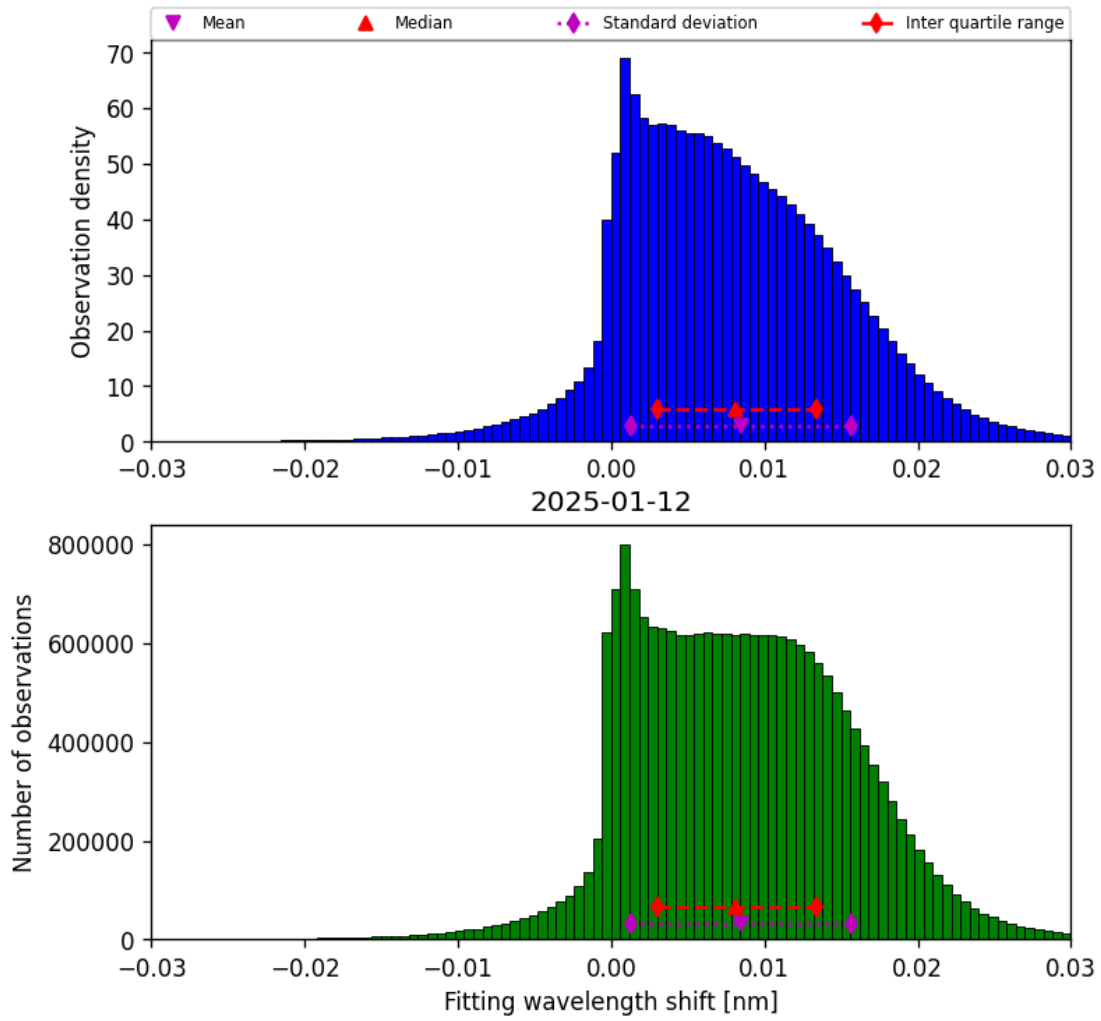
Figure 49: Histogram of “Fitting wavelength shift” for 2025-01-12 to 2025-01-13
