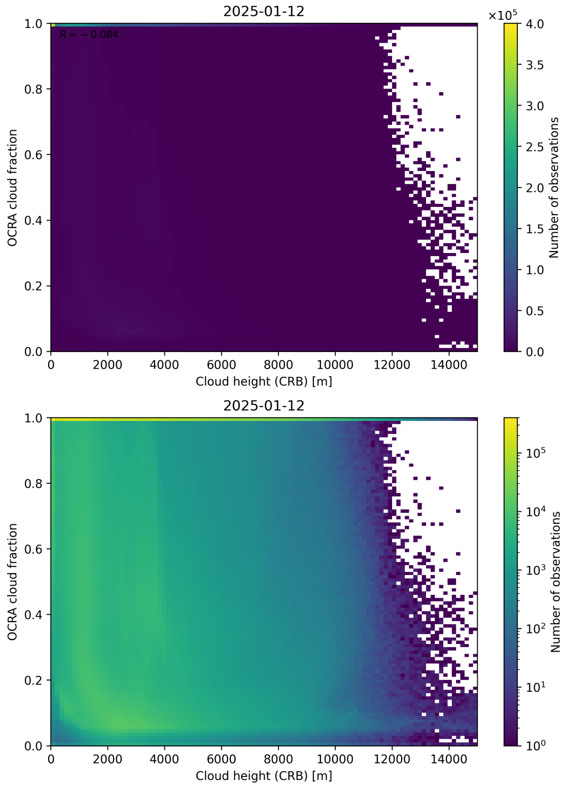
Figure 81: Scatter density plot of “Cloud height (CRB)” against “OCRA cloud fraction” for 2025-01-12 to 2025-01-13.
