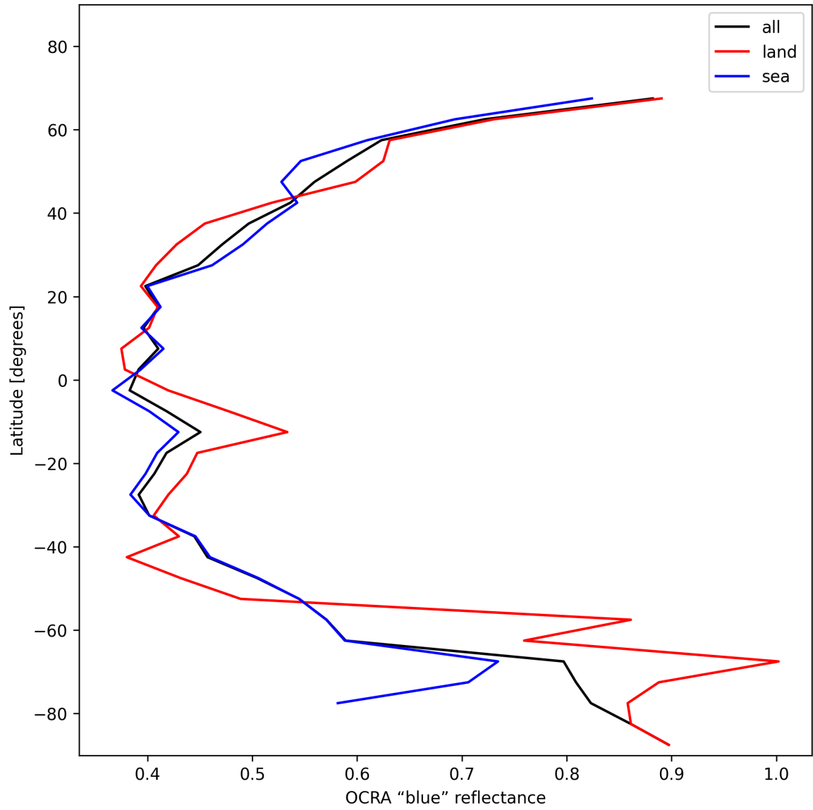
Figure 35: Zonal average of "OCRA "blue" reflectance" for 2025-01-12 to 2025-01-13.
