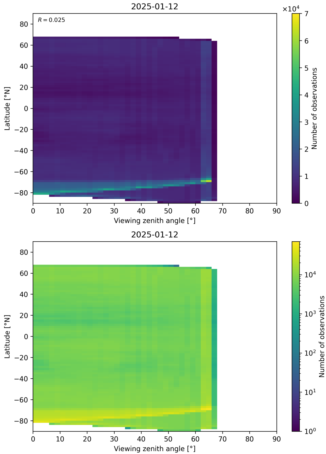
Figure 113: Scatter density plot of “Viewing zenith angle” against “Latitude” for 2025-01-12 to 2025-01-13.
