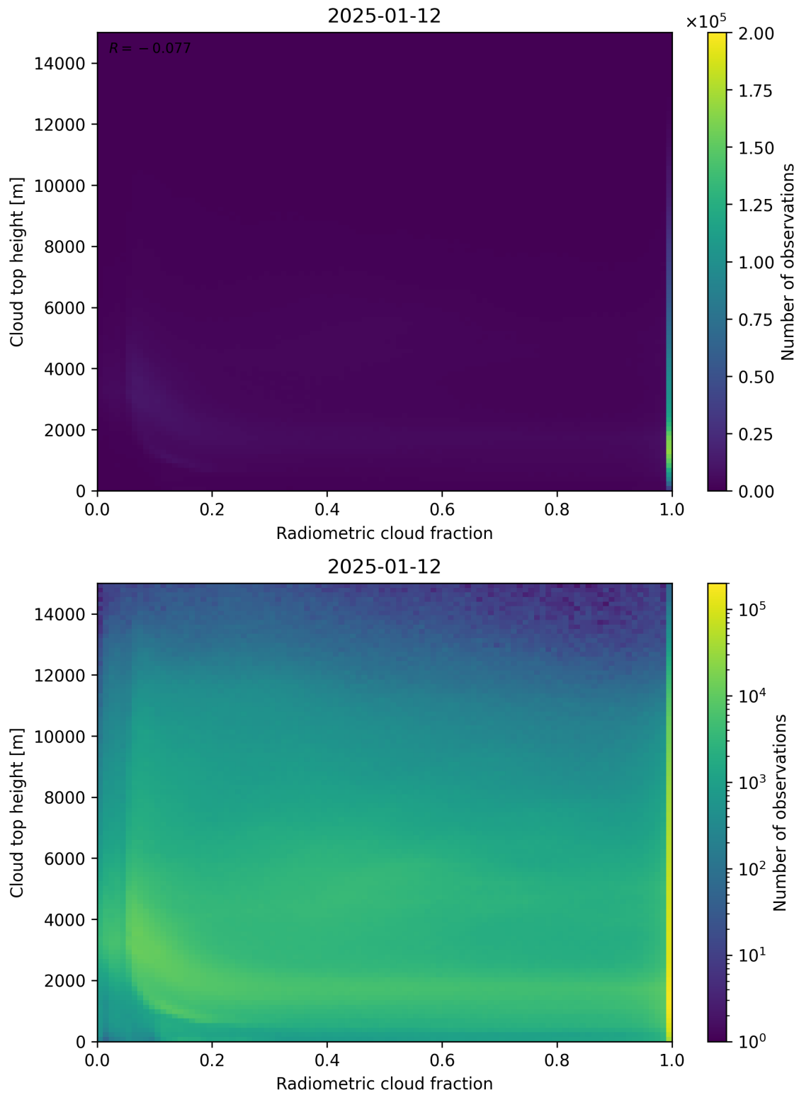
Figure 76: Scatter density plot of “Radiometric cloud fraction” against “Cloud top height” for 2025-01-12 to 2025-01-13.
