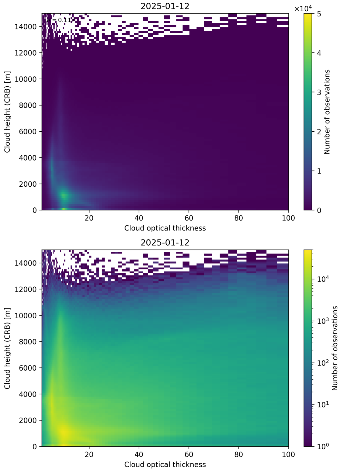
Figure 85: Scatter density plot of “Cloud optical thickness” against “Cloud height (CRB)” for 2025-01-12 to 2025-01-13.
