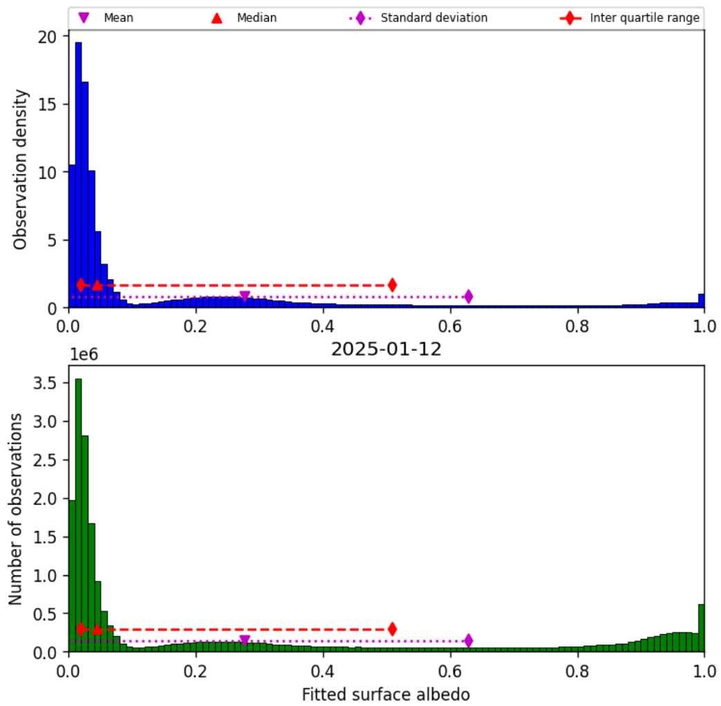
Figure 45: Histogram of “Fitted surface albedo” for 2025-01-12 to 2025-01-13
