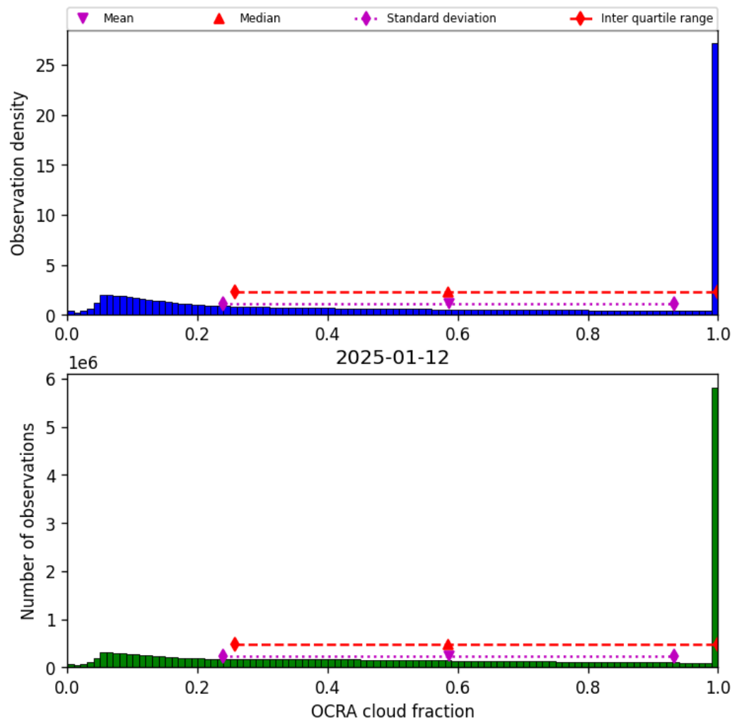
Figure 50: Histogram of “OCRA cloud fraction” for 2025-01-12 to 2025-01-13
