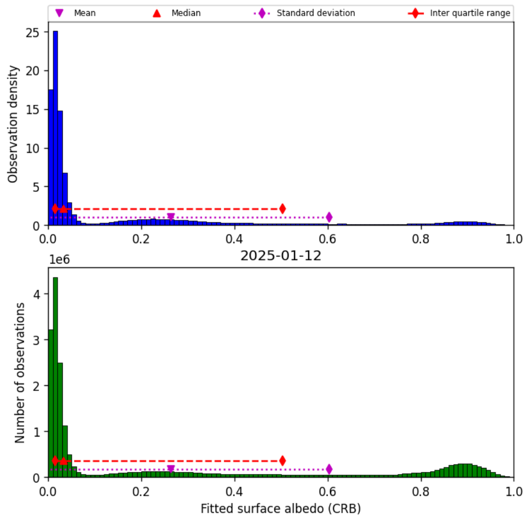
Figure 46: Histogram of “Fitted surface albedo (CRB)” for 2025-01-12 to 2025-01-13
