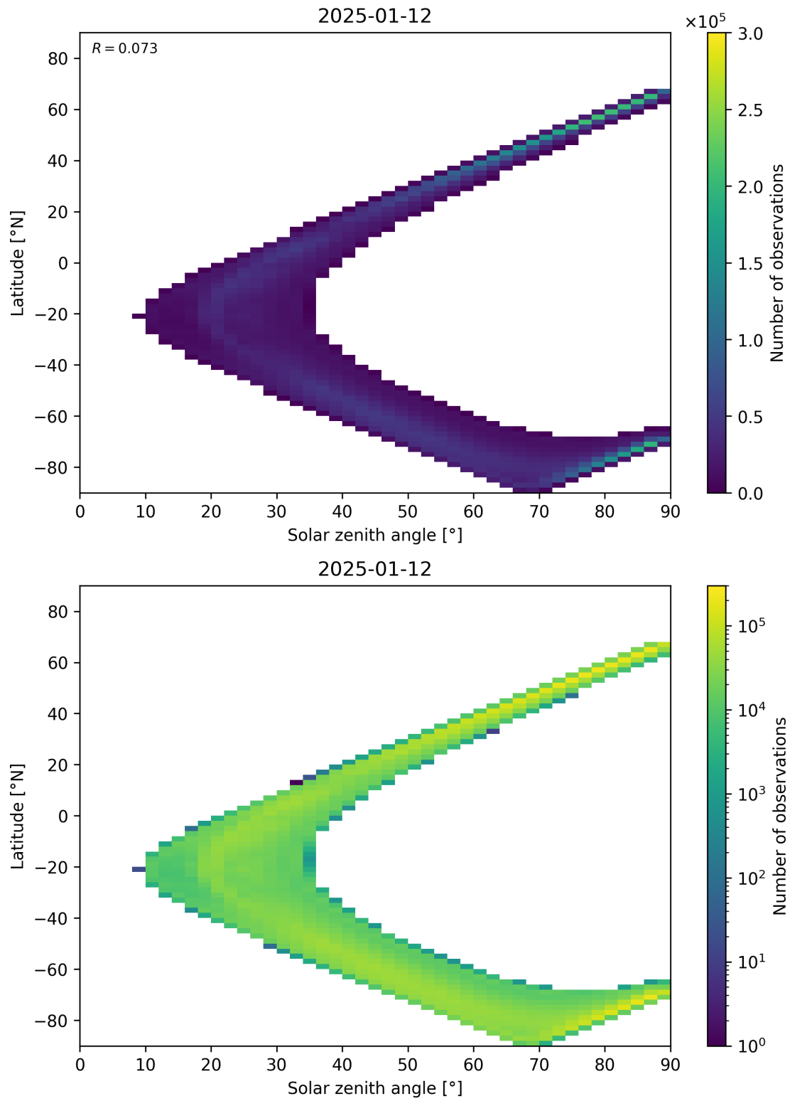
Figure 105: Scatter density plot of “Solar zenith angle” against “Latitude” for 2025-01-12 to 2025-01-13.
