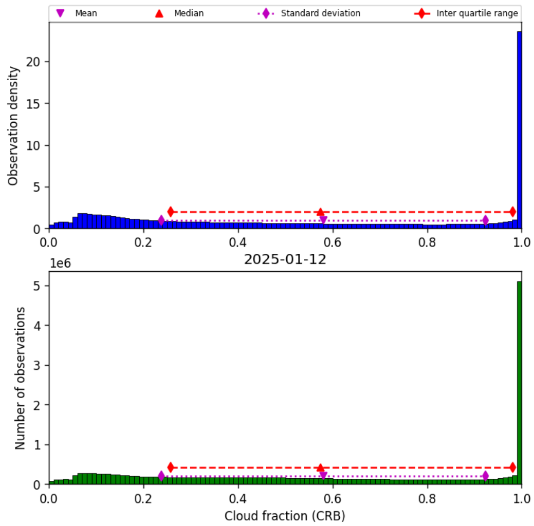
Figure 42: Histogram of “Cloud fraction (CRB)” for 2025-01-12 to 2025-01-13
