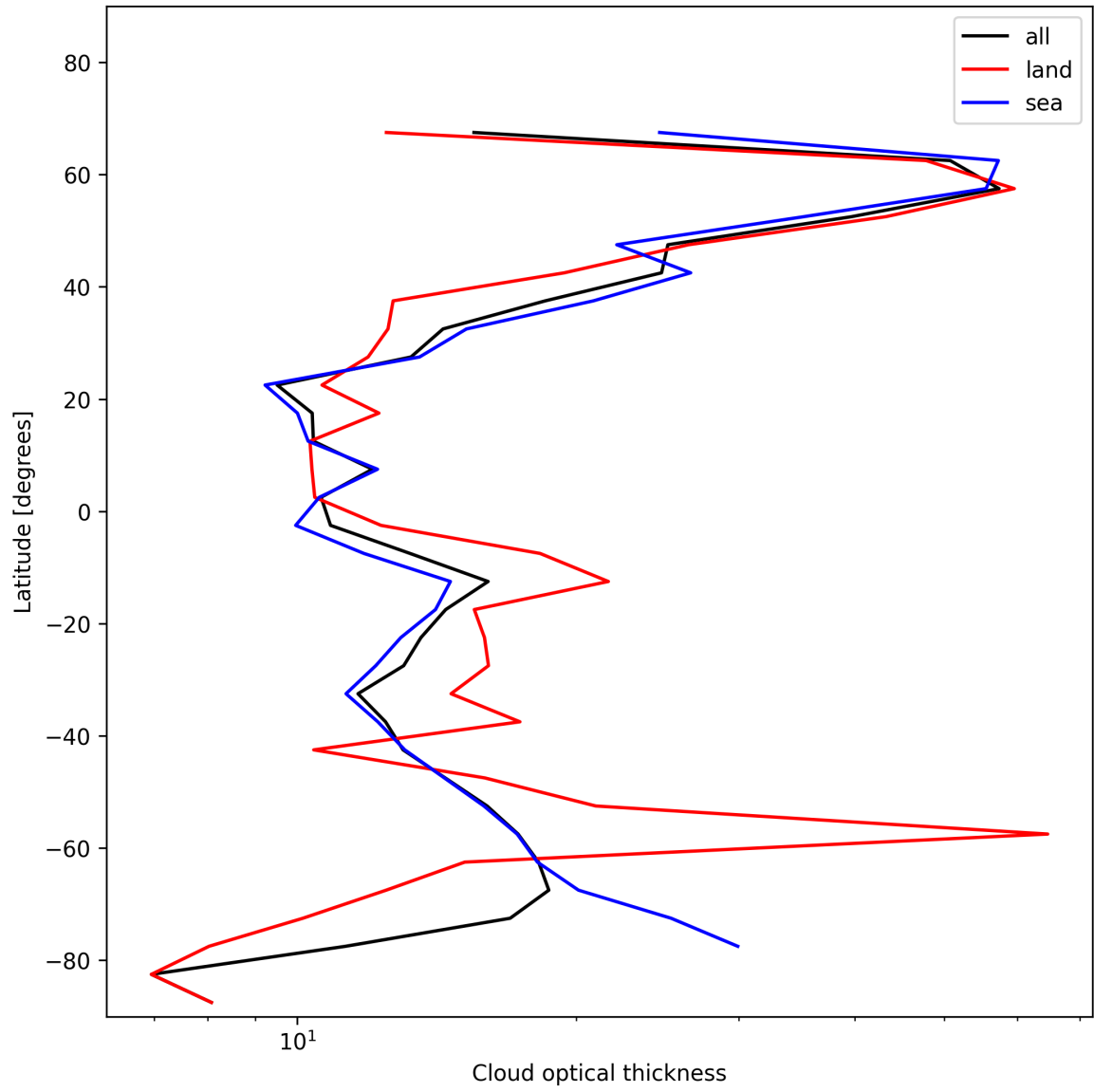
Figure 25: Zonal average of “Cloud optical thickness” for 2025-01-12 to 2025-01-13.
