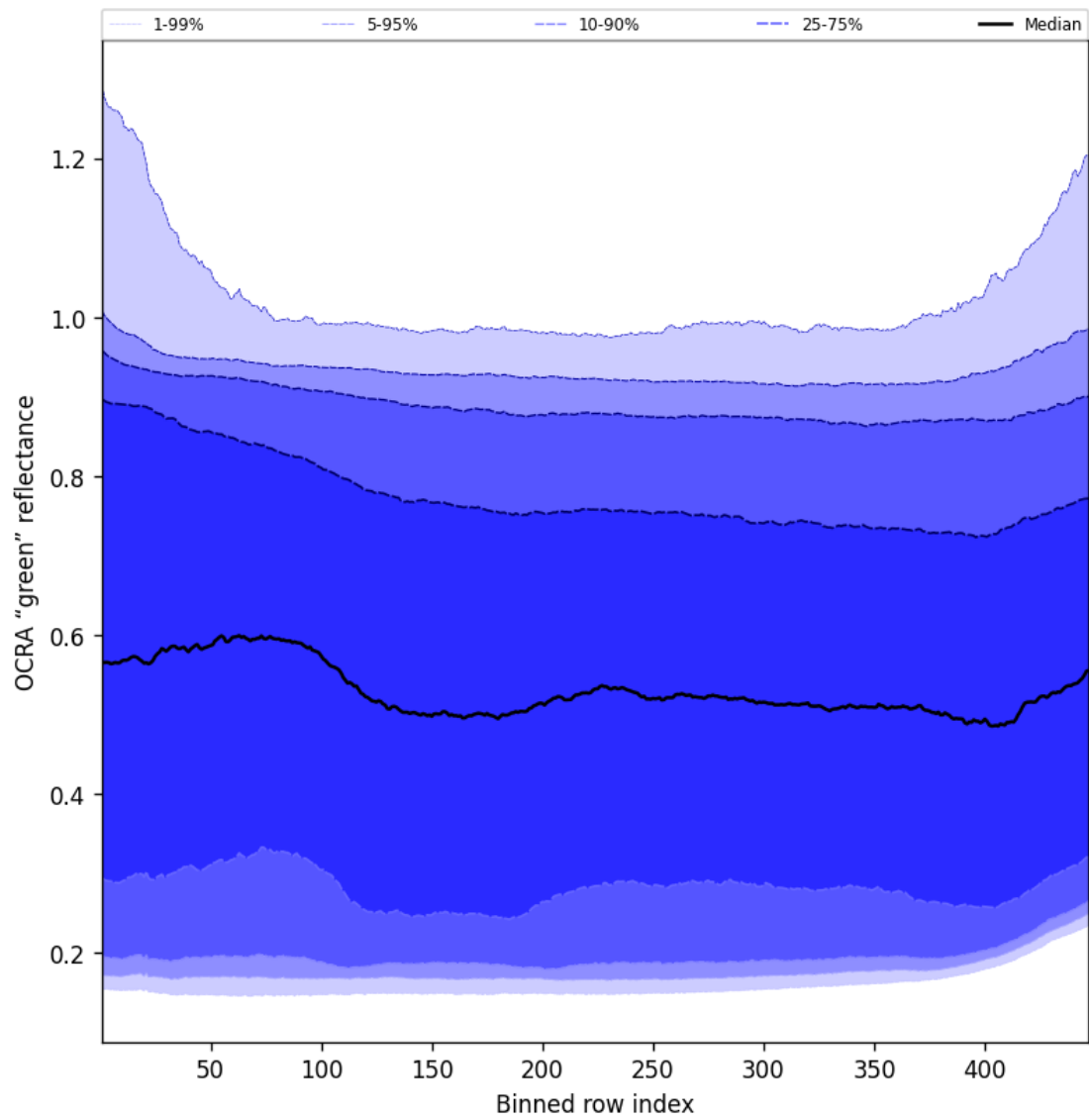
Figure 68: Along track statistics of “OCRA “green” reflectance” for 2025-01-12 to 2025-01-13
