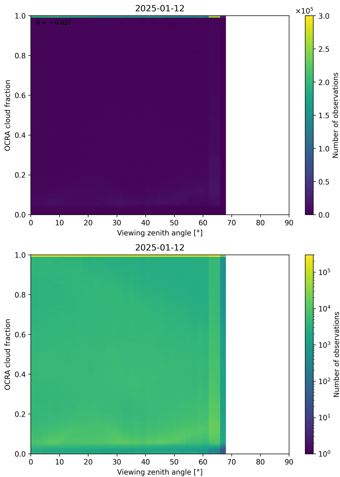
Figure 108: Scatter density plot of “Viewing zenith angle” against “OCRA cloud fraction” for 2025-01-12 to 2025-01-13.
