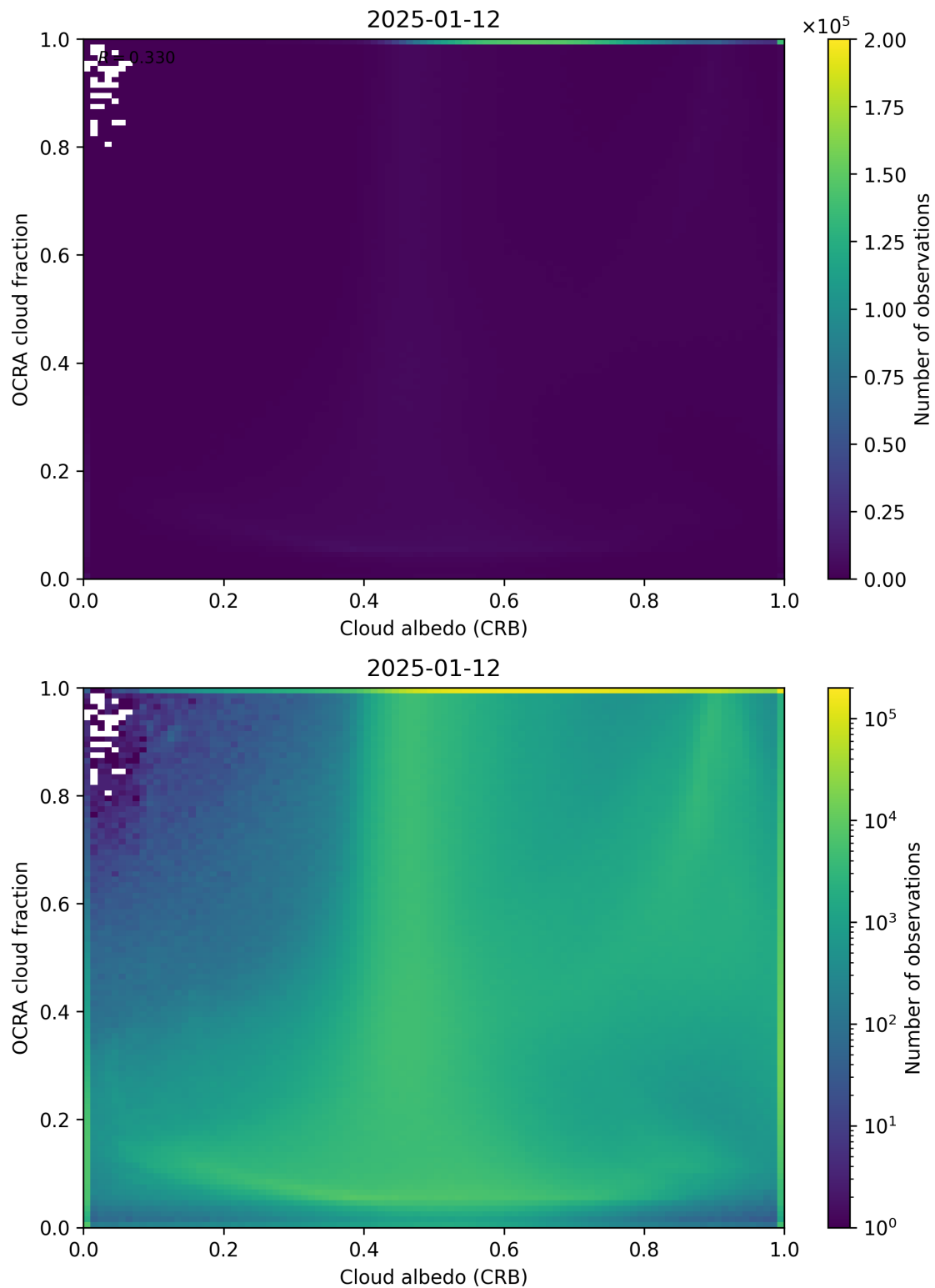
Figure 70: Scatter density plot of “Cloud albedo (CRB)” against “OCRA cloud fraction” for 2025-01-12 to 2025-01-13.
