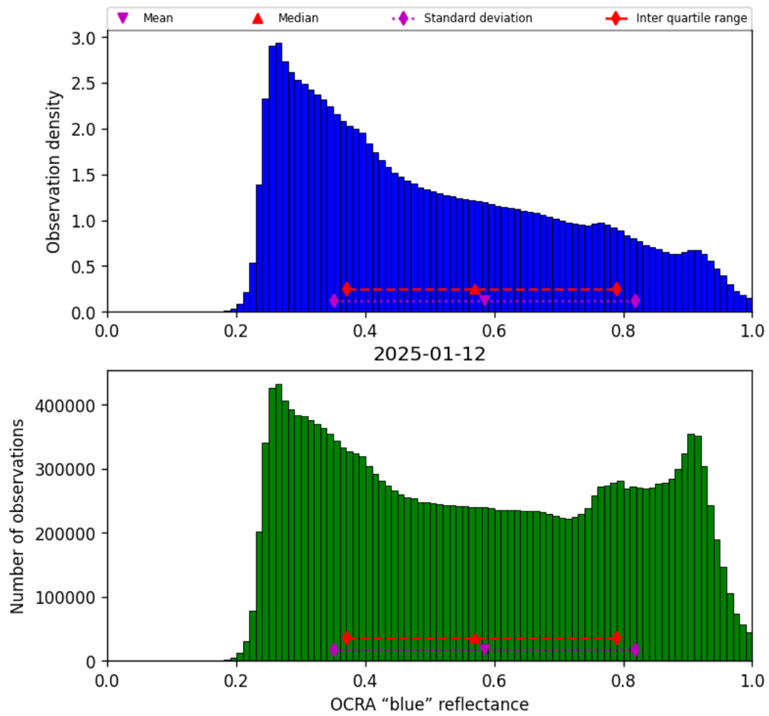
Figure 51: Histogram of “OCRA “blue” reflectance” for 2025-01-12 to 2025-01-13
