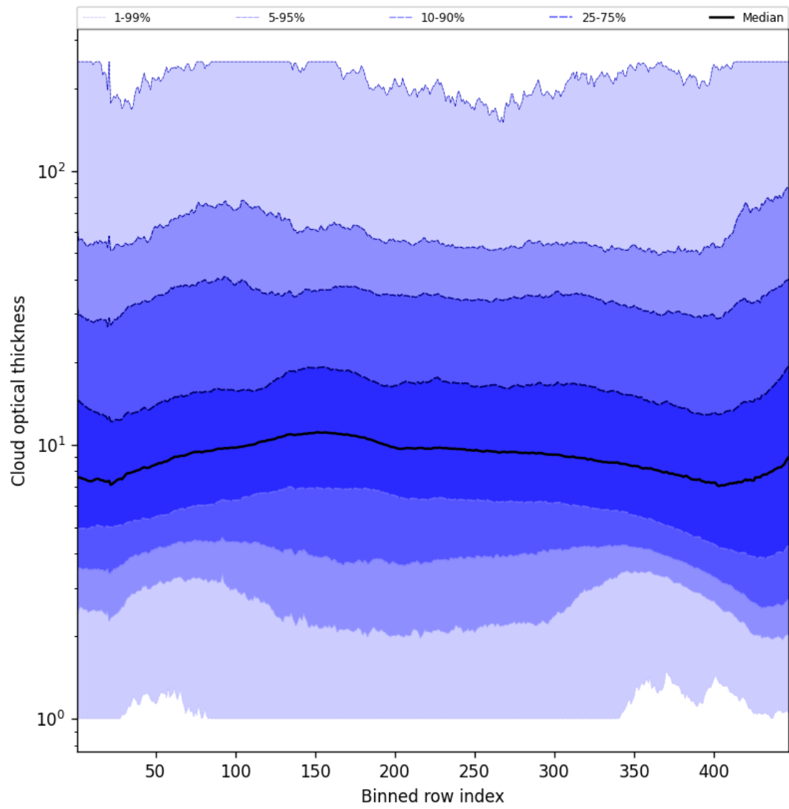
Figure 57: Along track statistics of “Cloud optical thickness” for 2025-01-12 to 2025-01-13
