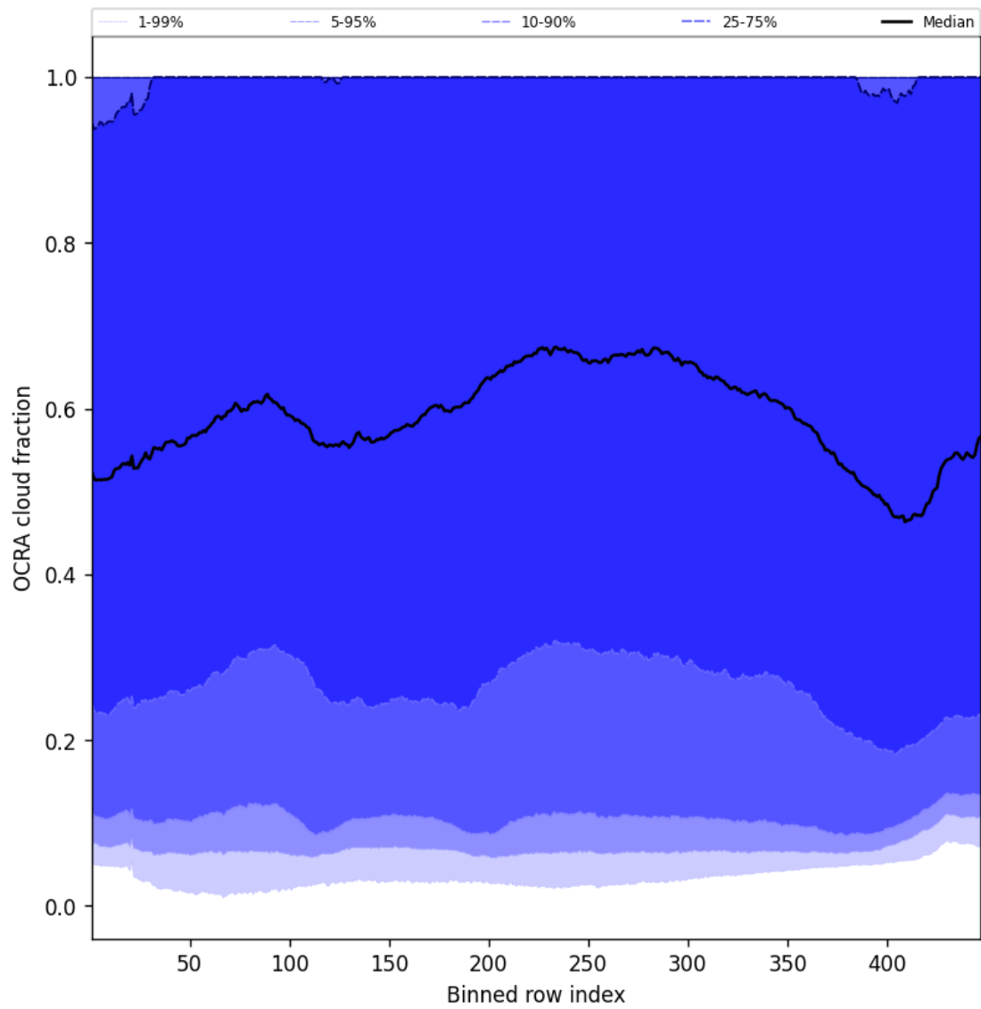
Figure 66: Along track statistics of “OCRA cloud fraction” for 2025-01-12 to 2025-01-13
