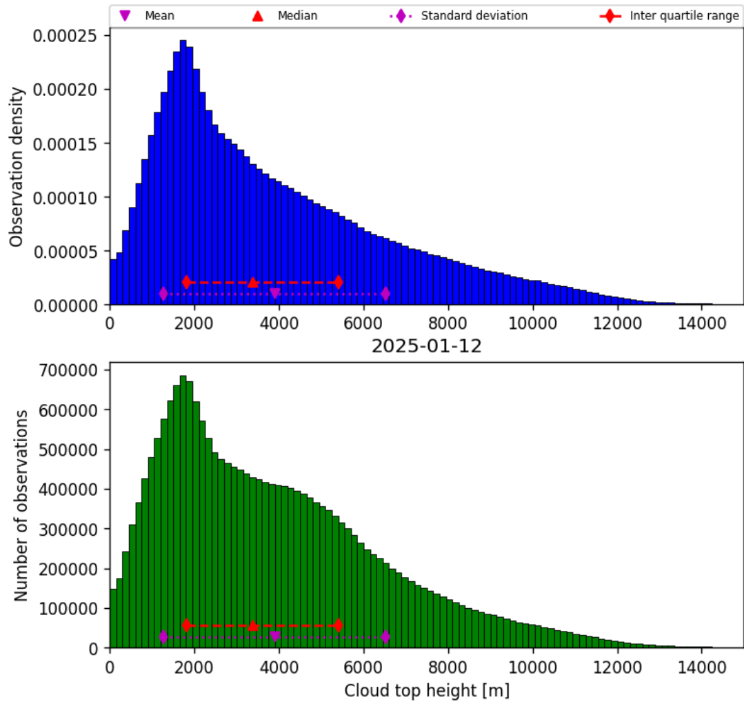
Figure 40: Histogram of “Cloud top height” for 2025-01-12 to 2025-01-13
