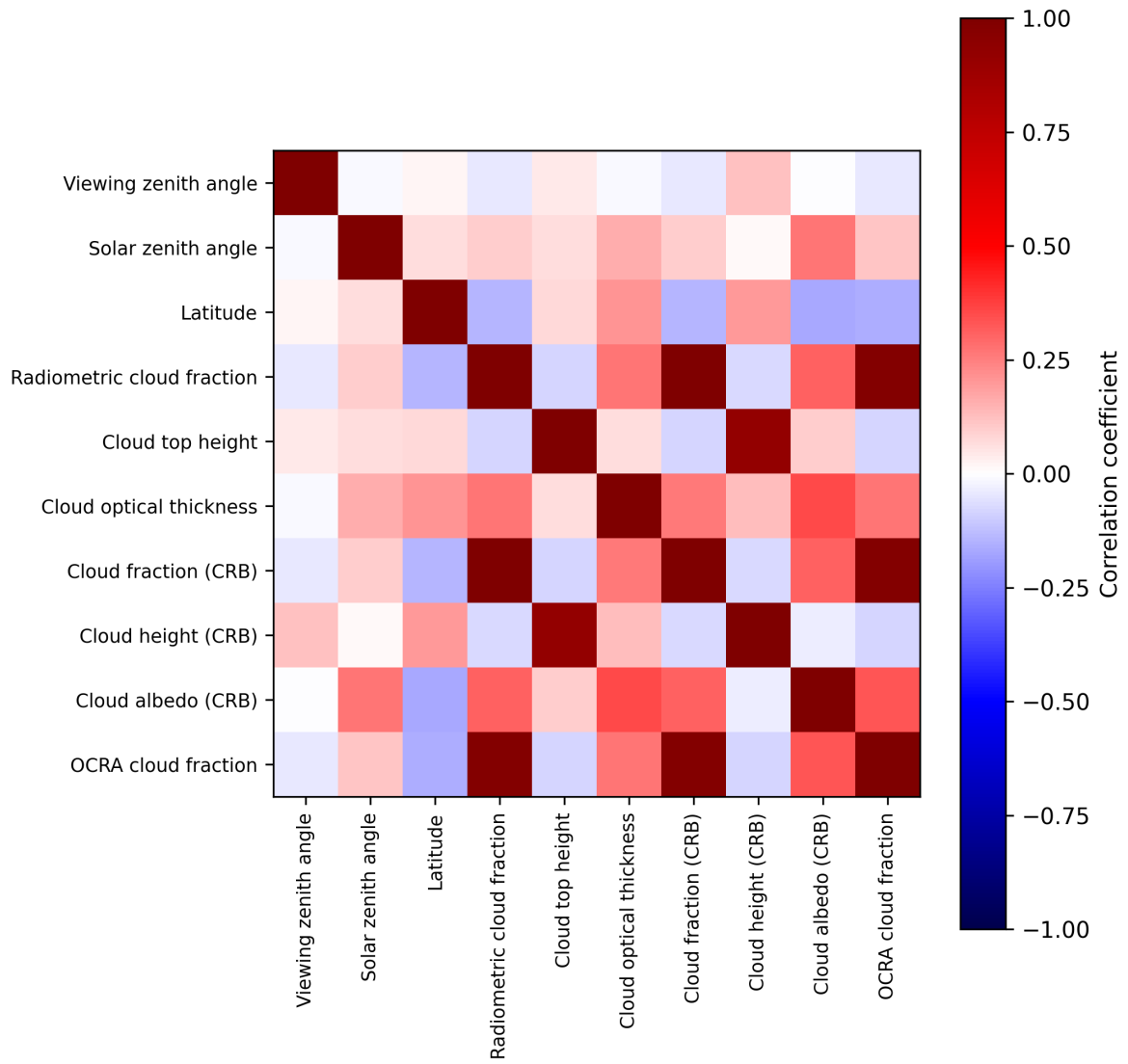
Figure 2: Map of correlation matrix for 2025-01-12 to 2025-01-14.
