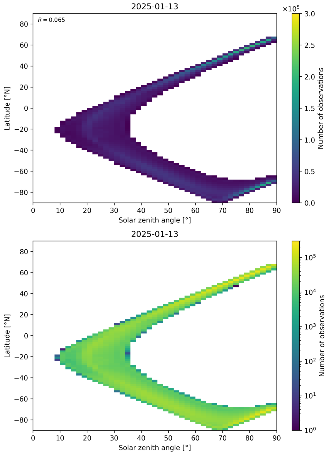
Figure 105: Scatter density plot of “Solar zenith angle” against “Latitude” for 2025-01-12 to 2025-01-14.
