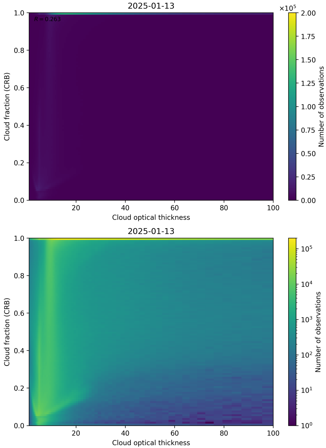
Figure 84: Scatter density plot of “Cloud optical thickness” against “Cloud fraction (CRB)” for 2025-01-12 to 2025-01-14.
