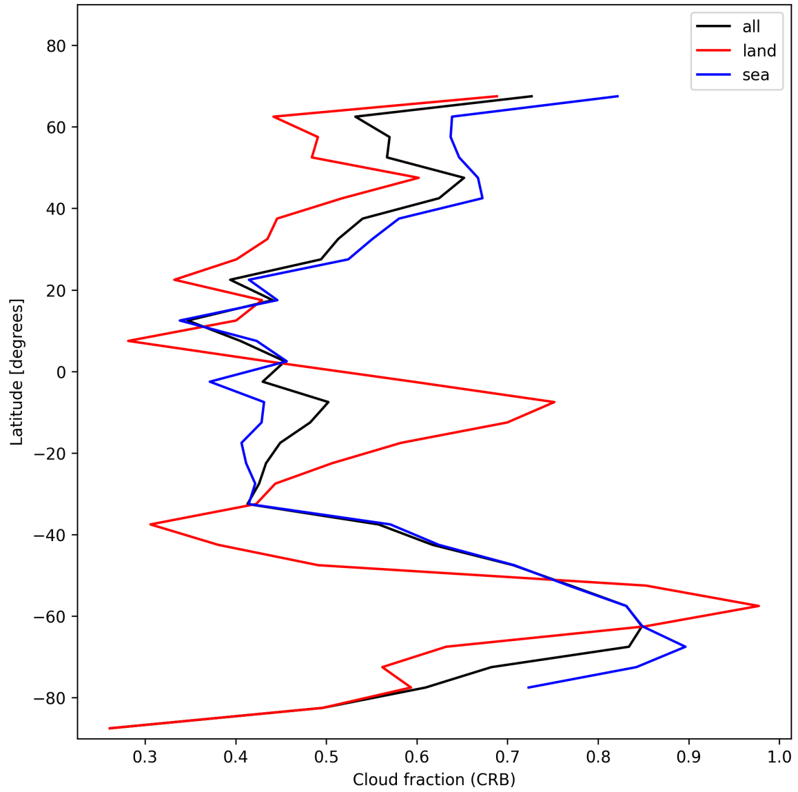
Figure 26: Zonal average of “Cloud fraction (CRB)” for 2025-01-12 to 2025-01-14.
