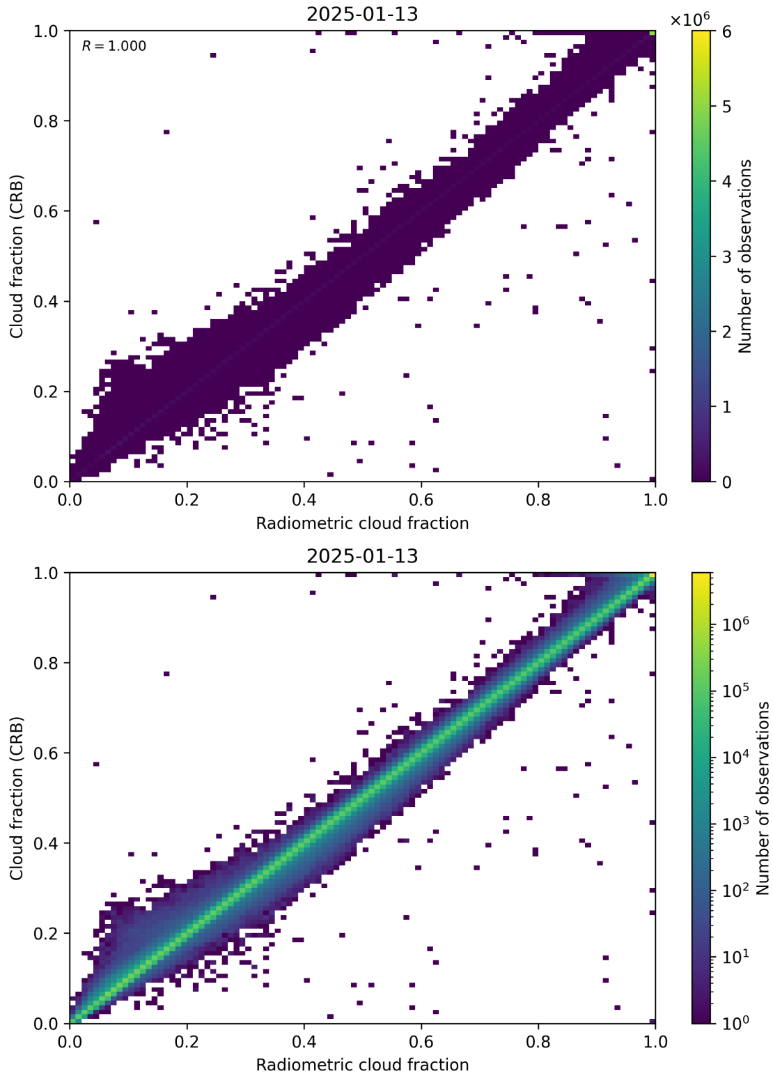
Figure 73: Scatter density plot of “Radiometric cloud fraction” against “Cloud fraction (CRB)” for 2025-01-12 to 2025-01-14.
