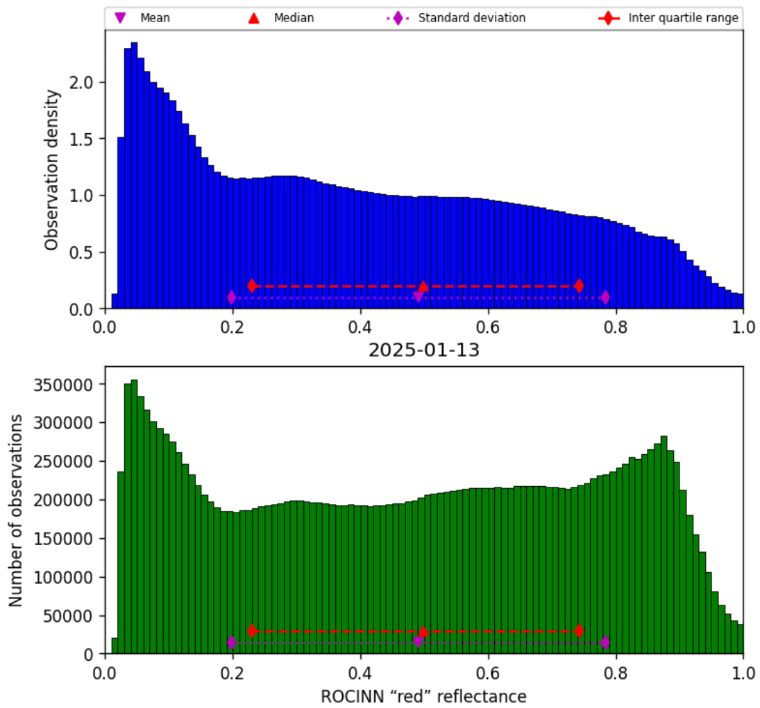
Figure 53: Histogram of “ROCINN “red” reflectance” for 2025-01-12 to 2025-01-14
