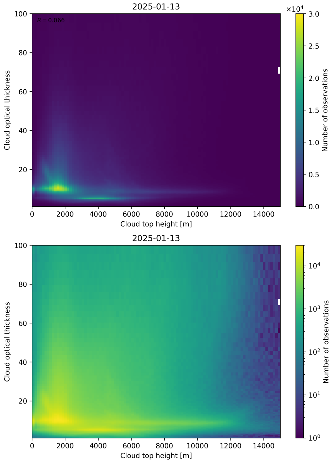
Figure 90: Scatter density plot of “Cloud top height” against “Cloud optical thickness” for 2025-01-12 to 2025-01-14.
