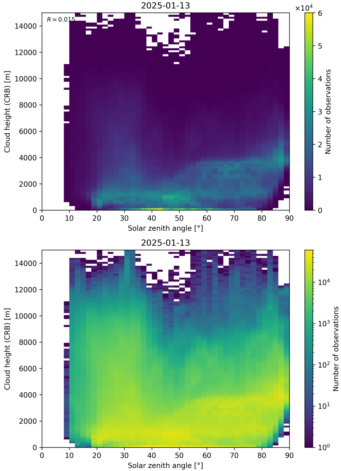
Figure 102: Scatter density plot of “Solar zenith angle” against “Cloud height (CRB)” for 2025-01-12 to 2025-01-14.
