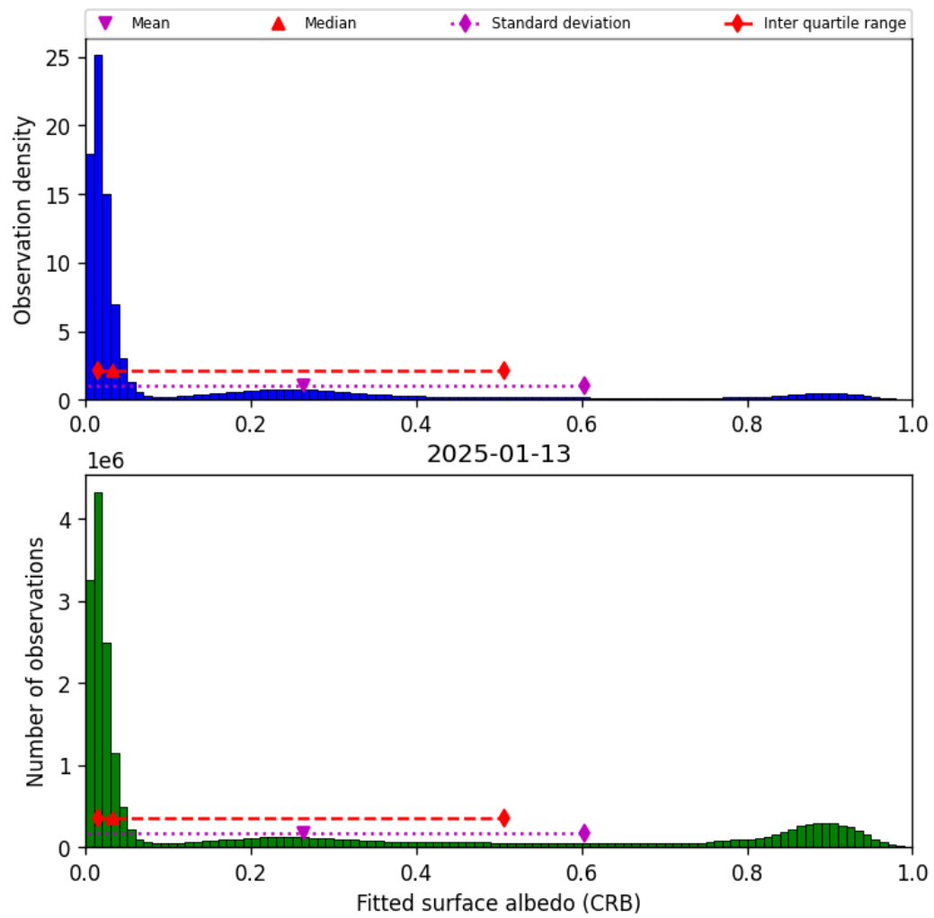
Figure 46: Histogram of “Fitted surface albedo (CRB)” for 2025-01-12 to 2025-01-14
