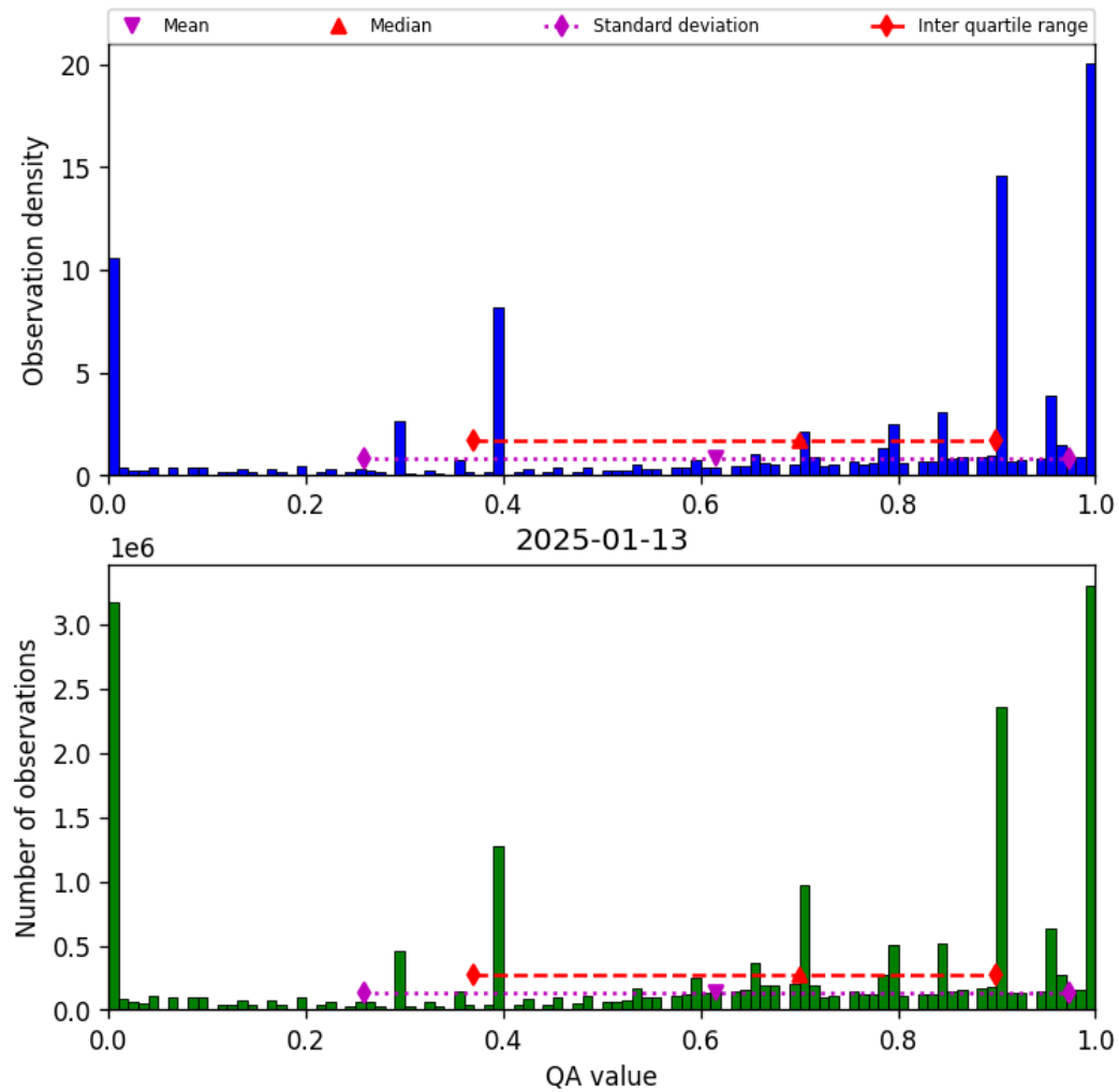
Figure 38: Histogram of “QA value” for 2025-01-12 to 2025-01-14
