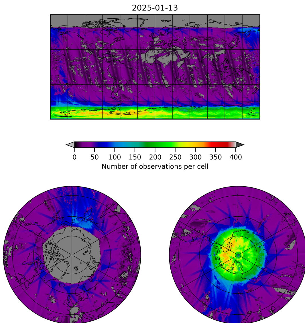
Figure 21: Map of the number of observations for 2025-01-12 to 2025-01-14
