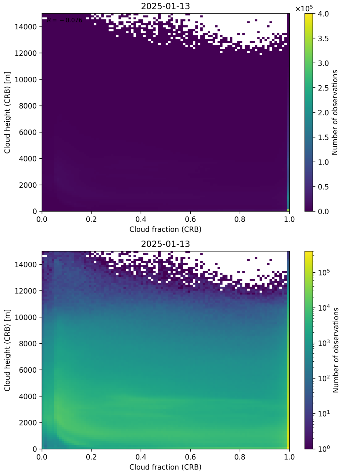
Figure 79: Scatter density plot of “Cloud fraction (CRB)” against “Cloud height (CRB)” for 2025-01-12 to 2025-01-14.
