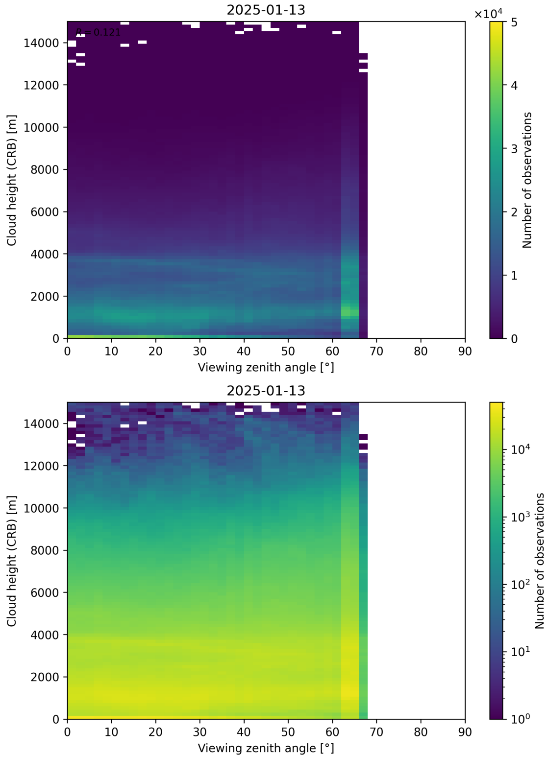
Figure 110: Scatter density plot of “Viewing zenith angle” against “Cloud height (CRB)” for 2025-01-12 to 2025-01-14.
