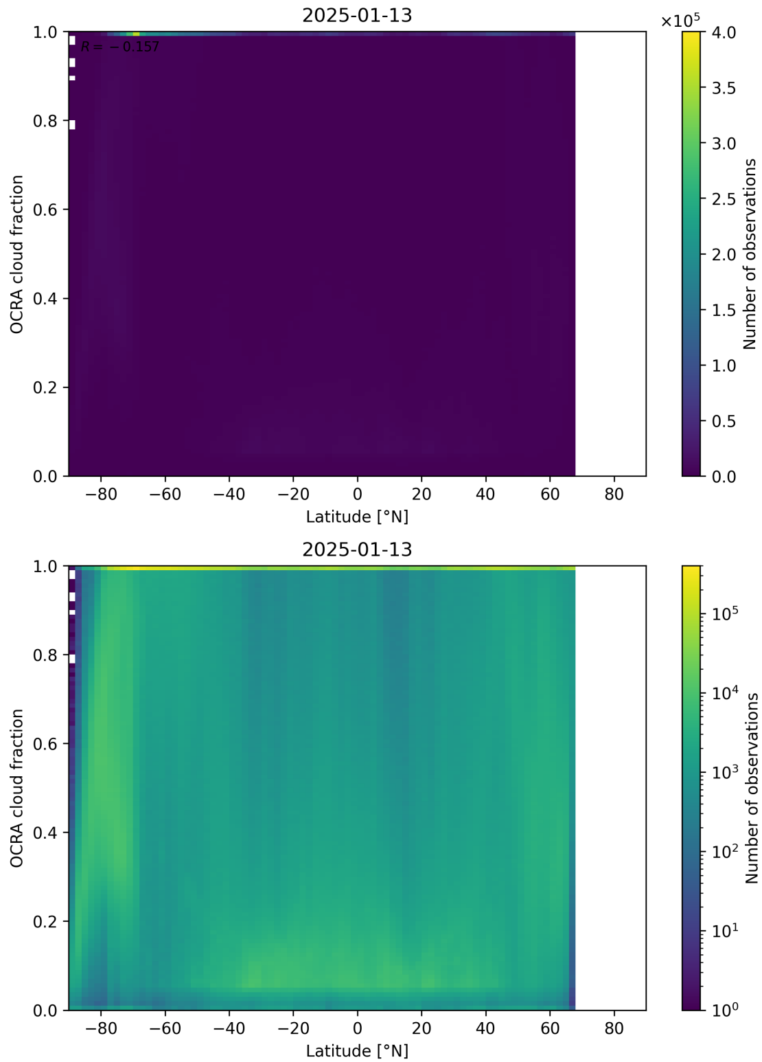
Figure 93: Scatter density plot of “Latitude” against “OCRA cloud fraction” for 2025-01-12 to 2025-01-14.
