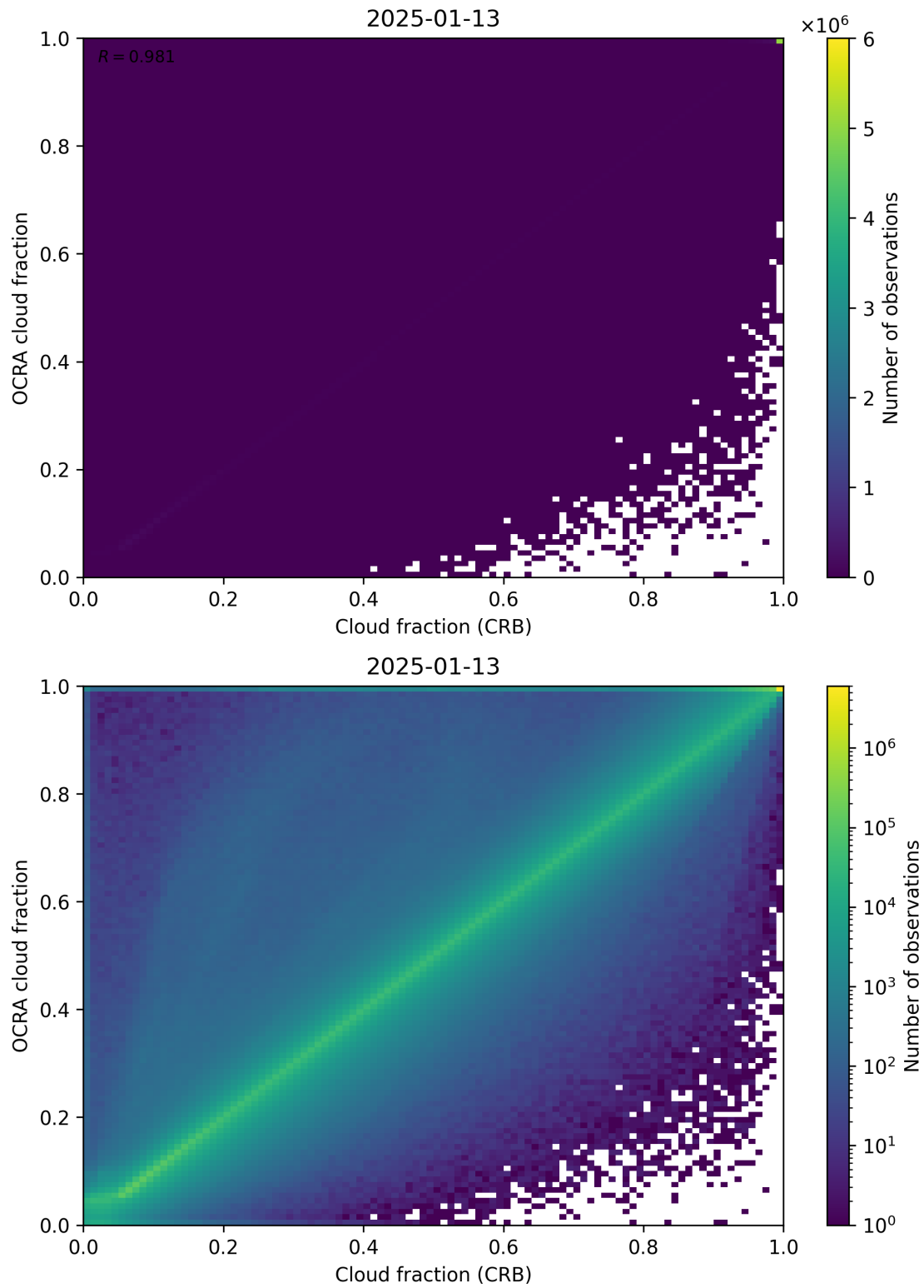
Figure 78: Scatter density plot of “Cloud fraction (CRB)” against “OCRA cloud fraction” for 2025-01-12 to 2025-01-14.
