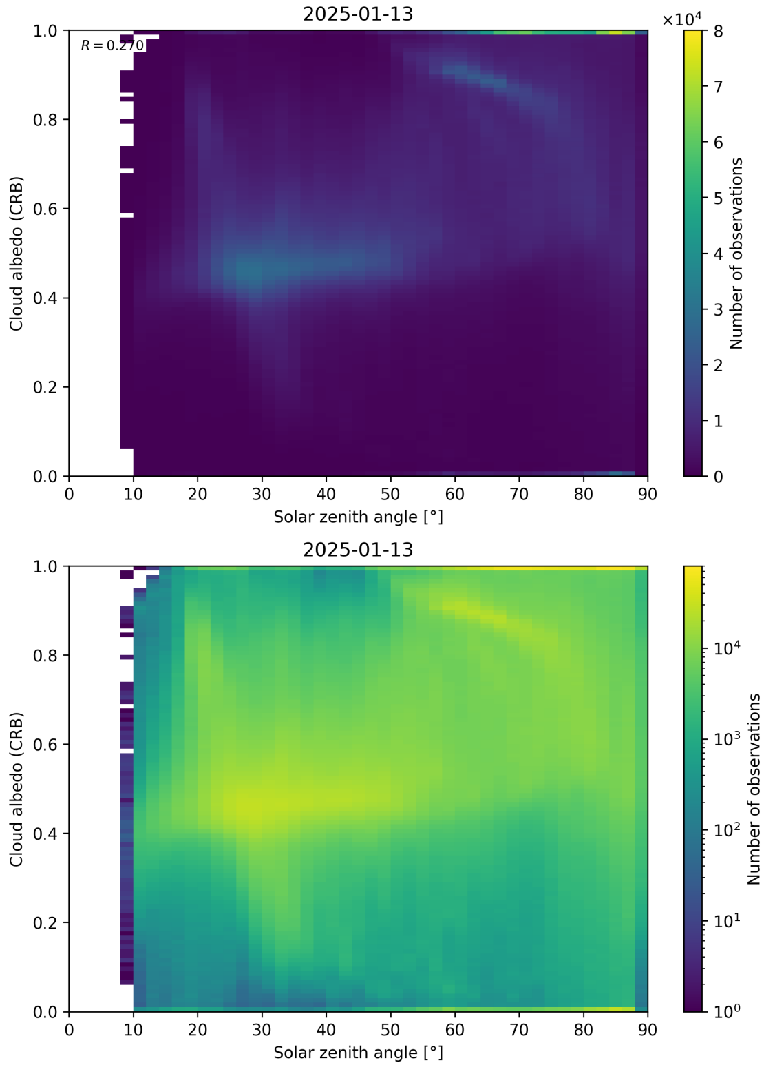
Figure 98: Scatter density plot of “Solar zenith angle” against “Cloud albedo (CRB)” for 2025-01-12 to 2025-01-14.
