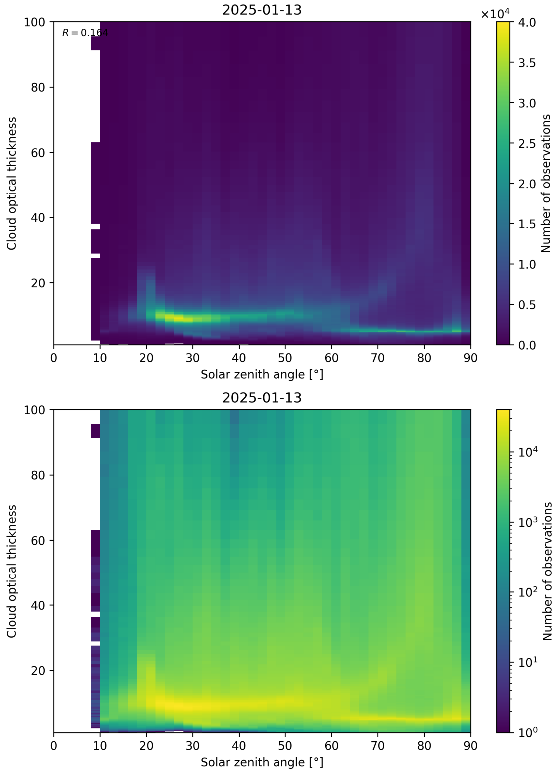
Figure 103: Scatter density plot of “Solar zenith angle” against “Cloud optical thickness” for 2025-01-12 to 2025-01-14.
