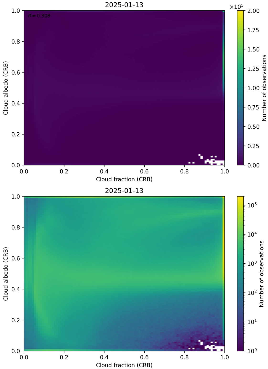
Figure 77: Scatter density plot of “Cloud fraction (CRB)” against “Cloud albedo (CRB)” for 2025-01-12 to 2025-01-14.
