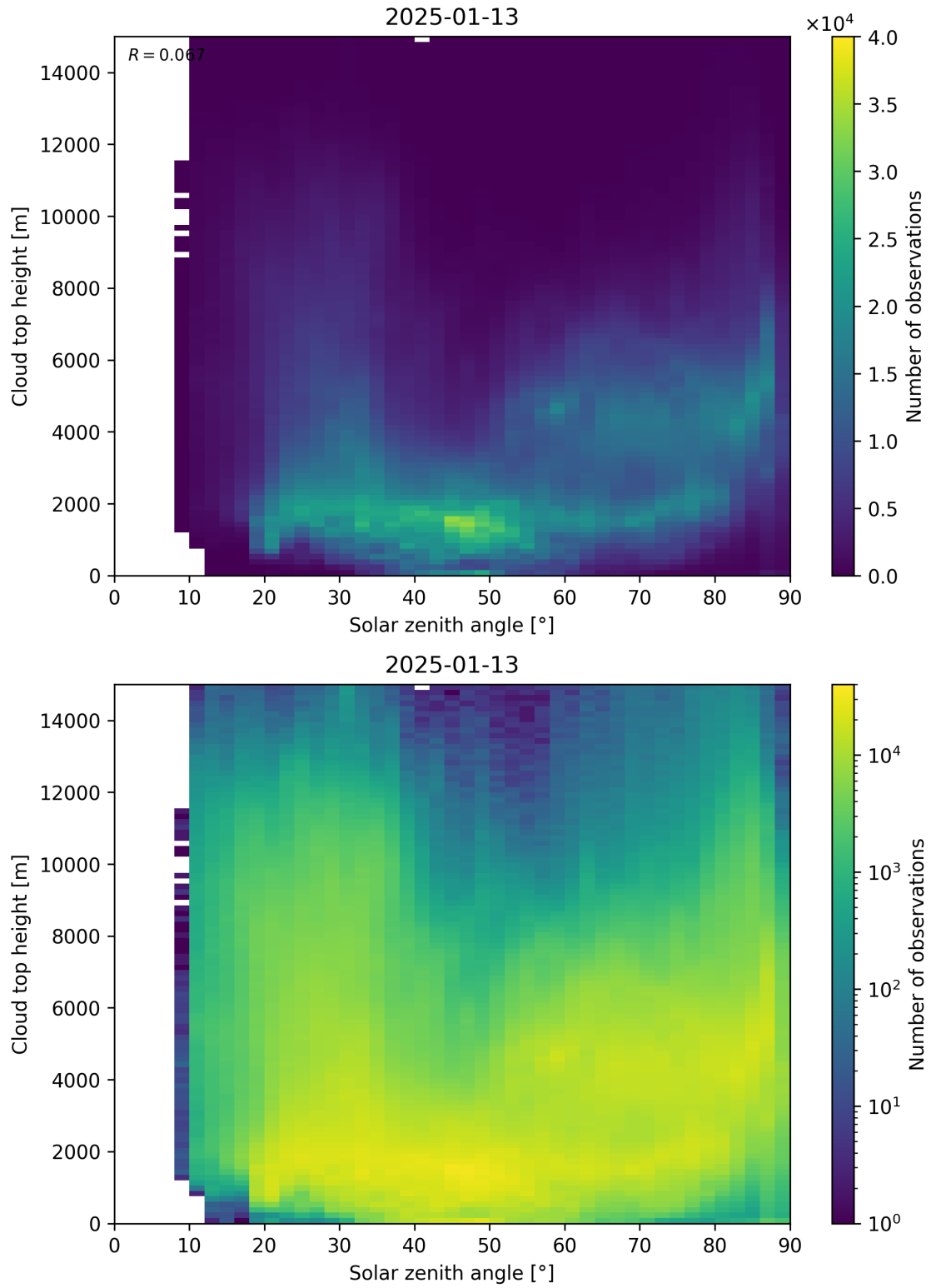
Figure 104: Scatter density plot of “Solar zenith angle” against “Cloud top height” for 2025-01-12 to 2025-01-14.
