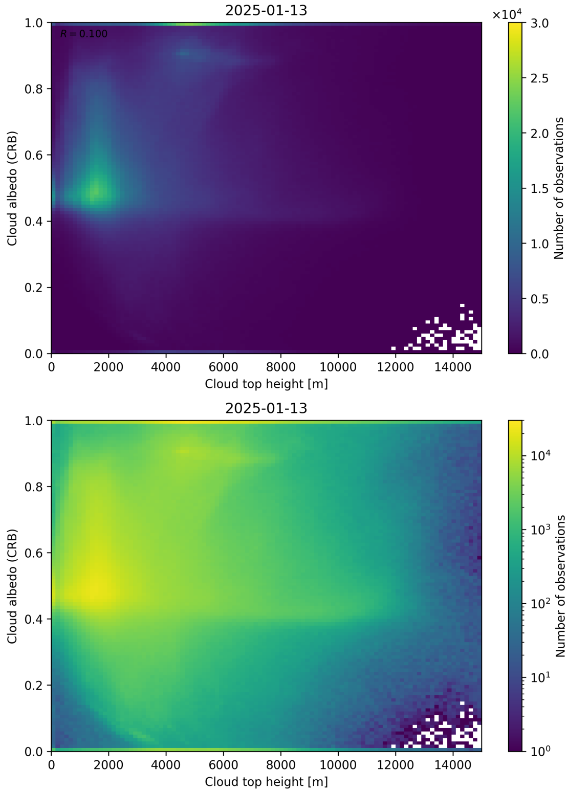
Figure 86: Scatter density plot of “Cloud top height” against “Cloud albedo (CRB)” for 2025-01-12 to 2025-01-14.
