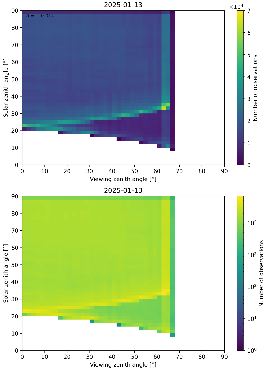
Figure 114: Scatter density plot of “Viewing zenith angle” against “Solar zenith angle” for 2025-01-12 to 2025-01-14.
