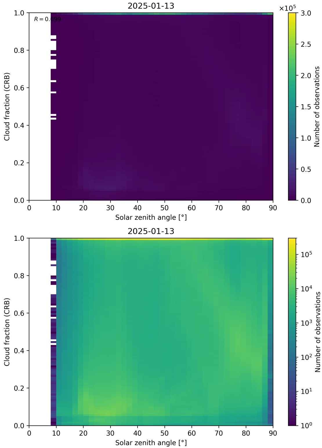
Figure 101: Scatter density plot of “Solar zenith angle” against “Cloud fraction (CRB)” for 2025-01-12 to 2025-01-14.
