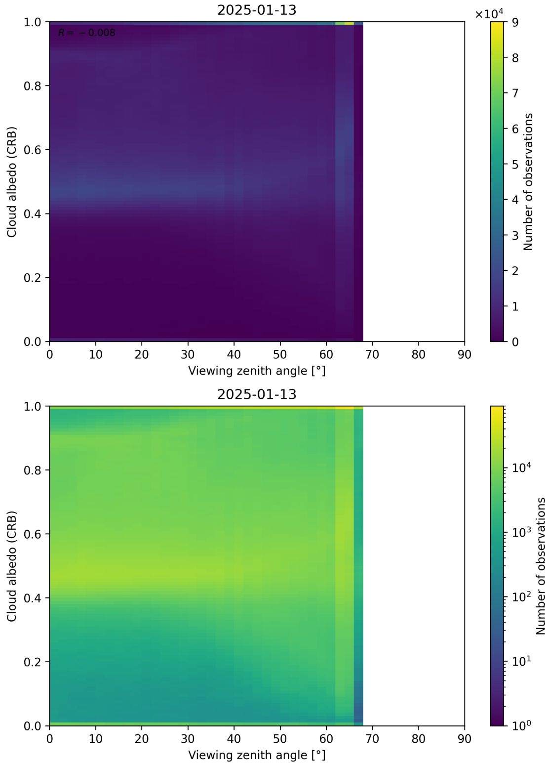
Figure 106: Scatter density plot of “Viewing zenith angle” against “Cloud albedo (CRB)” for 2025-01-12 to 2025-01-14.
