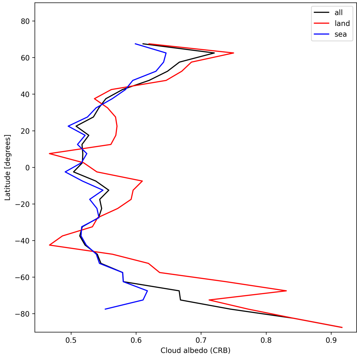
Figure 28: Zonal average of “Cloud albedo (CRB)” for 2025-01-12 to 2025-01-14.
