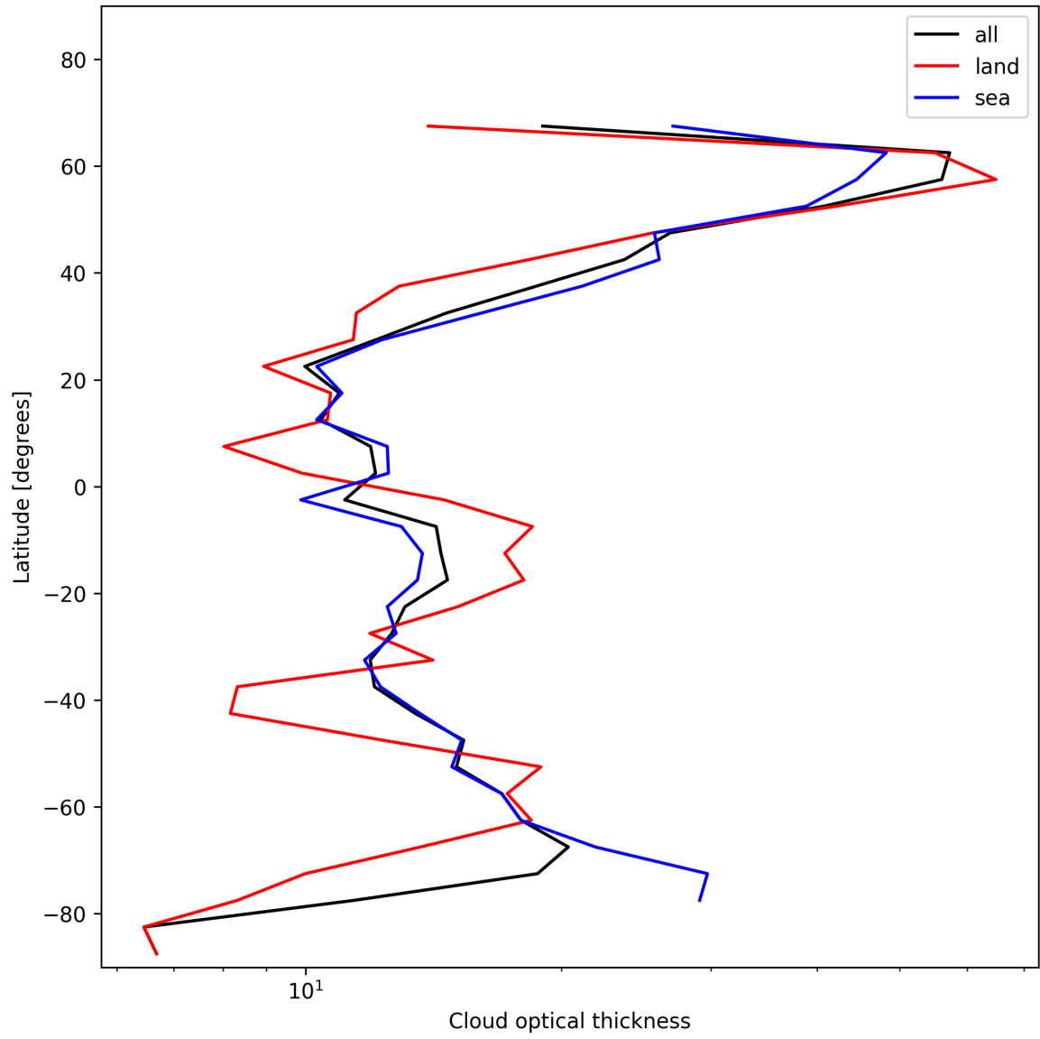
Figure 25: Zonal average of “Cloud optical thickness” for 2025-01-12 to 2025-01-14.
