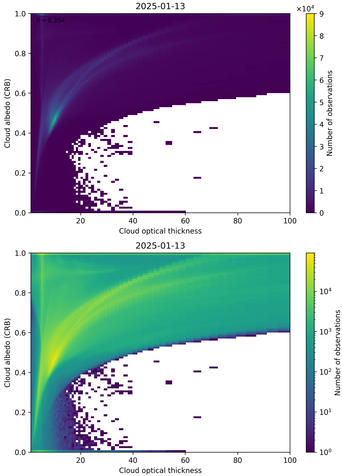
Figure 82: Scatter density plot of “Cloud optical thickness” against “Cloud albedo (CRB)” for 2025-01-12 to 2025-01-14.
