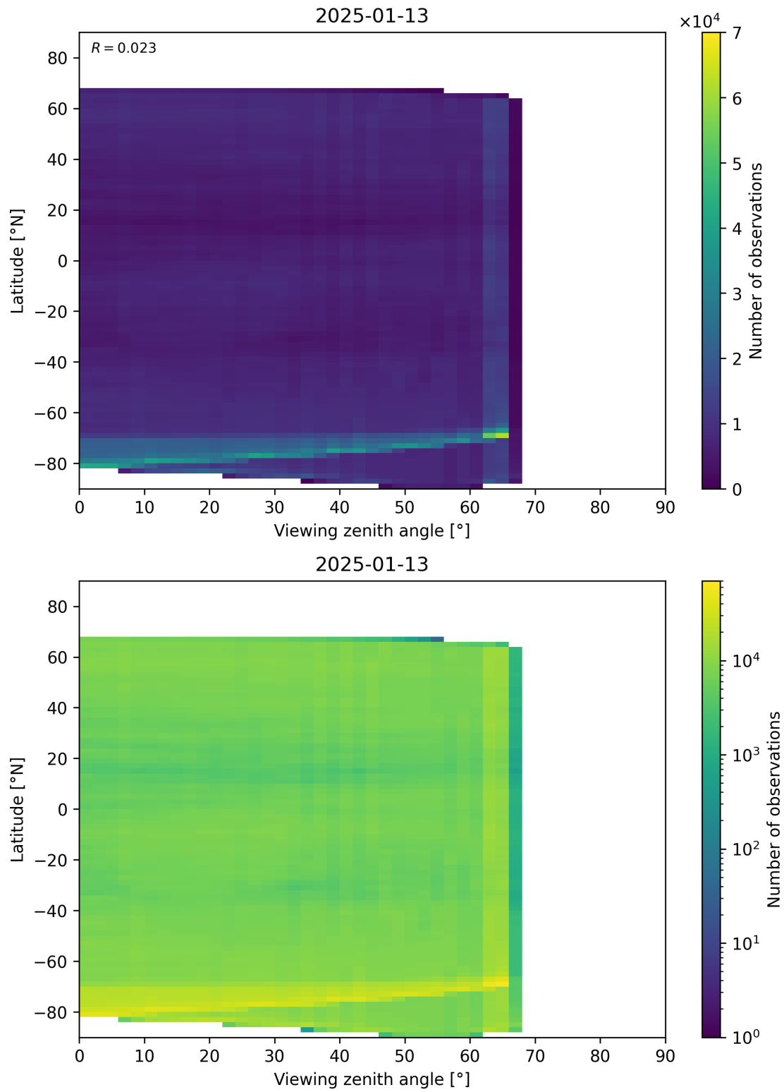
Figure 113: Scatter density plot of “Viewing zenith angle” against “Latitude” for 2025-01-12 to 2025-01-14.
