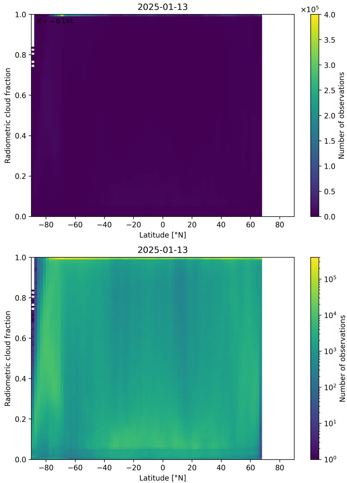
Figure 92: Scatter density plot of “Latitude” against “Radiometric cloud fraction” for 2025-01-12 to 2025-01-14.
