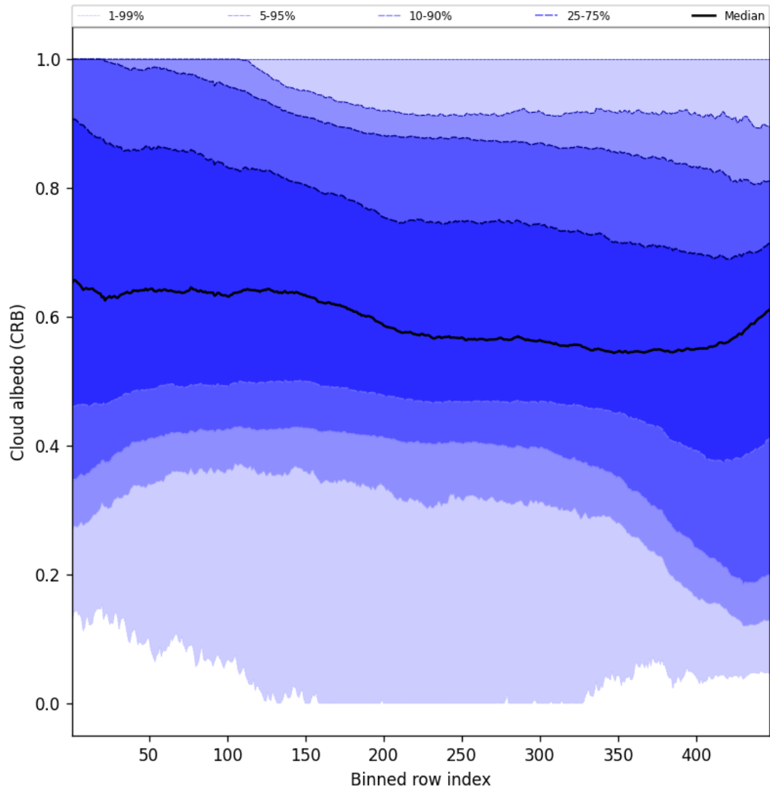
Figure 60: Along track statistics of “Cloud albedo (CRB)” for 2025-01-12 to 2025-01-14
