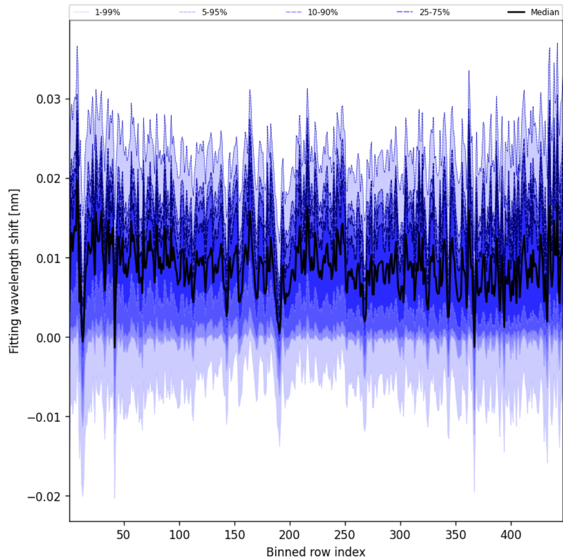
Figure 65: Along track statistics of “Fitting wavelength shift” for 2025-01-12 to 2025-01-14
