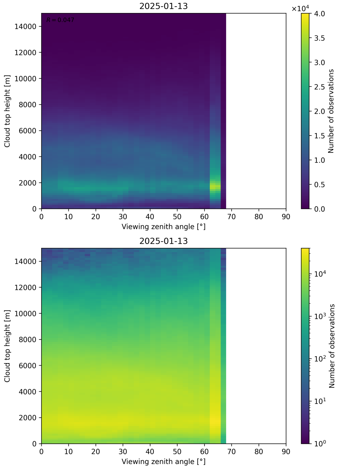
Figure 112: Scatter density plot of “Viewing zenith angle” against “Cloud top height” for 2025-01-12 to 2025-01-14.
