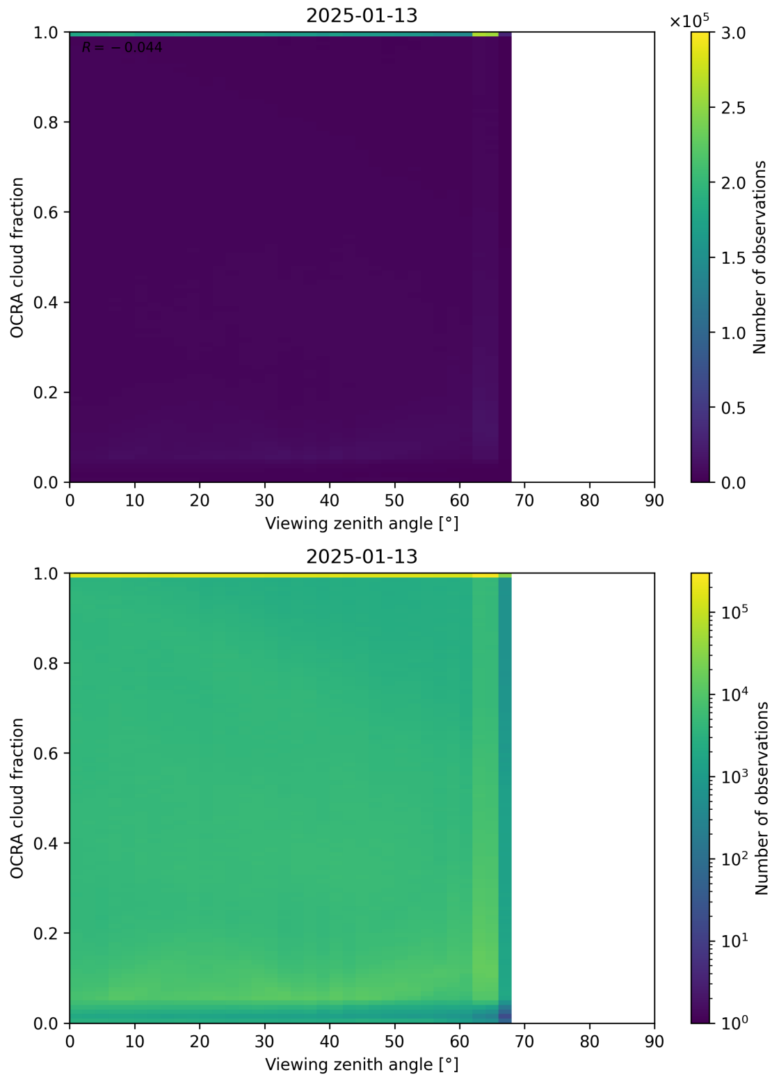
Figure 108: Scatter density plot of “Viewing zenith angle” against “OCRA cloud fraction” for 2025-01-12 to 2025-01-14.
