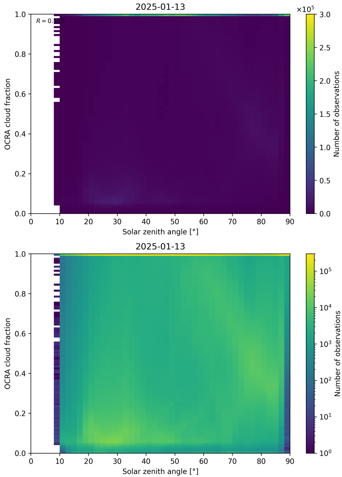
Figure 100: Scatter density plot of “Solar zenith angle” against “OCRA cloud fraction” for 2025-01-12 to 2025-01-14.
