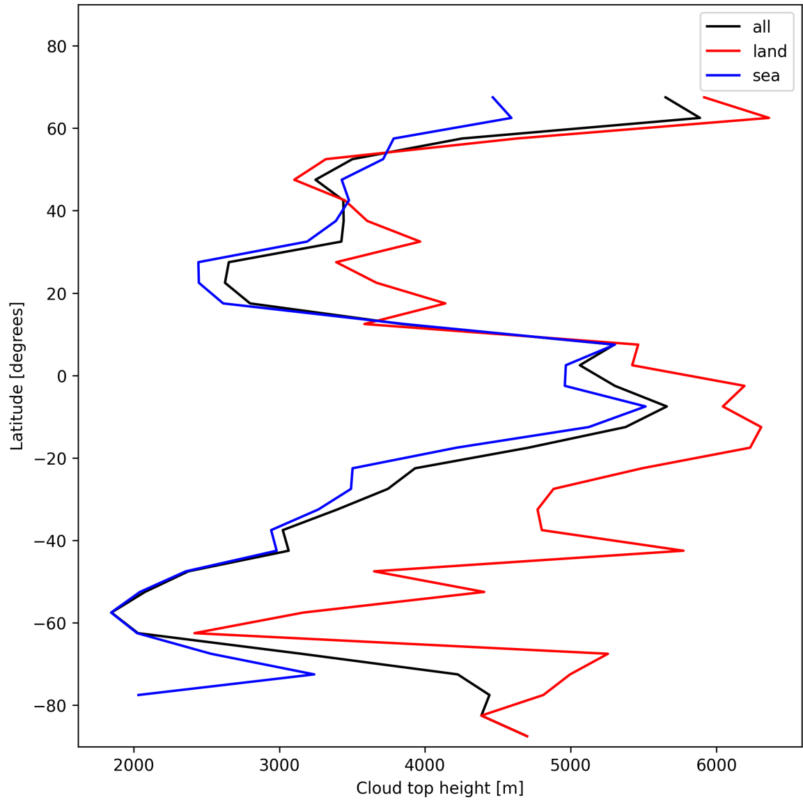
Figure 24: Zonal average of “Cloud top height” for 2025-01-12 to 2025-01-14.
