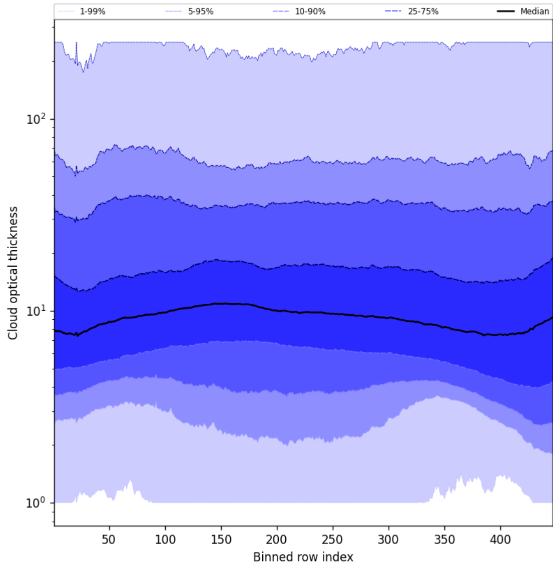
Figure 57: Along track statistics of “Cloud optical thickness” for 2025-01-12 to 2025-01-14
