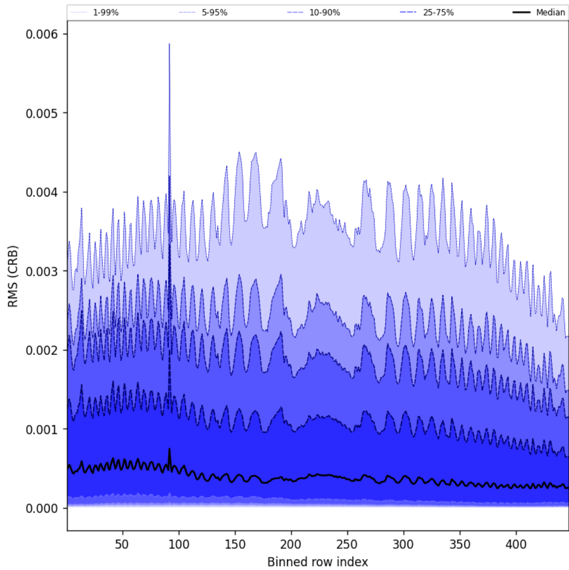
Figure 64: Along track statistics of “RMS (CRB)” for 2025-01-12 to 2025-01-14
