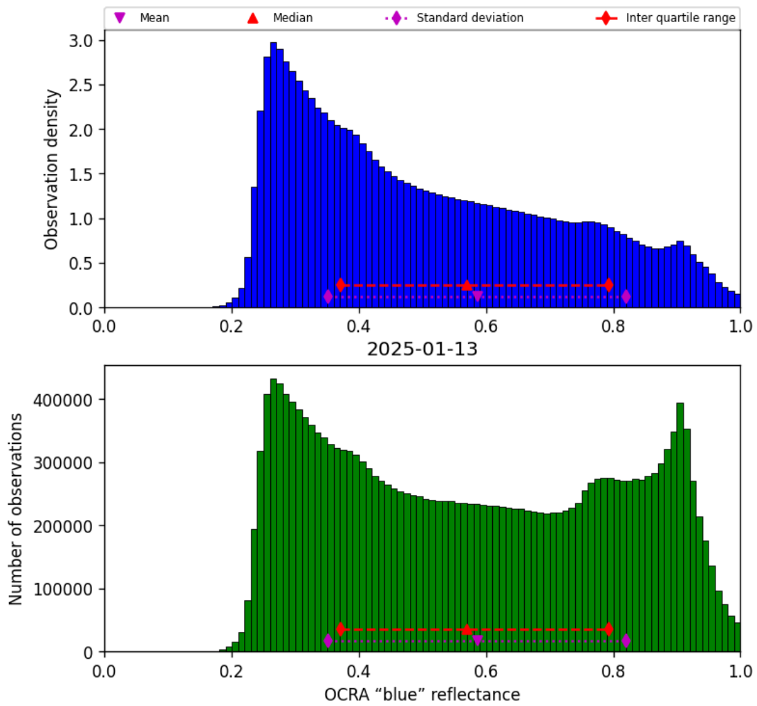
Figure 51: Histogram of “OCRA “blue” reflectance” for 2025-01-12 to 2025-01-14
