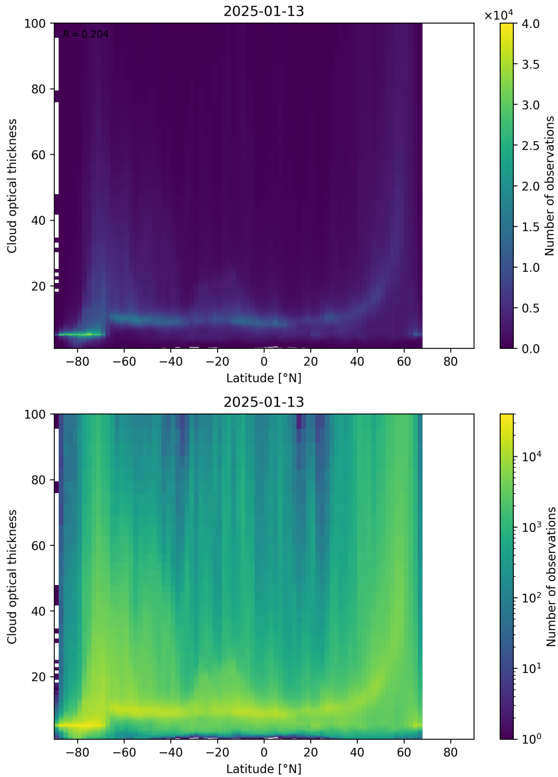
Figure 96: Scatter density plot of “Latitude” against “Cloud optical thickness” for 2025-01-12 to 2025-01-14.
