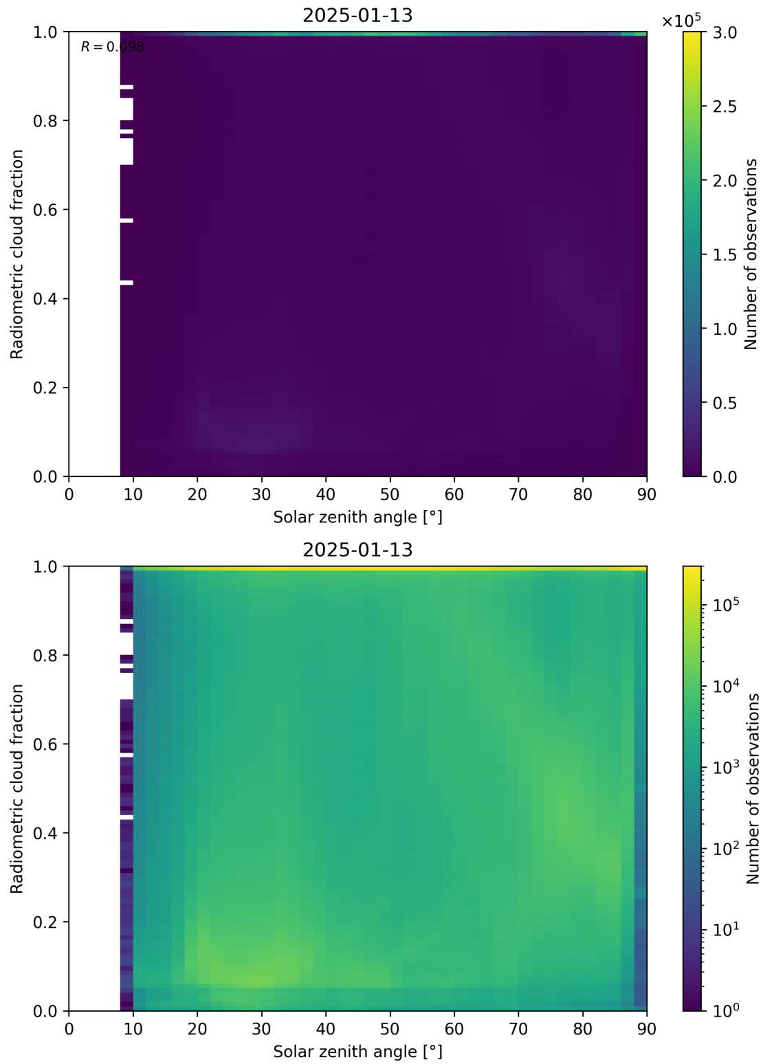
Figure 99: Scatter density plot of “Solar zenith angle” against “Radiometric cloud fraction” for 2025-01-12 to 2025-01-14.
