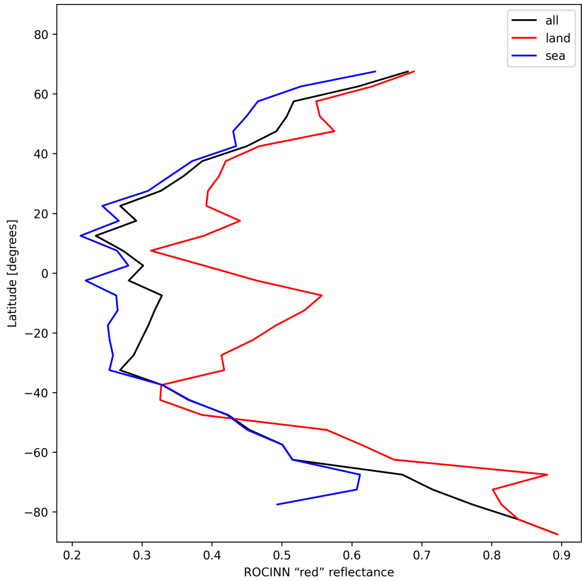
Figure 37: Zonal average of "ROCINN "red" reflectance" for 2025-01-12 to 2025-01-14.
