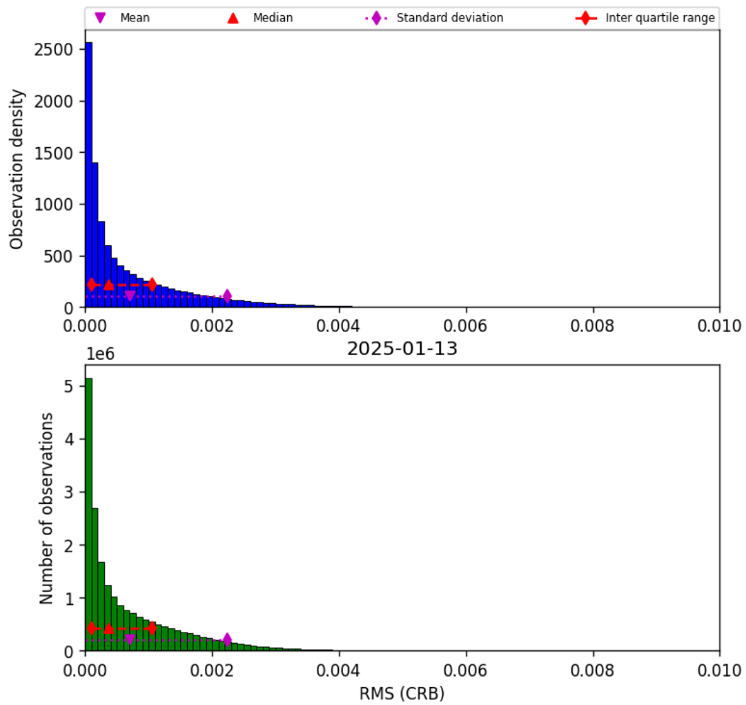
Figure 48: Histogram of “RMS (CRB)” for 2025-01-12 to 2025-01-14
