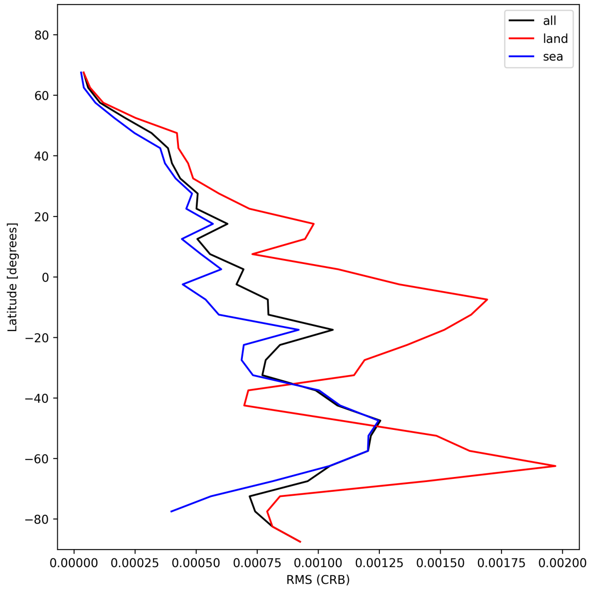
Figure 32: Zonal average of “RMS (CRB)” for 2025-01-12 to 2025-01-14.
