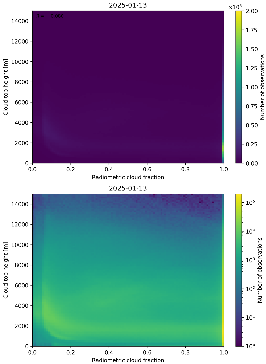
Figure 76: Scatter density plot of “Radiometric cloud fraction” against “Cloud top height” for 2025-01-12 to 2025-01-14.
