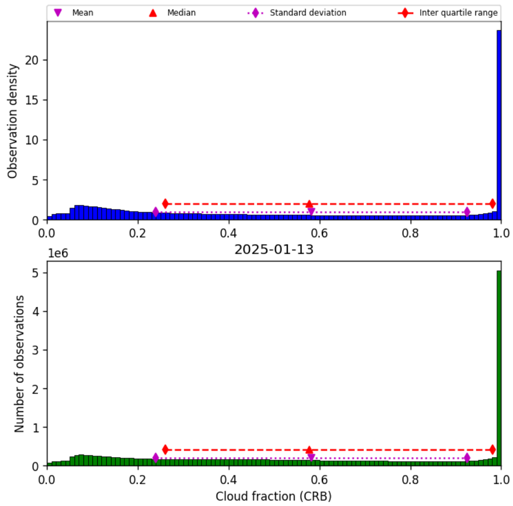
Figure 42: Histogram of “Cloud fraction (CRB)” for 2025-01-12 to 2025-01-14
