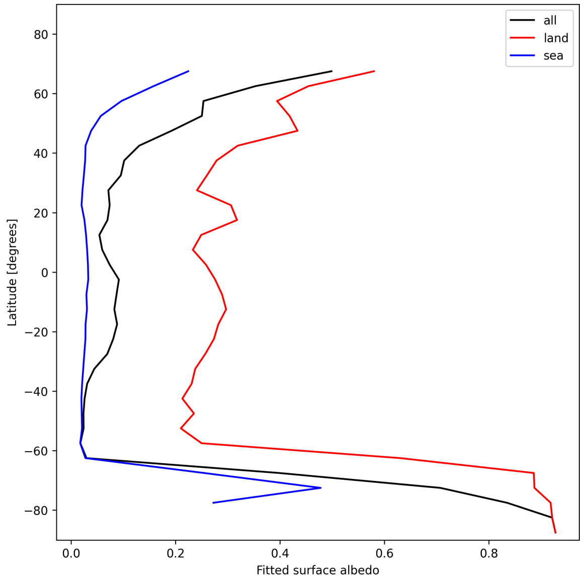
Figure 29: Zonal average of “Fitted surface albedo” for 2025-01-12 to 2025-01-14.
