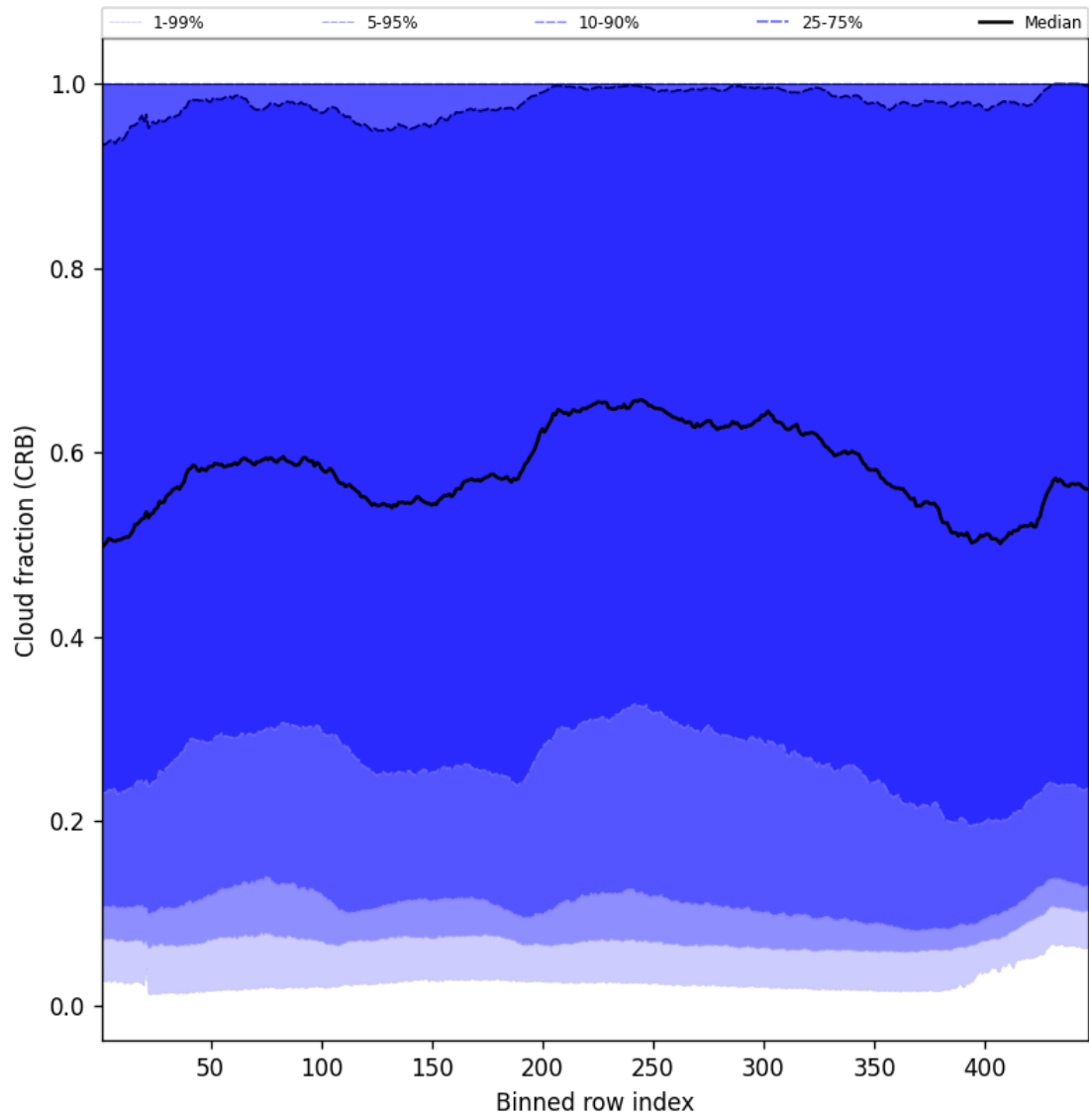
Figure 58: Along track statistics of “Cloud fraction (CRB)” for 2025-01-12 to 2025-01-14
