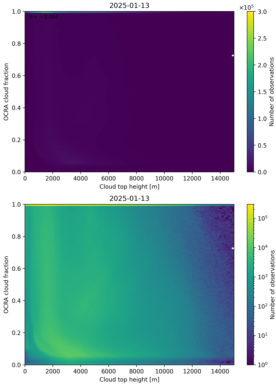
Figure 87: Scatter density plot of “Cloud top height” against “OCRA cloud fraction” for 2025-01-12 to 2025-01-14.
