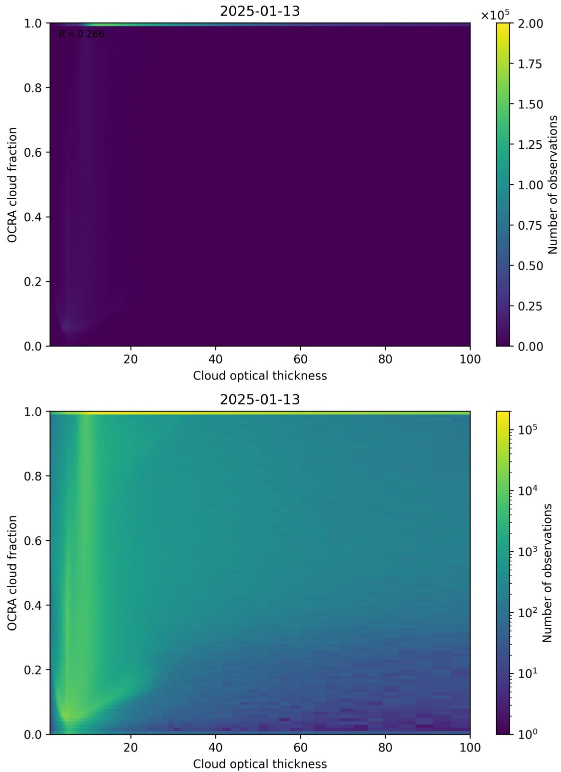
Figure 83: Scatter density plot of “Cloud optical thickness” against “OCRA cloud fraction” for 2025-01-12 to 2025-01-14.
