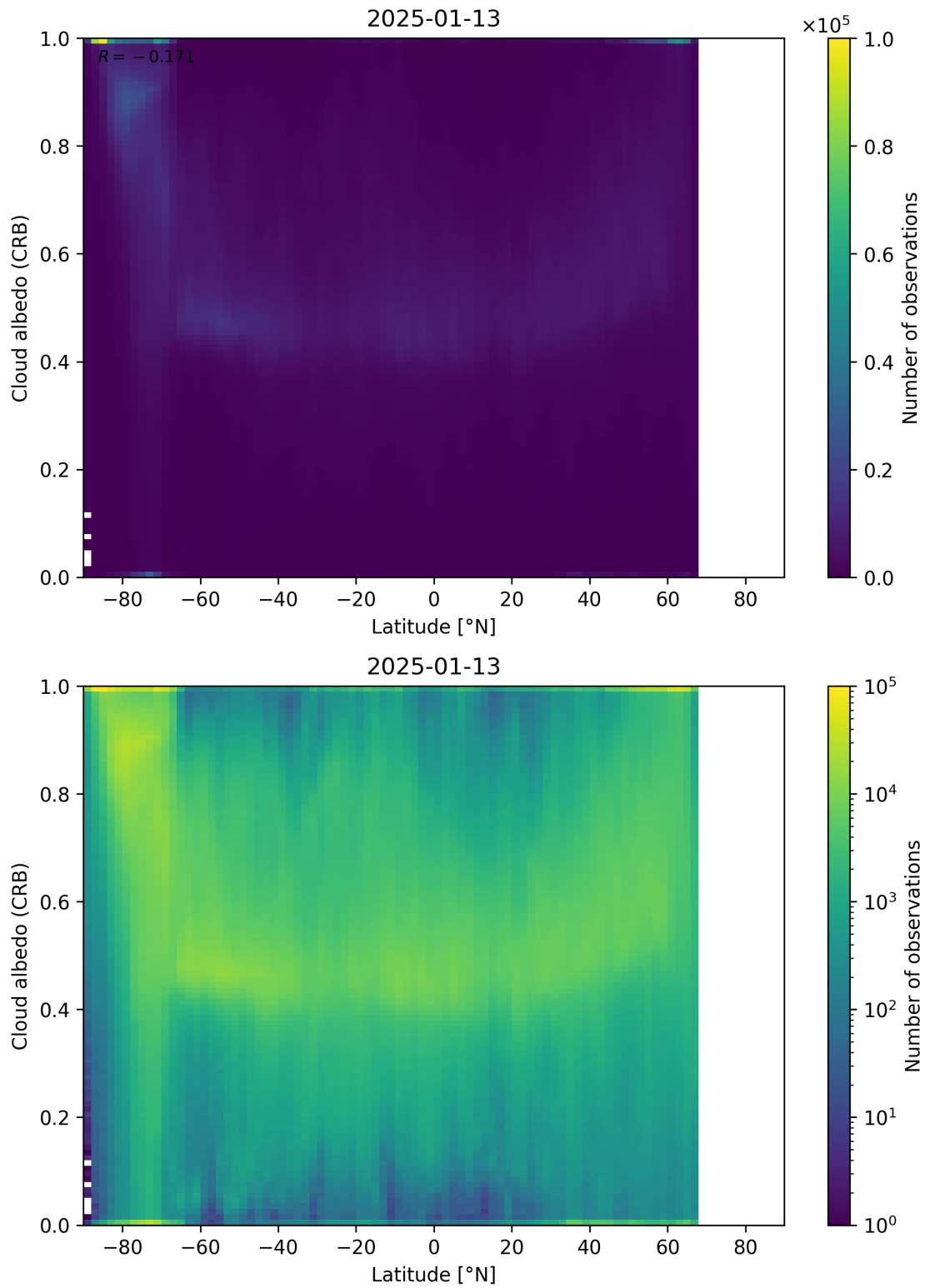
Figure 91: Scatter density plot of “Latitude” against “Cloud albedo (CRB)” for 2025-01-12 to 2025-01-14.
