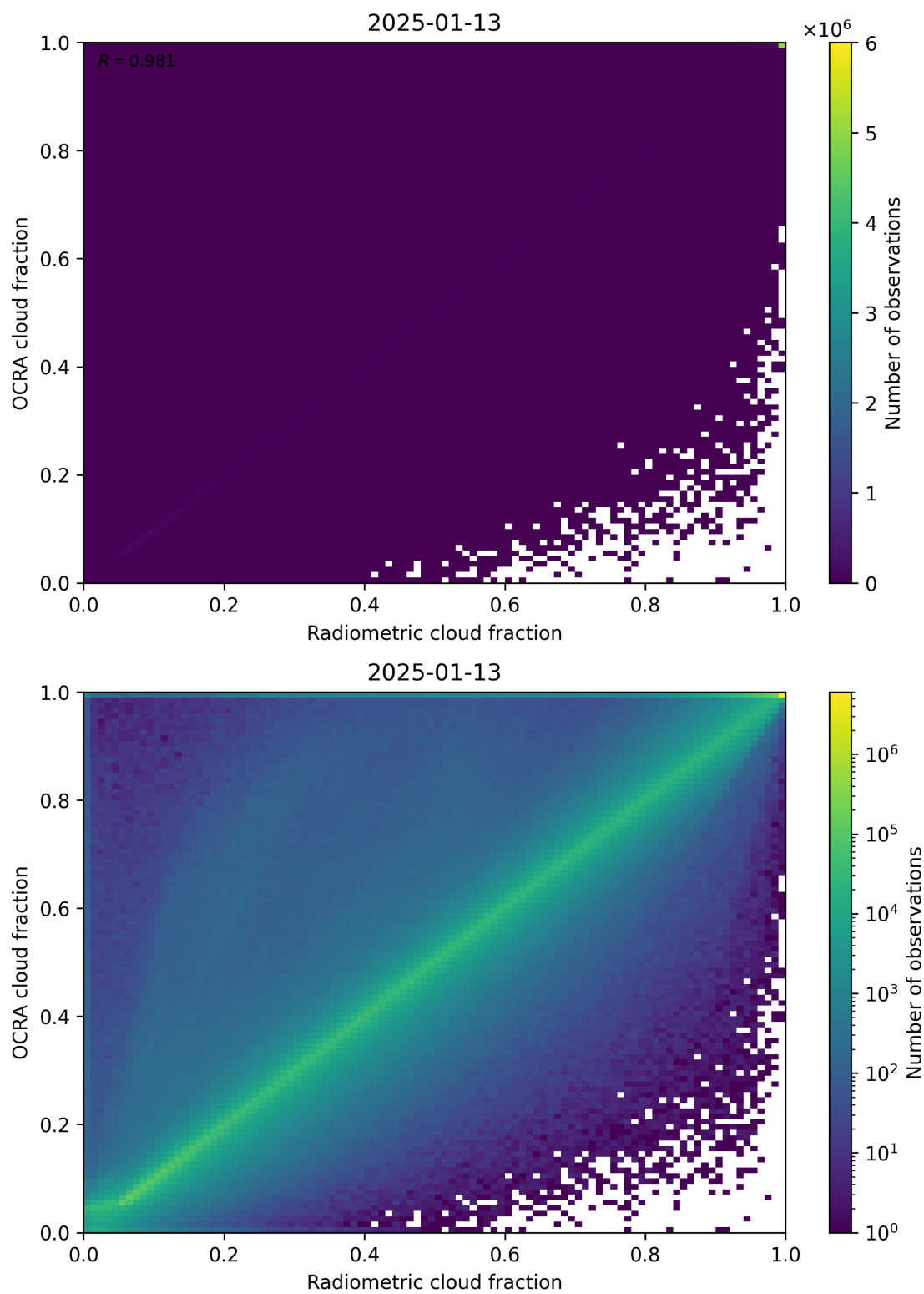
Figure 72: Scatter density plot of “Radiometric cloud fraction” against “OCRA cloud fraction” for 2025-01-12 to 2025-01-14.
