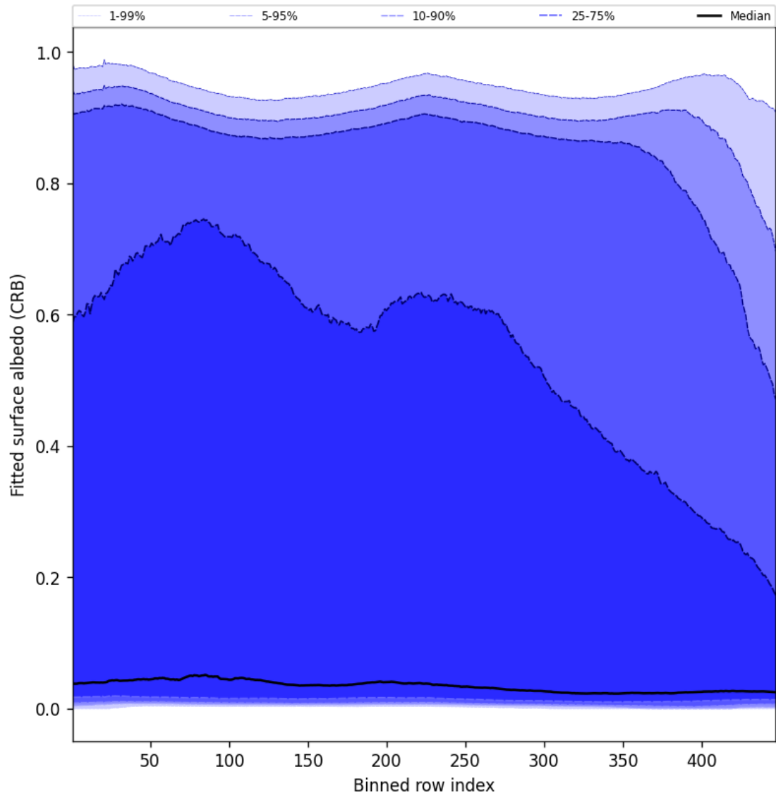
Figure 62: Along track statistics of “Fitted surface albedo (CRB)” for 2025-01-12 to 2025-01-14
