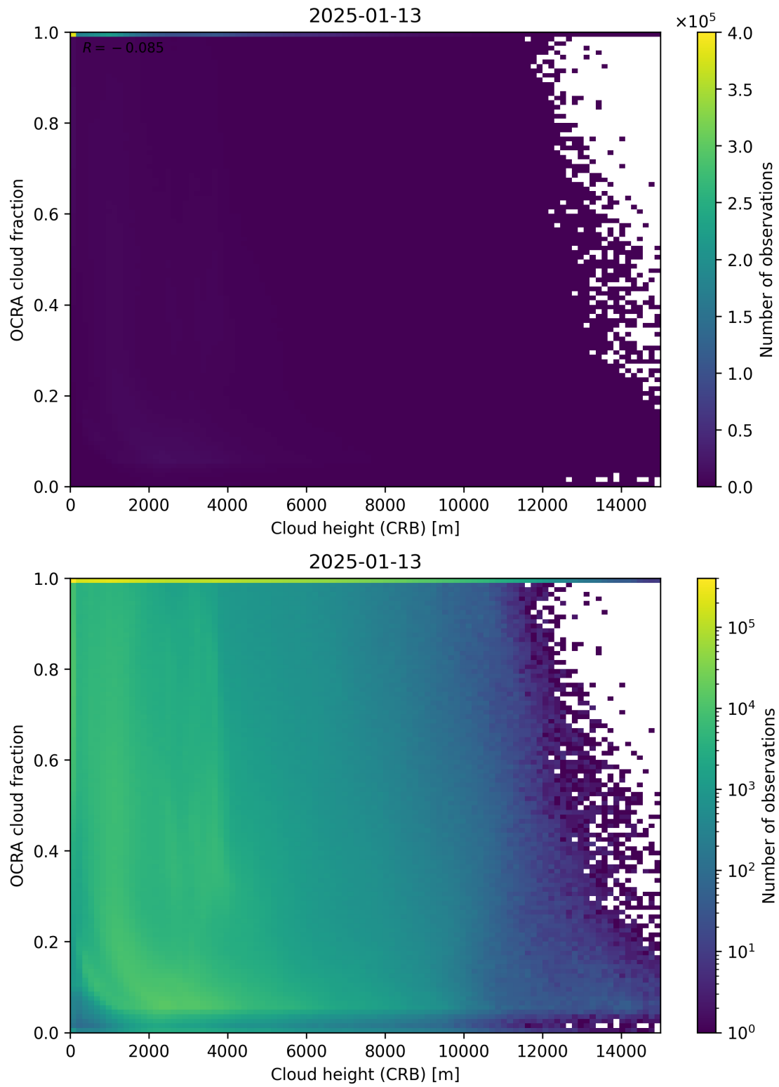
Figure 81: Scatter density plot of “Cloud height (CRB)” against “OCRA cloud fraction” for 2025-01-12 to 2025-01-14.
