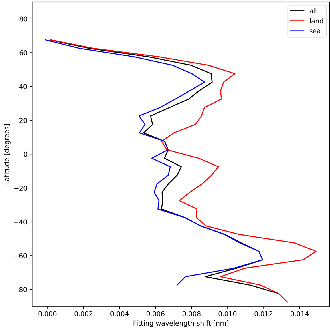
Figure 33: Zonal average of “Fitting wavelength shift” for 2025-01-12 to 2025-01-14.
