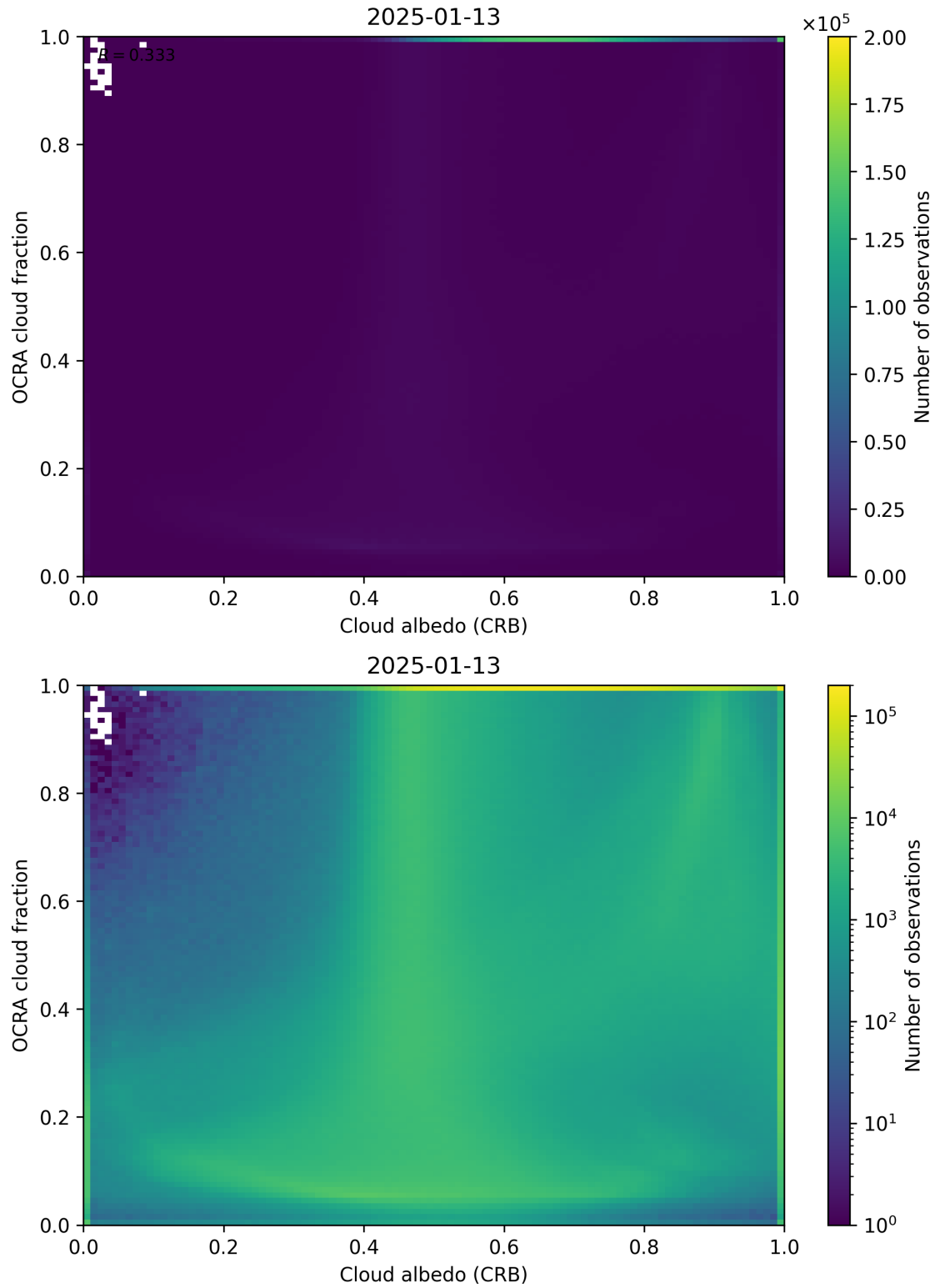
Figure 70: Scatter density plot of “Cloud albedo (CRB)” against “OCRA cloud fraction” for 2025-01-12 to 2025-01-14.
