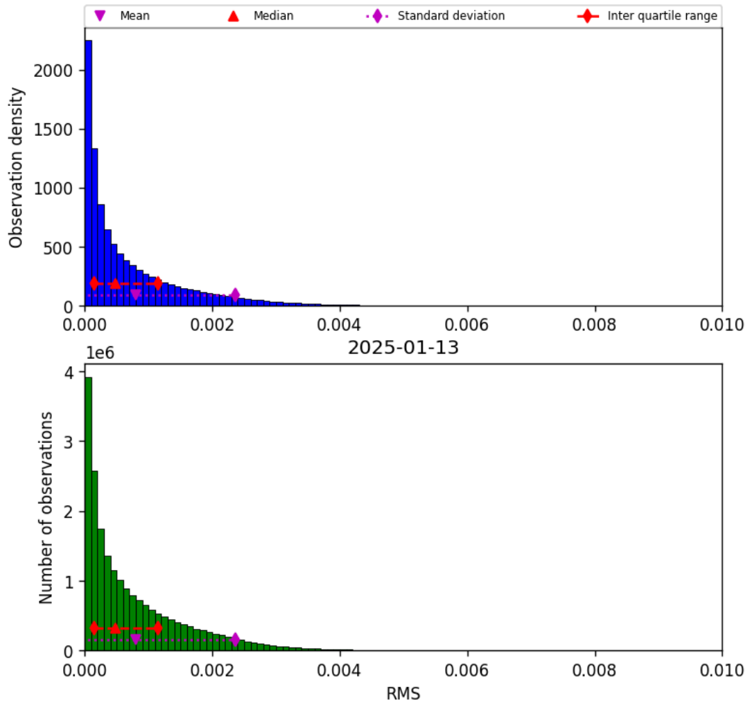
Figure 47: Histogram of “RMS” for 2025-01-12 to 2025-01-14
