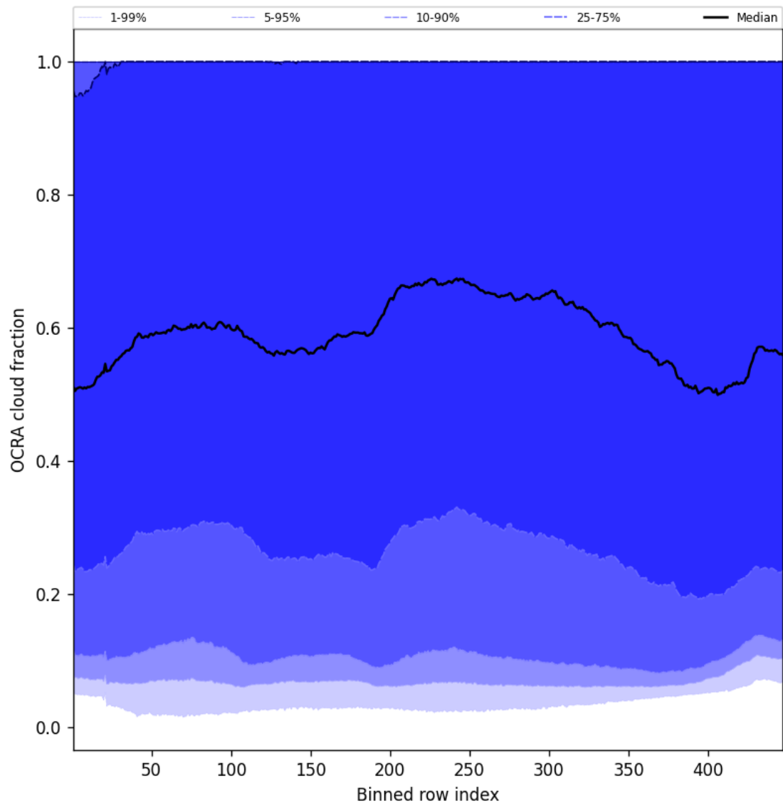
Figure 66: Along track statistics of “OCRA cloud fraction” for 2025-01-12 to 2025-01-14
