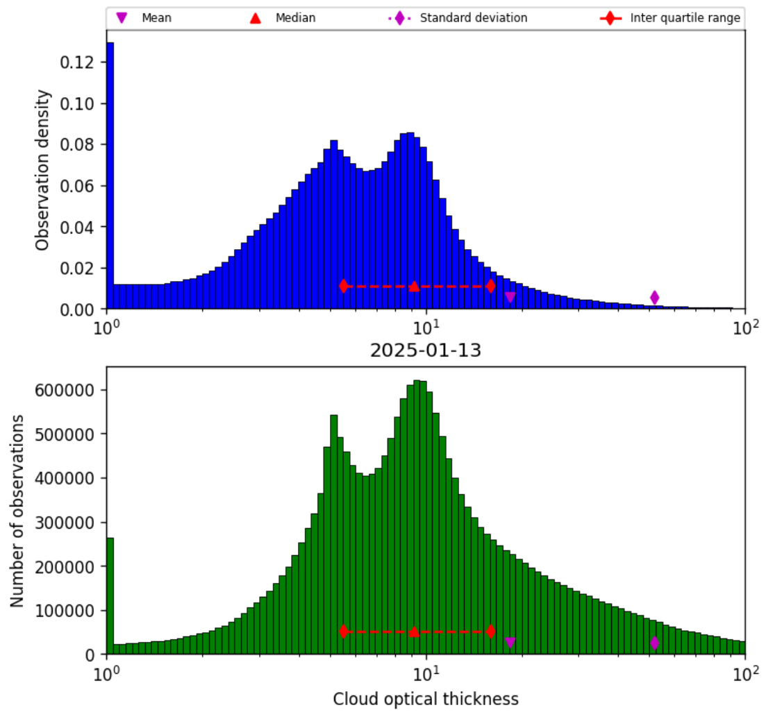
Figure 41: Histogram of “Cloud optical thickness” for 2025-01-12 to 2025-01-14
