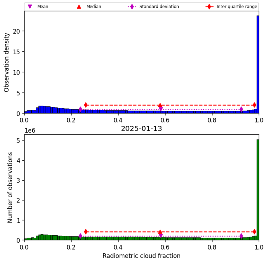
Figure 39: Histogram of “Radiometric cloud fraction” for 2025-01-12 to 2025-01-14
