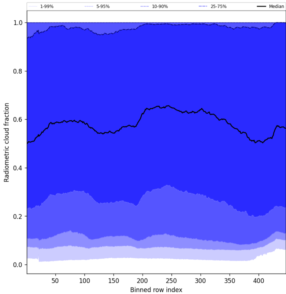
Figure 55: Along track statistics of “Radiometric cloud fraction” for 2025-01-12 to 2025-01-14
