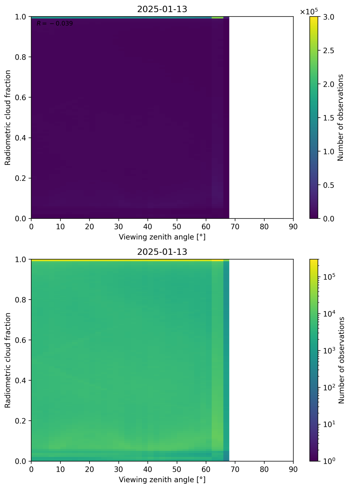
Figure 107: Scatter density plot of “Viewing zenith angle” against “Radiometric cloud fraction” for 2025-01-12 to 2025-01-14.
