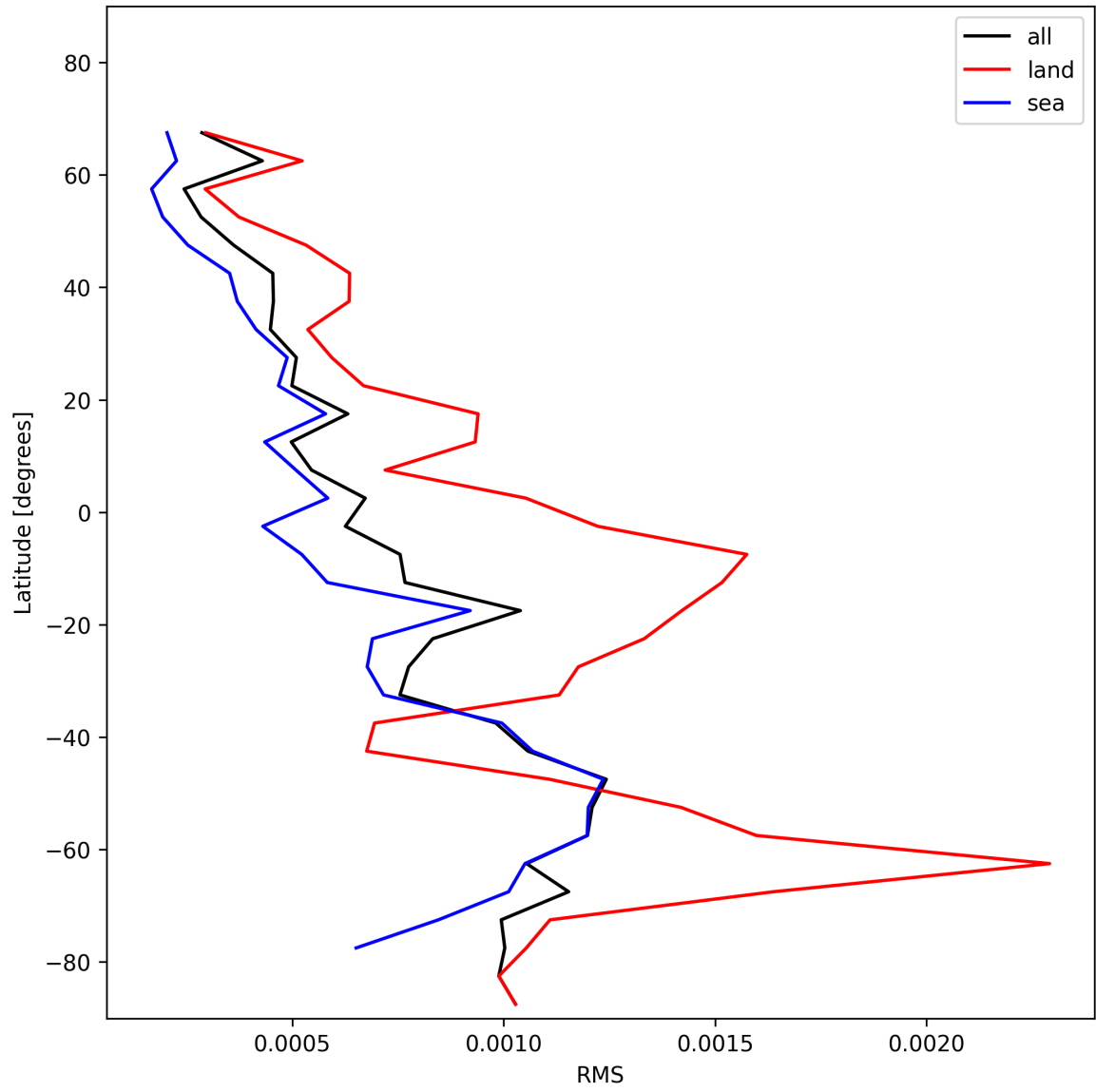
Figure 31: Zonal average of “RMS” for 2025-01-12 to 2025-01-14.
