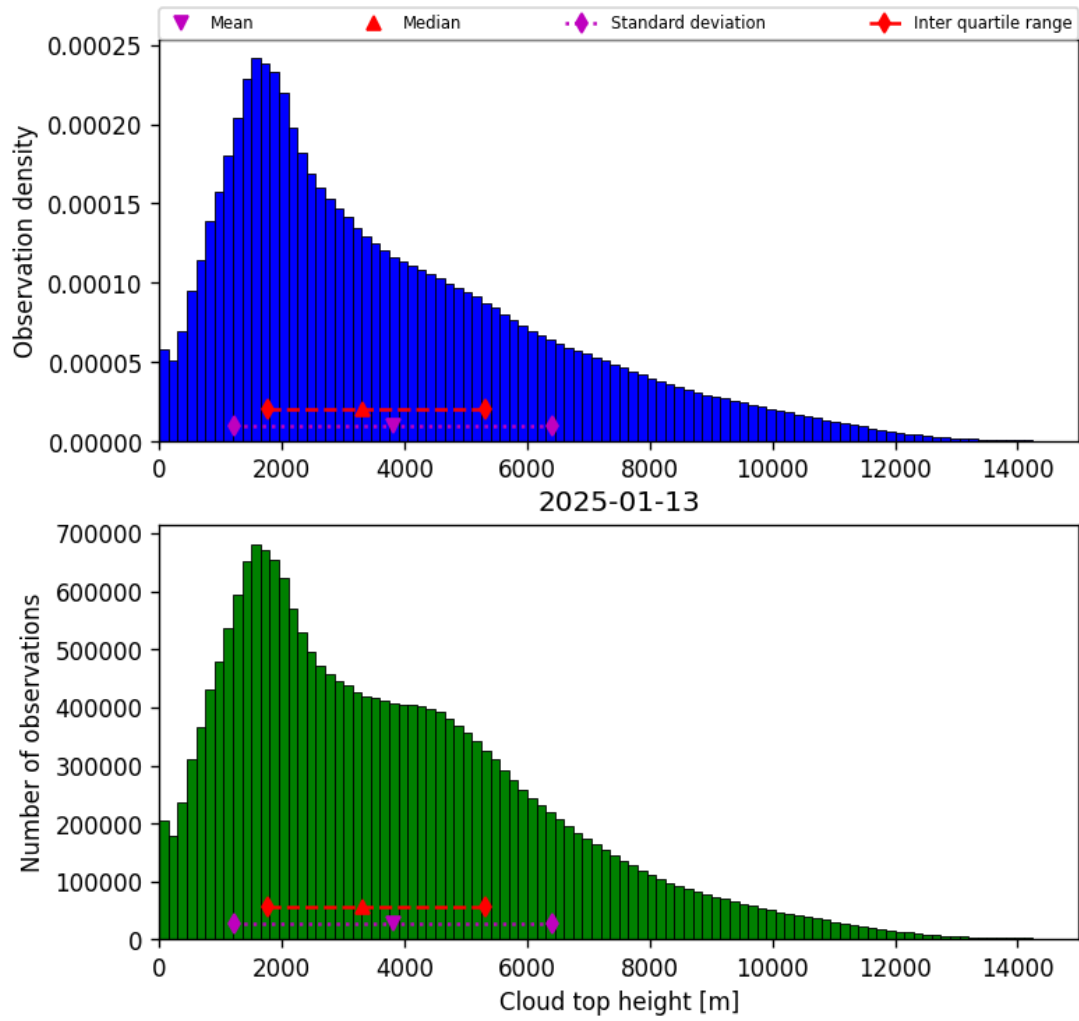
Figure 40: Histogram of “Cloud top height” for 2025-01-12 to 2025-01-14
