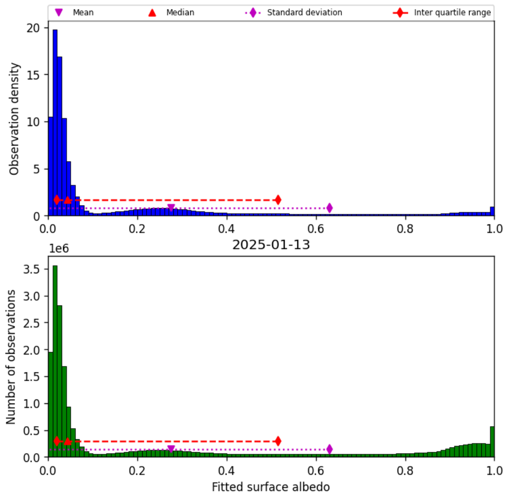
Figure 45: Histogram of “Fitted surface albedo” for 2025-01-12 to 2025-01-14
