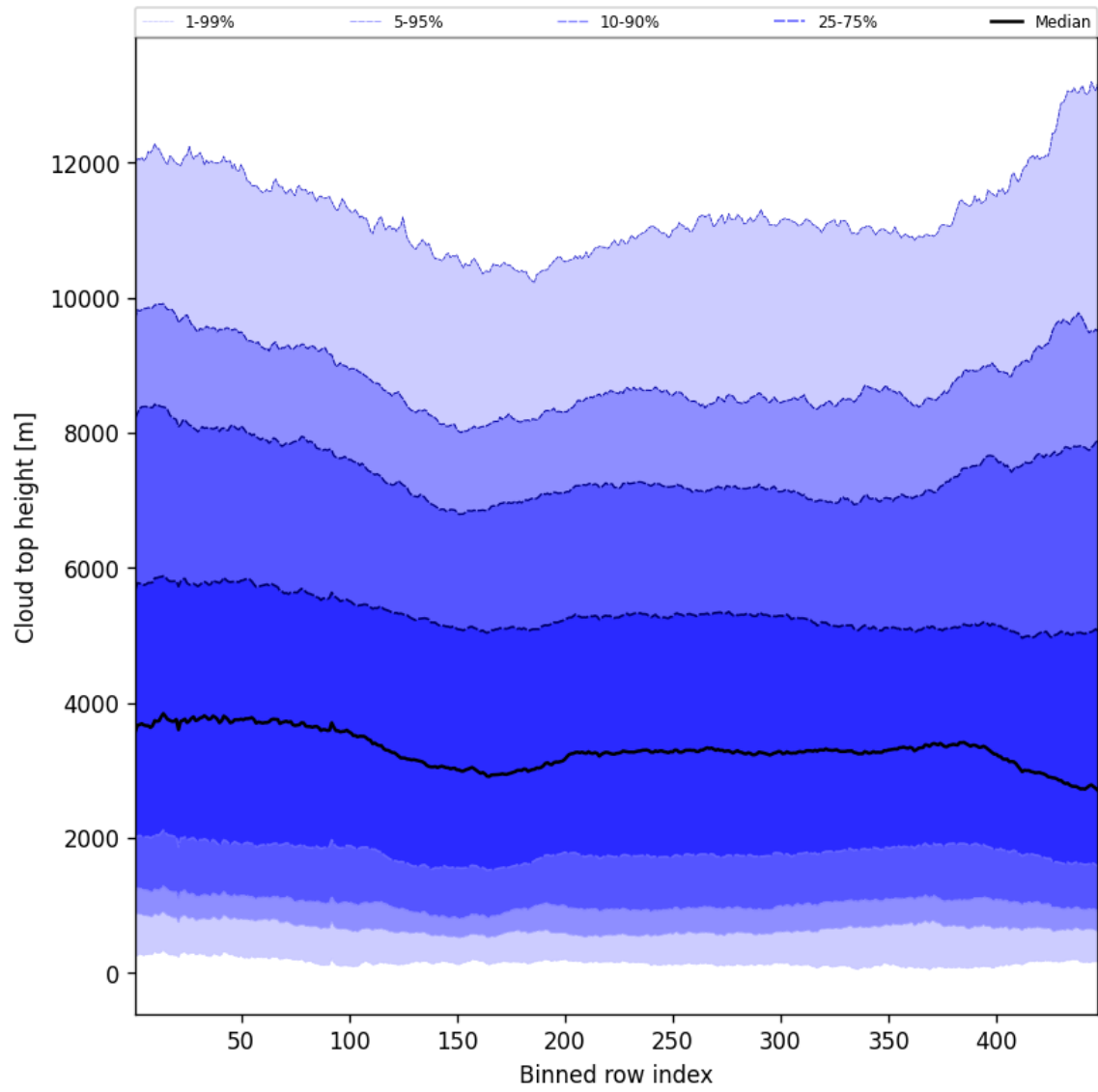
Figure 56: Along track statistics of “Cloud top height” for 2025-01-12 to 2025-01-14
