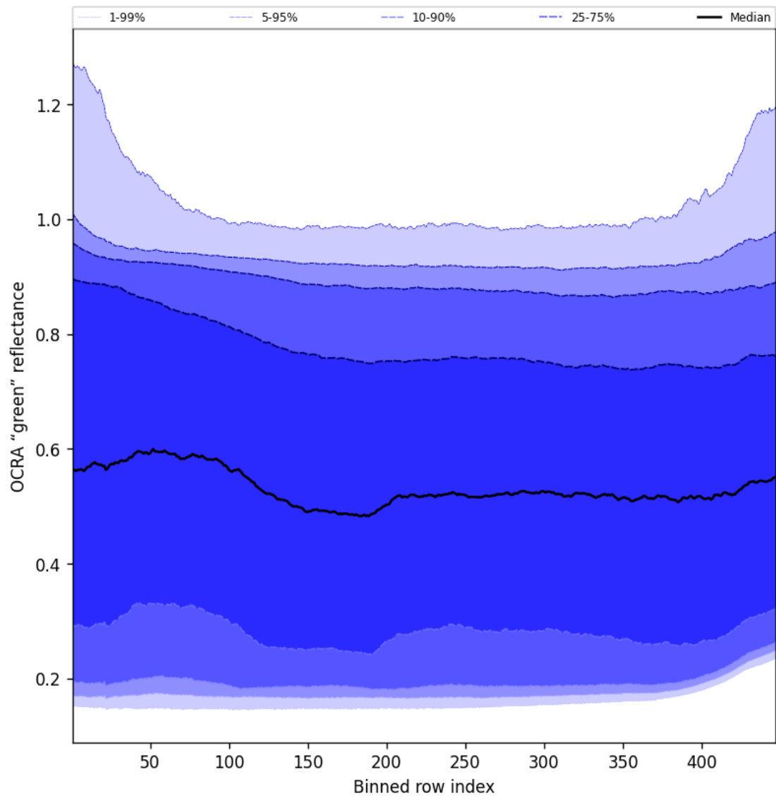
Figure 68: Along track statistics of "OCRA "green" reflectance" for 2025-01-12 to 2025-01-14
