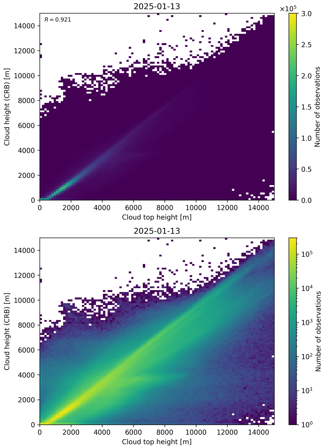
Figure 89: Scatter density plot of “Cloud top height” against “Cloud height (CRB)” for 2025-01-12 to 2025-01-14.
