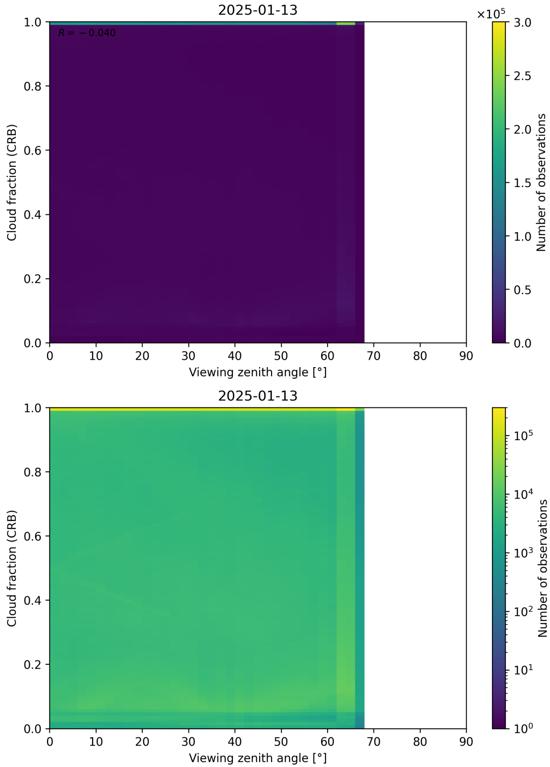
Figure 109: Scatter density plot of “Viewing zenith angle” against “Cloud fraction (CRB)” for 2025-01-12 to 2025-01-14.
