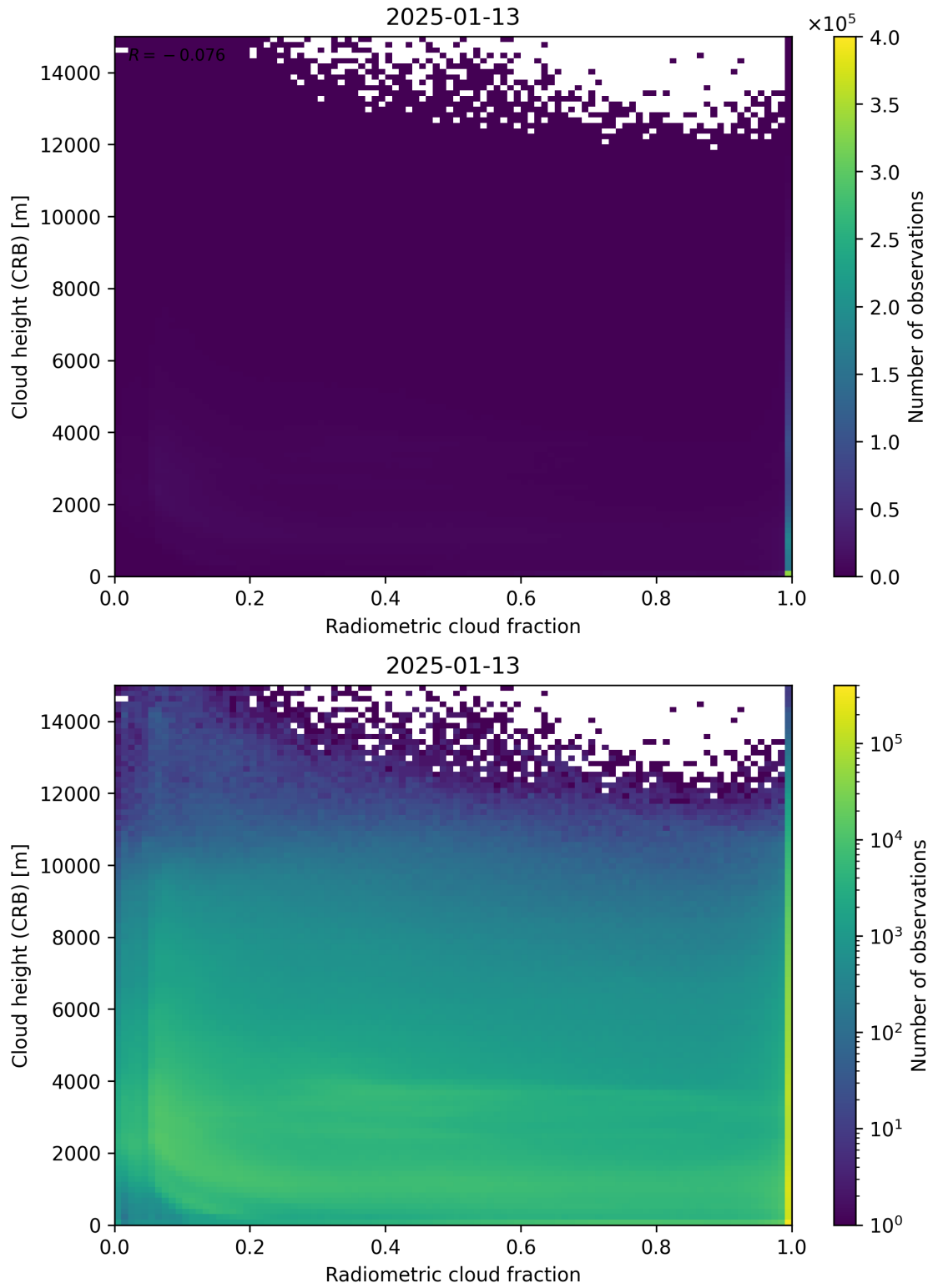
Figure 74: Scatter density plot of “Radiometric cloud fraction” against “Cloud height (CRB)” for 2025-01-12 to 2025-01-14.
