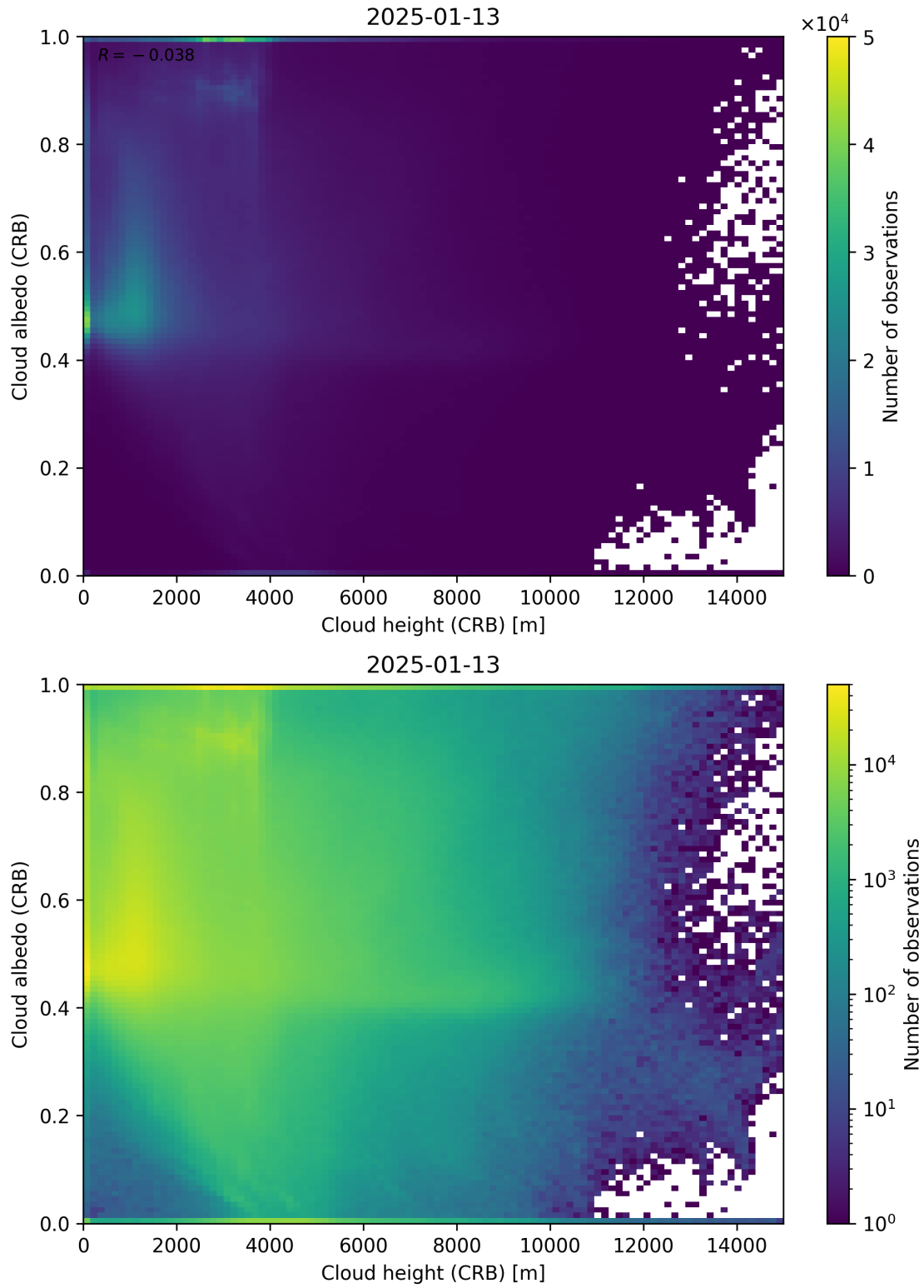
Figure 80: Scatter density plot of “Cloud height (CRB)” against “Cloud albedo (CRB)” for 2025-01-12 to 2025-01-14.
