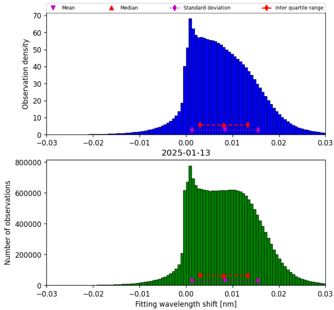
Figure 49: Histogram of “Fitting wavelength shift” for 2025-01-12 to 2025-01-14
