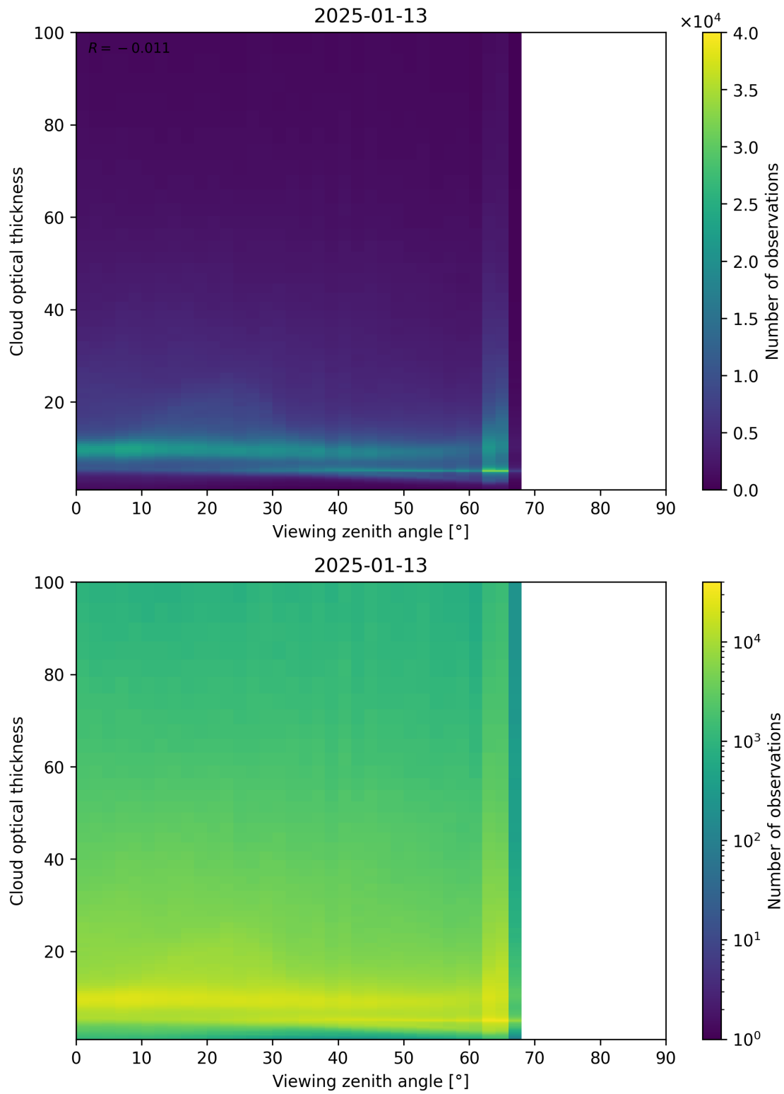
Figure 111: Scatter density plot of “Viewing zenith angle” against “Cloud optical thickness” for 2025-01-12 to 2025-01-14.
