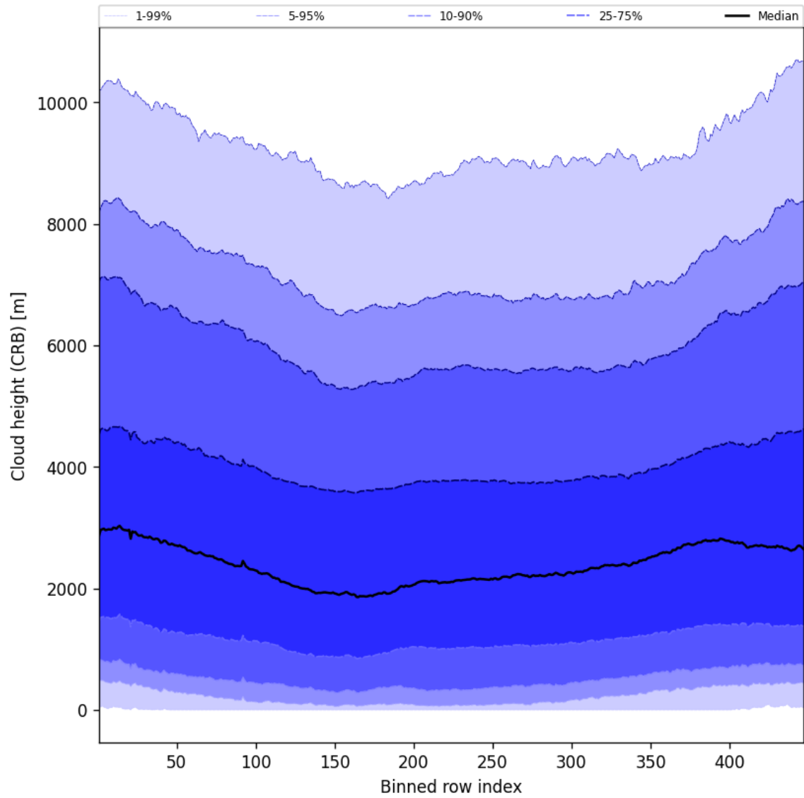
Figure 59: Along track statistics of “Cloud height (CRB)” for 2025-01-12 to 2025-01-14
