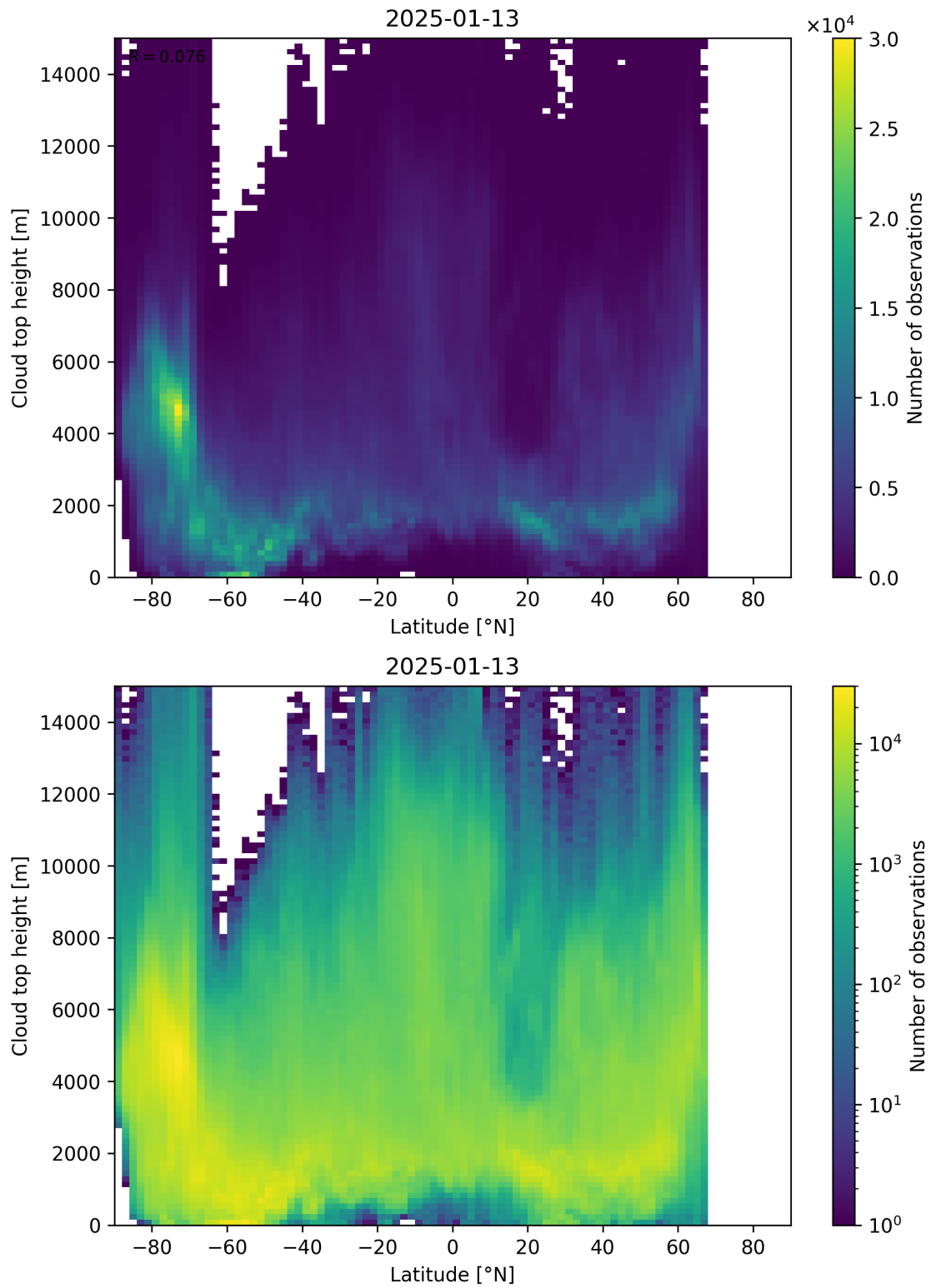
Figure 97: Scatter density plot of “Latitude” against “Cloud top height” for 2025-01-12 to 2025-01-14.
