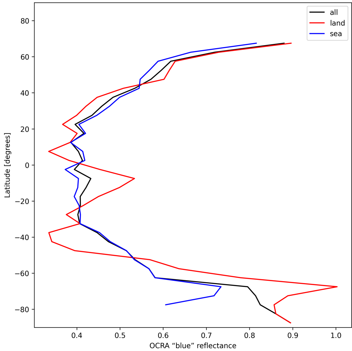
Figure 35: Zonal average of “OCRA “blue” reflectance” for 2025-01-12 to 2025-01-14.
