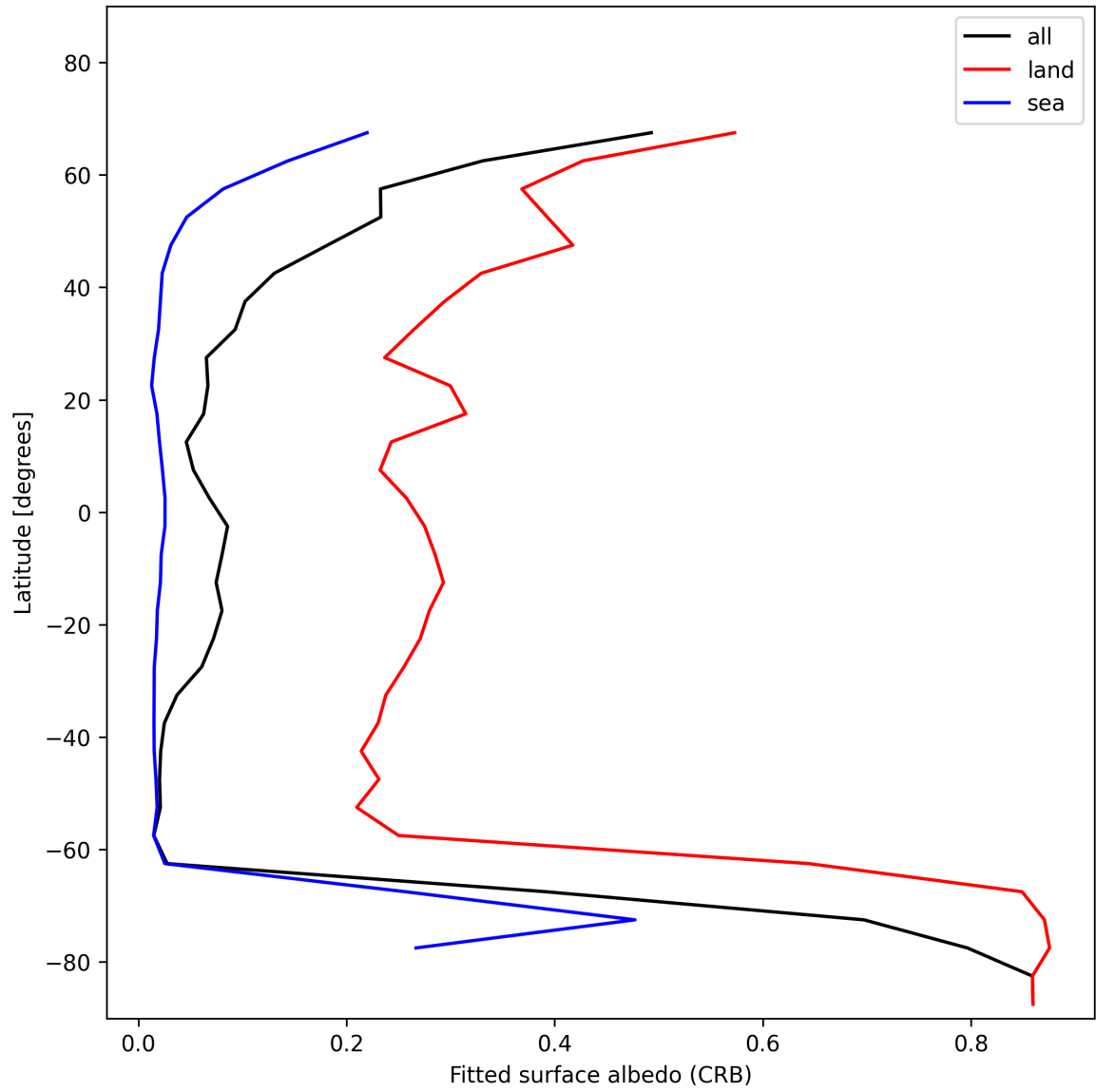
Figure 30: Zonal average of “Fitted surface albedo (CRB)” for 2025-01-12 to 2025-01-14.
