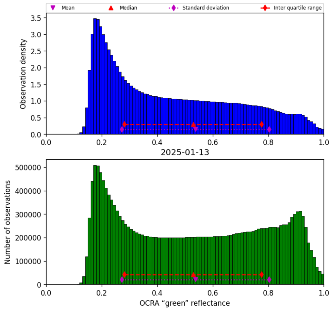
Figure 52: Histogram of “OCRA “green” reflectance” for 2025-01-12 to 2025-01-14
