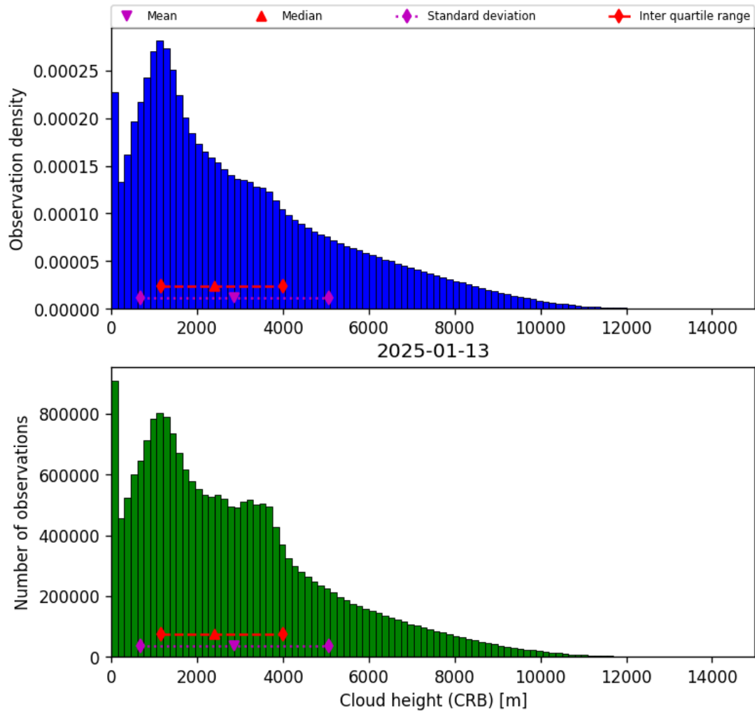
Figure 43: Histogram of “Cloud height (CRB)” for 2025-01-12 to 2025-01-14
