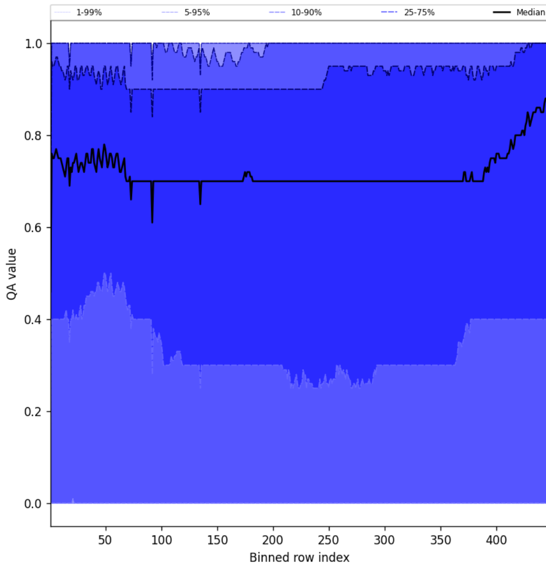
Figure 54: Along track statistics of “QA value” for 2025-01-12 to 2025-01-14
