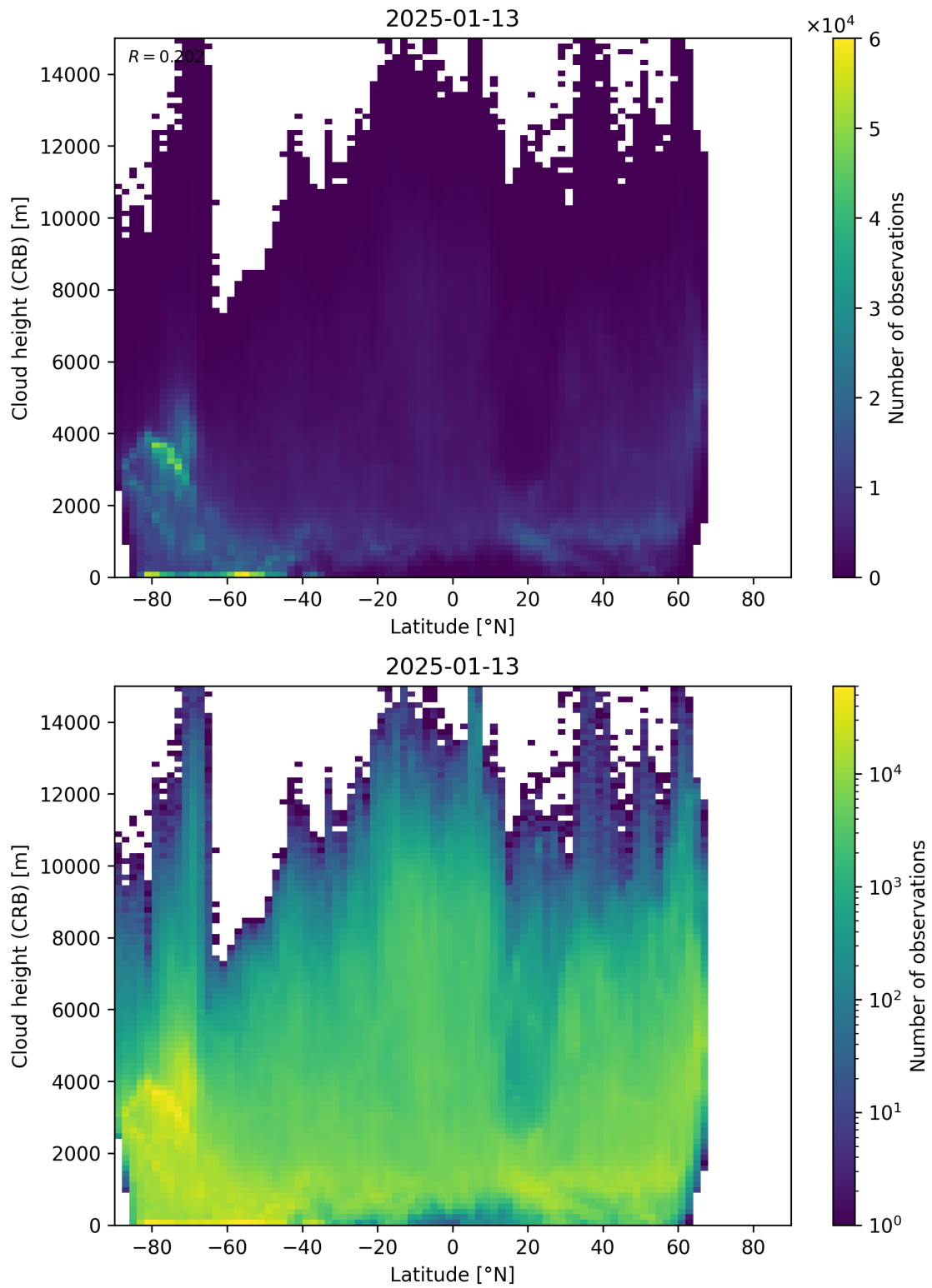
Figure 95: Scatter density plot of “Latitude” against “Cloud height (CRB)” for 2025-01-12 to 2025-01-14.
