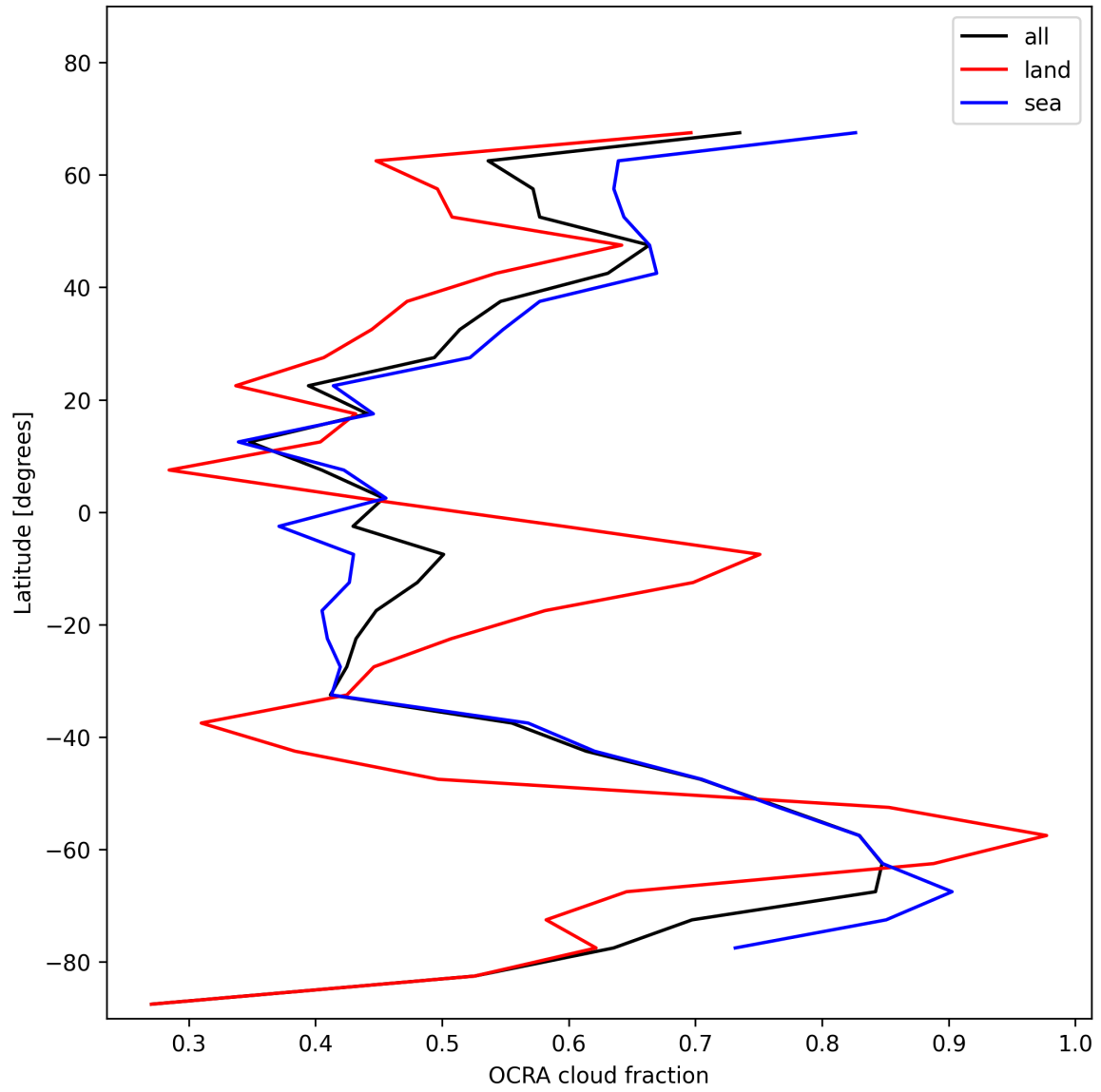
Figure 34: Zonal average of “OCRA cloud fraction” for 2025-01-12 to 2025-01-14.
