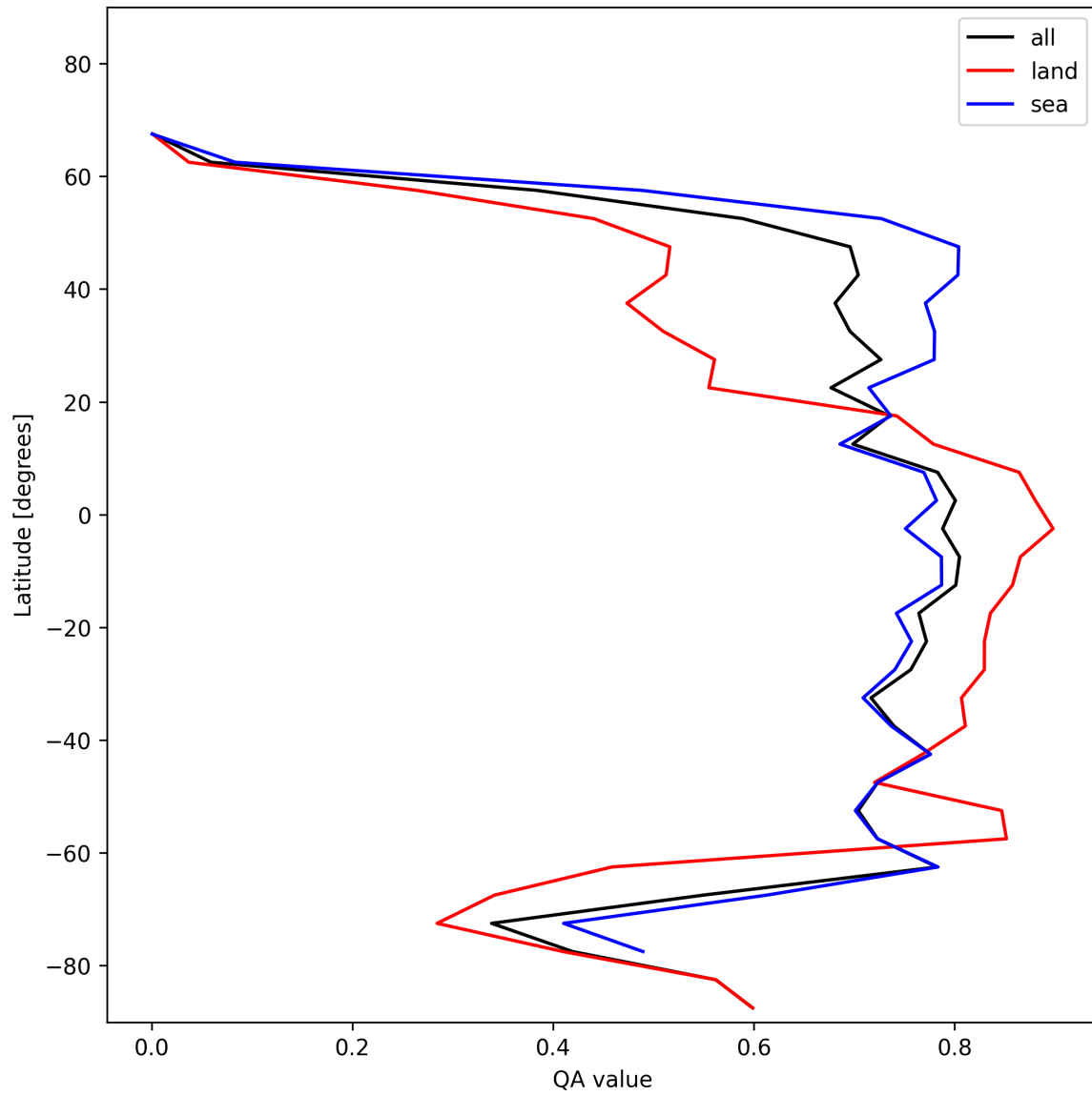
Figure 22: Zonal average of “QA value” for 2025-01-12 to 2025-01-14.
