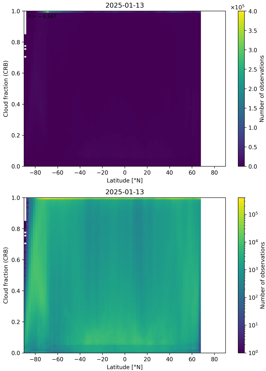
Figure 94: Scatter density plot of “Latitude” against “Cloud fraction (CRB)” for 2025-01-12 to 2025-01-14.
