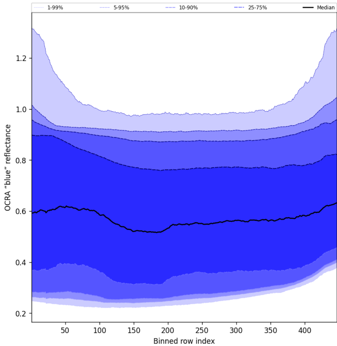
Figure 67: Along track statistics of “OCRA “blue” reflectance” for 2025-01-12 to 2025-01-14
