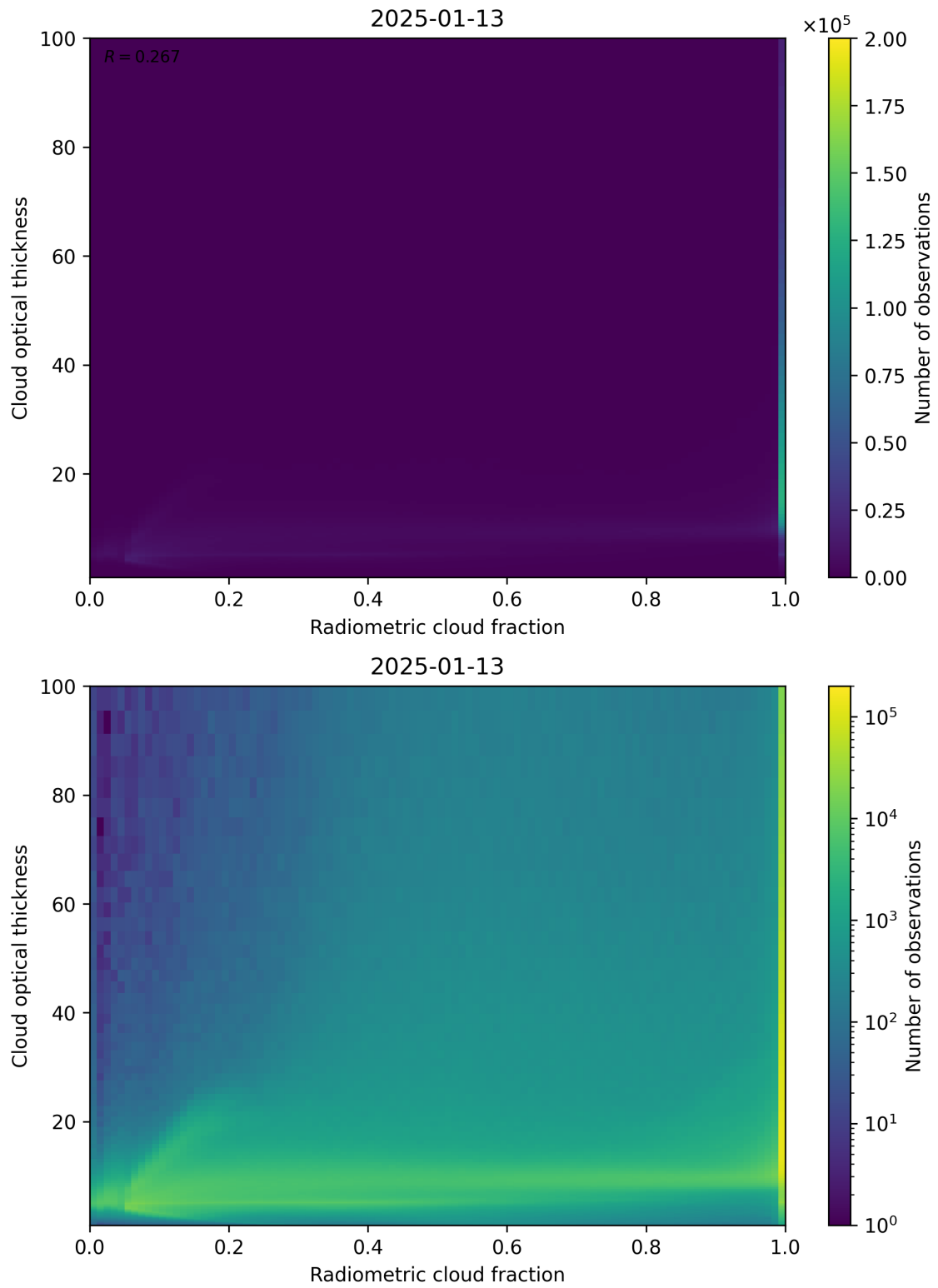
Figure 75: Scatter density plot of “Radiometric cloud fraction” against “Cloud optical thickness” for 2025-01-12 to 2025-01-14.
