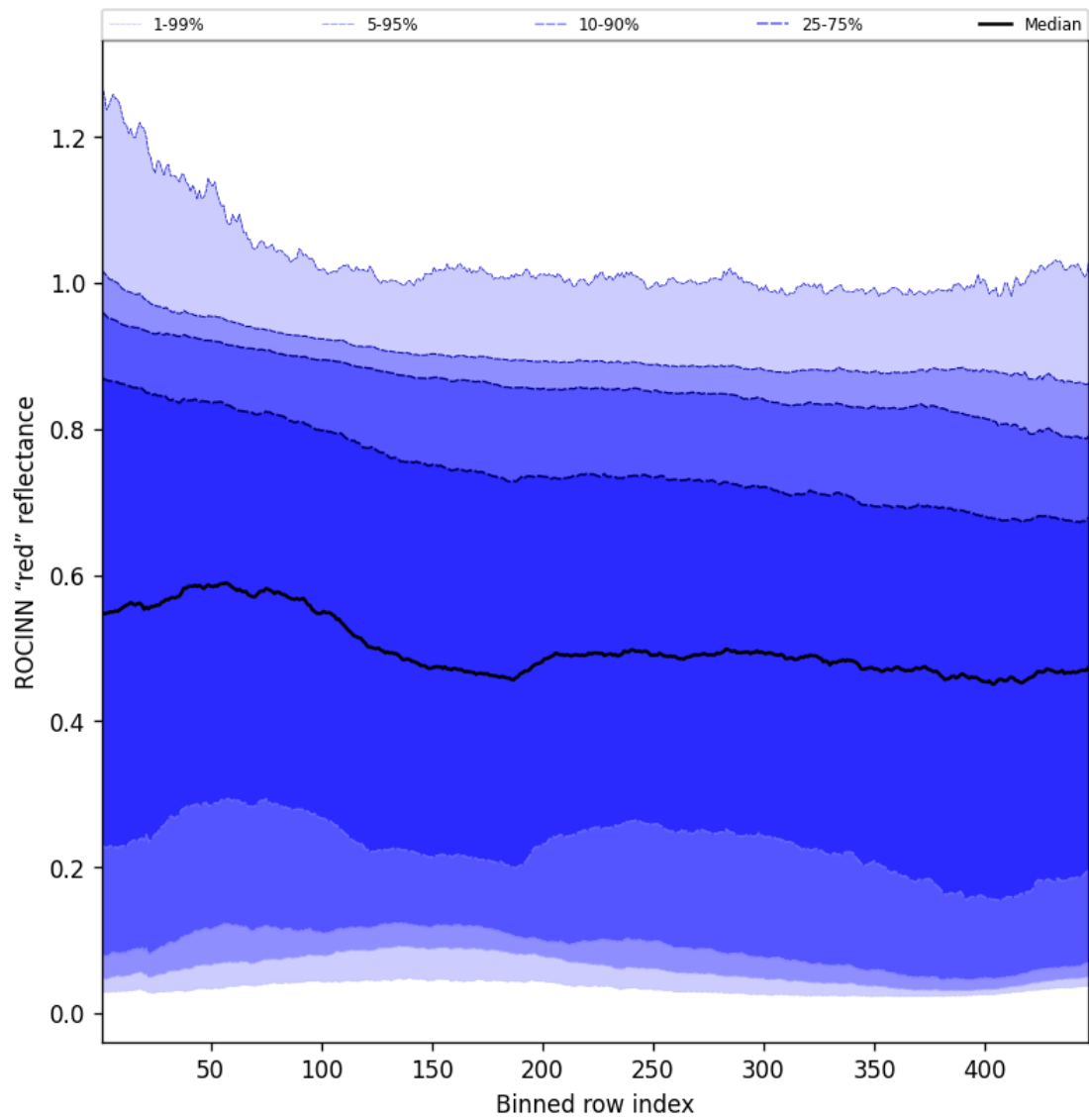
Figure 69: Along track statistics of “ROCINN “red” reflectance” for 2025-01-12 to 2025-01-14
