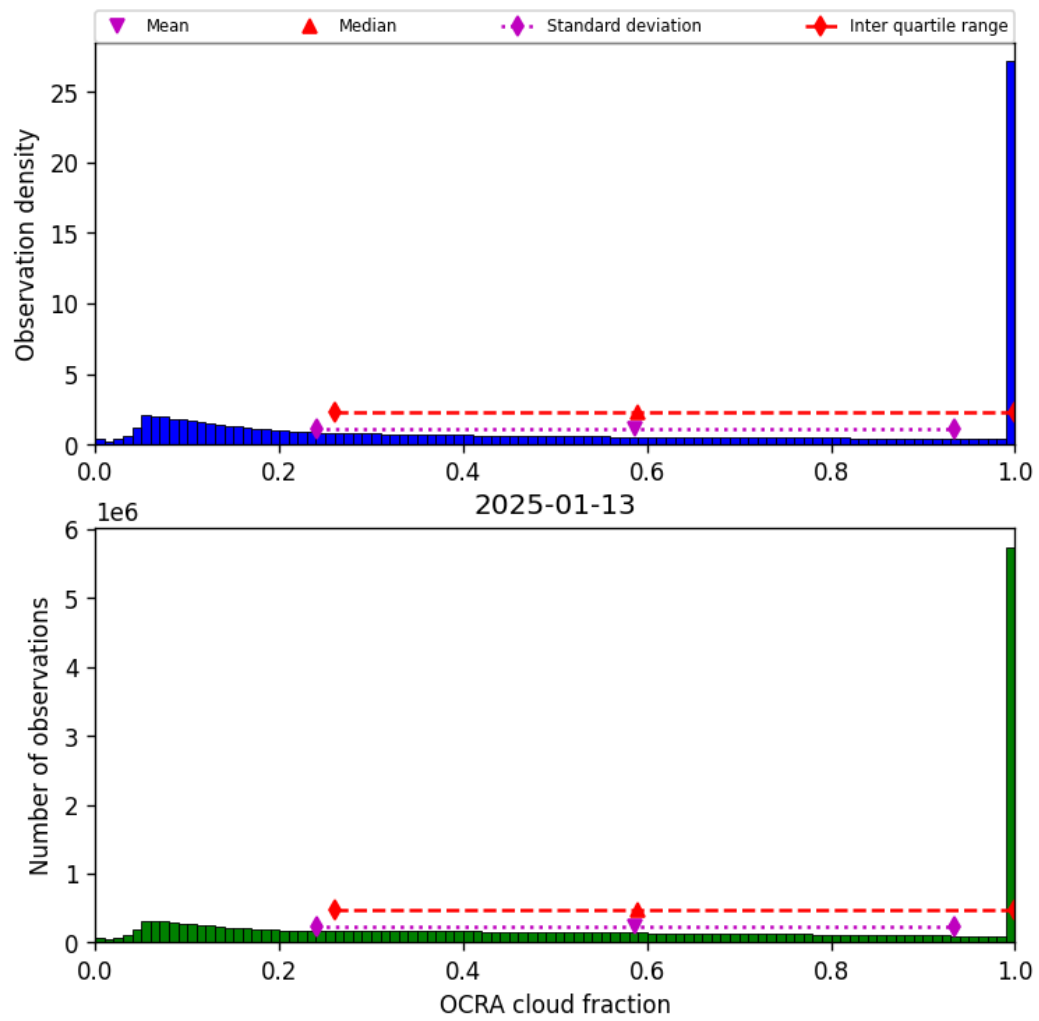
Figure 50: Histogram of “OCRA cloud fraction” for 2025-01-12 to 2025-01-14
