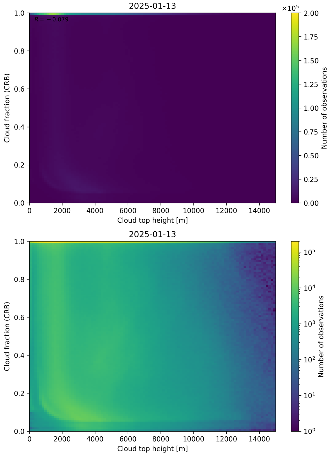
Figure 88: Scatter density plot of “Cloud top height” against “Cloud fraction (CRB)” for 2025-01-12 to 2025-01-14.
