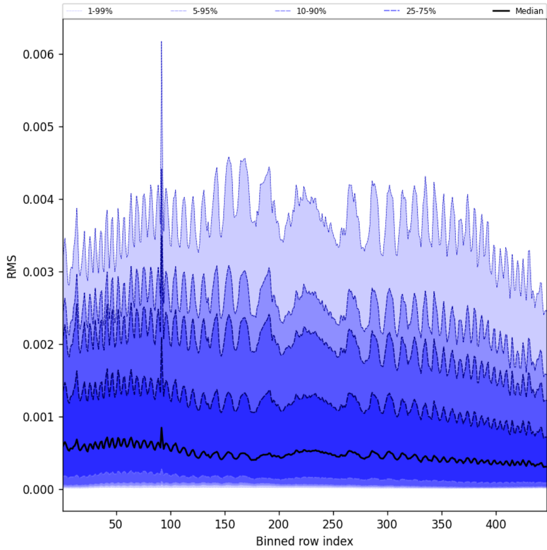
Figure 63: Along track statistics of “RMS” for 2025-01-12 to 2025-01-14
