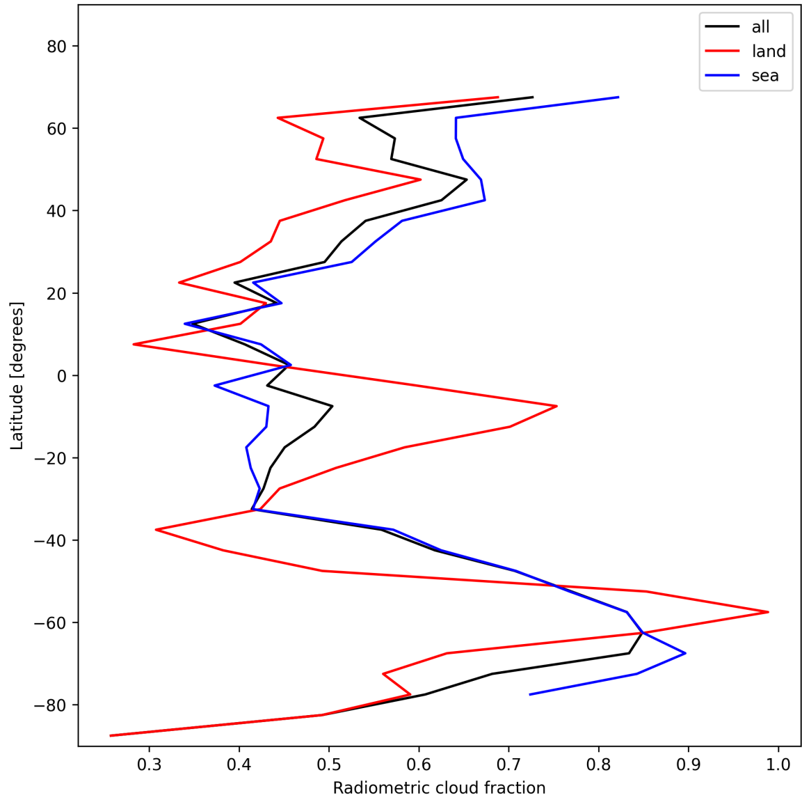
Figure 23: Zonal average of “Radiometric cloud fraction” for 2025-01-12 to 2025-01-14.
