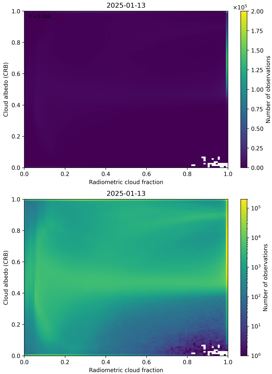
Figure 71: Scatter density plot of “Radiometric cloud fraction” against “Cloud albedo (CRB)” for 2025-01-12 to 2025-01-14.
