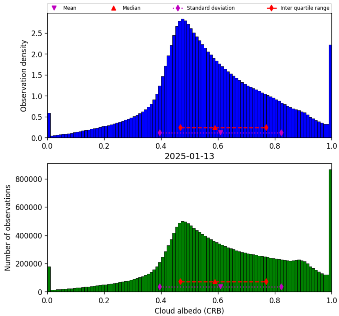
Figure 44: Histogram of “Cloud albedo (CRB)” for 2025-01-12 to 2025-01-14
