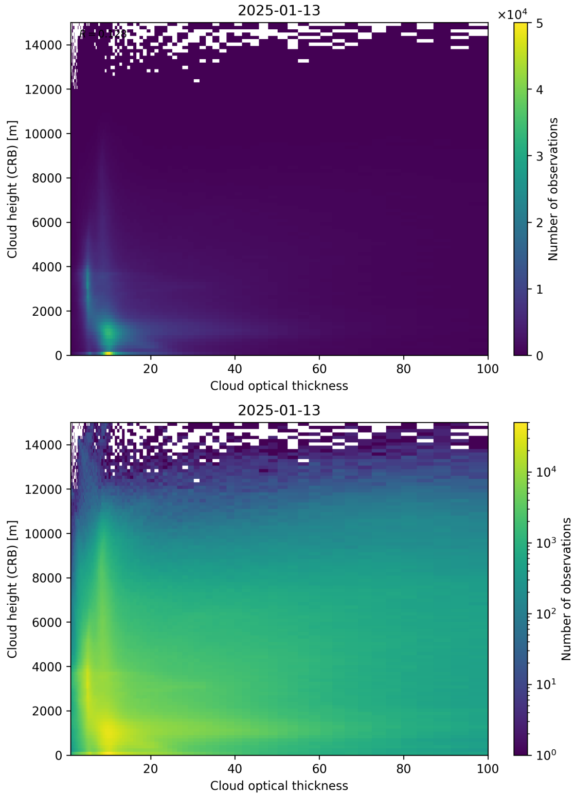
Figure 85: Scatter density plot of “Cloud optical thickness” against “Cloud height (CRB)” for 2025-01-12 to 2025-01-14.
