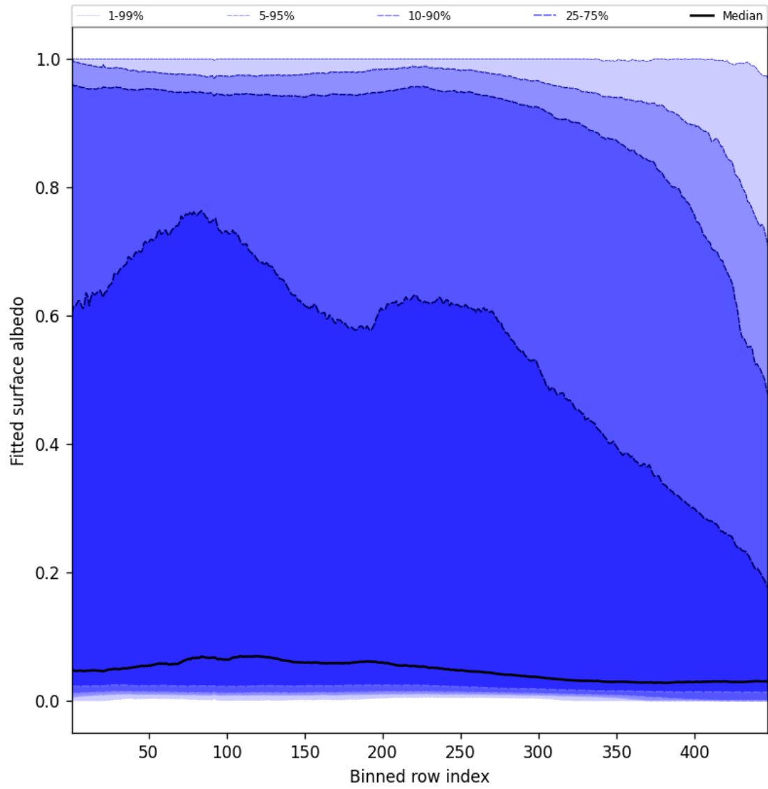
Figure 61: Along track statistics of “Fitted surface albedo” for 2025-01-12 to 2025-01-14
