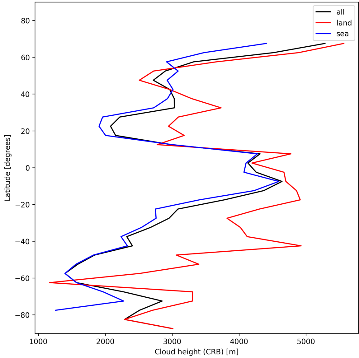
Figure 27: Zonal average of “Cloud height (CRB)” for 2025-01-12 to 2025-01-14.
