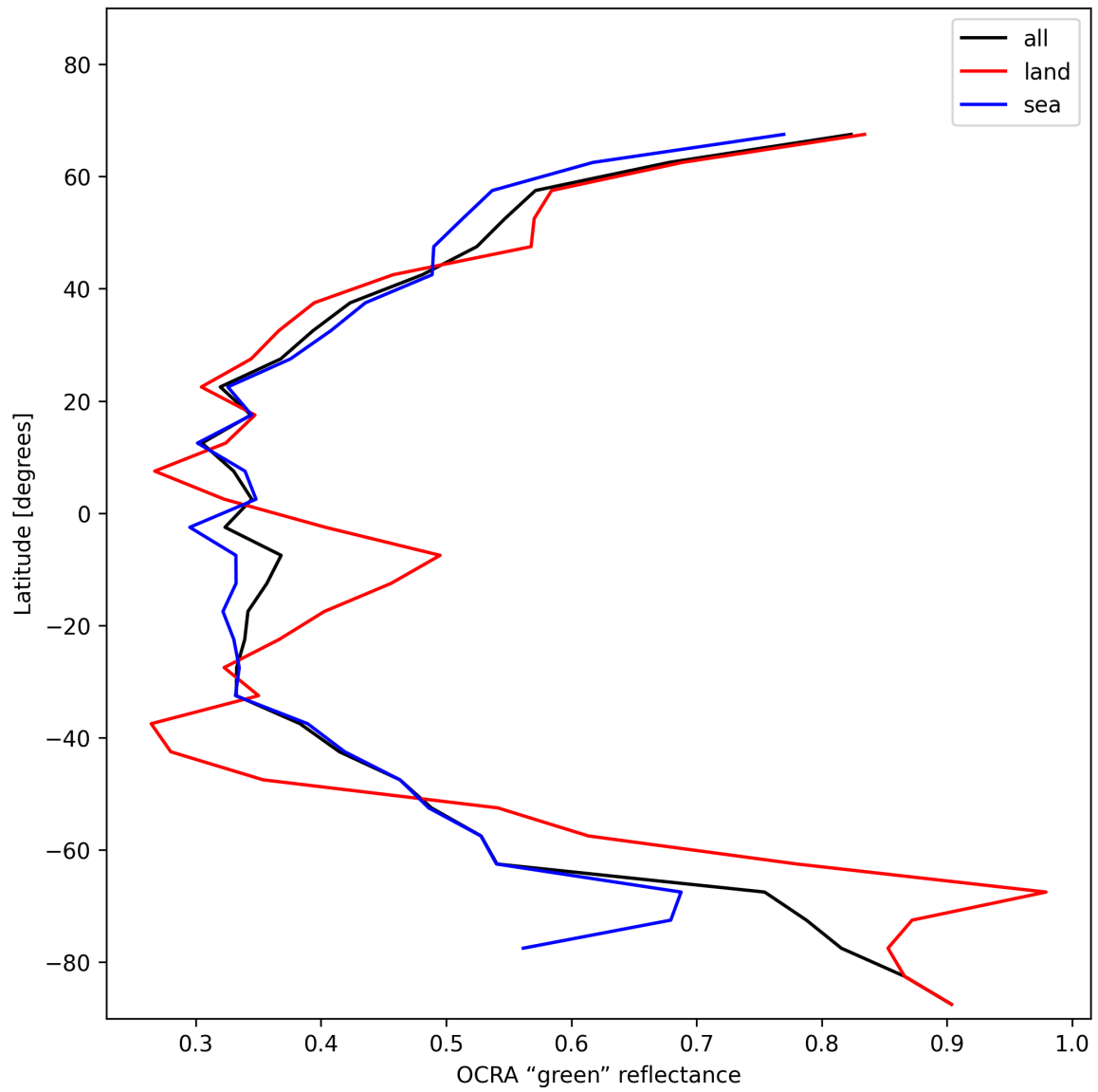
Figure 36: Zonal average of “OCRA “green” reflectance” for 2025-01-12 to 2025-01-14.
