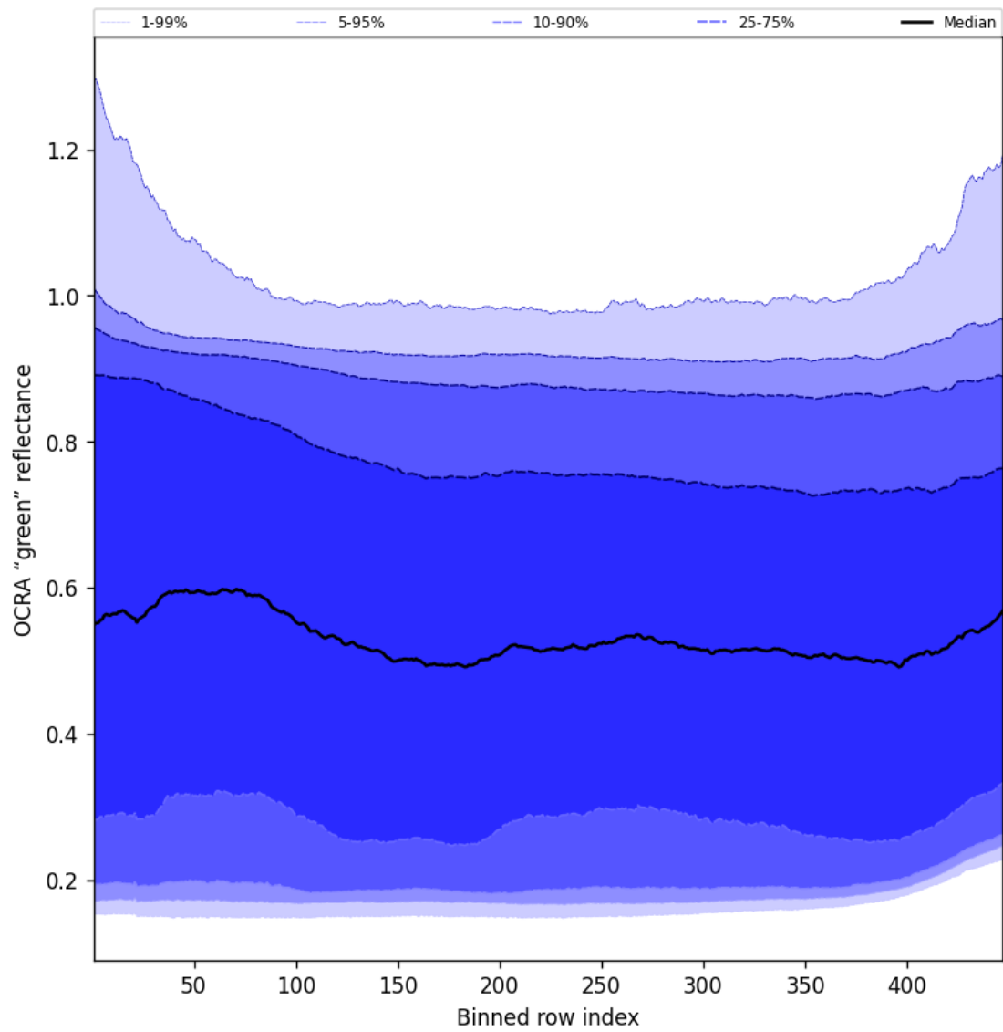
Figure 68: Along track statistics of "OCRA "green" reflectance" for 2025-01-13 to 2025-01-15
