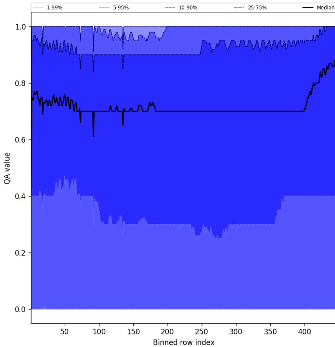
Figure 54: Along track statistics of “QA value” for 2025-01-13 to 2025-01-15
