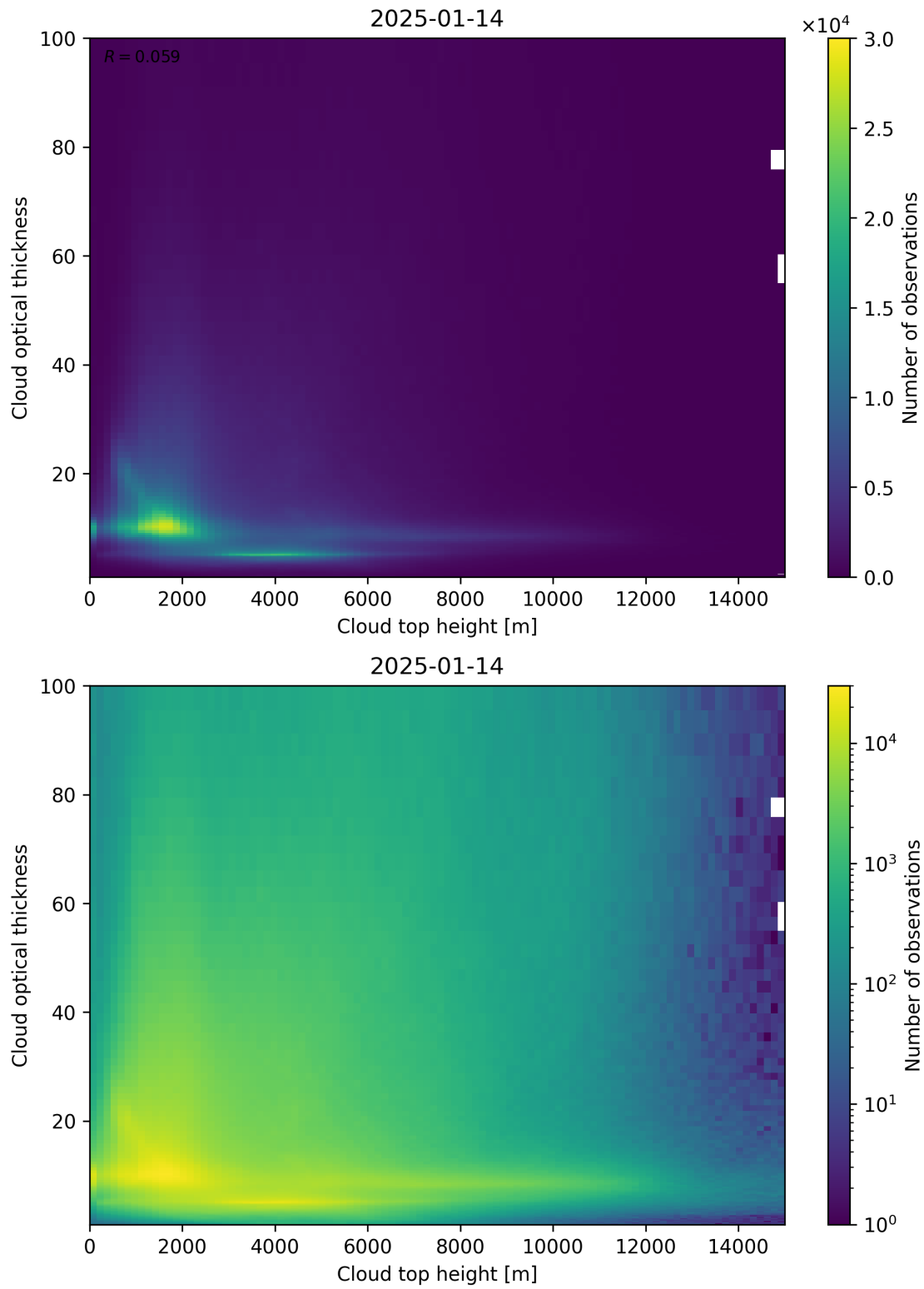
Figure 90: Scatter density plot of “Cloud top height” against “Cloud optical thickness” for 2025-01-13 to 2025-01-15.
