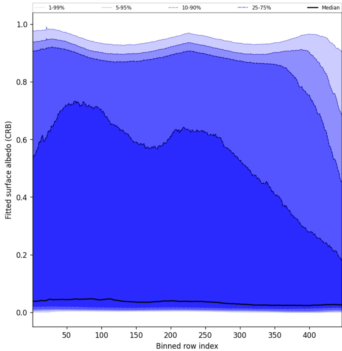
Figure 62: Along track statistics of “Fitted surface albedo (CRB)” for 2025-01-13 to 2025-01-15
