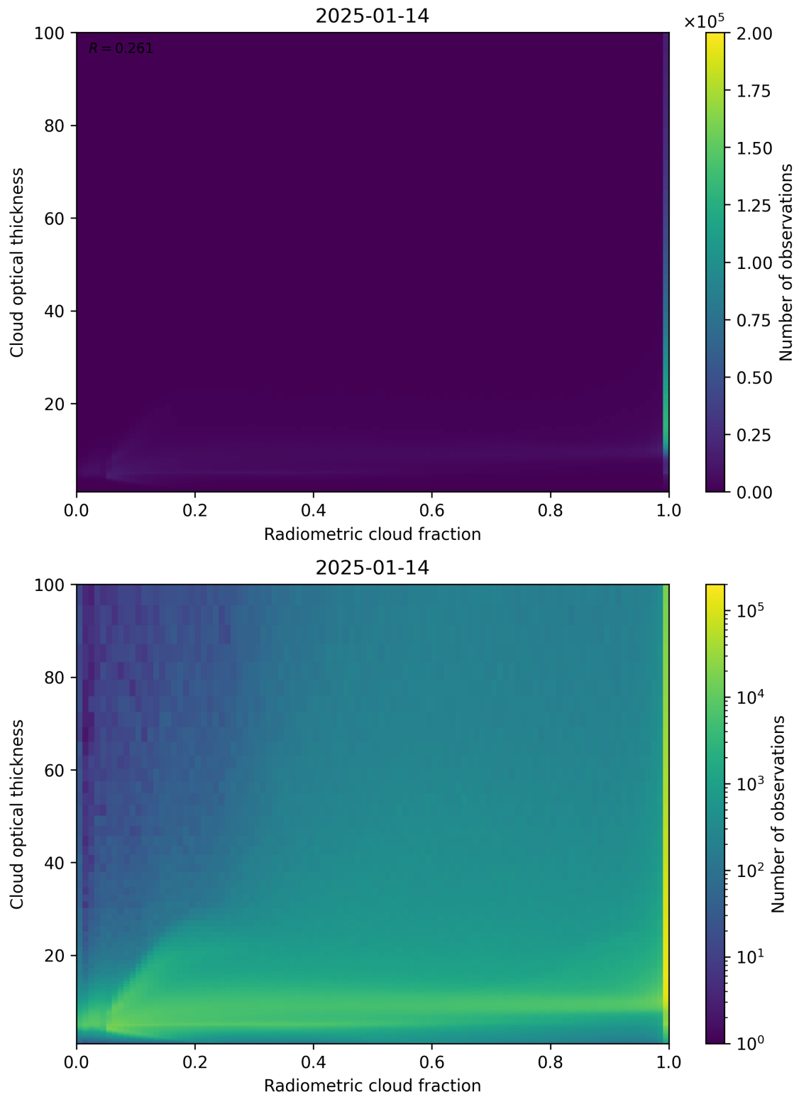
Figure 75: Scatter density plot of “Radiometric cloud fraction” against “Cloud optical thickness” for 2025-01-13 to 2025-01-15.
