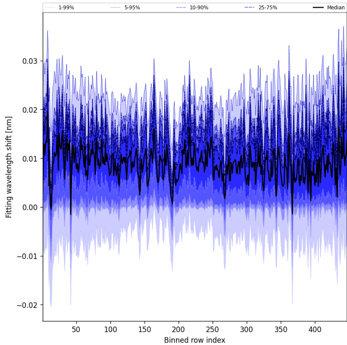
Figure 65: Along track statistics of “Fitting wavelength shift” for 2025-01-13 to 2025-01-15
