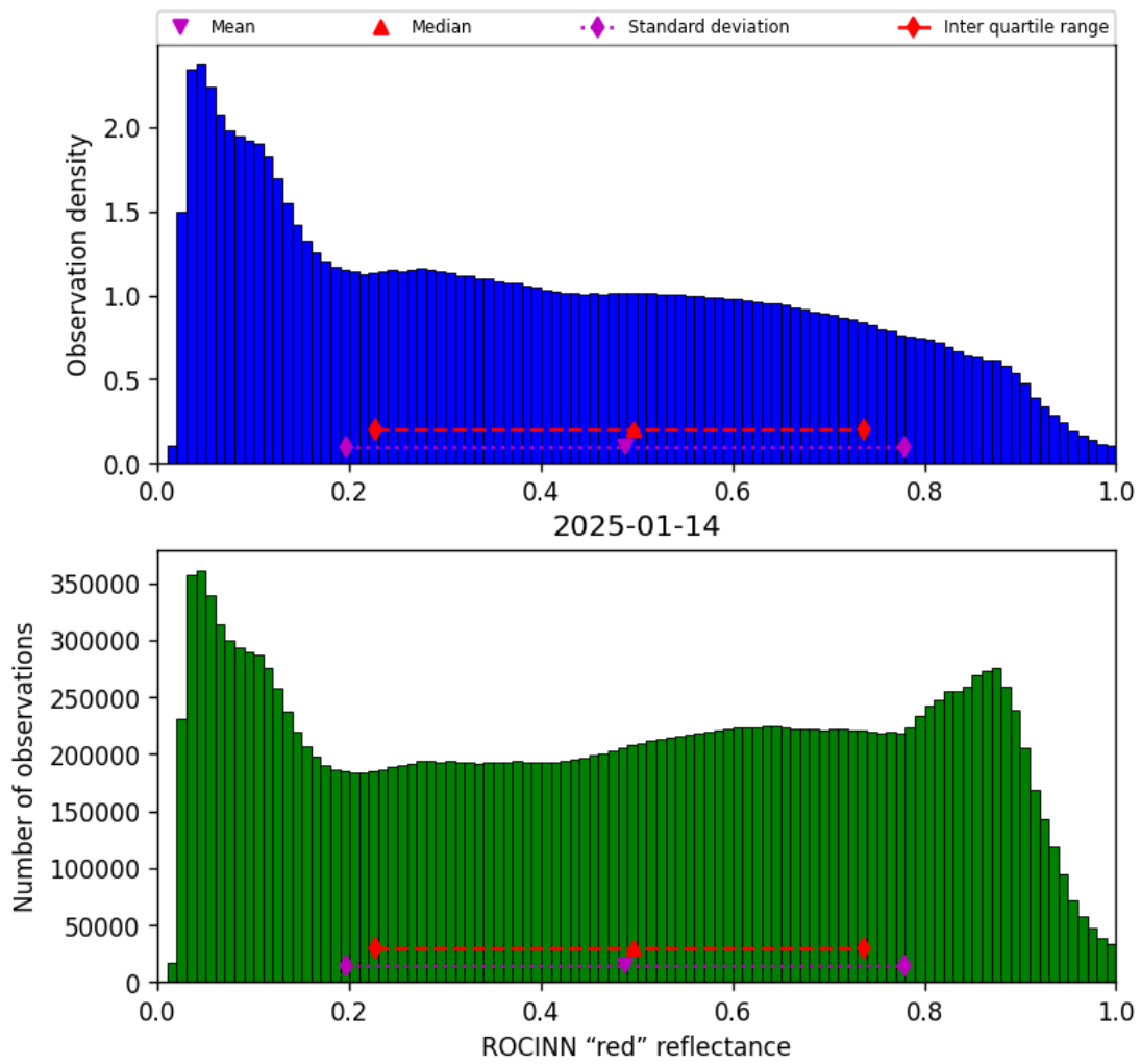
Figure 53: Histogram of “ROCINN “red” reflectance” for 2025-01-13 to 2025-01-15
