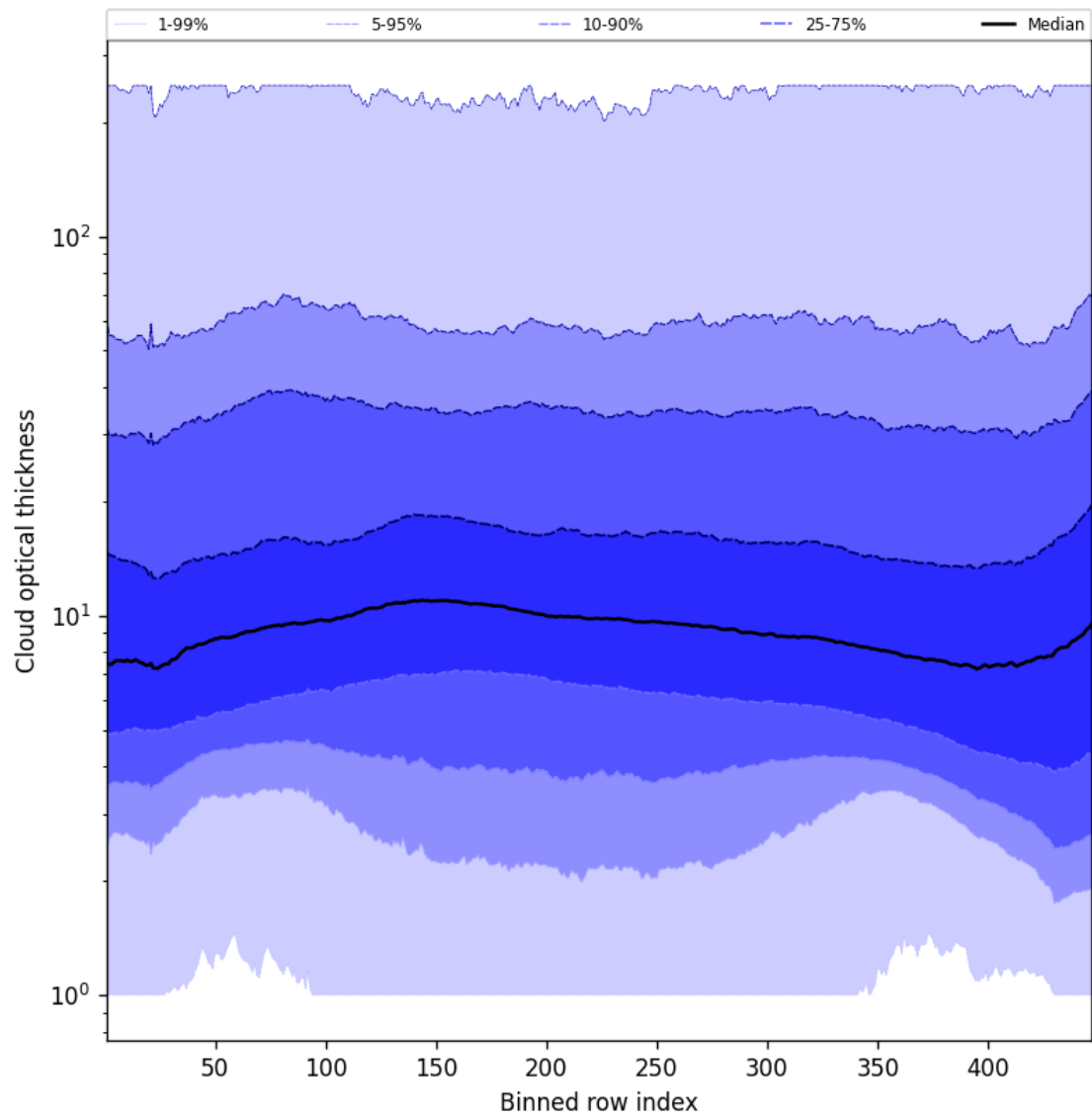
Figure 57: Along track statistics of “Cloud optical thickness” for 2025-01-13 to 2025-01-15
