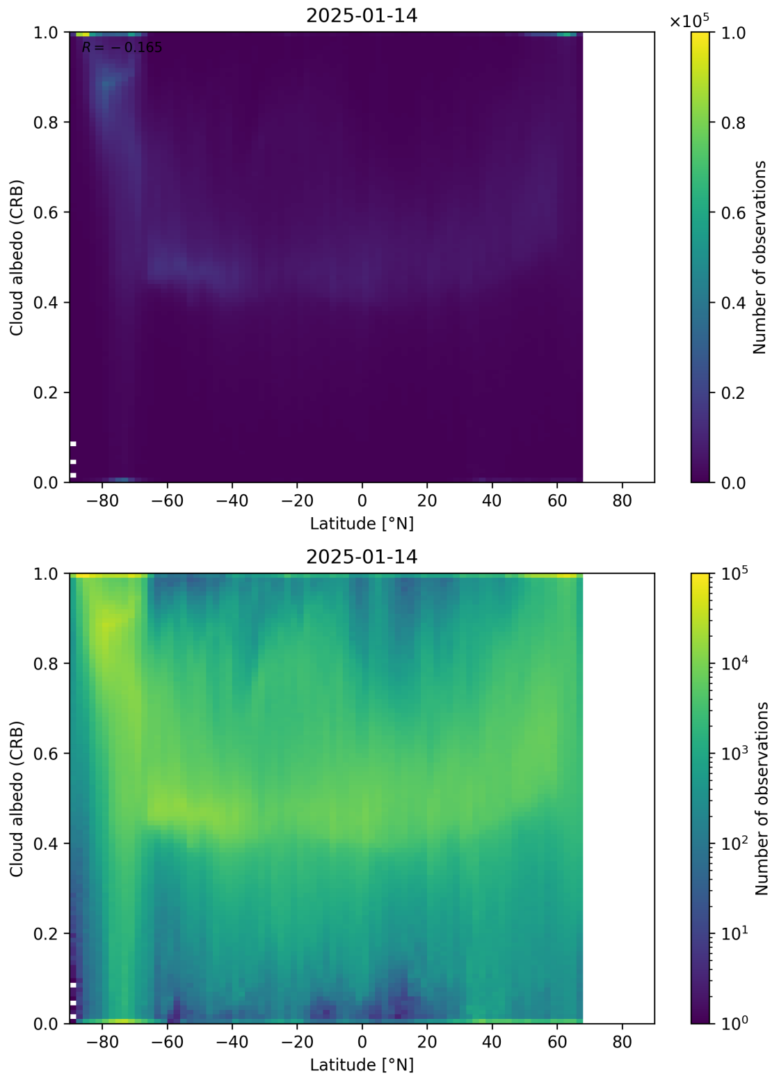
Figure 91: Scatter density plot of “Latitude” against “Cloud albedo (CRB)” for 2025-01-13 to 2025-01-15.
