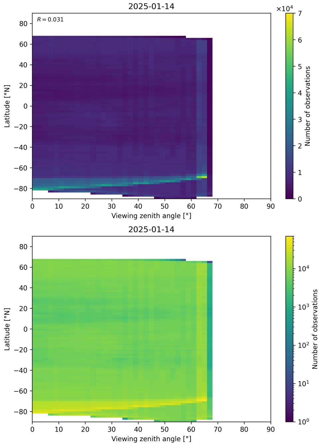
Figure 113: Scatter density plot of “Viewing zenith angle” against “Latitude” for 2025-01-13 to 2025-01-15.
