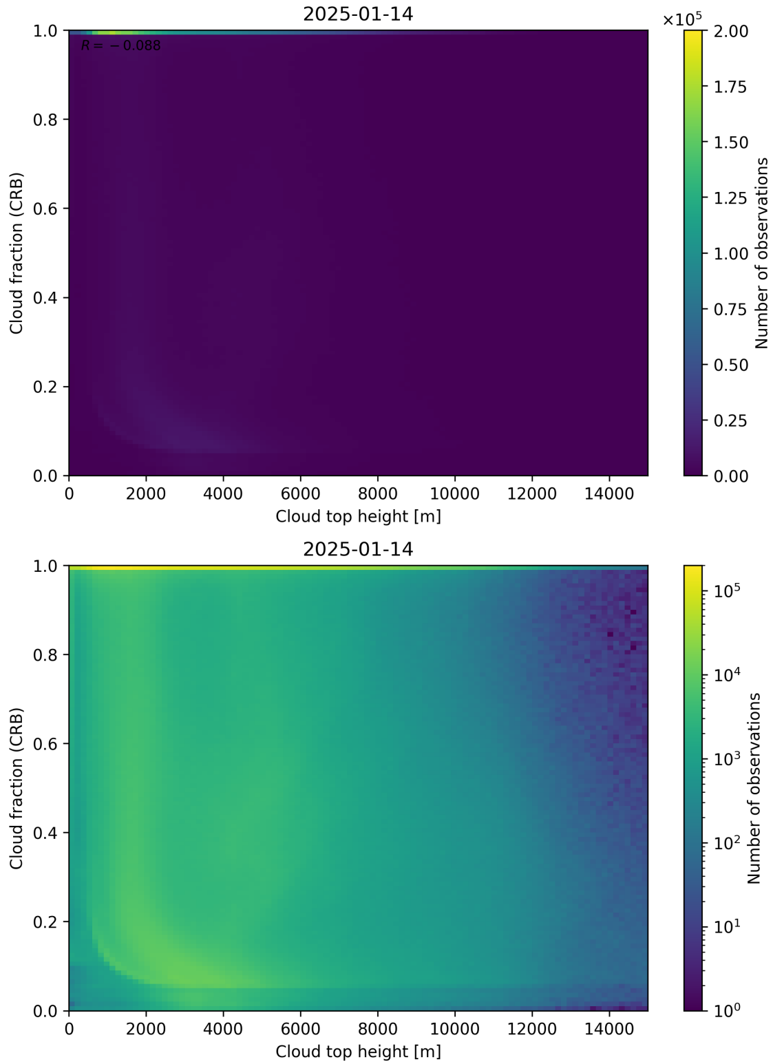
Figure 88: Scatter density plot of “Cloud top height” against “Cloud fraction (CRB)” for 2025-01-13 to 2025-01-15.
