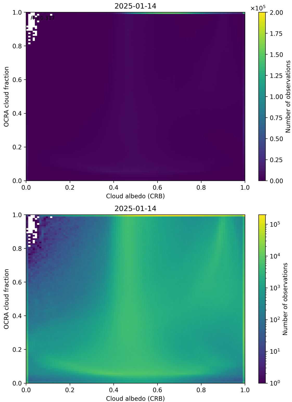
Figure 70: Scatter density plot of “Cloud albedo (CRB)” against “OCRA cloud fraction” for 2025-01-13 to 2025-01-15.
