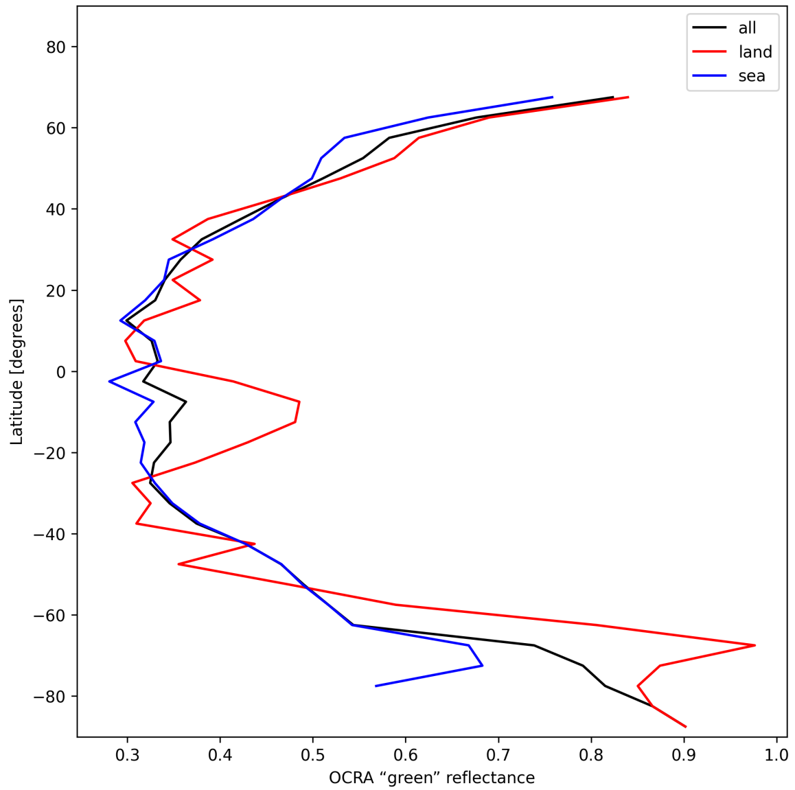
Figure 36: Zonal average of “OCRA “green” reflectance” for 2025-01-13 to 2025-01-15.
