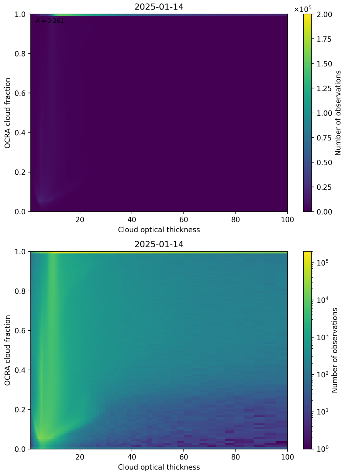
Figure 83: Scatter density plot of “Cloud optical thickness” against “OCRA cloud fraction” for 2025-01-13 to 2025-01-15.
