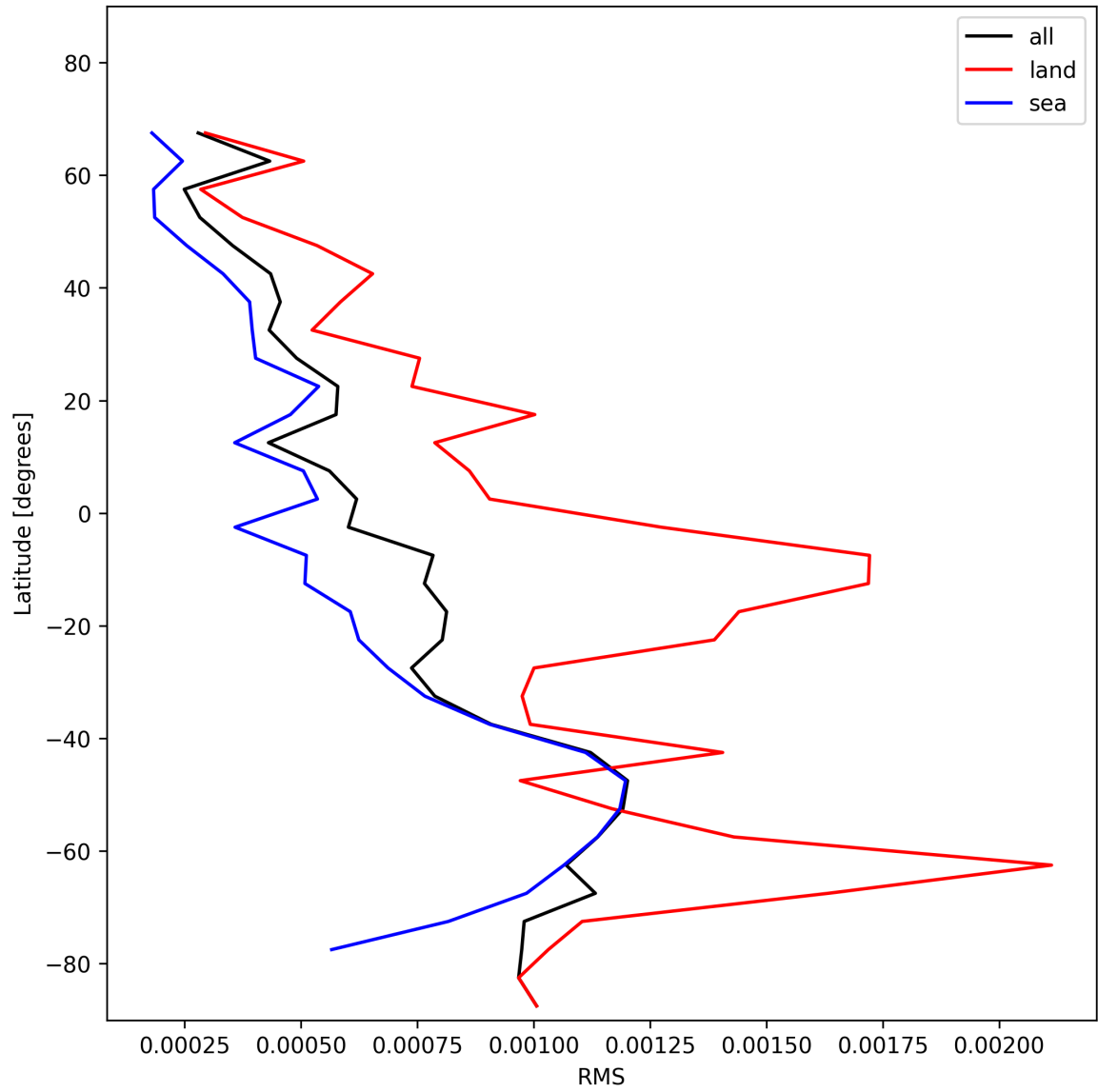
Figure 31: Zonal average of “RMS” for 2025-01-13 to 2025-01-15.
