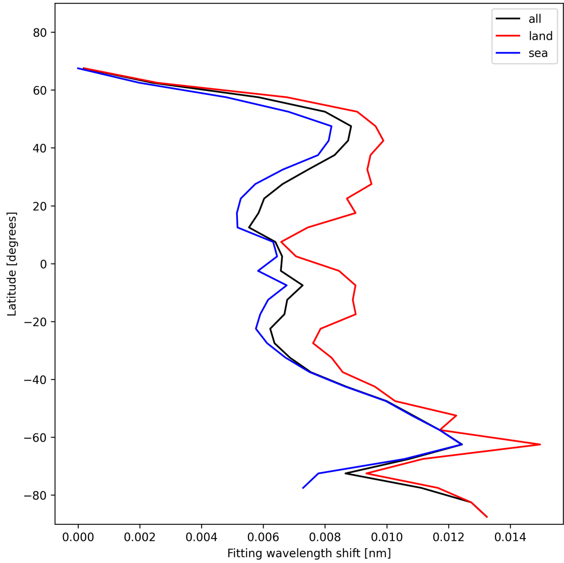
Figure 33: Zonal average of “Fitting wavelength shift” for 2025-01-13 to 2025-01-15.
