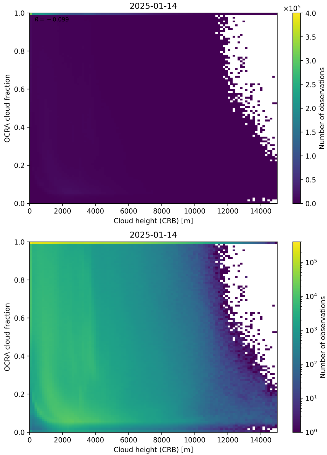
Figure 81: Scatter density plot of “Cloud height (CRB)” against “OCRA cloud fraction” for 2025-01-13 to 2025-01-15.
