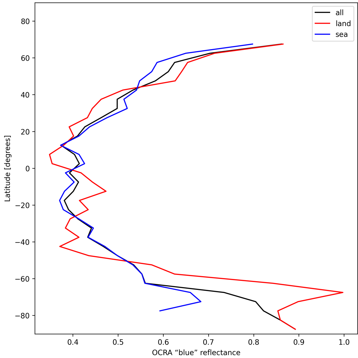
Figure 35: Zonal average of “OCRA “blue” reflectance” for 2025-01-15 to 2025-01-17.
