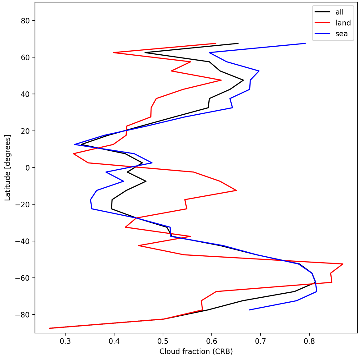
Figure 26: Zonal average of “Cloud fraction (CRB)” for 2025-01-15 to 2025-01-17.
