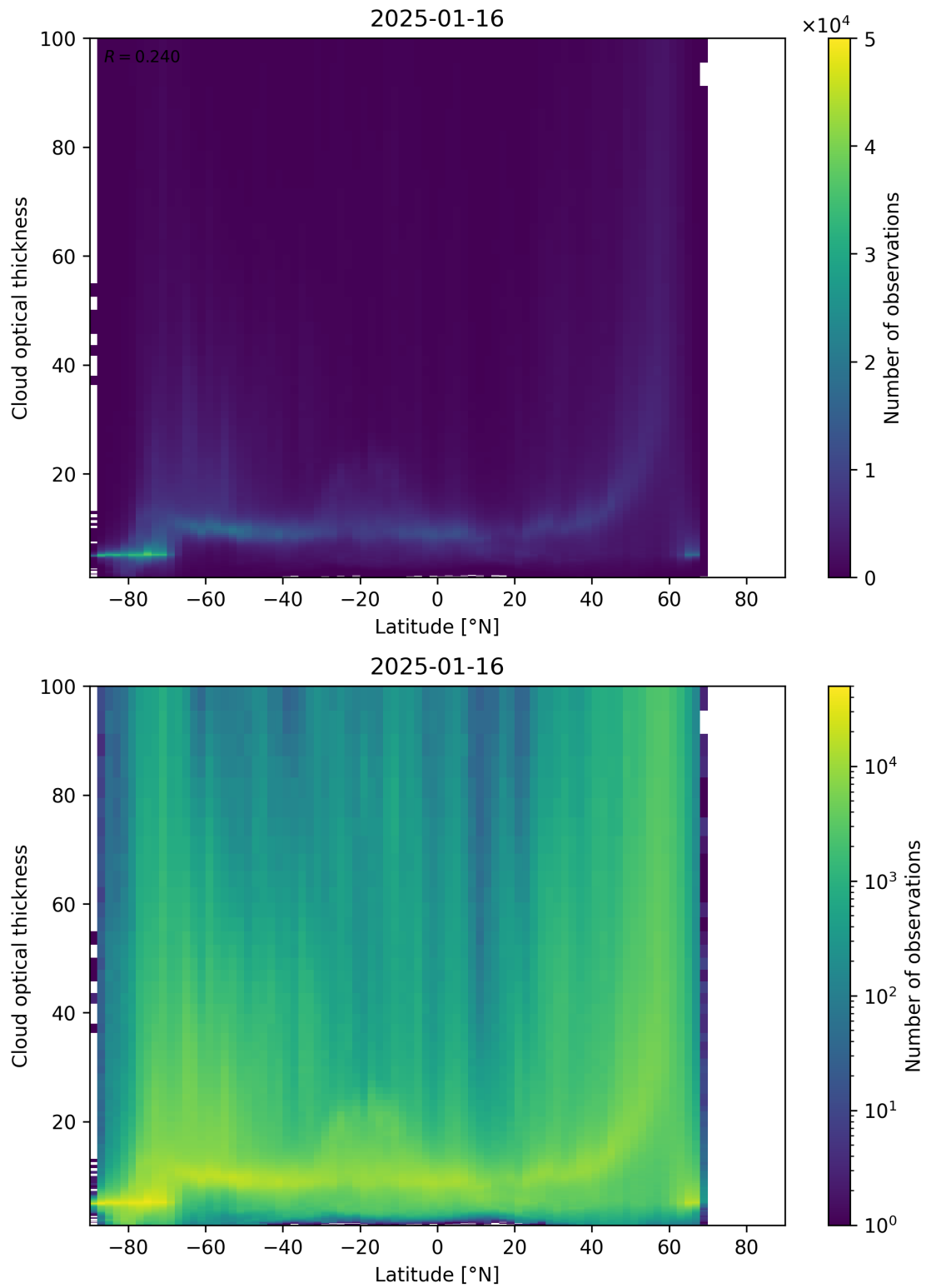
Figure 96: Scatter density plot of “Latitude” against “Cloud optical thickness” for 2025-01-15 to 2025-01-17.
