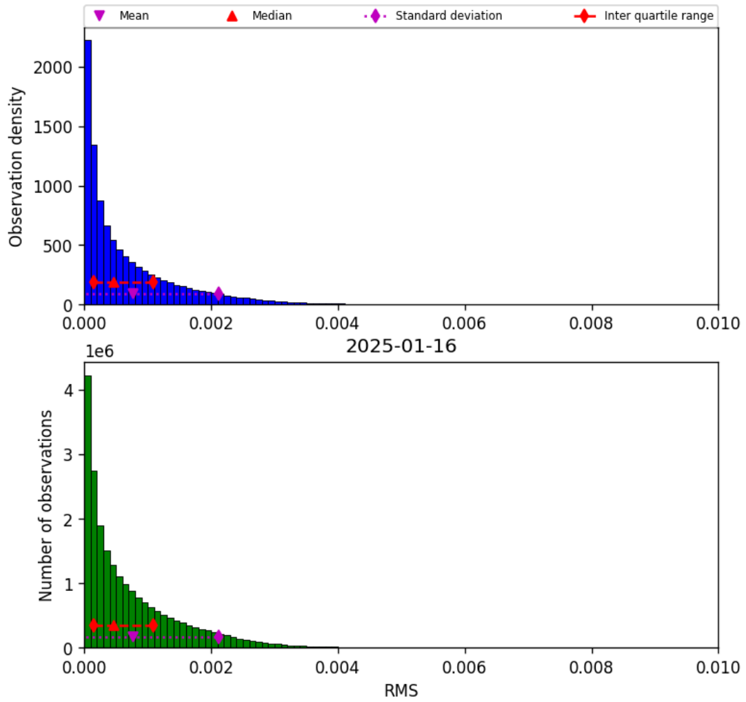
Figure 47: Histogram of “RMS” for 2025-01-15 to 2025-01-17
