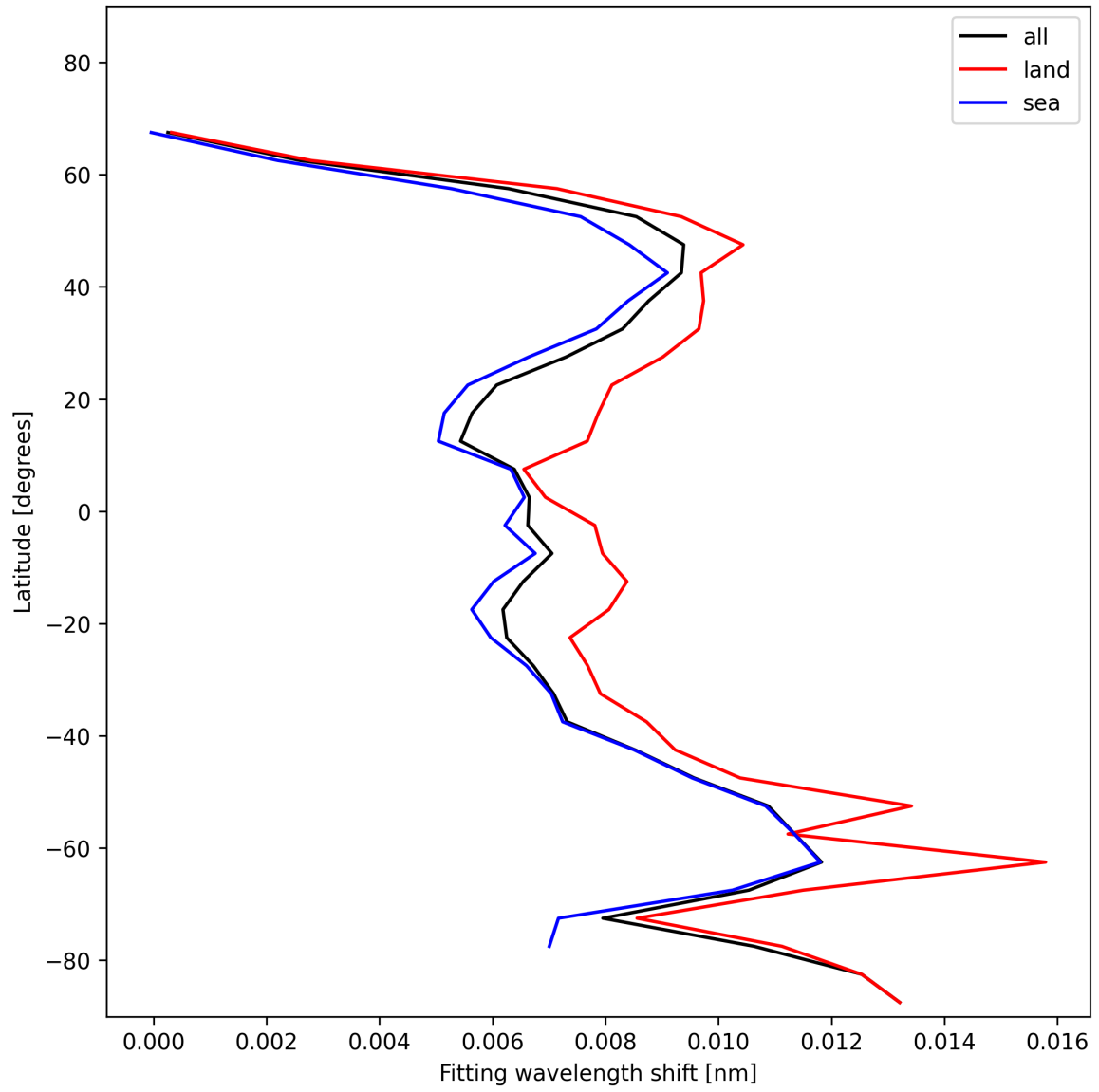
Figure 33: Zonal average of “Fitting wavelength shift” for 2025-01-15 to 2025-01-17.
