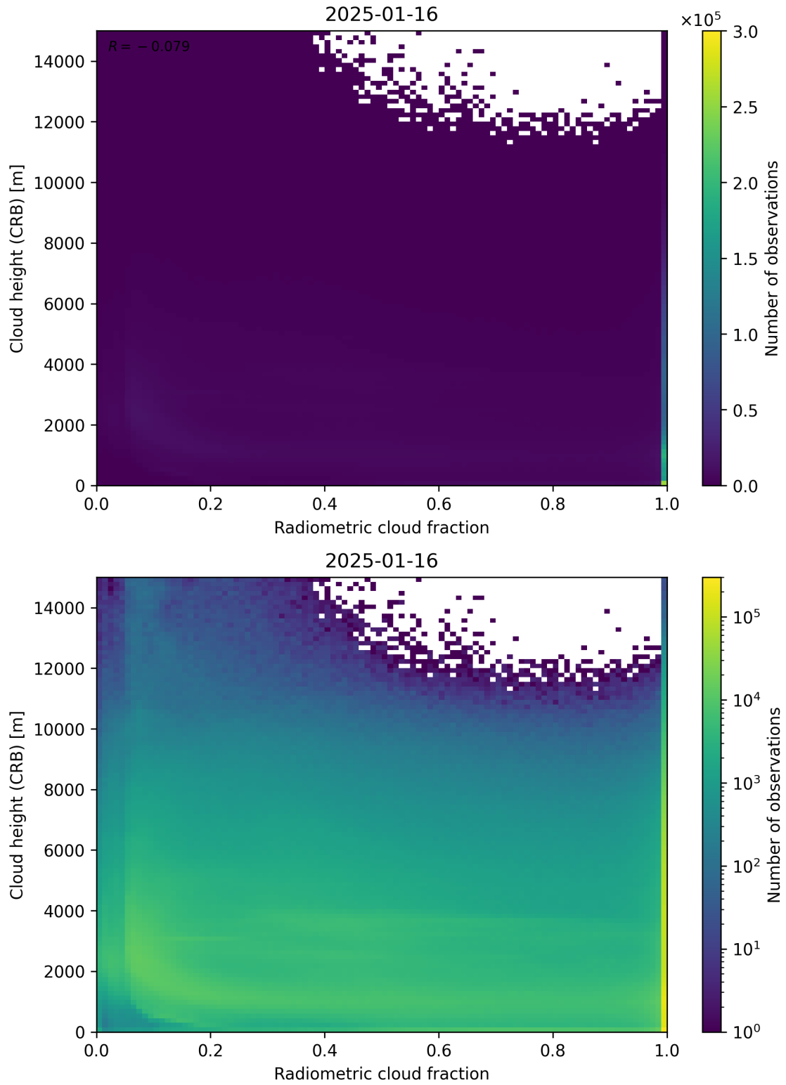
Figure 74: Scatter density plot of “Radiometric cloud fraction” against “Cloud height (CRB)” for 2025-01-15 to 2025-01-17.
