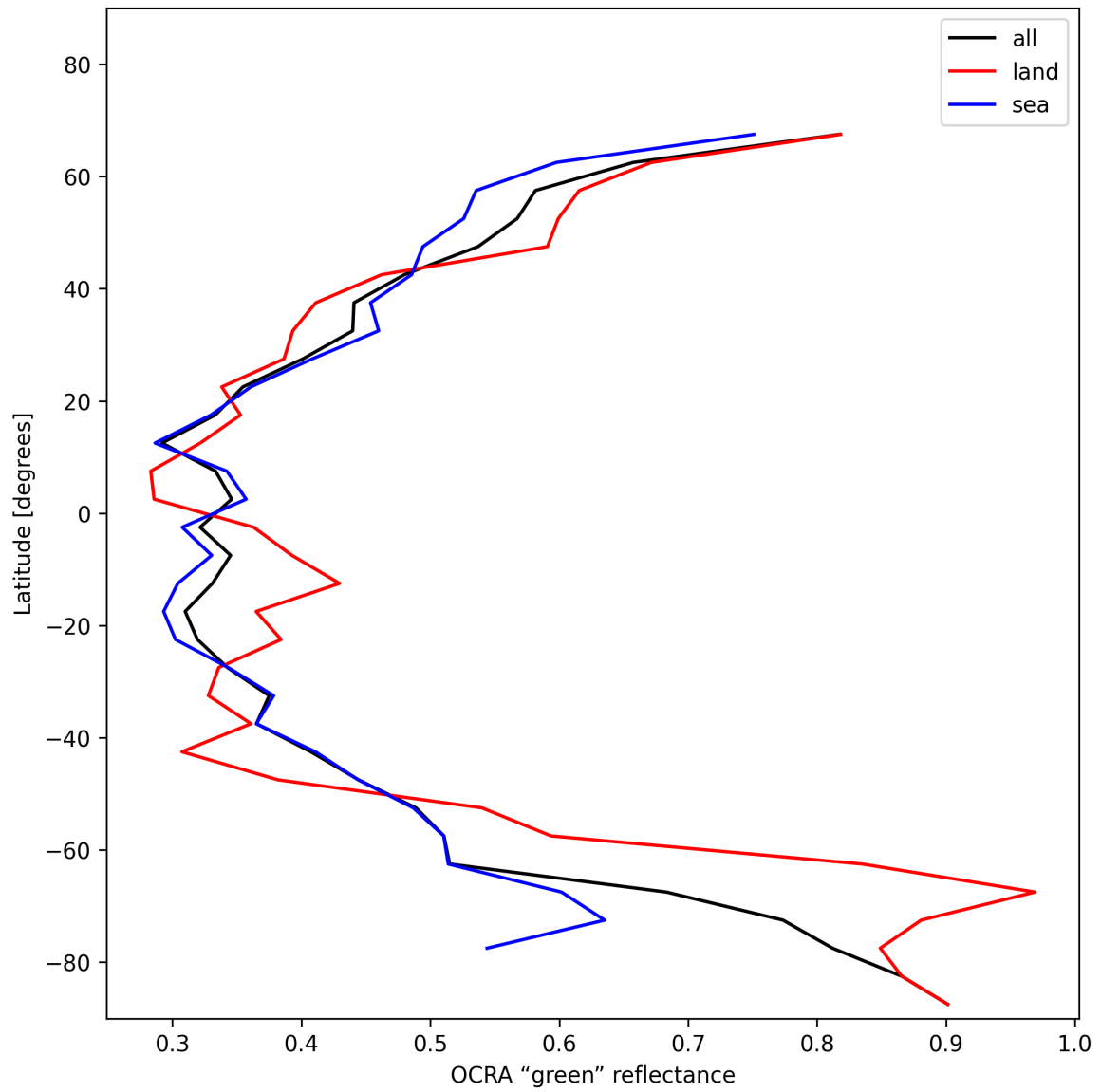
Figure 36: Zonal average of “OCRA “green” reflectance” for 2025-01-15 to 2025-01-17.
