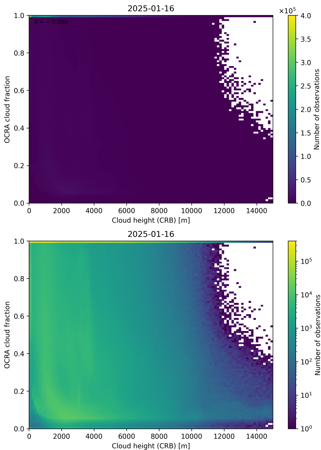
Figure 81: Scatter density plot of “Cloud height (CRB)” against “OCRA cloud fraction” for 2025-01-15 to 2025-01-17.
