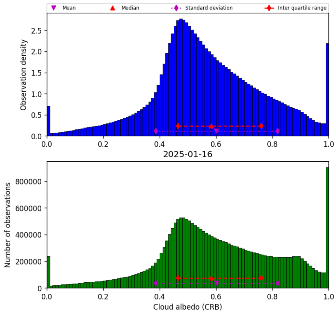
Figure 44: Histogram of “Cloud albedo (CRB)” for 2025-01-15 to 2025-01-17
