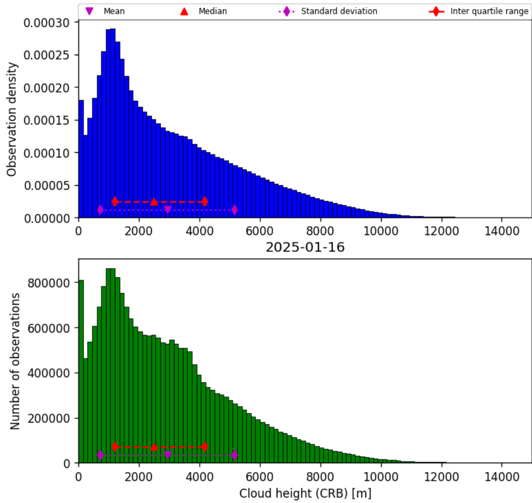
Figure 43: Histogram of “Cloud height (CRB)” for 2025-01-15 to 2025-01-17
