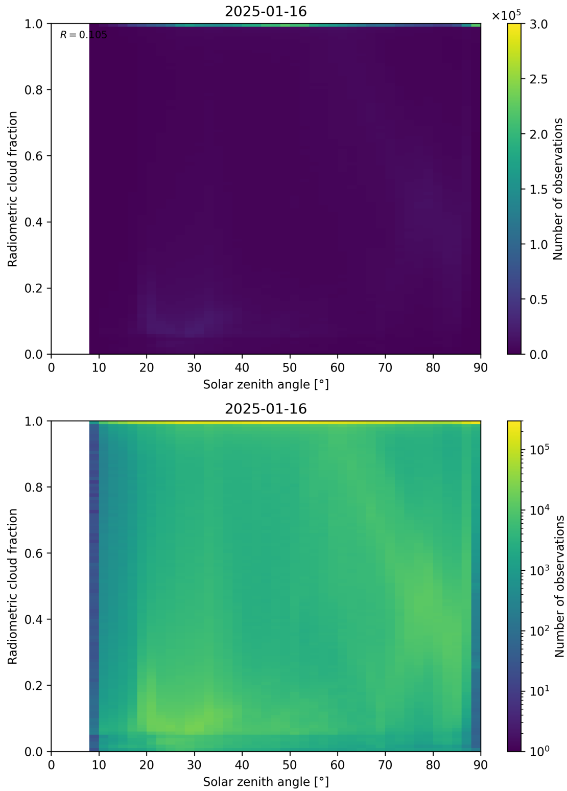
Figure 99: Scatter density plot of “Solar zenith angle” against “Radiometric cloud fraction” for 2025-01-15 to 2025-01-17.
