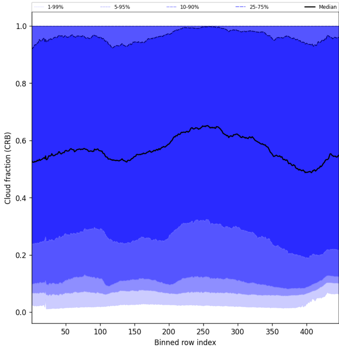
Figure 58: Along track statistics of “Cloud fraction (CRB)” for 2025-01-15 to 2025-01-17
