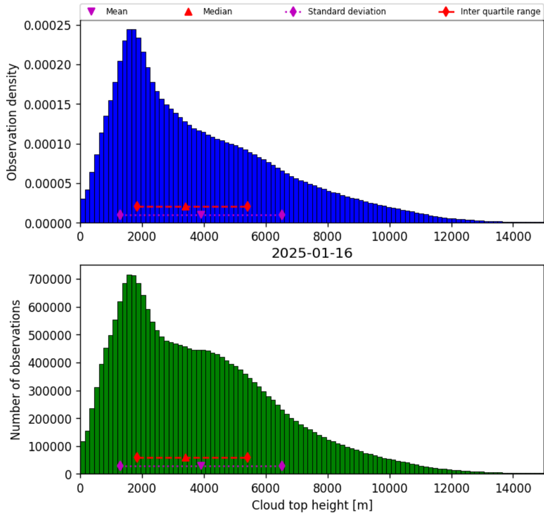
Figure 40: Histogram of “Cloud top height” for 2025-01-15 to 2025-01-17
