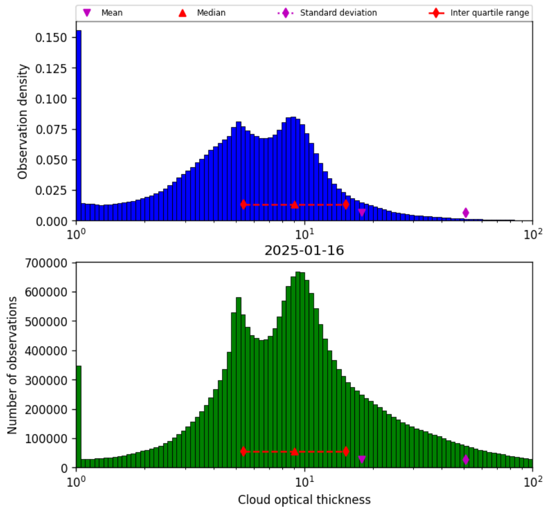
Figure 41: Histogram of “Cloud optical thickness” for 2025-01-15 to 2025-01-17
