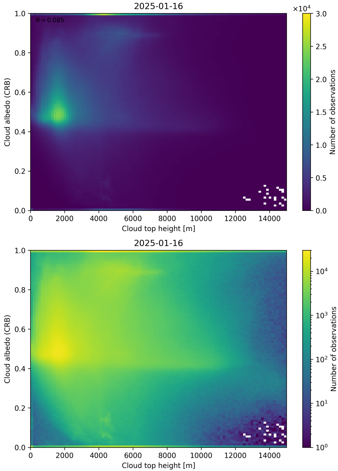
Figure 86: Scatter density plot of “Cloud top height” against “Cloud albedo (CRB)” for 2025-01-15 to 2025-01-17.
