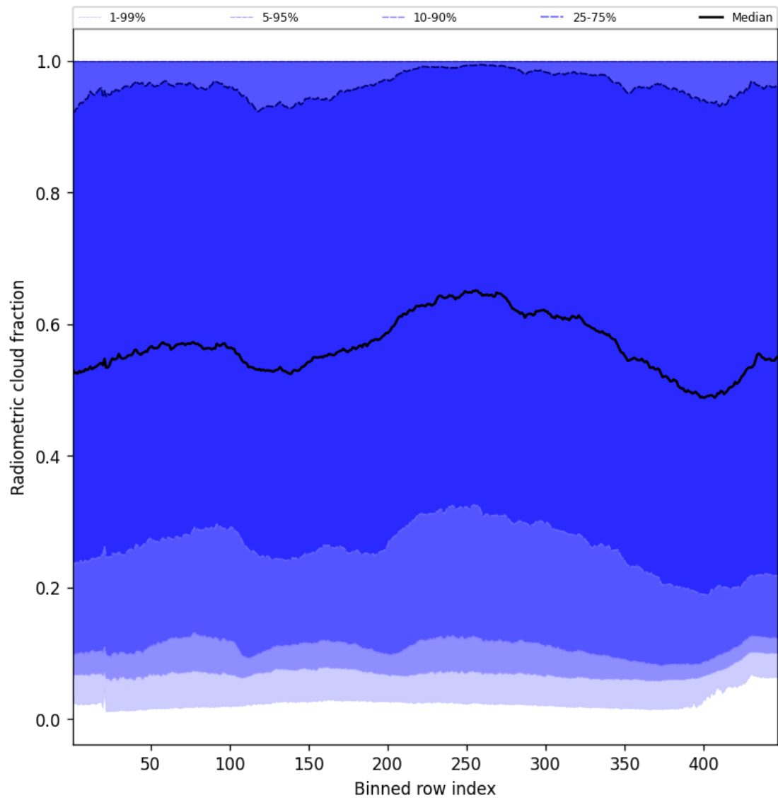
Figure 55: Along track statistics of “Radiometric cloud fraction” for 2025-01-15 to 2025-01-17
