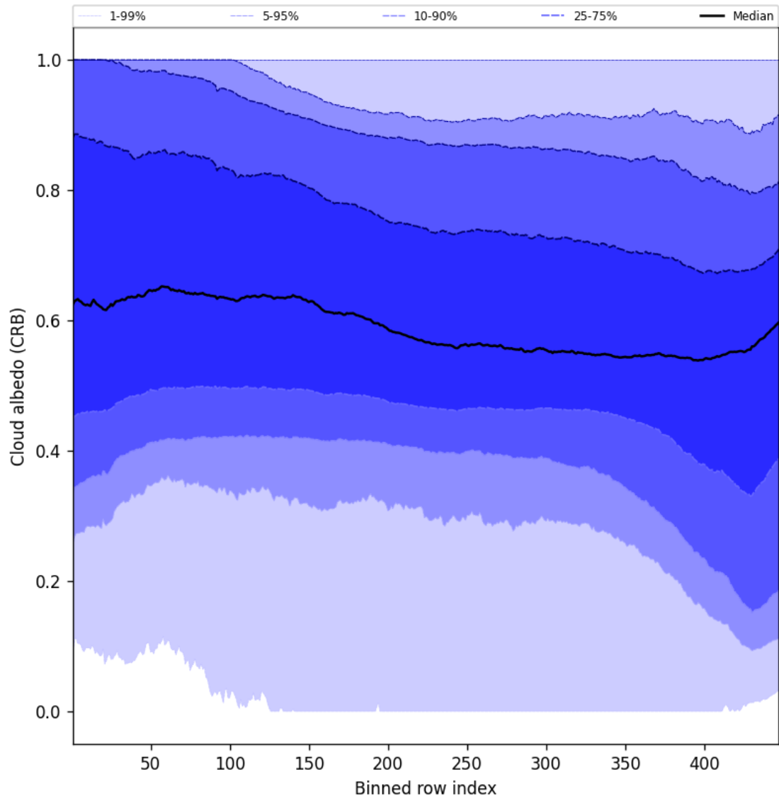
Figure 60: Along track statistics of “Cloud albedo (CRB)” for 2025-01-15 to 2025-01-17
