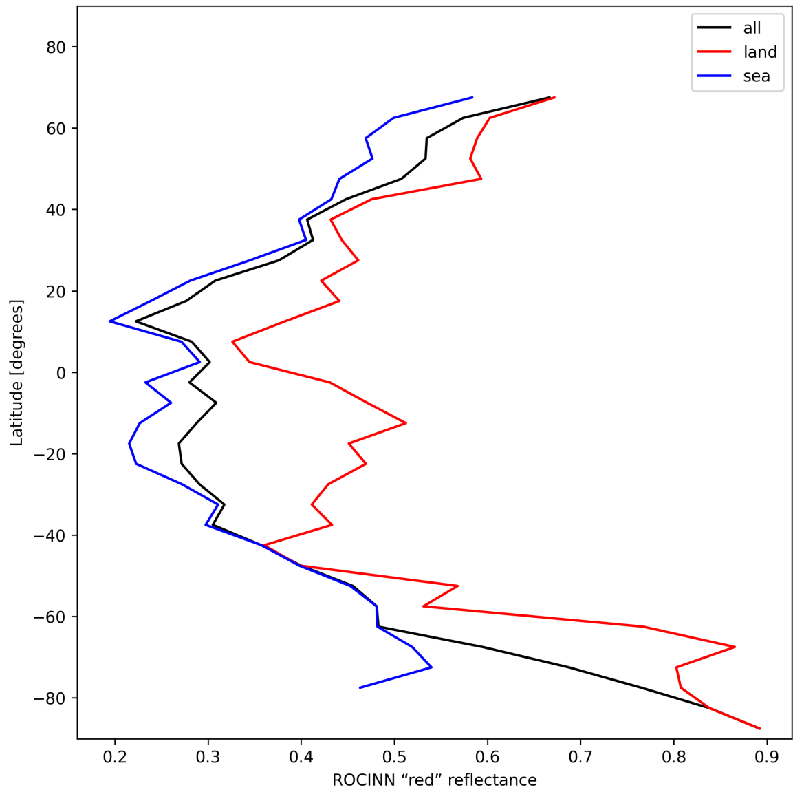
Figure 37: Zonal average of "ROCINN "red" reflectance" for 2025-01-15 to 2025-01-17.
