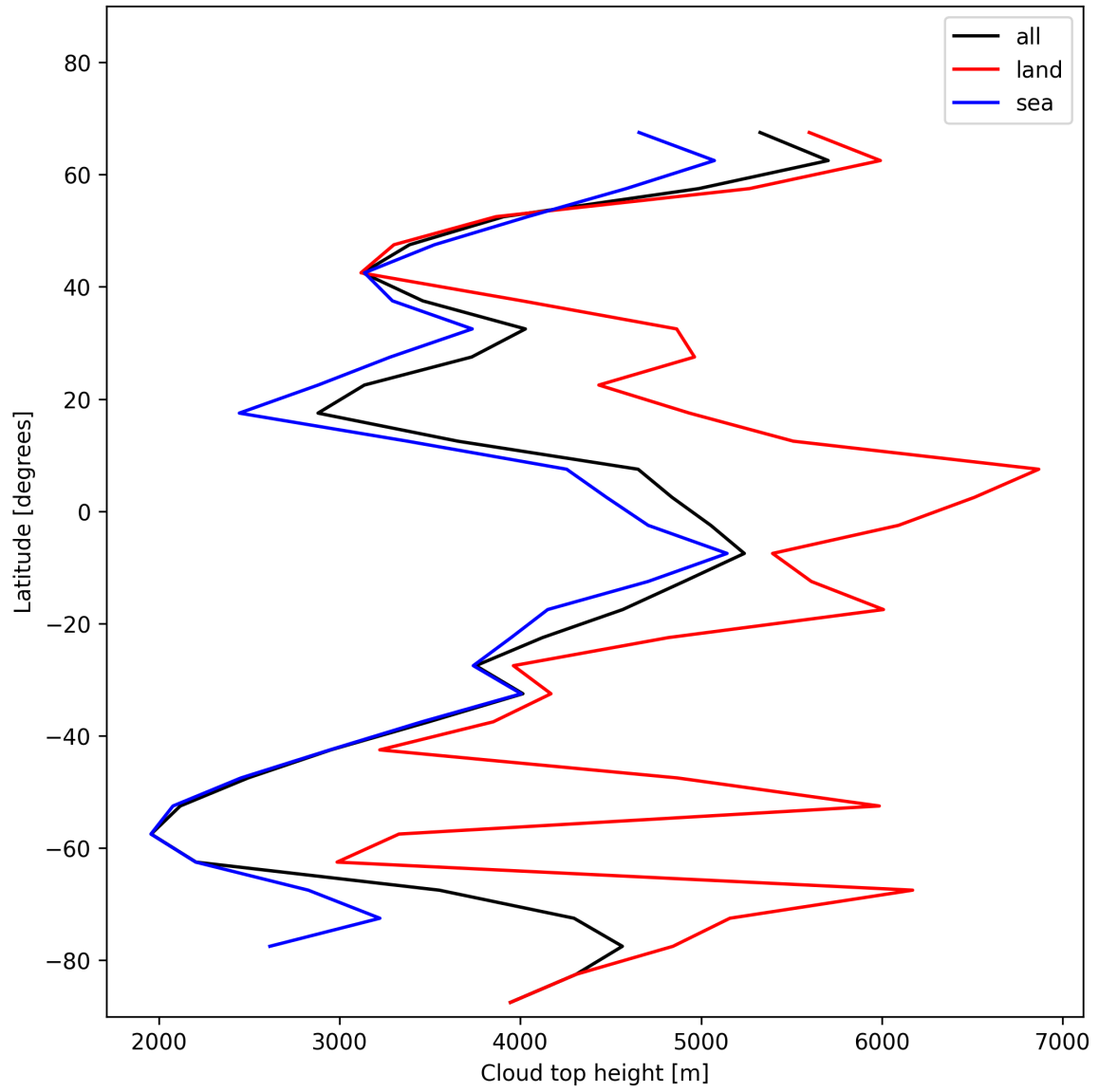
Figure 24: Zonal average of “Cloud top height” for 2025-01-15 to 2025-01-17.
