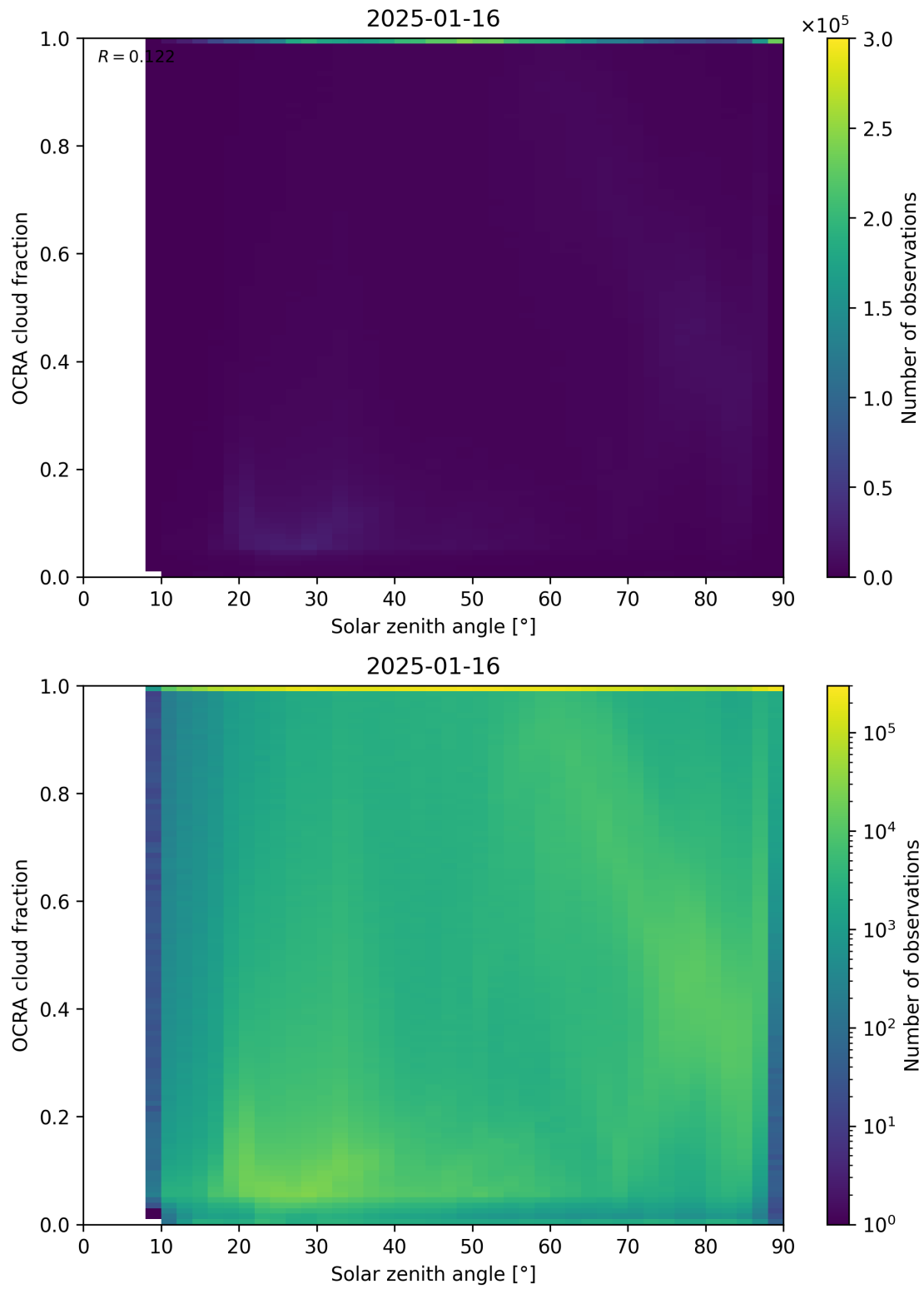
Figure 100: Scatter density plot of “Solar zenith angle” against “OCRA cloud fraction” for 2025-01-15 to 2025-01-17.
