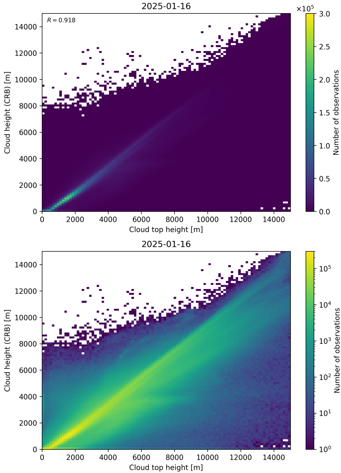
Figure 89: Scatter density plot of “Cloud top height” against “Cloud height (CRB)” for 2025-01-15 to 2025-01-17.
