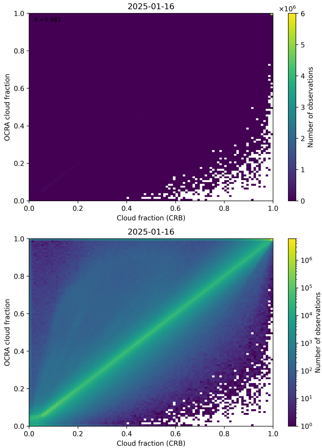
Figure 78: Scatter density plot of “Cloud fraction (CRB)” against “OCRA cloud fraction” for 2025-01-15 to 2025-01-17.
