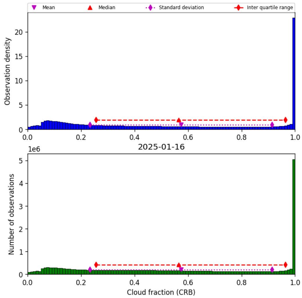
Figure 42: Histogram of “Cloud fraction (CRB)” for 2025-01-15 to 2025-01-17
