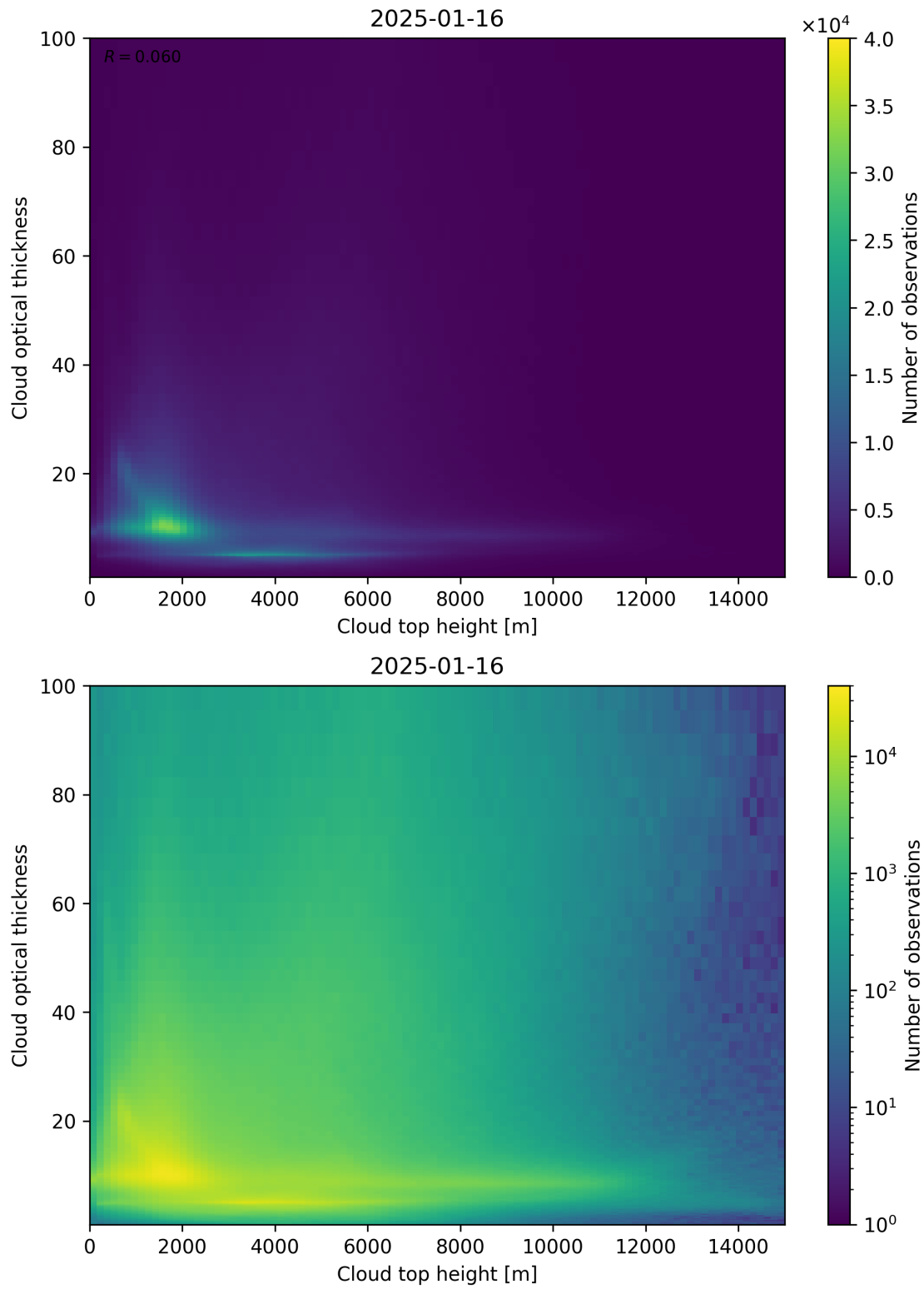
Figure 90: Scatter density plot of “Cloud top height” against “Cloud optical thickness” for 2025-01-15 to 2025-01-17.
