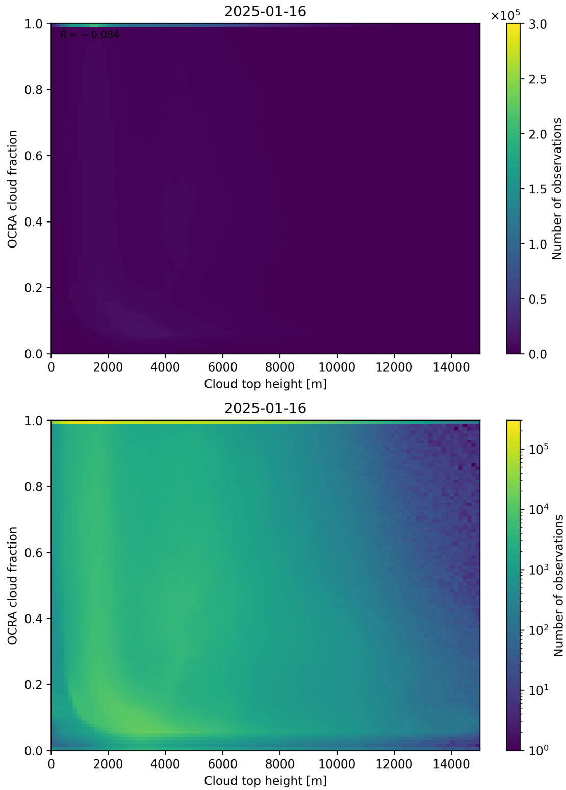
Figure 87: Scatter density plot of “Cloud top height” against “OCRA cloud fraction” for 2025-01-15 to 2025-01-17.
