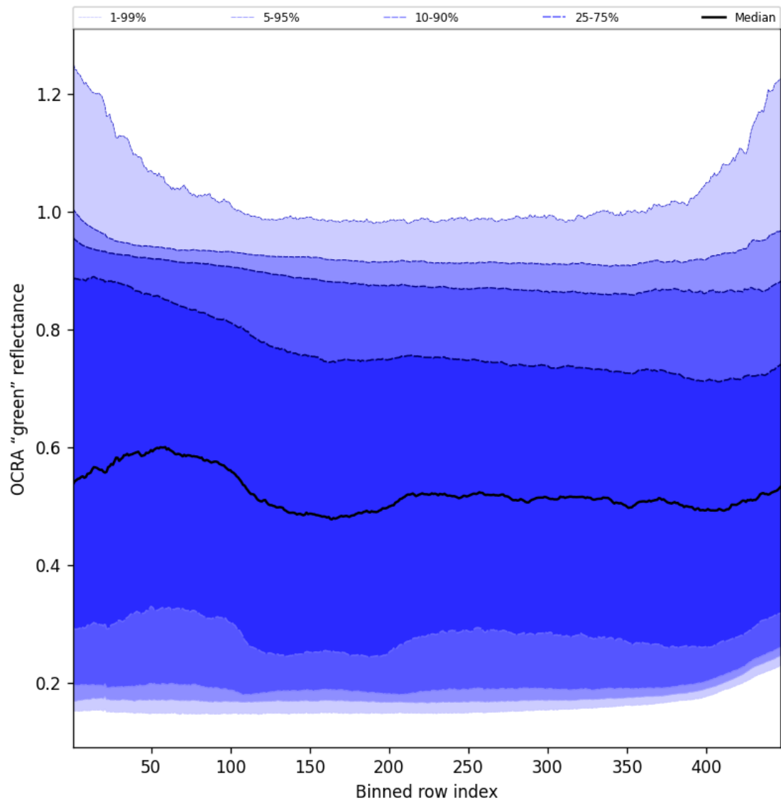
Figure 68: Along track statistics of "OCRA "green" reflectance" for 2025-01-15 to 2025-01-17
