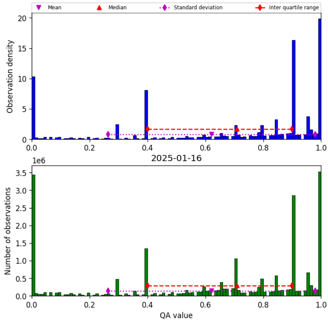
Figure 38: Histogram of “QA value” for 2025-01-15 to 2025-01-17
