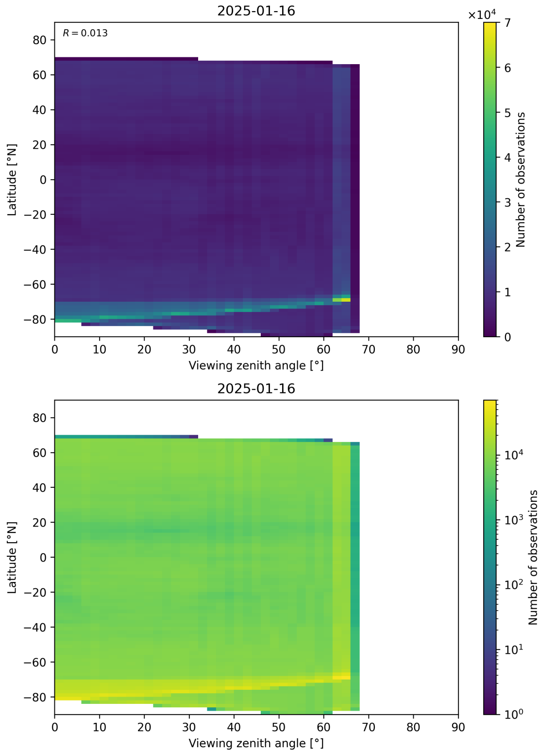
Figure 113: Scatter density plot of “Viewing zenith angle” against “Latitude” for 2025-01-15 to 2025-01-17.
