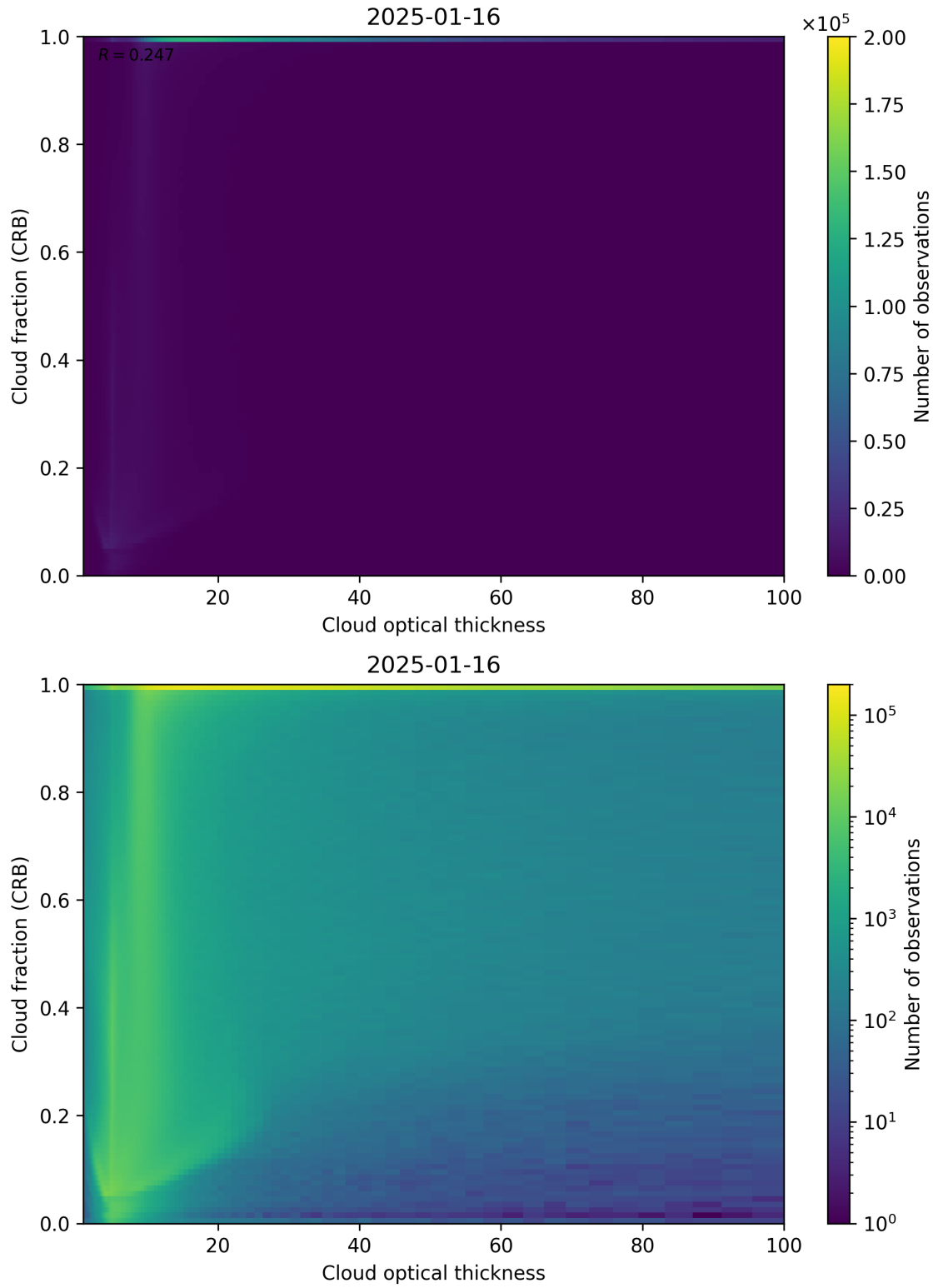
Figure 84: Scatter density plot of “Cloud optical thickness” against “Cloud fraction (CRB)” for 2025-01-15 to 2025-01-17.
