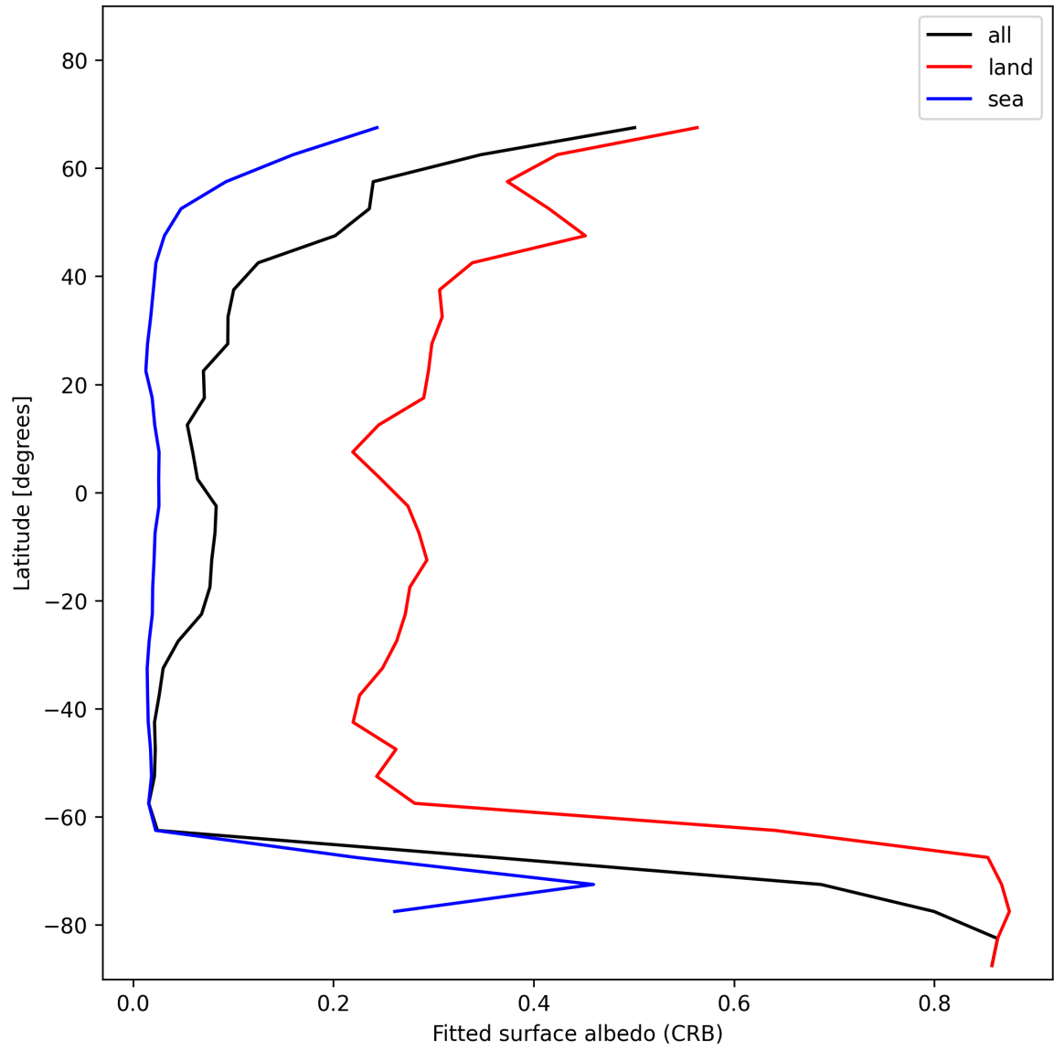
Figure 30: Zonal average of “Fitted surface albedo (CRB)” for 2025-01-15 to 2025-01-17.
