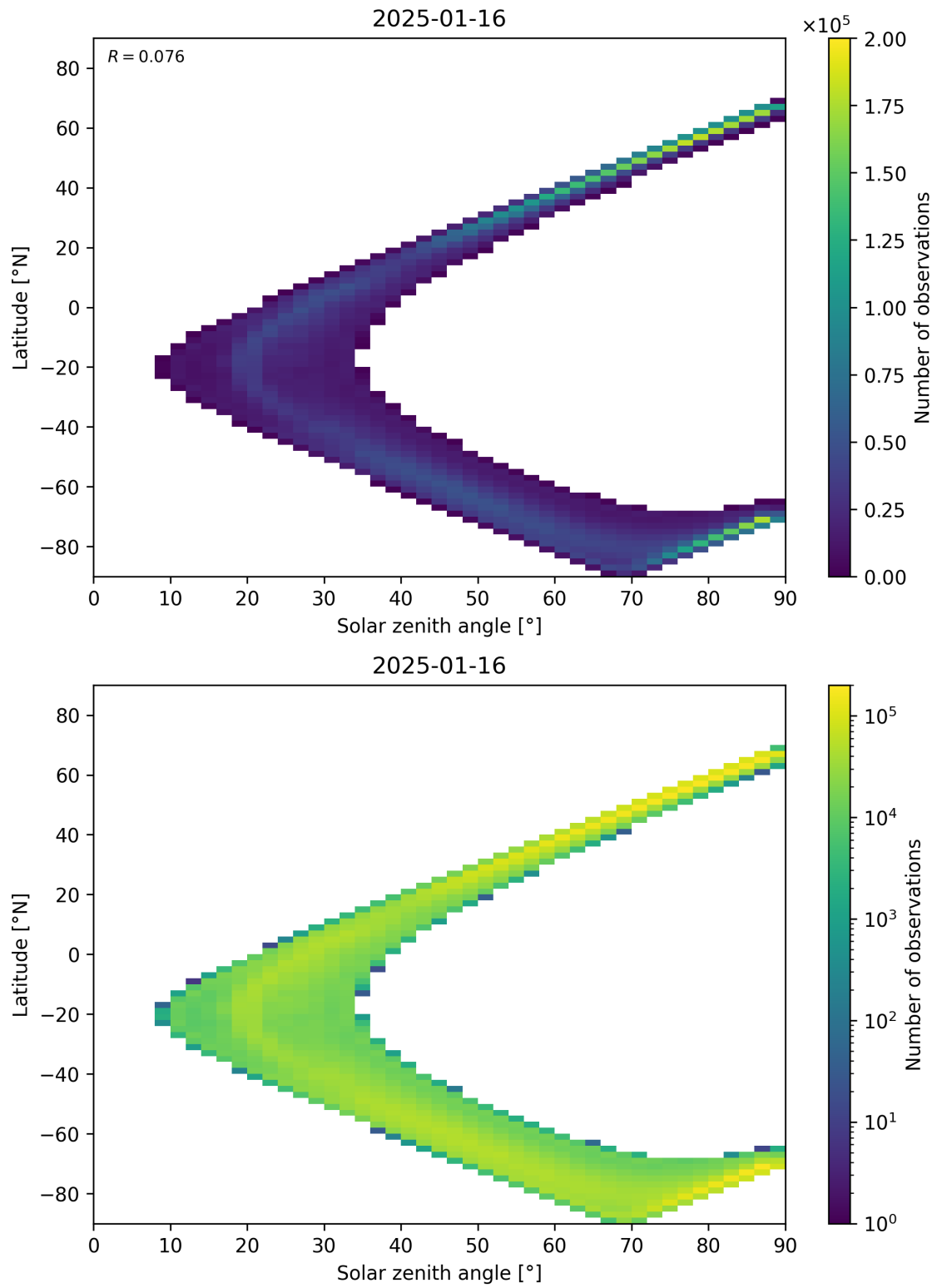
Figure 105: Scatter density plot of “Solar zenith angle” against “Latitude” for 2025-01-15 to 2025-01-17.
