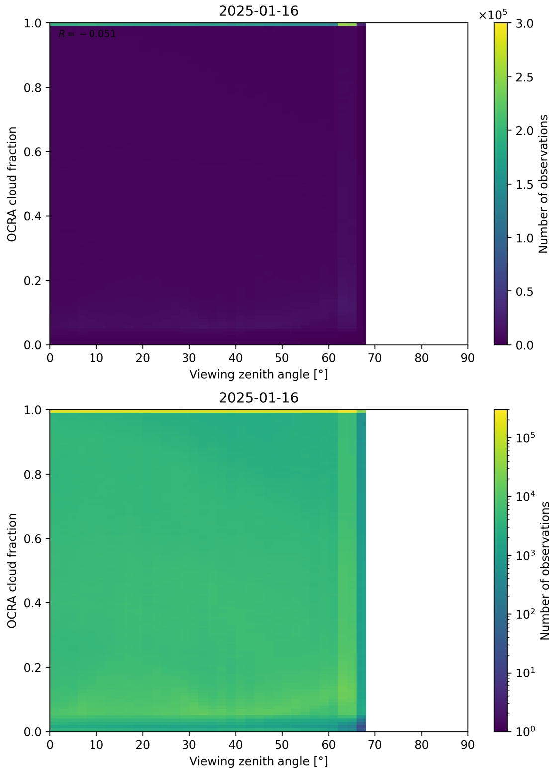
Figure 108: Scatter density plot of “Viewing zenith angle” against “OCRA cloud fraction” for 2025-01-15 to 2025-01-17.
