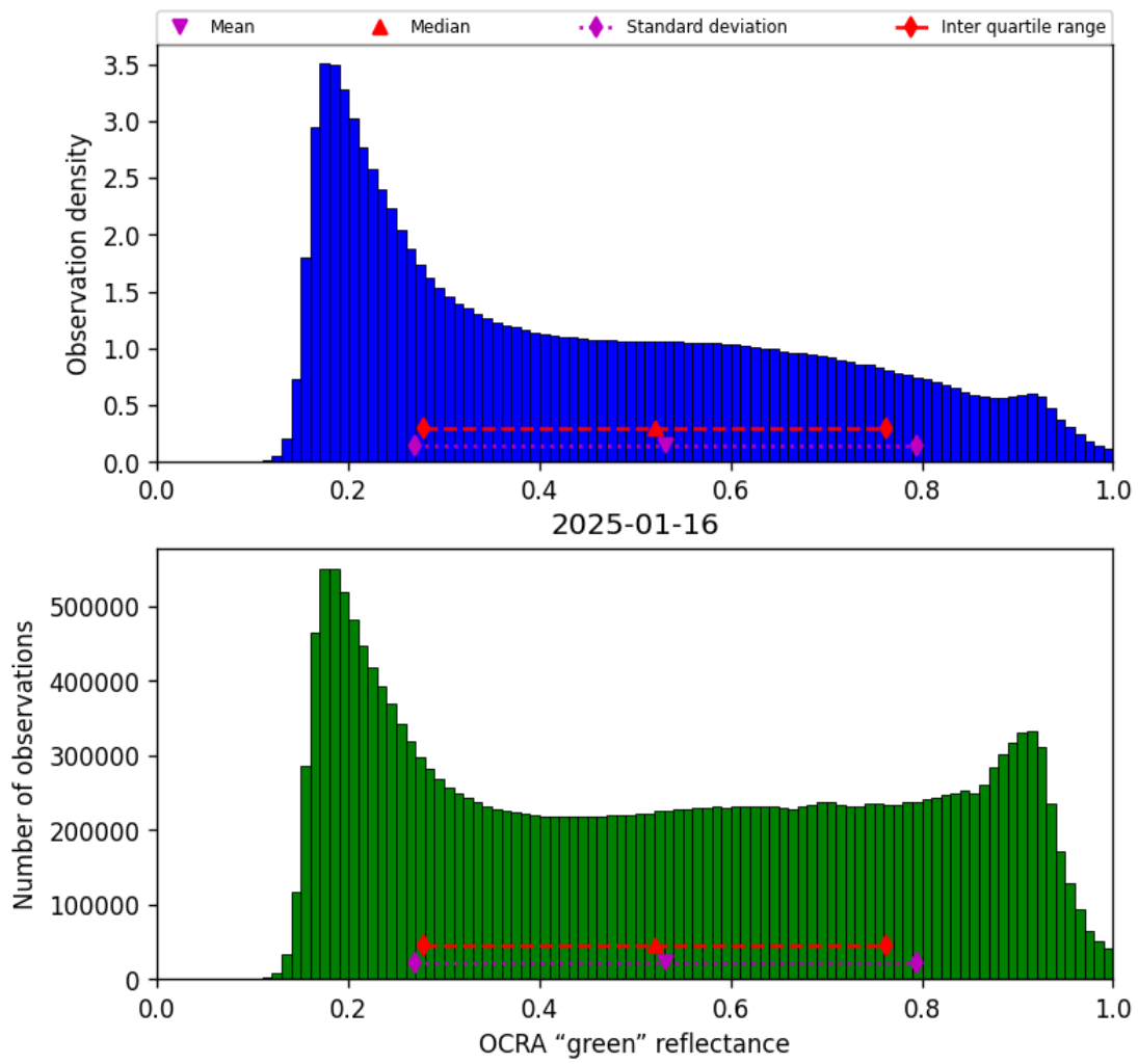
Figure 52: Histogram of “OCRA “green” reflectance” for 2025-01-15 to 2025-01-17
