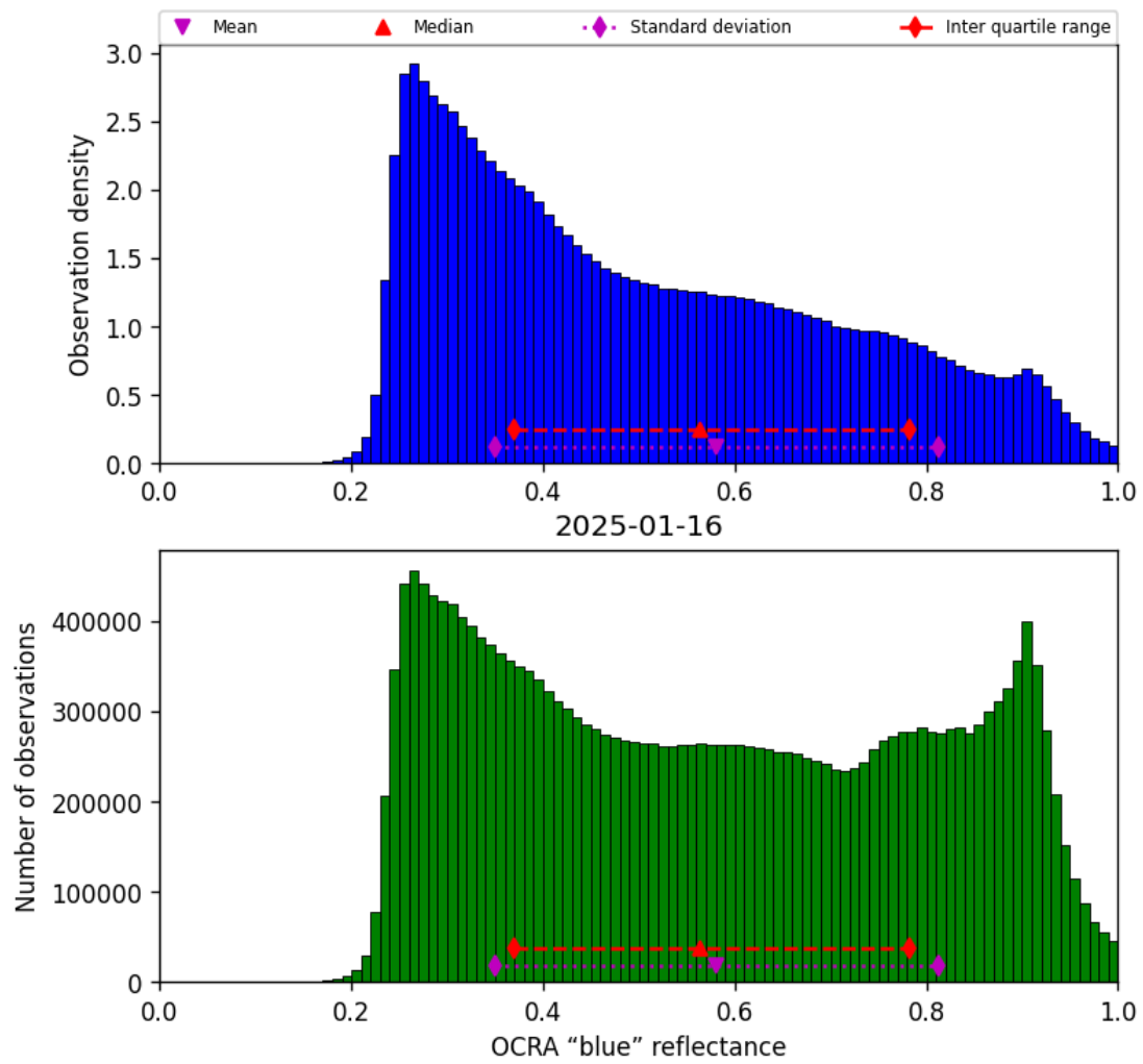
Figure 51: Histogram of “OCRA “blue” reflectance” for 2025-01-15 to 2025-01-17
