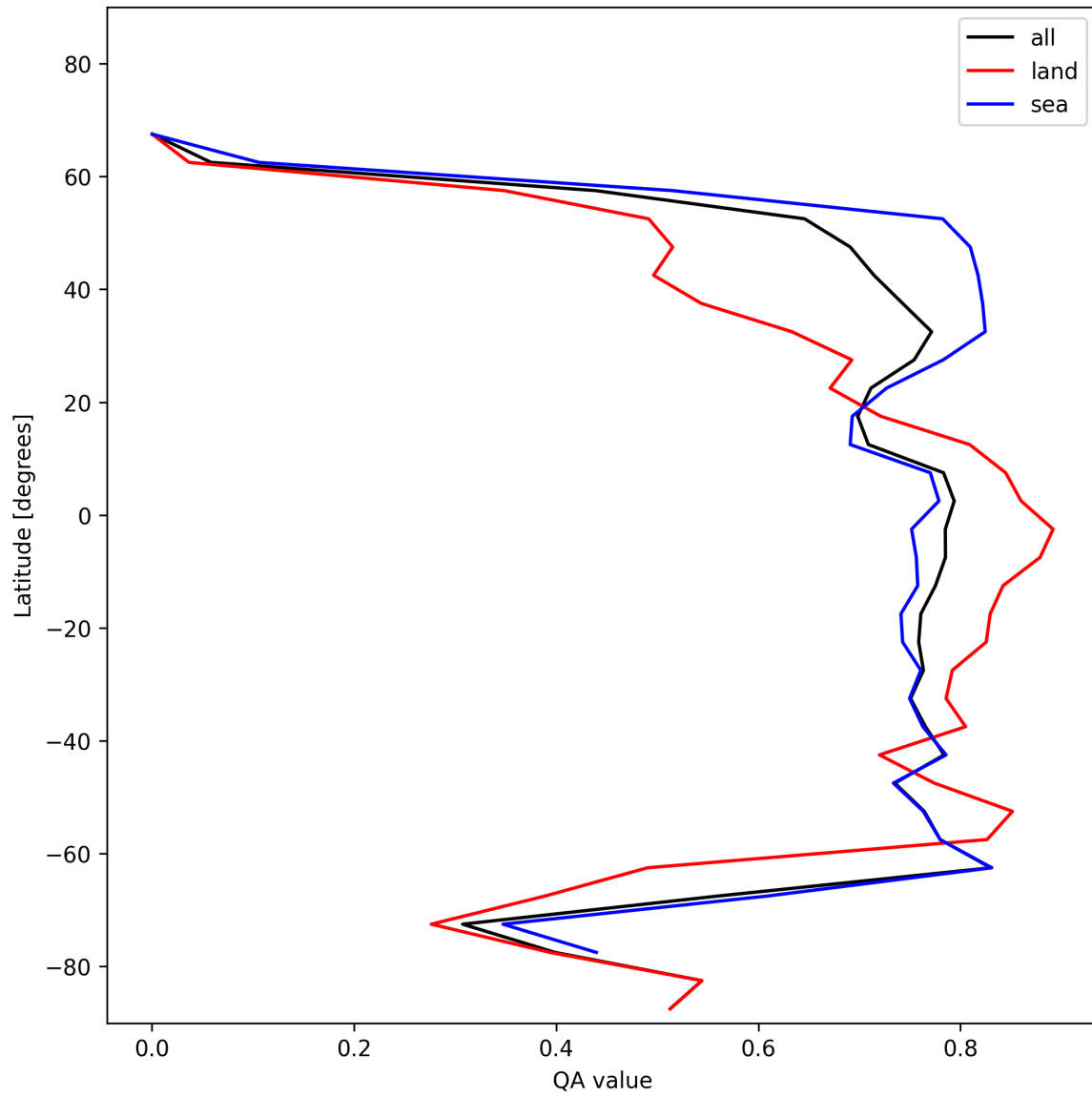
Figure 22: Zonal average of “QA value” for 2025-01-15 to 2025-01-17.
