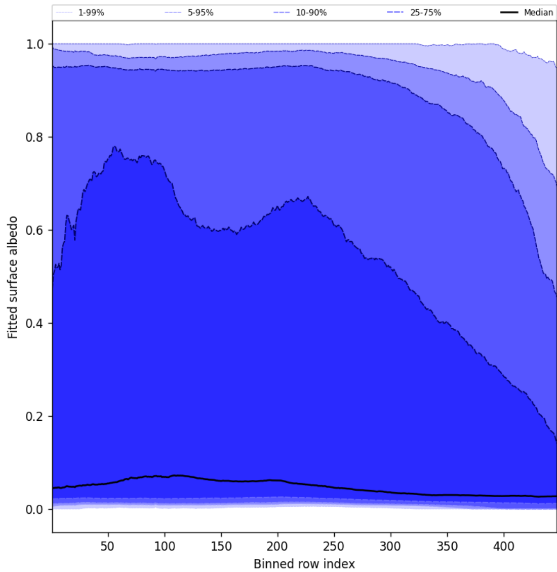
Figure 61: Along track statistics of “Fitted surface albedo” for 2025-01-15 to 2025-01-17
