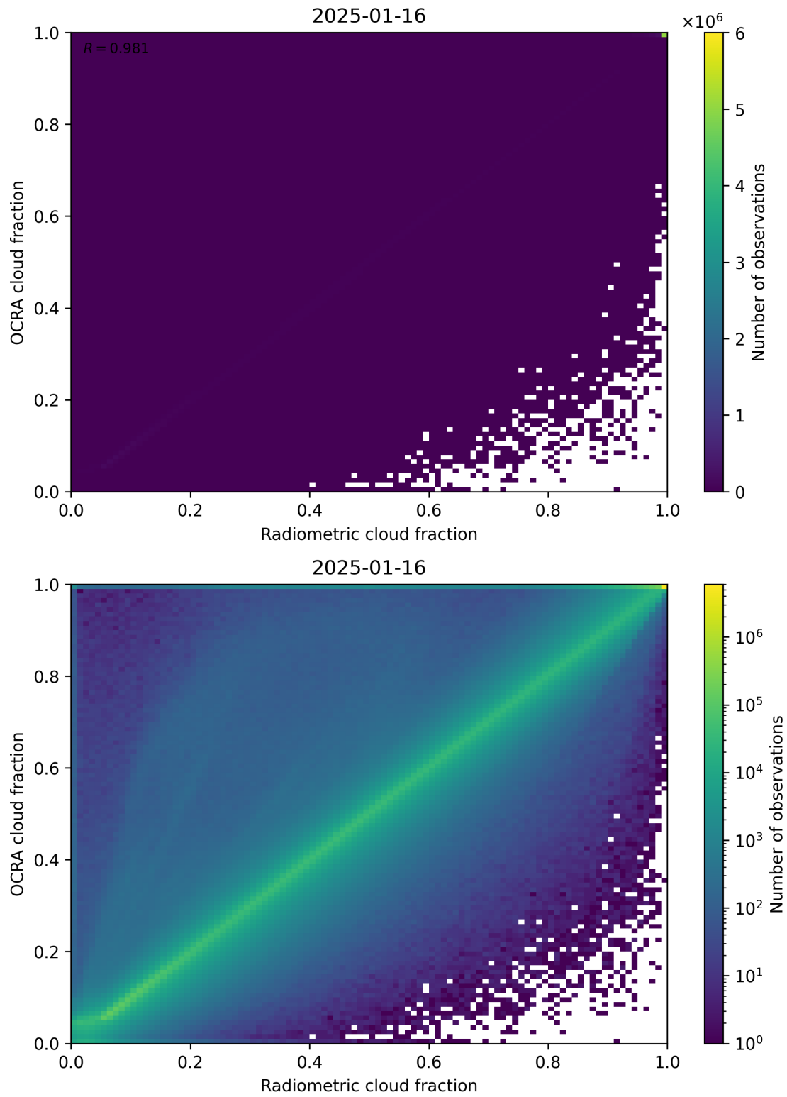
Figure 72: Scatter density plot of “Radiometric cloud fraction” against “OCRA cloud fraction” for 2025-01-15 to 2025-01-17.
