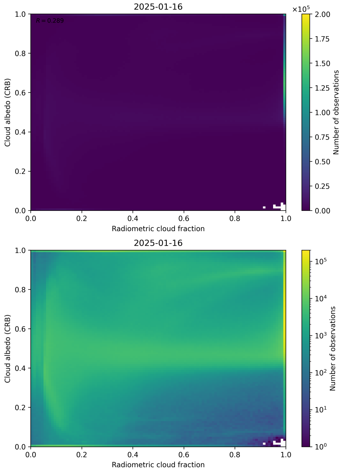
Figure 71: Scatter density plot of “Radiometric cloud fraction” against “Cloud albedo (CRB)” for 2025-01-15 to 2025-01-17.
