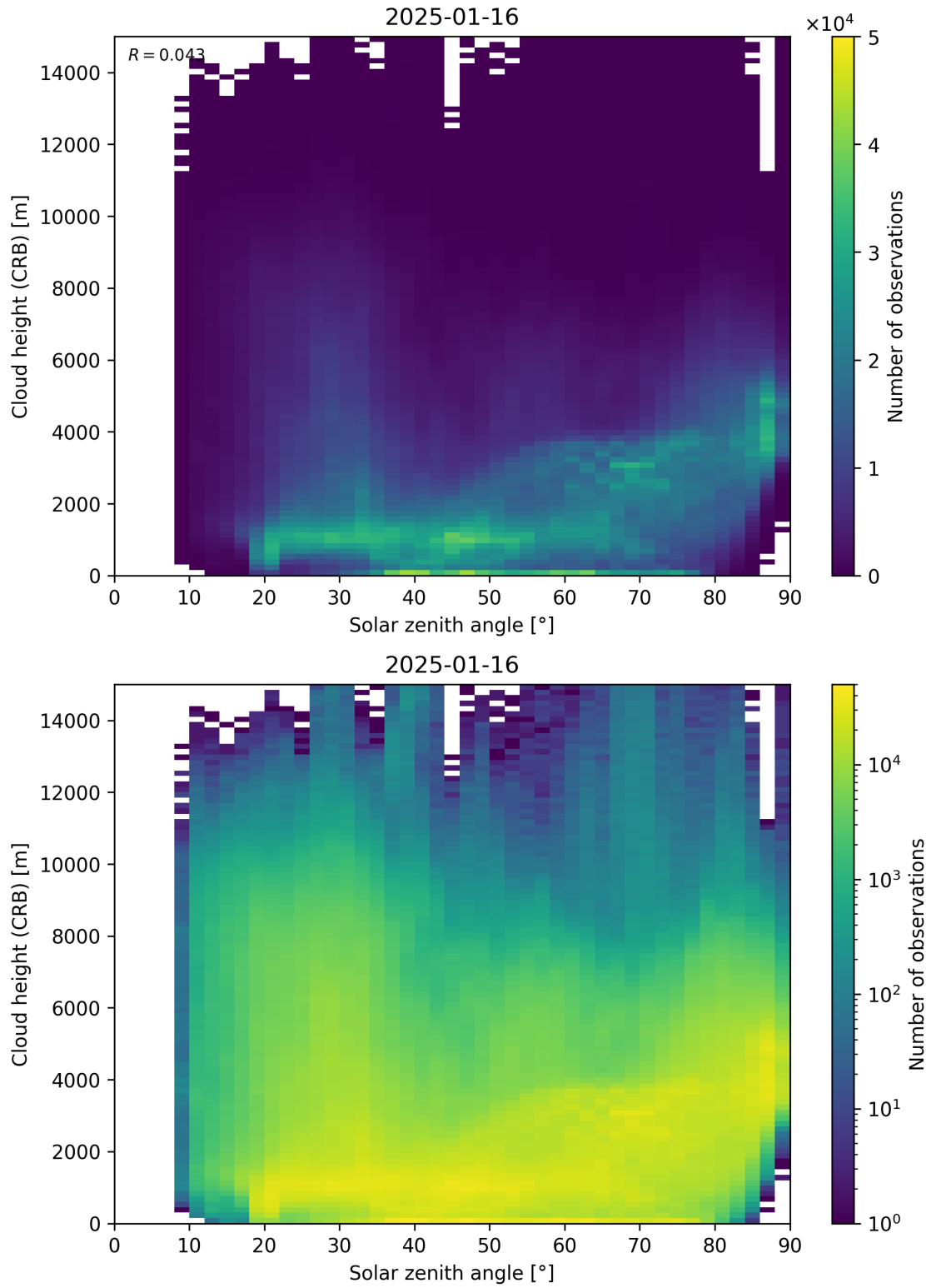
Figure 102: Scatter density plot of “Solar zenith angle” against “Cloud height (CRB)” for 2025-01-15 to 2025-01-17.
