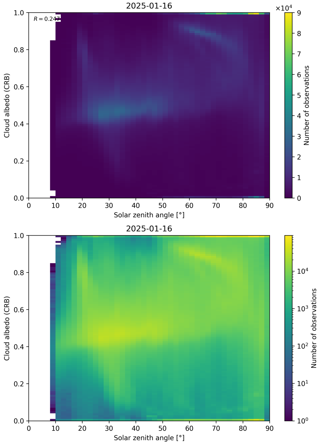
Figure 98: Scatter density plot of “Solar zenith angle” against “Cloud albedo (CRB)” for 2025-01-15 to 2025-01-17.
