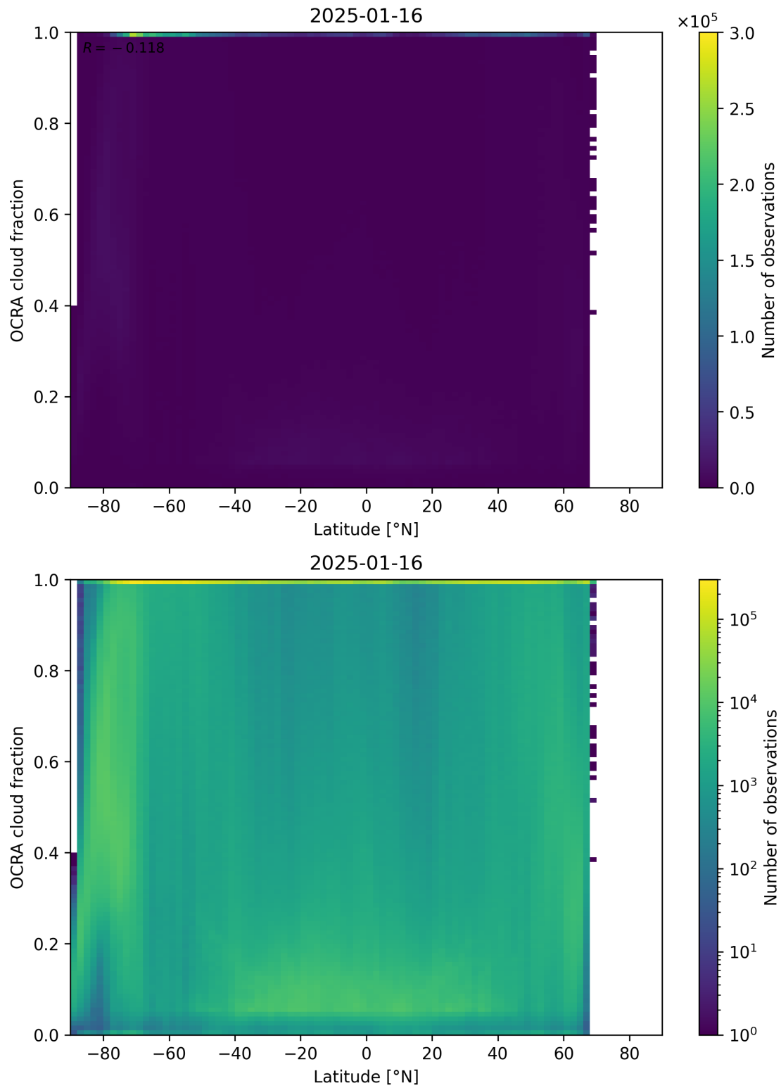
Figure 93: Scatter density plot of “Latitude” against “OCRA cloud fraction” for 2025-01-15 to 2025-01-17.
