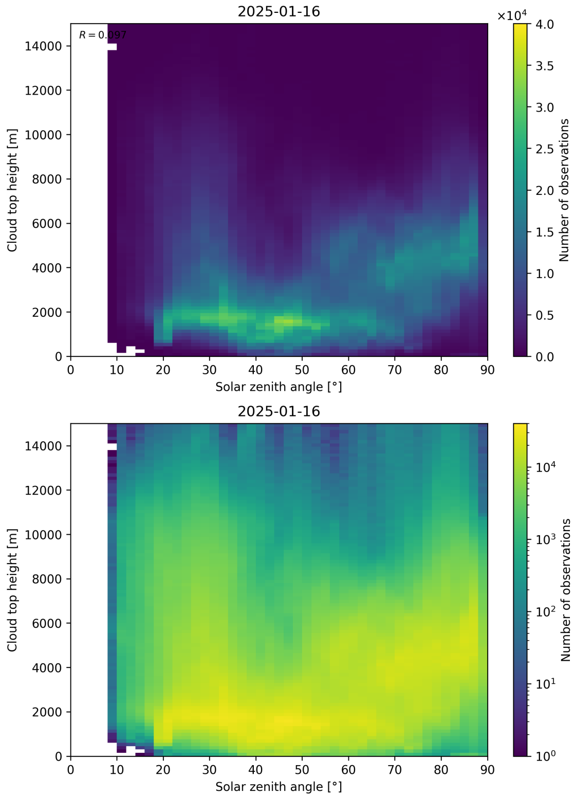
Figure 104: Scatter density plot of “Solar zenith angle” against “Cloud top height” for 2025-01-15 to 2025-01-17.
