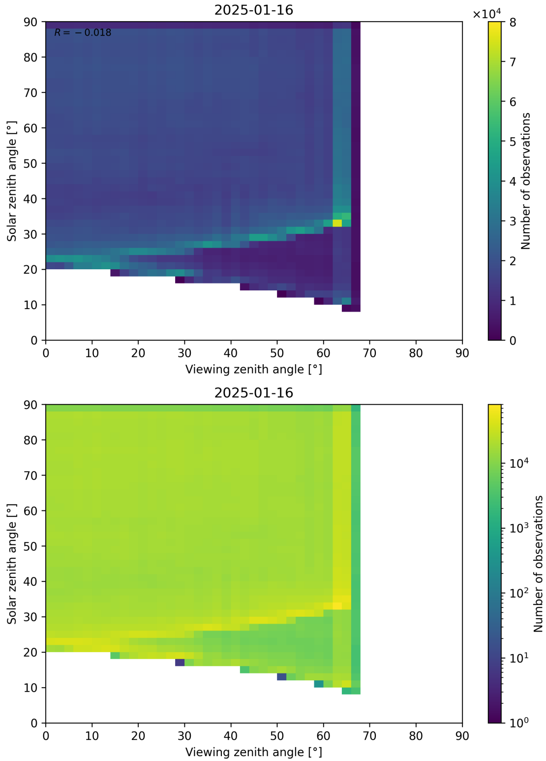
Figure 114: Scatter density plot of “Viewing zenith angle” against “Solar zenith angle” for 2025-01-15 to 2025-01-17.
