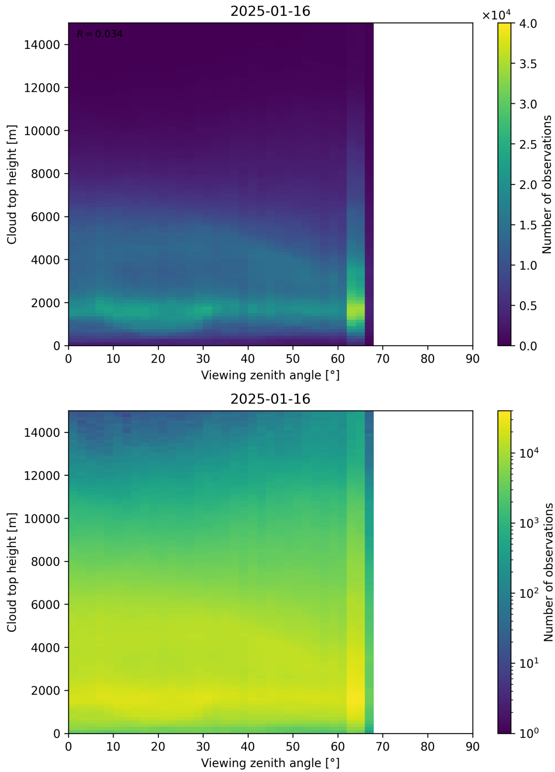
Figure 112: Scatter density plot of “Viewing zenith angle” against “Cloud top height” for 2025-01-15 to 2025-01-17.
