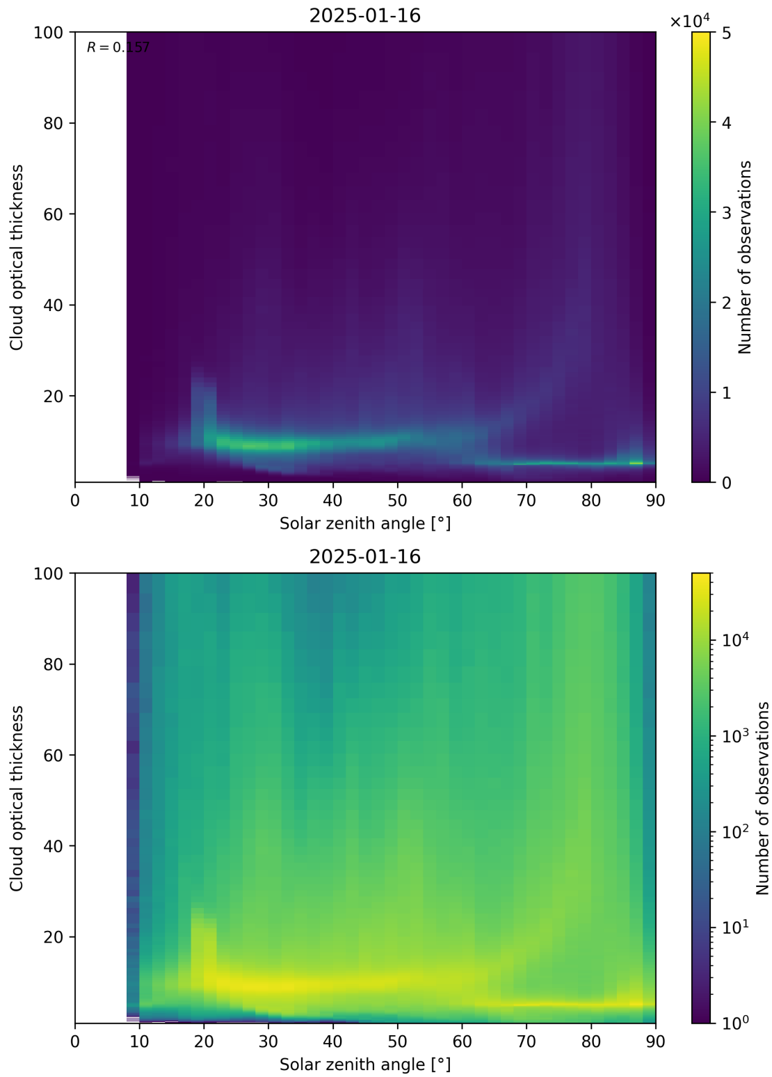
Figure 103: Scatter density plot of “Solar zenith angle” against “Cloud optical thickness” for 2025-01-15 to 2025-01-17.
