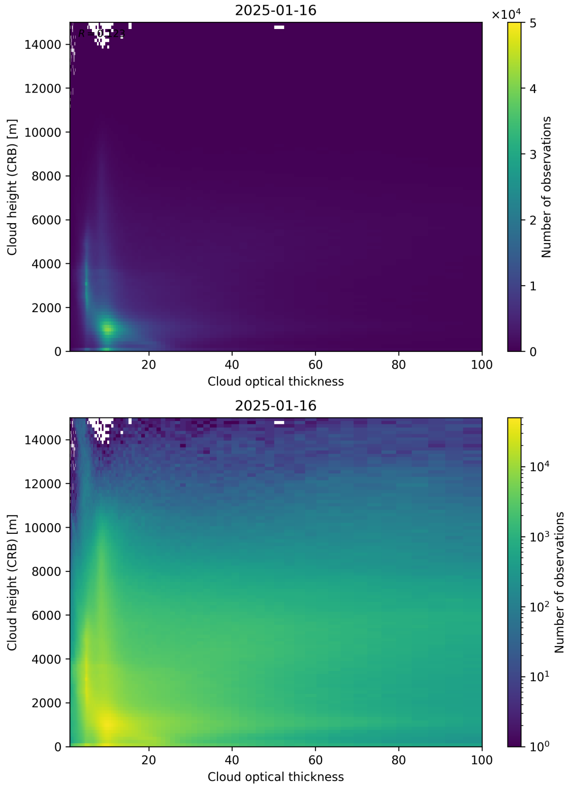
Figure 85: Scatter density plot of “Cloud optical thickness” against “Cloud height (CRB)” for 2025-01-15 to 2025-01-17.
