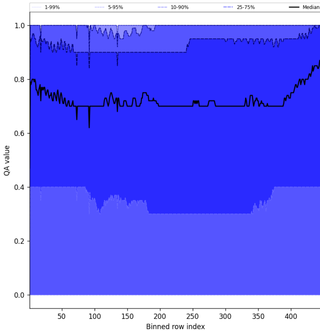
Figure 54: Along track statistics of “QA value” for 2025-01-15 to 2025-01-17
