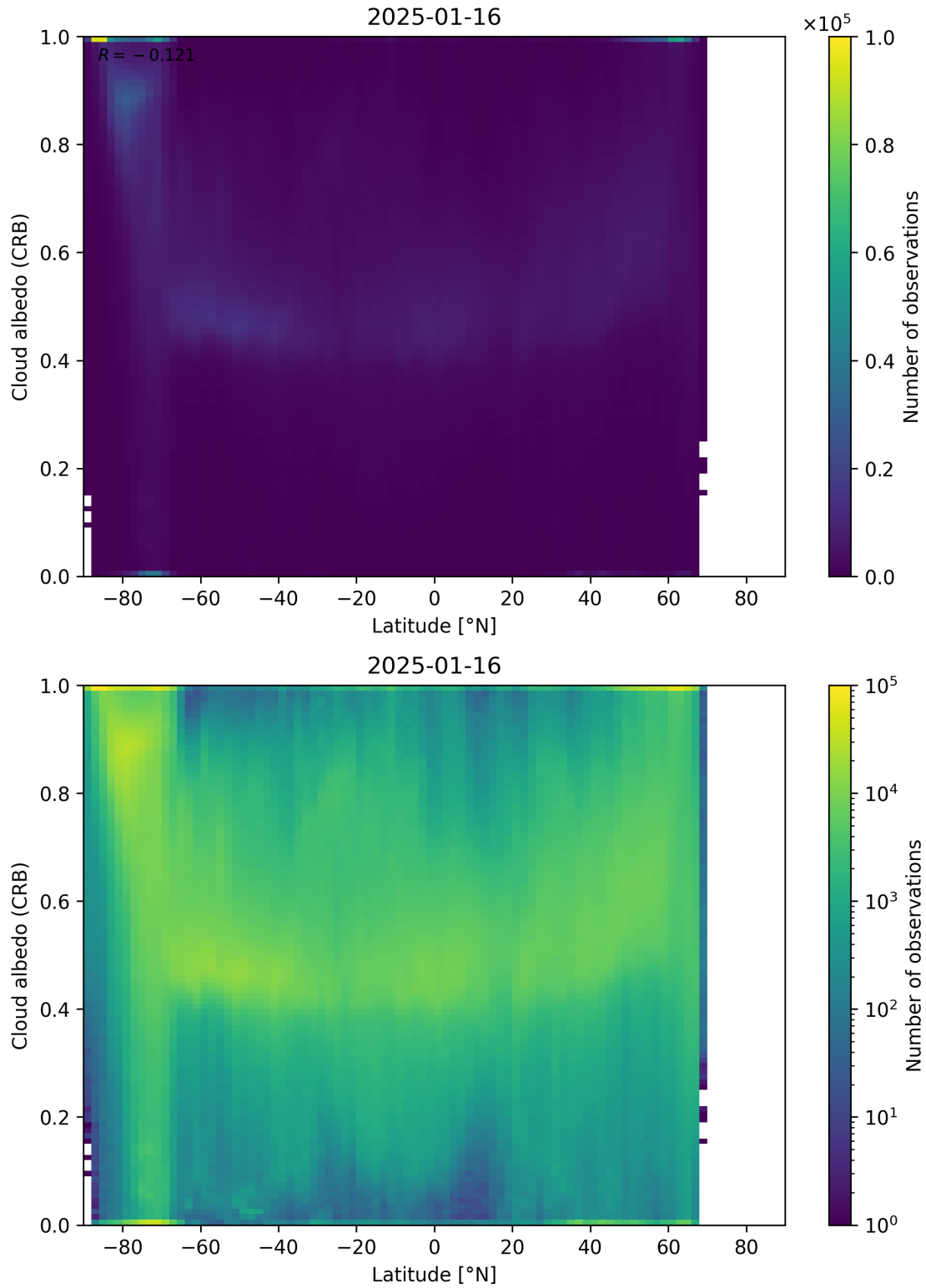
Figure 91: Scatter density plot of “Latitude” against “Cloud albedo (CRB)” for 2025-01-15 to 2025-01-17.
