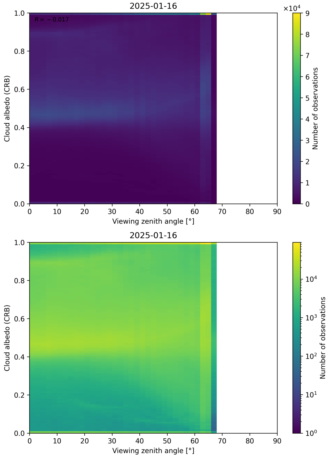
Figure 106: Scatter density plot of “Viewing zenith angle” against “Cloud albedo (CRB)” for 2025-01-15 to 2025-01-17.
