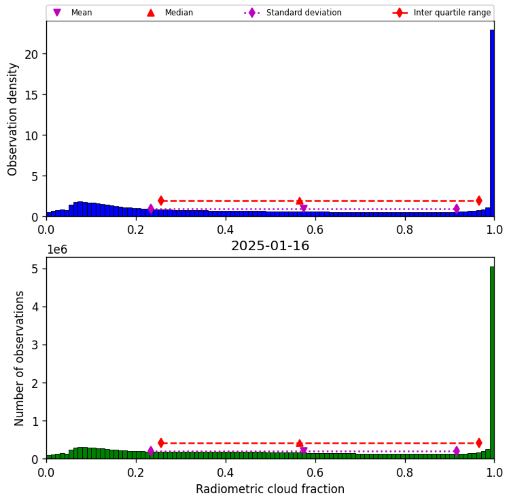
Figure 39: Histogram of “Radiometric cloud fraction” for 2025-01-15 to 2025-01-17
