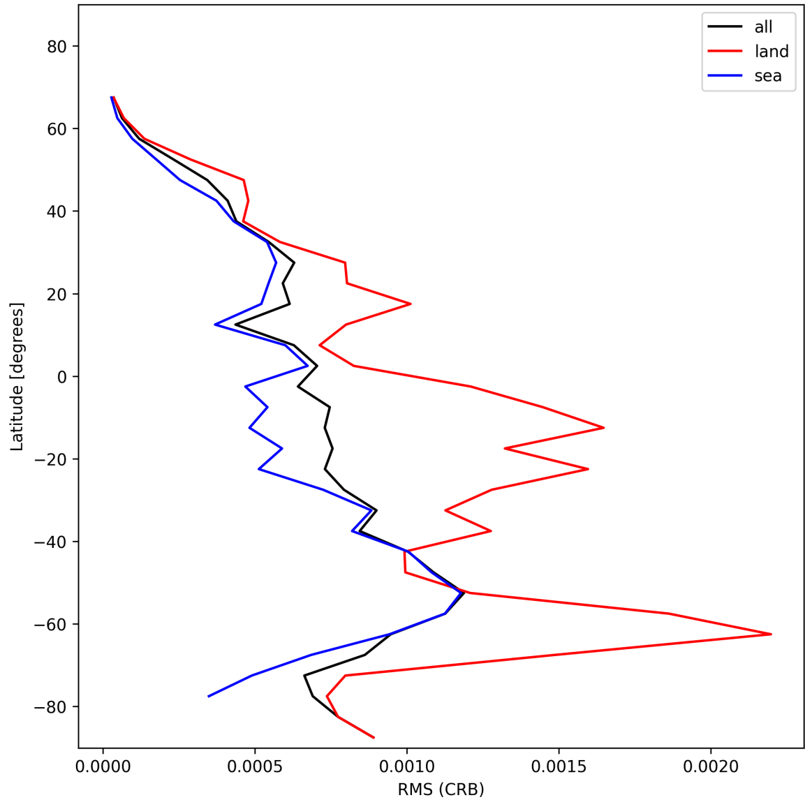
Figure 32: Zonal average of “RMS (CRB)” for 2025-01-15 to 2025-01-17.
