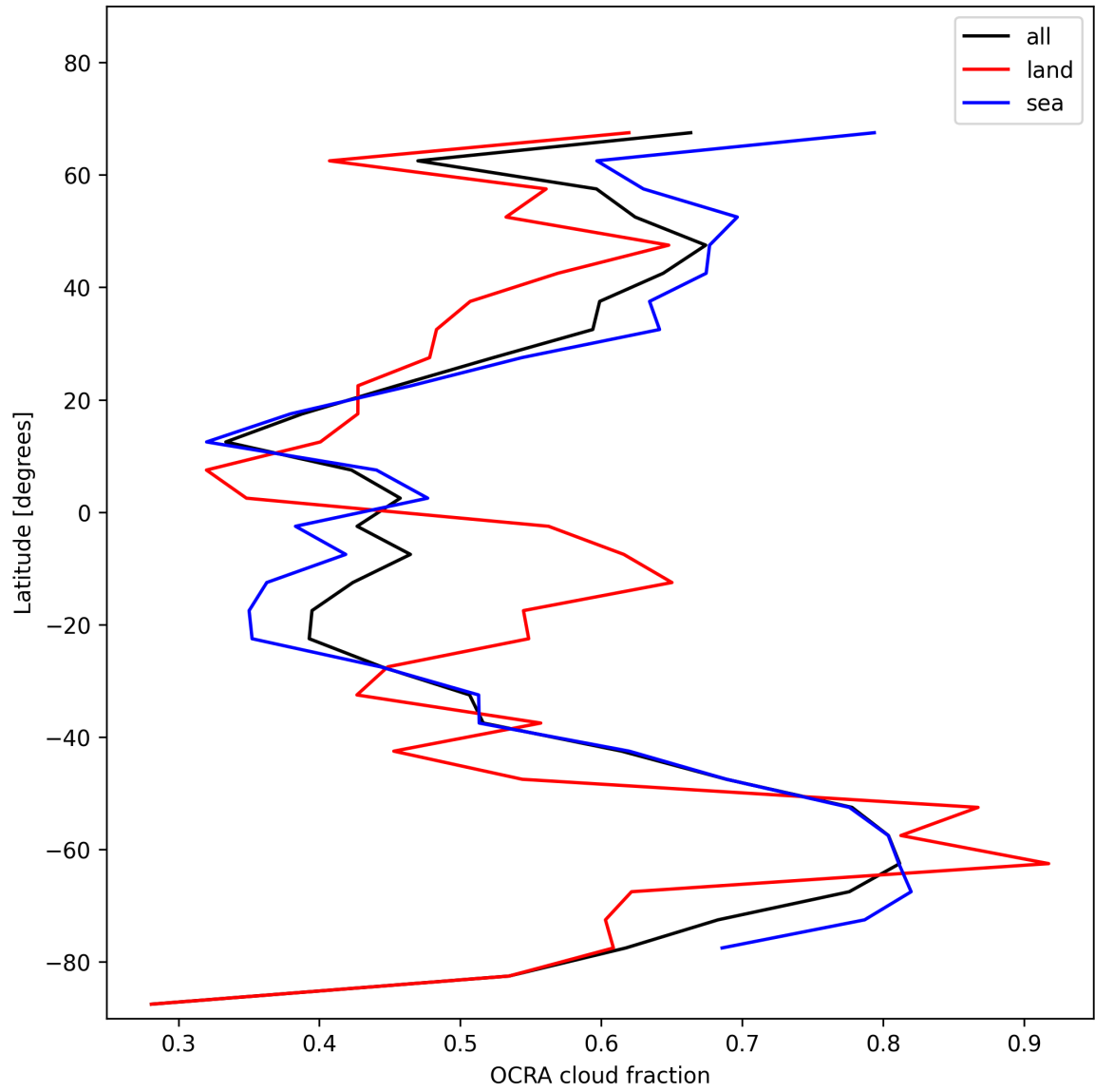
Figure 34: Zonal average of “OCRA cloud fraction” for 2025-01-15 to 2025-01-17.
