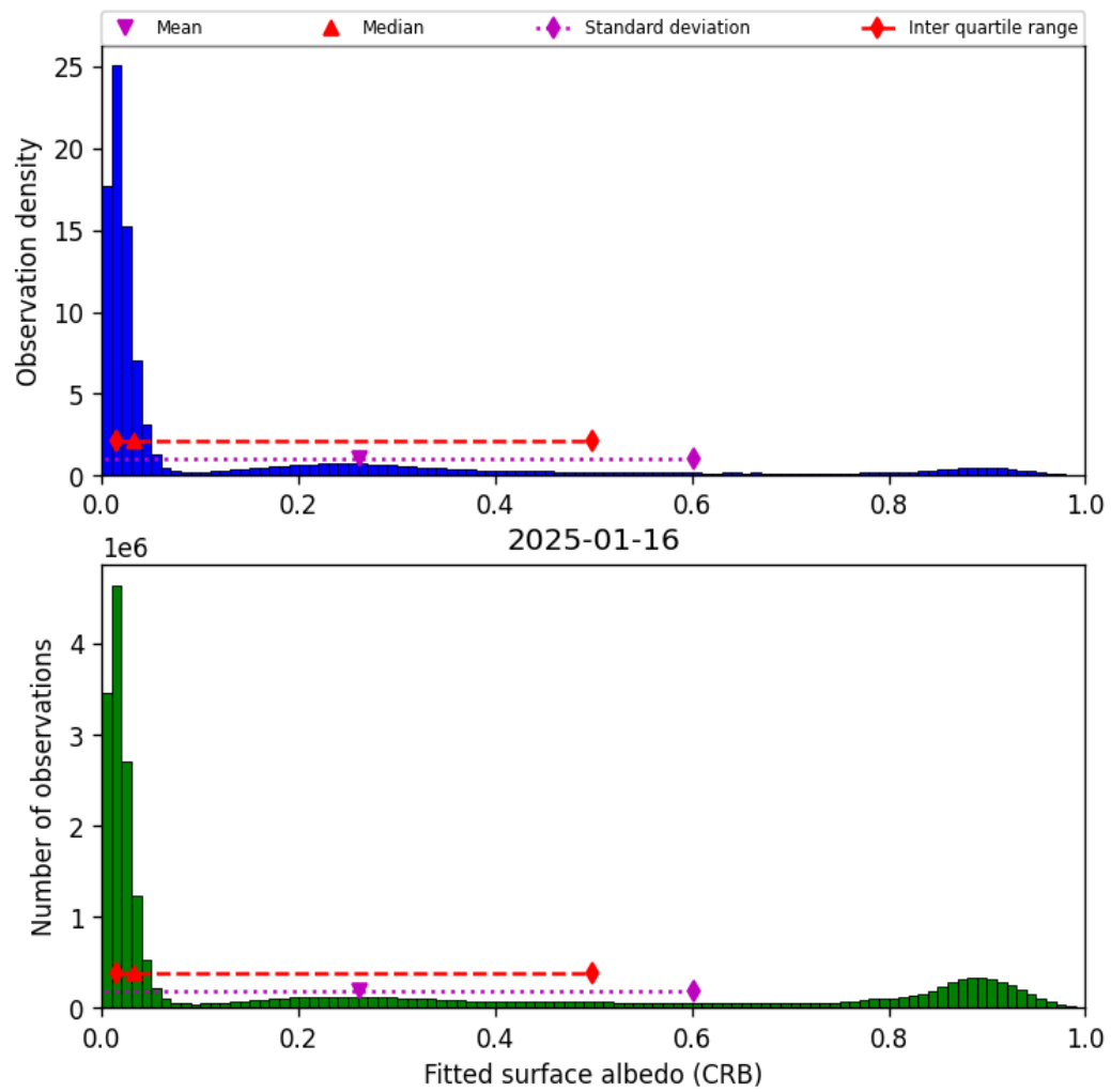
Figure 46: Histogram of “Fitted surface albedo (CRB)” for 2025-01-15 to 2025-01-17
