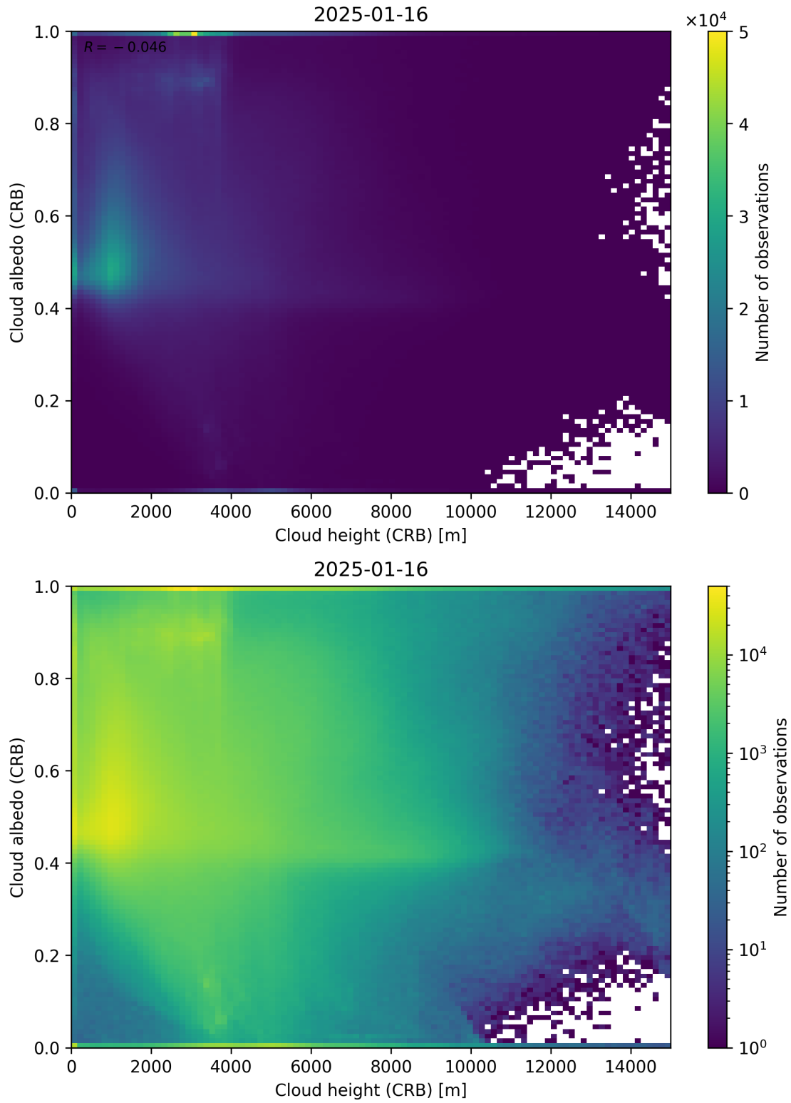
Figure 80: Scatter density plot of “Cloud height (CRB)” against “Cloud albedo (CRB)” for 2025-01-15 to 2025-01-17.
