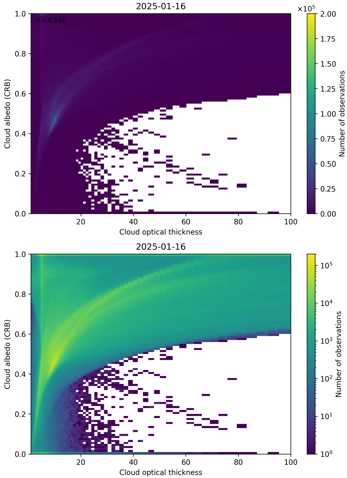
Figure 82: Scatter density plot of “Cloud optical thickness” against “Cloud albedo (CRB)” for 2025-01-15 to 2025-01-17.
