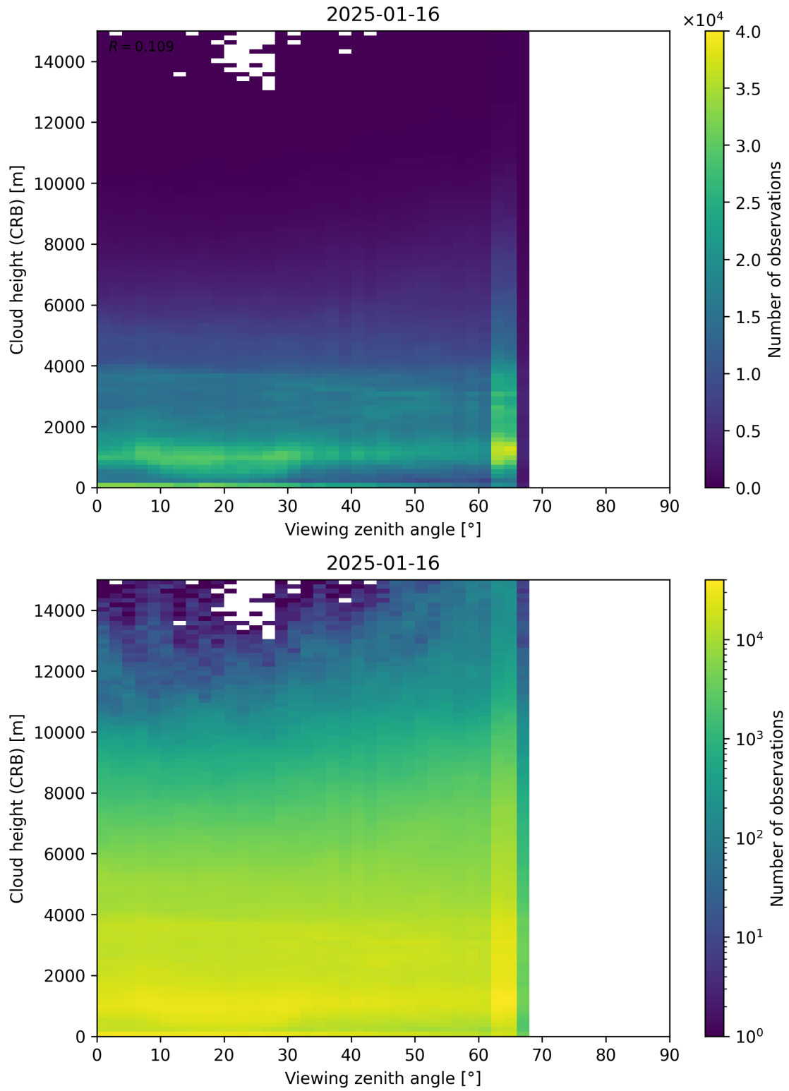
Figure 110: Scatter density plot of “Viewing zenith angle” against “Cloud height (CRB)” for 2025-01-15 to 2025-01-17.
