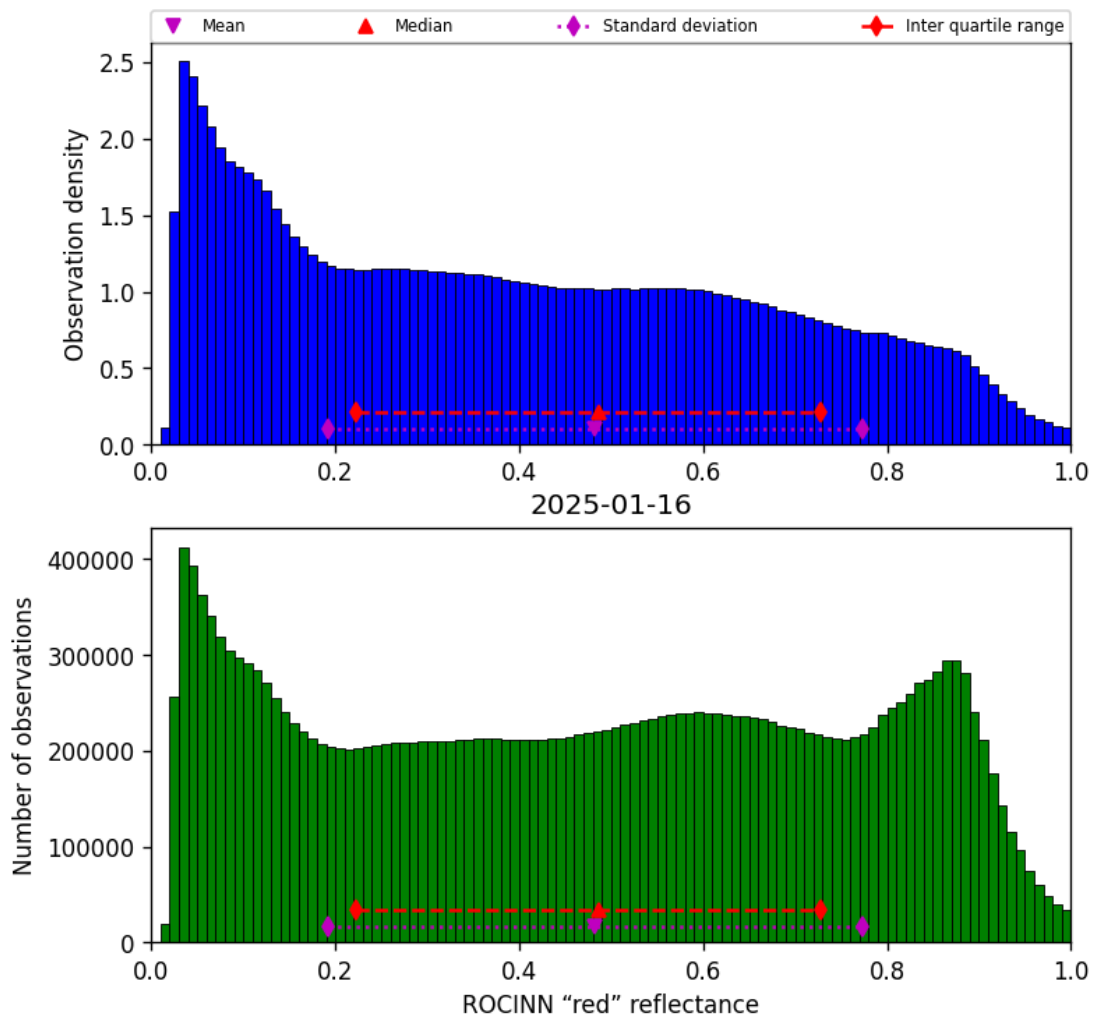
Figure 53: Histogram of “ROCINN “red” reflectance” for 2025-01-15 to 2025-01-17
