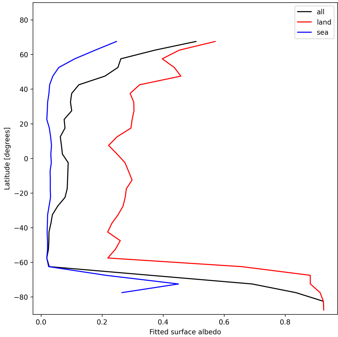
Figure 29: Zonal average of “Fitted surface albedo” for 2025-01-15 to 2025-01-17.
