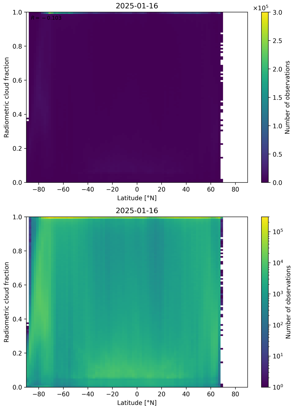
Figure 92: Scatter density plot of “Latitude” against “Radiometric cloud fraction” for 2025-01-15 to 2025-01-17.
