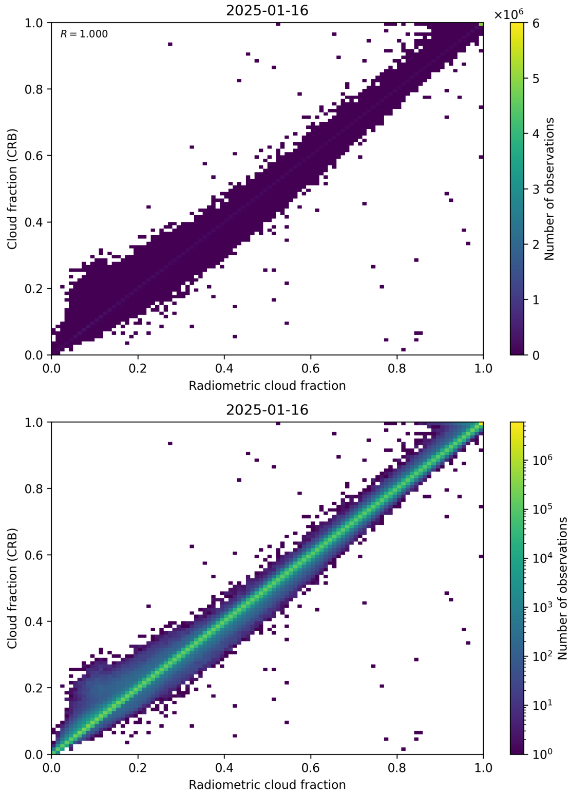
Figure 73: Scatter density plot of “Radiometric cloud fraction” against “Cloud fraction (CRB)” for 2025-01-15 to 2025-01-17.
