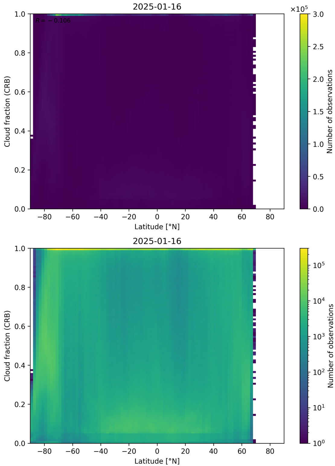
Figure 94: Scatter density plot of “Latitude” against “Cloud fraction (CRB)” for 2025-01-15 to 2025-01-17.
