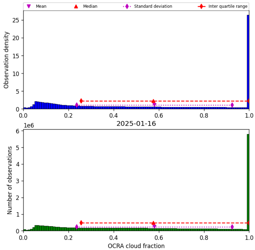
Figure 50: Histogram of “OCRA cloud fraction” for 2025-01-15 to 2025-01-17
