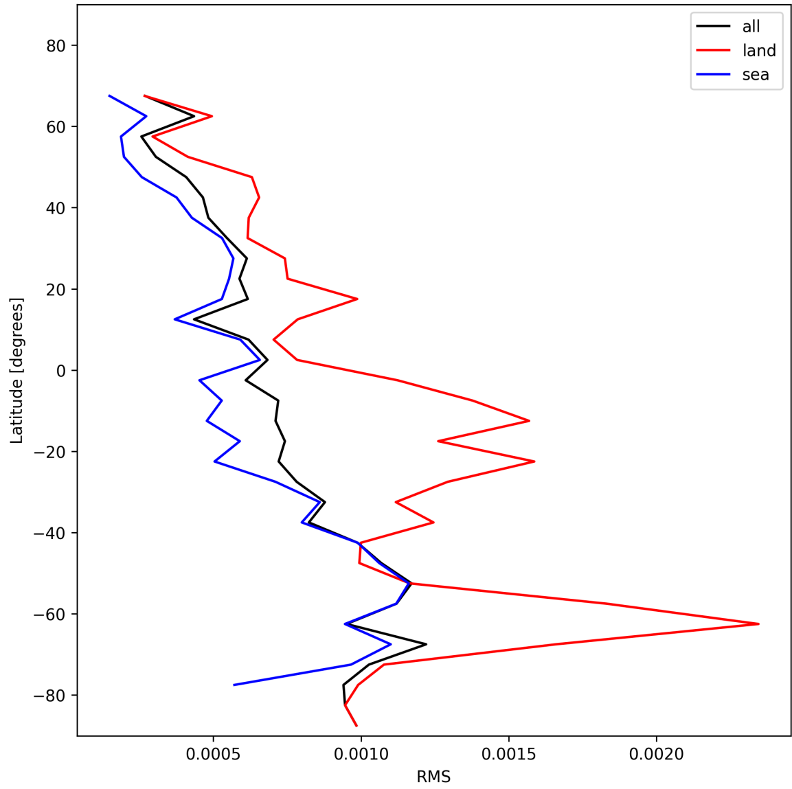
Figure 31: Zonal average of “RMS” for 2025-01-15 to 2025-01-17.
