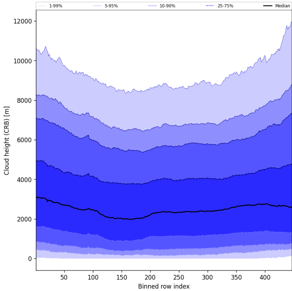
Figure 59: Along track statistics of “Cloud height (CRB)” for 2025-01-15 to 2025-01-17
