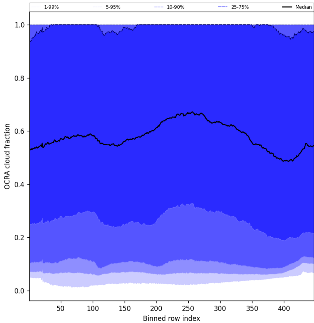
Figure 66: Along track statistics of “OCRA cloud fraction” for 2025-01-15 to 2025-01-17
