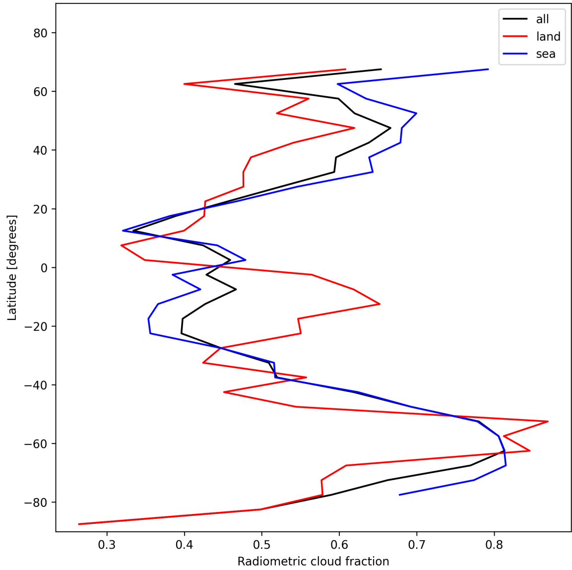
Figure 23: Zonal average of “Radiometric cloud fraction” for 2025-01-15 to 2025-01-17.
