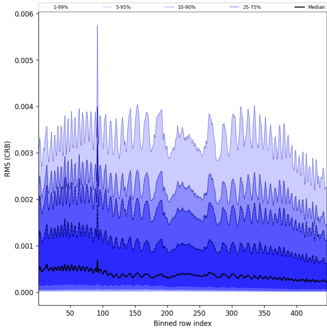
Figure 64: Along track statistics of “RMS (CRB)” for 2025-01-15 to 2025-01-17
