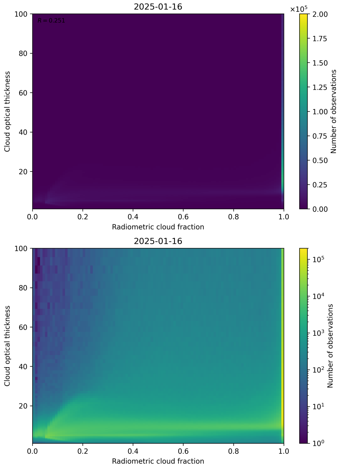
Figure 75: Scatter density plot of “Radiometric cloud fraction” against “Cloud optical thickness” for 2025-01-15 to 2025-01-17.
