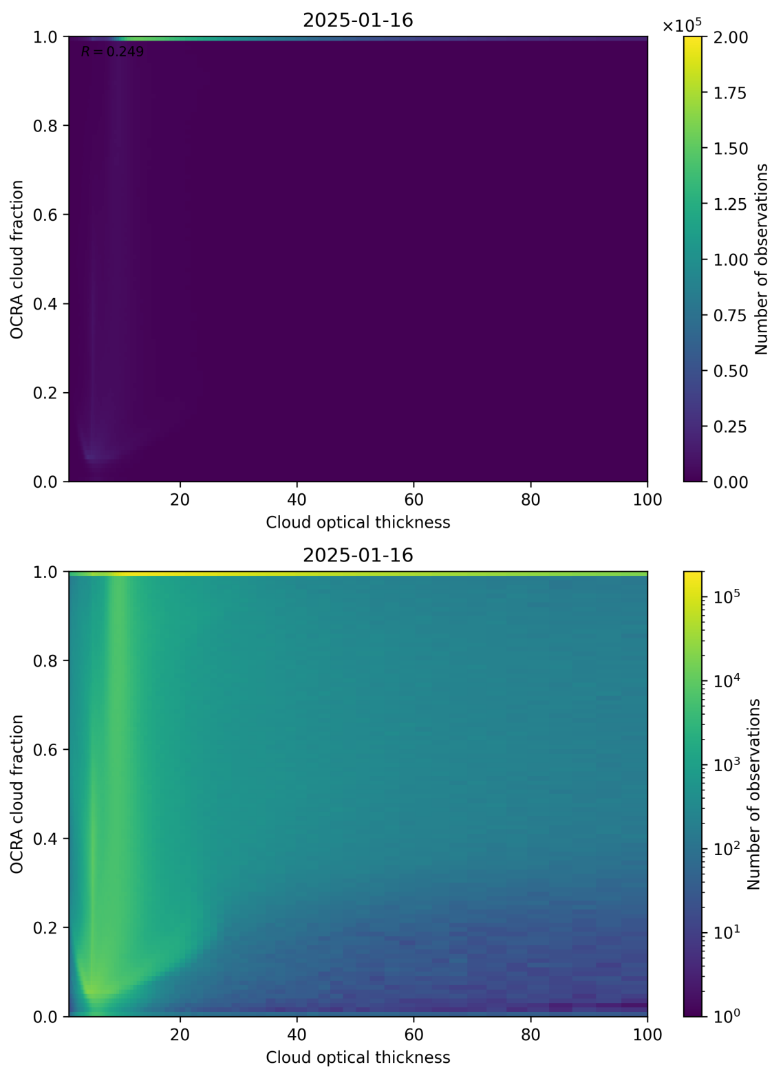
Figure 83: Scatter density plot of “Cloud optical thickness” against “OCRA cloud fraction” for 2025-01-15 to 2025-01-17.
