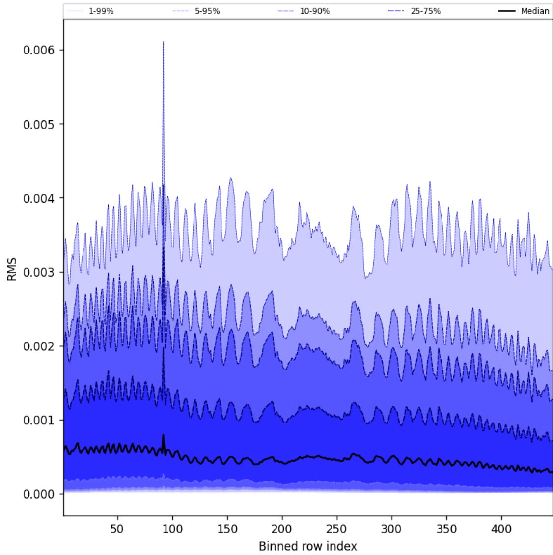
Figure 63: Along track statistics of “RMS” for 2025-01-15 to 2025-01-17
