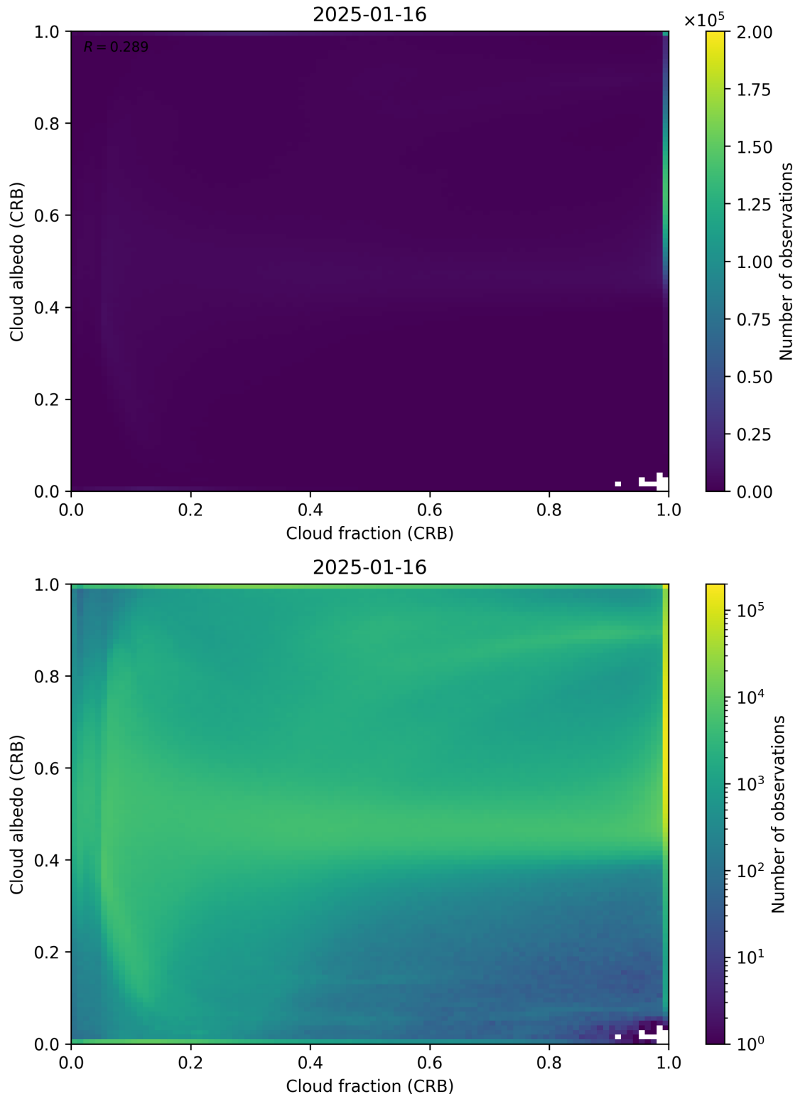
Figure 77: Scatter density plot of “Cloud fraction (CRB)” against “Cloud albedo (CRB)” for 2025-01-15 to 2025-01-17.
