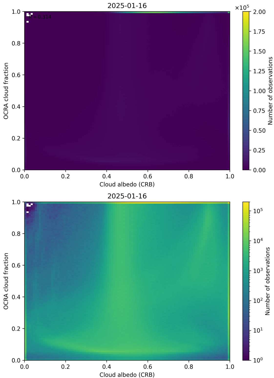
Figure 70: Scatter density plot of “Cloud albedo (CRB)” against “OCRA cloud fraction” for 2025-01-15 to 2025-01-17.
