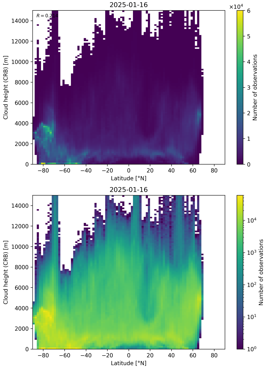
Figure 95: Scatter density plot of “Latitude” against “Cloud height (CRB)” for 2025-01-15 to 2025-01-17.
