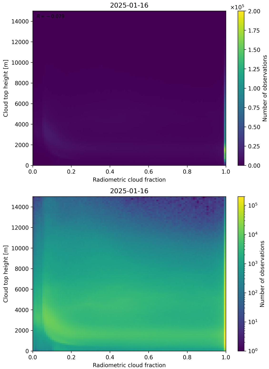
Figure 76: Scatter density plot of “Radiometric cloud fraction” against “Cloud top height” for 2025-01-15 to 2025-01-17.
