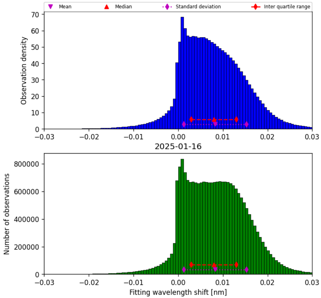
Figure 49: Histogram of “Fitting wavelength shift” for 2025-01-15 to 2025-01-17
