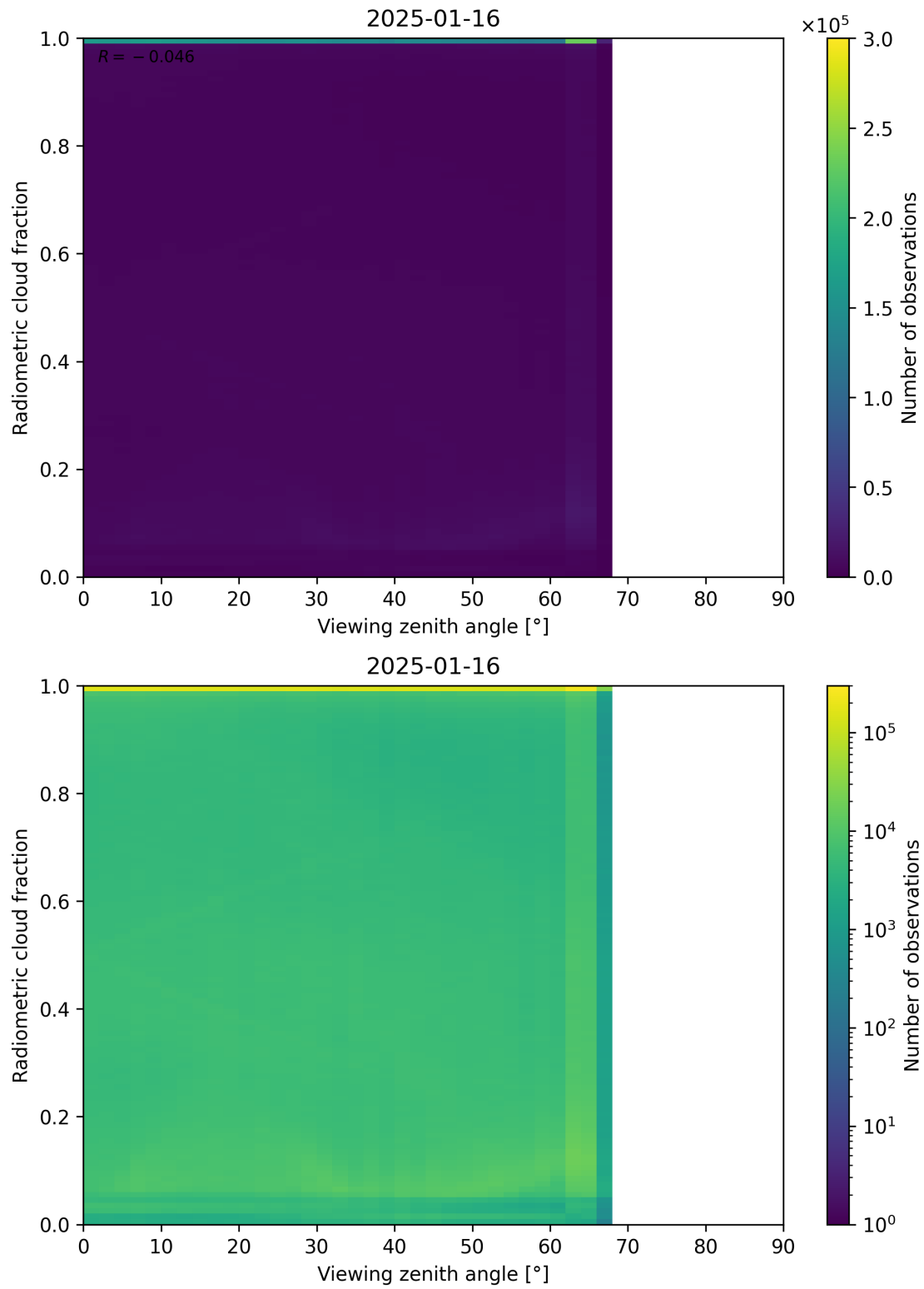
Figure 107: Scatter density plot of “Viewing zenith angle” against “Radiometric cloud fraction” for 2025-01-15 to 2025-01-17.
