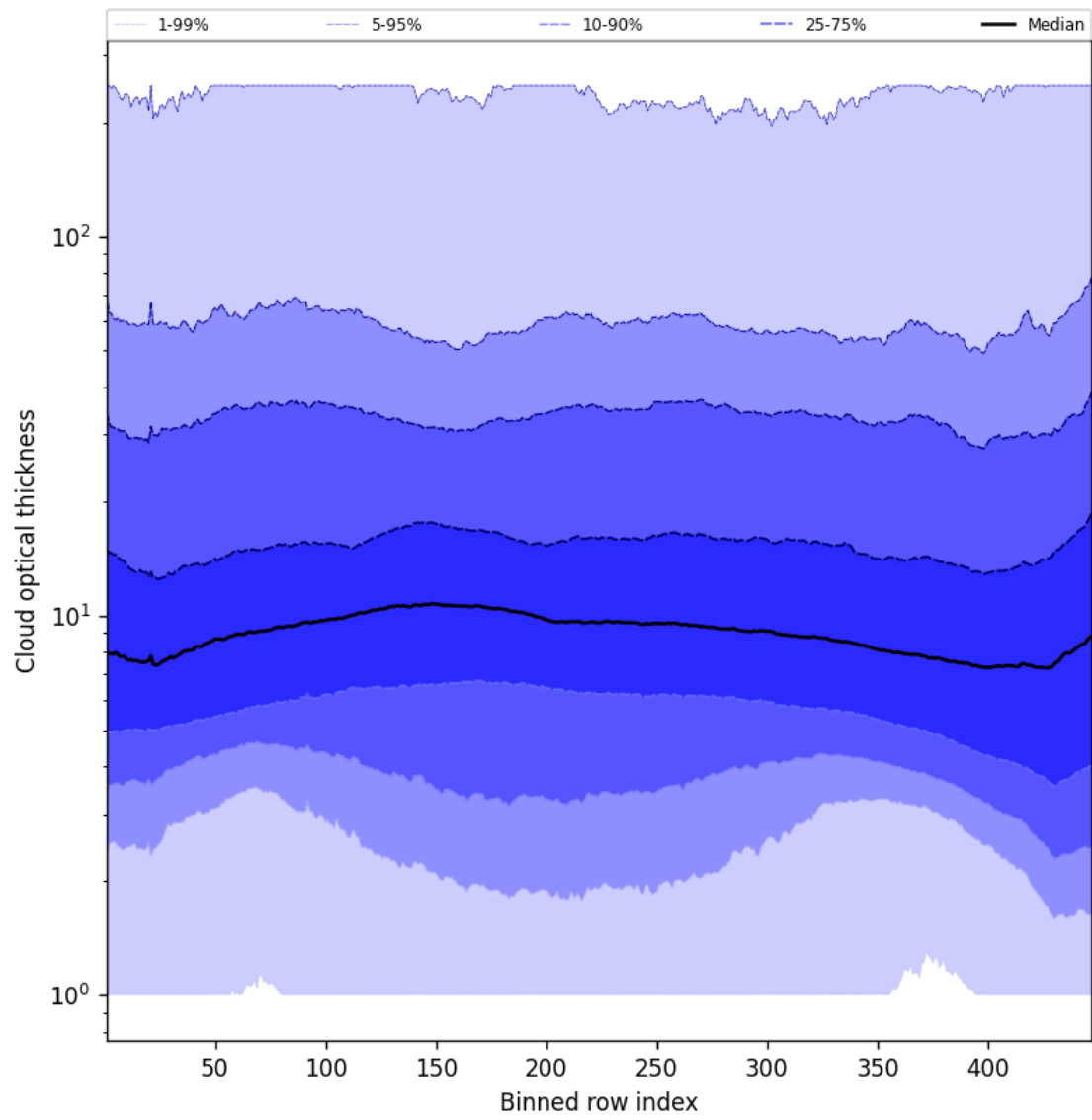
Figure 57: Along track statistics of “Cloud optical thickness” for 2025-01-15 to 2025-01-17
