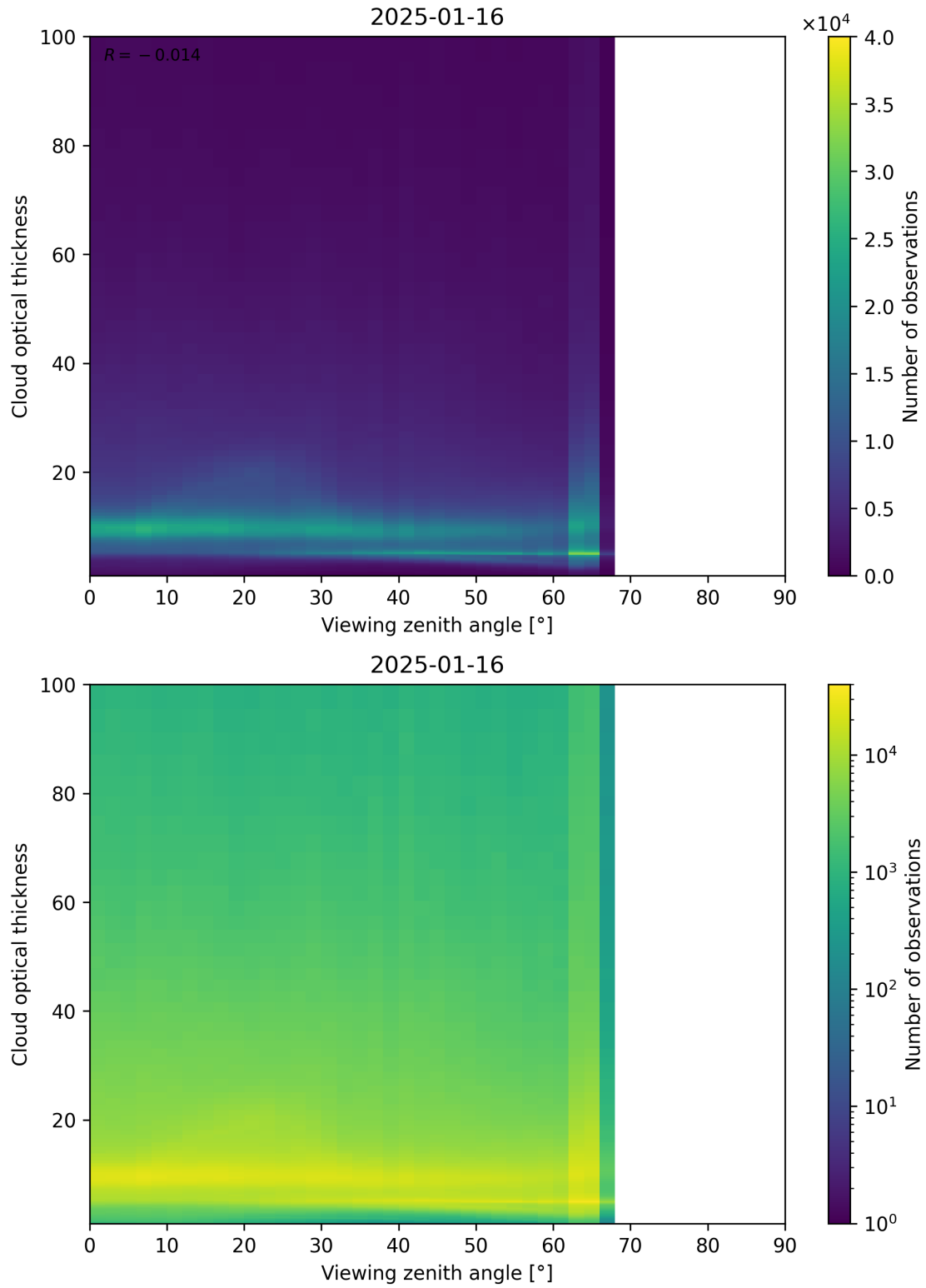
Figure 111: Scatter density plot of “Viewing zenith angle” against “Cloud optical thickness” for 2025-01-15 to 2025-01-17.
