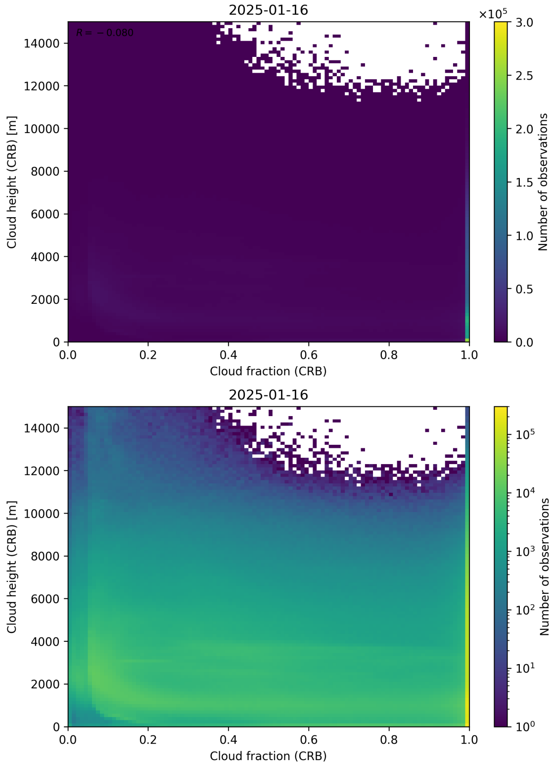
Figure 79: Scatter density plot of “Cloud fraction (CRB)” against “Cloud height (CRB)” for 2025-01-15 to 2025-01-17.
