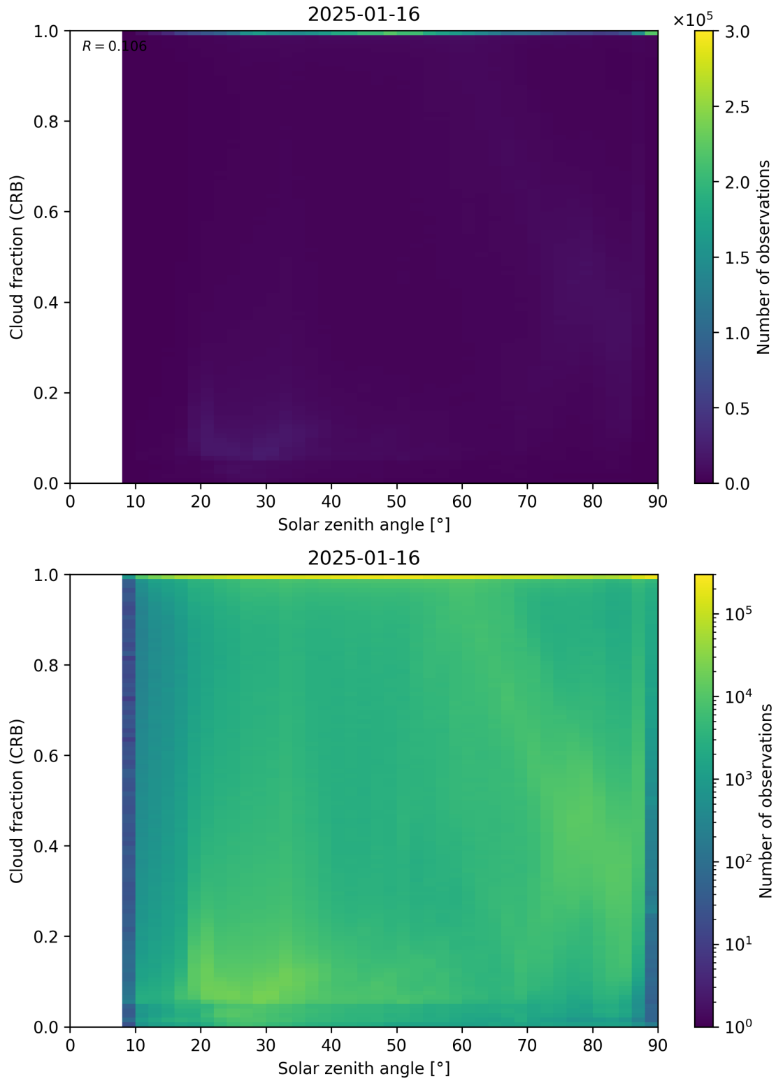
Figure 101: Scatter density plot of “Solar zenith angle” against “Cloud fraction (CRB)” for 2025-01-15 to 2025-01-17.
