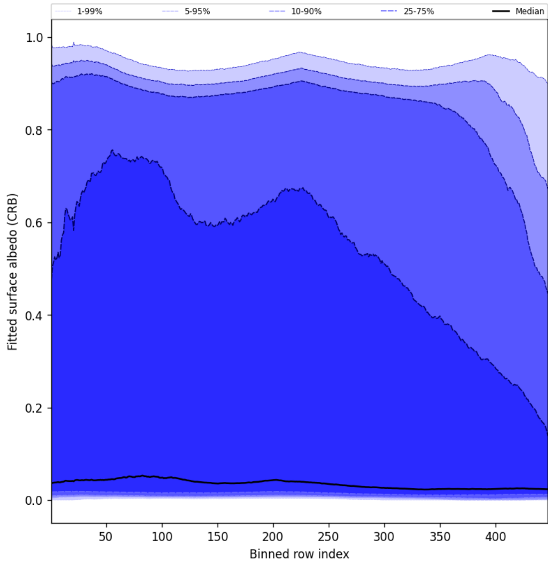
Figure 62: Along track statistics of “Fitted surface albedo (CRB)” for 2025-01-15 to 2025-01-17
