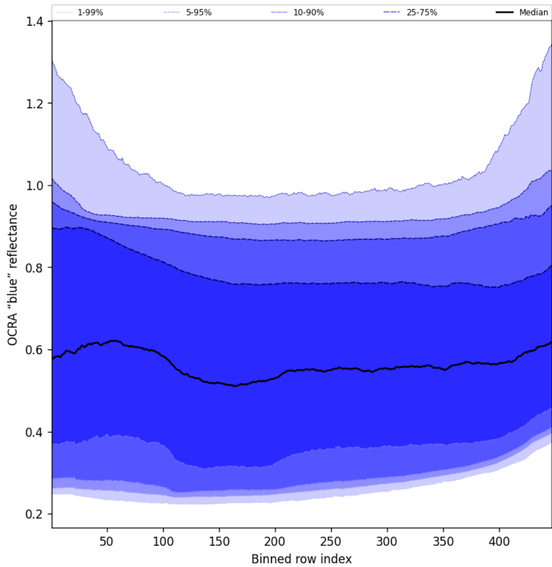
Figure 67: Along track statistics of “OCRA “blue” reflectance” for 2025-01-15 to 2025-01-17
