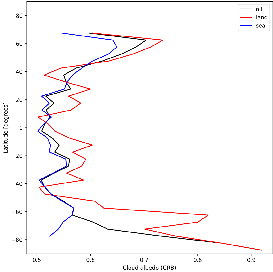
Figure 28: Zonal average of “Cloud albedo (CRB)” for 2025-01-15 to 2025-01-17.
