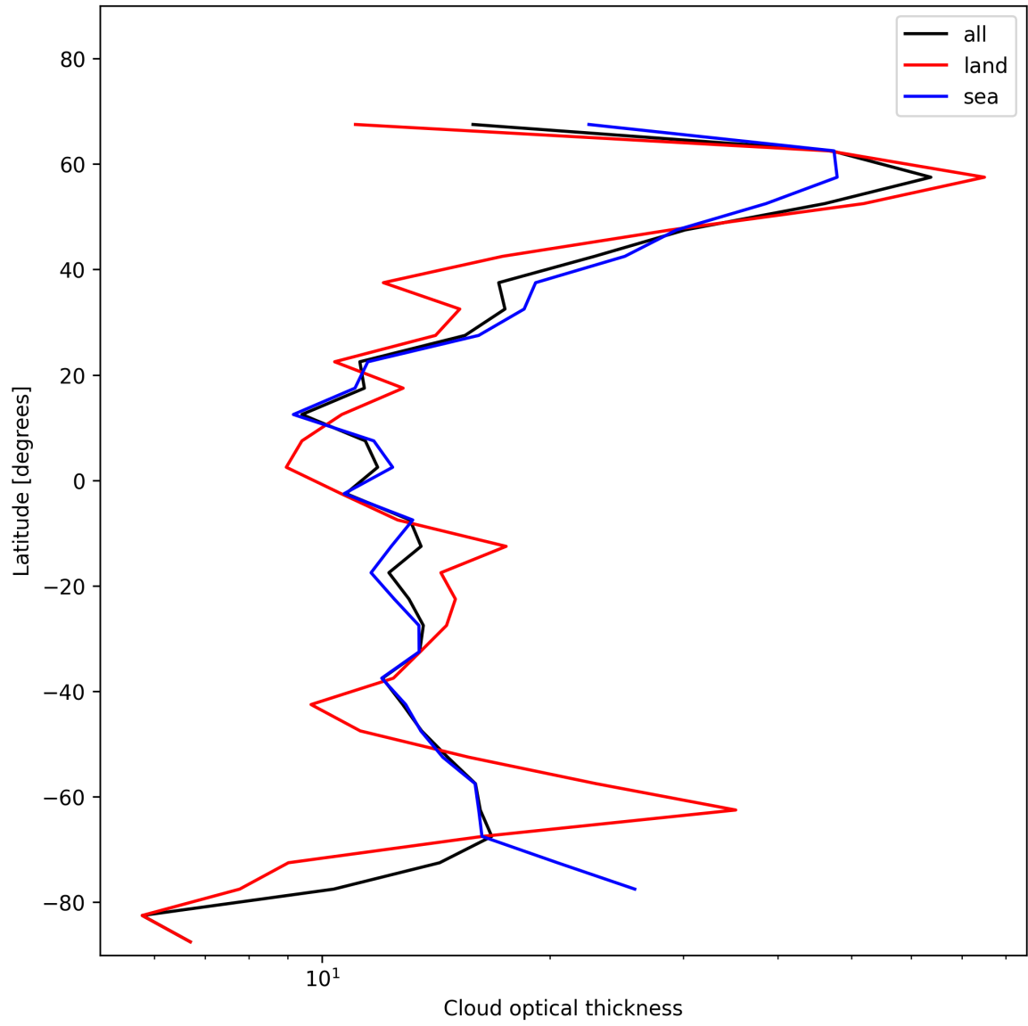
Figure 25: Zonal average of “Cloud optical thickness” for 2025-01-15 to 2025-01-17.
