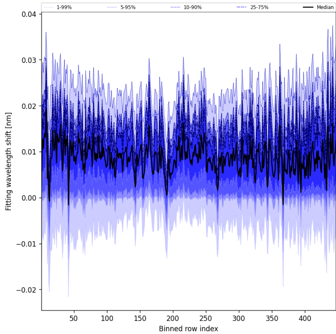
Figure 65: Along track statistics of “Fitting wavelength shift” for 2025-01-15 to 2025-01-17
