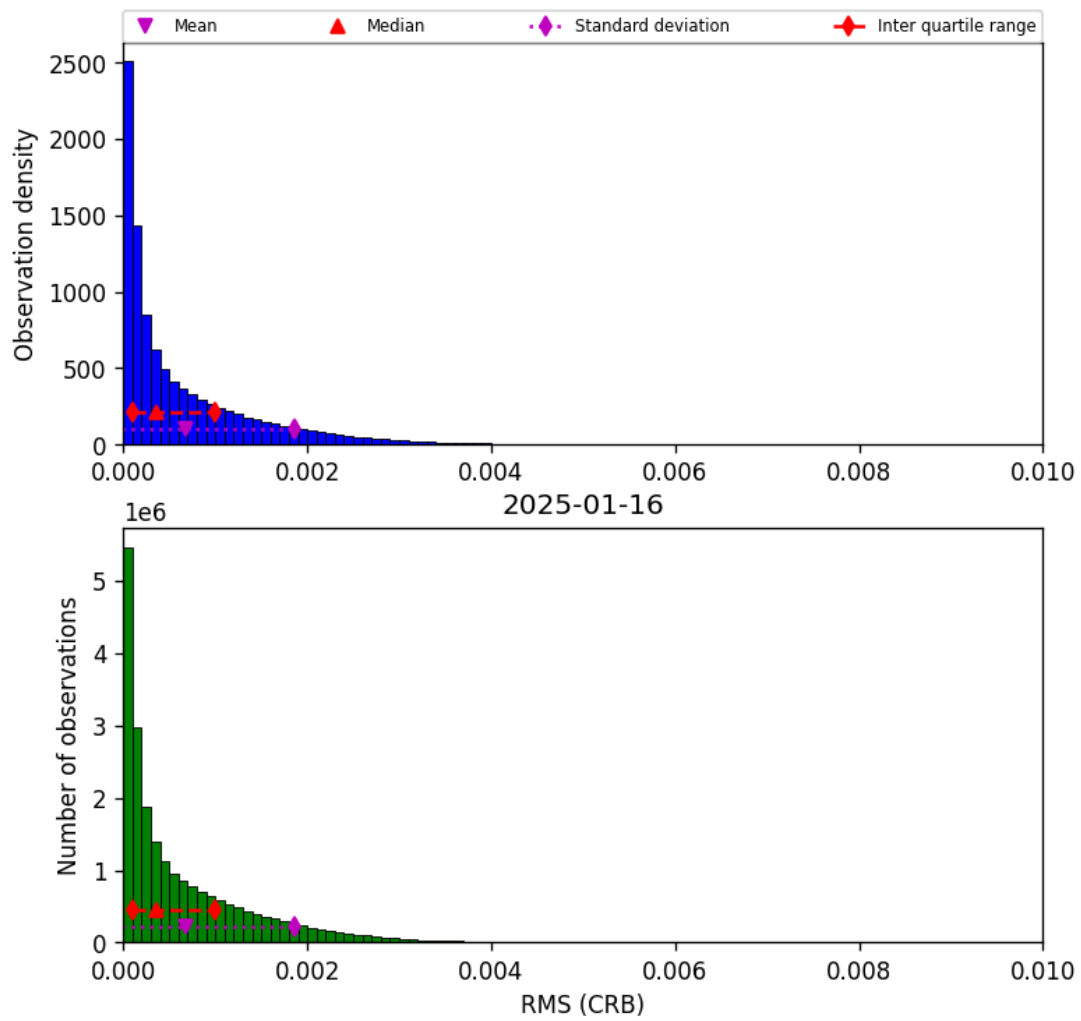
Figure 48: Histogram of “RMS (CRB)” for 2025-01-15 to 2025-01-17
