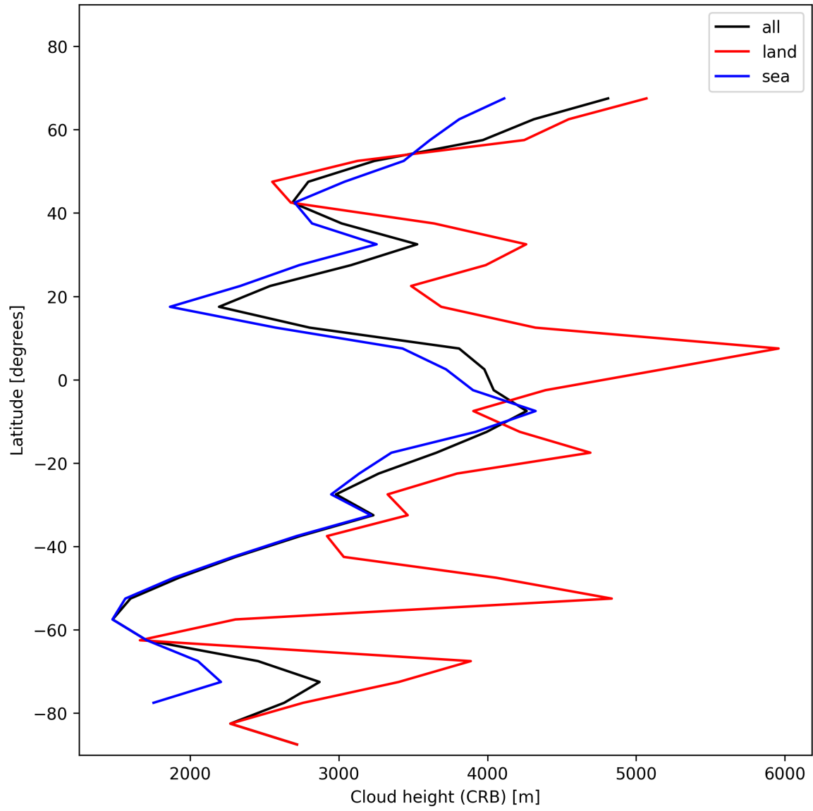
Figure 27: Zonal average of “Cloud height (CRB)” for 2025-01-15 to 2025-01-17.
