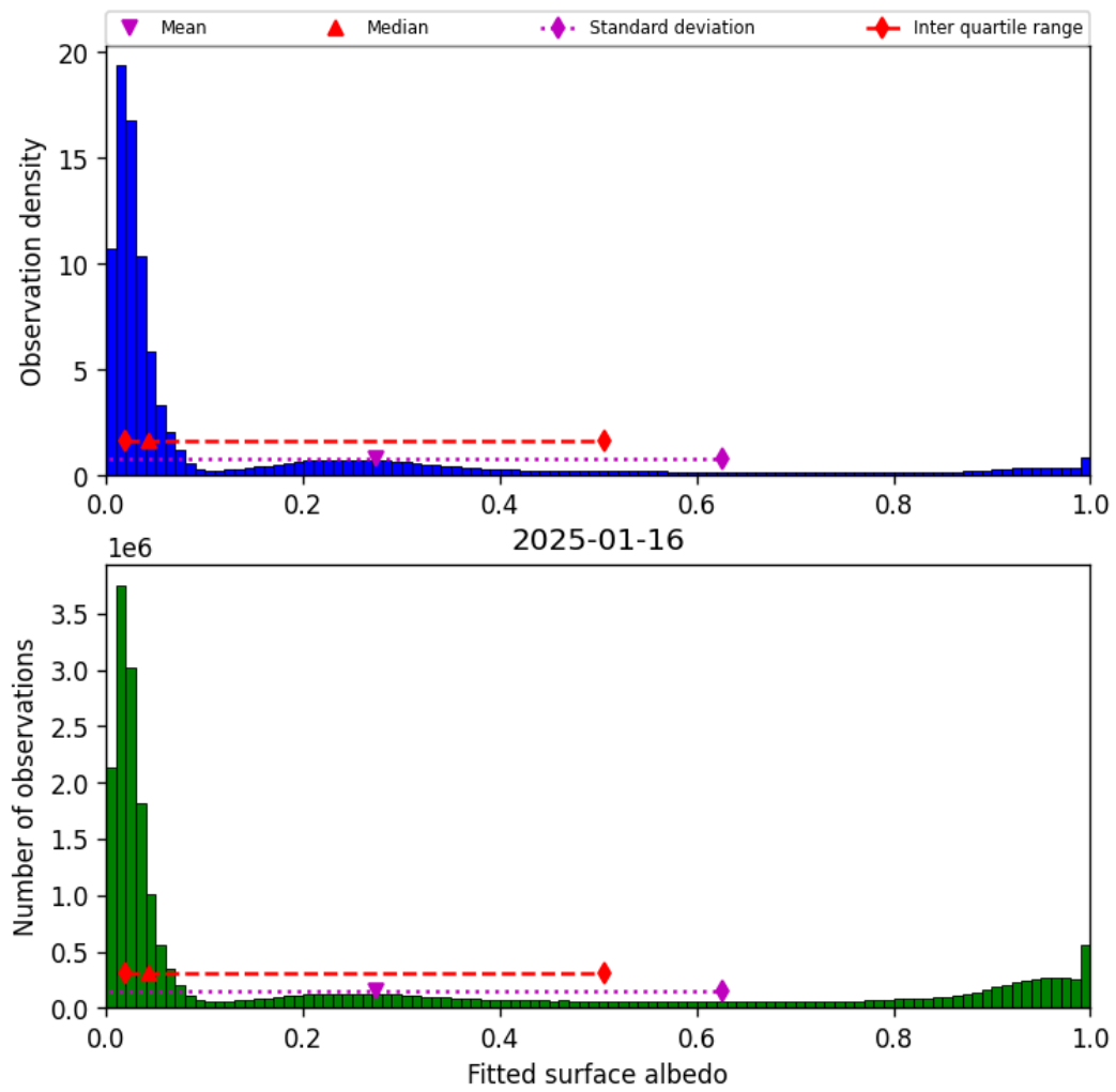
Figure 45: Histogram of “Fitted surface albedo” for 2025-01-15 to 2025-01-17
