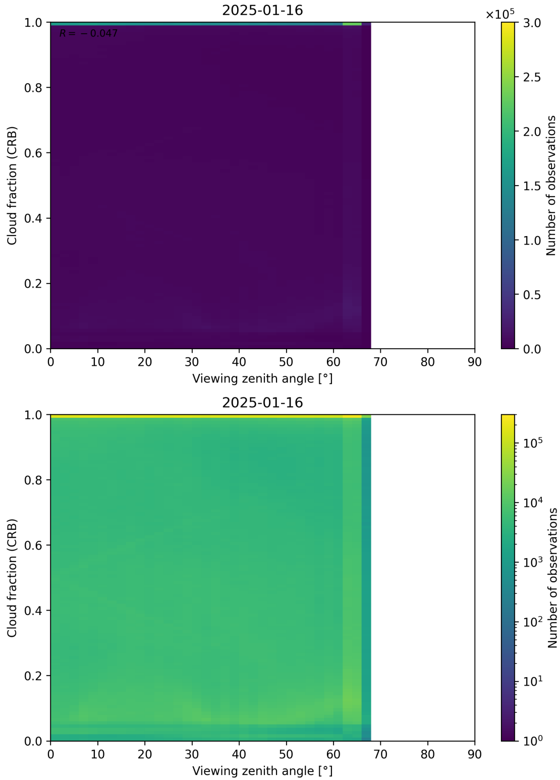
Figure 109: Scatter density plot of “Viewing zenith angle” against “Cloud fraction (CRB)” for 2025-01-15 to 2025-01-17.
