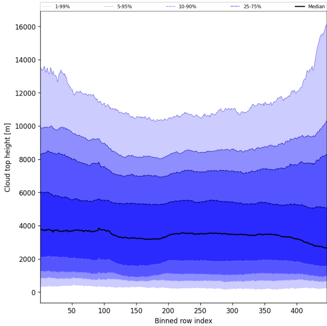
Figure 56: Along track statistics of “Cloud top height” for 2025-01-15 to 2025-01-17
