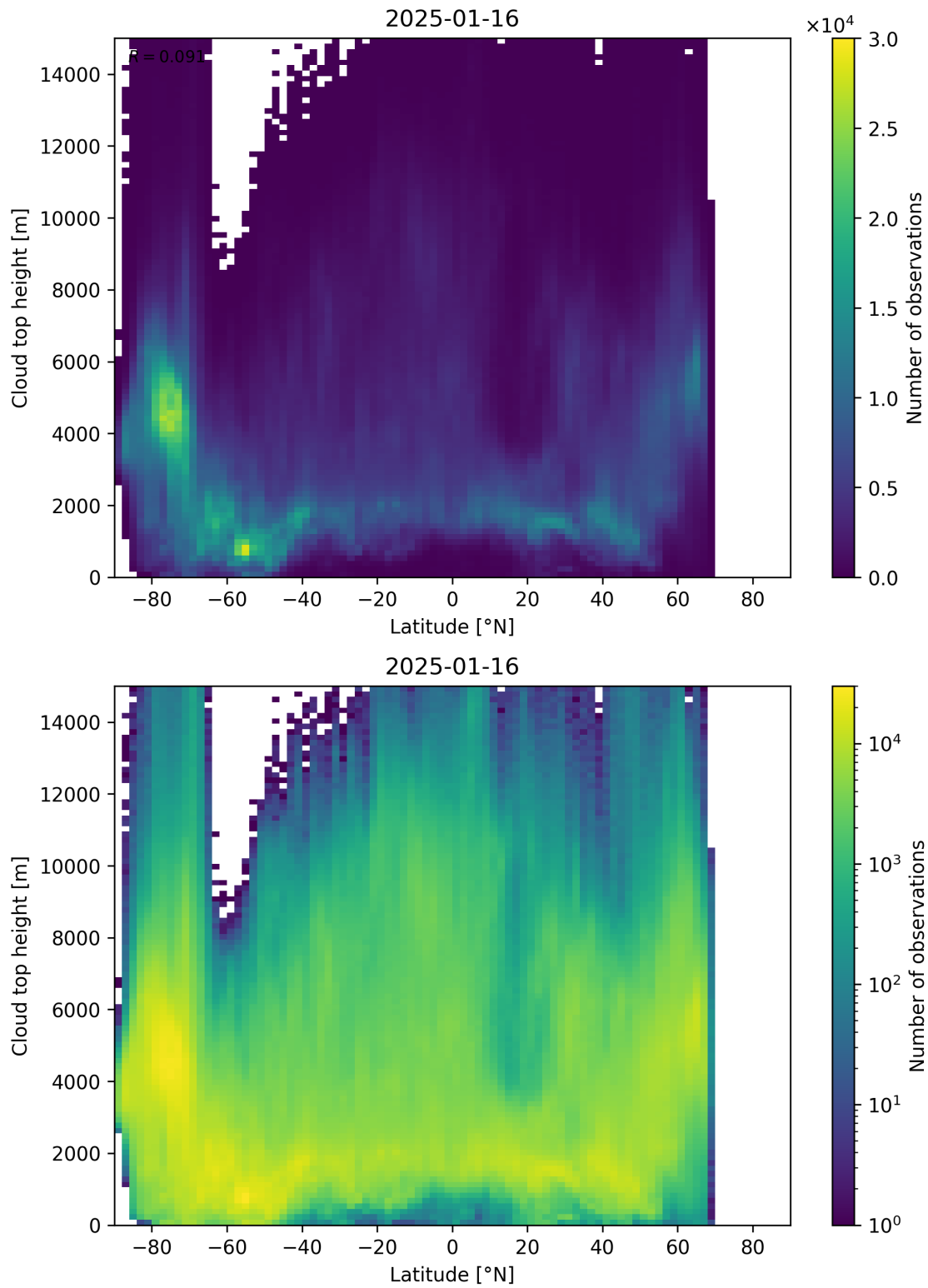
Figure 97: Scatter density plot of “Latitude” against “Cloud top height” for 2025-01-15 to 2025-01-17.
