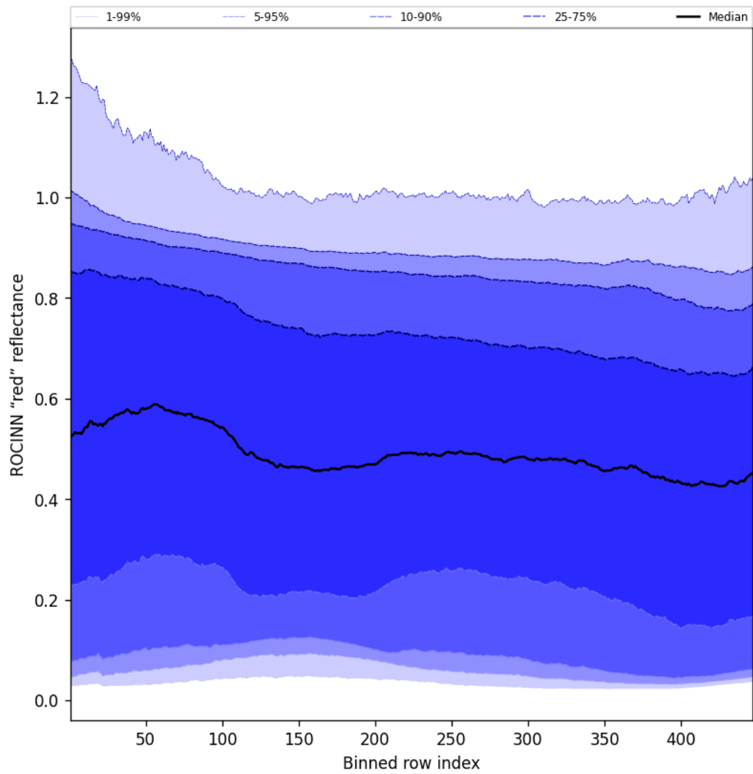
Figure 69: Along track statistics of “ROCINN “red” reflectance” for 2025-01-15 to 2025-01-17
