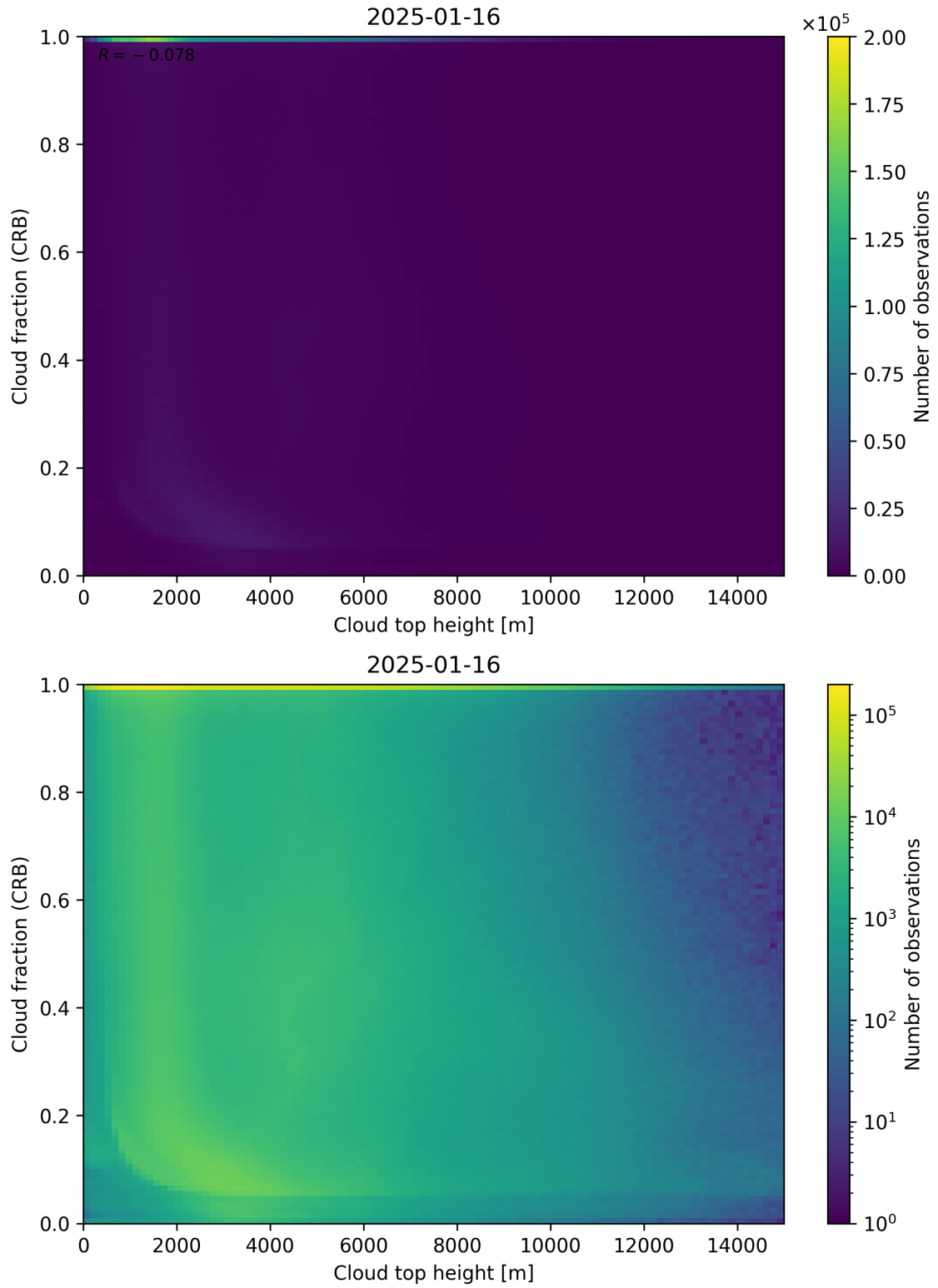
Figure 88: Scatter density plot of “Cloud top height” against “Cloud fraction (CRB)” for 2025-01-15 to 2025-01-17.
