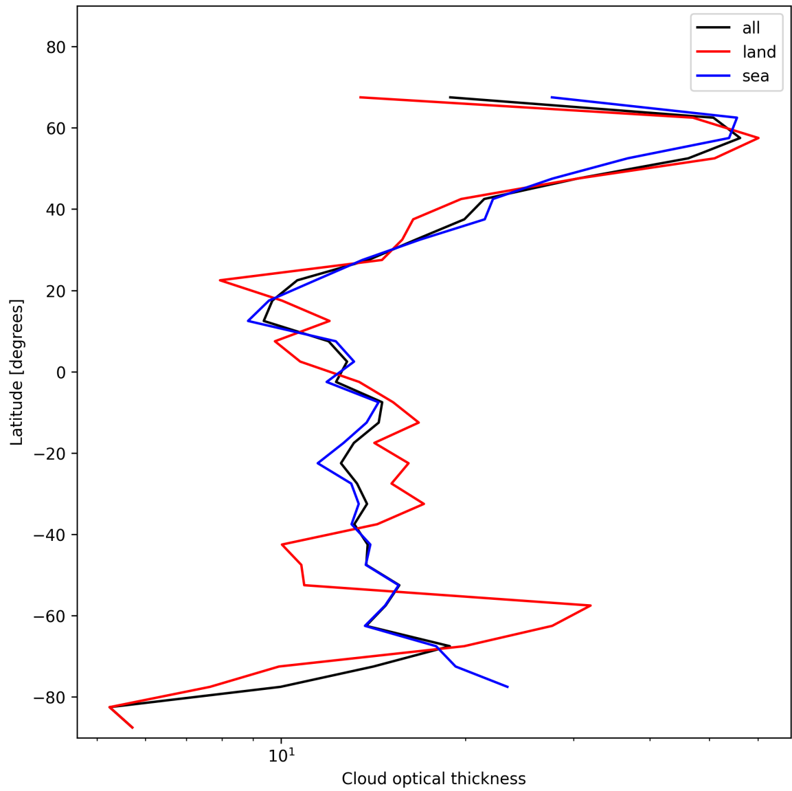
Figure 25: Zonal average of “Cloud optical thickness” for 2025-01-17 to 2025-01-18.
