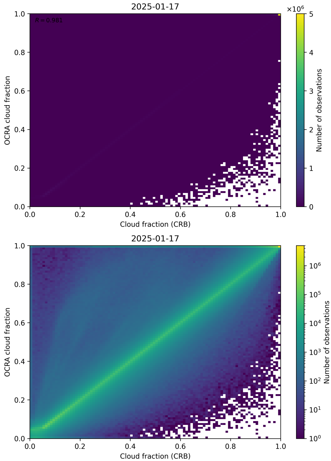
Figure 78: Scatter density plot of “Cloud fraction (CRB)” against “OCRA cloud fraction” for 2025-01-17 to 2025-01-18.
