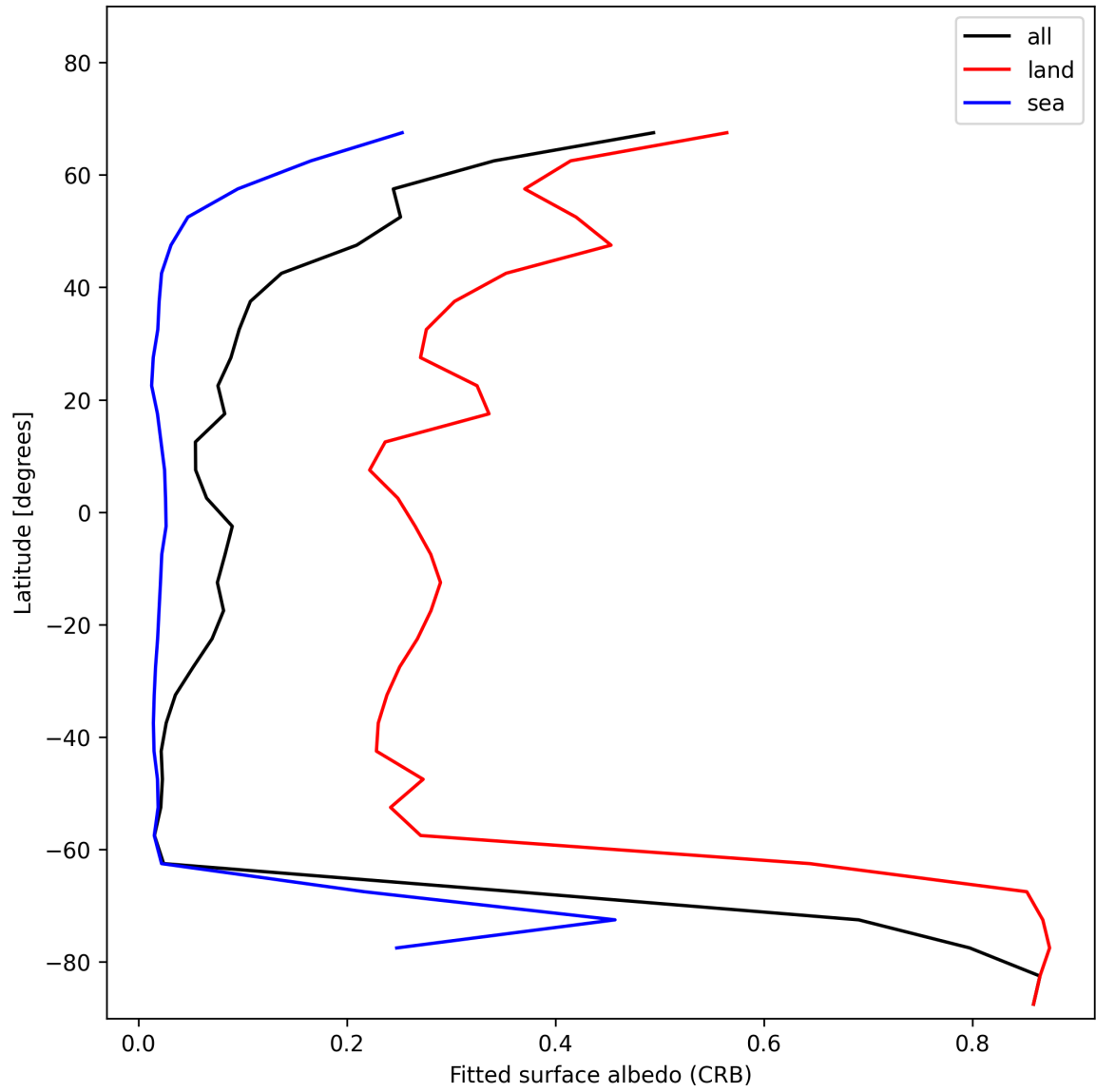
Figure 30: Zonal average of “Fitted surface albedo (CRB)” for 2025-01-17 to 2025-01-18.
