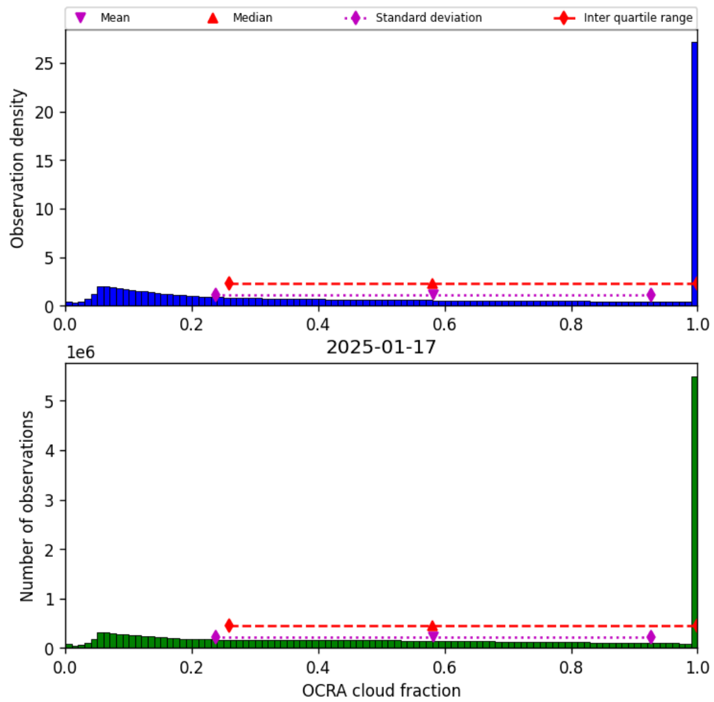
Figure 50: Histogram of “OCRA cloud fraction” for 2025-01-17 to 2025-01-18
