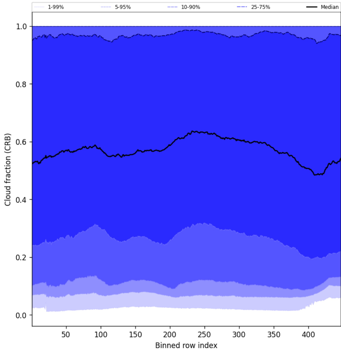
Figure 58: Along track statistics of “Cloud fraction (CRB)” for 2025-01-17 to 2025-01-18
