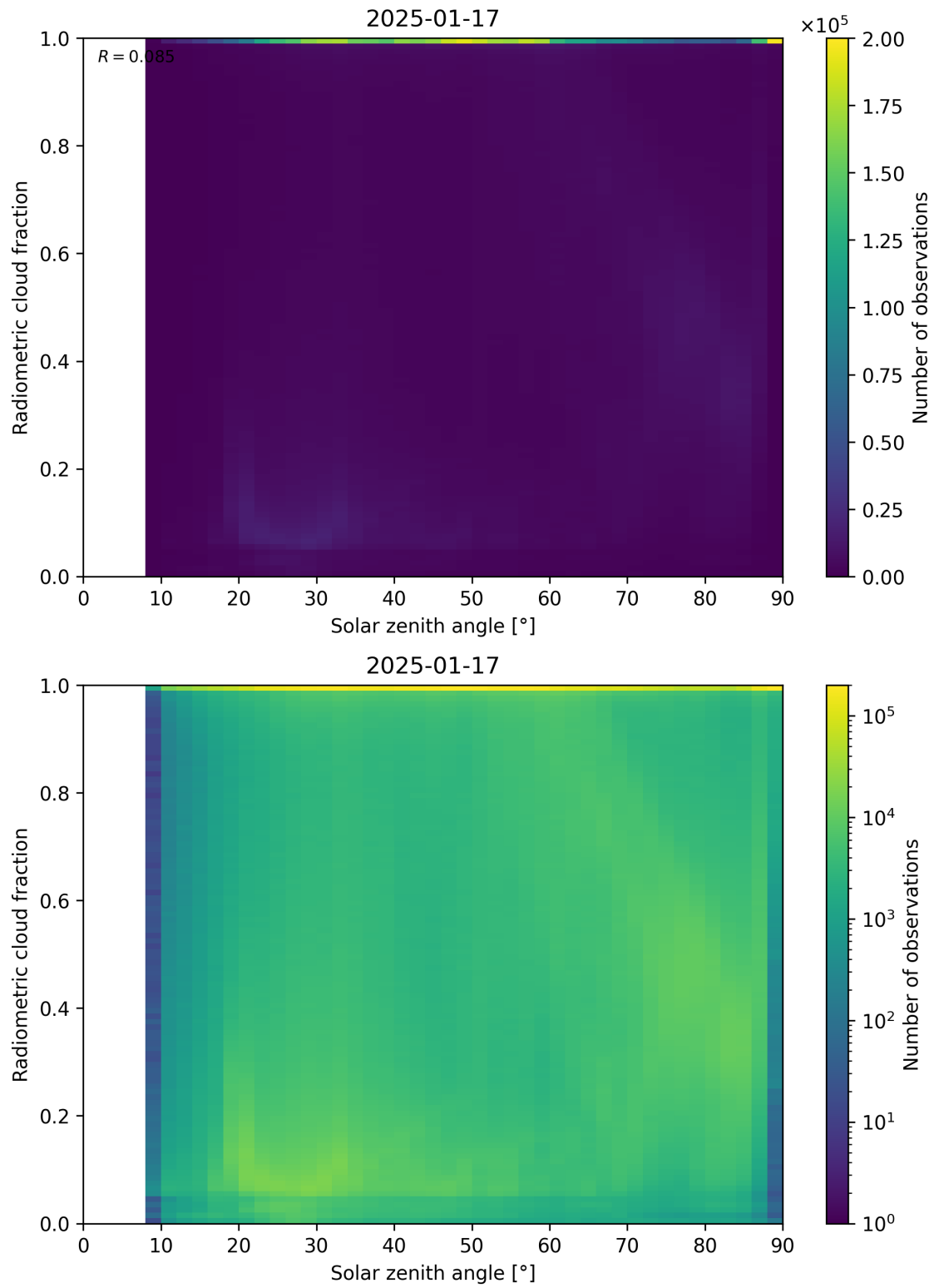
Figure 99: Scatter density plot of “Solar zenith angle” against “Radiometric cloud fraction” for 2025-01-17 to 2025-01-18.
