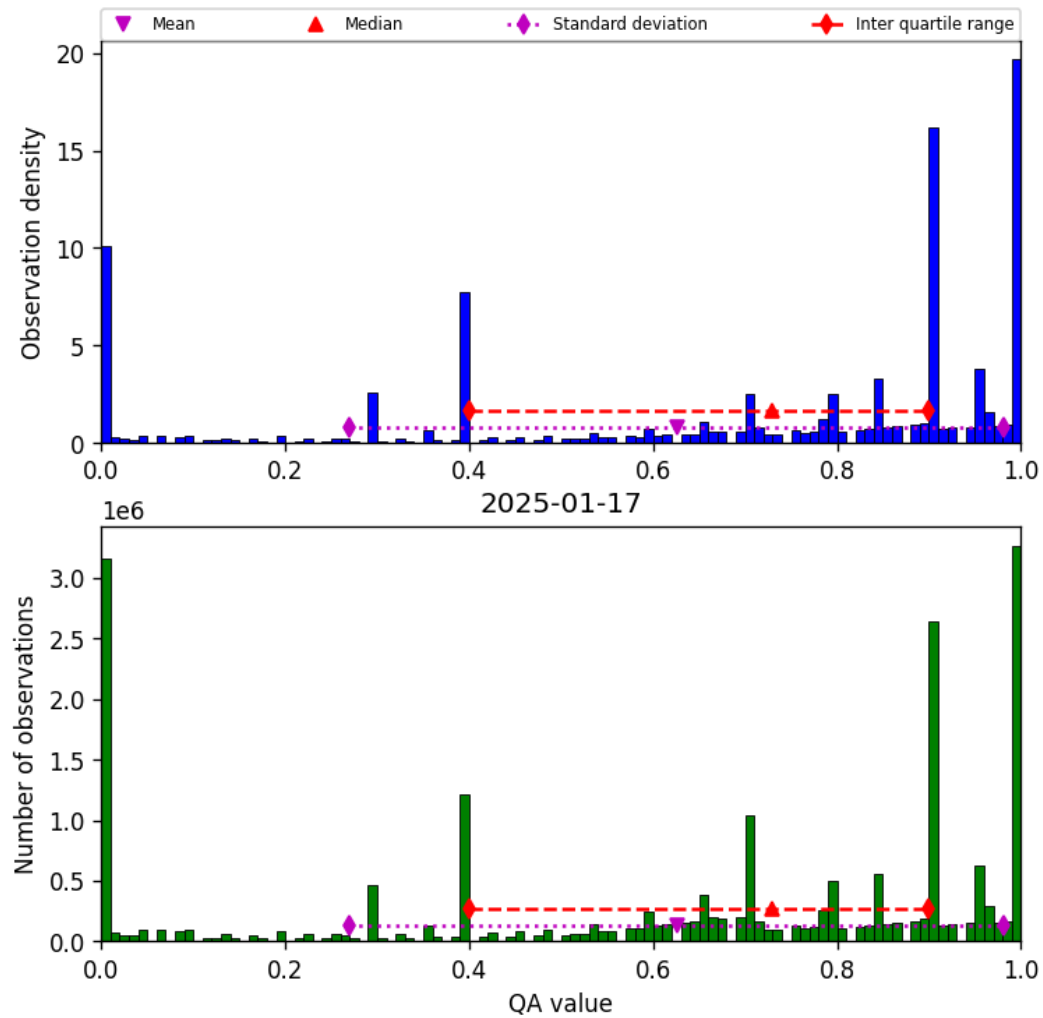
Figure 38: Histogram of “QA value” for 2025-01-17 to 2025-01-18
