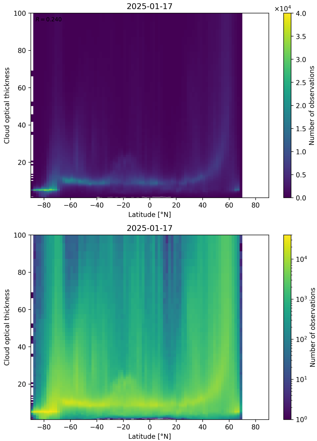
Figure 96: Scatter density plot of “Latitude” against “Cloud optical thickness” for 2025-01-17 to 2025-01-18.
