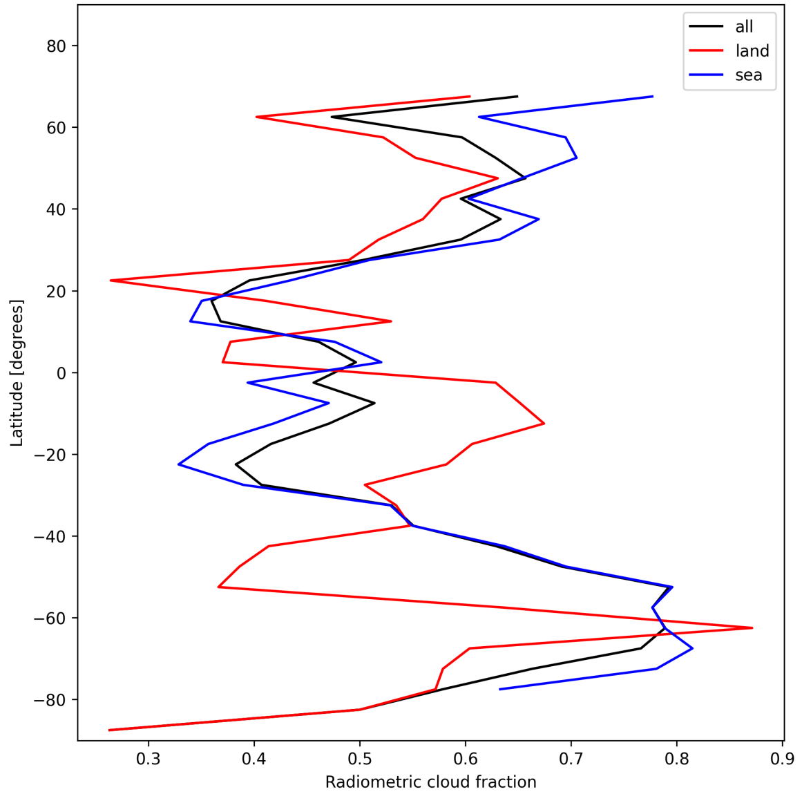
Figure 23: Zonal average of “Radiometric cloud fraction” for 2025-01-17 to 2025-01-18.
