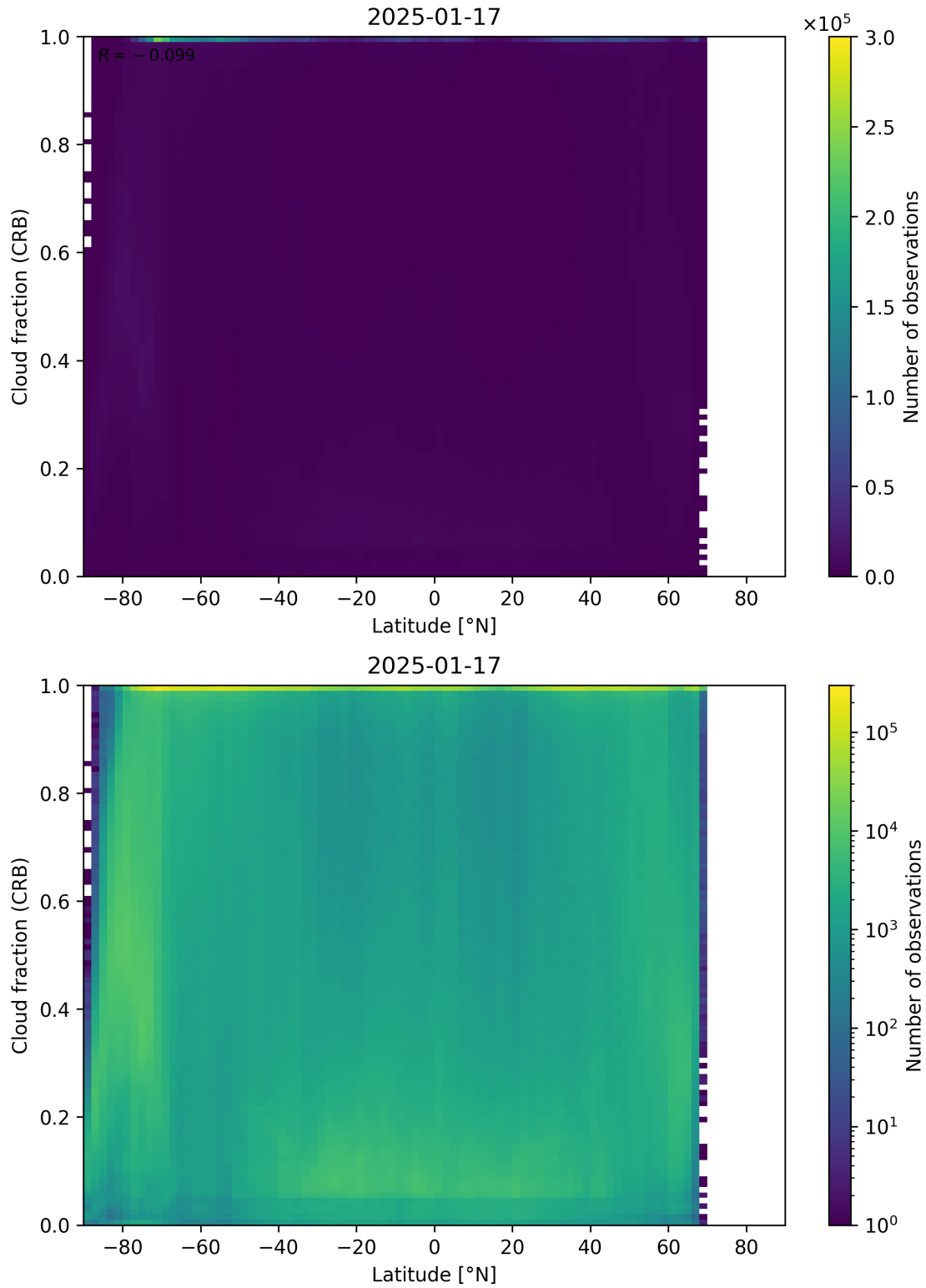
Figure 94: Scatter density plot of “Latitude” against “Cloud fraction (CRB)” for 2025-01-17 to 2025-01-18.
