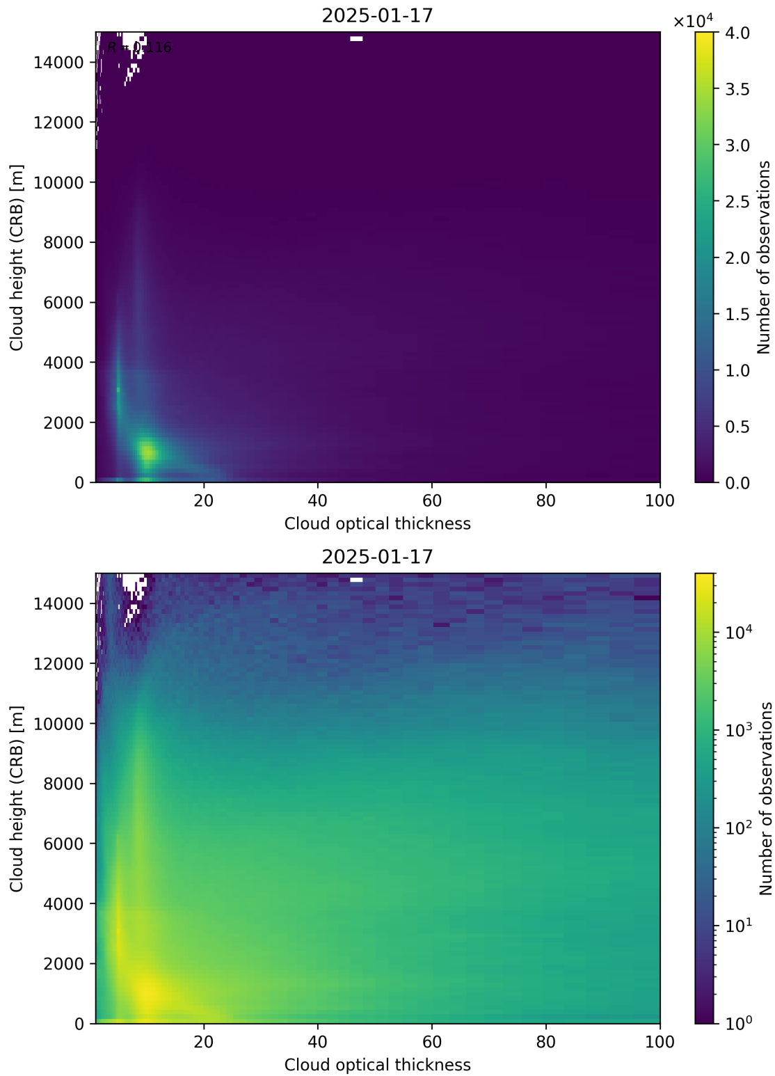
Figure 85: Scatter density plot of “Cloud optical thickness” against “Cloud height (CRB)” for 2025-01-17 to 2025-01-18.
