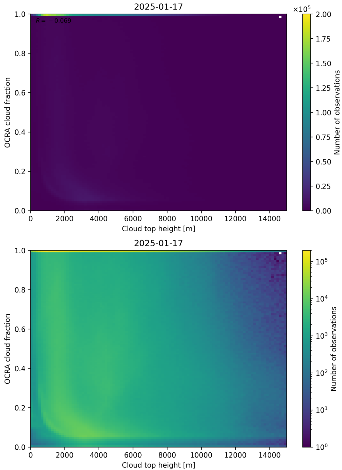
Figure 87: Scatter density plot of “Cloud top height” against “OCRA cloud fraction” for 2025-01-17 to 2025-01-18.
