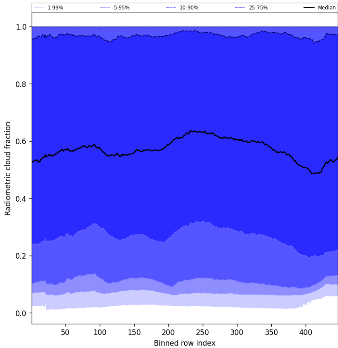
Figure 55: Along track statistics of “Radiometric cloud fraction” for 2025-01-17 to 2025-01-18
