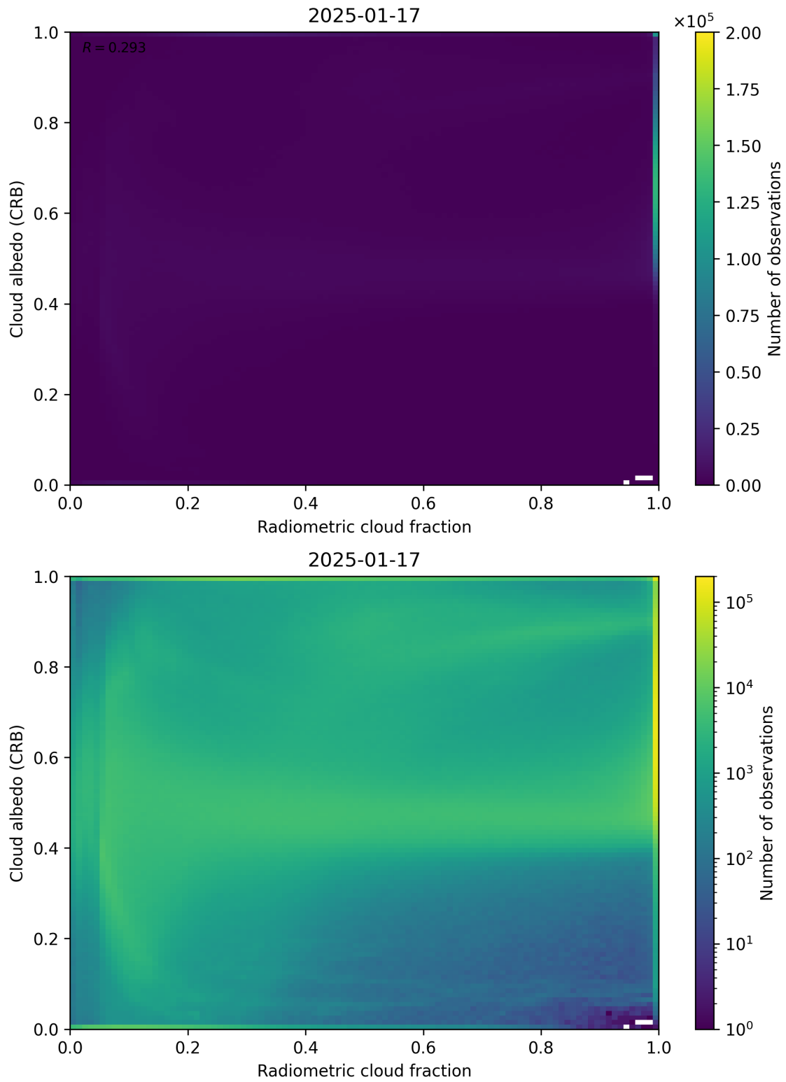
Figure 71: Scatter density plot of “Radiometric cloud fraction” against “Cloud albedo (CRB)” for 2025-01-17 to 2025-01-18.
