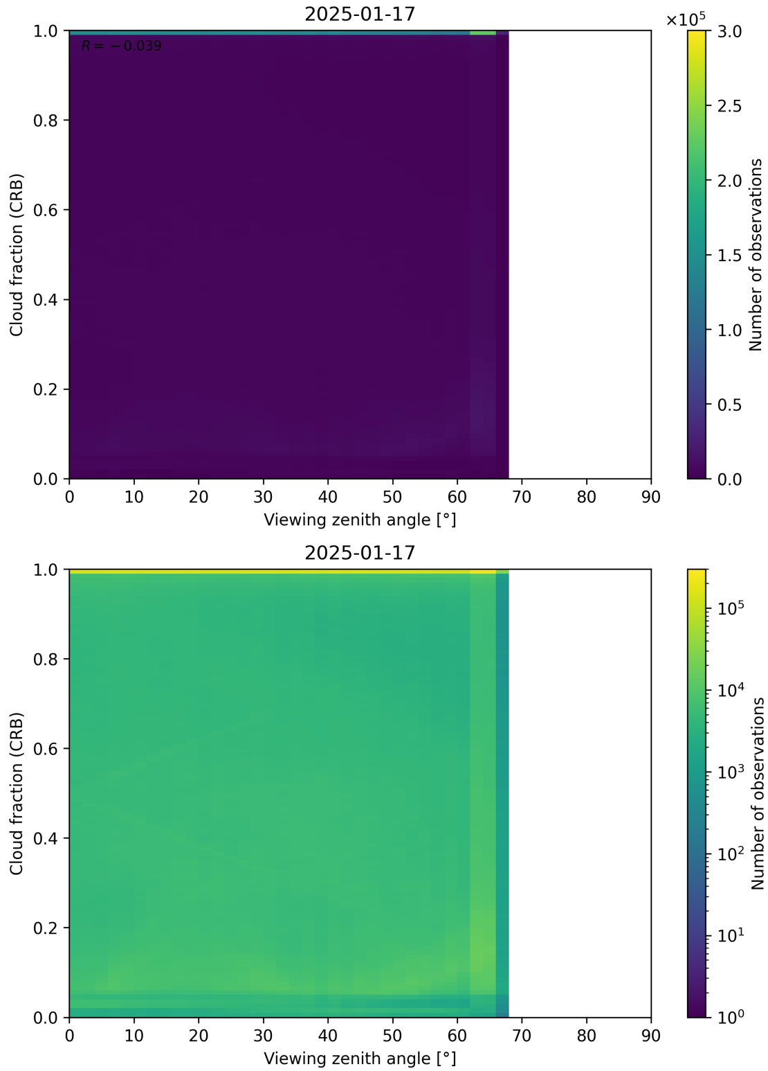
Figure 109: Scatter density plot of “Viewing zenith angle” against “Cloud fraction (CRB)” for 2025-01-17 to 2025-01-18.
