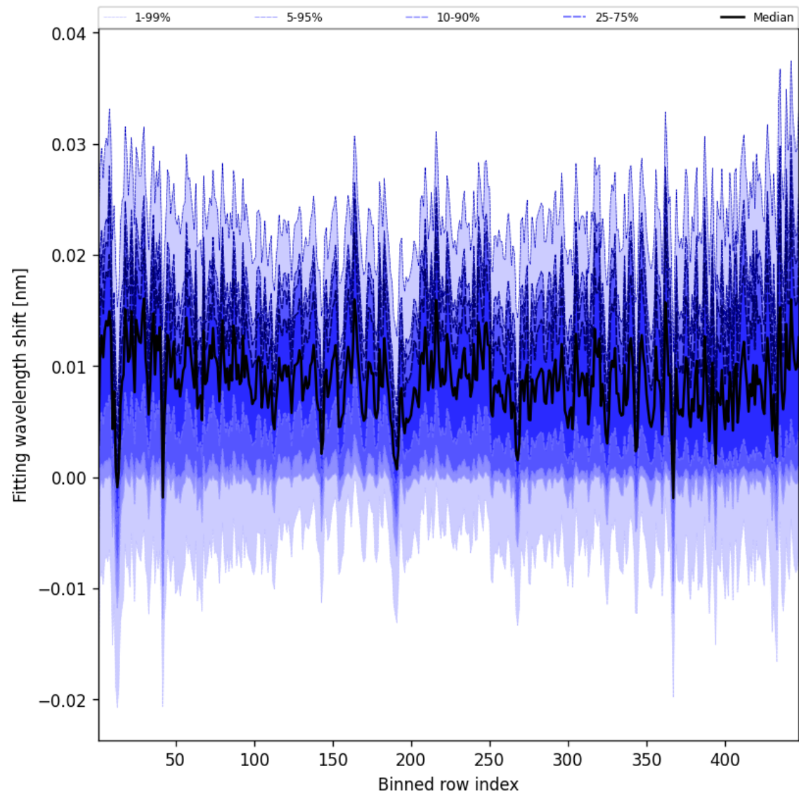
Figure 65: Along track statistics of “Fitting wavelength shift” for 2025-01-17 to 2025-01-18
