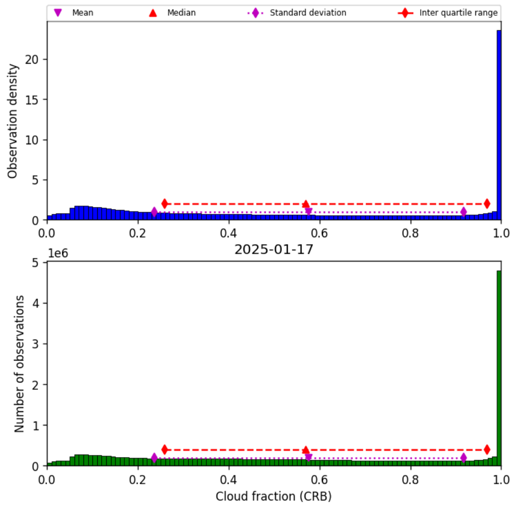
Figure 42: Histogram of “Cloud fraction (CRB)” for 2025-01-17 to 2025-01-18
