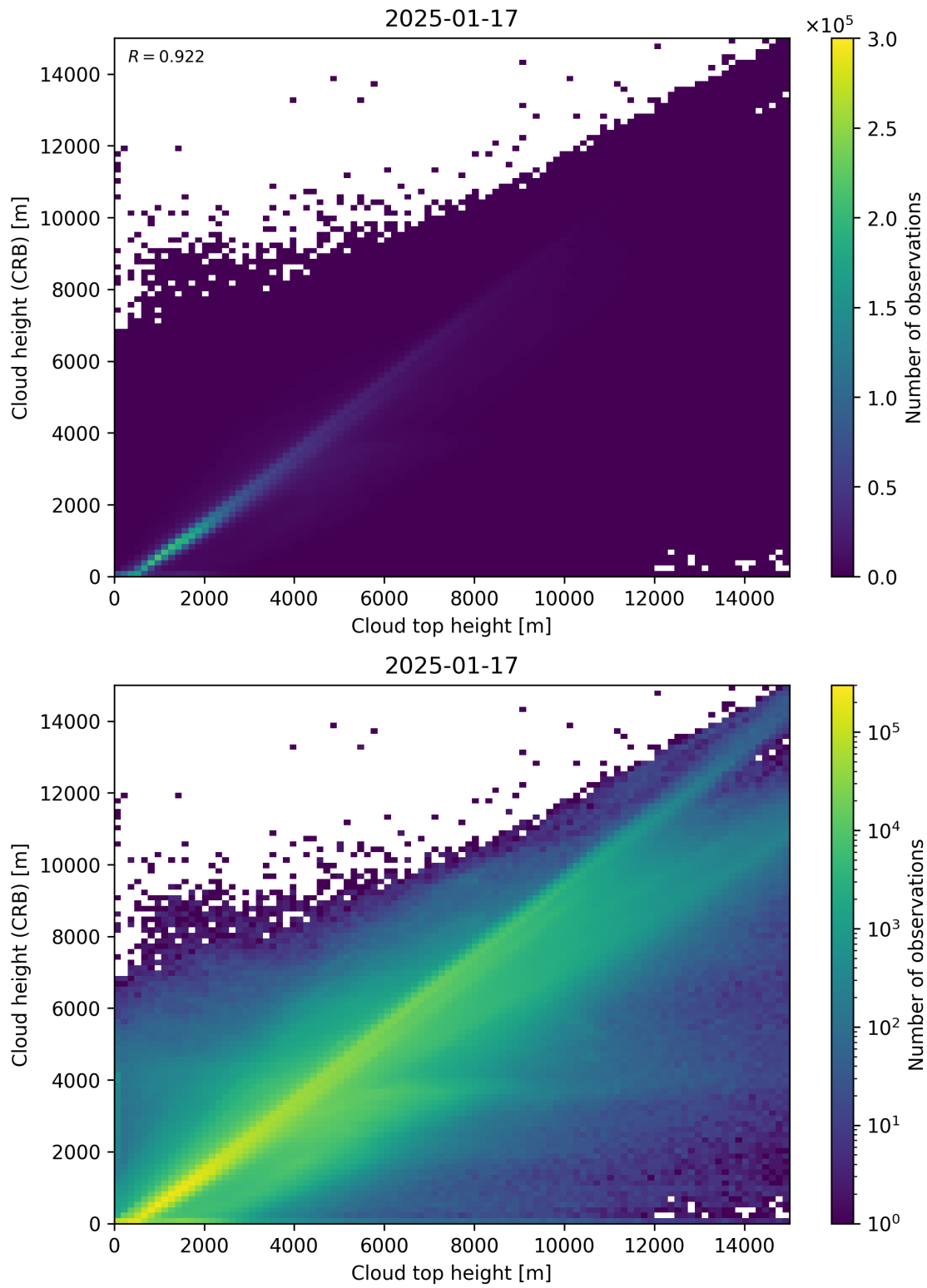
Figure 89: Scatter density plot of “Cloud top height” against “Cloud height (CRB)” for 2025-01-17 to 2025-01-18.
