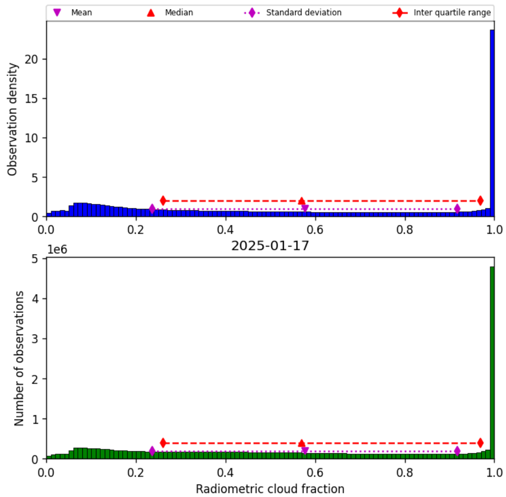
Figure 39: Histogram of “Radiometric cloud fraction” for 2025-01-17 to 2025-01-18
