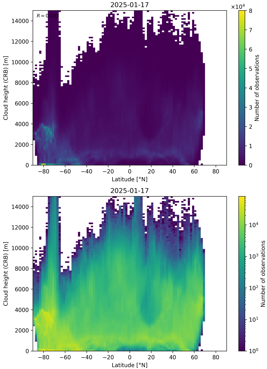
Figure 95: Scatter density plot of “Latitude” against “Cloud height (CRB)” for 2025-01-17 to 2025-01-18.
