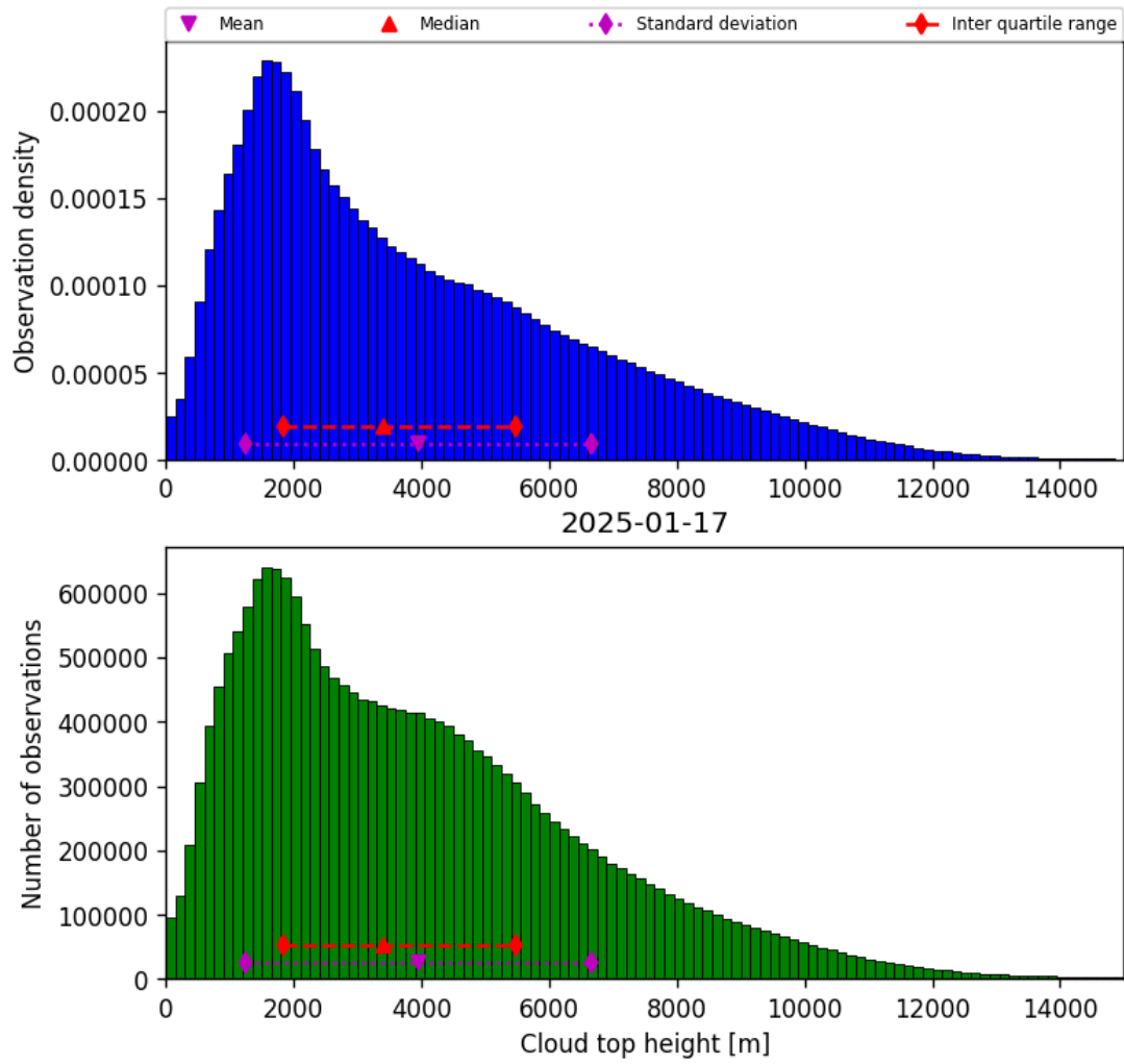
Figure 40: Histogram of “Cloud top height” for 2025-01-17 to 2025-01-18
