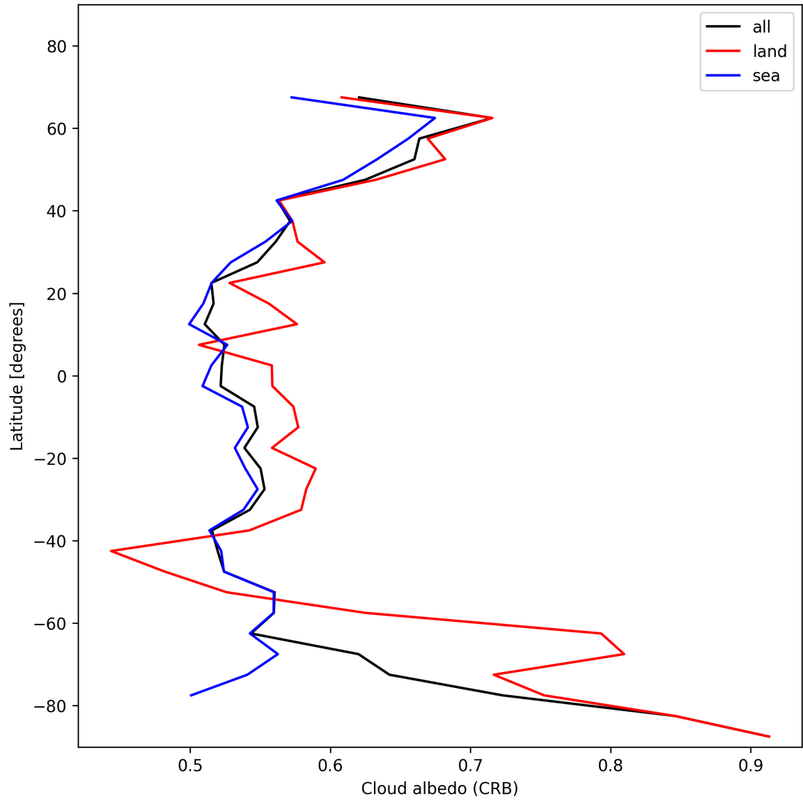
Figure 28: Zonal average of “Cloud albedo (CRB)” for 2025-01-17 to 2025-01-18.
