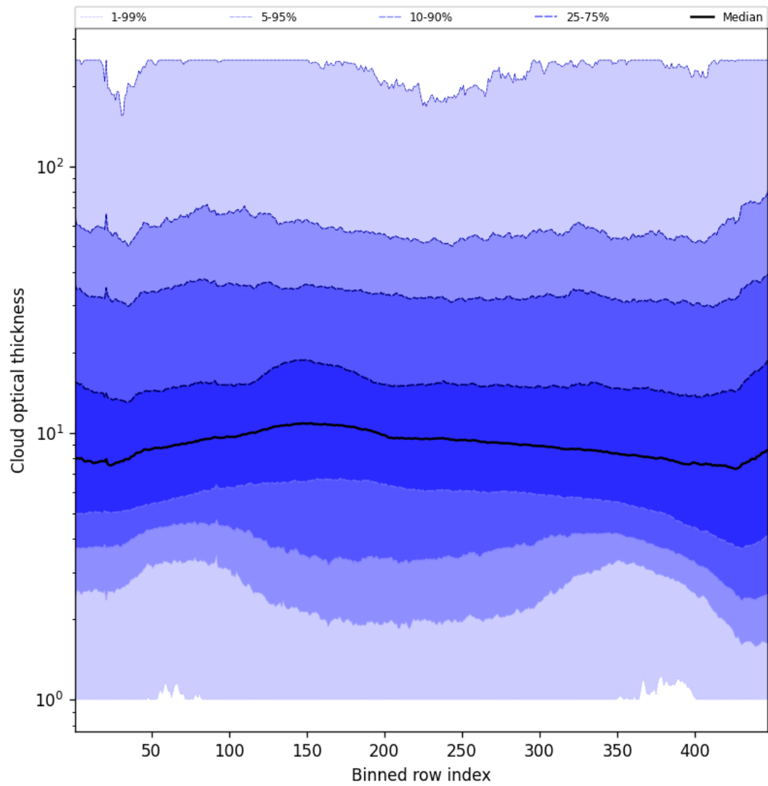
Figure 57: Along track statistics of “Cloud optical thickness” for 2025-01-17 to 2025-01-18
