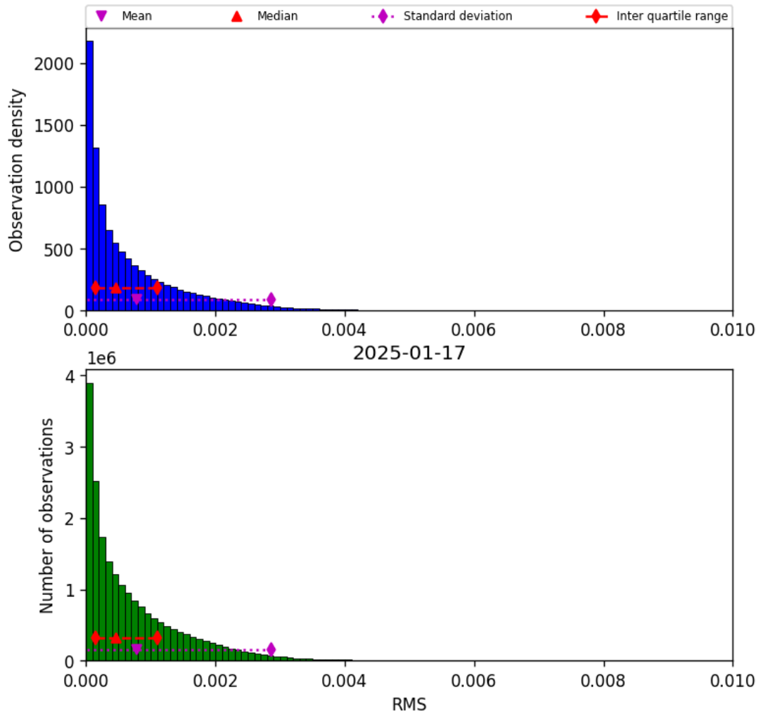
Figure 47: Histogram of “RMS” for 2025-01-17 to 2025-01-18
