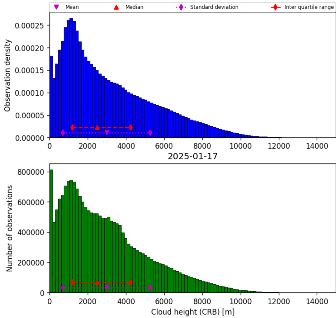
Figure 43: Histogram of “Cloud height (CRB)” for 2025-01-17 to 2025-01-18
