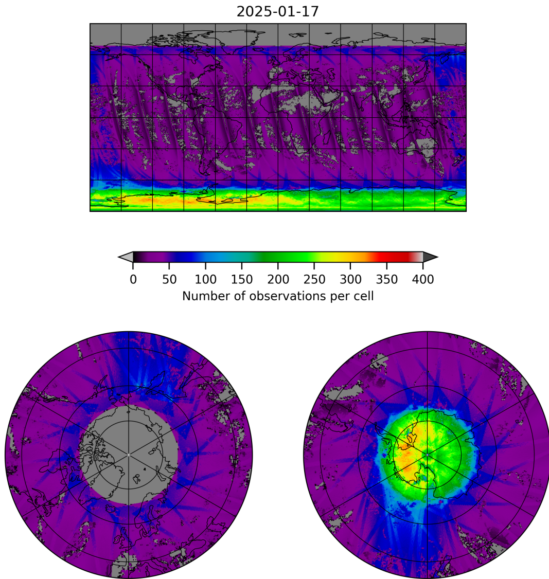
Figure 21: Map of the number of observations for 2025-01-17 to 2025-01-18
