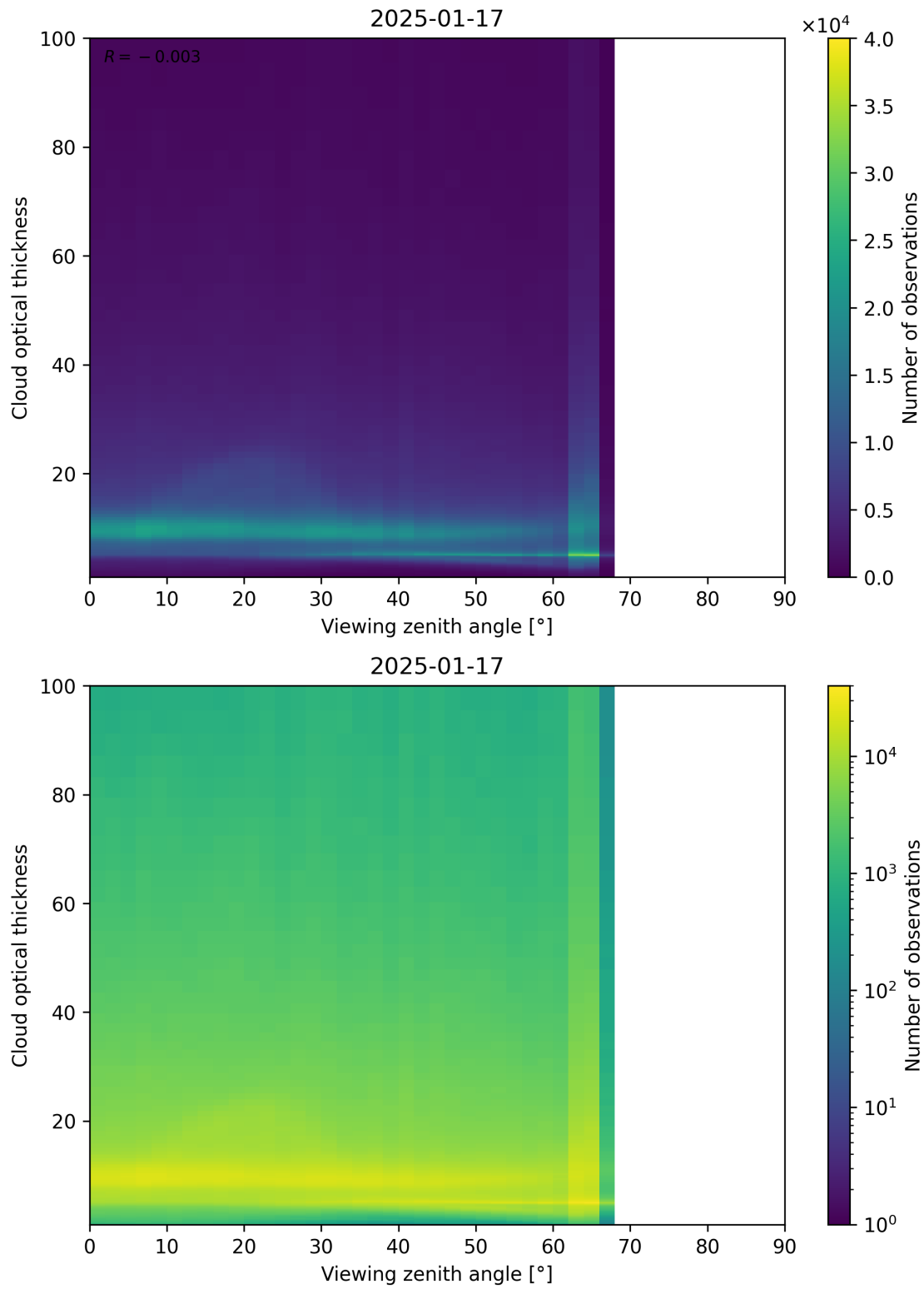
Figure 111: Scatter density plot of “Viewing zenith angle” against “Cloud optical thickness” for 2025-01-17 to 2025-01-18.
