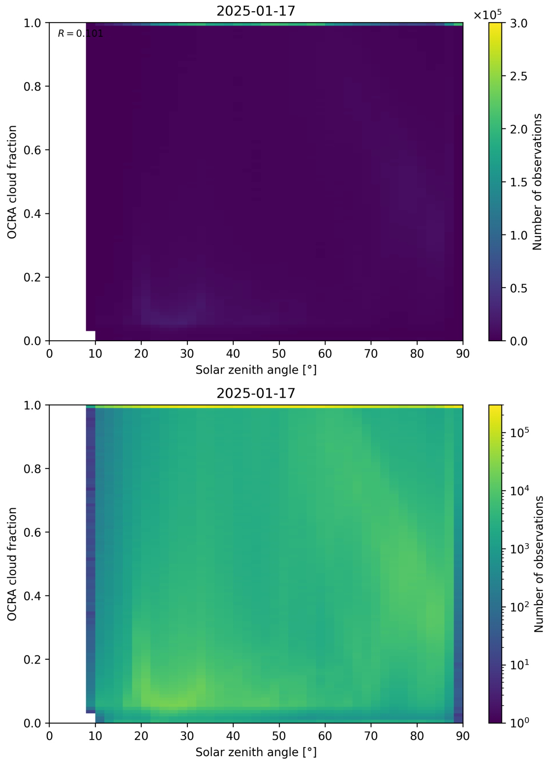
Figure 100: Scatter density plot of “Solar zenith angle” against “OCRA cloud fraction” for 2025-01-17 to 2025-01-18.
