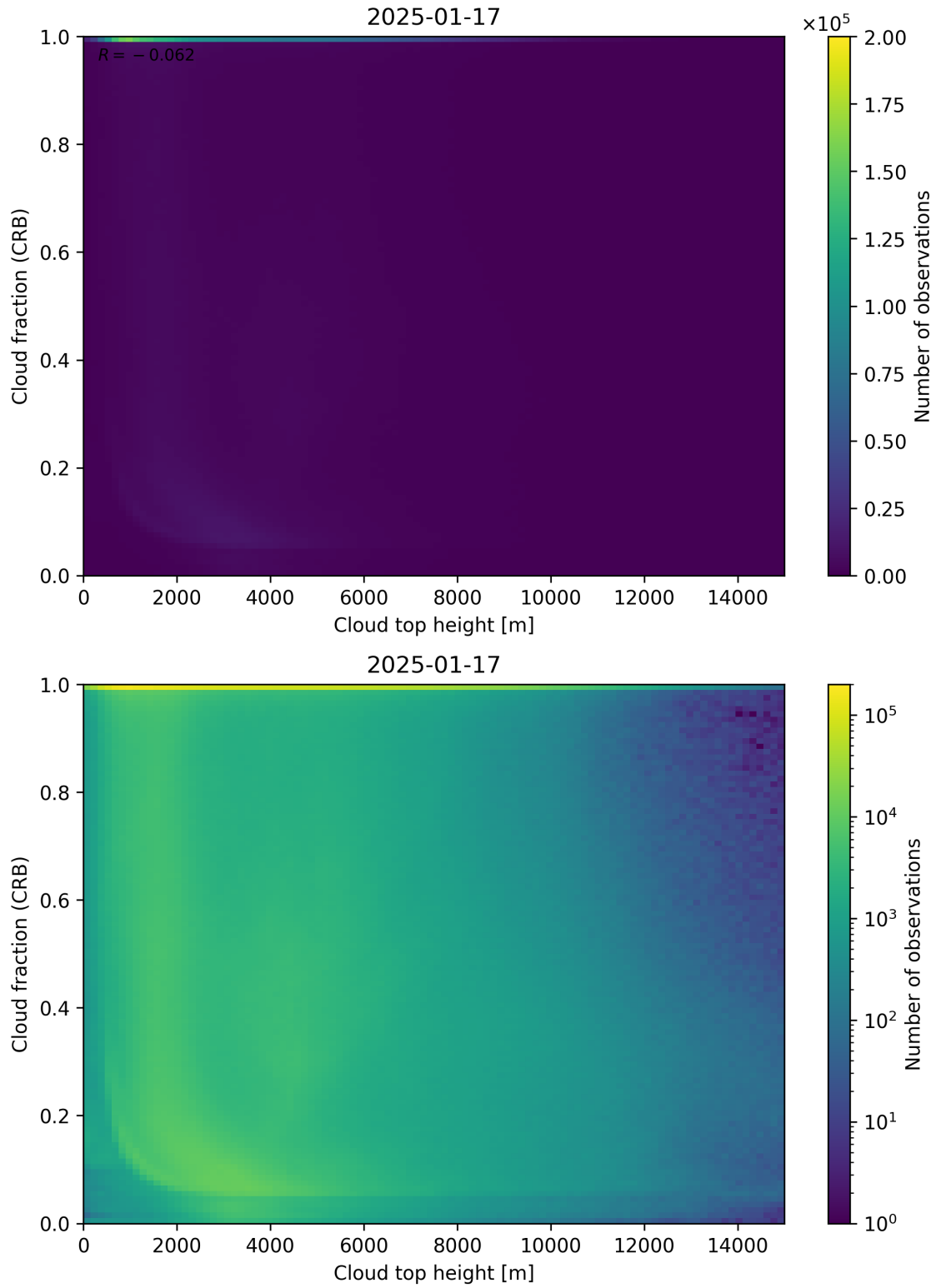
Figure 88: Scatter density plot of “Cloud top height” against “Cloud fraction (CRB)” for 2025-01-17 to 2025-01-18.
