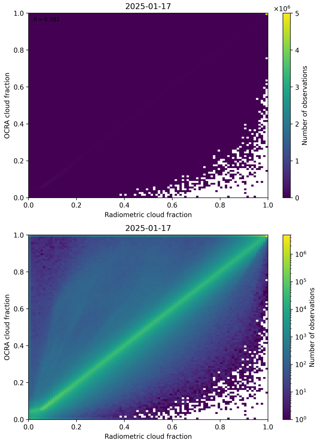
Figure 72: Scatter density plot of “Radiometric cloud fraction” against “OCRA cloud fraction” for 2025-01-17 to 2025-01-18.
