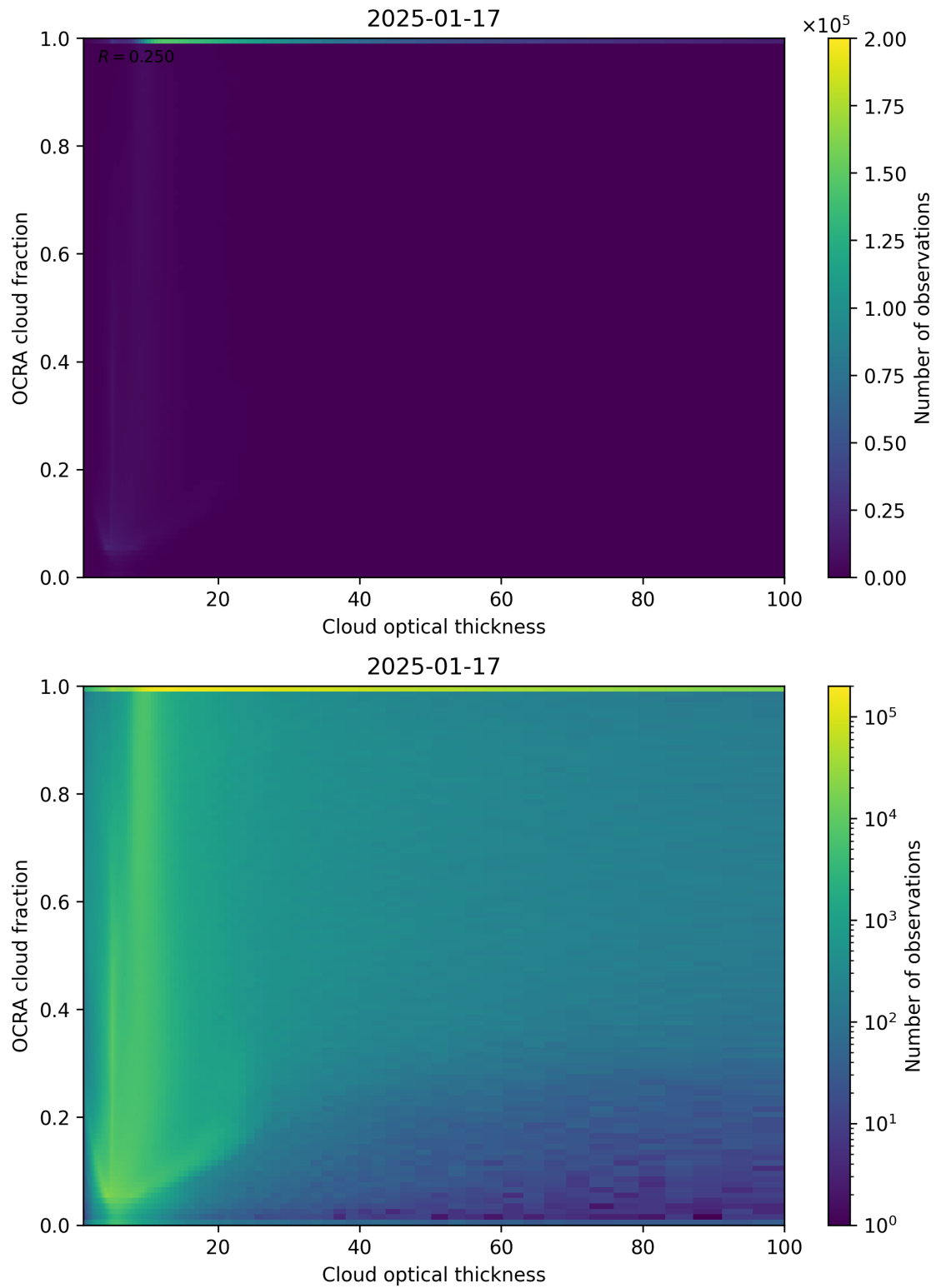
Figure 83: Scatter density plot of “Cloud optical thickness” against “OCRA cloud fraction” for 2025-01-17 to 2025-01-18.
