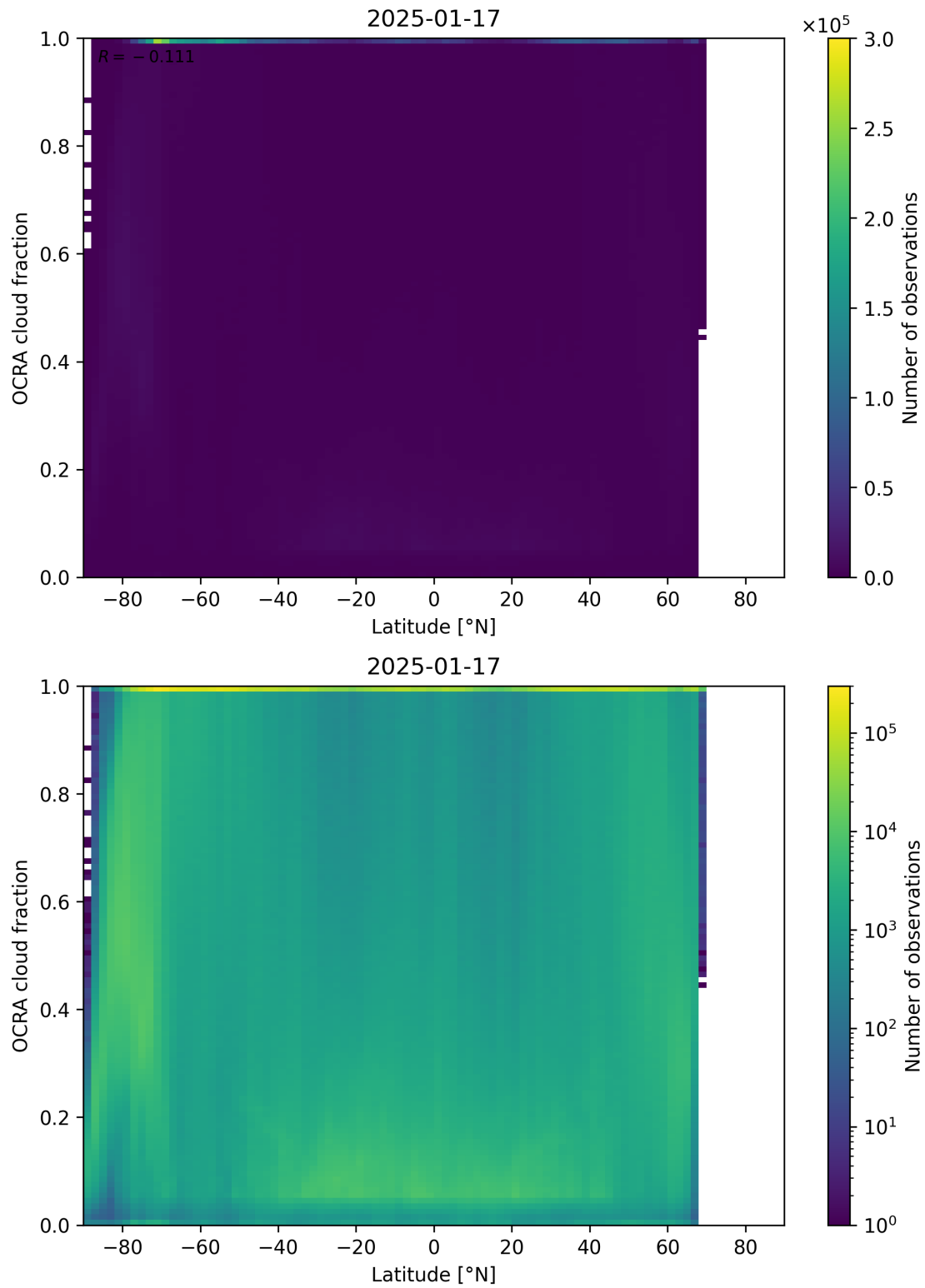
Figure 93: Scatter density plot of “Latitude” against “OCRA cloud fraction” for 2025-01-17 to 2025-01-18.
