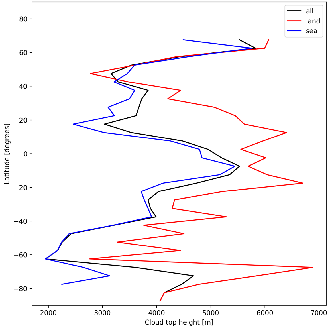
Figure 24: Zonal average of “Cloud top height” for 2025-01-17 to 2025-01-18.
