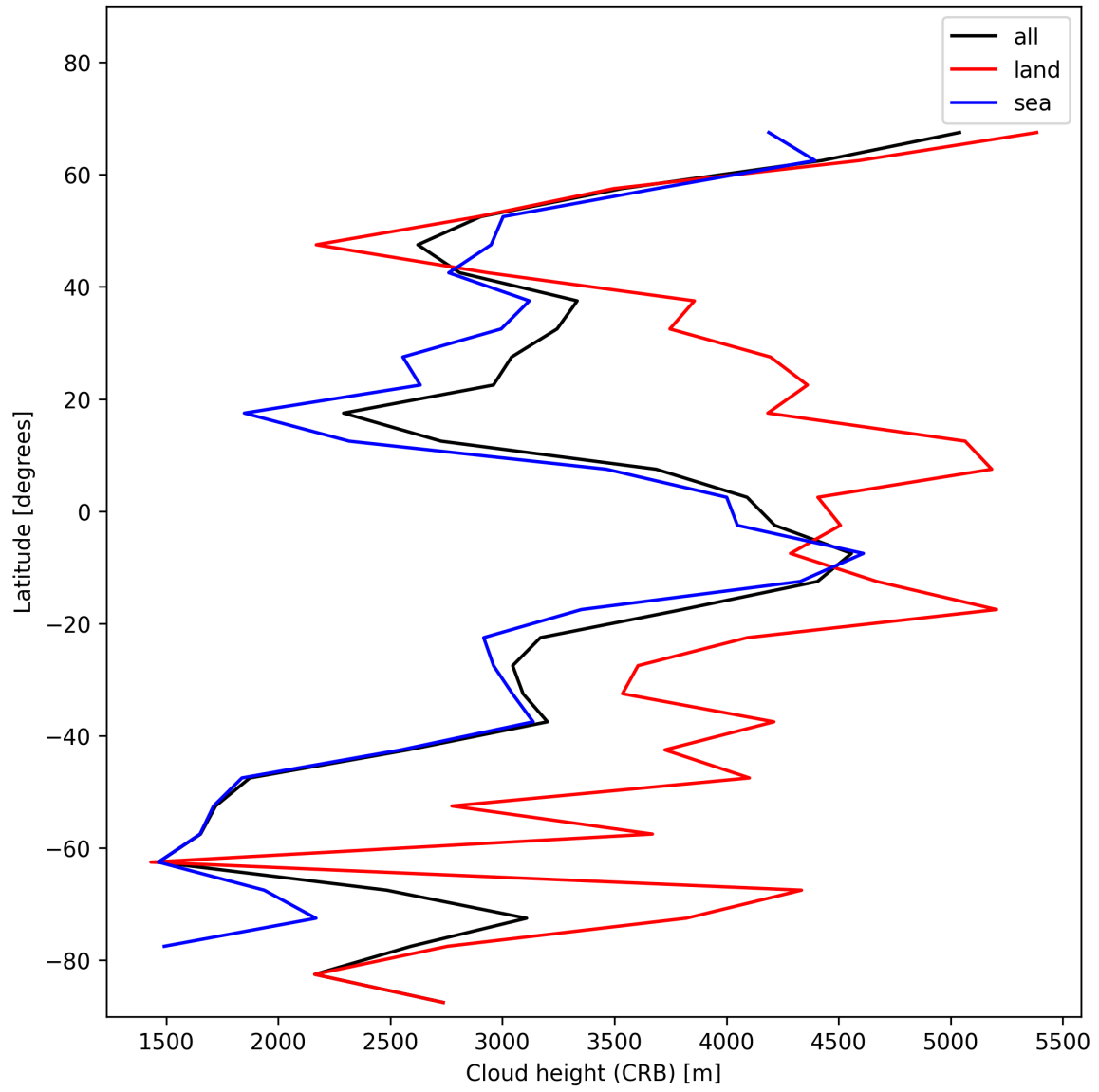
Figure 27: Zonal average of “Cloud height (CRB)” for 2025-01-17 to 2025-01-18.
