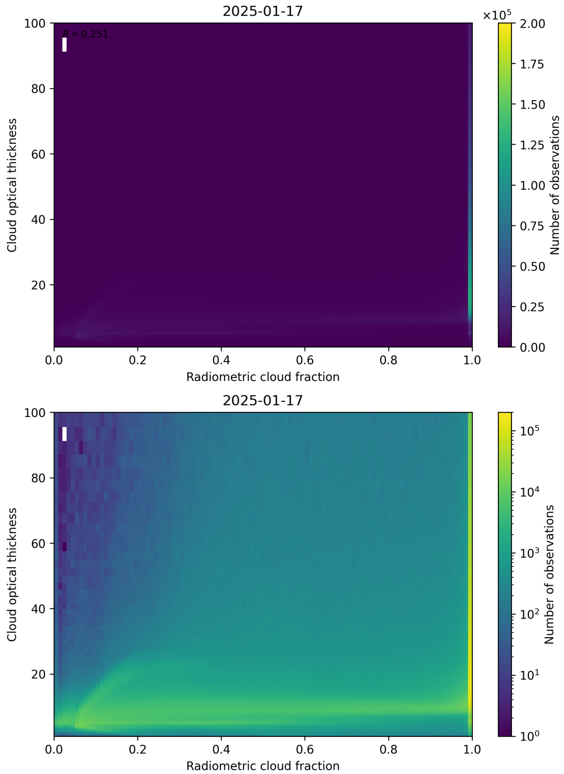
Figure 75: Scatter density plot of “Radiometric cloud fraction” against “Cloud optical thickness” for 2025-01-17 to 2025-01-18.
