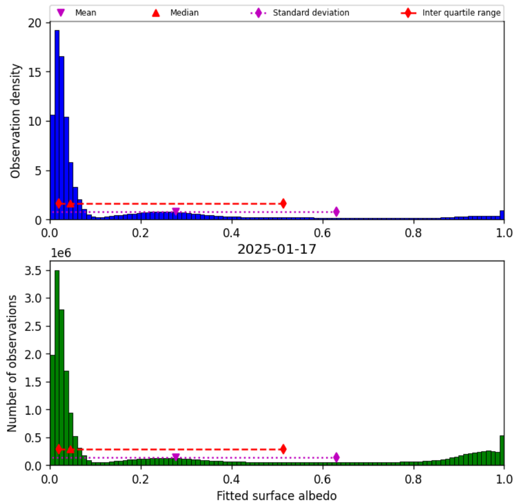
Figure 45: Histogram of “Fitted surface albedo” for 2025-01-17 to 2025-01-18
