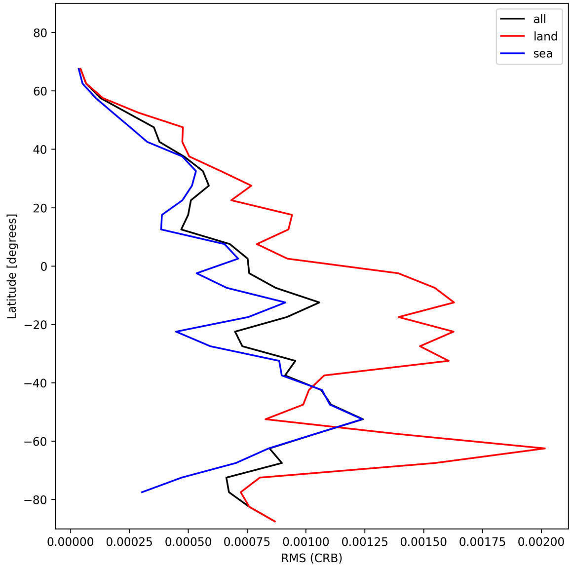
Figure 32: Zonal average of “RMS (CRB)” for 2025-01-17 to 2025-01-18.
