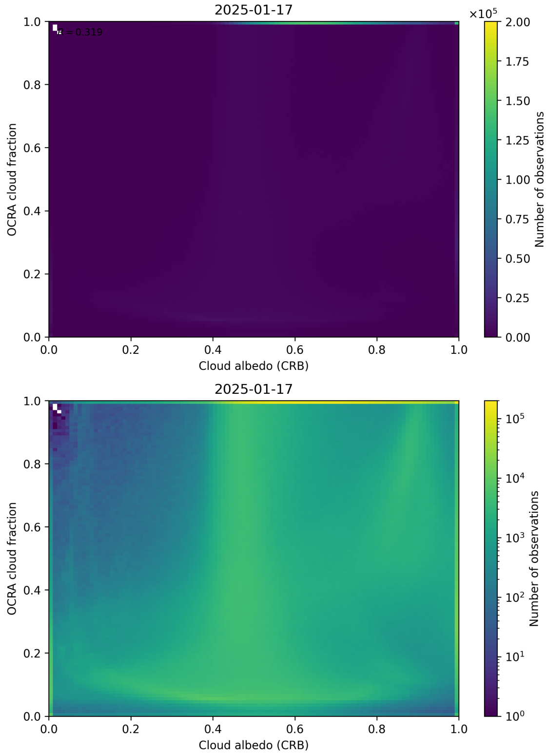
Figure 70: Scatter density plot of “Cloud albedo (CRB)” against “OCRA cloud fraction” for 2025-01-17 to 2025-01-18.
