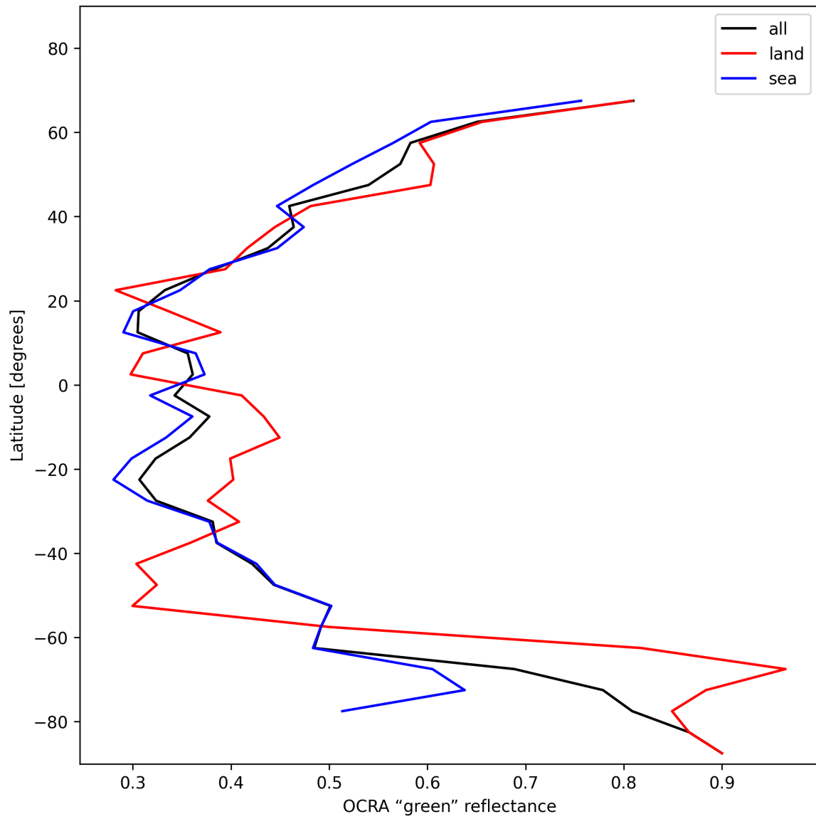
Figure 36: Zonal average of “OCRA “green” reflectance” for 2025-01-17 to 2025-01-18.
