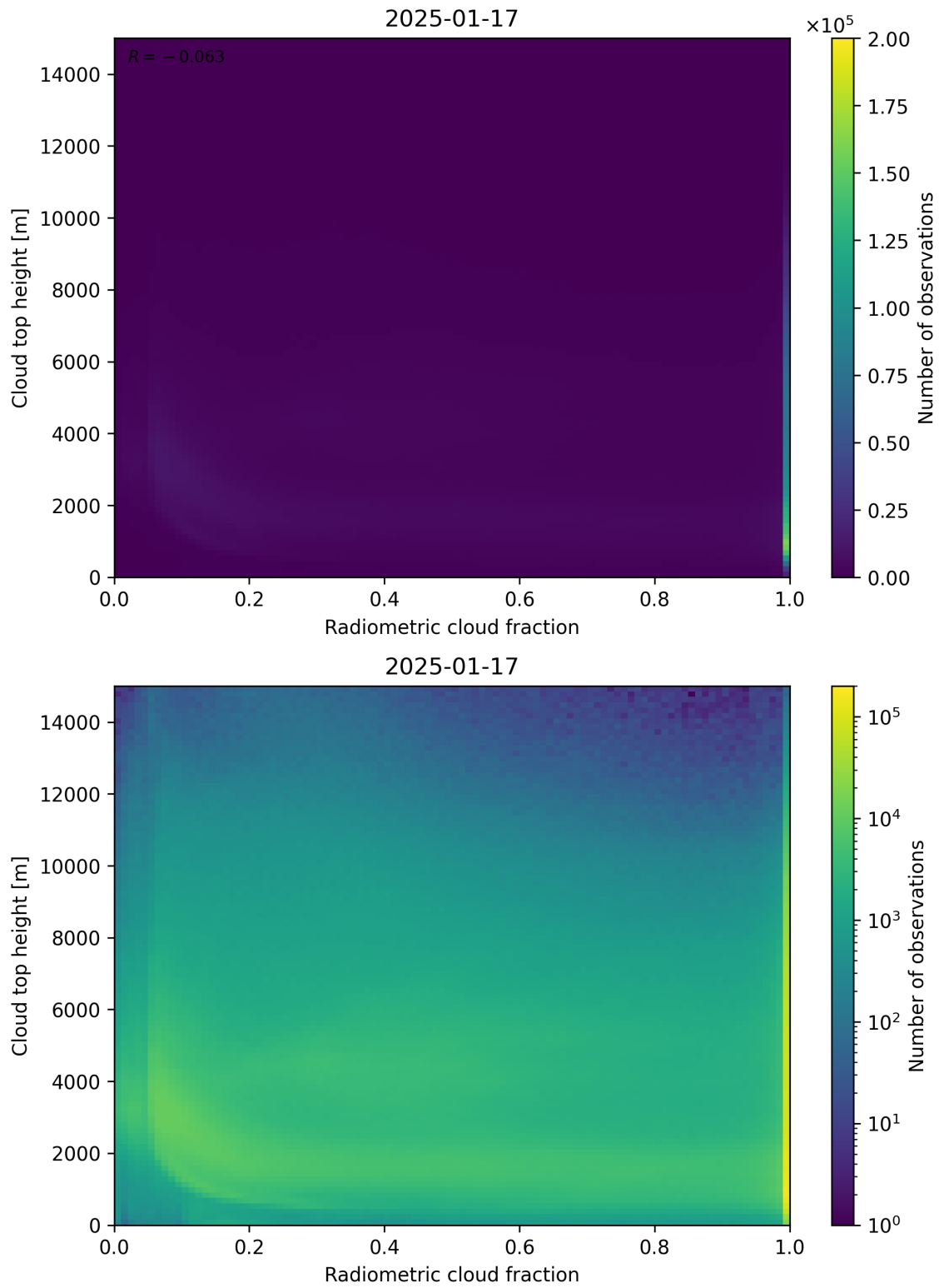
Figure 76: Scatter density plot of “Radiometric cloud fraction” against “Cloud top height” for 2025-01-17 to 2025-01-18.
