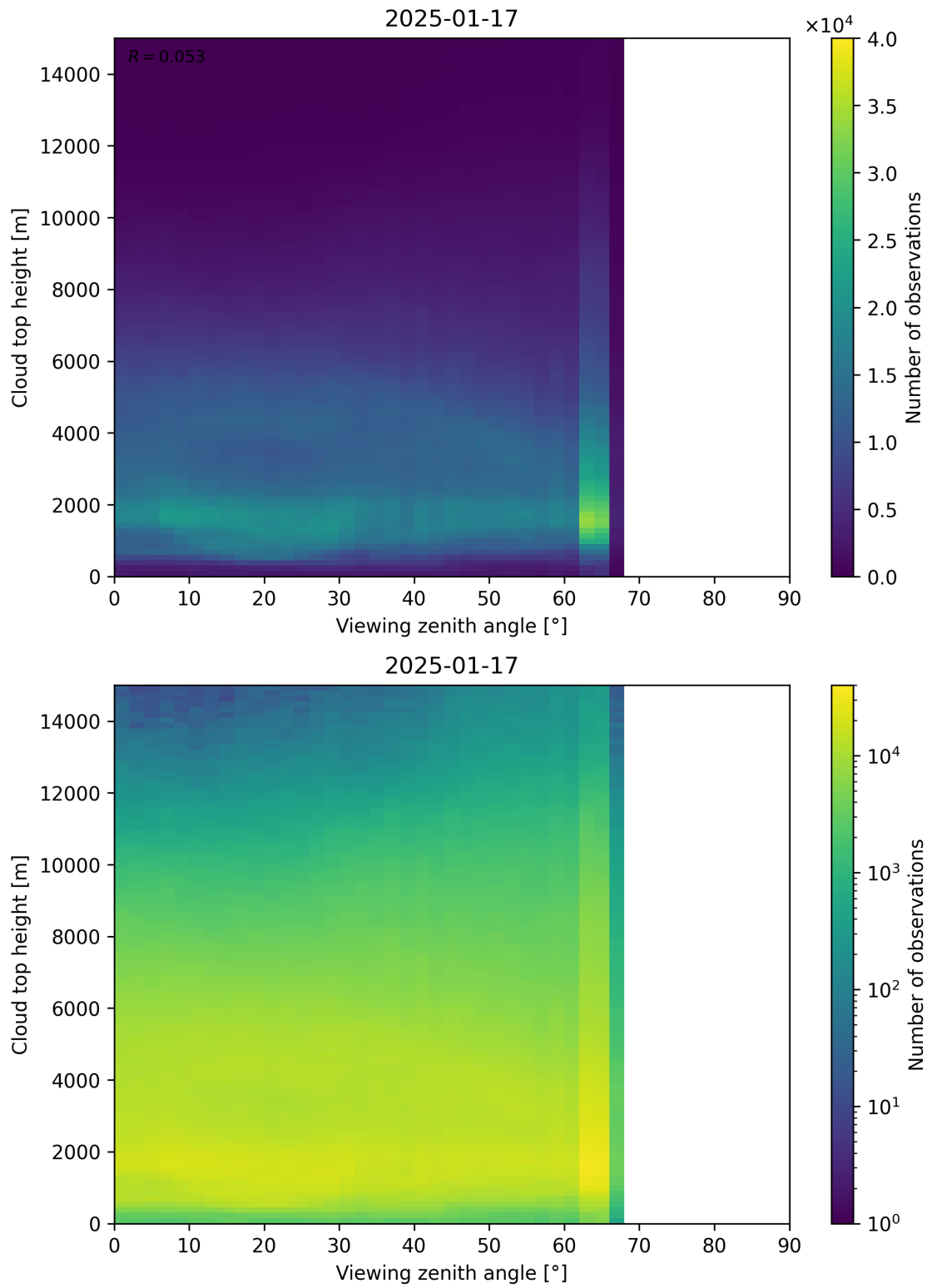
Figure 112: Scatter density plot of “Viewing zenith angle” against “Cloud top height” for 2025-01-17 to 2025-01-18.
