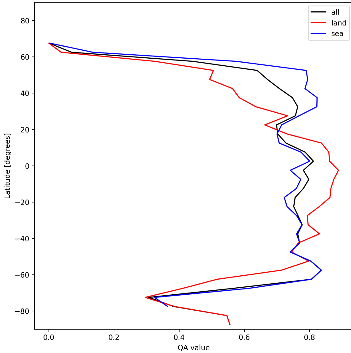
Figure 22: Zonal average of “QA value” for 2025-01-17 to 2025-01-18.
