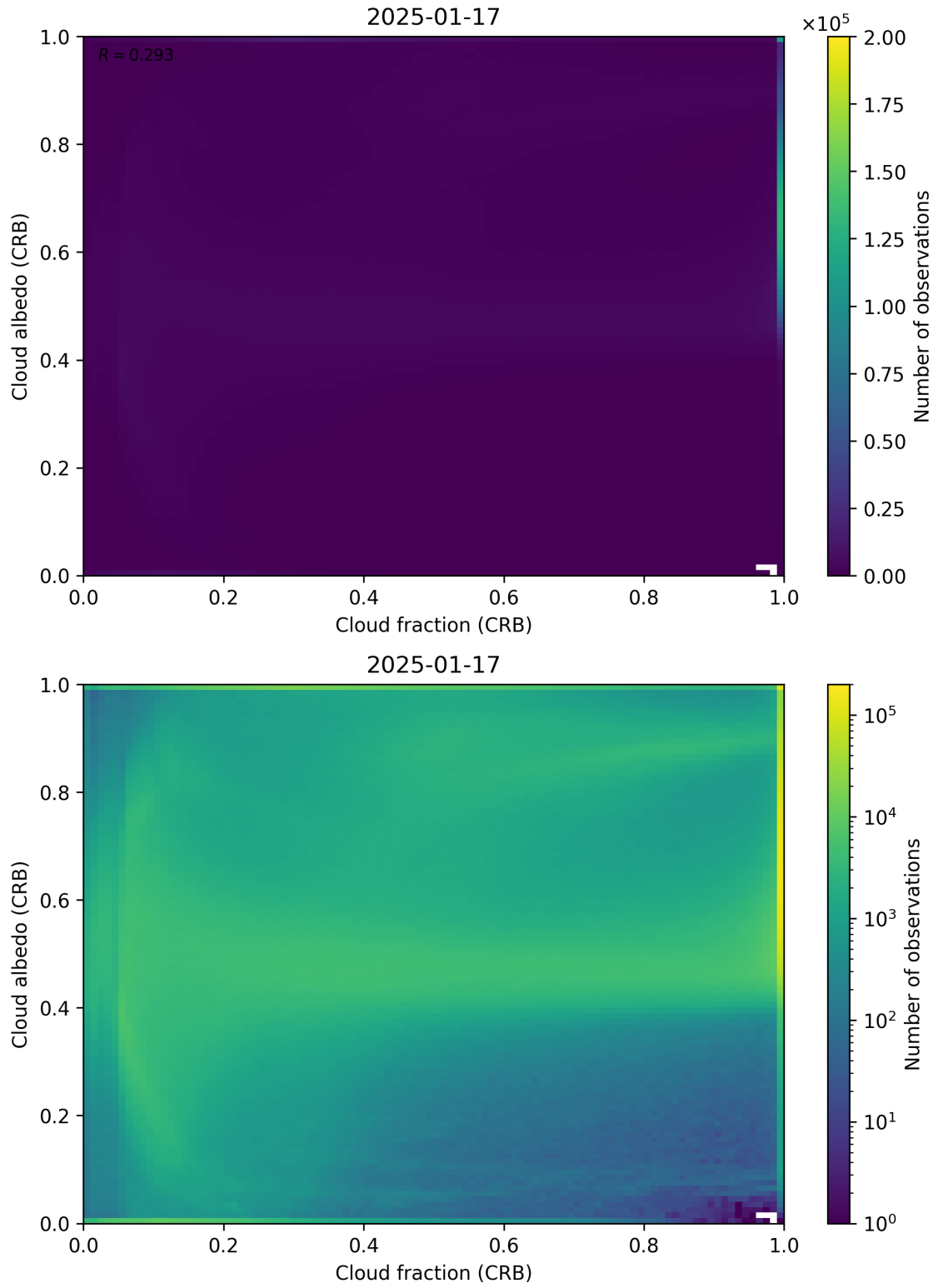
Figure 77: Scatter density plot of “Cloud fraction (CRB)” against “Cloud albedo (CRB)” for 2025-01-17 to 2025-01-18.
