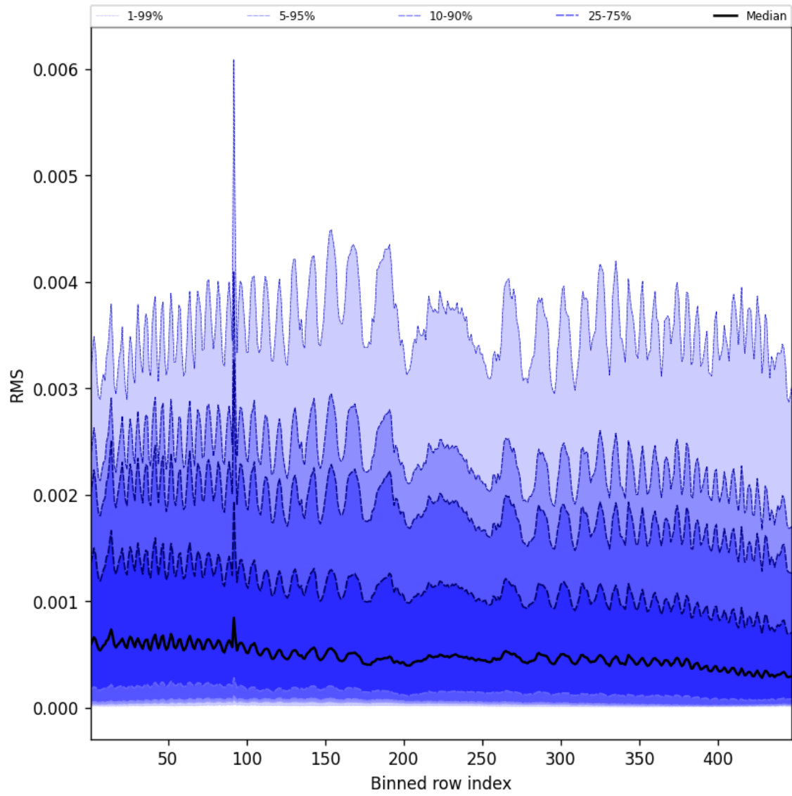
Figure 63: Along track statistics of “RMS” for 2025-01-17 to 2025-01-18
