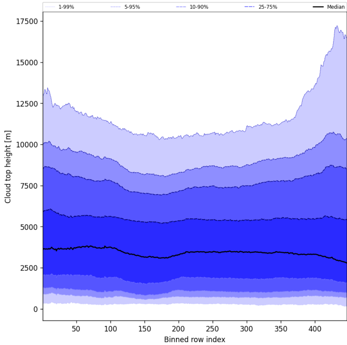
Figure 56: Along track statistics of “Cloud top height” for 2025-01-17 to 2025-01-18
