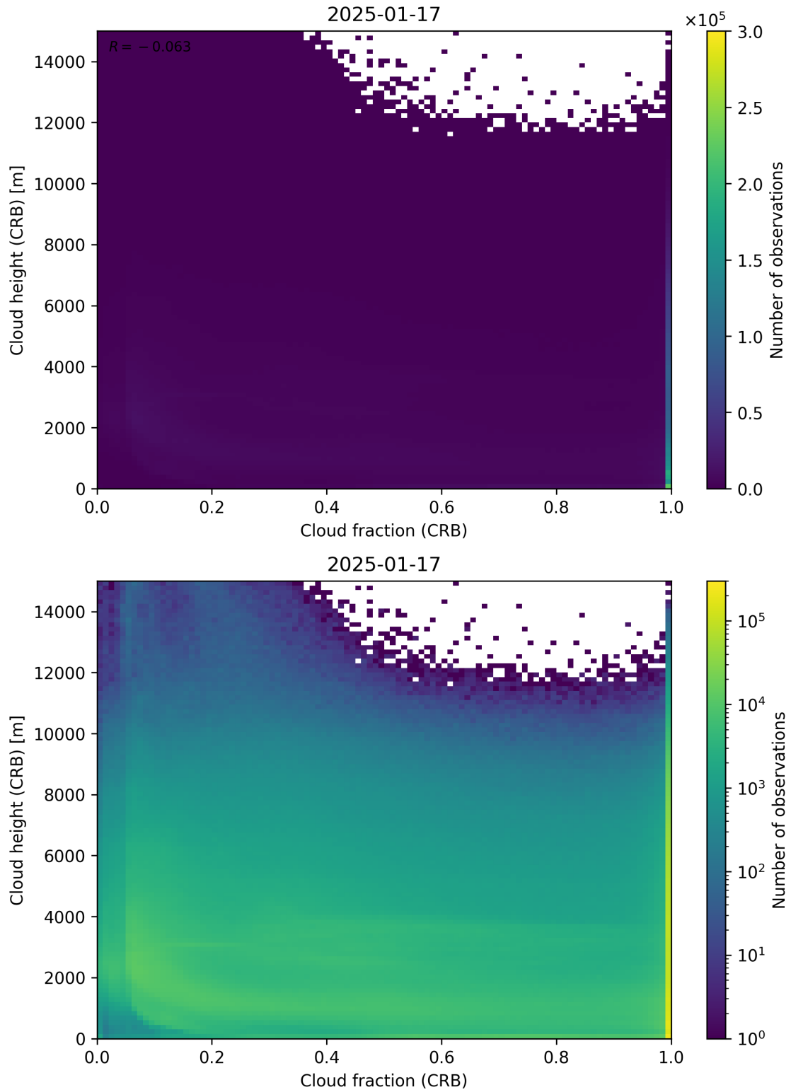
Figure 79: Scatter density plot of “Cloud fraction (CRB)” against “Cloud height (CRB)” for 2025-01-17 to 2025-01-18.
