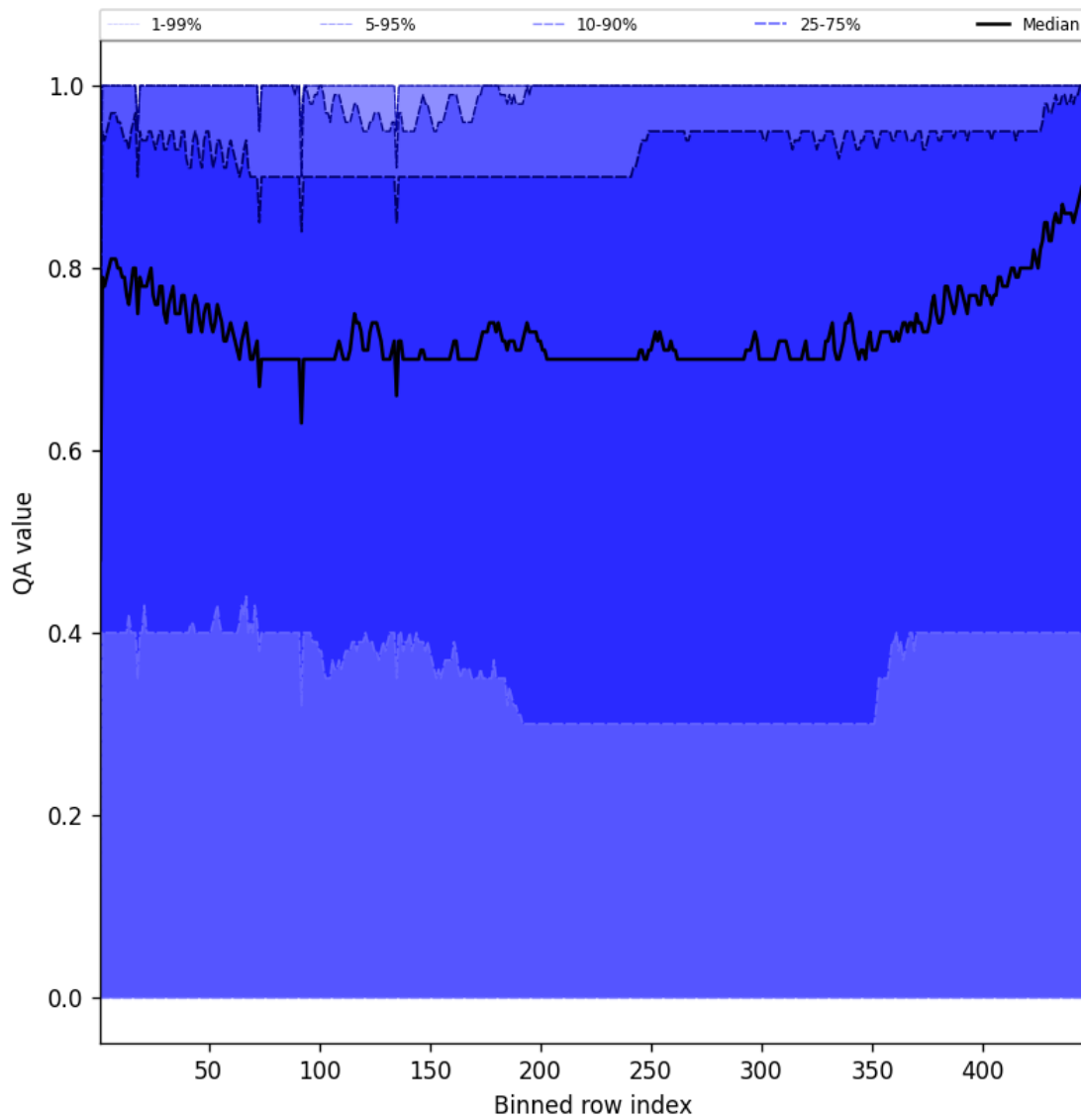
Figure 54: Along track statistics of “QA value” for 2025-01-17 to 2025-01-18
