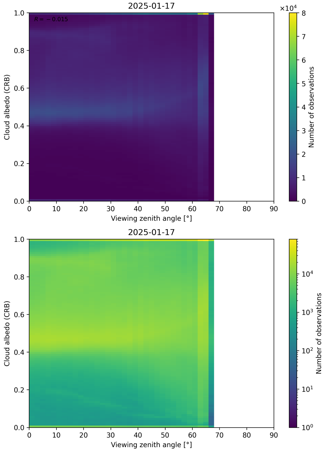
Figure 106: Scatter density plot of “Viewing zenith angle” against “Cloud albedo (CRB)” for 2025-01-17 to 2025-01-18.
