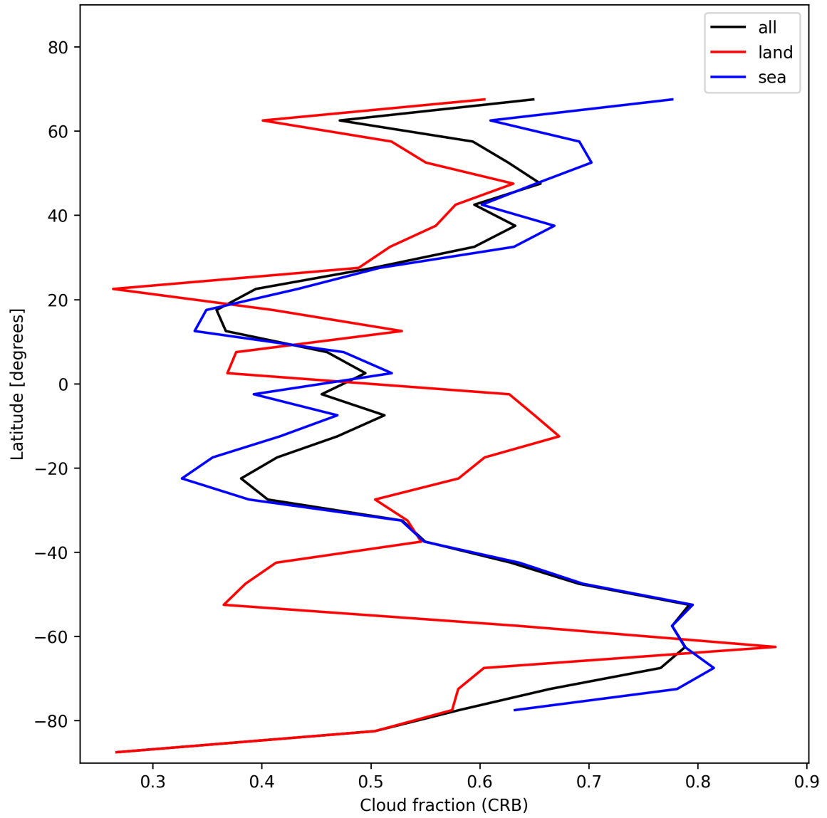
Figure 26: Zonal average of “Cloud fraction (CRB)” for 2025-01-17 to 2025-01-18.
