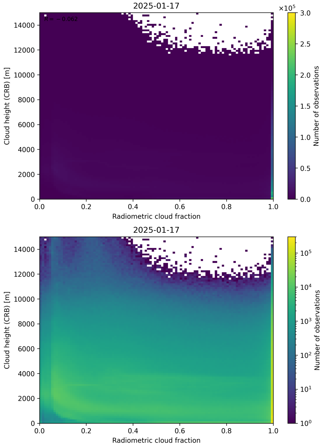
Figure 74: Scatter density plot of “Radiometric cloud fraction” against “Cloud height (CRB)” for 2025-01-17 to 2025-01-18.
