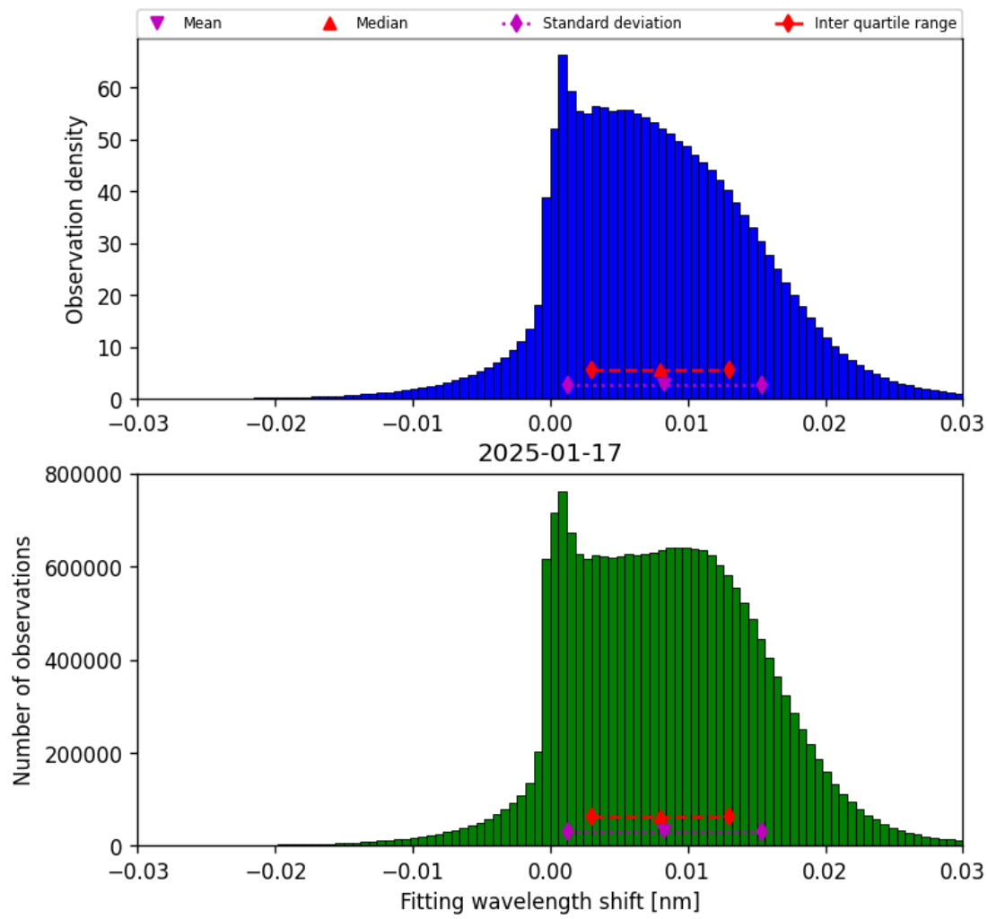
Figure 49: Histogram of “Fitting wavelength shift” for 2025-01-17 to 2025-01-18
