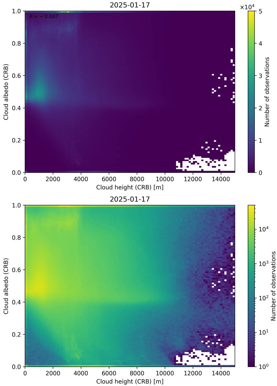
Figure 80: Scatter density plot of “Cloud height (CRB)” against “Cloud albedo (CRB)” for 2025-01-17 to 2025-01-18.
