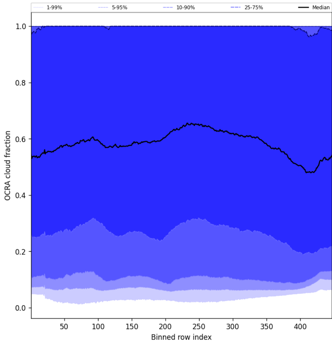
Figure 66: Along track statistics of “OCRA cloud fraction” for 2025-01-17 to 2025-01-18
