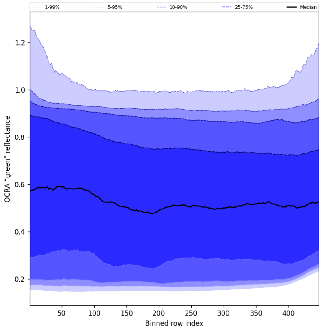
Figure 68: Along track statistics of "OCRA "green" reflectance" for 2025-01-17 to 2025-01-18
