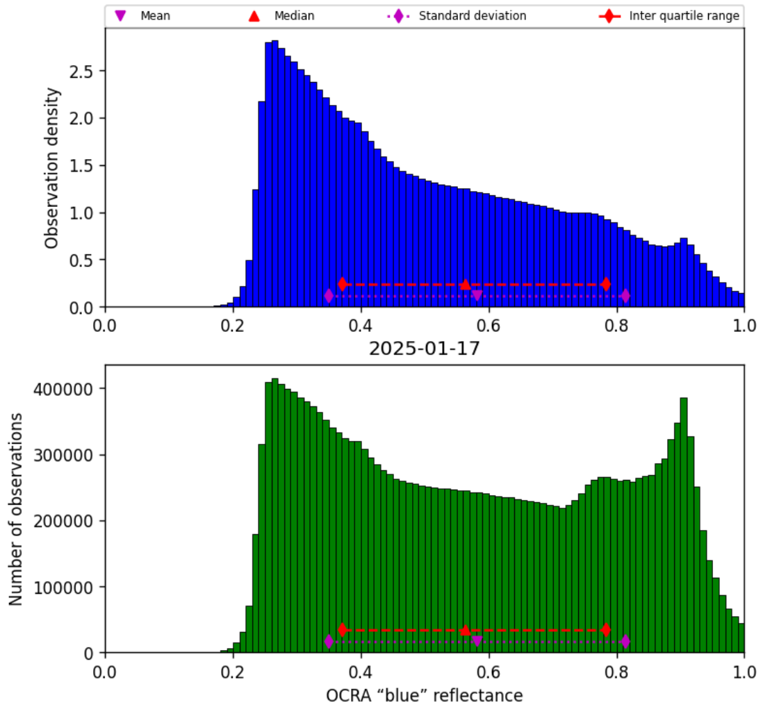
Figure 51: Histogram of “OCRA “blue” reflectance” for 2025-01-17 to 2025-01-18
