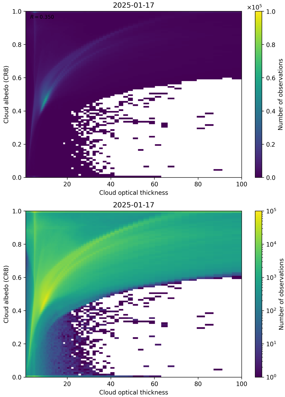
Figure 82: Scatter density plot of “Cloud optical thickness” against “Cloud albedo (CRB)” for 2025-01-17 to 2025-01-18.
