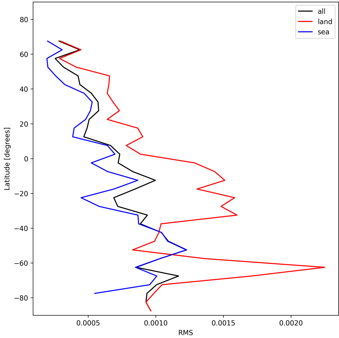
Figure 31: Zonal average of “RMS” for 2025-01-17 to 2025-01-18.
