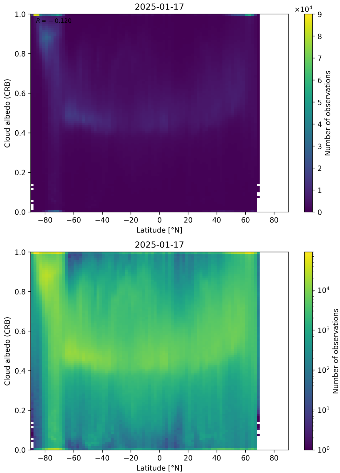
Figure 91: Scatter density plot of “Latitude” against “Cloud albedo (CRB)” for 2025-01-17 to 2025-01-18.
