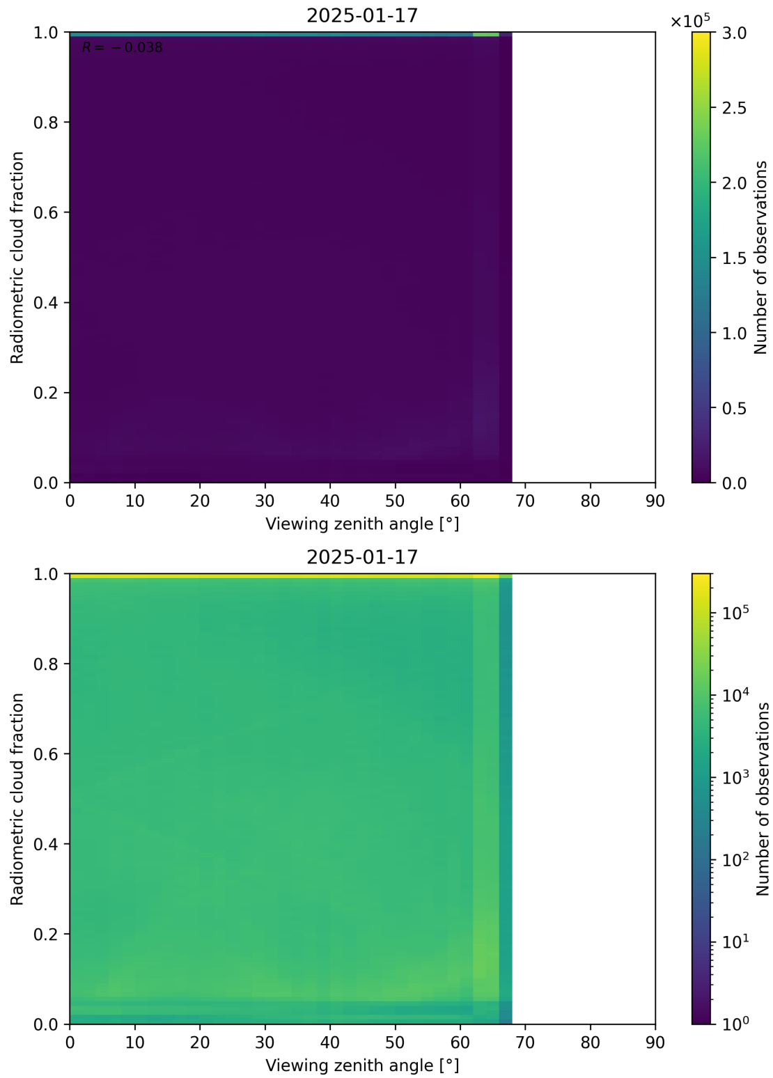
Figure 107: Scatter density plot of “Viewing zenith angle” against “Radiometric cloud fraction” for 2025-01-17 to 2025-01-18.
