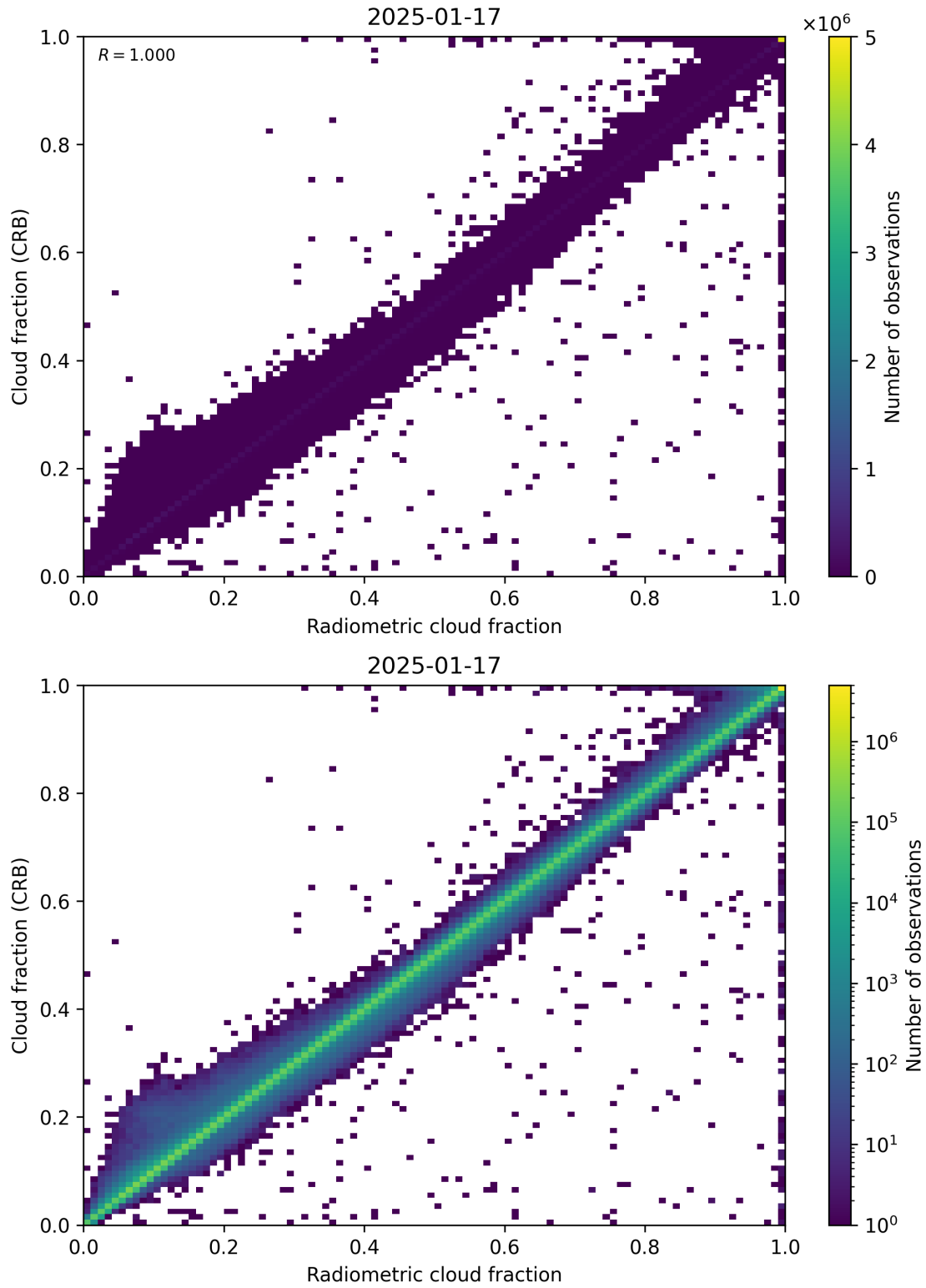
Figure 73: Scatter density plot of “Radiometric cloud fraction” against “Cloud fraction (CRB)” for 2025-01-17 to 2025-01-18.
