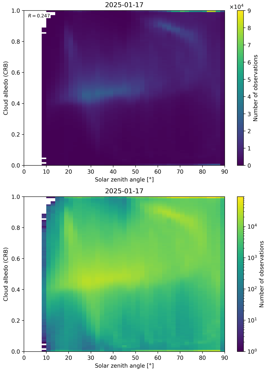
Figure 98: Scatter density plot of “Solar zenith angle” against “Cloud albedo (CRB)” for 2025-01-17 to 2025-01-18.
