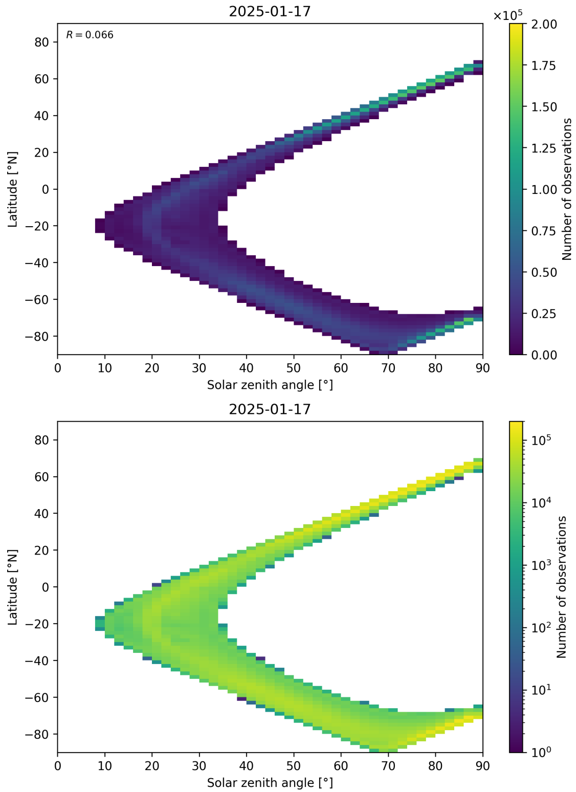
Figure 105: Scatter density plot of “Solar zenith angle” against “Latitude” for 2025-01-17 to 2025-01-18.
