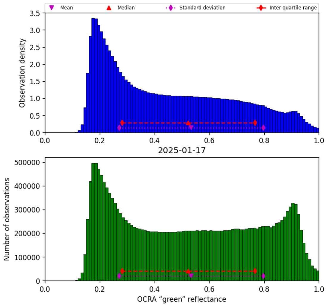
Figure 52: Histogram of “OCRA “green” reflectance” for 2025-01-17 to 2025-01-18
