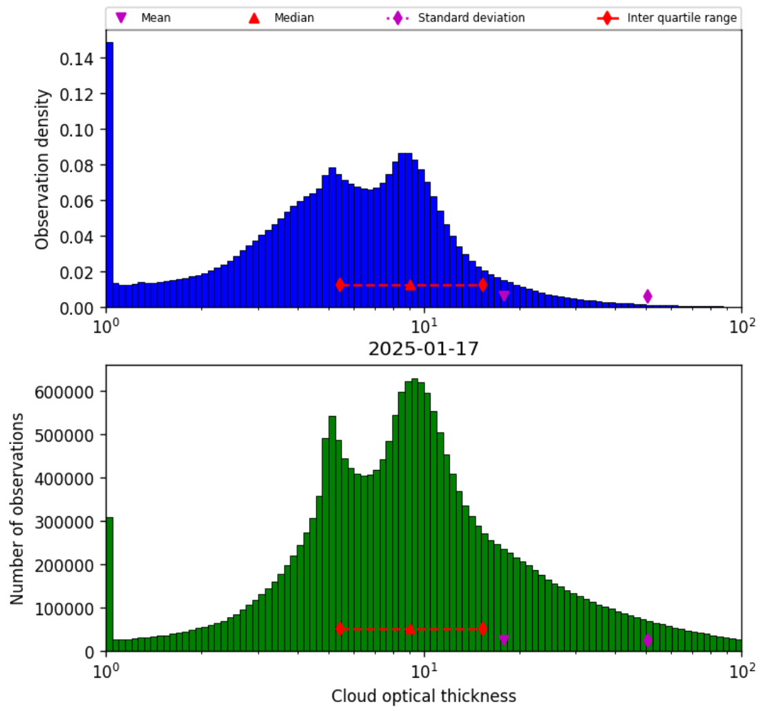
Figure 41: Histogram of “Cloud optical thickness” for 2025-01-17 to 2025-01-18
