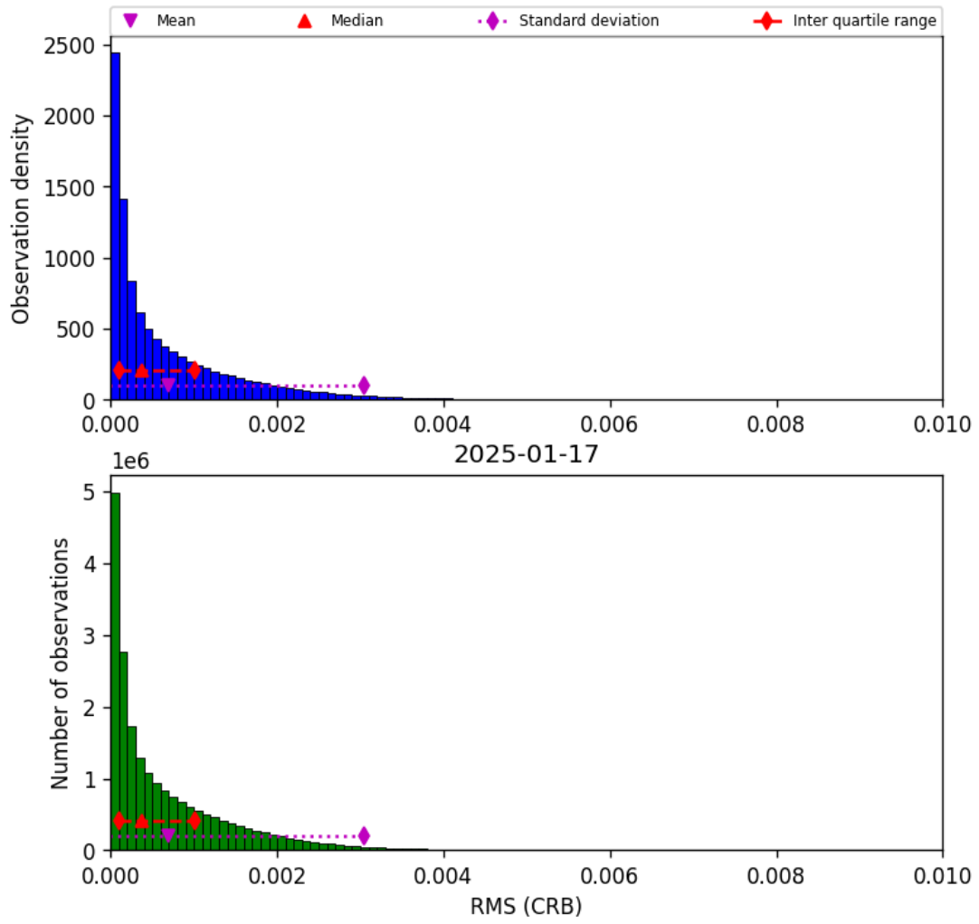
Figure 48: Histogram of “RMS (CRB)” for 2025-01-17 to 2025-01-18
