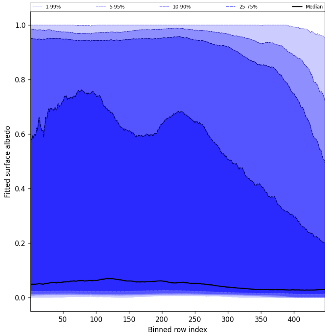
Figure 61: Along track statistics of “Fitted surface albedo” for 2025-01-17 to 2025-01-18
