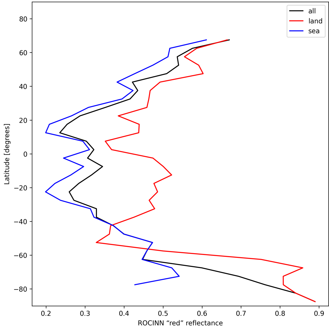
Figure 37: Zonal average of “ROCINN “red” reflectance” for 2025-01-17 to 2025-01-18.
