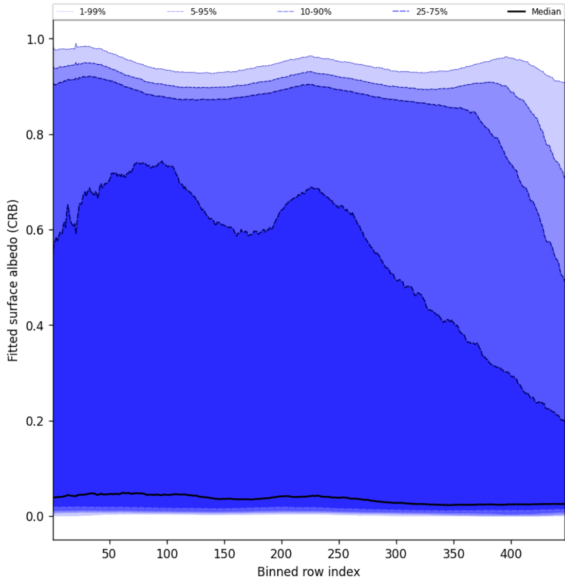
Figure 62: Along track statistics of “Fitted surface albedo (CRB)” for 2025-01-17 to 2025-01-18
