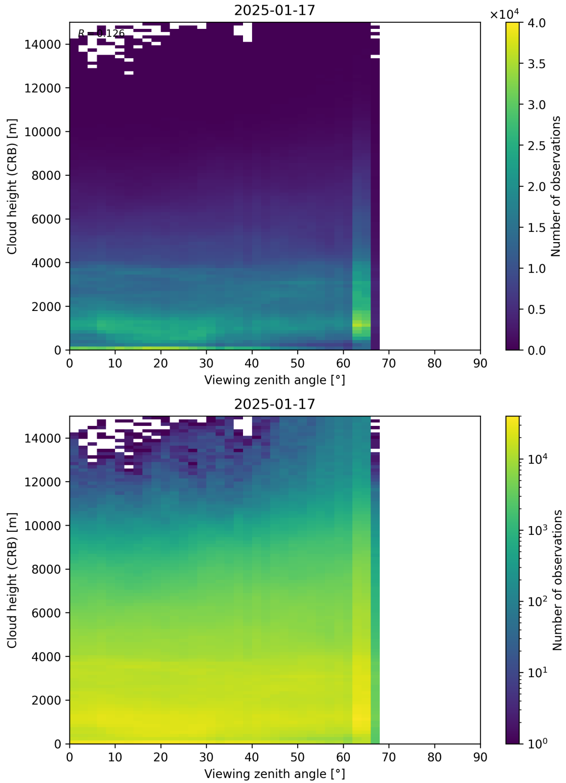
Figure 110: Scatter density plot of “Viewing zenith angle” against “Cloud height (CRB)” for 2025-01-17 to 2025-01-18.
