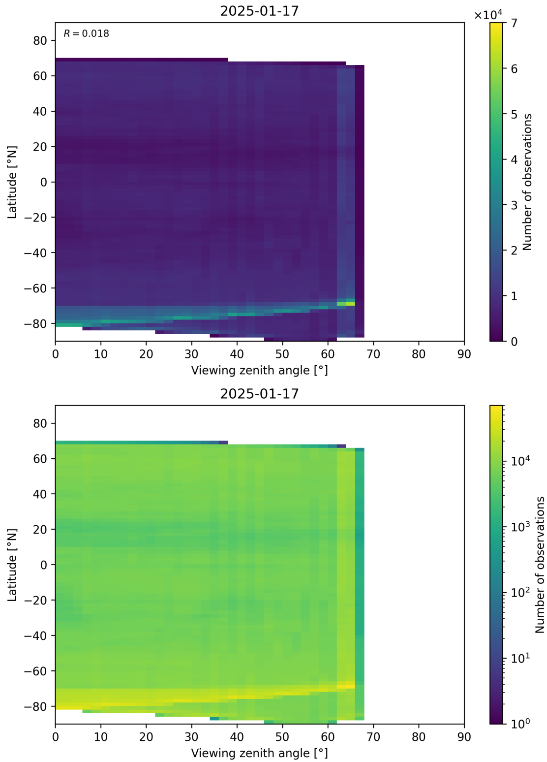
Figure 113: Scatter density plot of “Viewing zenith angle” against “Latitude” for 2025-01-17 to 2025-01-18.
