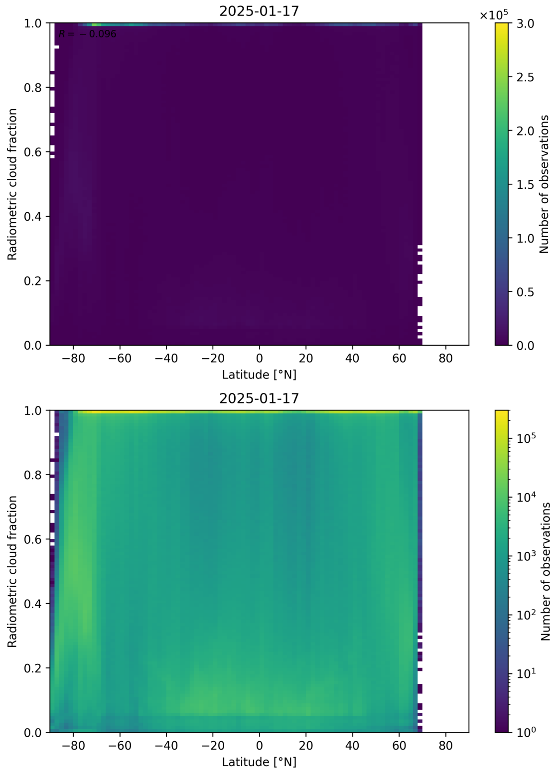
Figure 92: Scatter density plot of “Latitude” against “Radiometric cloud fraction” for 2025-01-17 to 2025-01-18.
