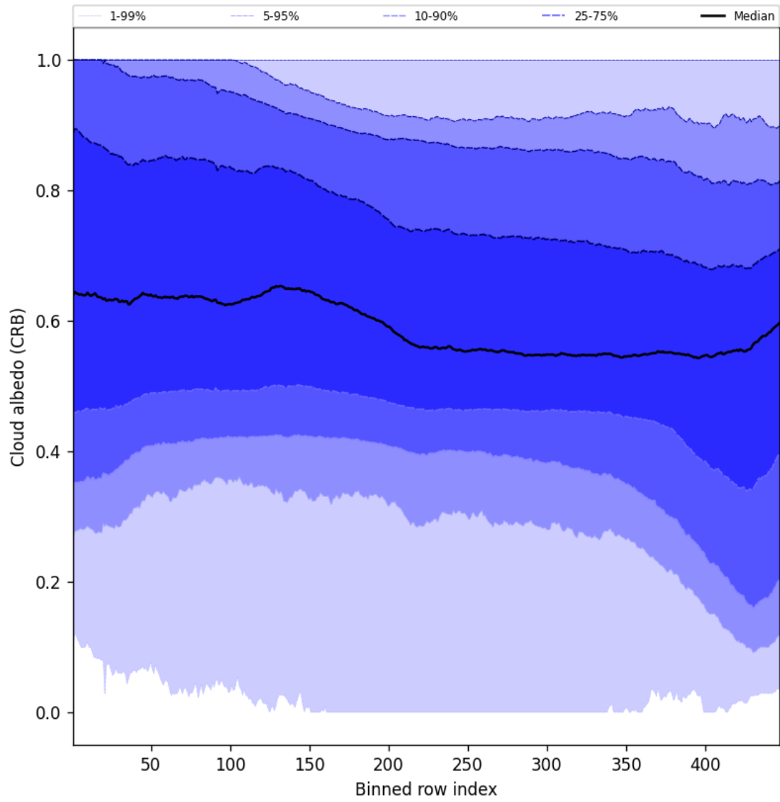
Figure 60: Along track statistics of “Cloud albedo (CRB)” for 2025-01-17 to 2025-01-18
