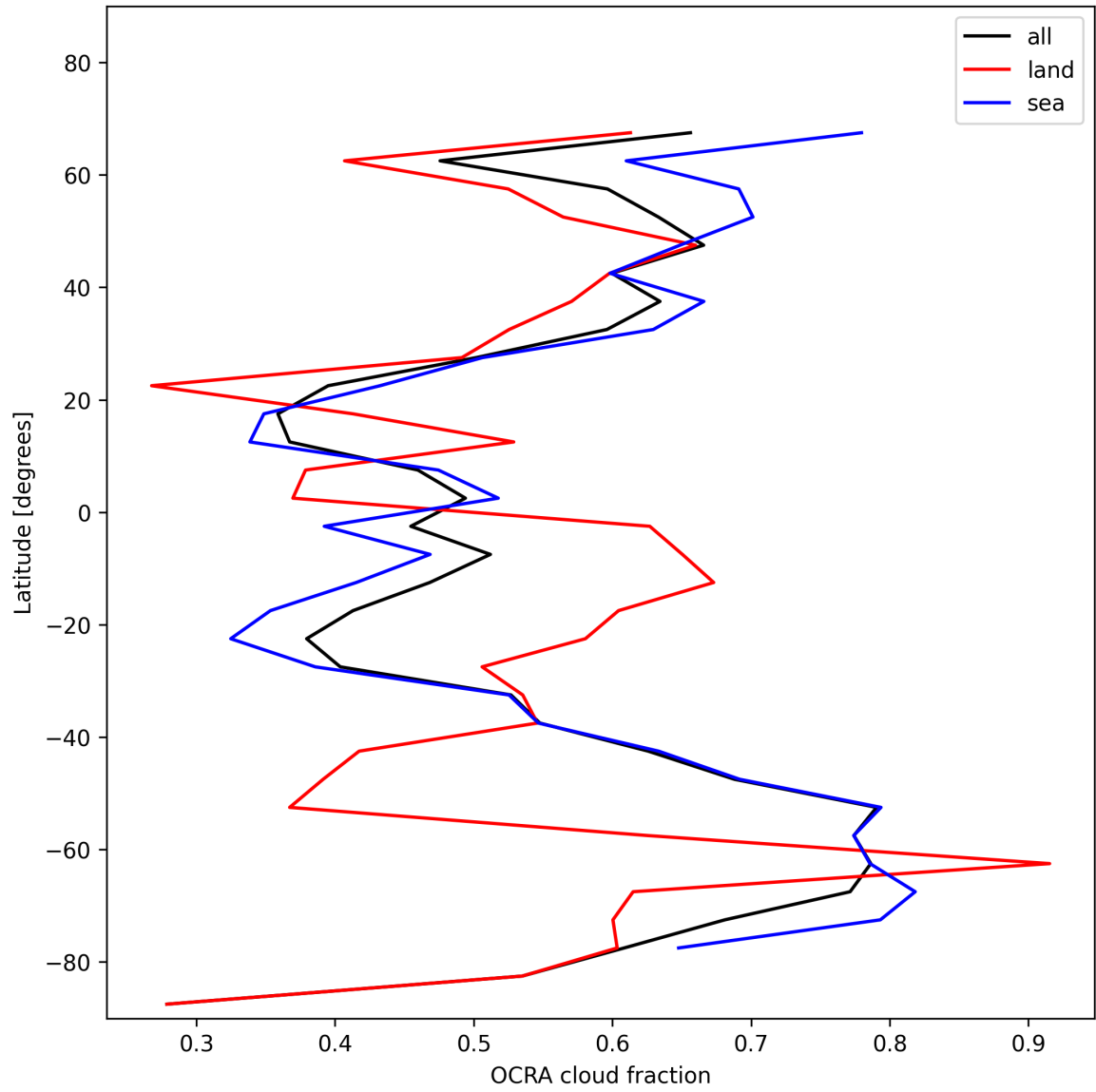
Figure 34: Zonal average of “OCRA cloud fraction” for 2025-01-17 to 2025-01-18.
