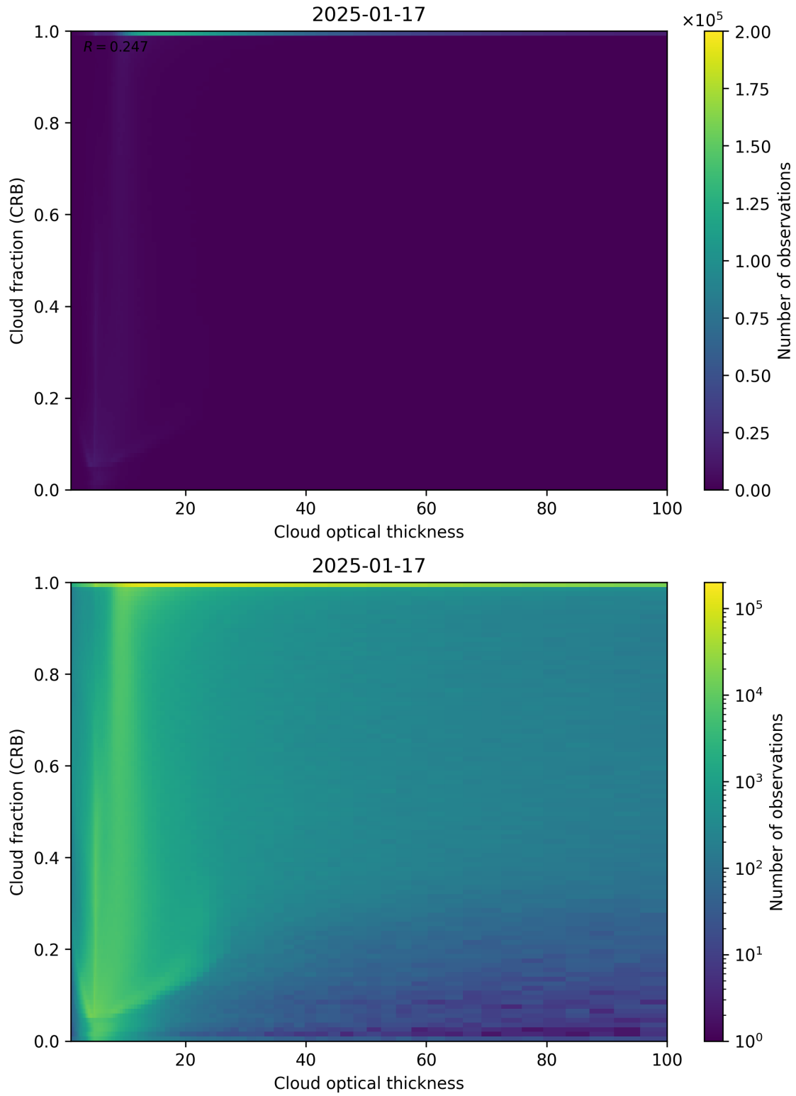
Figure 84: Scatter density plot of “Cloud optical thickness” against “Cloud fraction (CRB)” for 2025-01-17 to 2025-01-18.
