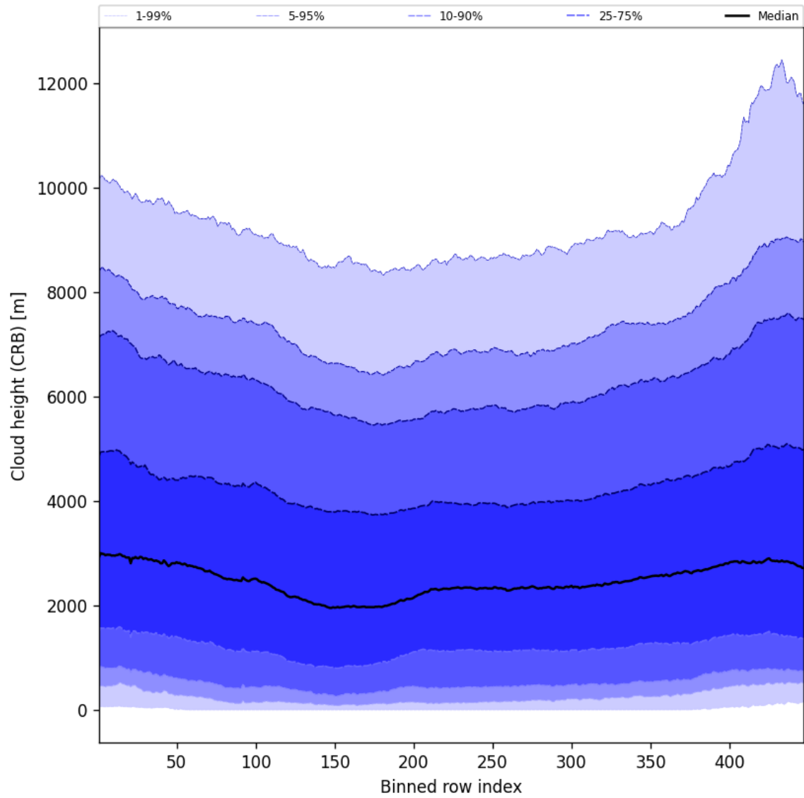
Figure 59: Along track statistics of “Cloud height (CRB)” for 2025-01-17 to 2025-01-18
