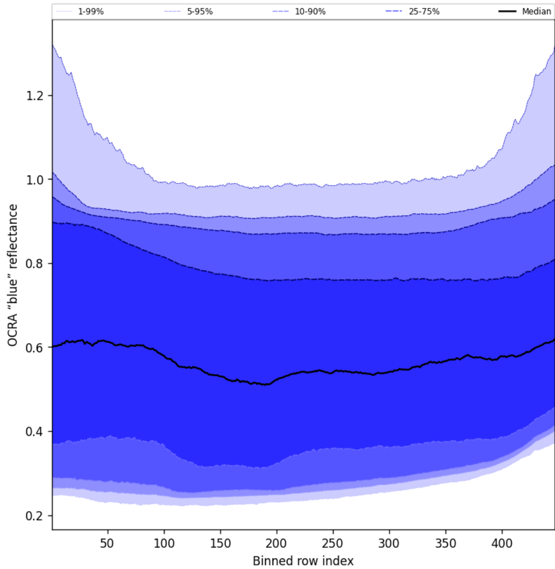
Figure 67: Along track statistics of “OCRA “blue” reflectance” for 2025-01-17 to 2025-01-18
