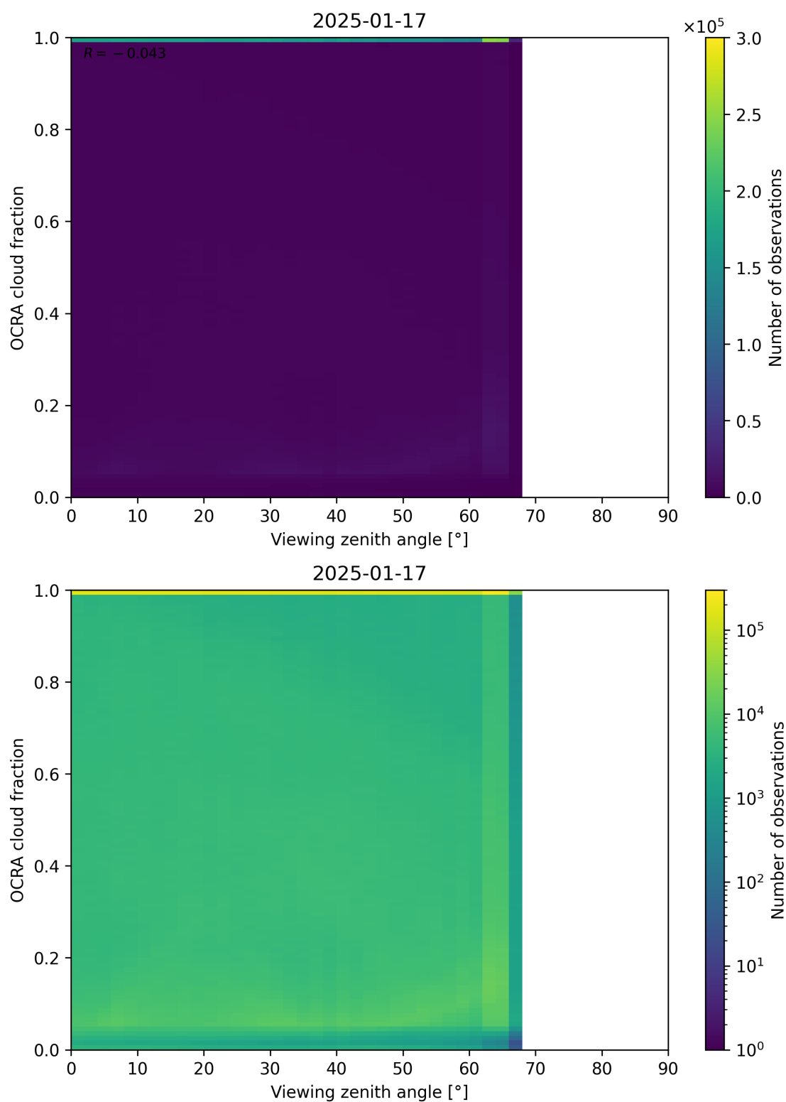
Figure 108: Scatter density plot of “Viewing zenith angle” against “OCRA cloud fraction” for 2025-01-17 to 2025-01-18.
