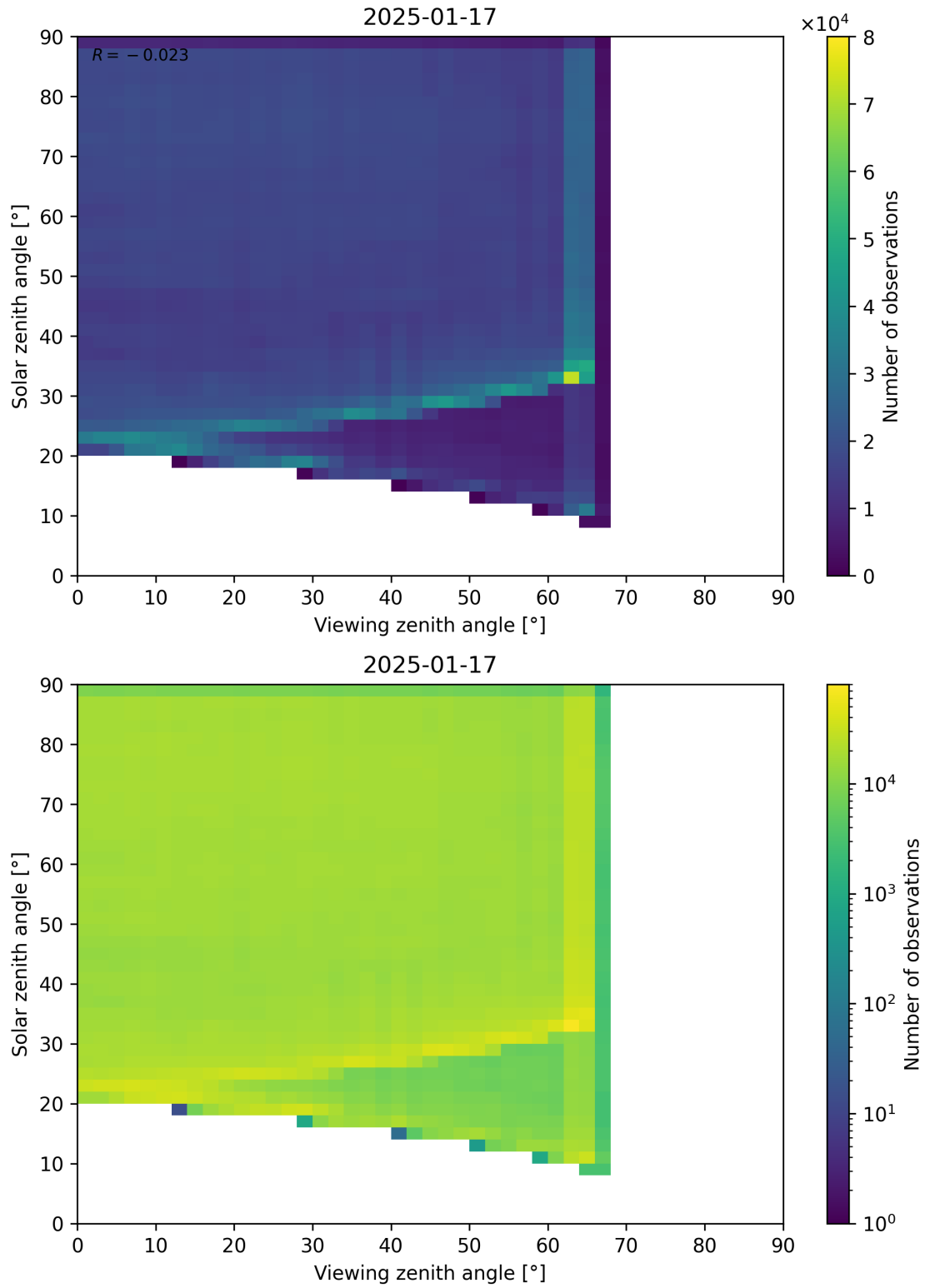
Figure 114: Scatter density plot of “Viewing zenith angle” against “Solar zenith angle” for 2025-01-17 to 2025-01-18.
