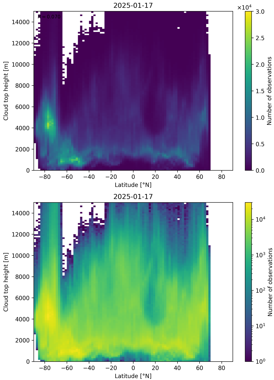
Figure 97: Scatter density plot of “Latitude” against “Cloud top height” for 2025-01-17 to 2025-01-18.
