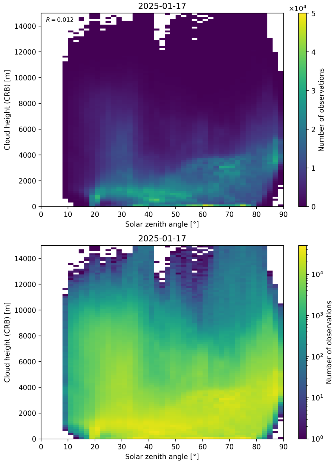
Figure 102: Scatter density plot of “Solar zenith angle” against “Cloud height (CRB)” for 2025-01-17 to 2025-01-18.
