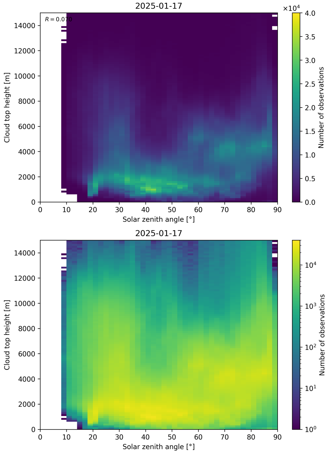
Figure 104: Scatter density plot of “Solar zenith angle” against “Cloud top height” for 2025-01-17 to 2025-01-18.
