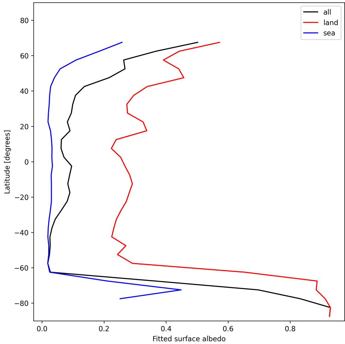
Figure 29: Zonal average of “Fitted surface albedo” for 2025-01-17 to 2025-01-18.
