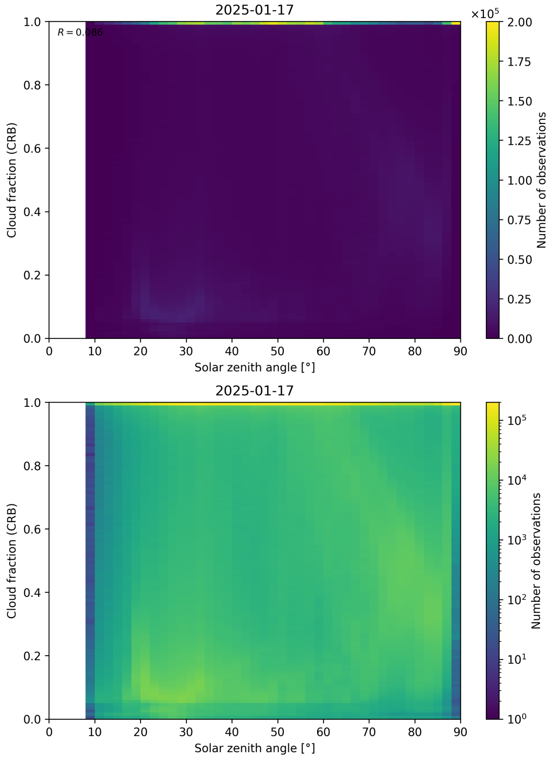
Figure 101: Scatter density plot of “Solar zenith angle” against “Cloud fraction (CRB)” for 2025-01-17 to 2025-01-18.
