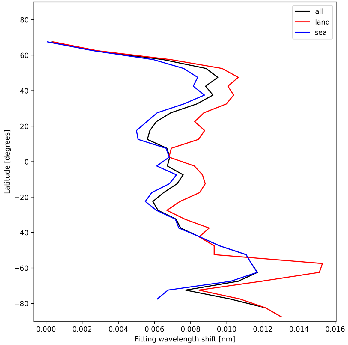
Figure 33: Zonal average of “Fitting wavelength shift” for 2025-01-17 to 2025-01-18.
