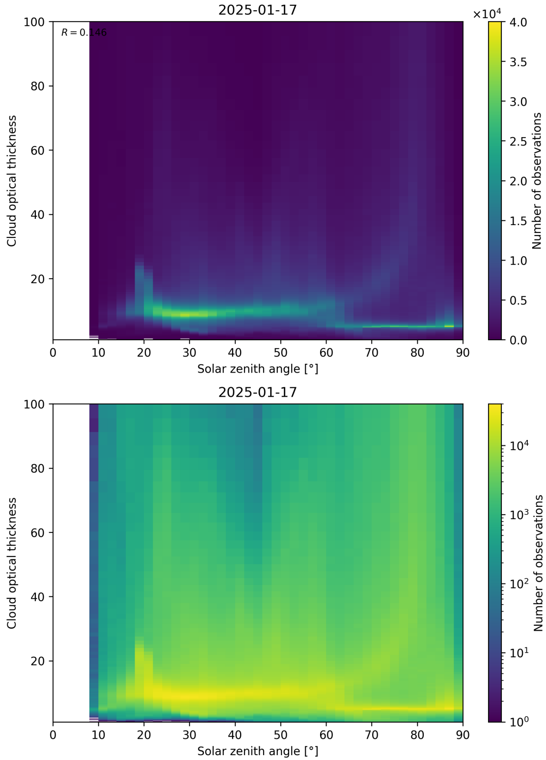
Figure 103: Scatter density plot of “Solar zenith angle” against “Cloud optical thickness” for 2025-01-17 to 2025-01-18.
