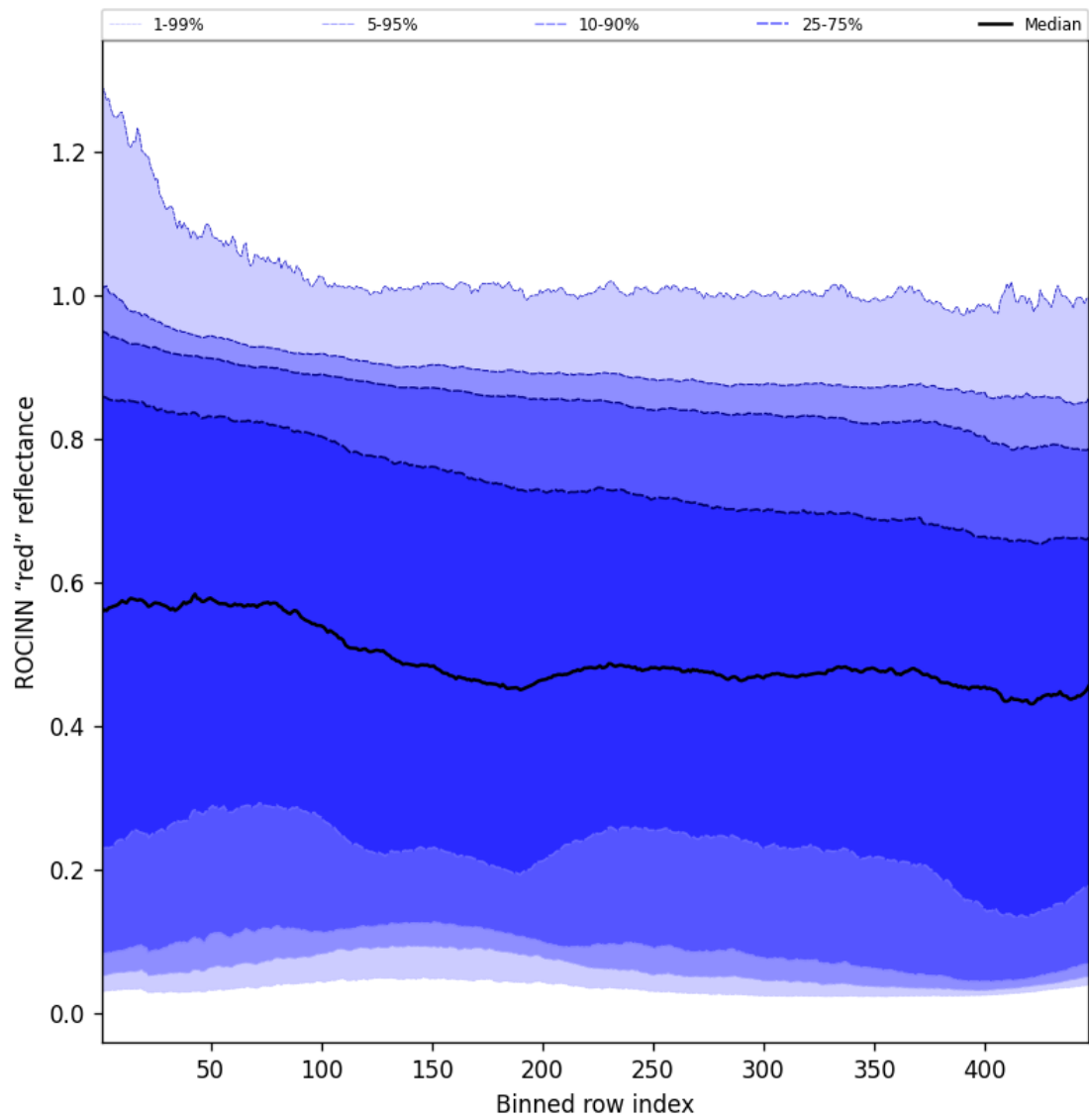
Figure 69: Along track statistics of "ROCINN "red" reflectance" for 2025-01-17 to 2025-01-18
