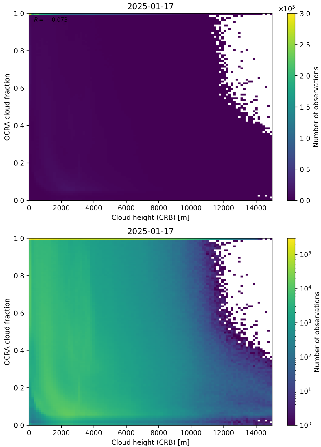
Figure 81: Scatter density plot of “Cloud height (CRB)” against “OCRA cloud fraction” for 2025-01-17 to 2025-01-18.
