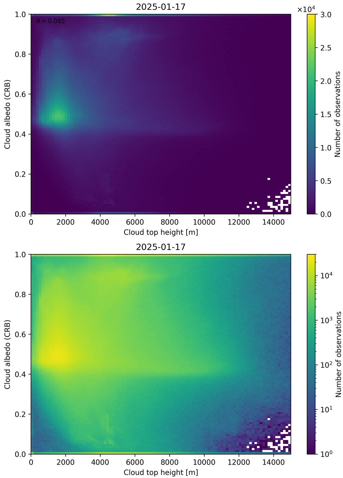
Figure 86: Scatter density plot of “Cloud top height” against “Cloud albedo (CRB)” for 2025-01-17 to 2025-01-18.
