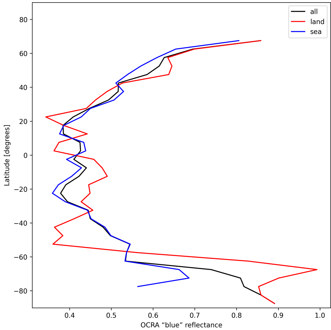
Figure 35: Zonal average of “OCRA “blue” reflectance” for 2025-01-17 to 2025-01-18.
