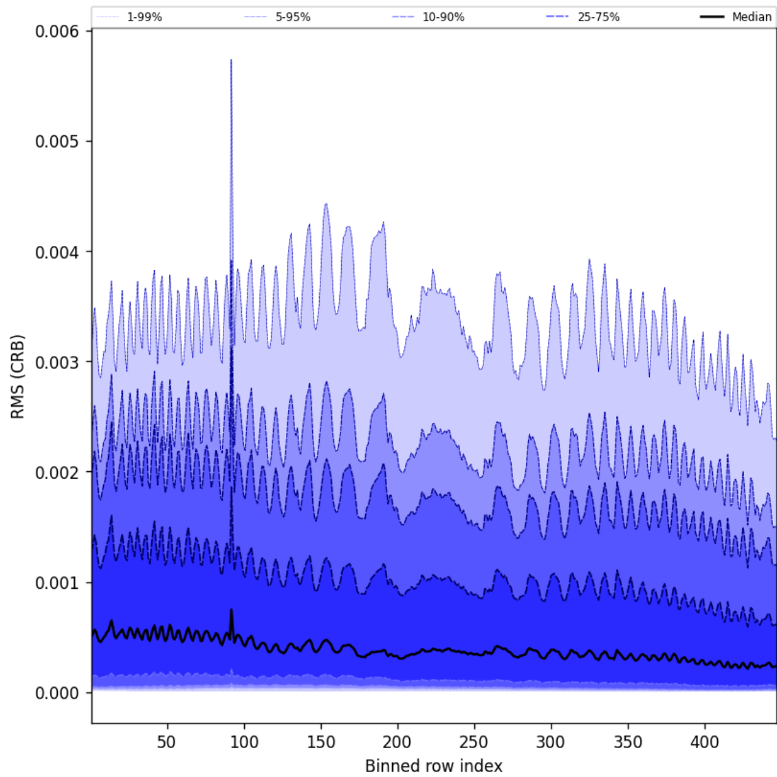
Figure 64: Along track statistics of “RMS (CRB)” for 2025-01-17 to 2025-01-18
