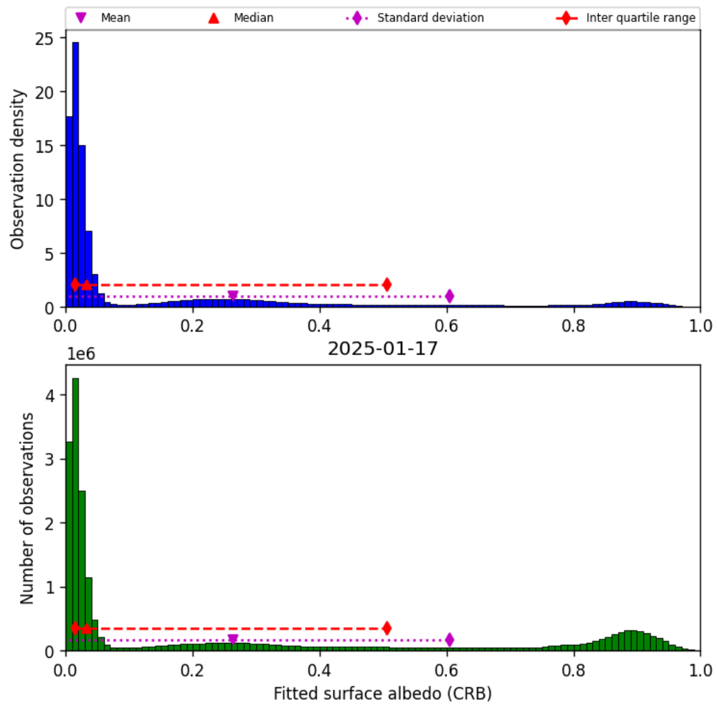
Figure 46: Histogram of “Fitted surface albedo (CRB)” for 2025-01-17 to 2025-01-18
