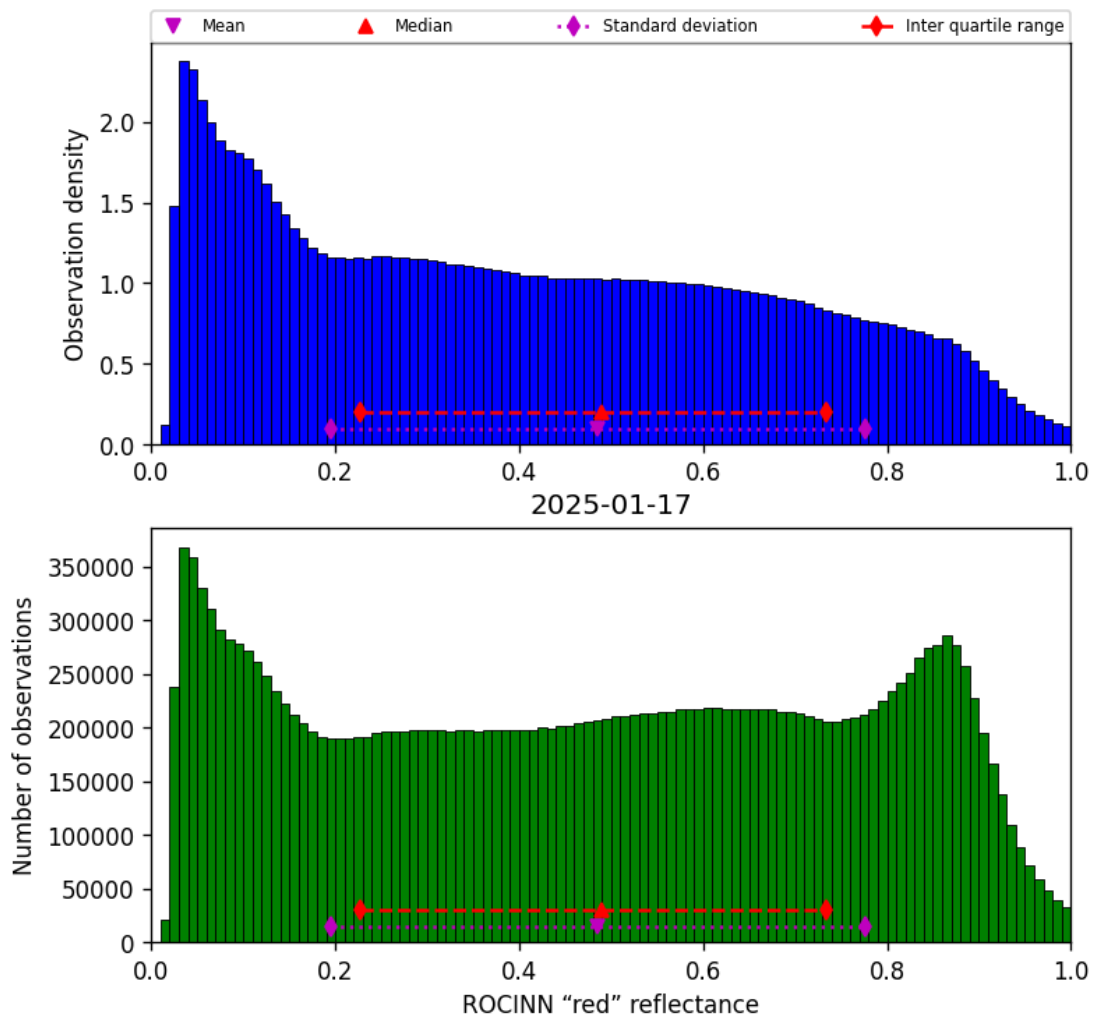
Figure 53: Histogram of “ROCINN “red” reflectance” for 2025-01-17 to 2025-01-18
