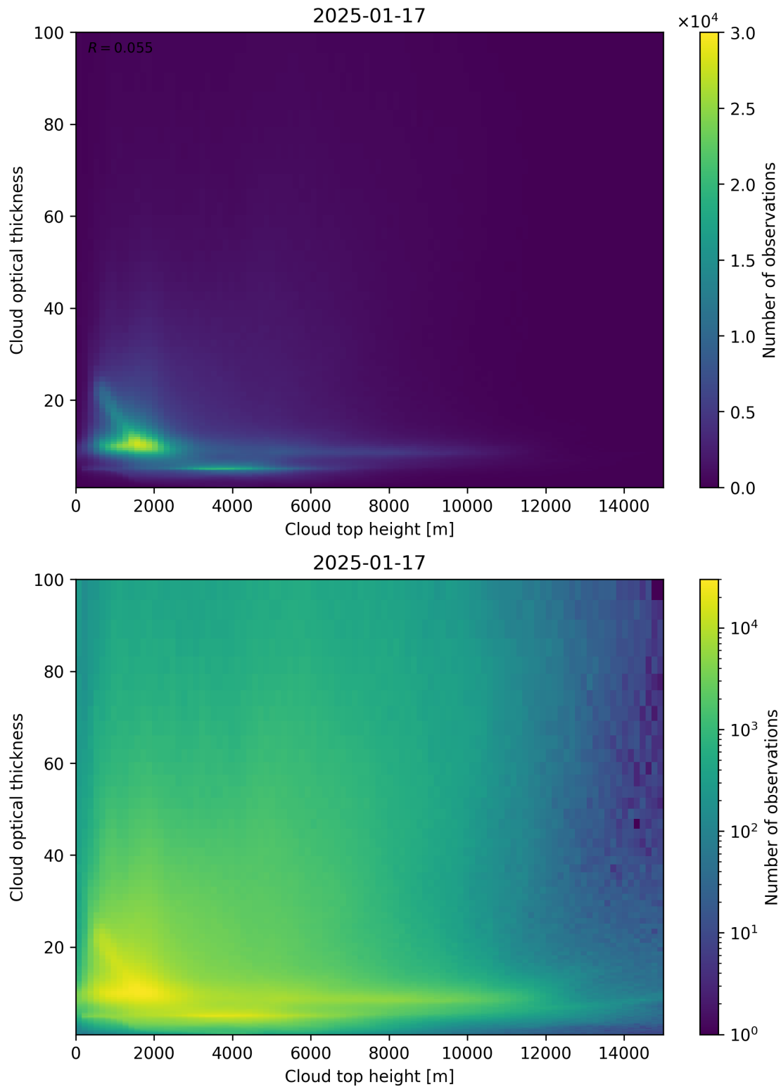
Figure 90: Scatter density plot of “Cloud top height” against “Cloud optical thickness” for 2025-01-17 to 2025-01-18.
