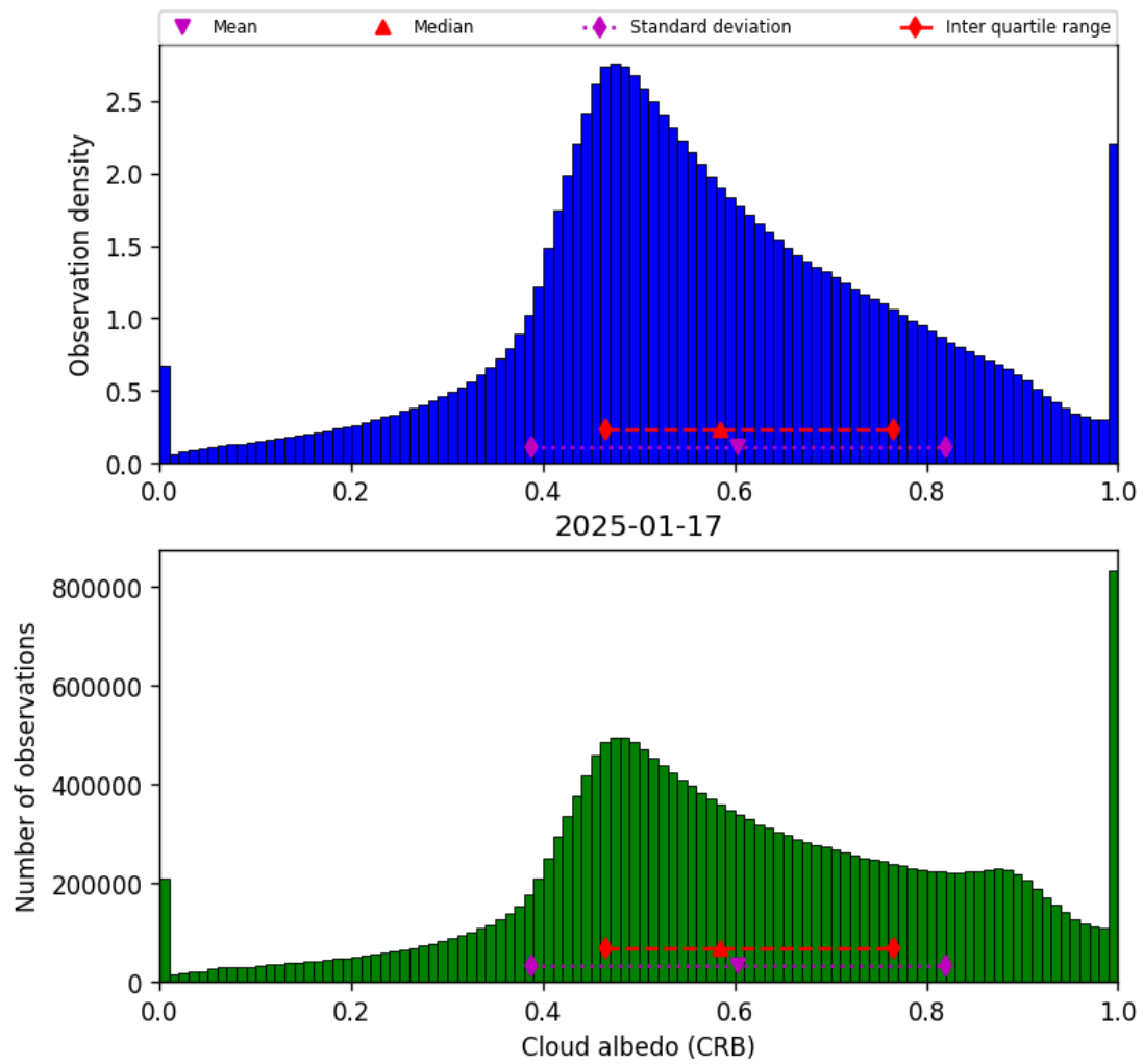
Figure 44: Histogram of “Cloud albedo (CRB)” for 2025-01-17 to 2025-01-18
