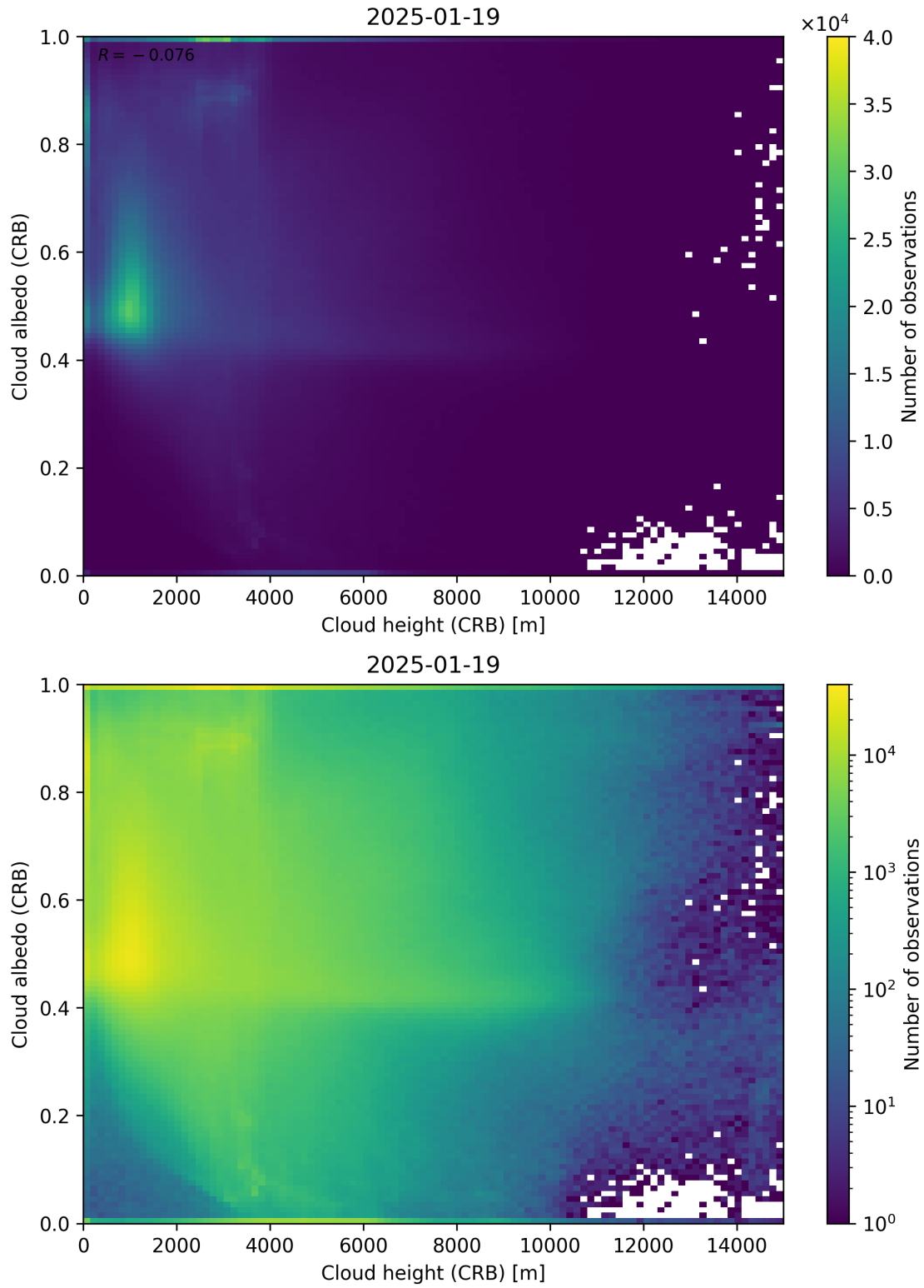
Figure 80: Scatter density plot of “Cloud height (CRB)” against “Cloud albedo (CRB)” for 2025-01-18 to 2025-01-20.
