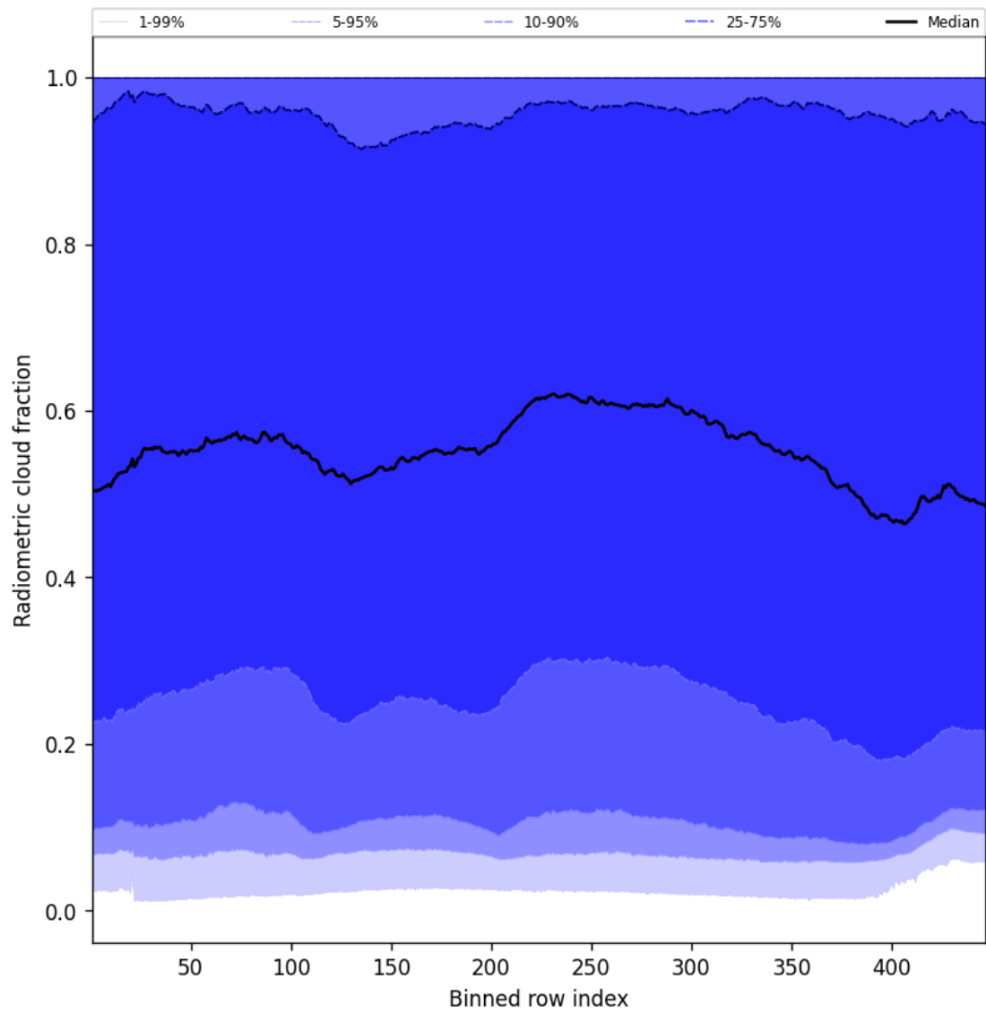
Figure 55: Along track statistics of “Radiometric cloud fraction” for 2025-01-18 to 2025-01-20
