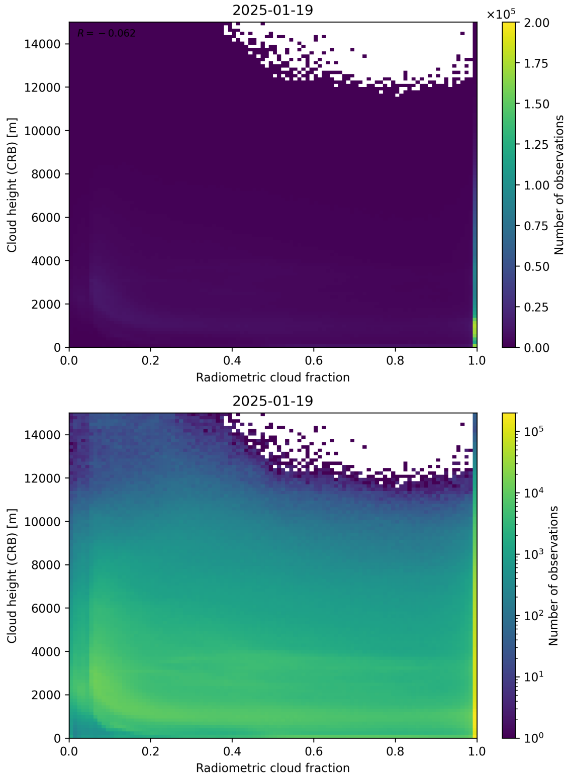
Figure 74: Scatter density plot of “Radiometric cloud fraction” against “Cloud height (CRB)” for 2025-01-18 to 2025-01-20.
