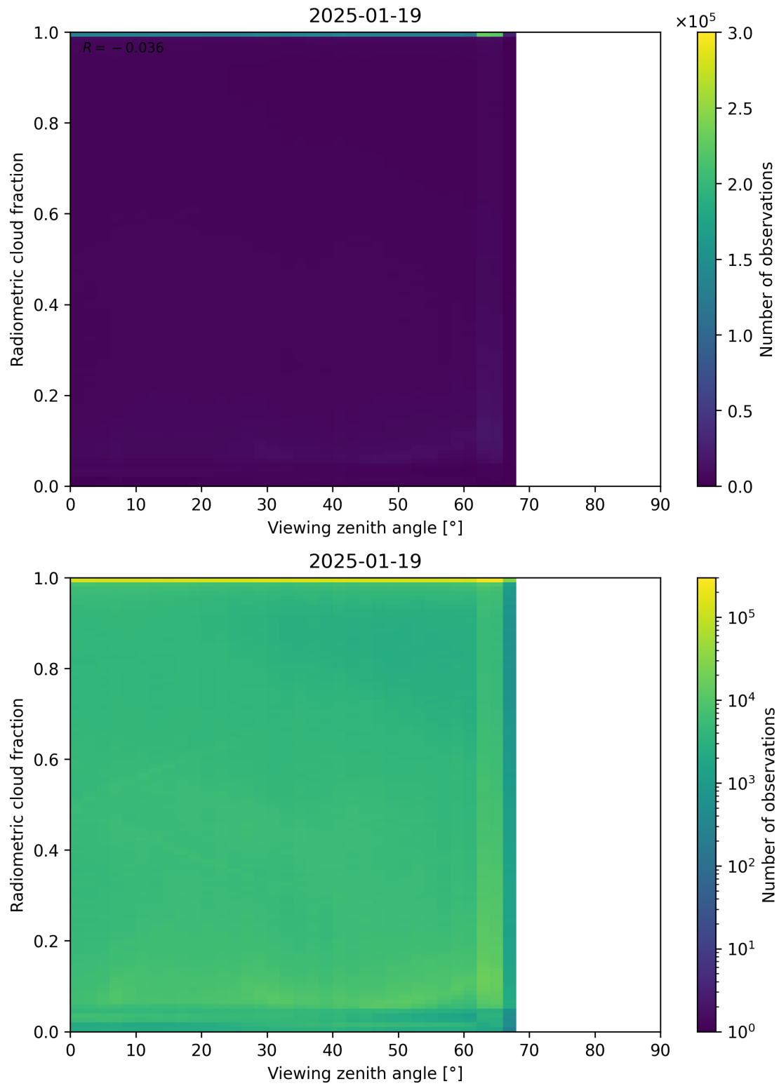
Figure 107: Scatter density plot of “Viewing zenith angle” against “Radiometric cloud fraction” for 2025-01-18 to 2025-01-20.
