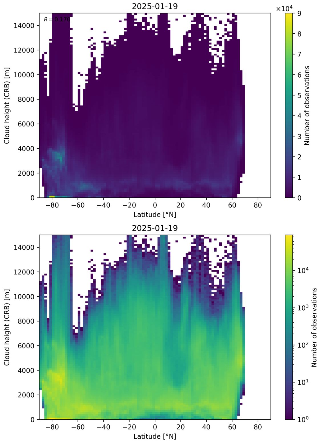
Figure 95: Scatter density plot of “Latitude” against “Cloud height (CRB)” for 2025-01-18 to 2025-01-20.
