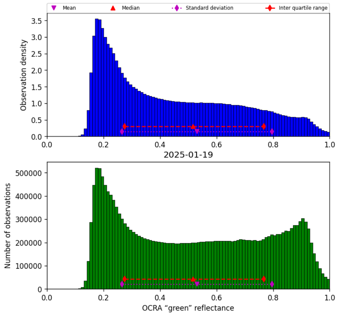
Figure 52: Histogram of “OCRA “green” reflectance” for 2025-01-18 to 2025-01-20
