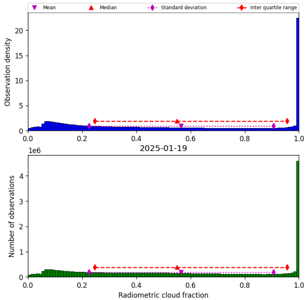
Figure 39: Histogram of “Radiometric cloud fraction” for 2025-01-18 to 2025-01-20
