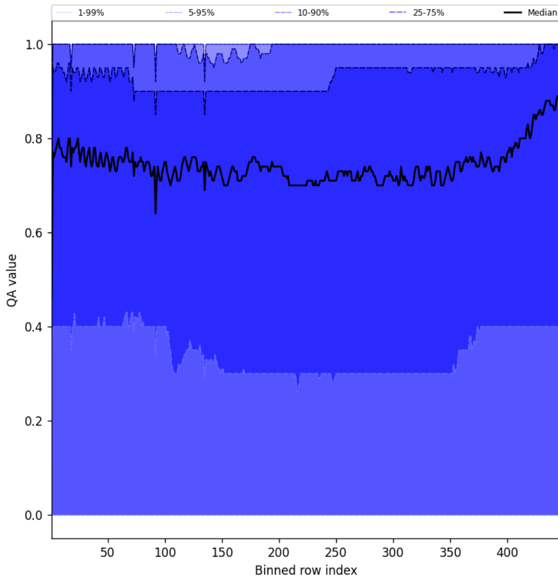
Figure 54: Along track statistics of “QA value” for 2025-01-18 to 2025-01-20
