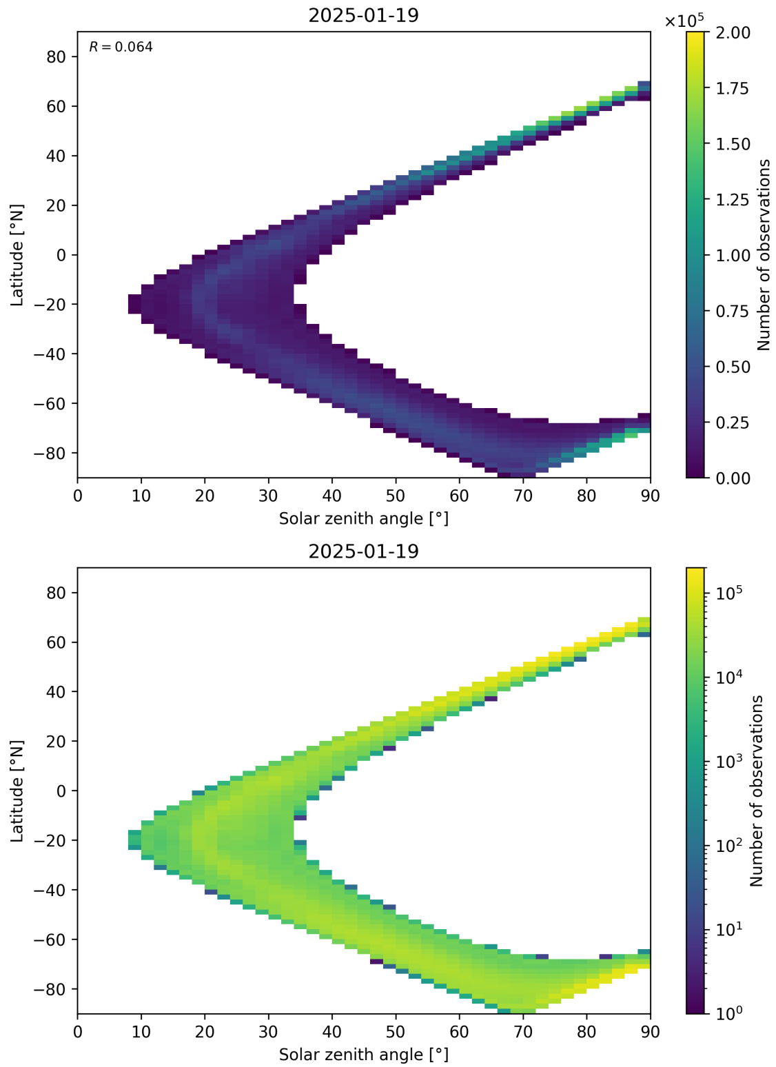
Figure 105: Scatter density plot of “Solar zenith angle” against “Latitude” for 2025-01-18 to 2025-01-20.
