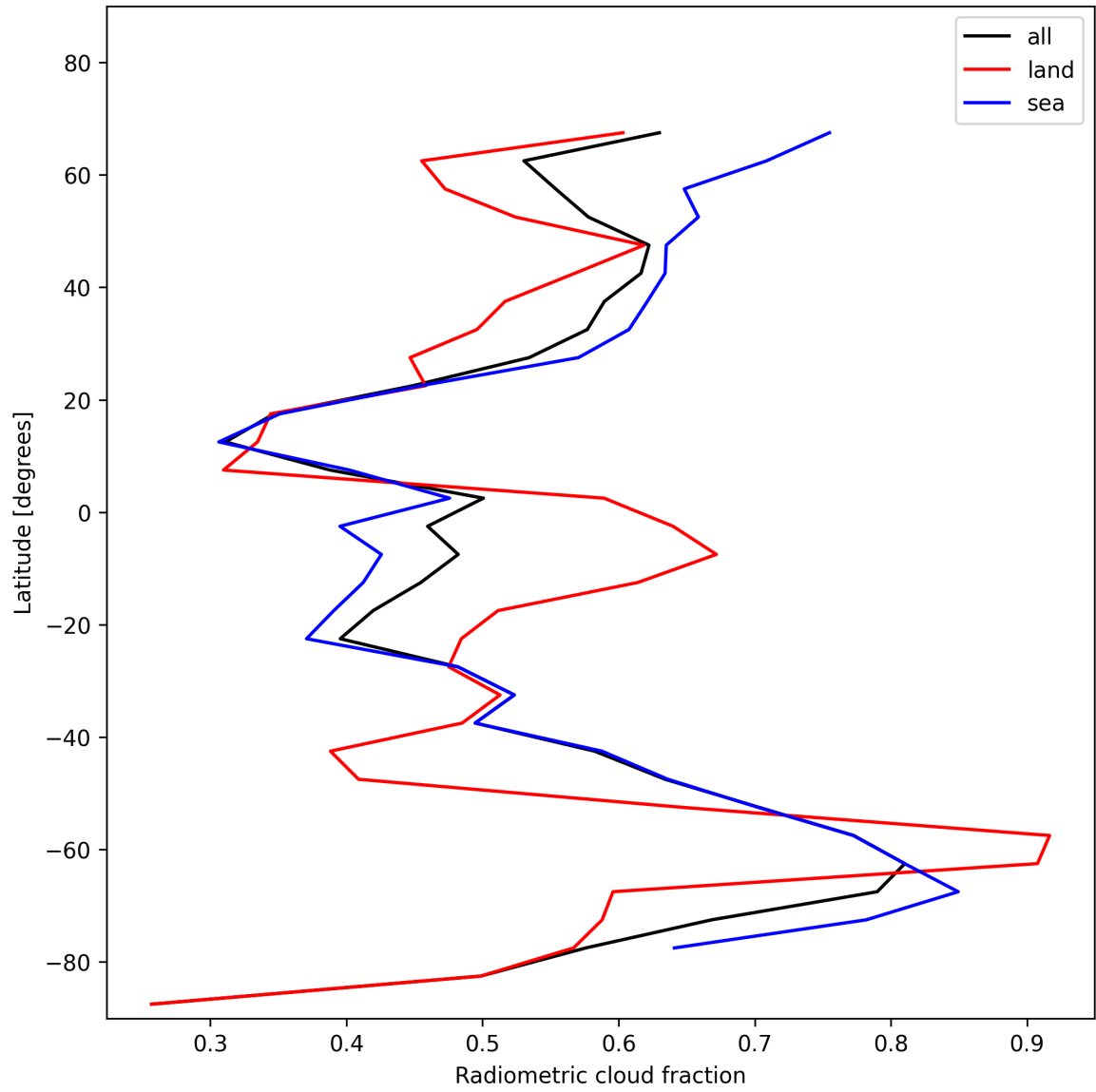
Figure 23: Zonal average of “Radiometric cloud fraction” for 2025-01-18 to 2025-01-20.
