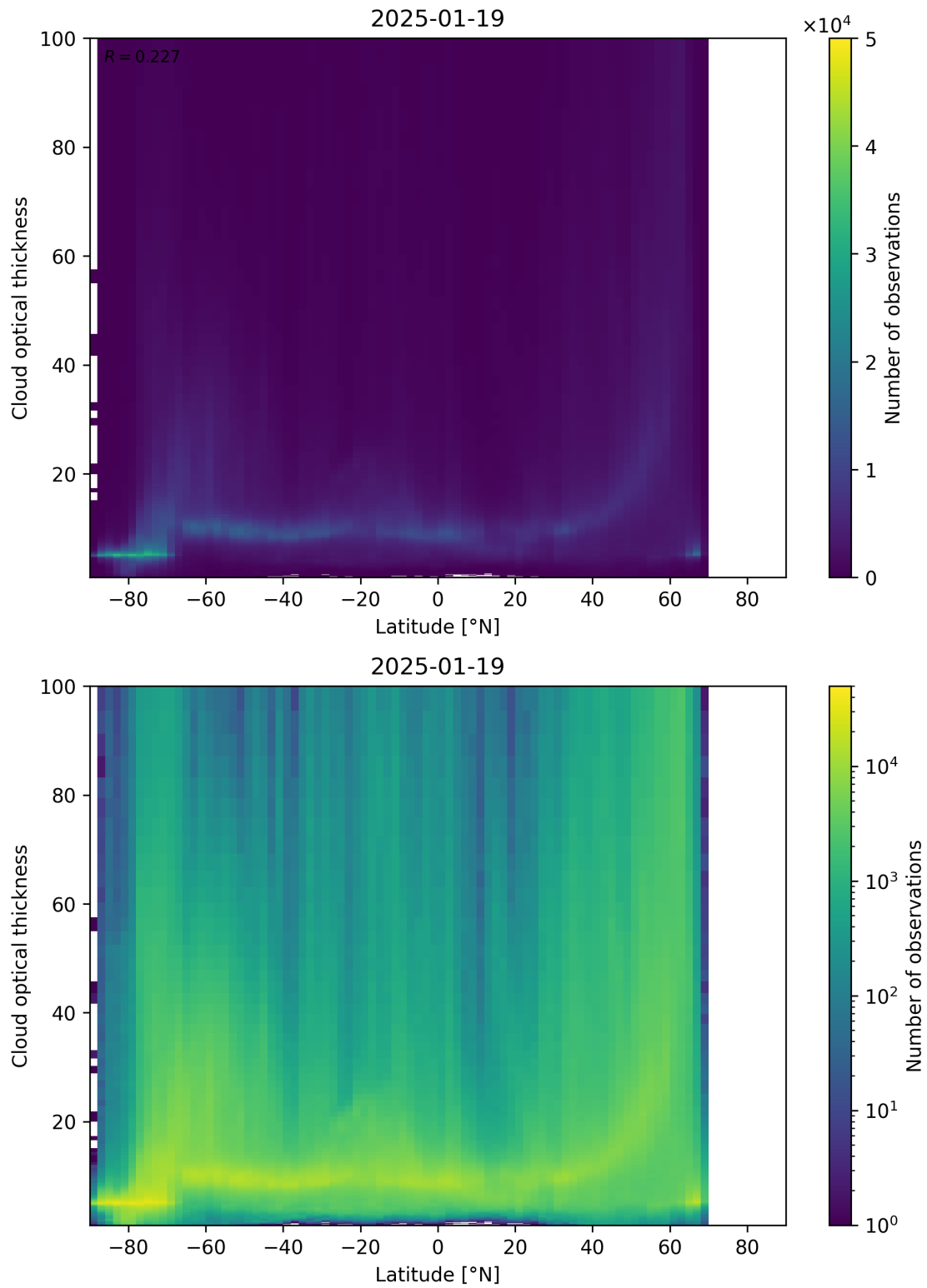
Figure 96: Scatter density plot of “Latitude” against “Cloud optical thickness” for 2025-01-18 to 2025-01-20.
