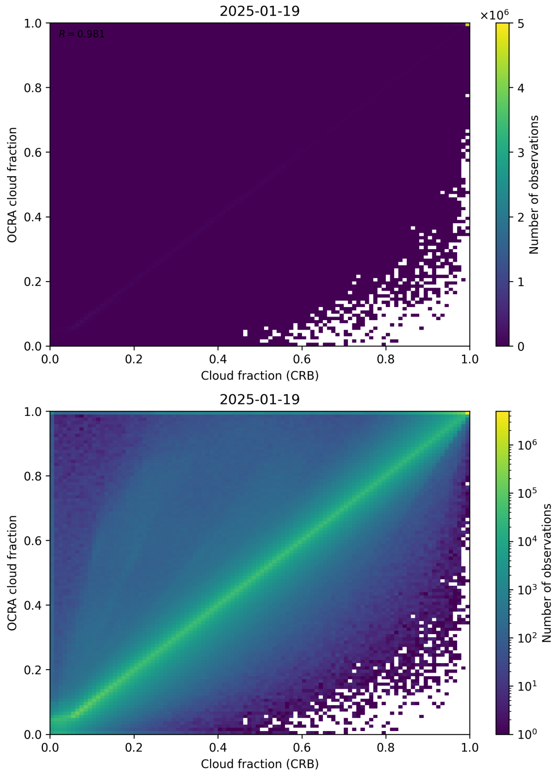
Figure 78: Scatter density plot of “Cloud fraction (CRB)” against “OCRA cloud fraction” for 2025-01-18 to 2025-01-20.
