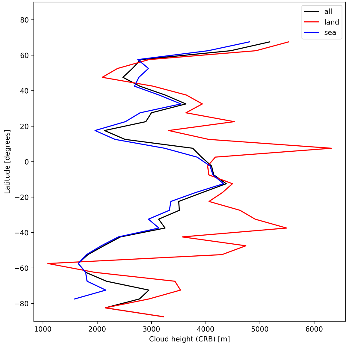
Figure 27: Zonal average of “Cloud height (CRB)” for 2025-01-18 to 2025-01-20.
