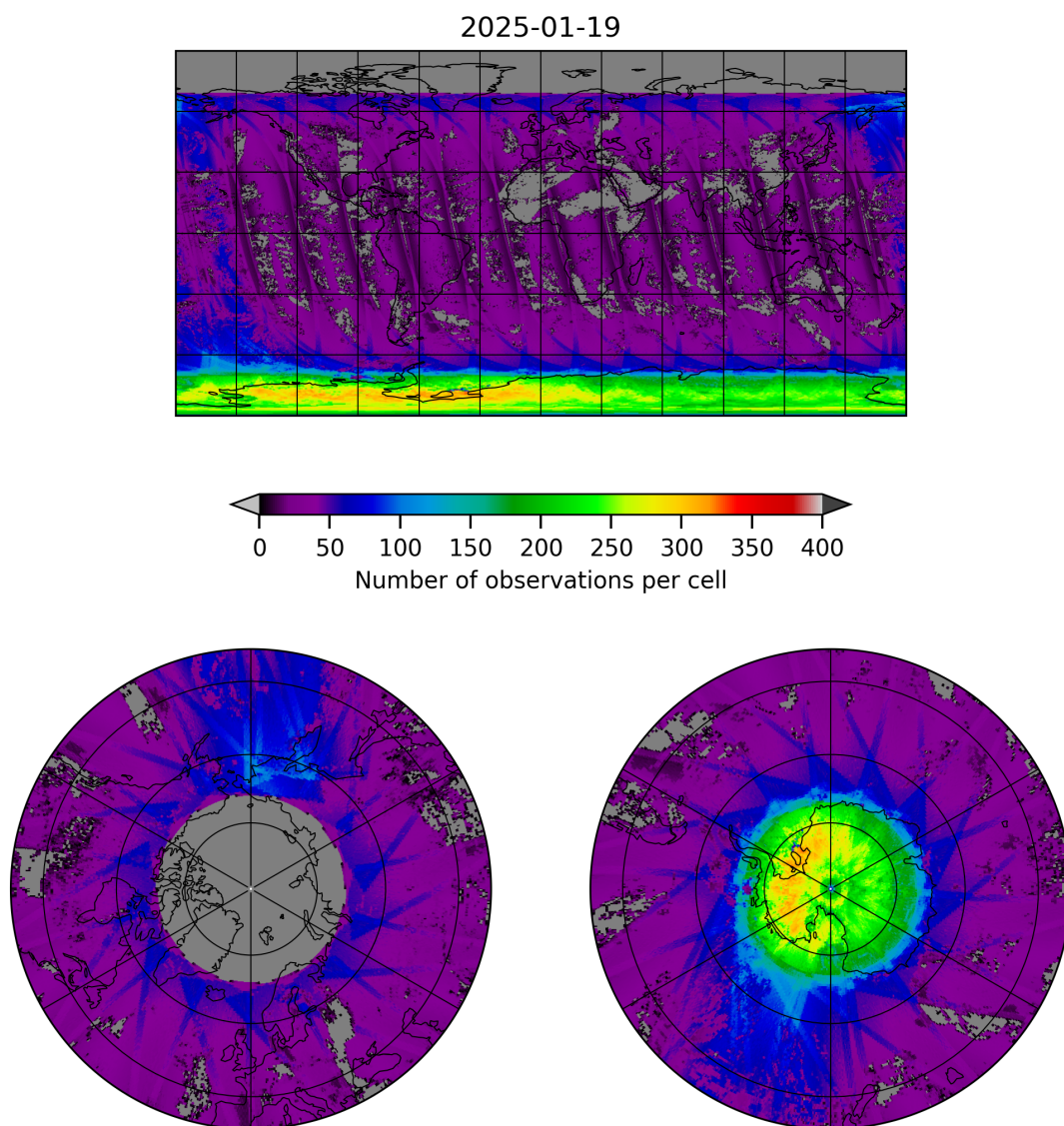
Figure 21: Map of the number of observations for 2025-01-18 to 2025-01-20
