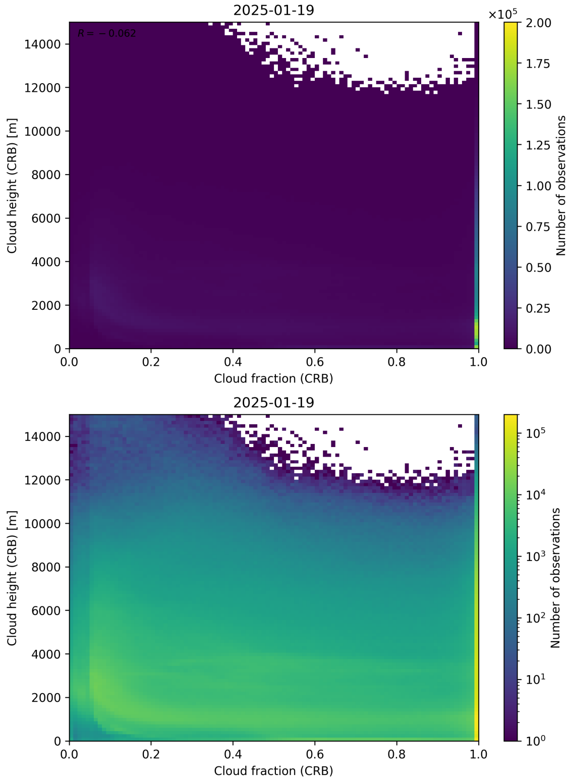
Figure 79: Scatter density plot of “Cloud fraction (CRB)” against “Cloud height (CRB)” for 2025-01-18 to 2025-01-20.
