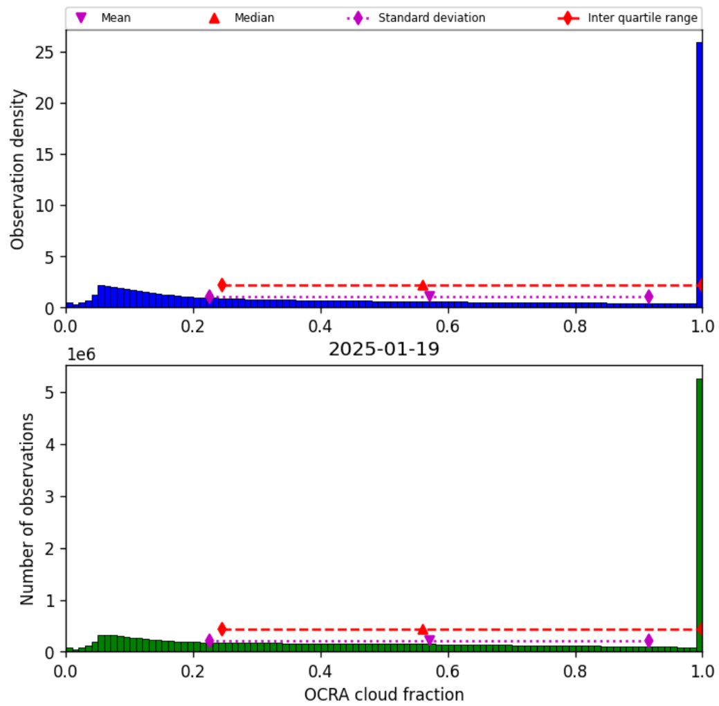
Figure 50: Histogram of “OCRA cloud fraction” for 2025-01-18 to 2025-01-20
