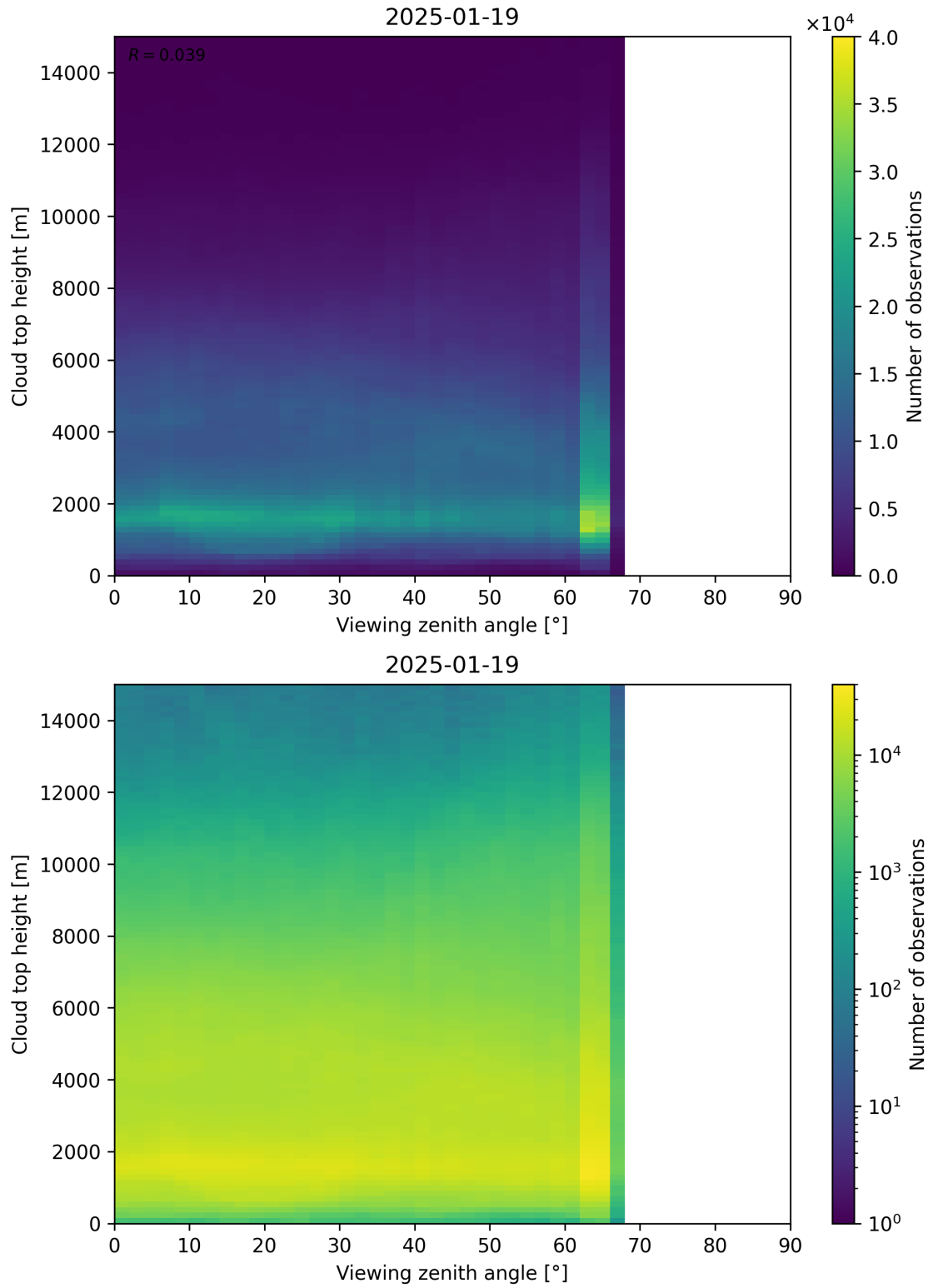
Figure 112: Scatter density plot of “Viewing zenith angle” against “Cloud top height” for 2025-01-18 to 2025-01-20.
