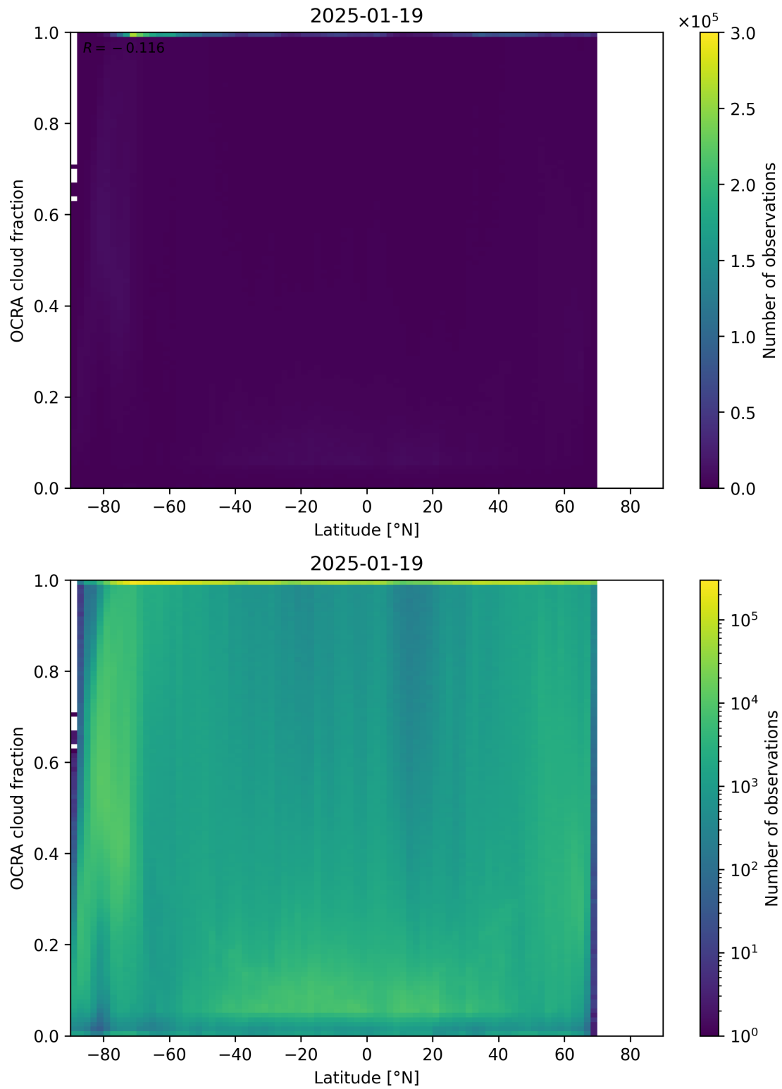
Figure 93: Scatter density plot of “Latitude” against “OCRA cloud fraction” for 2025-01-18 to 2025-01-20.
