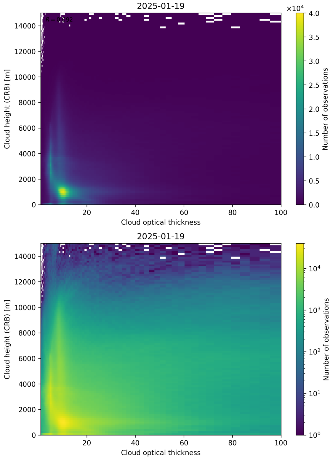
Figure 85: Scatter density plot of “Cloud optical thickness” against “Cloud height (CRB)” for 2025-01-18 to 2025-01-20.
