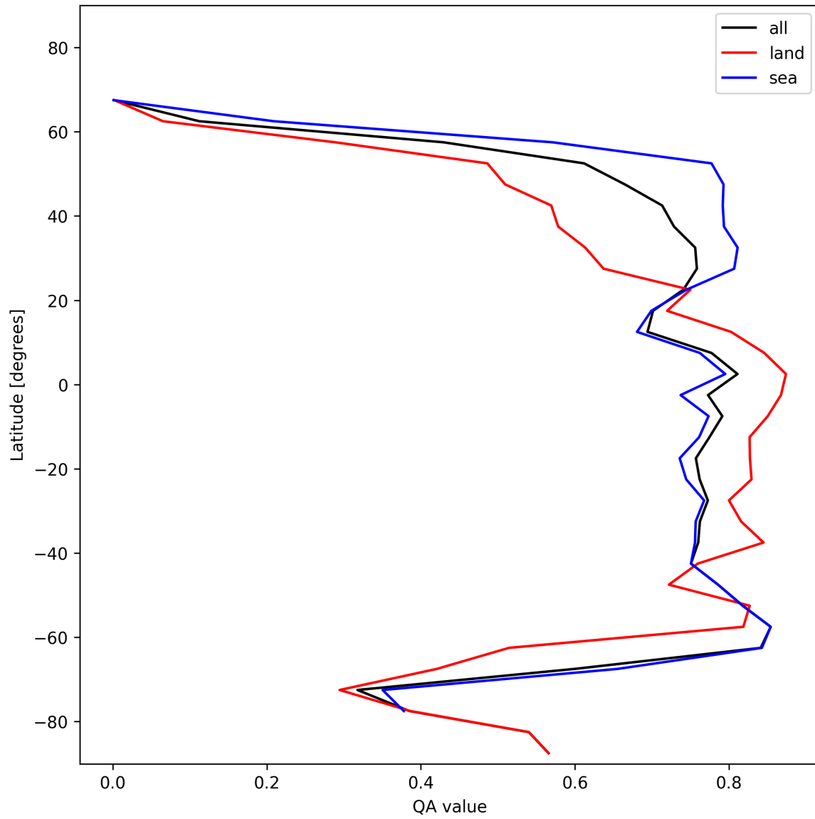
Figure 22: Zonal average of “QA value” for 2025-01-18 to 2025-01-20.
