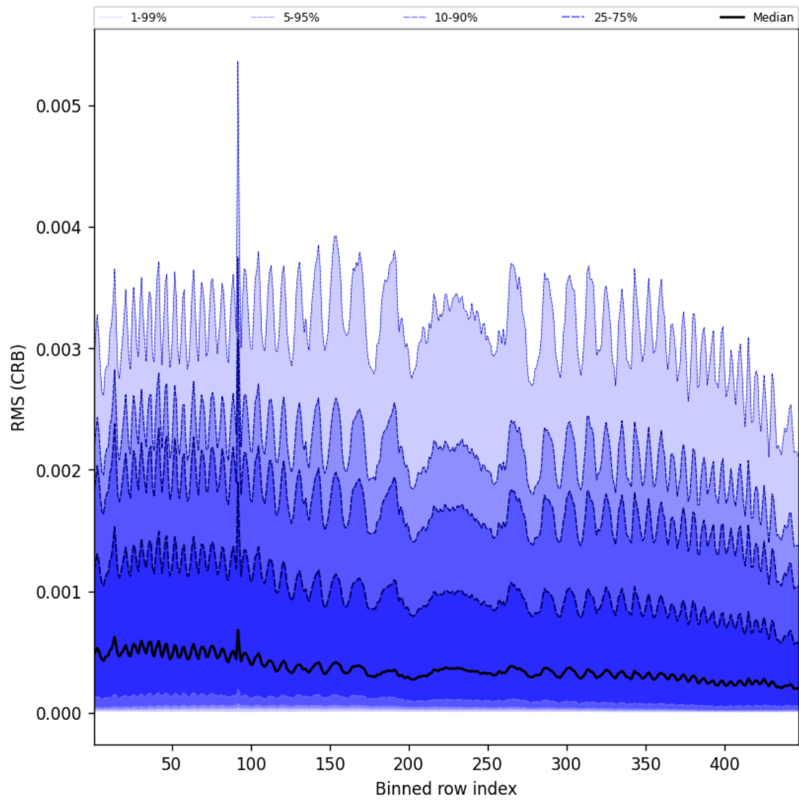
Figure 64: Along track statistics of “RMS (CRB)” for 2025-01-18 to 2025-01-20
