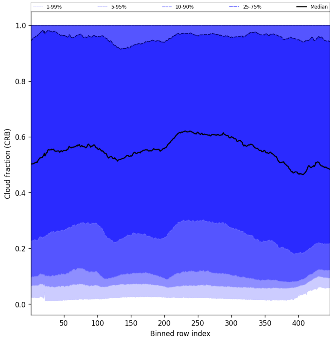
Figure 58: Along track statistics of “Cloud fraction (CRB)” for 2025-01-18 to 2025-01-20
