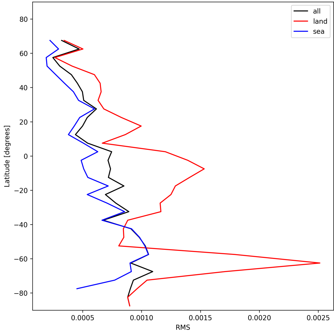
Figure 31: Zonal average of “RMS” for 2025-01-18 to 2025-01-20.
