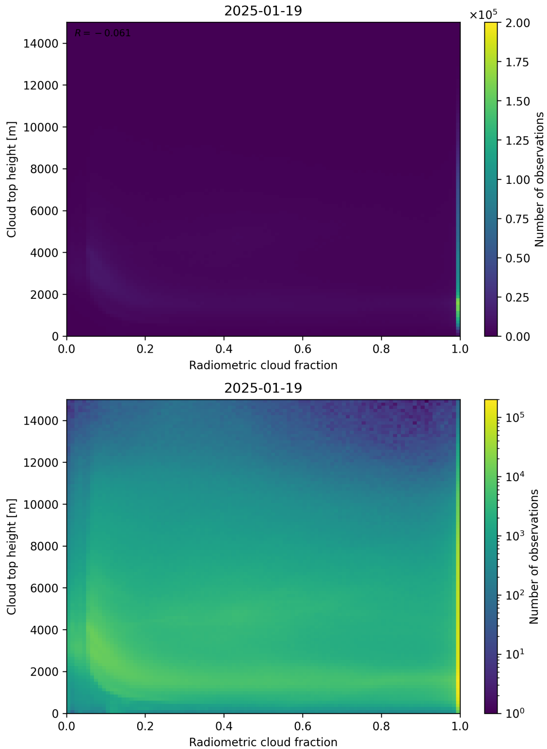
Figure 76: Scatter density plot of “Radiometric cloud fraction” against “Cloud top height” for 2025-01-18 to 2025-01-20.
