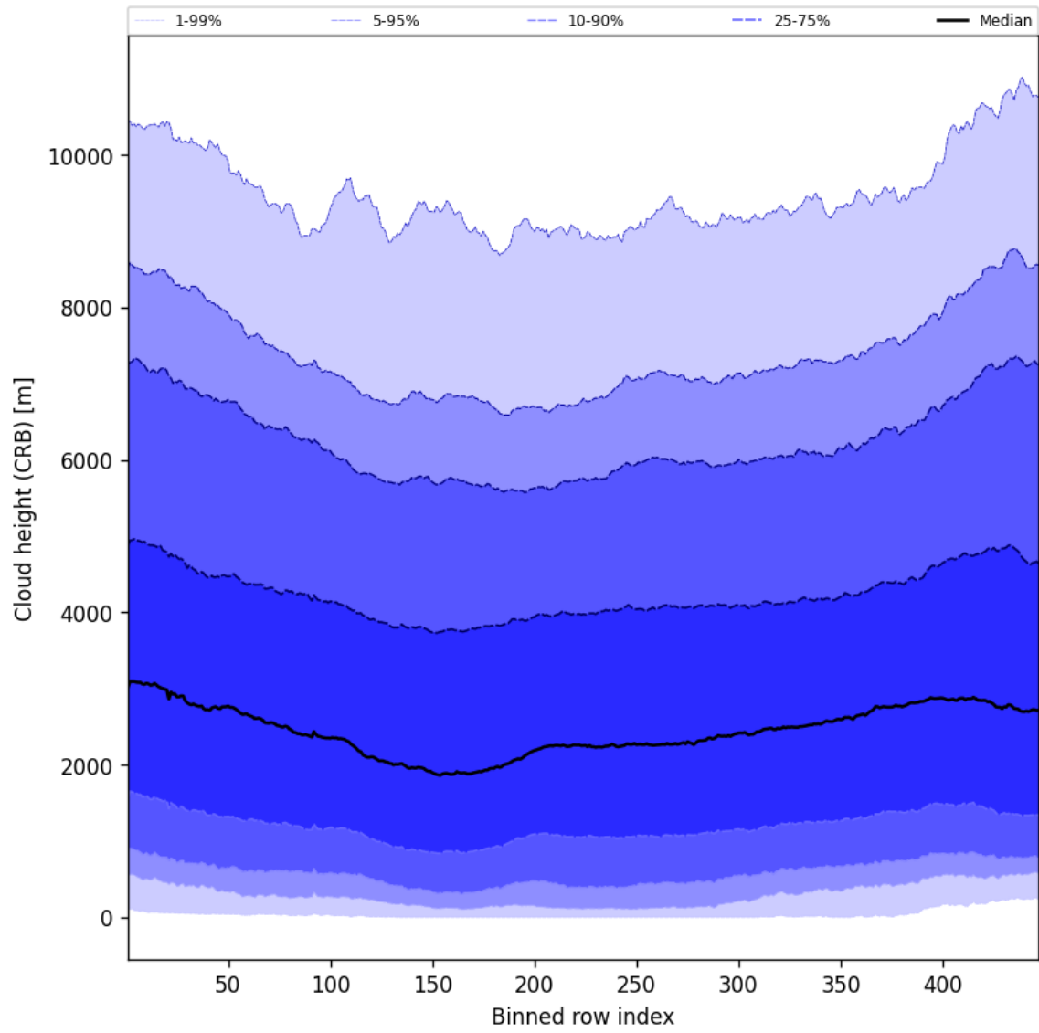
Figure 59: Along track statistics of “Cloud height (CRB)” for 2025-01-18 to 2025-01-20
