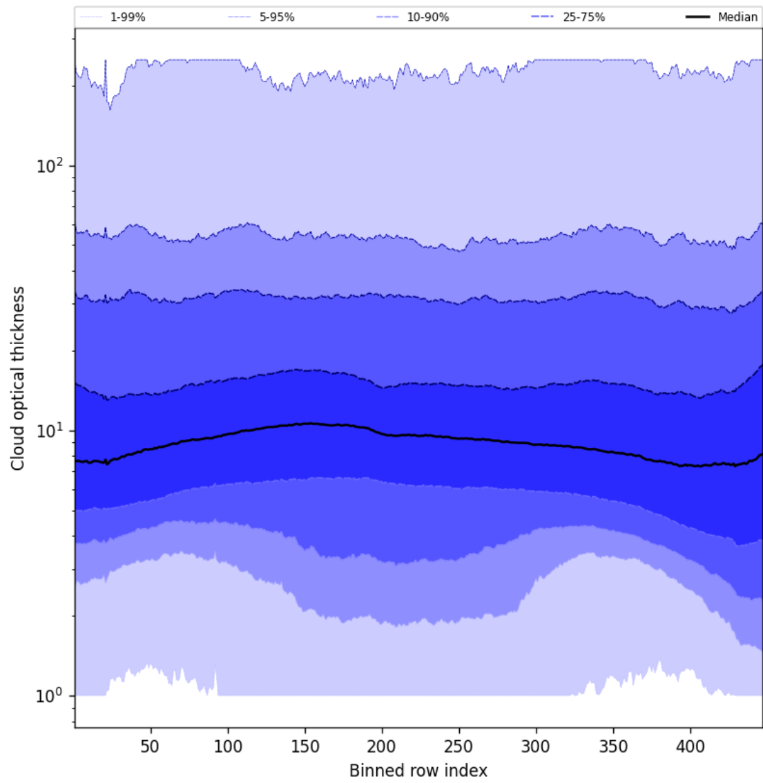
Figure 57: Along track statistics of “Cloud optical thickness” for 2025-01-18 to 2025-01-20
