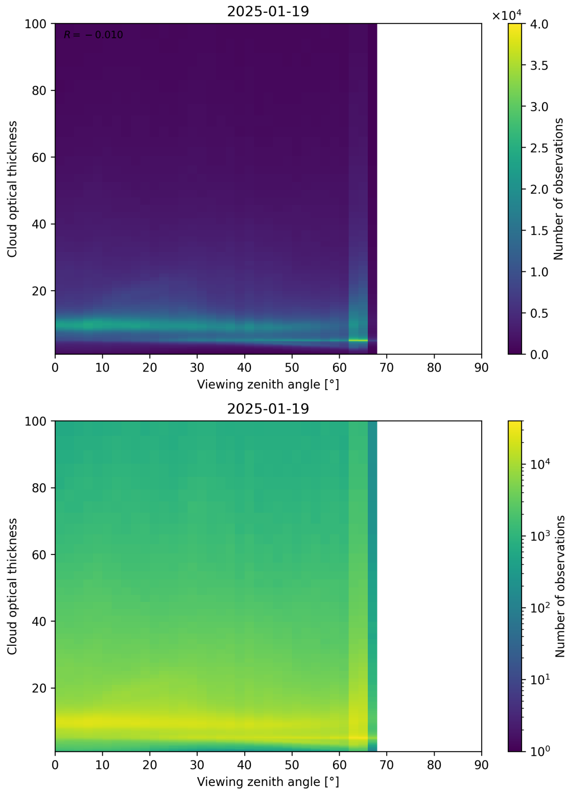
Figure 111: Scatter density plot of “Viewing zenith angle” against “Cloud optical thickness” for 2025-01-18 to 2025-01-20.
