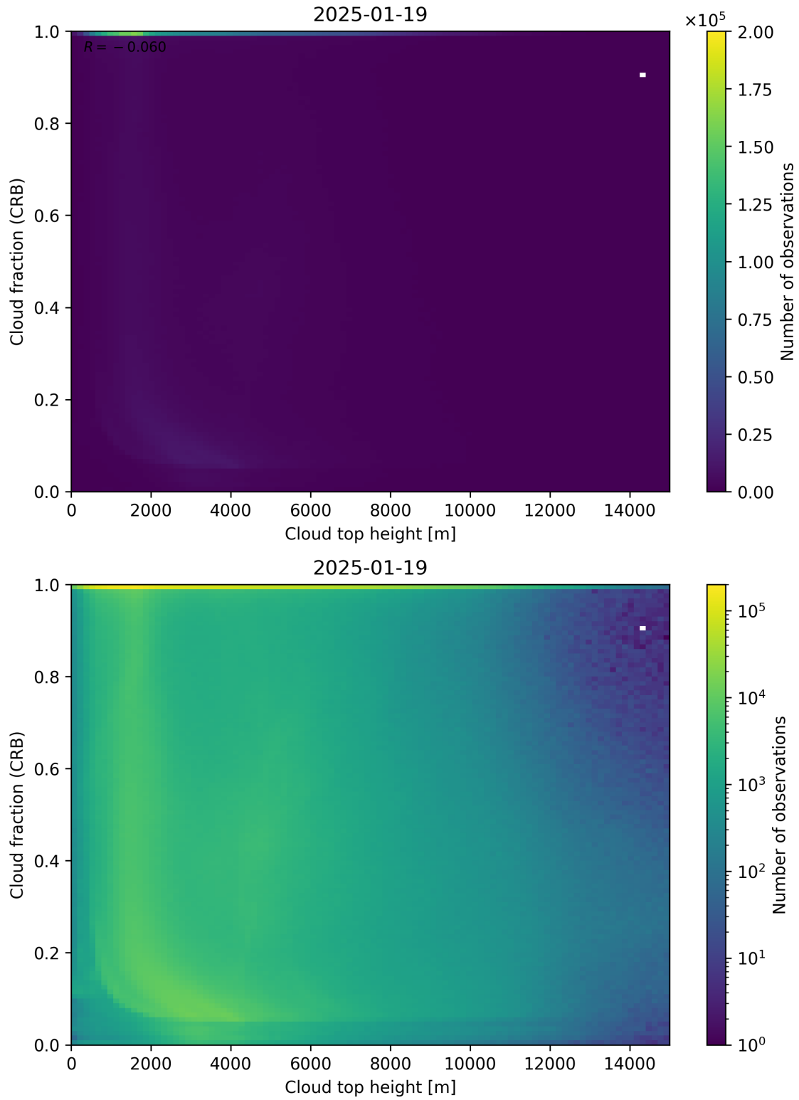
Figure 88: Scatter density plot of “Cloud top height” against “Cloud fraction (CRB)” for 2025-01-18 to 2025-01-20.
