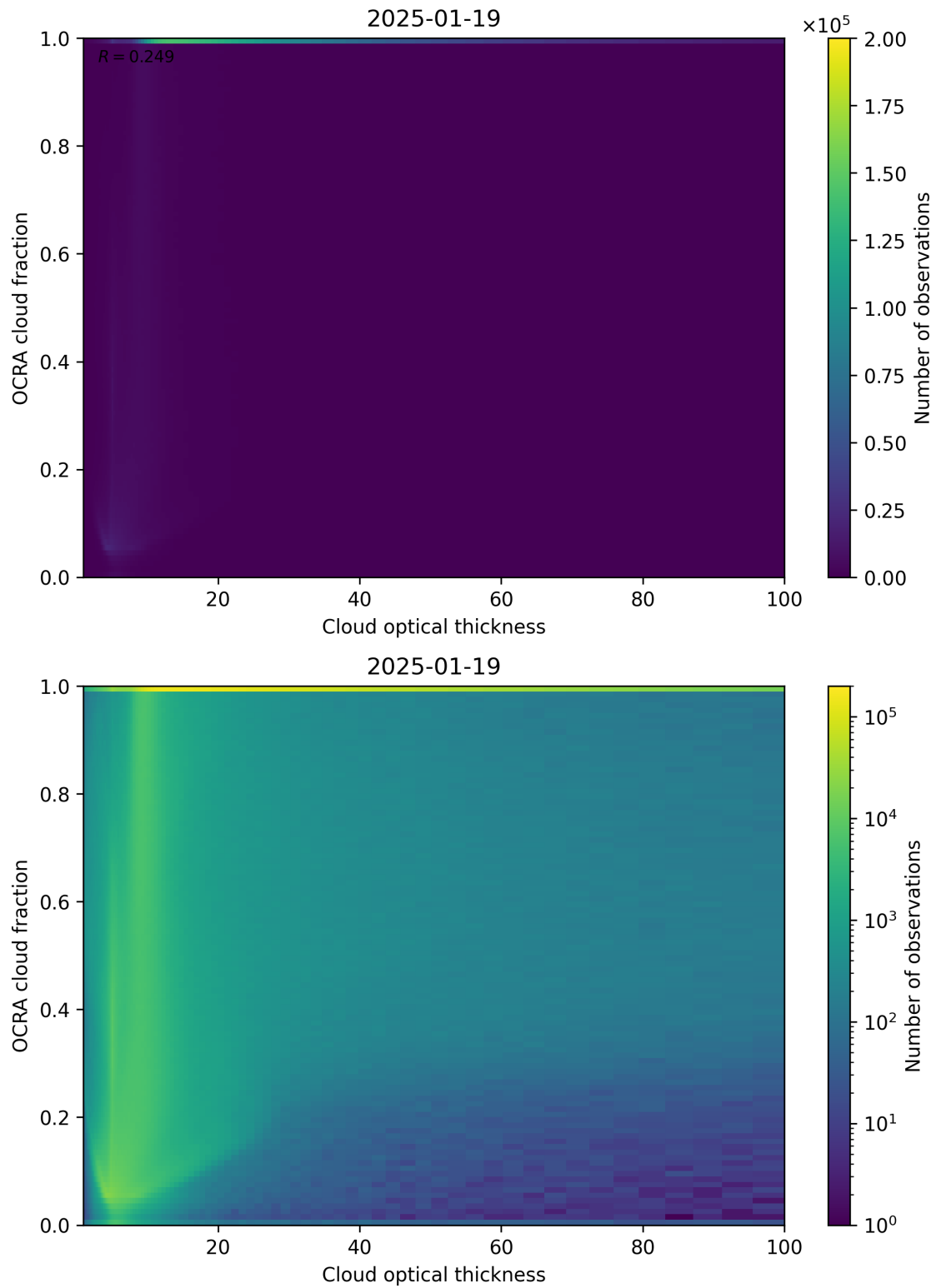
Figure 83: Scatter density plot of “Cloud optical thickness” against “OCRA cloud fraction” for 2025-01-18 to 2025-01-20.
