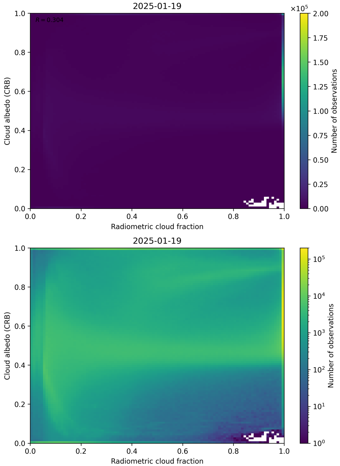
Figure 71: Scatter density plot of “Radiometric cloud fraction” against “Cloud albedo (CRB)” for 2025-01-18 to 2025-01-20.
