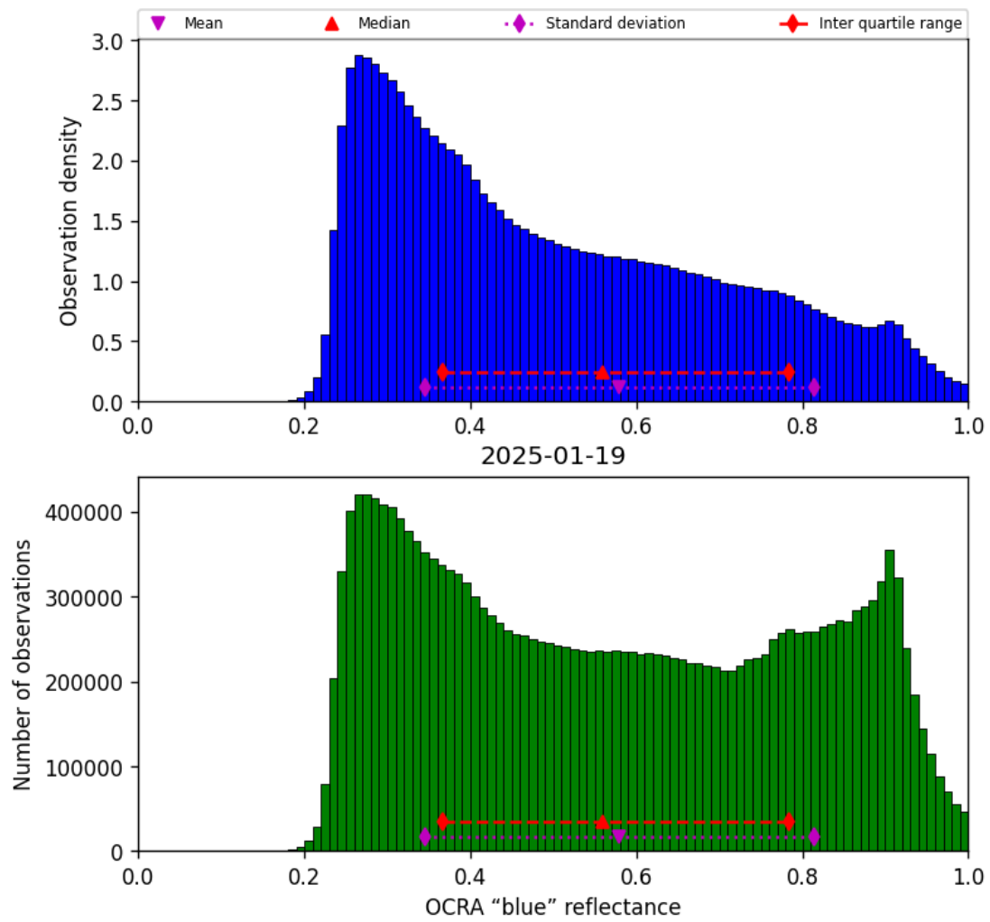
Figure 51: Histogram of “OCRA “blue” reflectance” for 2025-01-18 to 2025-01-20
