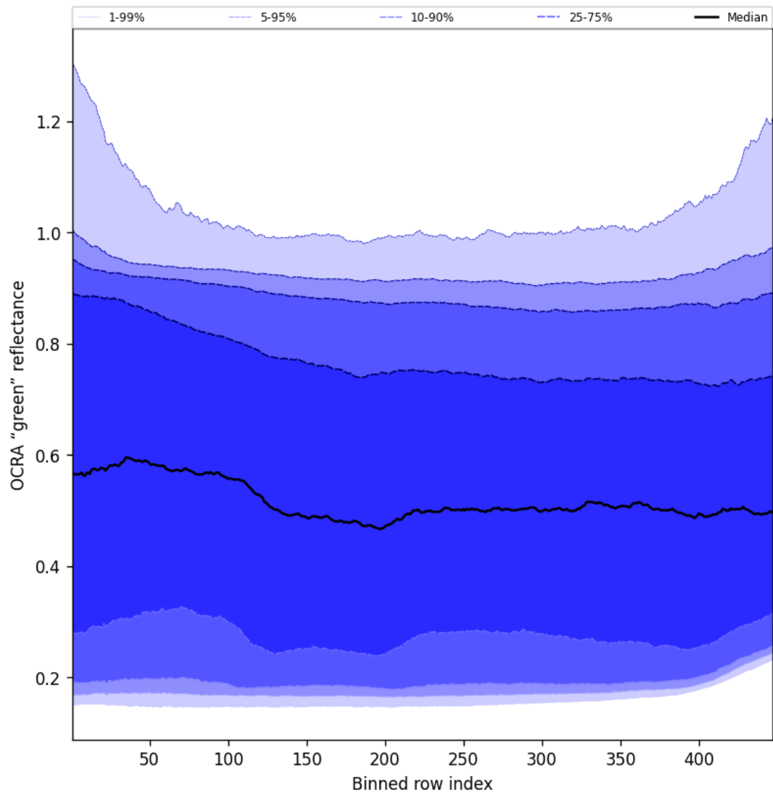
Figure 68: Along track statistics of "OCRA "green" reflectance" for 2025-01-18 to 2025-01-20
