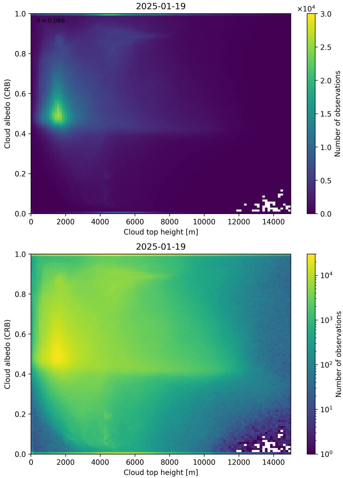
Figure 86: Scatter density plot of “Cloud top height” against “Cloud albedo (CRB)” for 2025-01-18 to 2025-01-20.
