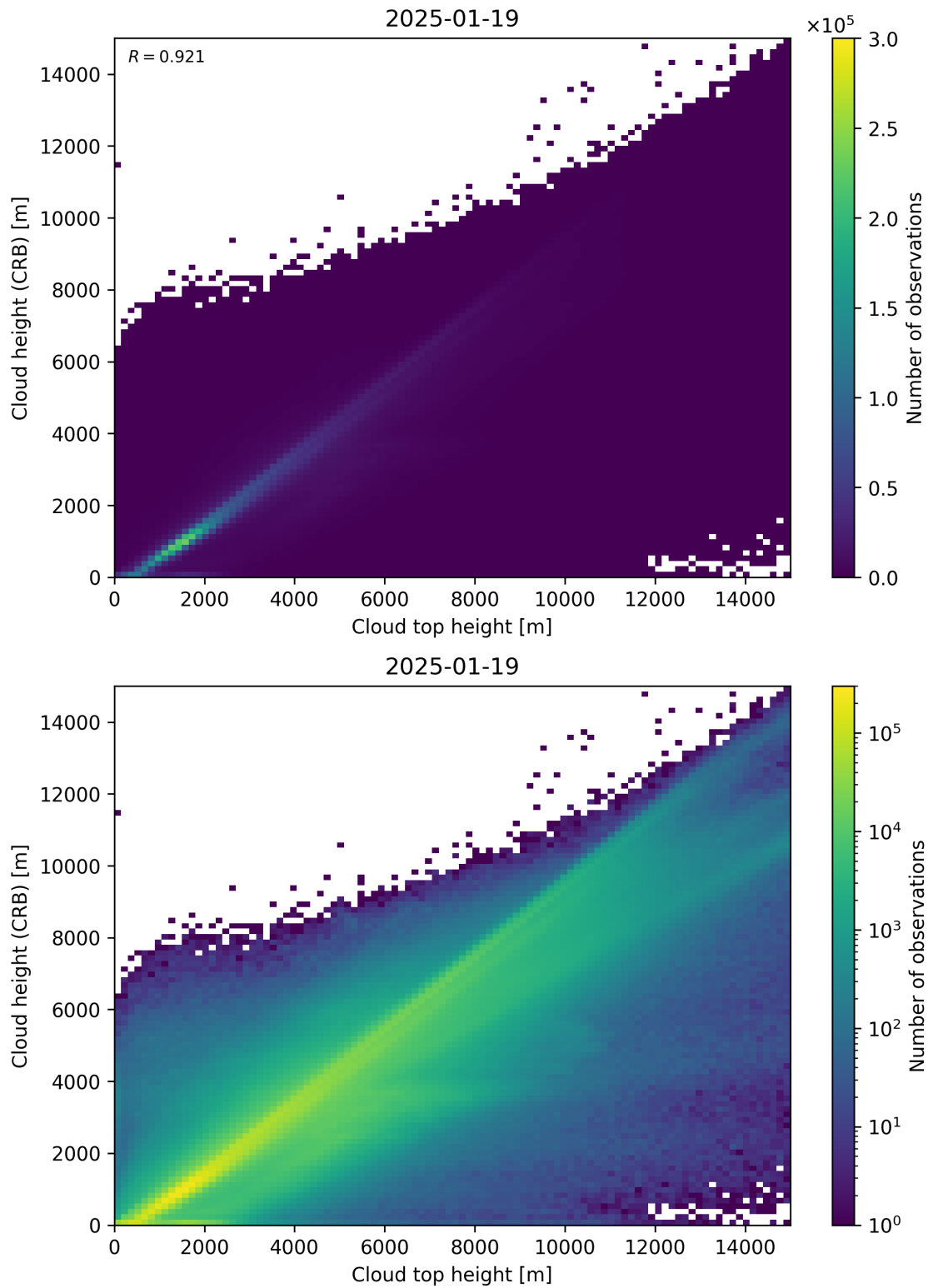
Figure 89: Scatter density plot of “Cloud top height” against “Cloud height (CRB)” for 2025-01-18 to 2025-01-20.
