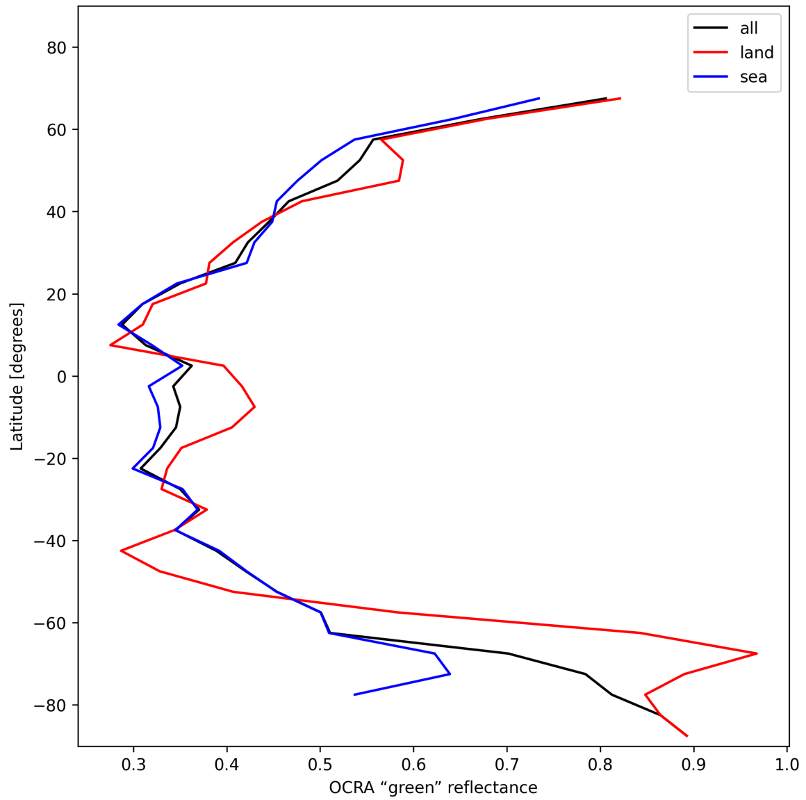
Figure 36: Zonal average of "OCRA "green" reflectance" for 2025-01-18 to 2025-01-20.
