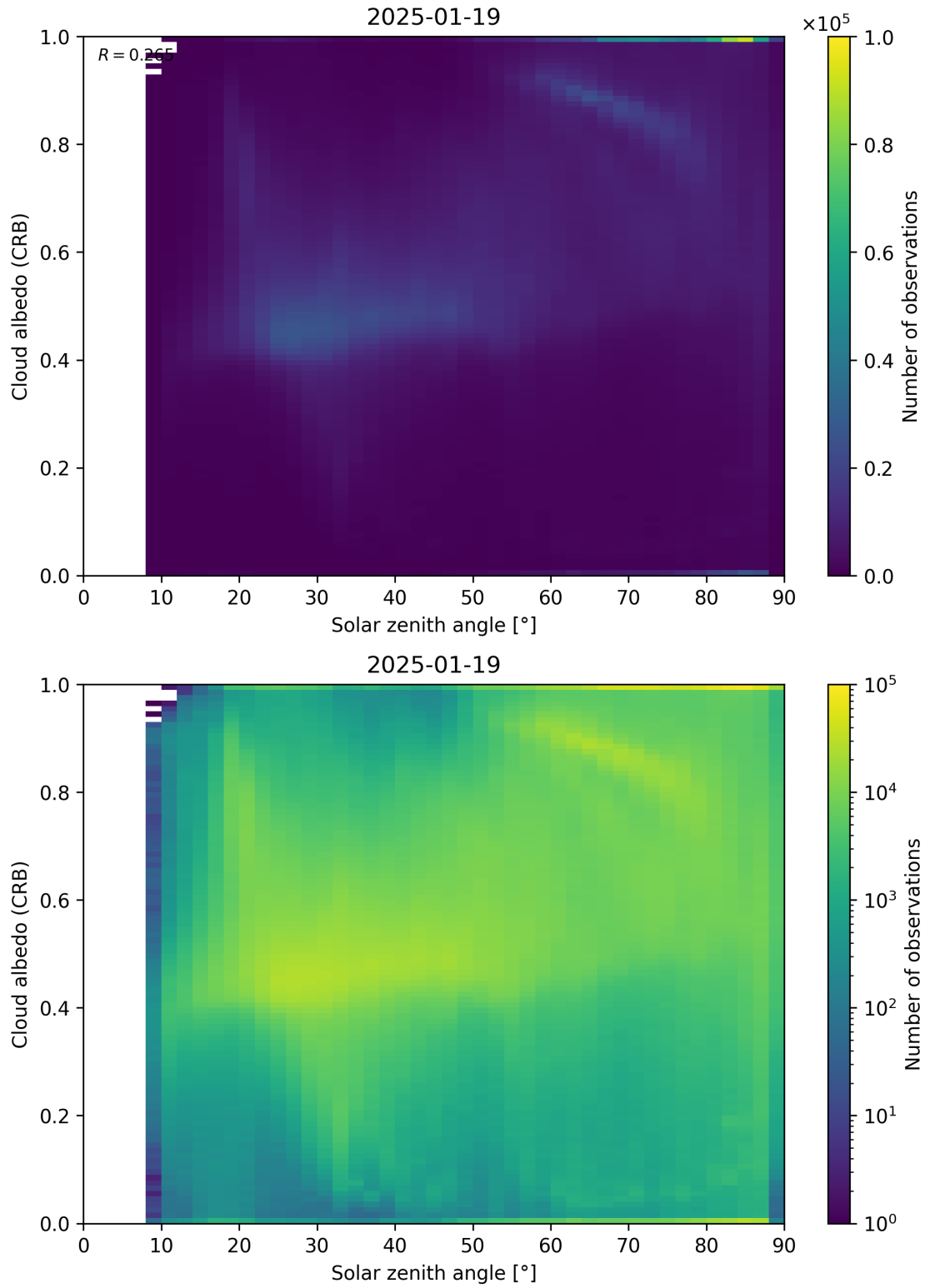
Figure 98: Scatter density plot of “Solar zenith angle” against “Cloud albedo (CRB)” for 2025-01-18 to 2025-01-20.
