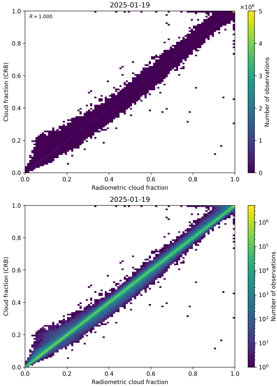
Figure 73: Scatter density plot of “Radiometric cloud fraction” against “Cloud fraction (CRB)” for 2025-01-18 to 2025-01-20.
