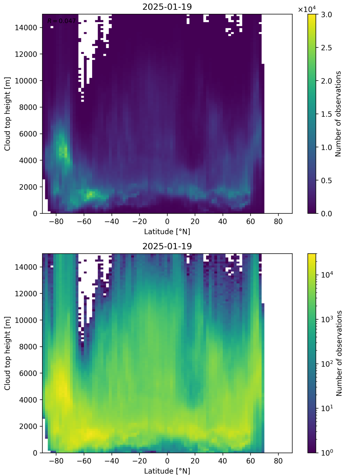
Figure 97: Scatter density plot of “Latitude” against “Cloud top height” for 2025-01-18 to 2025-01-20.
