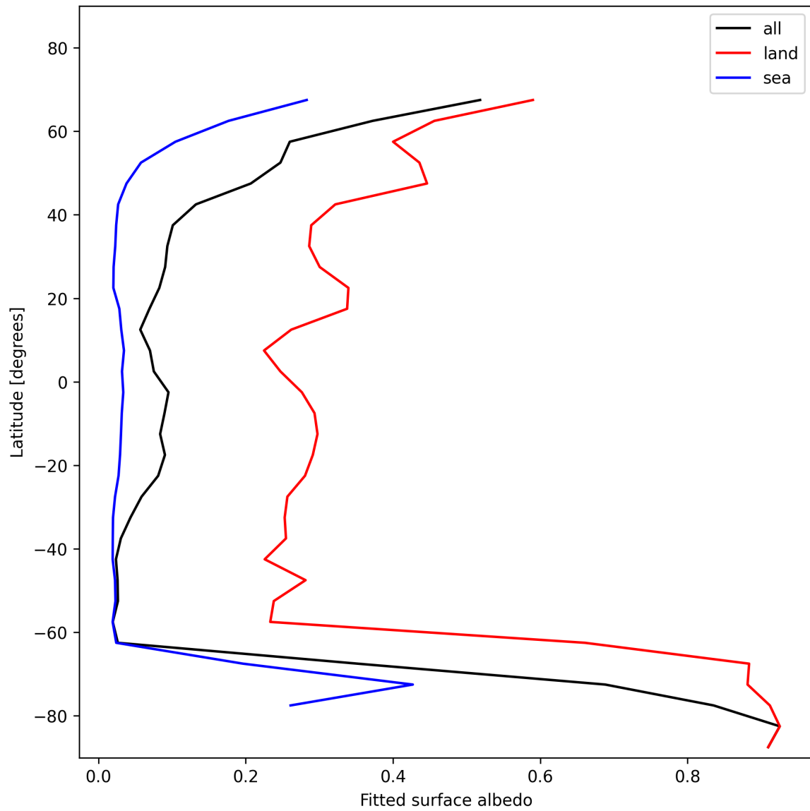
Figure 29: Zonal average of “Fitted surface albedo” for 2025-01-18 to 2025-01-20.
