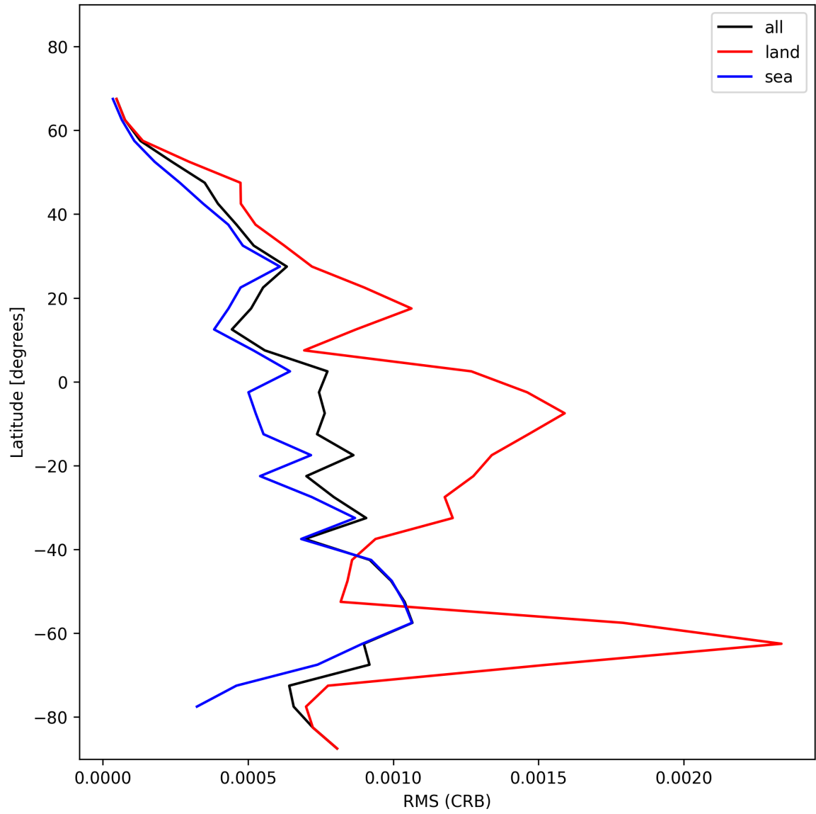
Figure 32: Zonal average of “RMS (CRB)” for 2025-01-18 to 2025-01-20.
