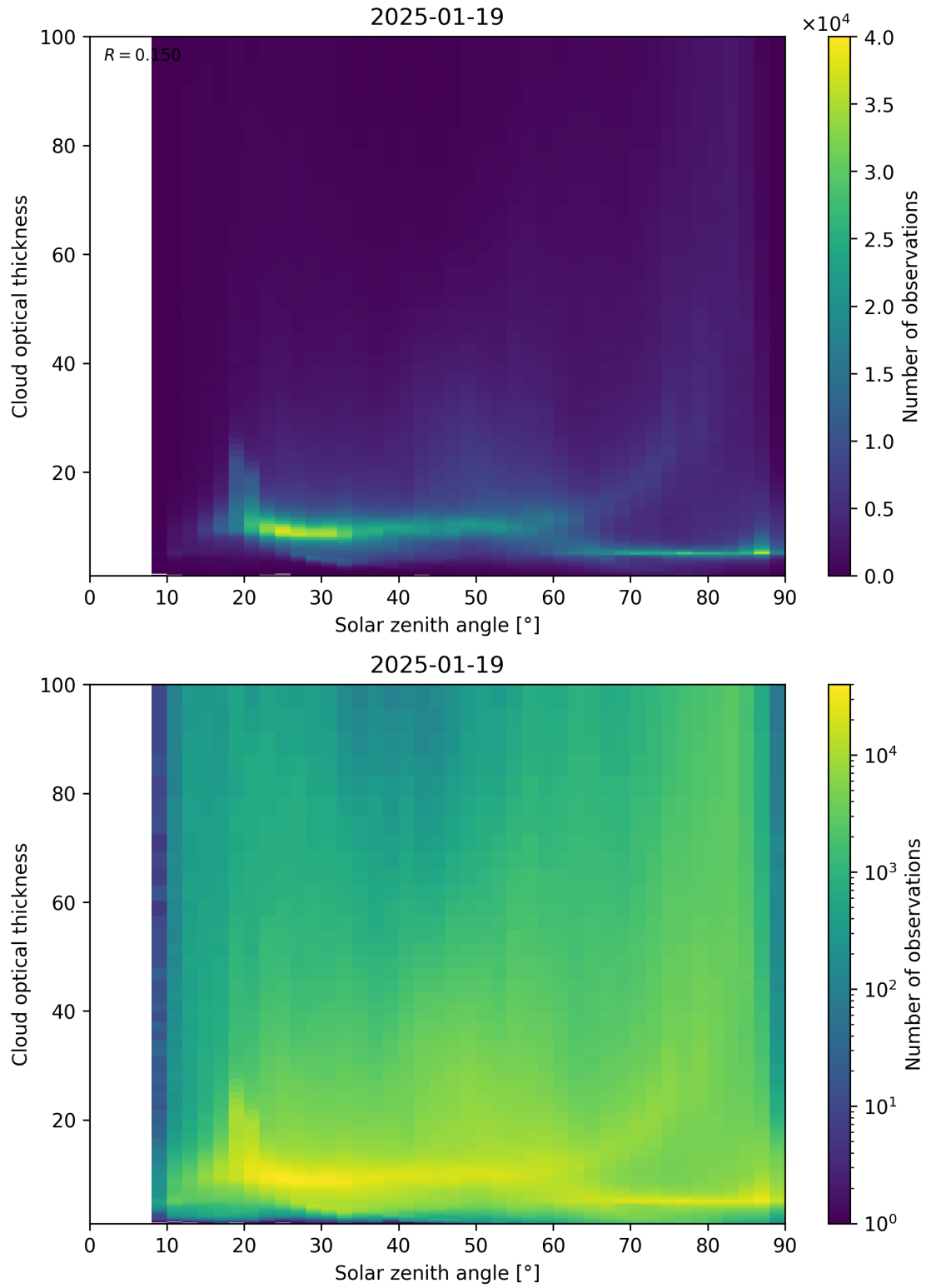
Figure 103: Scatter density plot of “Solar zenith angle” against “Cloud optical thickness” for 2025-01-18 to 2025-01-20.
