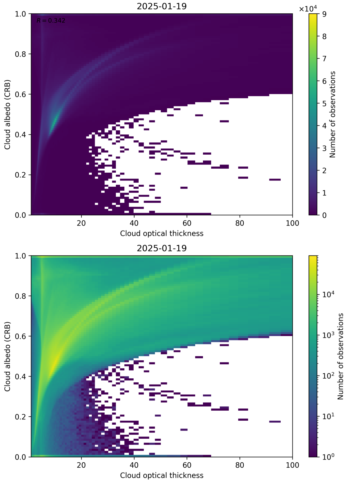
Figure 82: Scatter density plot of “Cloud optical thickness” against “Cloud albedo (CRB)” for 2025-01-18 to 2025-01-20.
