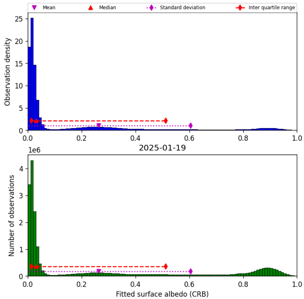
Figure 46: Histogram of “Fitted surface albedo (CRB)” for 2025-01-18 to 2025-01-20
