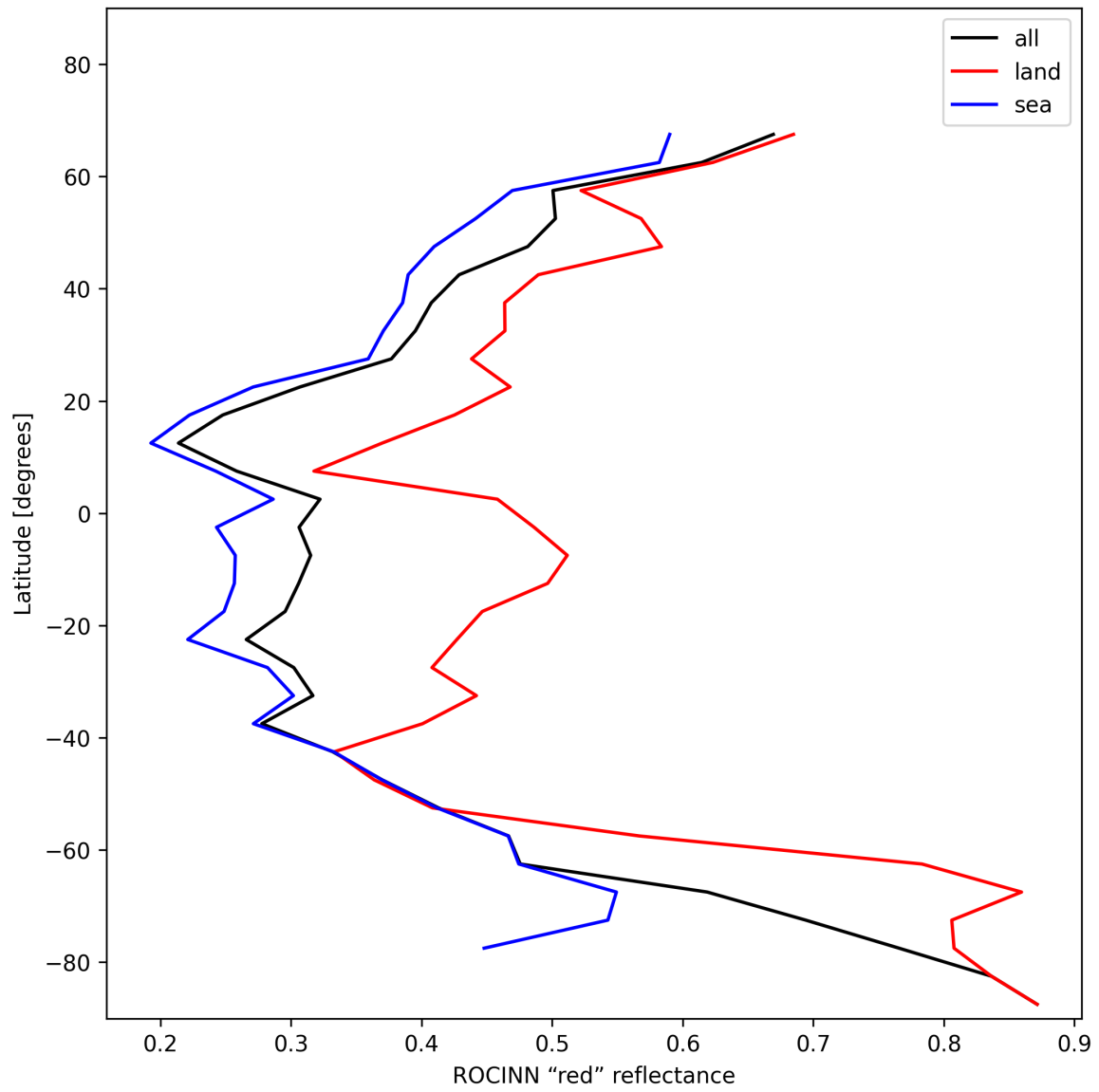
Figure 37: Zonal average of “ROCINN “red” reflectance” for 2025-01-18 to 2025-01-20.
