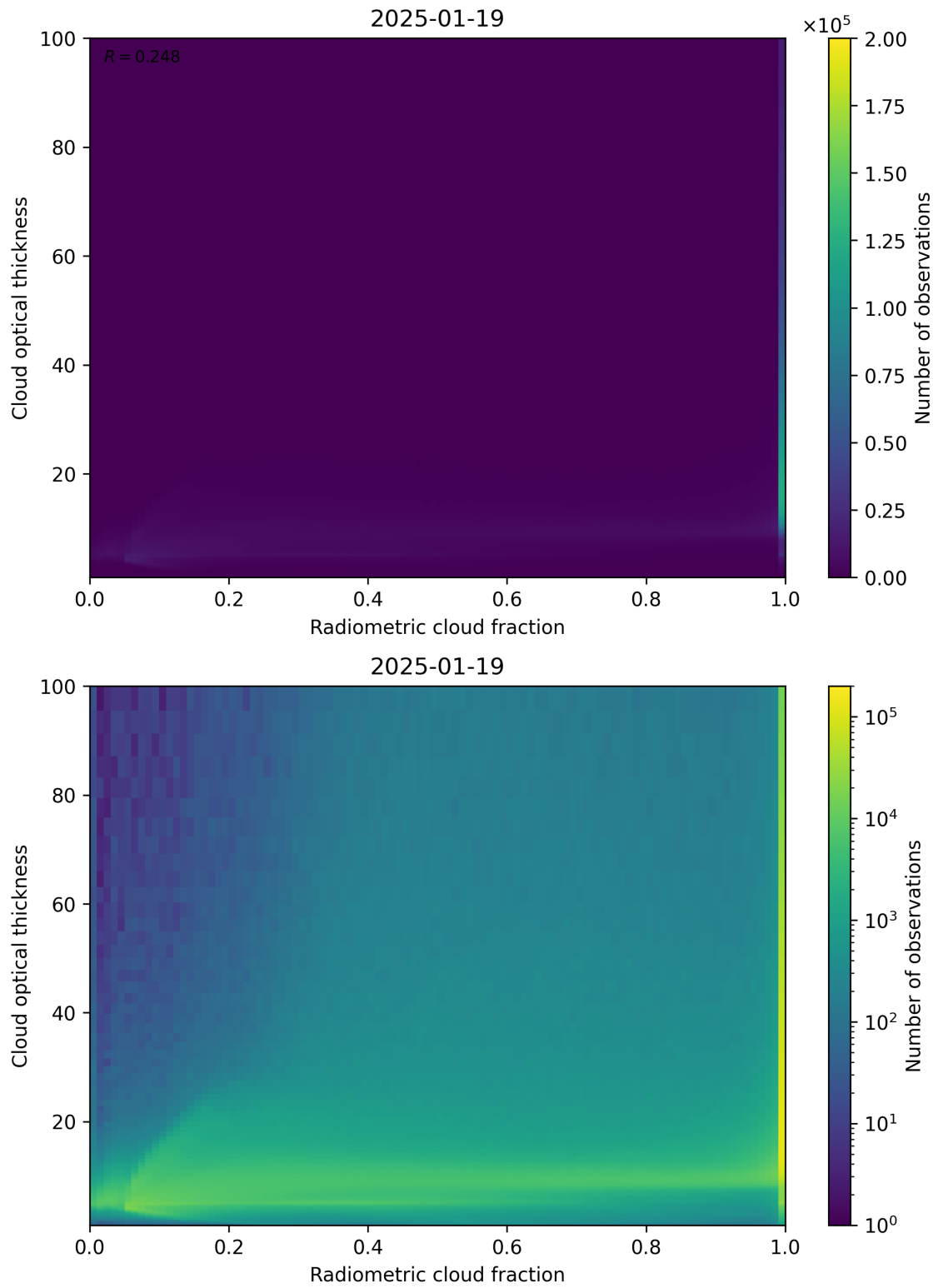
Figure 75: Scatter density plot of “Radiometric cloud fraction” against “Cloud optical thickness” for 2025-01-18 to 2025-01-20.
