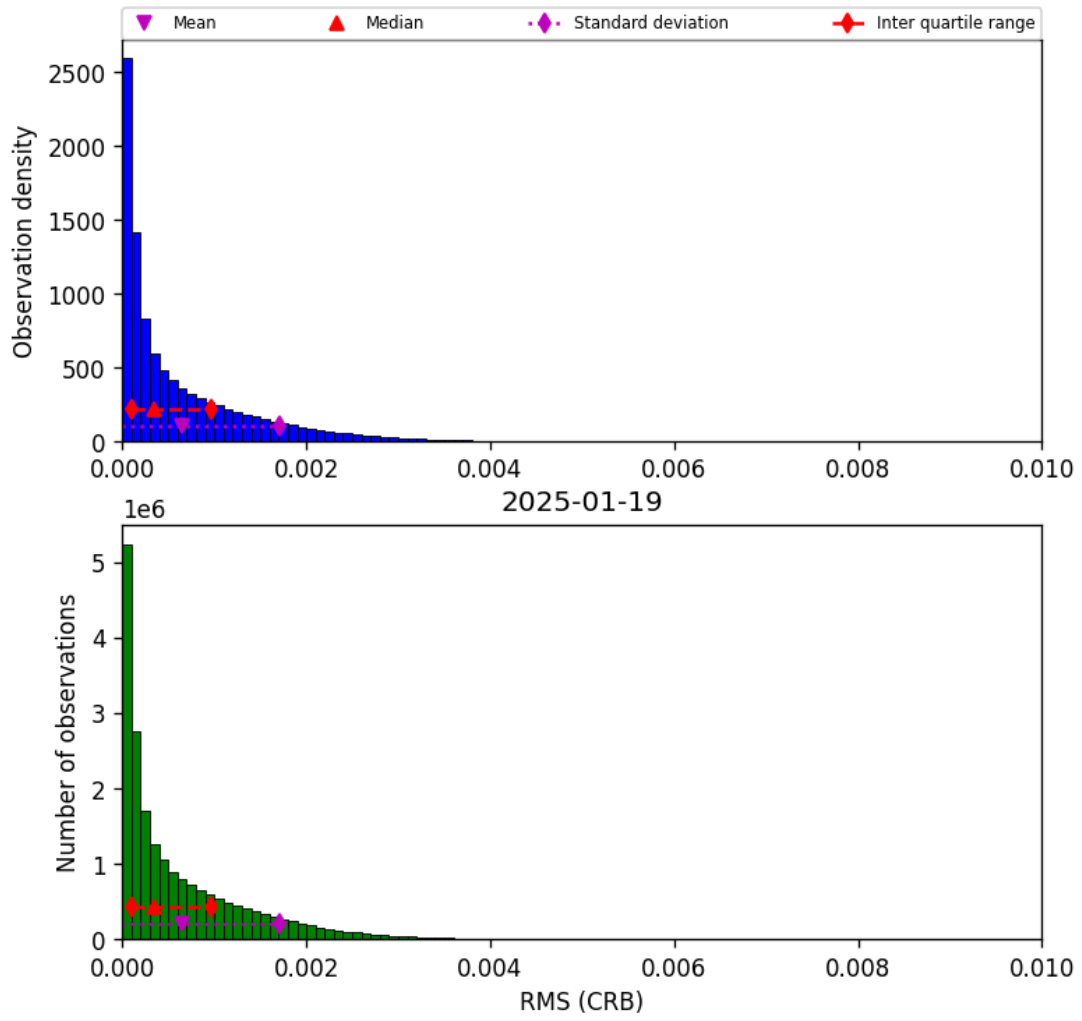
Figure 48: Histogram of “RMS (CRB)” for 2025-01-18 to 2025-01-20
