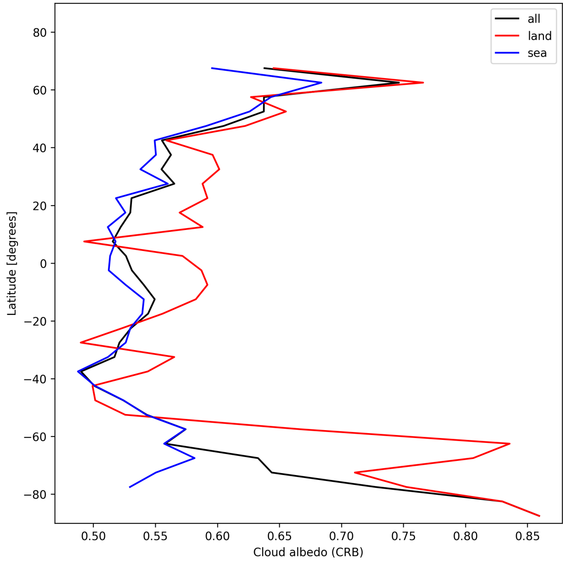
Figure 28: Zonal average of “Cloud albedo (CRB)” for 2025-01-18 to 2025-01-20.
