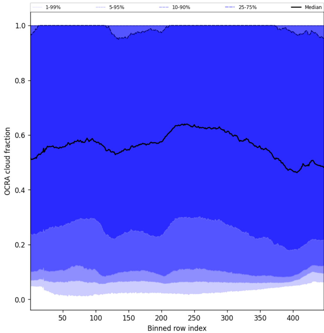
Figure 66: Along track statistics of “OCRA cloud fraction” for 2025-01-18 to 2025-01-20
