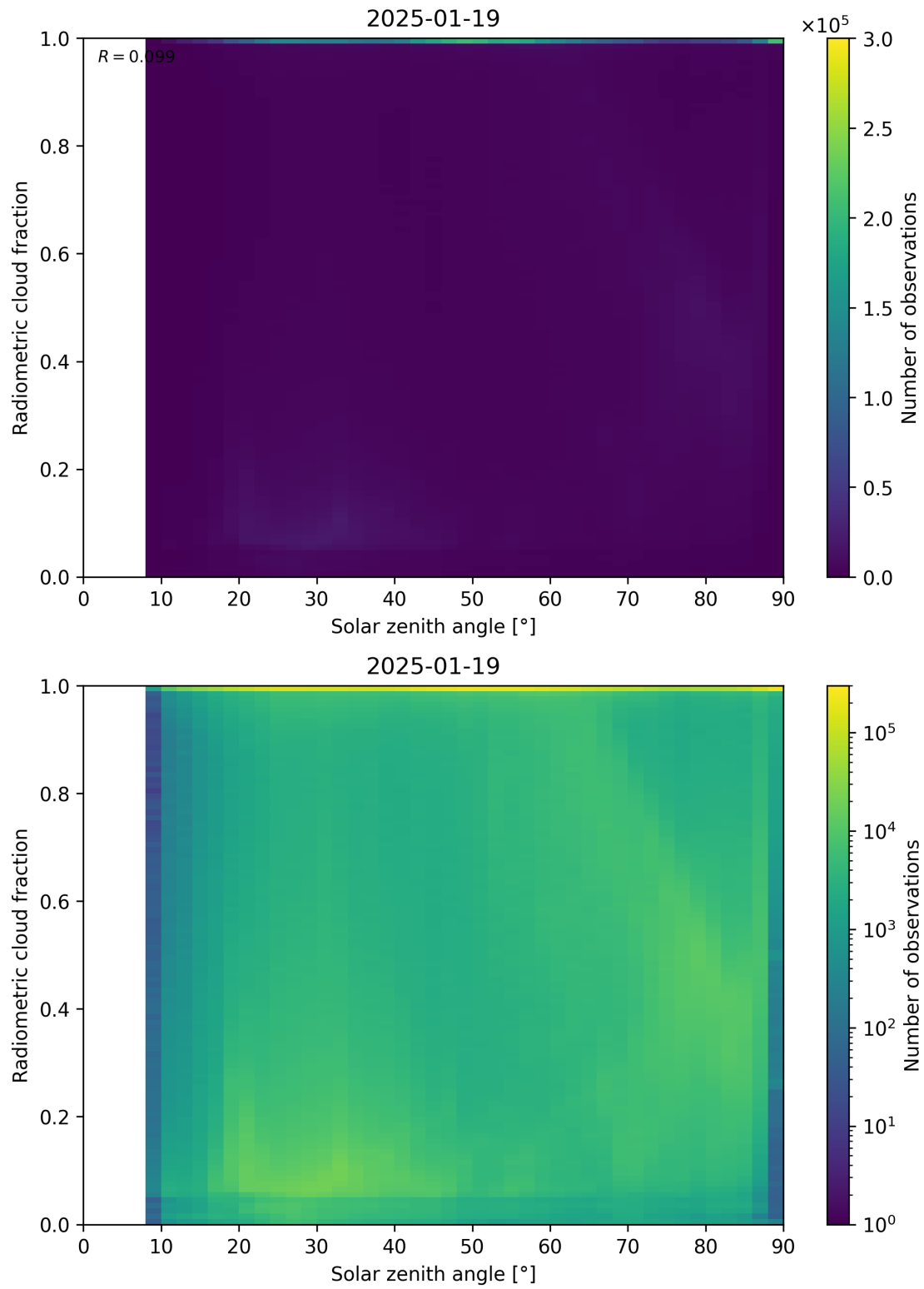
Figure 99: Scatter density plot of “Solar zenith angle” against “Radiometric cloud fraction” for 2025-01-18 to 2025-01-20.
