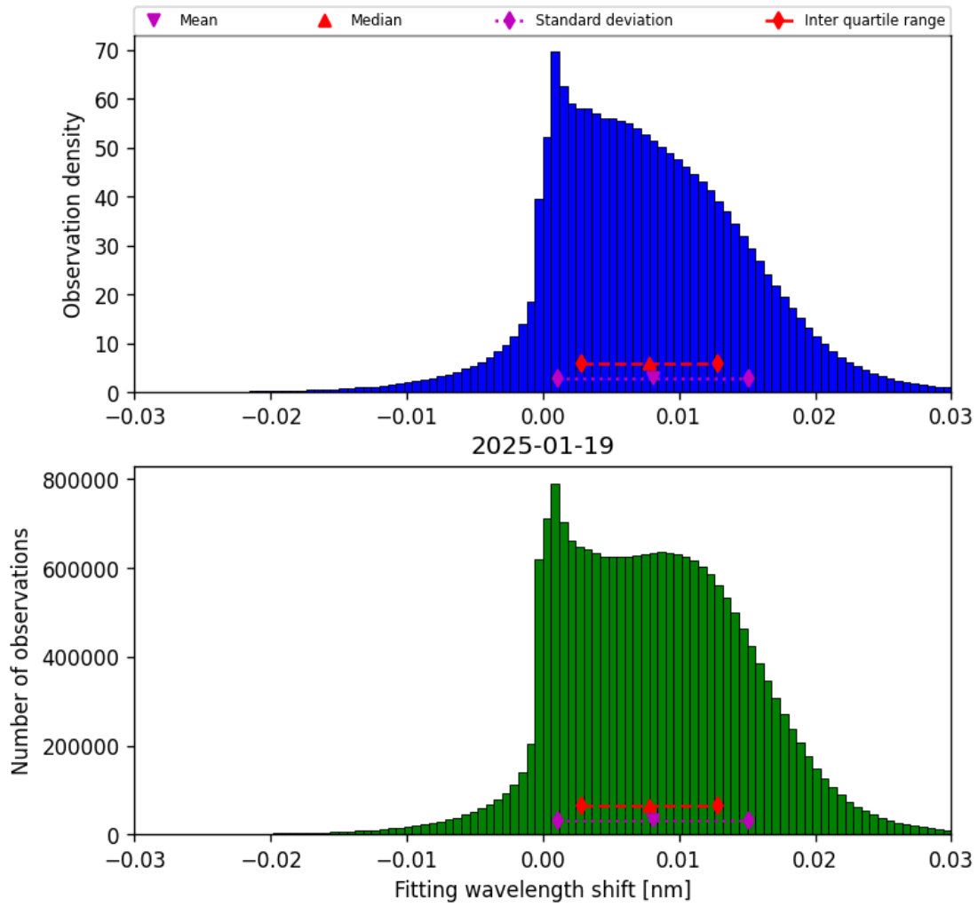
Figure 49: Histogram of “Fitting wavelength shift” for 2025-01-18 to 2025-01-20
