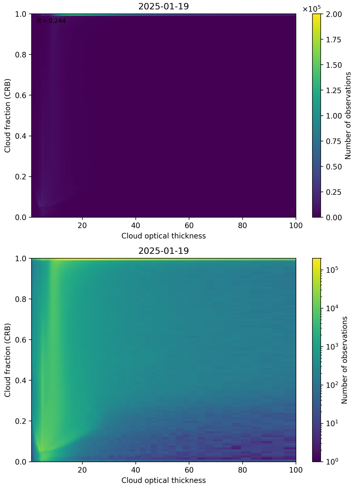
Figure 84: Scatter density plot of “Cloud optical thickness” against “Cloud fraction (CRB)” for 2025-01-18 to 2025-01-20.
