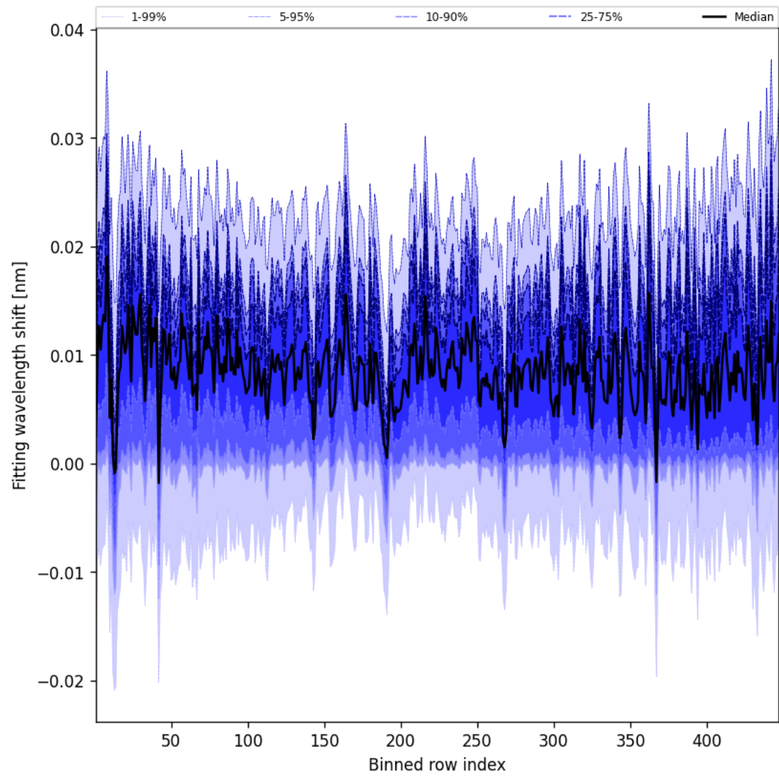
Figure 65: Along track statistics of “Fitting wavelength shift” for 2025-01-18 to 2025-01-20
