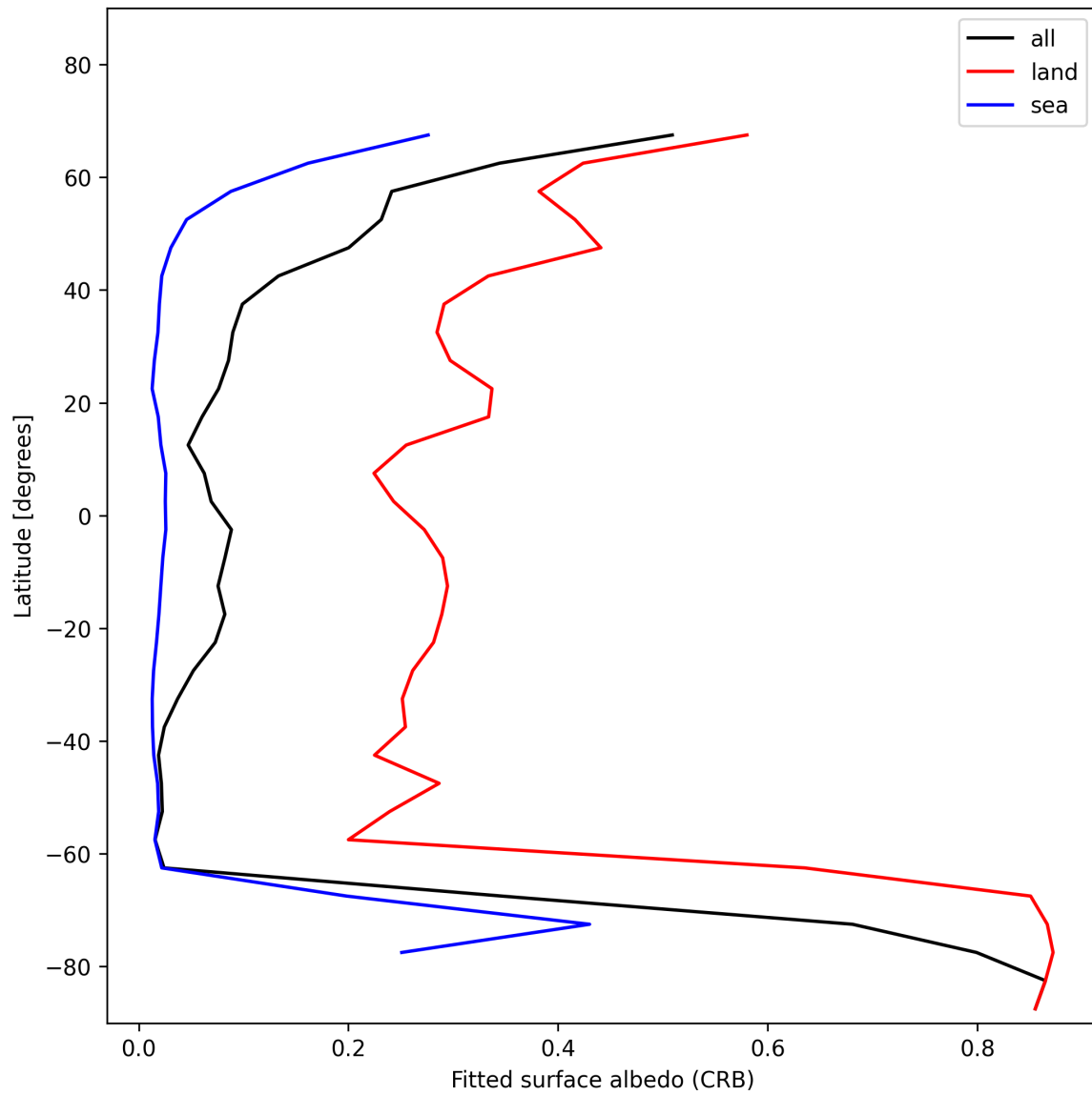
Figure 30: Zonal average of “Fitted surface albedo (CRB)” for 2025-01-18 to 2025-01-20.
