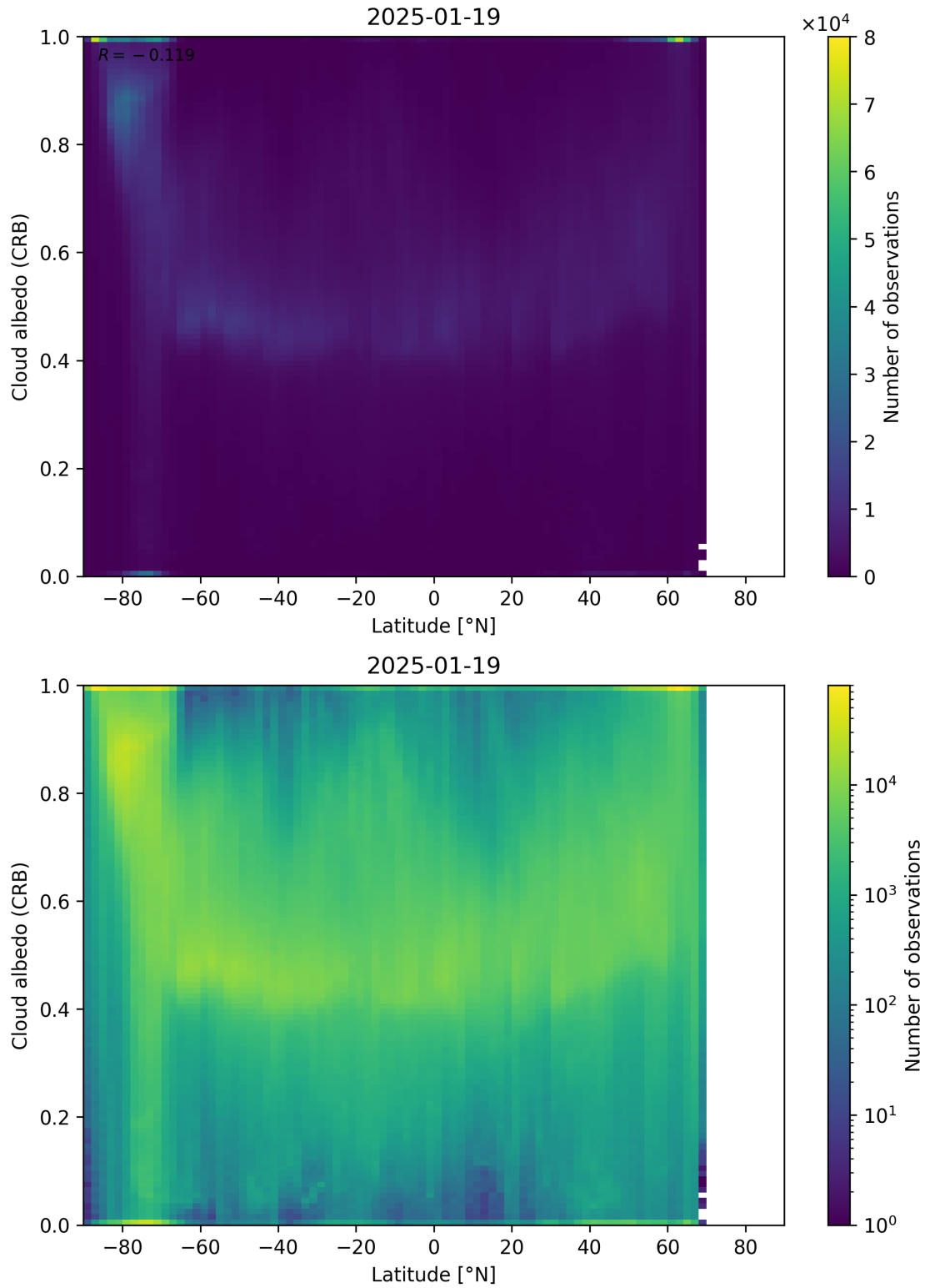
Figure 91: Scatter density plot of “Latitude” against “Cloud albedo (CRB)” for 2025-01-18 to 2025-01-20.
