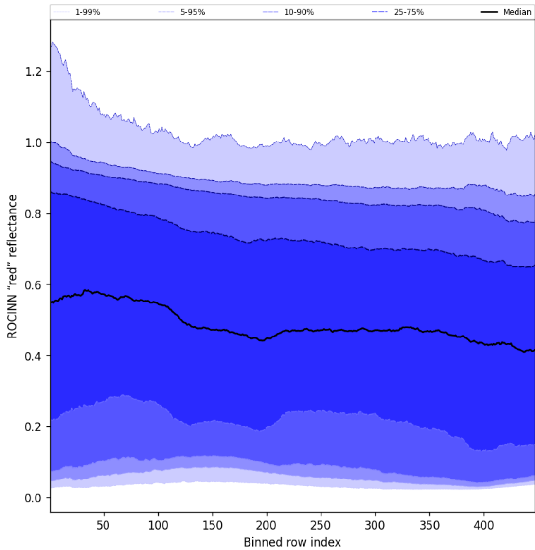
Figure 69: Along track statistics of “ROCINN “red” reflectance” for 2025-01-18 to 2025-01-20
