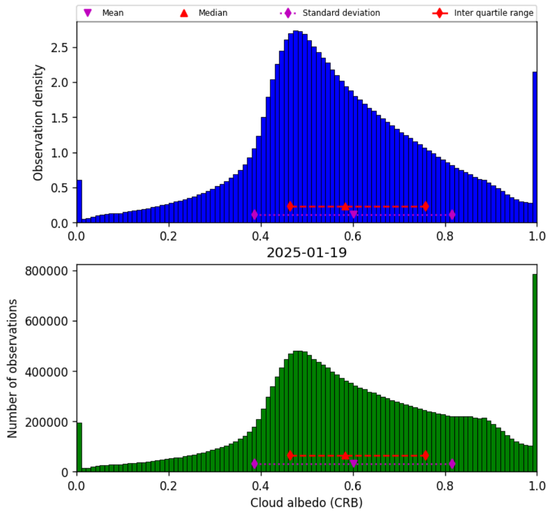
Figure 44: Histogram of “Cloud albedo (CRB)” for 2025-01-18 to 2025-01-20
