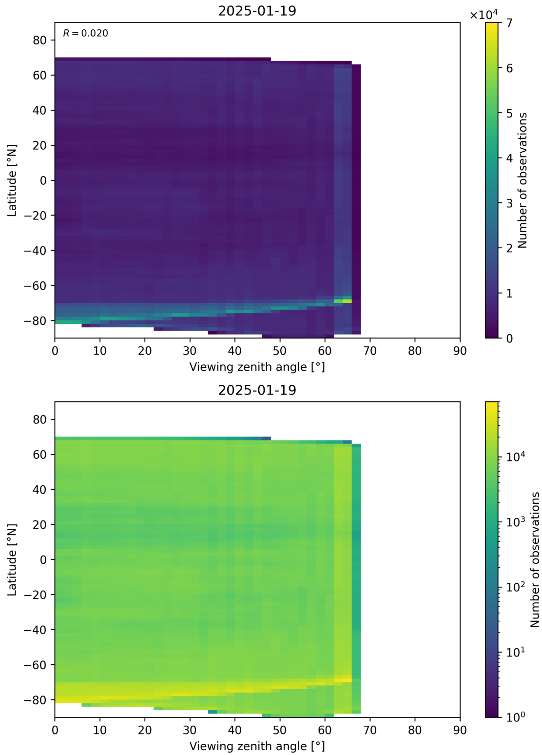
Figure 113: Scatter density plot of “Viewing zenith angle” against “Latitude” for 2025-01-18 to 2025-01-20.
