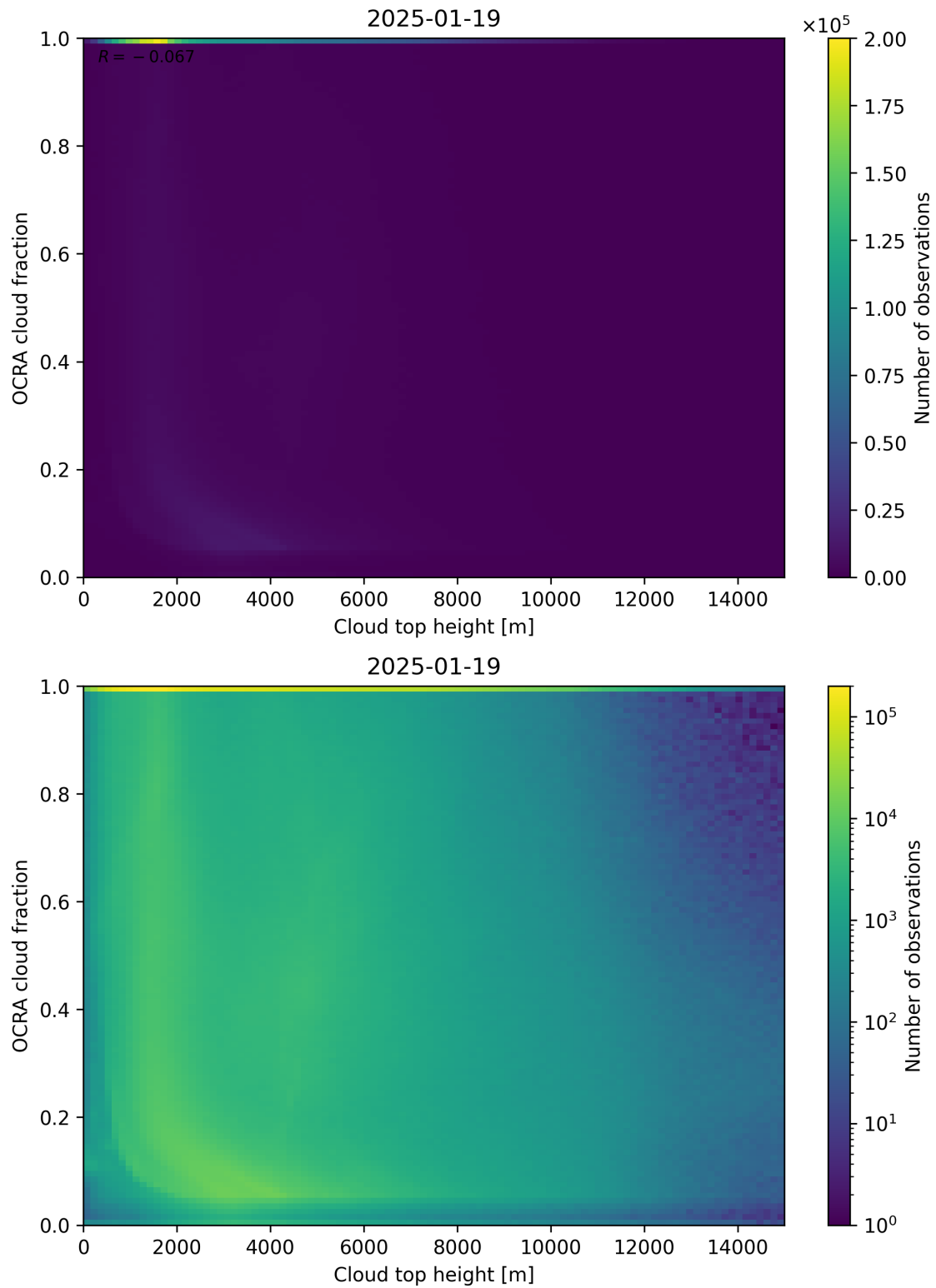
Figure 87: Scatter density plot of “Cloud top height” against “OCRA cloud fraction” for 2025-01-18 to 2025-01-20.
