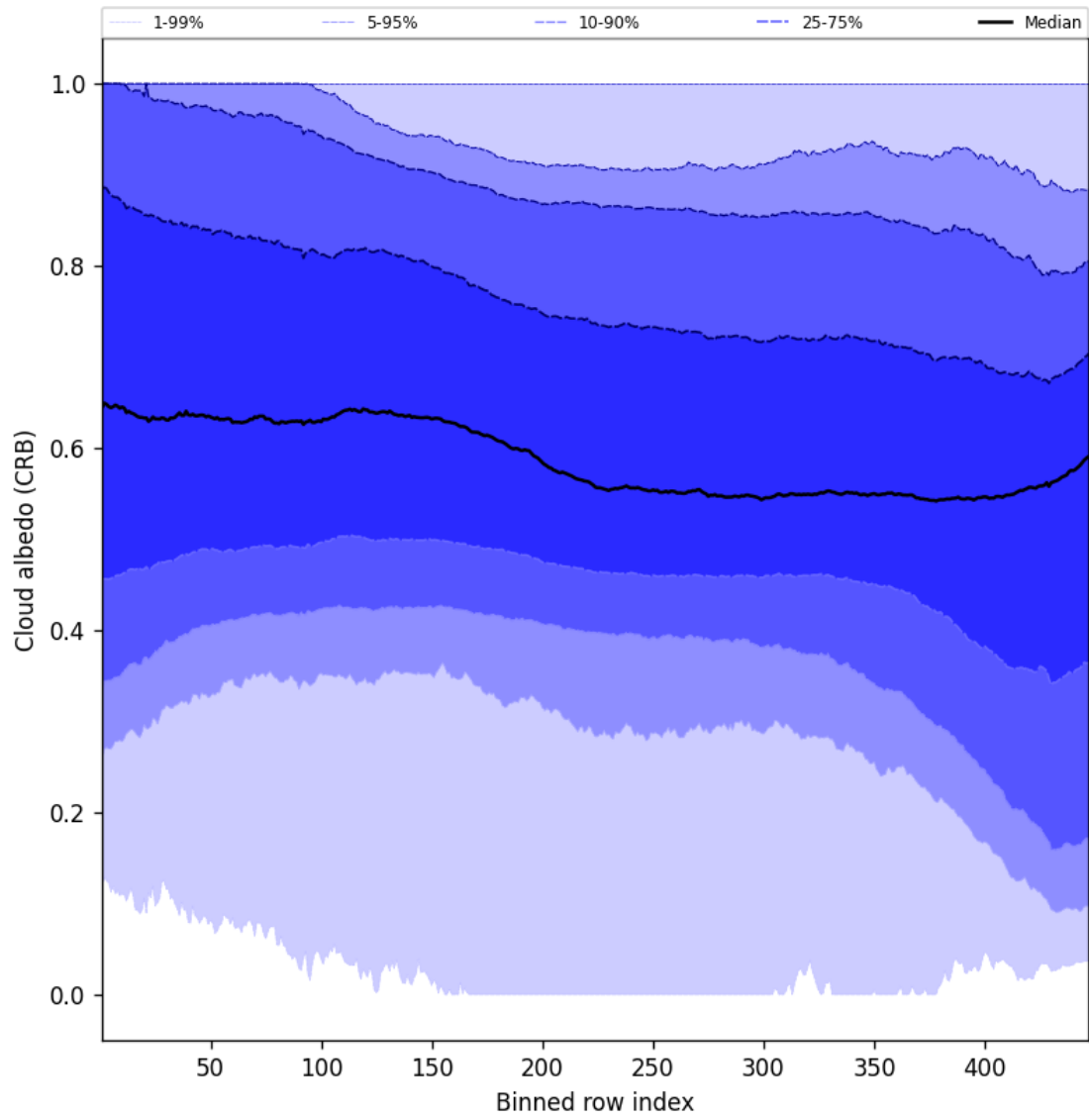
Figure 60: Along track statistics of “Cloud albedo (CRB)” for 2025-01-18 to 2025-01-20
