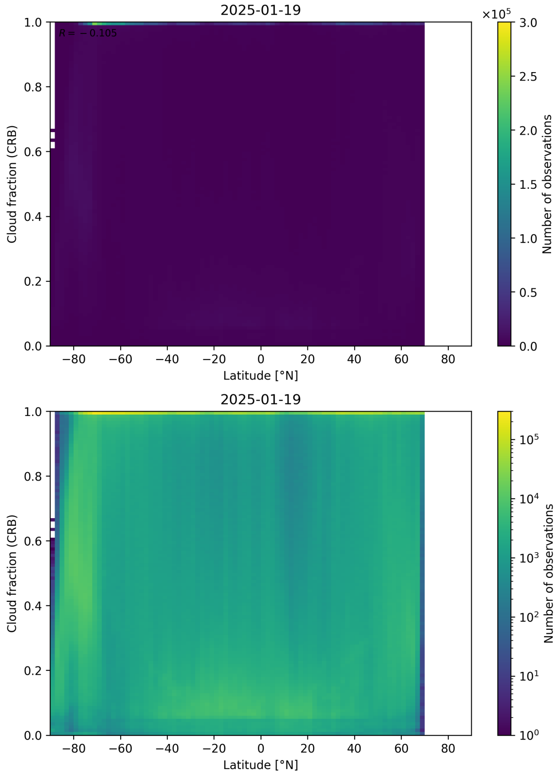
Figure 94: Scatter density plot of “Latitude” against “Cloud fraction (CRB)” for 2025-01-18 to 2025-01-20.
