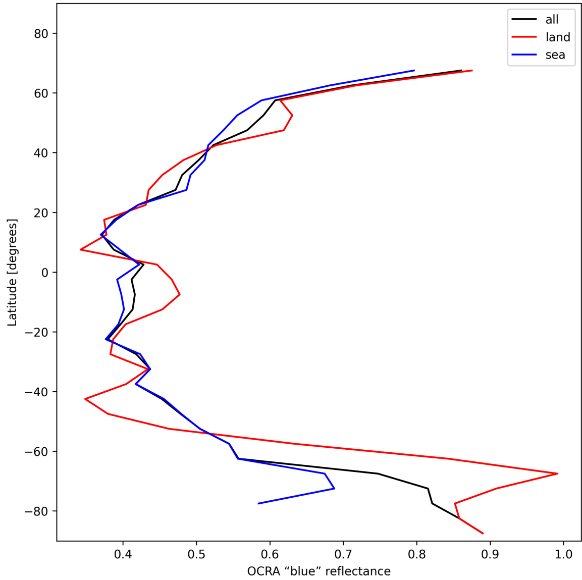
Figure 35: Zonal average of “OCRA “blue” reflectance” for 2025-01-18 to 2025-01-20.
