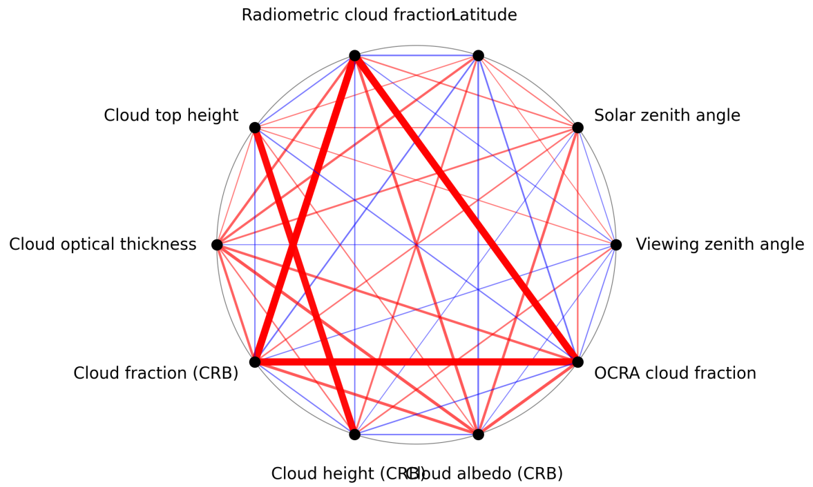
Figure 1: Map of correlation graph for 2025-01-18 to 2025-01-20.
