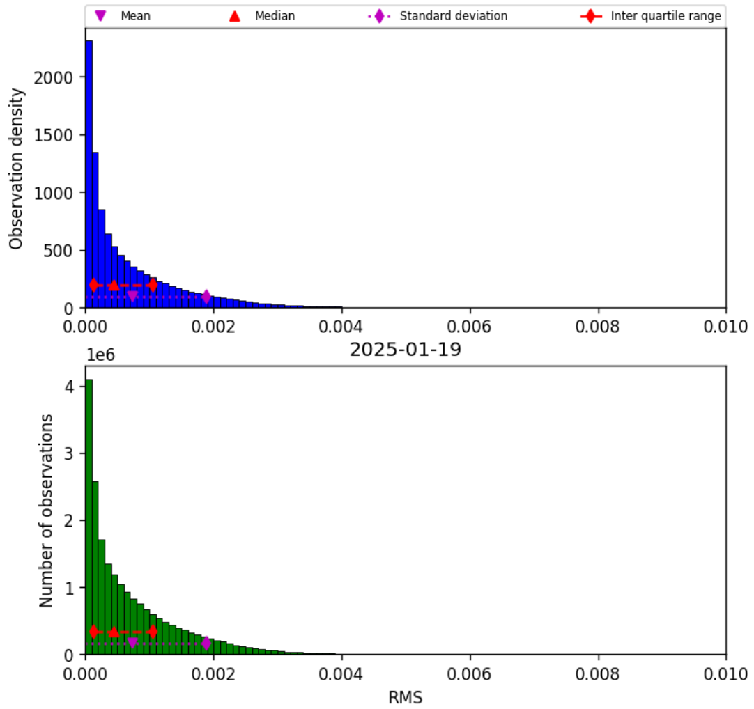
Figure 47: Histogram of “RMS” for 2025-01-18 to 2025-01-20
