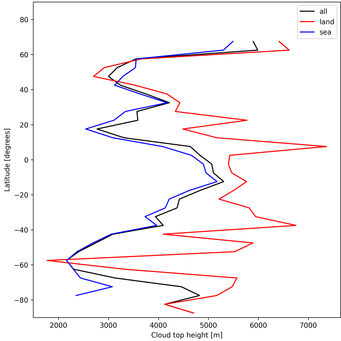
Figure 24: Zonal average of “Cloud top height” for 2025-01-18 to 2025-01-20.
