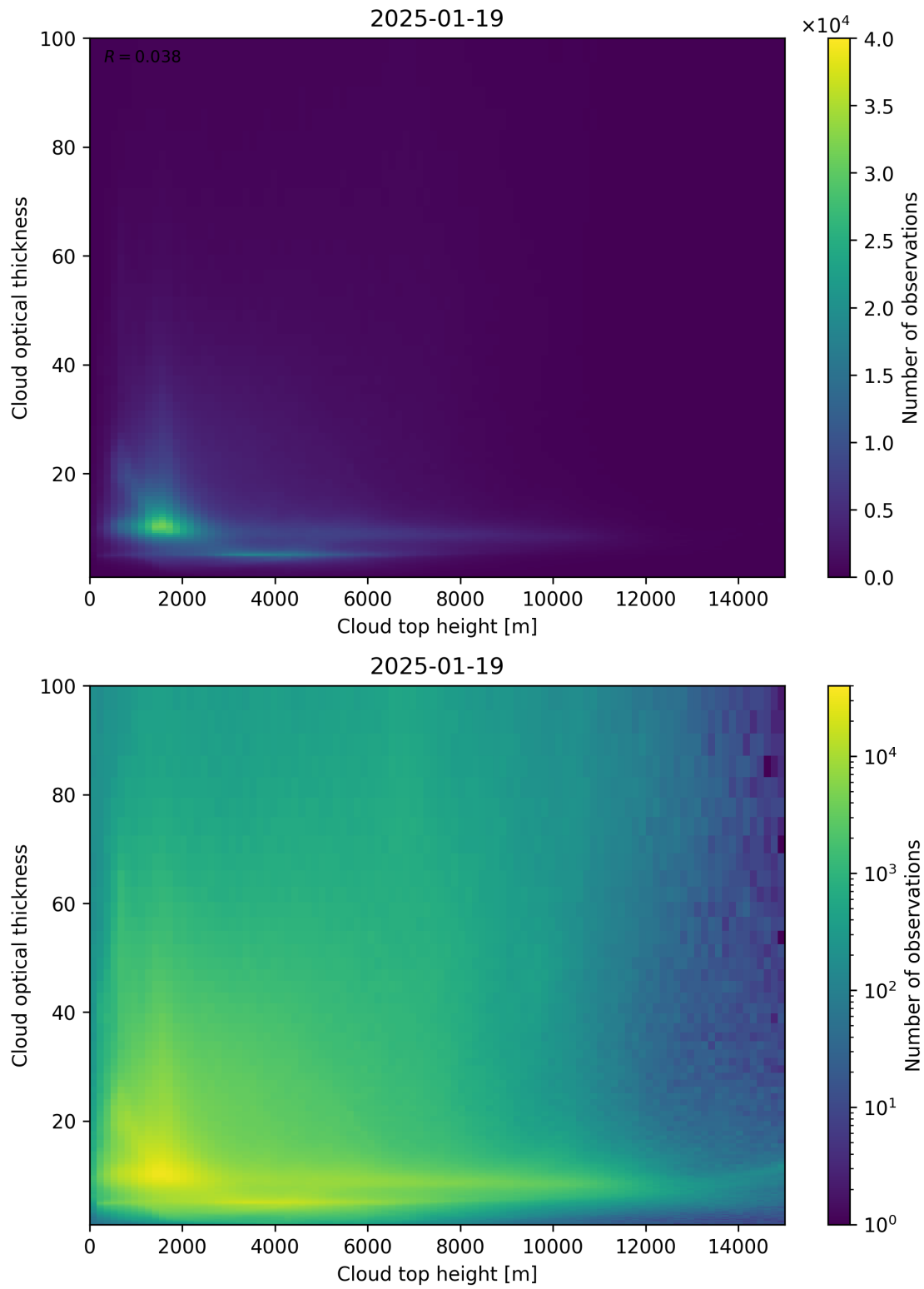
Figure 90: Scatter density plot of “Cloud top height” against “Cloud optical thickness” for 2025-01-18 to 2025-01-20.
