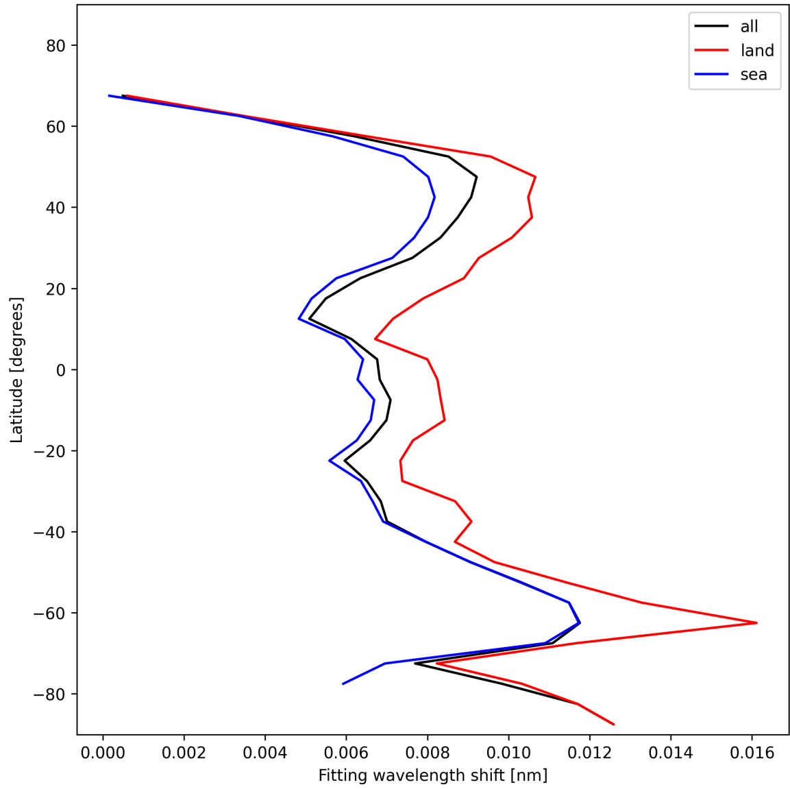
Figure 33: Zonal average of “Fitting wavelength shift” for 2025-01-18 to 2025-01-20.
