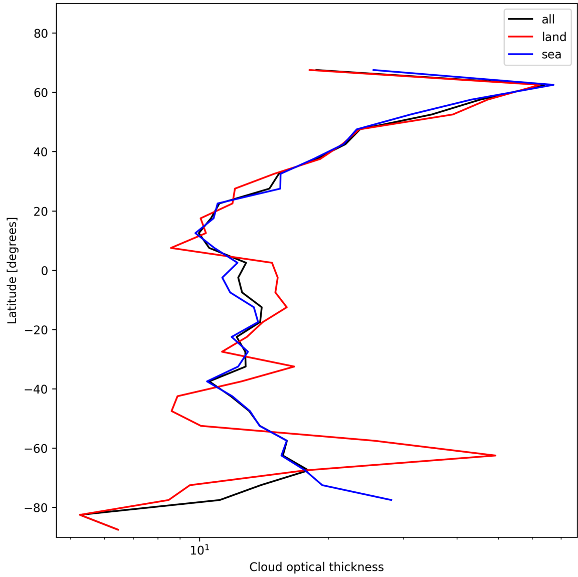
Figure 25: Zonal average of “Cloud optical thickness” for 2025-01-18 to 2025-01-20.
