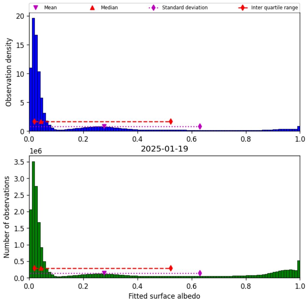
Figure 45: Histogram of “Fitted surface albedo” for 2025-01-18 to 2025-01-20
