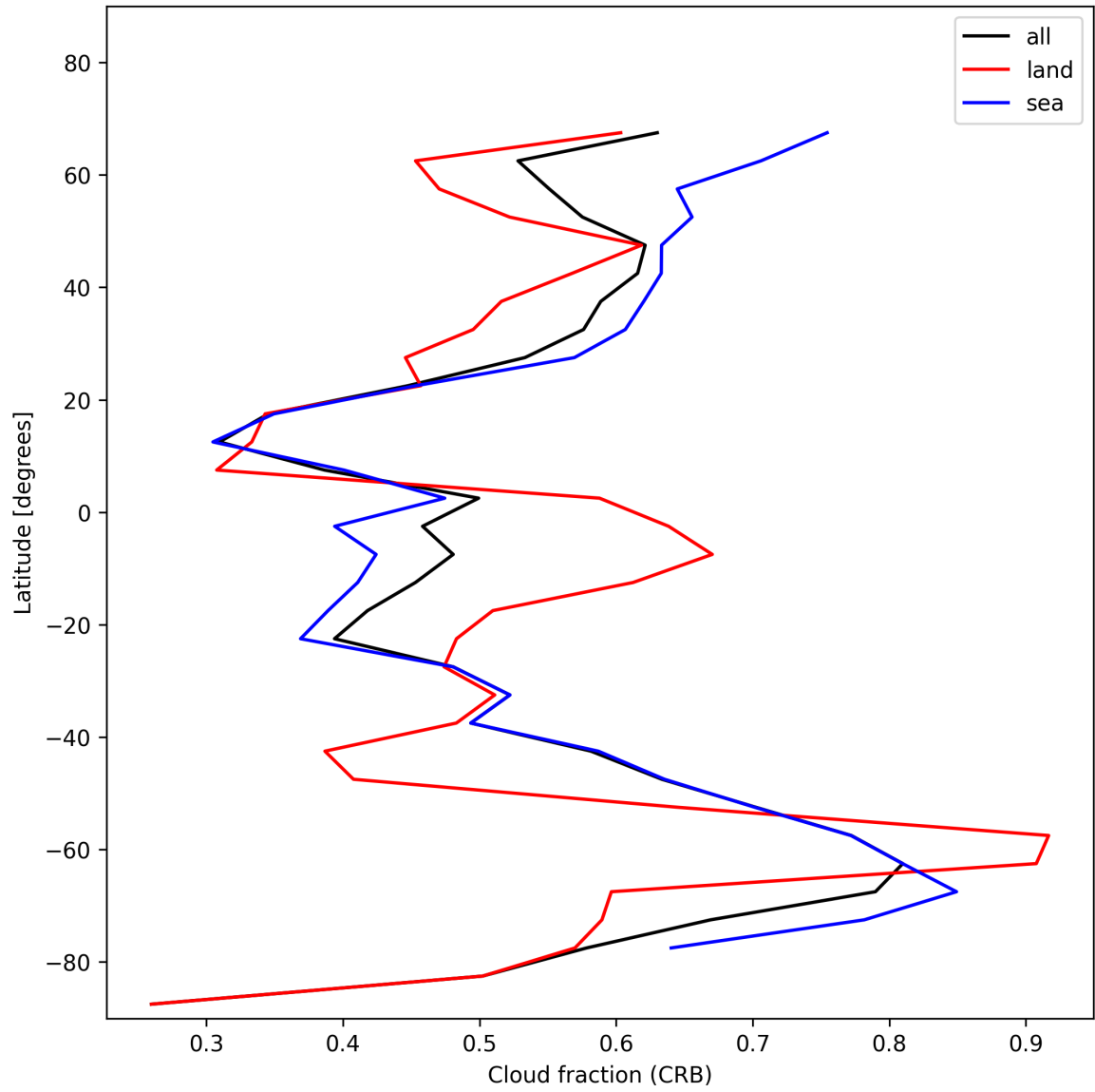
Figure 26: Zonal average of “Cloud fraction (CRB)” for 2025-01-18 to 2025-01-20.
