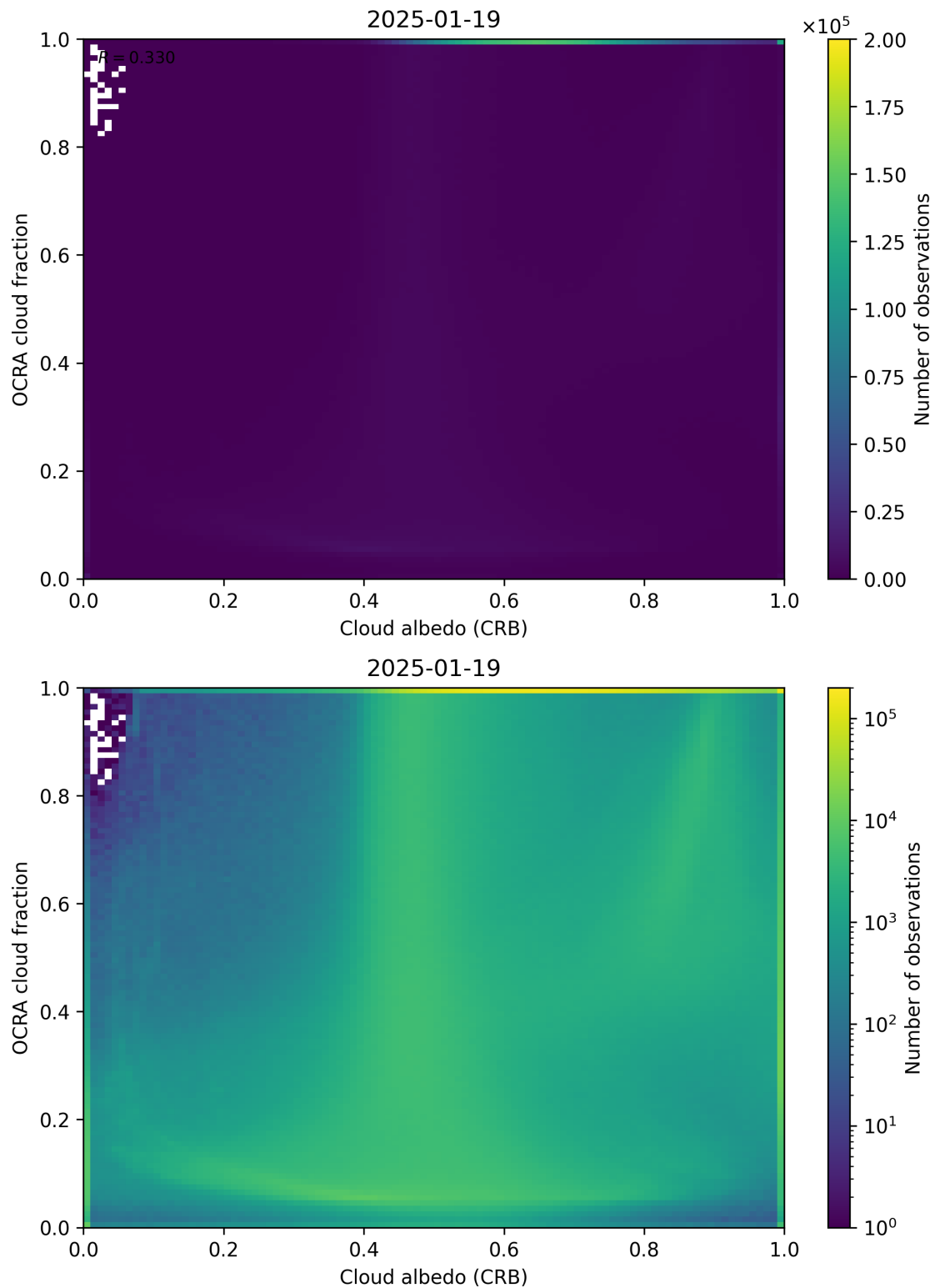
Figure 70: Scatter density plot of “Cloud albedo (CRB)” against “OCRA cloud fraction” for 2025-01-18 to 2025-01-20.
