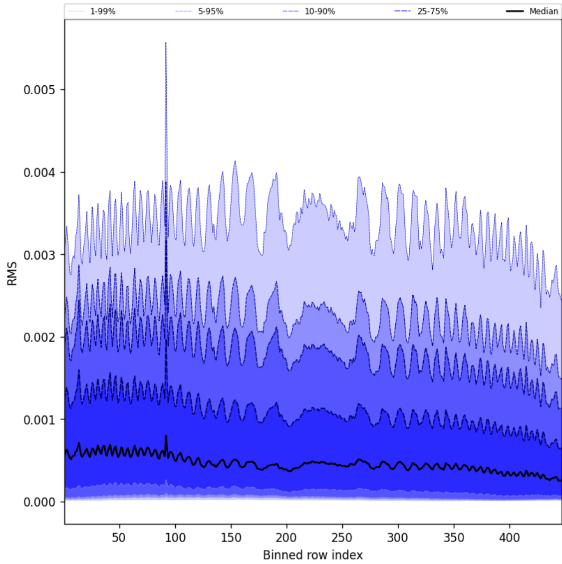
Figure 63: Along track statistics of “RMS” for 2025-01-18 to 2025-01-20
