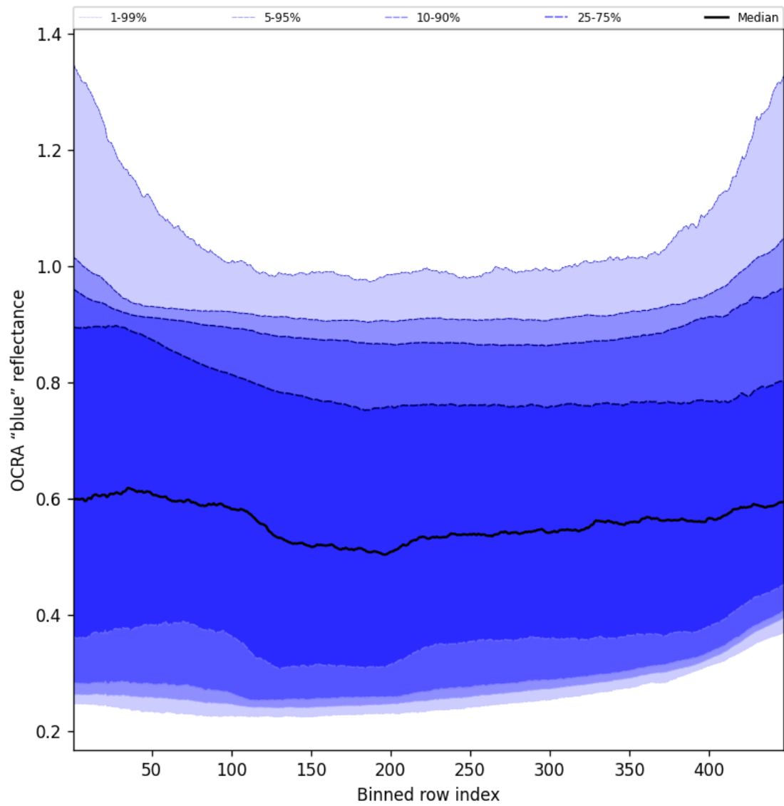
Figure 67: Along track statistics of “OCRA “blue” reflectance” for 2025-01-18 to 2025-01-20
