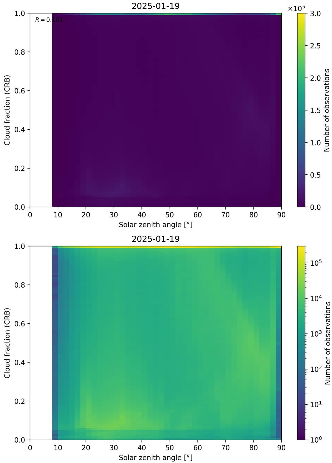
Figure 101: Scatter density plot of “Solar zenith angle” against “Cloud fraction (CRB)” for 2025-01-18 to 2025-01-20.
