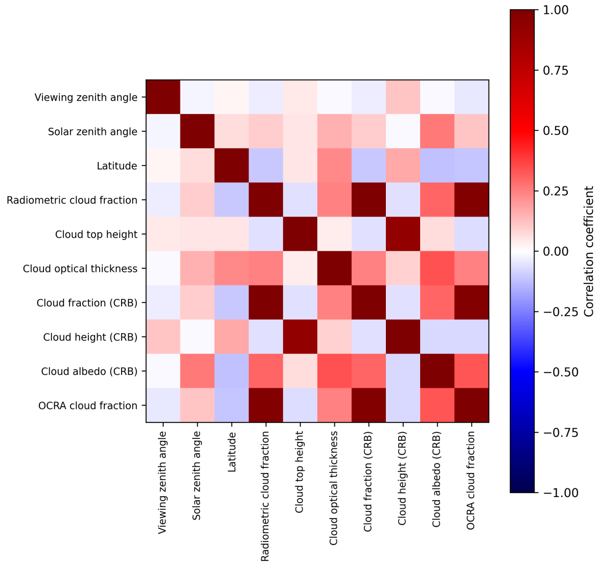
Figure 2: Map of correlation matrix for 2025-01-18 to 2025-01-20.
