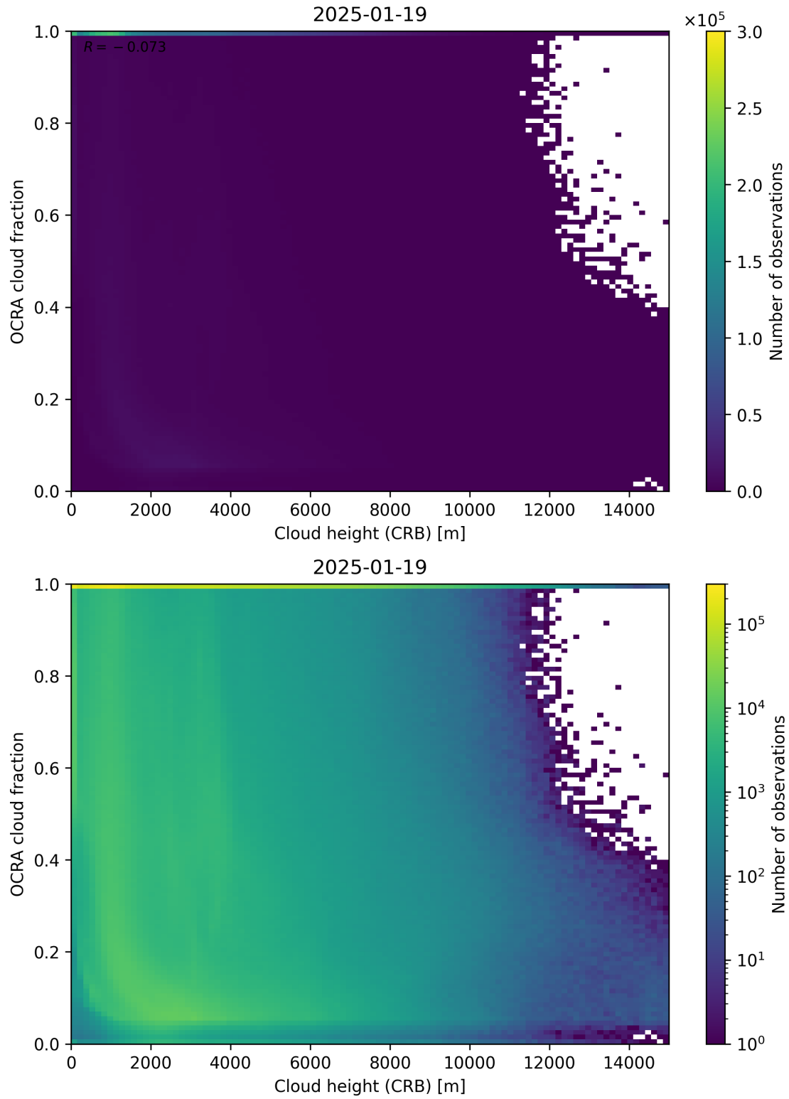
Figure 81: Scatter density plot of “Cloud height (CRB)” against “OCRA cloud fraction” for 2025-01-18 to 2025-01-20.
