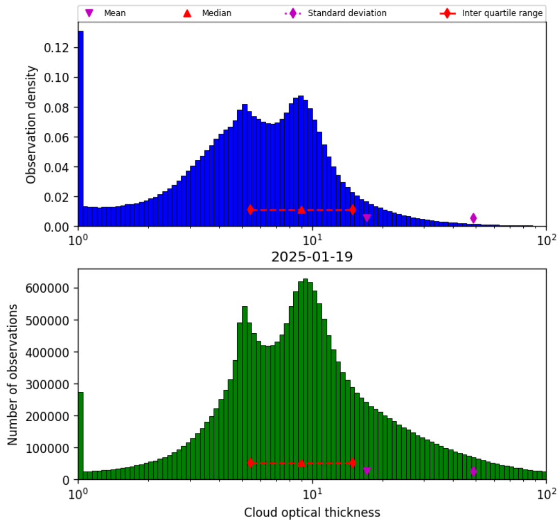
Figure 41: Histogram of “Cloud optical thickness” for 2025-01-18 to 2025-01-20
