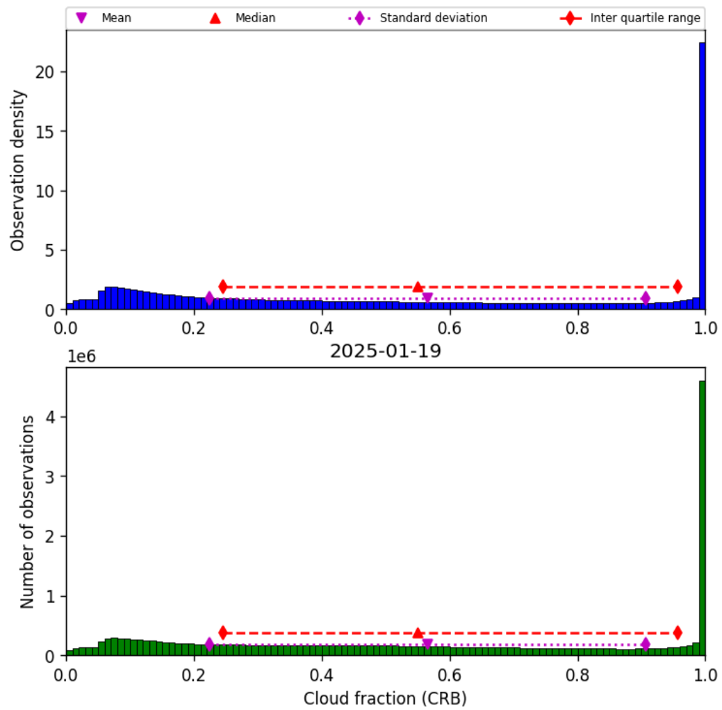
Figure 42: Histogram of “Cloud fraction (CRB)” for 2025-01-18 to 2025-01-20
