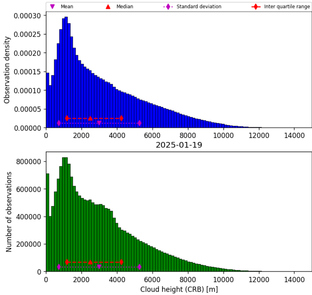
Figure 43: Histogram of “Cloud height (CRB)” for 2025-01-18 to 2025-01-20
