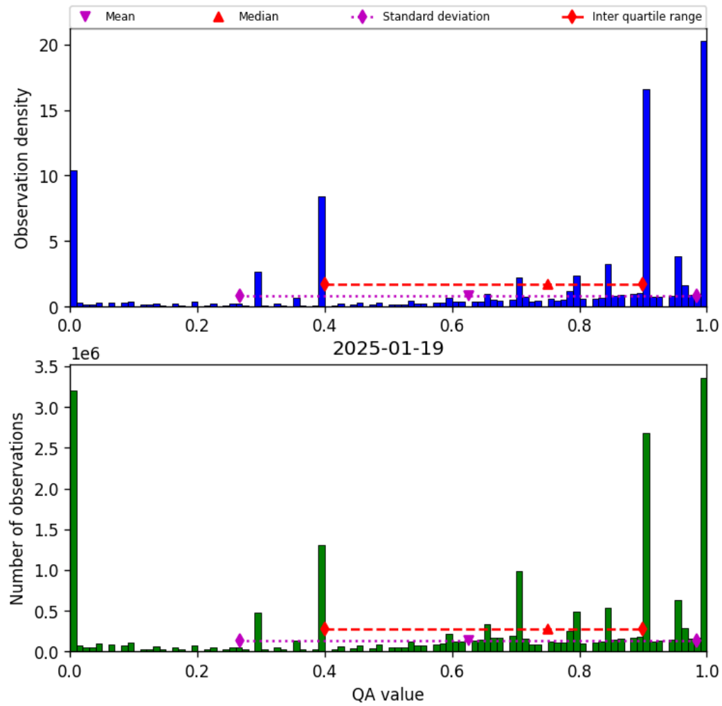
Figure 38: Histogram of “QA value” for 2025-01-18 to 2025-01-20
