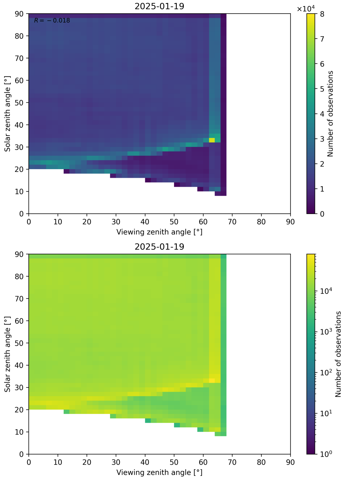
Figure 114: Scatter density plot of “Viewing zenith angle” against “Solar zenith angle” for 2025-01-18 to 2025-01-20.
