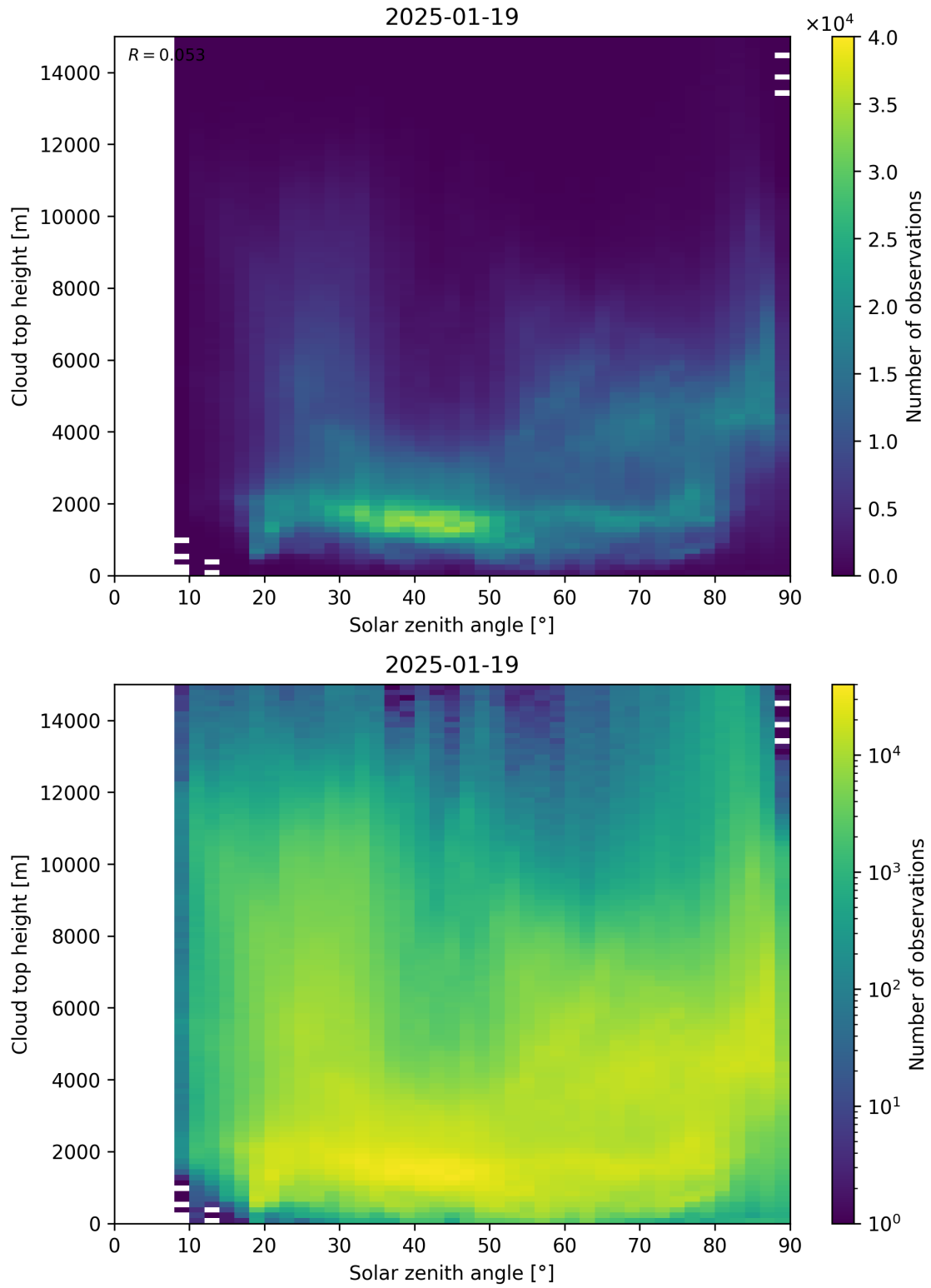
Figure 104: Scatter density plot of “Solar zenith angle” against “Cloud top height” for 2025-01-18 to 2025-01-20.
