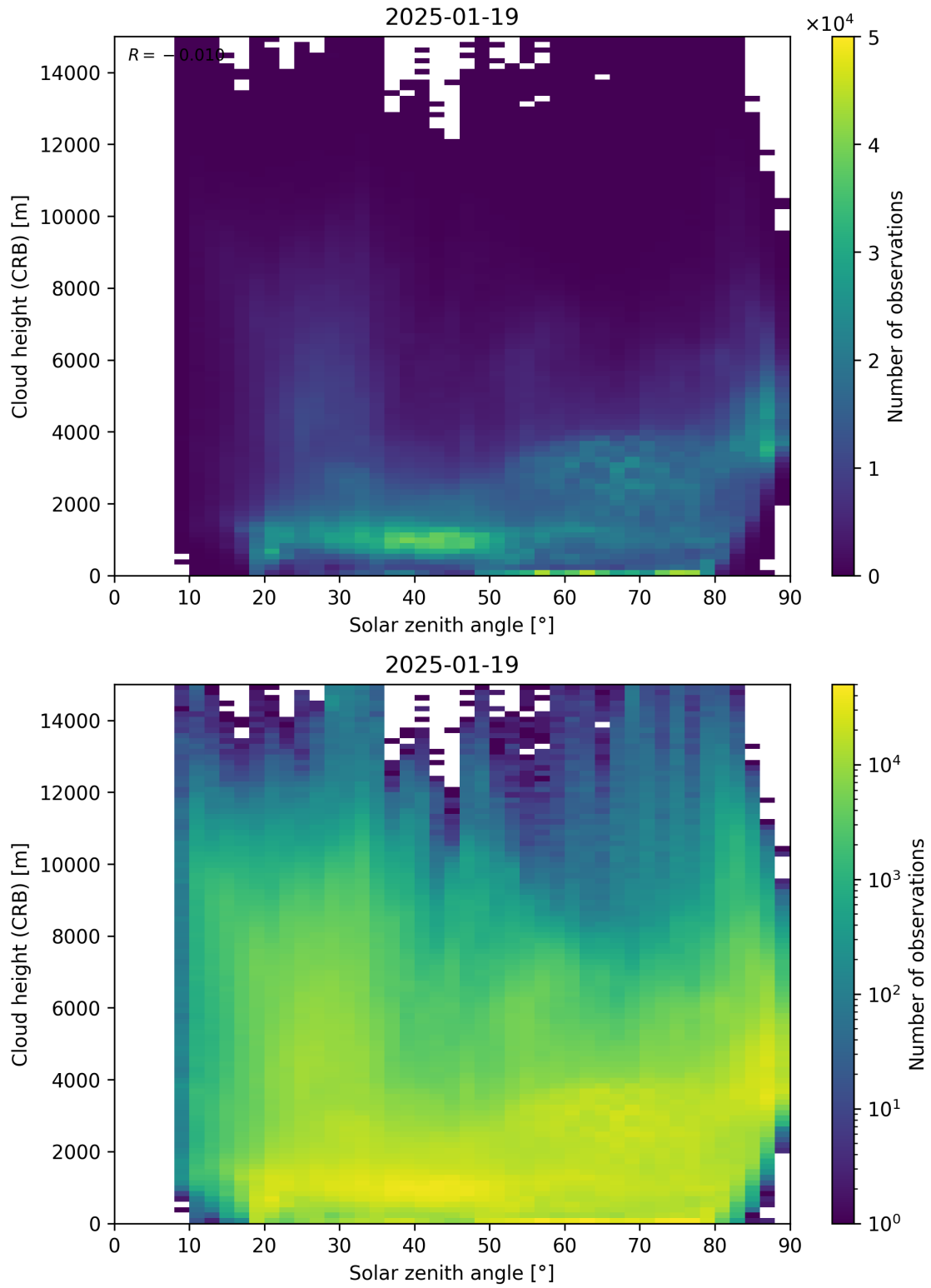
Figure 102: Scatter density plot of “Solar zenith angle” against “Cloud height (CRB)” for 2025-01-18 to 2025-01-20.
