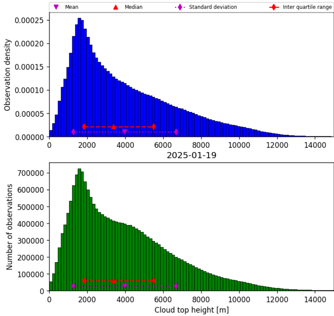
Figure 40: Histogram of “Cloud top height” for 2025-01-18 to 2025-01-20
