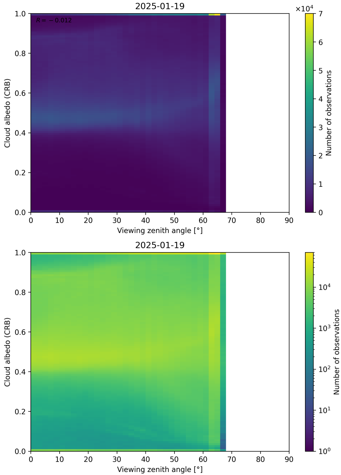
Figure 106: Scatter density plot of “Viewing zenith angle” against “Cloud albedo (CRB)” for 2025-01-18 to 2025-01-20.
