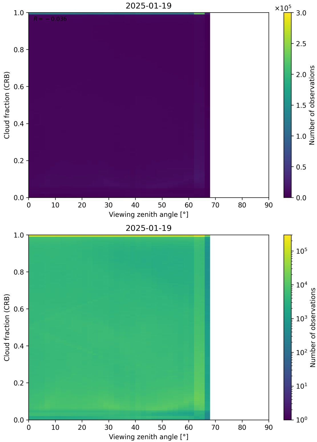
Figure 109: Scatter density plot of “Viewing zenith angle” against “Cloud fraction (CRB)” for 2025-01-18 to 2025-01-20.
