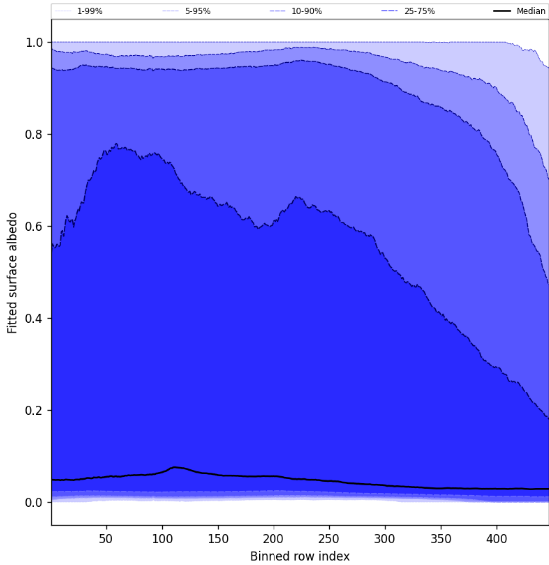
Figure 61: Along track statistics of “Fitted surface albedo” for 2025-01-18 to 2025-01-20
