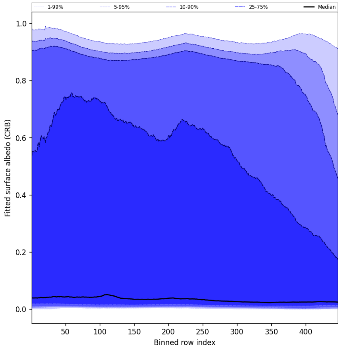
Figure 62: Along track statistics of “Fitted surface albedo (CRB)” for 2025-01-18 to 2025-01-20
