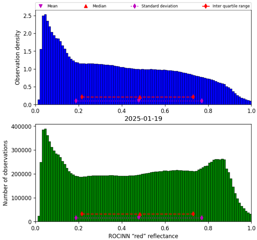
Figure 53: Histogram of “ROCINN “red” reflectance” for 2025-01-18 to 2025-01-20
