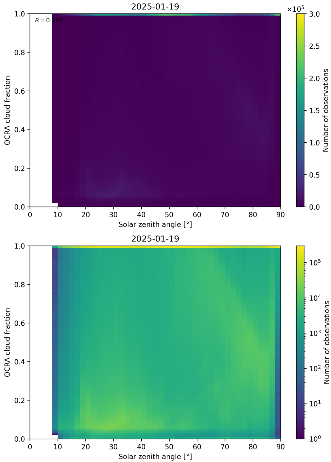
Figure 100: Scatter density plot of “Solar zenith angle” against “OCRA cloud fraction” for 2025-01-18 to 2025-01-20.
