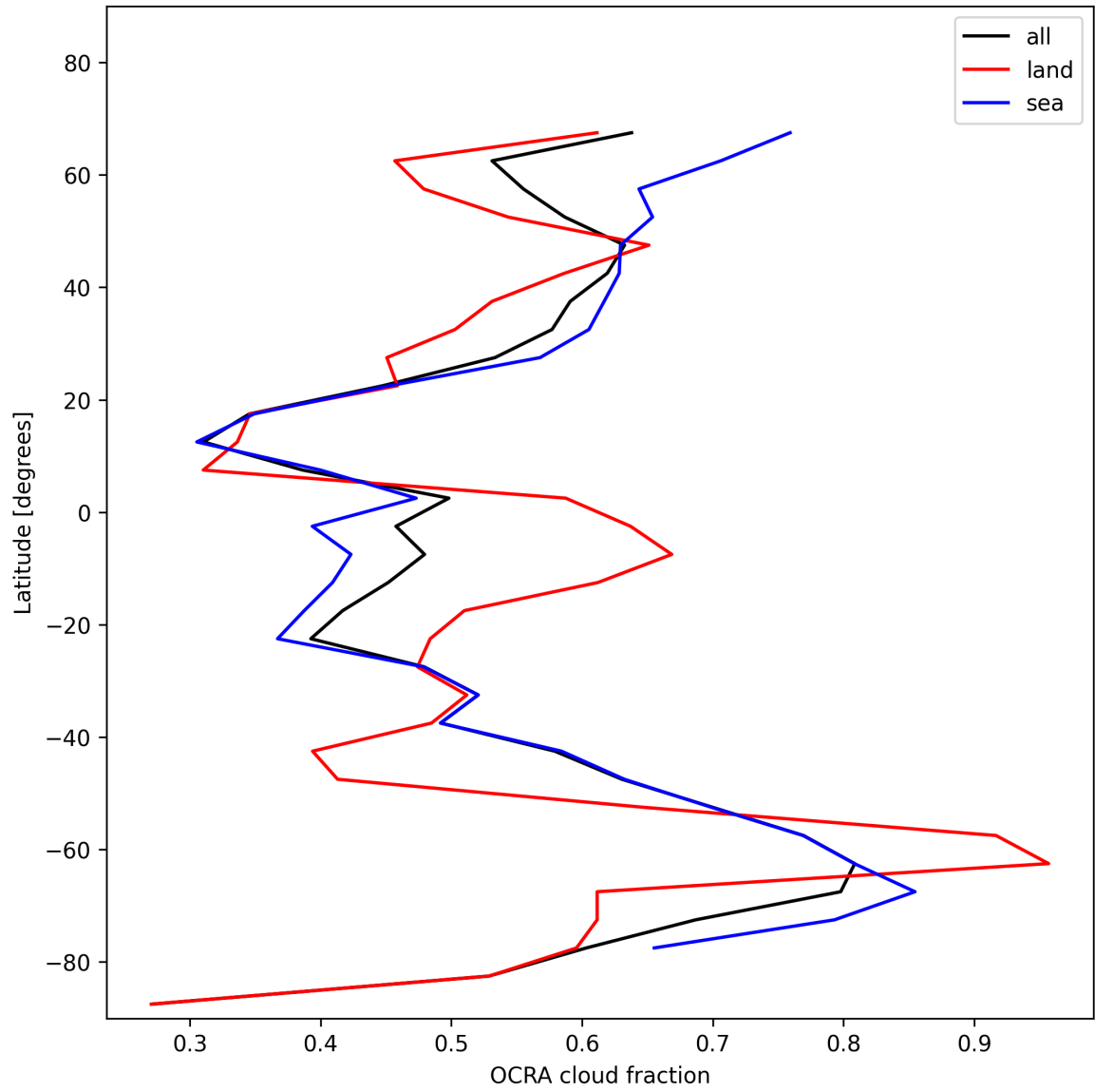
Figure 34: Zonal average of “OCRA cloud fraction” for 2025-01-18 to 2025-01-20.
