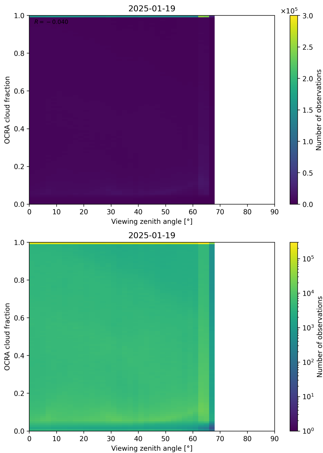
Figure 108: Scatter density plot of “Viewing zenith angle” against “OCRA cloud fraction” for 2025-01-18 to 2025-01-20.
