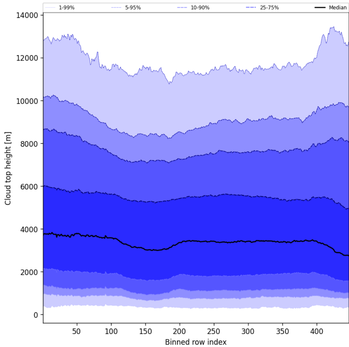
Figure 56: Along track statistics of “Cloud top height” for 2025-01-18 to 2025-01-20
