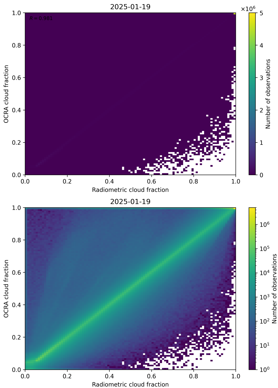
Figure 72: Scatter density plot of “Radiometric cloud fraction” against “OCRA cloud fraction” for 2025-01-18 to 2025-01-20.
