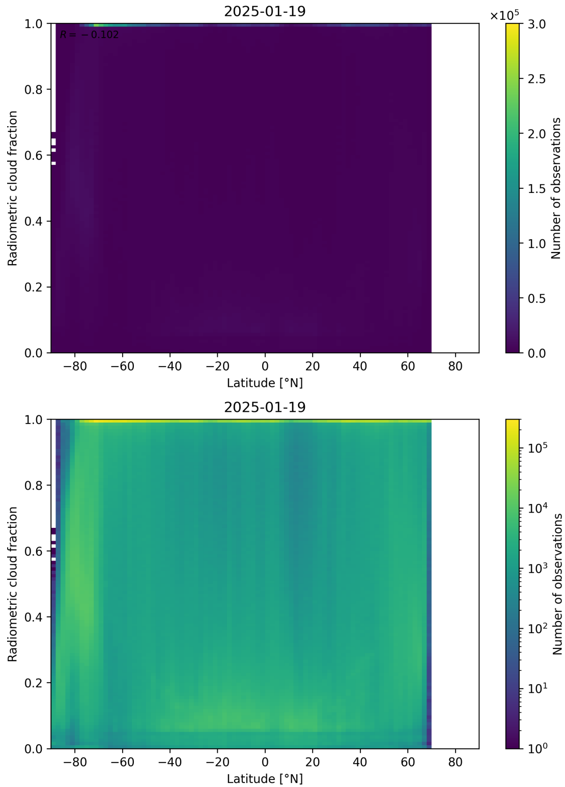
Figure 92: Scatter density plot of “Latitude” against “Radiometric cloud fraction” for 2025-01-18 to 2025-01-20.
