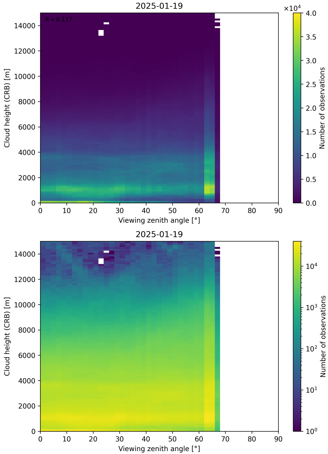
Figure 110: Scatter density plot of “Viewing zenith angle” against “Cloud height (CRB)” for 2025-01-18 to 2025-01-20.
