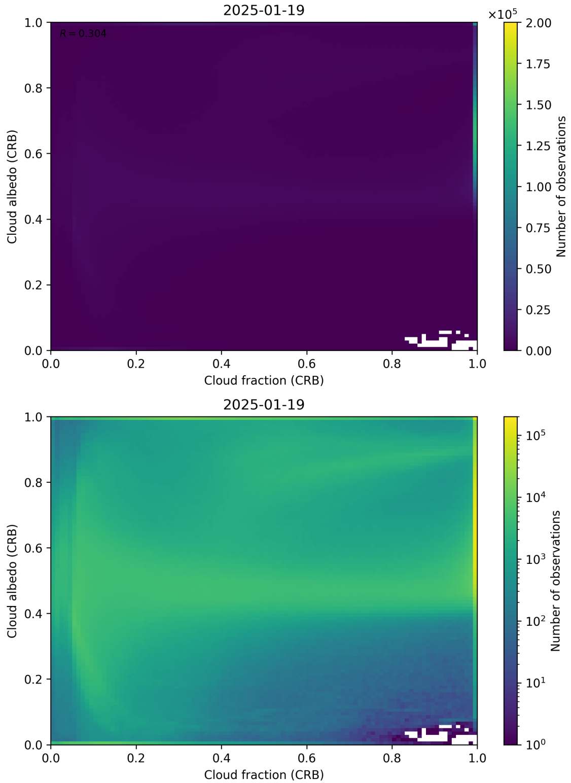
Figure 77: Scatter density plot of “Cloud fraction (CRB)” against “Cloud albedo (CRB)” for 2025-01-18 to 2025-01-20.
