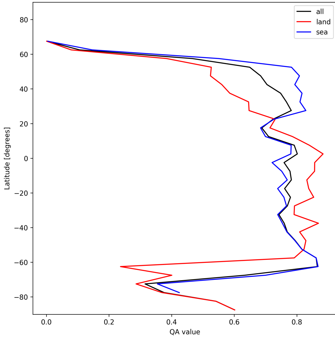
Figure 22: Zonal average of “QA value” for 2025-01-19 to 2025-01-21.
