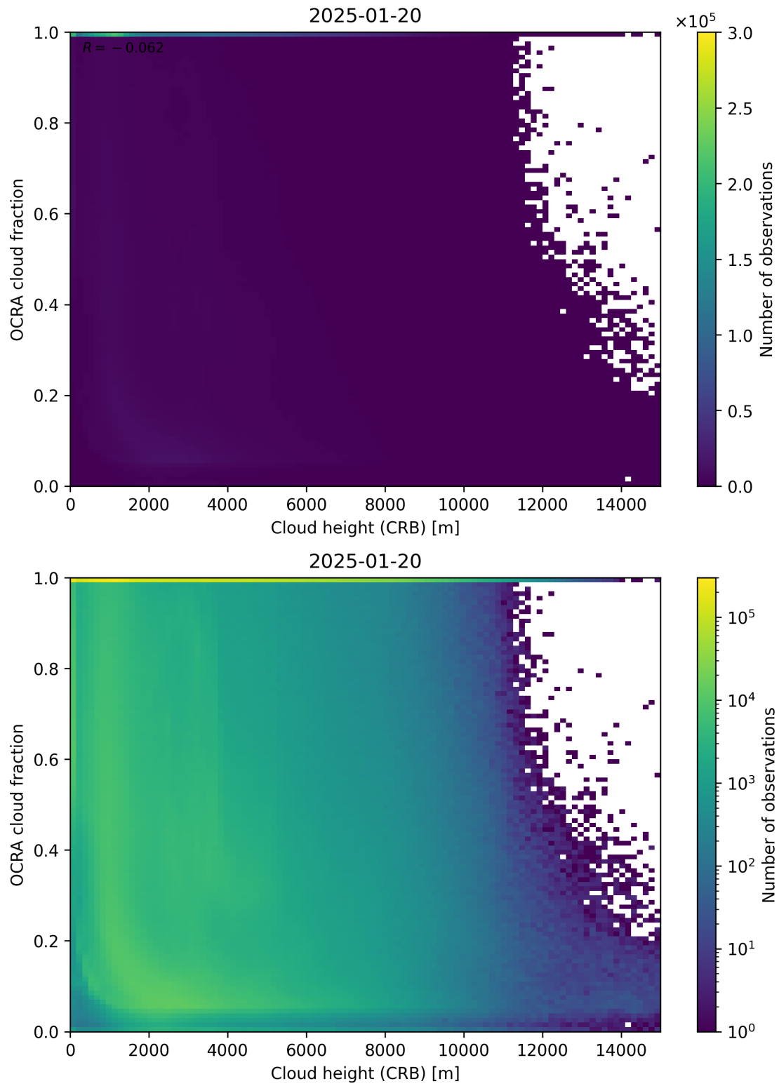
Figure 81: Scatter density plot of “Cloud height (CRB)” against “OCRA cloud fraction” for 2025-01-19 to 2025-01-21.
