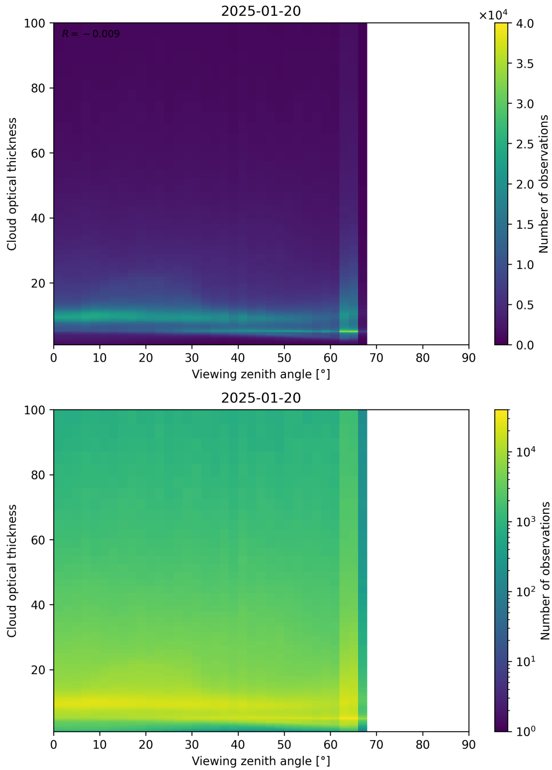
Figure 111: Scatter density plot of “Viewing zenith angle” against “Cloud optical thickness” for 2025-01-19 to 2025-01-21.
