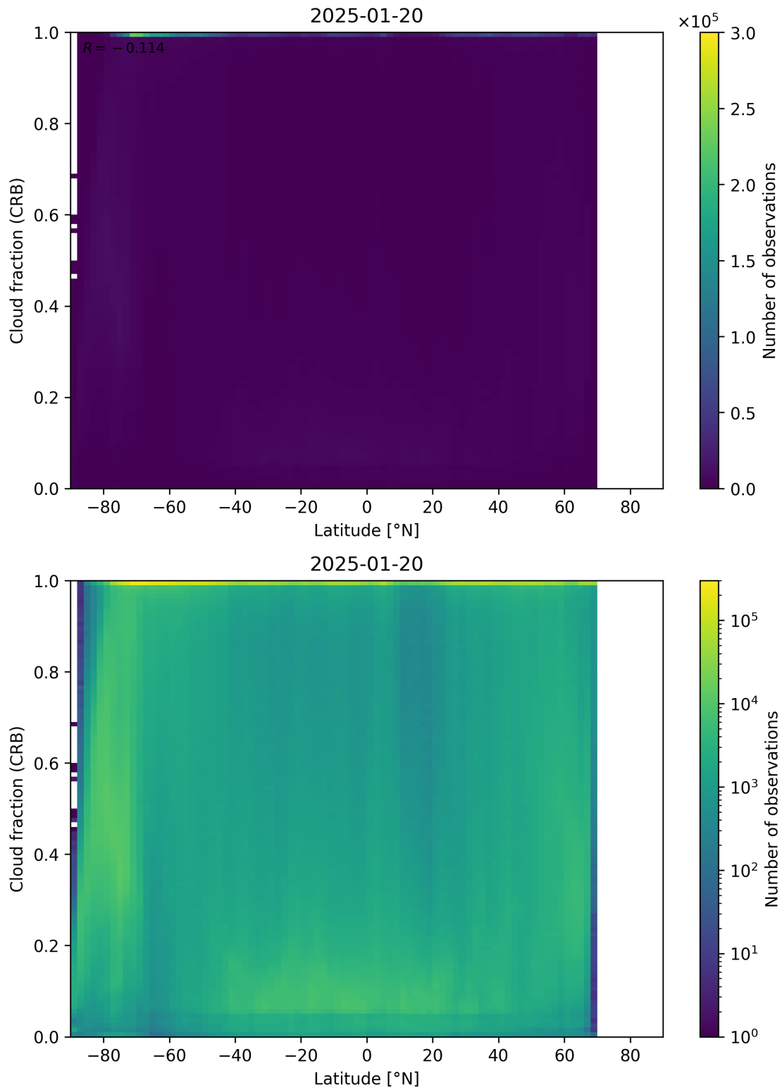
Figure 94: Scatter density plot of “Latitude” against “Cloud fraction (CRB)” for 2025-01-19 to 2025-01-21.
