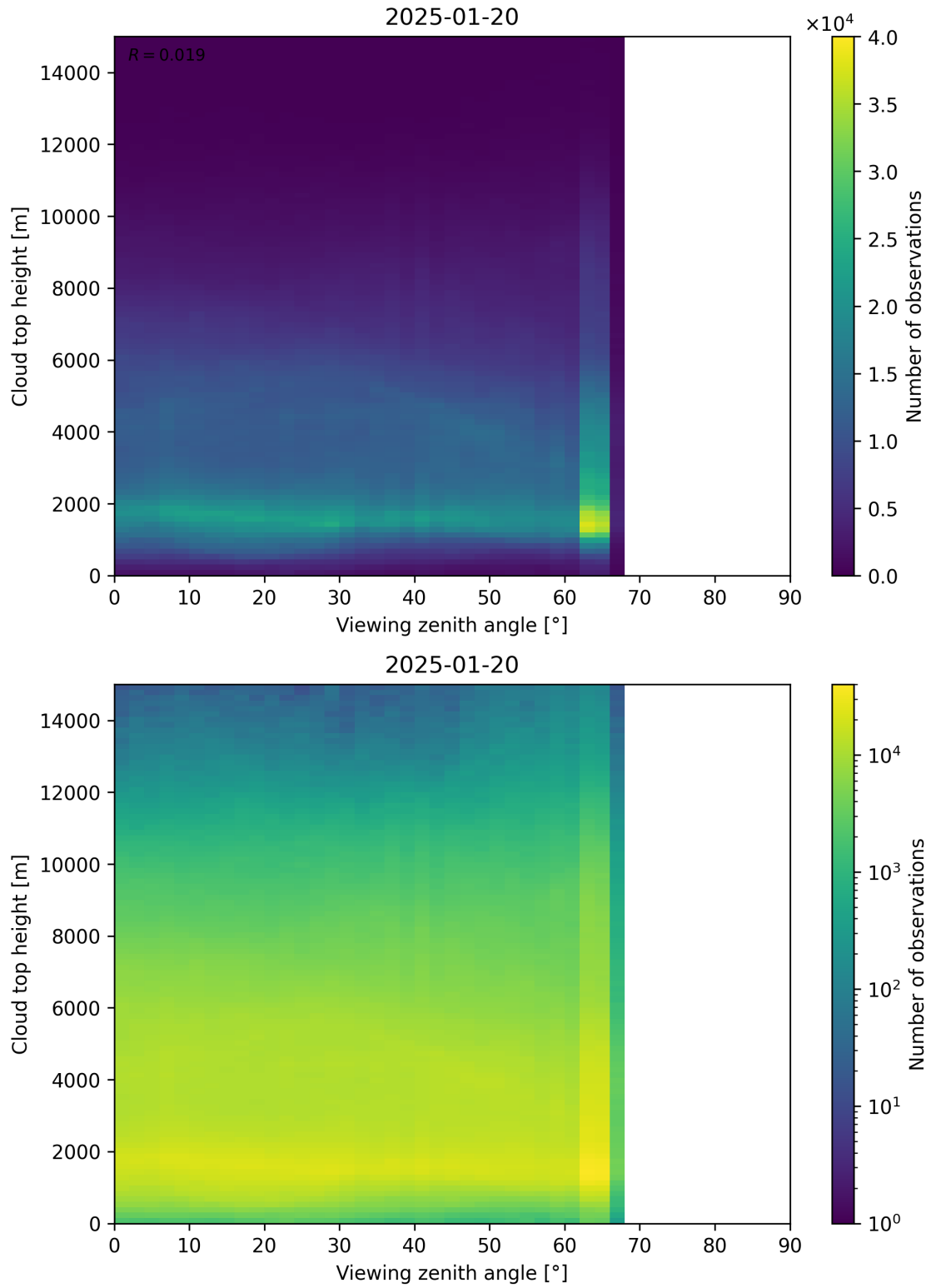
Figure 112: Scatter density plot of “Viewing zenith angle” against “Cloud top height” for 2025-01-19 to 2025-01-21.
