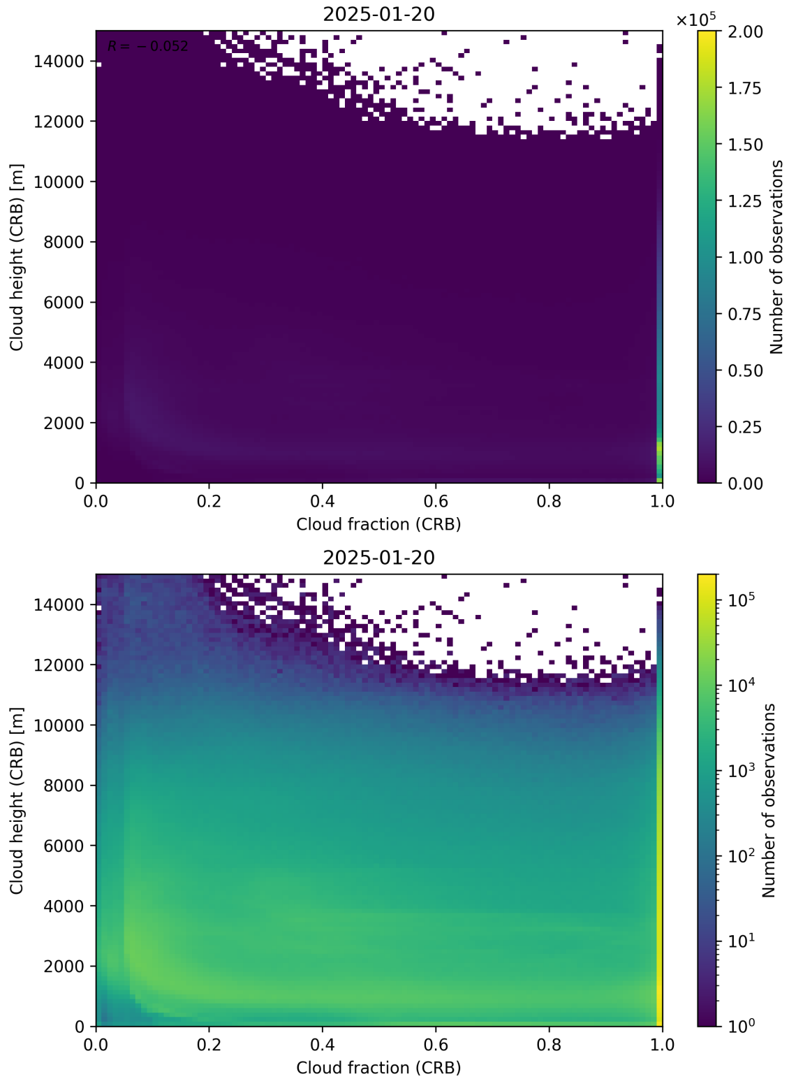
Figure 79: Scatter density plot of “Cloud fraction (CRB)” against “Cloud height (CRB)” for 2025-01-19 to 2025-01-21.
