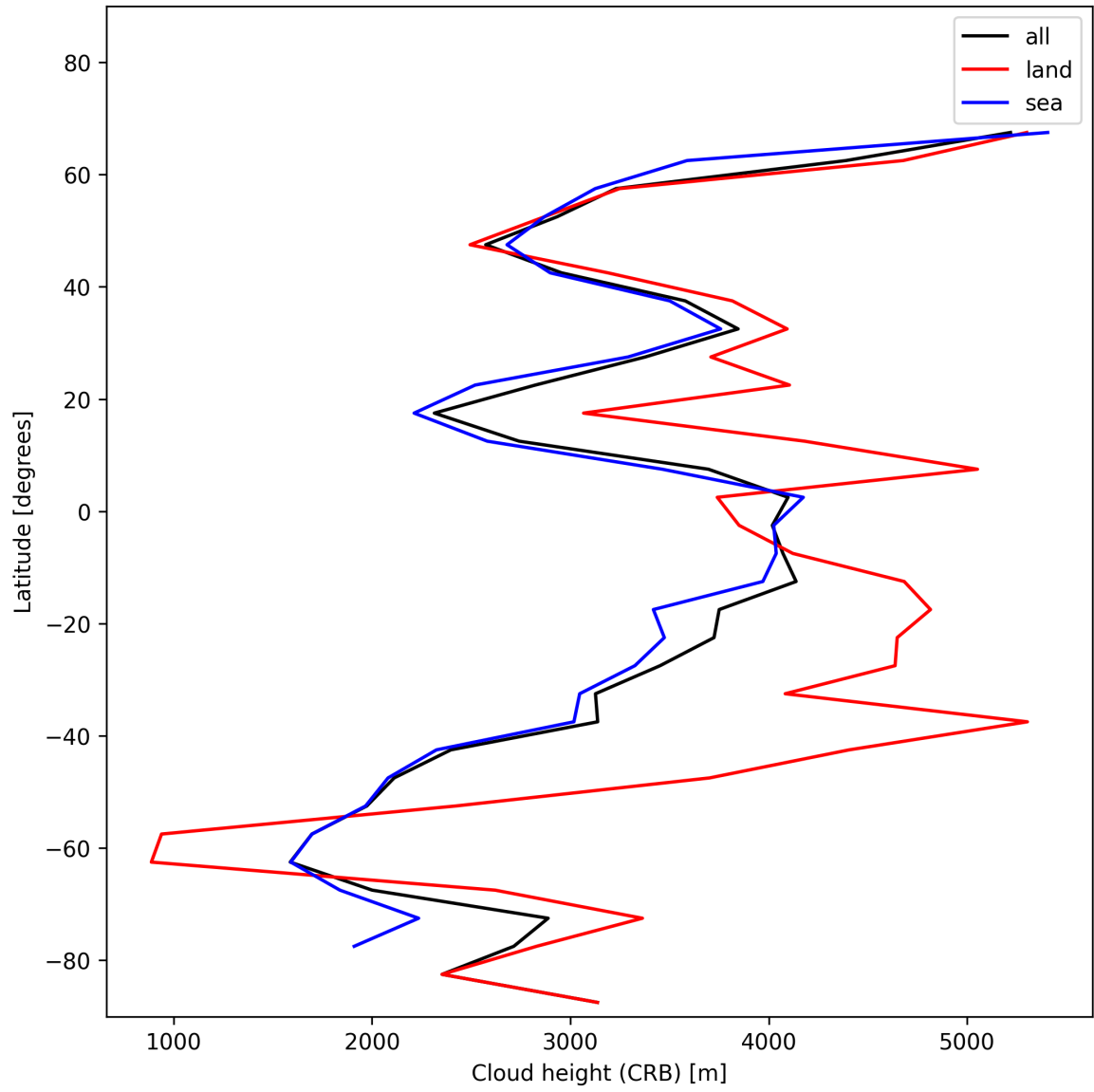
Figure 27: Zonal average of “Cloud height (CRB)” for 2025-01-19 to 2025-01-21.
