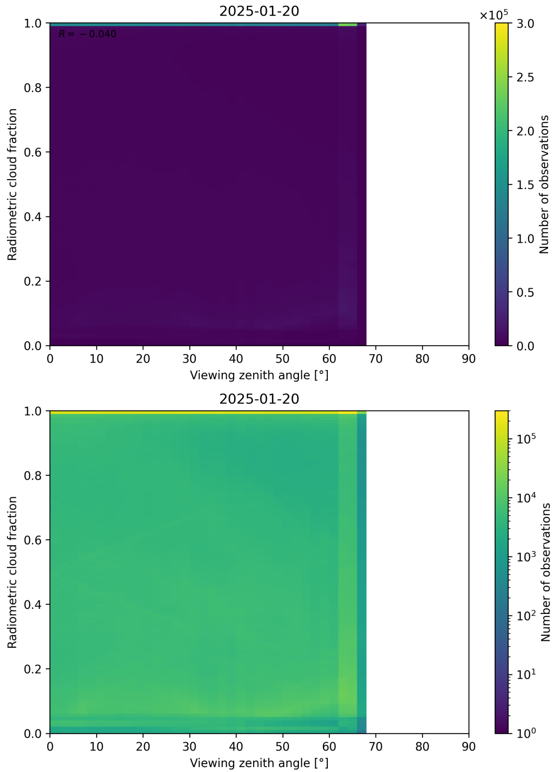
Figure 107: Scatter density plot of “Viewing zenith angle” against “Radiometric cloud fraction” for 2025-01-19 to 2025-01-21.
