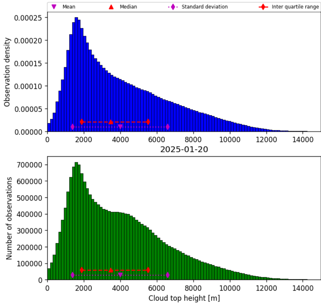
Figure 40: Histogram of “Cloud top height” for 2025-01-19 to 2025-01-21
