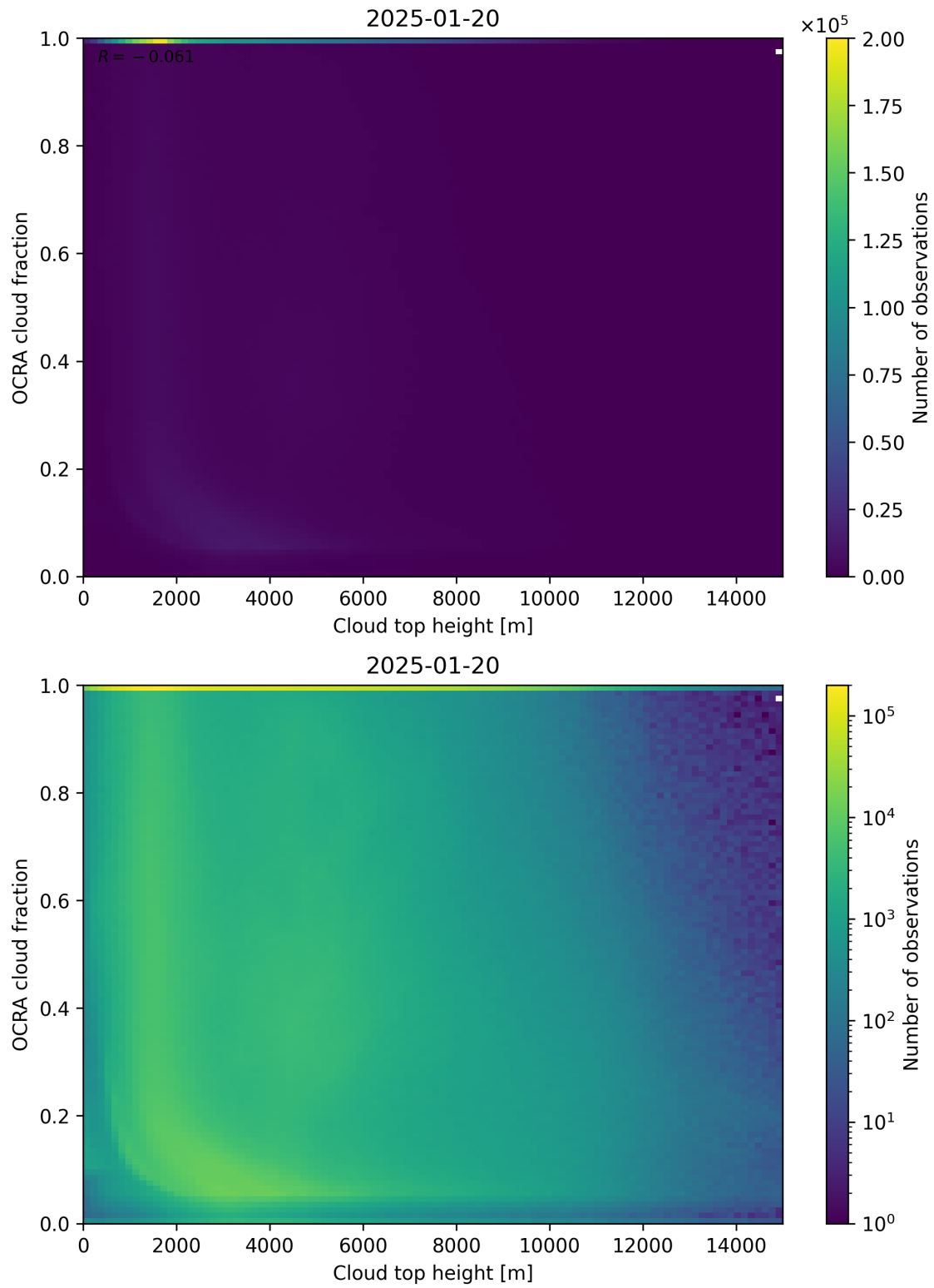
Figure 87: Scatter density plot of “Cloud top height” against “OCRA cloud fraction” for 2025-01-19 to 2025-01-21.
