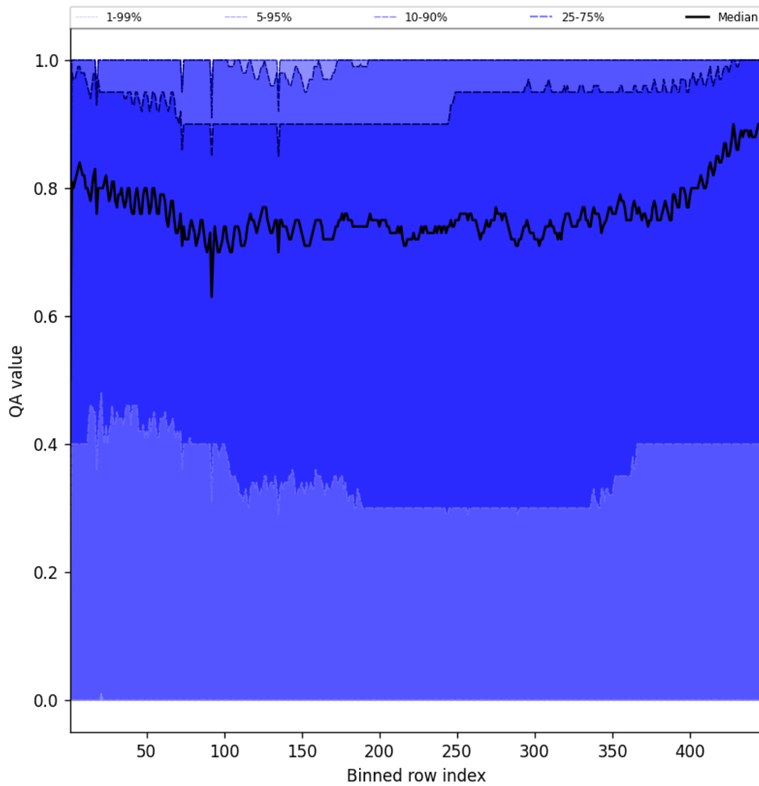
Figure 54: Along track statistics of “QA value” for 2025-01-19 to 2025-01-21
