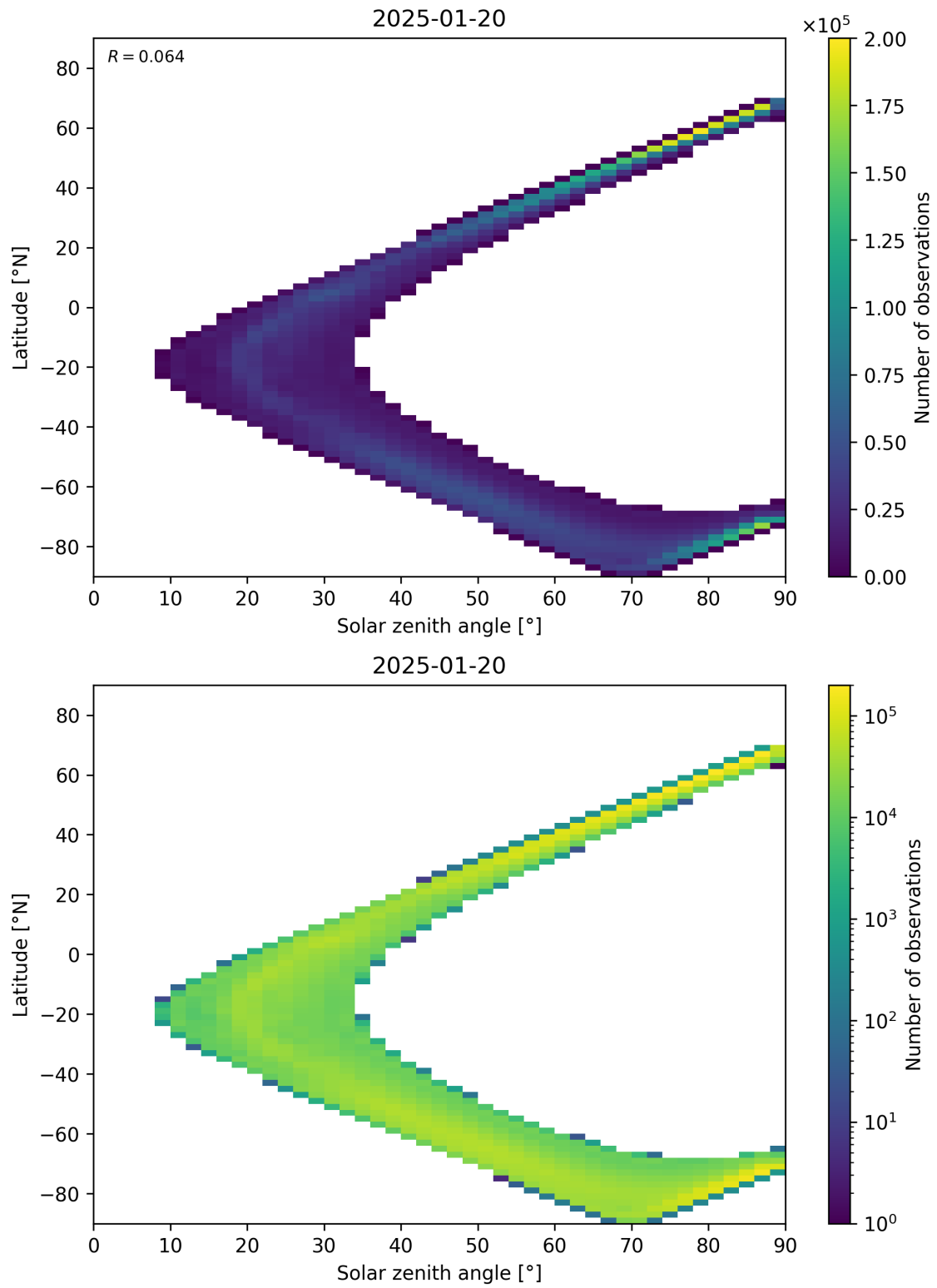
Figure 105: Scatter density plot of “Solar zenith angle” against “Latitude” for 2025-01-19 to 2025-01-21.
