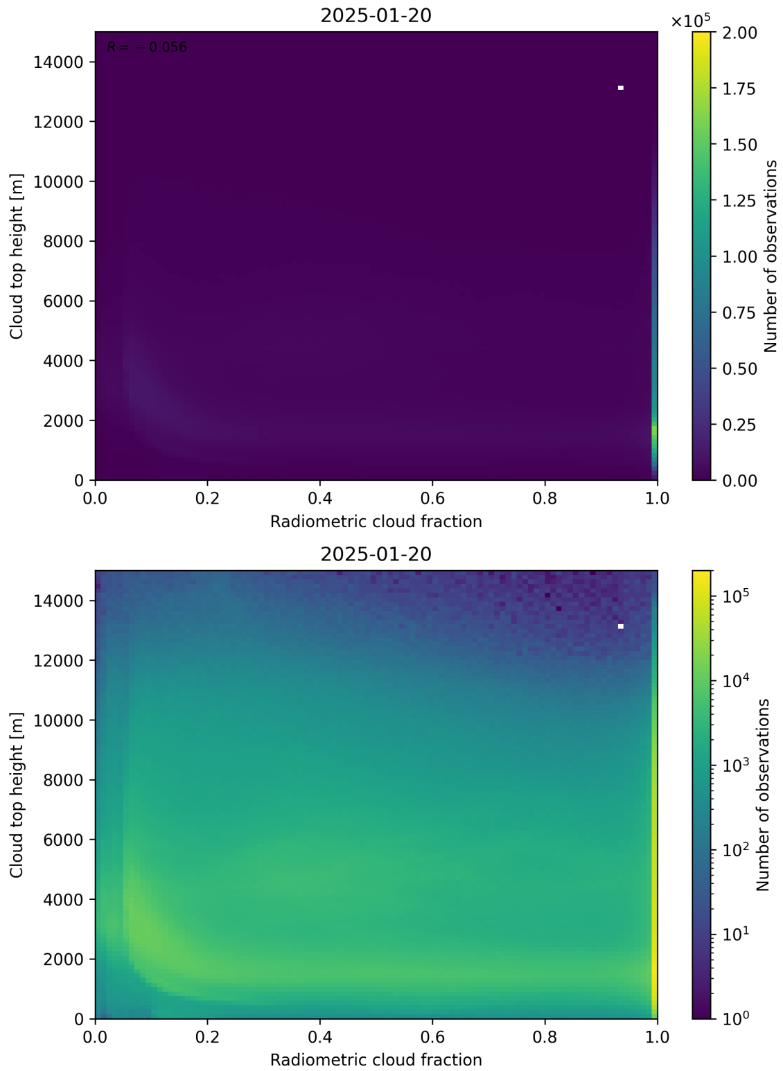
Figure 76: Scatter density plot of “Radiometric cloud fraction” against “Cloud top height” for 2025-01-19 to 2025-01-21.
