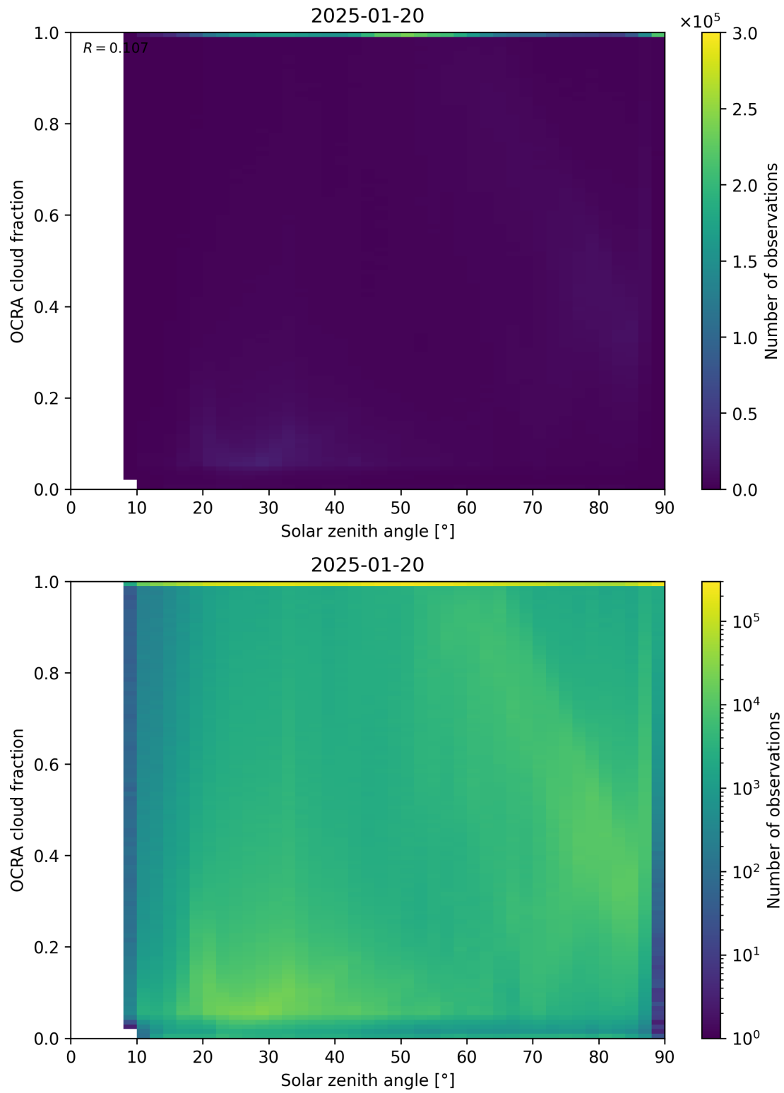
Figure 100: Scatter density plot of “Solar zenith angle” against “OCRA cloud fraction” for 2025-01-19 to 2025-01-21.
