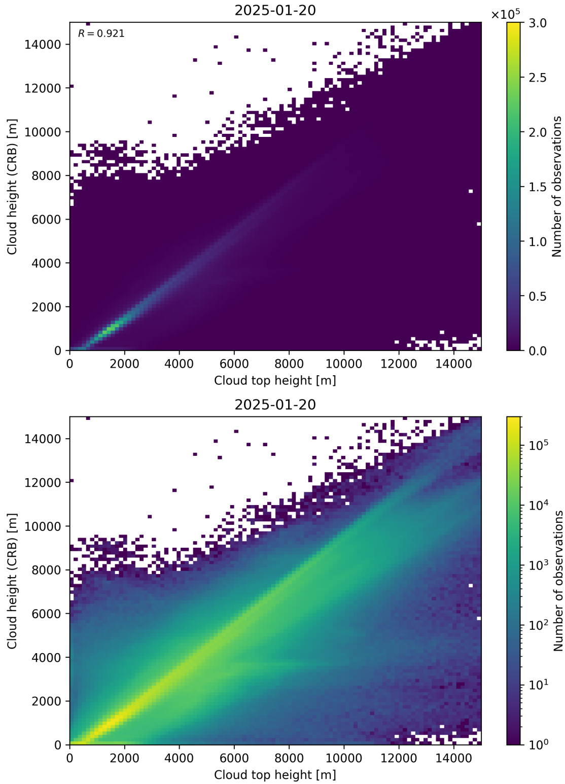
Figure 89: Scatter density plot of “Cloud top height” against “Cloud height (CRB)” for 2025-01-19 to 2025-01-21.
