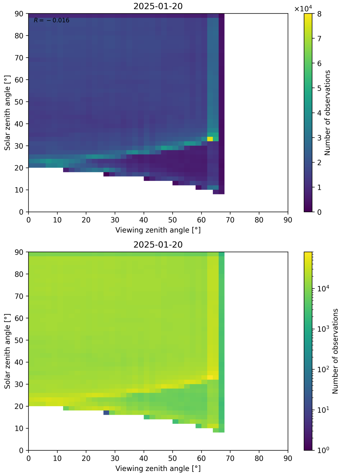
Figure 114: Scatter density plot of “Viewing zenith angle” against “Solar zenith angle” for 2025-01-19 to 2025-01-21.
