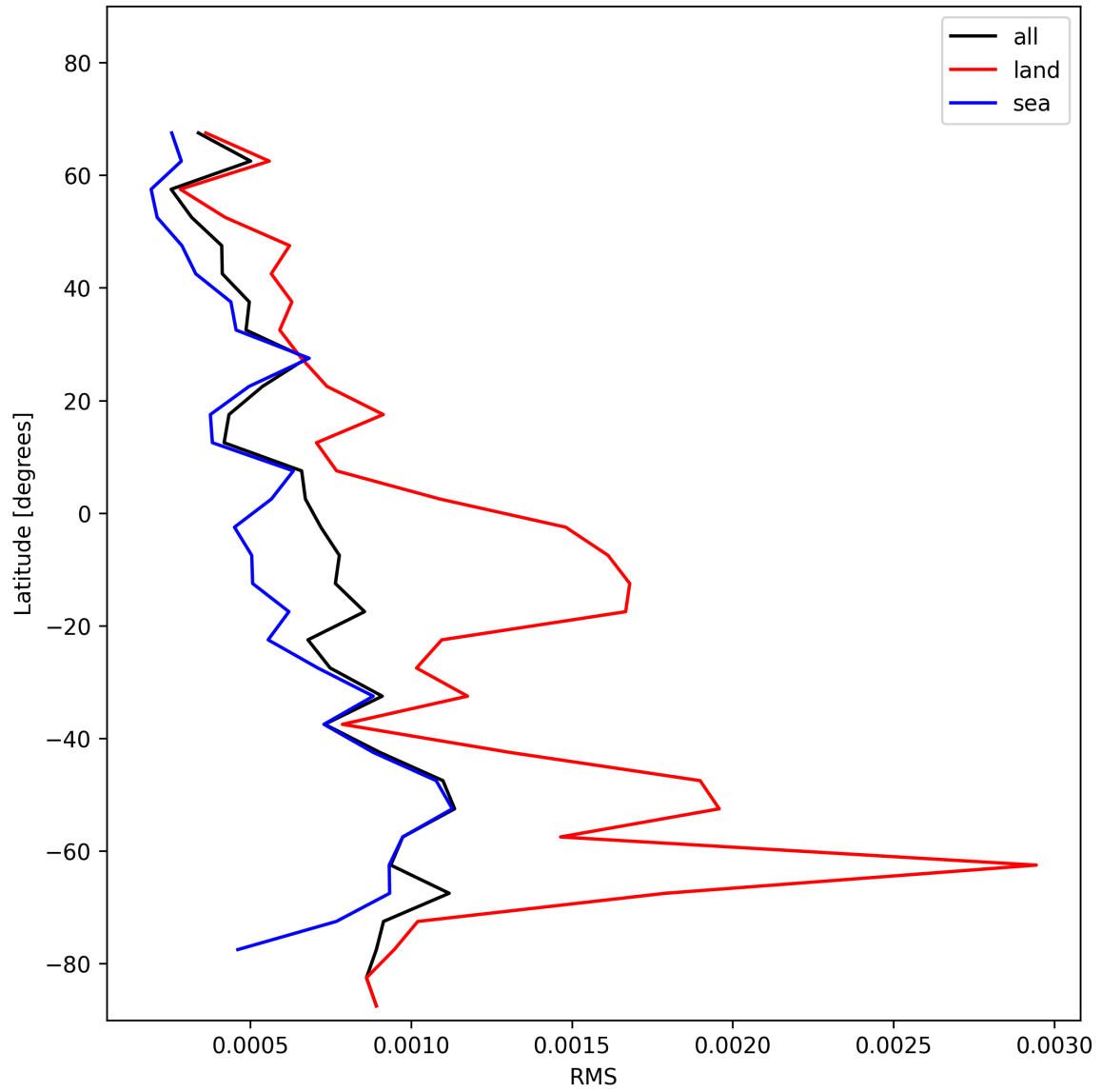
Figure 31: Zonal average of “RMS” for 2025-01-19 to 2025-01-21.
