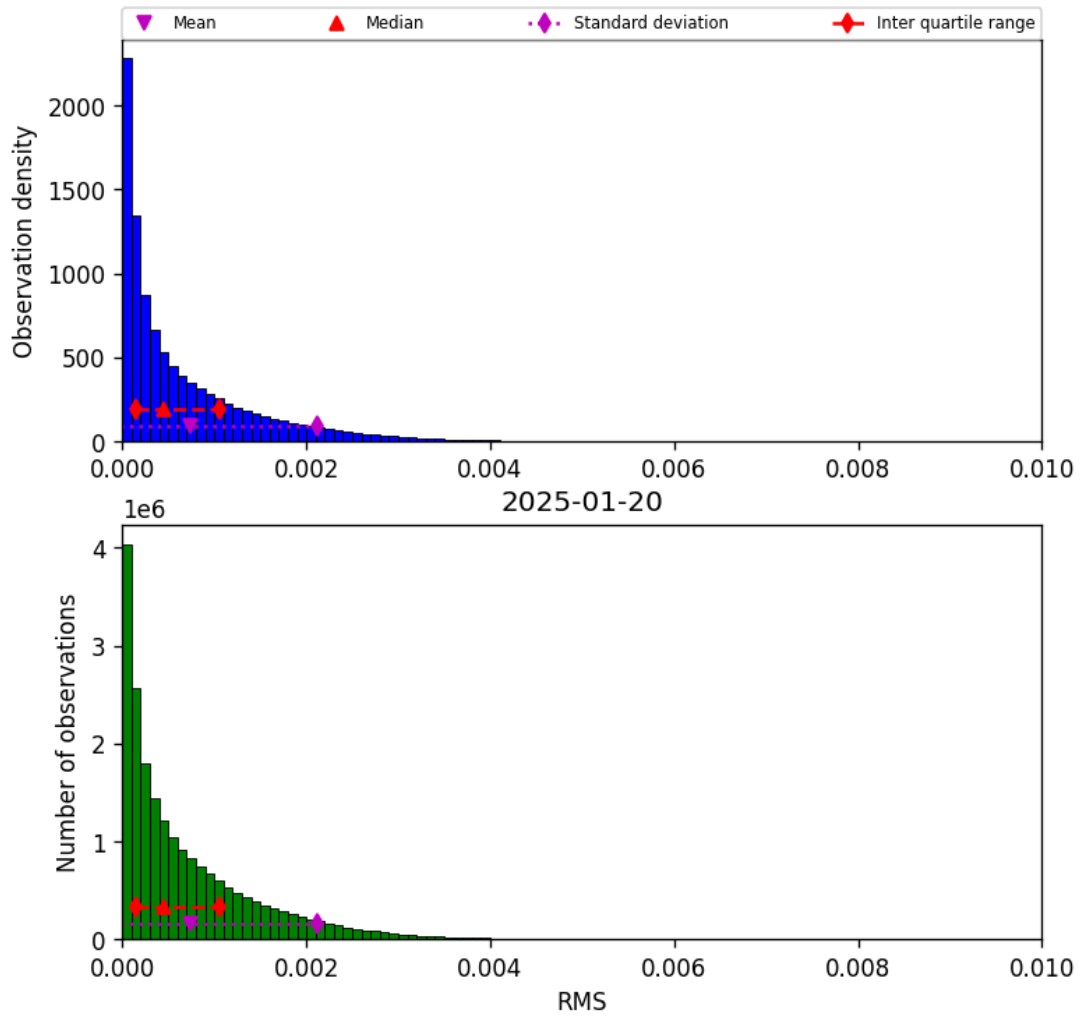
Figure 47: Histogram of “RMS” for 2025-01-19 to 2025-01-21
