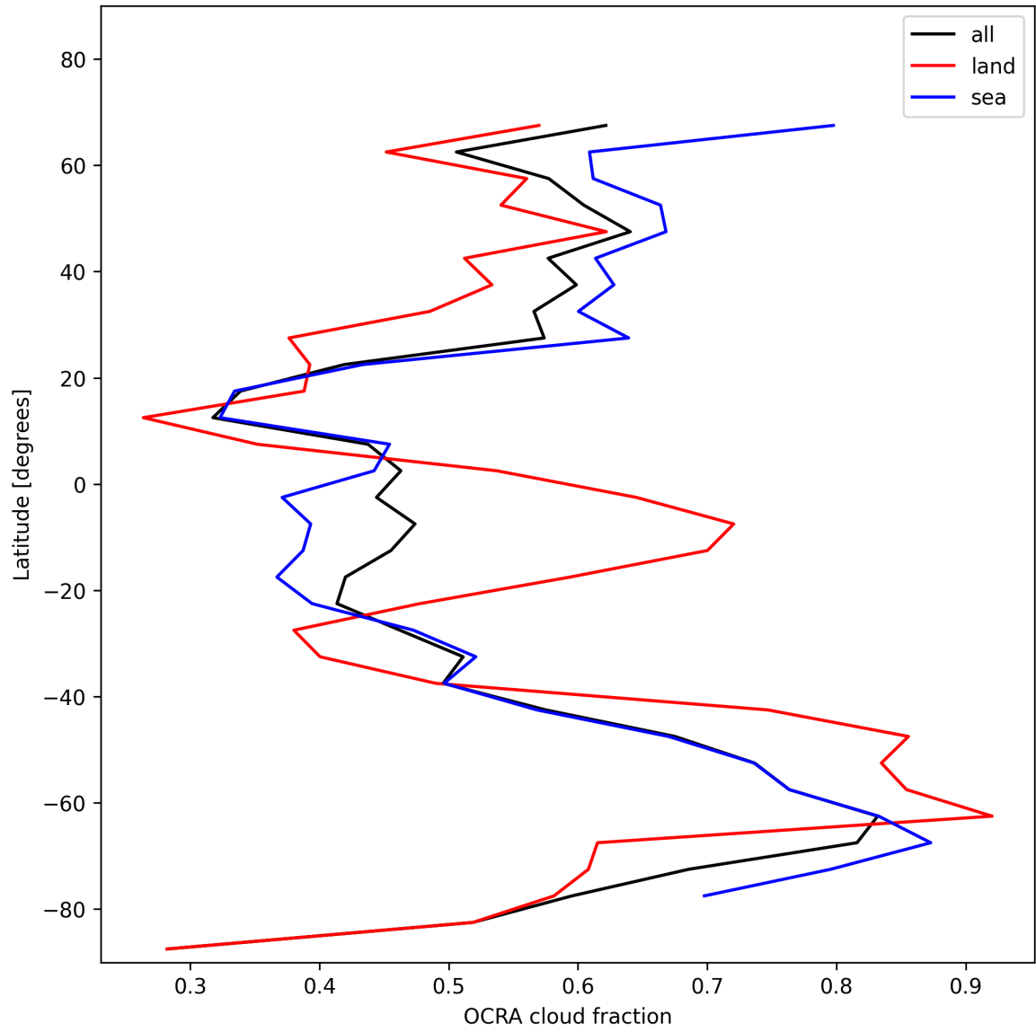
Figure 34: Zonal average of “OCRA cloud fraction” for 2025-01-19 to 2025-01-21.
