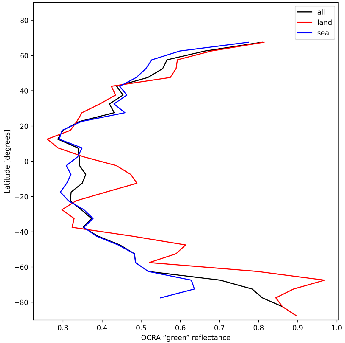
Figure 36: Zonal average of “OCRA “green” reflectance” for 2025-01-19 to 2025-01-21.
