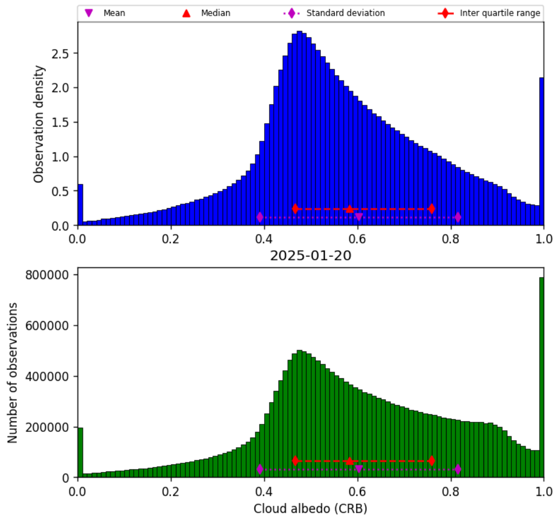
Figure 44: Histogram of “Cloud albedo (CRB)” for 2025-01-19 to 2025-01-21
