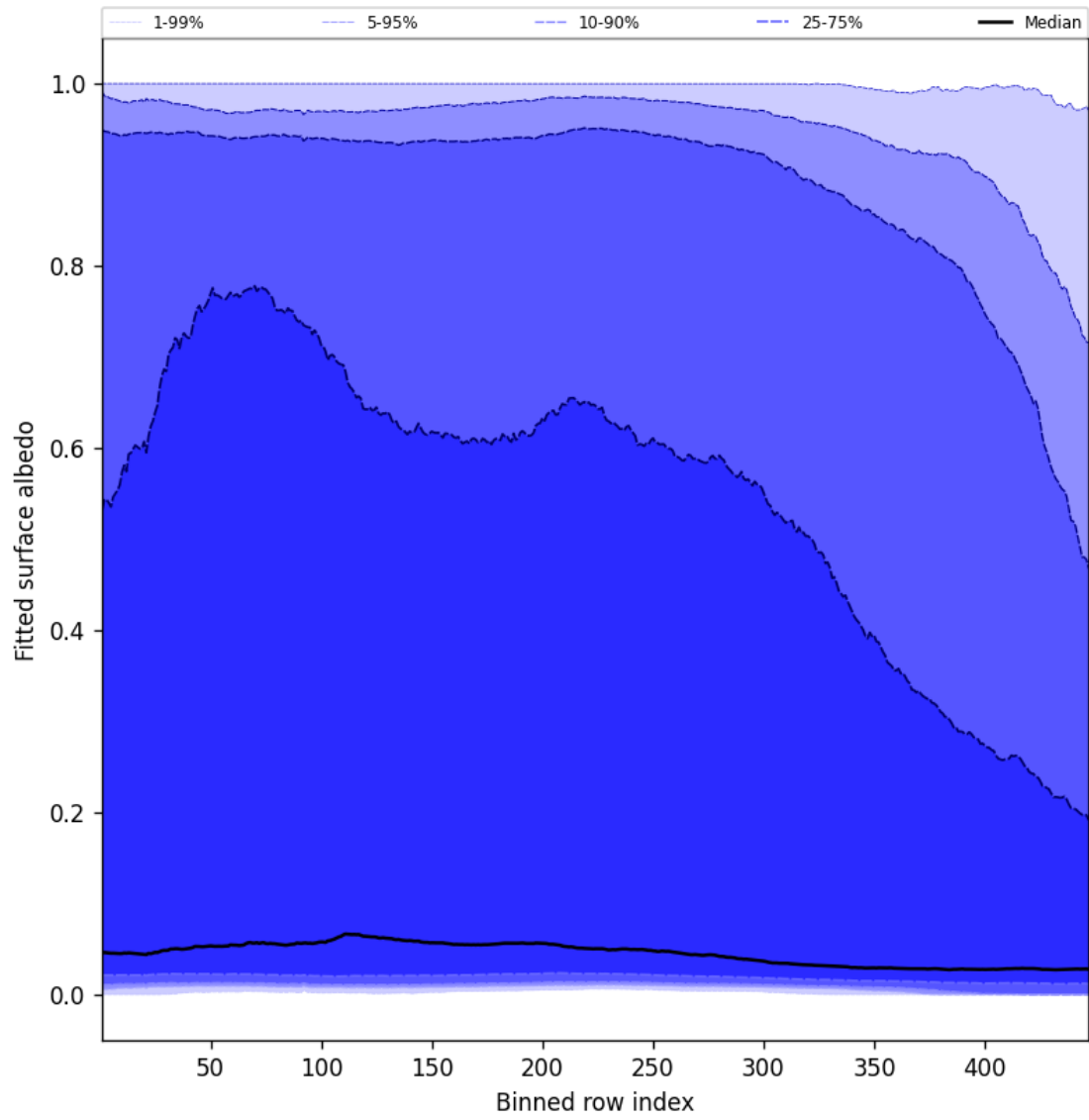
Figure 61: Along track statistics of “Fitted surface albedo” for 2025-01-19 to 2025-01-21
