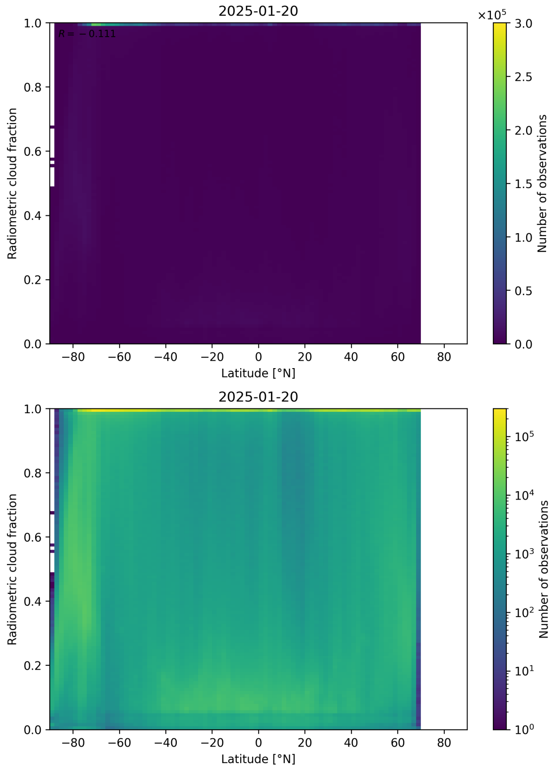
Figure 92: Scatter density plot of “Latitude” against “Radiometric cloud fraction” for 2025-01-19 to 2025-01-21.
