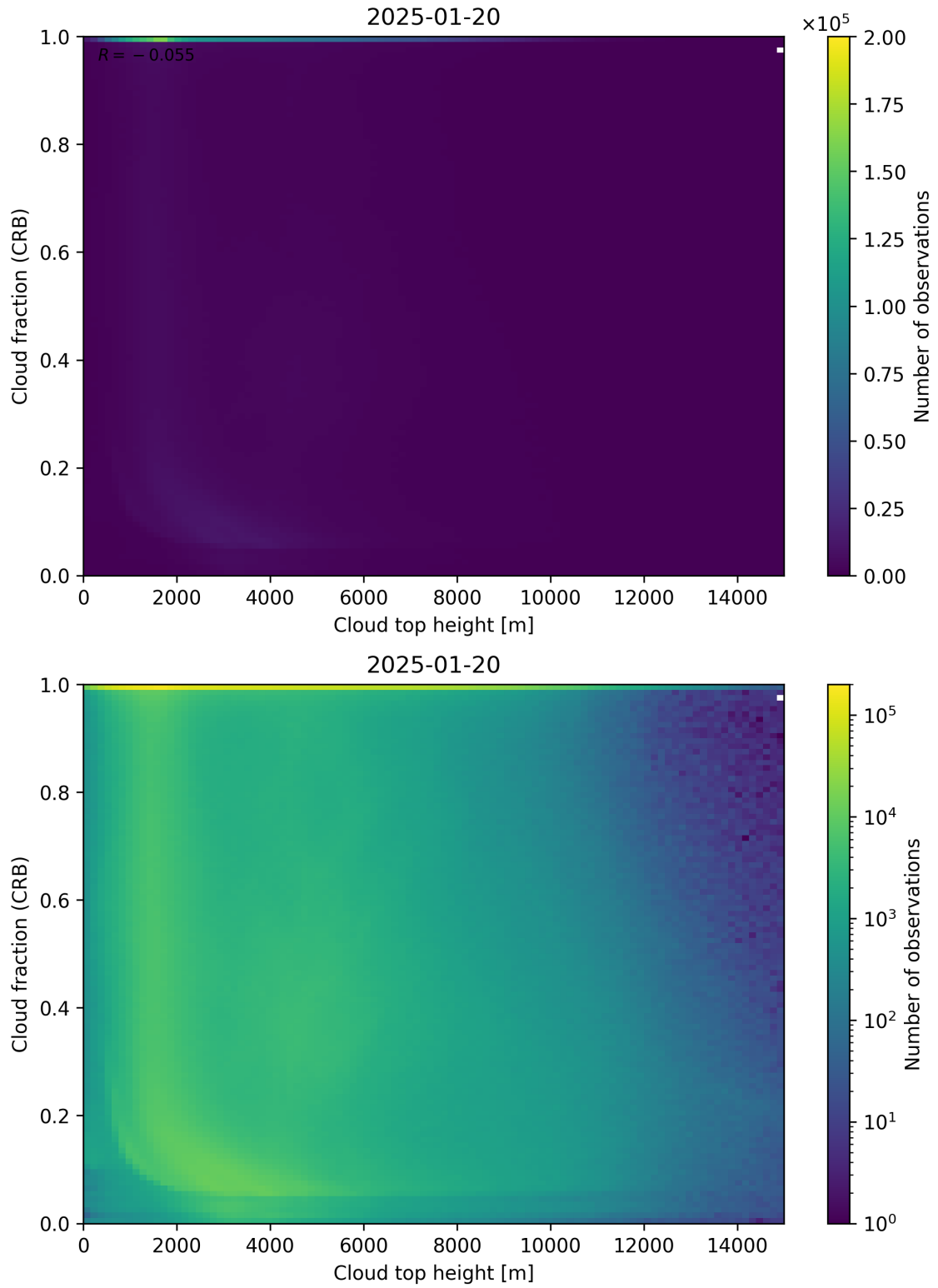
Figure 88: Scatter density plot of “Cloud top height” against “Cloud fraction (CRB)” for 2025-01-19 to 2025-01-21.
