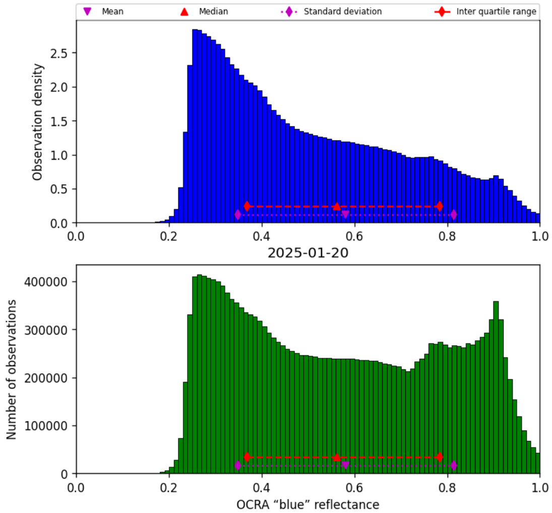
Figure 51: Histogram of “OCRA “blue” reflectance” for 2025-01-19 to 2025-01-21
