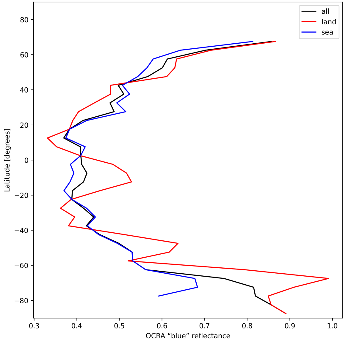
Figure 35: Zonal average of “OCRA “blue” reflectance” for 2025-01-19 to 2025-01-21.
