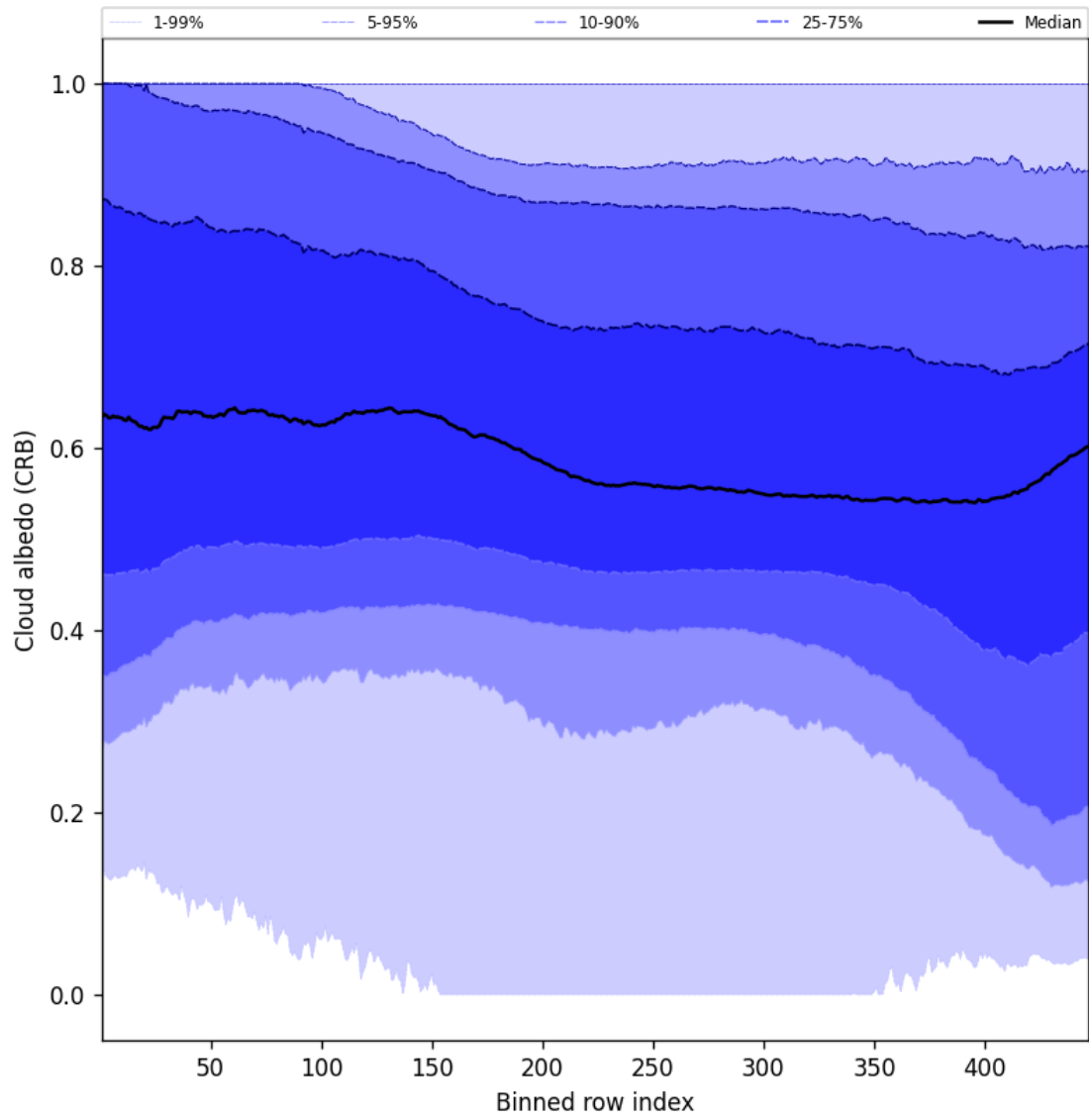
Figure 60: Along track statistics of “Cloud albedo (CRB)” for 2025-01-19 to 2025-01-21
