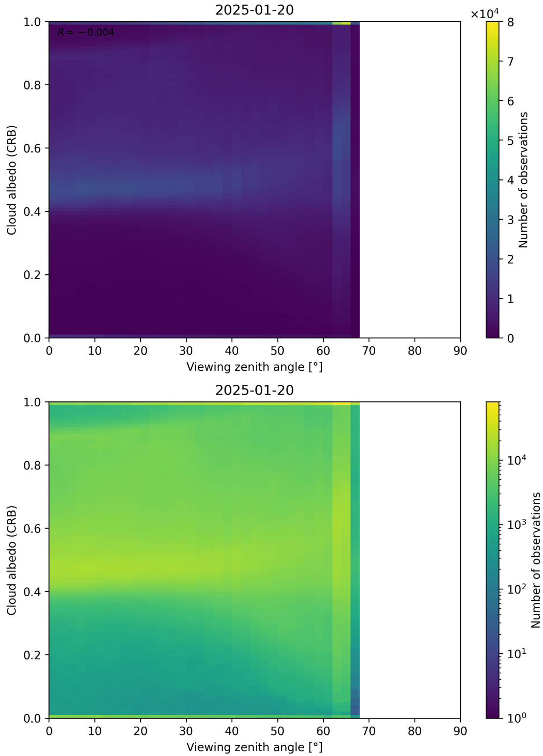
Figure 106: Scatter density plot of “Viewing zenith angle” against “Cloud albedo (CRB)” for 2025-01-19 to 2025-01-21.
