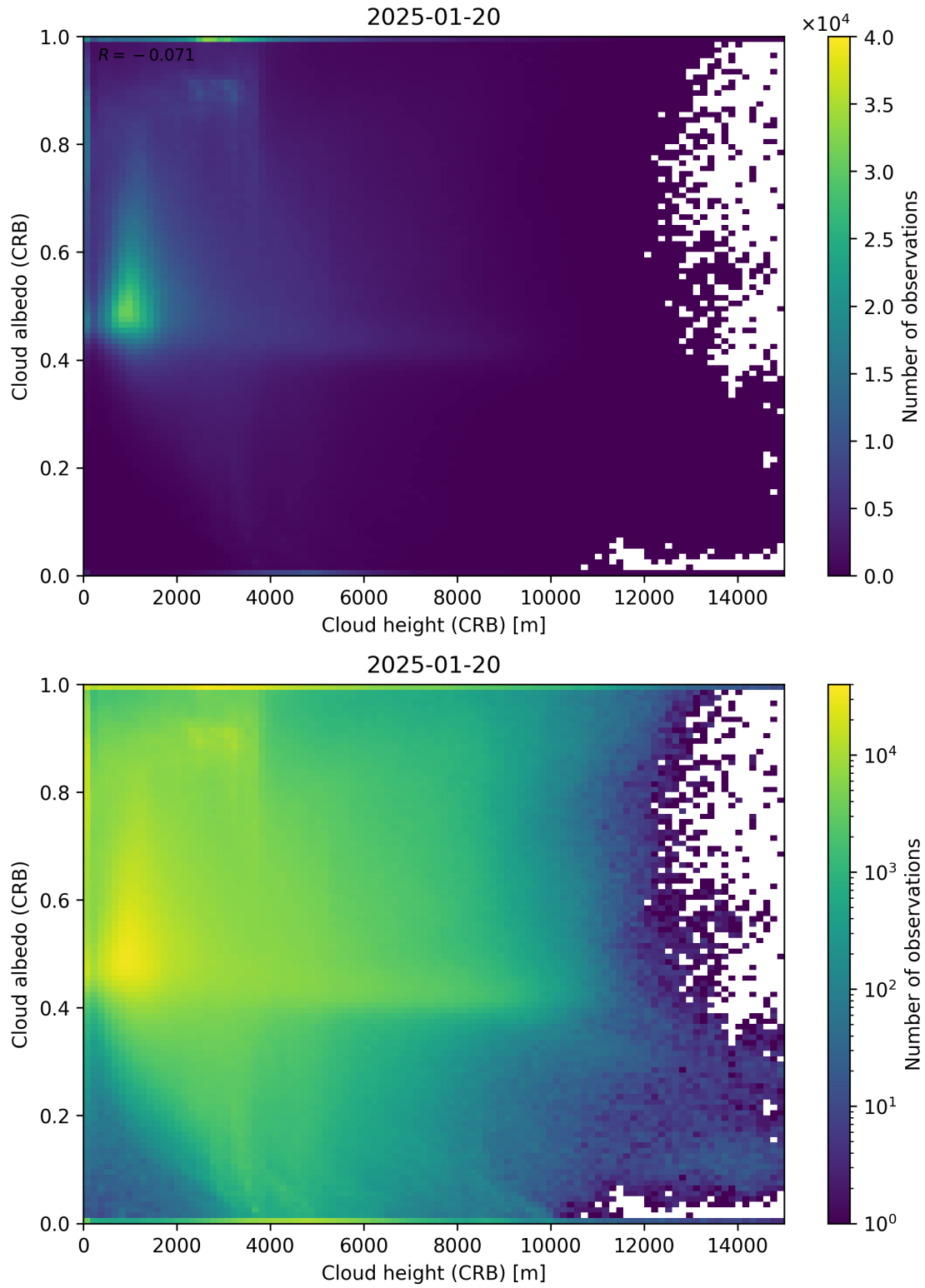
Figure 80: Scatter density plot of “Cloud height (CRB)” against “Cloud albedo (CRB)” for 2025-01-19 to 2025-01-21.
