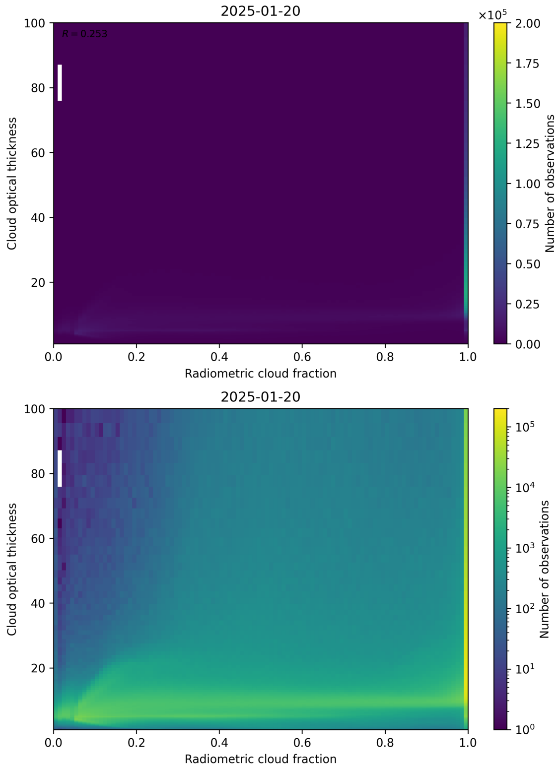
Figure 75: Scatter density plot of “Radiometric cloud fraction” against “Cloud optical thickness” for 2025-01-19 to 2025-01-21.
