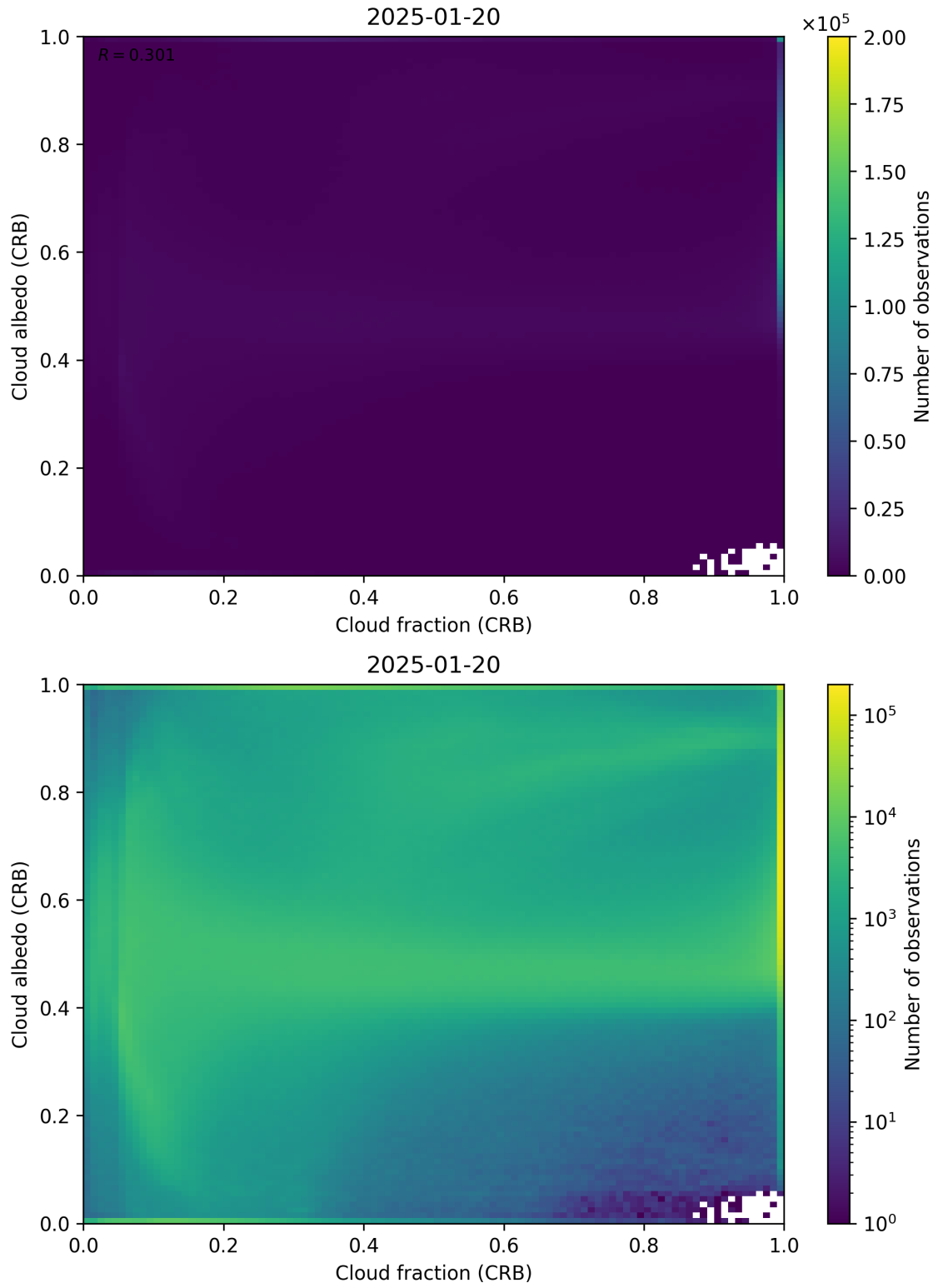
Figure 77: Scatter density plot of “Cloud fraction (CRB)” against “Cloud albedo (CRB)” for 2025-01-19 to 2025-01-21.
