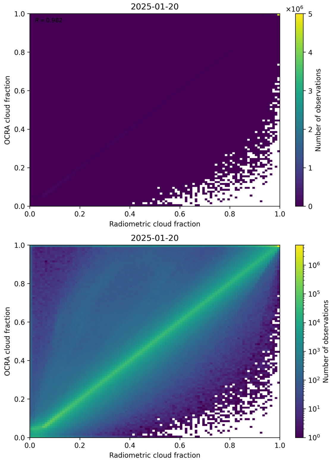
Figure 72: Scatter density plot of “Radiometric cloud fraction” against “OCRA cloud fraction” for 2025-01-19 to 2025-01-21.
