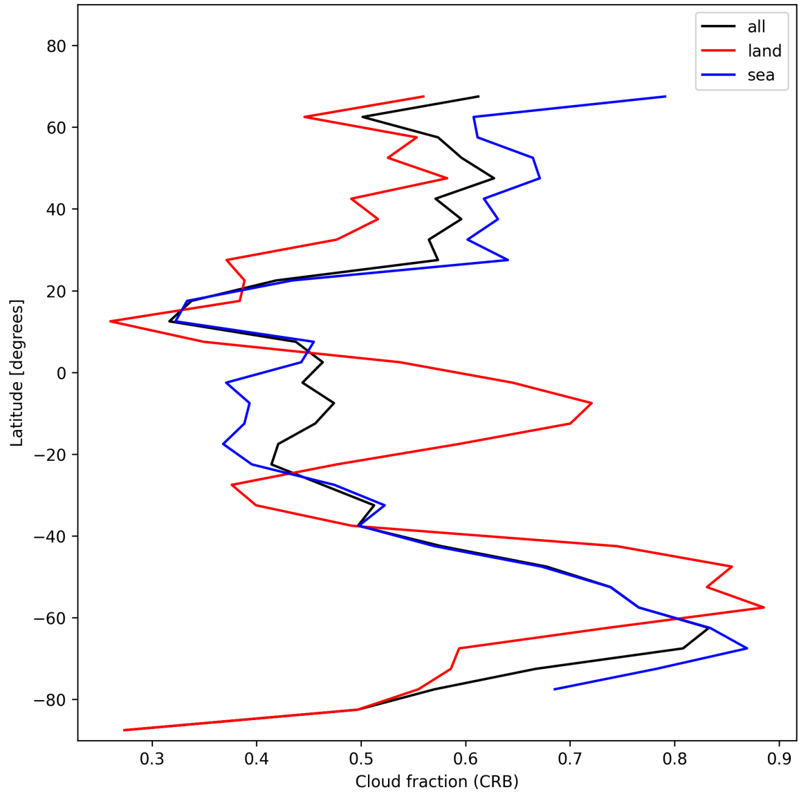
Figure 26: Zonal average of “Cloud fraction (CRB)” for 2025-01-19 to 2025-01-21.
