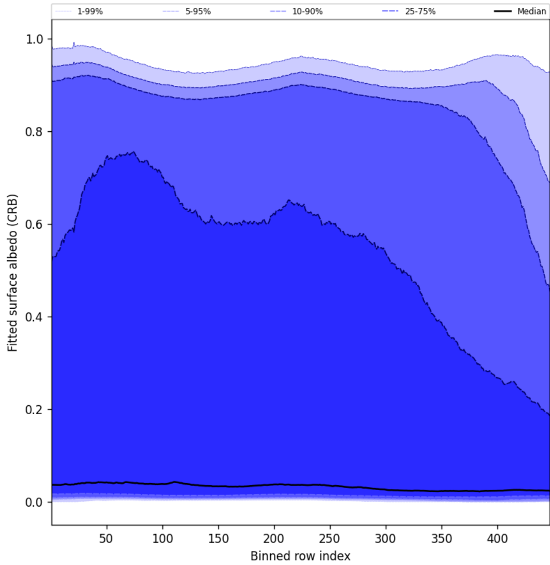
Figure 62: Along track statistics of “Fitted surface albedo (CRB)” for 2025-01-19 to 2025-01-21
