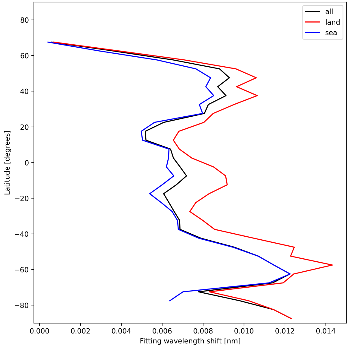
Figure 33: Zonal average of “Fitting wavelength shift” for 2025-01-19 to 2025-01-21.
