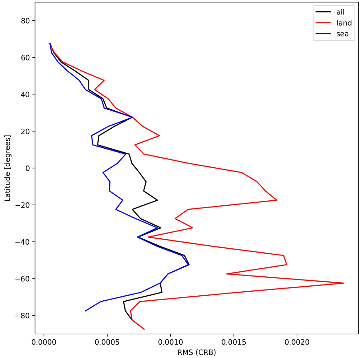
Figure 32: Zonal average of “RMS (CRB)” for 2025-01-19 to 2025-01-21.
