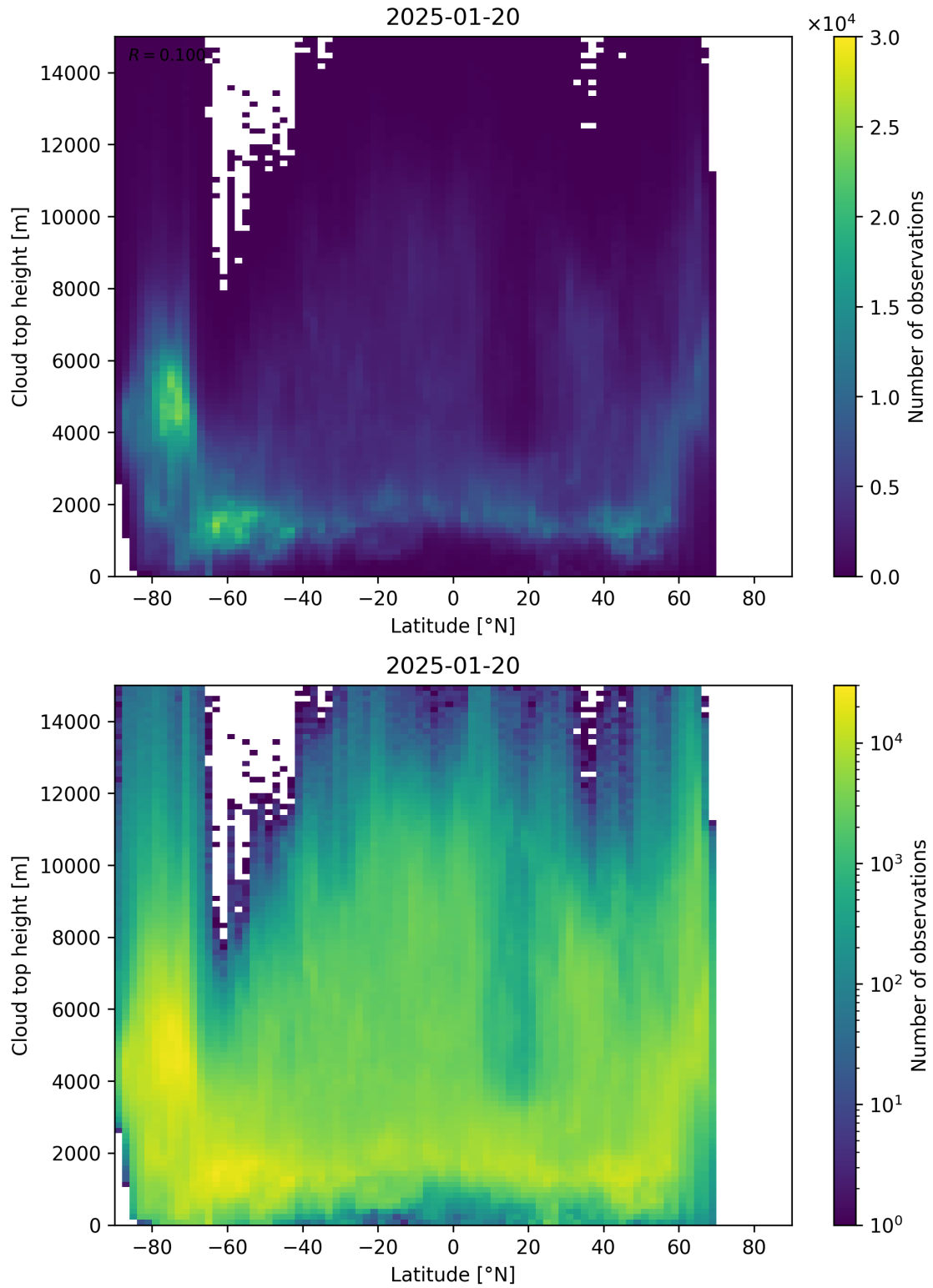
Figure 97: Scatter density plot of “Latitude” against “Cloud top height” for 2025-01-19 to 2025-01-21.
