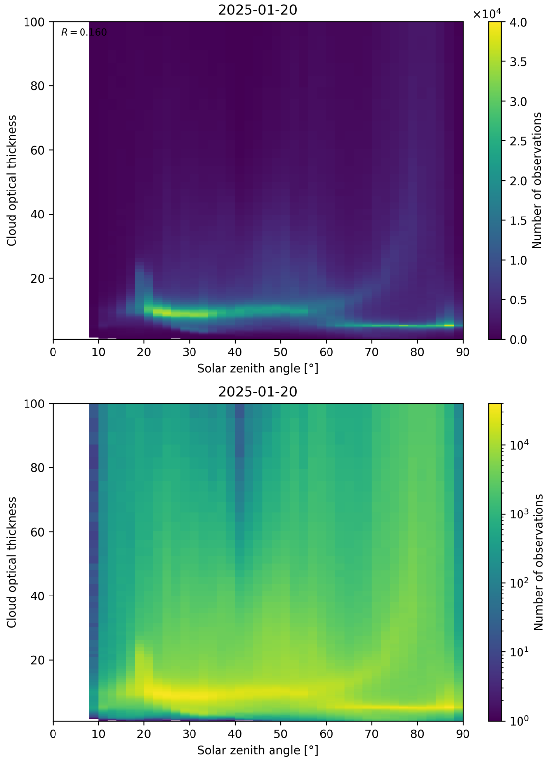
Figure 103: Scatter density plot of “Solar zenith angle” against “Cloud optical thickness” for 2025-01-19 to 2025-01-21.
