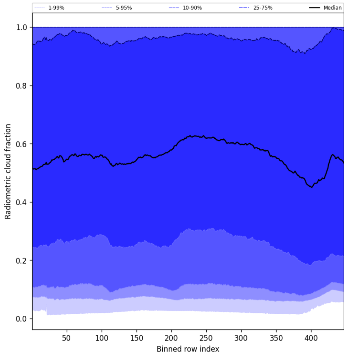
Figure 55: Along track statistics of “Radiometric cloud fraction” for 2025-01-19 to 2025-01-21
