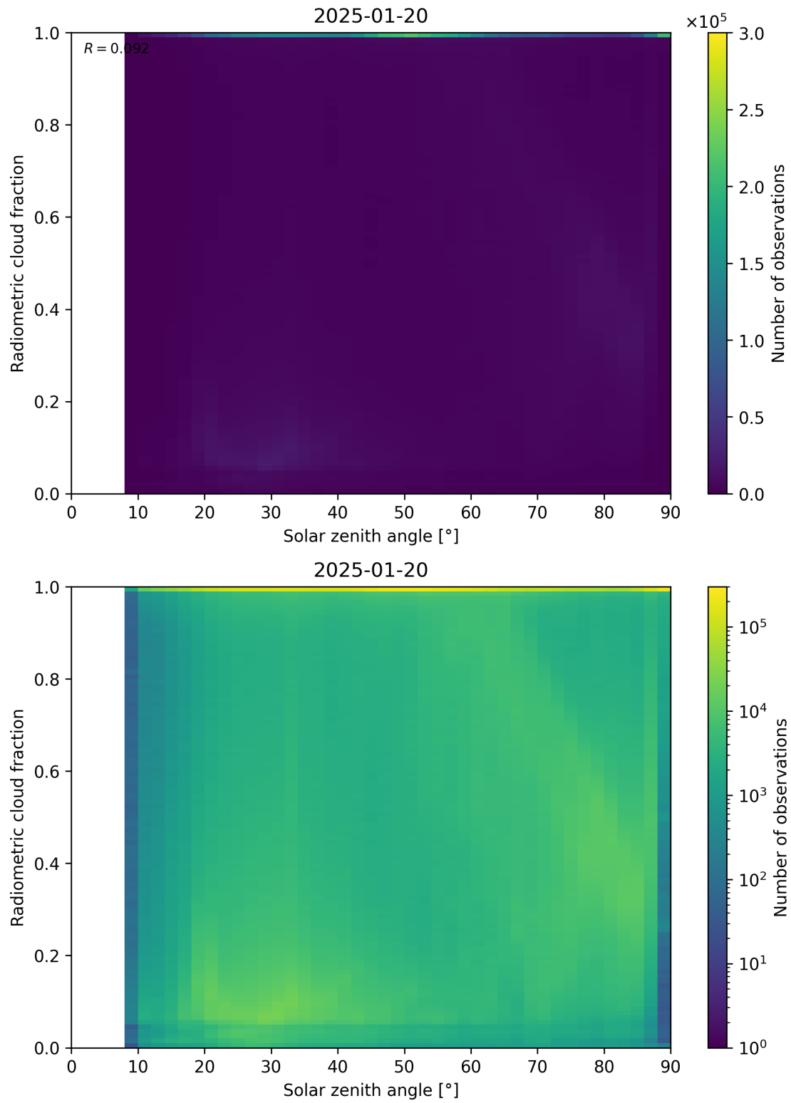
Figure 99: Scatter density plot of “Solar zenith angle” against “Radiometric cloud fraction” for 2025-01-19 to 2025-01-21.
