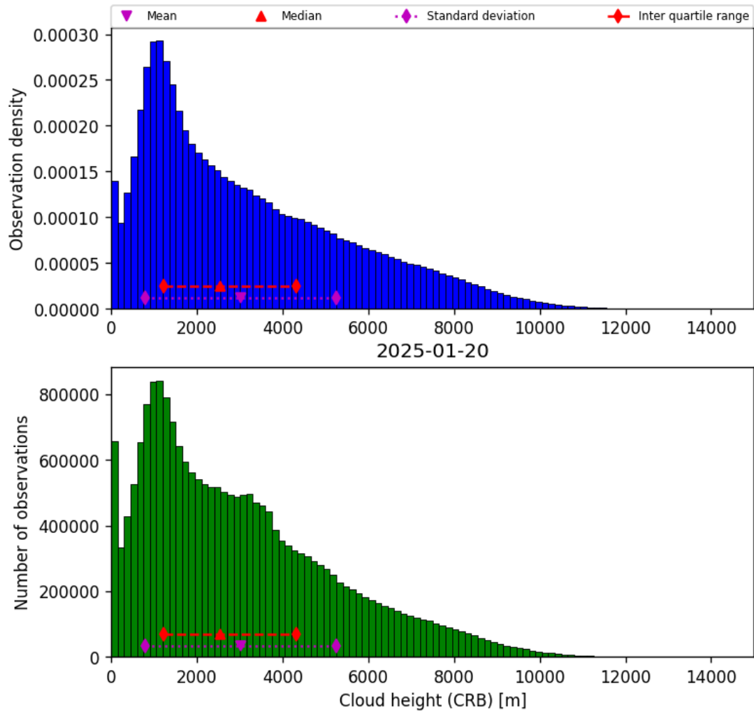
Figure 43: Histogram of “Cloud height (CRB)” for 2025-01-19 to 2025-01-21
