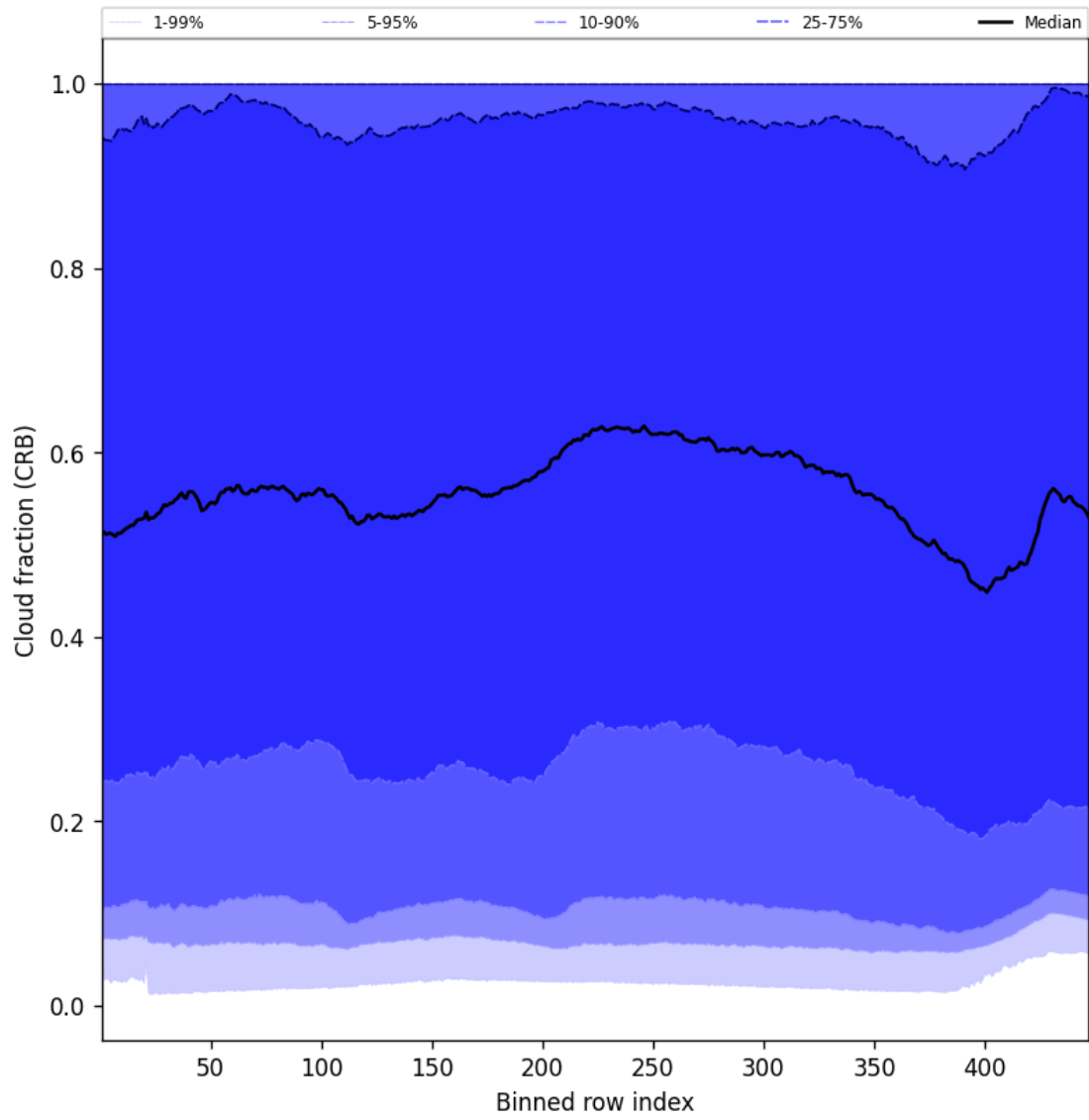
Figure 58: Along track statistics of “Cloud fraction (CRB)” for 2025-01-19 to 2025-01-21
