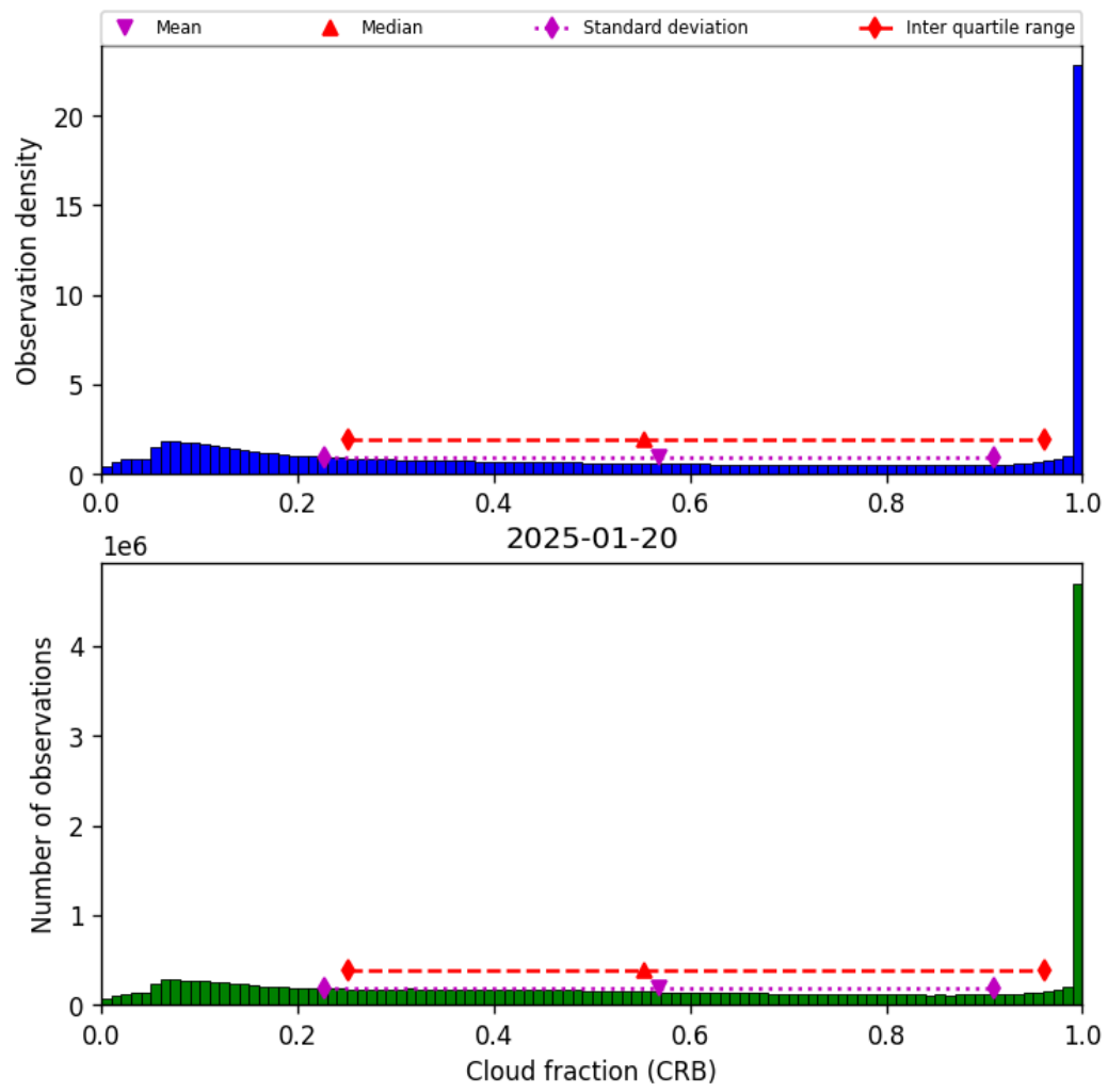
Figure 42: Histogram of “Cloud fraction (CRB)” for 2025-01-19 to 2025-01-21
