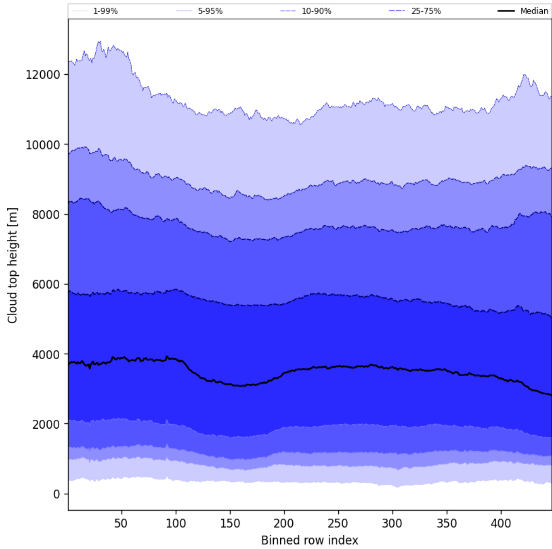
Figure 56: Along track statistics of “Cloud top height” for 2025-01-19 to 2025-01-21
