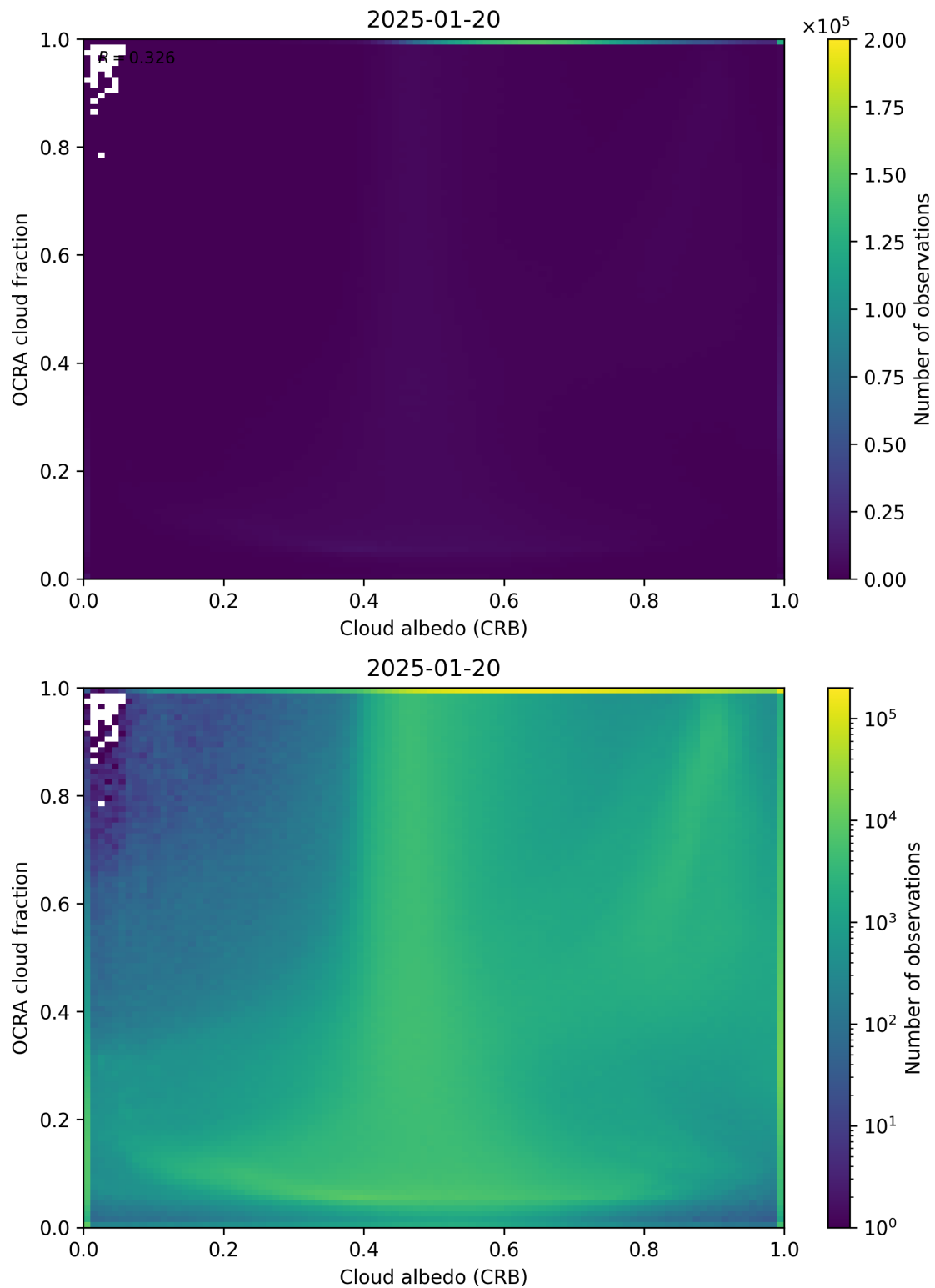
Figure 70: Scatter density plot of “Cloud albedo (CRB)” against “OCRA cloud fraction” for 2025-01-19 to 2025-01-21.
