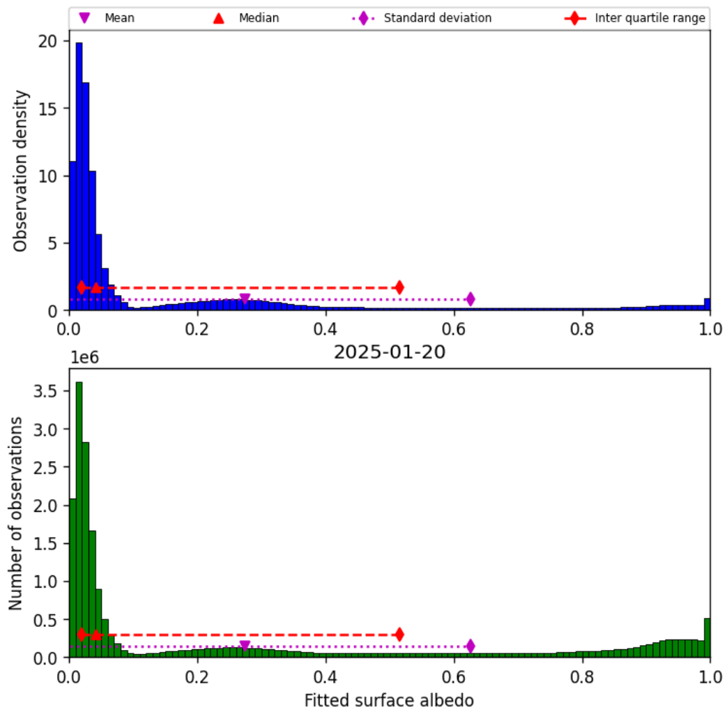
Figure 45: Histogram of “Fitted surface albedo” for 2025-01-19 to 2025-01-21
