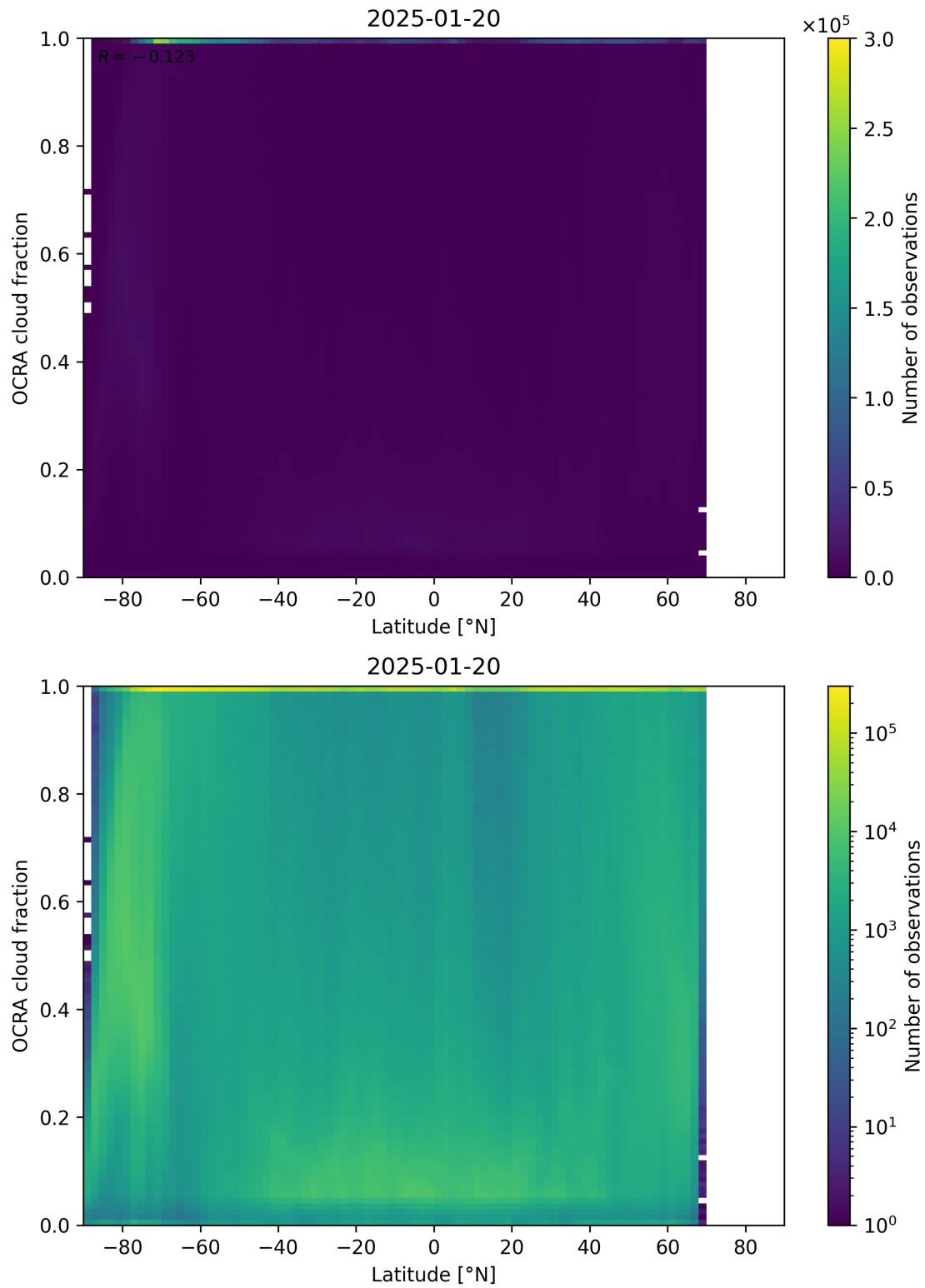
Figure 93: Scatter density plot of “Latitude” against “OCRA cloud fraction” for 2025-01-19 to 2025-01-21.
