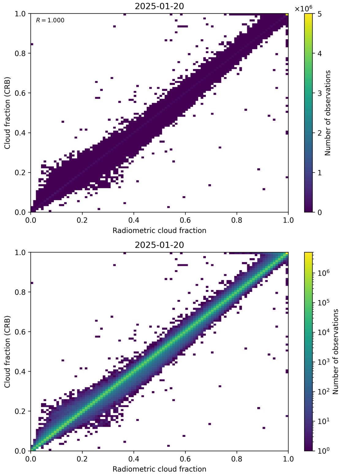
Figure 73: Scatter density plot of “Radiometric cloud fraction” against “Cloud fraction (CRB)” for 2025-01-19 to 2025-01-21.
