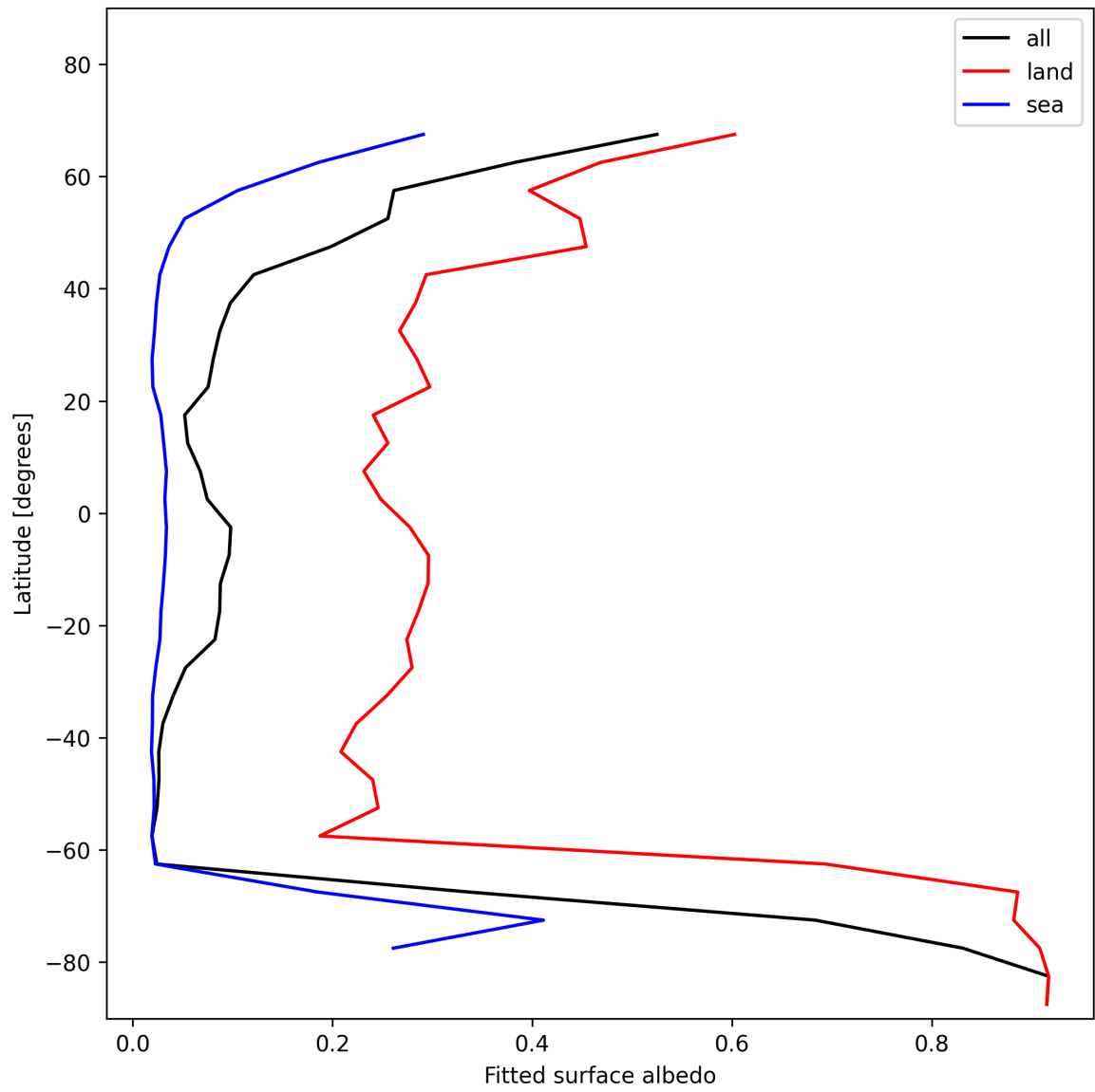
Figure 29: Zonal average of “Fitted surface albedo” for 2025-01-19 to 2025-01-21.
