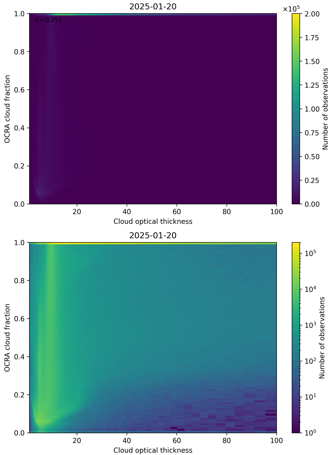
Figure 83: Scatter density plot of “Cloud optical thickness” against “OCRA cloud fraction” for 2025-01-19 to 2025-01-21.
