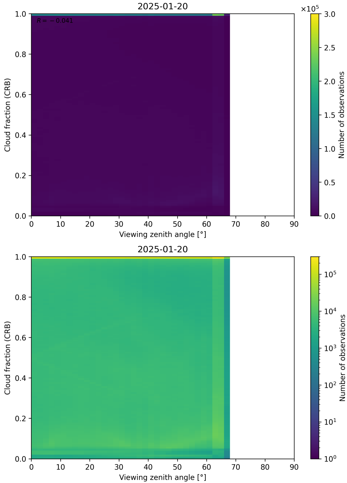
Figure 109: Scatter density plot of “Viewing zenith angle” against “Cloud fraction (CRB)” for 2025-01-19 to 2025-01-21.
