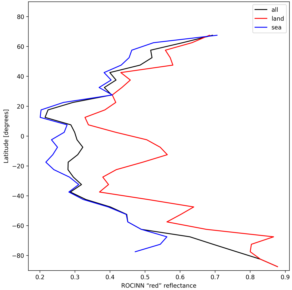
Figure 37: Zonal average of “ROCINN “red” reflectance” for 2025-01-19 to 2025-01-21.
