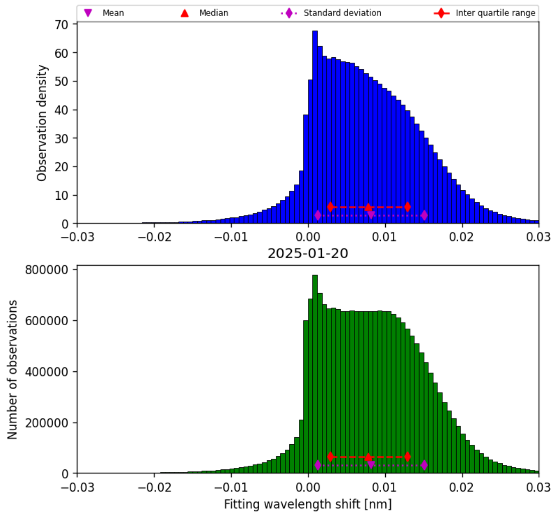
Figure 49: Histogram of “Fitting wavelength shift” for 2025-01-19 to 2025-01-21
