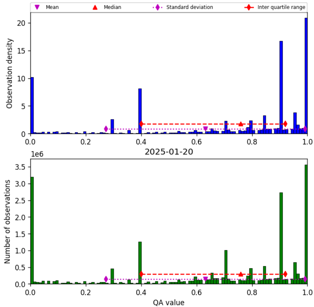
Figure 38: Histogram of “QA value” for 2025-01-19 to 2025-01-21
