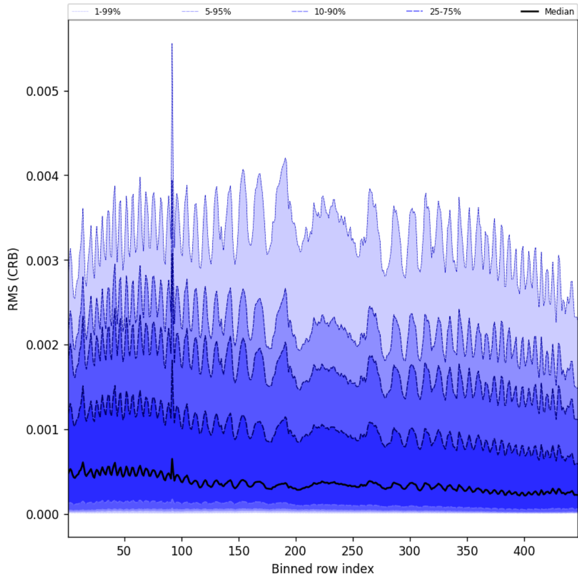
Figure 64: Along track statistics of “RMS (CRB)” for 2025-01-19 to 2025-01-21
