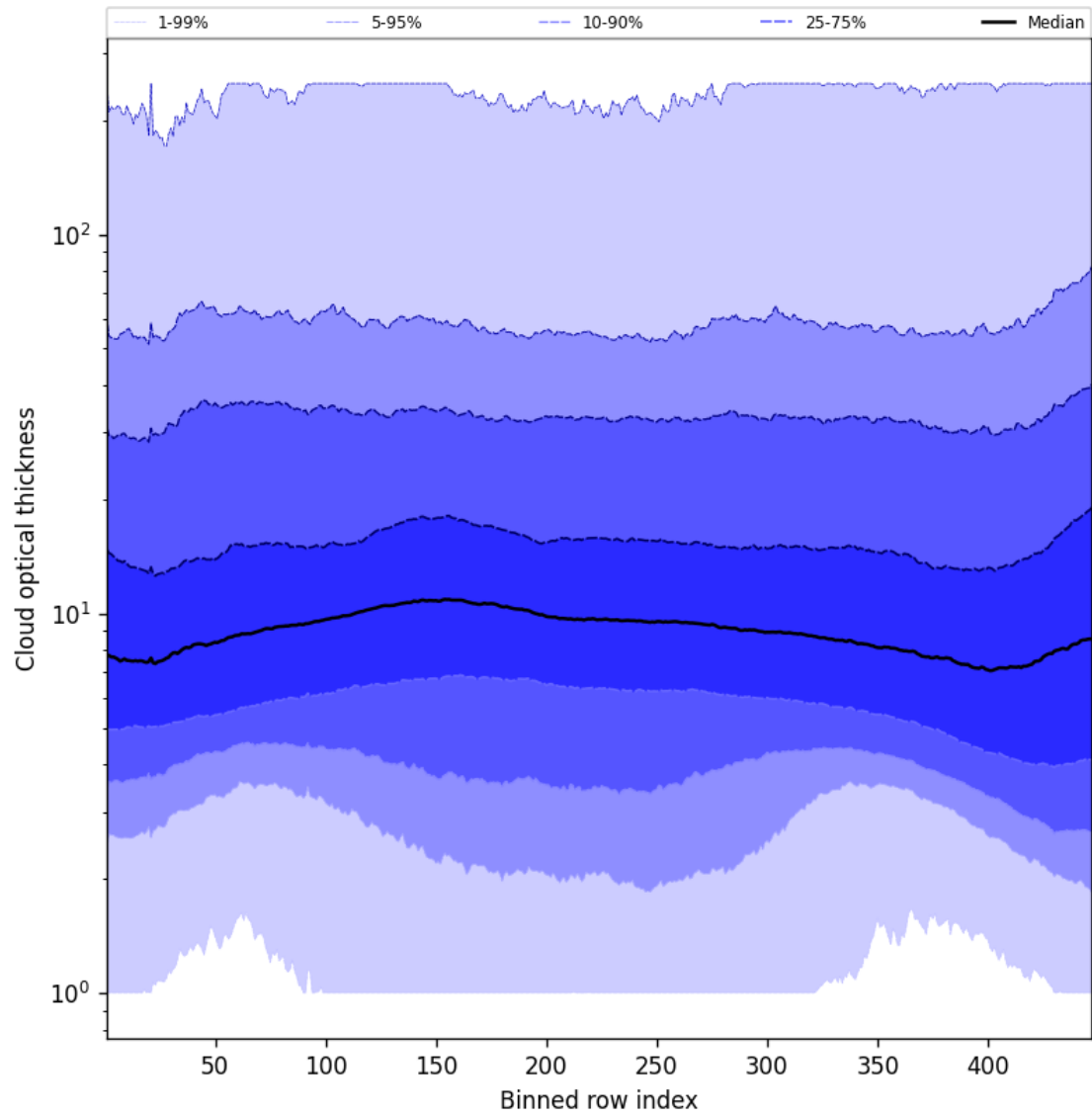
Figure 57: Along track statistics of “Cloud optical thickness” for 2025-01-19 to 2025-01-21
