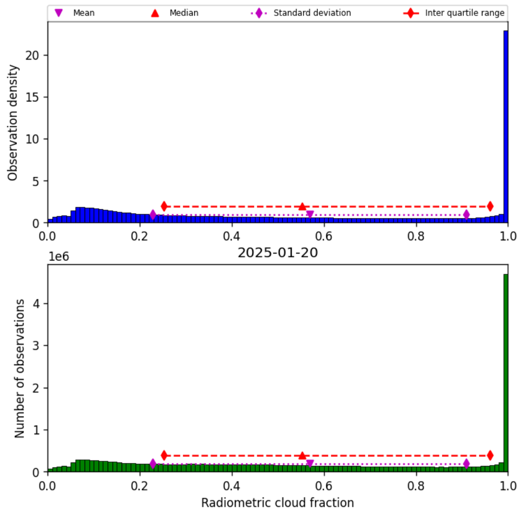
Figure 39: Histogram of “Radiometric cloud fraction” for 2025-01-19 to 2025-01-21
