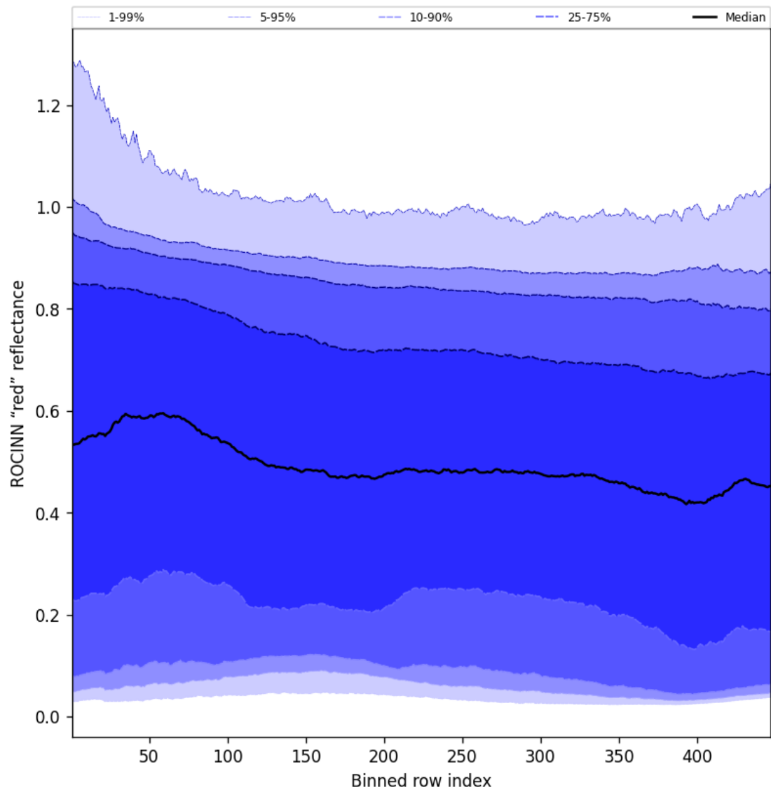
Figure 69: Along track statistics of "ROCINN "red" reflectance" for 2025-01-19 to 2025-01-21
