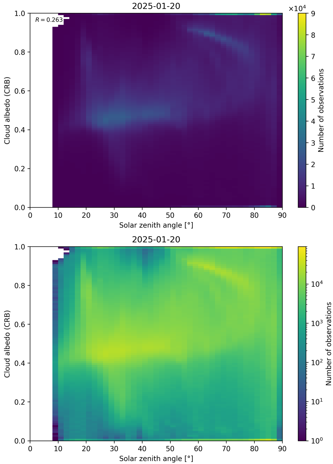
Figure 98: Scatter density plot of “Solar zenith angle” against “Cloud albedo (CRB)” for 2025-01-19 to 2025-01-21.
