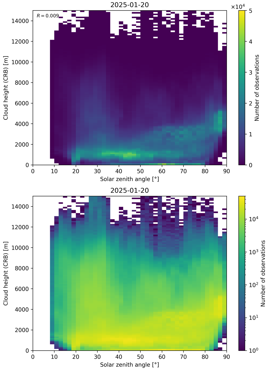
Figure 102: Scatter density plot of “Solar zenith angle” against “Cloud height (CRB)” for 2025-01-19 to 2025-01-21.
