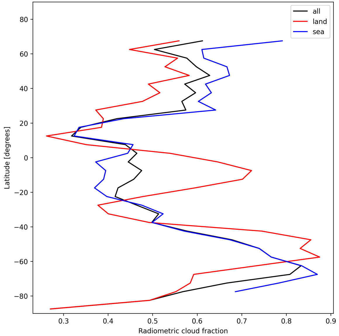
Figure 23: Zonal average of “Radiometric cloud fraction” for 2025-01-19 to 2025-01-21.
