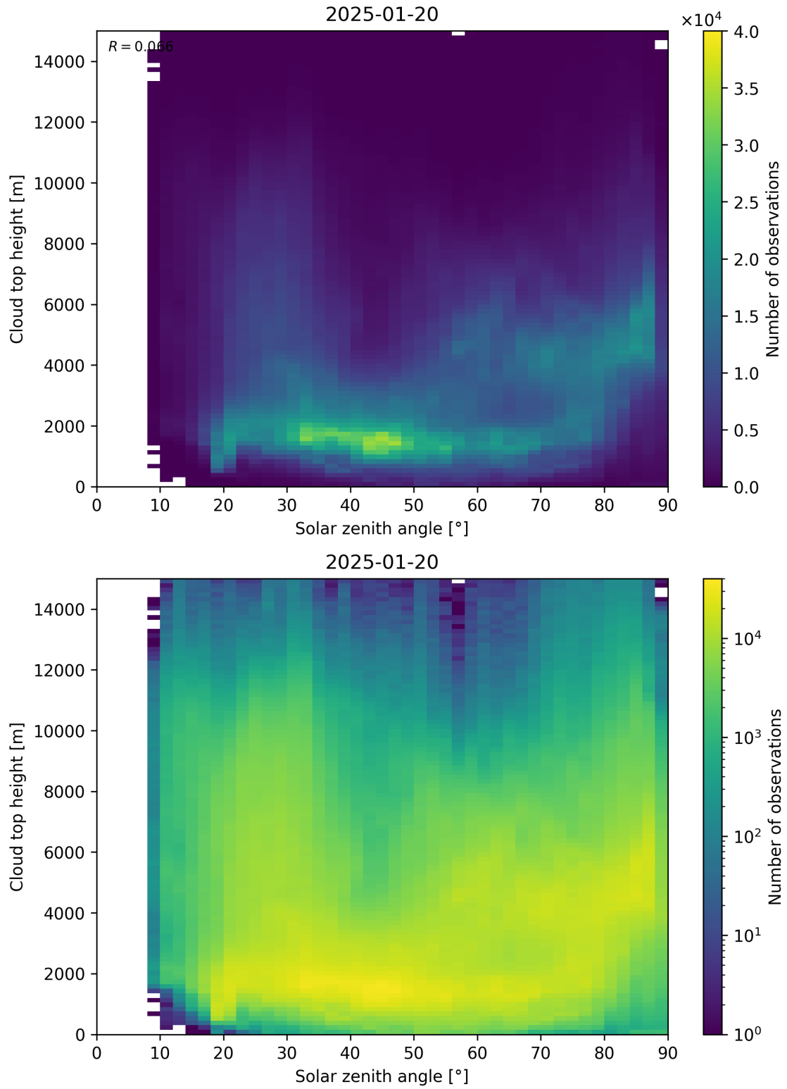
Figure 104: Scatter density plot of “Solar zenith angle” against “Cloud top height” for 2025-01-19 to 2025-01-21.
