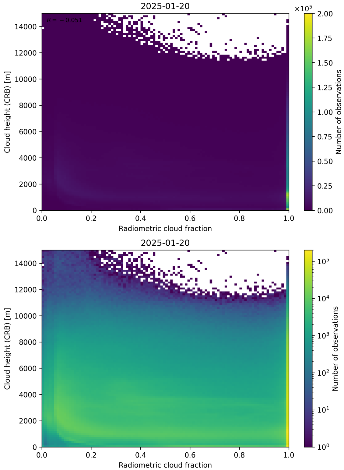
Figure 74: Scatter density plot of “Radiometric cloud fraction” against “Cloud height (CRB)” for 2025-01-19 to 2025-01-21.
