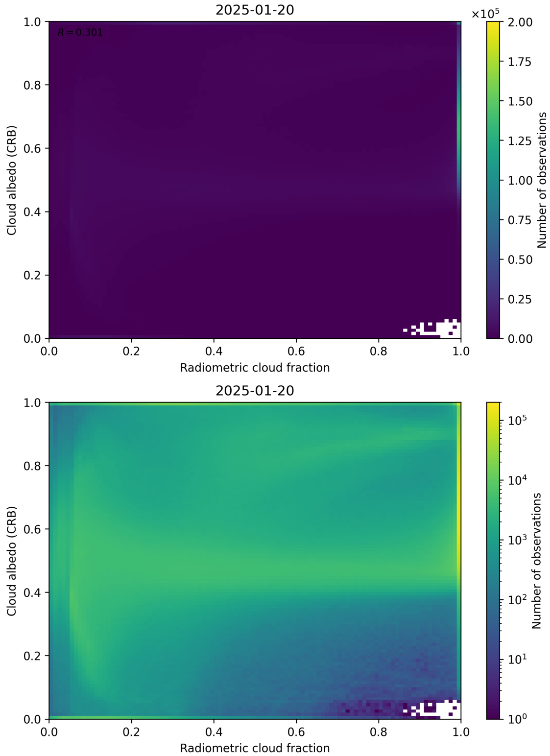
Figure 71: Scatter density plot of “Radiometric cloud fraction” against “Cloud albedo (CRB)” for 2025-01-19 to 2025-01-21.
