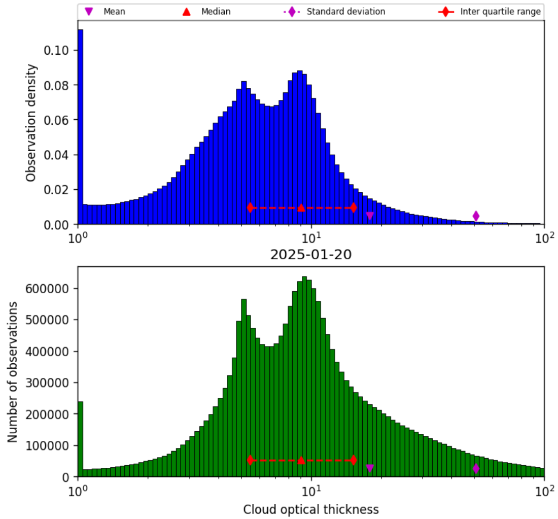
Figure 41: Histogram of “Cloud optical thickness” for 2025-01-19 to 2025-01-21
