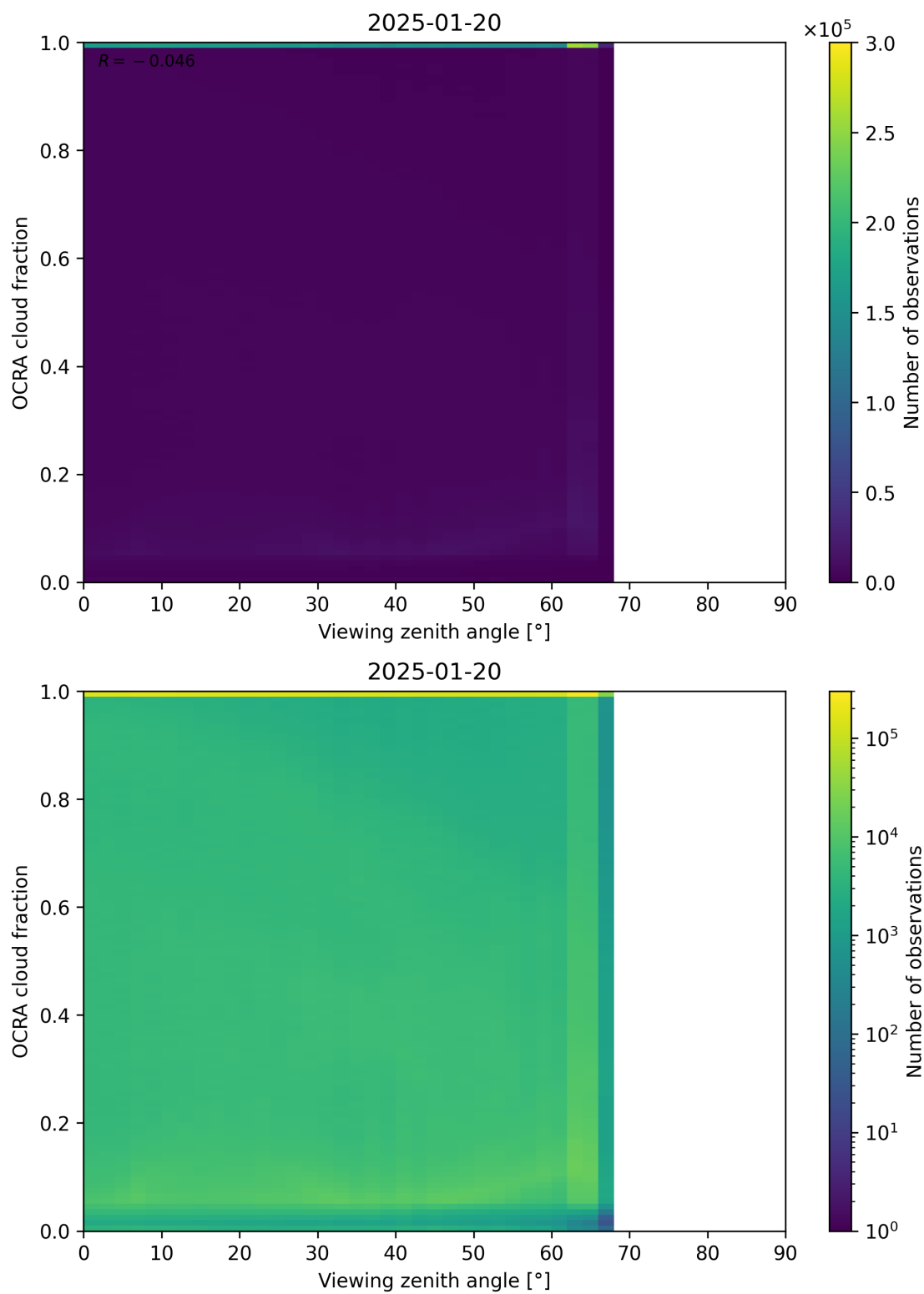
Figure 108: Scatter density plot of “Viewing zenith angle” against “OCRA cloud fraction” for 2025-01-19 to 2025-01-21.
