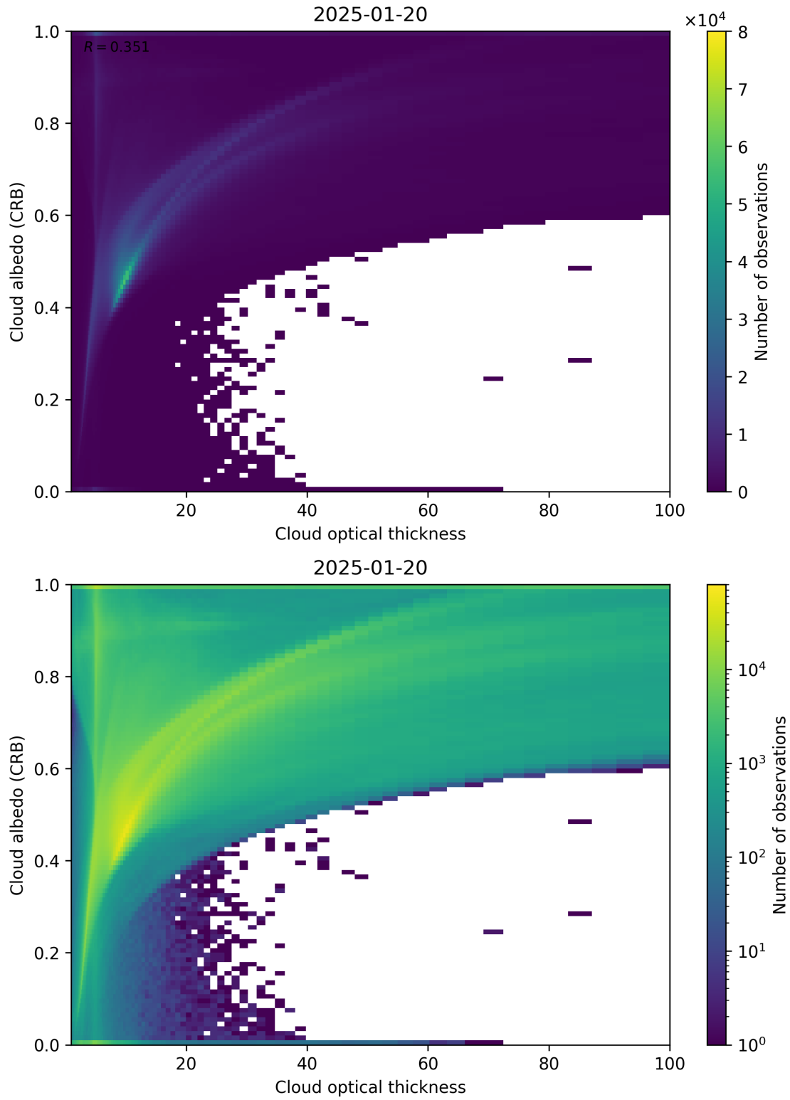
Figure 82: Scatter density plot of “Cloud optical thickness” against “Cloud albedo (CRB)” for 2025-01-19 to 2025-01-21.
