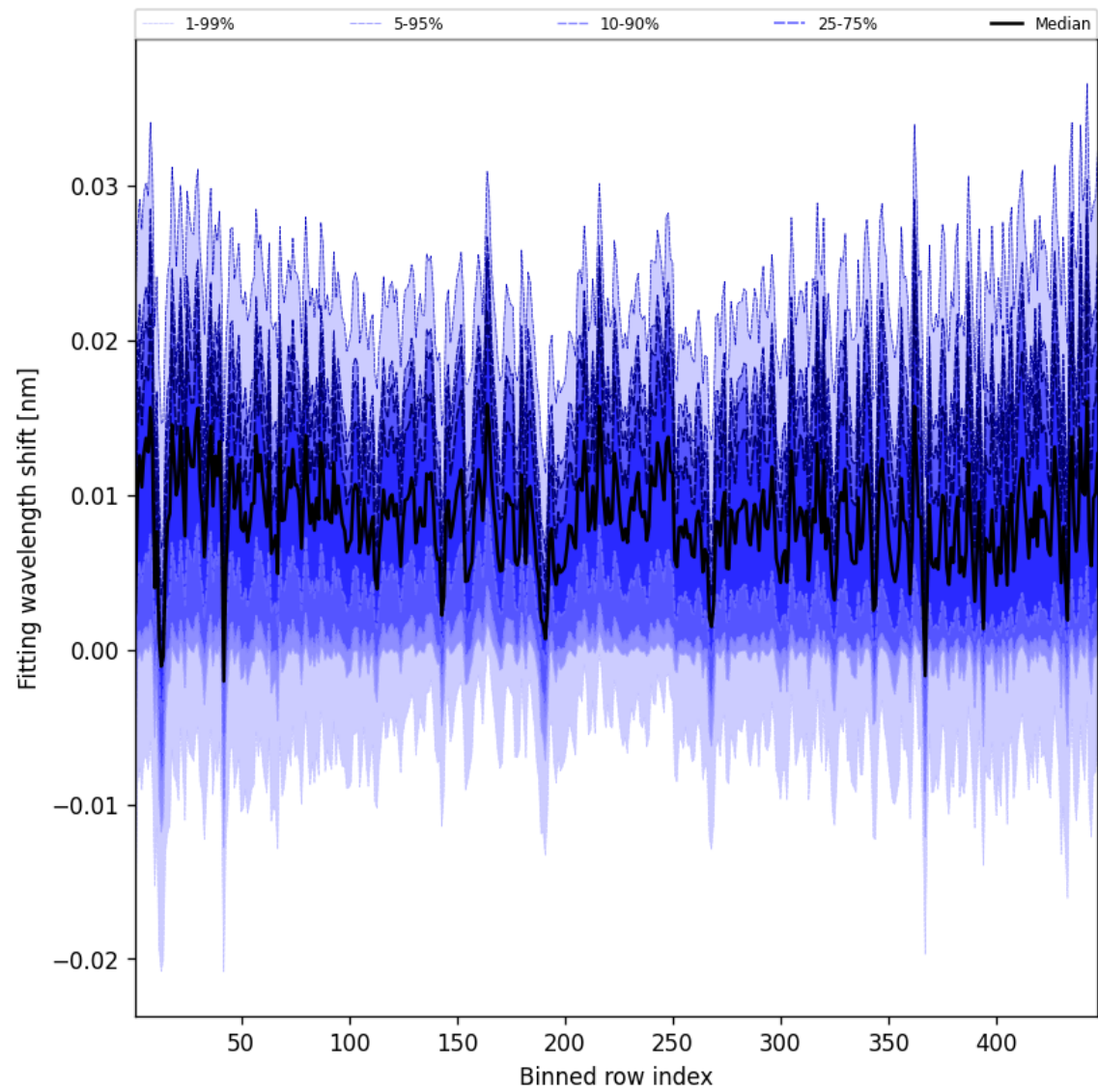
Figure 65: Along track statistics of “Fitting wavelength shift” for 2025-01-19 to 2025-01-21
