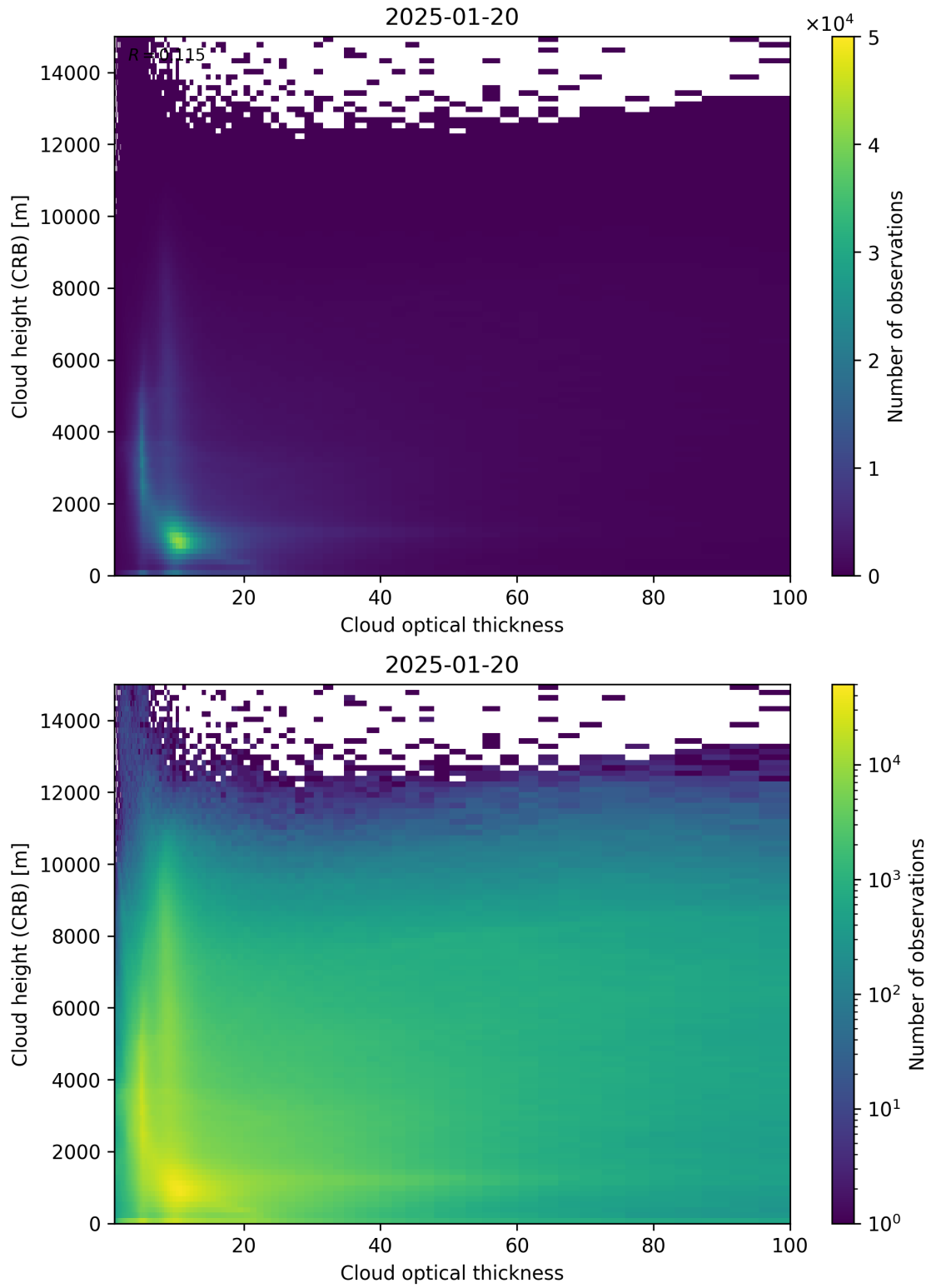
Figure 85: Scatter density plot of “Cloud optical thickness” against “Cloud height (CRB)” for 2025-01-19 to 2025-01-21.
