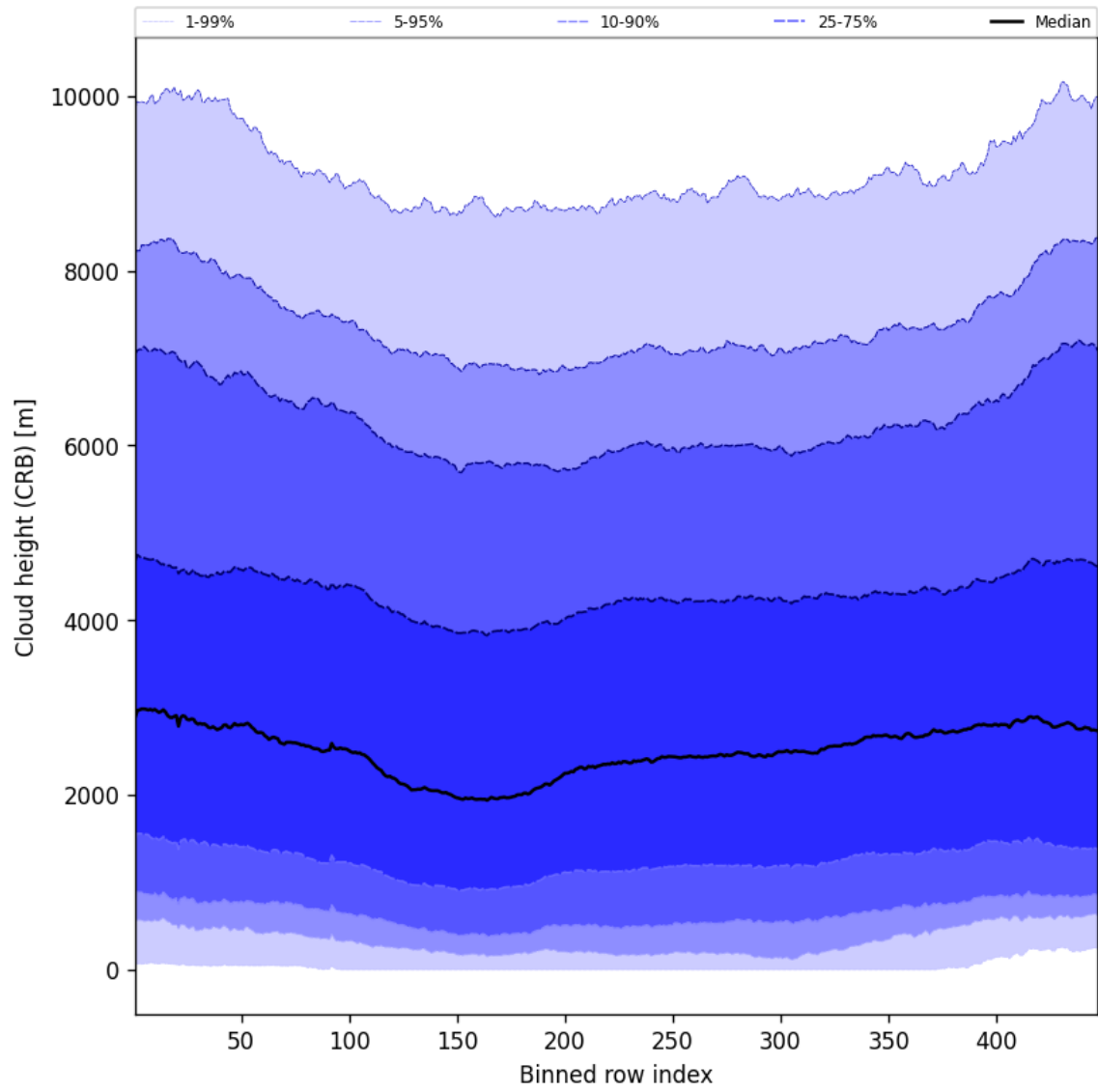
Figure 59: Along track statistics of “Cloud height (CRB)” for 2025-01-19 to 2025-01-21
