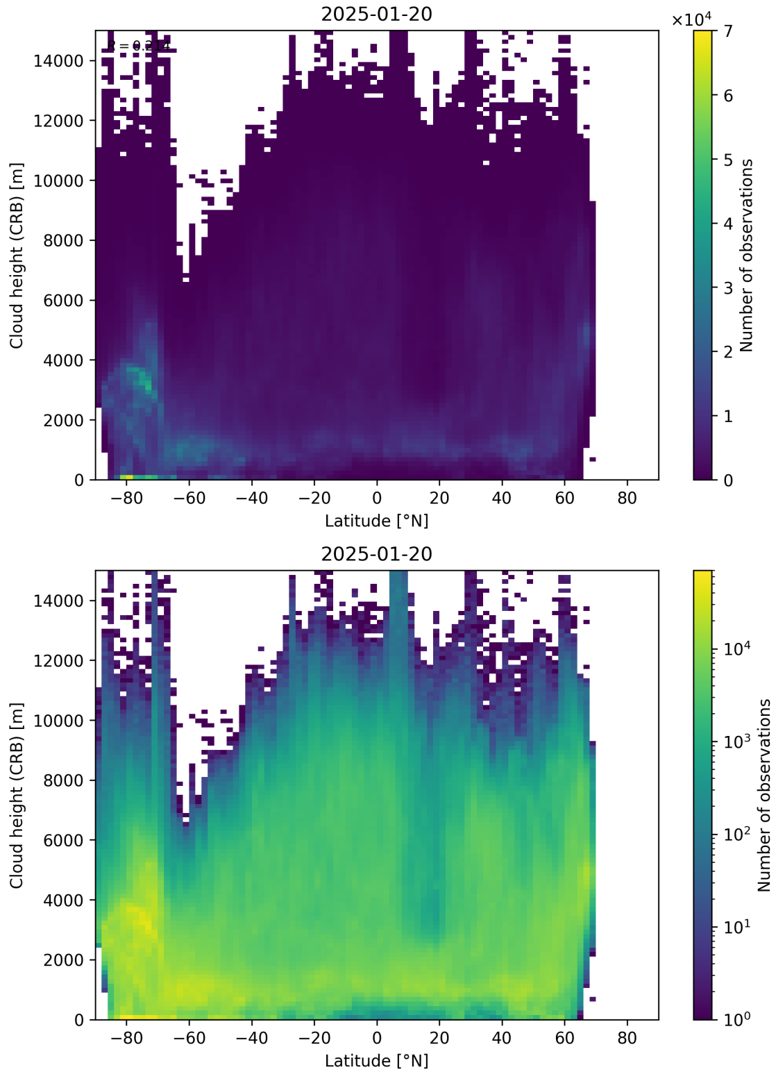
Figure 95: Scatter density plot of “Latitude” against “Cloud height (CRB)” for 2025-01-19 to 2025-01-21.
