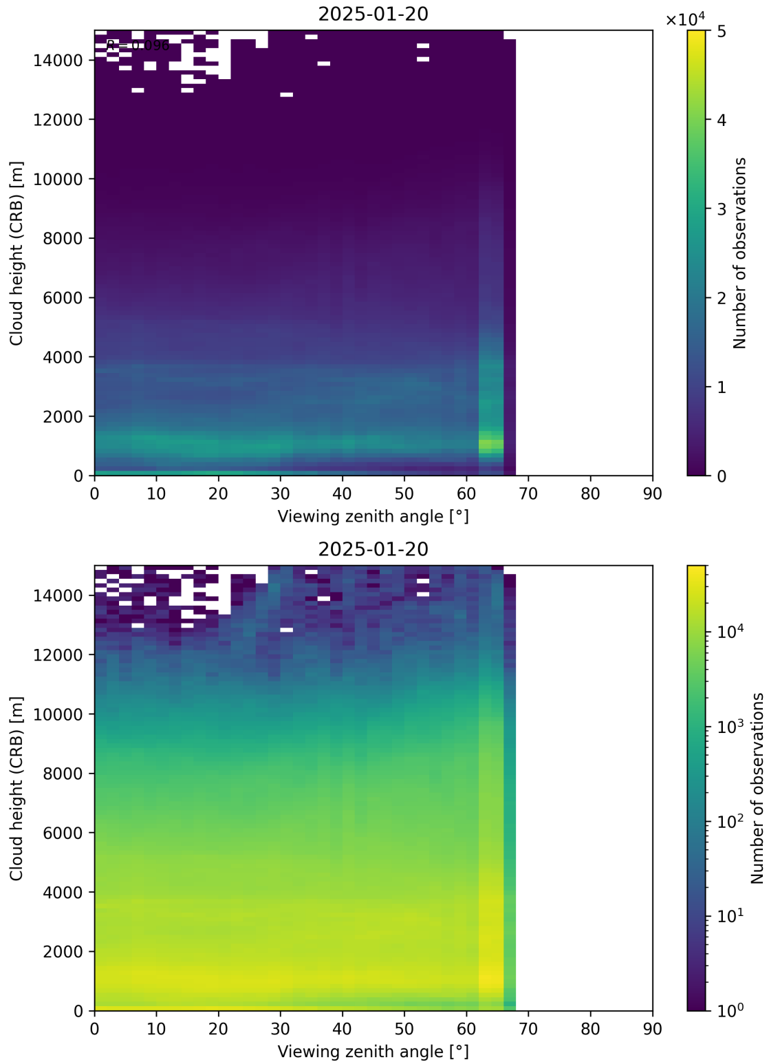
Figure 110: Scatter density plot of “Viewing zenith angle” against “Cloud height (CRB)” for 2025-01-19 to 2025-01-21.
