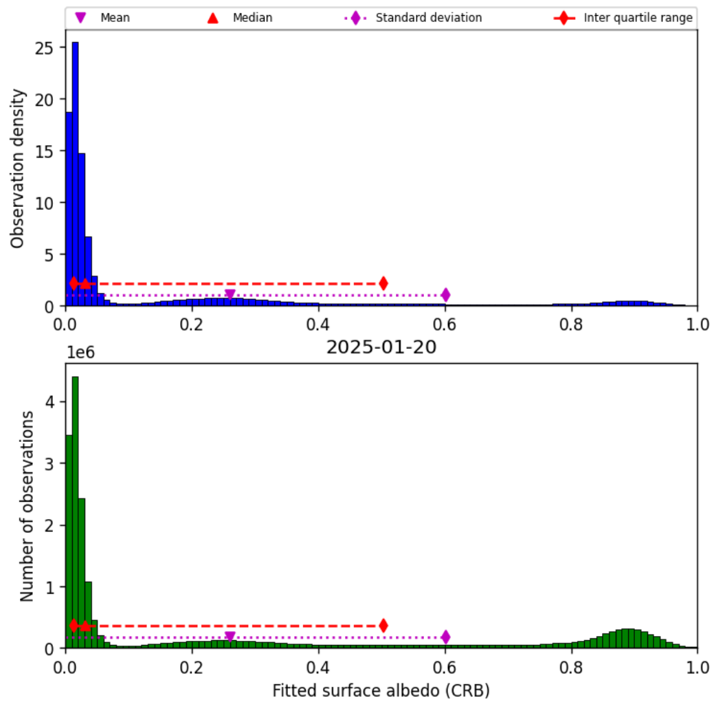
Figure 46: Histogram of “Fitted surface albedo (CRB)” for 2025-01-19 to 2025-01-21
