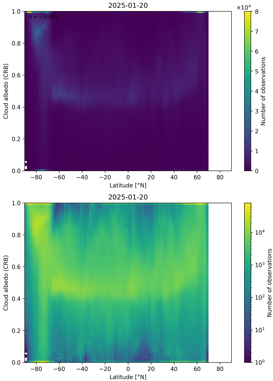
Figure 91: Scatter density plot of “Latitude” against “Cloud albedo (CRB)” for 2025-01-19 to 2025-01-21.
