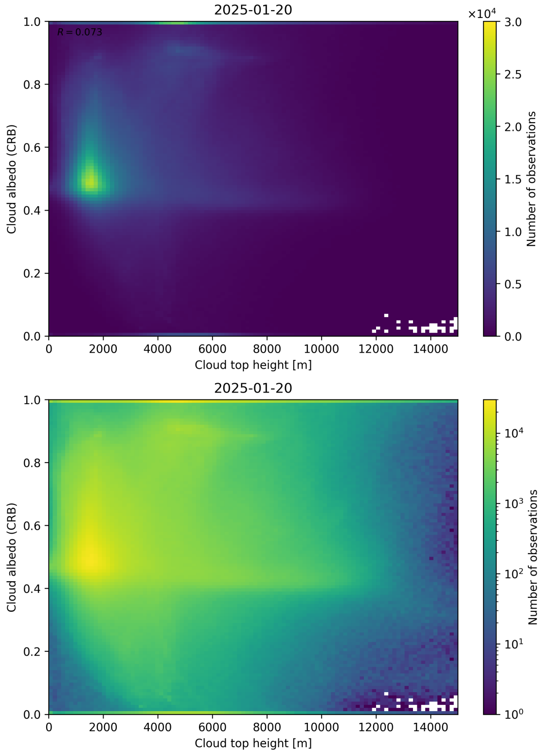
Figure 86: Scatter density plot of “Cloud top height” against “Cloud albedo (CRB)” for 2025-01-19 to 2025-01-21.
