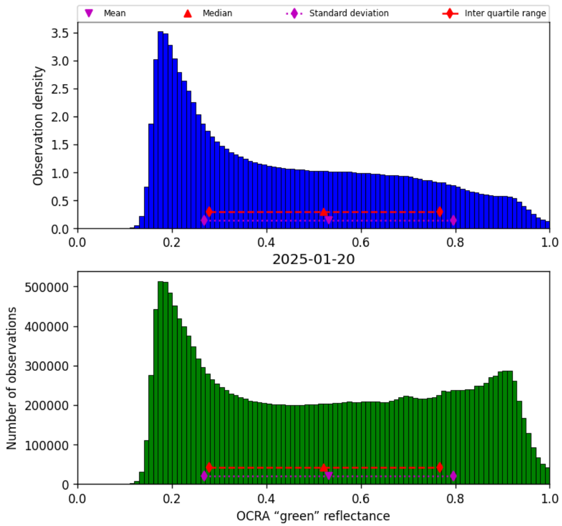
Figure 52: Histogram of “OCRA “green” reflectance” for 2025-01-19 to 2025-01-21
