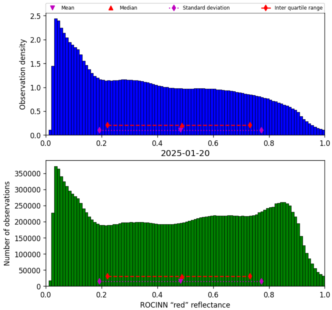
Figure 53: Histogram of “ROCINN “red” reflectance” for 2025-01-19 to 2025-01-21
