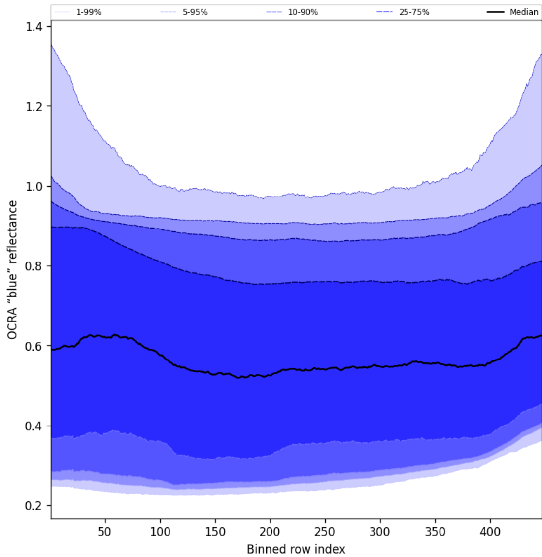
Figure 67: Along track statistics of "OCRA "blue" reflectance" for 2025-01-19 to 2025-01-21
