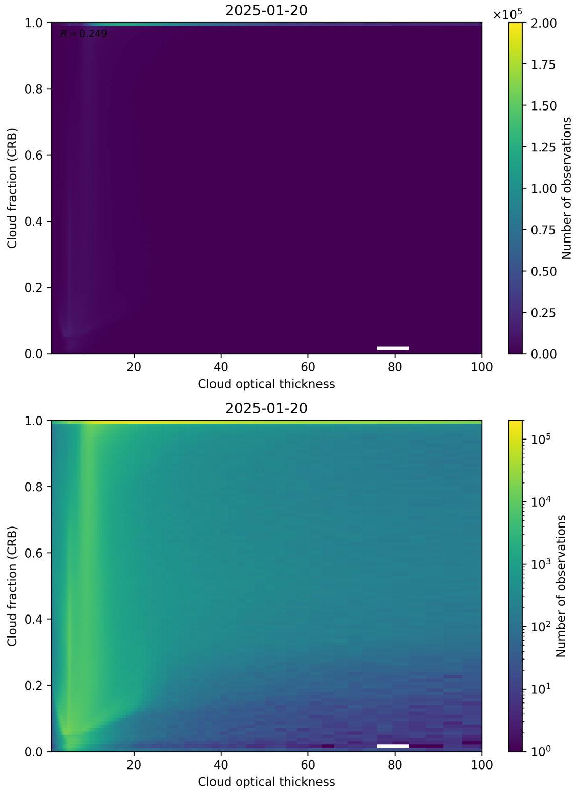
Figure 84: Scatter density plot of “Cloud optical thickness” against “Cloud fraction (CRB)” for 2025-01-19 to 2025-01-21.
