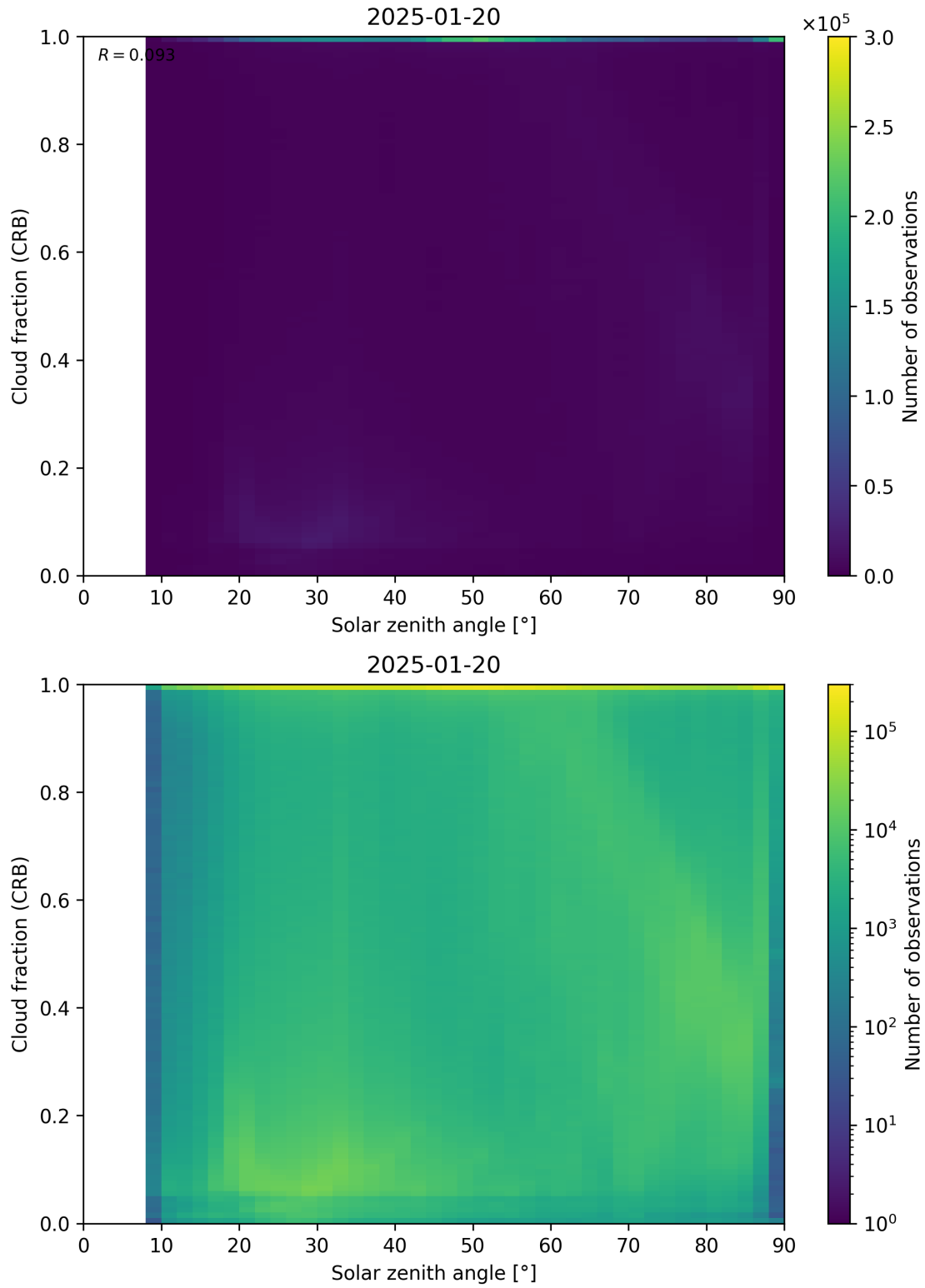
Figure 101: Scatter density plot of “Solar zenith angle” against “Cloud fraction (CRB)” for 2025-01-19 to 2025-01-21.
