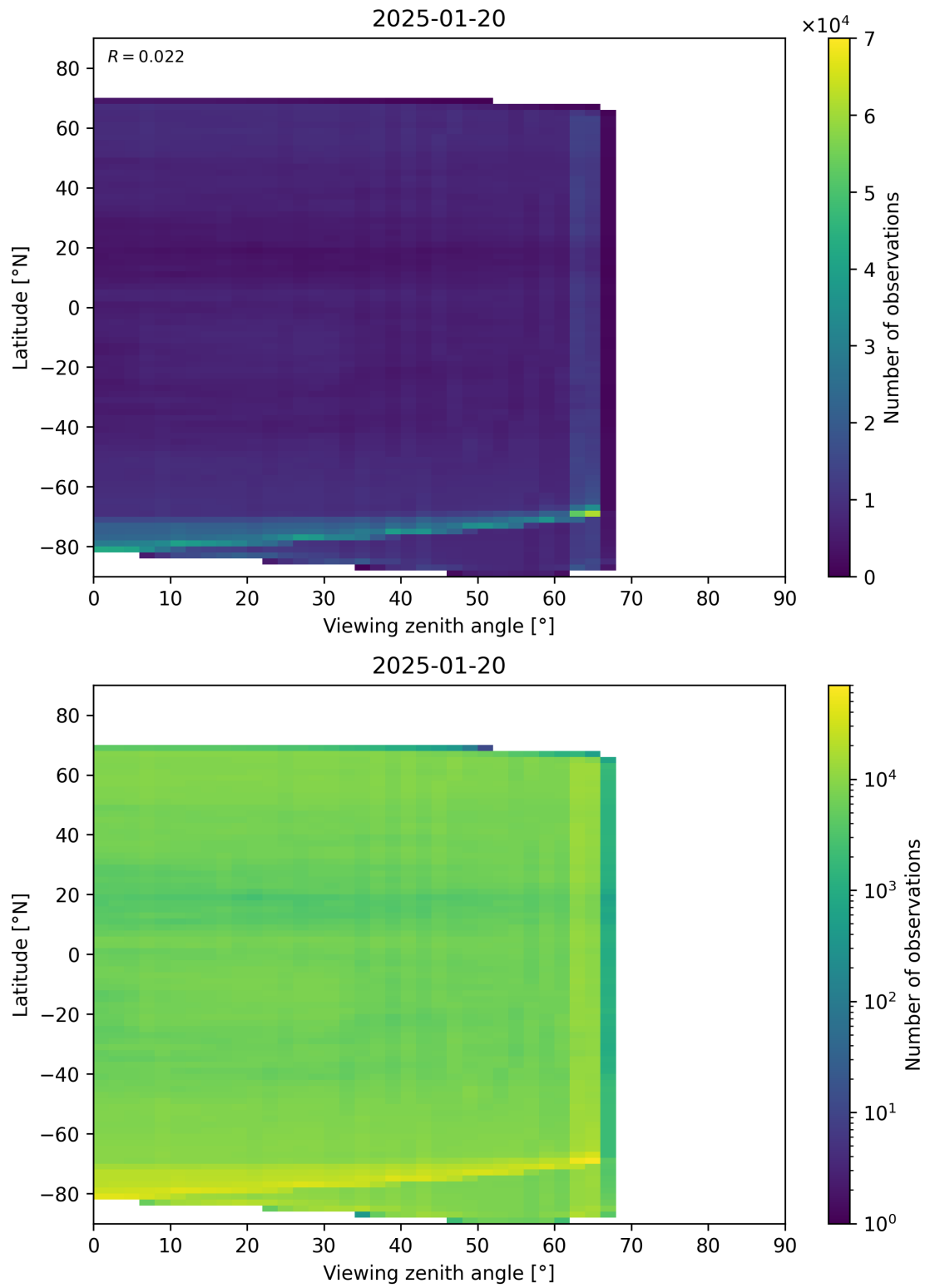
Figure 113: Scatter density plot of “Viewing zenith angle” against “Latitude” for 2025-01-19 to 2025-01-21.
