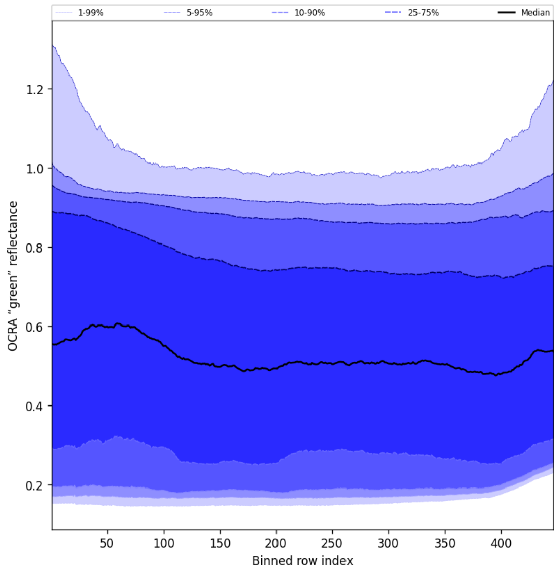
Figure 68: Along track statistics of “OCRA “green” reflectance” for 2025-01-19 to 2025-01-21
