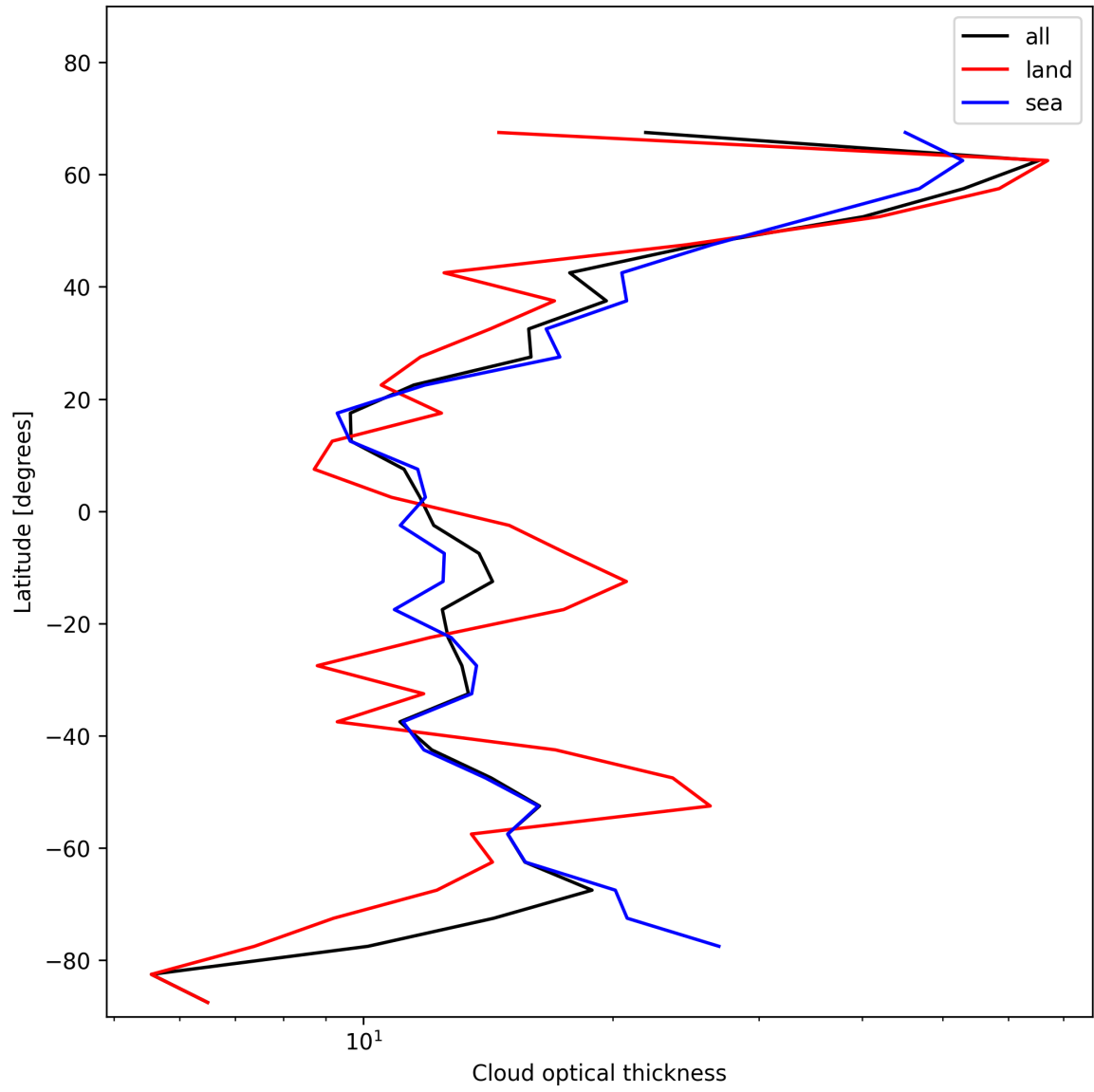
Figure 25: Zonal average of “Cloud optical thickness” for 2025-01-19 to 2025-01-21.
