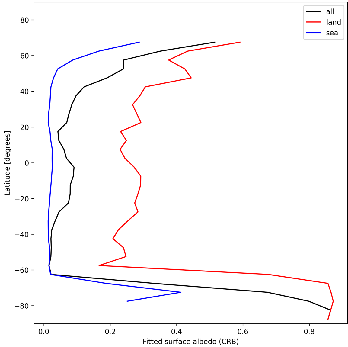
Figure 30: Zonal average of “Fitted surface albedo (CRB)” for 2025-01-19 to 2025-01-21.
