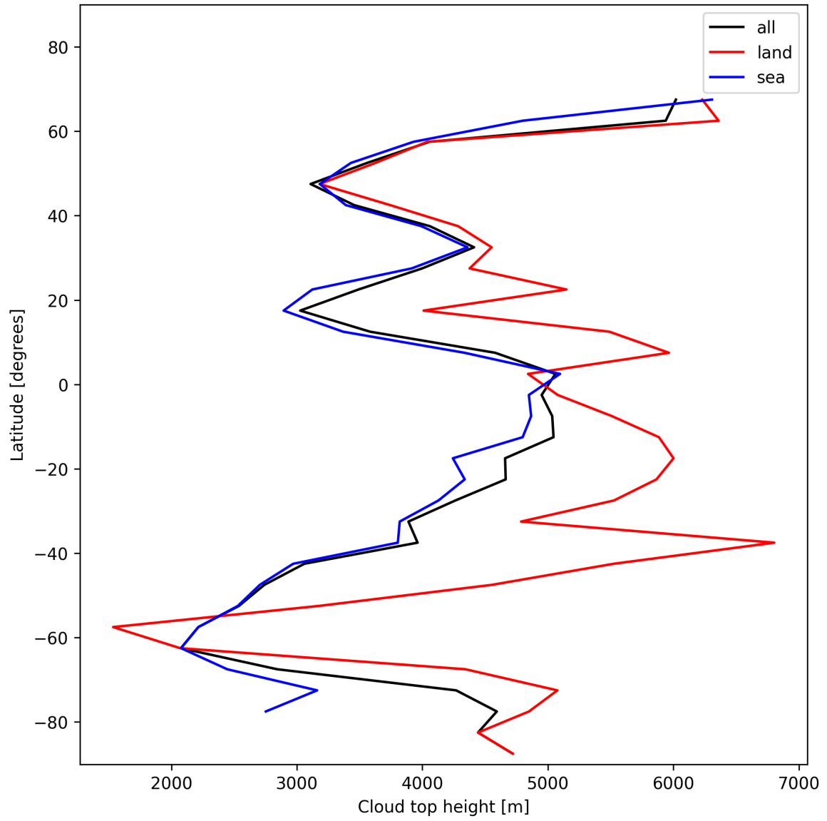
Figure 24: Zonal average of “Cloud top height” for 2025-01-19 to 2025-01-21.
