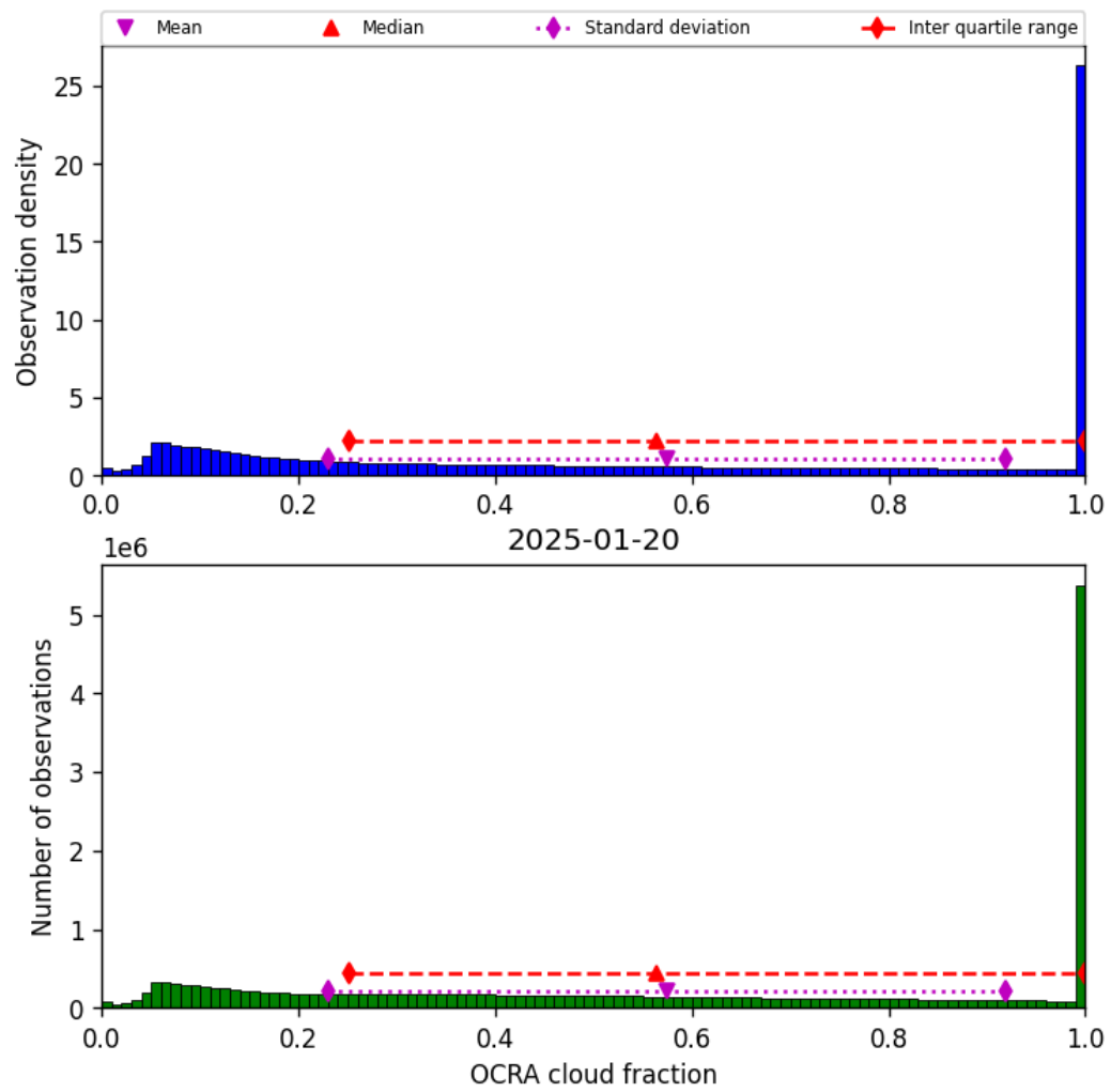
Figure 50: Histogram of “OCRA cloud fraction” for 2025-01-19 to 2025-01-21
