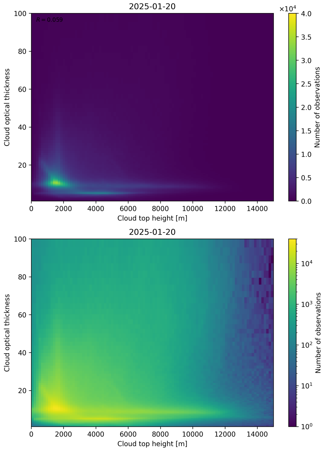
Figure 90: Scatter density plot of “Cloud top height” against “Cloud optical thickness” for 2025-01-19 to 2025-01-21.
