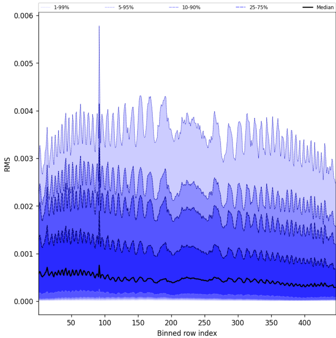
Figure 63: Along track statistics of “RMS” for 2025-01-19 to 2025-01-21
