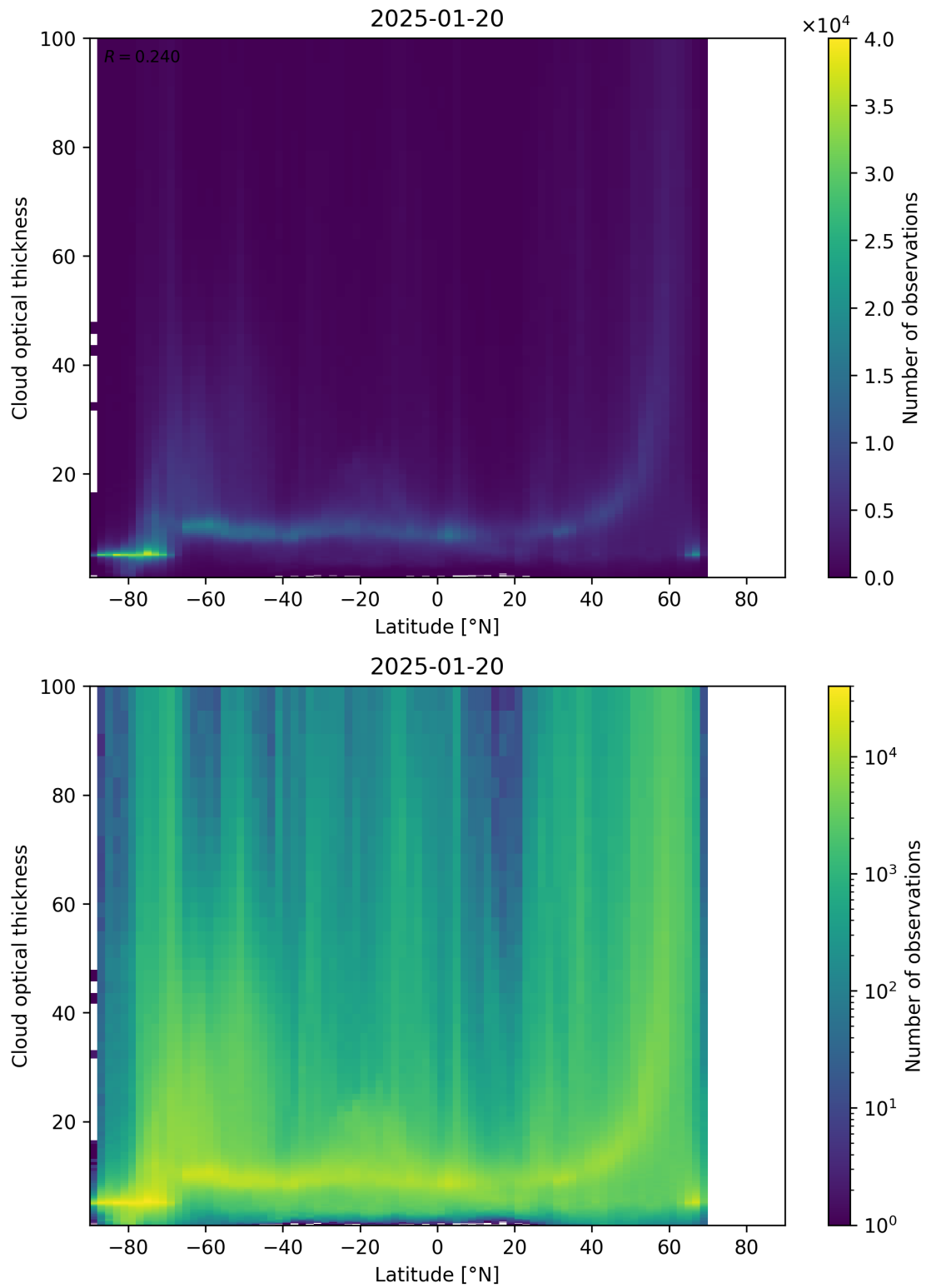
Figure 96: Scatter density plot of “Latitude” against “Cloud optical thickness” for 2025-01-19 to 2025-01-21.
