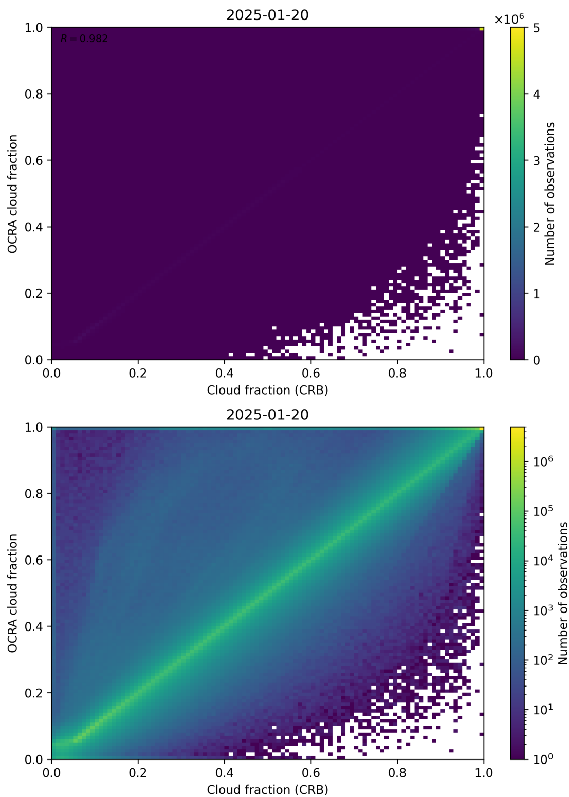
Figure 78: Scatter density plot of “Cloud fraction (CRB)” against “OCRA cloud fraction” for 2025-01-19 to 2025-01-21.
