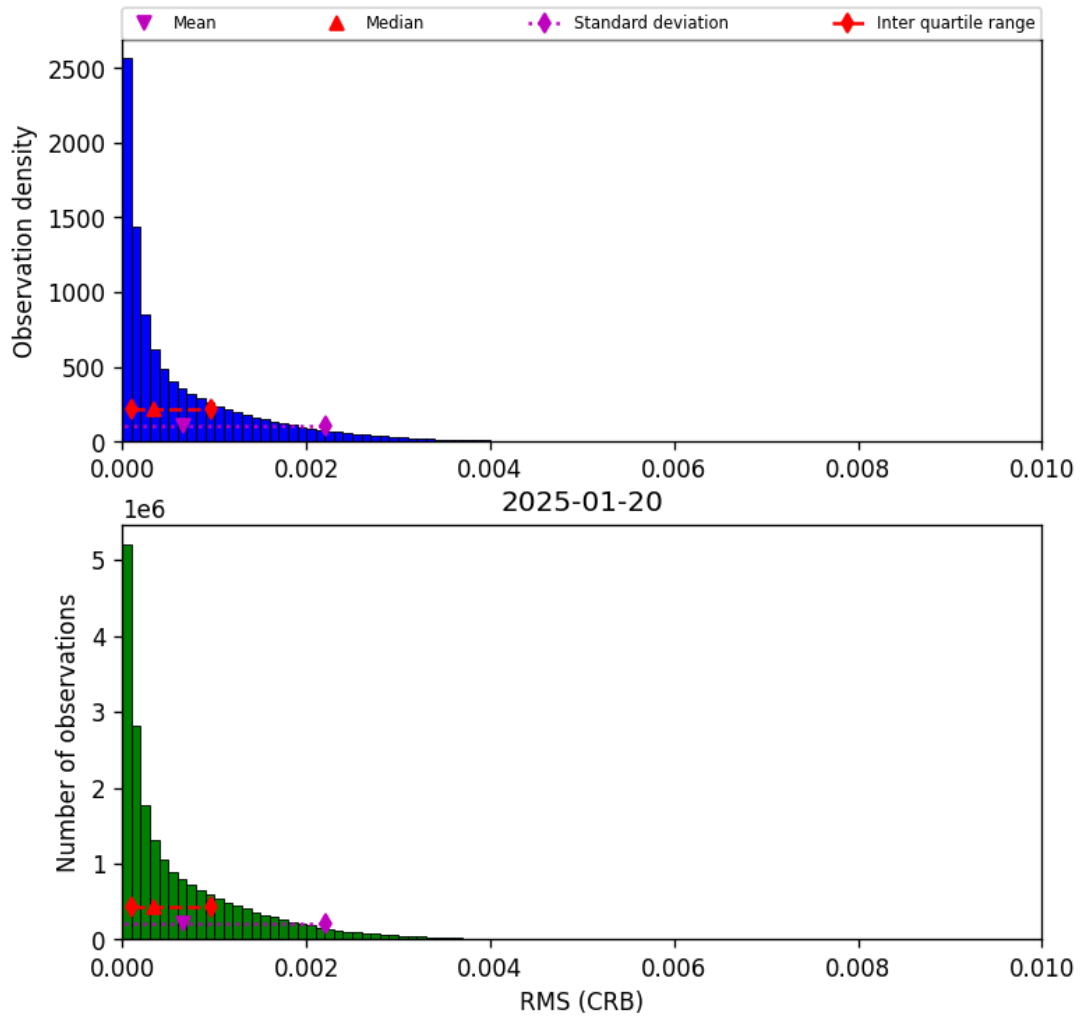
Figure 48: Histogram of “RMS (CRB)” for 2025-01-19 to 2025-01-21
