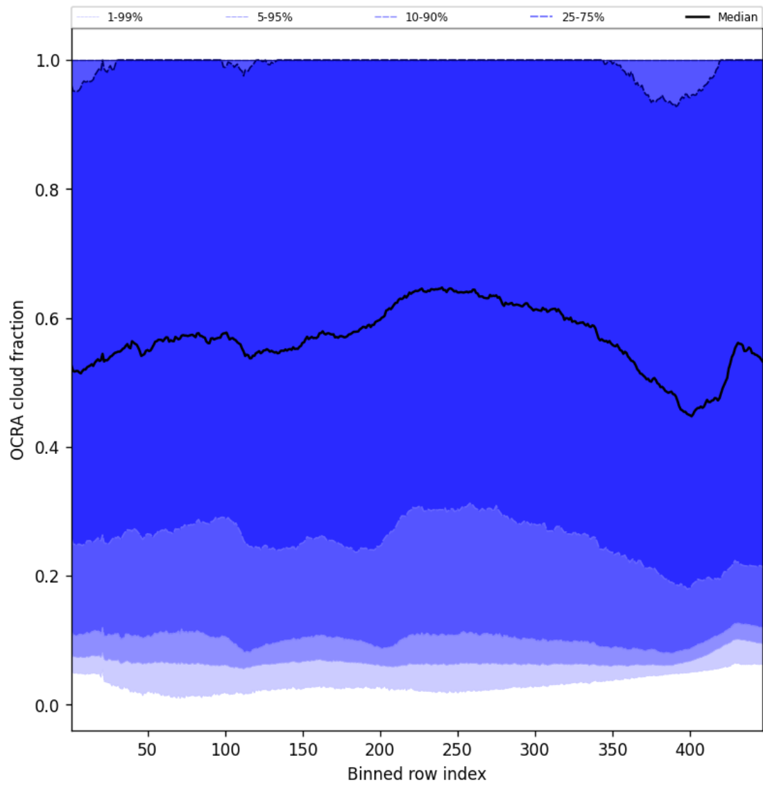
Figure 66: Along track statistics of “OCRA cloud fraction” for 2025-01-19 to 2025-01-21
