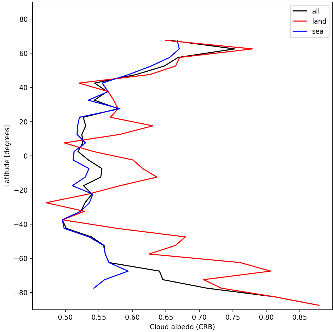
Figure 28: Zonal average of “Cloud albedo (CRB)” for 2025-01-19 to 2025-01-21.
