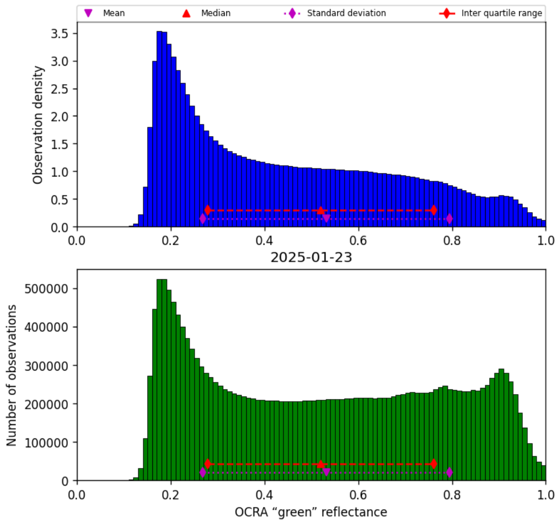
Figure 52: Histogram of “OCRA “green” reflectance” for 2025-01-23 to 2025-01-24
