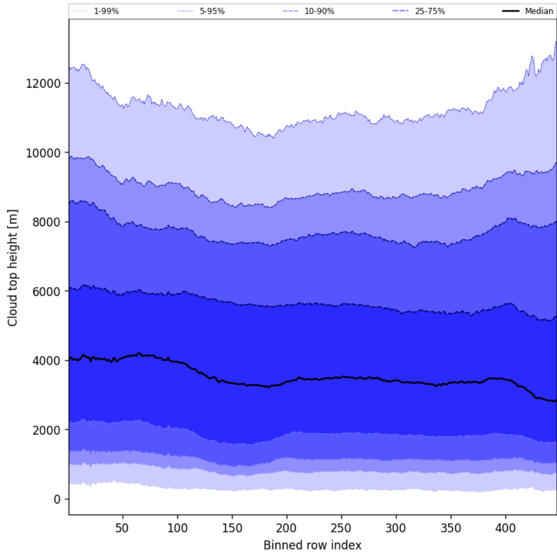
Figure 56: Along track statistics of “Cloud top height” for 2025-01-23 to 2025-01-24
