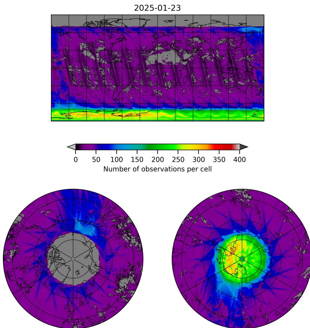
Figure 21: Map of the number of observations for 2025-01-23 to 2025-01-24
