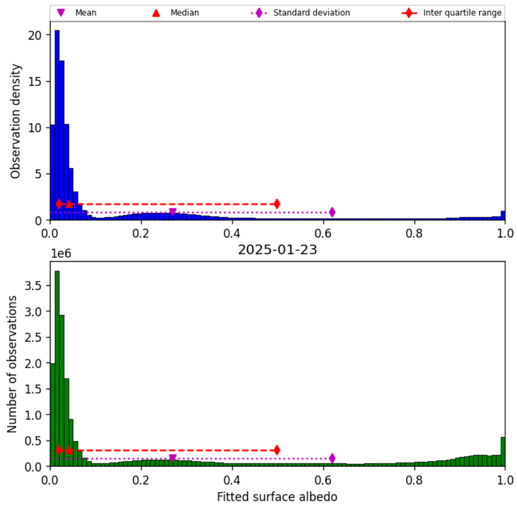
Figure 45: Histogram of “Fitted surface albedo” for 2025-01-23 to 2025-01-24
