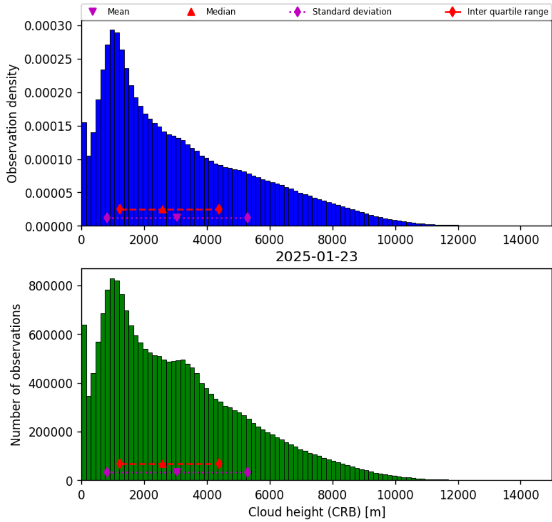
Figure 43: Histogram of “Cloud height (CRB)” for 2025-01-23 to 2025-01-24
