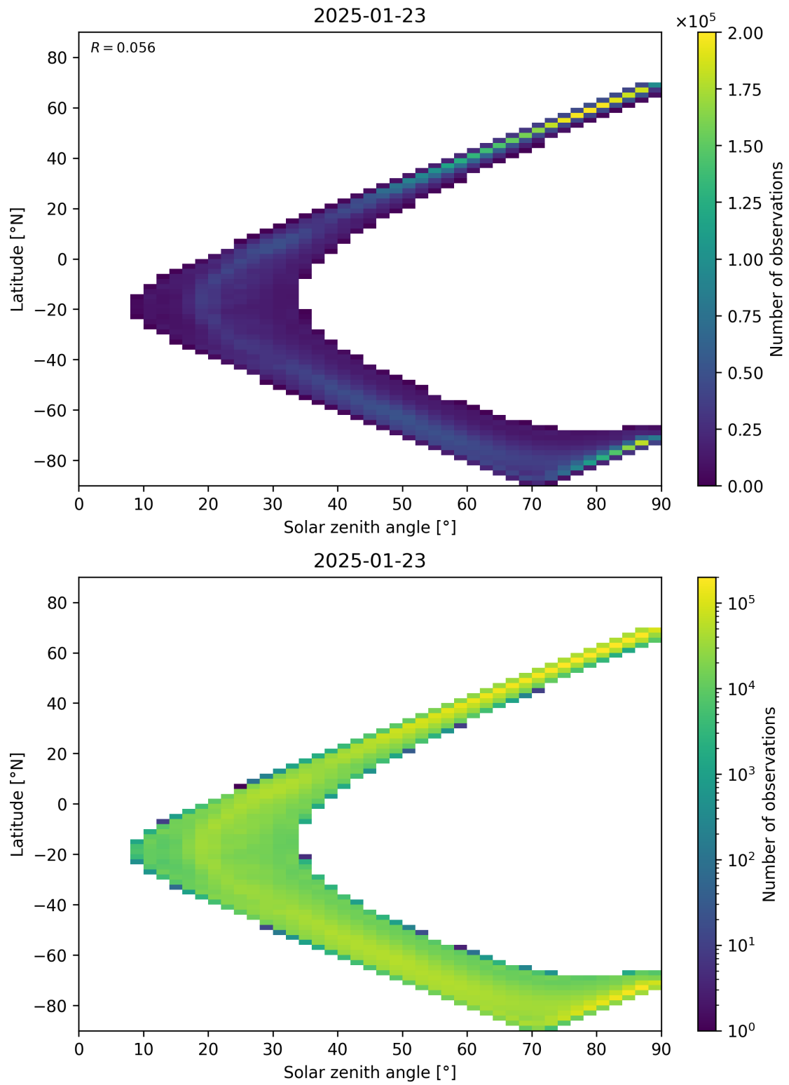
Figure 105: Scatter density plot of “Solar zenith angle” against “Latitude” for 2025-01-23 to 2025-01-24.
