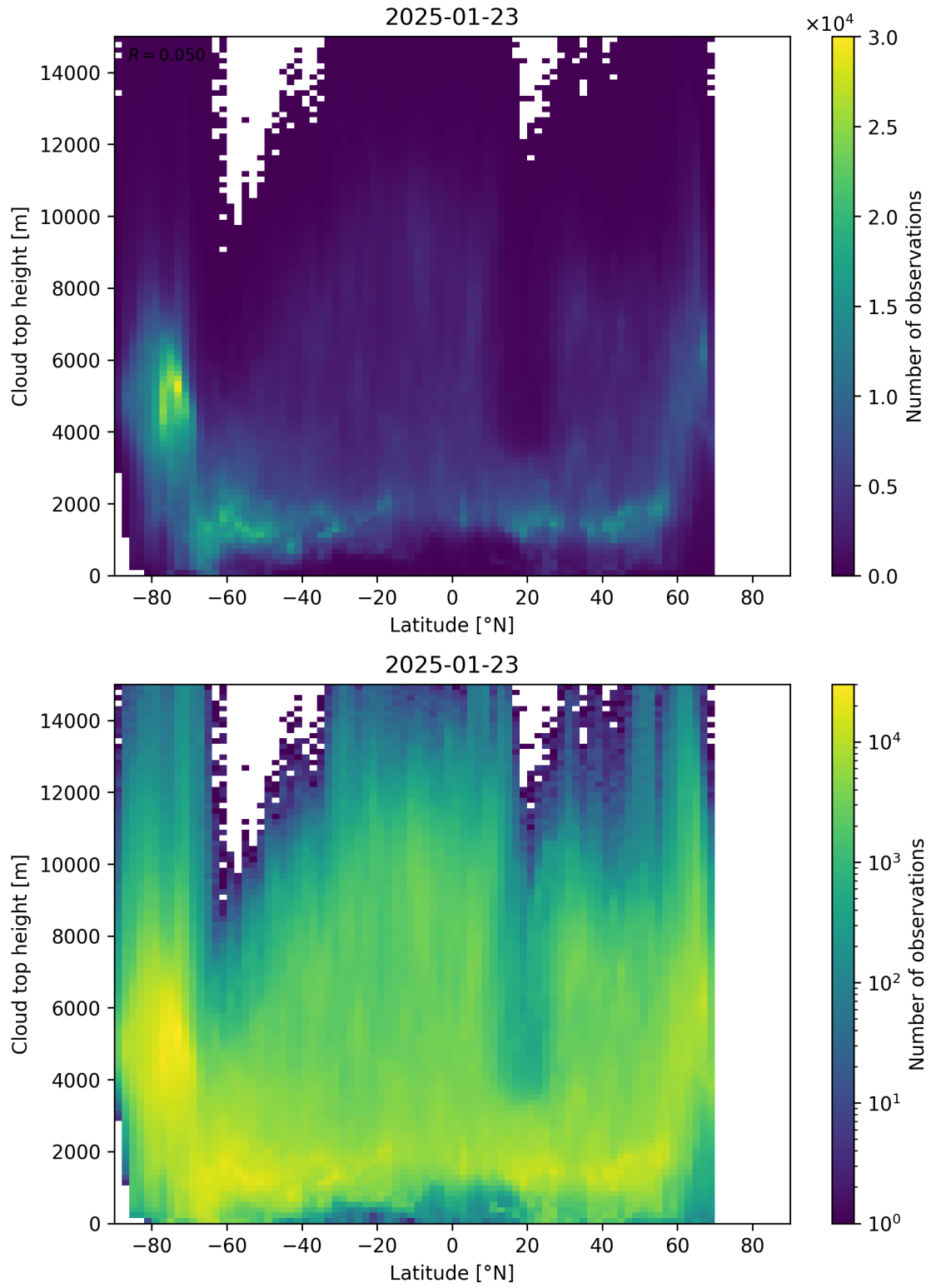
Figure 97: Scatter density plot of “Latitude” against “Cloud top height” for 2025-01-23 to 2025-01-24.
