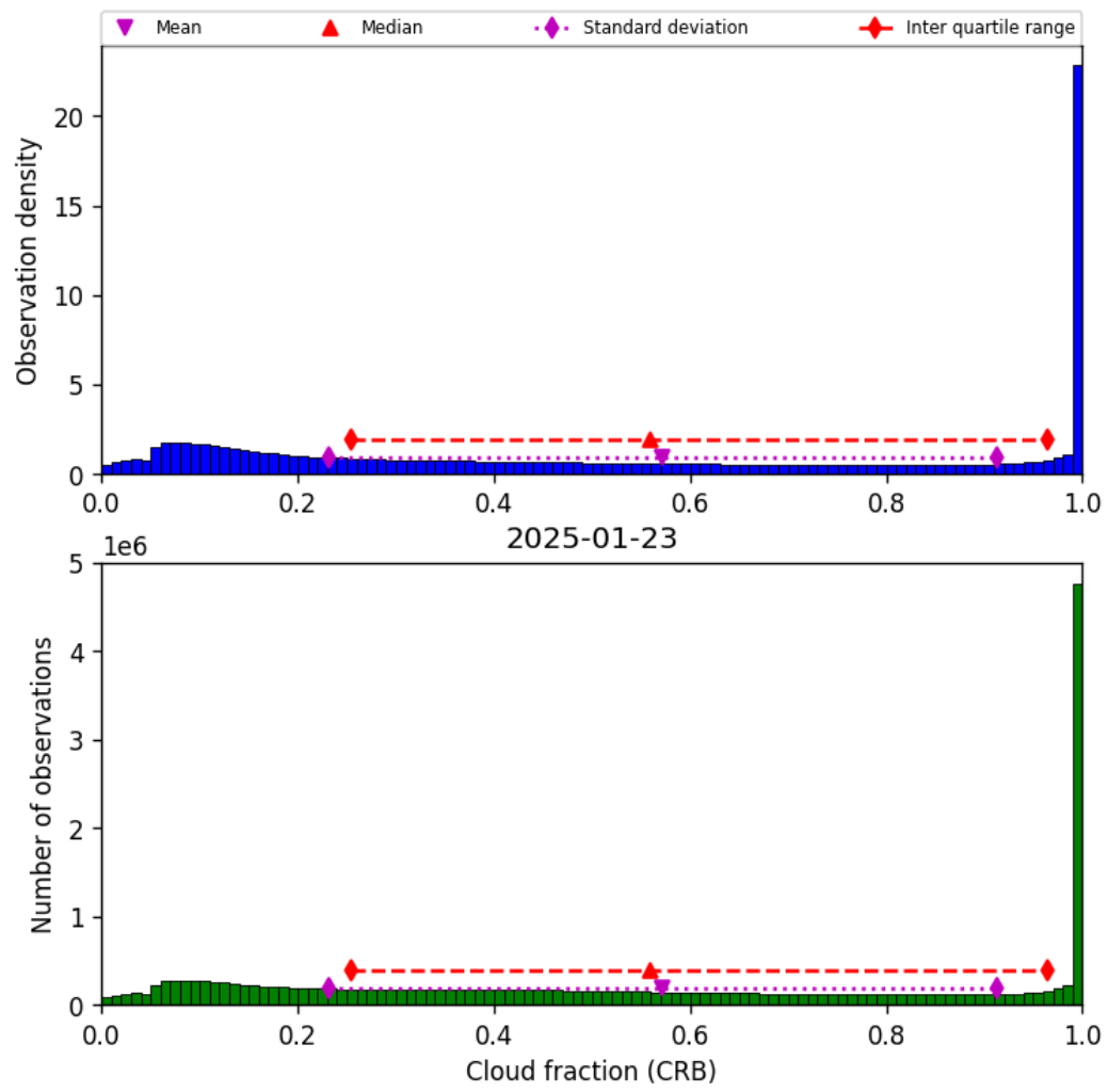
Figure 42: Histogram of "Cloud fraction (CRB)" for 2025-01-23 to 2025-01-24
