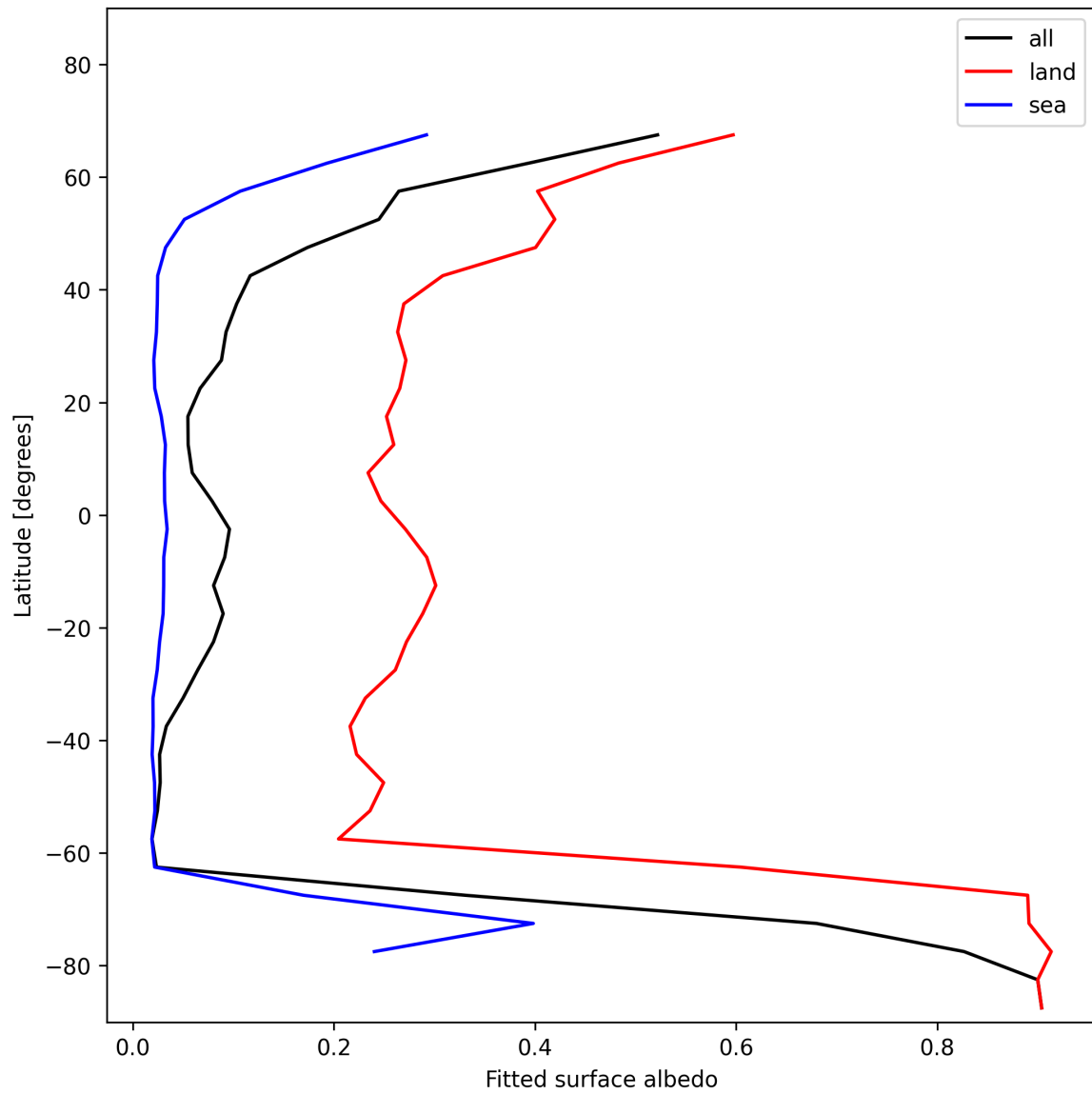
Figure 29: Zonal average of “Fitted surface albedo” for 2025-01-23 to 2025-01-24.
