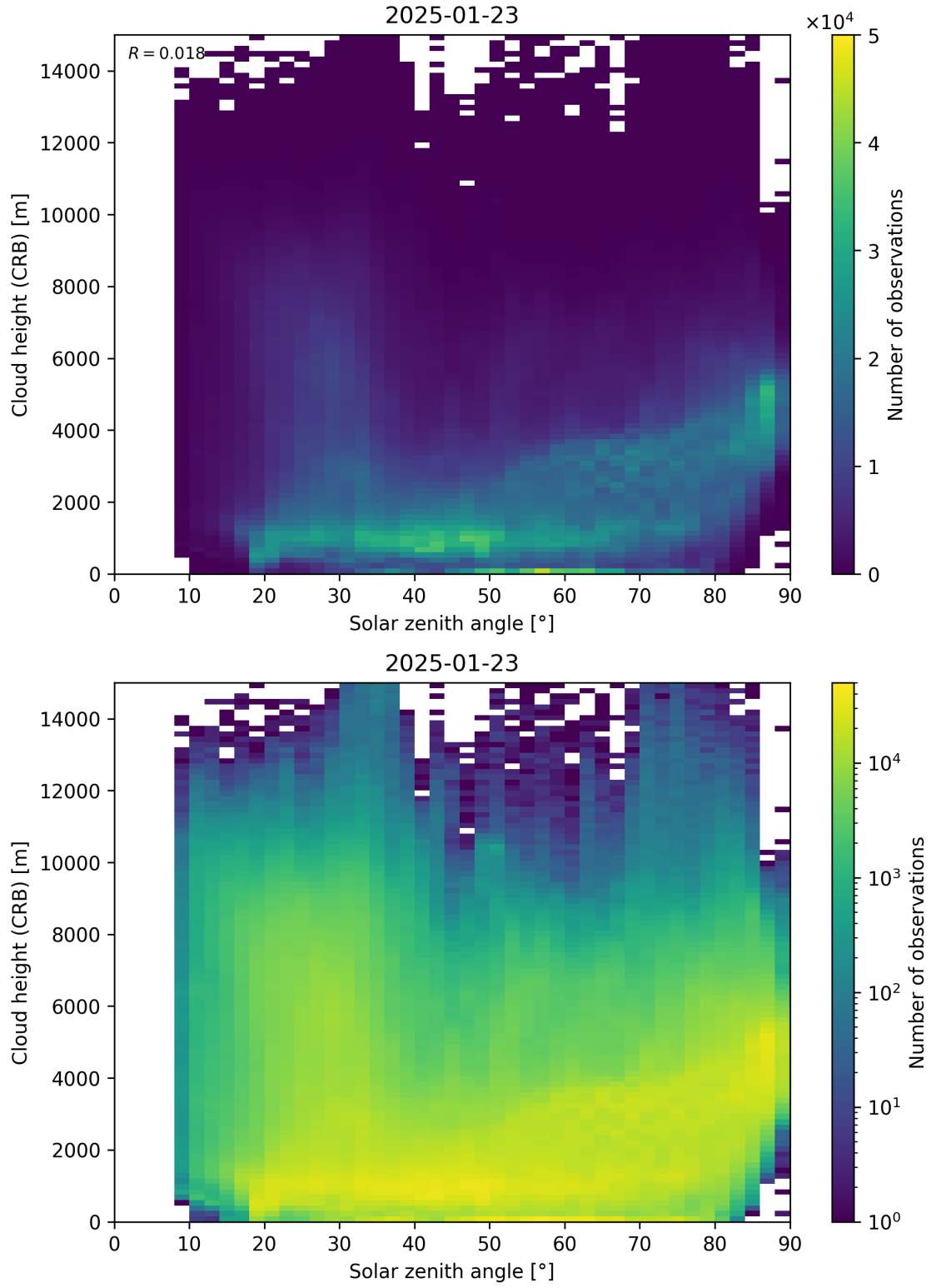
Figure 102: Scatter density plot of “Solar zenith angle” against “Cloud height (CRB)” for 2025-01-23 to 2025-01-24.
