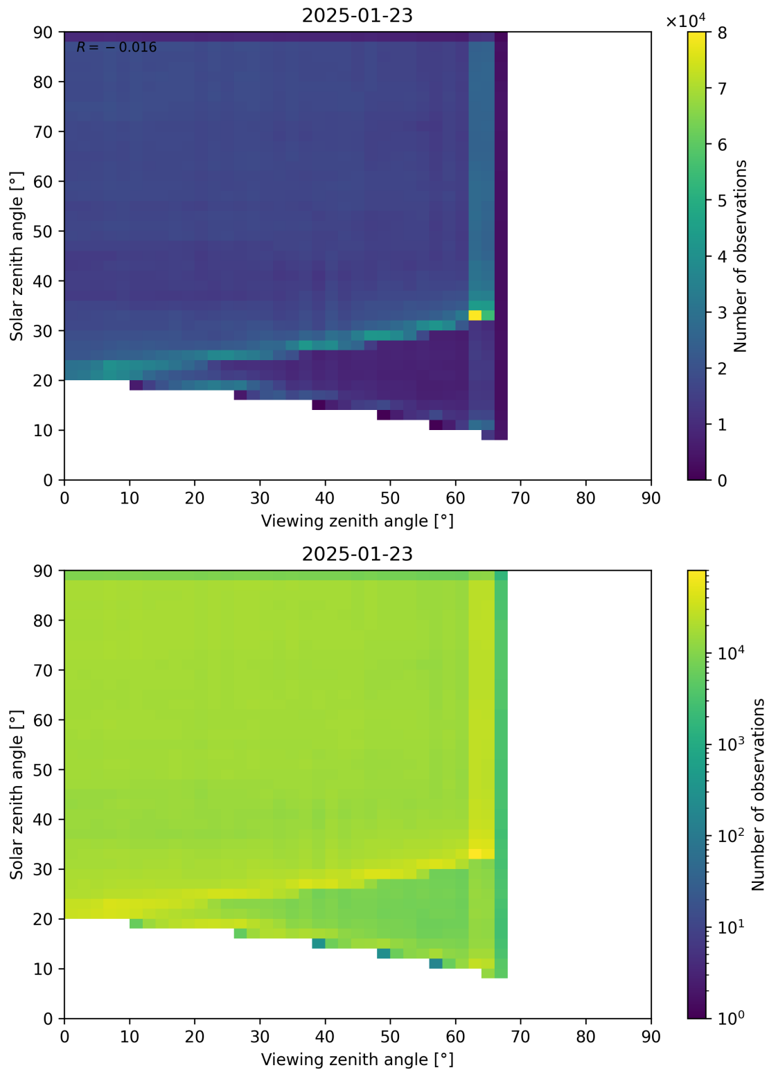
Figure 114: Scatter density plot of “Viewing zenith angle” against “Solar zenith angle” for 2025-01-23 to 2025-01-24.
