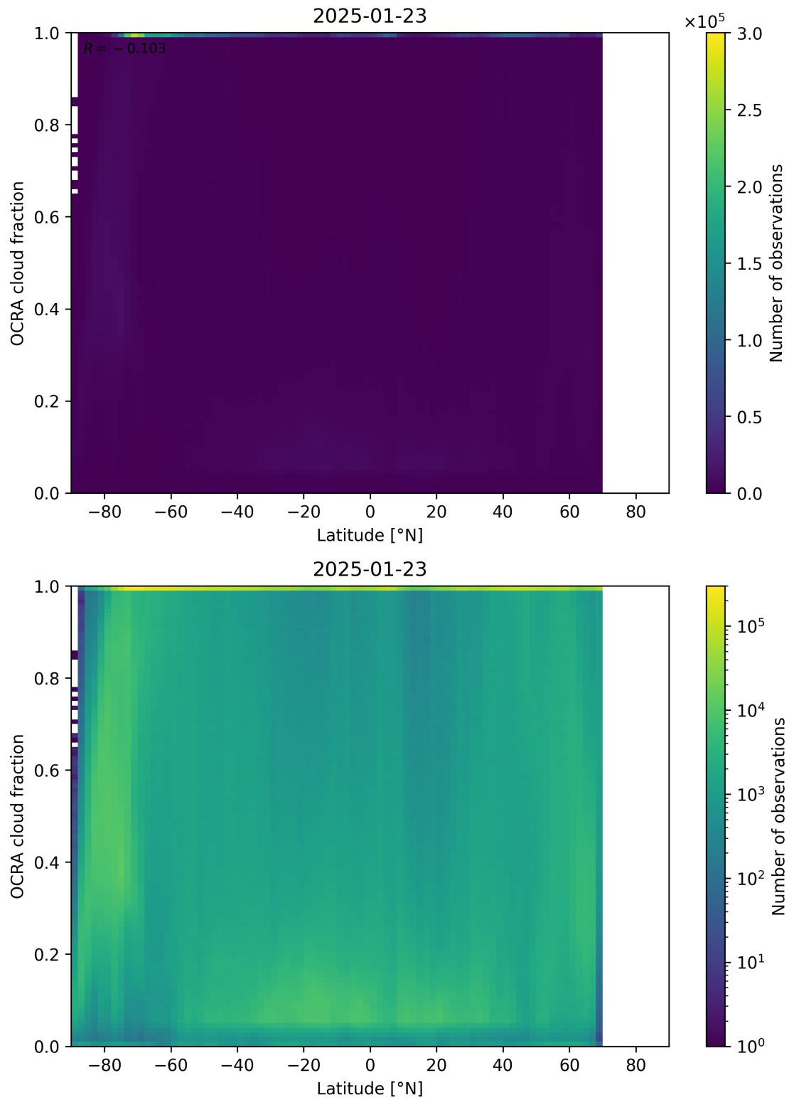
Figure 93: Scatter density plot of “Latitude” against “OCRA cloud fraction” for 2025-01-23 to 2025-01-24.
