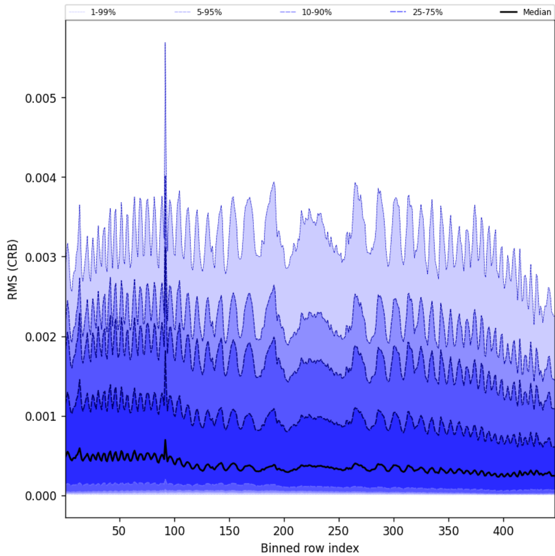
Figure 64: Along track statistics of “RMS (CRB)” for 2025-01-23 to 2025-01-24
