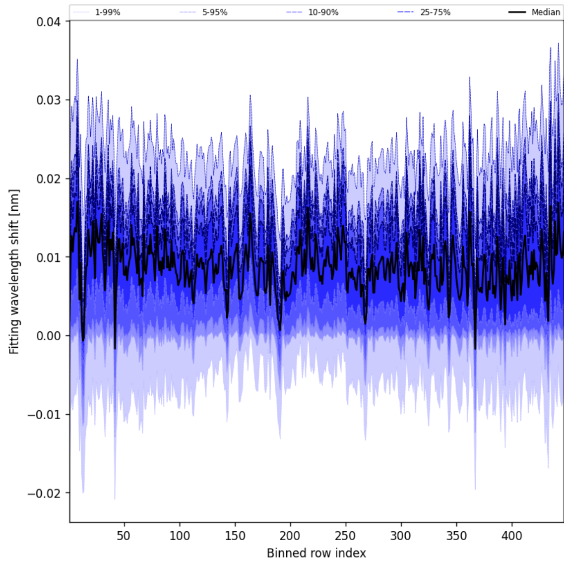
Figure 65: Along track statistics of “Fitting wavelength shift” for 2025-01-23 to 2025-01-24
