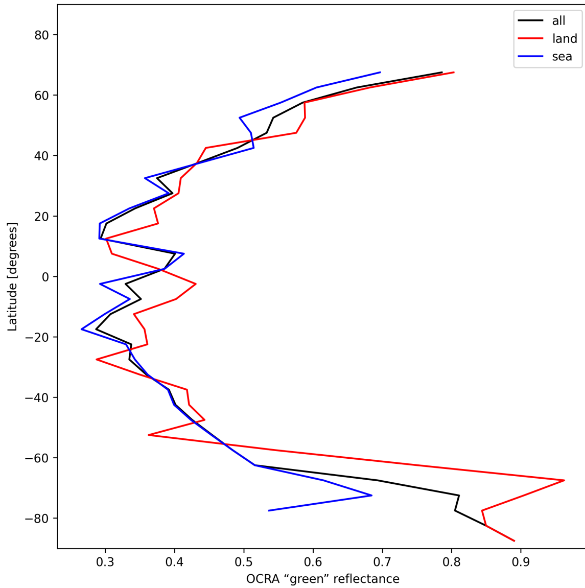
Figure 36: Zonal average of “OCRA “green” reflectance” for 2025-01-23 to 2025-01-24.
