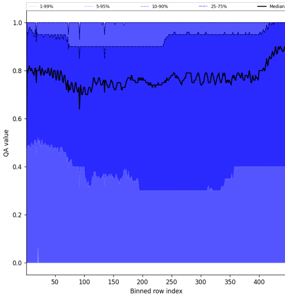
Figure 54: Along track statistics of “QA value” for 2025-01-23 to 2025-01-24
