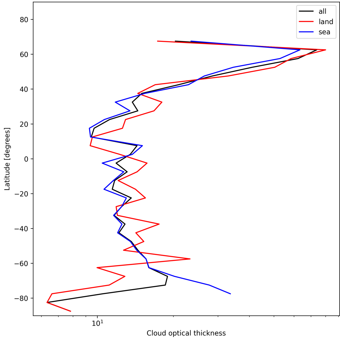
Figure 25: Zonal average of “Cloud optical thickness” for 2025-01-23 to 2025-01-24.
