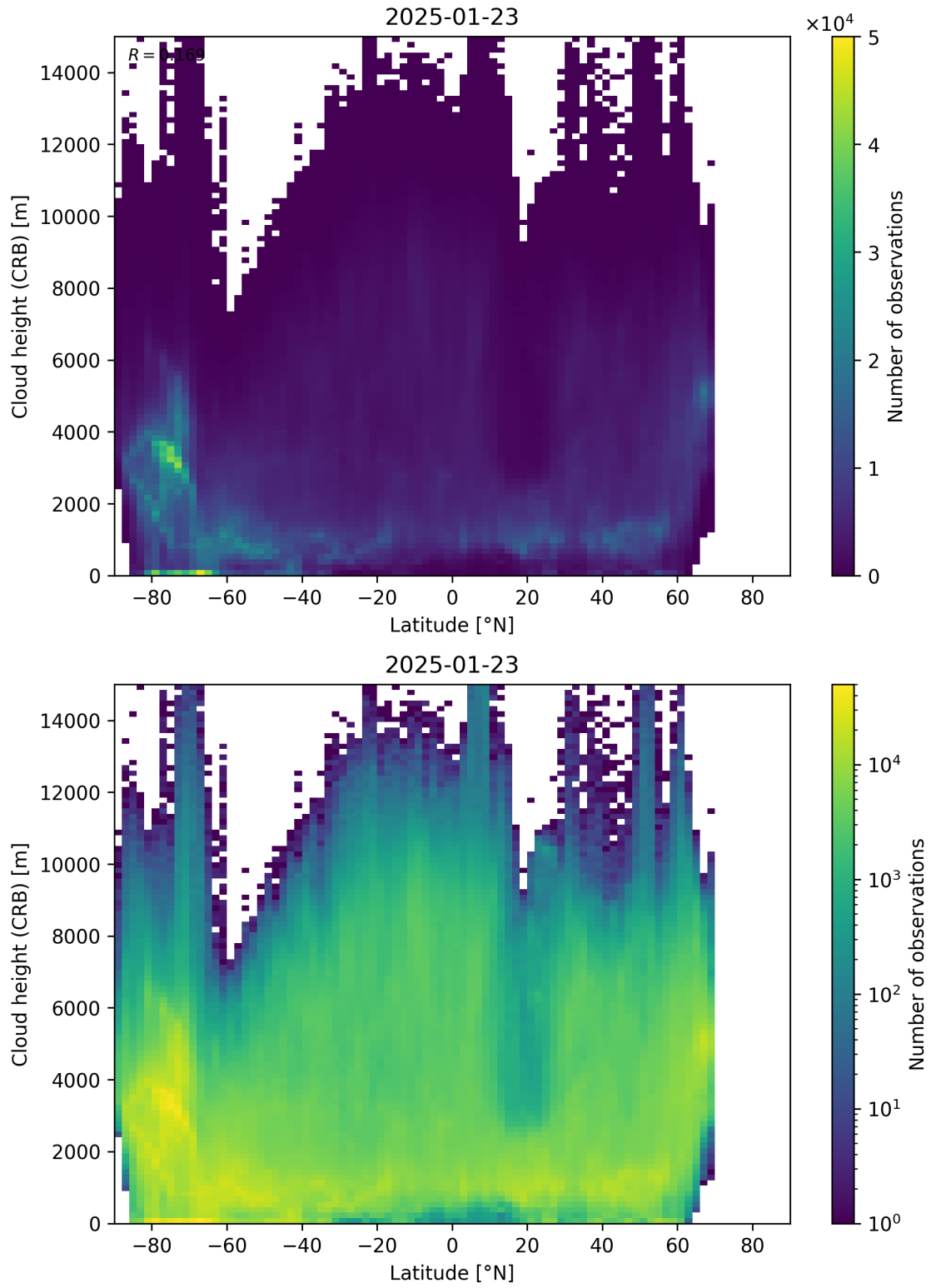
Figure 95: Scatter density plot of “Latitude” against “Cloud height (CRB)” for 2025-01-23 to 2025-01-24.
