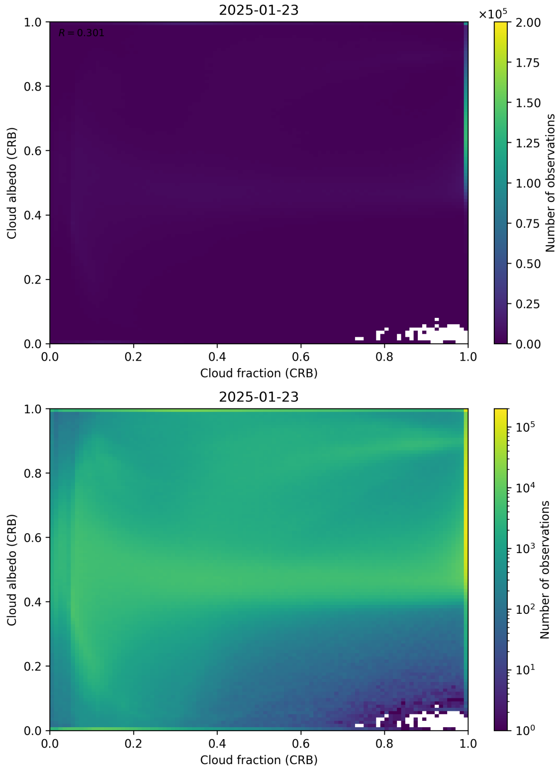
Figure 77: Scatter density plot of “Cloud fraction (CRB)” against “Cloud albedo (CRB)” for 2025-01-23 to 2025-01-24.
