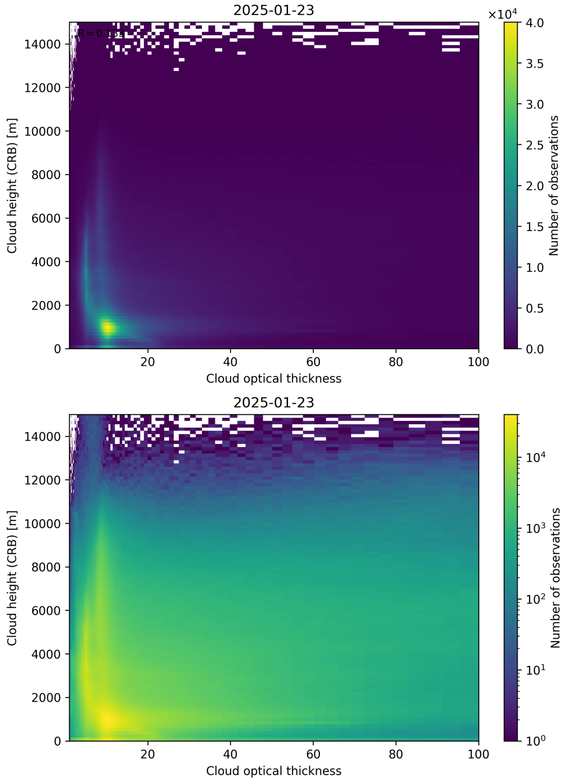
Figure 85: Scatter density plot of “Cloud optical thickness” against “Cloud height (CRB)” for 2025-01-23 to 2025-01-24.
