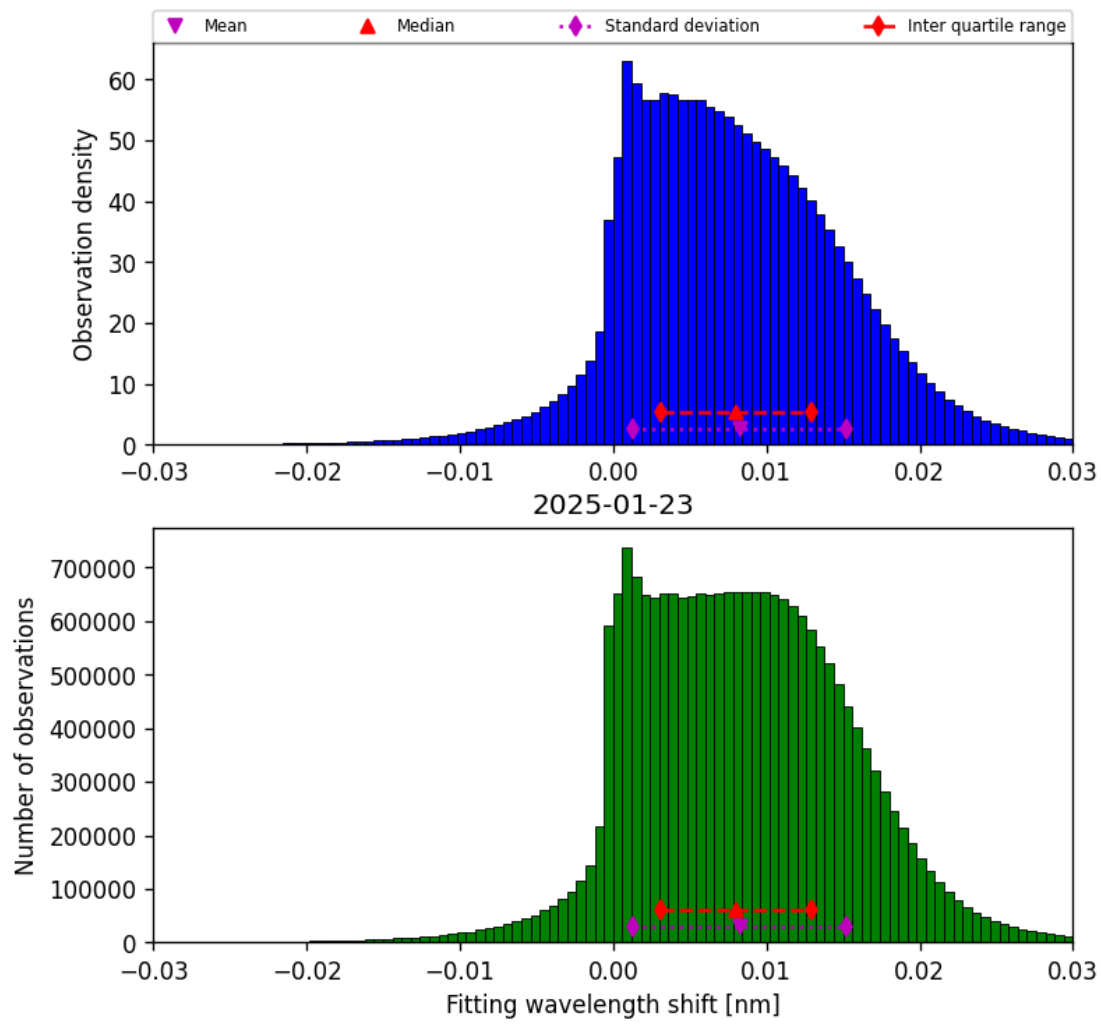
Figure 49: Histogram of “Fitting wavelength shift” for 2025-01-23 to 2025-01-24
