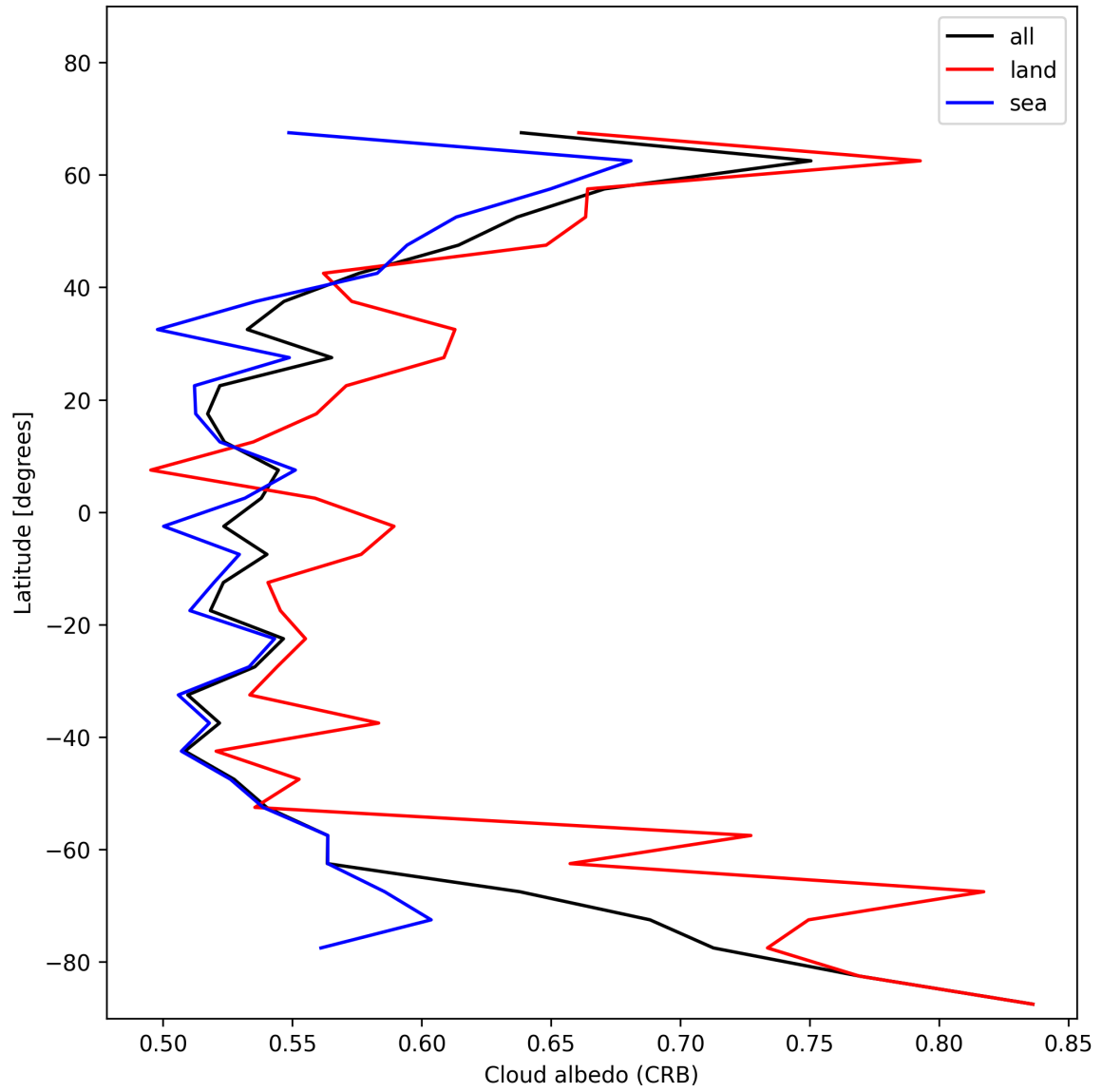
Figure 28: Zonal average of “Cloud albedo (CRB)” for 2025-01-23 to 2025-01-24.
