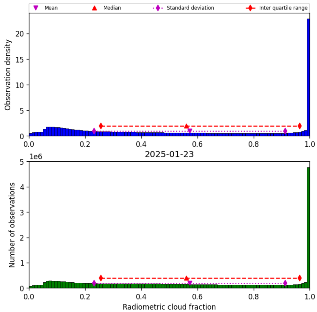
Figure 39: Histogram of “Radiometric cloud fraction” for 2025-01-23 to 2025-01-24
