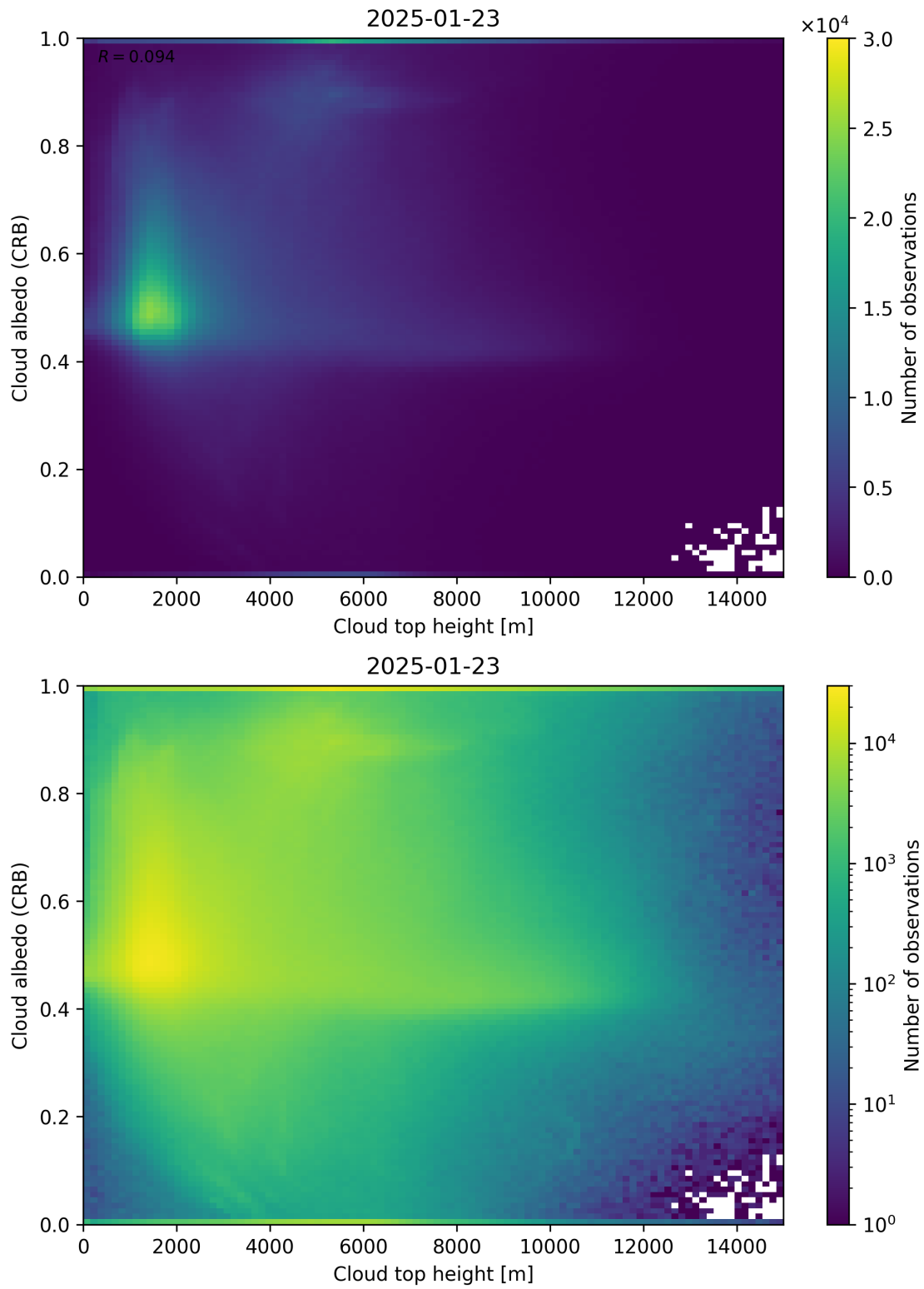
Figure 86: Scatter density plot of “Cloud top height” against “Cloud albedo (CRB)” for 2025-01-23 to 2025-01-24.
