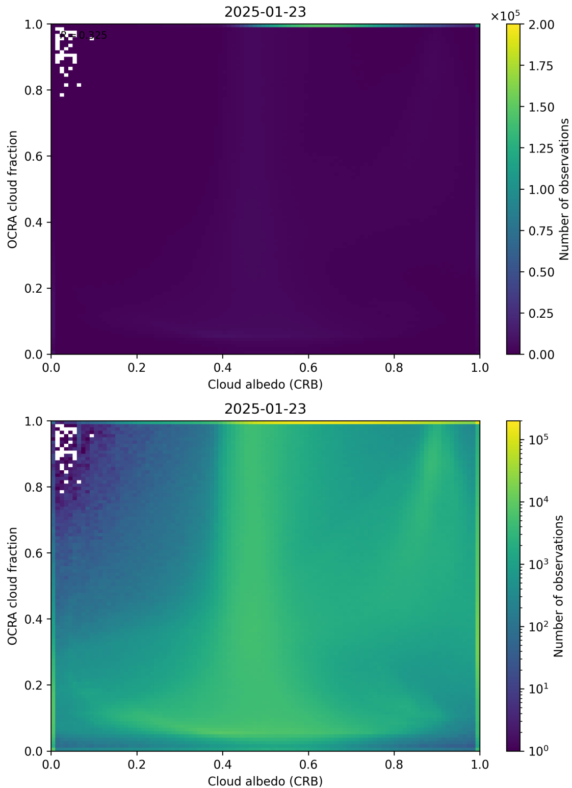
Figure 70: Scatter density plot of “Cloud albedo (CRB)” against “OCRA cloud fraction” for 2025-01-23 to 2025-01-24.
