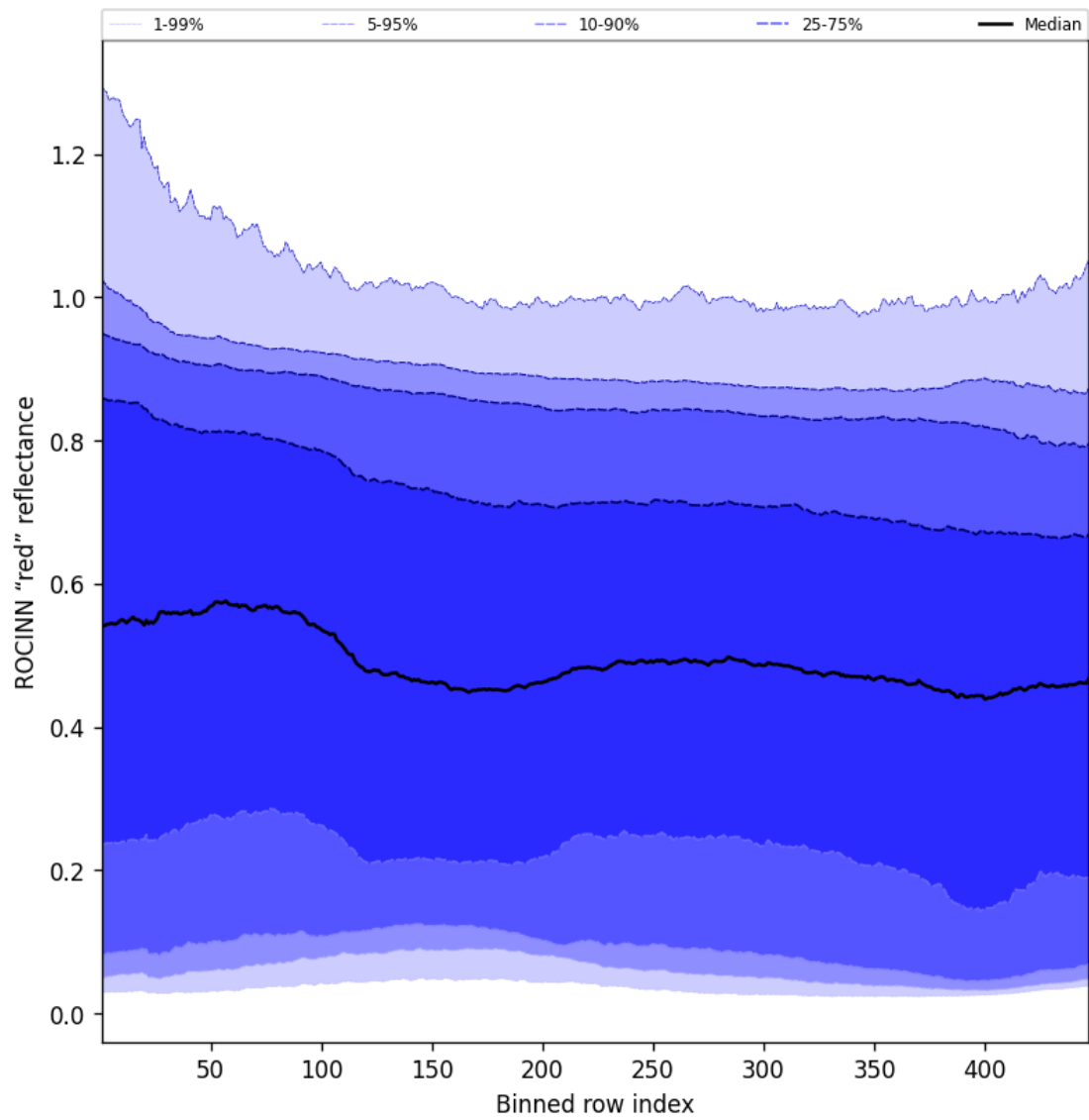
Figure 69: Along track statistics of “ROCINN “red” reflectance” for 2025-01-23 to 2025-01-24
