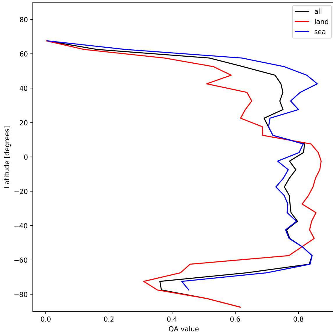
Figure 22: Zonal average of “QA value” for 2025-01-23 to 2025-01-24.
