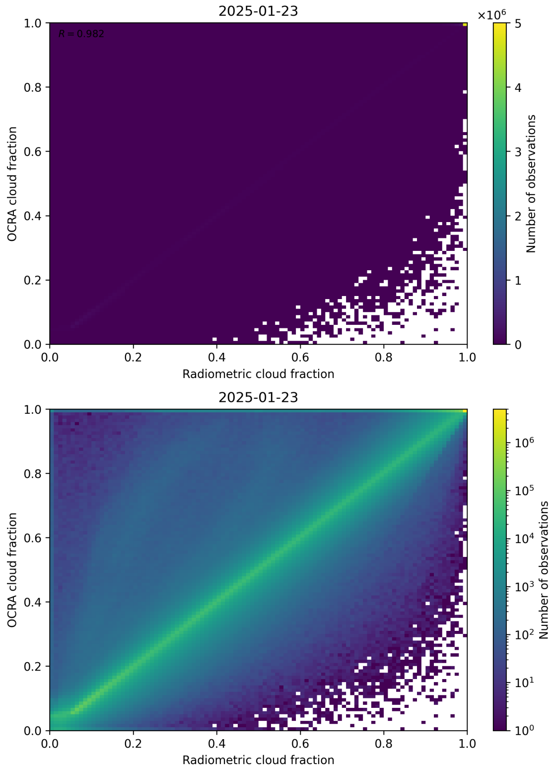
Figure 72: Scatter density plot of “Radiometric cloud fraction” against “OCRA cloud fraction” for 2025-01-23 to 2025-01-24.
