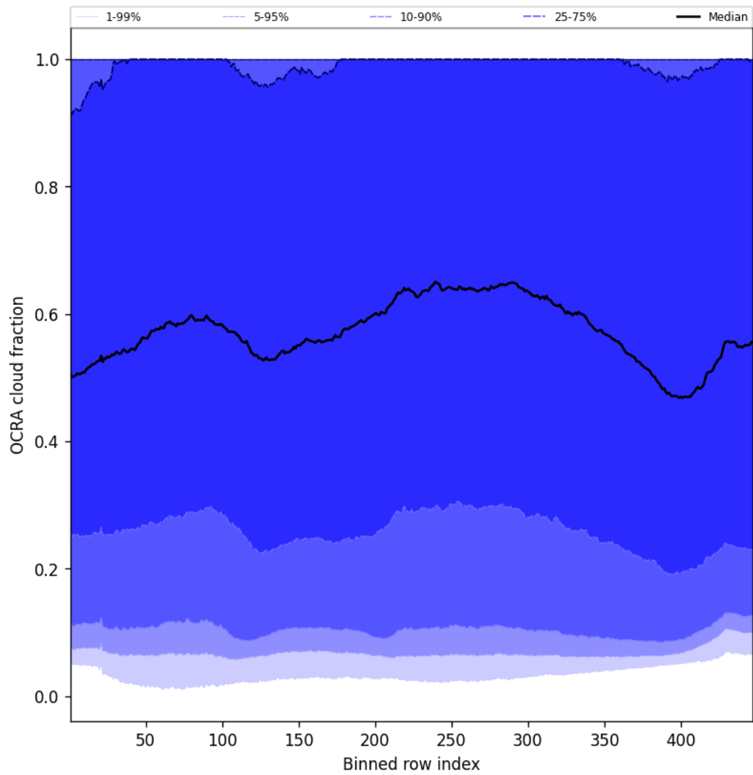
Figure 66: Along track statistics of “OCRA cloud fraction” for 2025-01-23 to 2025-01-24
