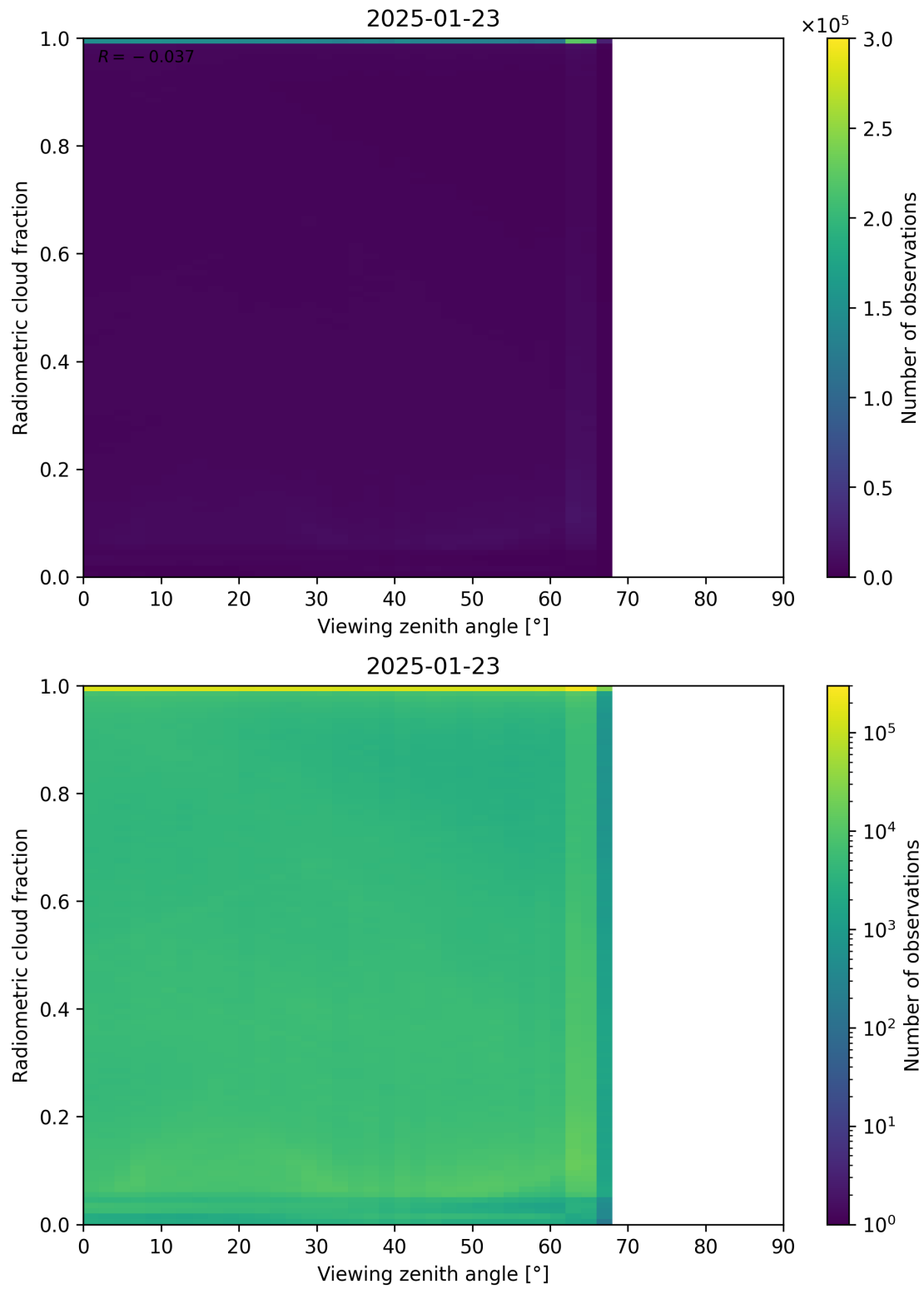
Figure 107: Scatter density plot of “Viewing zenith angle” against “Radiometric cloud fraction” for 2025-01-23 to 2025-01-24.
