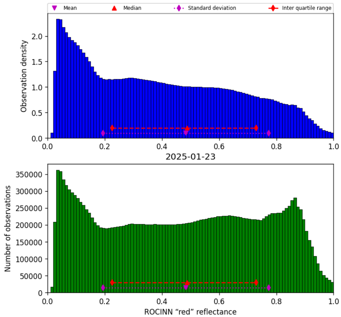
Figure 53: Histogram of “ROCINN “red” reflectance” for 2025-01-23 to 2025-01-24
