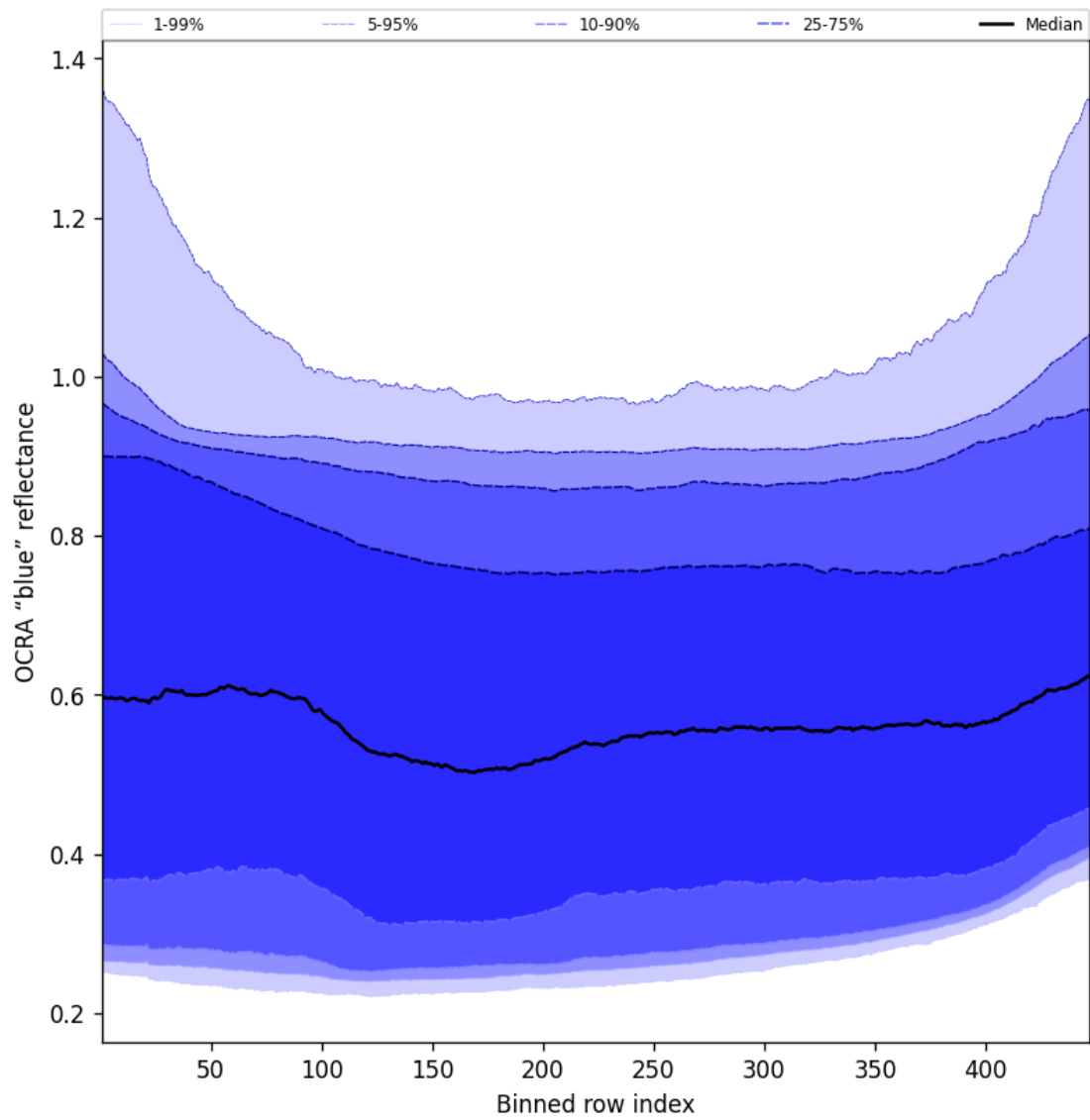
Figure 67: Along track statistics of “OCRA “blue” reflectance” for 2025-01-23 to 2025-01-24
