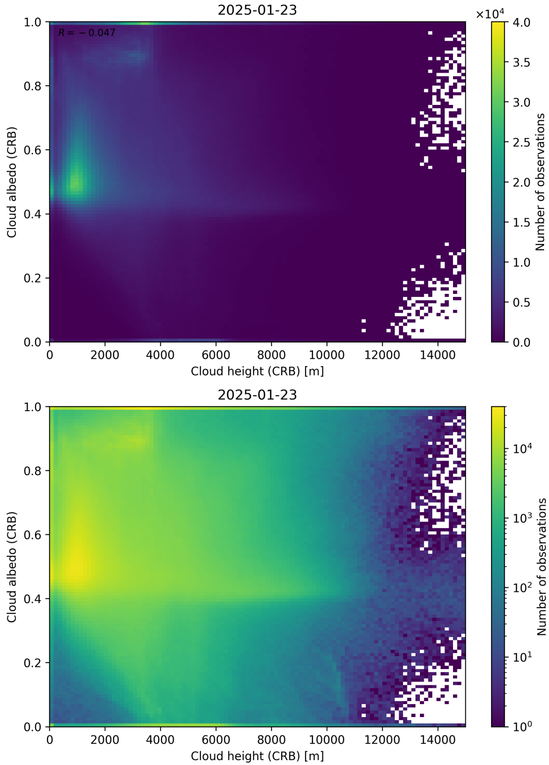
Figure 80: Scatter density plot of “Cloud height (CRB)” against “Cloud albedo (CRB)” for 2025-01-23 to 2025-01-24.
