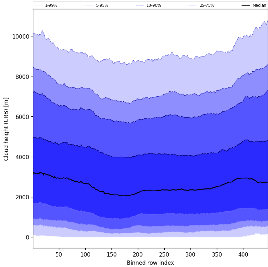
Figure 59: Along track statistics of “Cloud height (CRB)” for 2025-01-23 to 2025-01-24
