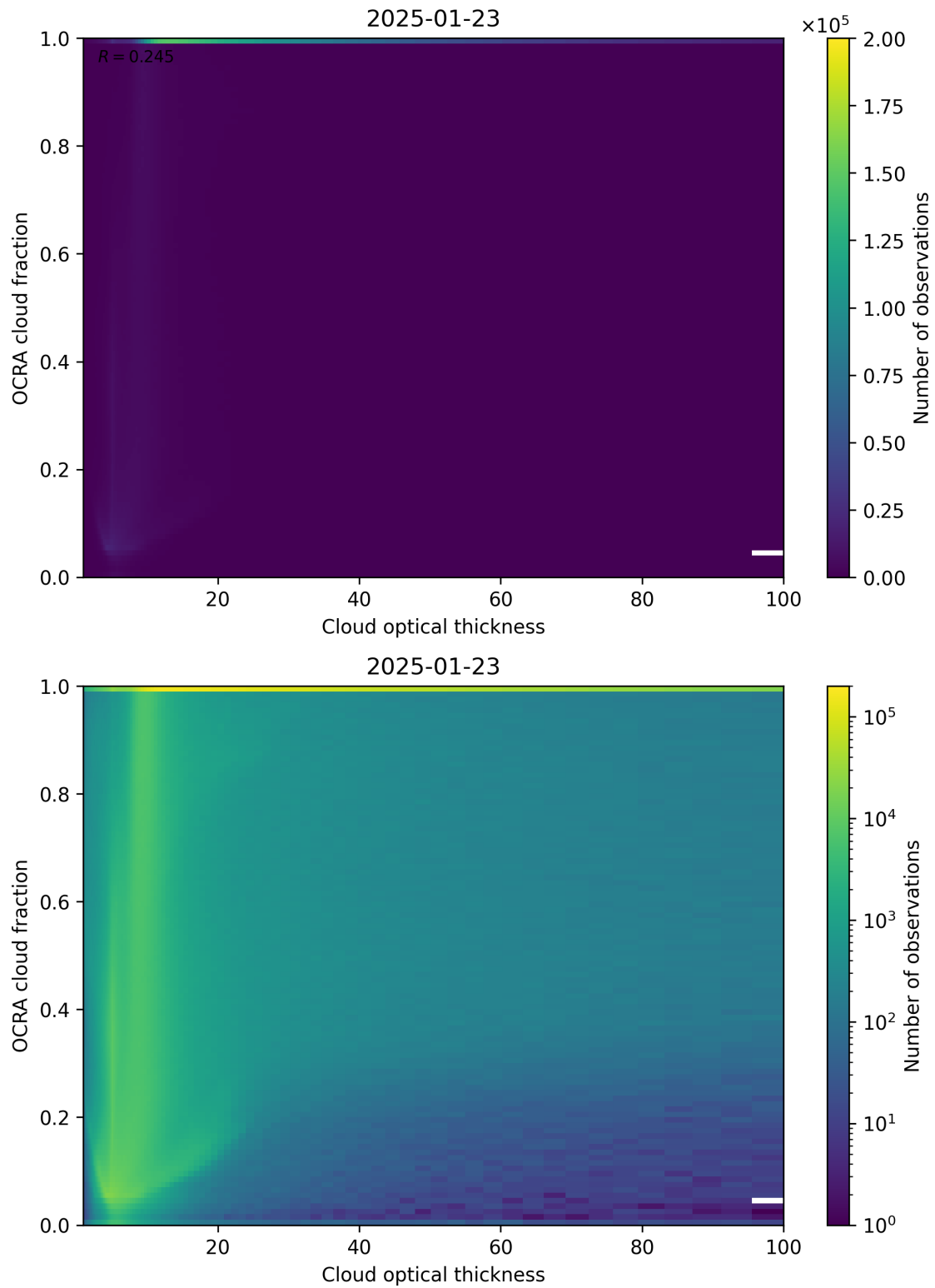
Figure 83: Scatter density plot of “Cloud optical thickness” against “OCRA cloud fraction” for 2025-01-23 to 2025-01-24.
