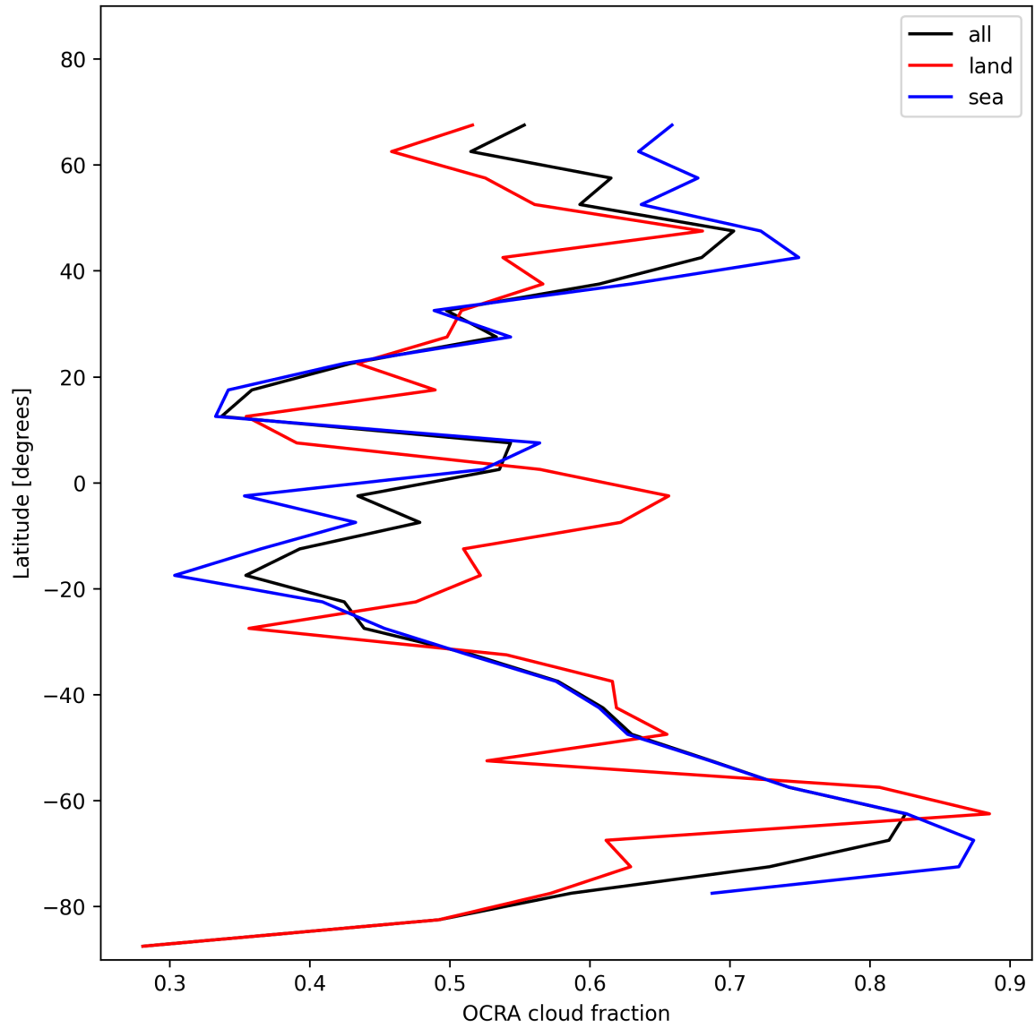
Figure 34: Zonal average of “OCRA cloud fraction” for 2025-01-23 to 2025-01-24.
