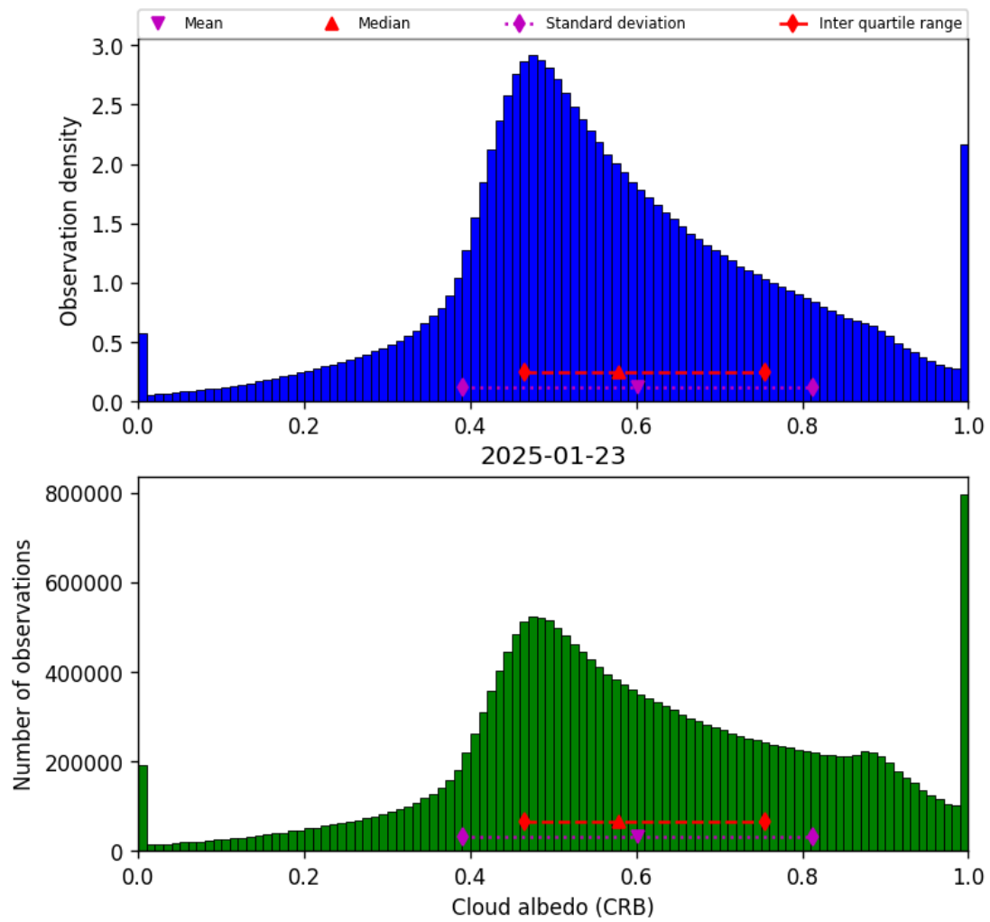
Figure 44: Histogram of “Cloud albedo (CRB)” for 2025-01-23 to 2025-01-24
