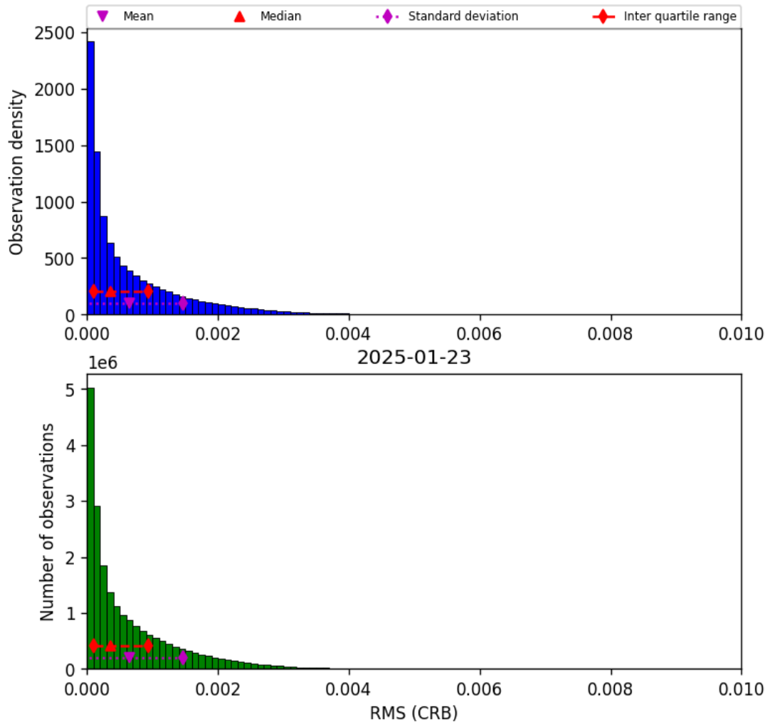
Figure 48: Histogram of “RMS (CRB)” for 2025-01-23 to 2025-01-24
