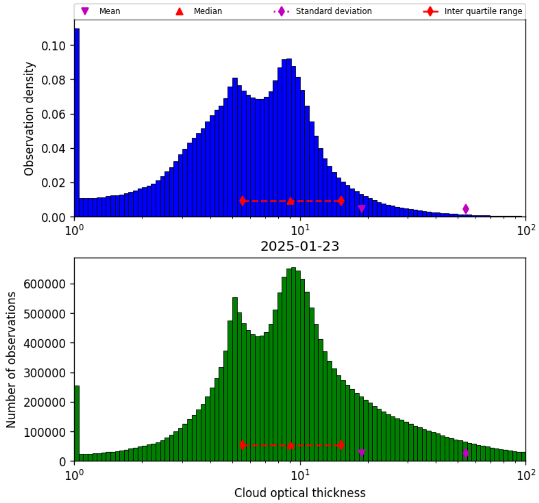
Figure 41: Histogram of “Cloud optical thickness” for 2025-01-23 to 2025-01-24
