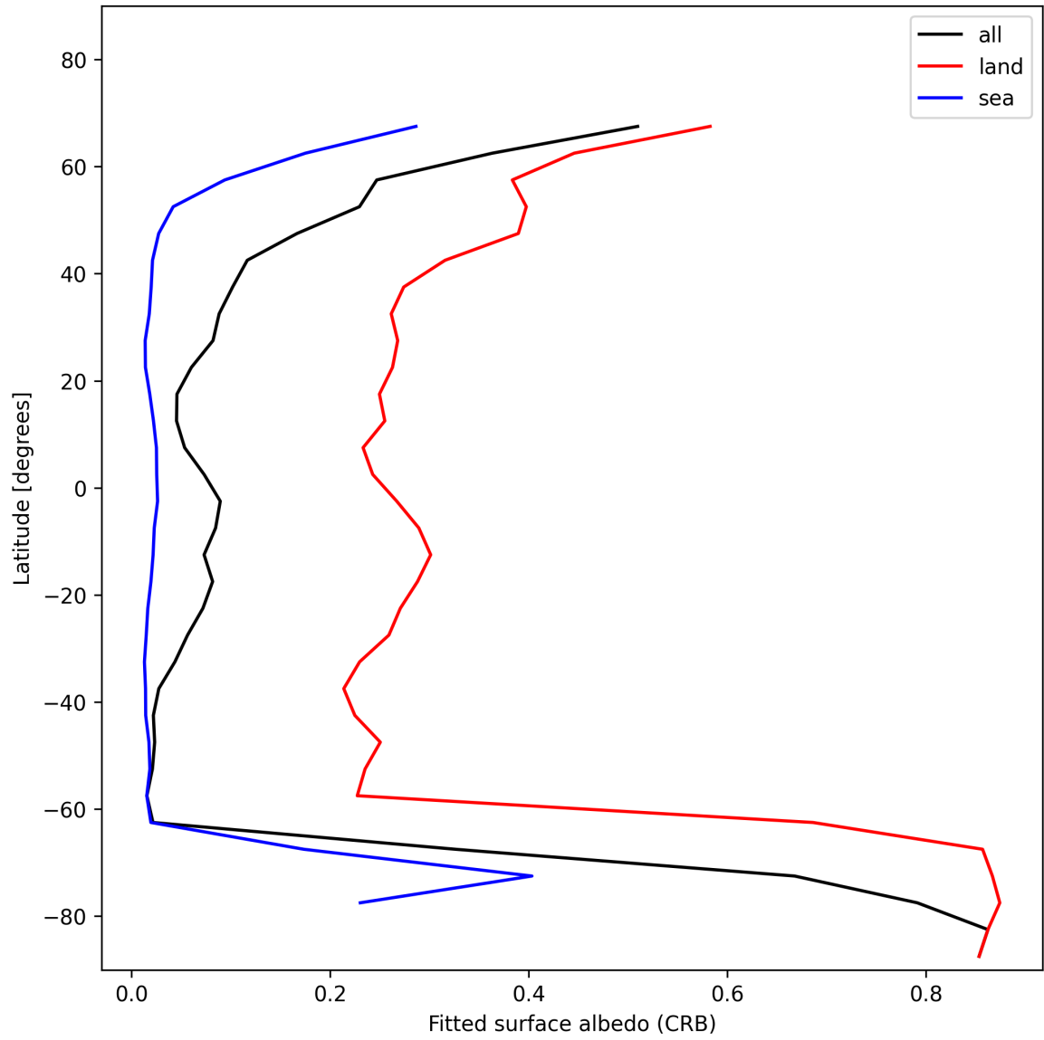
Figure 30: Zonal average of “Fitted surface albedo (CRB)” for 2025-01-23 to 2025-01-24.
