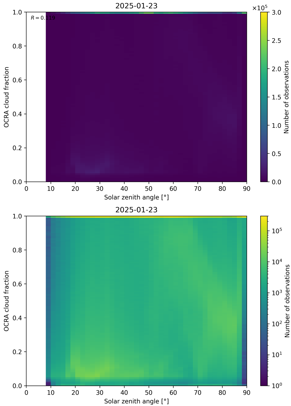
Figure 100: Scatter density plot of “Solar zenith angle” against “OCRA cloud fraction” for 2025-01-23 to 2025-01-24.
