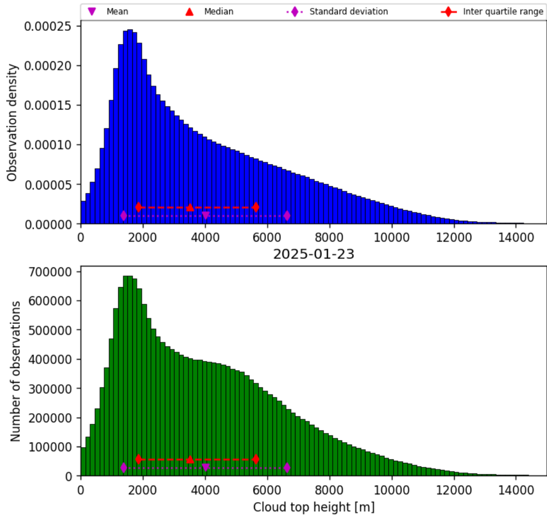
Figure 40: Histogram of “Cloud top height” for 2025-01-23 to 2025-01-24
