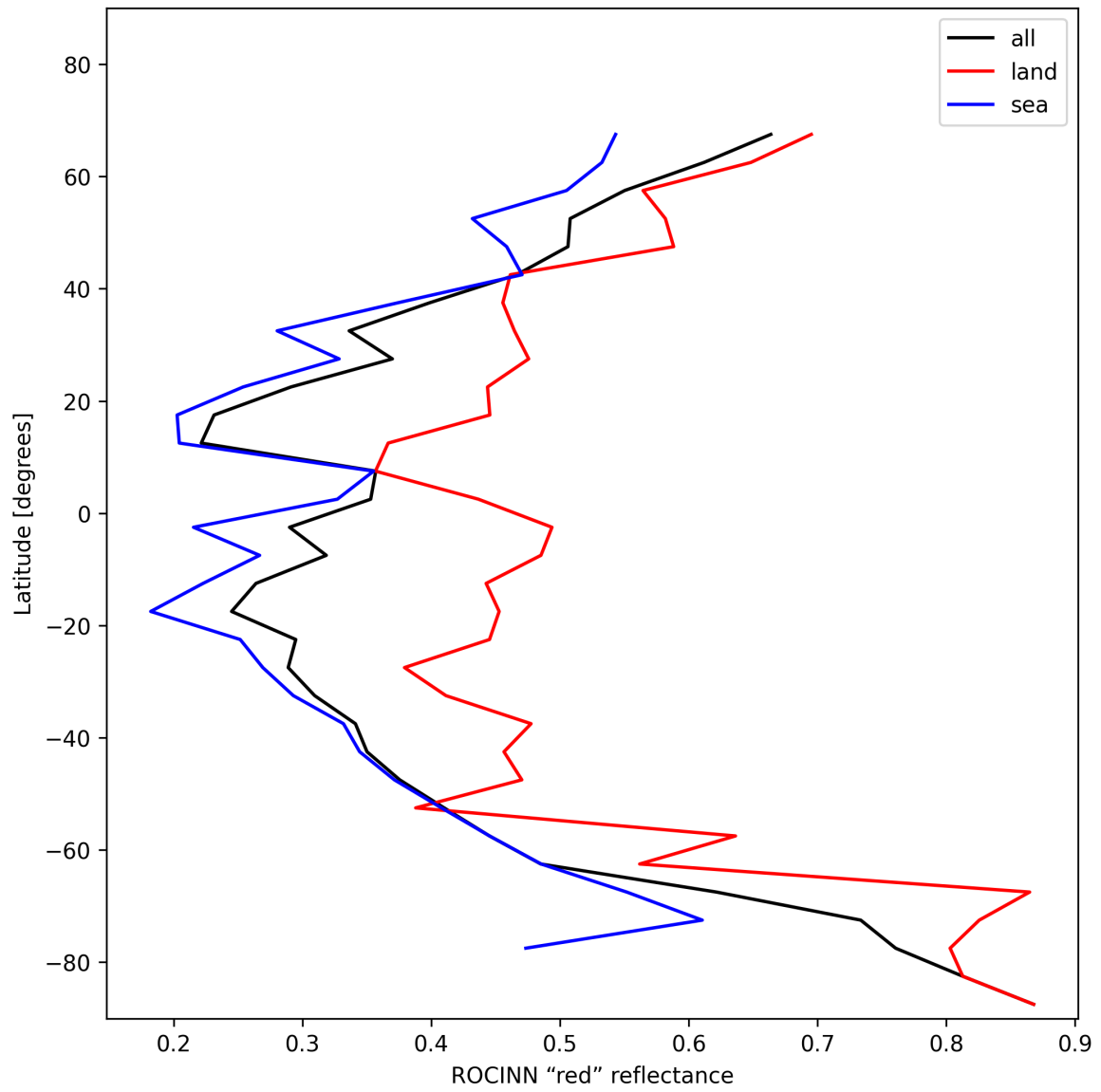
Figure 37: Zonal average of “ROCINN “red” reflectance” for 2025-01-23 to 2025-01-24.
