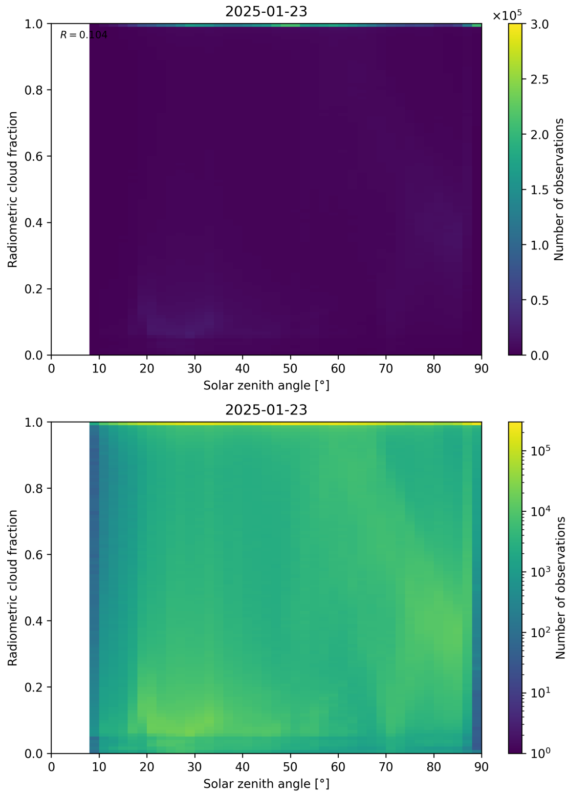
Figure 99: Scatter density plot of “Solar zenith angle” against “Radiometric cloud fraction” for 2025-01-23 to 2025-01-24.
