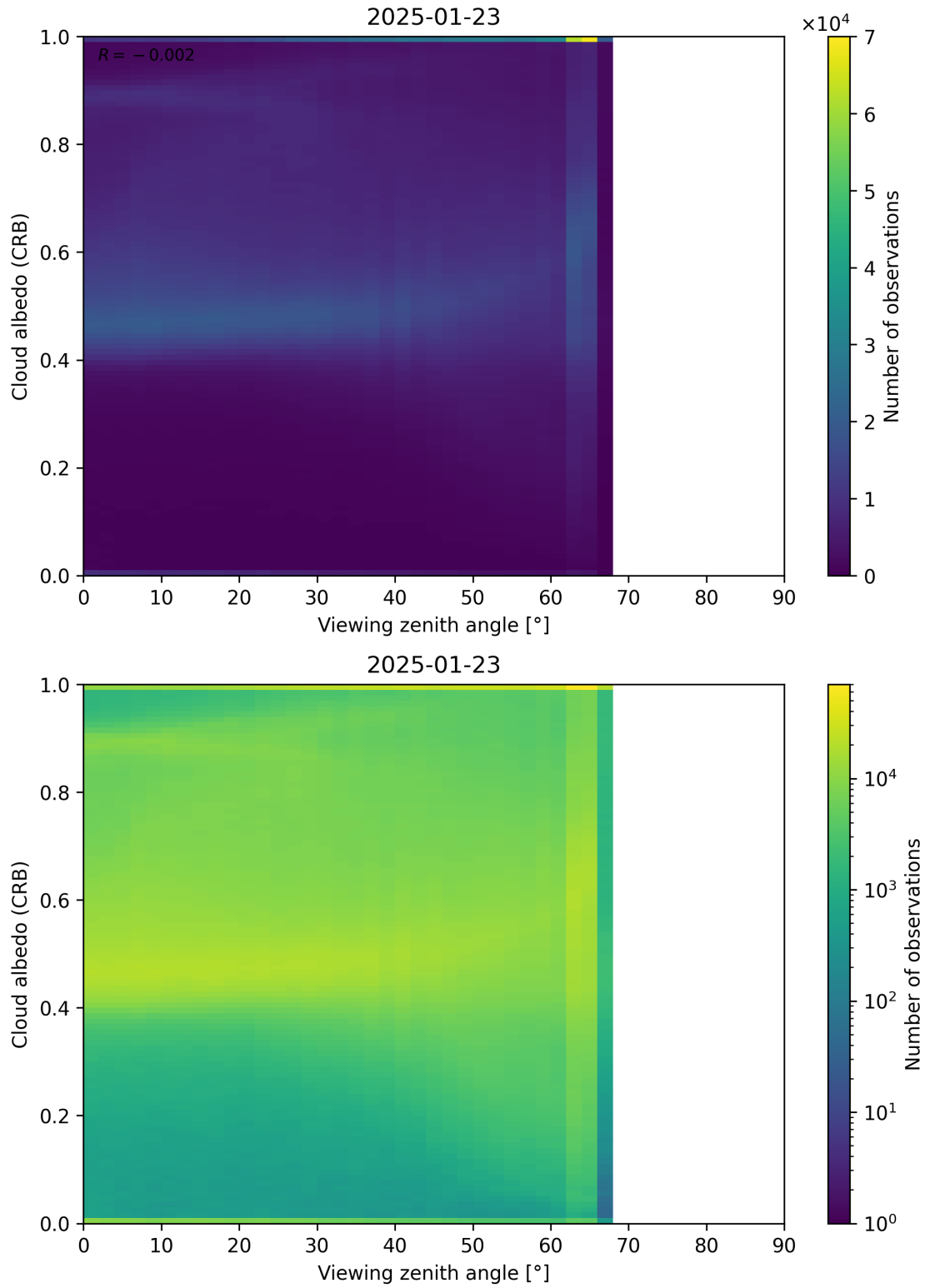
Figure 106: Scatter density plot of “Viewing zenith angle” against “Cloud albedo (CRB)” for 2025-01-23 to 2025-01-24.
