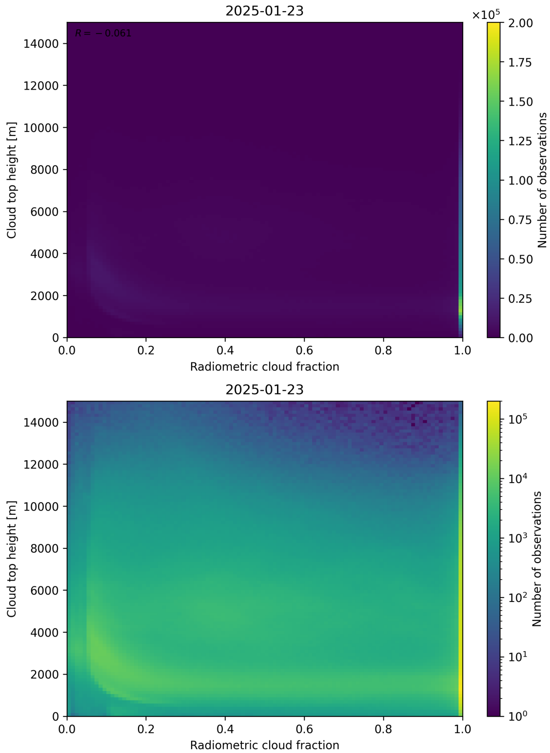
Figure 76: Scatter density plot of “Radiometric cloud fraction” against “Cloud top height” for 2025-01-23 to 2025-01-24.
