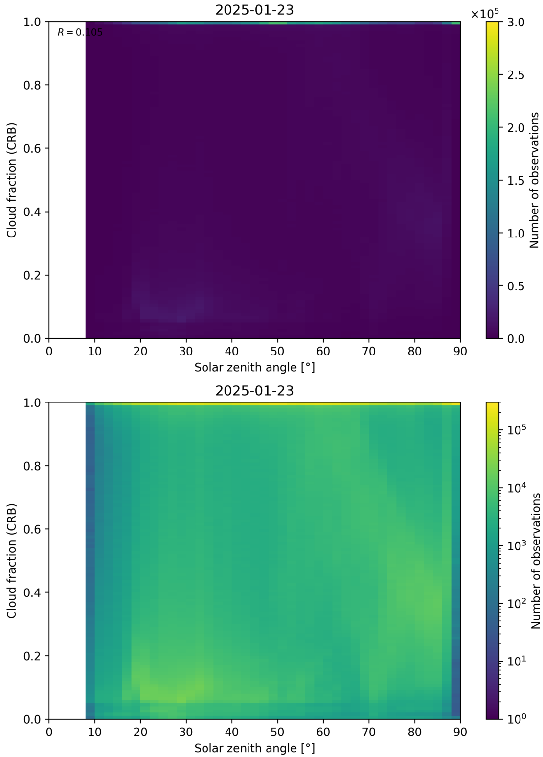
Figure 101: Scatter density plot of “Solar zenith angle” against “Cloud fraction (CRB)” for 2025-01-23 to 2025-01-24.
