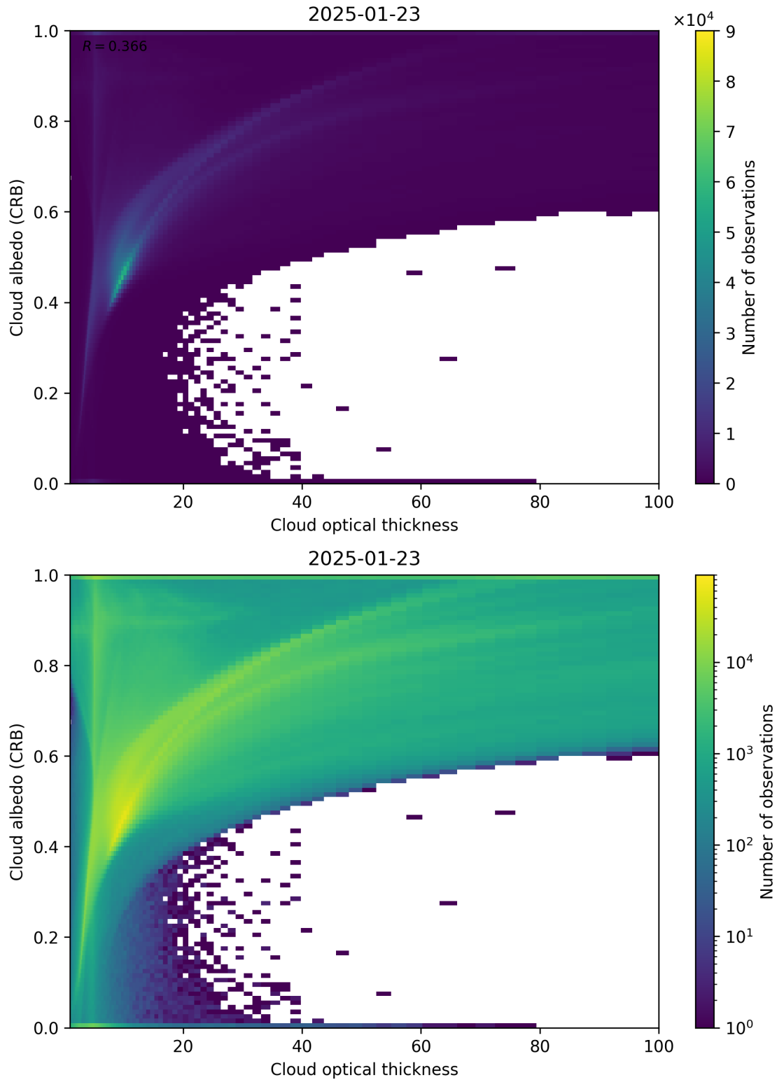
Figure 82: Scatter density plot of “Cloud optical thickness” against “Cloud albedo (CRB)” for 2025-01-23 to 2025-01-24.
