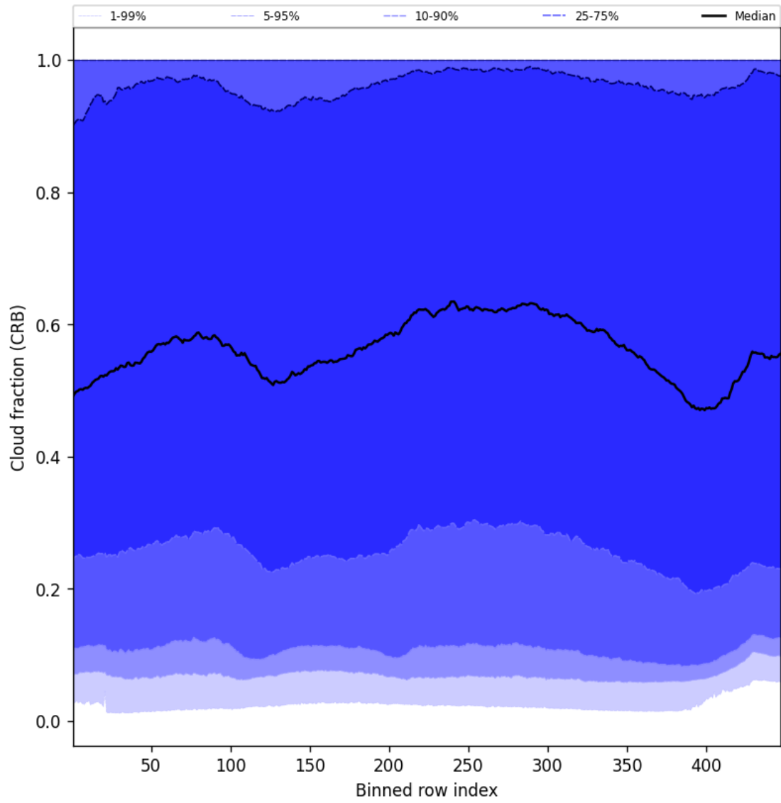
Figure 58: Along track statistics of “Cloud fraction (CRB)” for 2025-01-23 to 2025-01-24
