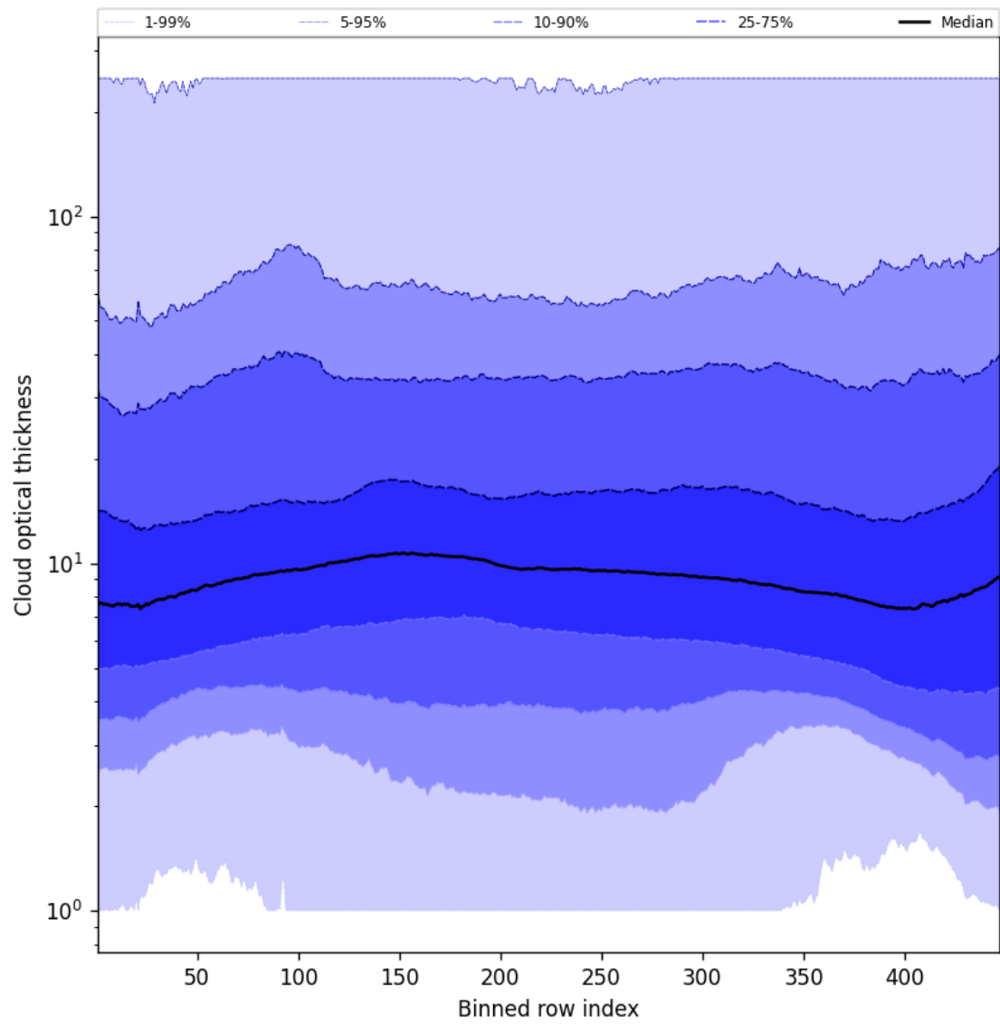
Figure 57: Along track statistics of “Cloud optical thickness” for 2025-01-23 to 2025-01-24
