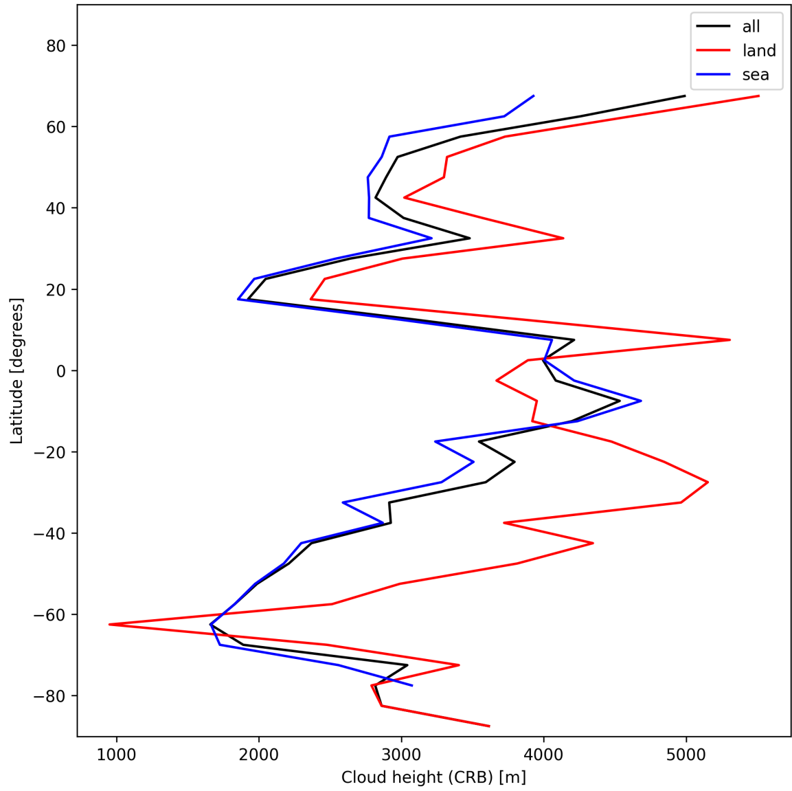
Figure 27: Zonal average of “Cloud height (CRB)” for 2025-01-23 to 2025-01-24.
