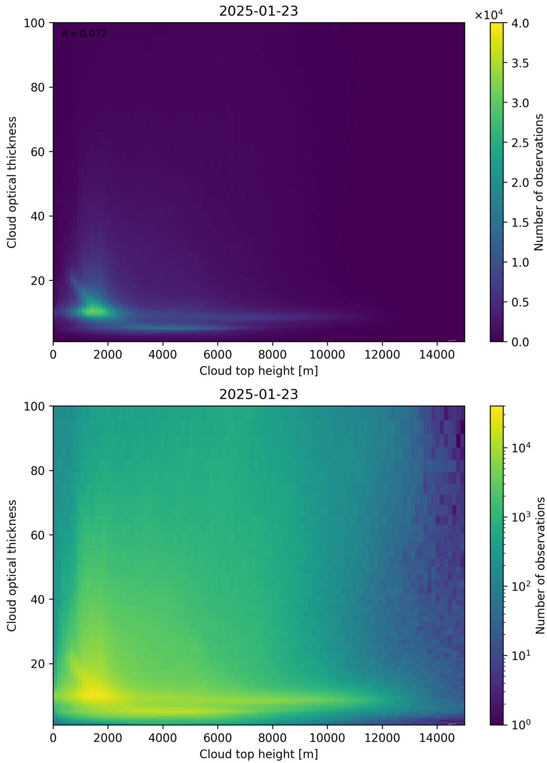
Figure 90: Scatter density plot of “Cloud top height” against “Cloud optical thickness” for 2025-01-23 to 2025-01-24.
