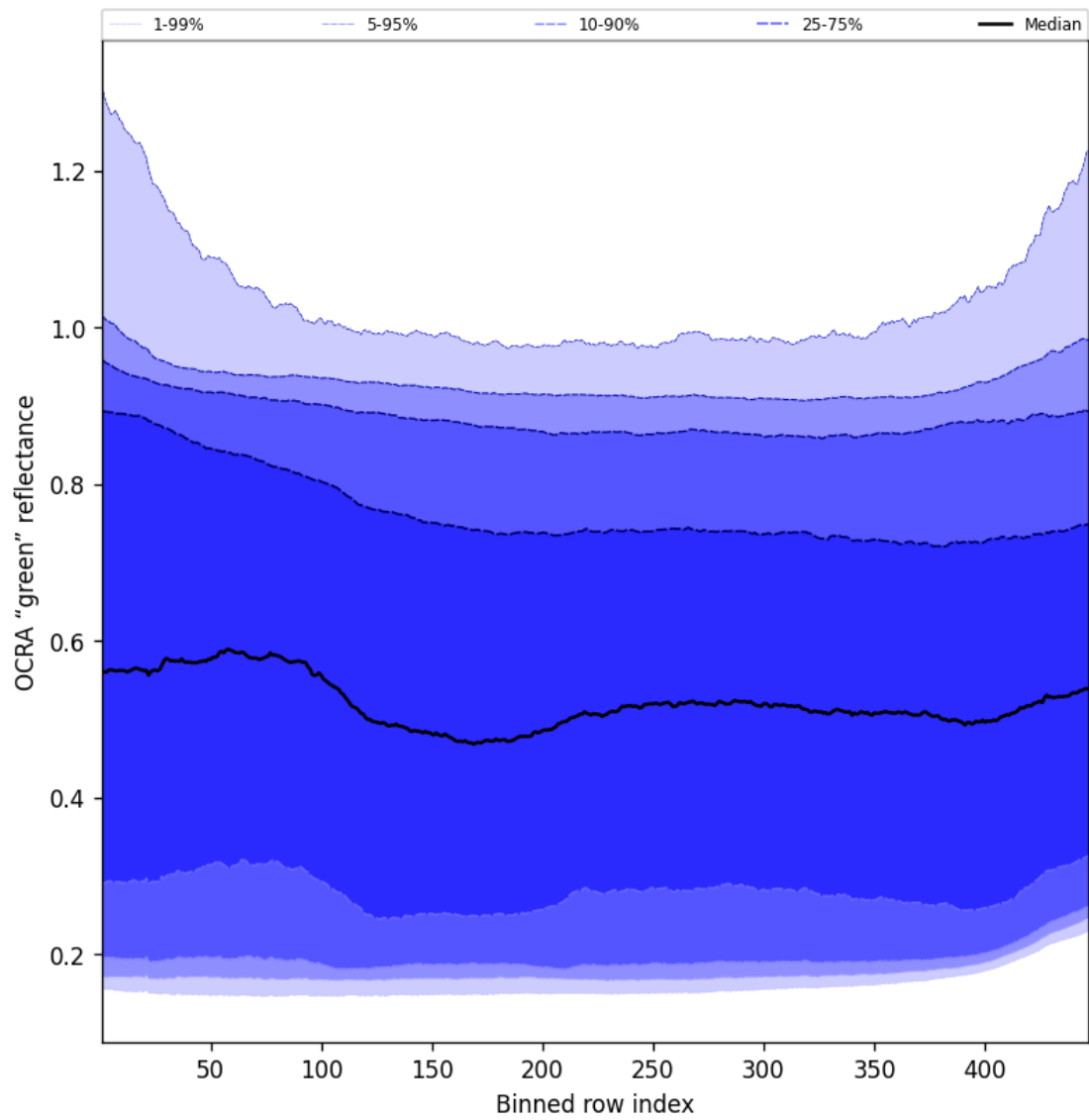
Figure 68: Along track statistics of “OCRA “green” reflectance” for 2025-01-23 to 2025-01-24
