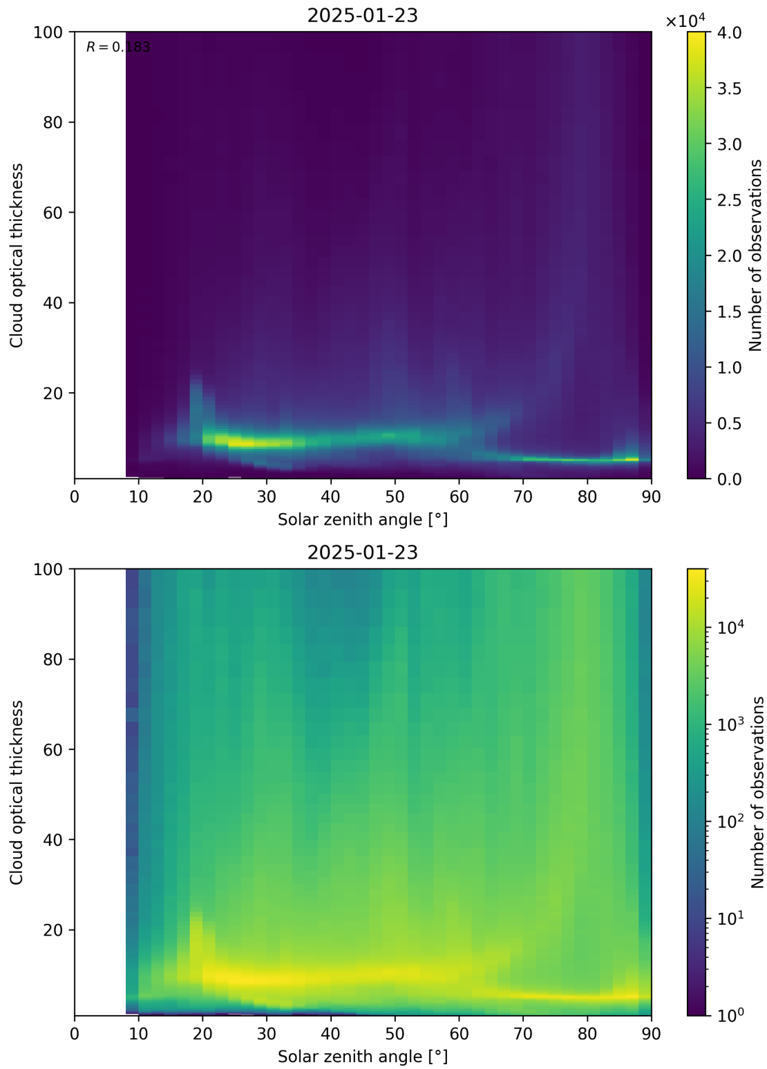
Figure 103: Scatter density plot of “Solar zenith angle” against “Cloud optical thickness” for 2025-01-23 to 2025-01-24.
