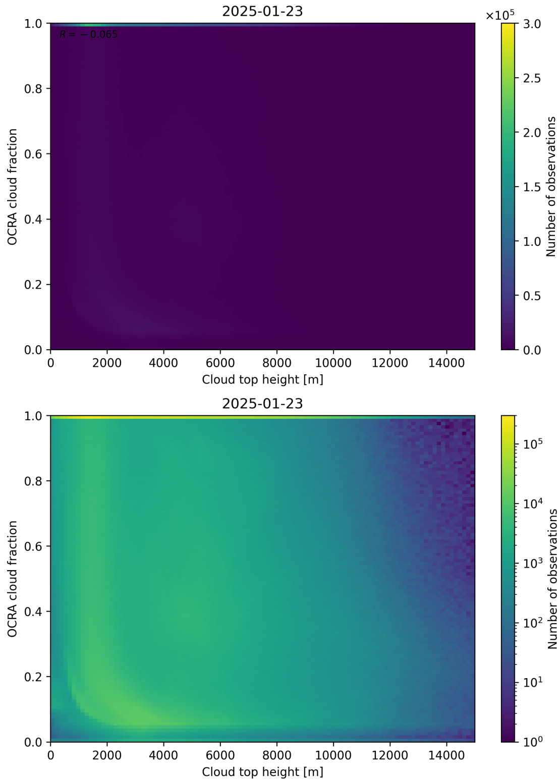
Figure 87: Scatter density plot of “Cloud top height” against “OCRA cloud fraction” for 2025-01-23 to 2025-01-24.
