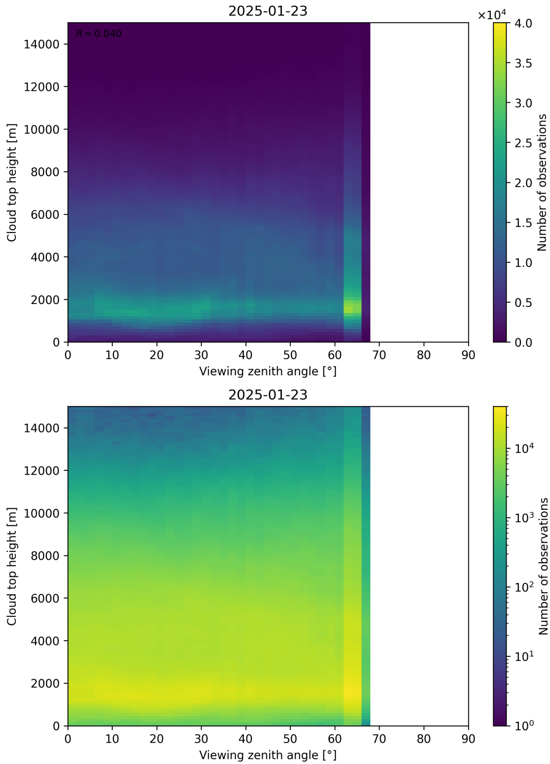
Figure 112: Scatter density plot of “Viewing zenith angle” against “Cloud top height” for 2025-01-23 to 2025-01-24.
