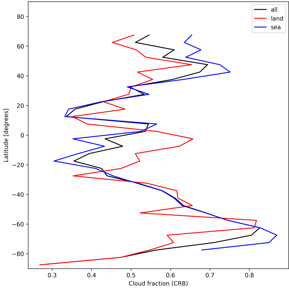
Figure 26: Zonal average of “Cloud fraction (CRB)” for 2025-01-23 to 2025-01-24.
