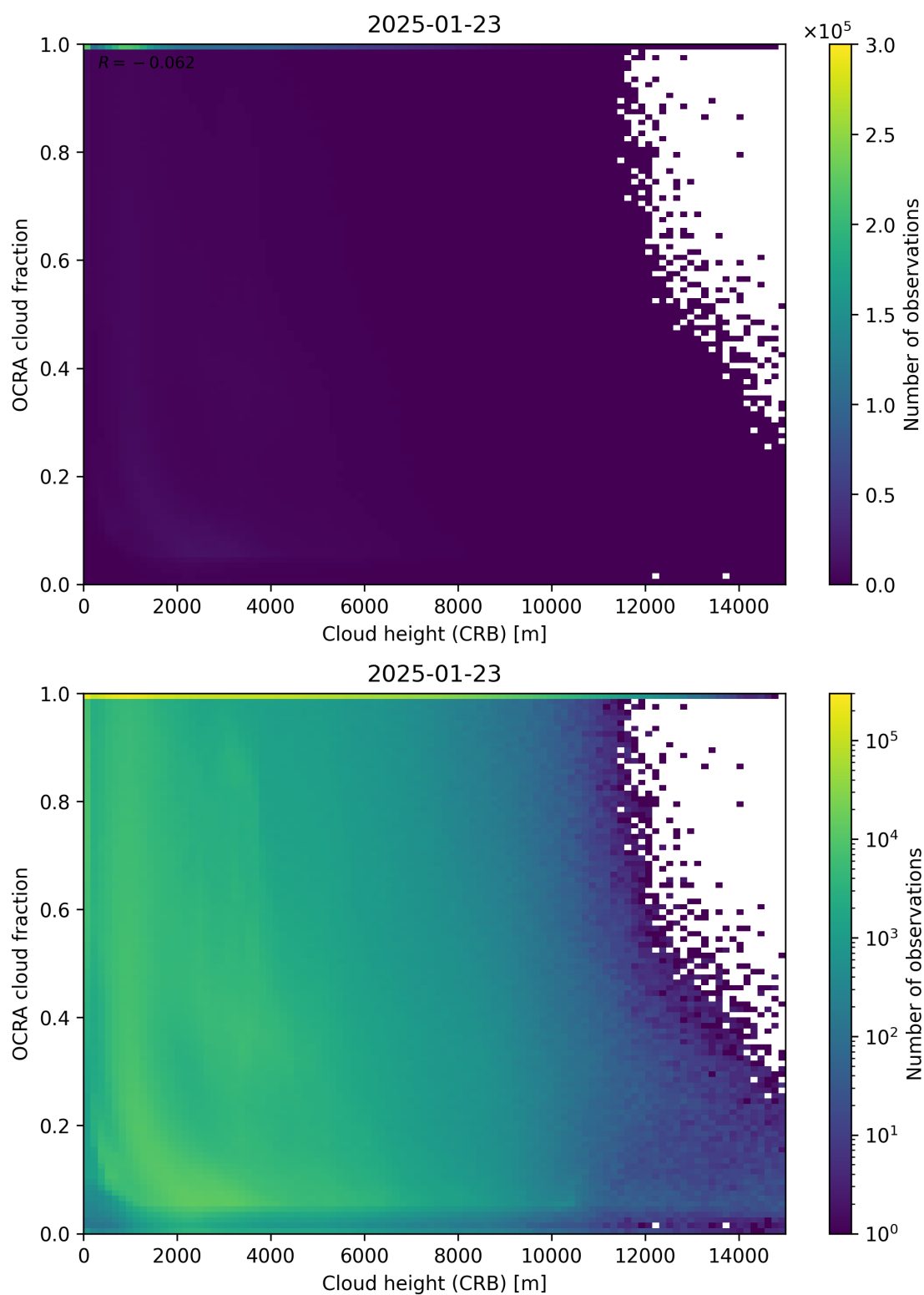
Figure 81: Scatter density plot of “Cloud height (CRB)” against “OCRA cloud fraction” for 2025-01-23 to 2025-01-24.
