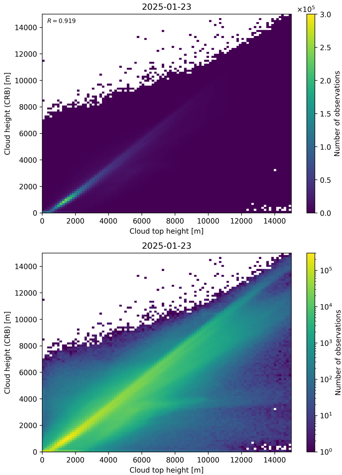
Figure 89: Scatter density plot of “Cloud top height” against “Cloud height (CRB)” for 2025-01-23 to 2025-01-24.
