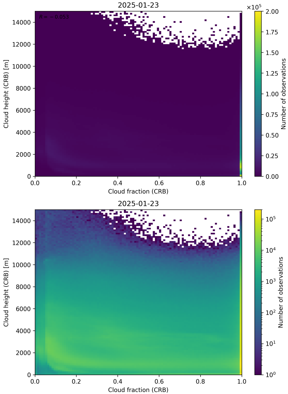
Figure 79: Scatter density plot of “Cloud fraction (CRB)” against “Cloud height (CRB)” for 2025-01-23 to 2025-01-24.
