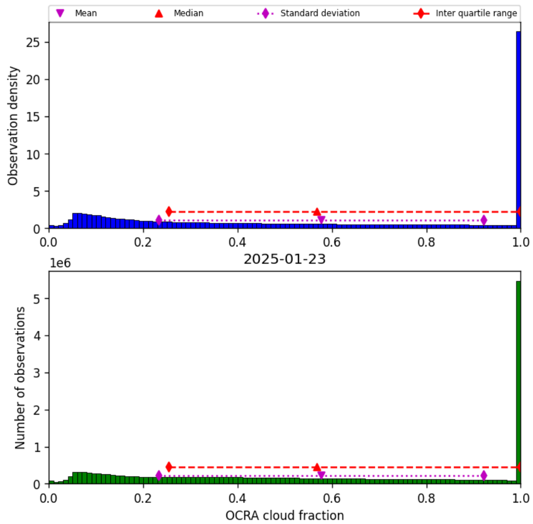
Figure 50: Histogram of “OCRA cloud fraction” for 2025-01-23 to 2025-01-24
