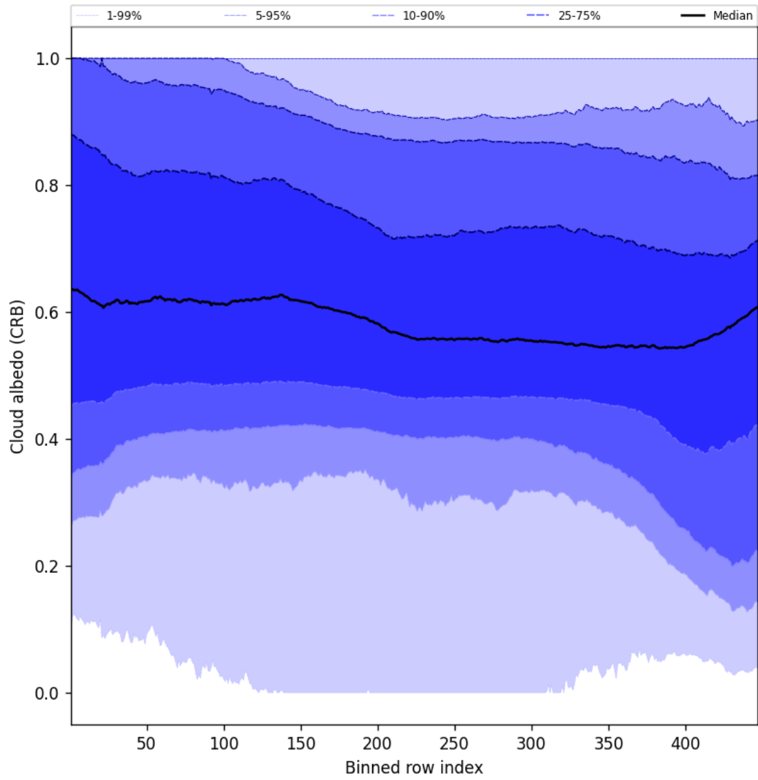
Figure 60: Along track statistics of “Cloud albedo (CRB)” for 2025-01-23 to 2025-01-24
