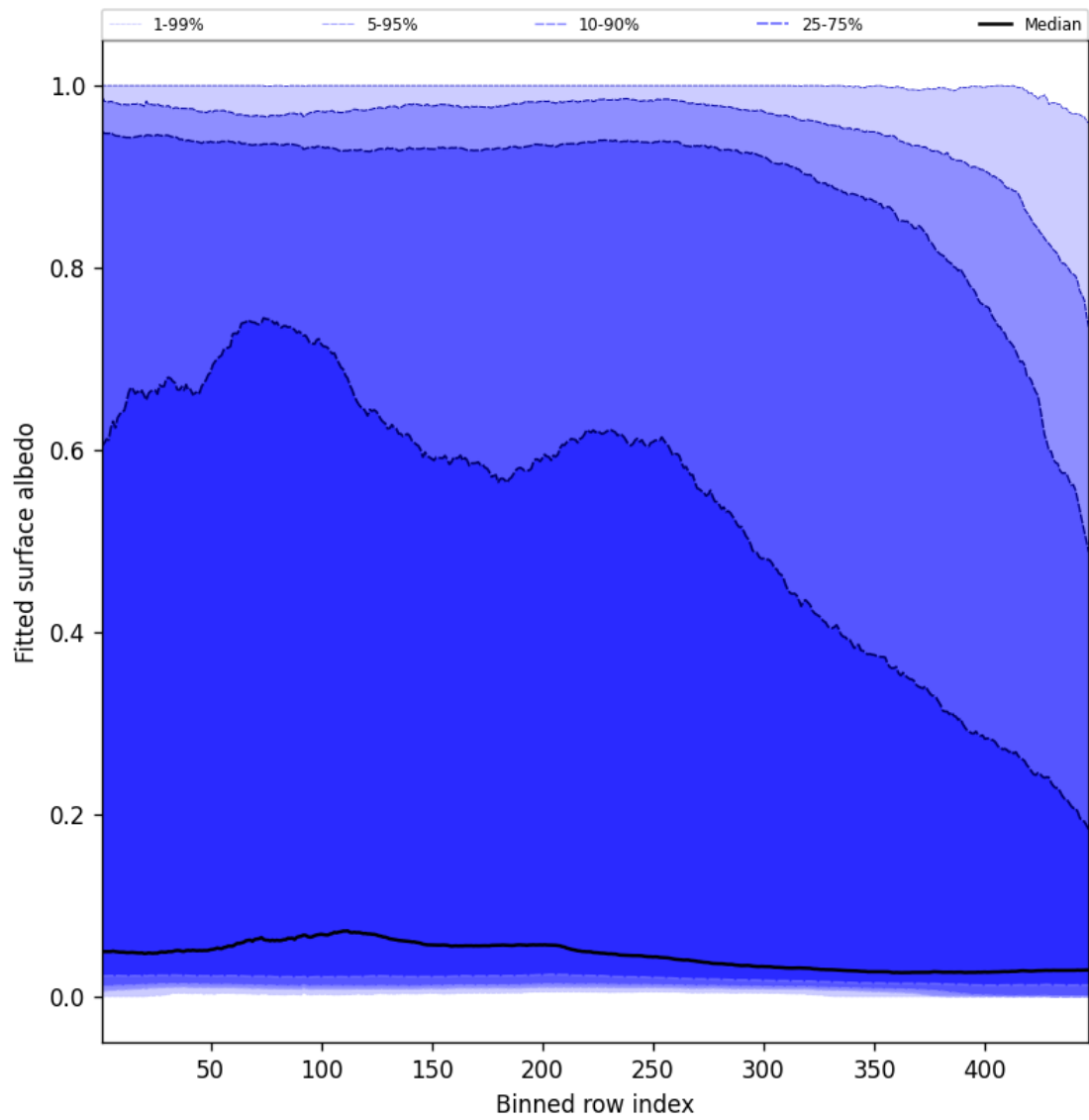
Figure 61: Along track statistics of “Fitted surface albedo” for 2025-01-23 to 2025-01-24
