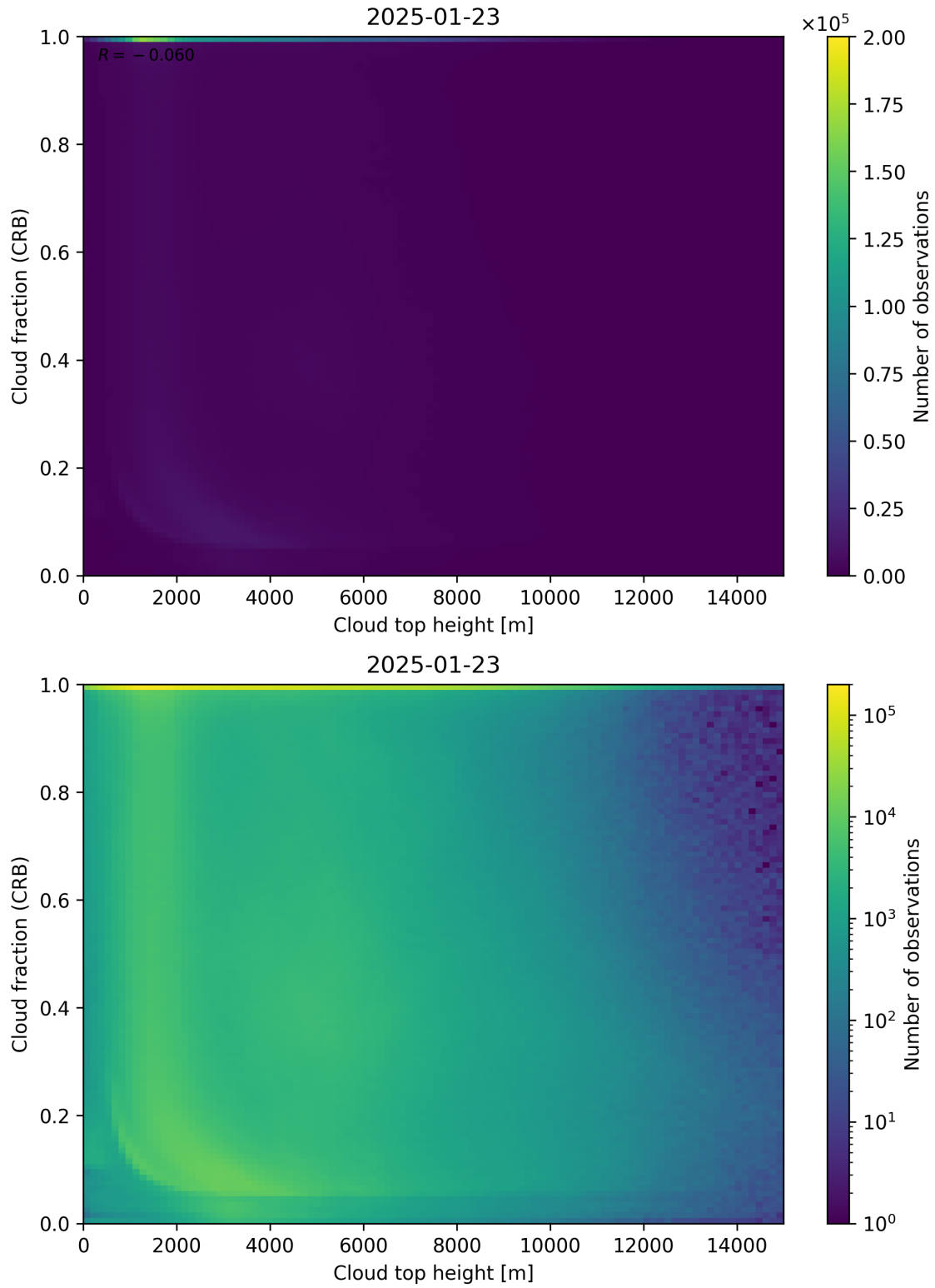
Figure 88: Scatter density plot of “Cloud top height” against “Cloud fraction (CRB)” for 2025-01-23 to 2025-01-24.
