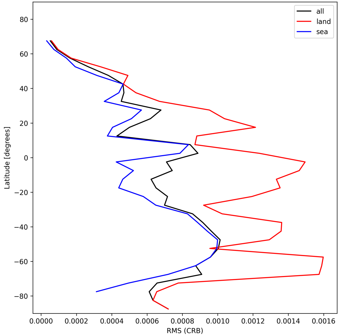
Figure 32: Zonal average of “RMS (CRB)” for 2025-01-23 to 2025-01-24.
