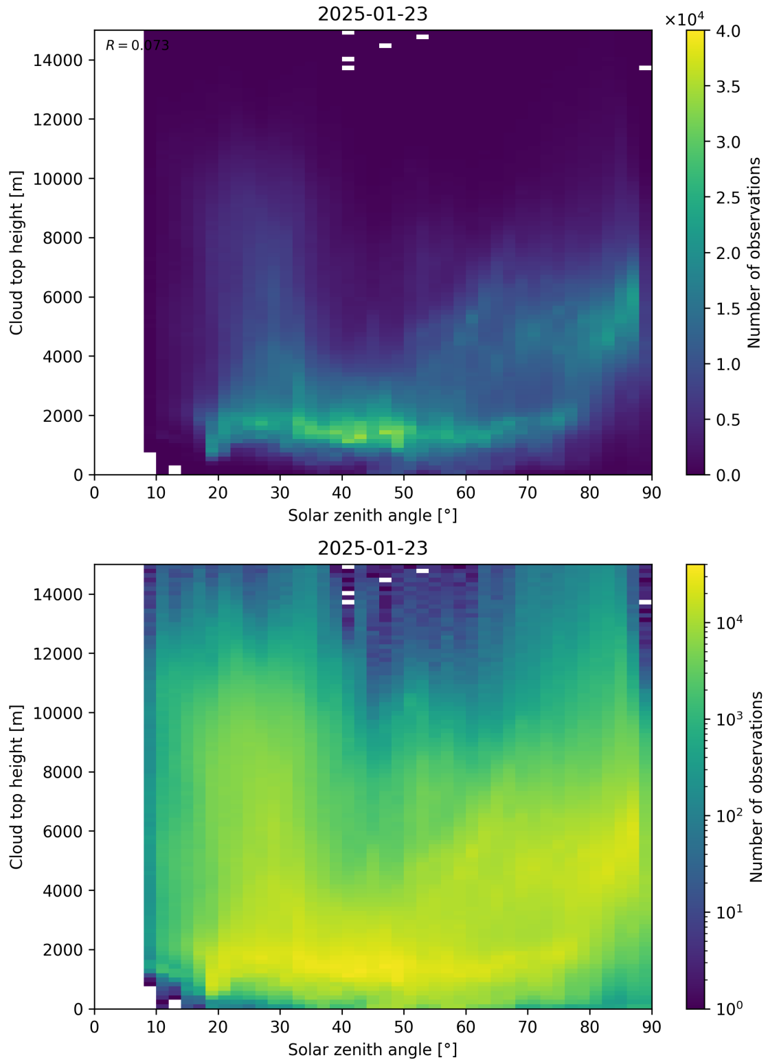
Figure 104: Scatter density plot of “Solar zenith angle” against “Cloud top height” for 2025-01-23 to 2025-01-24.
