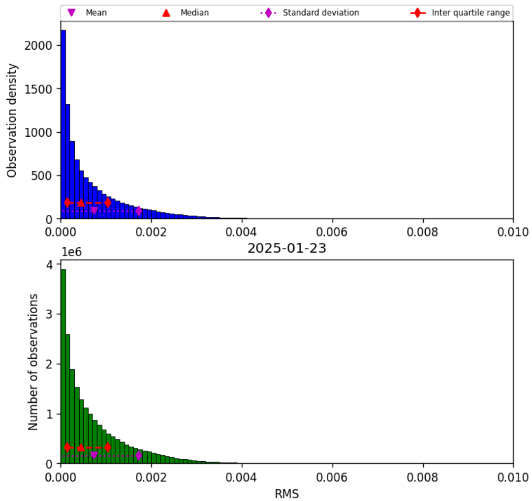
Figure 47: Histogram of “RMS” for 2025-01-23 to 2025-01-24
