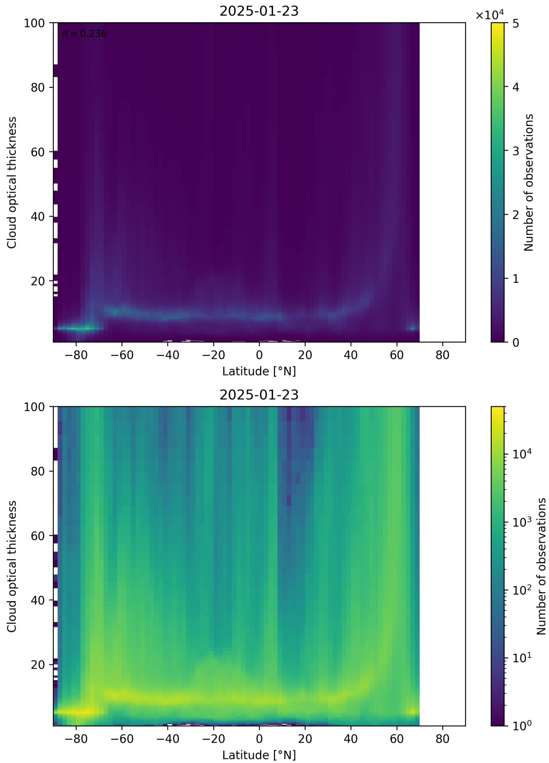
Figure 96: Scatter density plot of “Latitude” against “Cloud optical thickness” for 2025-01-23 to 2025-01-24.
