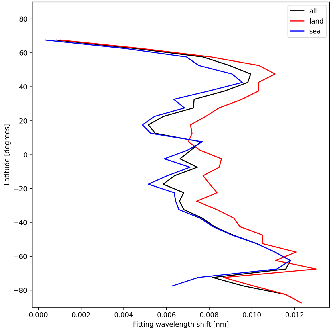
Figure 33: Zonal average of “Fitting wavelength shift” for 2025-01-23 to 2025-01-24.
