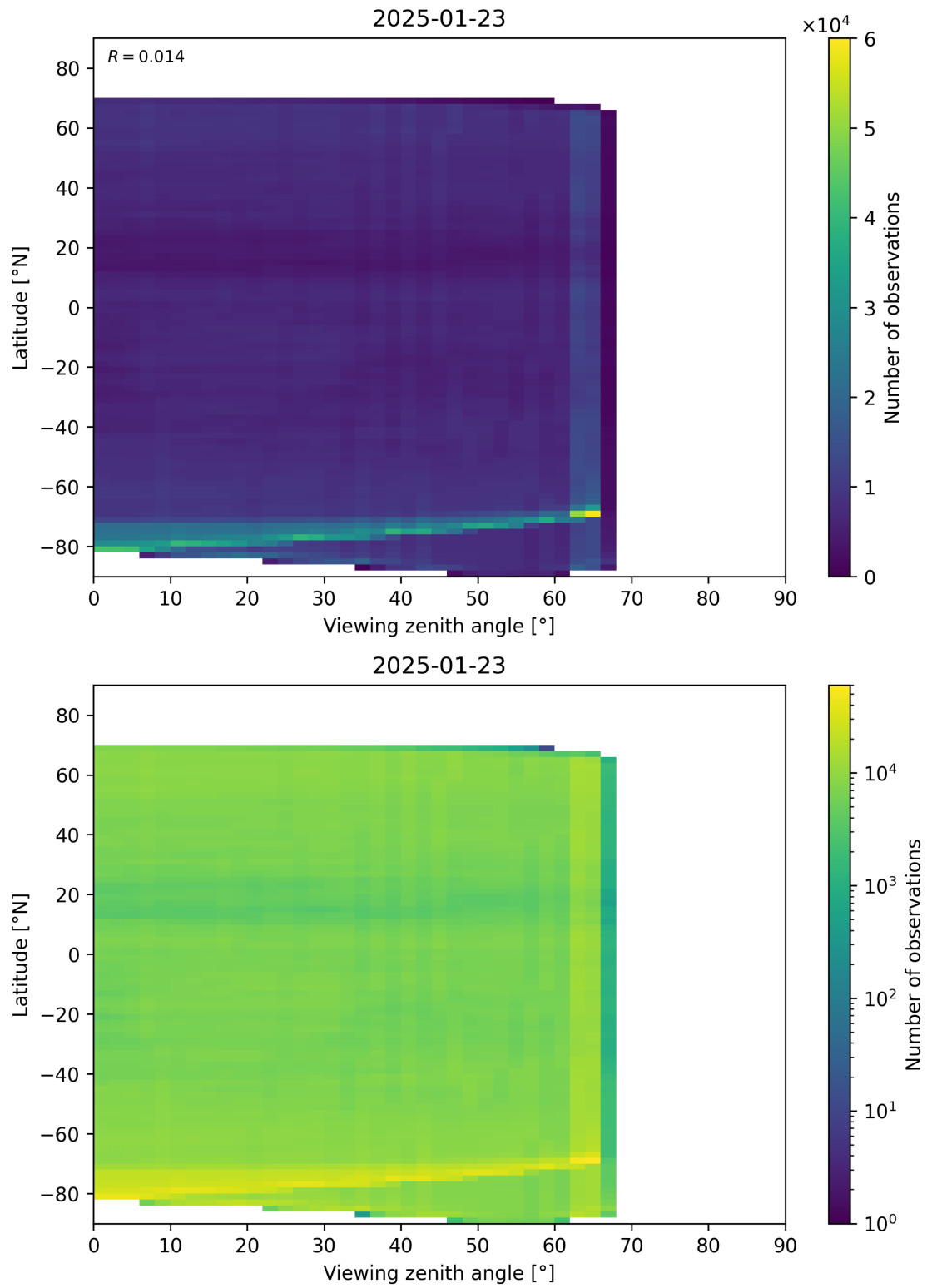
Figure 113: Scatter density plot of “Viewing zenith angle” against “Latitude” for 2025-01-23 to 2025-01-24.
