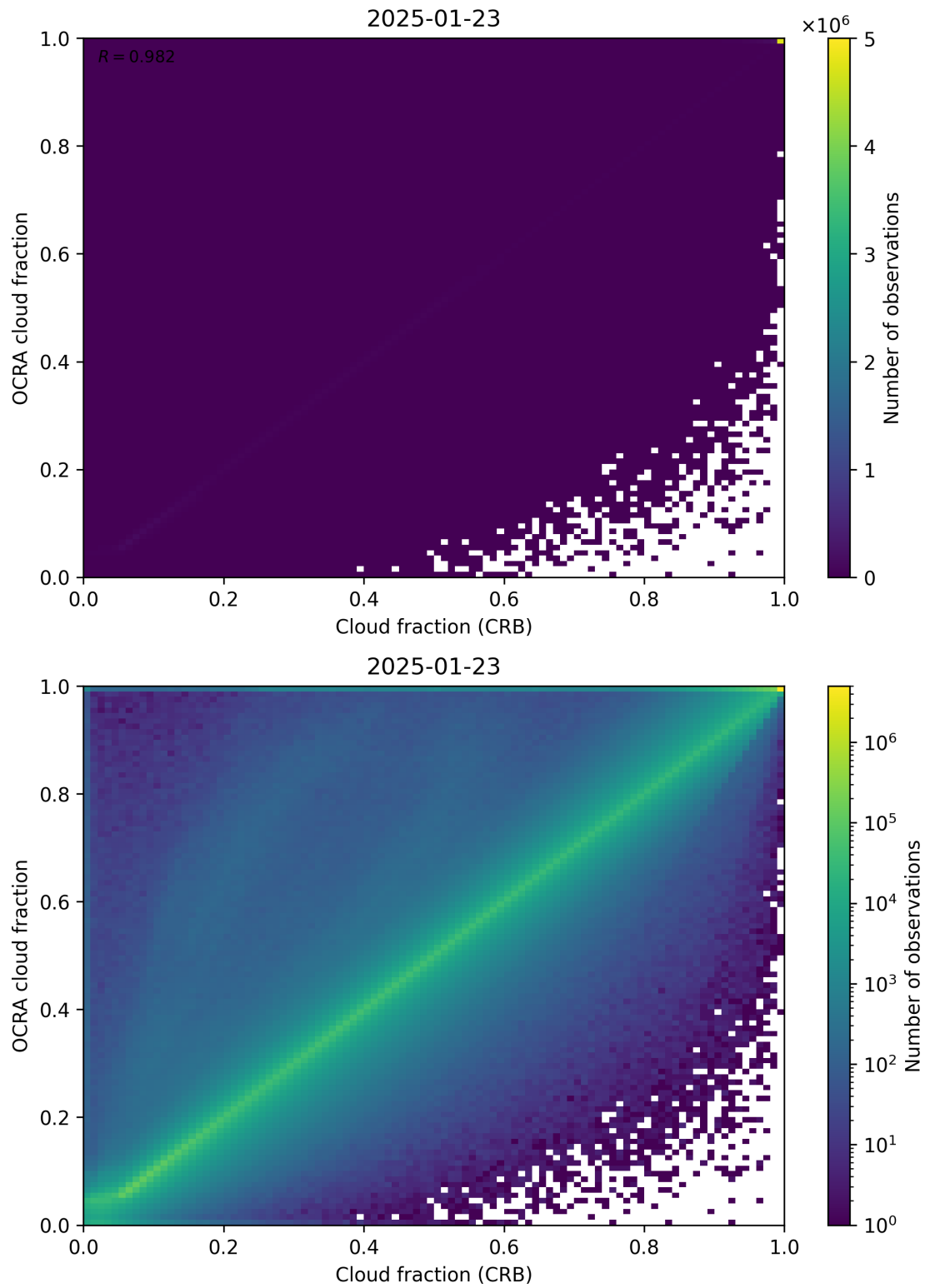
Figure 78: Scatter density plot of “Cloud fraction (CRB)” against “OCRA cloud fraction” for 2025-01-23 to 2025-01-24.
