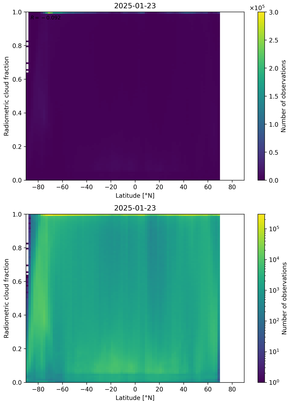
Figure 92: Scatter density plot of “Latitude” against “Radiometric cloud fraction” for 2025-01-23 to 2025-01-24.
