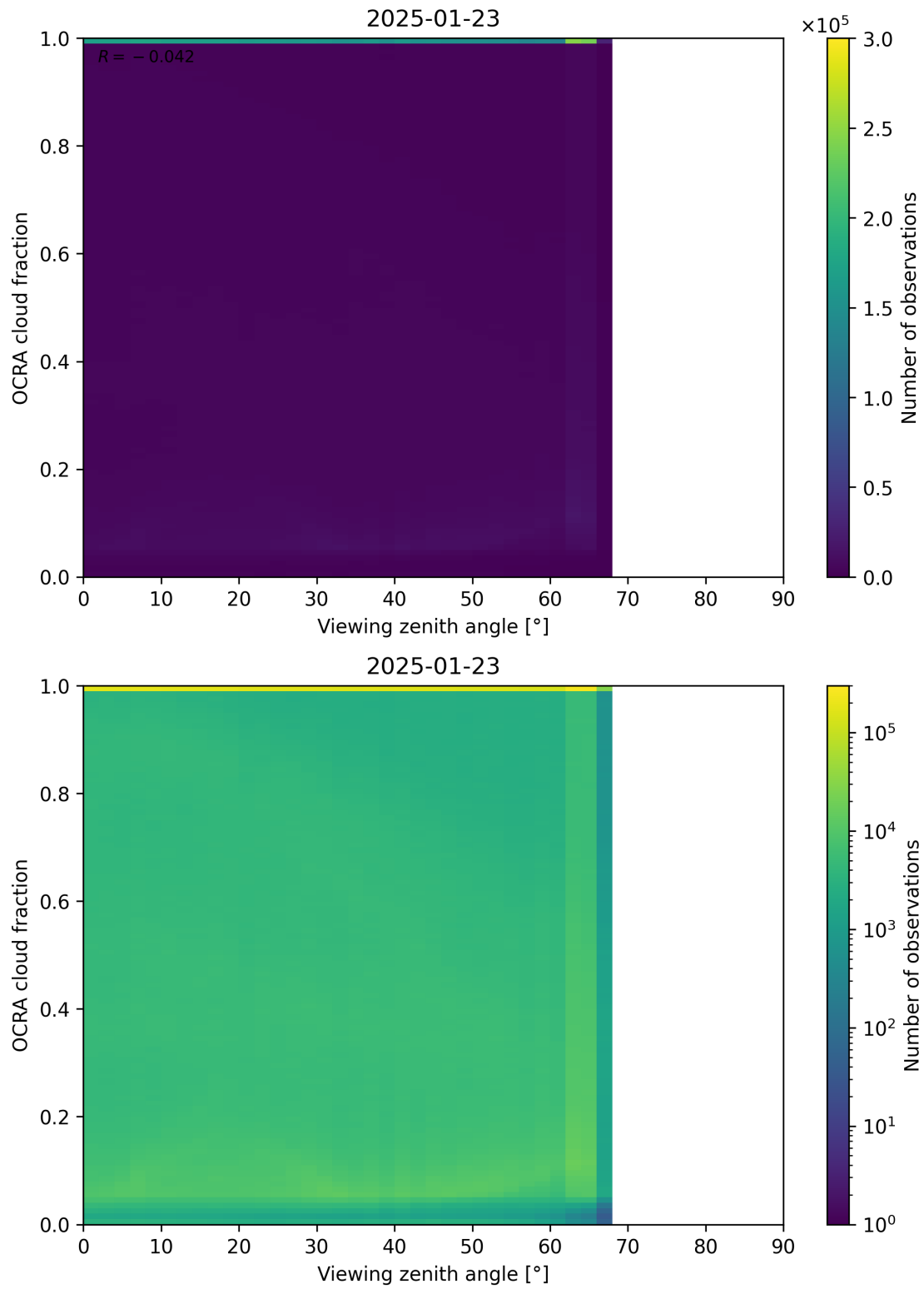
Figure 108: Scatter density plot of “Viewing zenith angle” against “OCRA cloud fraction” for 2025-01-23 to 2025-01-24.
