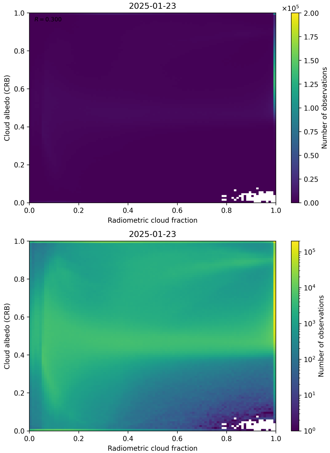
Figure 71: Scatter density plot of “Radiometric cloud fraction” against “Cloud albedo (CRB)” for 2025-01-23 to 2025-01-24.
