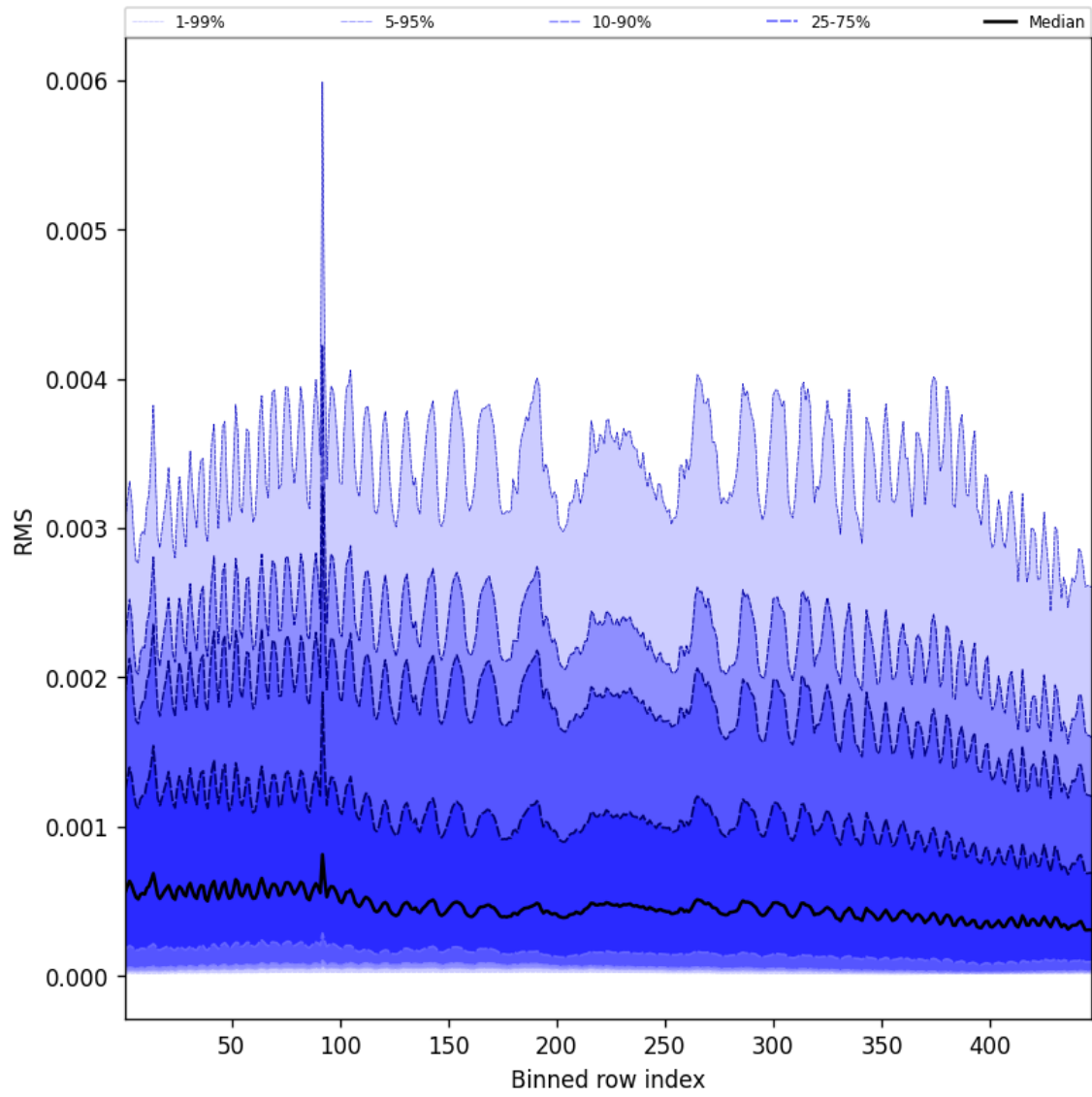
Figure 63: Along track statistics of “RMS” for 2025-01-23 to 2025-01-24
