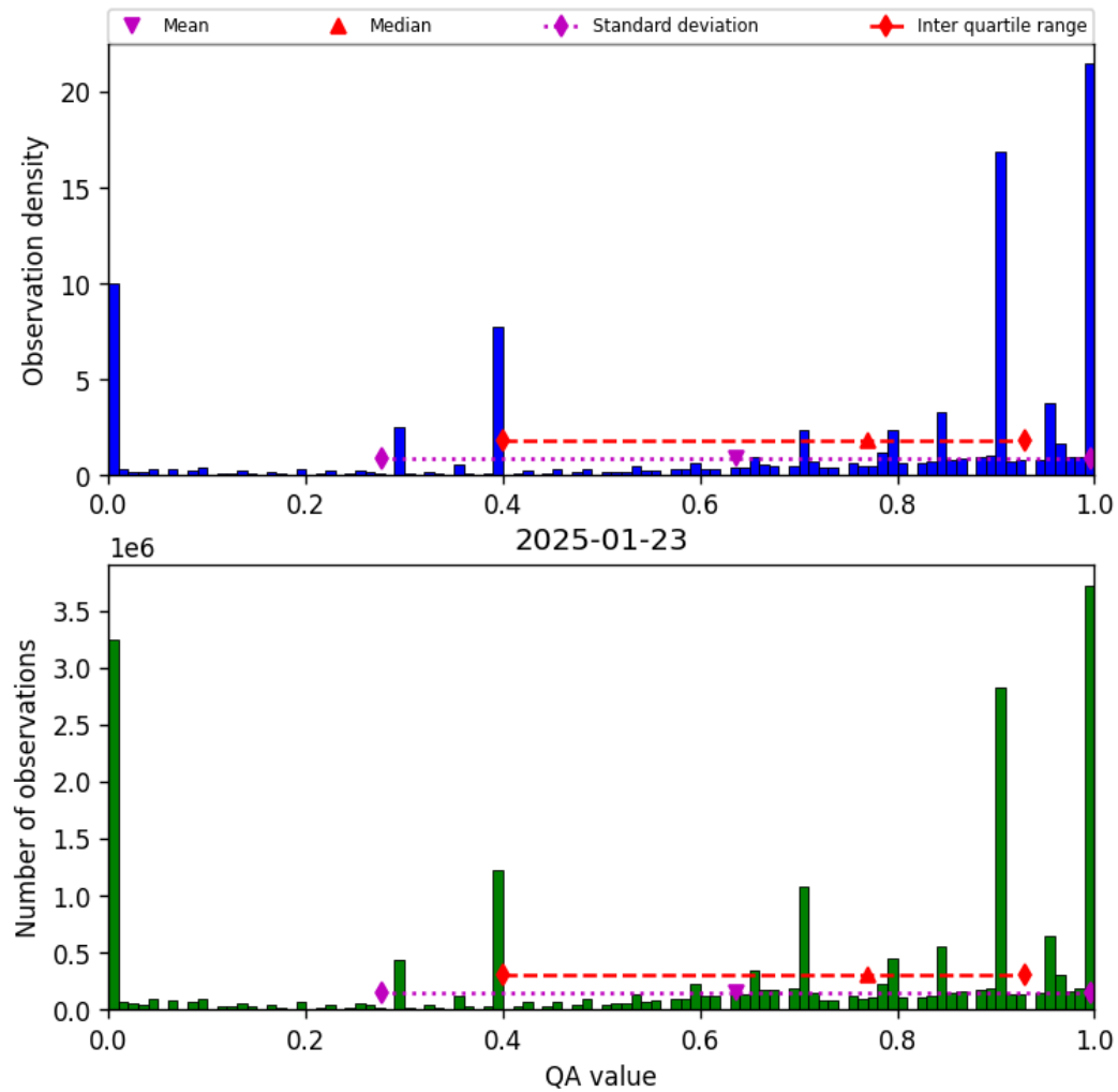
Figure 38: Histogram of “QA value” for 2025-01-23 to 2025-01-24
