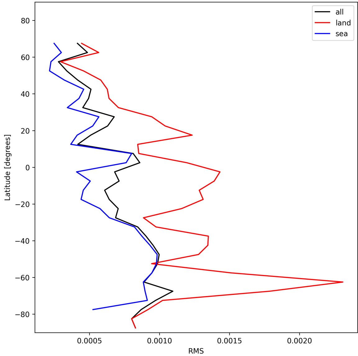
Figure 31: Zonal average of “RMS” for 2025-01-23 to 2025-01-24.
