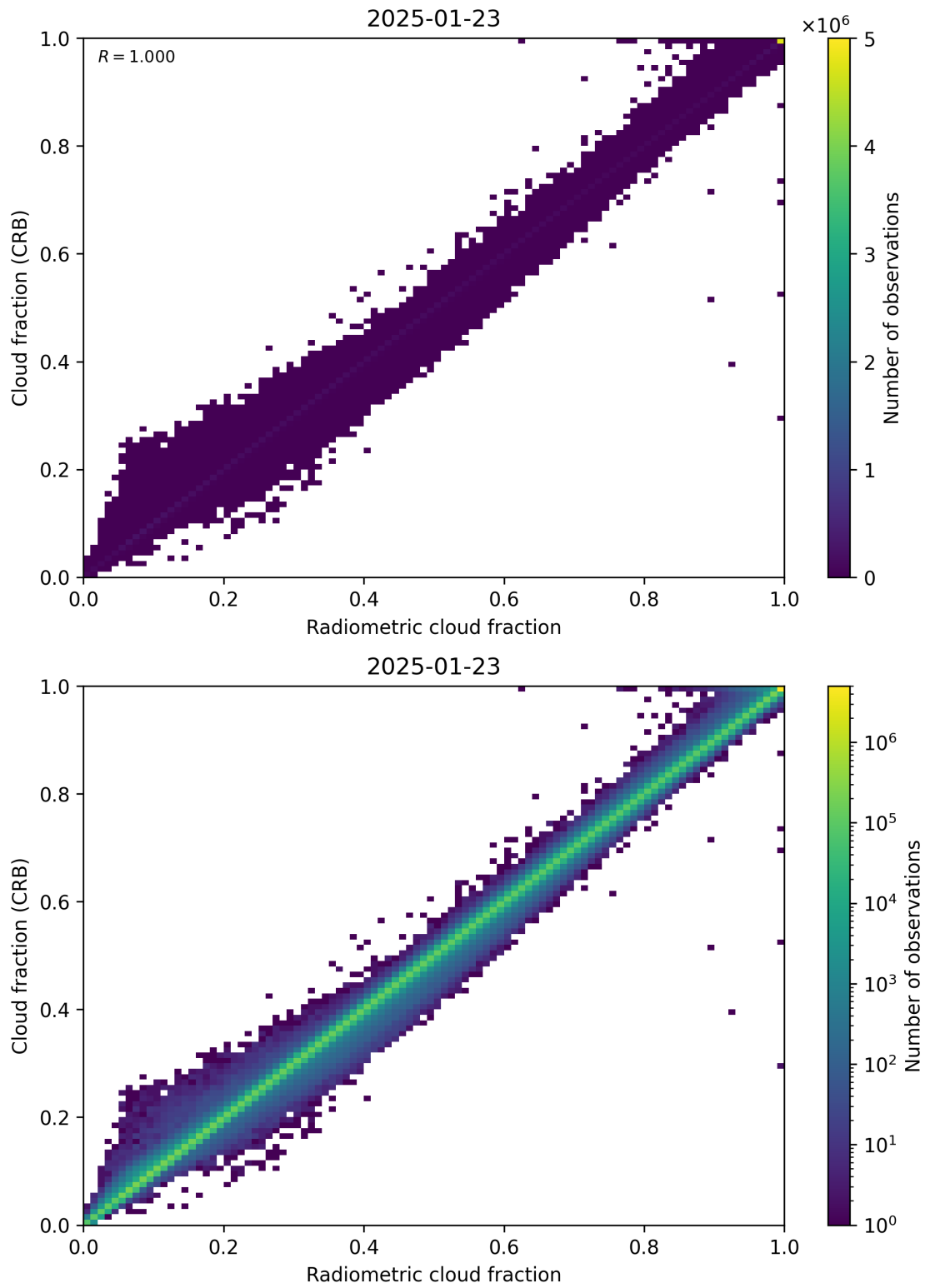
Figure 73: Scatter density plot of “Radiometric cloud fraction” against “Cloud fraction (CRB)” for 2025-01-23 to 2025-01-24.
