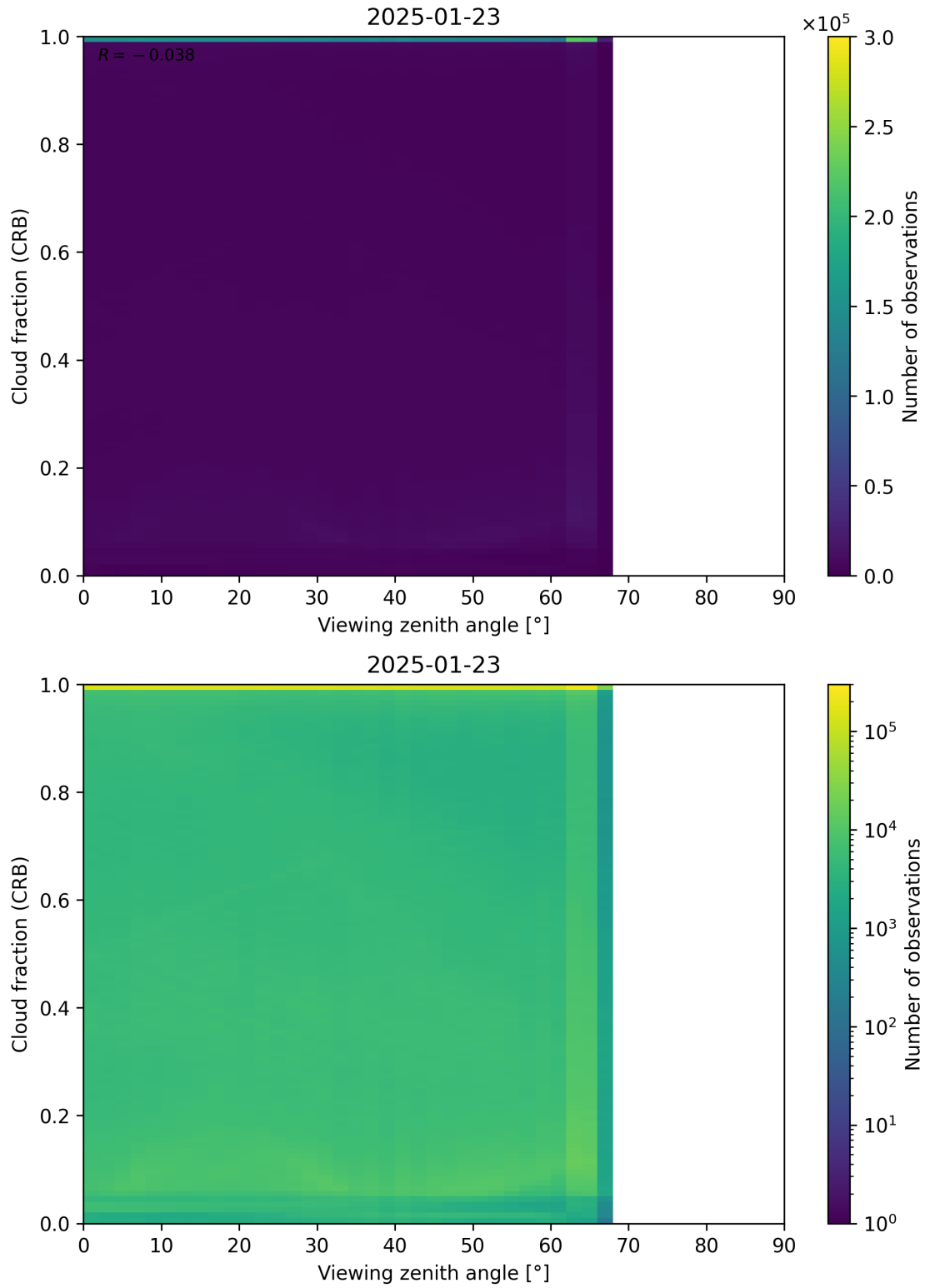
Figure 109: Scatter density plot of “Viewing zenith angle” against “Cloud fraction (CRB)” for 2025-01-23 to 2025-01-24.
