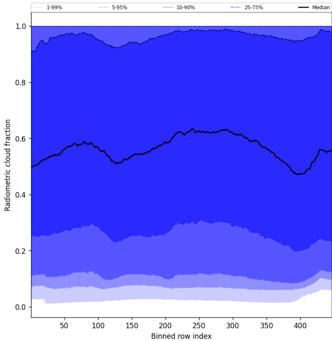
Figure 55: Along track statistics of “Radiometric cloud fraction” for 2025-01-23 to 2025-01-24
