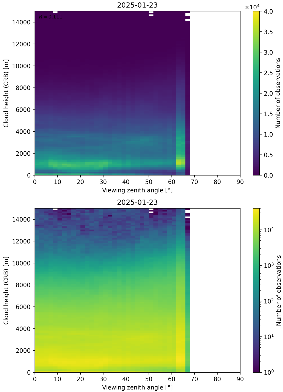
Figure 110: Scatter density plot of “Viewing zenith angle” against “Cloud height (CRB)” for 2025-01-23 to 2025-01-24.
