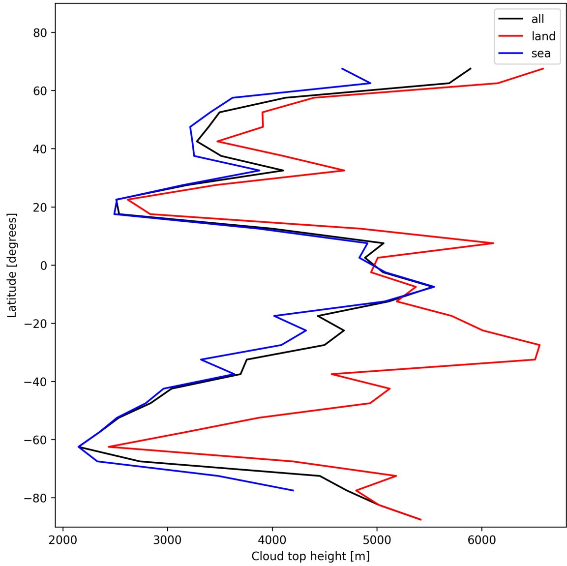
Figure 24: Zonal average of “Cloud top height” for 2025-01-23 to 2025-01-24.
