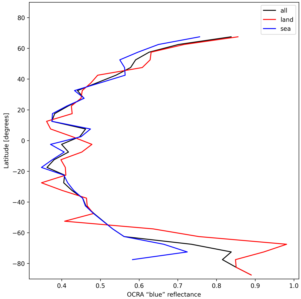
Figure 35: Zonal average of “OCRA “blue” reflectance” for 2025-01-23 to 2025-01-24.
