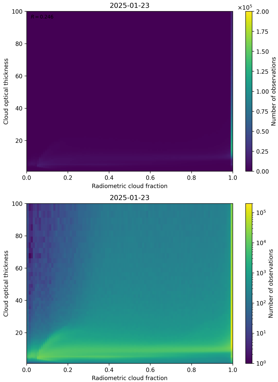
Figure 75: Scatter density plot of “Radiometric cloud fraction” against “Cloud optical thickness” for 2025-01-23 to 2025-01-24.
