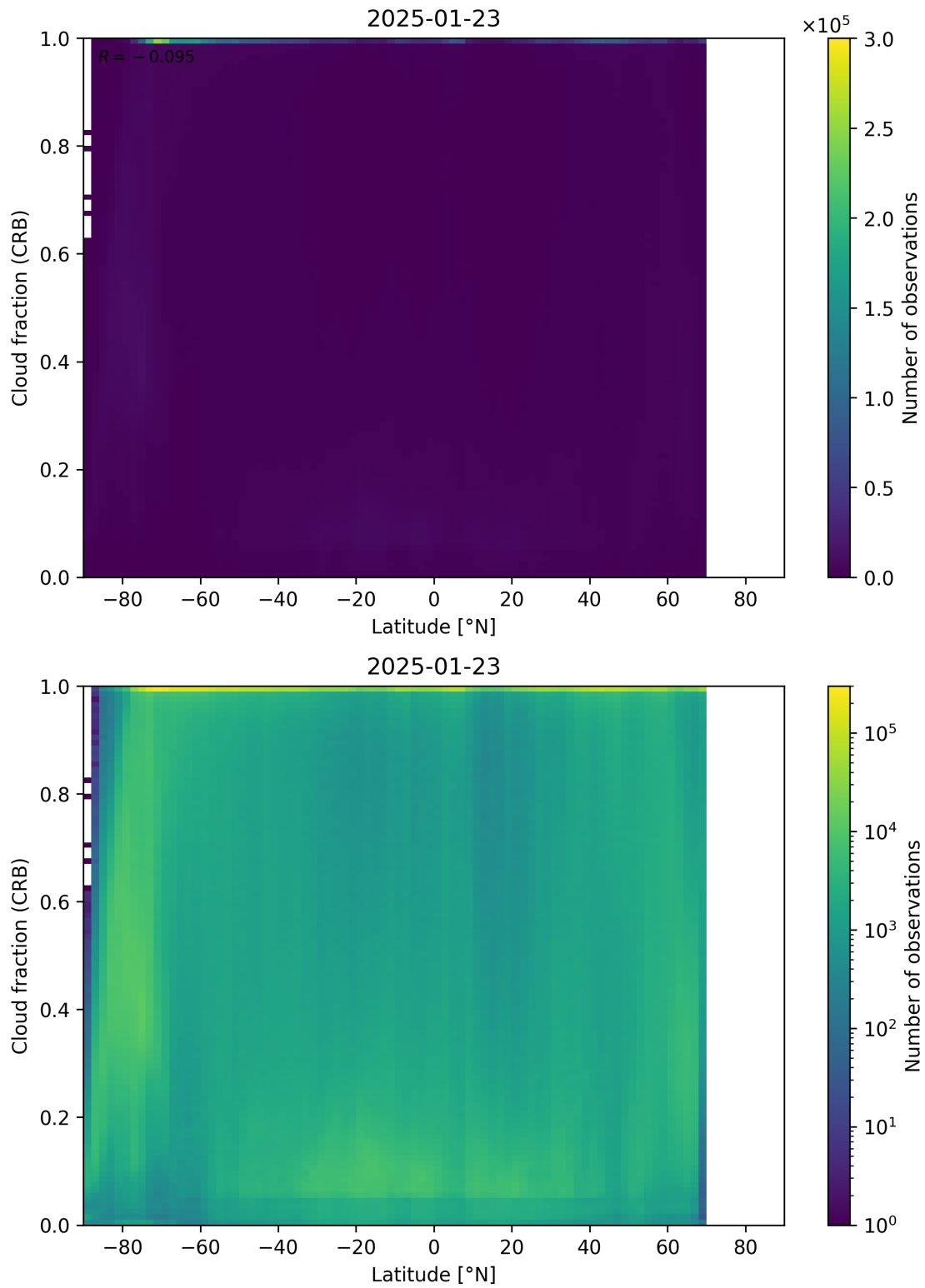
Figure 94: Scatter density plot of “Latitude” against “Cloud fraction (CRB)” for 2025-01-23 to 2025-01-24.
