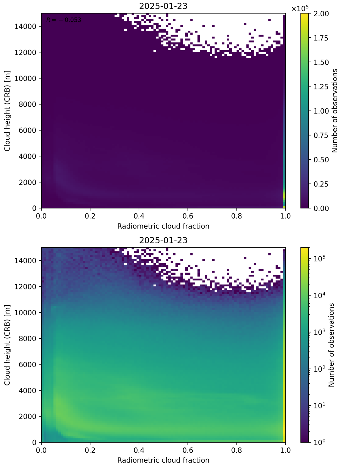
Figure 74: Scatter density plot of “Radiometric cloud fraction” against “Cloud height (CRB)” for 2025-01-23 to 2025-01-24.
