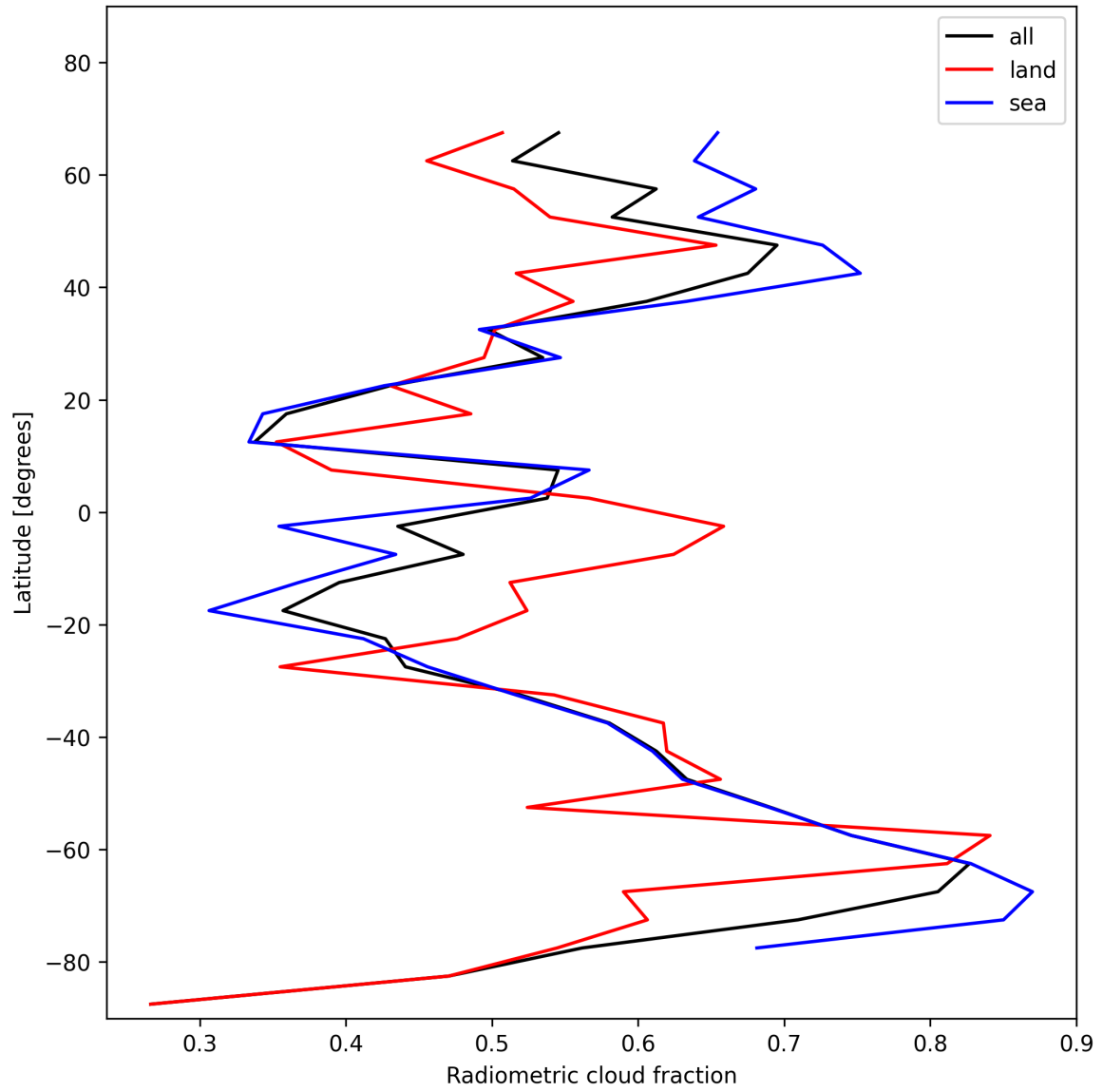
Figure 23: Zonal average of “Radiometric cloud fraction” for 2025-01-23 to 2025-01-24.
