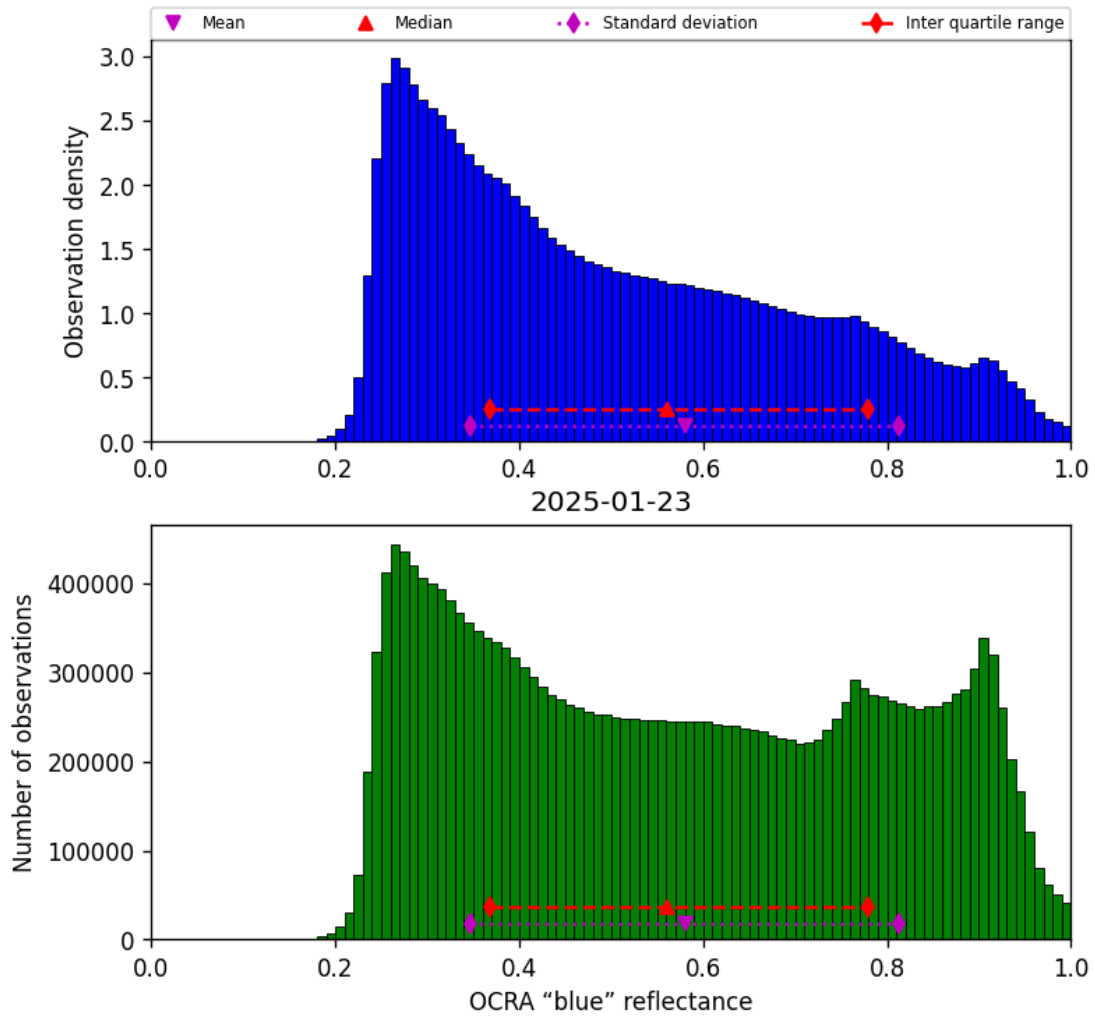
Figure 51: Histogram of “OCRA “blue” reflectance” for 2025-01-23 to 2025-01-24
