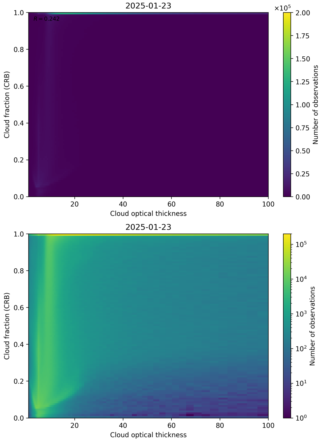
Figure 84: Scatter density plot of “Cloud optical thickness” against “Cloud fraction (CRB)” for 2025-01-23 to 2025-01-24.
