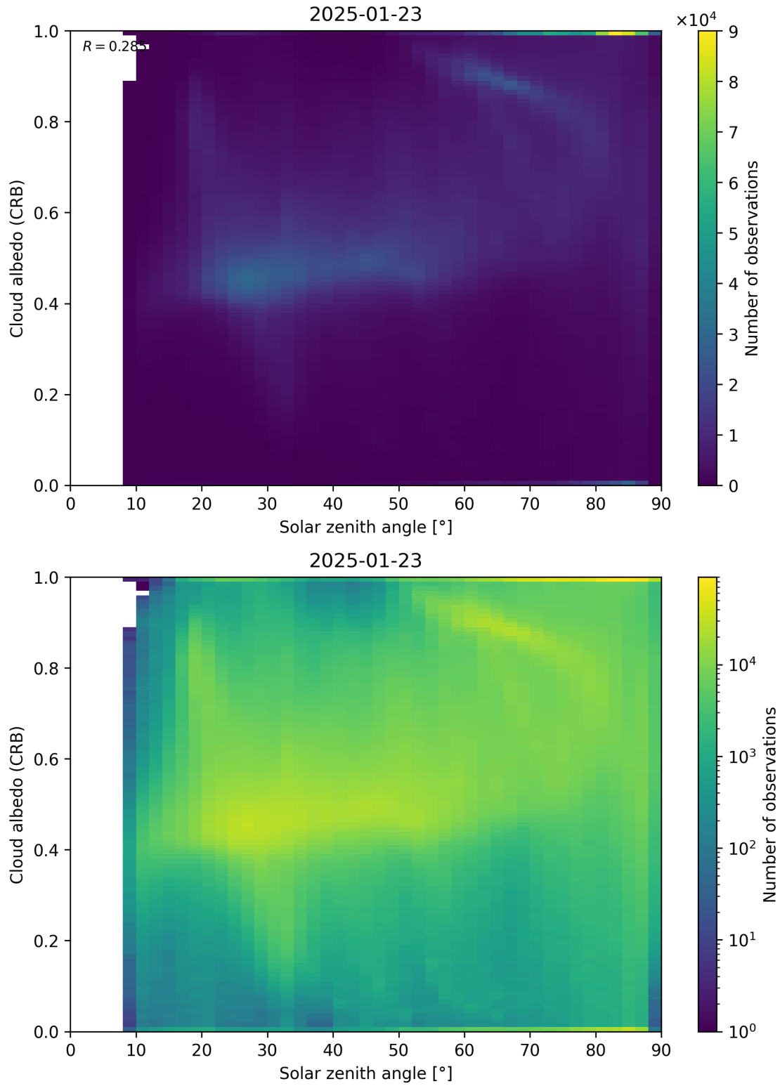
Figure 98: Scatter density plot of “Solar zenith angle” against “Cloud albedo (CRB)” for 2025-01-23 to 2025-01-24.
