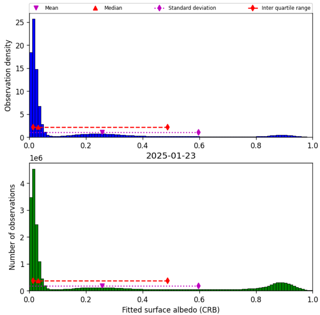
Figure 46: Histogram of “Fitted surface albedo (CRB)” for 2025-01-23 to 2025-01-24
