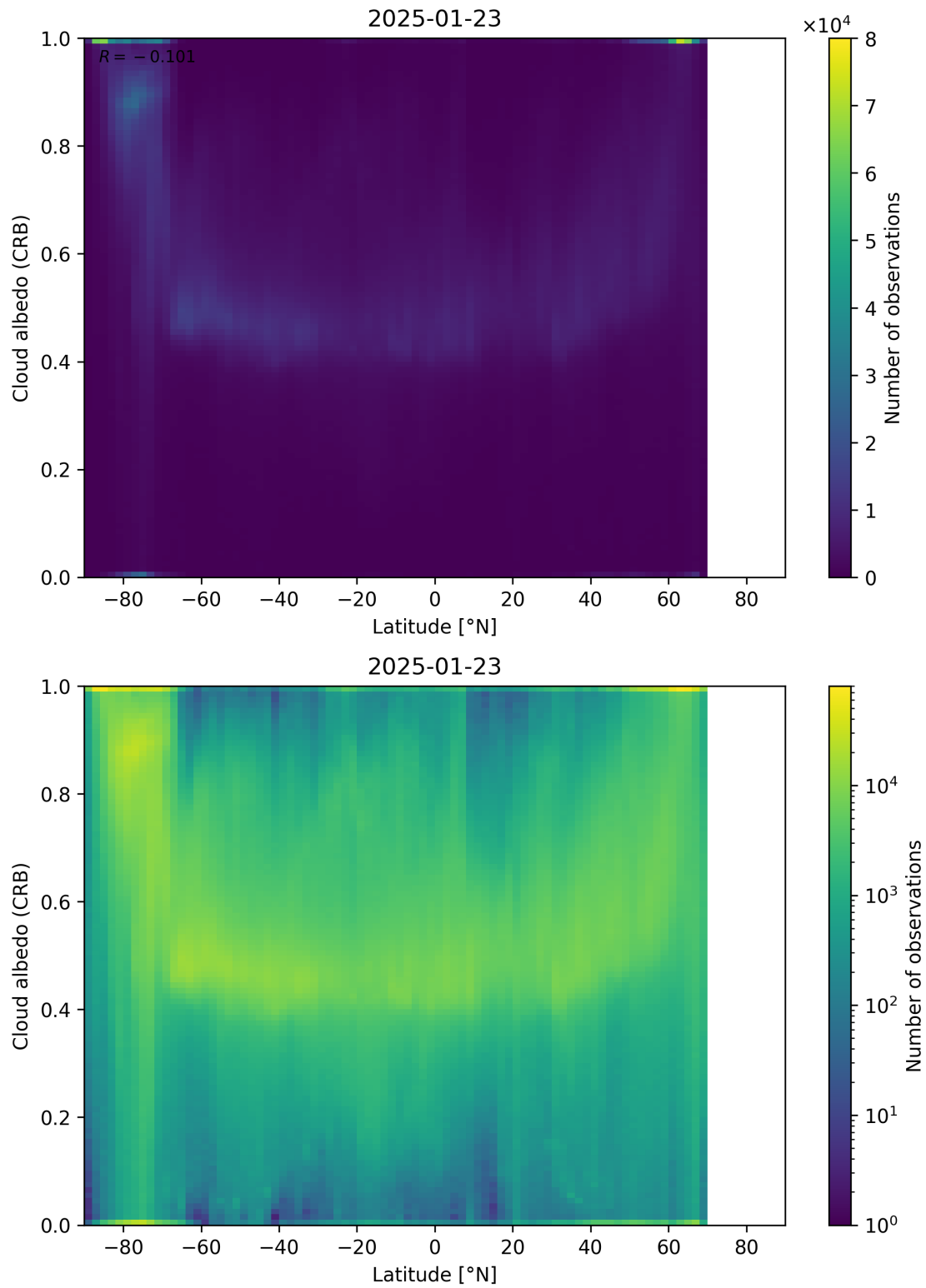
Figure 91: Scatter density plot of “Latitude” against “Cloud albedo (CRB)” for 2025-01-23 to 2025-01-24.
