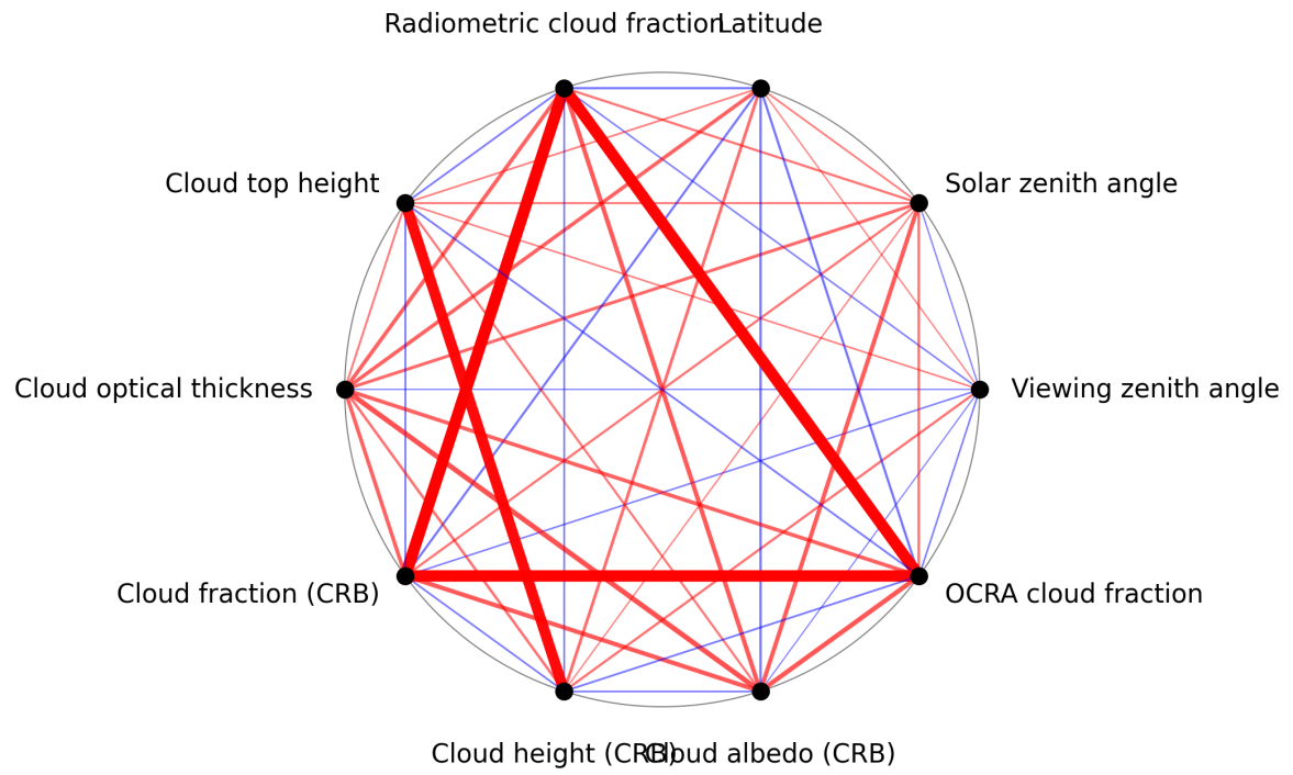
Figure 1: Map of correlation graph for 2025-01-23 to 2025-01-24.
