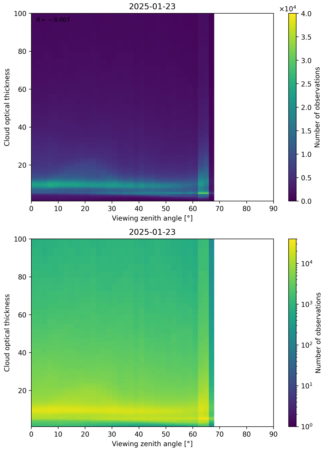
Figure 111: Scatter density plot of “Viewing zenith angle” against “Cloud optical thickness” for 2025-01-23 to 2025-01-24.
