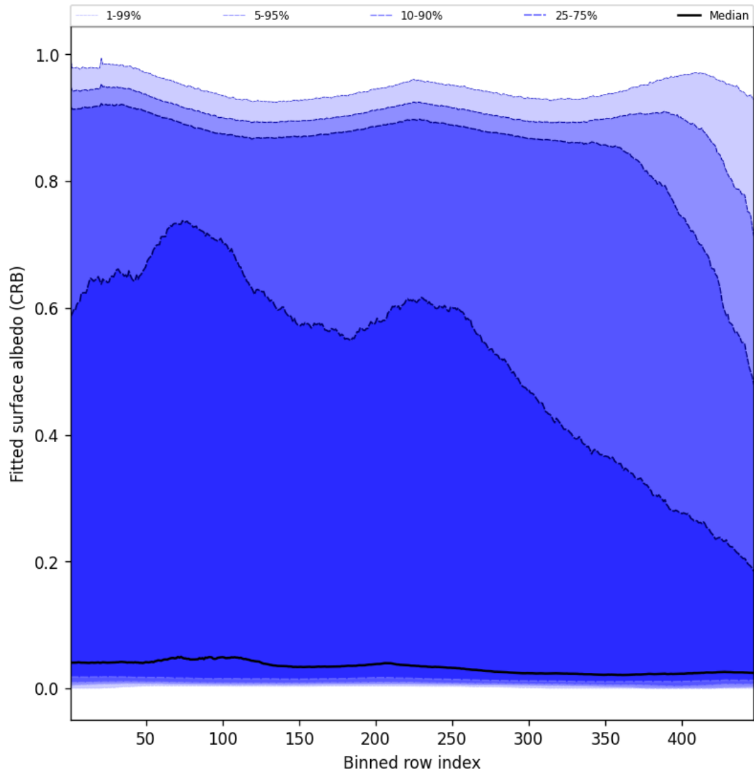
Figure 62: Along track statistics of “Fitted surface albedo (CRB)” for 2025-01-23 to 2025-01-24
