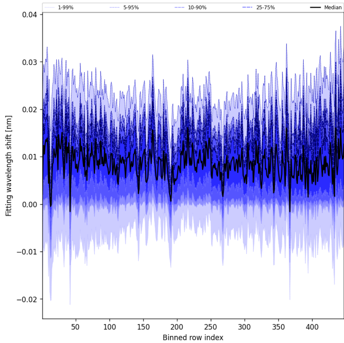
Figure 65: Along track statistics of “Fitting wavelength shift” for 2025-01-23 to 2025-01-25
