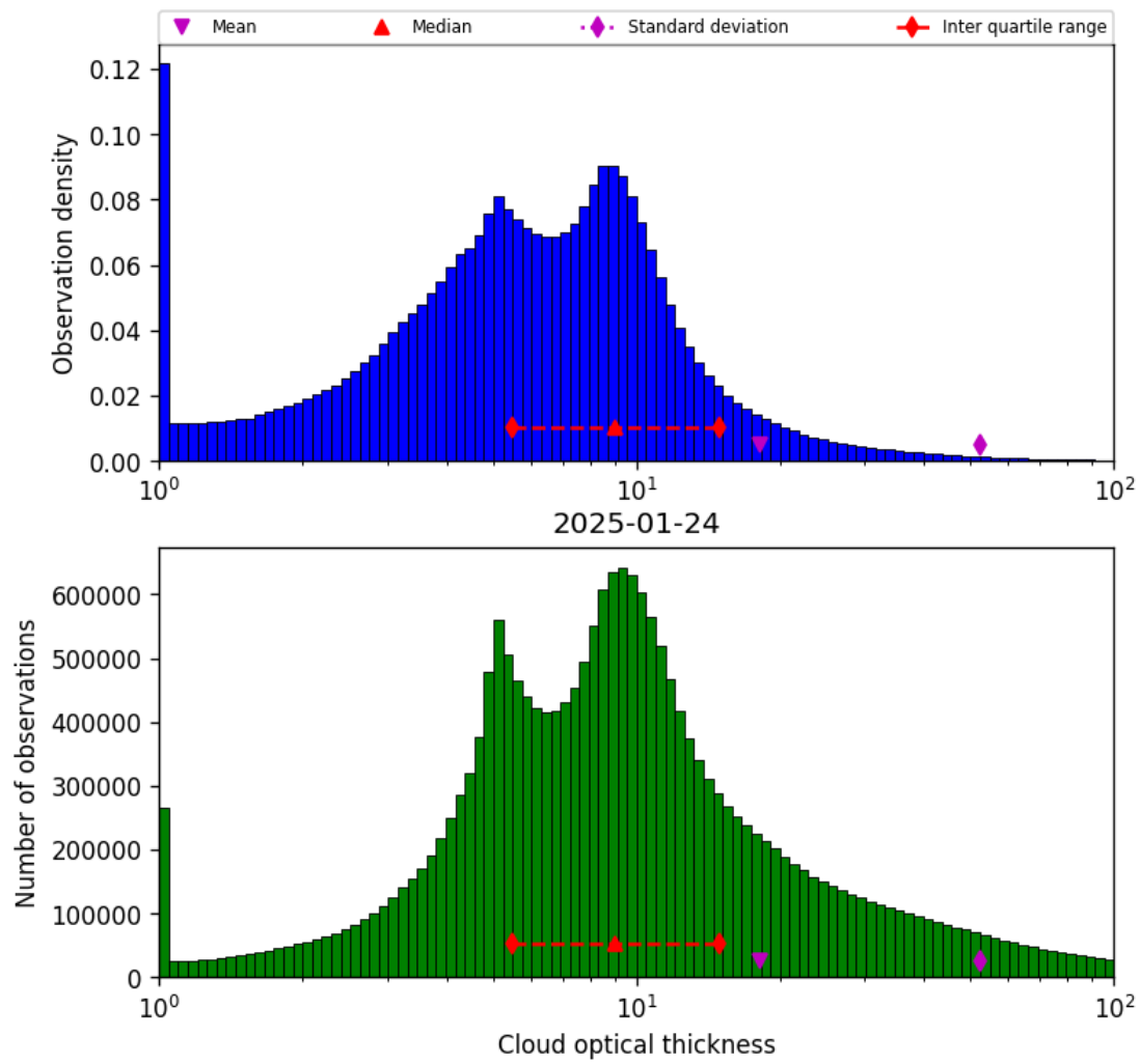
Figure 41: Histogram of “Cloud optical thickness” for 2025-01-23 to 2025-01-25
