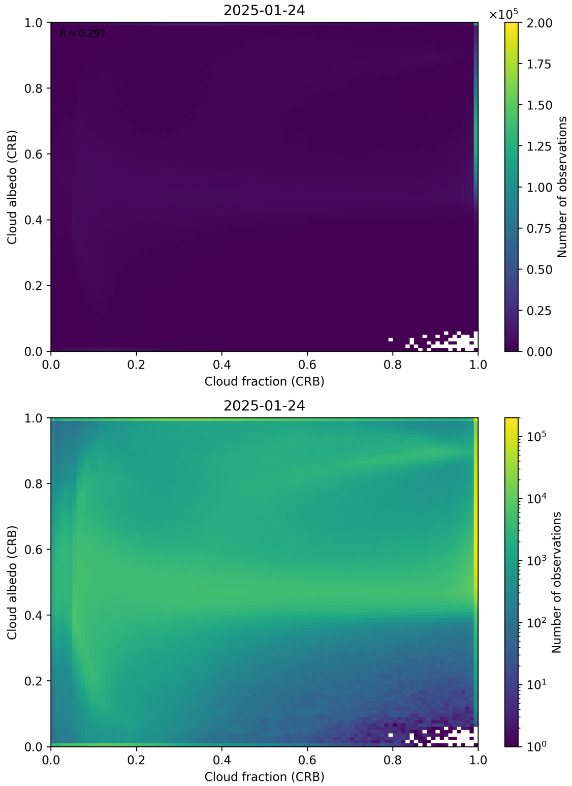
Figure 77: Scatter density plot of “Cloud fraction (CRB)” against “Cloud albedo (CRB)” for 2025-01-23 to 2025-01-25.
