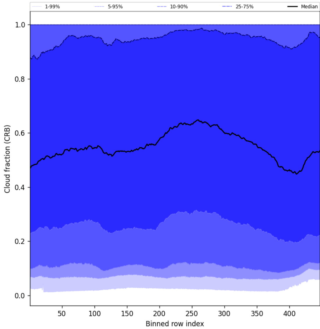
Figure 58: Along track statistics of “Cloud fraction (CRB)” for 2025-01-23 to 2025-01-25
