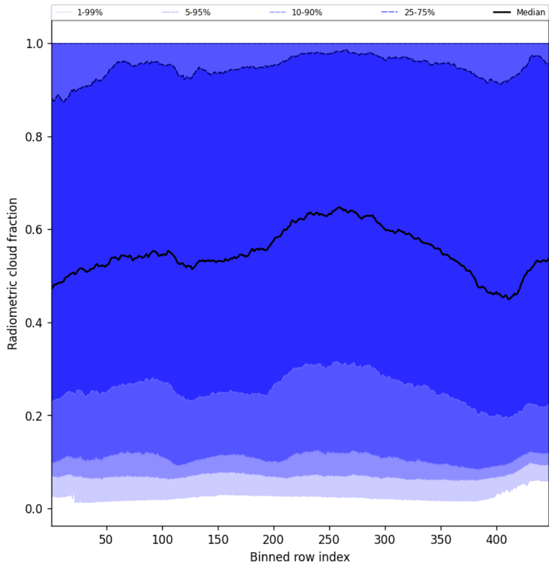
Figure 55: Along track statistics of “Radiometric cloud fraction” for 2025-01-23 to 2025-01-25
