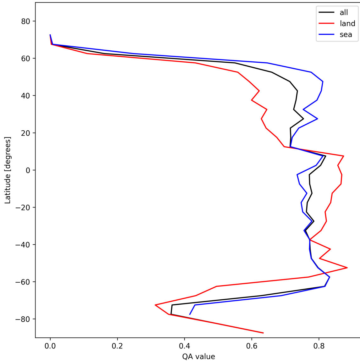
Figure 22: Zonal average of “QA value” for 2025-01-23 to 2025-01-25.
