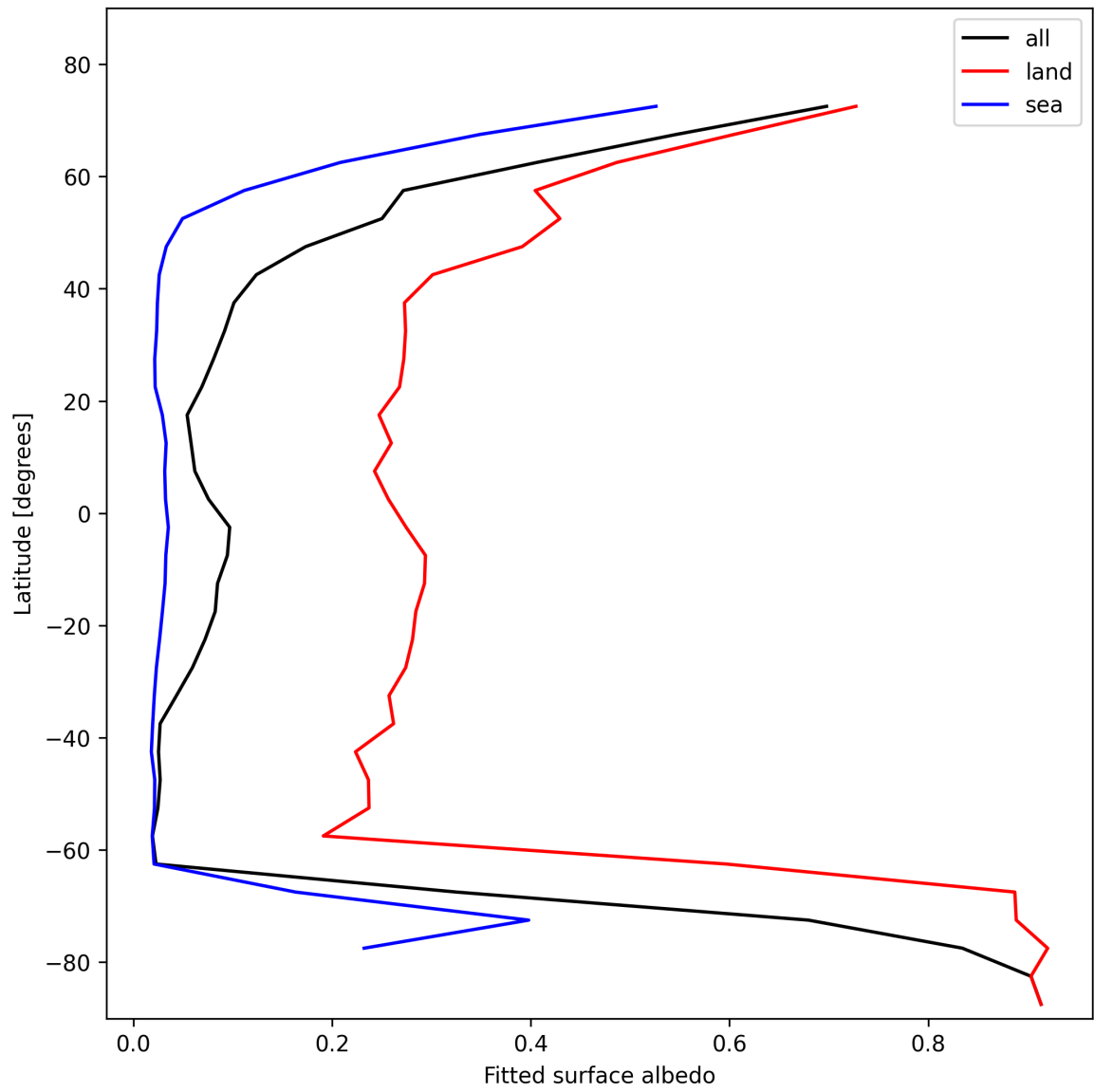
Figure 29: Zonal average of “Fitted surface albedo” for 2025-01-23 to 2025-01-25.
