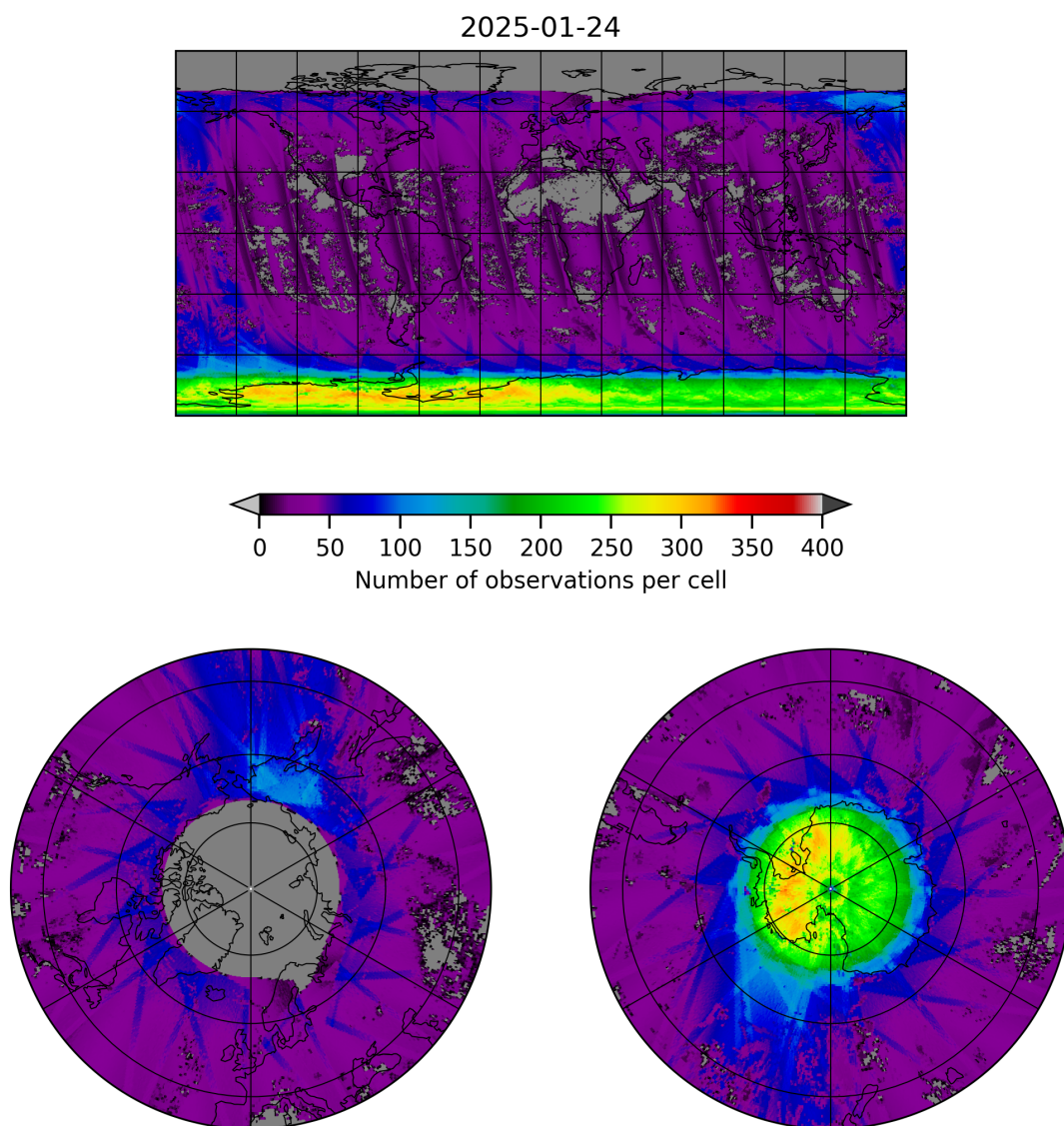
Figure 21: Map of the number of observations for 2025-01-23 to 2025-01-25
