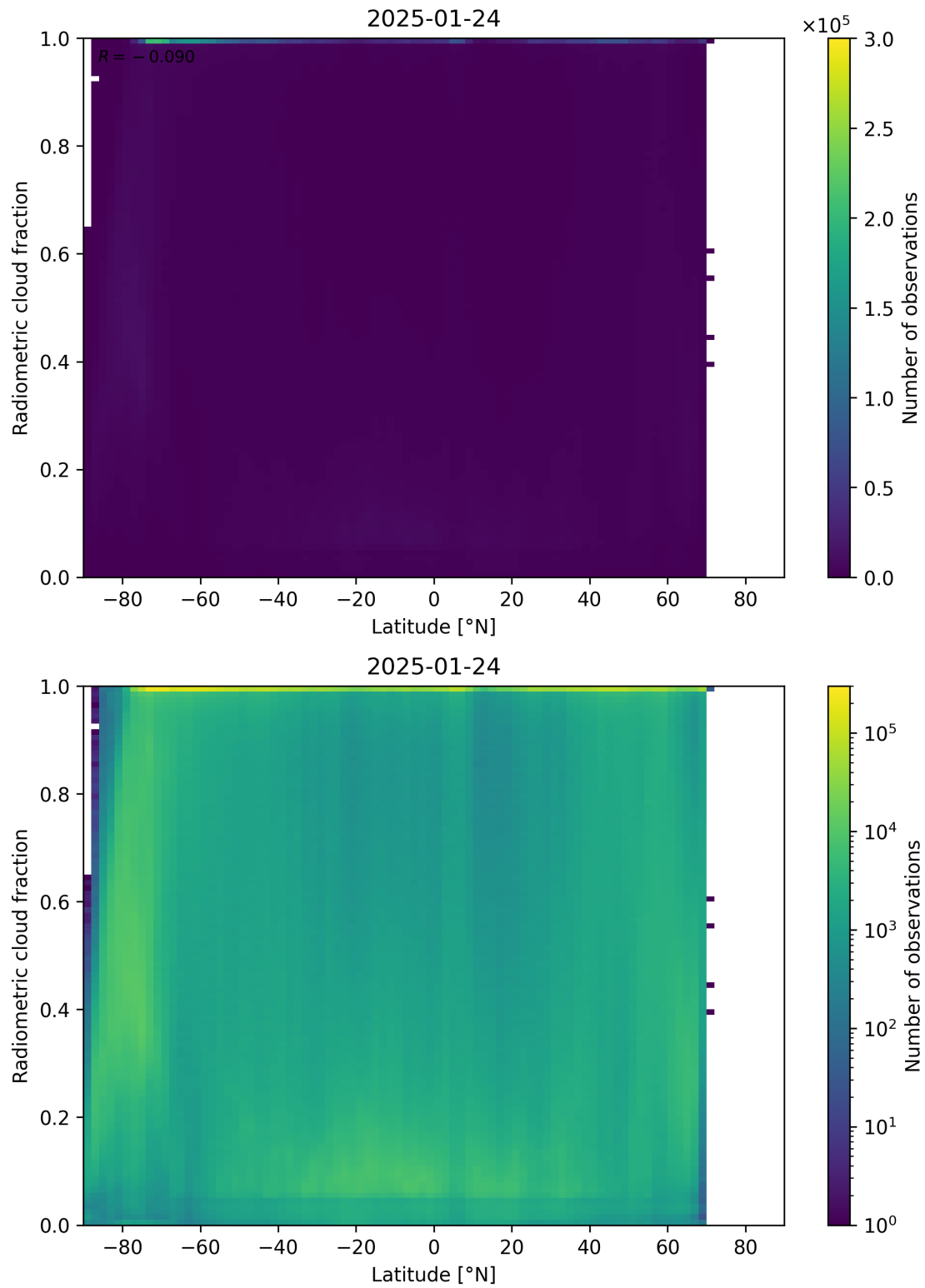
Figure 92: Scatter density plot of “Latitude” against “Radiometric cloud fraction” for 2025-01-23 to 2025-01-25.
