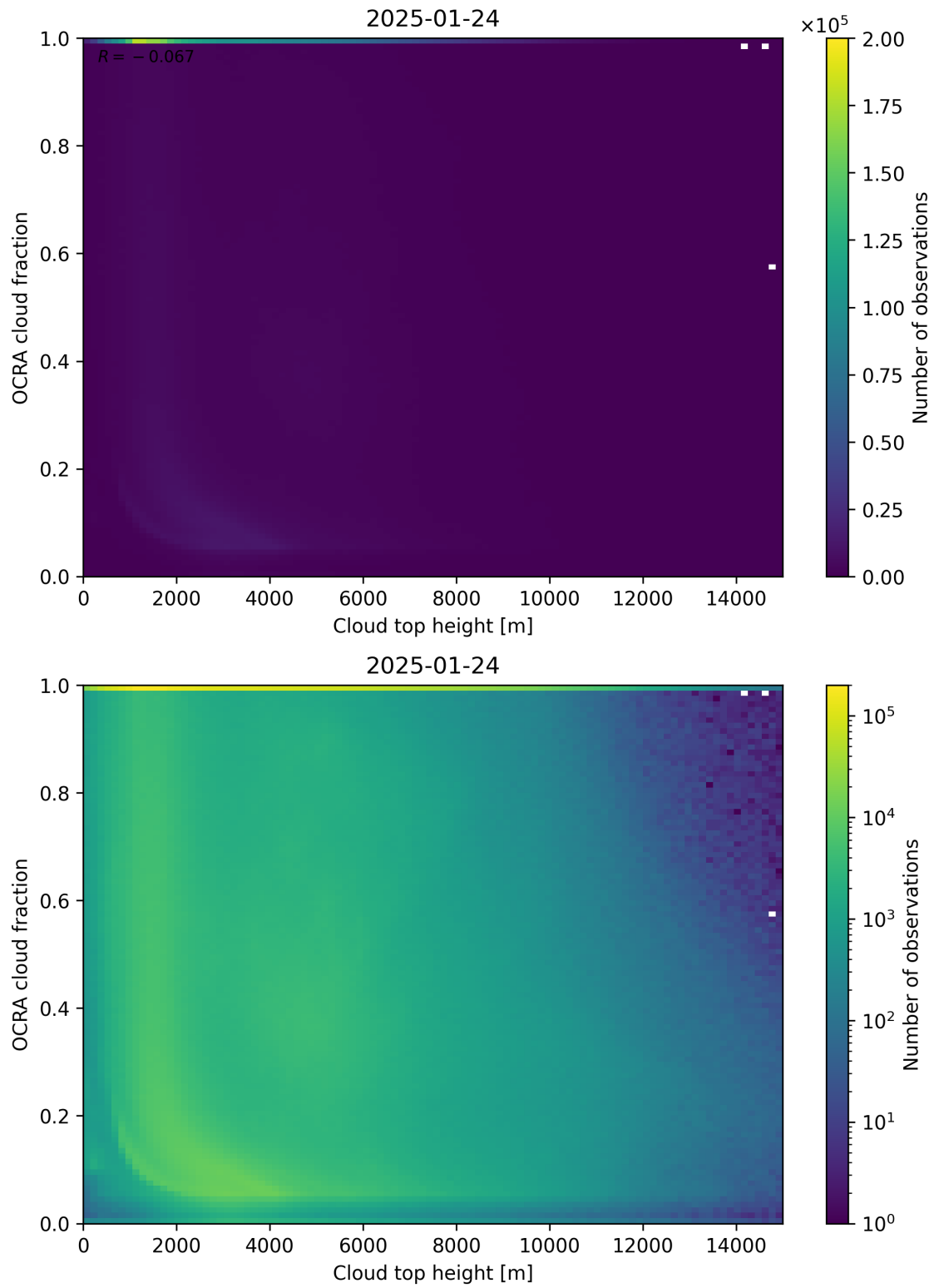
Figure 87: Scatter density plot of “Cloud top height” against “OCRA cloud fraction” for 2025-01-23 to 2025-01-25.
