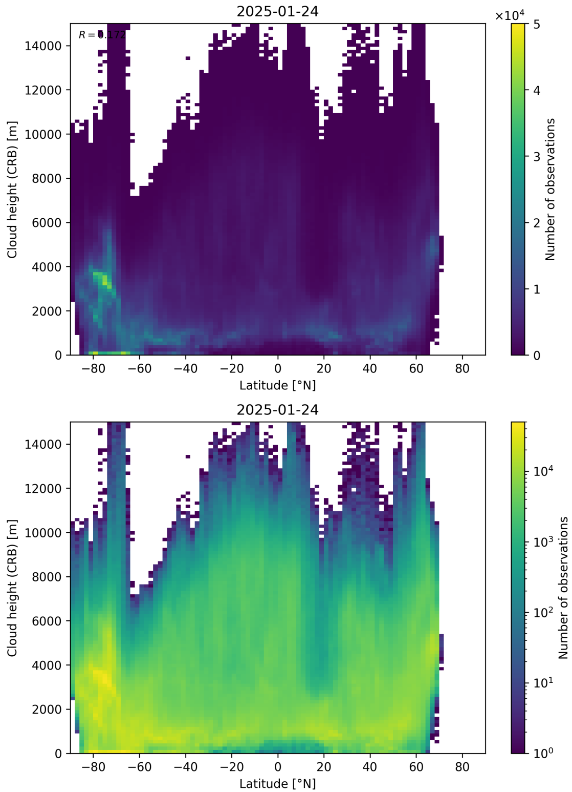
Figure 95: Scatter density plot of “Latitude” against “Cloud height (CRB)” for 2025-01-23 to 2025-01-25.
