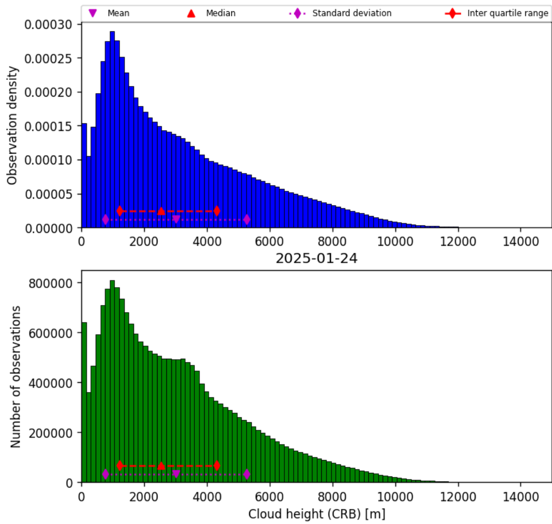
Figure 43: Histogram of “Cloud height (CRB)” for 2025-01-23 to 2025-01-25
