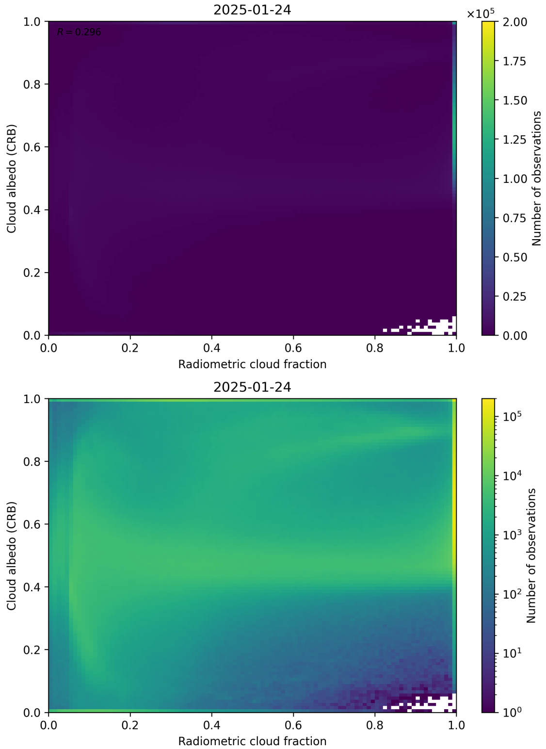
Figure 71: Scatter density plot of “Radiometric cloud fraction” against “Cloud albedo (CRB)” for 2025-01-23 to 2025-01-25.
