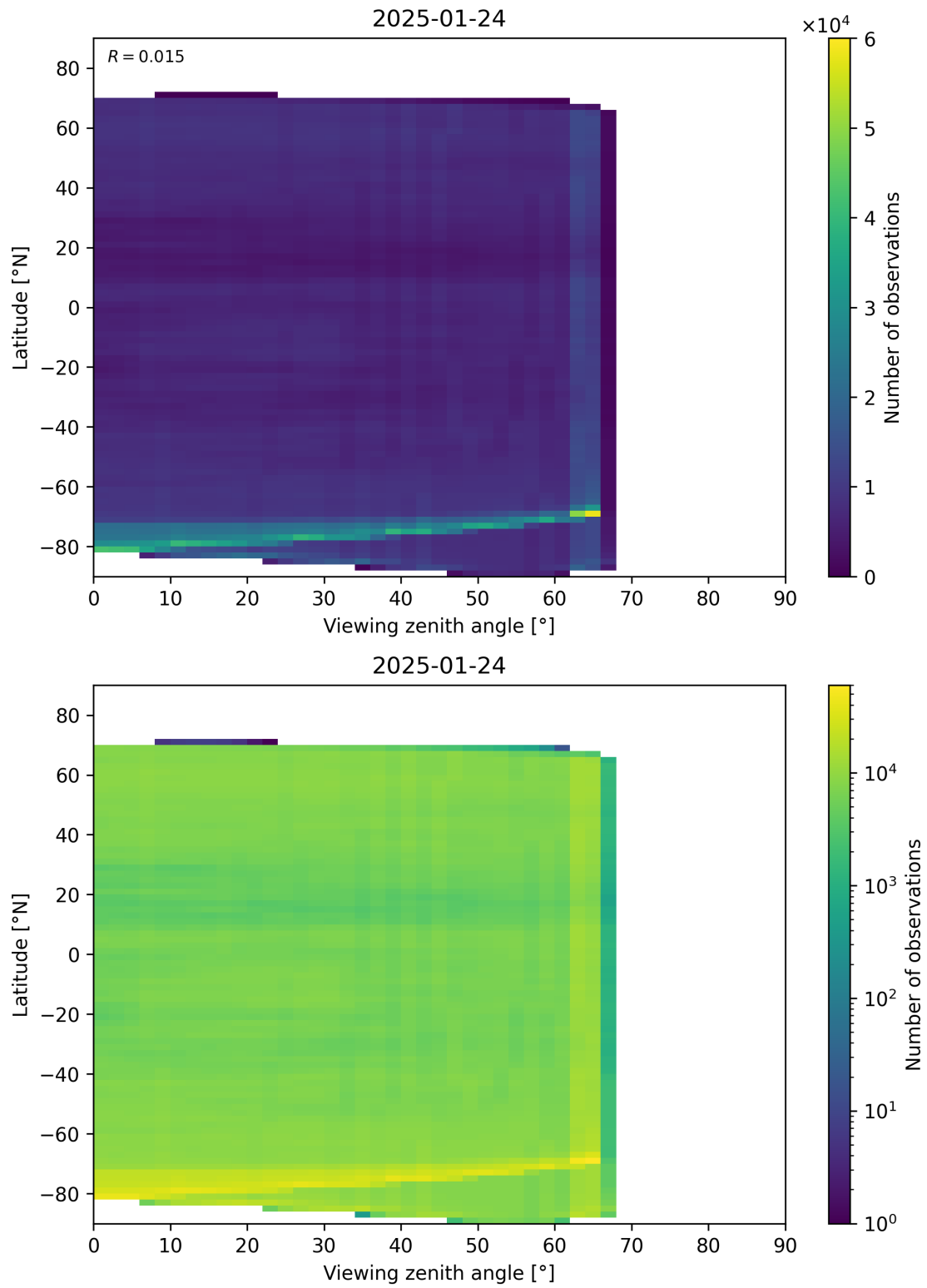
Figure 113: Scatter density plot of “Viewing zenith angle” against “Latitude” for 2025-01-23 to 2025-01-25.
