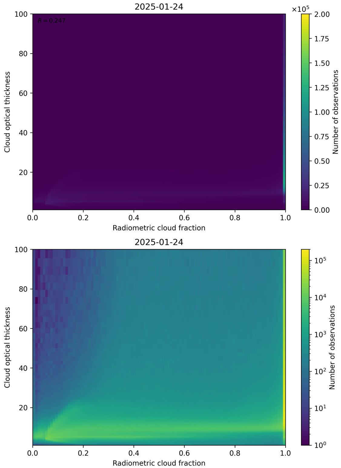
Figure 75: Scatter density plot of “Radiometric cloud fraction” against “Cloud optical thickness” for 2025-01-23 to 2025-01-25.
