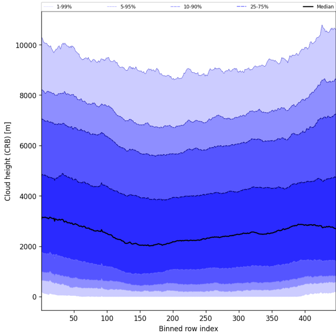
Figure 59: Along track statistics of “Cloud height (CRB)” for 2025-01-23 to 2025-01-25
