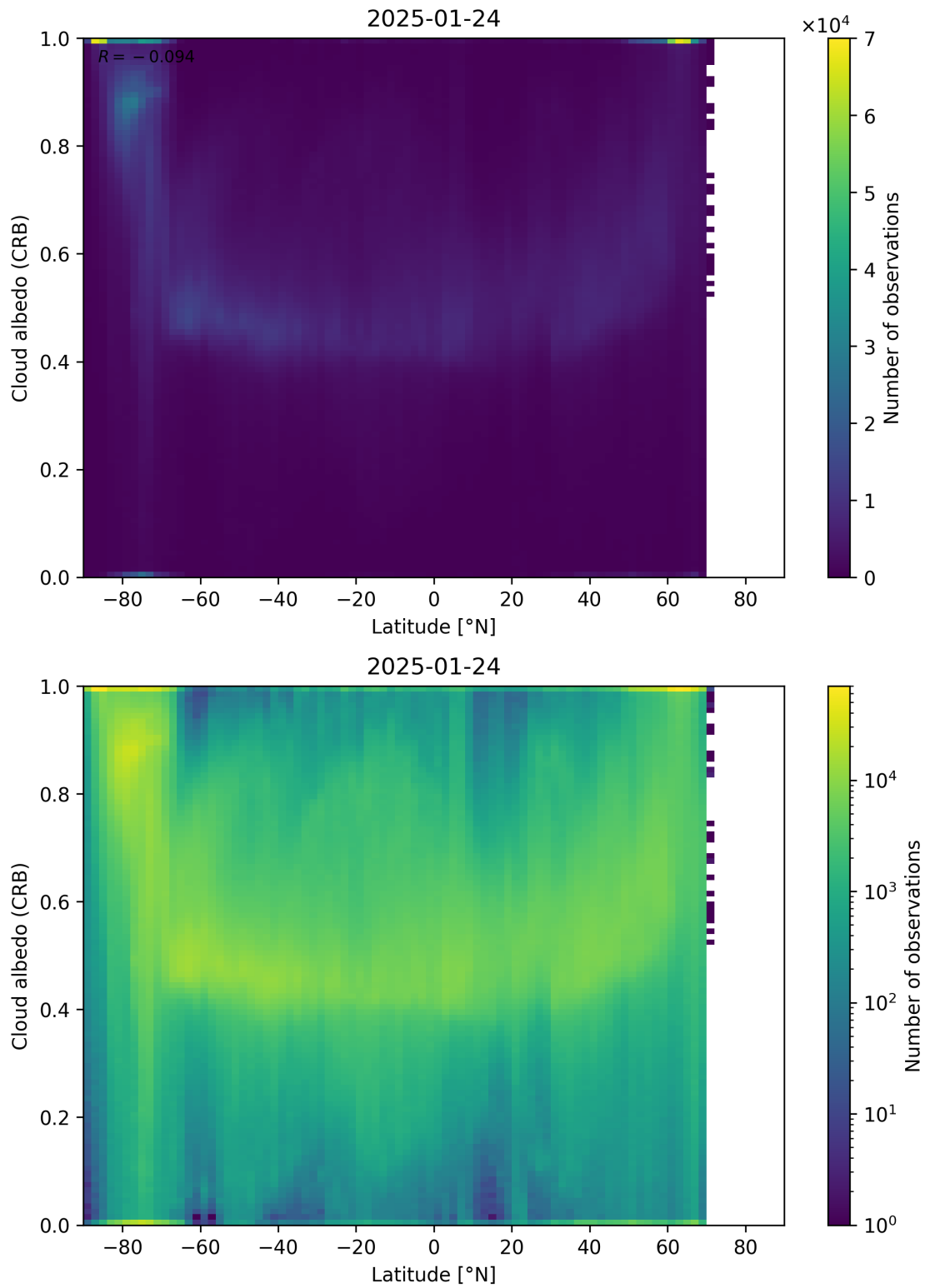
Figure 91: Scatter density plot of “Latitude” against “Cloud albedo (CRB)” for 2025-01-23 to 2025-01-25.
