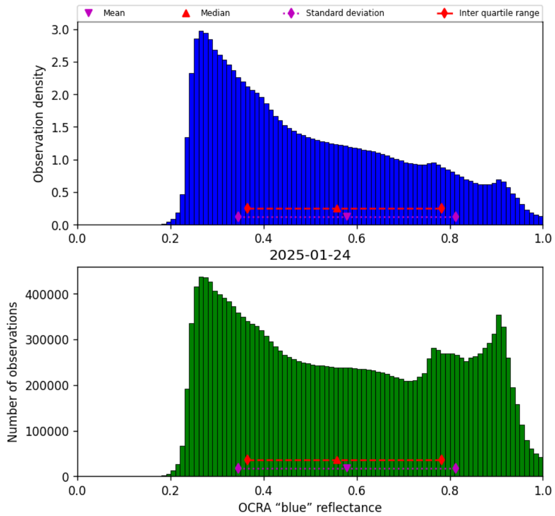
Figure 51: Histogram of “OCRA “blue” reflectance” for 2025-01-23 to 2025-01-25
