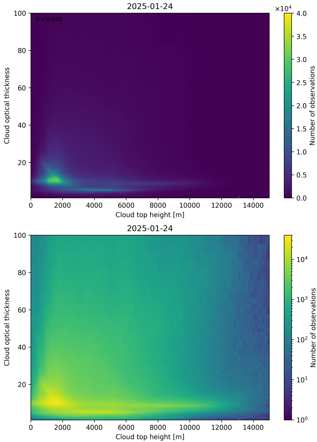
Figure 90: Scatter density plot of “Cloud top height” against “Cloud optical thickness” for 2025-01-23 to 2025-01-25.
