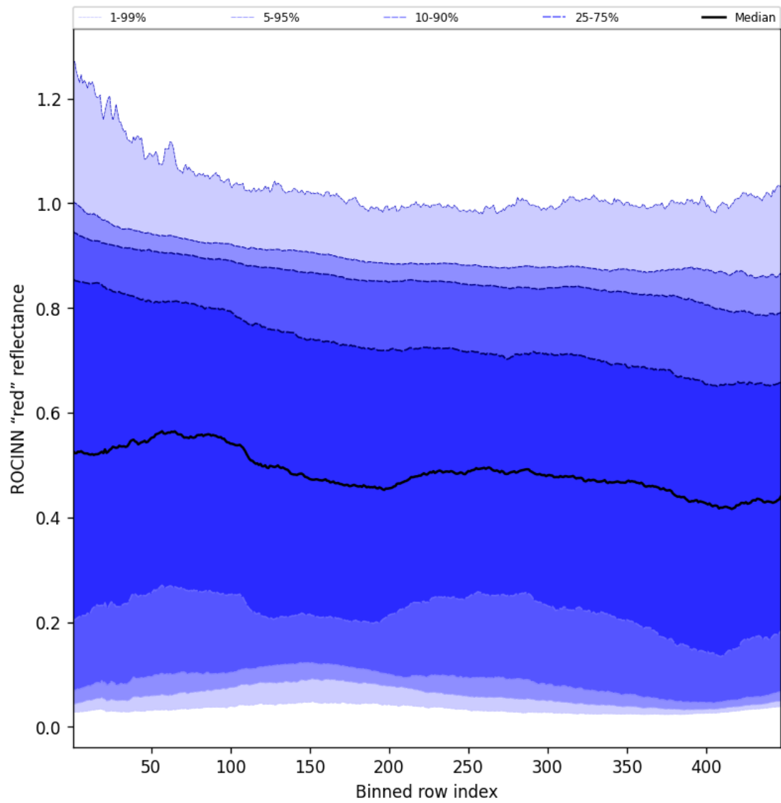
Figure 69: Along track statistics of “ROCINN “red” reflectance” for 2025-01-23 to 2025-01-25
