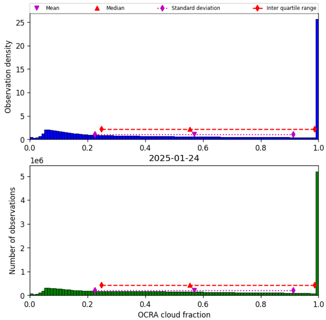
Figure 50: Histogram of “OCRA cloud fraction” for 2025-01-23 to 2025-01-25
