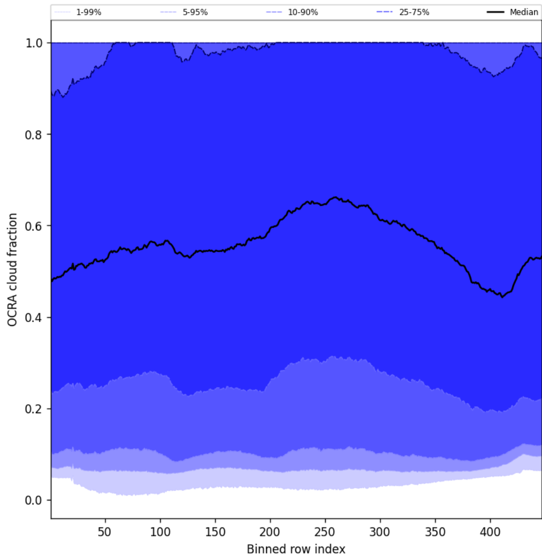
Figure 66: Along track statistics of “OCRA cloud fraction” for 2025-01-23 to 2025-01-25
