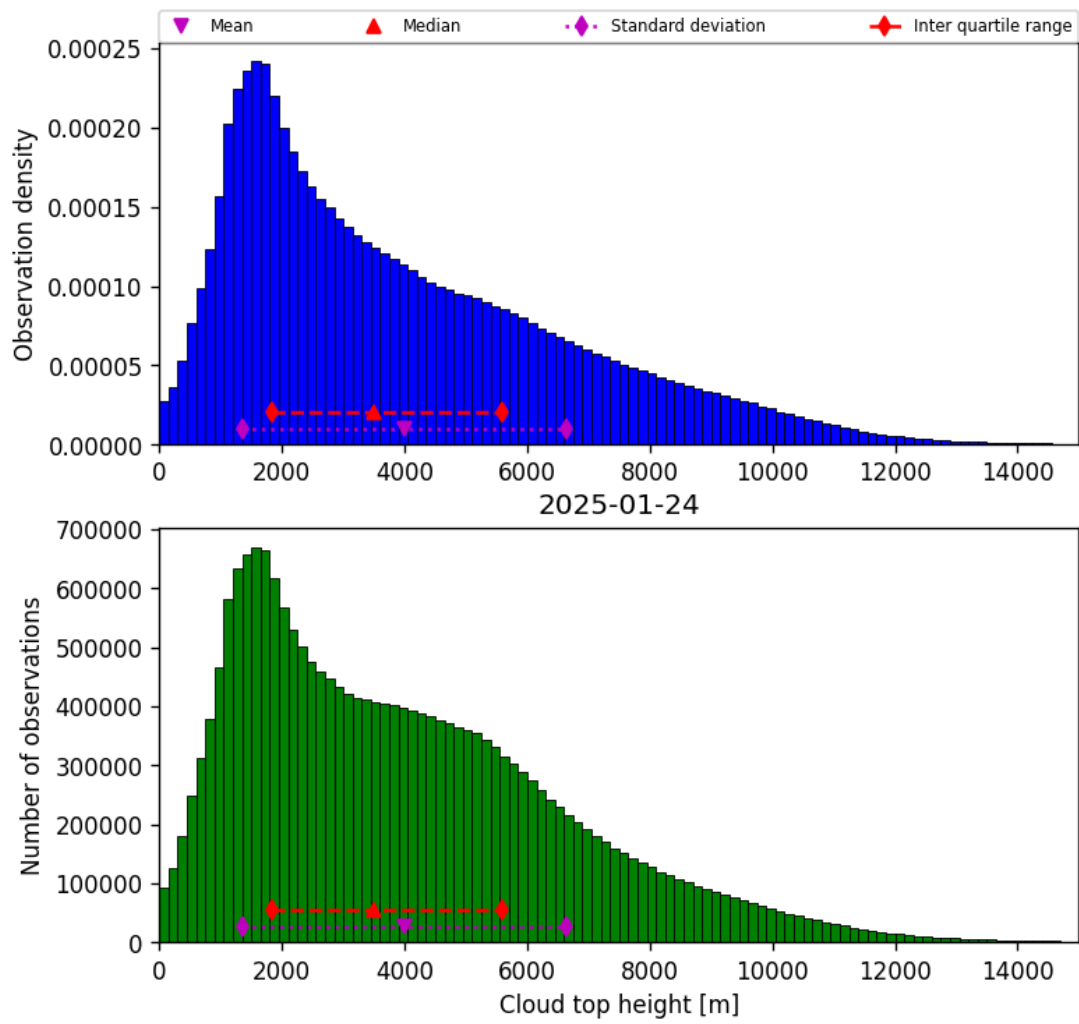
Figure 40: Histogram of “Cloud top height” for 2025-01-23 to 2025-01-25
