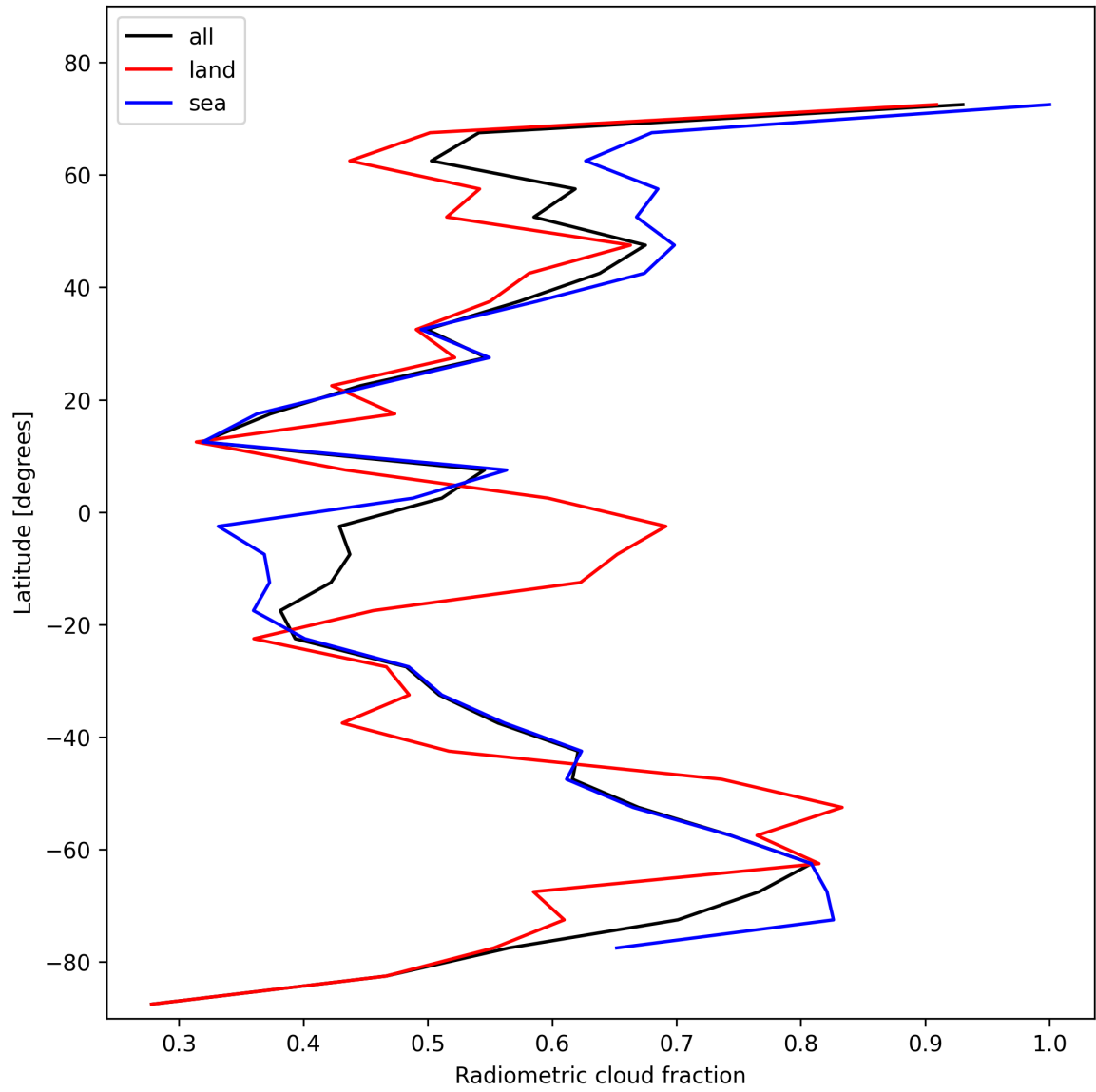
Figure 23: Zonal average of “Radiometric cloud fraction” for 2025-01-23 to 2025-01-25.
