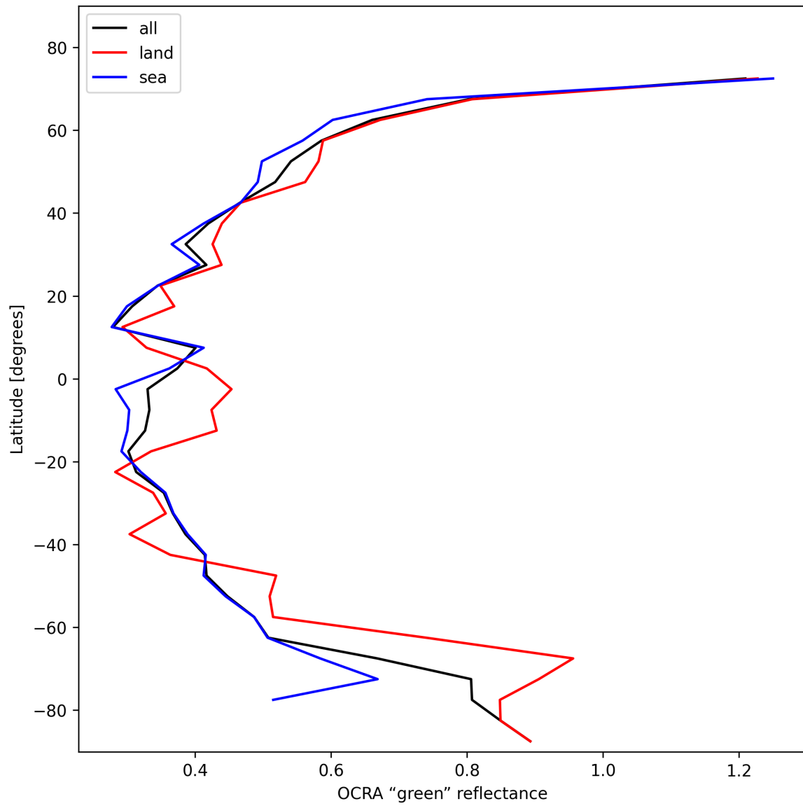
Figure 36: Zonal average of “OCRA “green” reflectance” for 2025-01-23 to 2025-01-25.
