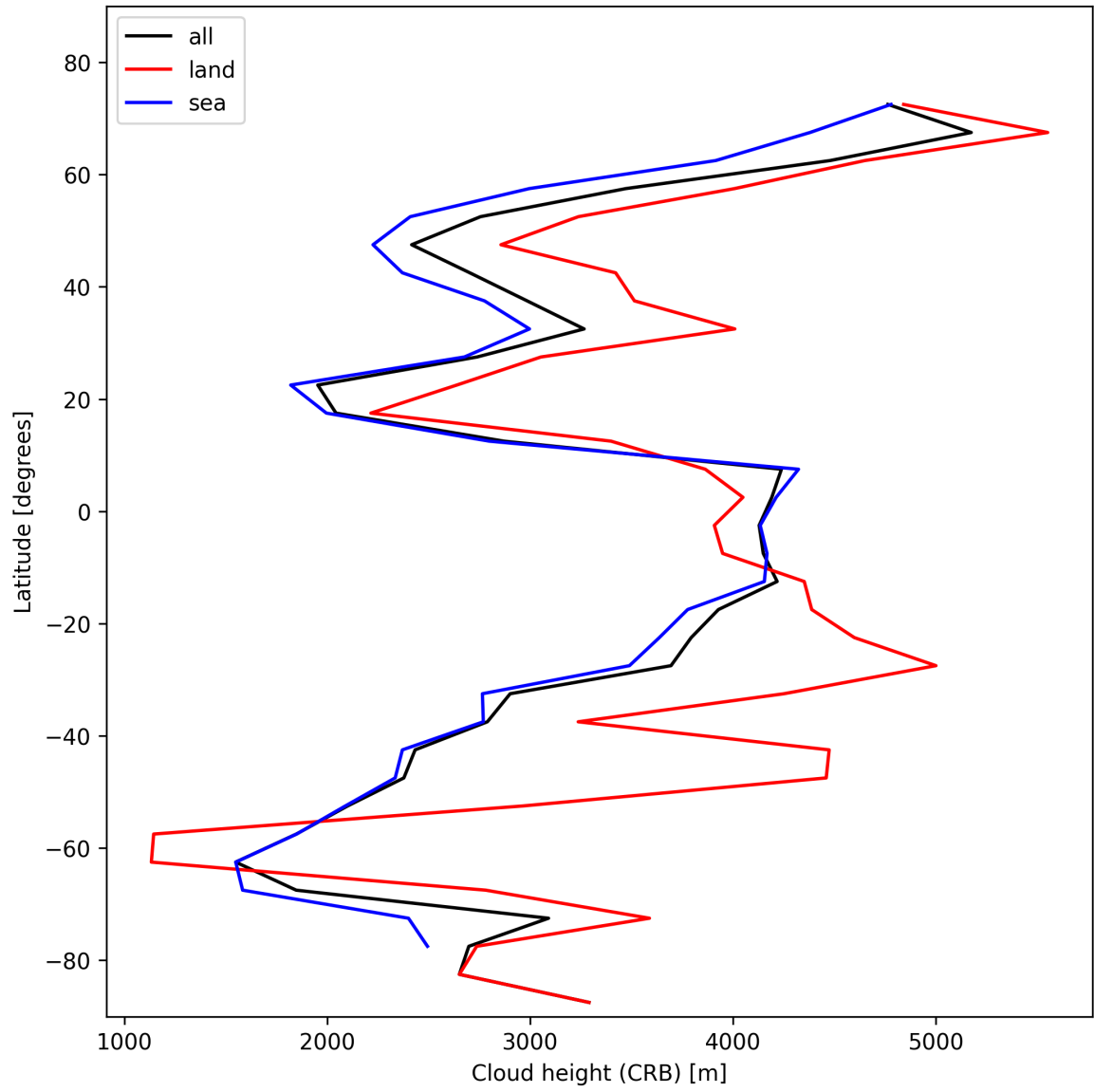
Figure 27: Zonal average of “Cloud height (CRB)” for 2025-01-23 to 2025-01-25.
