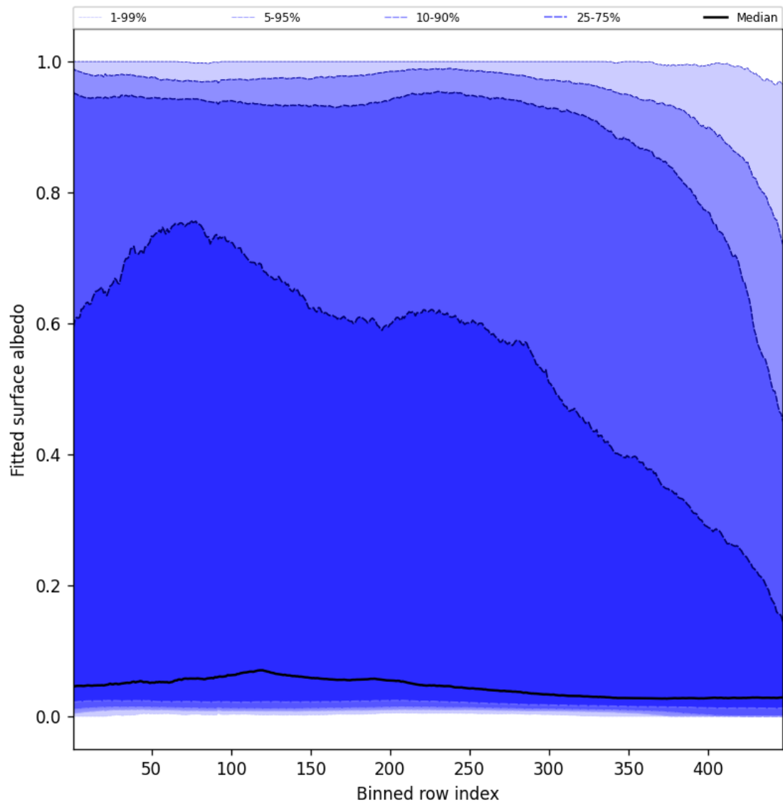
Figure 61: Along track statistics of “Fitted surface albedo” for 2025-01-23 to 2025-01-25
