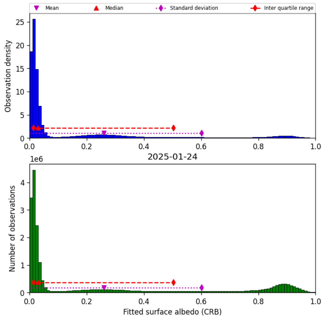
Figure 46: Histogram of “Fitted surface albedo (CRB)” for 2025-01-23 to 2025-01-25
