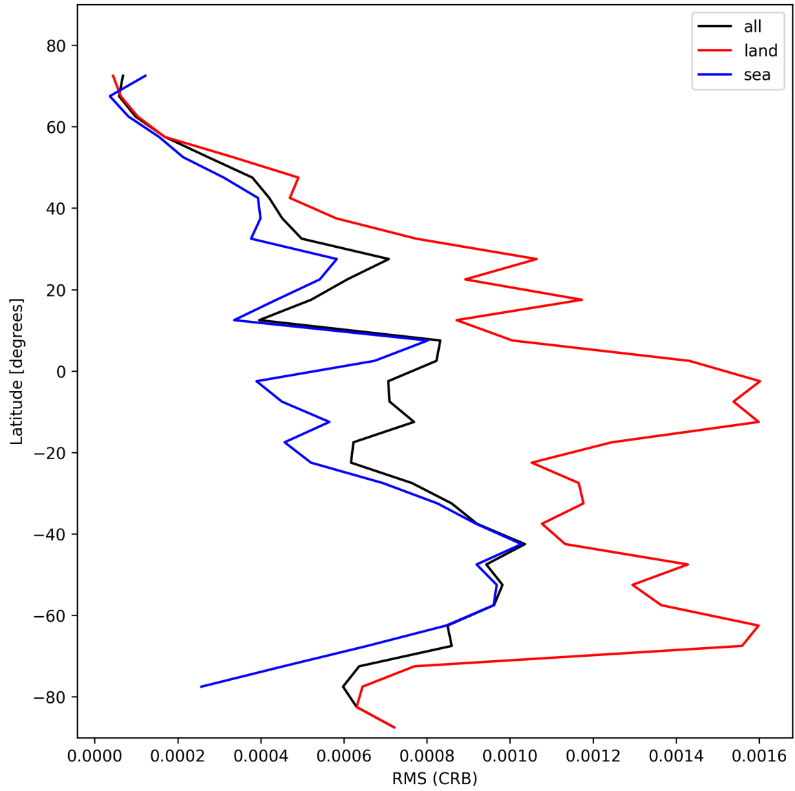
Figure 32: Zonal average of “RMS (CRB)” for 2025-01-23 to 2025-01-25.
