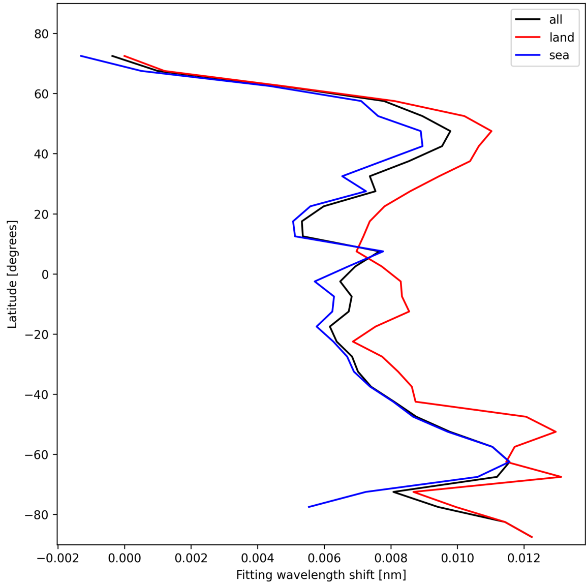
Figure 33: Zonal average of “Fitting wavelength shift” for 2025-01-23 to 2025-01-25.
