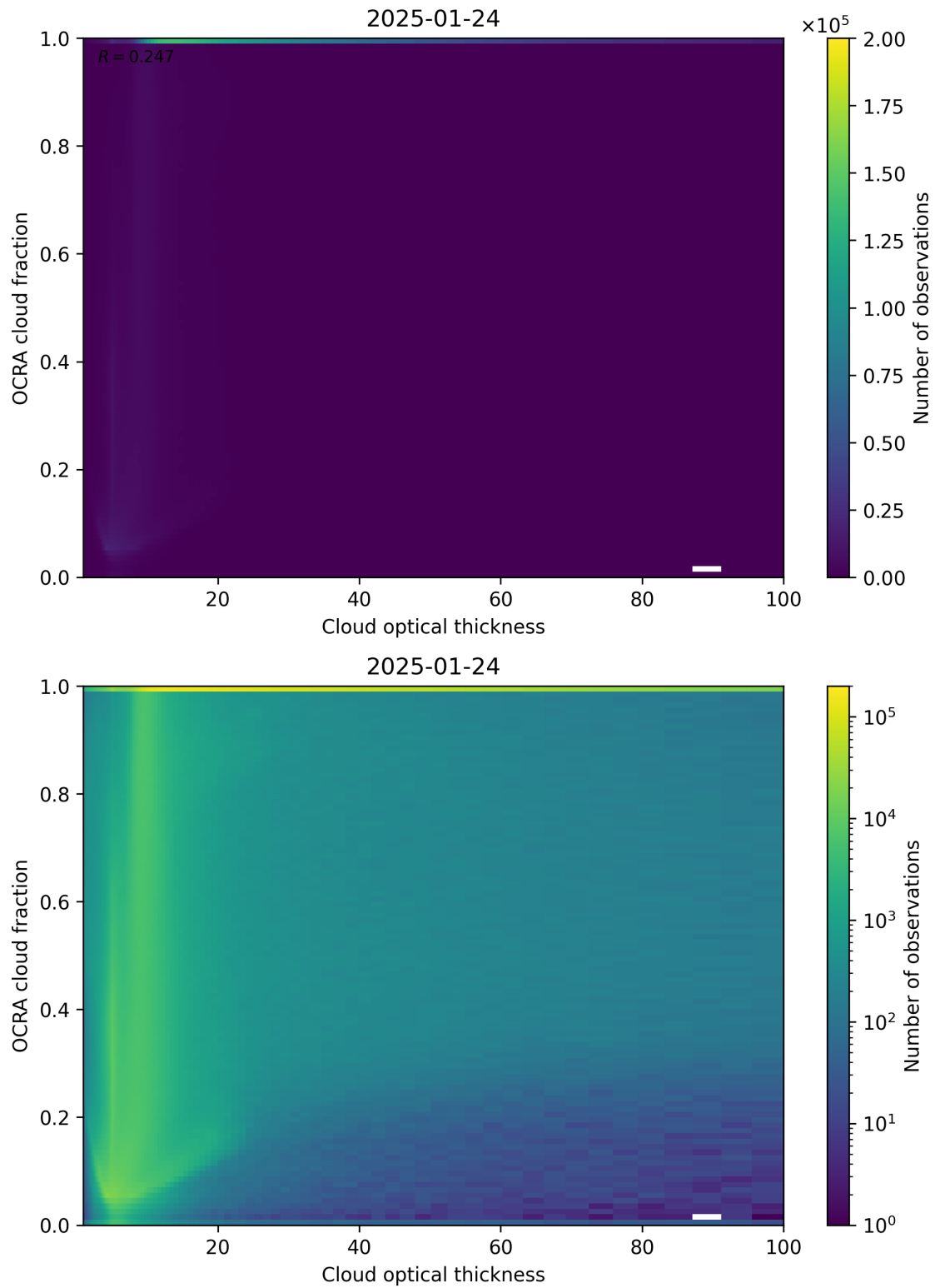
Figure 83: Scatter density plot of “Cloud optical thickness” against “OCRA cloud fraction” for 2025-01-23 to 2025-01-25.
