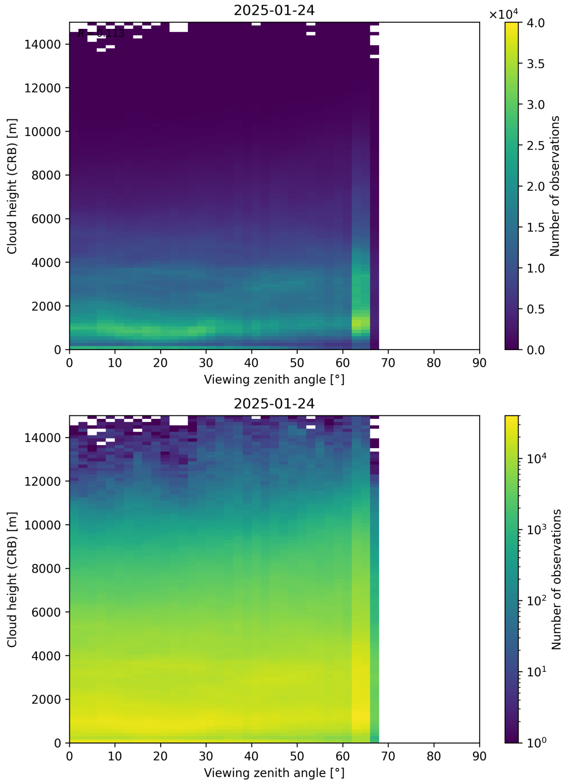
Figure 110: Scatter density plot of “Viewing zenith angle” against “Cloud height (CRB)” for 2025-01-23 to 2025-01-25.
