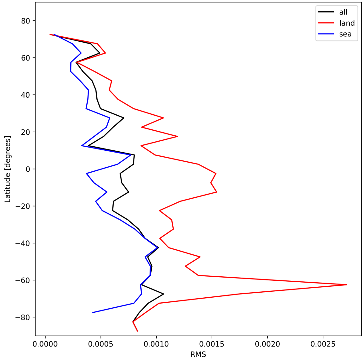
Figure 31: Zonal average of “RMS” for 2025-01-23 to 2025-01-25.
