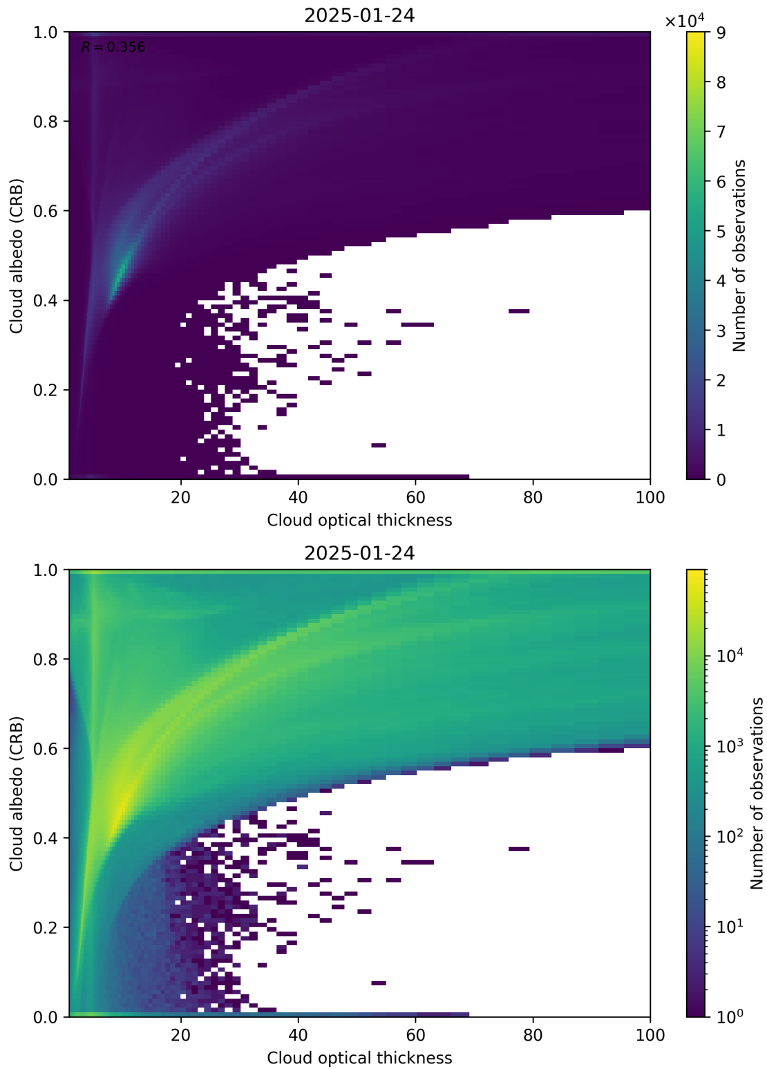
Figure 82: Scatter density plot of “Cloud optical thickness” against “Cloud albedo (CRB)” for 2025-01-23 to 2025-01-25.
