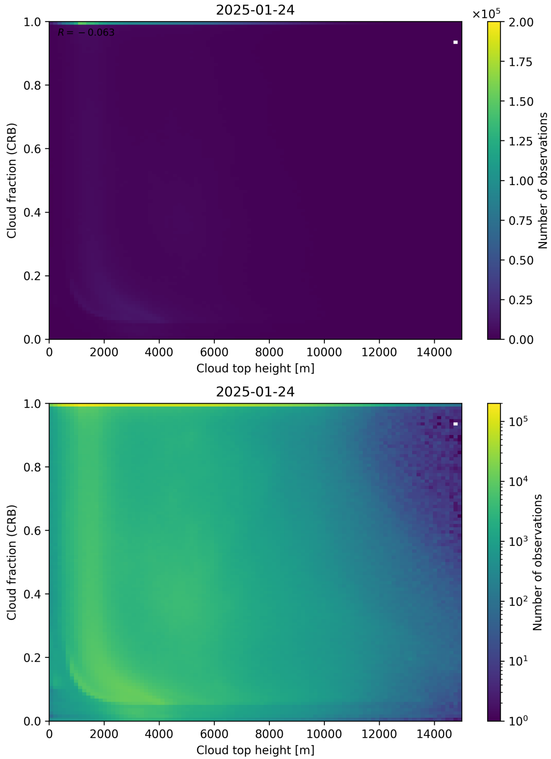
Figure 88: Scatter density plot of “Cloud top height” against “Cloud fraction (CRB)” for 2025-01-23 to 2025-01-25.
