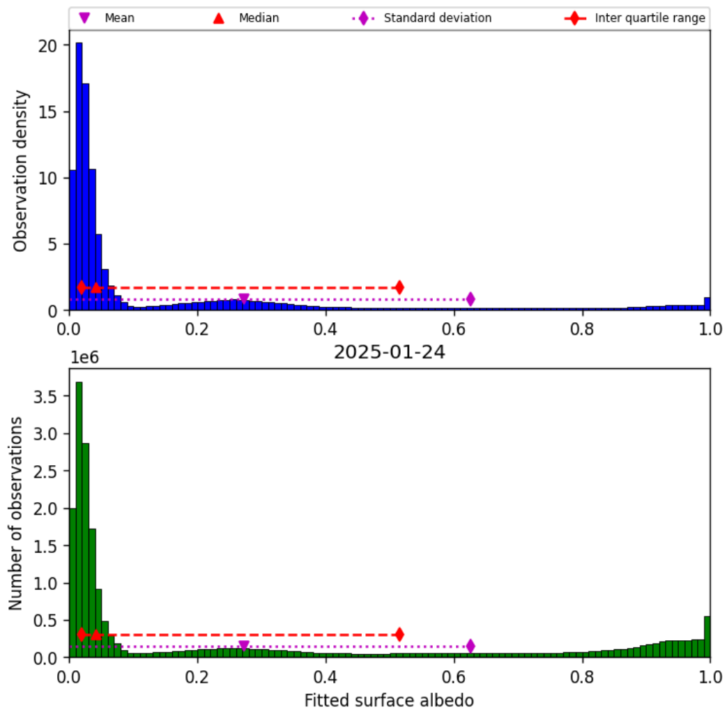
Figure 45: Histogram of “Fitted surface albedo” for 2025-01-23 to 2025-01-25
