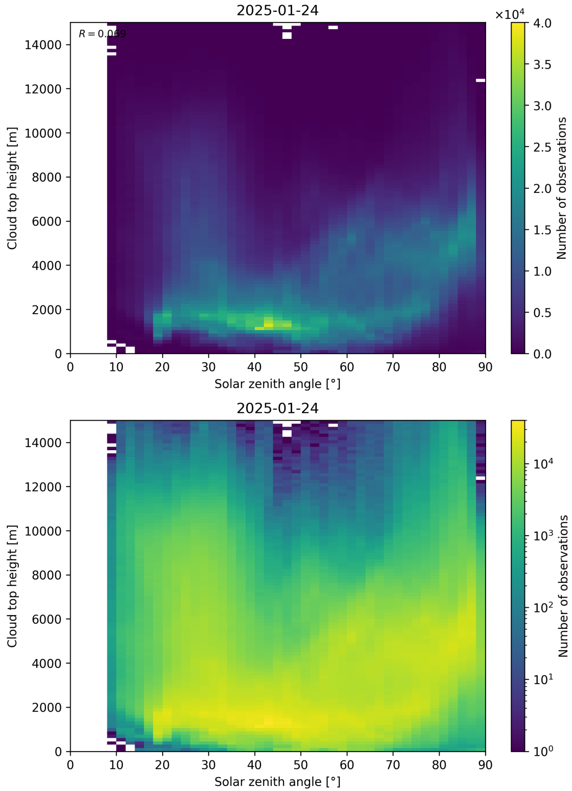
Figure 104: Scatter density plot of “Solar zenith angle” against “Cloud top height” for 2025-01-23 to 2025-01-25.
