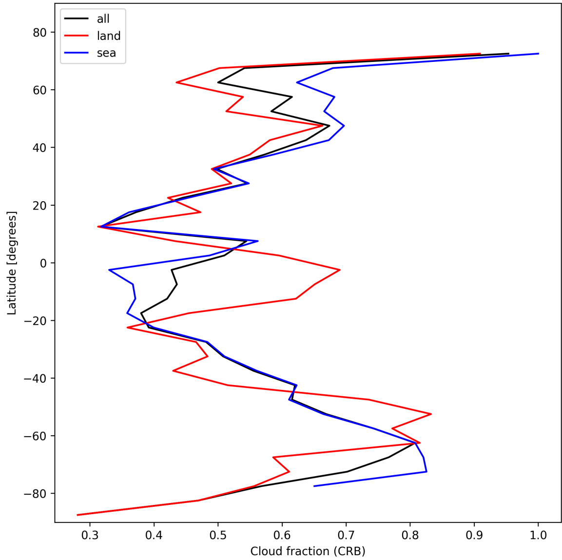
Figure 26: Zonal average of “Cloud fraction (CRB)” for 2025-01-23 to 2025-01-25.
