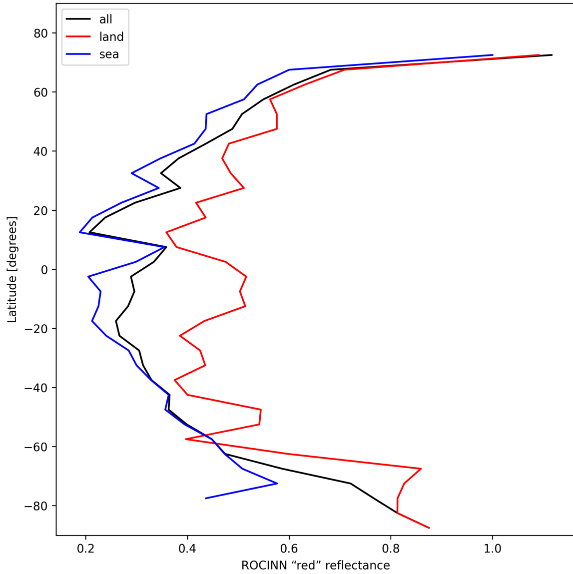
Figure 37: Zonal average of “ROCINN “red” reflectance” for 2025-01-23 to 2025-01-25.
