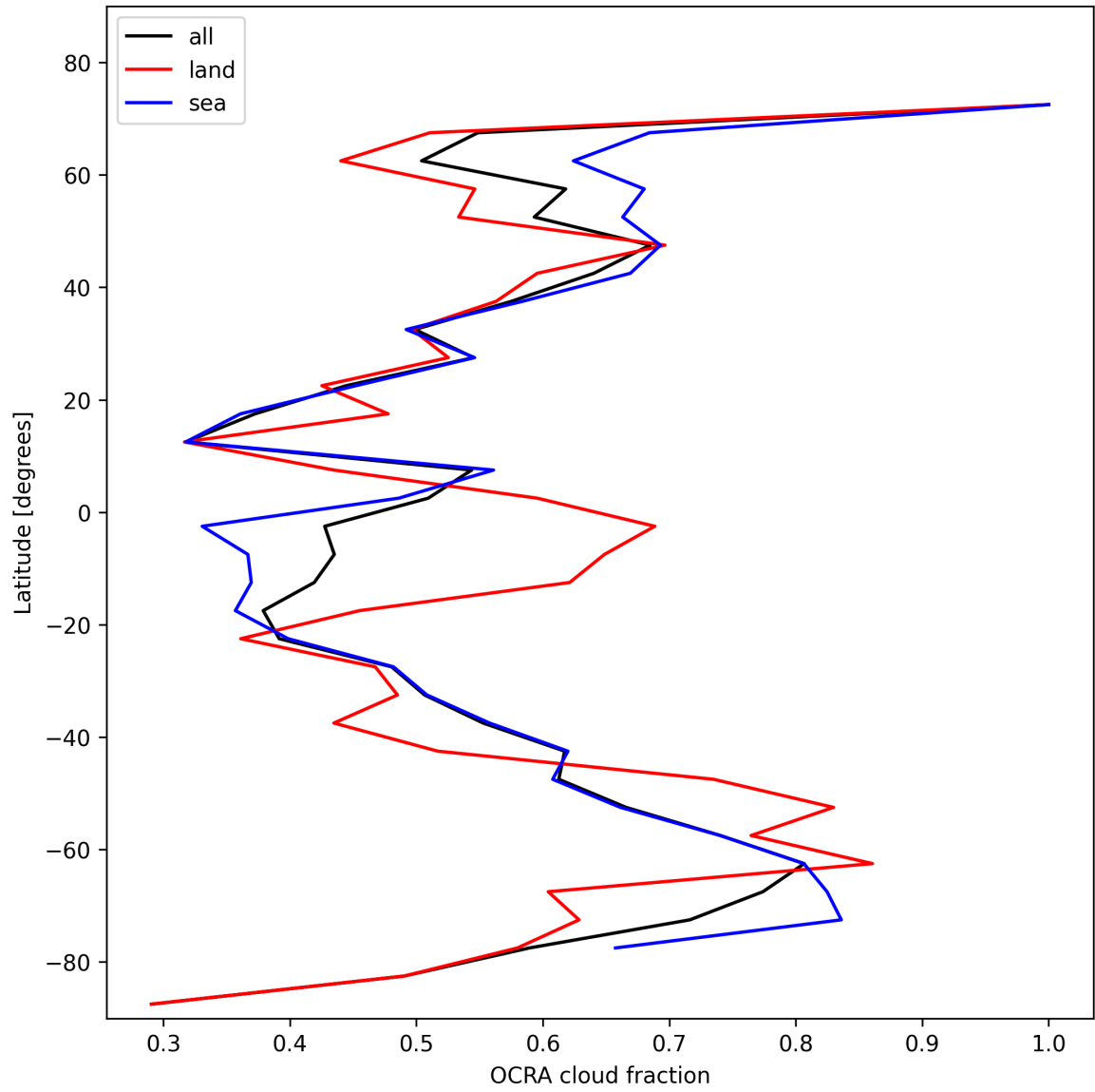
Figure 34: Zonal average of “OCRA cloud fraction” for 2025-01-23 to 2025-01-25.
