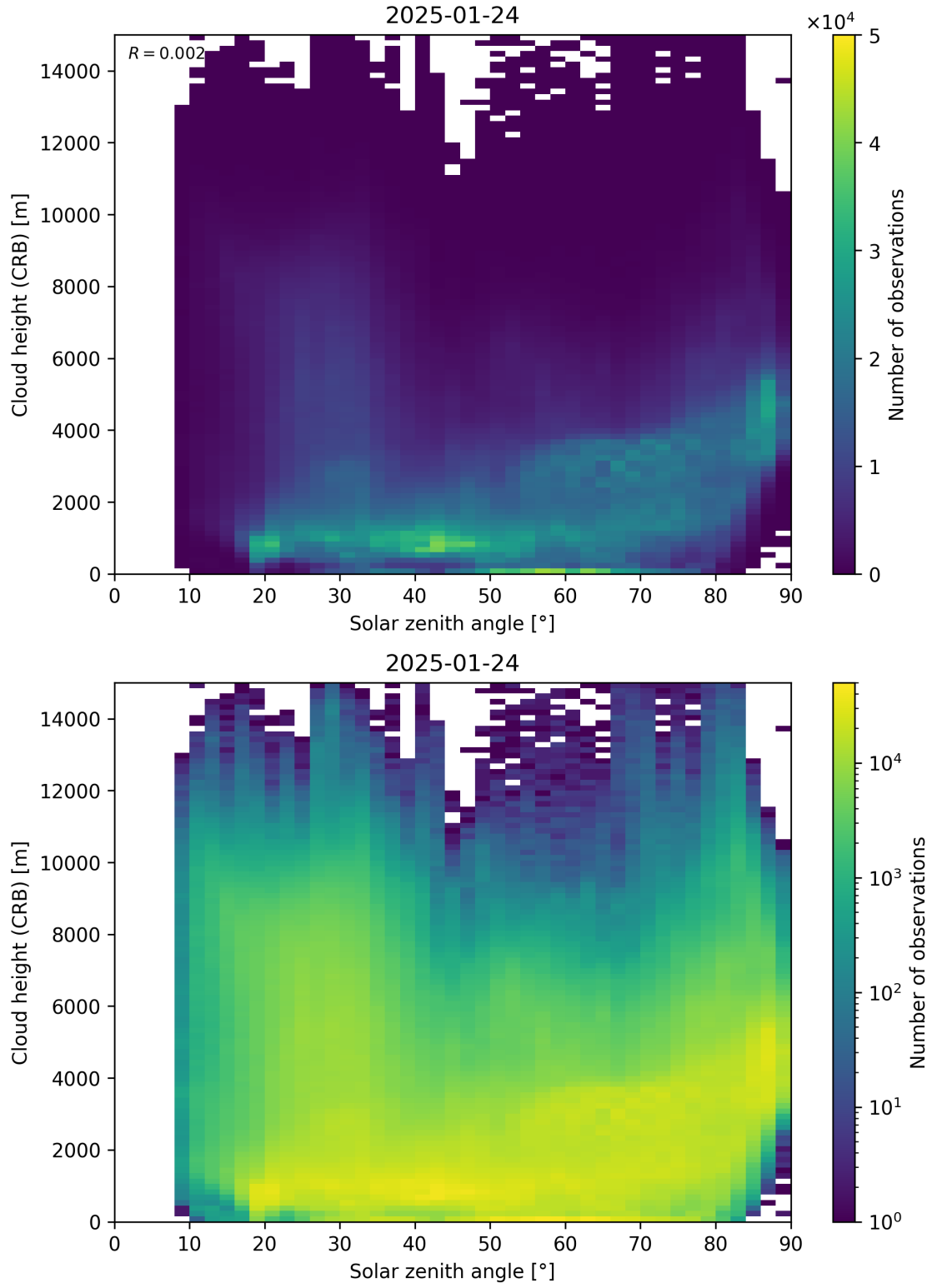
Figure 102: Scatter density plot of “Solar zenith angle” against “Cloud height (CRB)” for 2025-01-23 to 2025-01-25.
