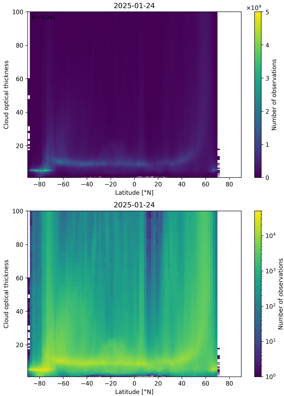
Figure 96: Scatter density plot of “Latitude” against “Cloud optical thickness” for 2025-01-23 to 2025-01-25.
