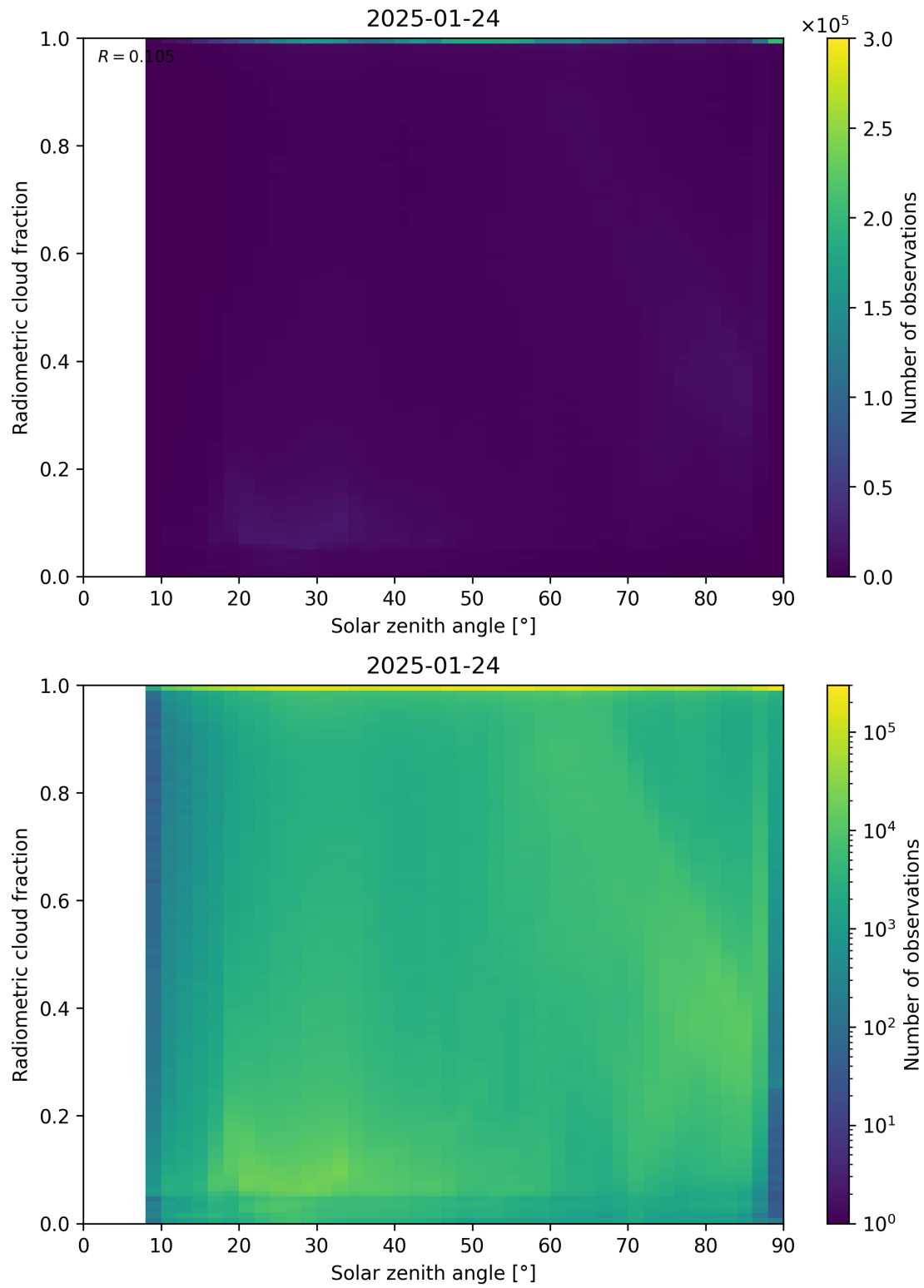
Figure 99: Scatter density plot of “Solar zenith angle” against “Radiometric cloud fraction” for 2025-01-23 to 2025-01-25.
