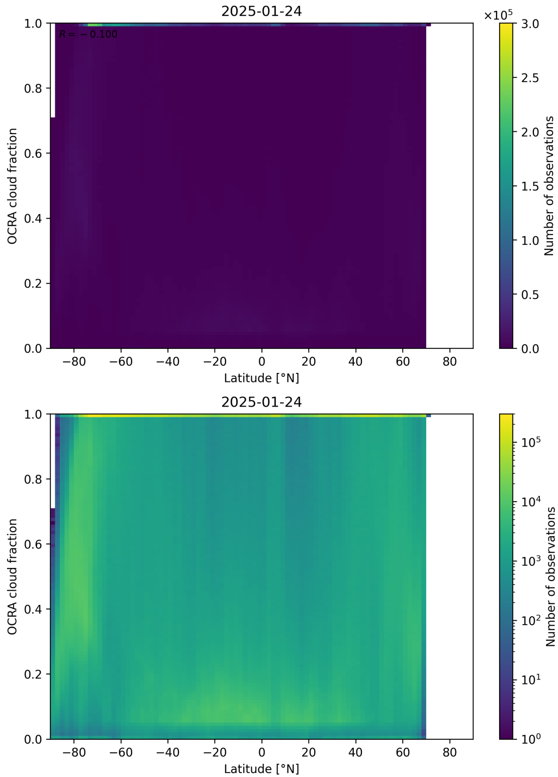
Figure 93: Scatter density plot of “Latitude” against “OCRA cloud fraction” for 2025-01-23 to 2025-01-25.
