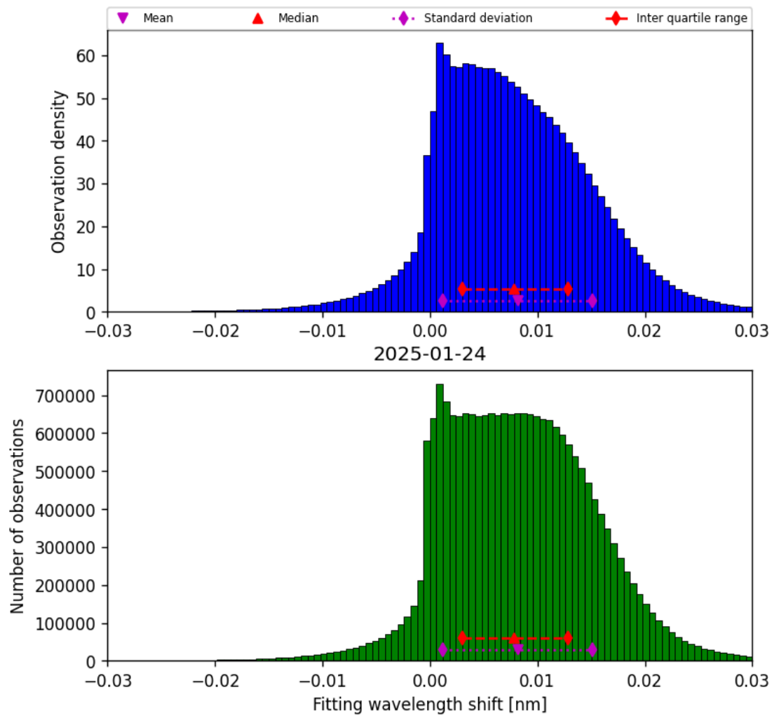
Figure 49: Histogram of “Fitting wavelength shift” for 2025-01-23 to 2025-01-25
