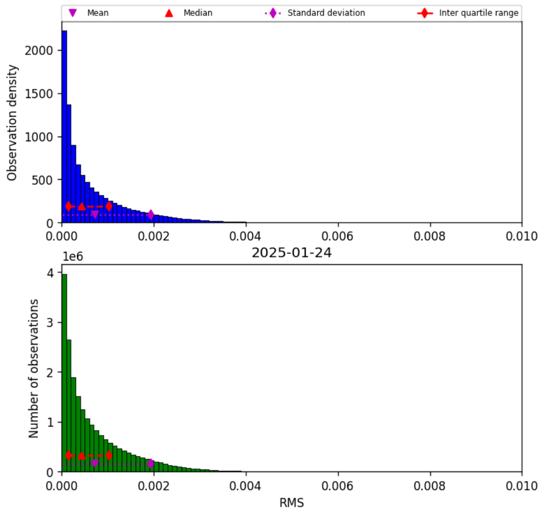
Figure 47: Histogram of “RMS” for 2025-01-23 to 2025-01-25
