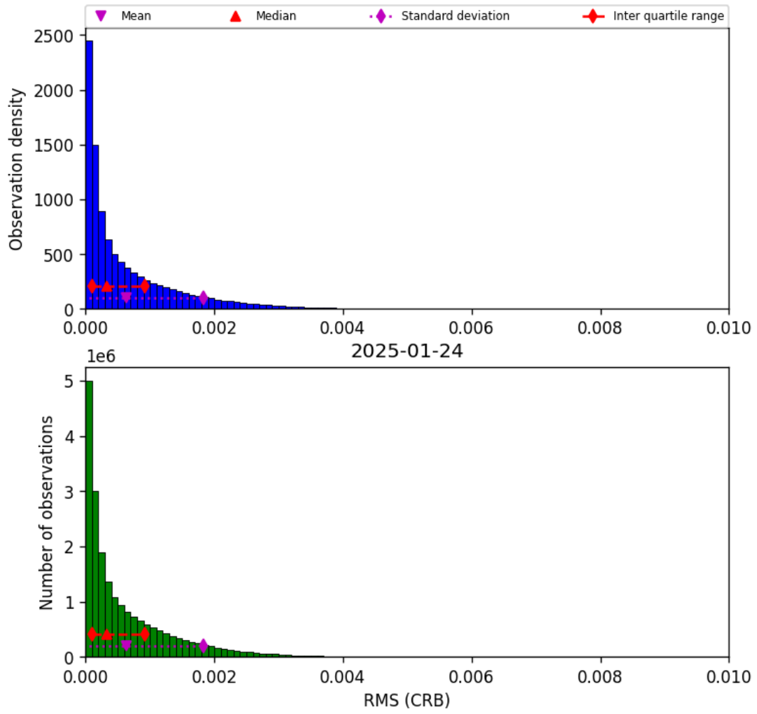
Figure 48: Histogram of “RMS (CRB)” for 2025-01-23 to 2025-01-25
