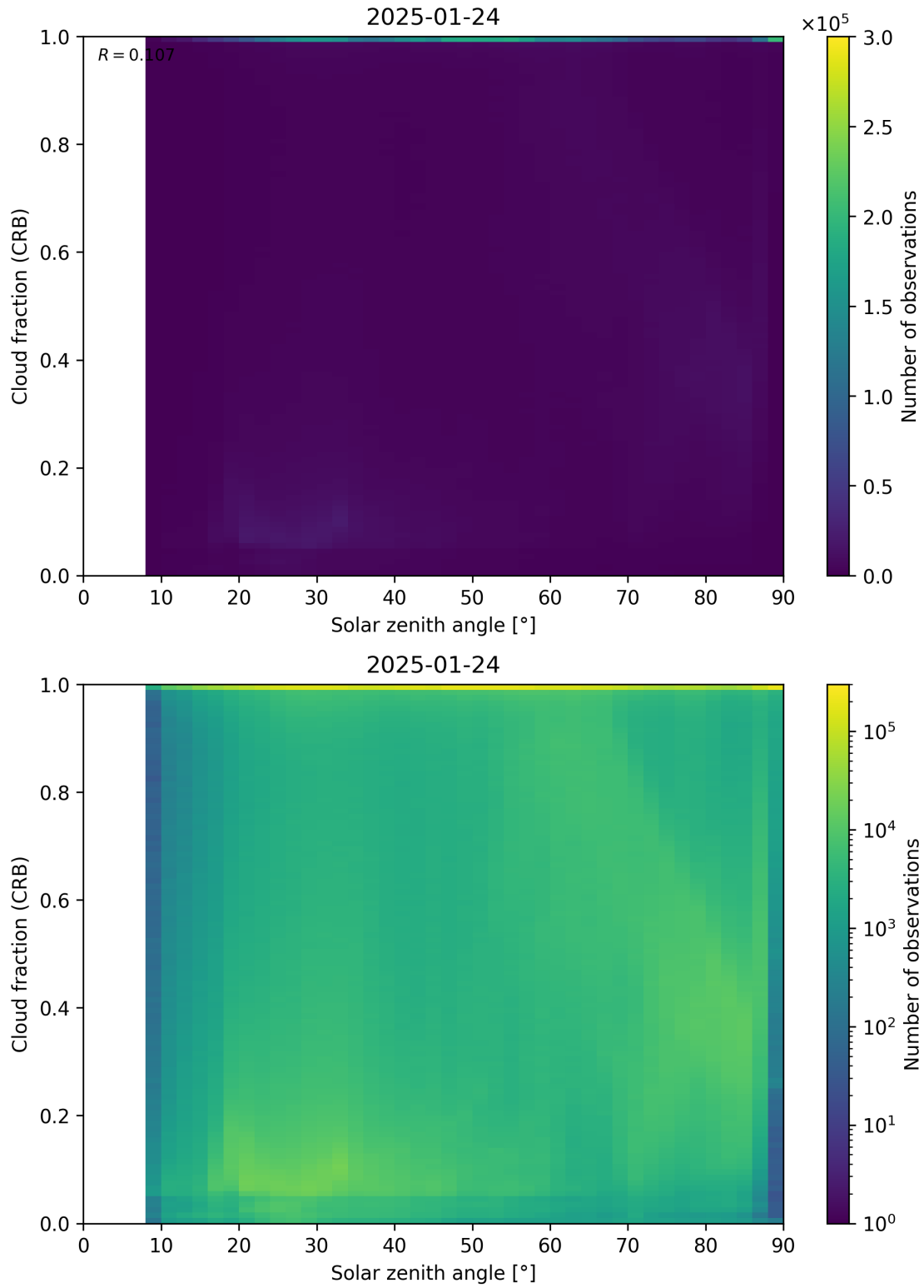
Figure 101: Scatter density plot of “Solar zenith angle” against “Cloud fraction (CRB)” for 2025-01-23 to 2025-01-25.
