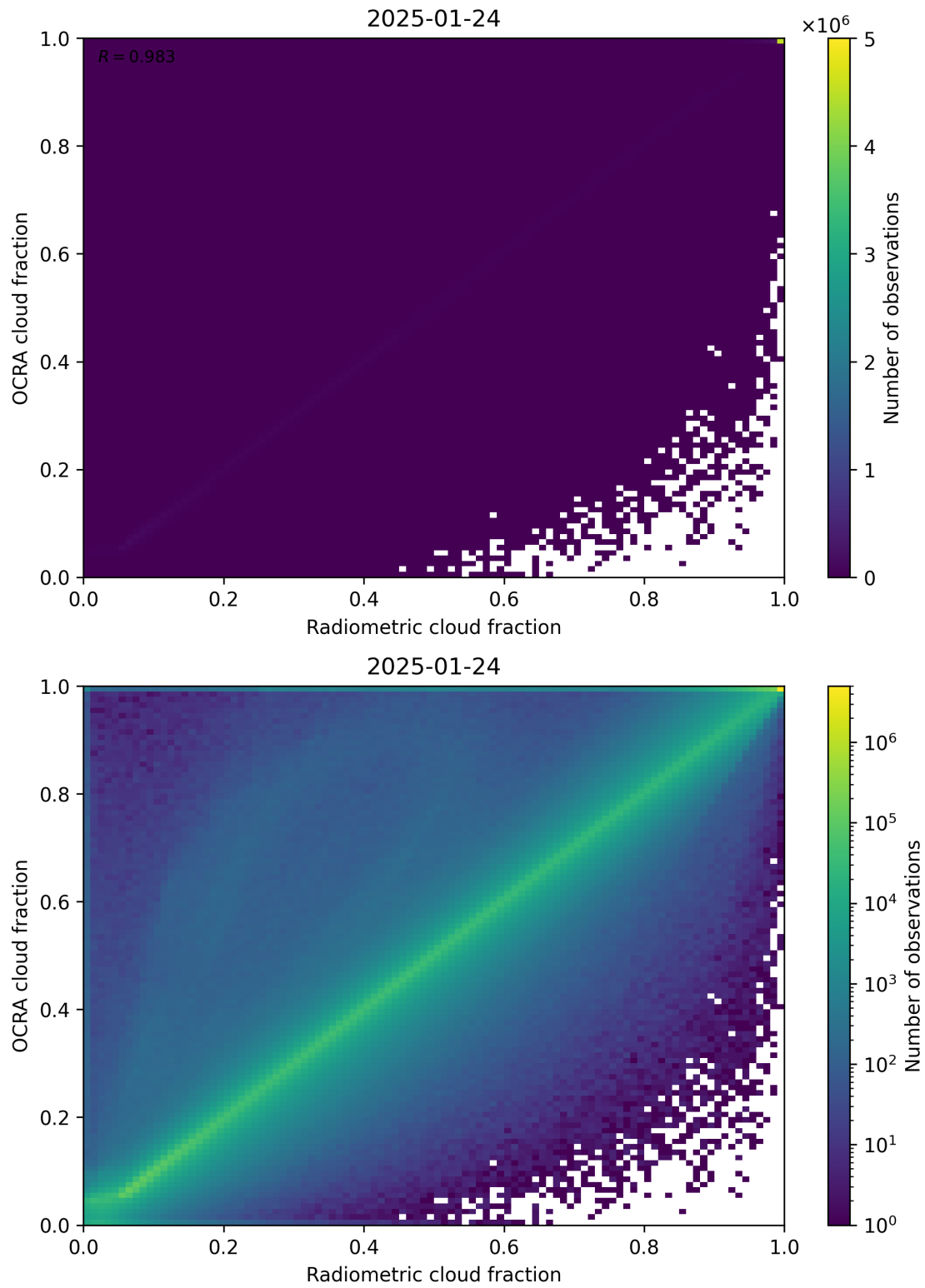
Figure 72: Scatter density plot of “Radiometric cloud fraction” against “OCRA cloud fraction” for 2025-01-23 to 2025-01-25.
