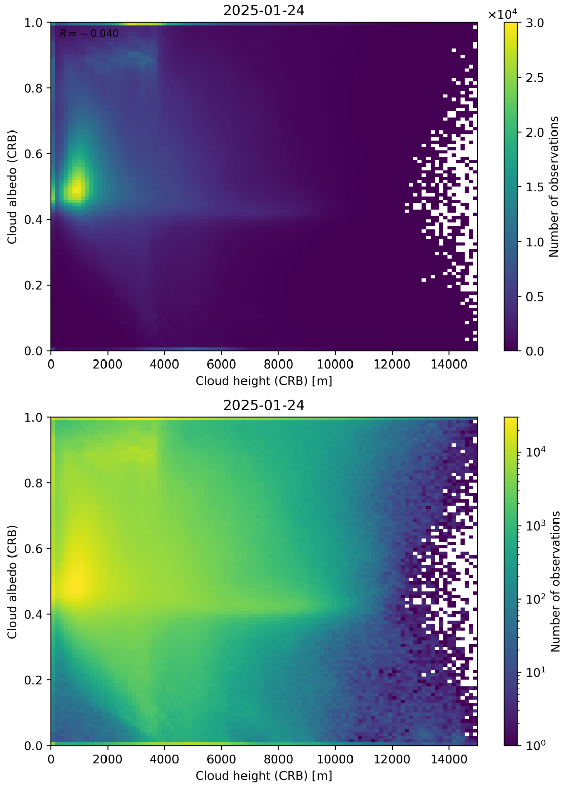
Figure 80: Scatter density plot of “Cloud height (CRB)” against “Cloud albedo (CRB)” for 2025-01-23 to 2025-01-25.
