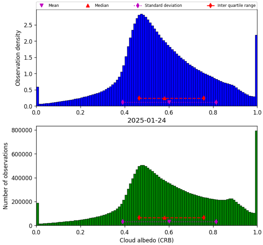
Figure 44: Histogram of “Cloud albedo (CRB)” for 2025-01-23 to 2025-01-25
