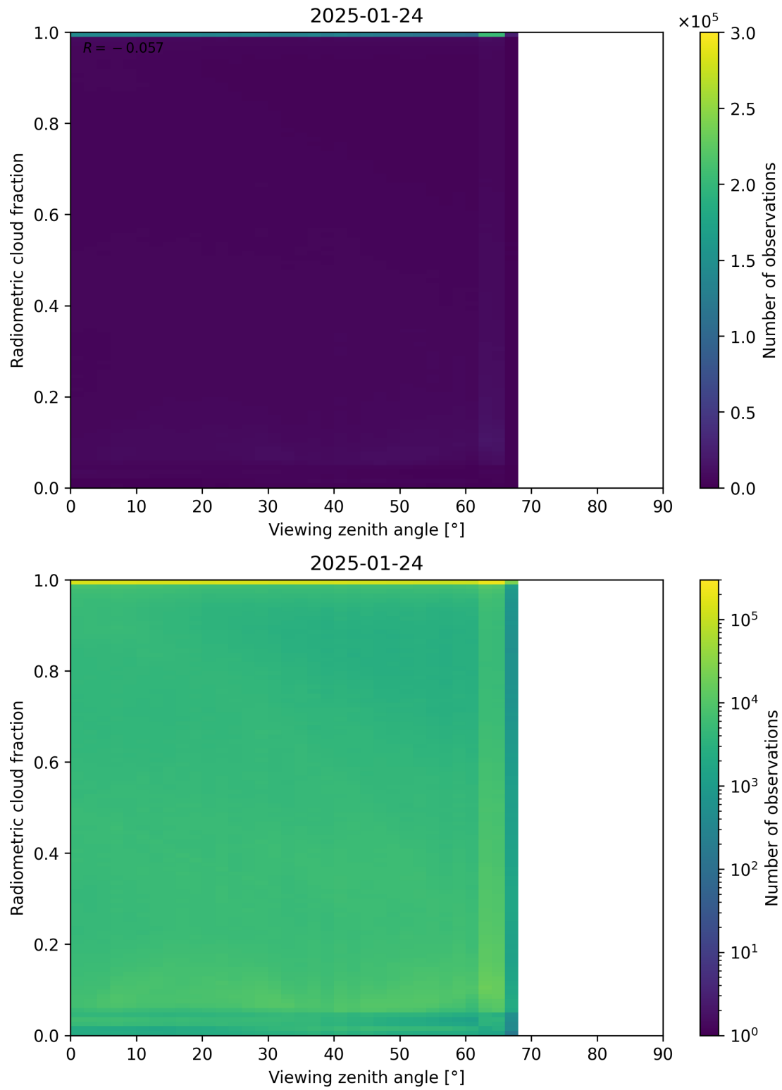
Figure 107: Scatter density plot of “Viewing zenith angle” against “Radiometric cloud fraction” for 2025-01-23 to 2025-01-25.
