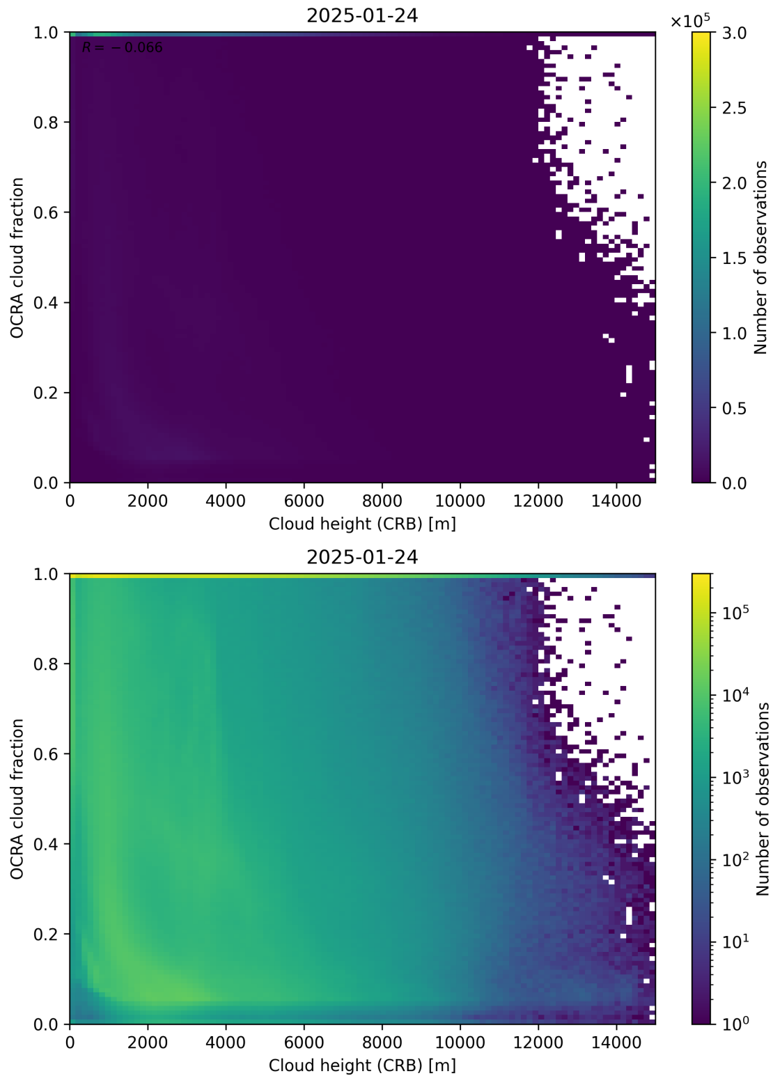
Figure 81: Scatter density plot of “Cloud height (CRB)” against “OCRA cloud fraction” for 2025-01-23 to 2025-01-25.
