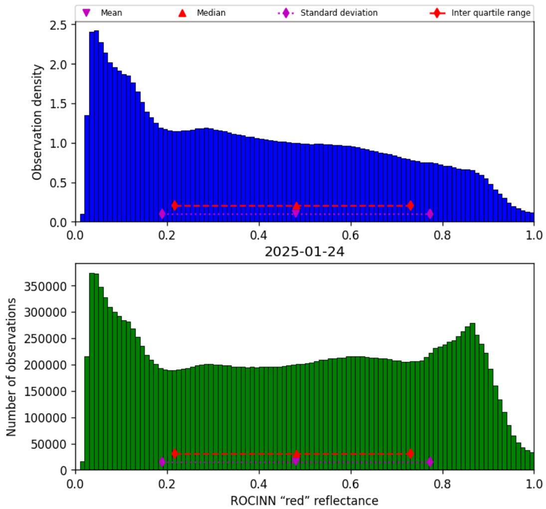
Figure 53: Histogram of “ROCINN “red” reflectance” for 2025-01-23 to 2025-01-25
