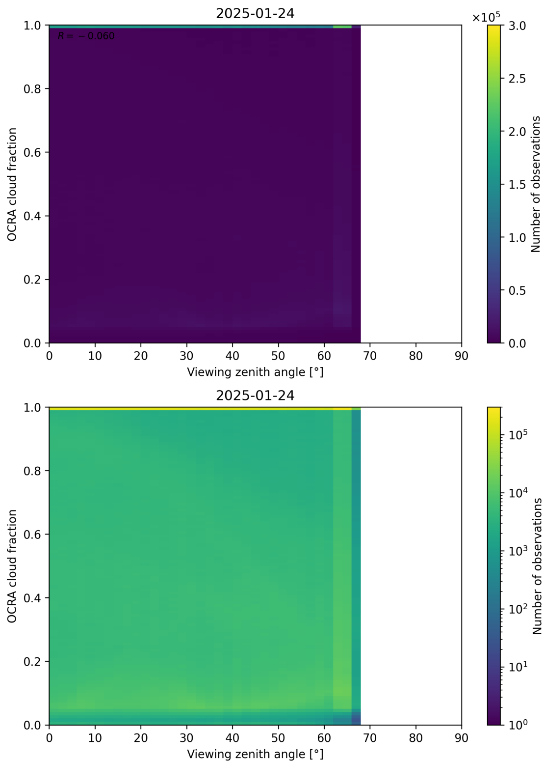
Figure 108: Scatter density plot of “Viewing zenith angle” against “OCRA cloud fraction” for 2025-01-23 to 2025-01-25.
