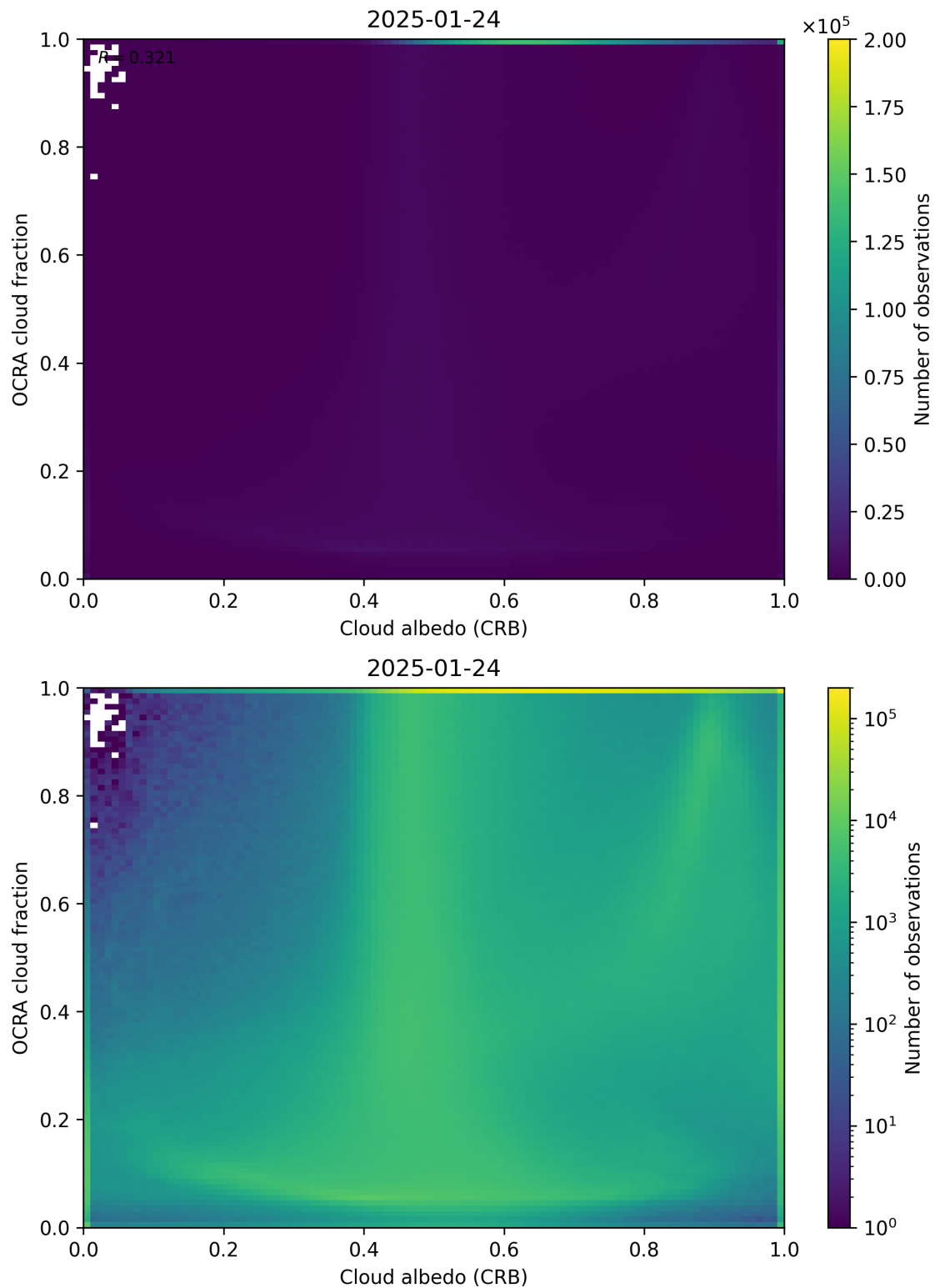
Figure 70: Scatter density plot of “Cloud albedo (CRB)” against “OCRA cloud fraction” for 2025-01-23 to 2025-01-25.
