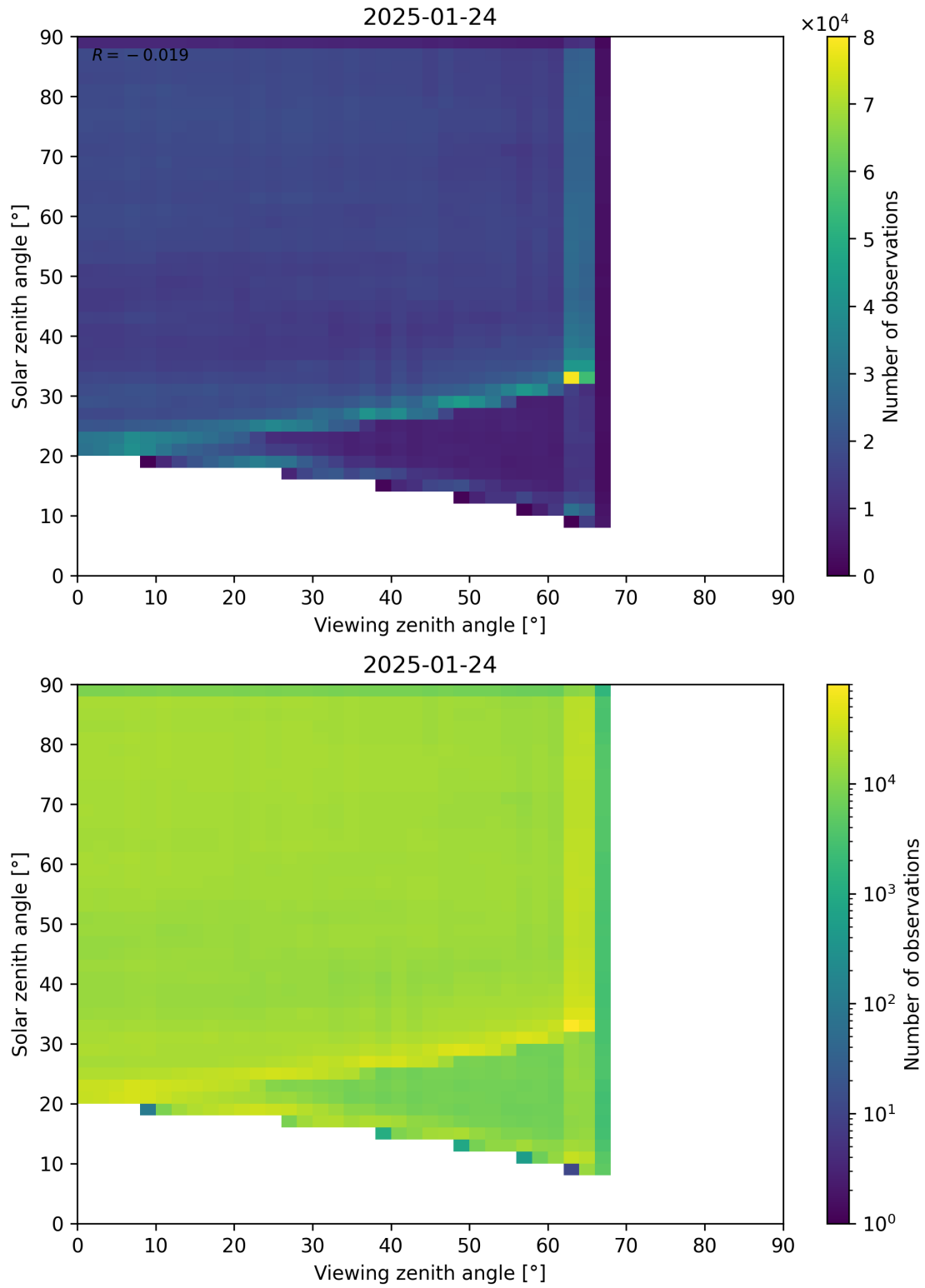
Figure 114: Scatter density plot of “Viewing zenith angle” against “Solar zenith angle” for 2025-01-23 to 2025-01-25.
