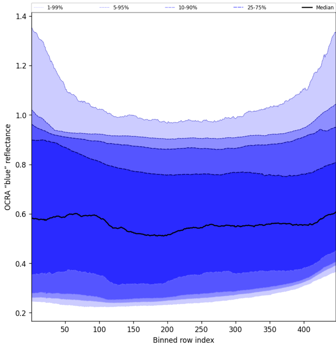
Figure 67: Along track statistics of “OCRA “blue” reflectance” for 2025-01-23 to 2025-01-25
