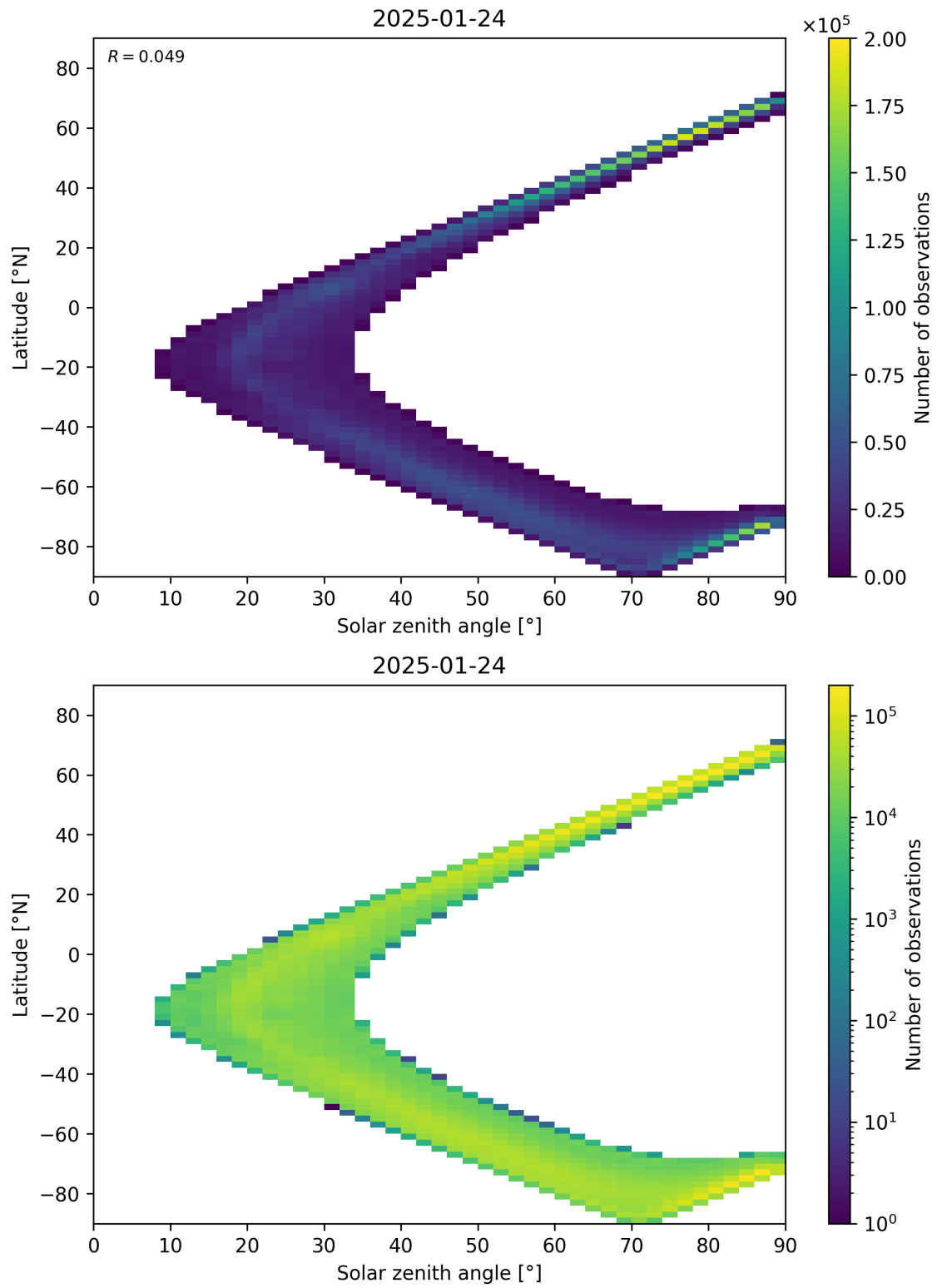
Figure 105: Scatter density plot of “Solar zenith angle” against “Latitude” for 2025-01-23 to 2025-01-25.
