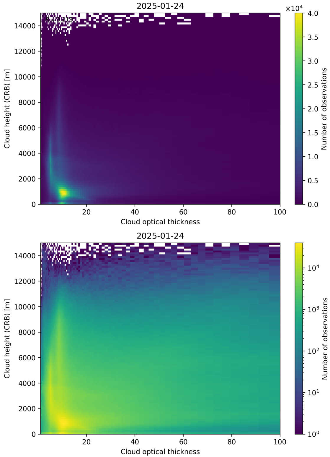
Figure 85: Scatter density plot of “Cloud optical thickness” against “Cloud height (CRB)” for 2025-01-23 to 2025-01-25.
