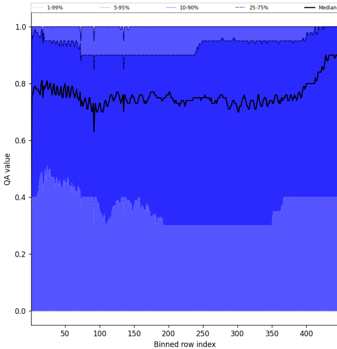
Figure 54: Along track statistics of “QA value” for 2025-01-23 to 2025-01-25
