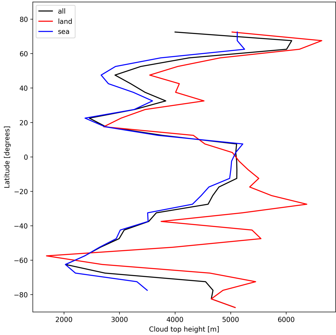
Figure 24: Zonal average of “Cloud top height” for 2025-01-23 to 2025-01-25.
