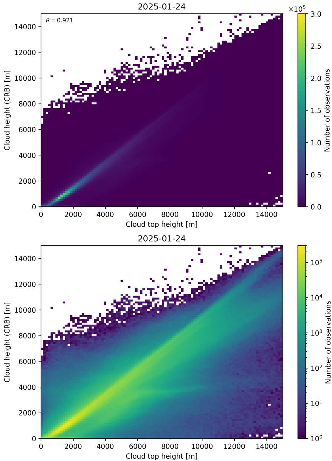
Figure 89: Scatter density plot of “Cloud top height” against “Cloud height (CRB)” for 2025-01-23 to 2025-01-25.
