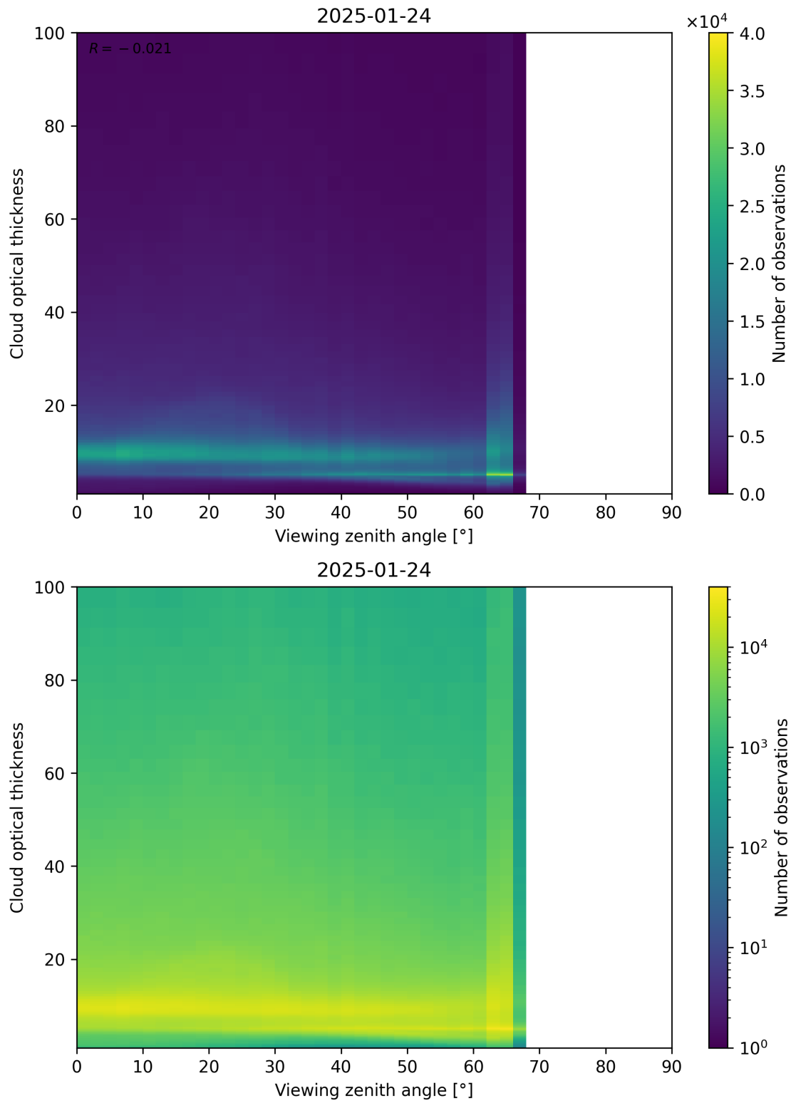
Figure 111: Scatter density plot of “Viewing zenith angle” against “Cloud optical thickness” for 2025-01-23 to 2025-01-25.
