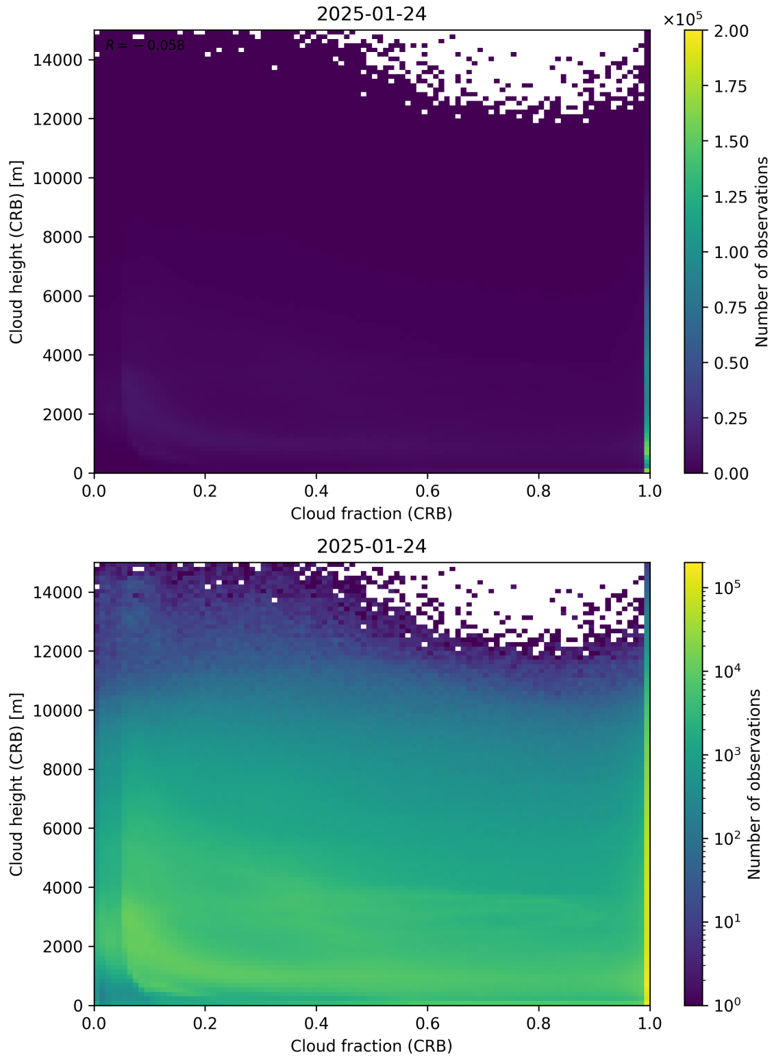
Figure 79: Scatter density plot of “Cloud fraction (CRB)” against “Cloud height (CRB)” for 2025-01-23 to 2025-01-25.
