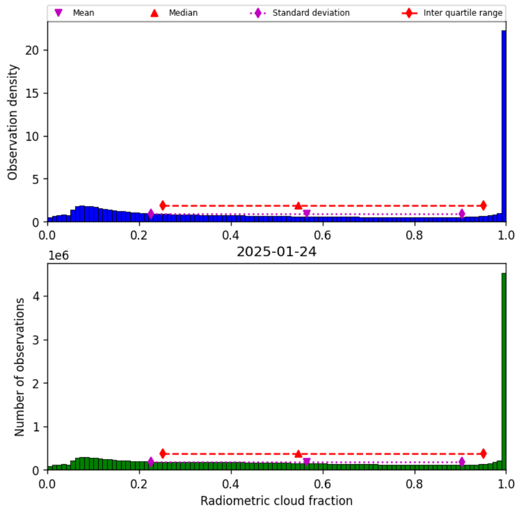
Figure 39: Histogram of “Radiometric cloud fraction” for 2025-01-23 to 2025-01-25
