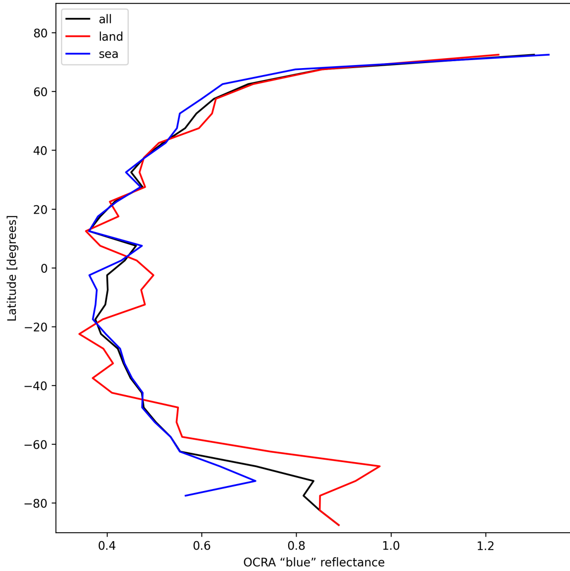
Figure 35: Zonal average of “OCRA “blue” reflectance” for 2025-01-23 to 2025-01-25.
