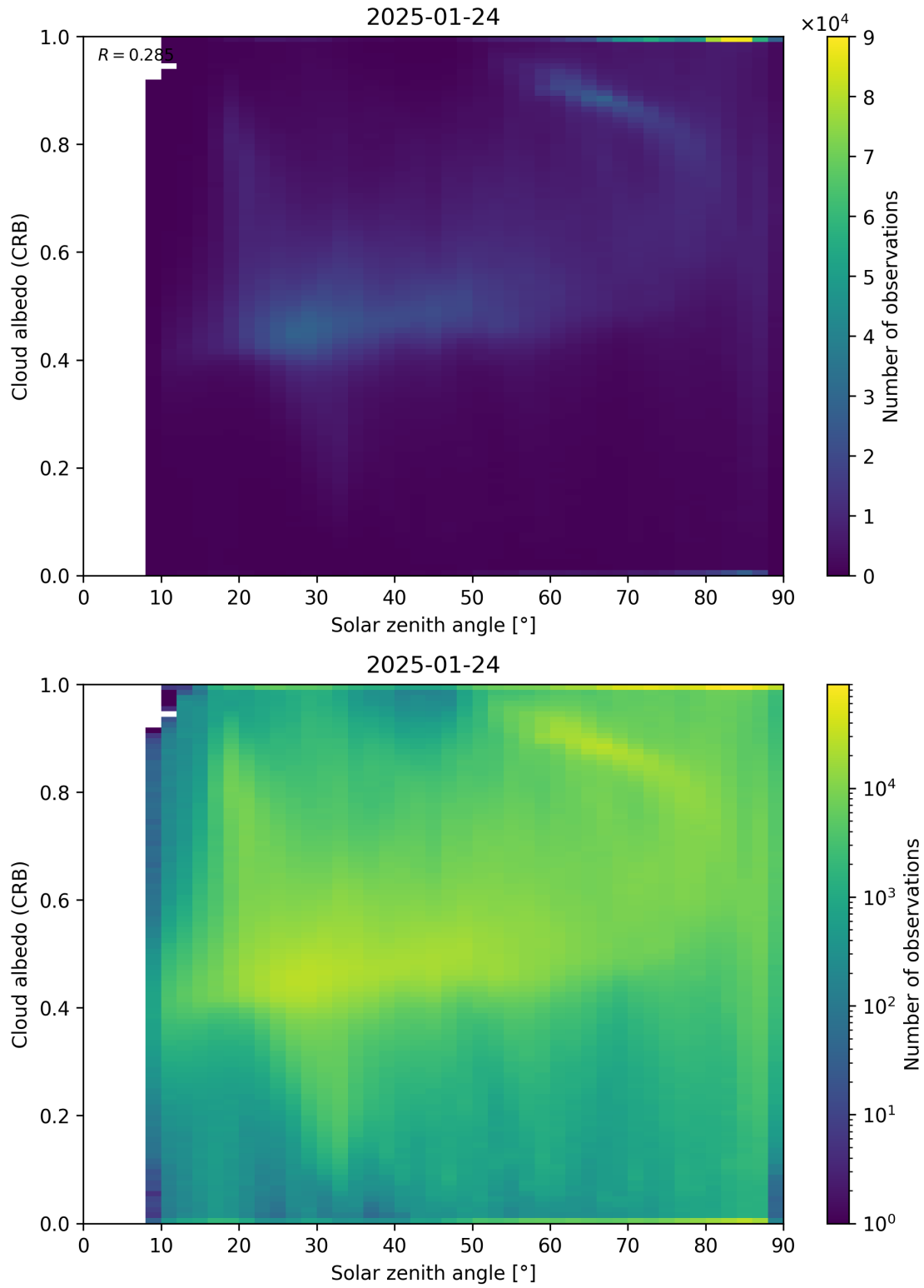
Figure 98: Scatter density plot of “Solar zenith angle” against “Cloud albedo (CRB)” for 2025-01-23 to 2025-01-25.
