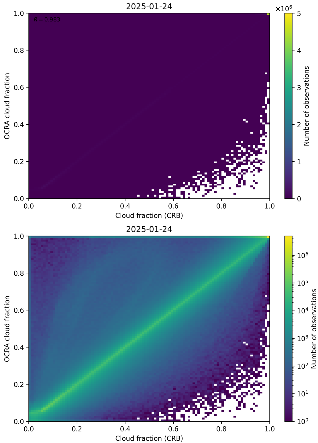
Figure 78: Scatter density plot of “Cloud fraction (CRB)” against “OCRA cloud fraction” for 2025-01-23 to 2025-01-25.
