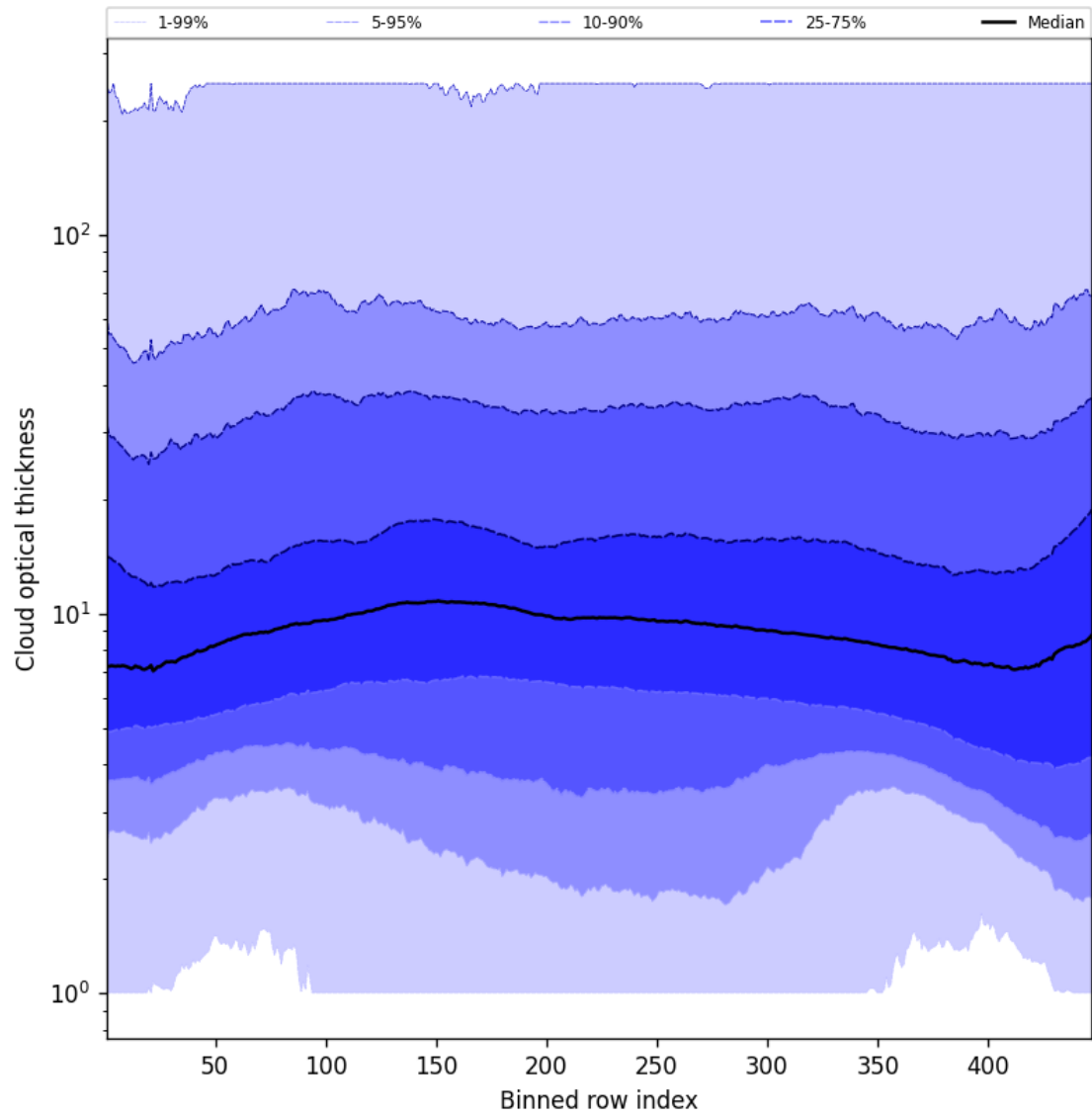
Figure 57: Along track statistics of “Cloud optical thickness” for 2025-01-23 to 2025-01-25
