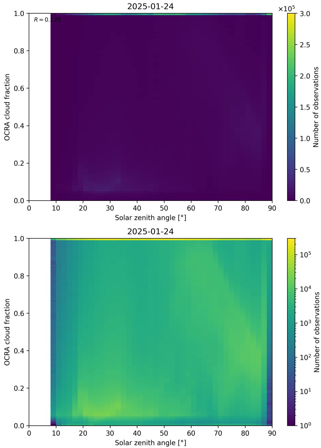
Figure 100: Scatter density plot of “Solar zenith angle” against “OCRA cloud fraction” for 2025-01-23 to 2025-01-25.
