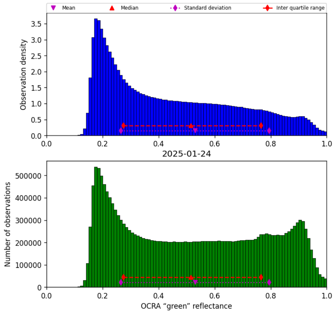
Figure 52: Histogram of “OCRA “green” reflectance” for 2025-01-23 to 2025-01-25
