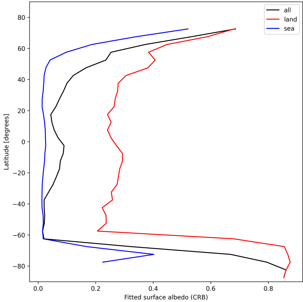
Figure 30: Zonal average of “Fitted surface albedo (CRB)” for 2025-01-23 to 2025-01-25.
