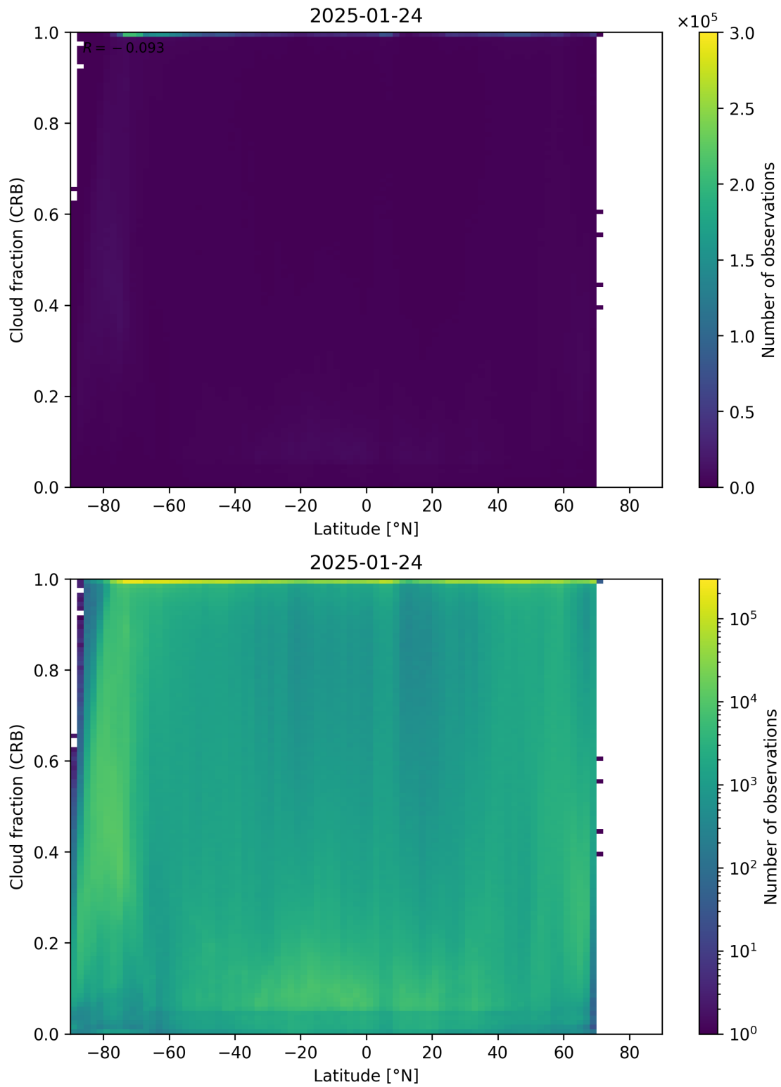
Figure 94: Scatter density plot of “Latitude” against “Cloud fraction (CRB)” for 2025-01-23 to 2025-01-25.
