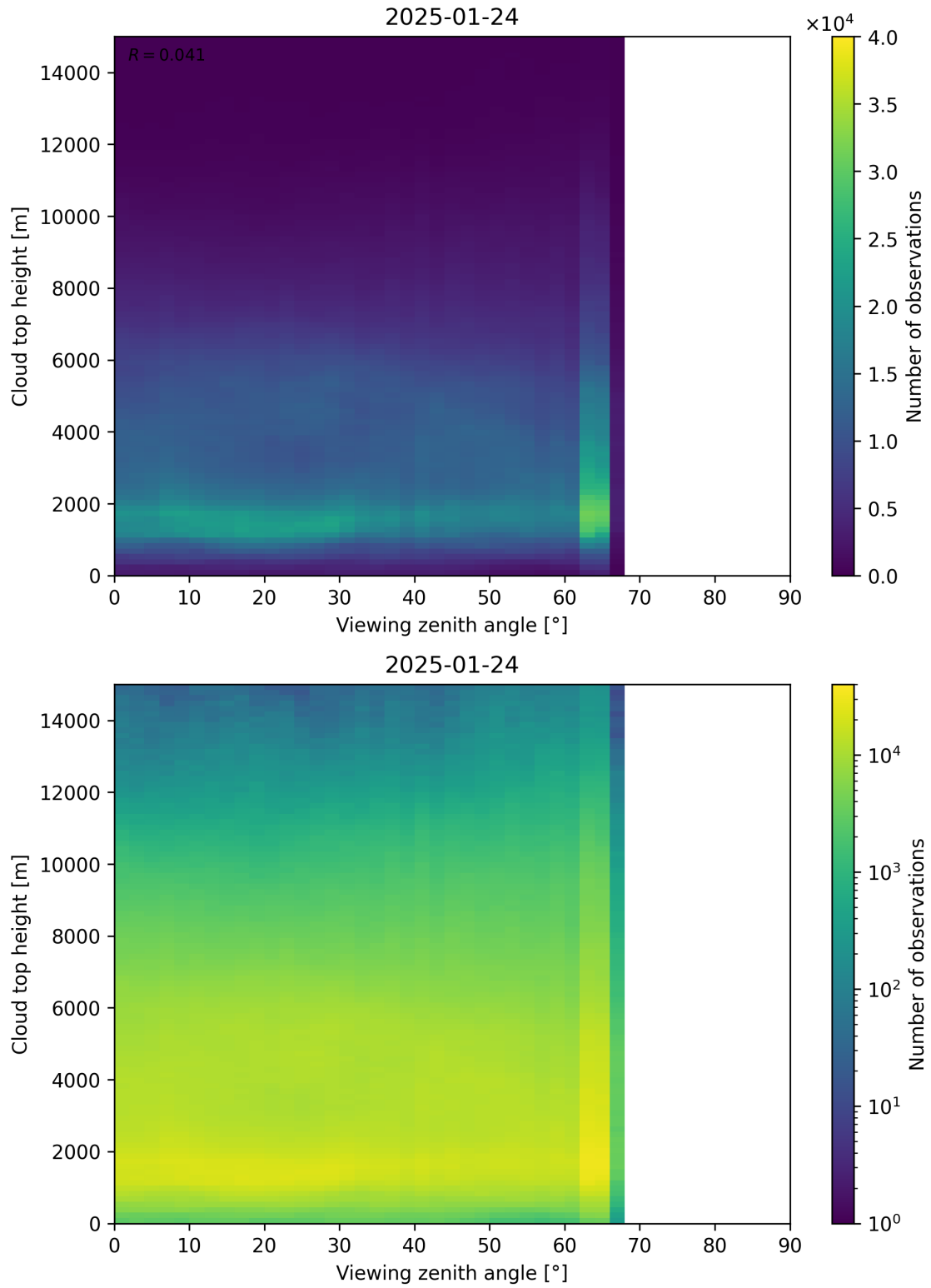
Figure 112: Scatter density plot of “Viewing zenith angle” against “Cloud top height” for 2025-01-23 to 2025-01-25.
