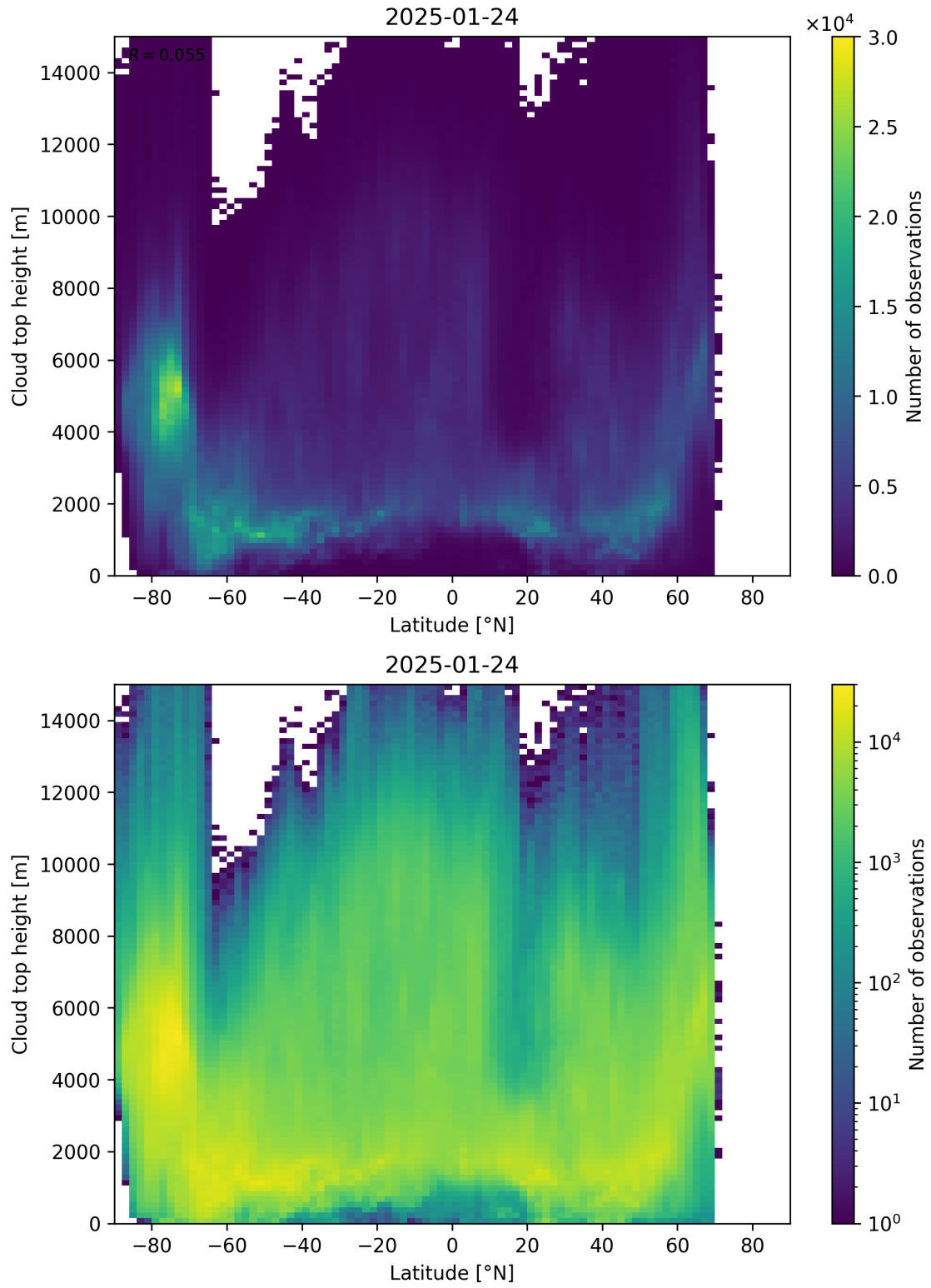
Figure 97: Scatter density plot of “Latitude” against “Cloud top height” for 2025-01-23 to 2025-01-25.
