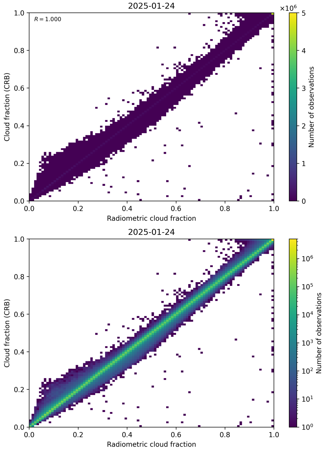
Figure 73: Scatter density plot of “Radiometric cloud fraction” against “Cloud fraction (CRB)” for 2025-01-23 to 2025-01-25.
