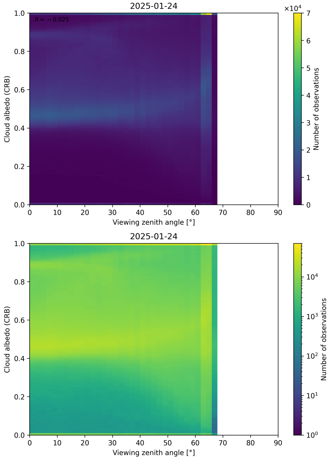
Figure 106: Scatter density plot of “Viewing zenith angle” against “Cloud albedo (CRB)” for 2025-01-23 to 2025-01-25.
