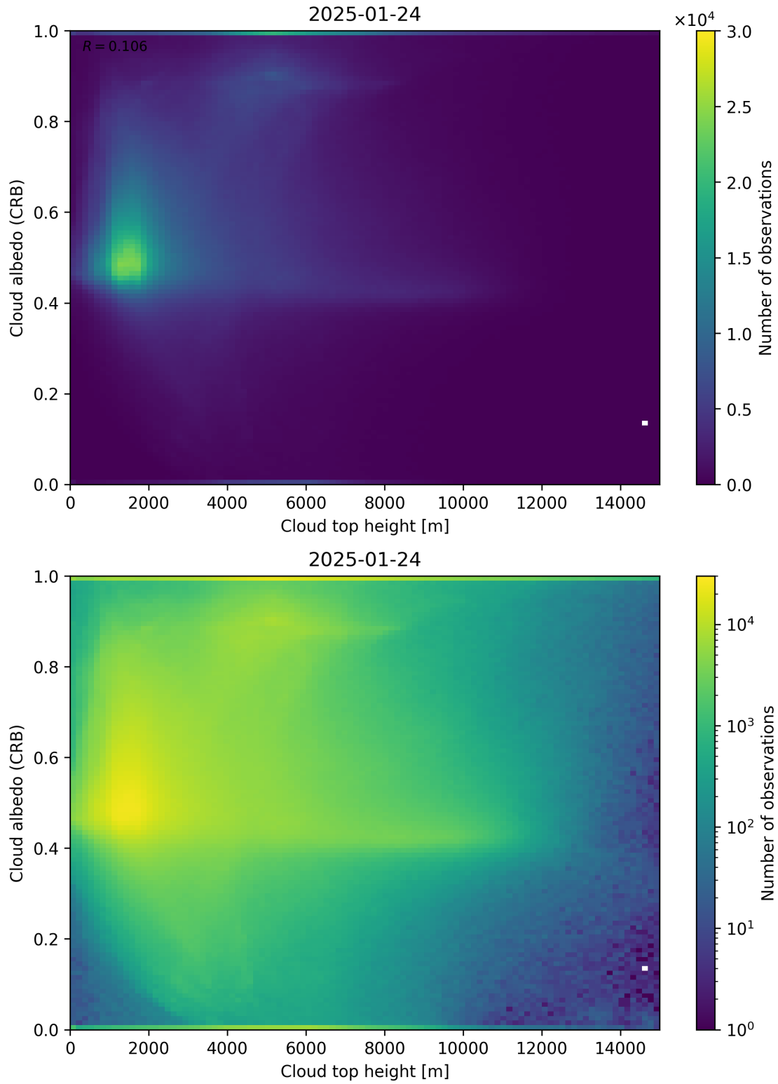
Figure 86: Scatter density plot of “Cloud top height” against “Cloud albedo (CRB)” for 2025-01-23 to 2025-01-25.
