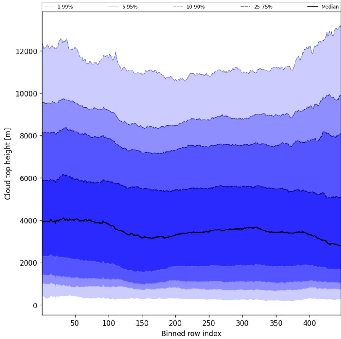
Figure 56: Along track statistics of “Cloud top height” for 2025-01-23 to 2025-01-25
