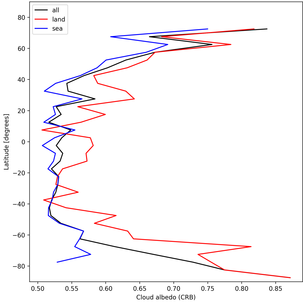
Figure 28: Zonal average of “Cloud albedo (CRB)” for 2025-01-23 to 2025-01-25.
