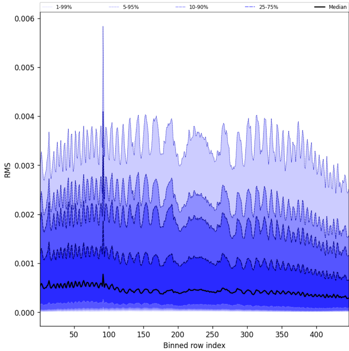
Figure 63: Along track statistics of “RMS” for 2025-01-23 to 2025-01-25
