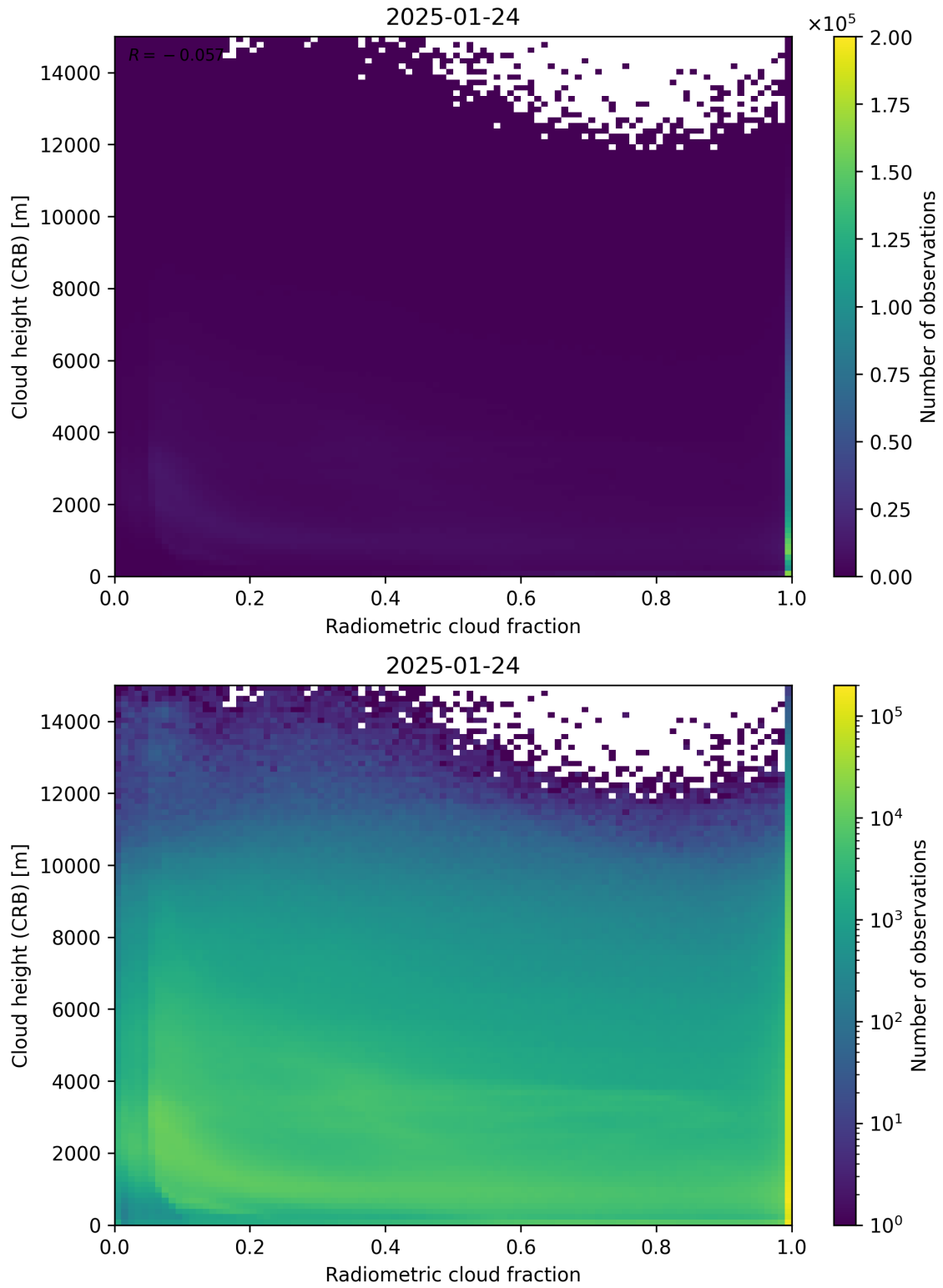
Figure 74: Scatter density plot of “Radiometric cloud fraction” against “Cloud height (CRB)” for 2025-01-23 to 2025-01-25.
