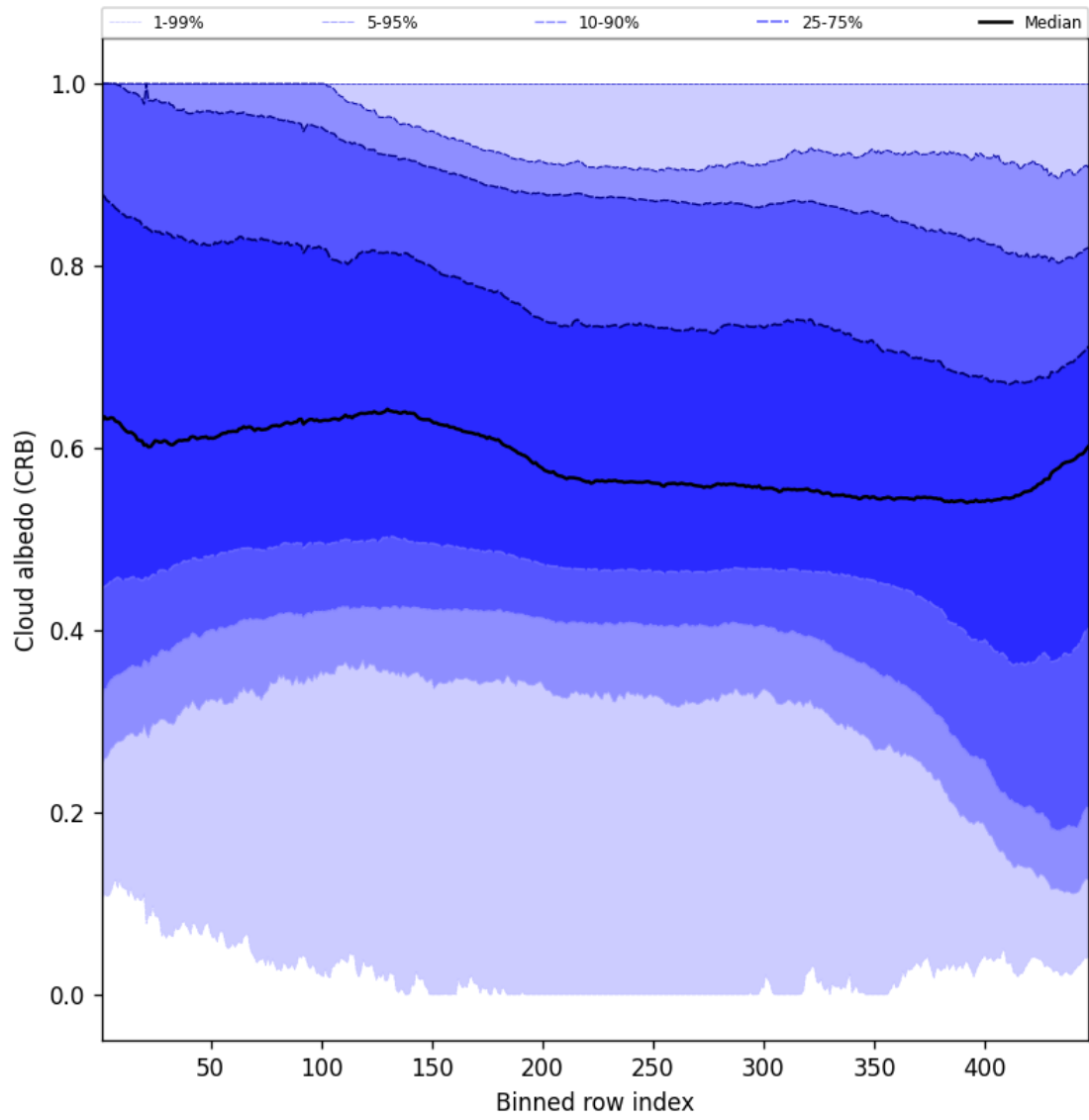
Figure 60: Along track statistics of “Cloud albedo (CRB)” for 2025-01-23 to 2025-01-25
