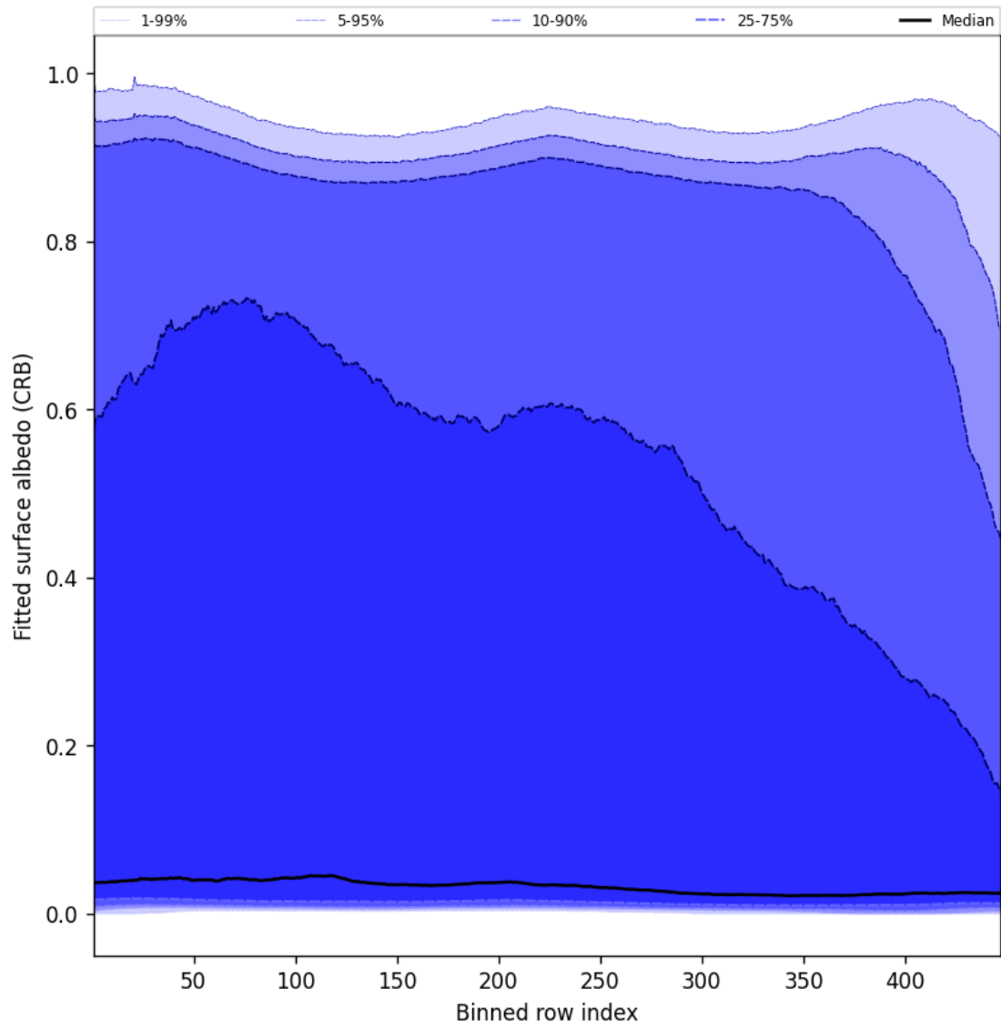
Figure 62: Along track statistics of “Fitted surface albedo (CRB)” for 2025-01-23 to 2025-01-25
