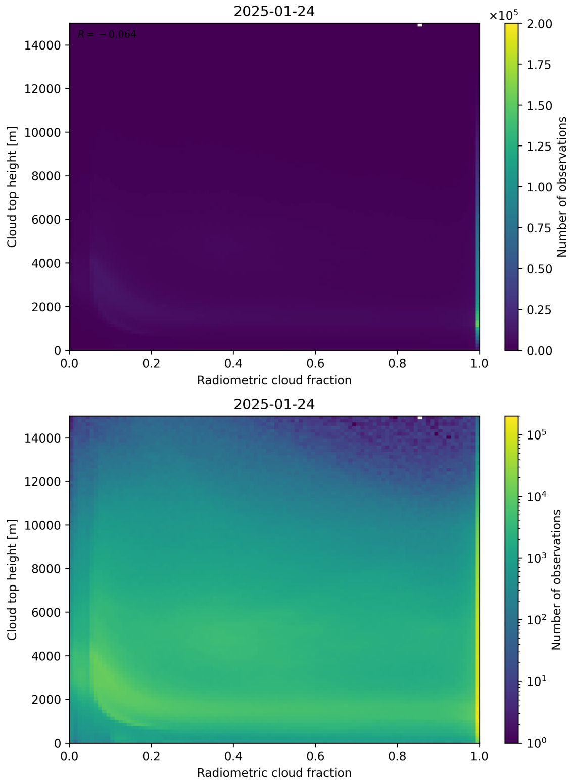
Figure 76: Scatter density plot of “Radiometric cloud fraction” against “Cloud top height” for 2025-01-23 to 2025-01-25.
