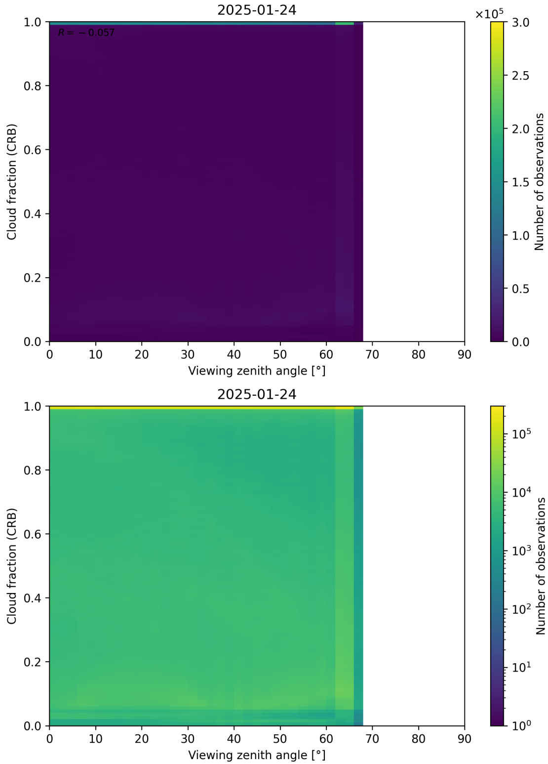
Figure 109: Scatter density plot of “Viewing zenith angle” against “Cloud fraction (CRB)” for 2025-01-23 to 2025-01-25.
