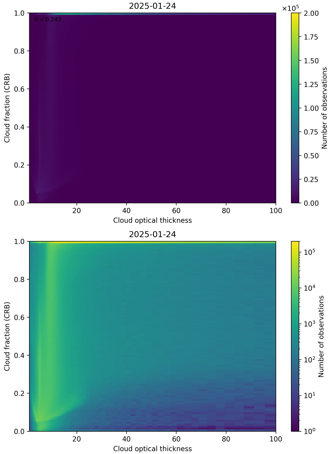
Figure 84: Scatter density plot of “Cloud optical thickness” against “Cloud fraction (CRB)” for 2025-01-23 to 2025-01-25.
