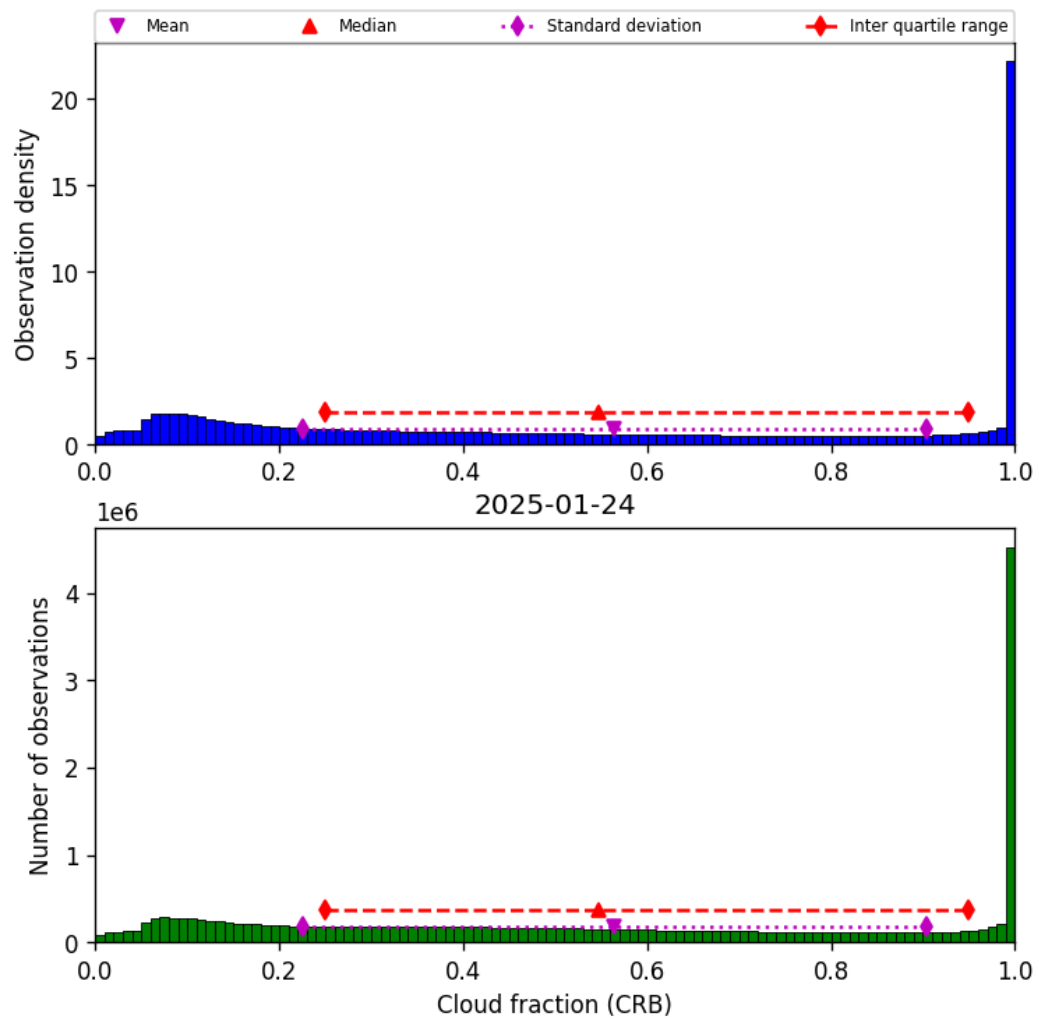
Figure 42: Histogram of “Cloud fraction (CRB)” for 2025-01-23 to 2025-01-25
