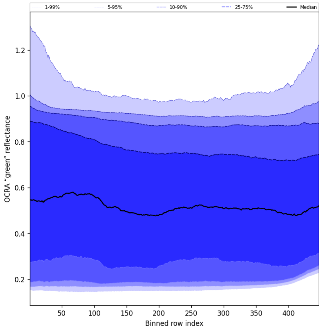
Figure 68: Along track statistics of “OCRA “green” reflectance” for 2025-01-23 to 2025-01-25
