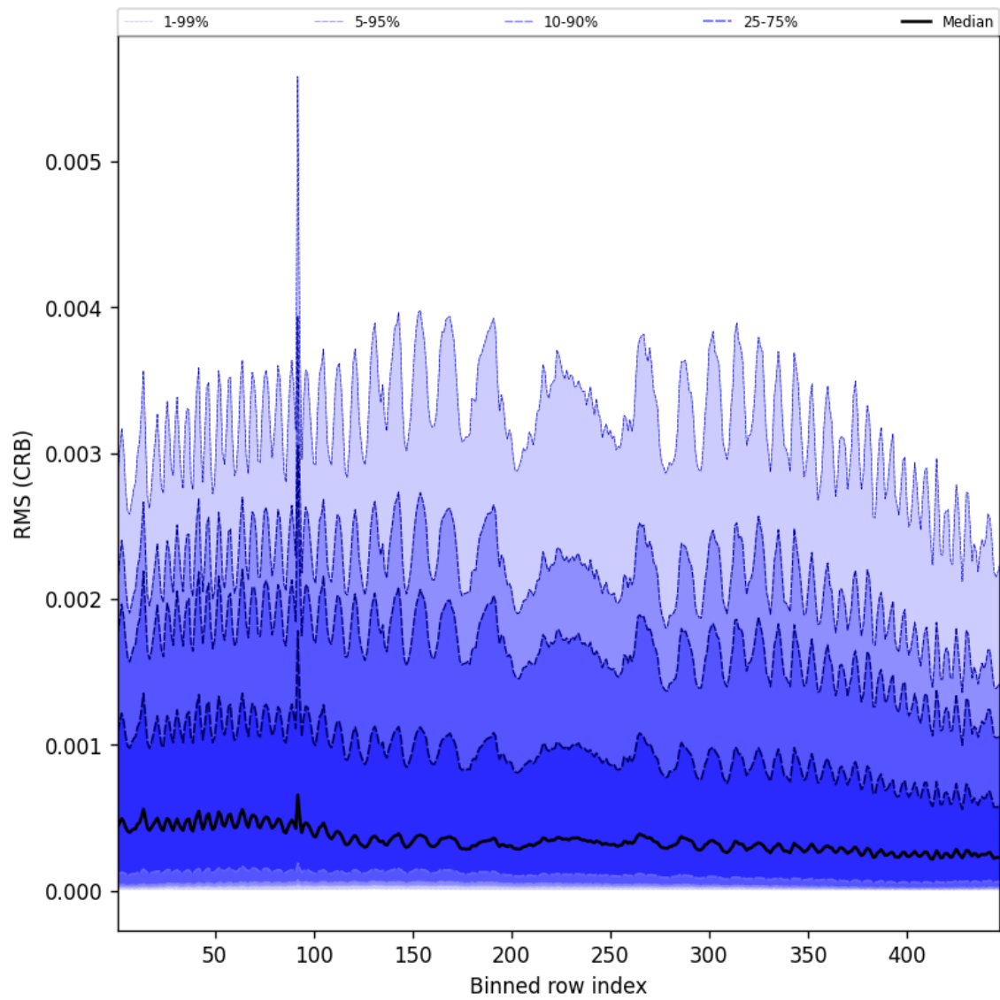
Figure 64: Along track statistics of “RMS (CRB)” for 2025-01-23 to 2025-01-25
