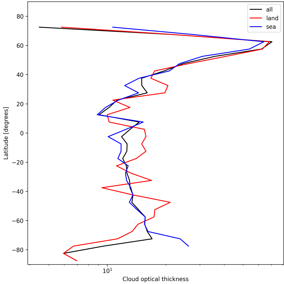
Figure 25: Zonal average of “Cloud optical thickness” for 2025-01-23 to 2025-01-25.
