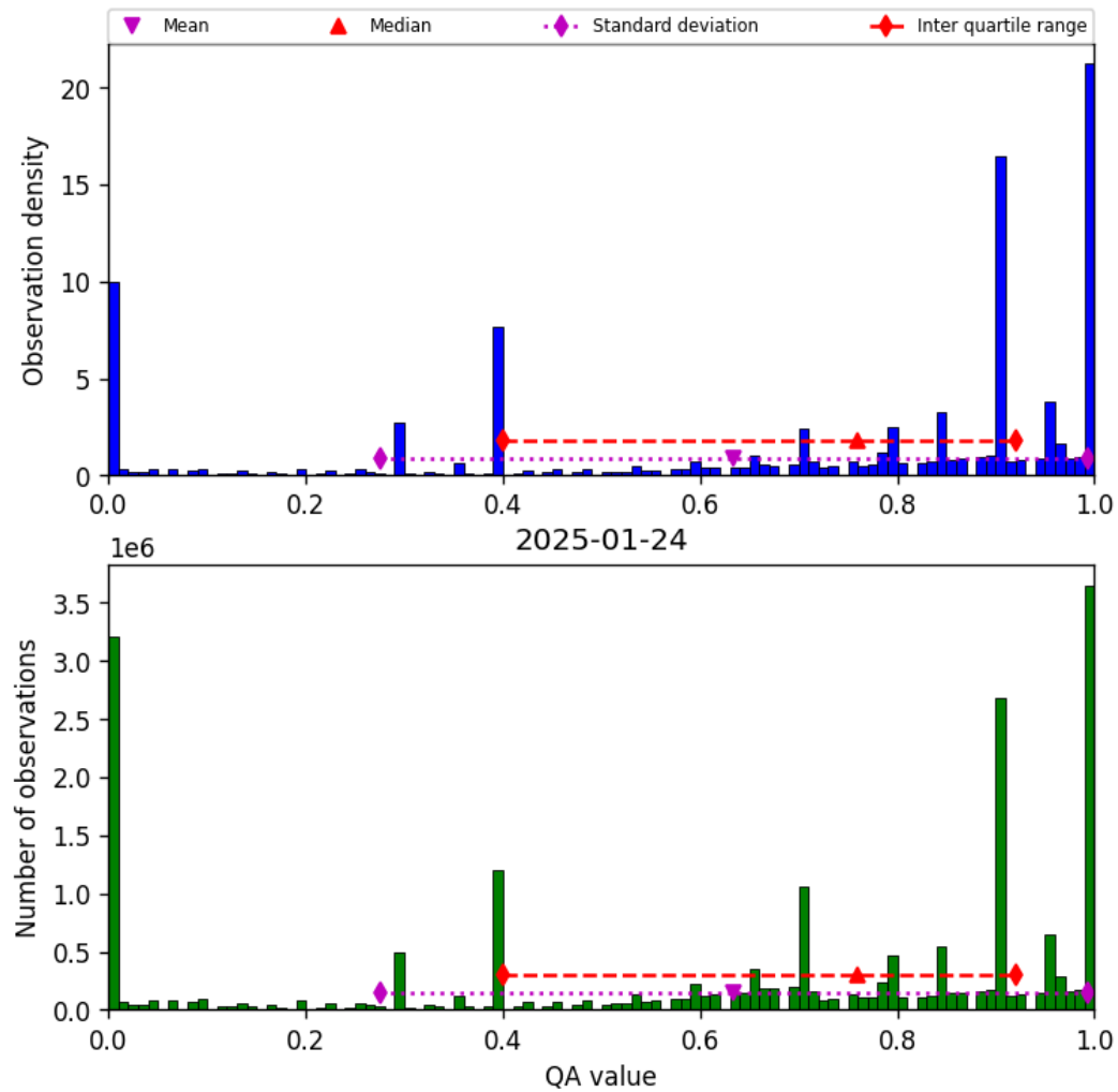
Figure 38: Histogram of “QA value” for 2025-01-23 to 2025-01-25
