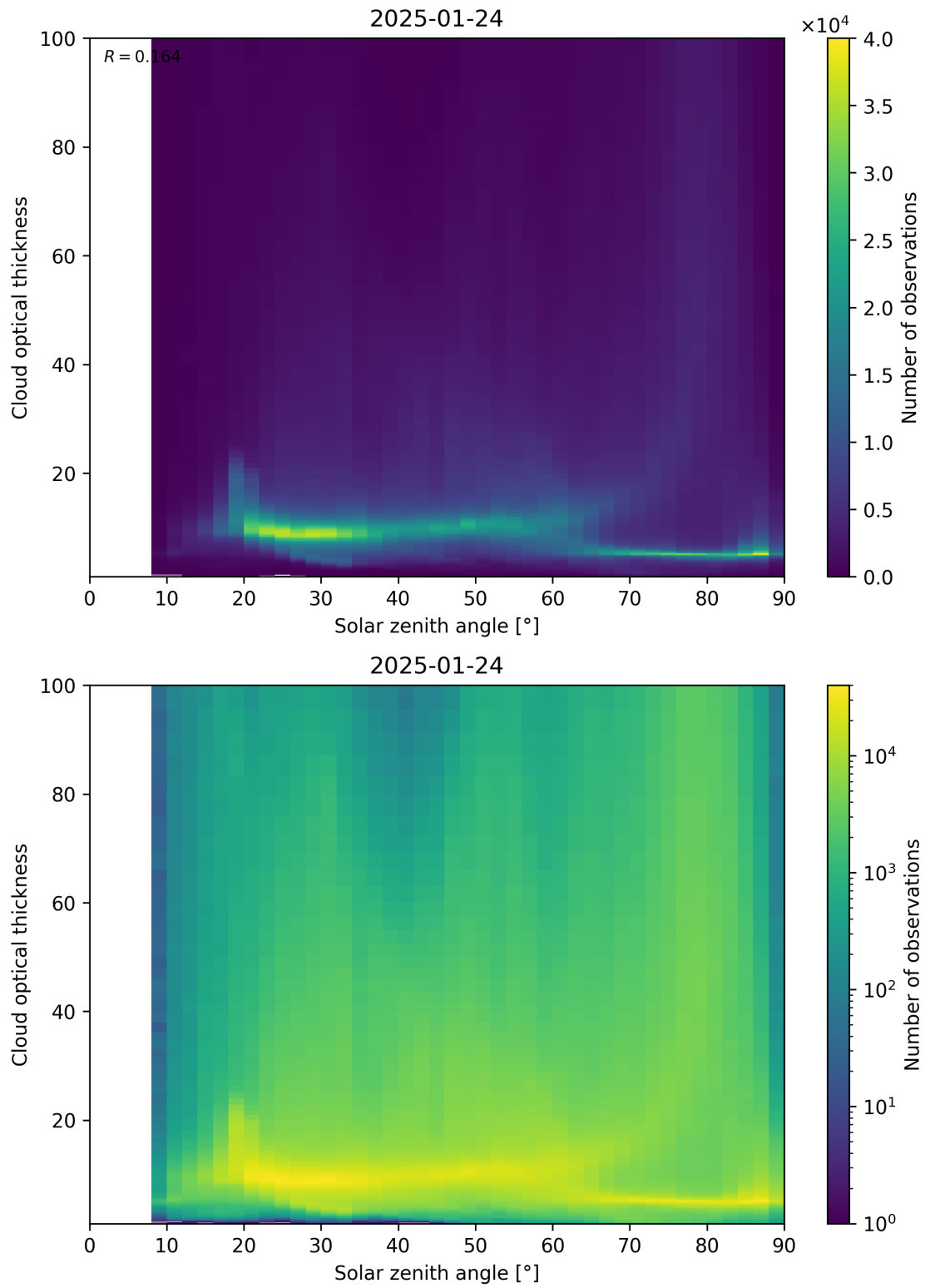
Figure 103: Scatter density plot of “Solar zenith angle” against “Cloud optical thickness” for 2025-01-23 to 2025-01-25.
