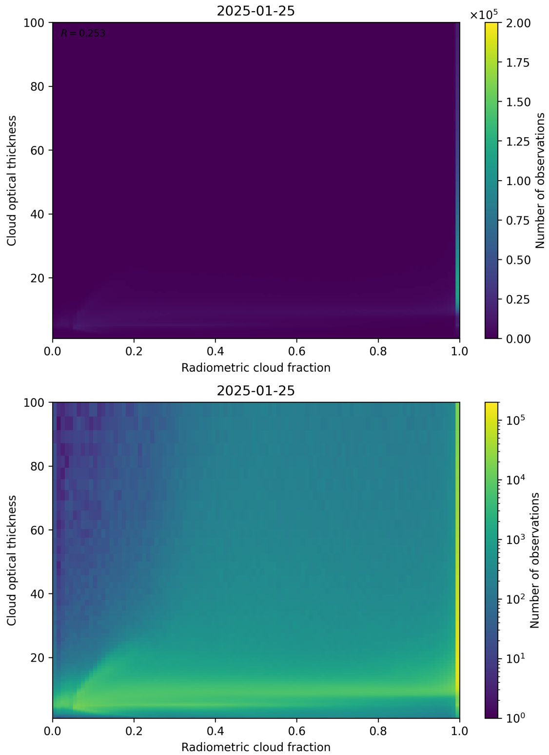
Figure 75: Scatter density plot of “Radiometric cloud fraction” against “Cloud optical thickness” for 2025-01-24 to 2025-01-26.
