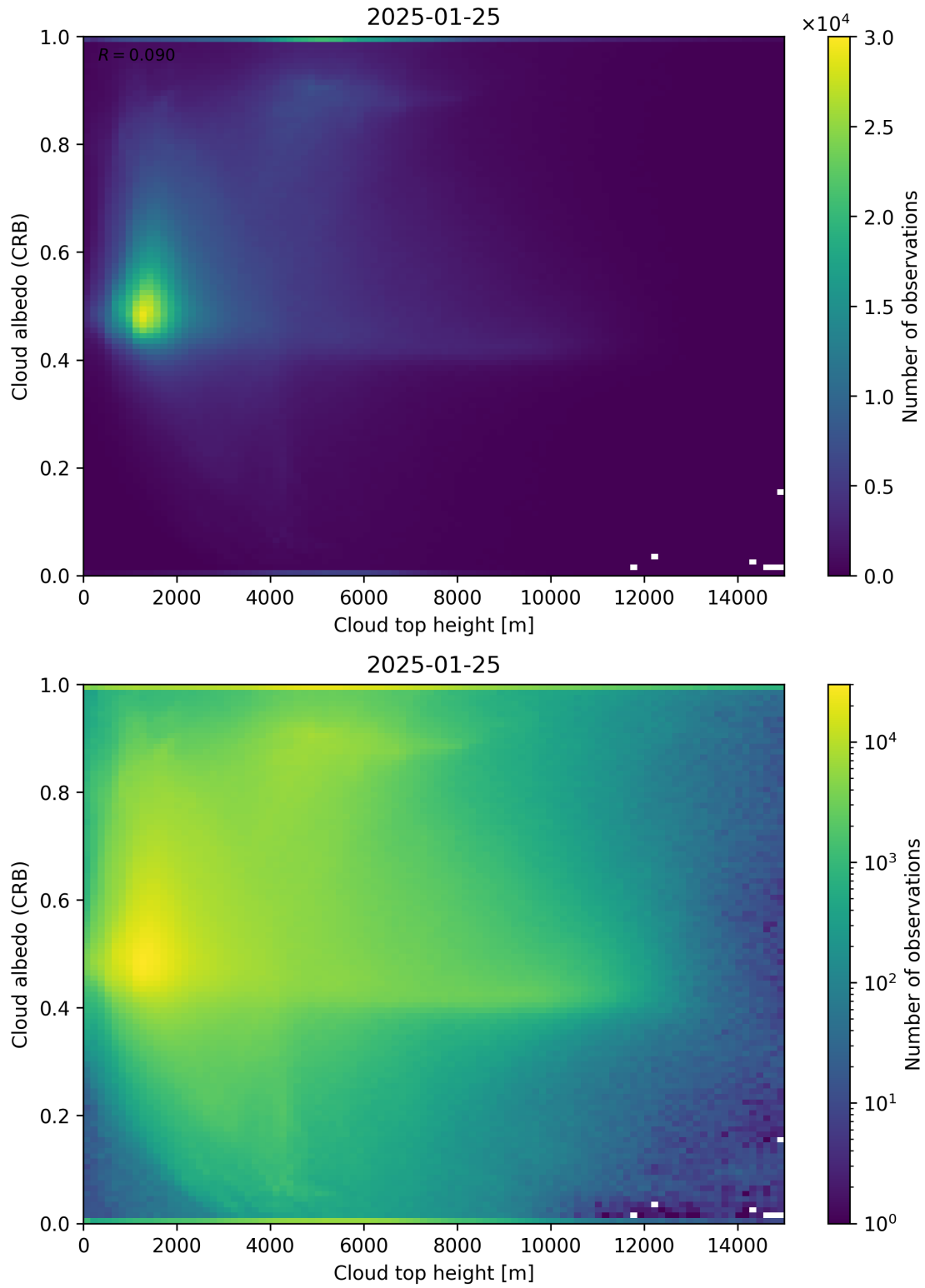
Figure 86: Scatter density plot of “Cloud top height” against “Cloud albedo (CRB)” for 2025-01-24 to 2025-01-26.
