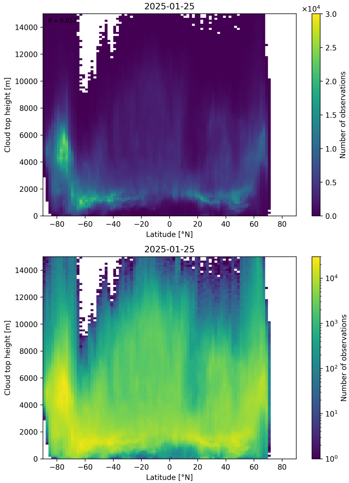
Figure 97: Scatter density plot of “Latitude” against “Cloud top height” for 2025-01-24 to 2025-01-26.
