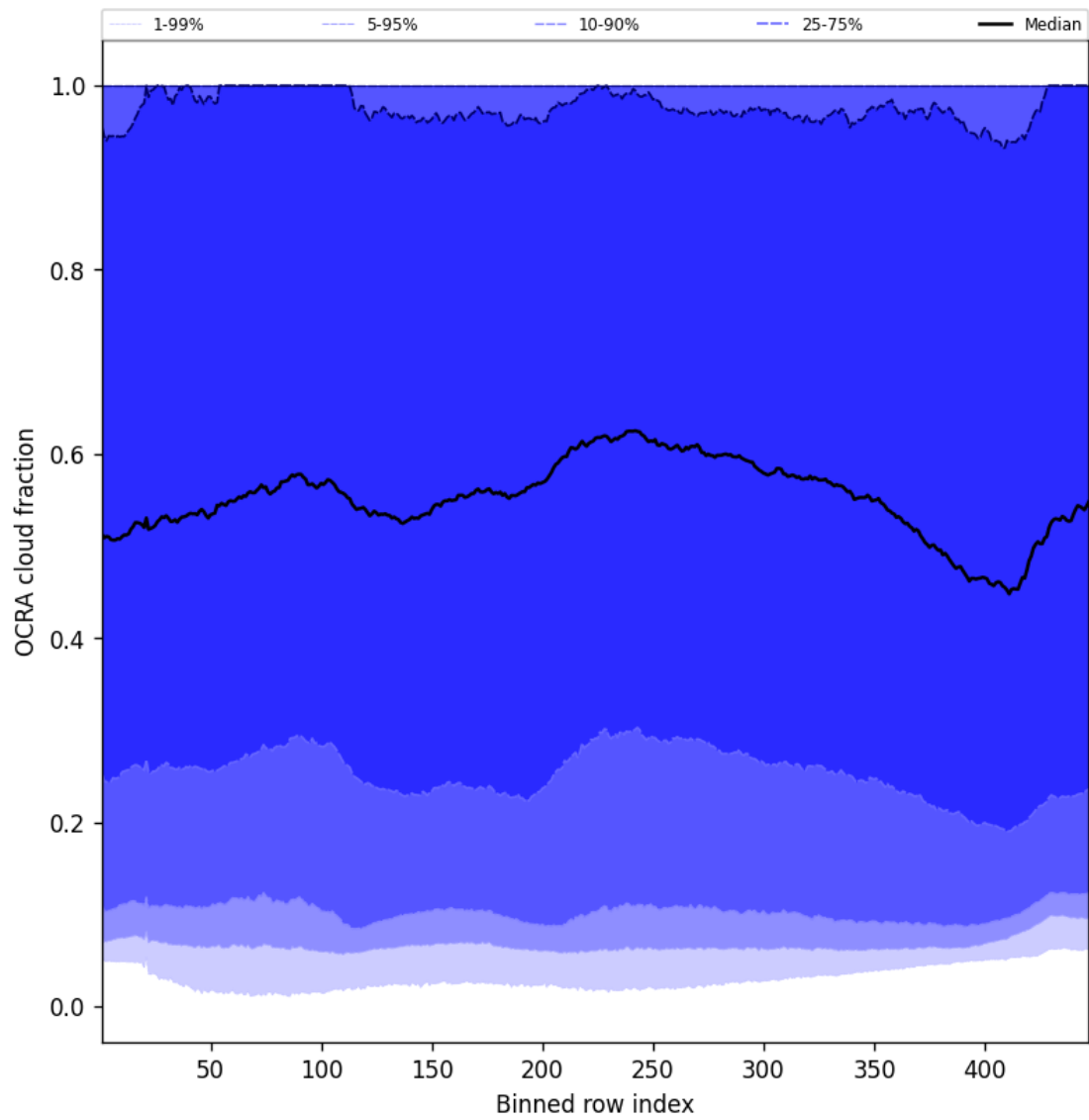
Figure 66: Along track statistics of “OCRA cloud fraction” for 2025-01-24 to 2025-01-26
