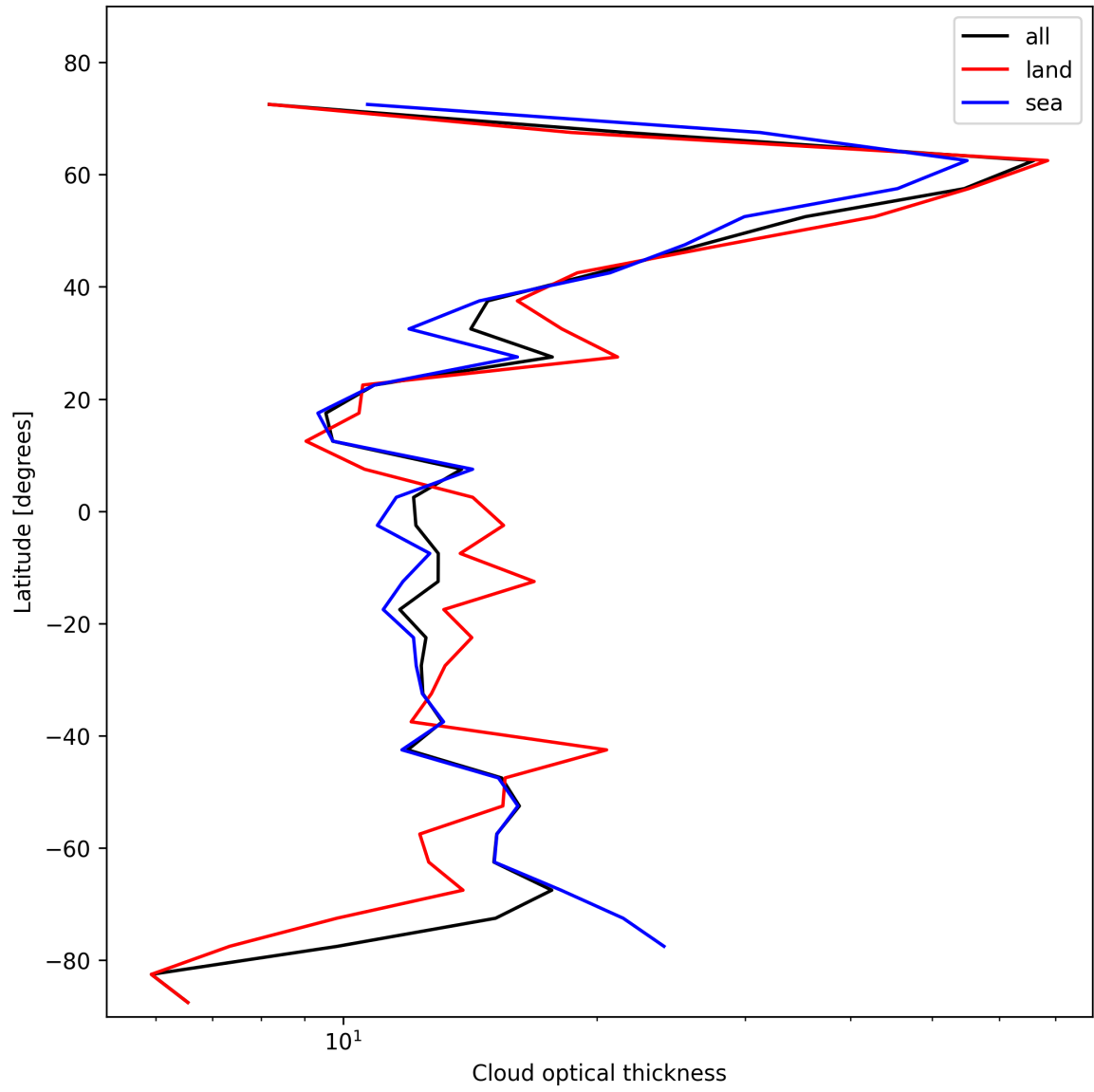
Figure 25: Zonal average of “Cloud optical thickness” for 2025-01-24 to 2025-01-26.
