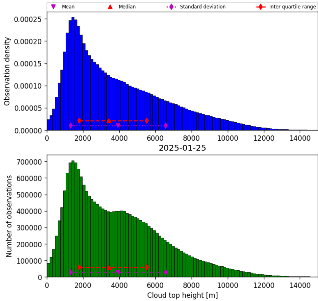
Figure 40: Histogram of “Cloud top height” for 2025-01-24 to 2025-01-26
