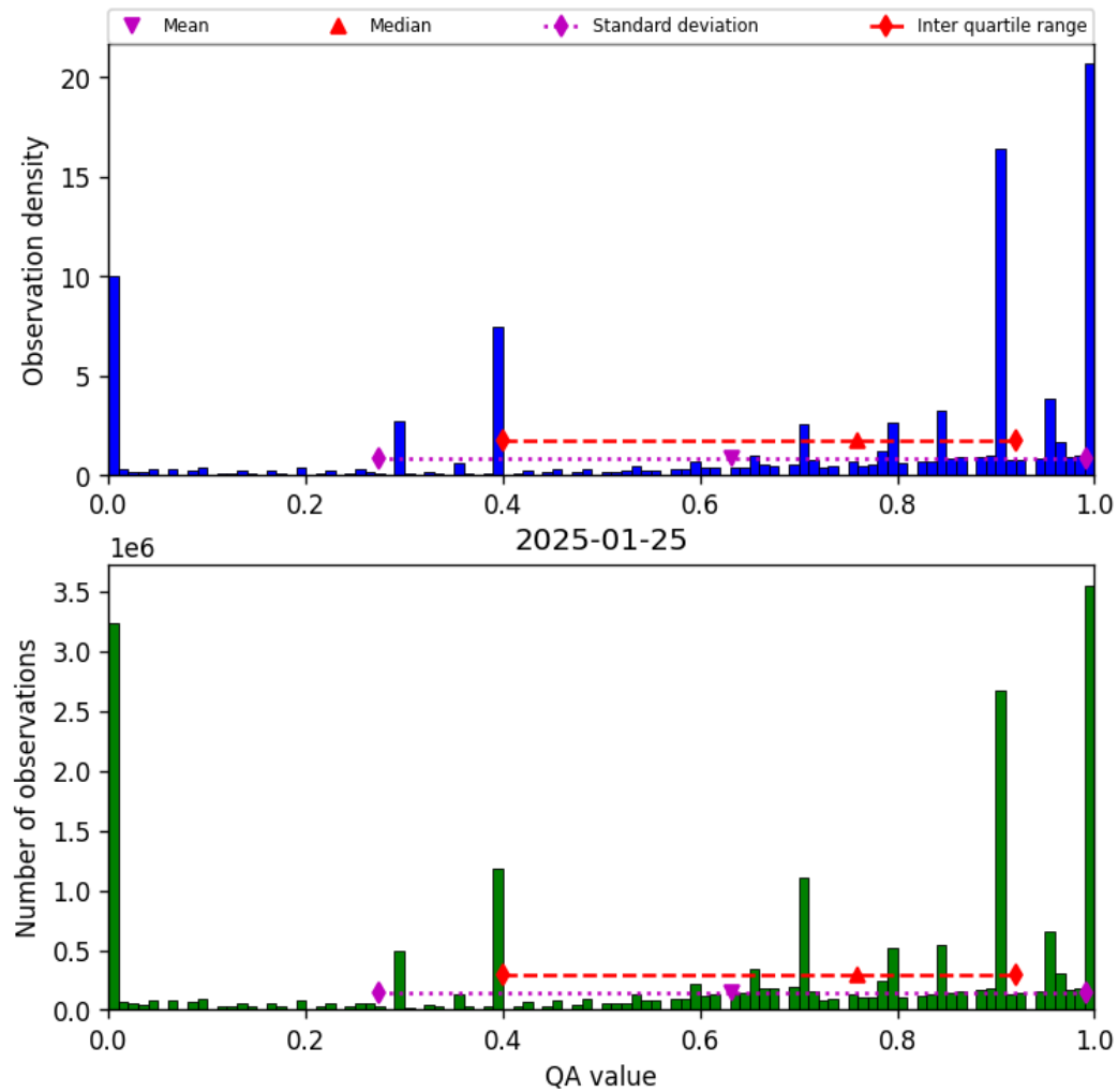
Figure 38: Histogram of “QA value” for 2025-01-24 to 2025-01-26
