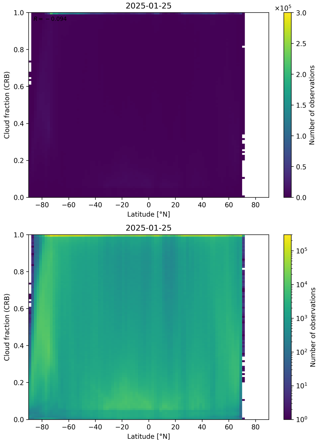
Figure 94: Scatter density plot of “Latitude” against “Cloud fraction (CRB)” for 2025-01-24 to 2025-01-26.
