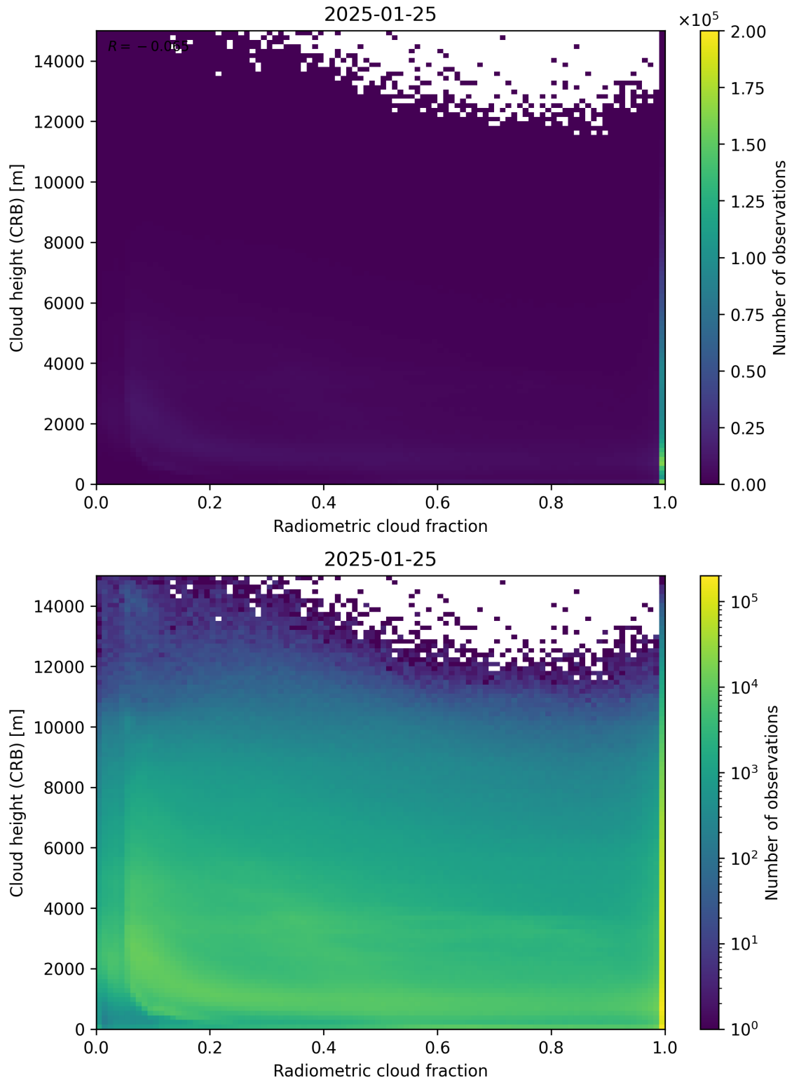
Figure 74: Scatter density plot of “Radiometric cloud fraction” against “Cloud height (CRB)” for 2025-01-24 to 2025-01-26.
