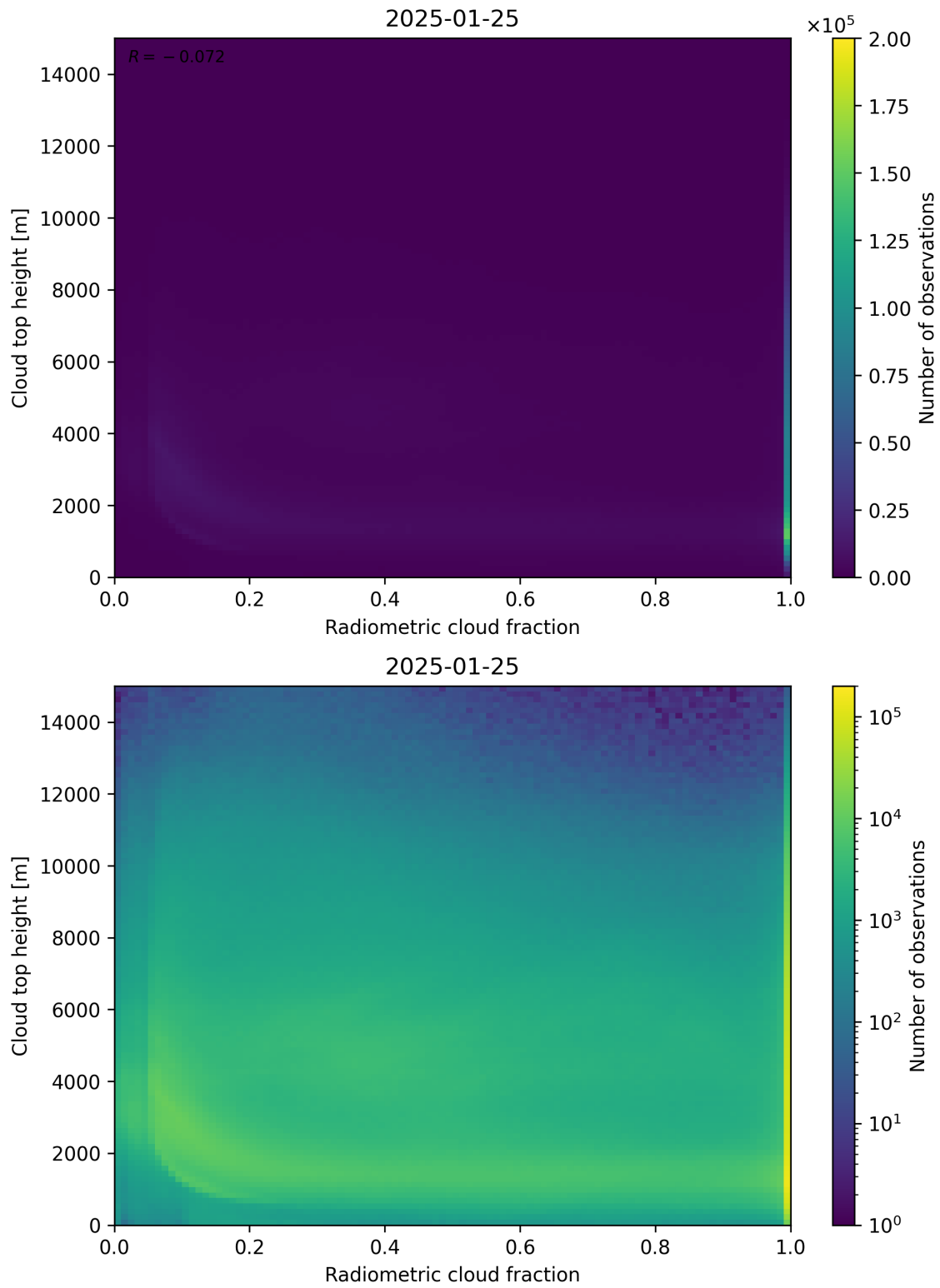
Figure 76: Scatter density plot of “Radiometric cloud fraction” against “Cloud top height” for 2025-01-24 to 2025-01-26.
