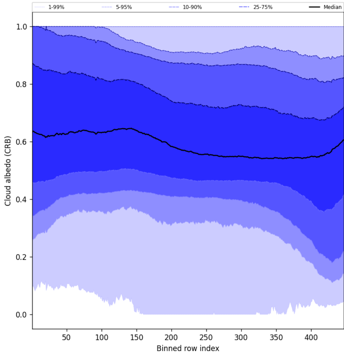
Figure 60: Along track statistics of “Cloud albedo (CRB)” for 2025-01-24 to 2025-01-26
