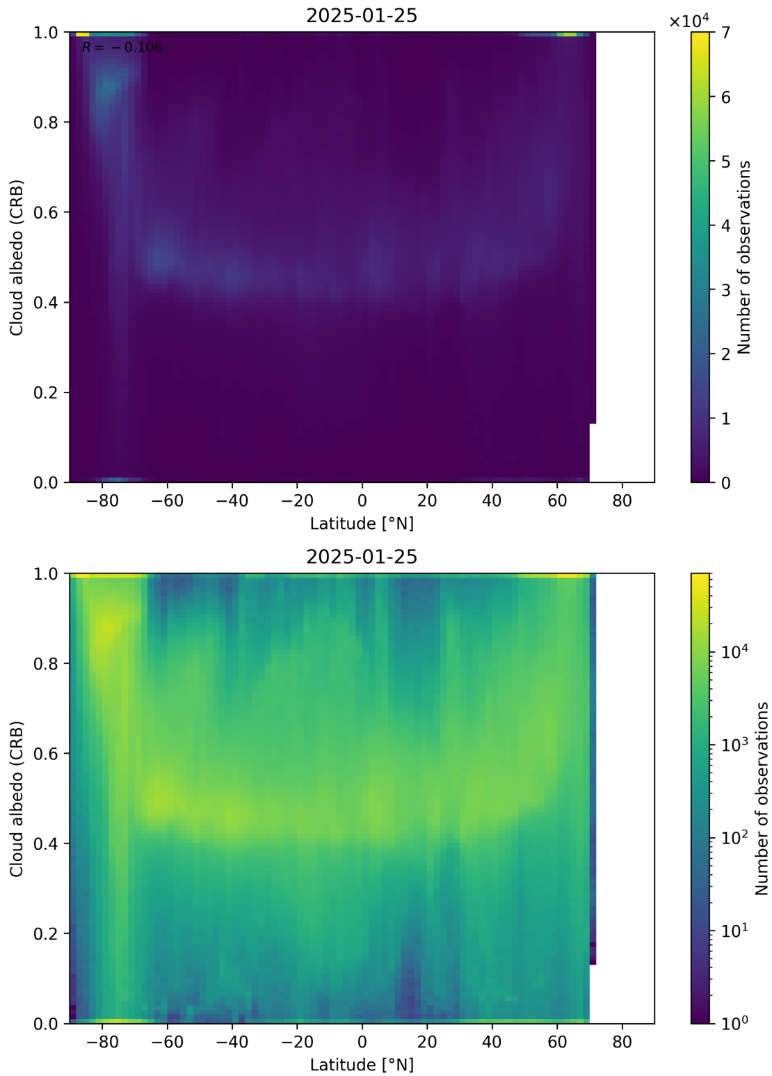
Figure 91: Scatter density plot of “Latitude” against “Cloud albedo (CRB)” for 2025-01-24 to 2025-01-26.
