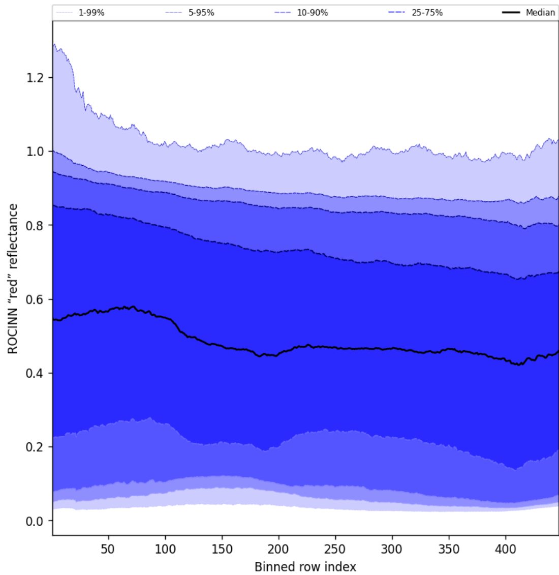
Figure 69: Along track statistics of “ROCINN “red” reflectance” for 2025-01-24 to 2025-01-26
