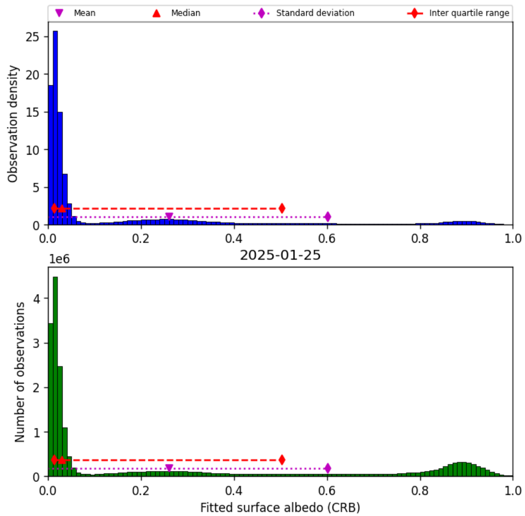
Figure 46: Histogram of “Fitted surface albedo (CRB)” for 2025-01-24 to 2025-01-26
