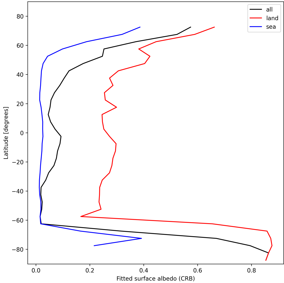
Figure 30: Zonal average of “Fitted surface albedo (CRB)” for 2025-01-24 to 2025-01-26.
