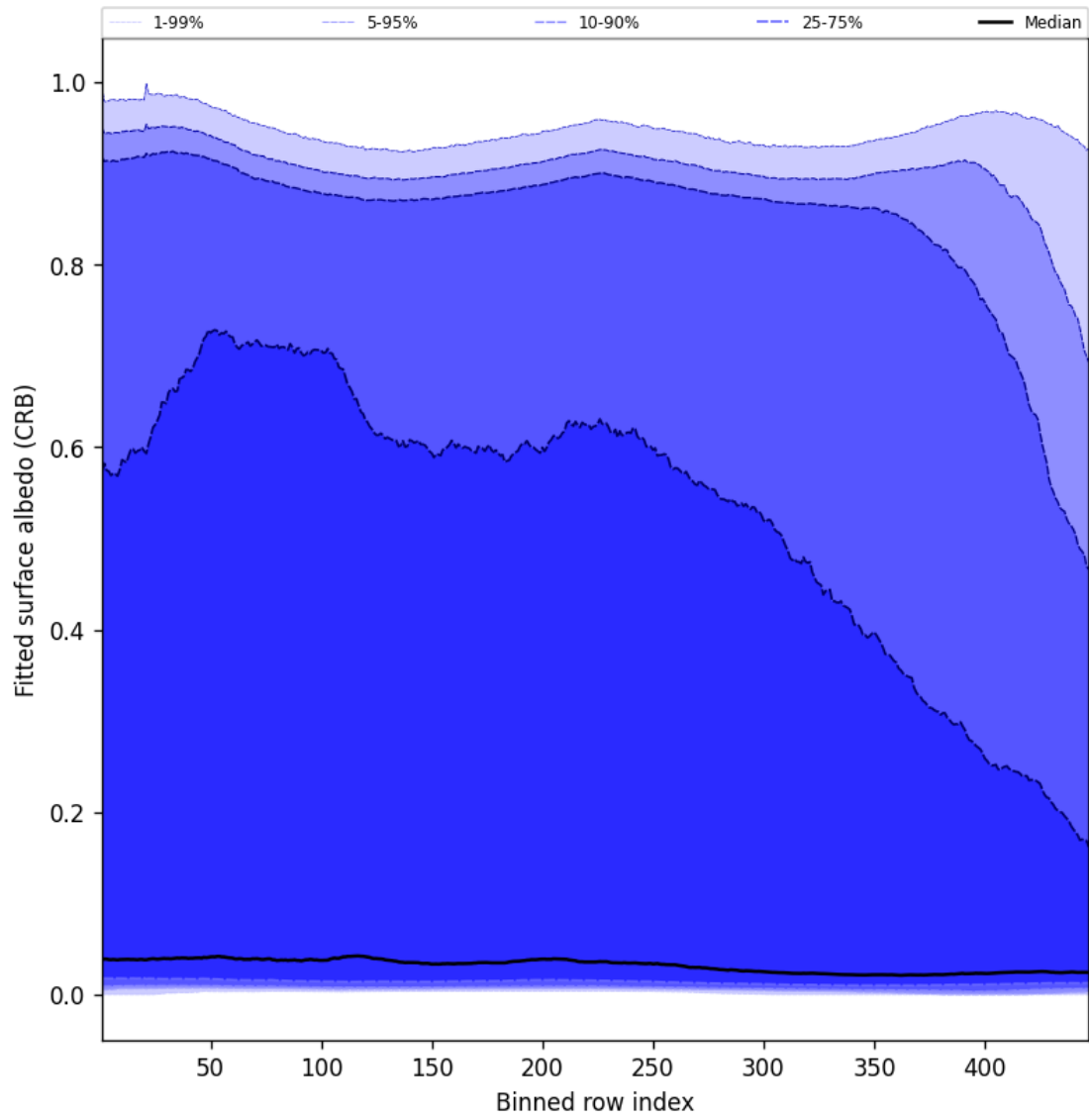
Figure 62: Along track statistics of “Fitted surface albedo (CRB)” for 2025-01-24 to 2025-01-26
