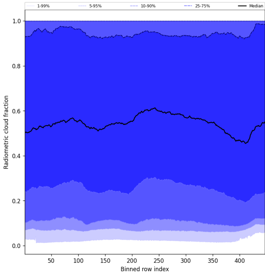
Figure 55: Along track statistics of “Radiometric cloud fraction” for 2025-01-24 to 2025-01-26
