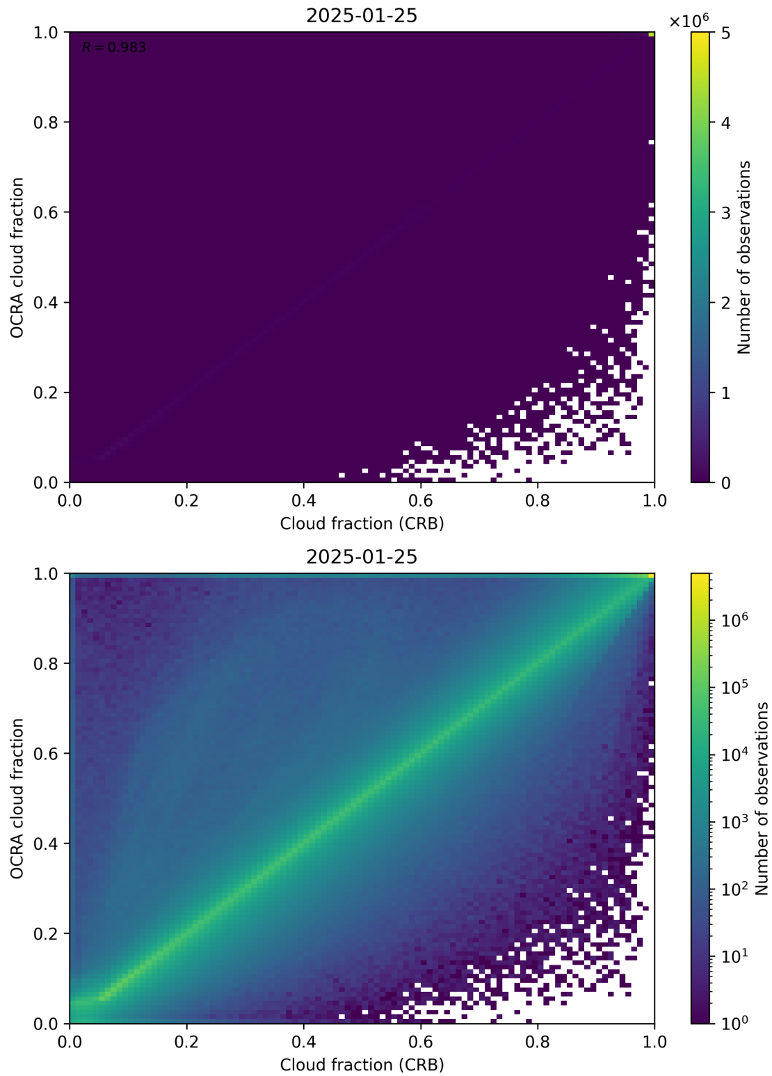
Figure 78: Scatter density plot of “Cloud fraction (CRB)” against “OCRA cloud fraction” for 2025-01-24 to 2025-01-26.
