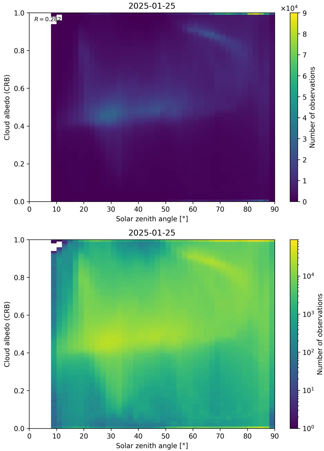
Figure 98: Scatter density plot of “Solar zenith angle” against “Cloud albedo (CRB)” for 2025-01-24 to 2025-01-26.
