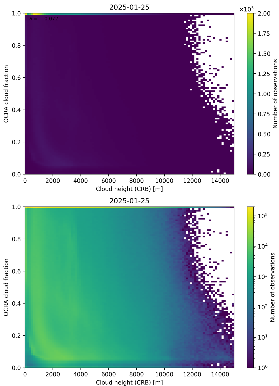
Figure 81: Scatter density plot of “Cloud height (CRB)” against “OCRA cloud fraction” for 2025-01-24 to 2025-01-26.
