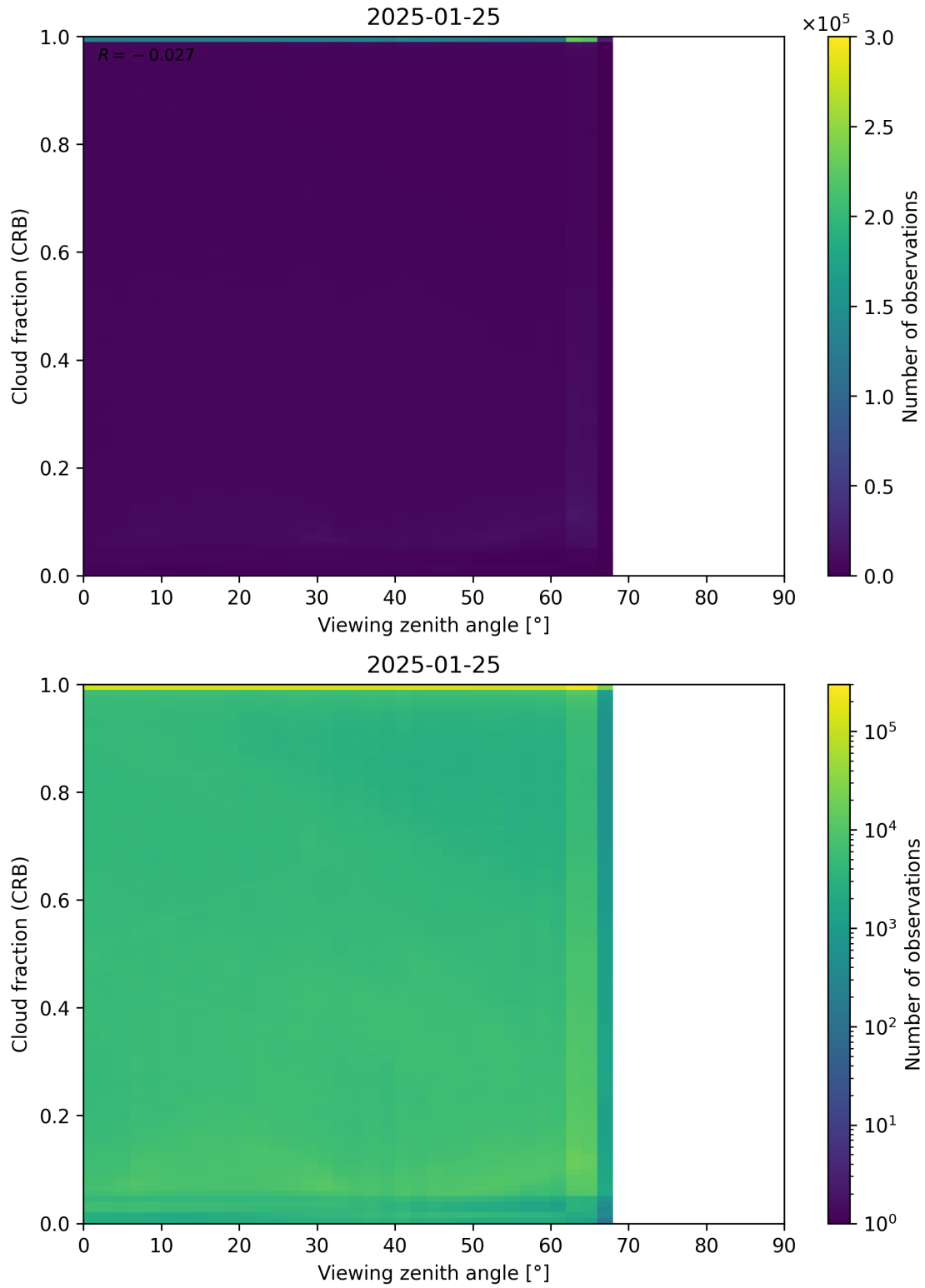
Figure 109: Scatter density plot of “Viewing zenith angle” against “Cloud fraction (CRB)” for 2025-01-24 to 2025-01-26.
