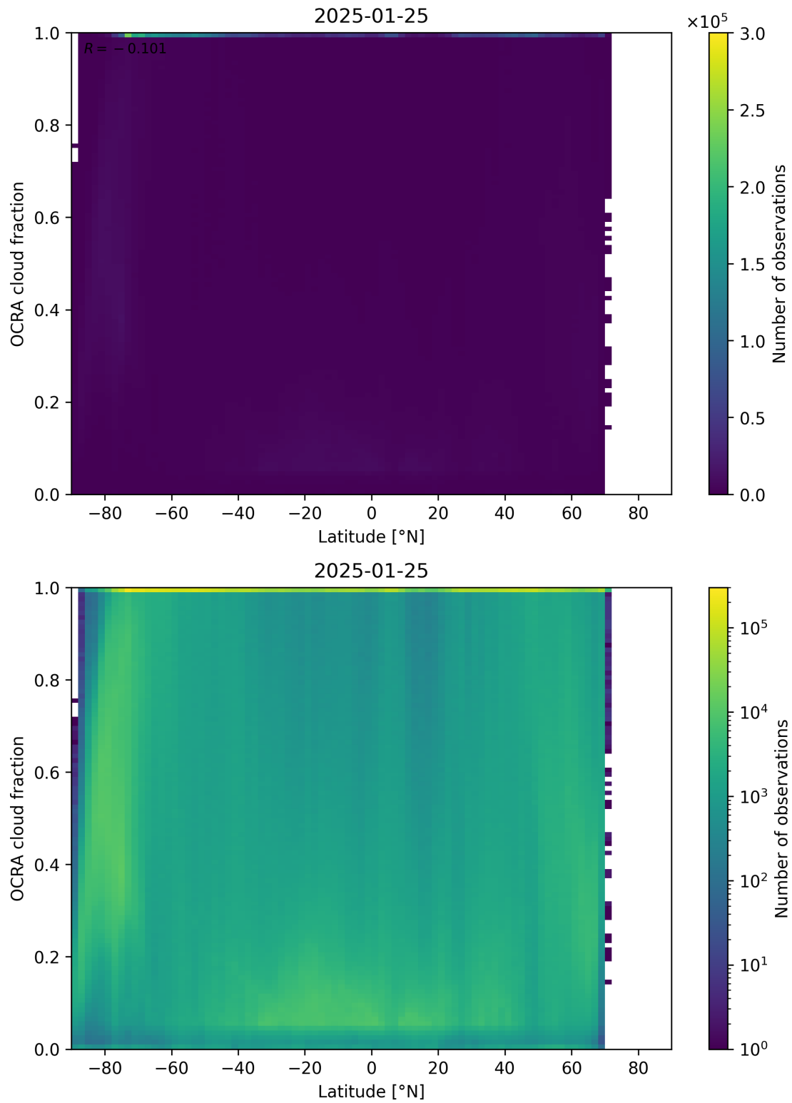
Figure 93: Scatter density plot of “Latitude” against “OCRA cloud fraction” for 2025-01-24 to 2025-01-26.
