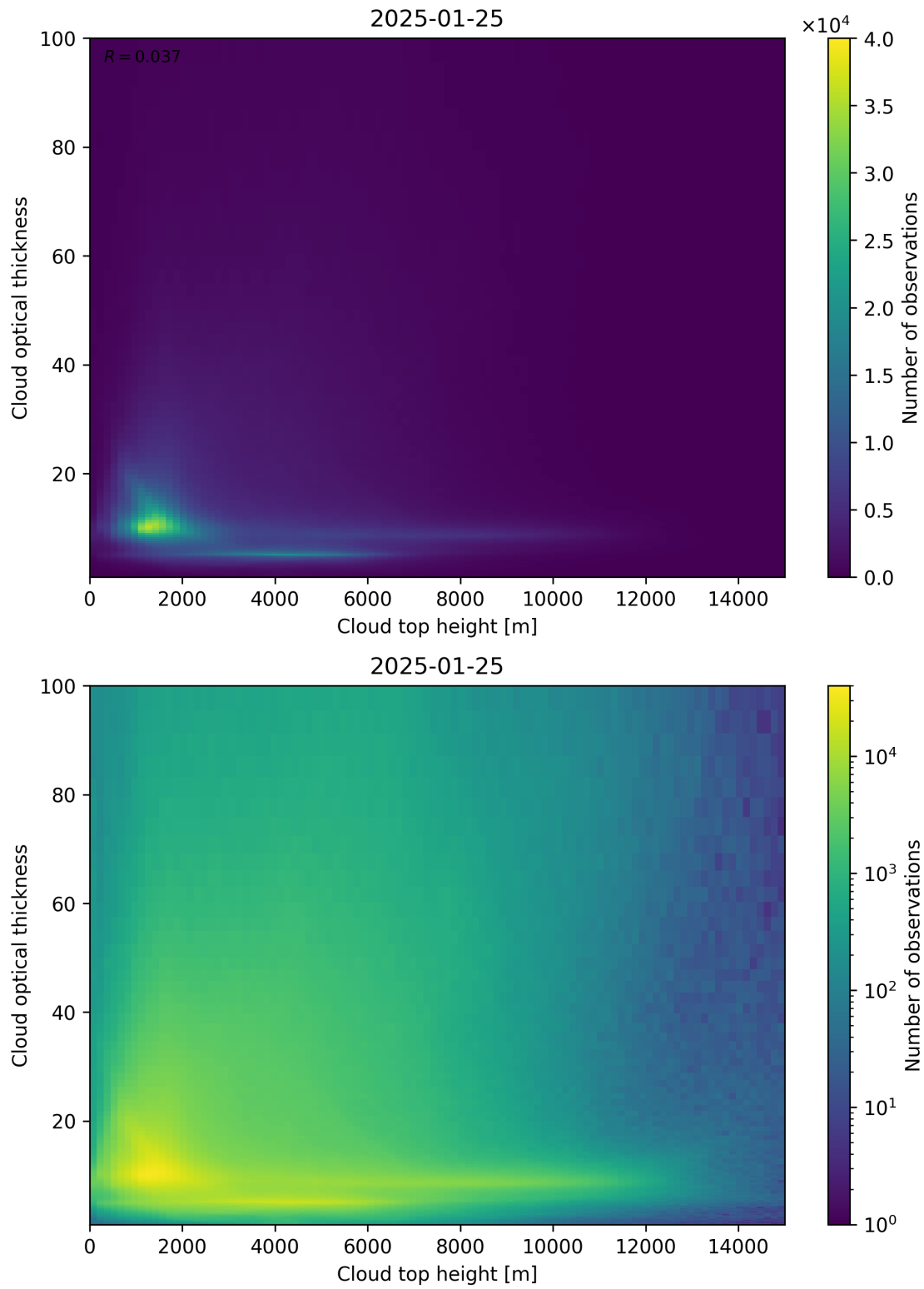
Figure 90: Scatter density plot of “Cloud top height” against “Cloud optical thickness” for 2025-01-24 to 2025-01-26.
