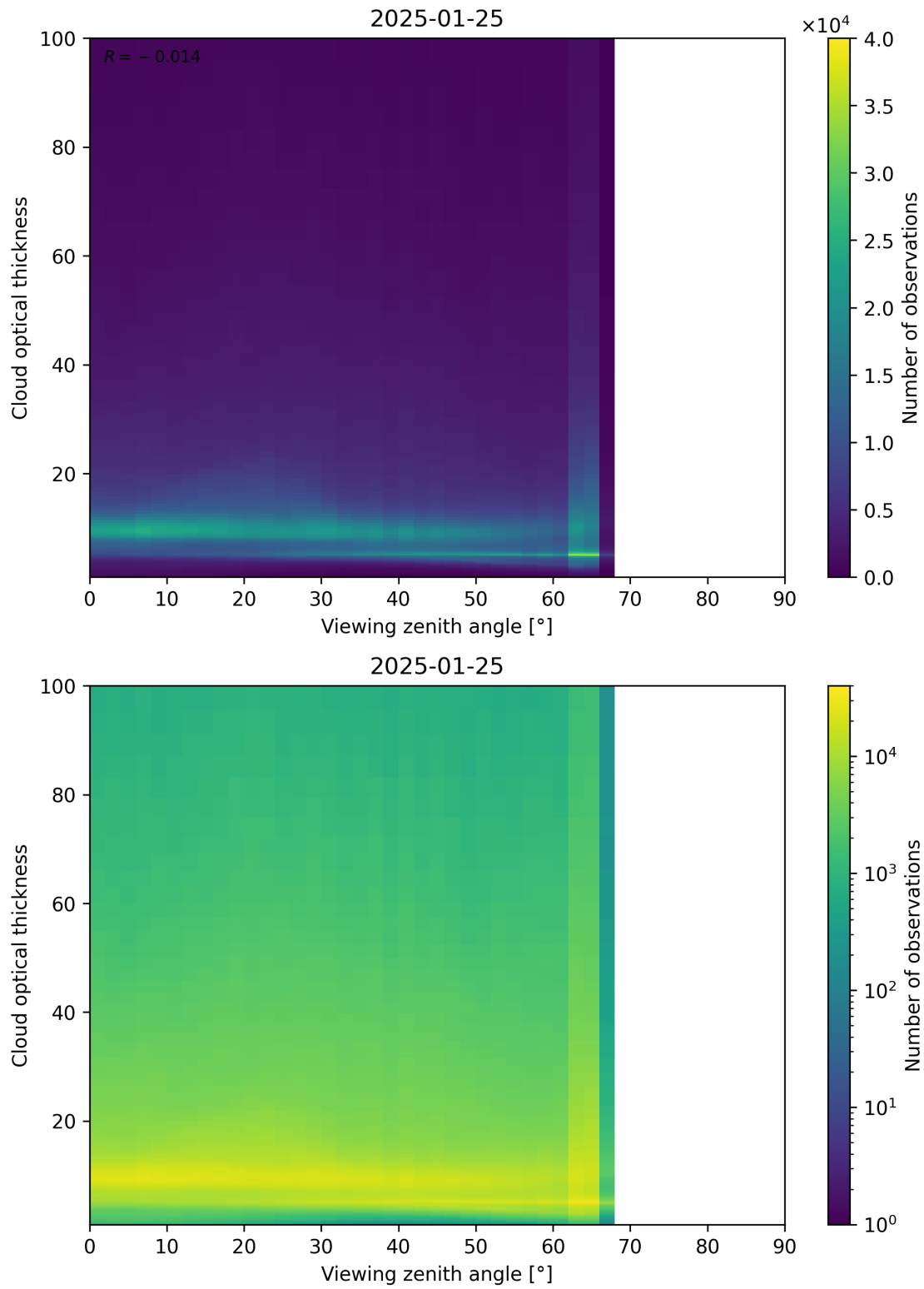
Figure 111: Scatter density plot of “Viewing zenith angle” against “Cloud optical thickness” for 2025-01-24 to 2025-01-26.
