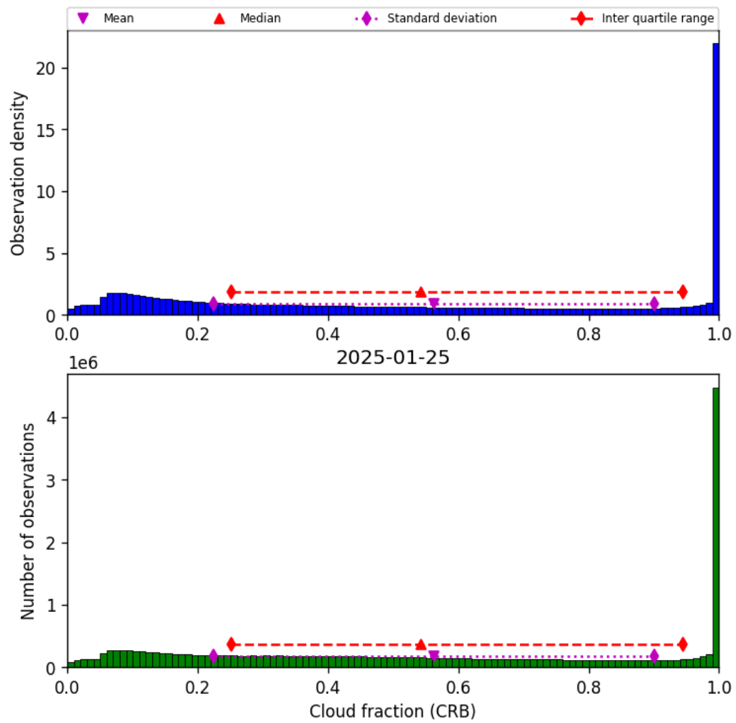
Figure 42: Histogram of “Cloud fraction (CRB)” for 2025-01-24 to 2025-01-26
