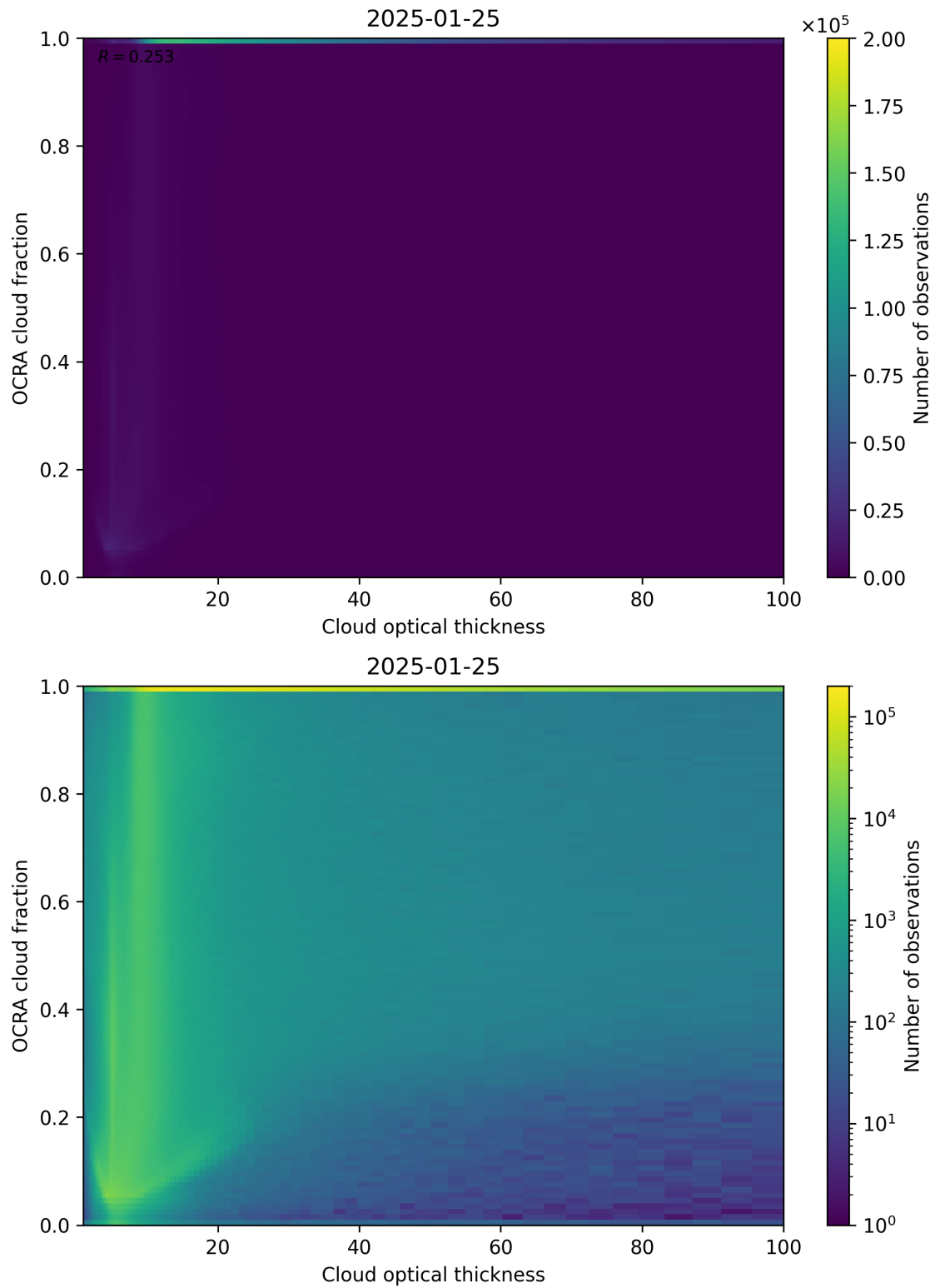
Figure 83: Scatter density plot of “Cloud optical thickness” against “OCRA cloud fraction” for 2025-01-24 to 2025-01-26.
