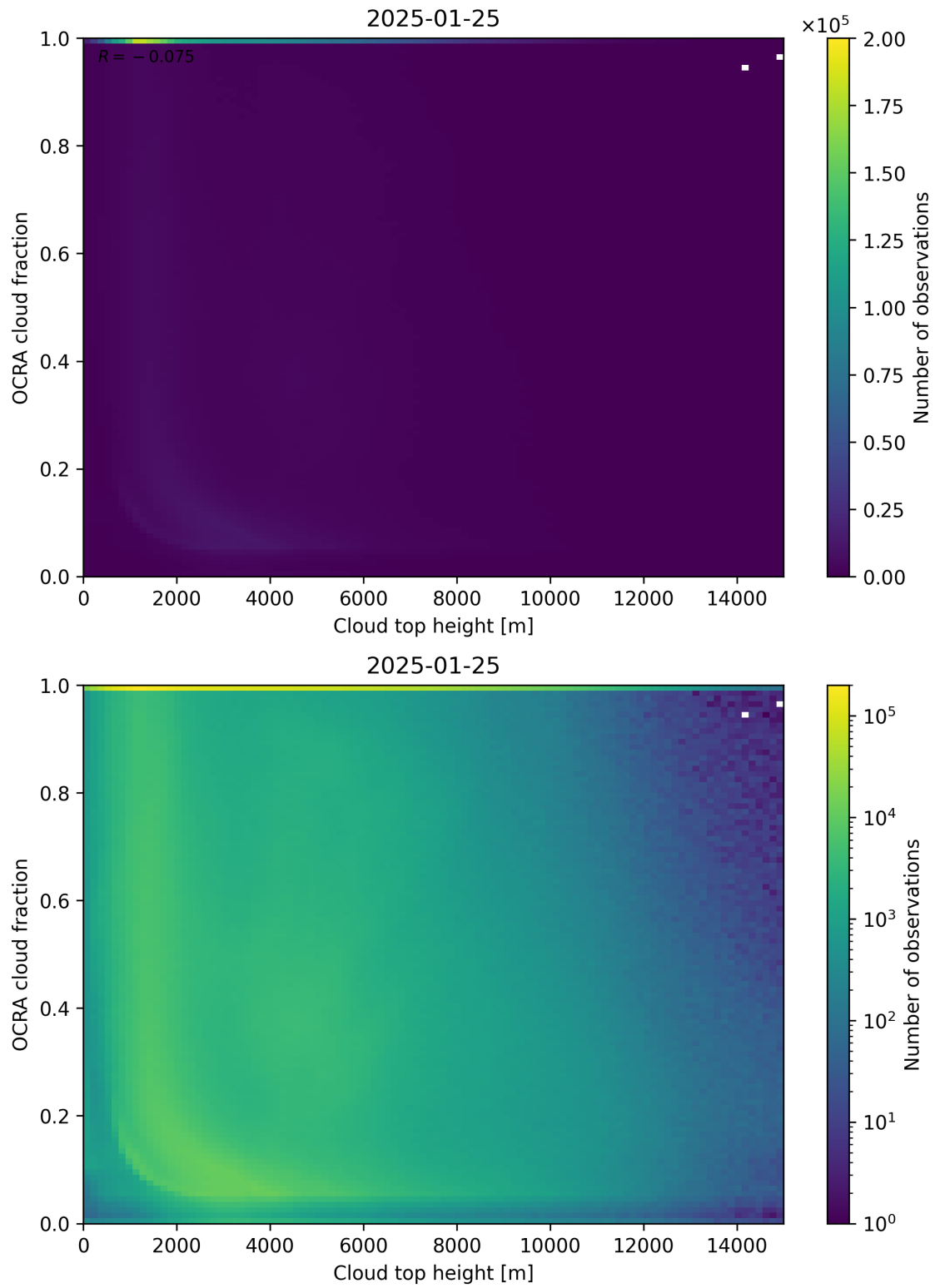
Figure 87: Scatter density plot of “Cloud top height” against “OCRA cloud fraction” for 2025-01-24 to 2025-01-26.
