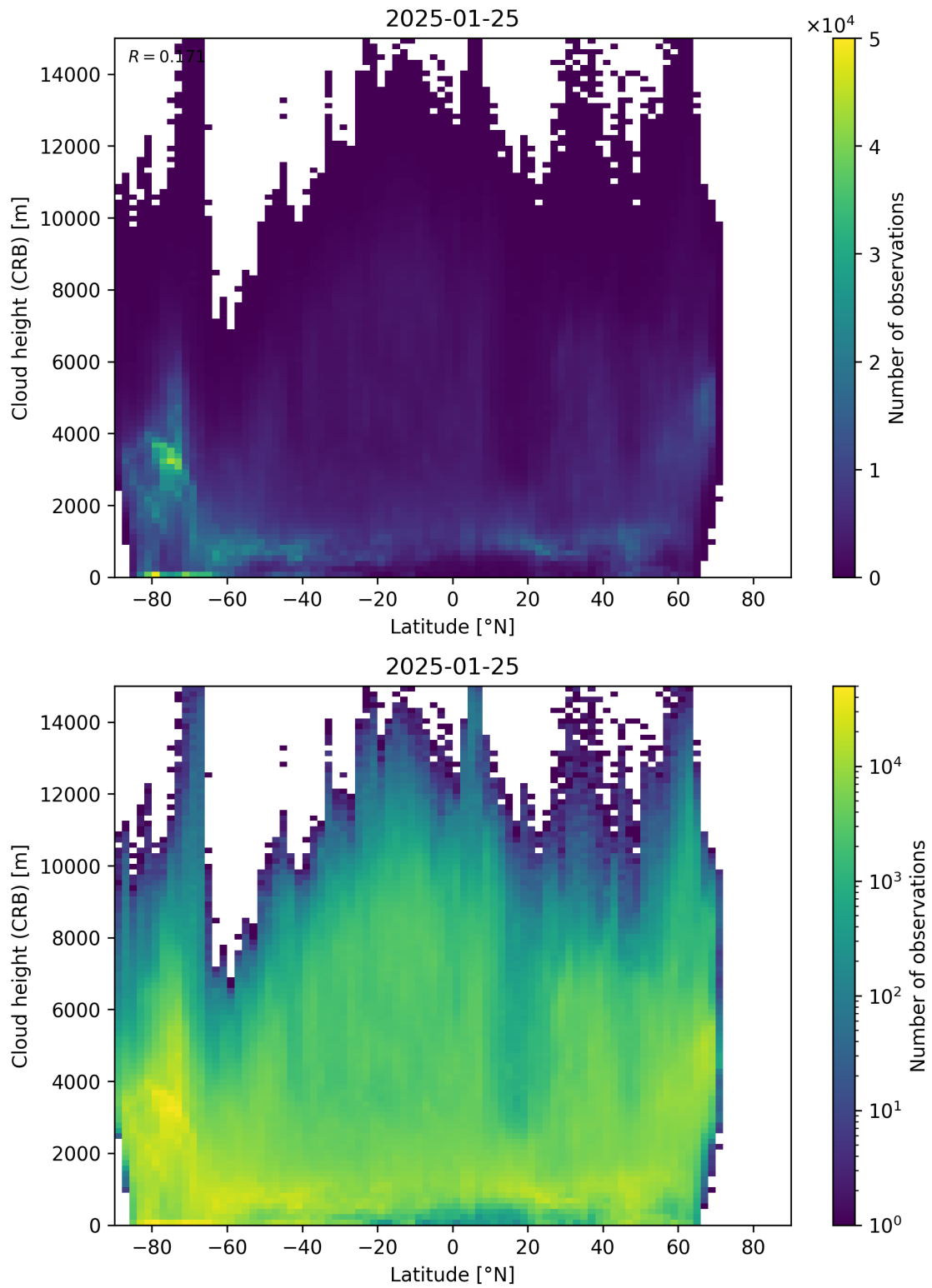
Figure 95: Scatter density plot of “Latitude” against “Cloud height (CRB)” for 2025-01-24 to 2025-01-26.
