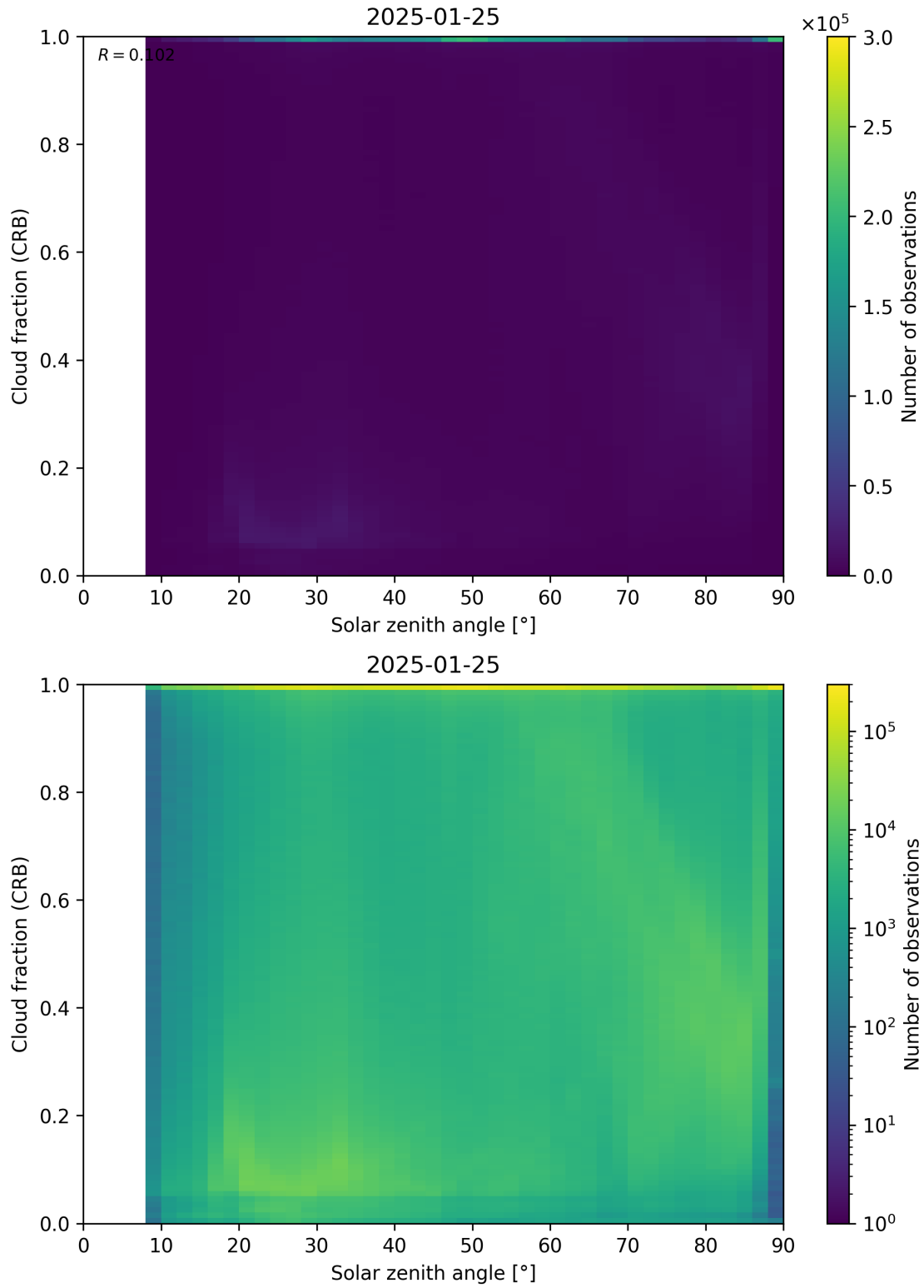
Figure 101: Scatter density plot of “Solar zenith angle” against “Cloud fraction (CRB)” for 2025-01-24 to 2025-01-26.
