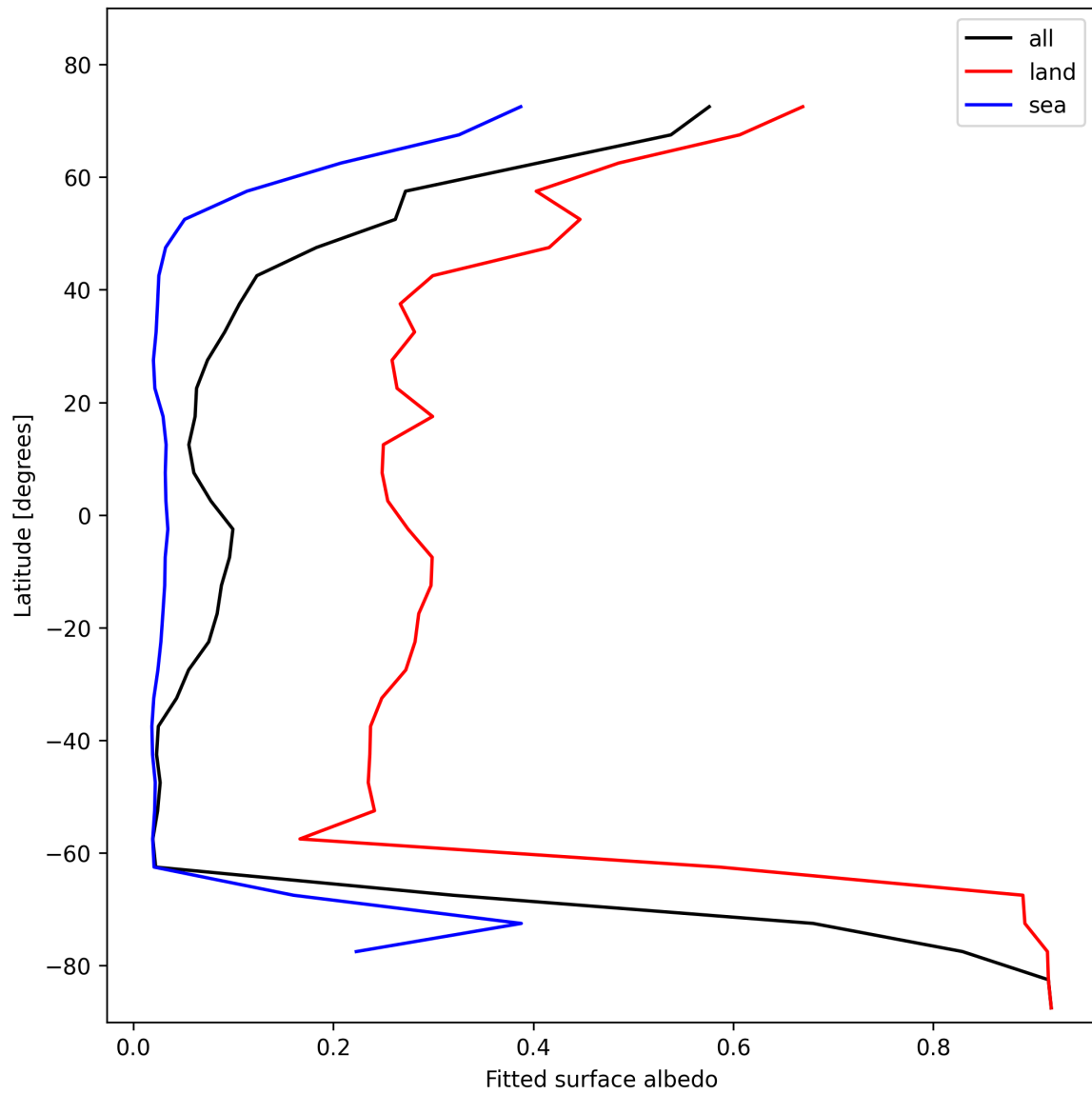
Figure 29: Zonal average of “Fitted surface albedo” for 2025-01-24 to 2025-01-26.
