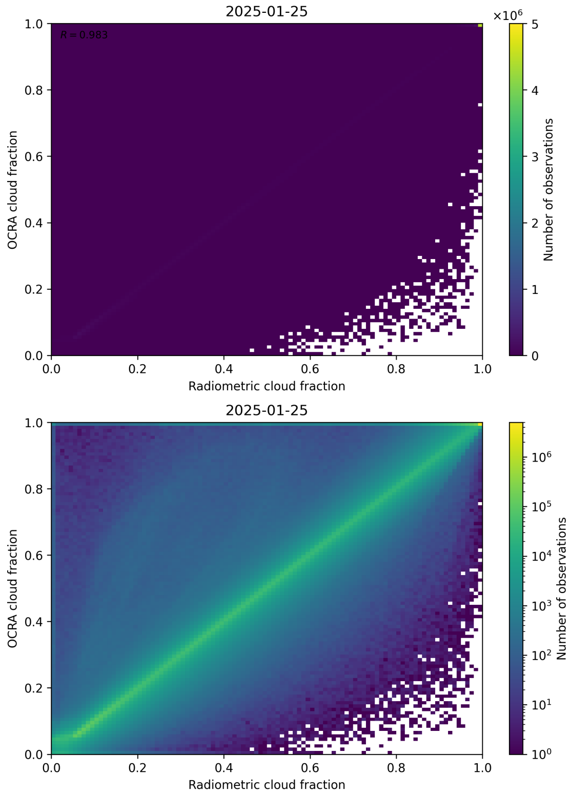
Figure 72: Scatter density plot of “Radiometric cloud fraction” against “OCRA cloud fraction” for 2025-01-24 to 2025-01-26.
