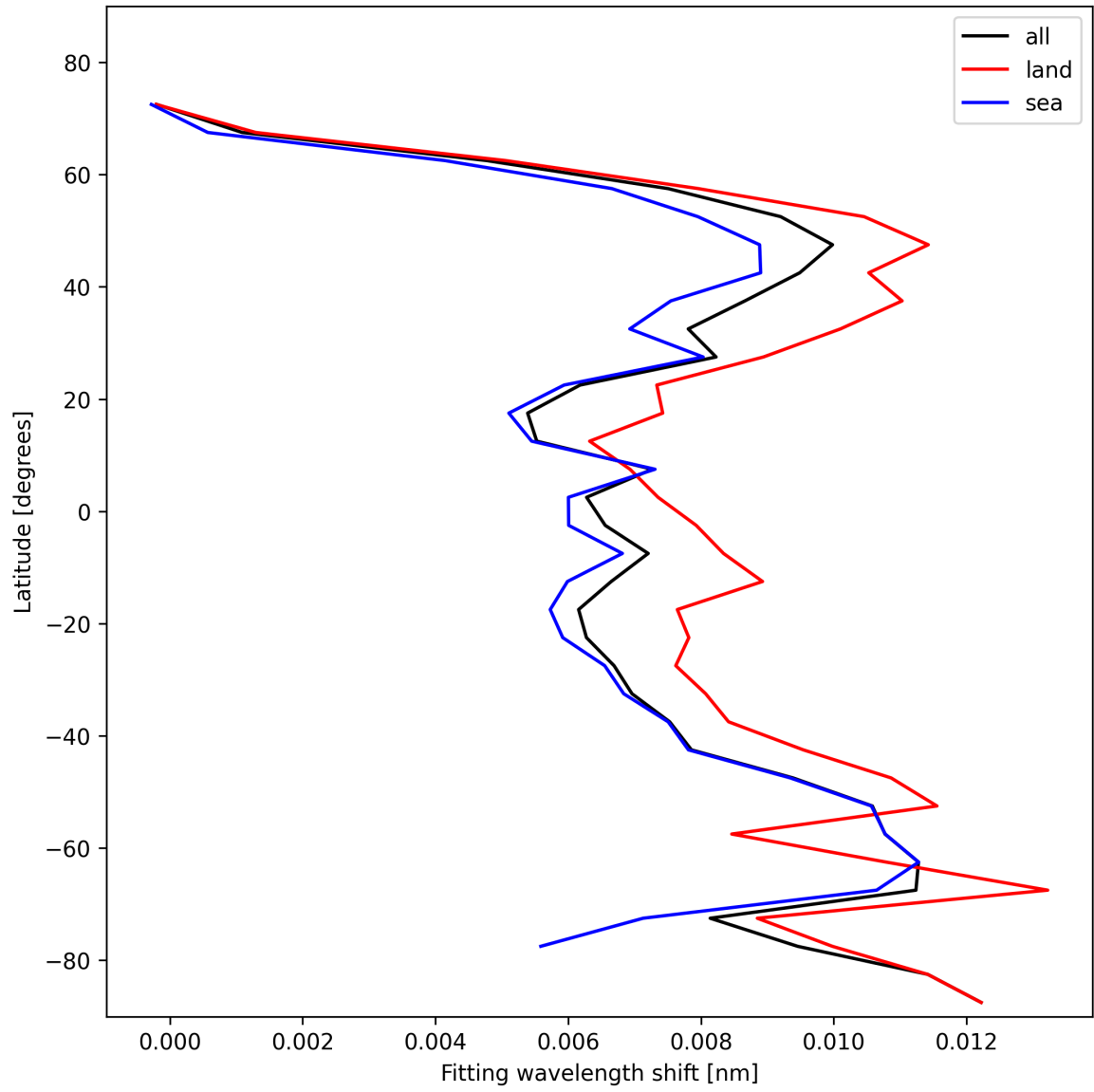
Figure 33: Zonal average of “Fitting wavelength shift” for 2025-01-24 to 2025-01-26.
