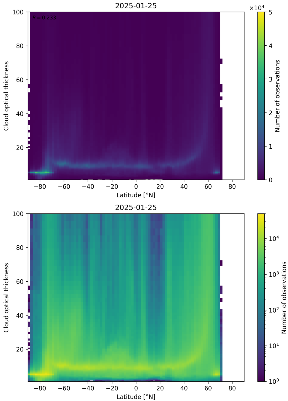
Figure 96: Scatter density plot of “Latitude” against “Cloud optical thickness” for 2025-01-24 to 2025-01-26.
