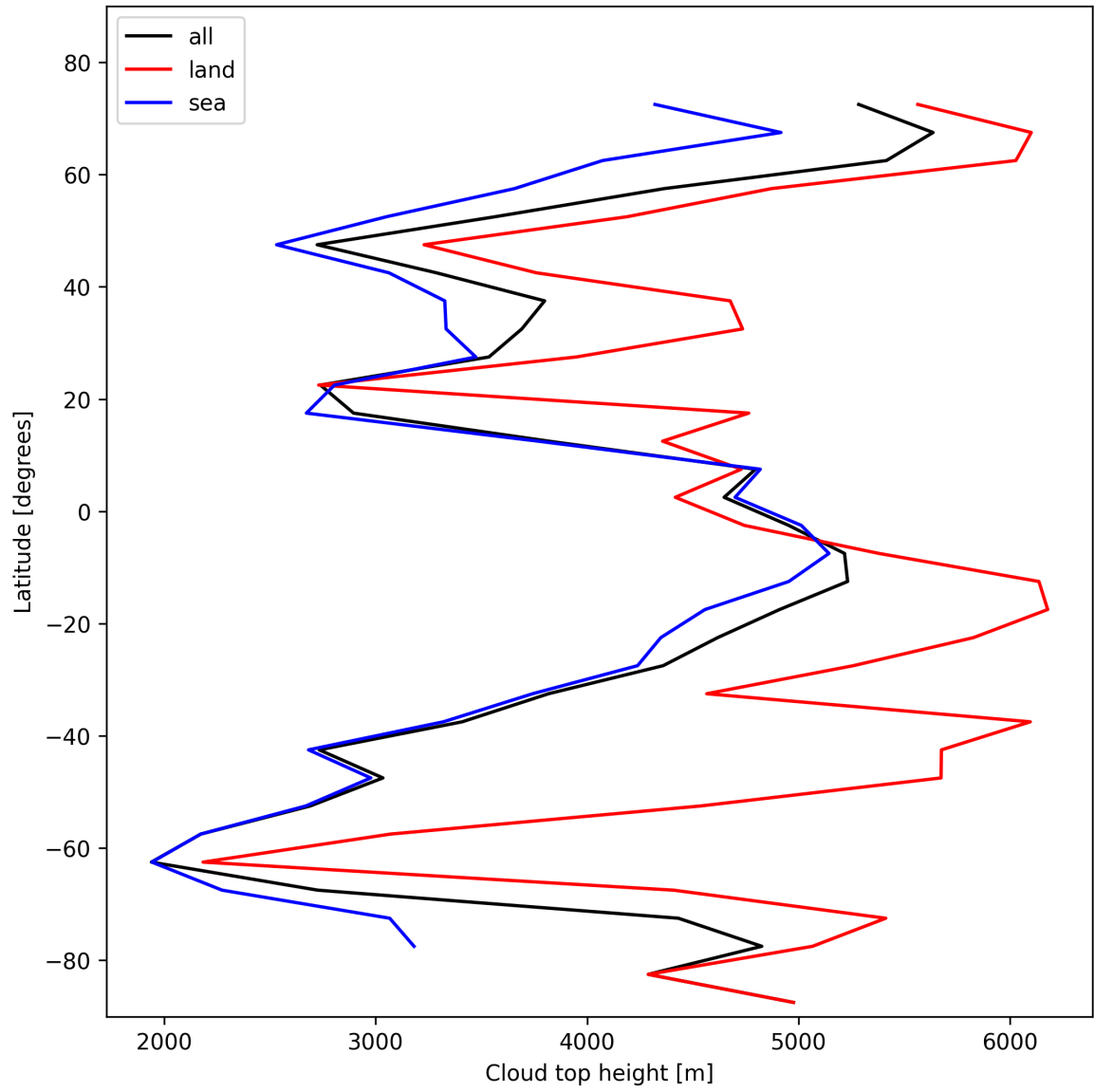
Figure 24: Zonal average of “Cloud top height” for 2025-01-24 to 2025-01-26.
