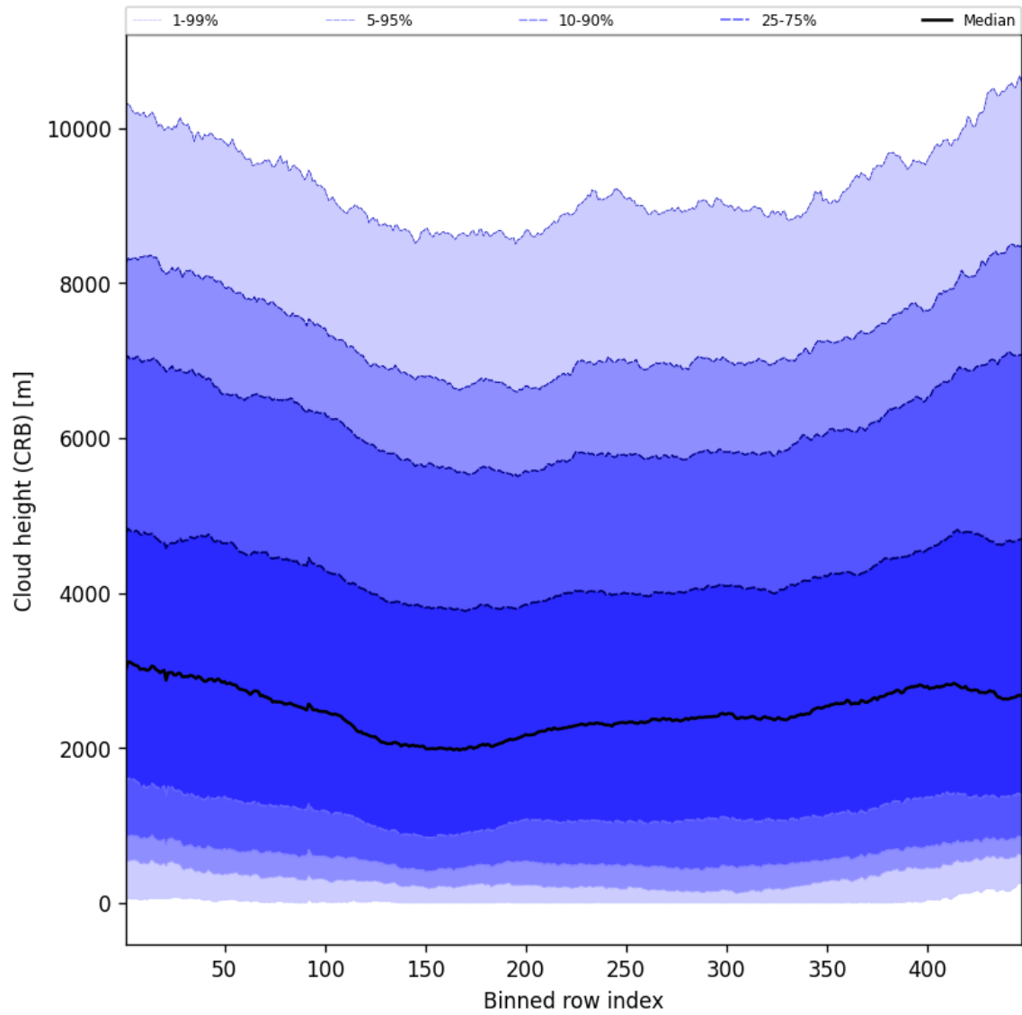
Figure 59: Along track statistics of “Cloud height (CRB)” for 2025-01-24 to 2025-01-26
