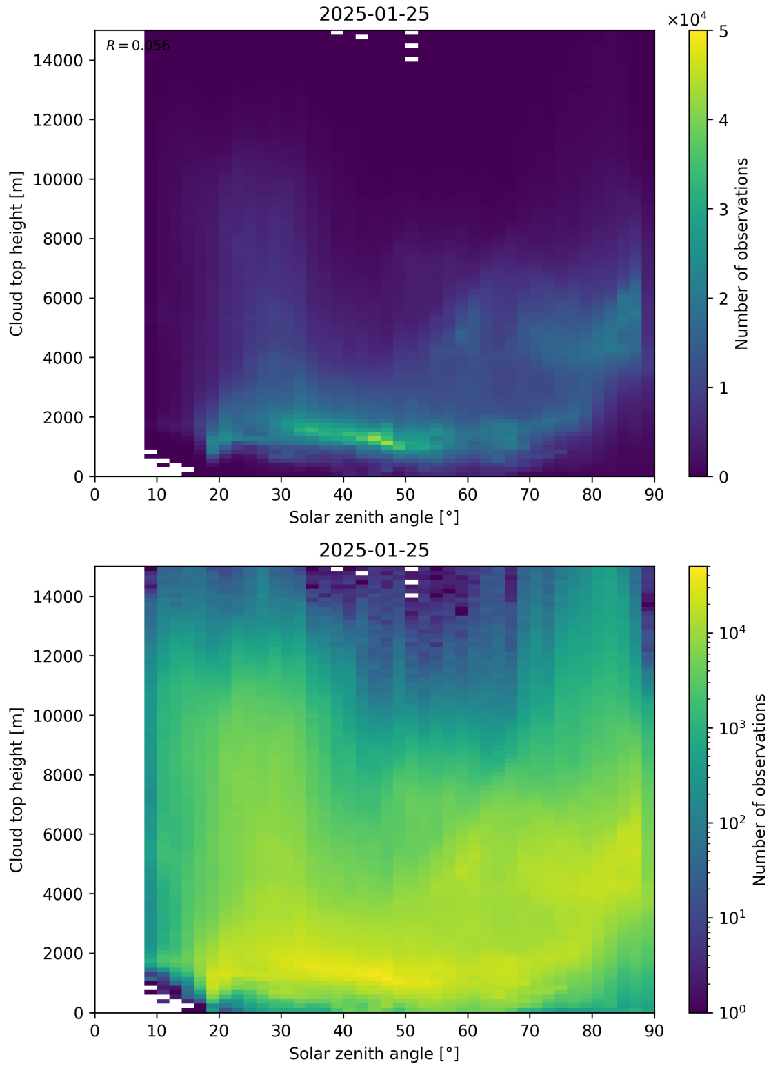
Figure 104: Scatter density plot of “Solar zenith angle” against “Cloud top height” for 2025-01-24 to 2025-01-26.
