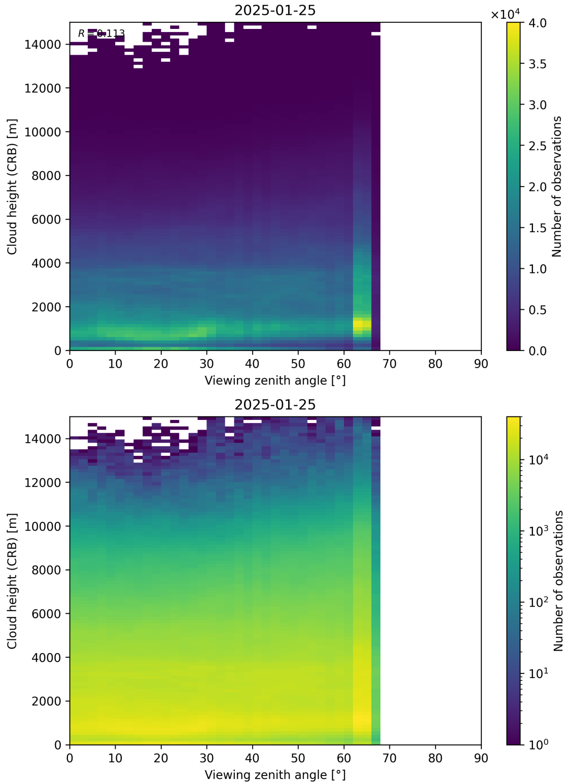
Figure 110: Scatter density plot of “Viewing zenith angle” against “Cloud height (CRB)” for 2025-01-24 to 2025-01-26.
