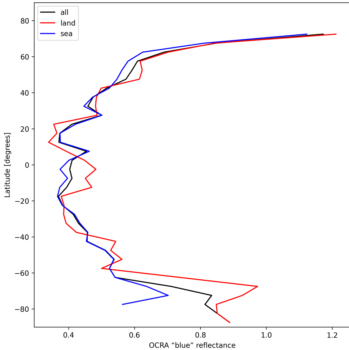
Figure 35: Zonal average of “OCRA “blue” reflectance” for 2025-01-24 to 2025-01-26.
