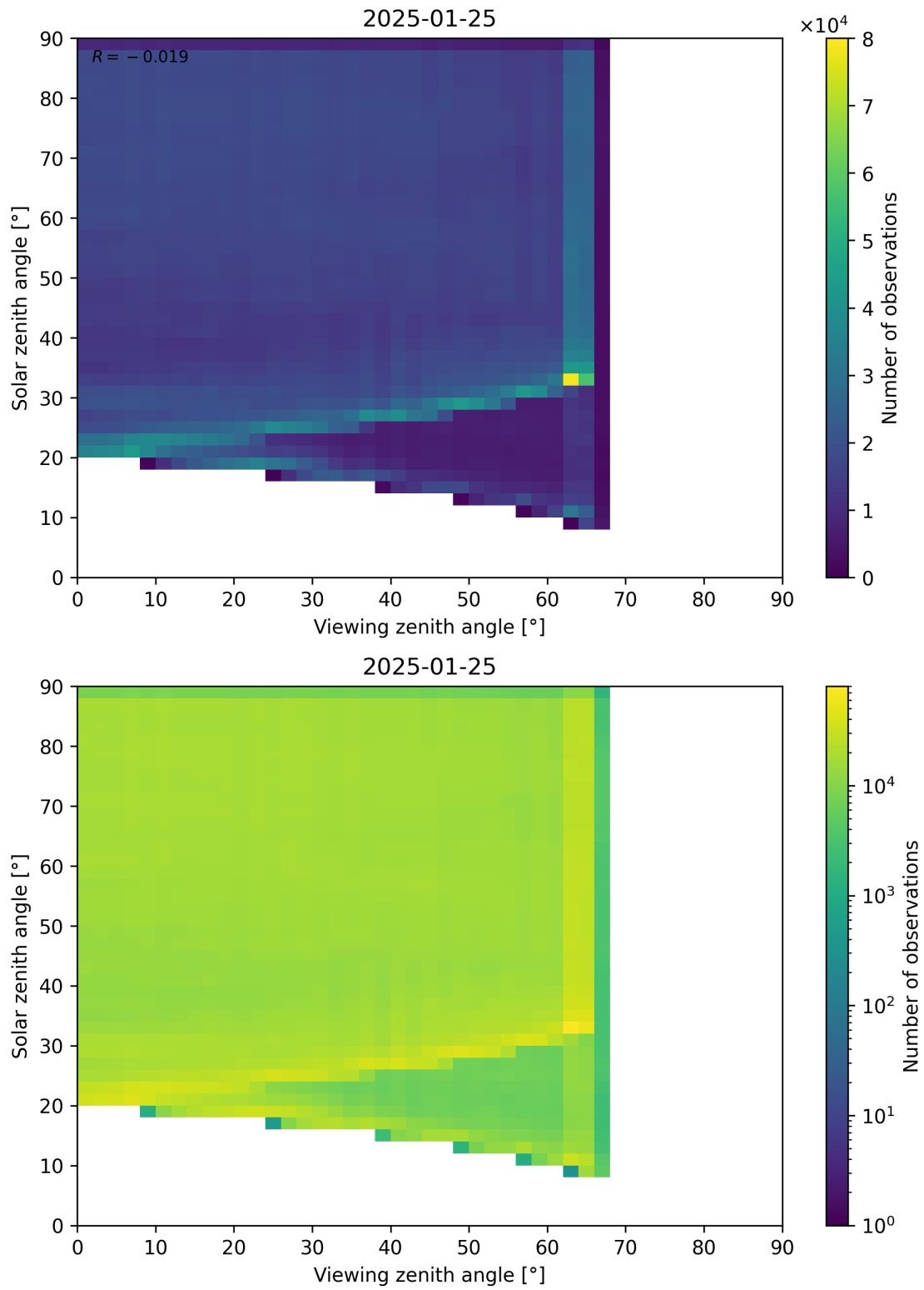
Figure 114: Scatter density plot of “Viewing zenith angle” against “Solar zenith angle” for 2025-01-24 to 2025-01-26.
