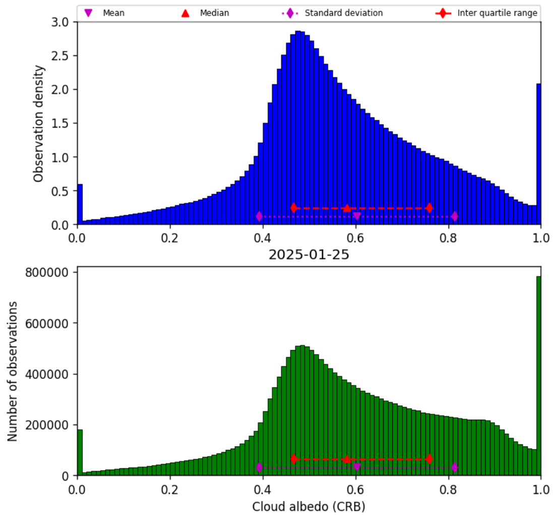
Figure 44: Histogram of “Cloud albedo (CRB)” for 2025-01-24 to 2025-01-26
