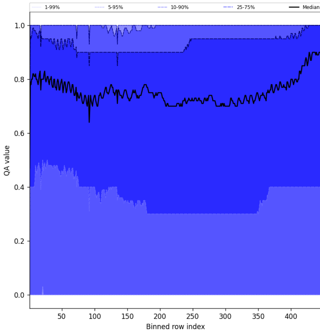
Figure 54: Along track statistics of “QA value” for 2025-01-24 to 2025-01-26
