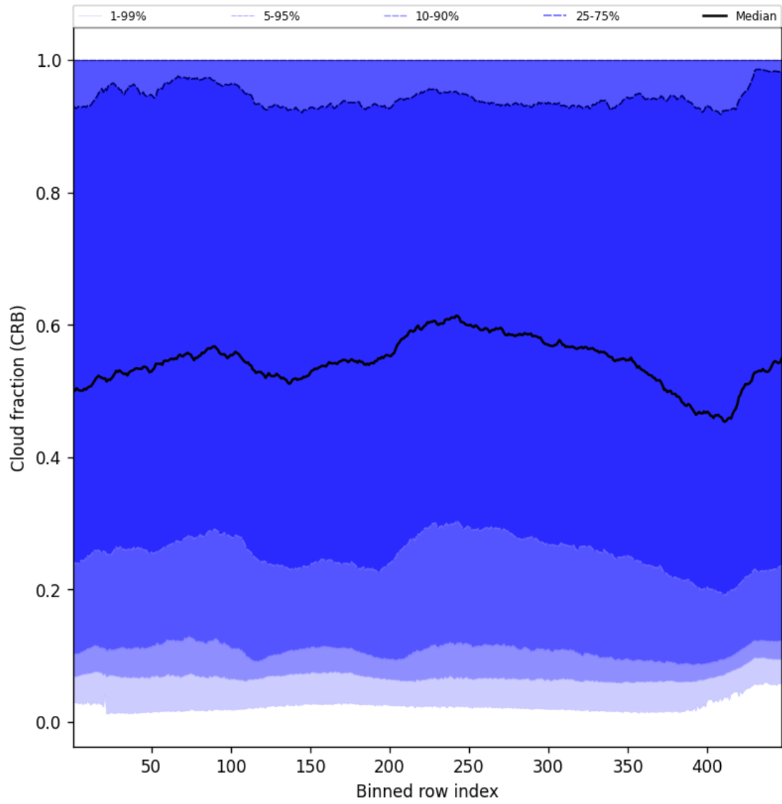
Figure 58: Along track statistics of “Cloud fraction (CRB)” for 2025-01-24 to 2025-01-26
