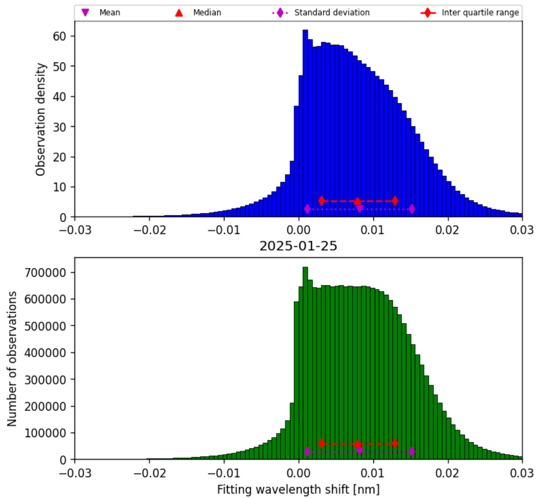
Figure 49: Histogram of “Fitting wavelength shift” for 2025-01-24 to 2025-01-26
