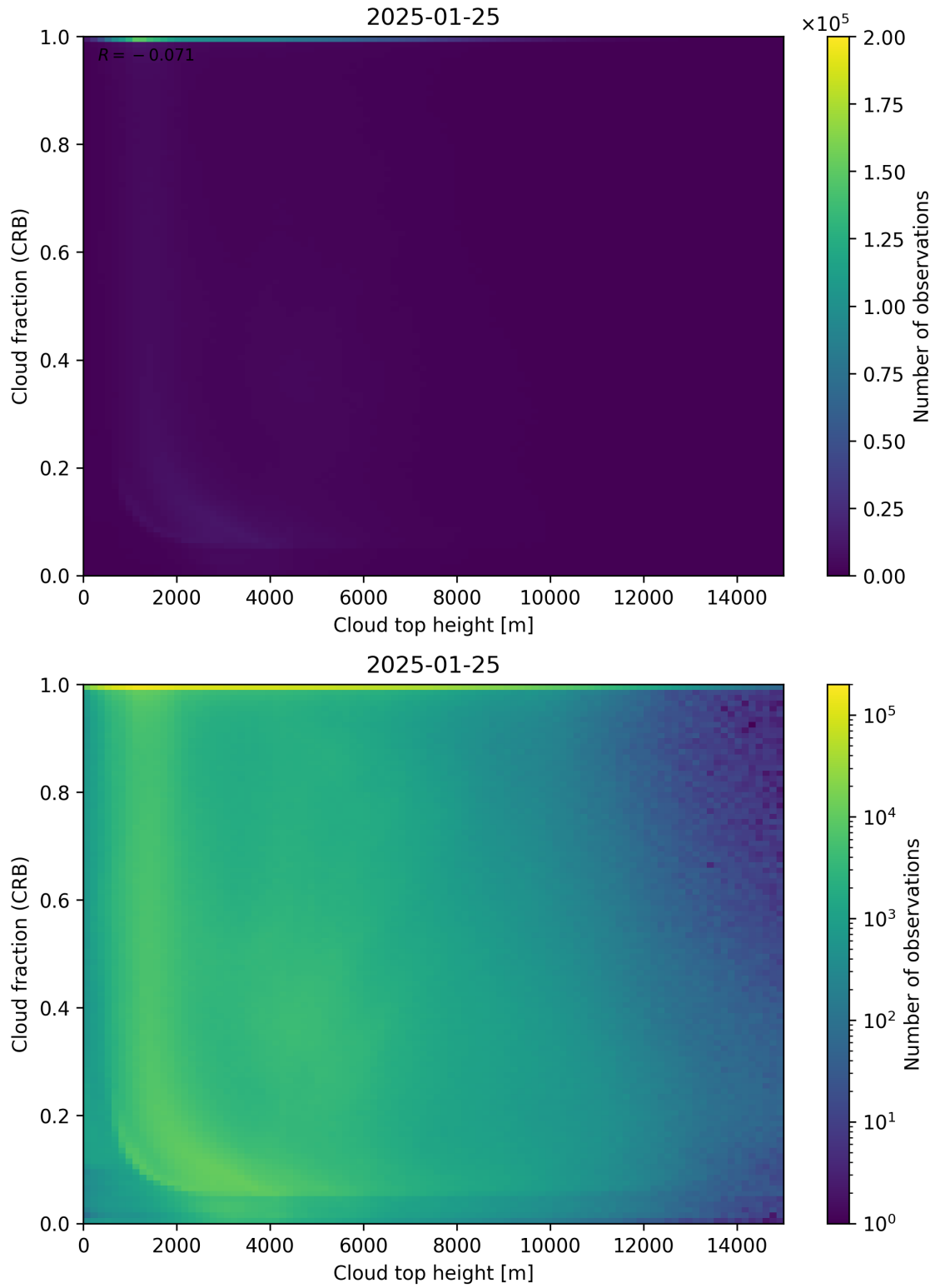
Figure 88: Scatter density plot of “Cloud top height” against “Cloud fraction (CRB)” for 2025-01-24 to 2025-01-26.
