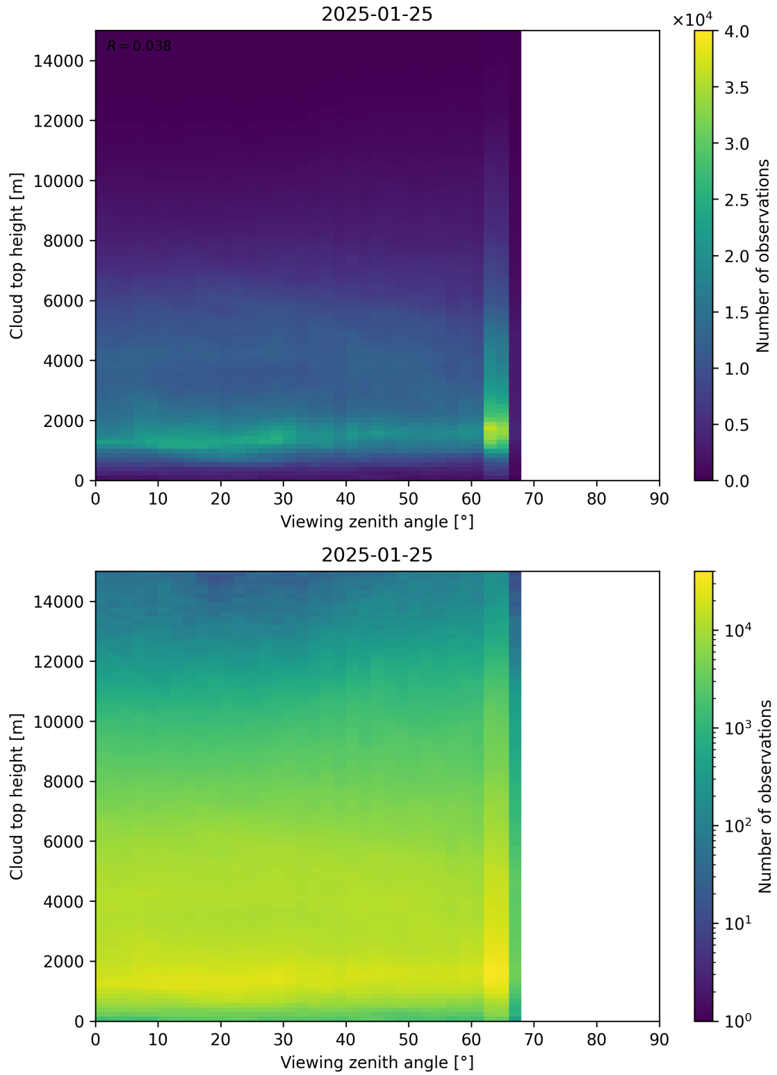
Figure 112: Scatter density plot of “Viewing zenith angle” against “Cloud top height” for 2025-01-24 to 2025-01-26.
