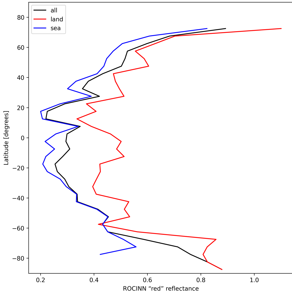
Figure 37: Zonal average of “ROCINN “red” reflectance” for 2025-01-24 to 2025-01-26.
