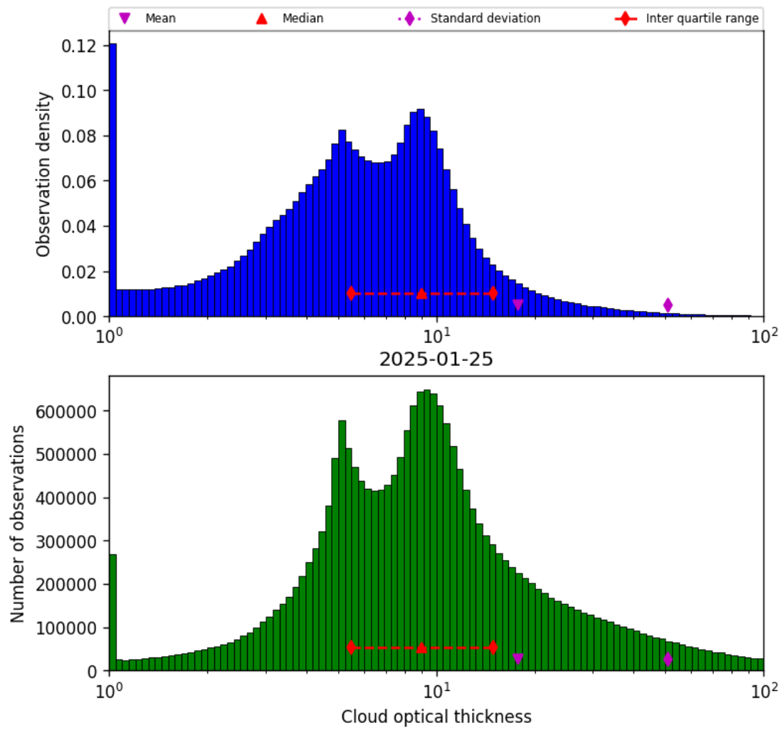
Figure 41: Histogram of “Cloud optical thickness” for 2025-01-24 to 2025-01-26
