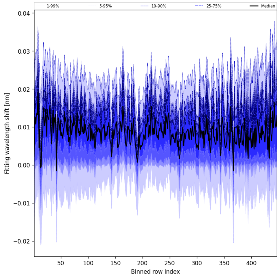
Figure 65: Along track statistics of “Fitting wavelength shift” for 2025-01-24 to 2025-01-26
