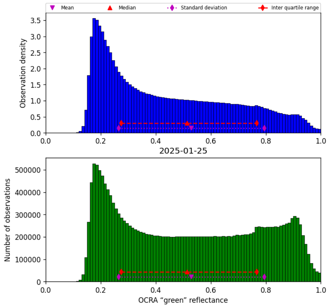
Figure 52: Histogram of “OCRA “green” reflectance” for 2025-01-24 to 2025-01-26
