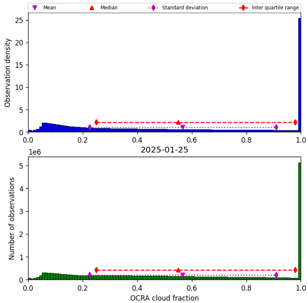
Figure 50: Histogram of “OCRA cloud fraction” for 2025-01-24 to 2025-01-26
