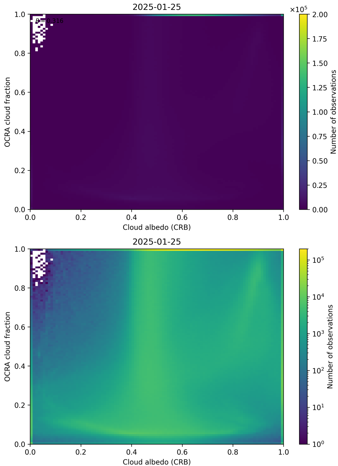
Figure 70: Scatter density plot of “Cloud albedo (CRB)” against “OCRA cloud fraction” for 2025-01-24 to 2025-01-26.
