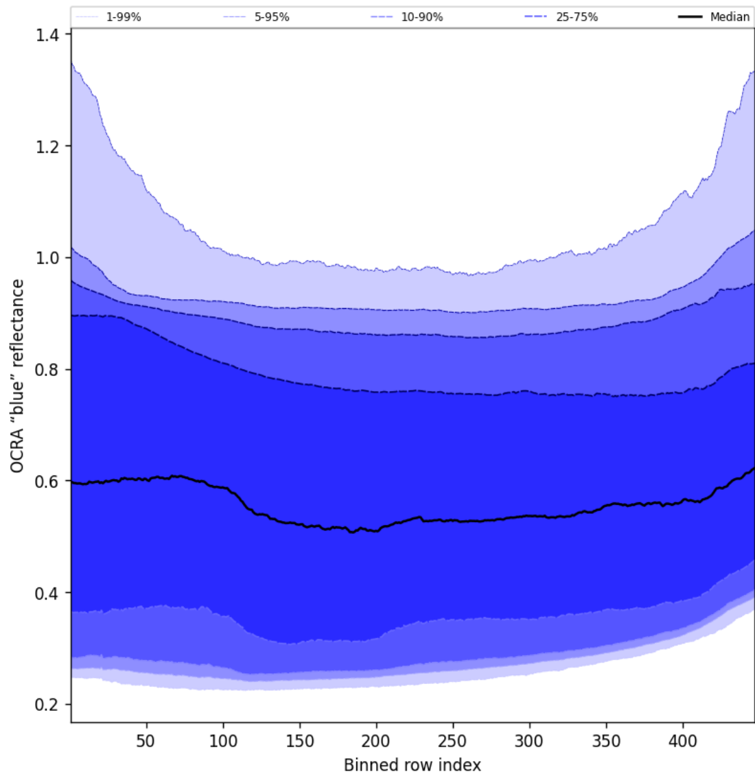
Figure 67: Along track statistics of “OCRA “blue” reflectance” for 2025-01-24 to 2025-01-26
