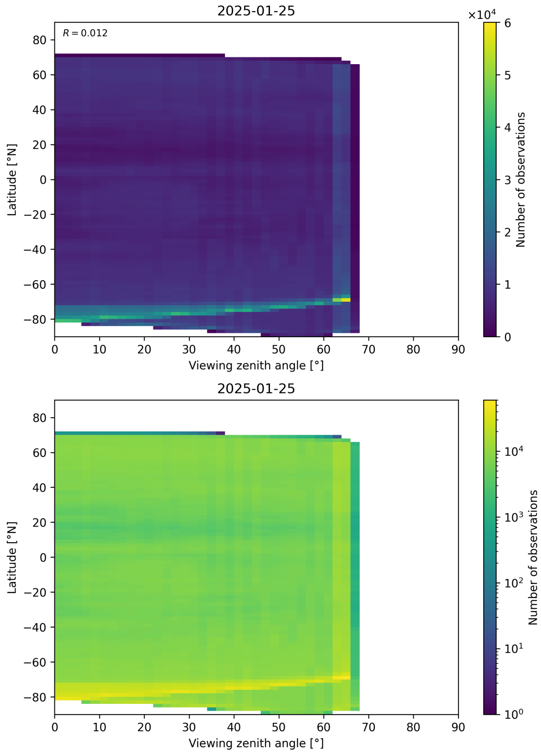
Figure 113: Scatter density plot of “Viewing zenith angle” against “Latitude” for 2025-01-24 to 2025-01-26.
