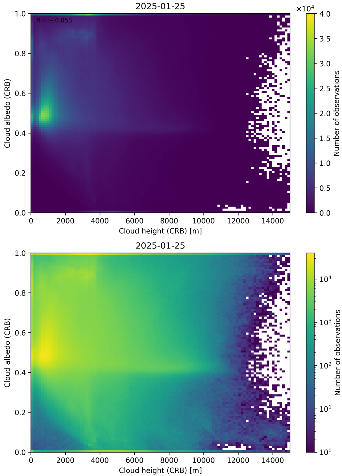
Figure 80: Scatter density plot of “Cloud height (CRB)” against “Cloud albedo (CRB)” for 2025-01-24 to 2025-01-26.
