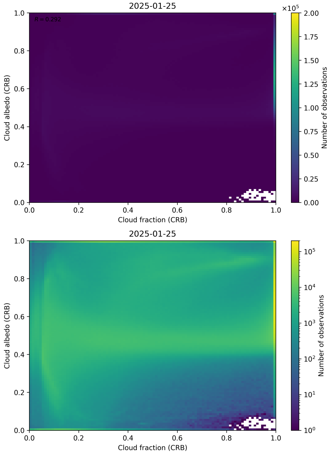
Figure 77: Scatter density plot of “Cloud fraction (CRB)” against “Cloud albedo (CRB)” for 2025-01-24 to 2025-01-26.
