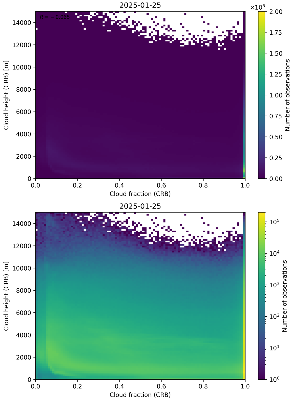
Figure 79: Scatter density plot of “Cloud fraction (CRB)” against “Cloud height (CRB)” for 2025-01-24 to 2025-01-26.
