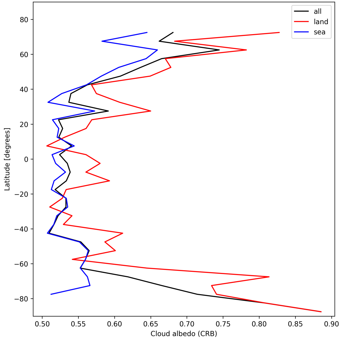
Figure 28: Zonal average of “Cloud albedo (CRB)” for 2025-01-24 to 2025-01-26.
