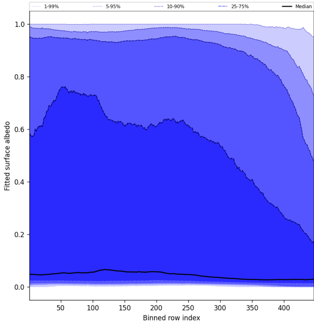
Figure 61: Along track statistics of “Fitted surface albedo” for 2025-01-24 to 2025-01-26
