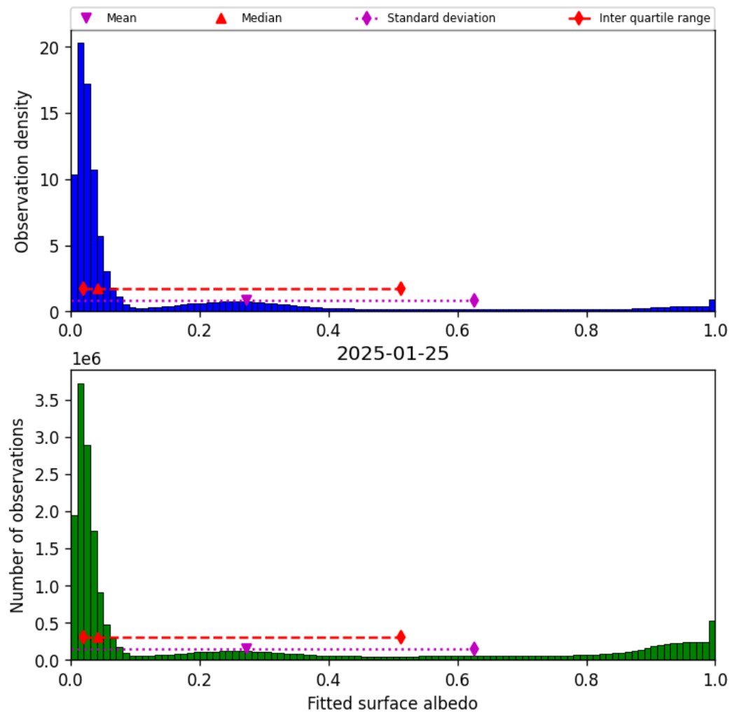
Figure 45: Histogram of “Fitted surface albedo” for 2025-01-24 to 2025-01-26
