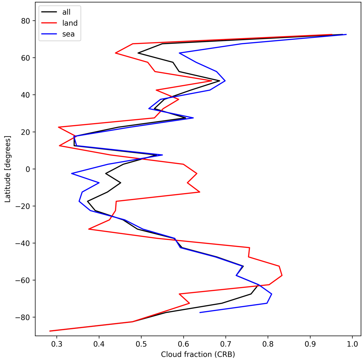
Figure 26: Zonal average of “Cloud fraction (CRB)” for 2025-01-24 to 2025-01-26.
