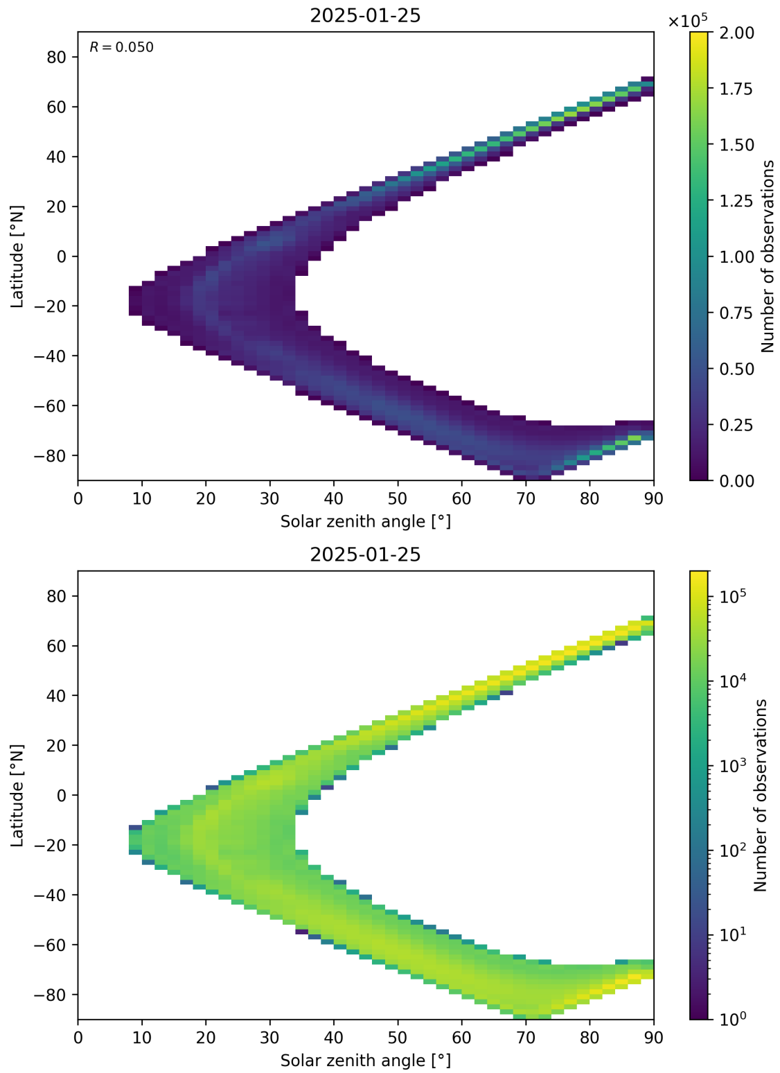
Figure 105: Scatter density plot of “Solar zenith angle” against “Latitude” for 2025-01-24 to 2025-01-26.
