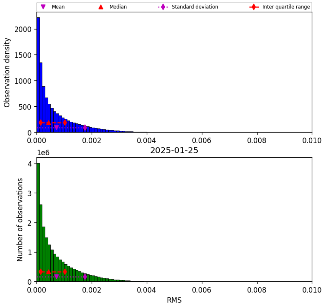
Figure 47: Histogram of “RMS” for 2025-01-24 to 2025-01-26
