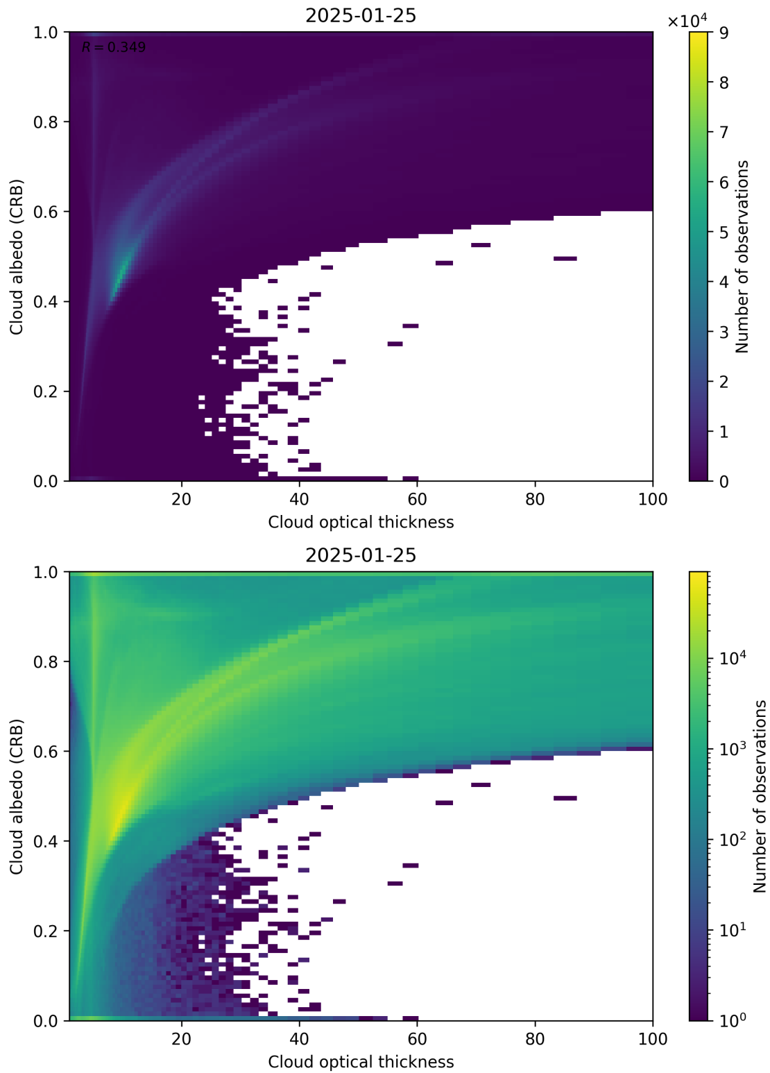
Figure 82: Scatter density plot of “Cloud optical thickness” against “Cloud albedo (CRB)” for 2025-01-24 to 2025-01-26.
