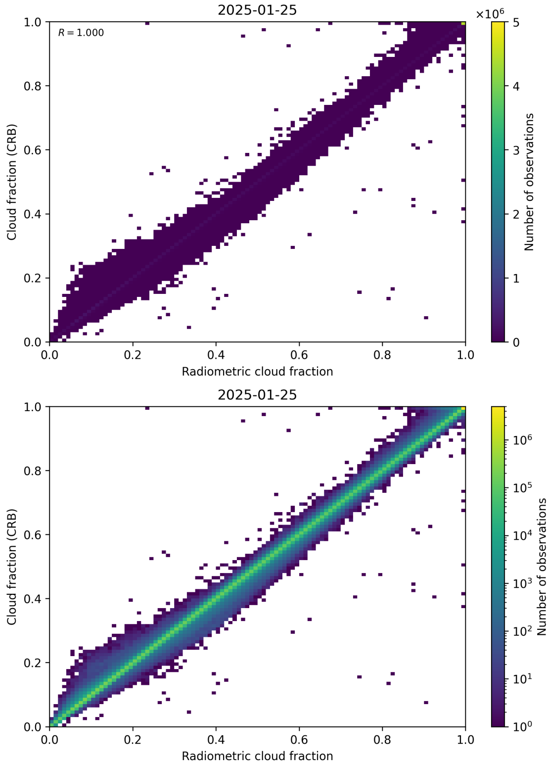
Figure 73: Scatter density plot of “Radiometric cloud fraction” against “Cloud fraction (CRB)” for 2025-01-24 to 2025-01-26.
