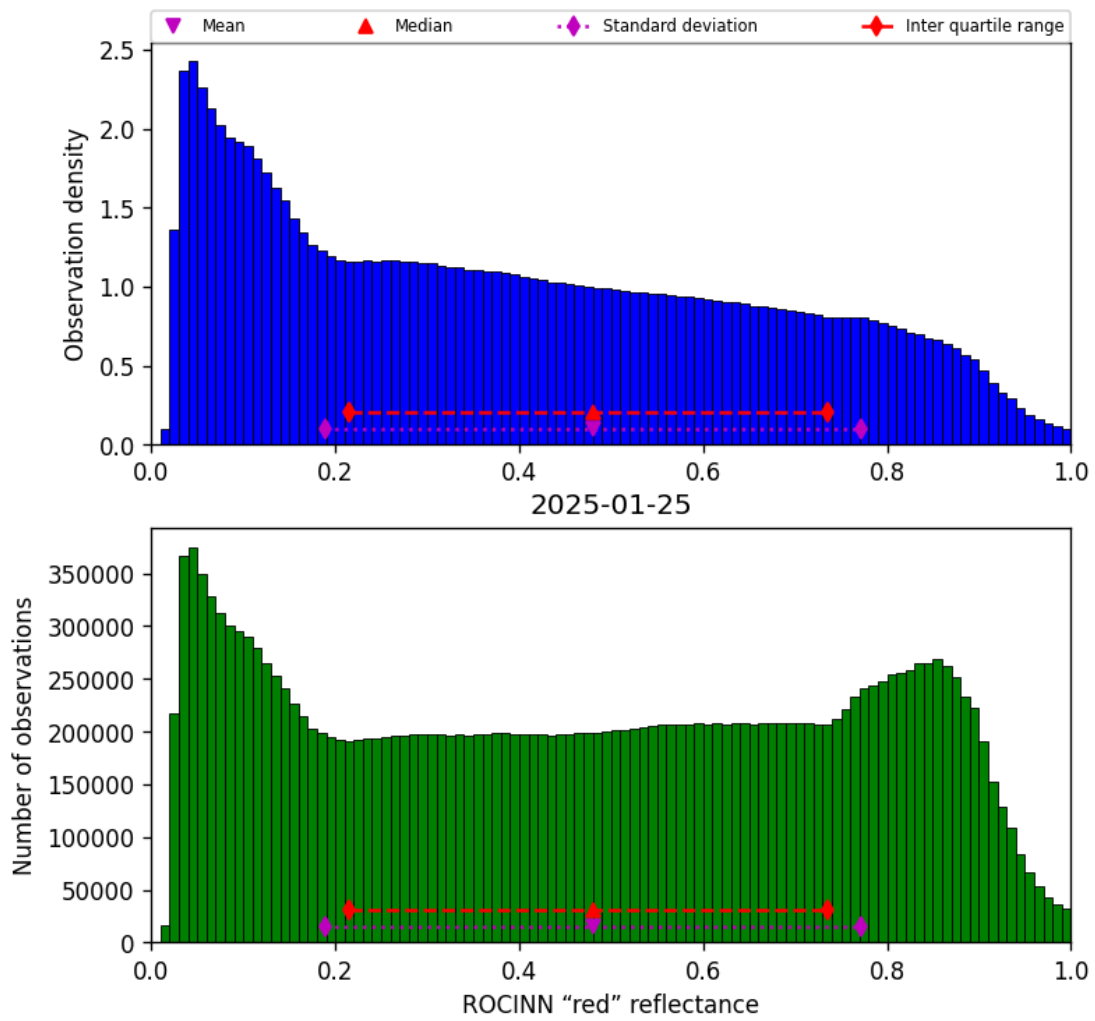
Figure 53: Histogram of “ROCINN “red” reflectance” for 2025-01-24 to 2025-01-26
