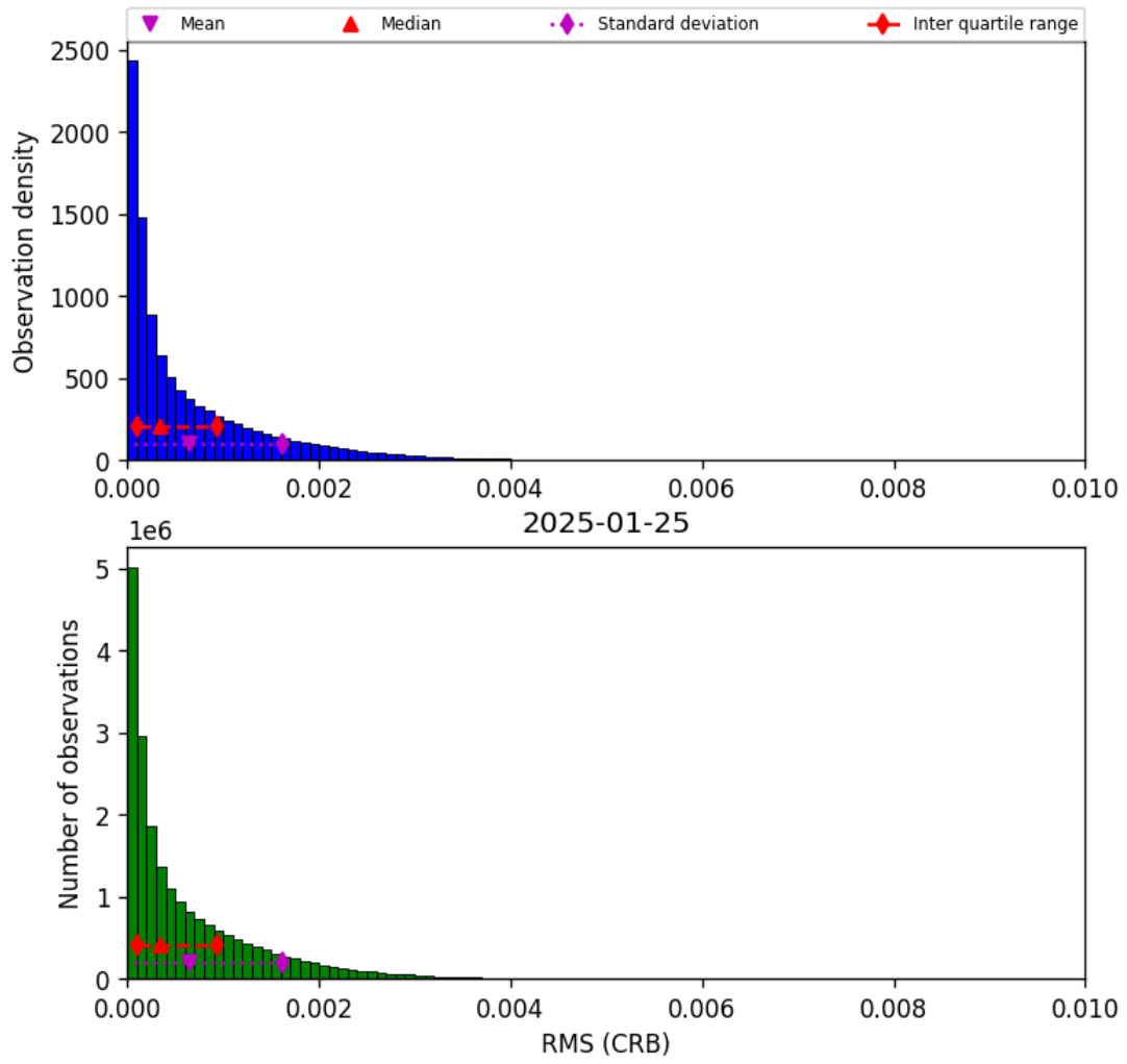
Figure 48: Histogram of “RMS (CRB)” for 2025-01-24 to 2025-01-26
