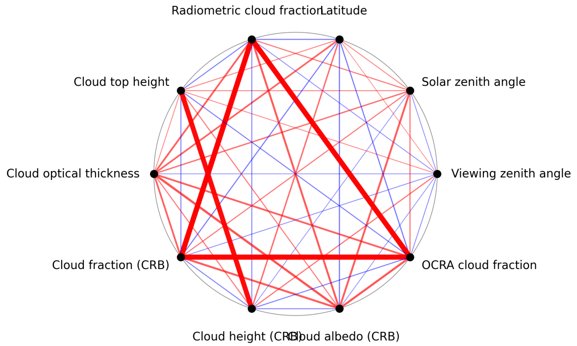
Figure 1: Map of correlation graph for 2025-01-24 to 2025-01-26.
