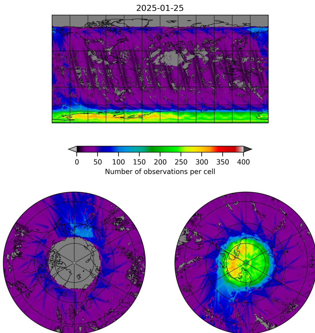
Figure 21: Map of the number of observations for 2025-01-24 to 2025-01-26
