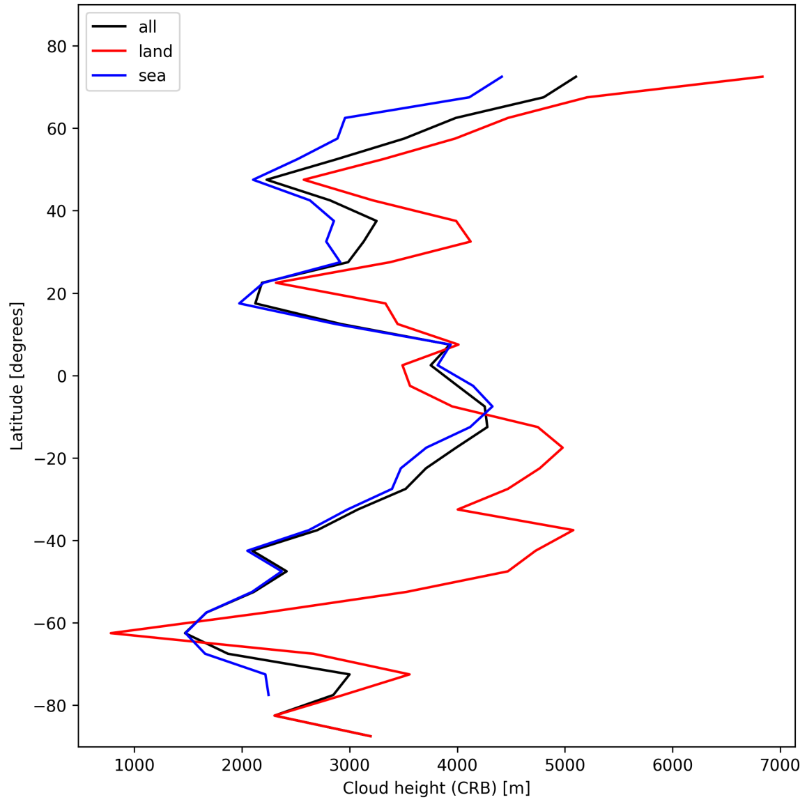
Figure 27: Zonal average of “Cloud height (CRB)” for 2025-01-24 to 2025-01-26.
