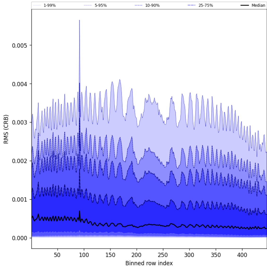
Figure 64: Along track statistics of “RMS (CRB)” for 2025-01-24 to 2025-01-26
