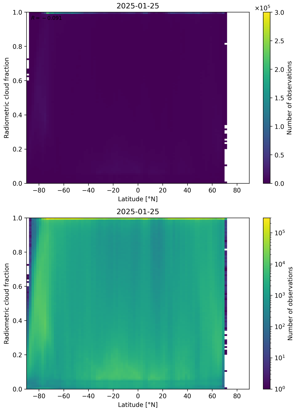
Figure 92: Scatter density plot of “Latitude” against “Radiometric cloud fraction” for 2025-01-24 to 2025-01-26.
