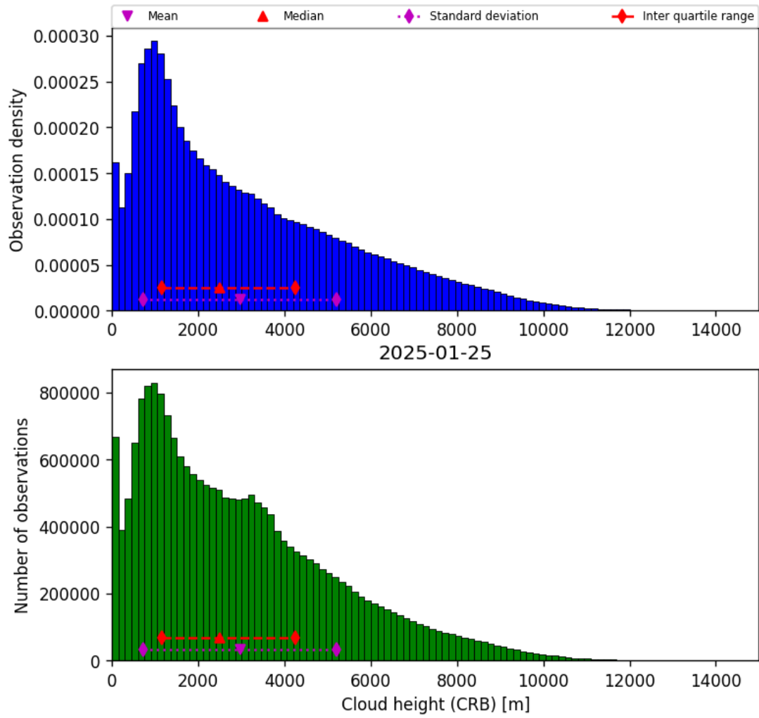
Figure 43: Histogram of “Cloud height (CRB)” for 2025-01-24 to 2025-01-26
