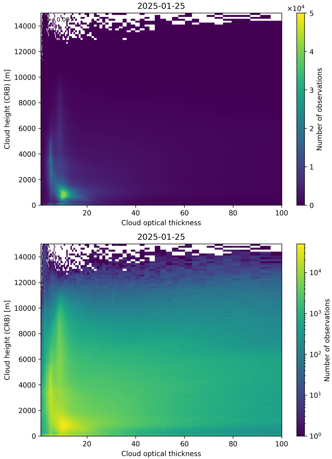
Figure 85: Scatter density plot of “Cloud optical thickness” against “Cloud height (CRB)” for 2025-01-24 to 2025-01-26.
