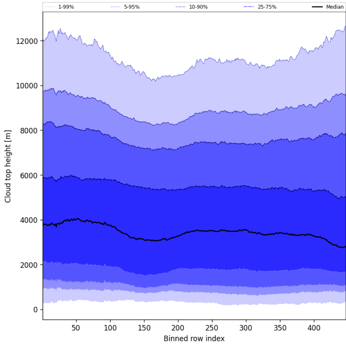
Figure 56: Along track statistics of “Cloud top height” for 2025-01-24 to 2025-01-26
