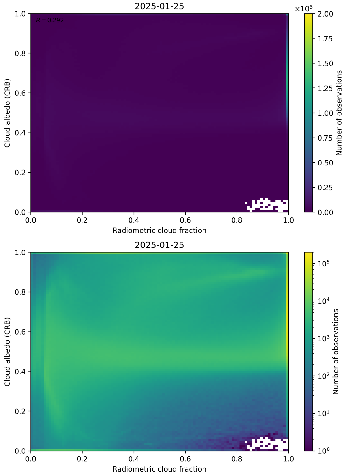
Figure 71: Scatter density plot of “Radiometric cloud fraction” against “Cloud albedo (CRB)” for 2025-01-24 to 2025-01-26.
