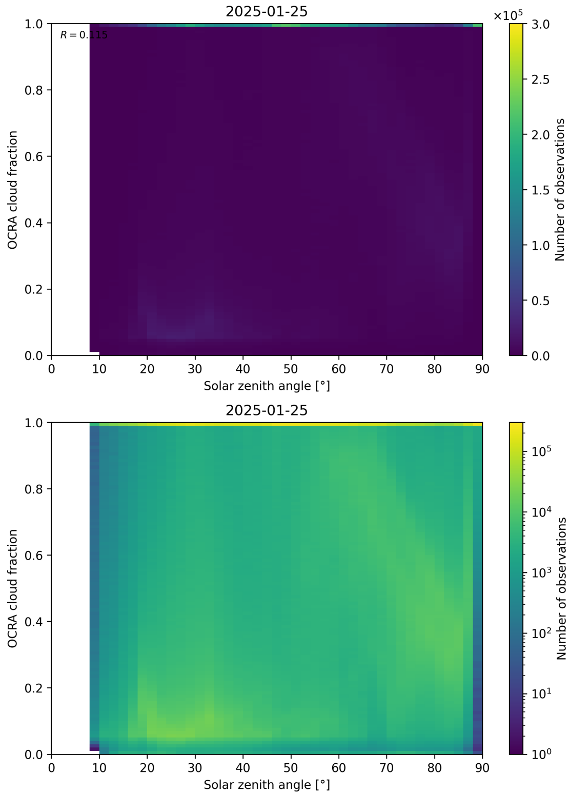
Figure 100: Scatter density plot of “Solar zenith angle” against “OCRA cloud fraction” for 2025-01-24 to 2025-01-26.
