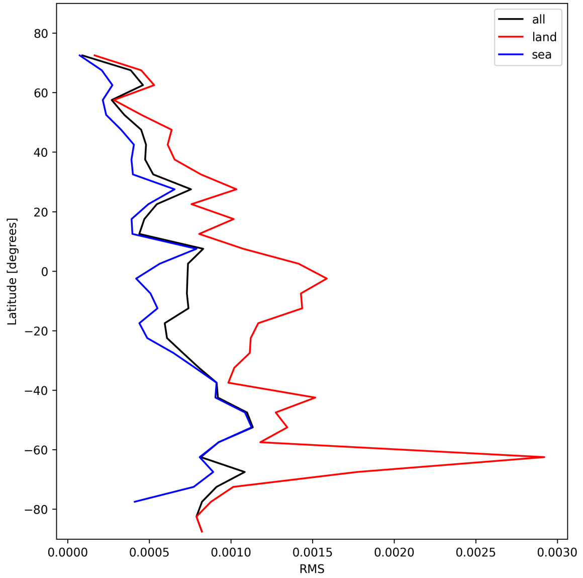
Figure 31: Zonal average of “RMS” for 2025-01-24 to 2025-01-26.
