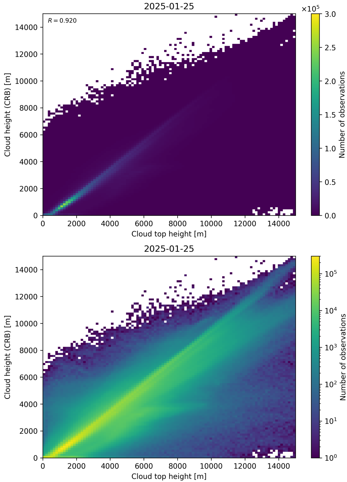
Figure 89: Scatter density plot of “Cloud top height” against “Cloud height (CRB)” for 2025-01-24 to 2025-01-26.
