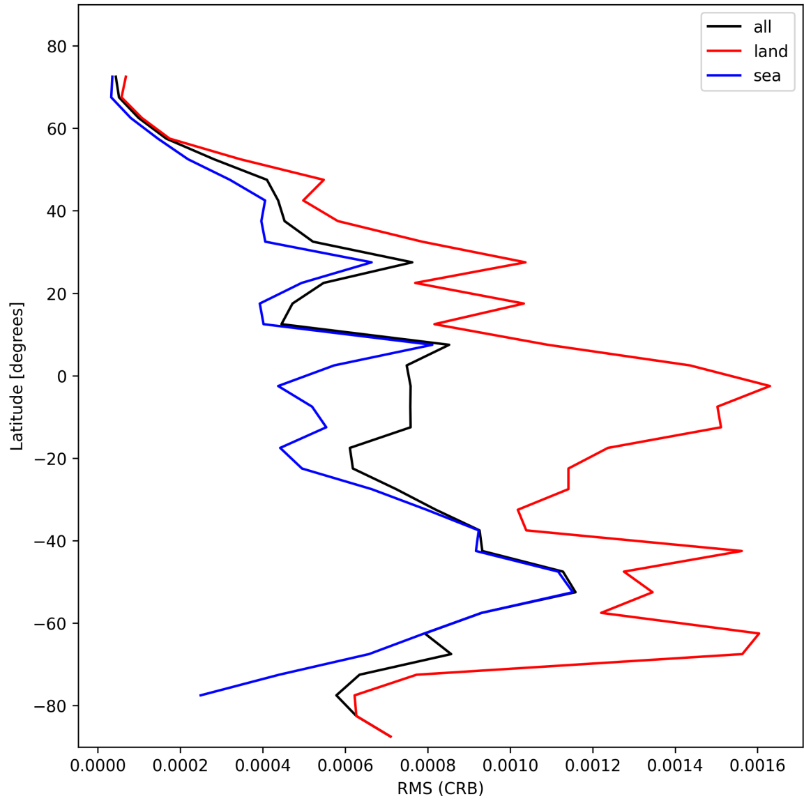
Figure 32: Zonal average of “RMS (CRB)” for 2025-01-24 to 2025-01-26.
