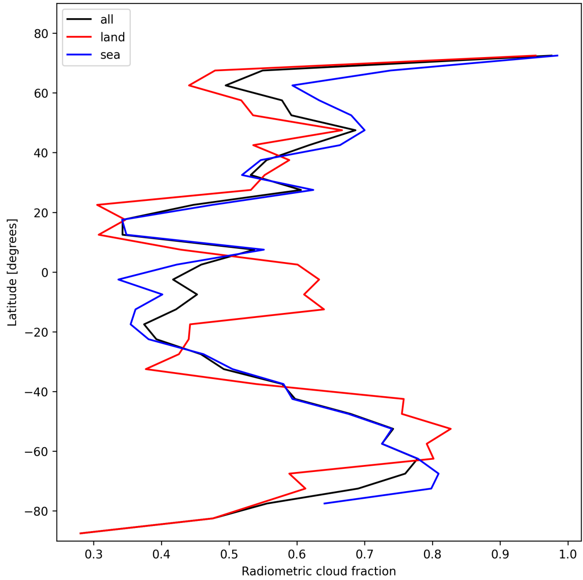
Figure 23: Zonal average of “Radiometric cloud fraction” for 2025-01-24 to 2025-01-26.
