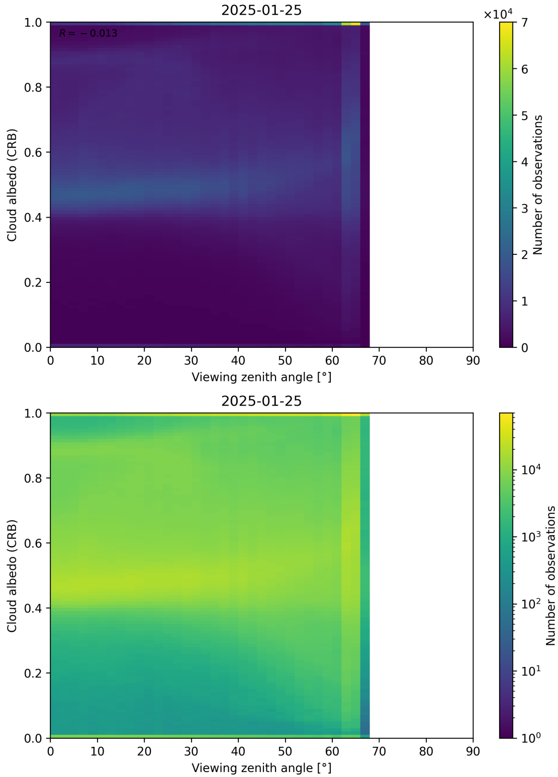
Figure 106: Scatter density plot of “Viewing zenith angle” against “Cloud albedo (CRB)” for 2025-01-24 to 2025-01-26.
