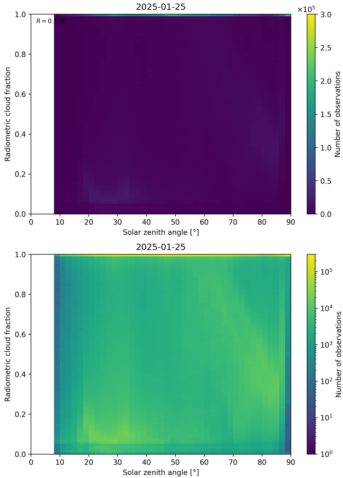
Figure 99: Scatter density plot of “Solar zenith angle” against “Radiometric cloud fraction” for 2025-01-24 to 2025-01-26.
