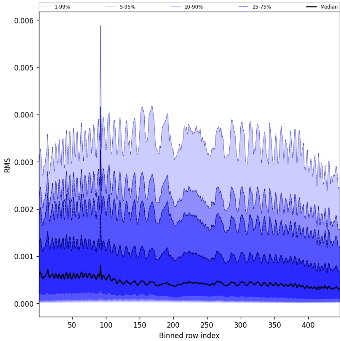
Figure 63: Along track statistics of “RMS” for 2025-01-24 to 2025-01-26
