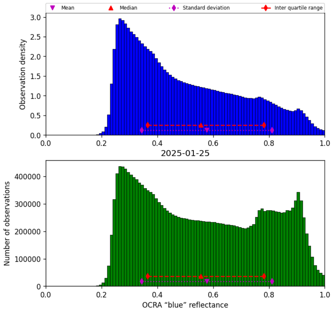
Figure 51: Histogram of “OCRA “blue” reflectance” for 2025-01-24 to 2025-01-26
