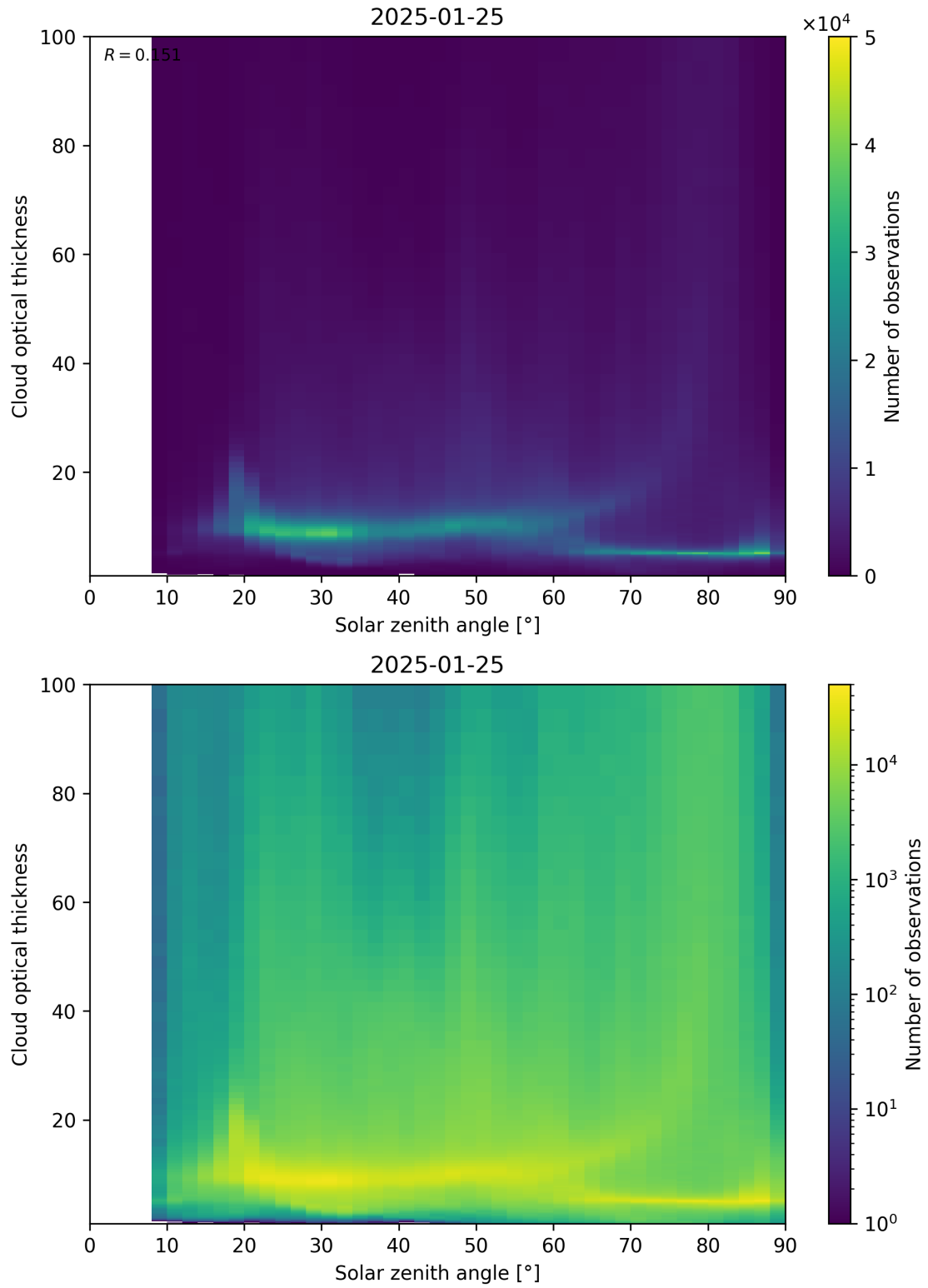
Figure 103: Scatter density plot of “Solar zenith angle” against “Cloud optical thickness” for 2025-01-24 to 2025-01-26.
