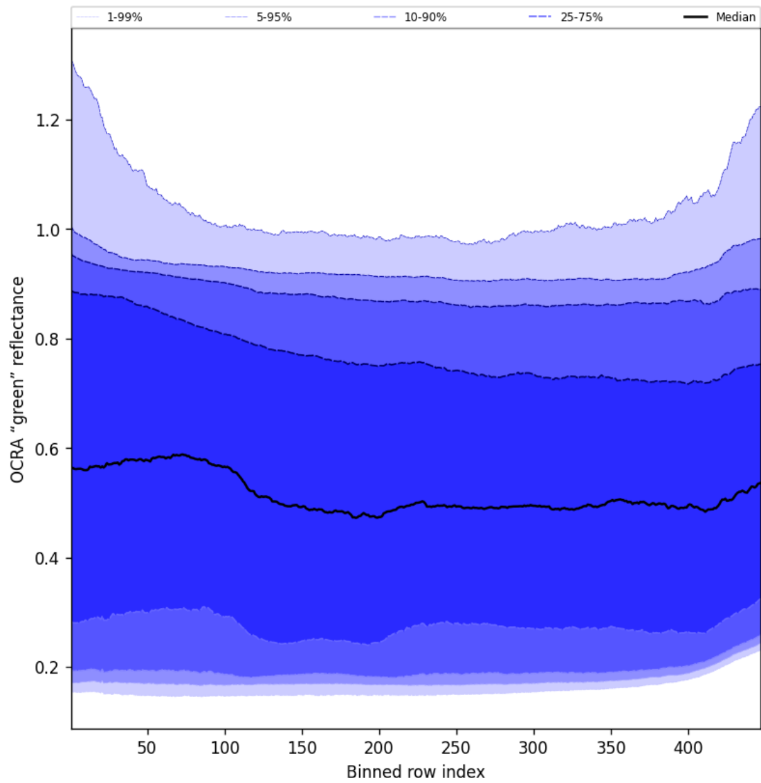
Figure 68: Along track statistics of "OCRA "green" reflectance" for 2025-01-24 to 2025-01-26
