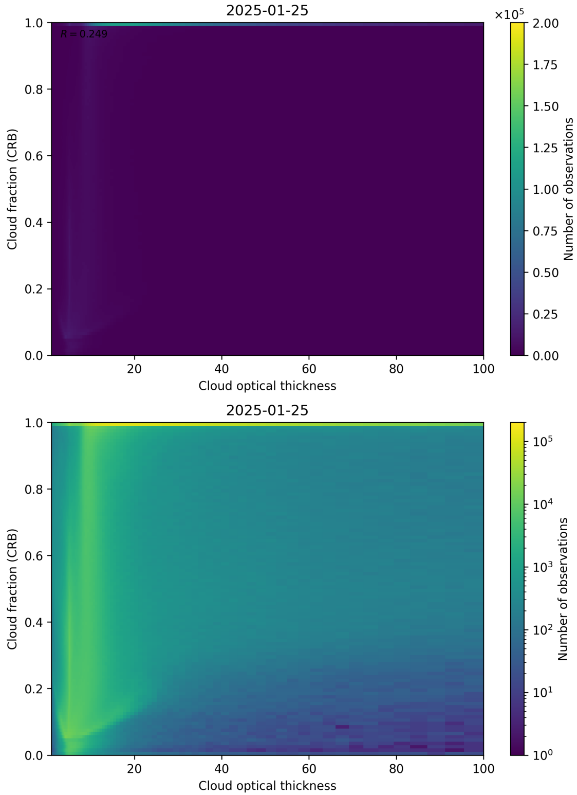
Figure 84: Scatter density plot of “Cloud optical thickness” against “Cloud fraction (CRB)” for 2025-01-24 to 2025-01-26.
