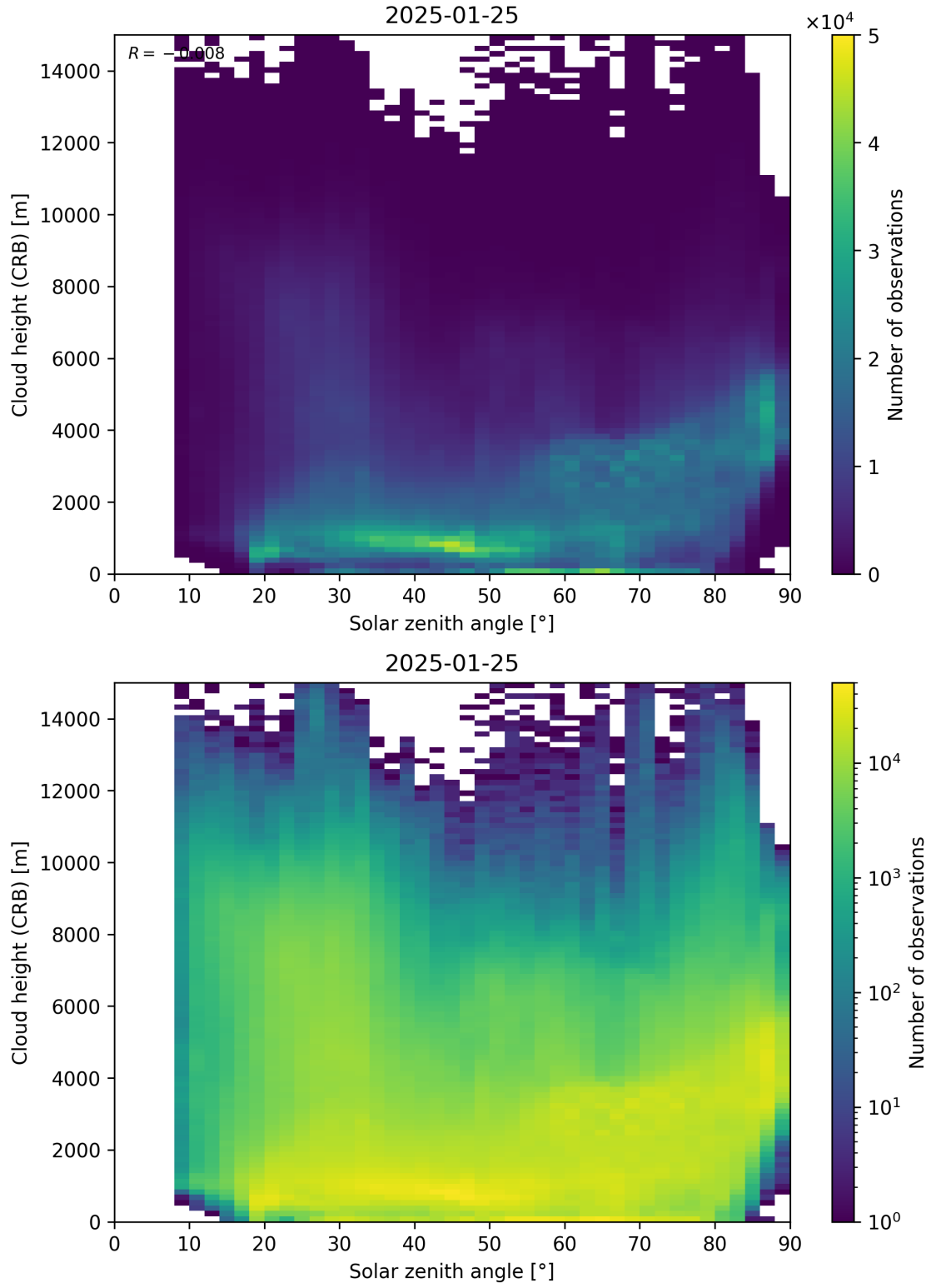
Figure 102: Scatter density plot of “Solar zenith angle” against “Cloud height (CRB)” for 2025-01-24 to 2025-01-26.
