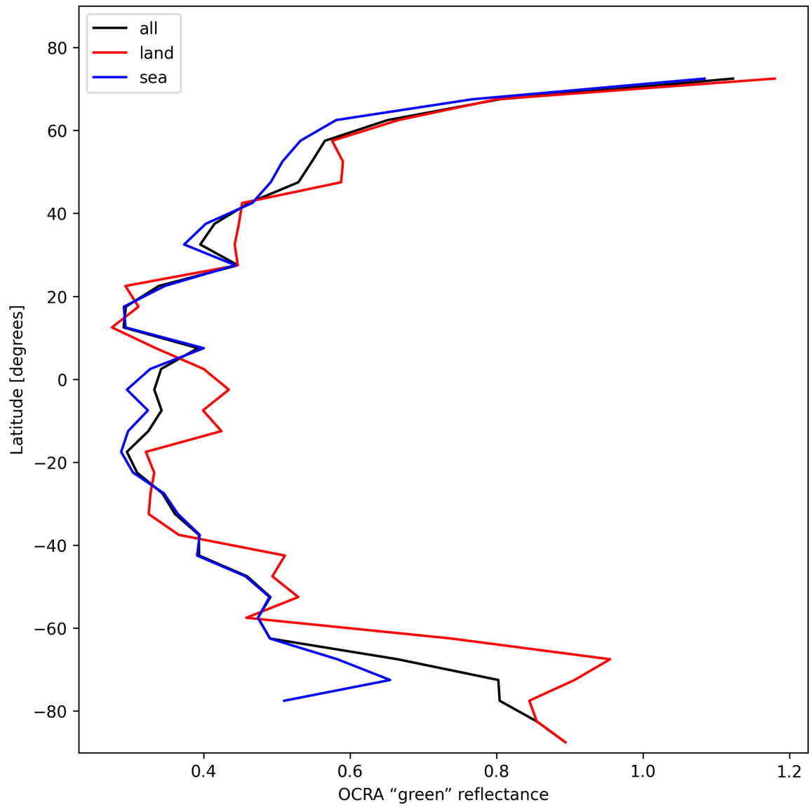
Figure 36: Zonal average of “OCRA “green” reflectance” for 2025-01-24 to 2025-01-26.
