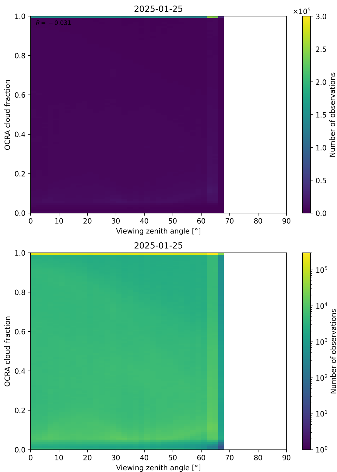
Figure 108: Scatter density plot of “Viewing zenith angle” against “OCRA cloud fraction” for 2025-01-24 to 2025-01-26.
