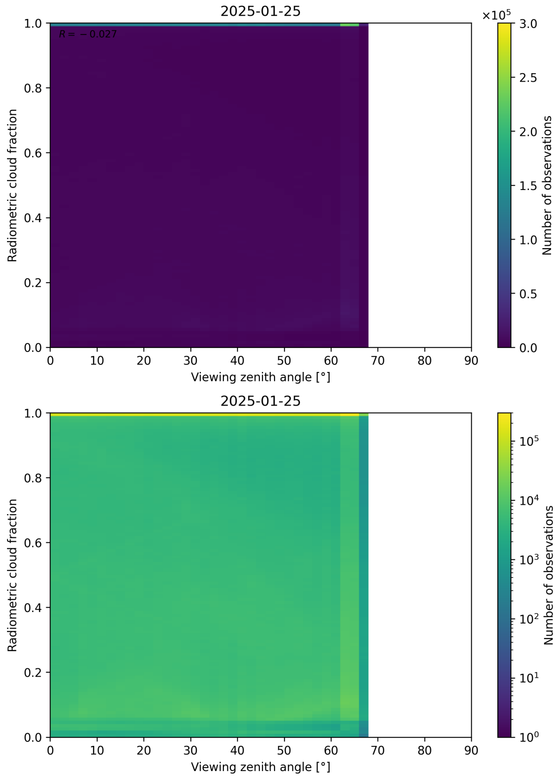
Figure 107: Scatter density plot of “Viewing zenith angle” against “Radiometric cloud fraction” for 2025-01-24 to 2025-01-26.
