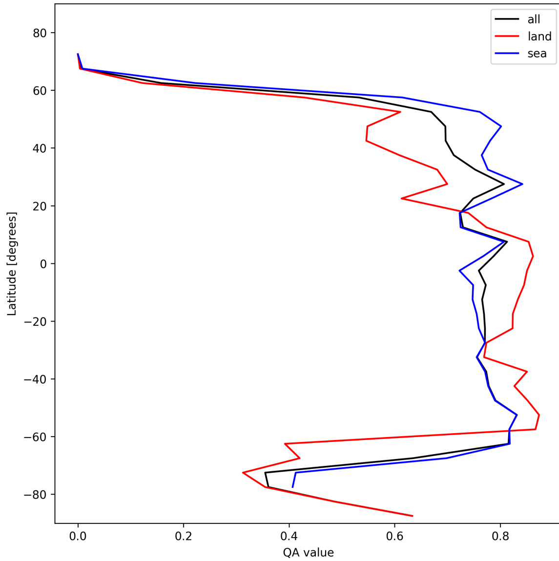
Figure 22: Zonal average of “QA value” for 2025-01-24 to 2025-01-26.
