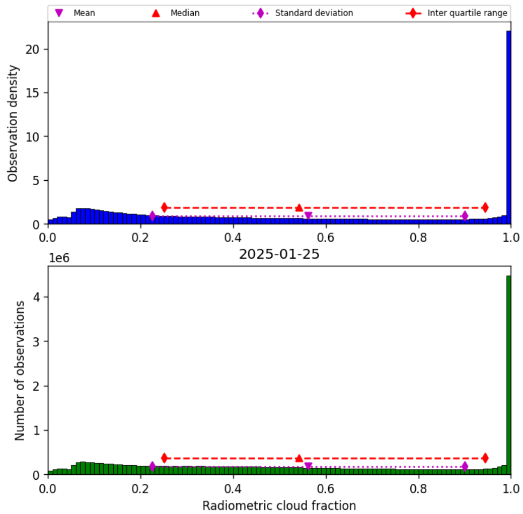
Figure 39: Histogram of “Radiometric cloud fraction” for 2025-01-24 to 2025-01-26
