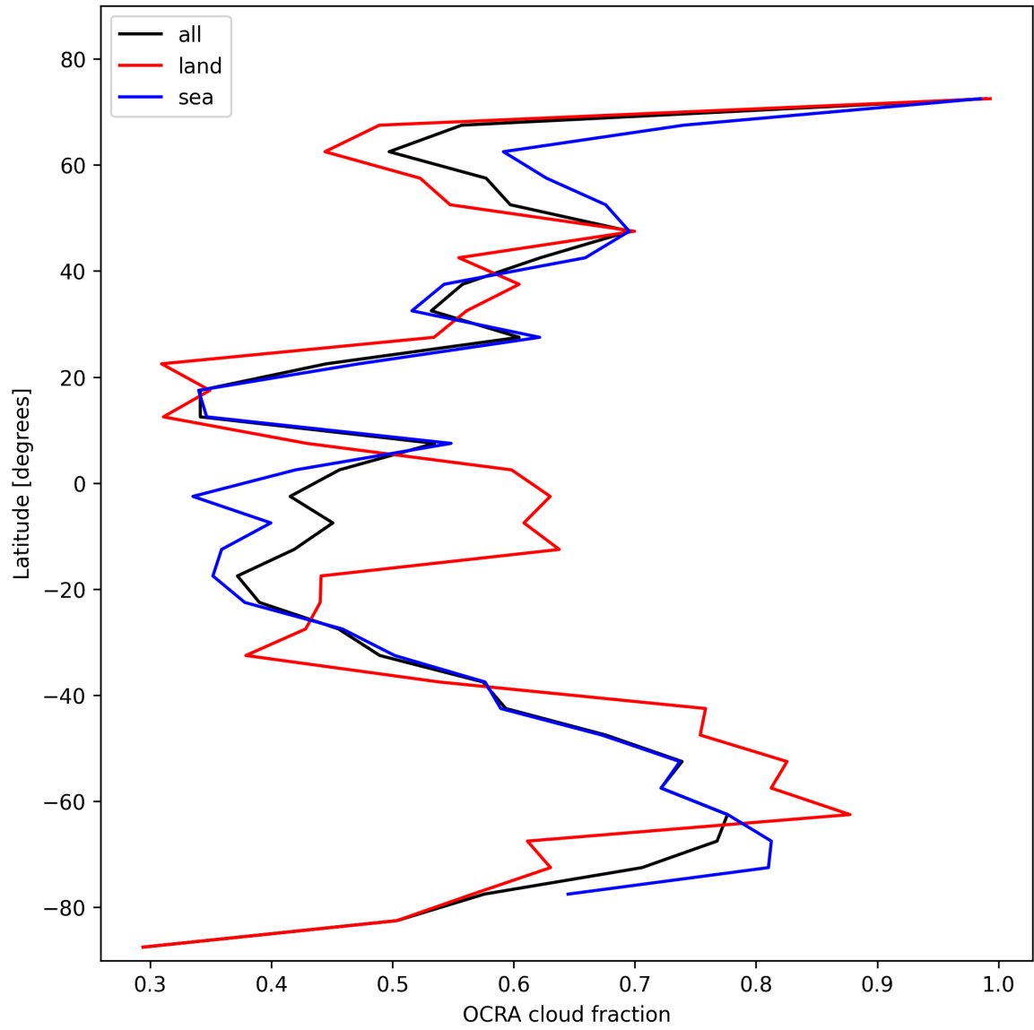
Figure 34: Zonal average of “OCRA cloud fraction” for 2025-01-24 to 2025-01-26.
