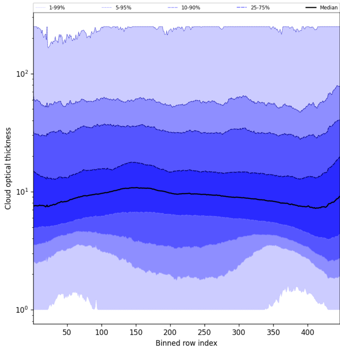
Figure 57: Along track statistics of “Cloud optical thickness” for 2025-01-24 to 2025-01-26
