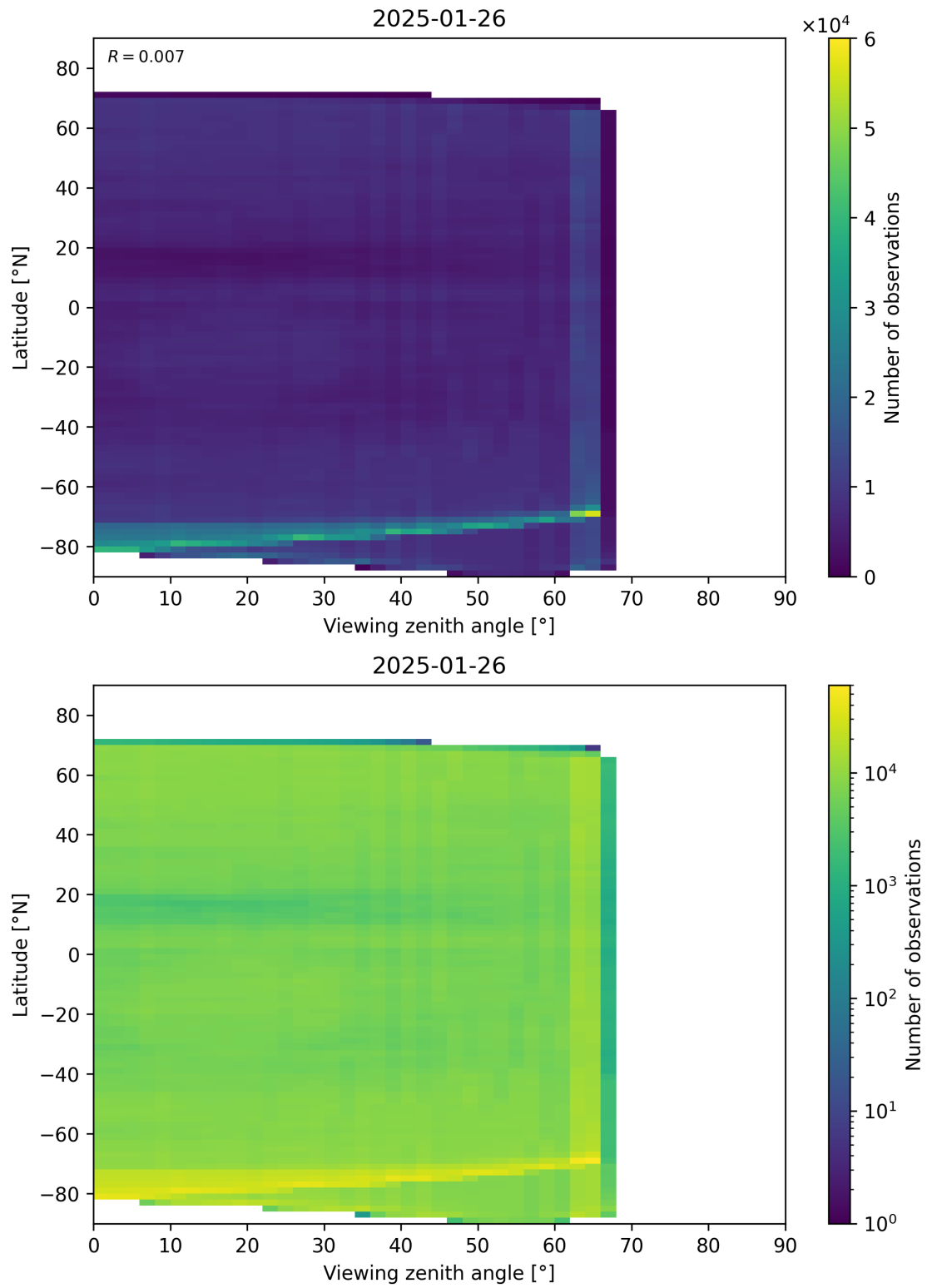
Figure 113: Scatter density plot of “Viewing zenith angle” against “Latitude” for 2025-01-25 to 2025-01-27.
