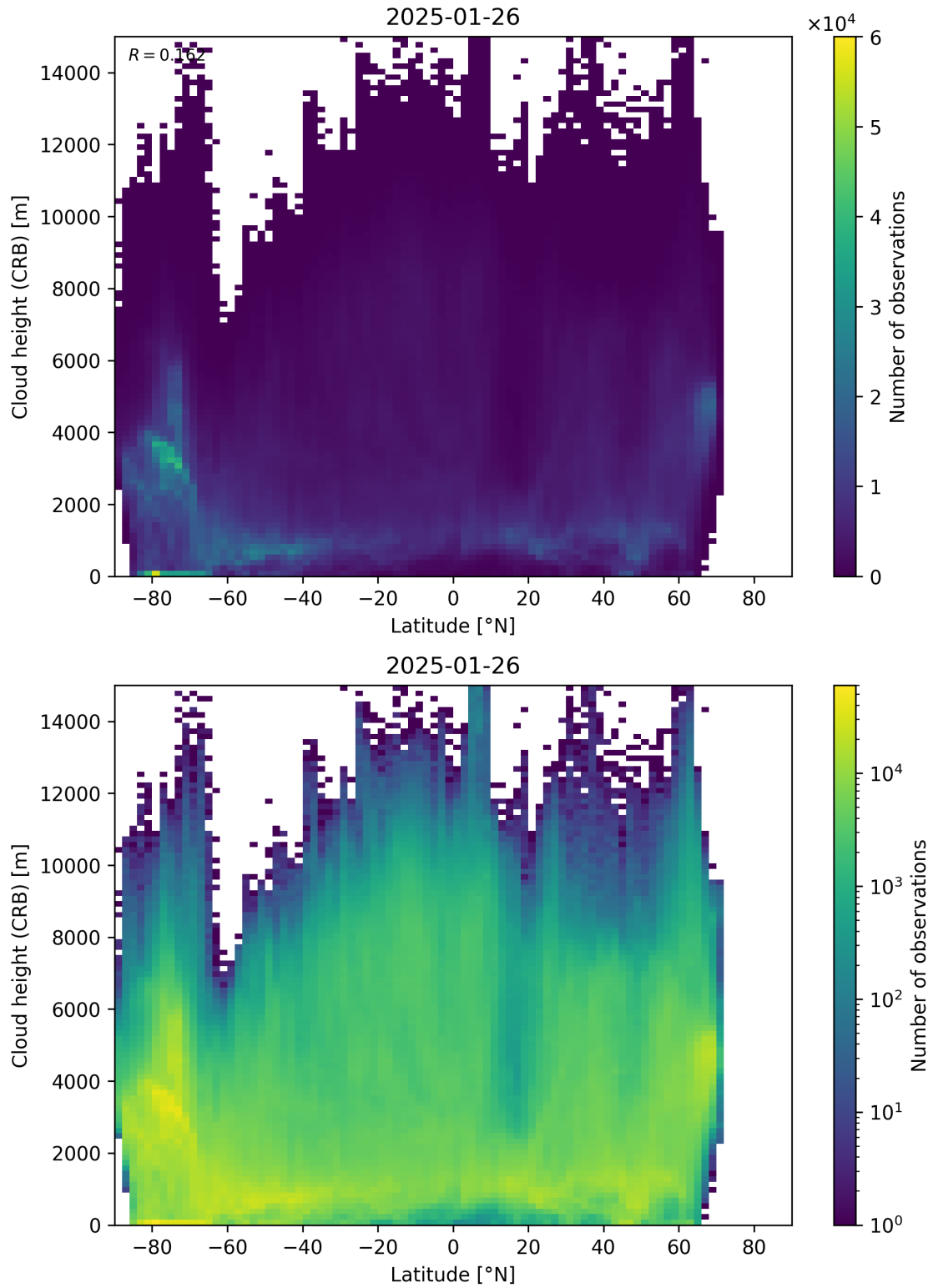
Figure 95: Scatter density plot of “Latitude” against “Cloud height (CRB)” for 2025-01-25 to 2025-01-27.
