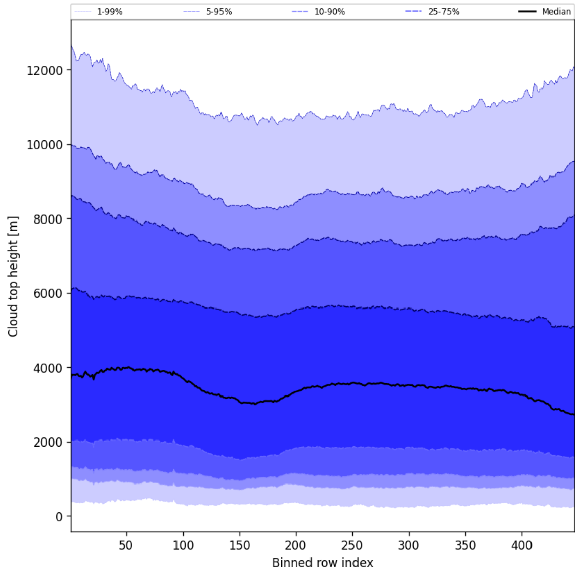
Figure 56: Along track statistics of “Cloud top height” for 2025-01-25 to 2025-01-27
