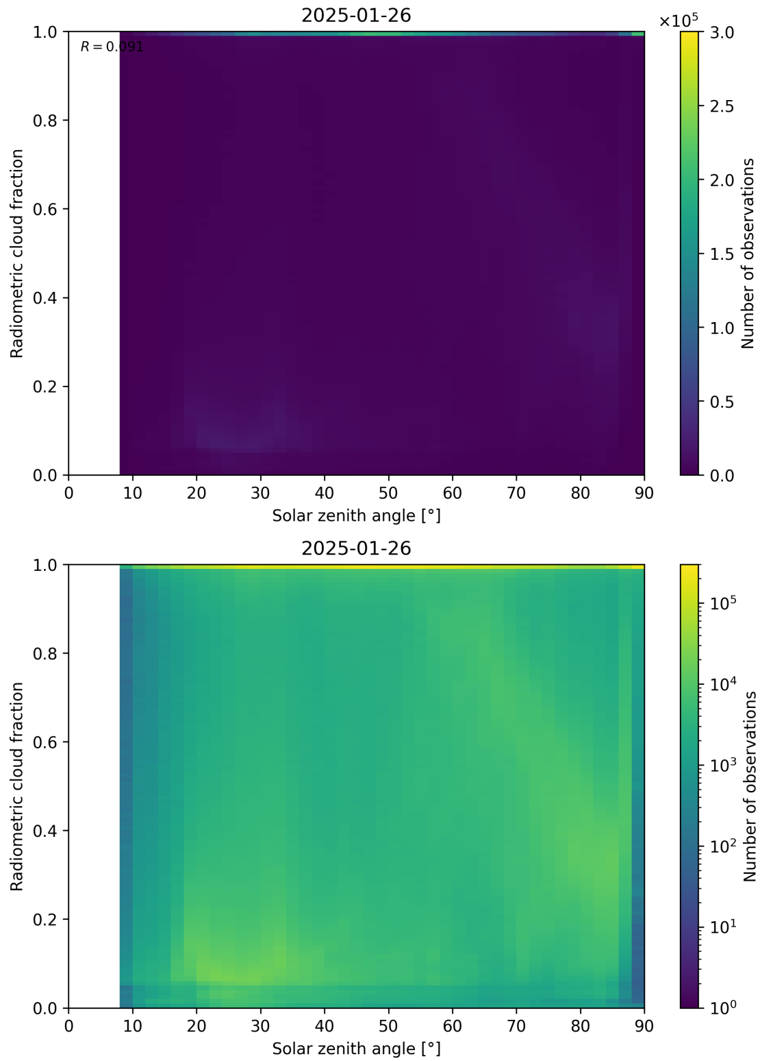
Figure 99: Scatter density plot of “Solar zenith angle” against “Radiometric cloud fraction” for 2025-01-25 to 2025-01-27.
