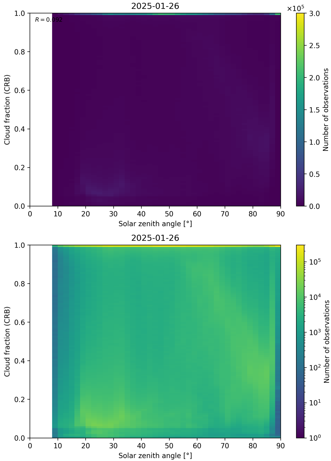
Figure 101: Scatter density plot of “Solar zenith angle” against “Cloud fraction (CRB)” for 2025-01-25 to 2025-01-27.
