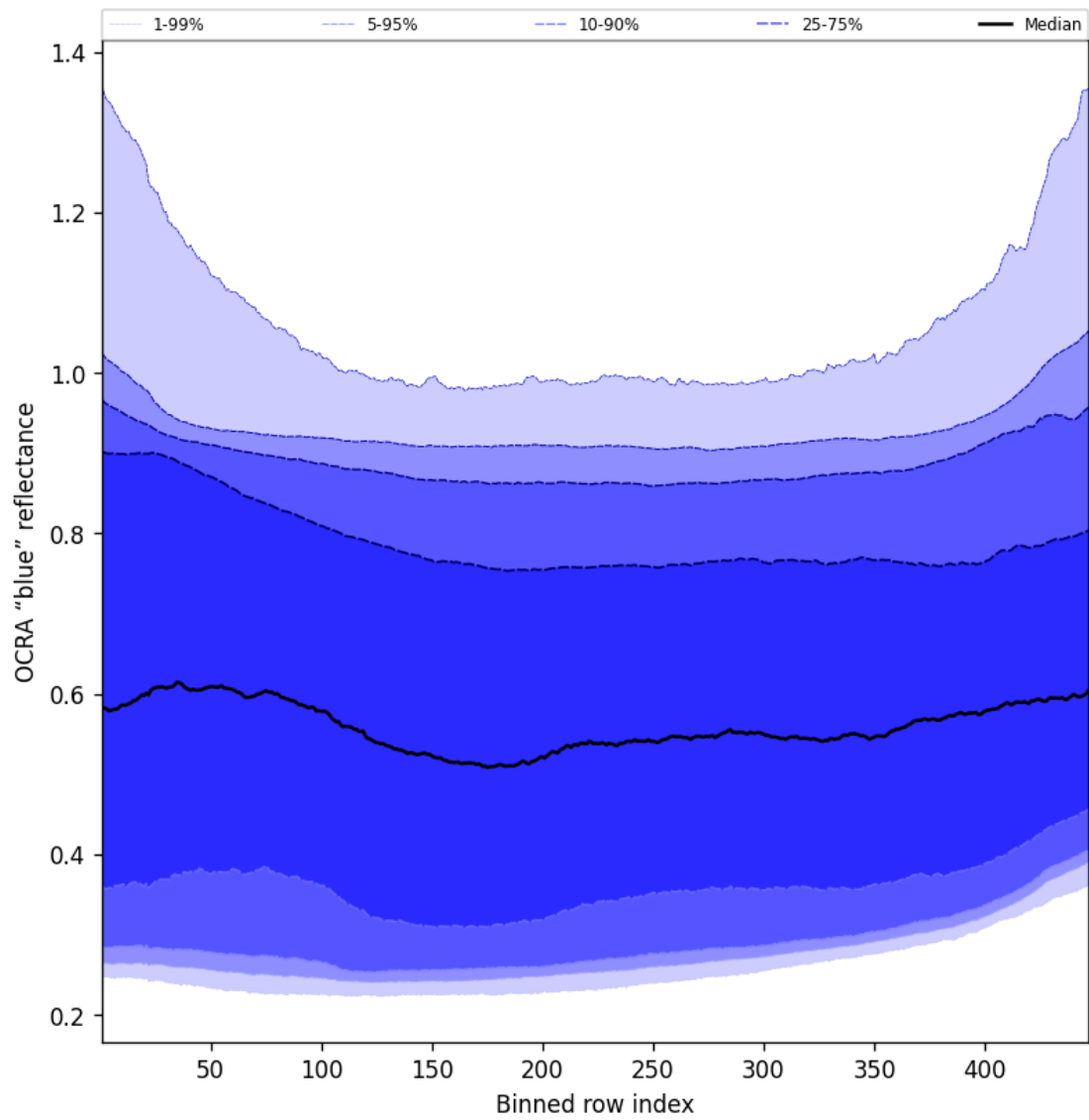
Figure 67: Along track statistics of “OCRA “blue” reflectance” for 2025-01-25 to 2025-01-27
