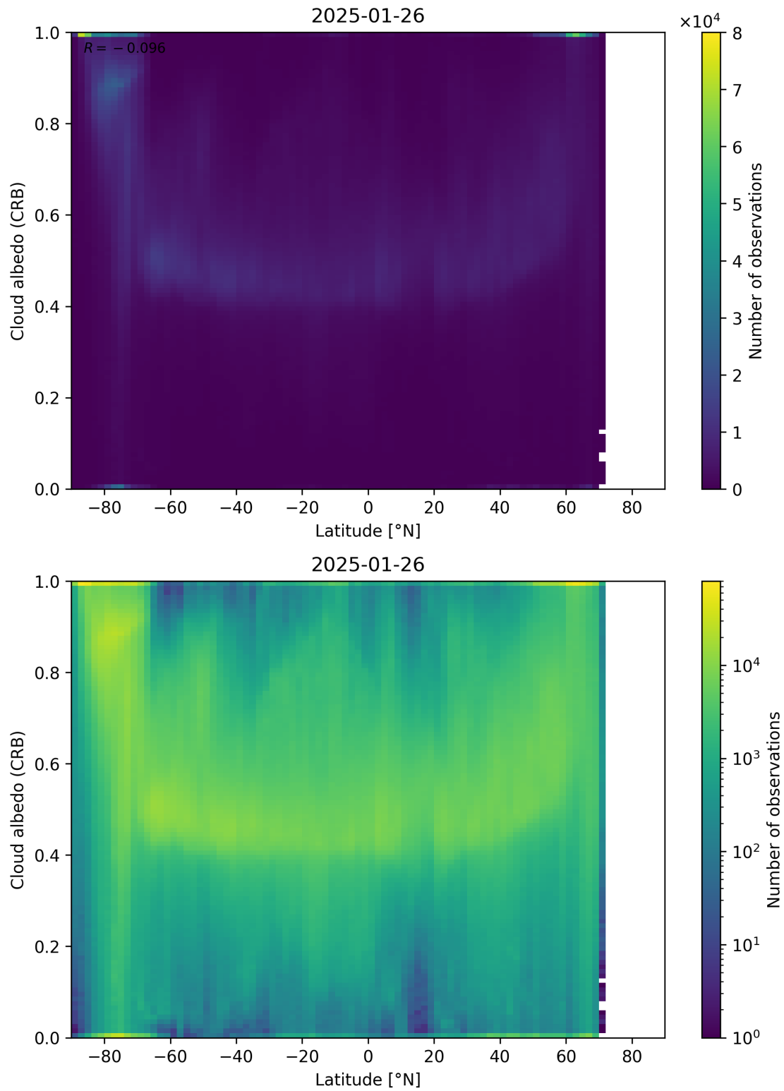
Figure 91: Scatter density plot of “Latitude” against “Cloud albedo (CRB)” for 2025-01-25 to 2025-01-27.
