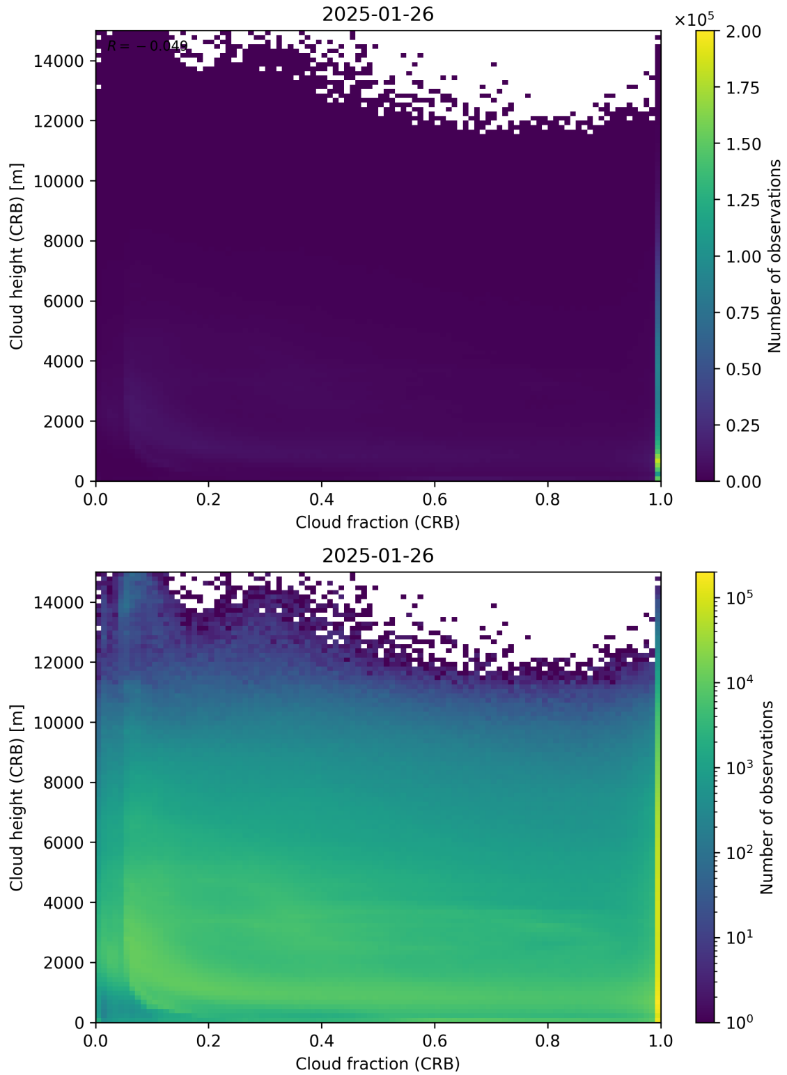
Figure 79: Scatter density plot of “Cloud fraction (CRB)” against “Cloud height (CRB)” for 2025-01-25 to 2025-01-27.
