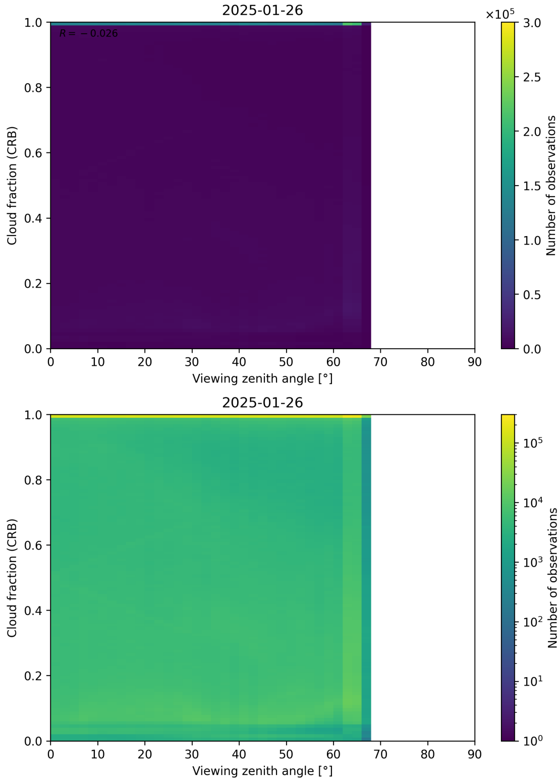
Figure 109: Scatter density plot of “Viewing zenith angle” against “Cloud fraction (CRB)” for 2025-01-25 to 2025-01-27.
