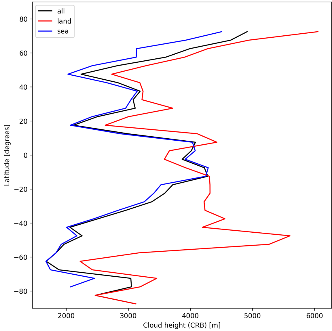
Figure 27: Zonal average of “Cloud height (CRB)” for 2025-01-25 to 2025-01-27.
