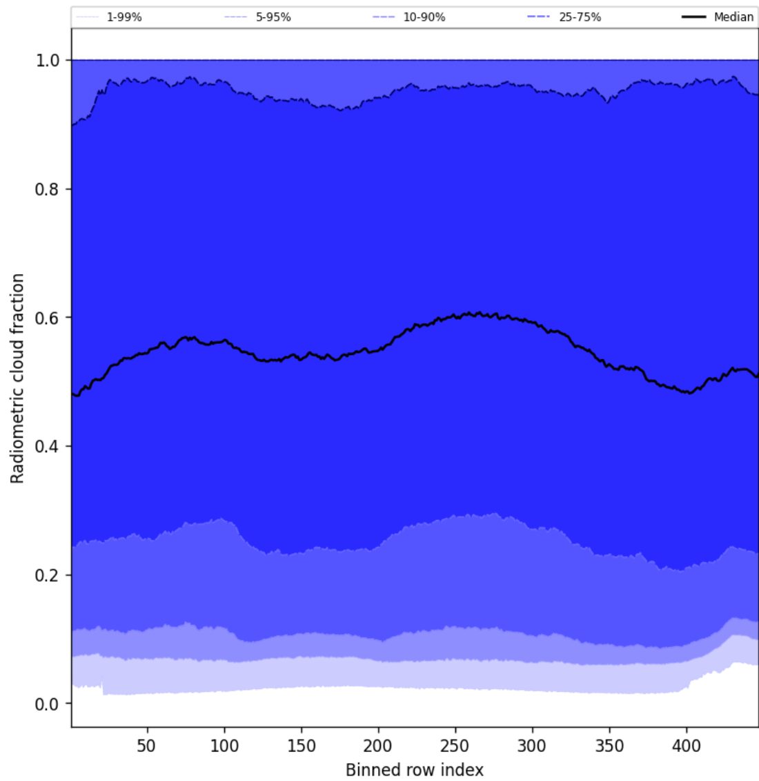
Figure 55: Along track statistics of “Radiometric cloud fraction” for 2025-01-25 to 2025-01-27
