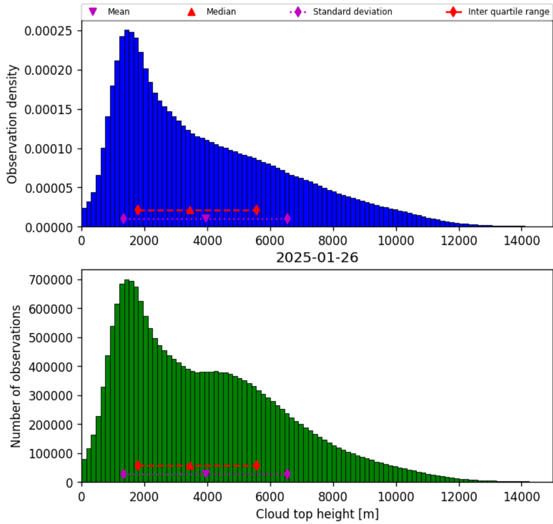
Figure 40: Histogram of “Cloud top height” for 2025-01-25 to 2025-01-27
