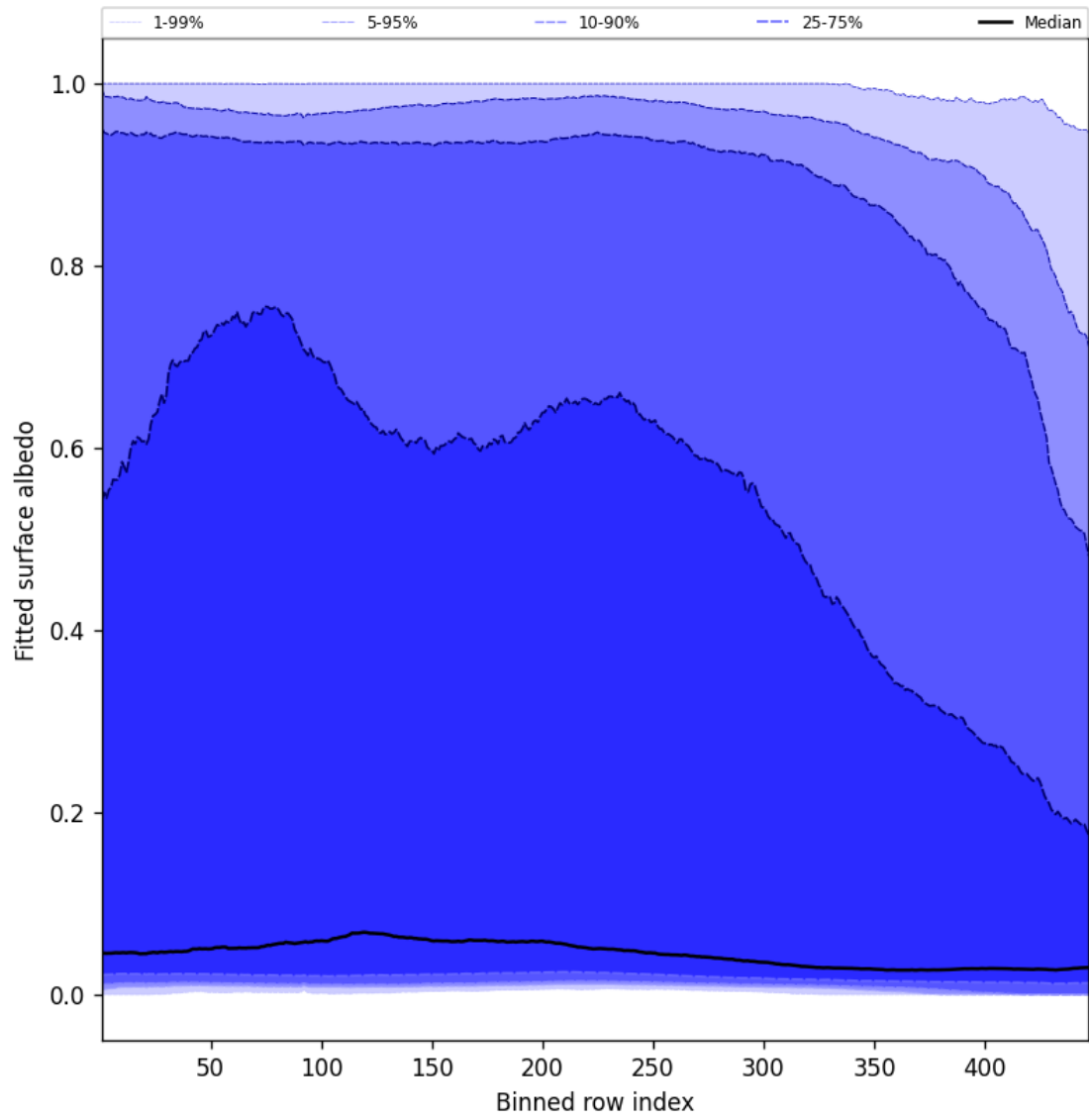
Figure 61: Along track statistics of “Fitted surface albedo” for 2025-01-25 to 2025-01-27
