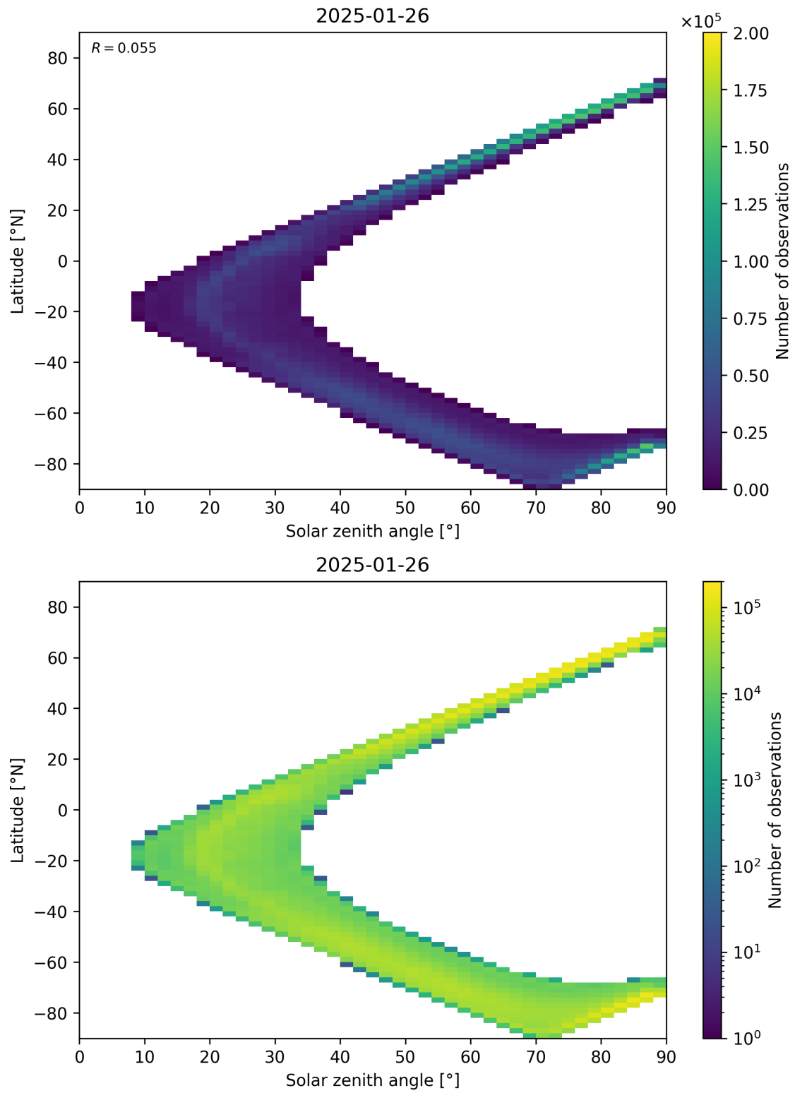
Figure 105: Scatter density plot of “Solar zenith angle” against “Latitude” for 2025-01-25 to 2025-01-27.
