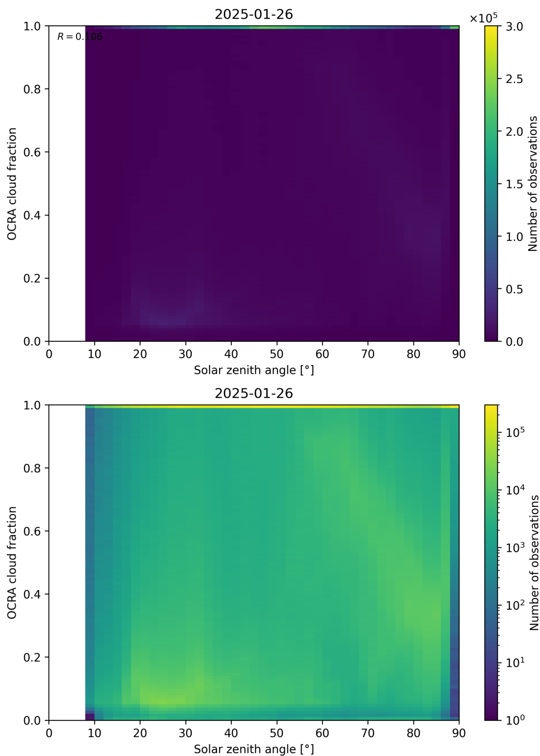
Figure 100: Scatter density plot of “Solar zenith angle” against “OCRA cloud fraction” for 2025-01-25 to 2025-01-27.
