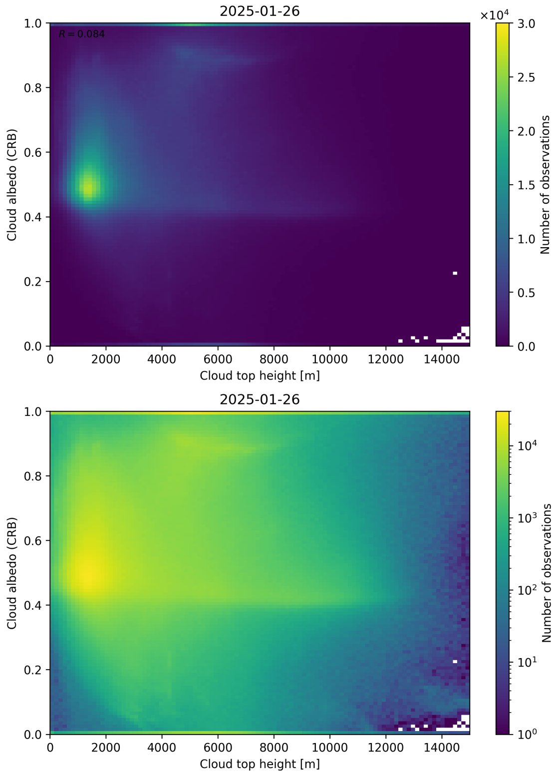
Figure 86: Scatter density plot of “Cloud top height” against “Cloud albedo (CRB)” for 2025-01-25 to 2025-01-27.
