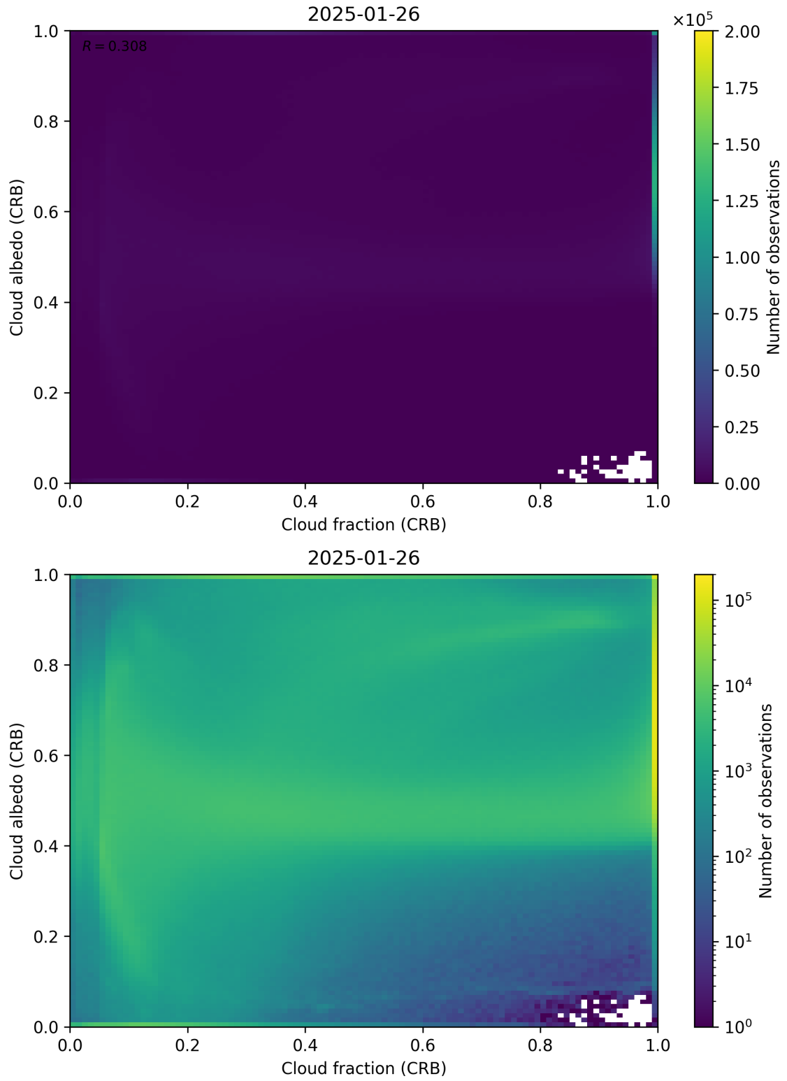
Figure 77: Scatter density plot of “Cloud fraction (CRB)” against “Cloud albedo (CRB)” for 2025-01-25 to 2025-01-27.
