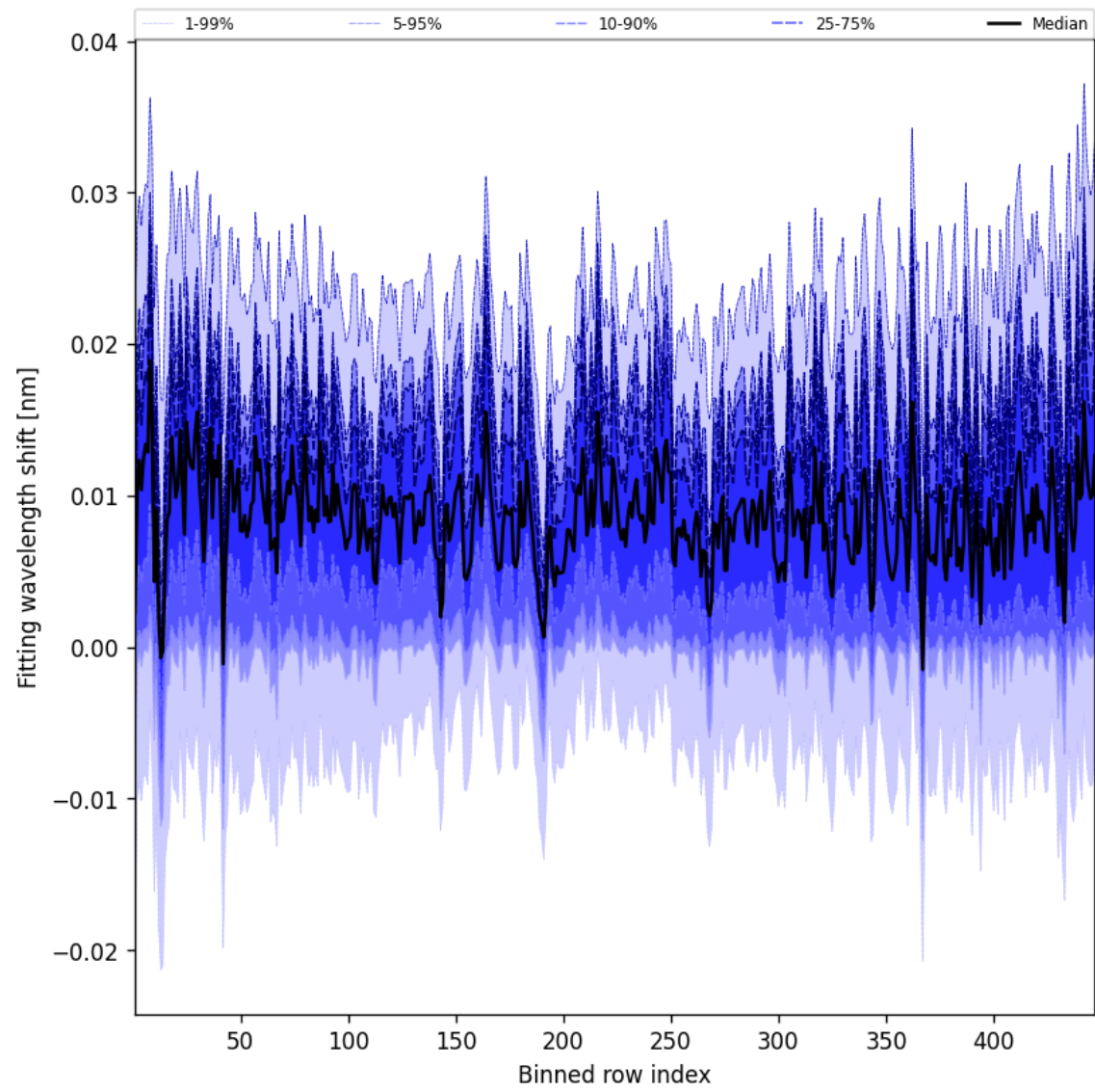
Figure 65: Along track statistics of “Fitting wavelength shift” for 2025-01-25 to 2025-01-27
