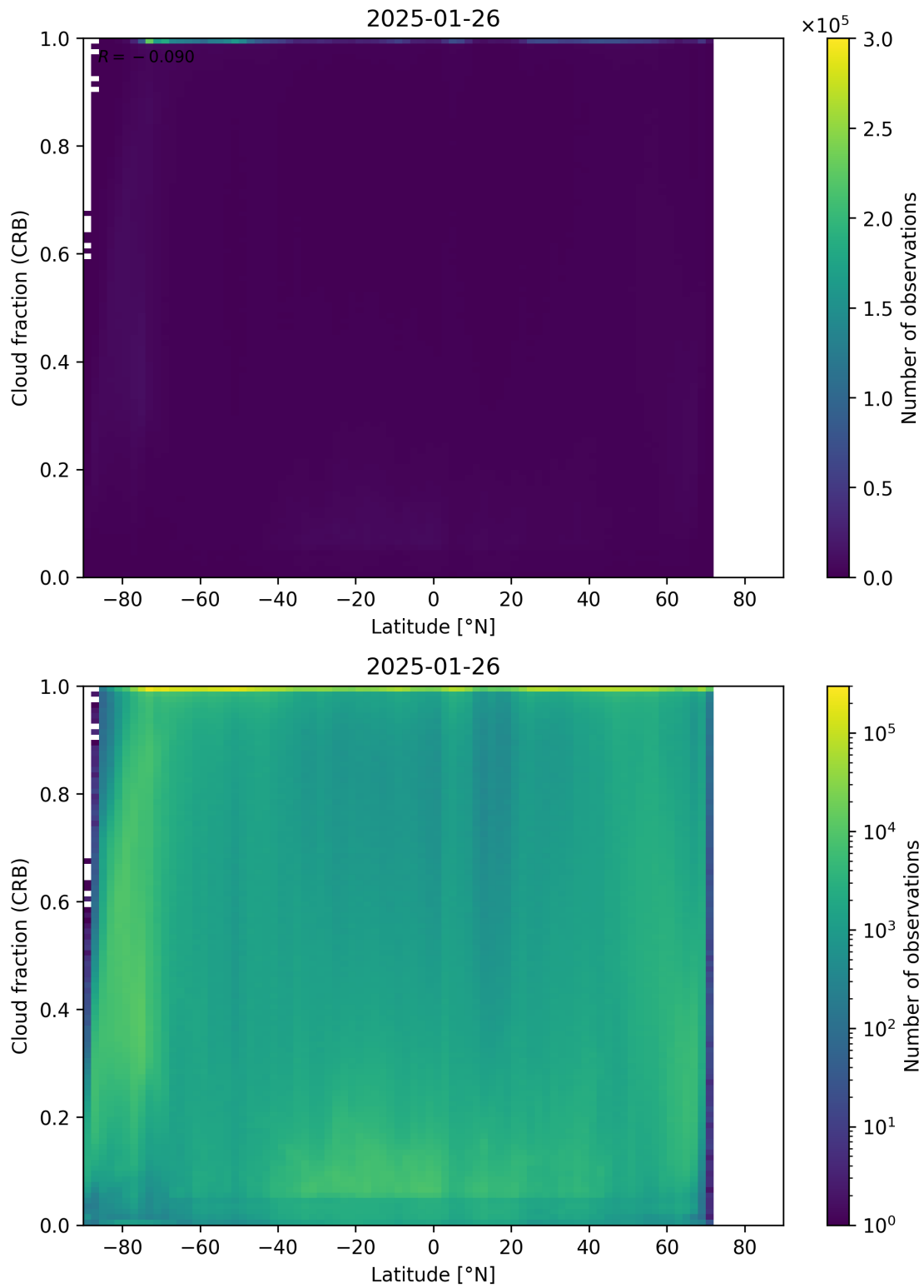
Figure 94: Scatter density plot of “Latitude” against “Cloud fraction (CRB)” for 2025-01-25 to 2025-01-27.
