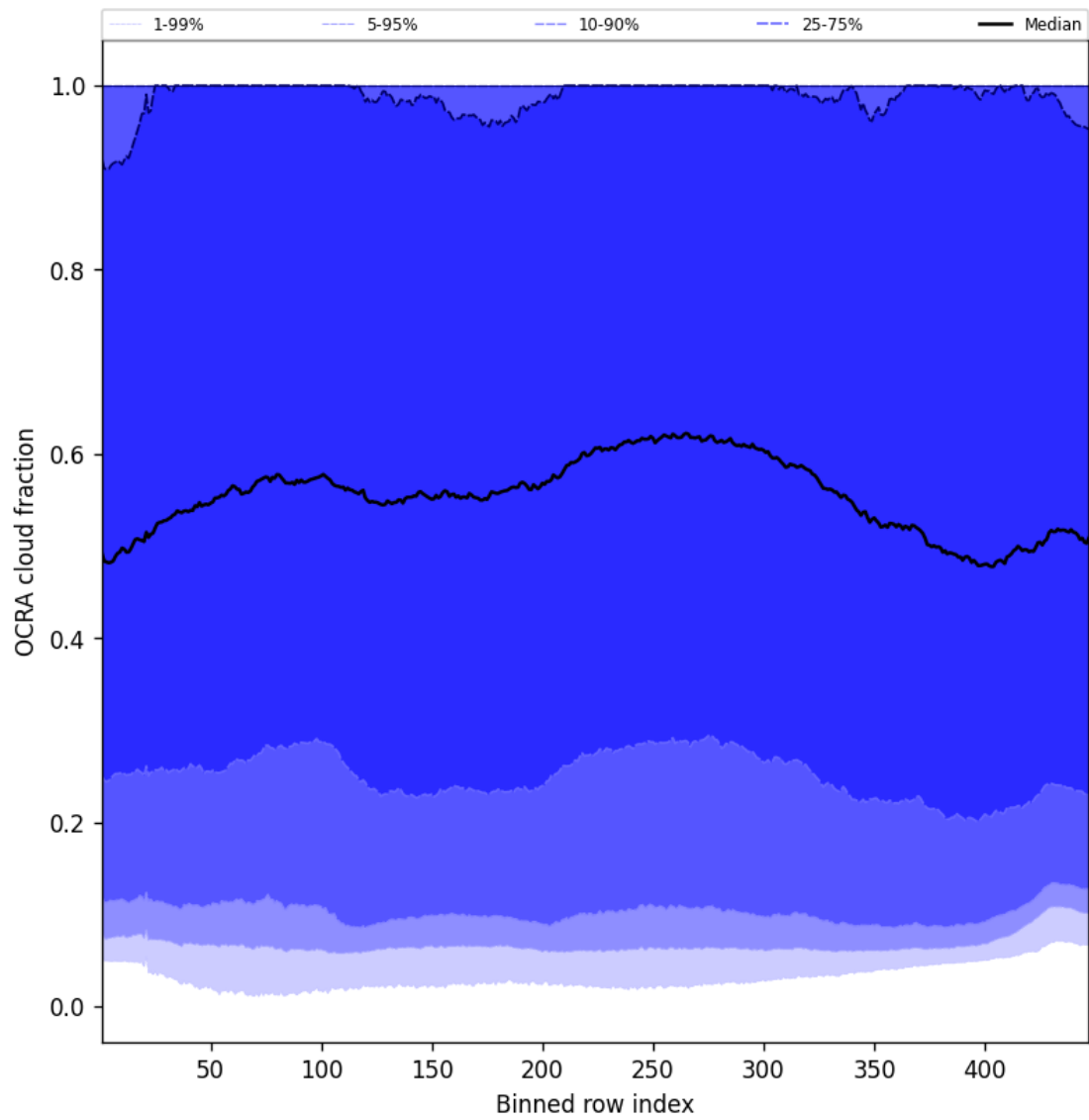
Figure 66: Along track statistics of “OCRA cloud fraction” for 2025-01-25 to 2025-01-27
