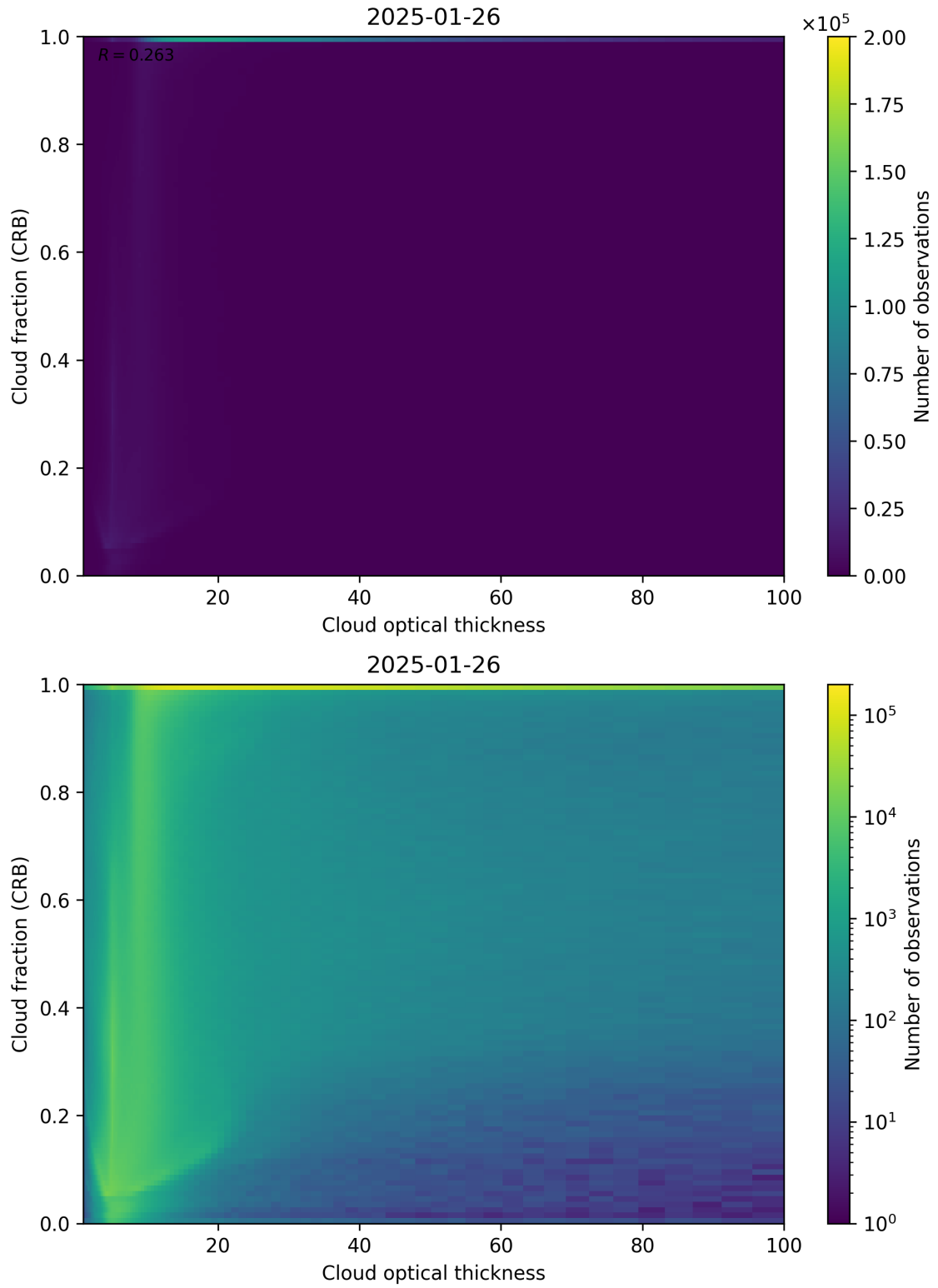
Figure 84: Scatter density plot of “Cloud optical thickness” against “Cloud fraction (CRB)” for 2025-01-25 to 2025-01-27.
