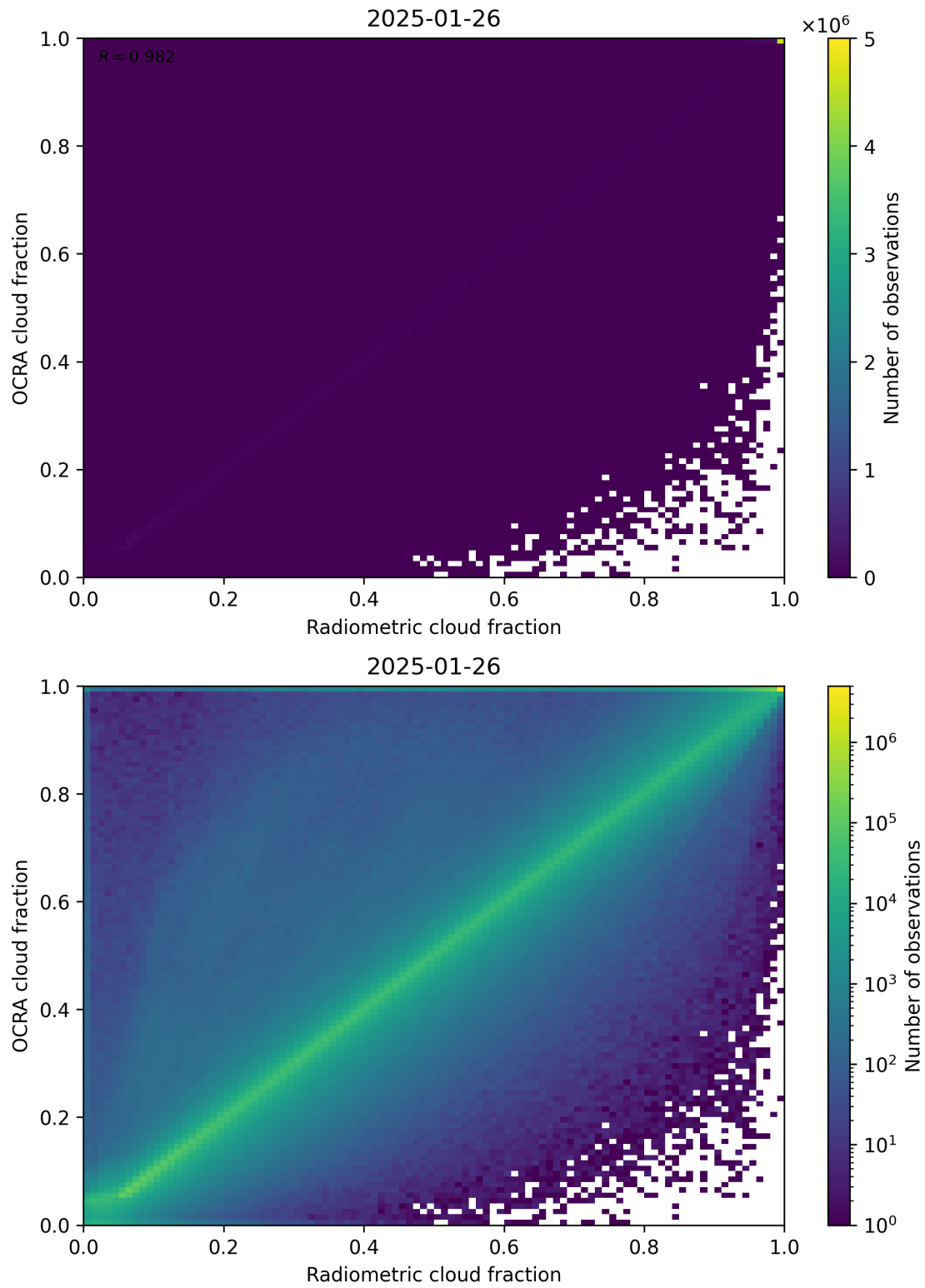
Figure 72: Scatter density plot of “Radiometric cloud fraction” against “OCRA cloud fraction” for 2025-01-25 to 2025-01-27.
