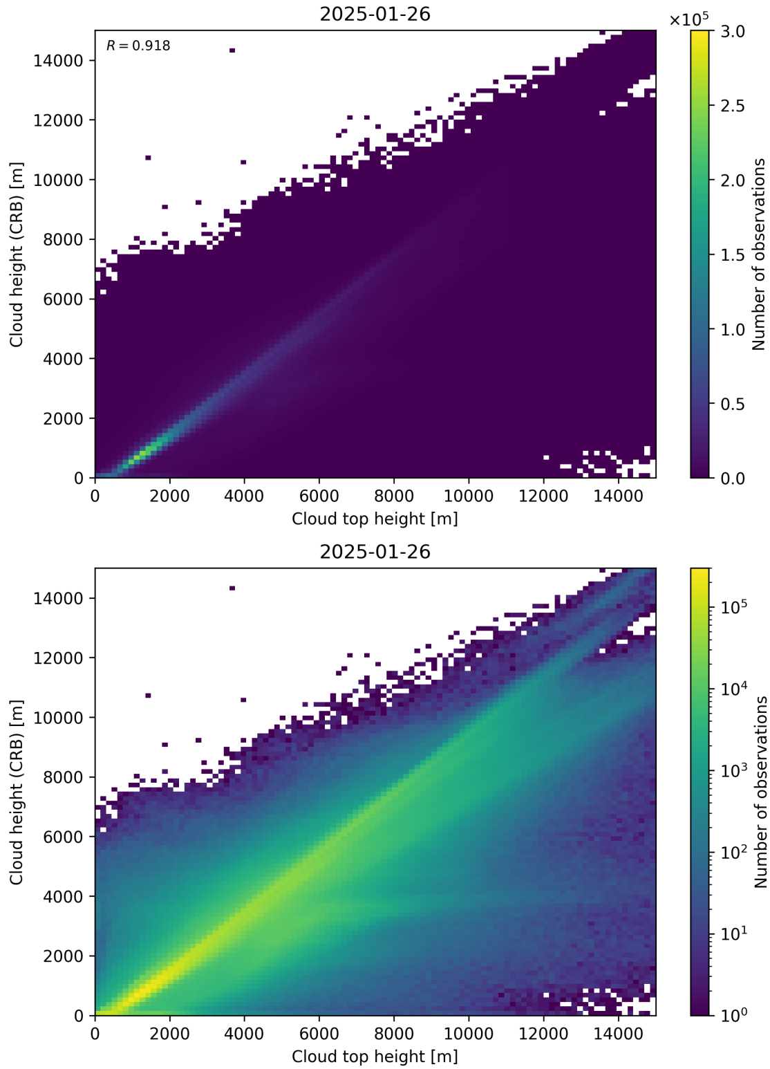
Figure 89: Scatter density plot of “Cloud top height” against “Cloud height (CRB)” for 2025-01-25 to 2025-01-27.
