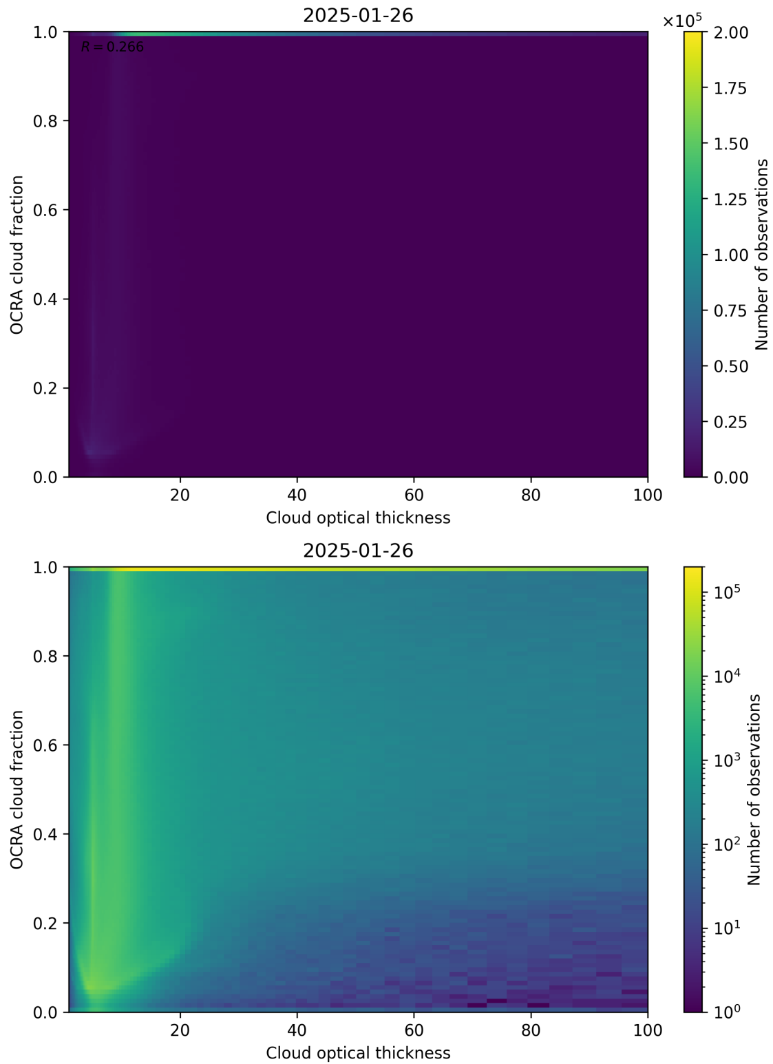
Figure 83: Scatter density plot of “Cloud optical thickness” against “OCRA cloud fraction” for 2025-01-25 to 2025-01-27.
