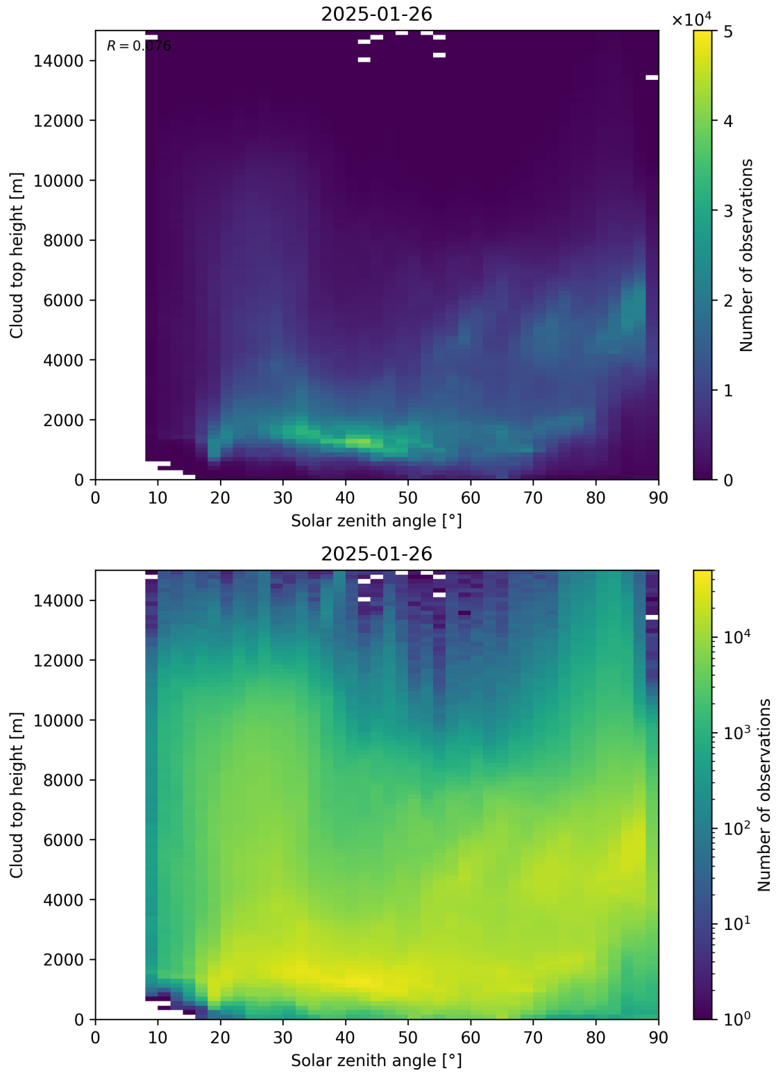
Figure 104: Scatter density plot of “Solar zenith angle” against “Cloud top height” for 2025-01-25 to 2025-01-27.
