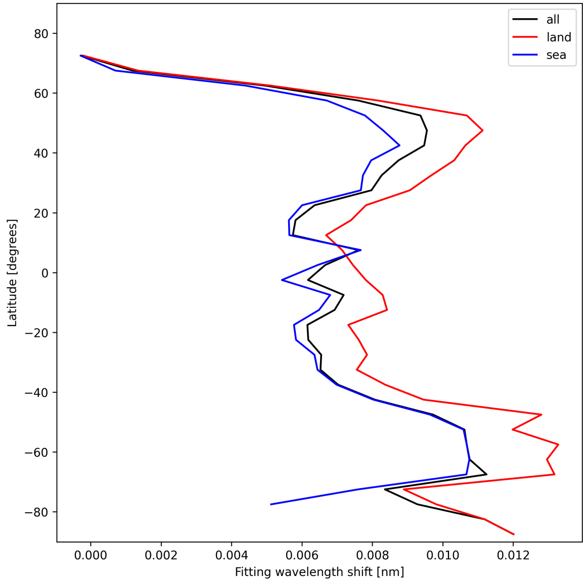
Figure 33: Zonal average of “Fitting wavelength shift” for 2025-01-25 to 2025-01-27.
