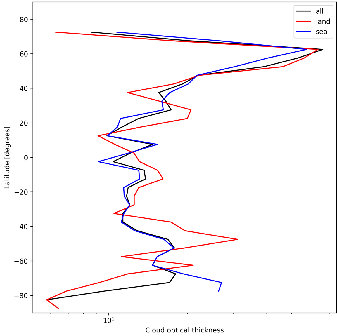
Figure 25: Zonal average of “Cloud optical thickness” for 2025-01-25 to 2025-01-27.
