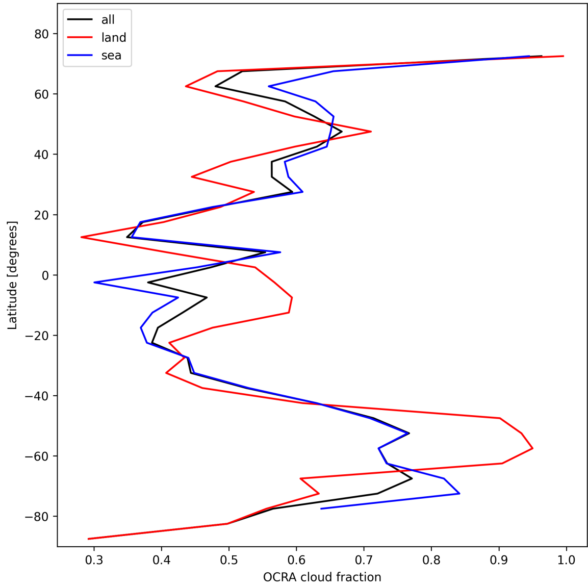
Figure 34: Zonal average of “OCRA cloud fraction” for 2025-01-25 to 2025-01-27.
