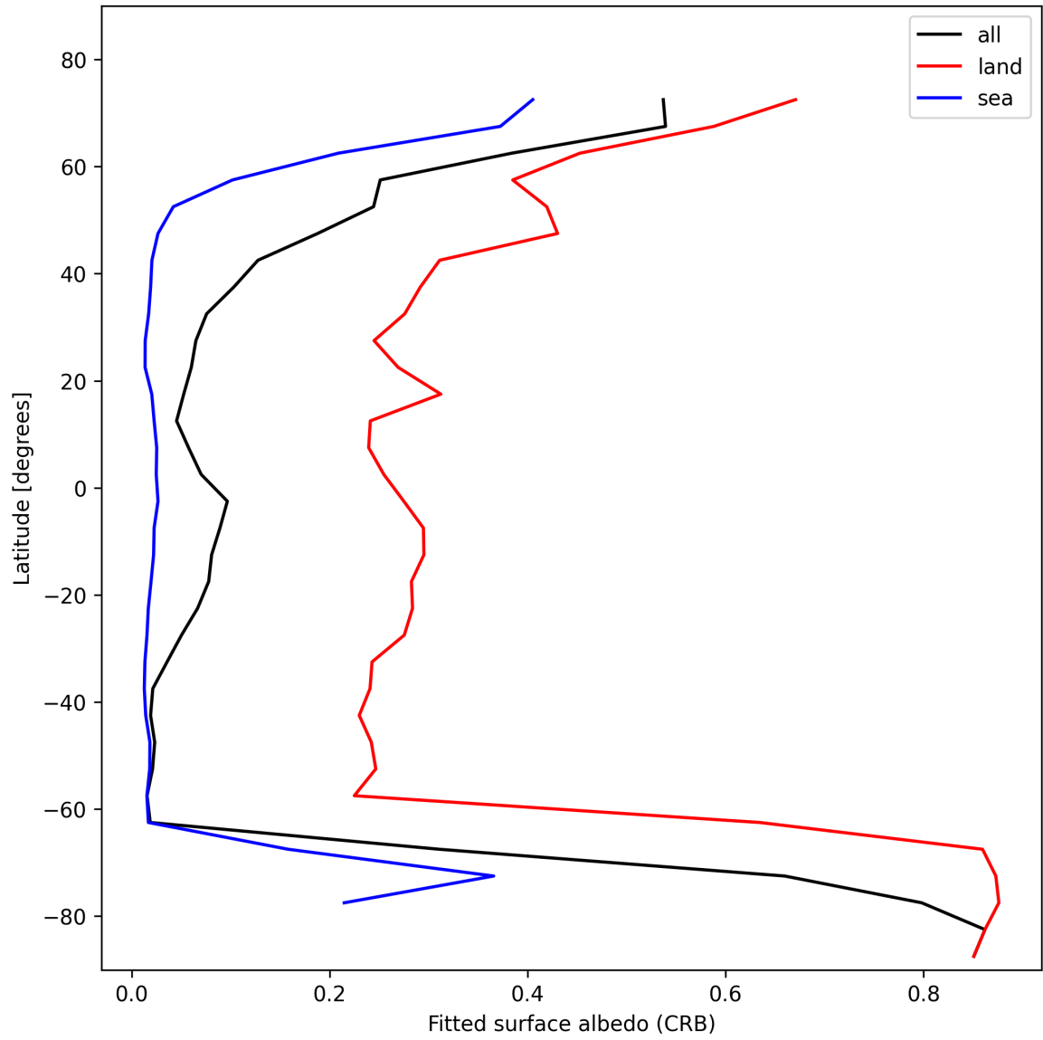
Figure 30: Zonal average of “Fitted surface albedo (CRB)” for 2025-01-25 to 2025-01-27.
