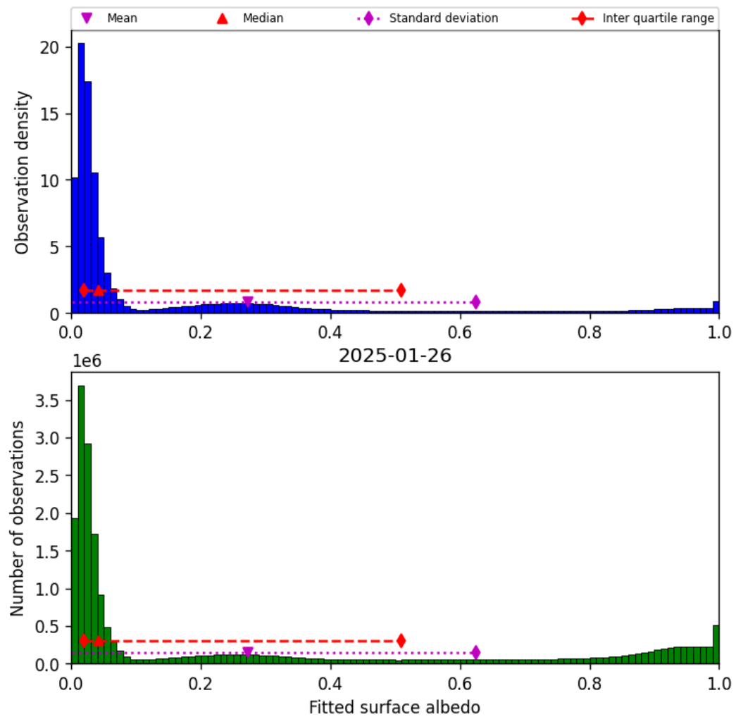
Figure 45: Histogram of “Fitted surface albedo” for 2025-01-25 to 2025-01-27
