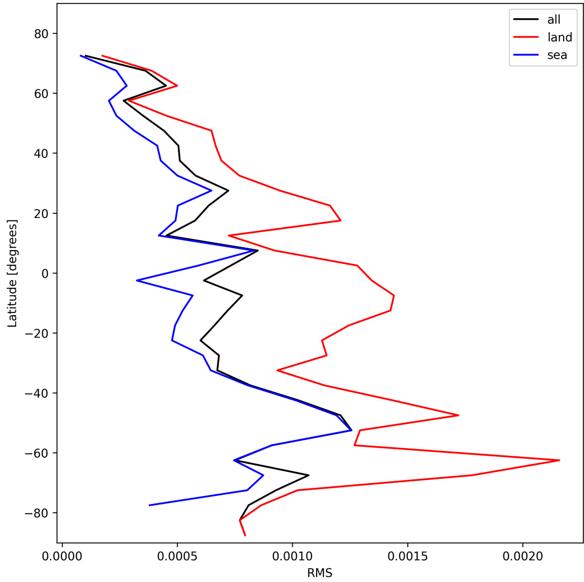
Figure 31: Zonal average of “RMS” for 2025-01-25 to 2025-01-27.
