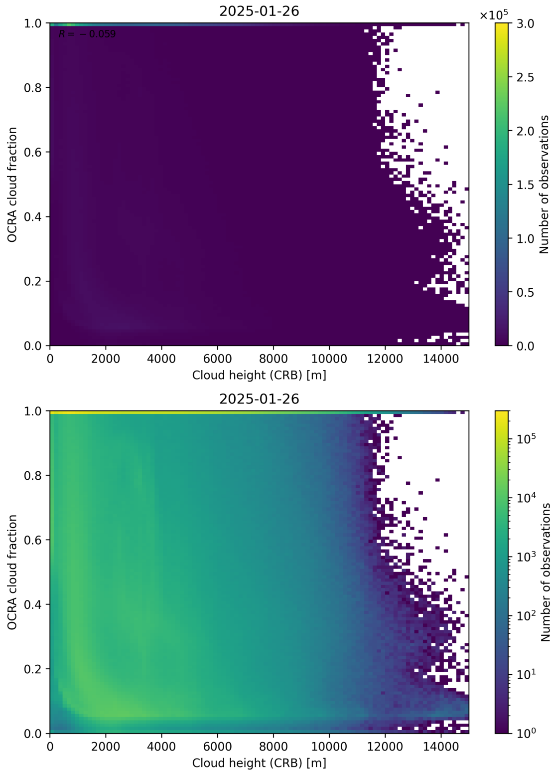
Figure 81: Scatter density plot of “Cloud height (CRB)” against “OCRA cloud fraction” for 2025-01-25 to 2025-01-27.
