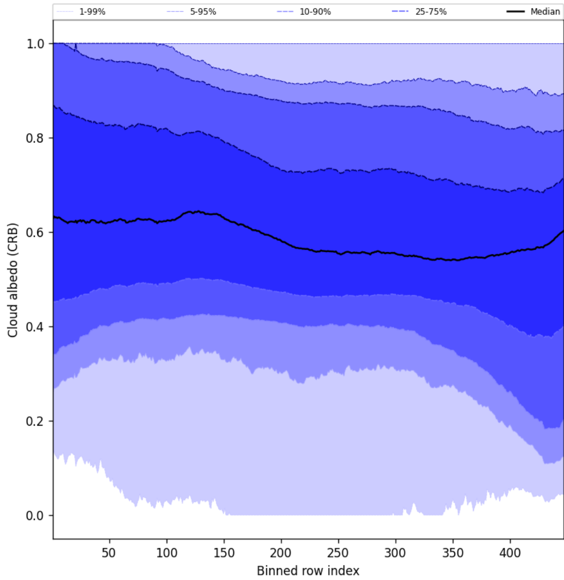
Figure 60: Along track statistics of “Cloud albedo (CRB)” for 2025-01-25 to 2025-01-27
