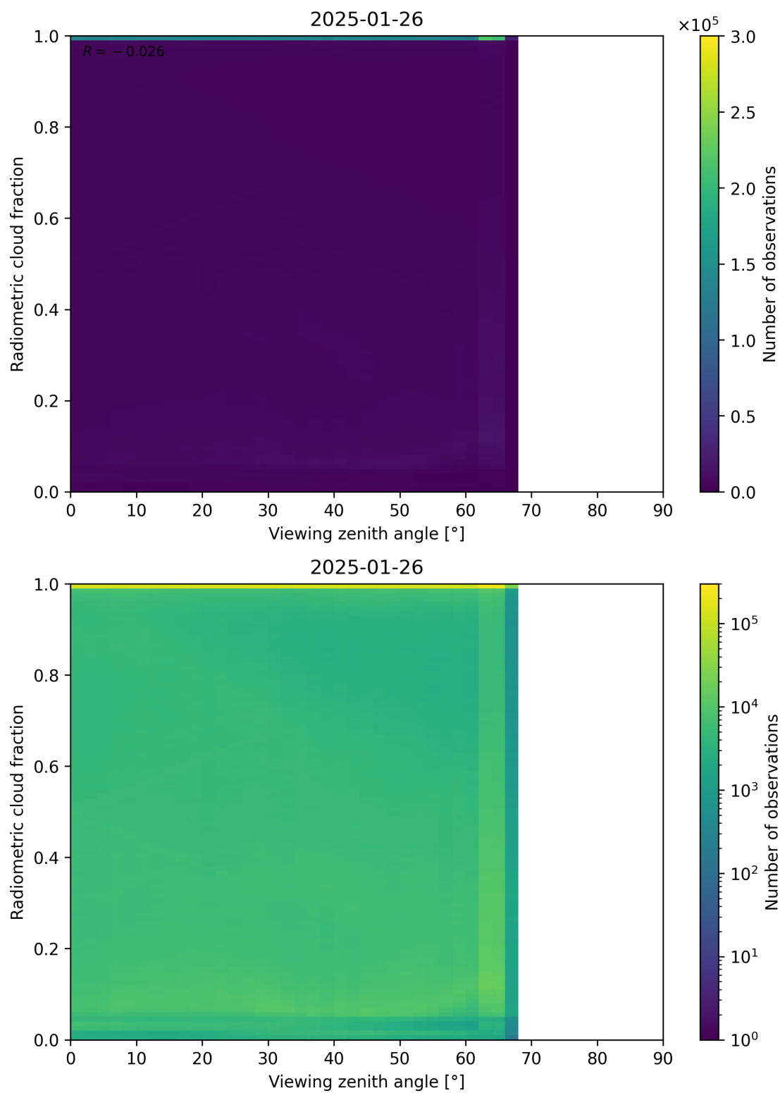
Figure 107: Scatter density plot of “Viewing zenith angle” against “Radiometric cloud fraction” for 2025-01-25 to 2025-01-27.
