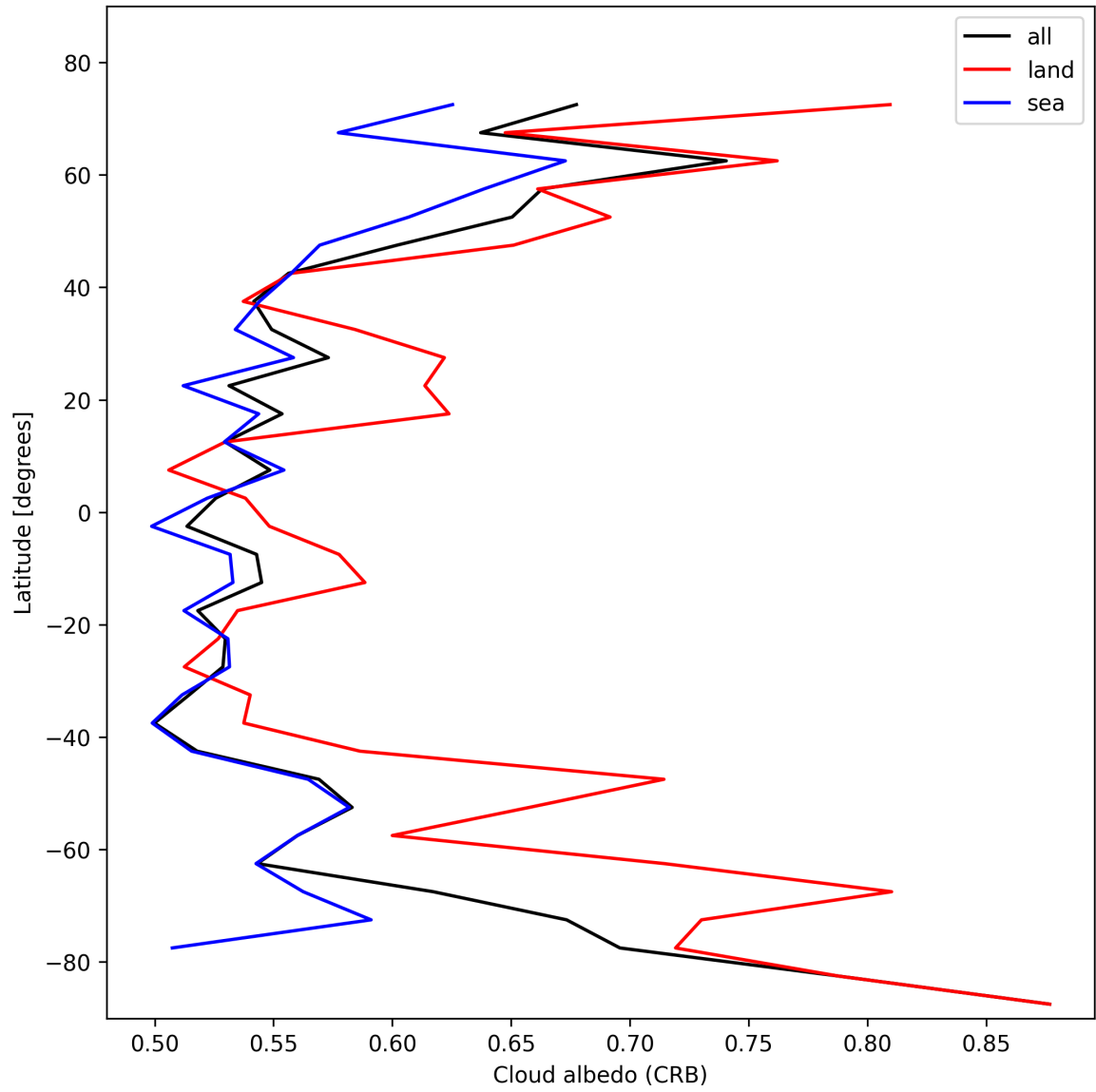
Figure 28: Zonal average of “Cloud albedo (CRB)” for 2025-01-25 to 2025-01-27.
