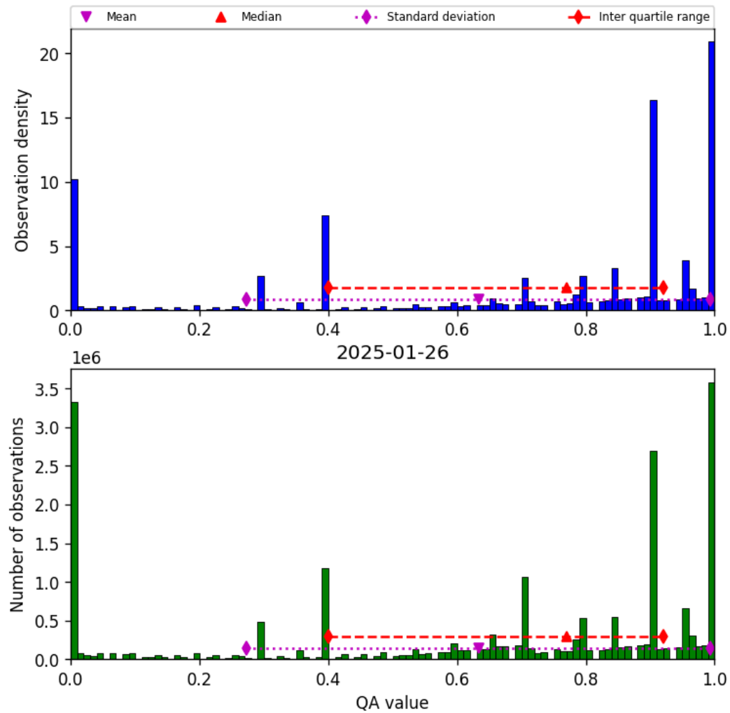
Figure 38: Histogram of “QA value” for 2025-01-25 to 2025-01-27
