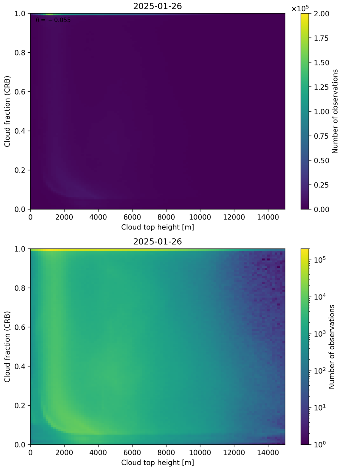
Figure 88: Scatter density plot of “Cloud top height” against “Cloud fraction (CRB)” for 2025-01-25 to 2025-01-27.
