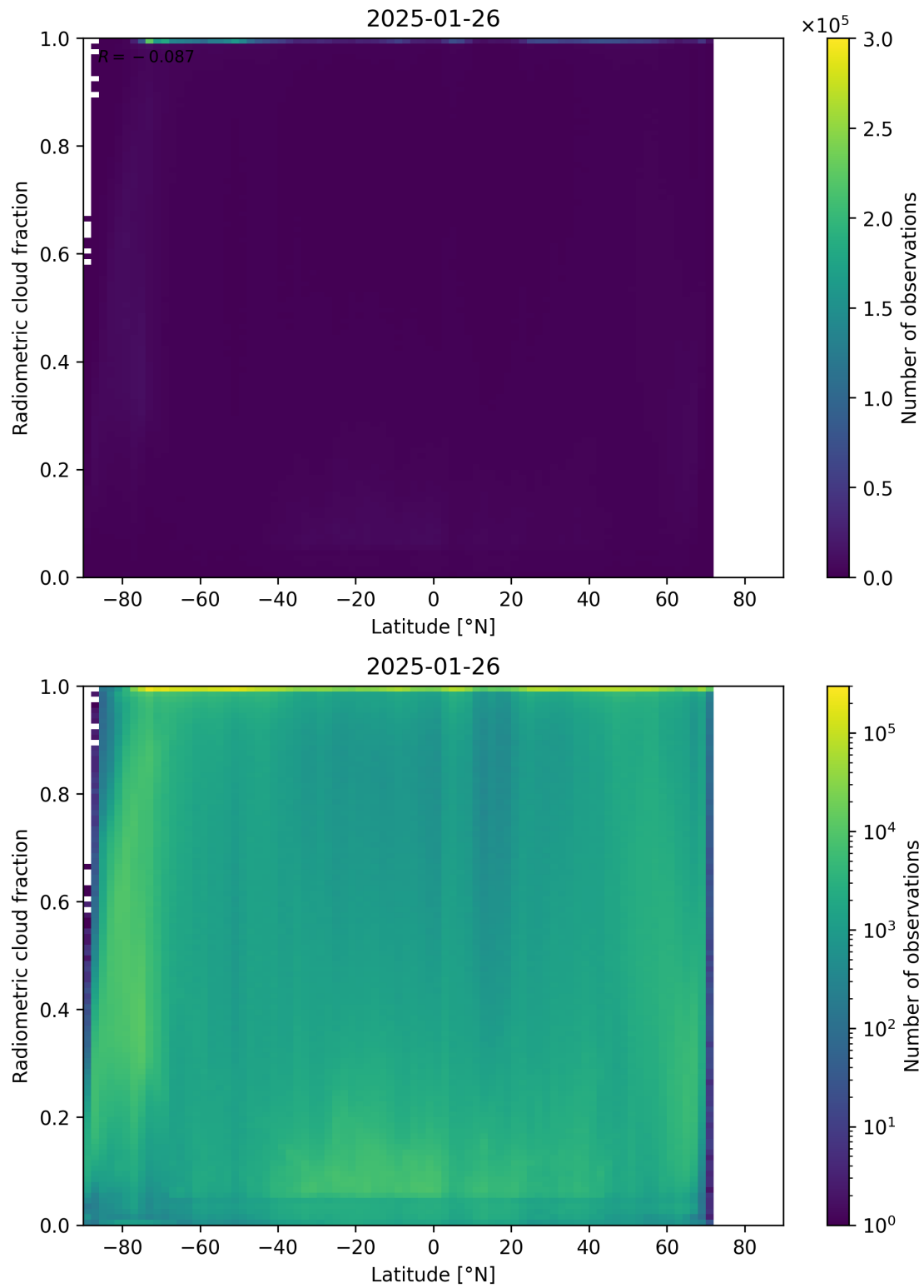
Figure 92: Scatter density plot of “Latitude” against “Radiometric cloud fraction” for 2025-01-25 to 2025-01-27.
