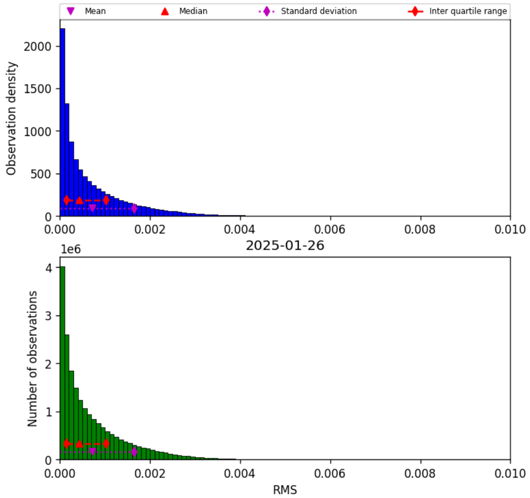
Figure 47: Histogram of “RMS” for 2025-01-25 to 2025-01-27
