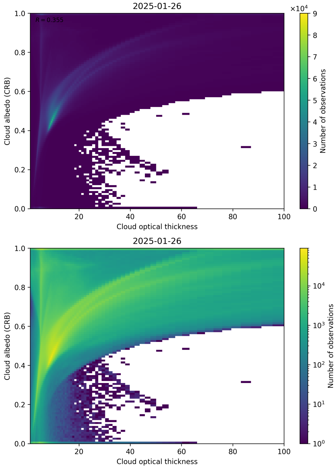
Figure 82: Scatter density plot of “Cloud optical thickness” against “Cloud albedo (CRB)” for 2025-01-25 to 2025-01-27.
