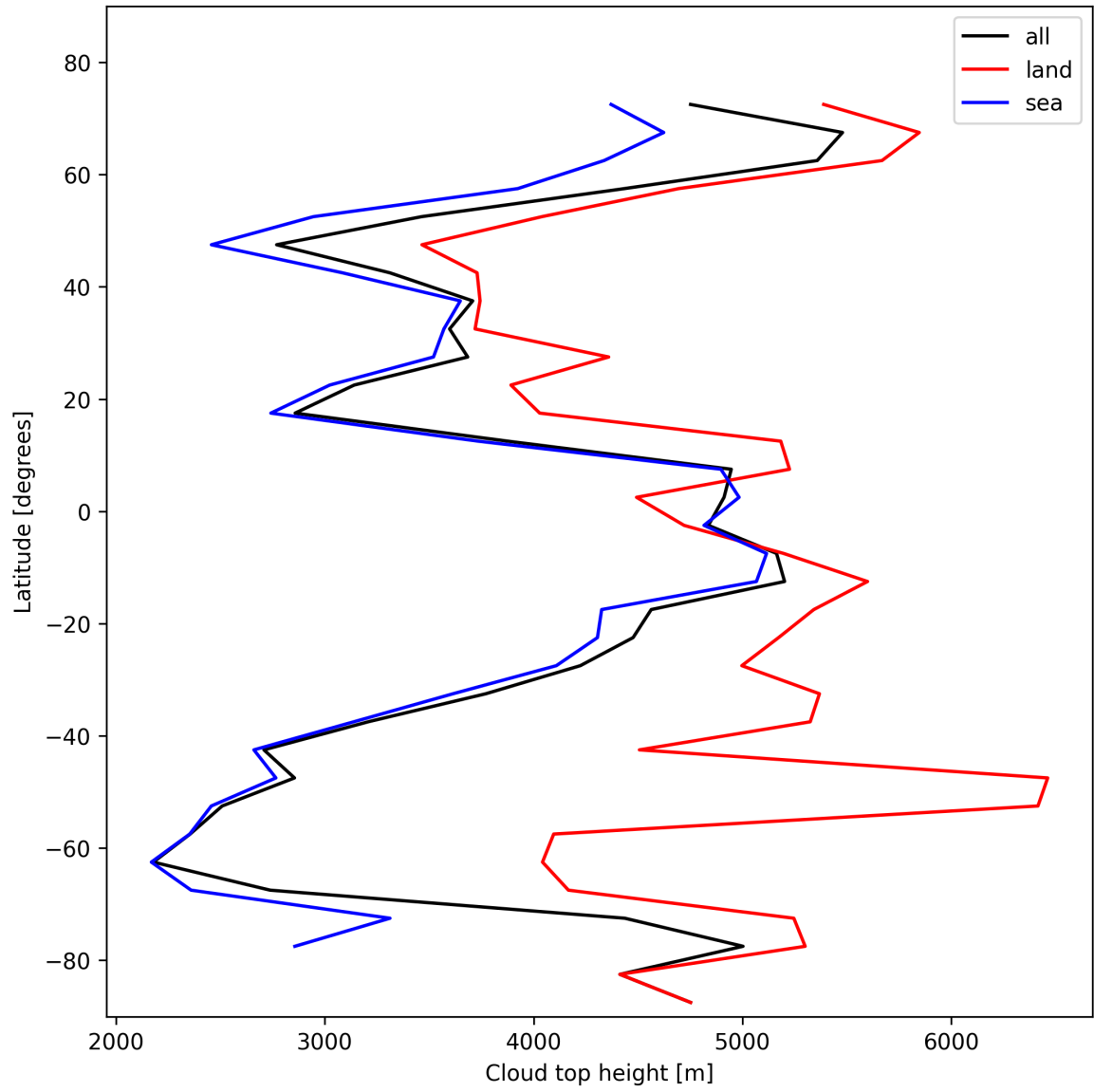
Figure 24: Zonal average of “Cloud top height” for 2025-01-25 to 2025-01-27.
