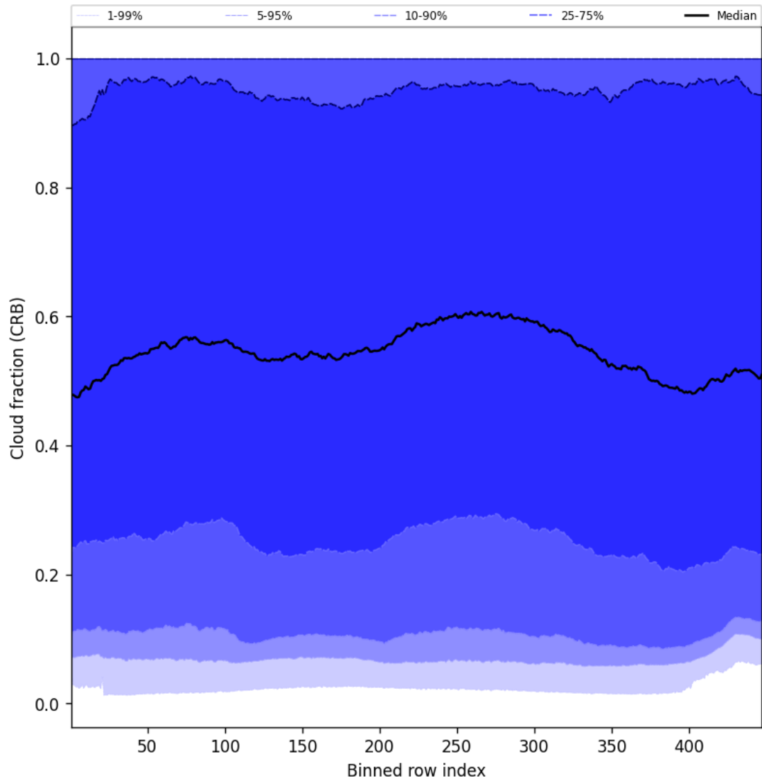
Figure 58: Along track statistics of “Cloud fraction (CRB)” for 2025-01-25 to 2025-01-27
