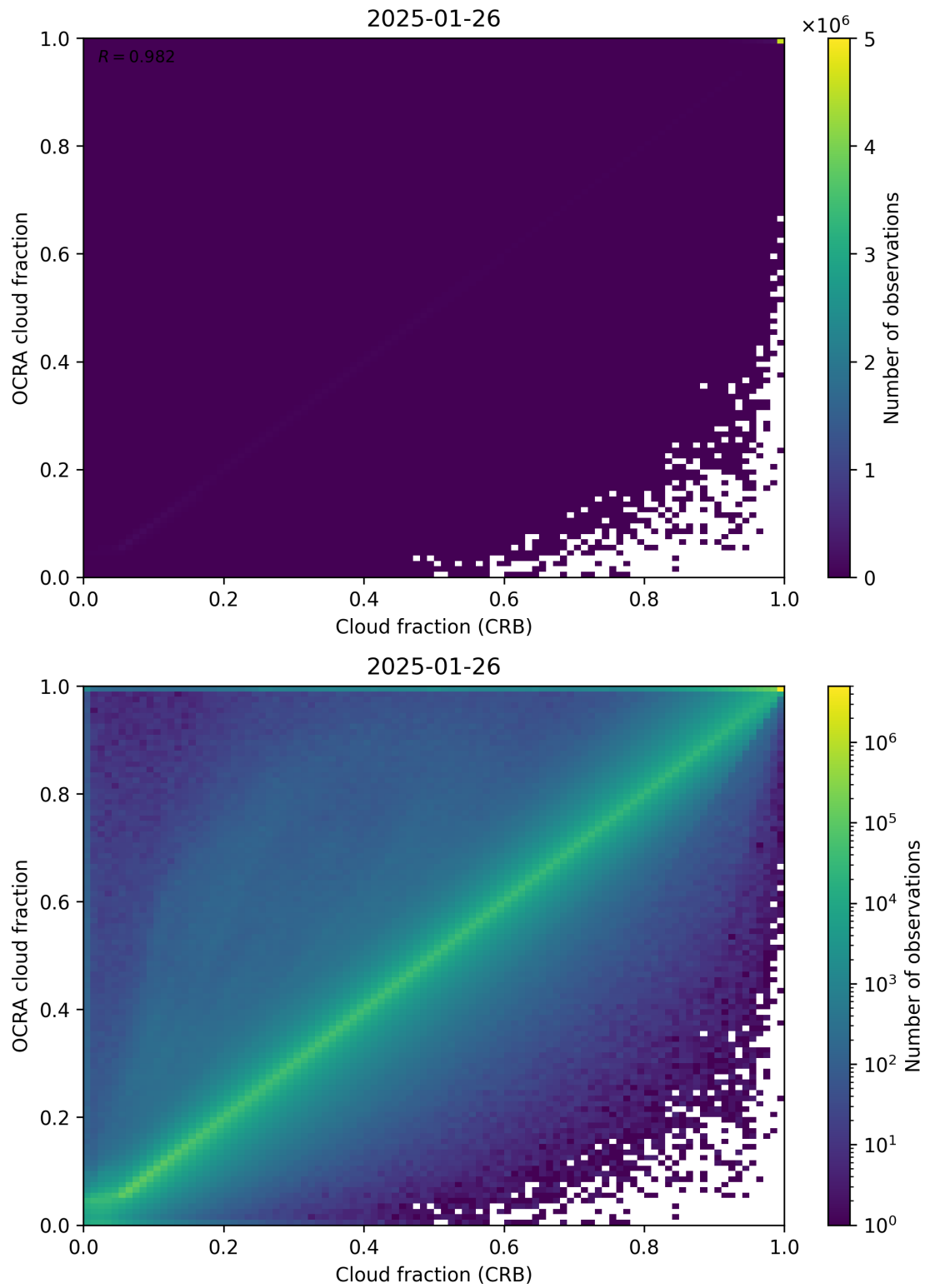
Figure 78: Scatter density plot of “Cloud fraction (CRB)” against “OCRA cloud fraction” for 2025-01-25 to 2025-01-27.
