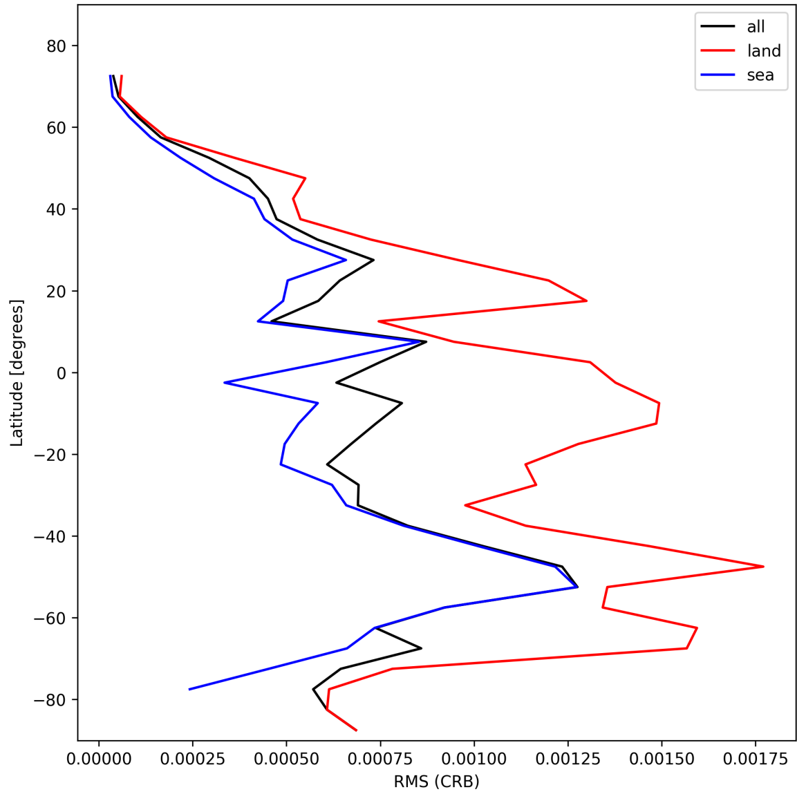
Figure 32: Zonal average of “RMS (CRB)” for 2025-01-25 to 2025-01-27.
