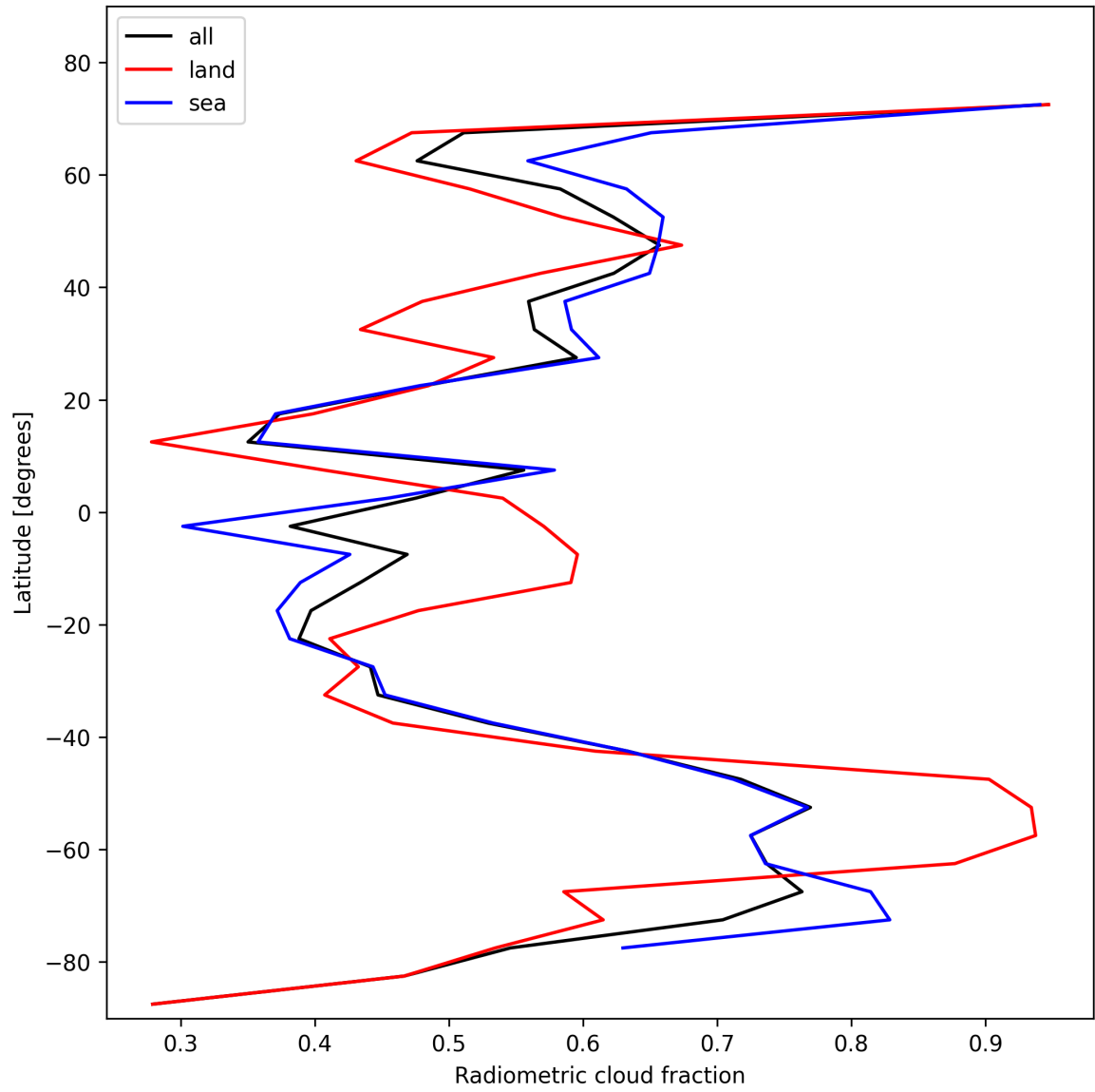
Figure 23: Zonal average of “Radiometric cloud fraction” for 2025-01-25 to 2025-01-27.
