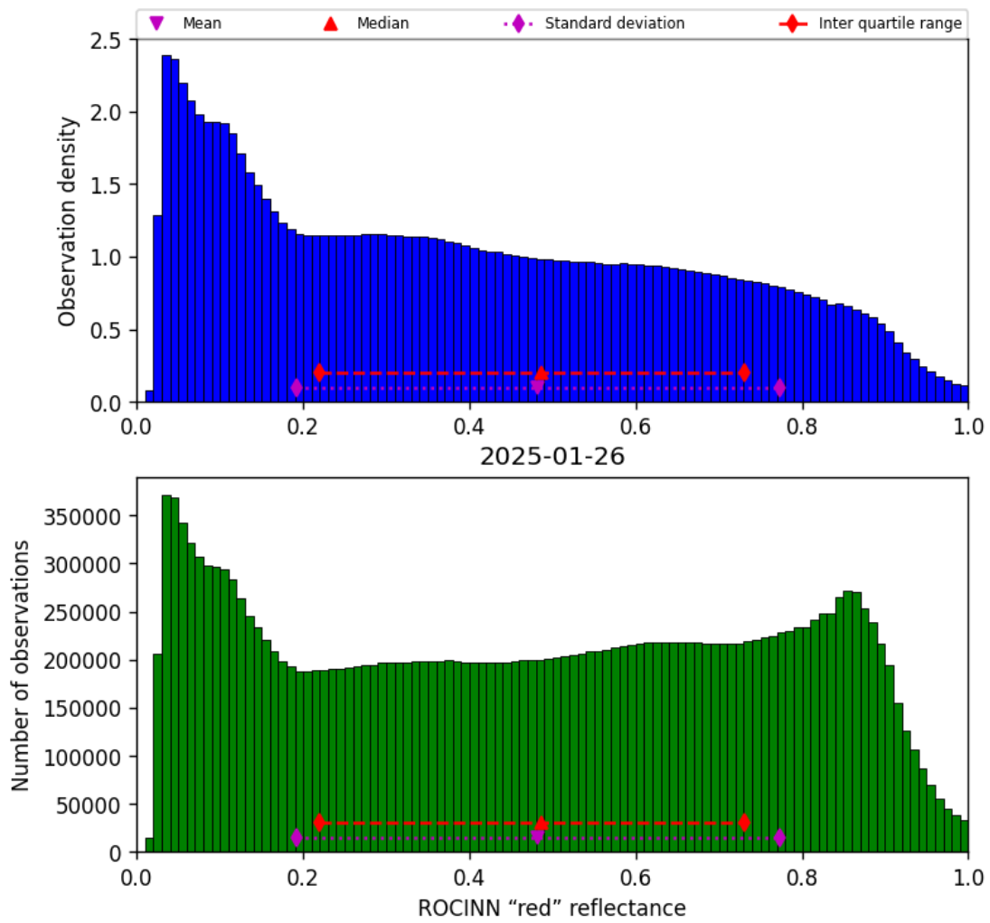
Figure 53: Histogram of “ROCINN “red” reflectance” for 2025-01-25 to 2025-01-27
