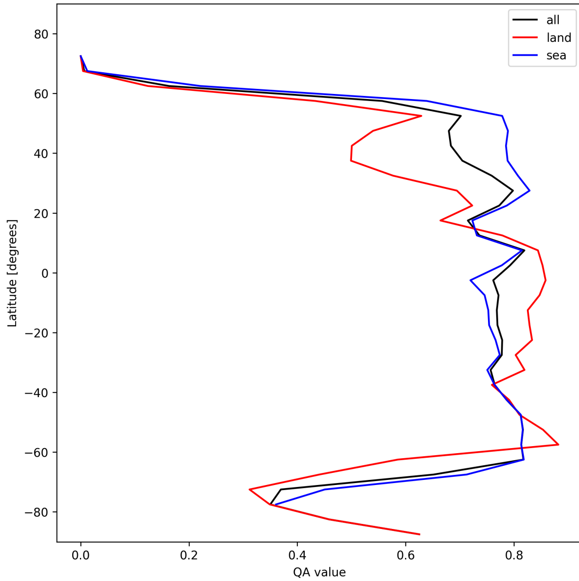
Figure 22: Zonal average of “QA value” for 2025-01-25 to 2025-01-27.
