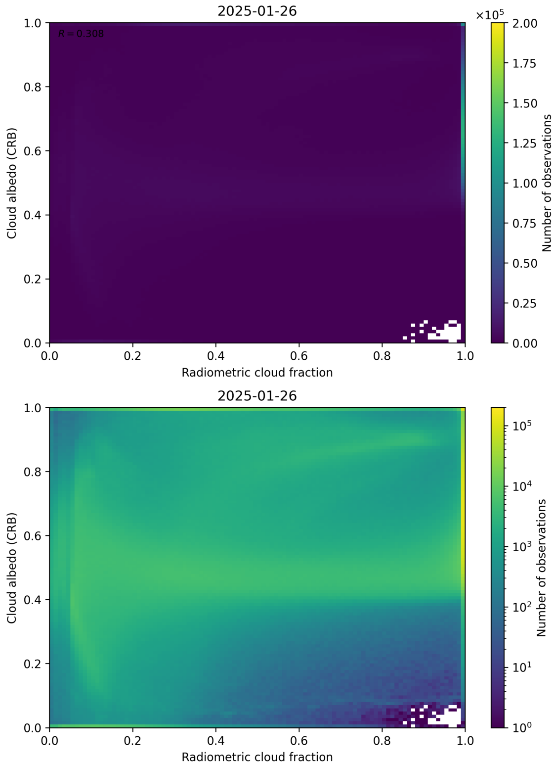
Figure 71: Scatter density plot of “Radiometric cloud fraction” against “Cloud albedo (CRB)” for 2025-01-25 to 2025-01-27.
