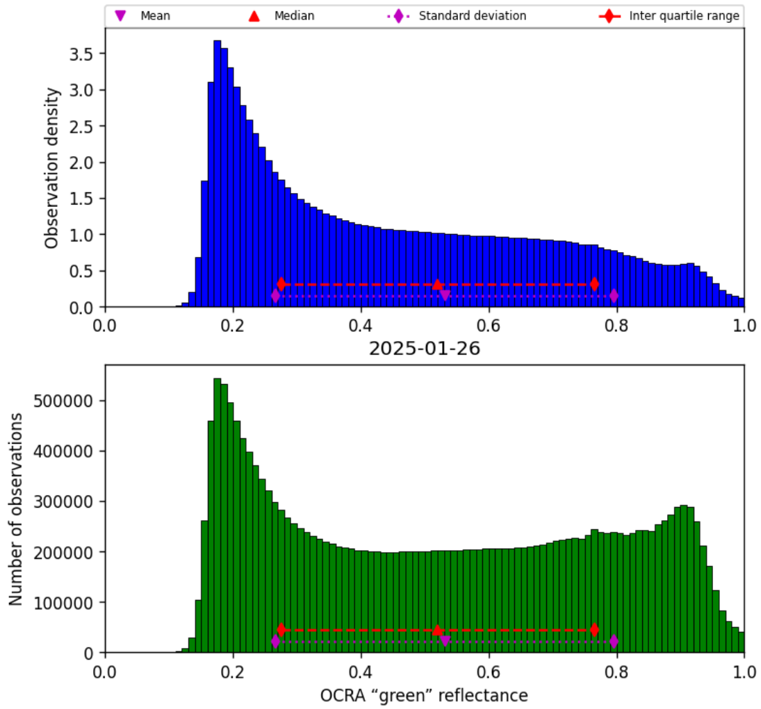
Figure 52: Histogram of “OCRA “green” reflectance” for 2025-01-25 to 2025-01-27
