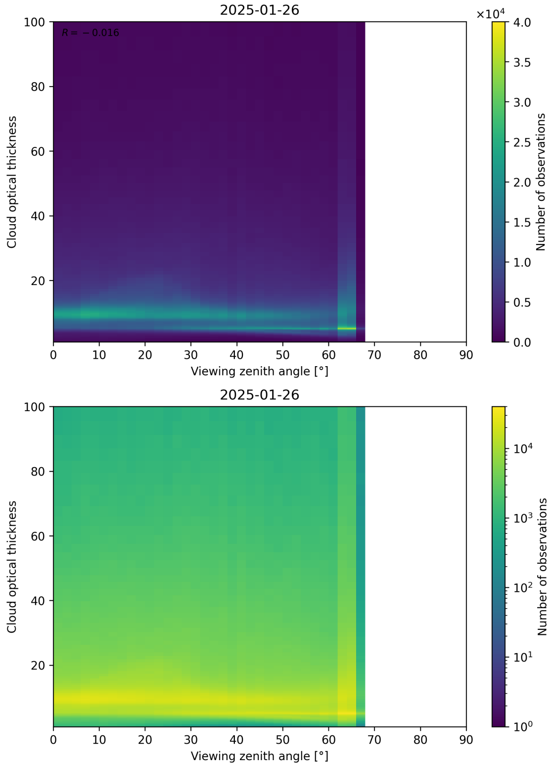
Figure 111: Scatter density plot of “Viewing zenith angle” against “Cloud optical thickness” for 2025-01-25 to 2025-01-27.
