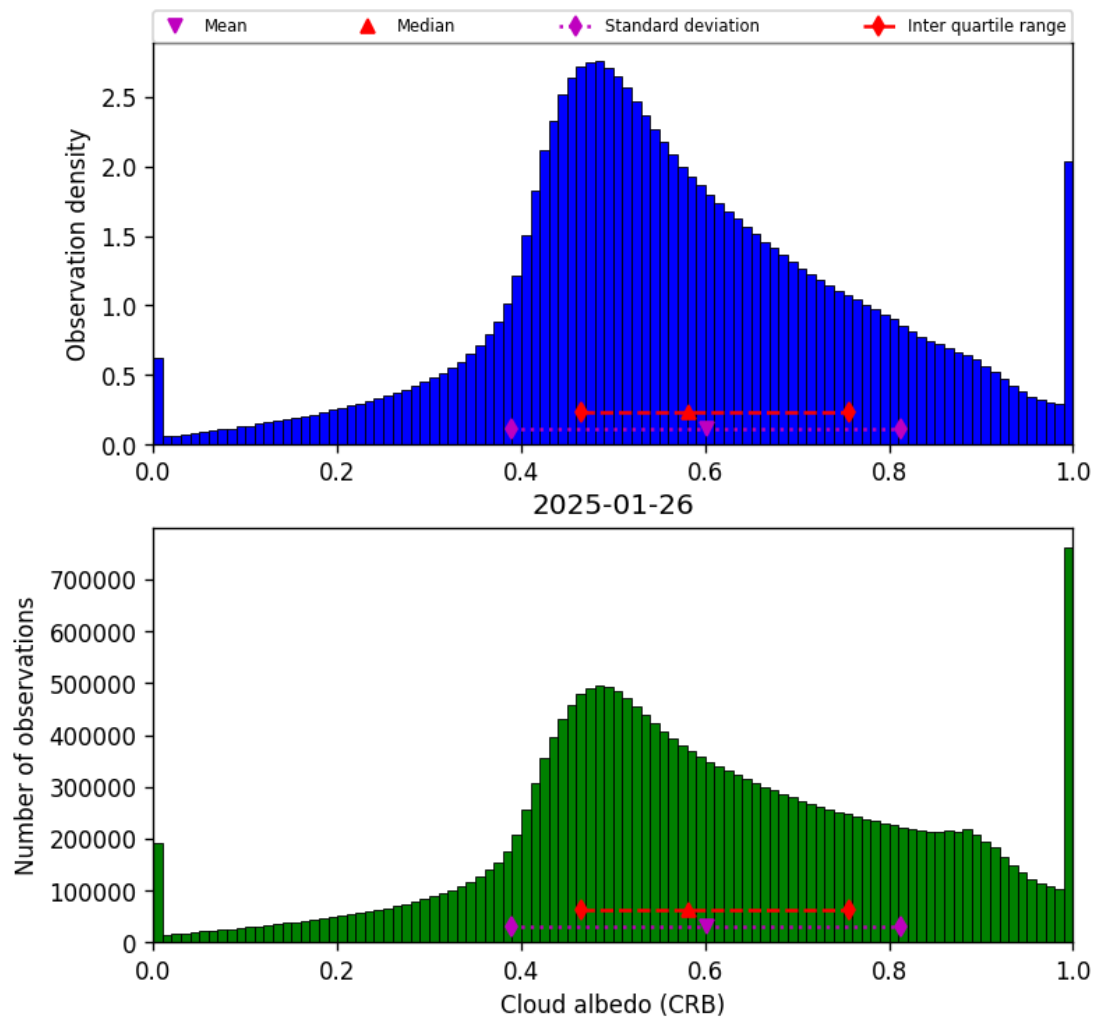
Figure 44: Histogram of “Cloud albedo (CRB)” for 2025-01-25 to 2025-01-27
