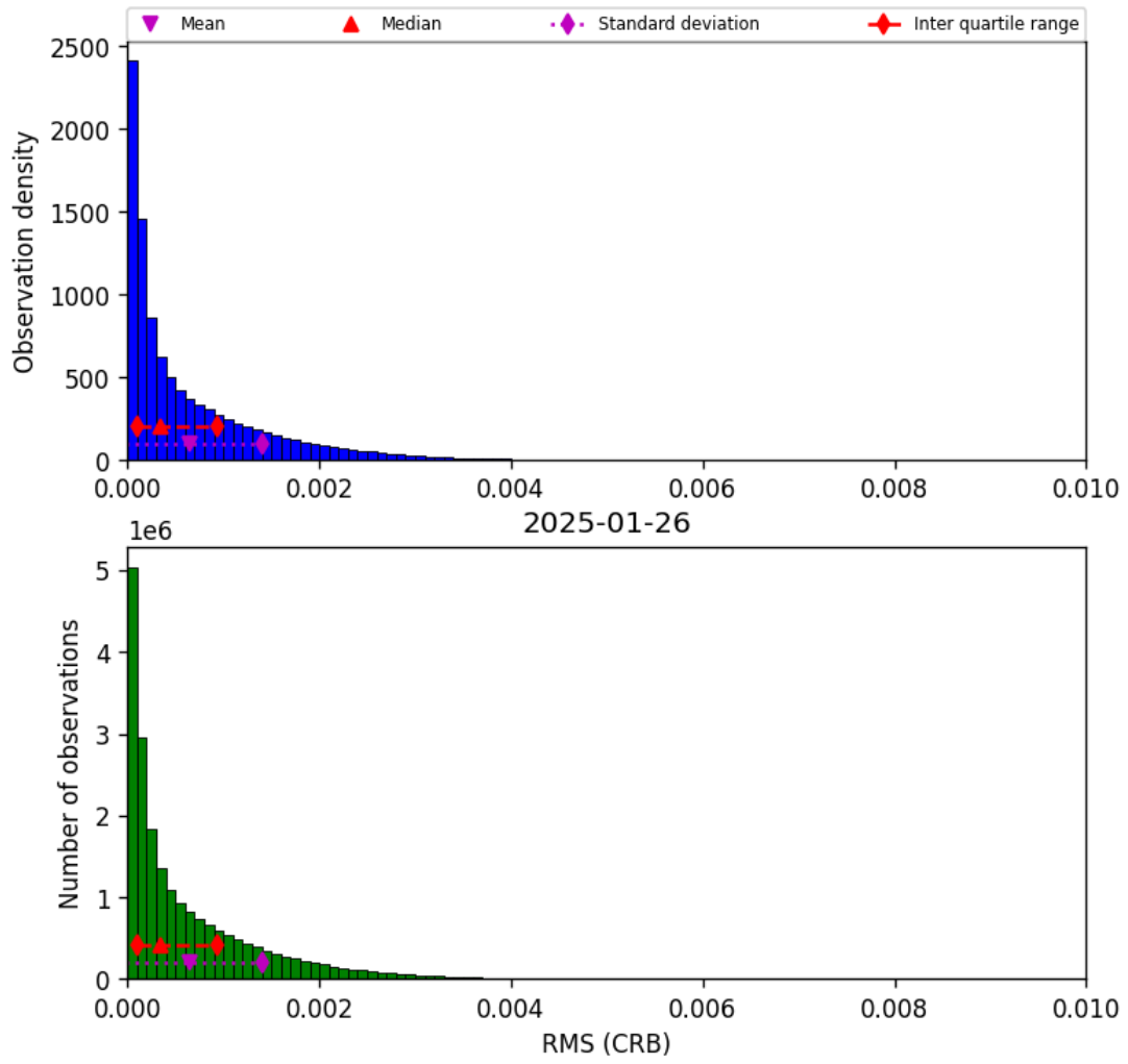
Figure 48: Histogram of “RMS (CRB)” for 2025-01-25 to 2025-01-27
