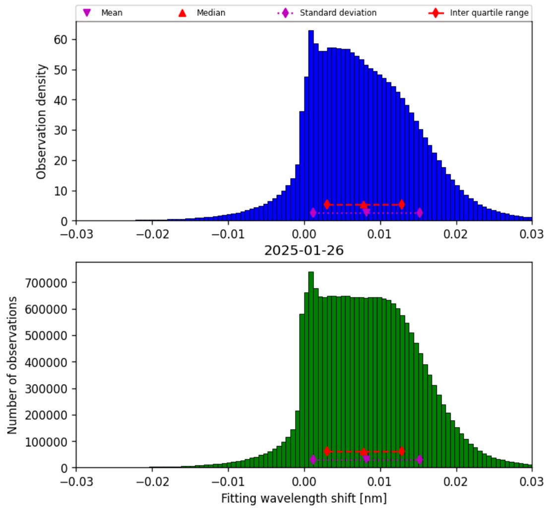
Figure 49: Histogram of “Fitting wavelength shift” for 2025-01-25 to 2025-01-27
