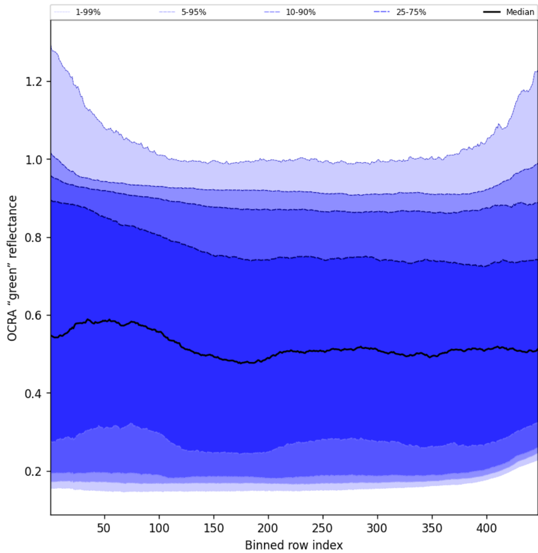
Figure 68: Along track statistics of “OCRA “green” reflectance” for 2025-01-25 to 2025-01-27
