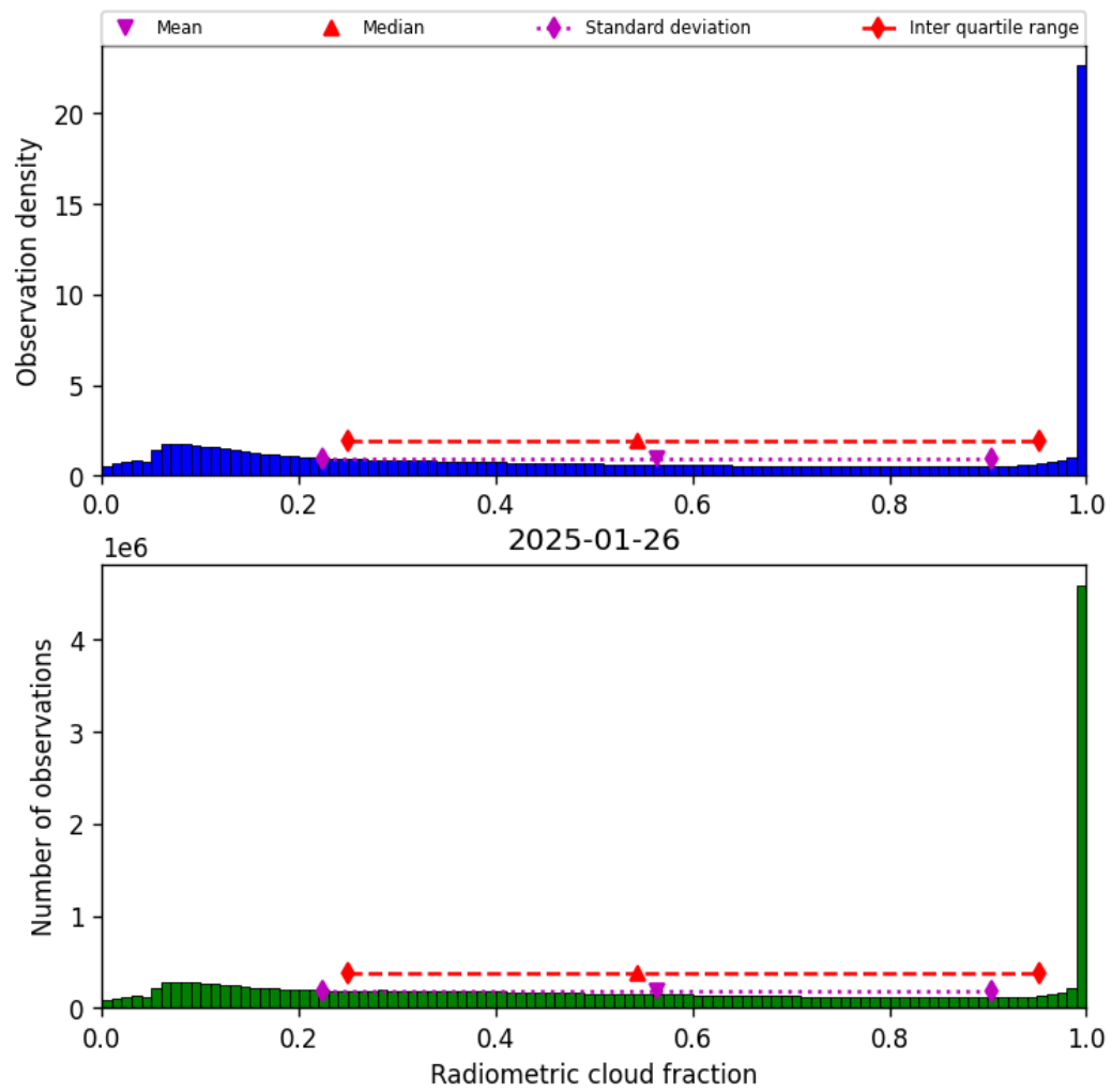
Figure 39: Histogram of “Radiometric cloud fraction” for 2025-01-25 to 2025-01-27
