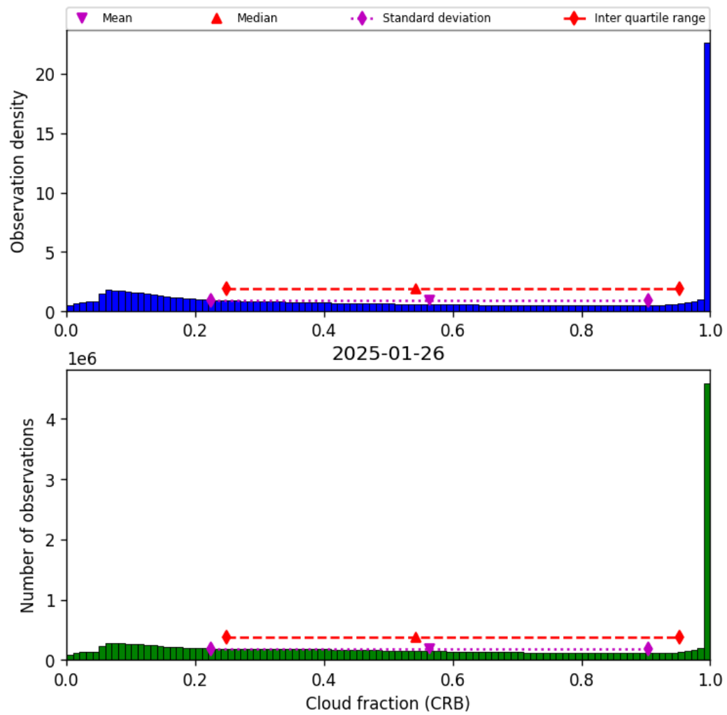
Figure 42: Histogram of “Cloud fraction (CRB)” for 2025-01-25 to 2025-01-27
