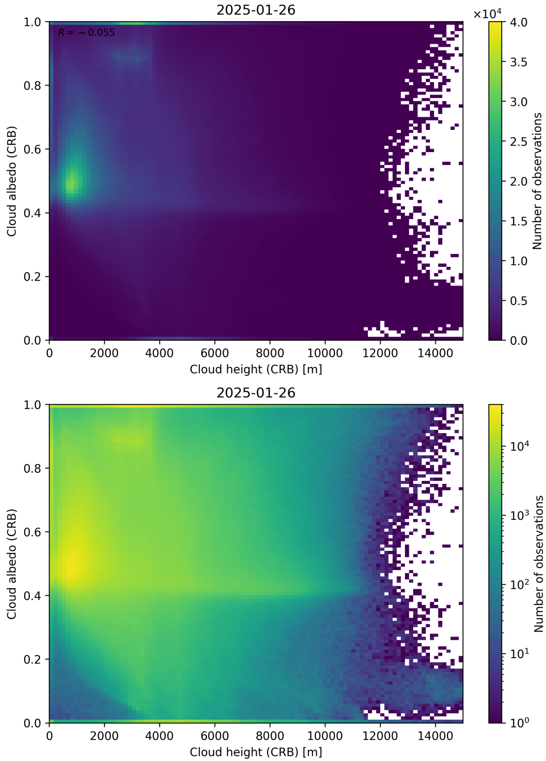
Figure 80: Scatter density plot of “Cloud height (CRB)” against “Cloud albedo (CRB)” for 2025-01-25 to 2025-01-27.
