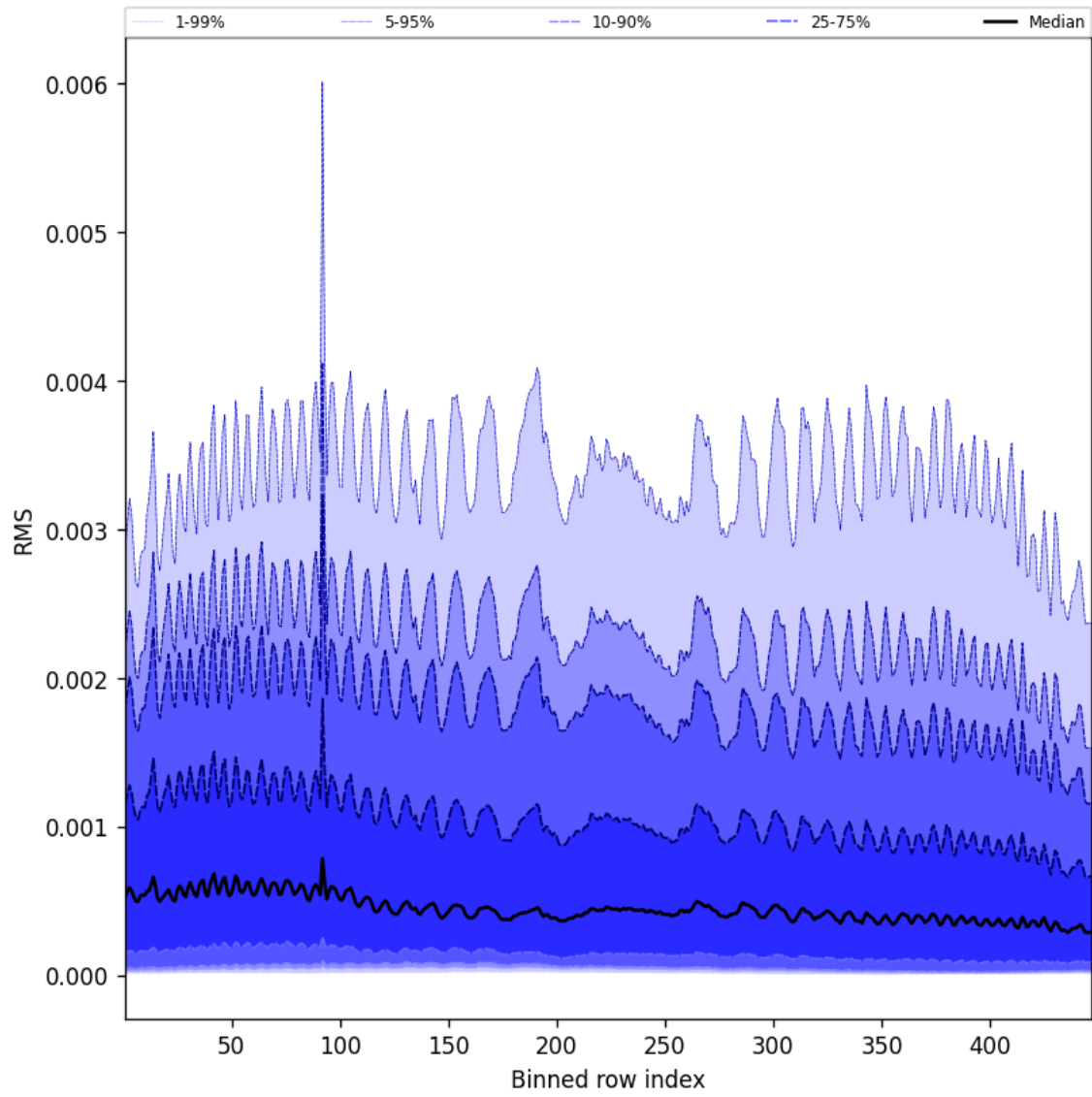
Figure 63: Along track statistics of “RMS” for 2025-01-25 to 2025-01-27
