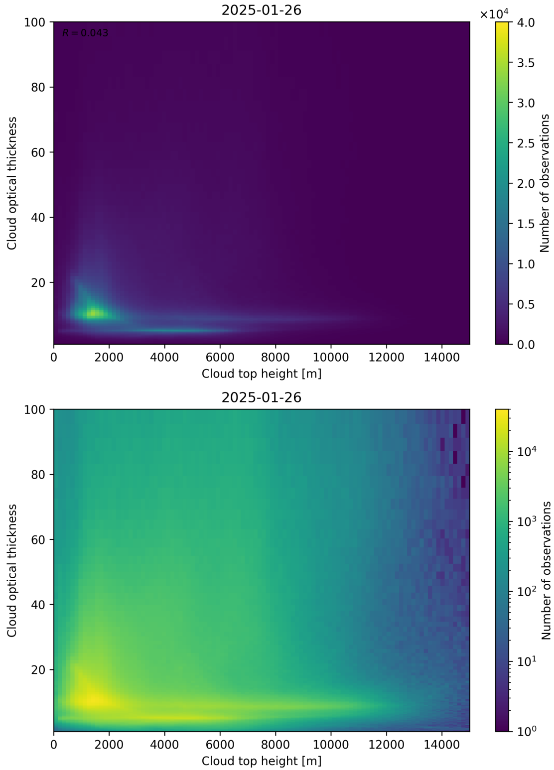
Figure 90: Scatter density plot of “Cloud top height” against “Cloud optical thickness” for 2025-01-25 to 2025-01-27.
