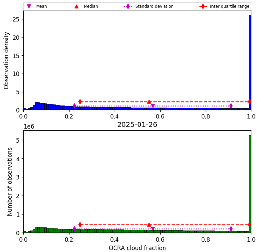
Figure 50: Histogram of “OCRA cloud fraction” for 2025-01-25 to 2025-01-27
