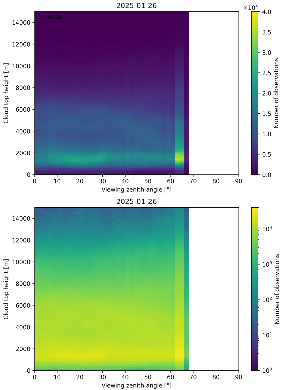
Figure 112: Scatter density plot of “Viewing zenith angle” against “Cloud top height” for 2025-01-25 to 2025-01-27.
