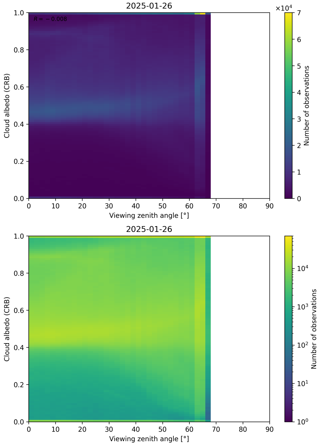
Figure 106: Scatter density plot of “Viewing zenith angle” against “Cloud albedo (CRB)” for 2025-01-25 to 2025-01-27.
