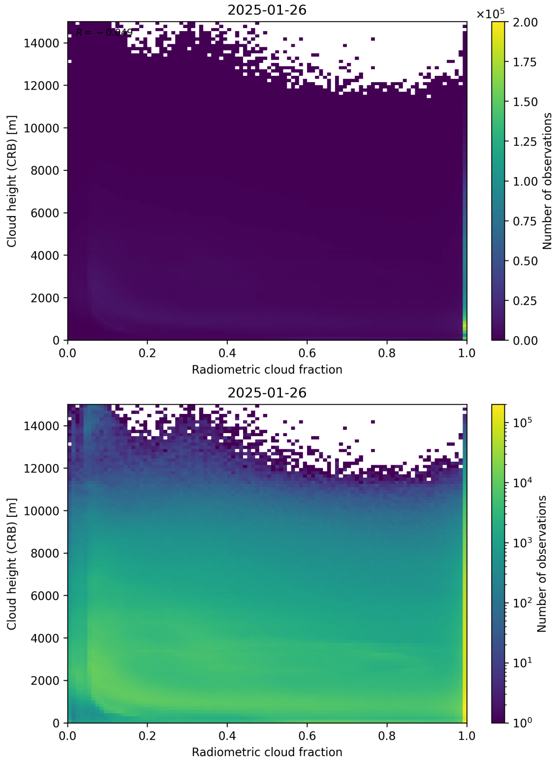
Figure 74: Scatter density plot of “Radiometric cloud fraction” against “Cloud height (CRB)” for 2025-01-25 to 2025-01-27.
