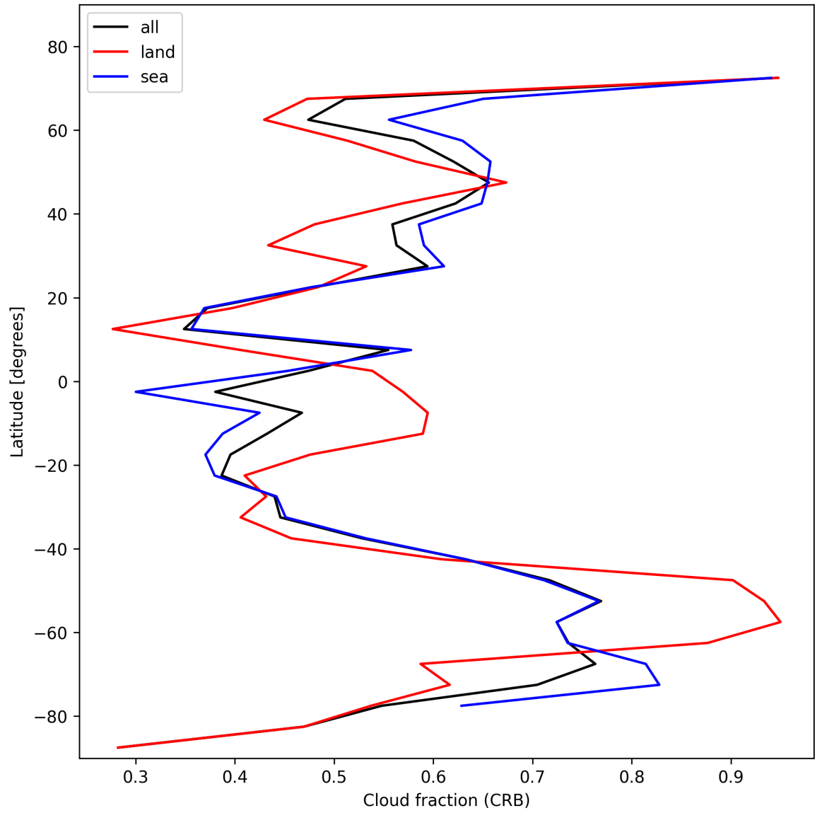
Figure 26: Zonal average of “Cloud fraction (CRB)” for 2025-01-25 to 2025-01-27.
