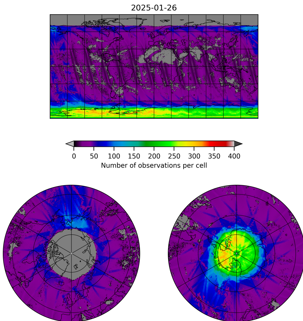
Figure 21: Map of the number of observations for 2025-01-25 to 2025-01-27
