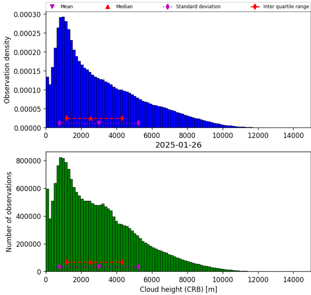
Figure 43: Histogram of “Cloud height (CRB)” for 2025-01-25 to 2025-01-27
