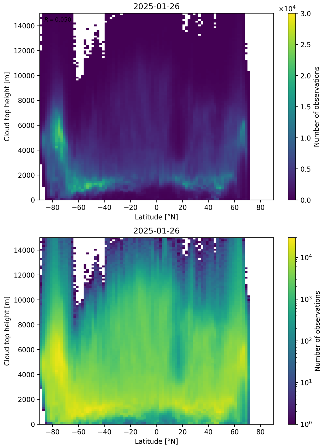
Figure 97: Scatter density plot of “Latitude” against “Cloud top height” for 2025-01-25 to 2025-01-27.
