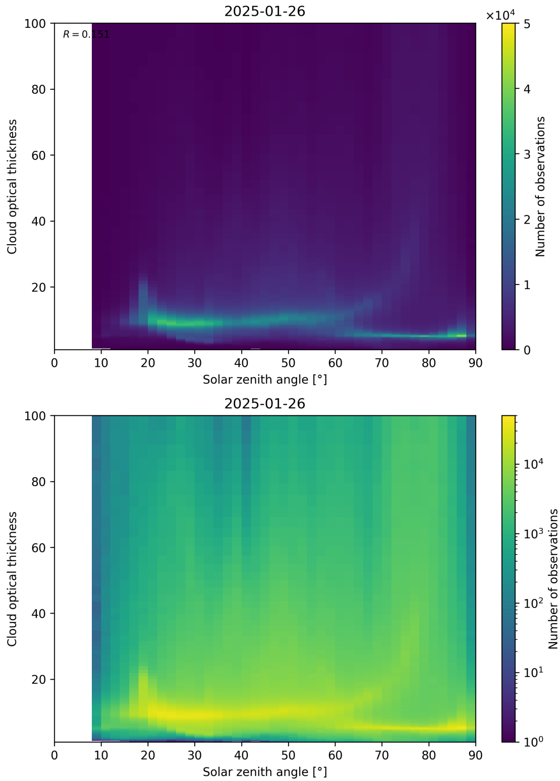
Figure 103: Scatter density plot of “Solar zenith angle” against “Cloud optical thickness” for 2025-01-25 to 2025-01-27.
