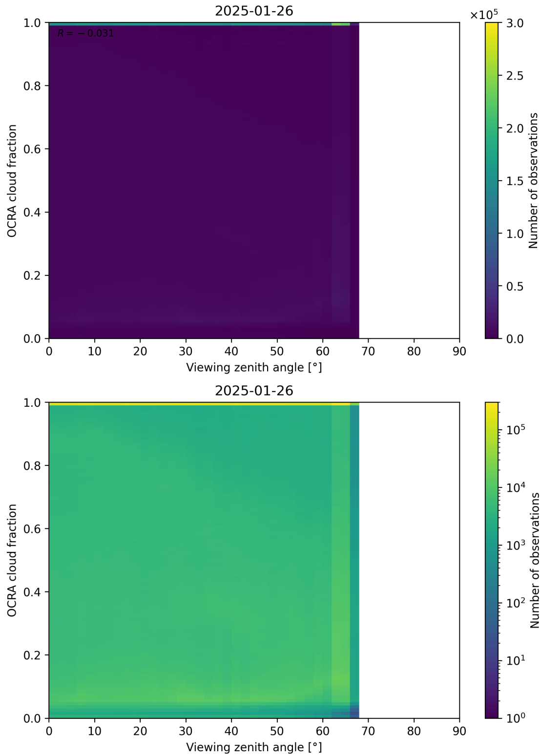
Figure 108: Scatter density plot of “Viewing zenith angle” against “OCRA cloud fraction” for 2025-01-25 to 2025-01-27.
