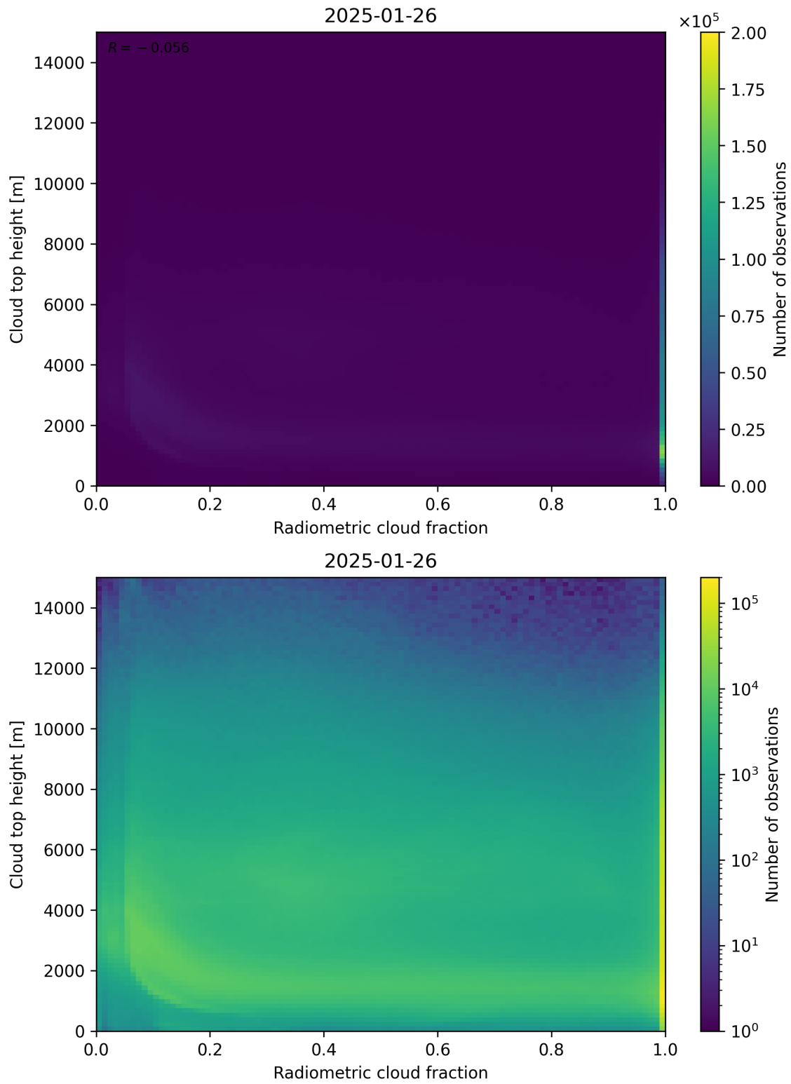
Figure 76: Scatter density plot of “Radiometric cloud fraction” against “Cloud top height” for 2025-01-25 to 2025-01-27.
