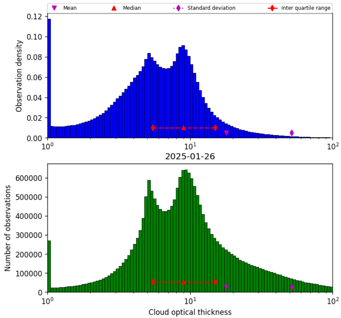
Figure 41: Histogram of “Cloud optical thickness” for 2025-01-25 to 2025-01-27
