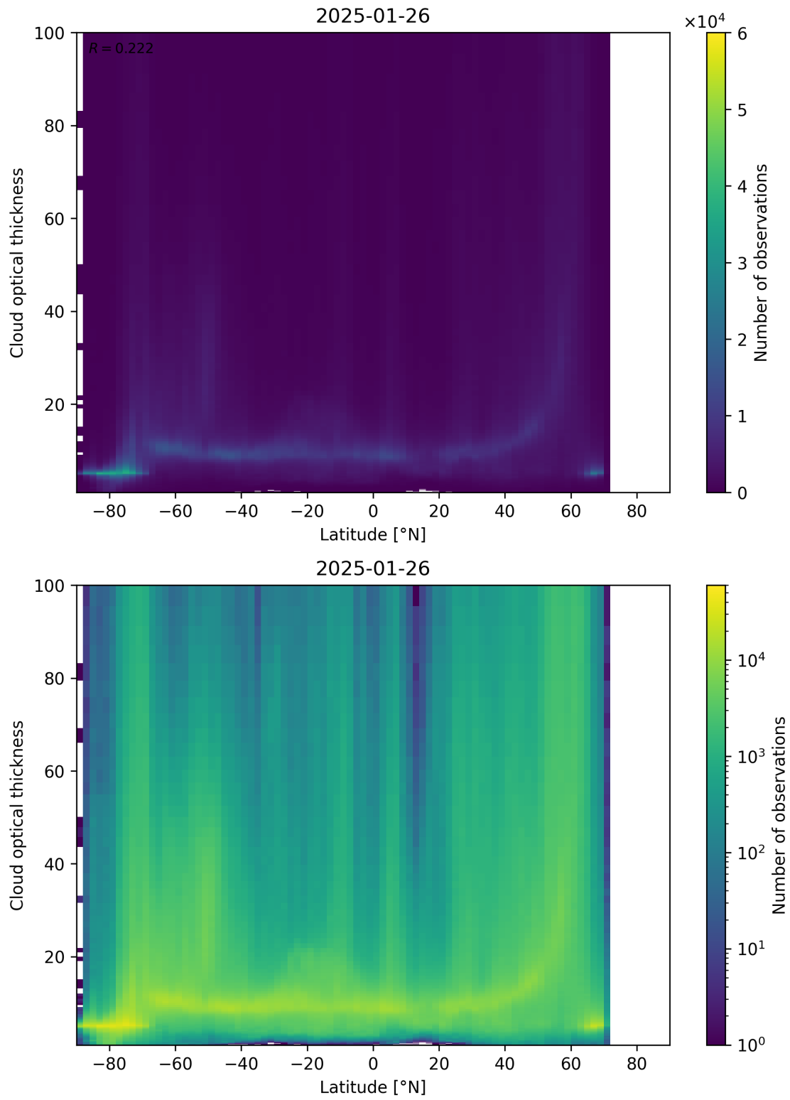
Figure 96: Scatter density plot of “Latitude” against “Cloud optical thickness” for 2025-01-25 to 2025-01-27.
