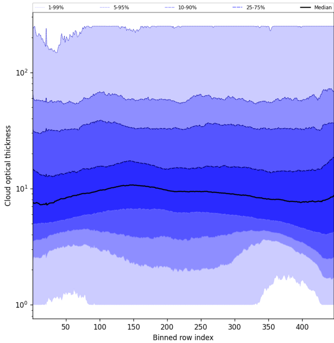
Figure 57: Along track statistics of “Cloud optical thickness” for 2025-01-25 to 2025-01-27
