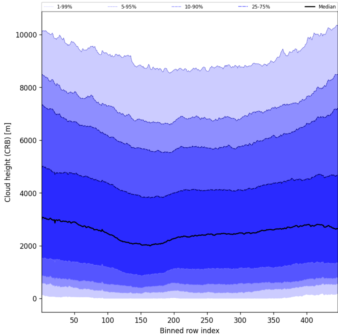
Figure 59: Along track statistics of “Cloud height (CRB)” for 2025-01-25 to 2025-01-27
