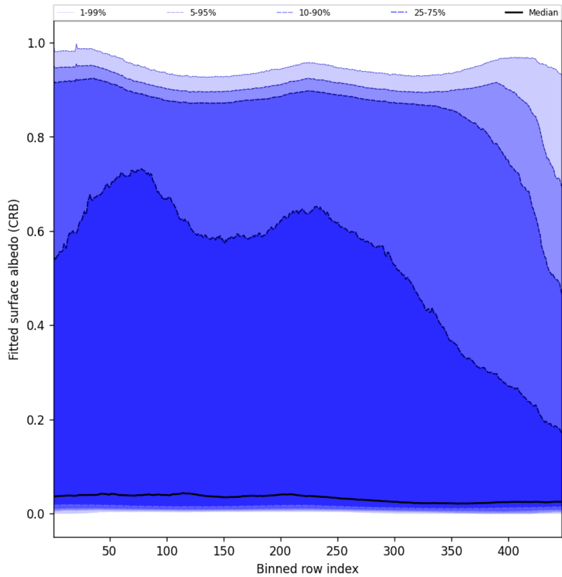
Figure 62: Along track statistics of “Fitted surface albedo (CRB)” for 2025-01-25 to 2025-01-27
