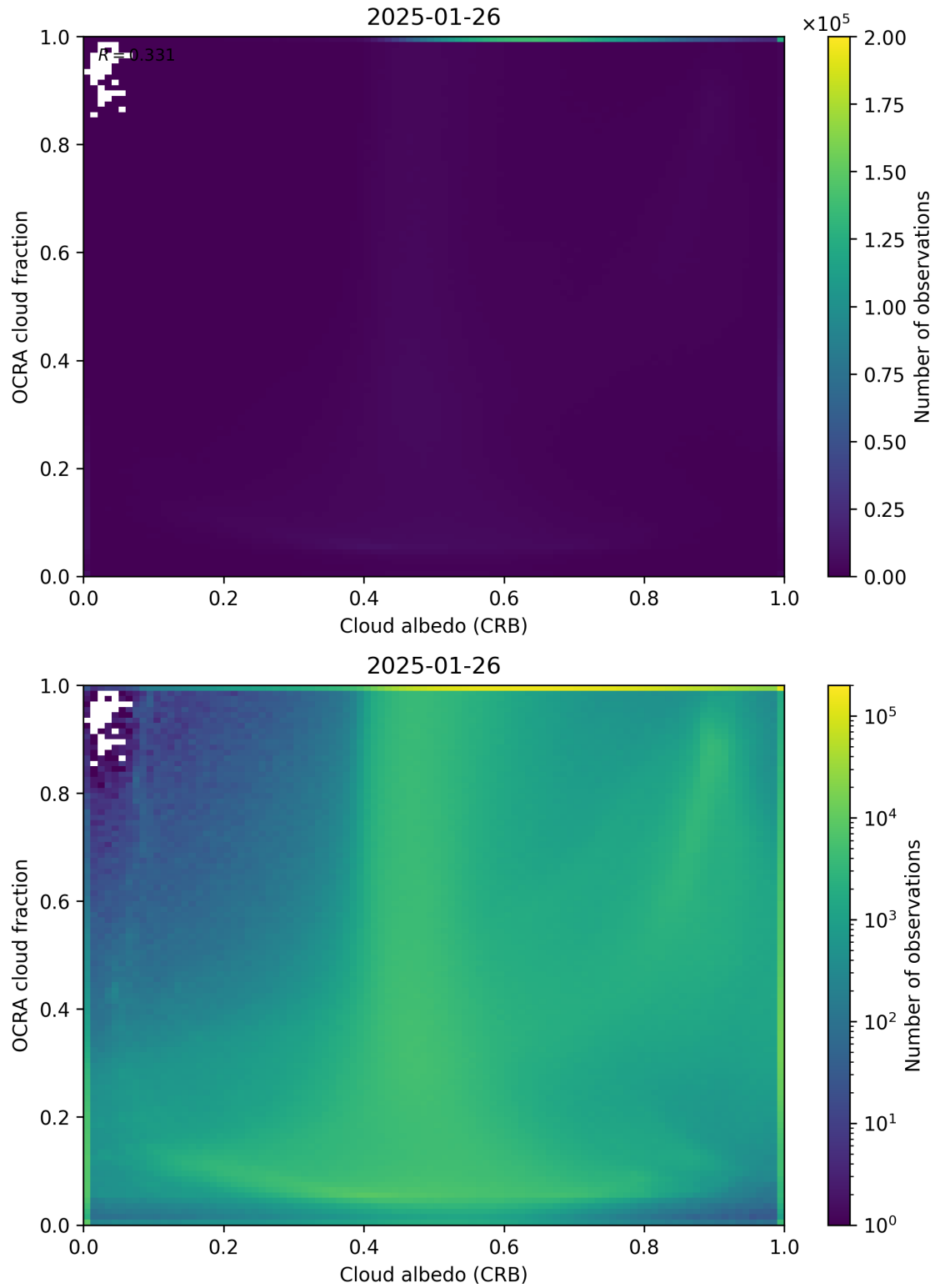
Figure 70: Scatter density plot of “Cloud albedo (CRB)” against “OCRA cloud fraction” for 2025-01-25 to 2025-01-27.
