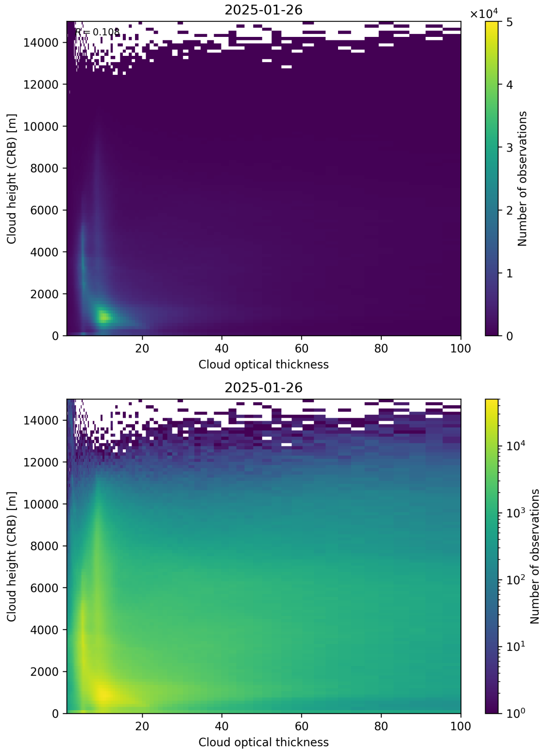
Figure 85: Scatter density plot of “Cloud optical thickness” against “Cloud height (CRB)” for 2025-01-25 to 2025-01-27.
