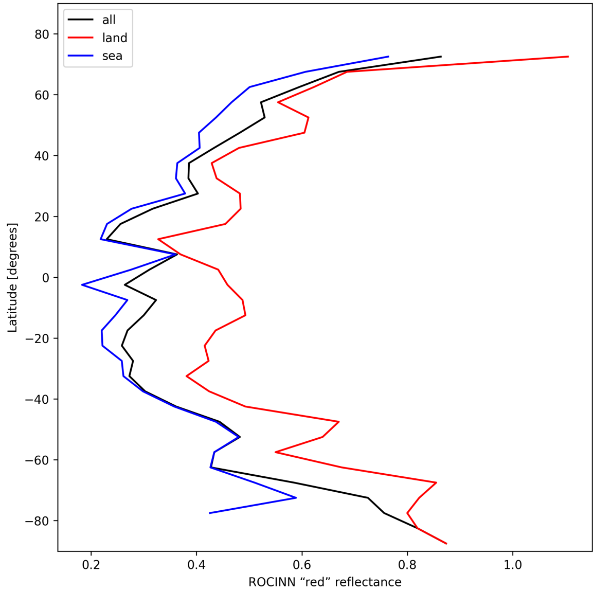
Figure 37: Zonal average of “ROCINN “red” reflectance” for 2025-01-25 to 2025-01-27.
