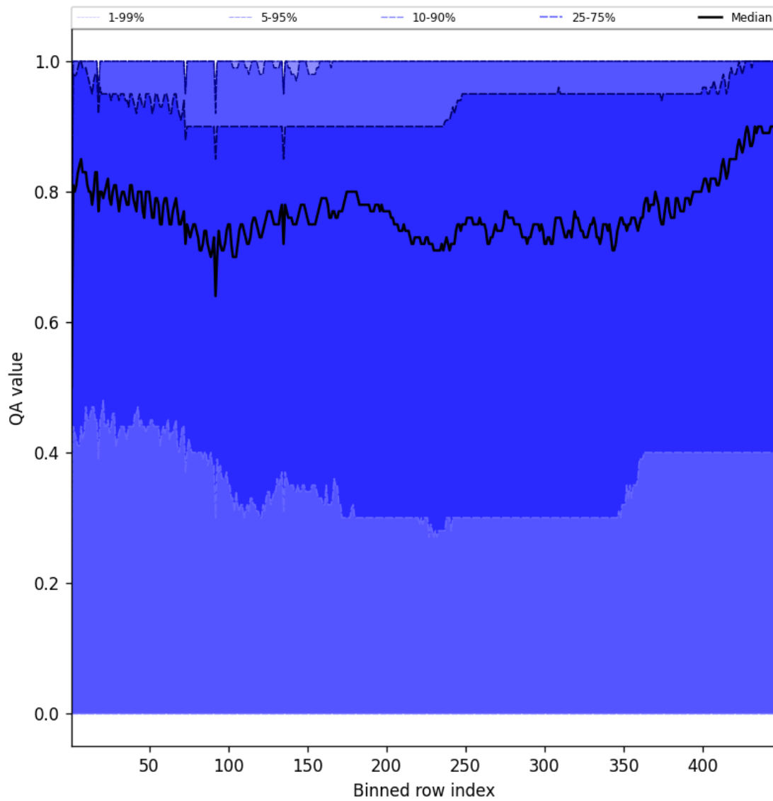
Figure 54: Along track statistics of “QA value” for 2025-01-25 to 2025-01-27
