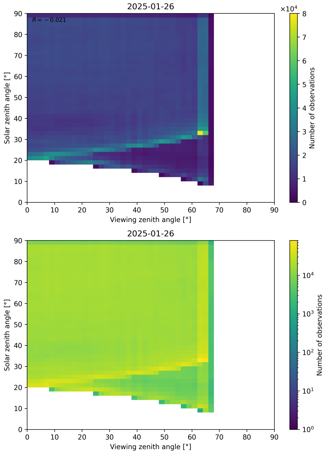
Figure 114: Scatter density plot of “Viewing zenith angle” against “Solar zenith angle” for 2025-01-25 to 2025-01-27.
