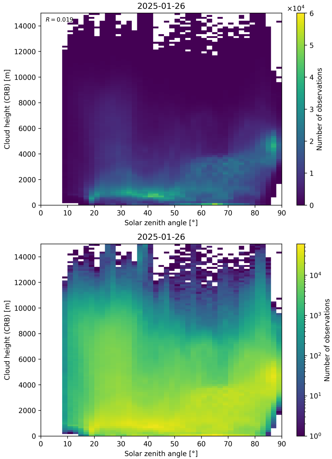
Figure 102: Scatter density plot of “Solar zenith angle” against “Cloud height (CRB)” for 2025-01-25 to 2025-01-27.
