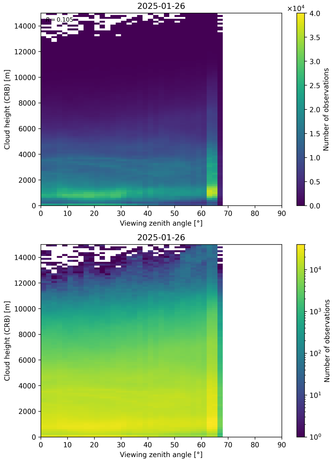
Figure 110: Scatter density plot of “Viewing zenith angle” against “Cloud height (CRB)” for 2025-01-25 to 2025-01-27.
