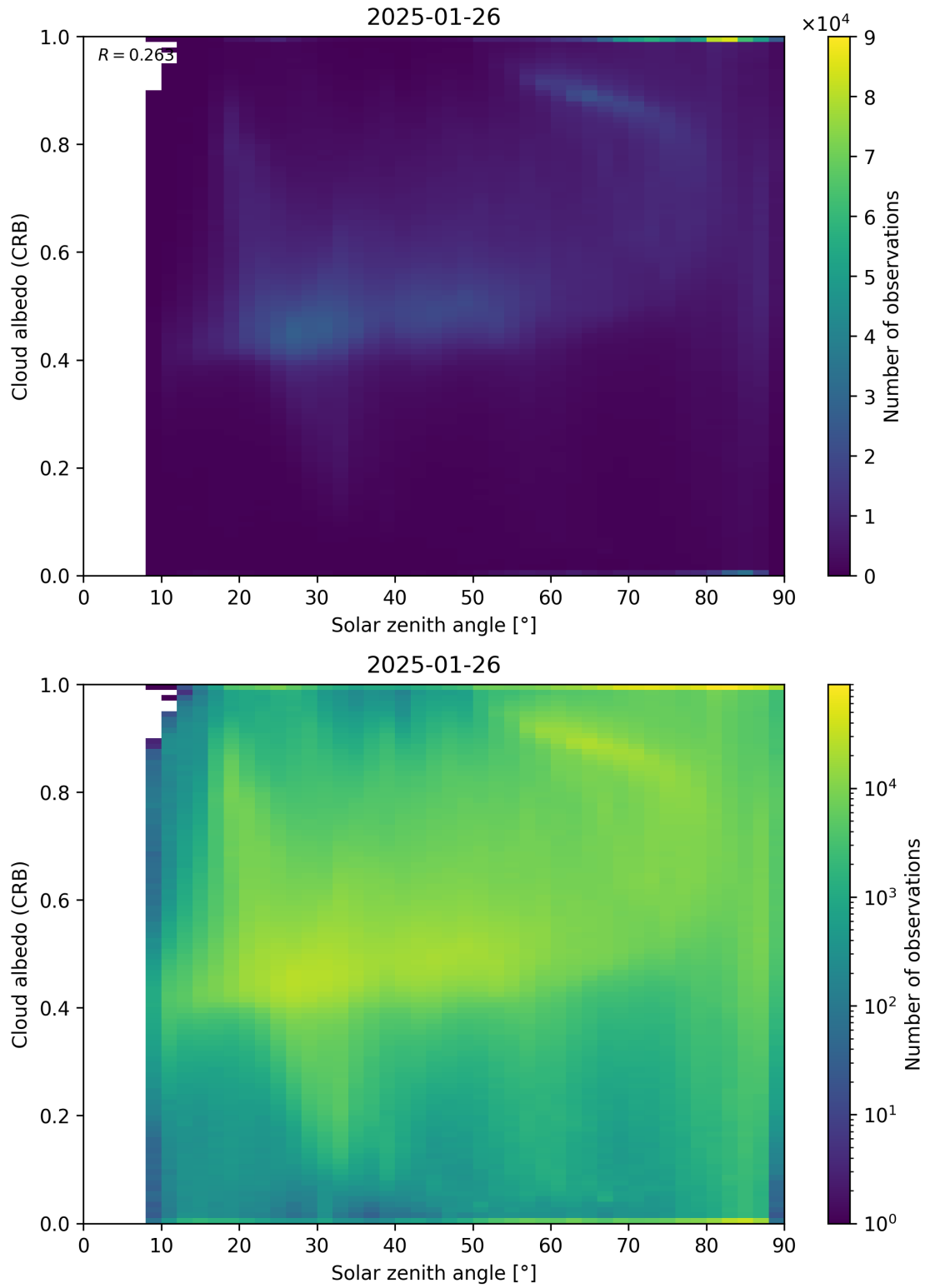
Figure 98: Scatter density plot of “Solar zenith angle” against “Cloud albedo (CRB)” for 2025-01-25 to 2025-01-27.
