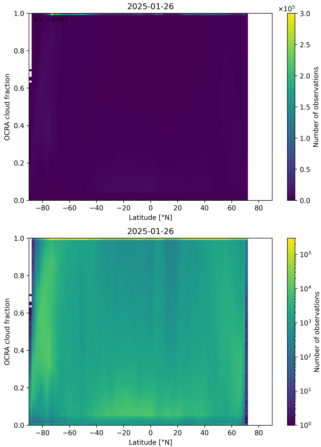
Figure 93: Scatter density plot of “Latitude” against “OCRA cloud fraction” for 2025-01-25 to 2025-01-27.
