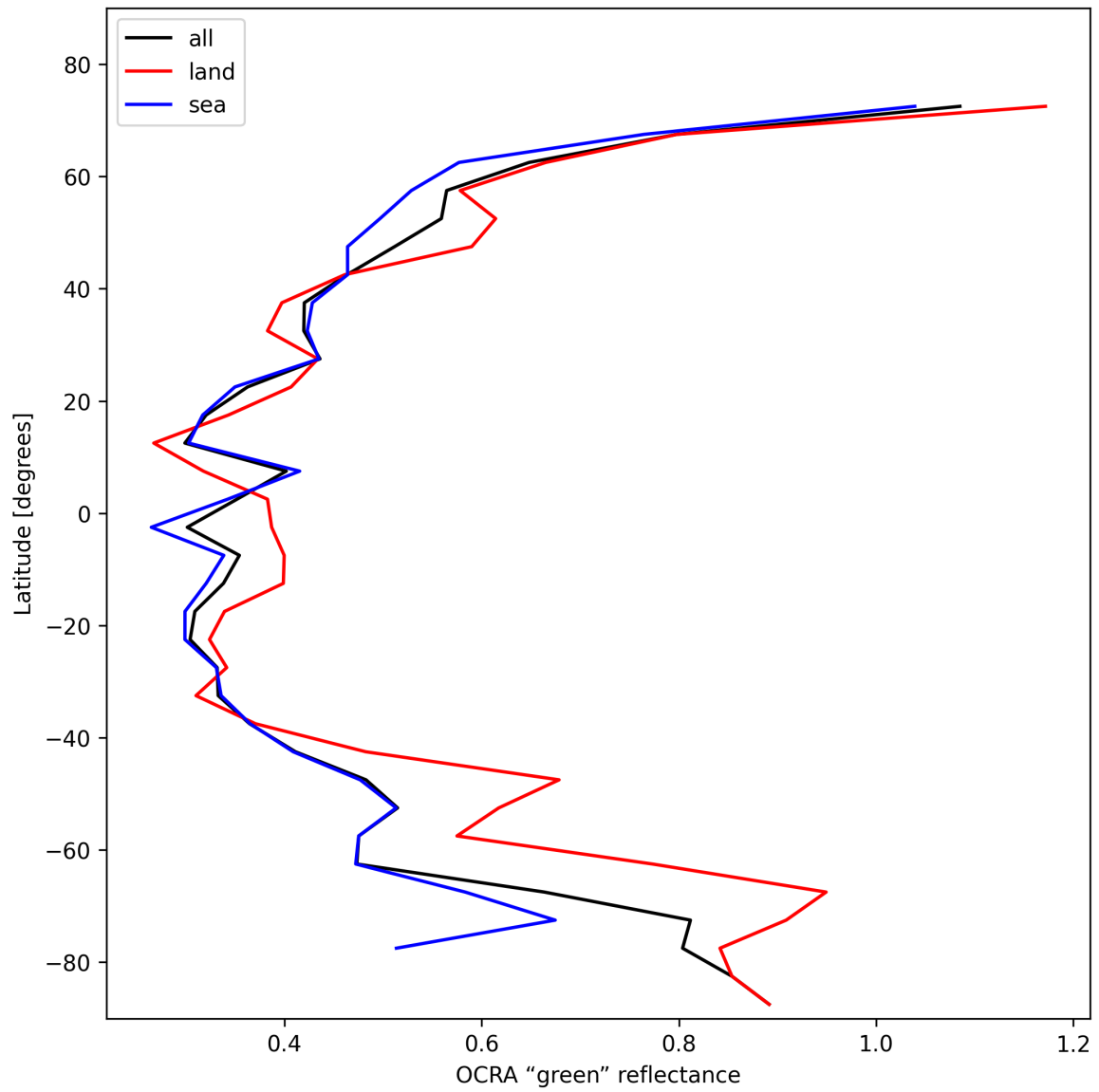
Figure 36: Zonal average of “OCRA “green” reflectance” for 2025-01-25 to 2025-01-27.
