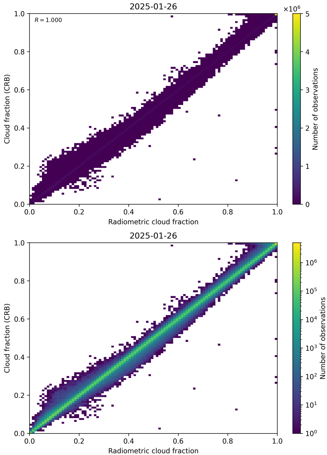
Figure 73: Scatter density plot of “Radiometric cloud fraction” against “Cloud fraction (CRB)” for 2025-01-25 to 2025-01-27.
