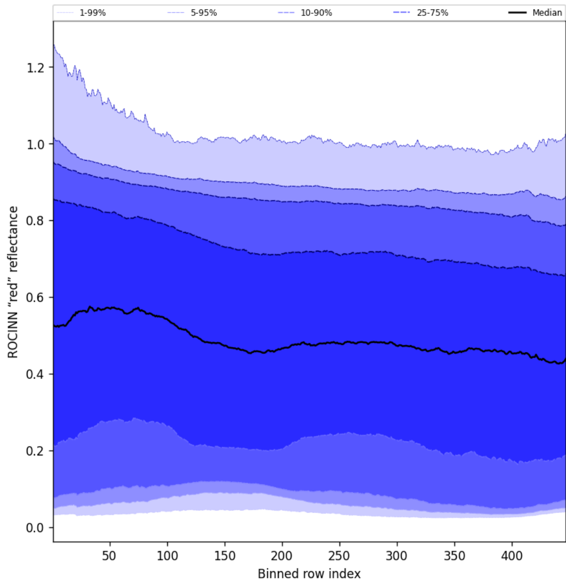
Figure 69: Along track statistics of "ROCINN "red" reflectance" for 2025-01-25 to 2025-01-27
