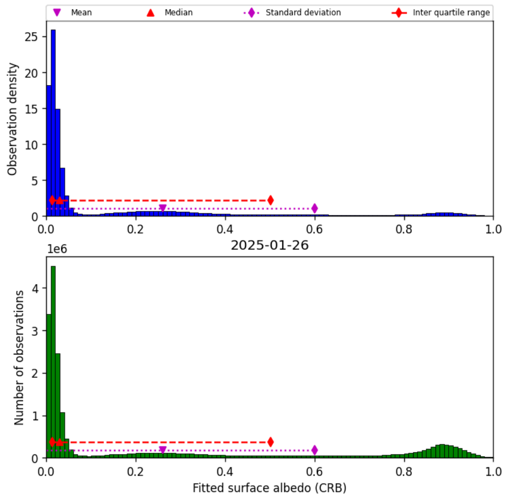
Figure 46: Histogram of “Fitted surface albedo (CRB)” for 2025-01-25 to 2025-01-27
