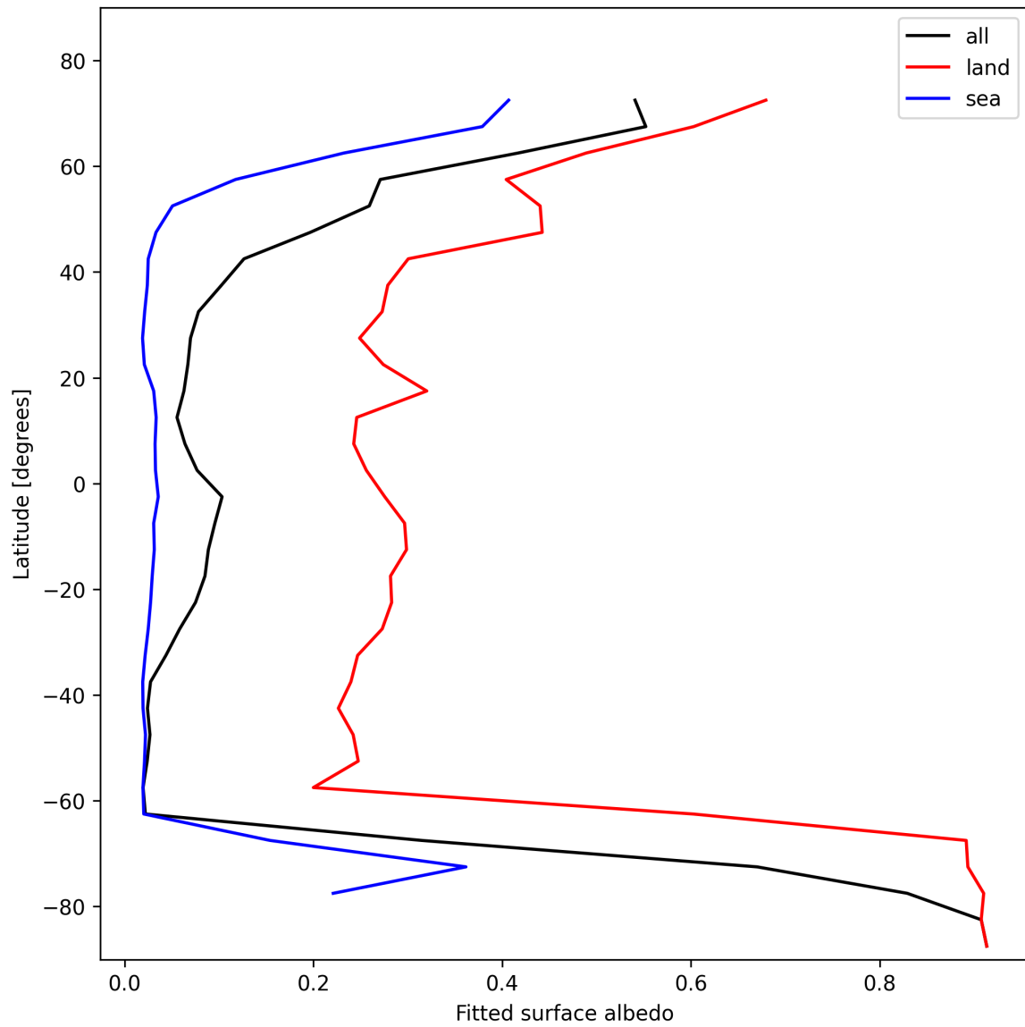
Figure 29: Zonal average of “Fitted surface albedo” for 2025-01-25 to 2025-01-27.
