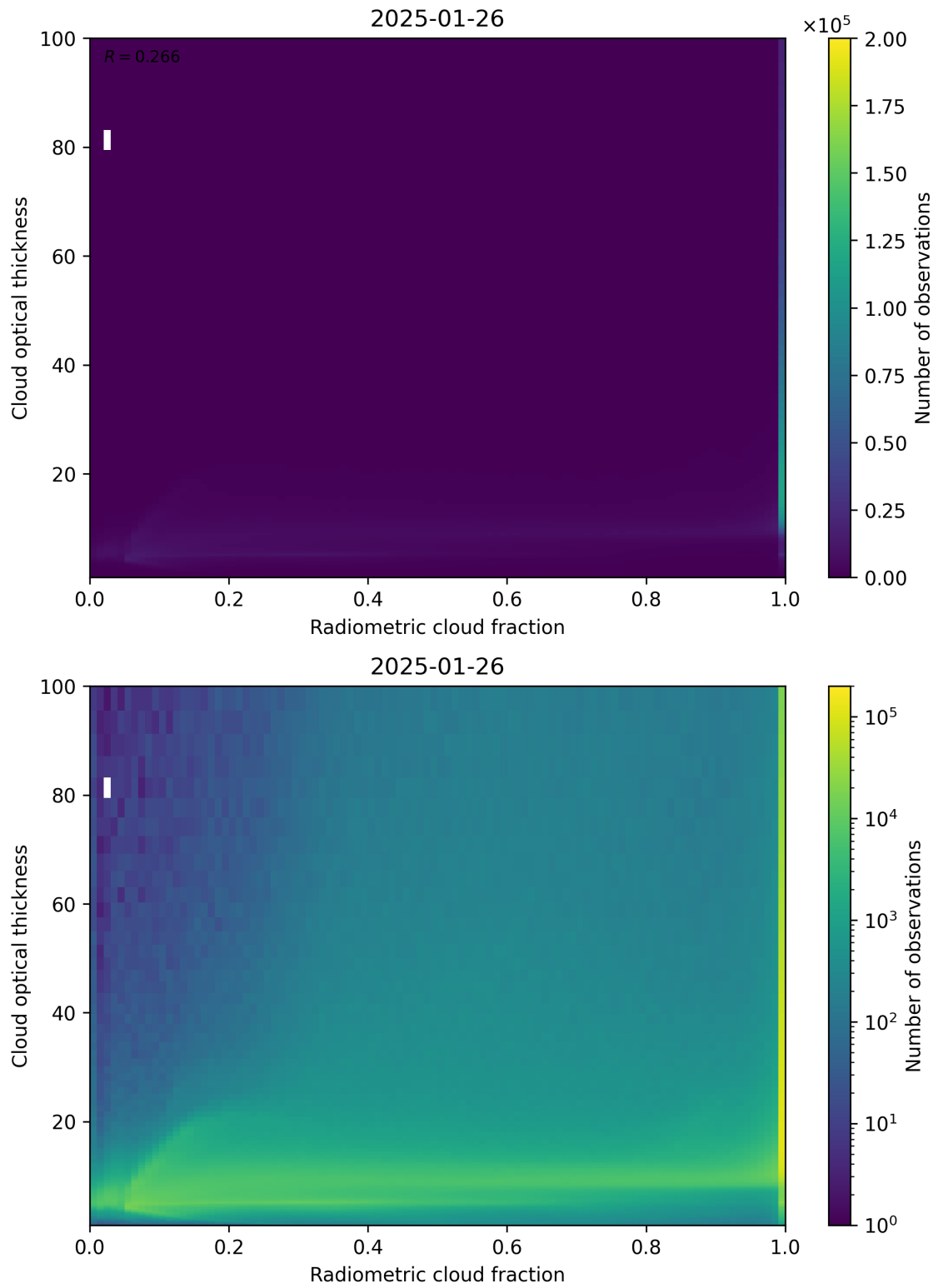
Figure 75: Scatter density plot of “Radiometric cloud fraction” against “Cloud optical thickness” for 2025-01-25 to 2025-01-27.
