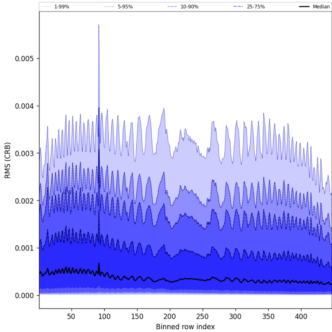
Figure 64: Along track statistics of “RMS (CRB)” for 2025-01-25 to 2025-01-27
