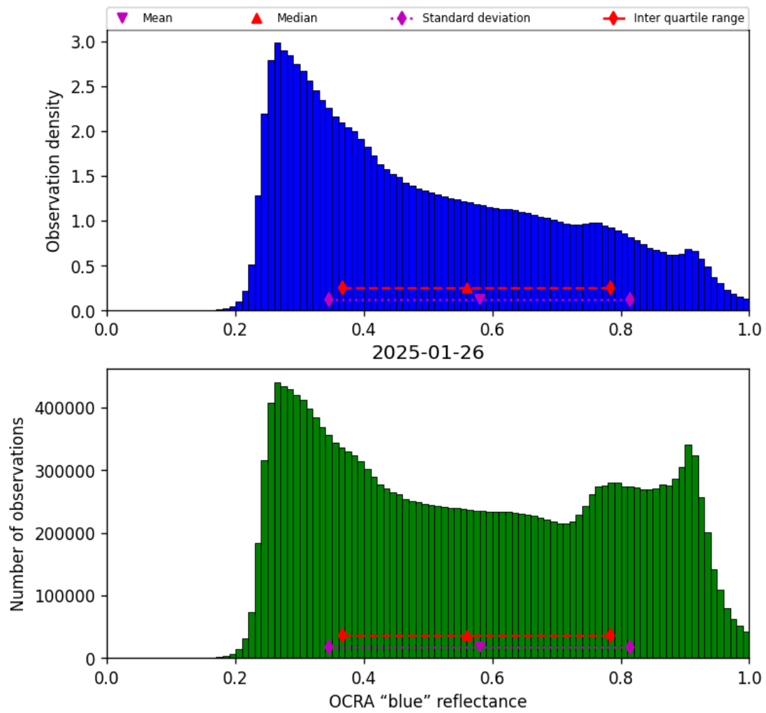
Figure 51: Histogram of “OCRA “blue” reflectance” for 2025-01-25 to 2025-01-27
