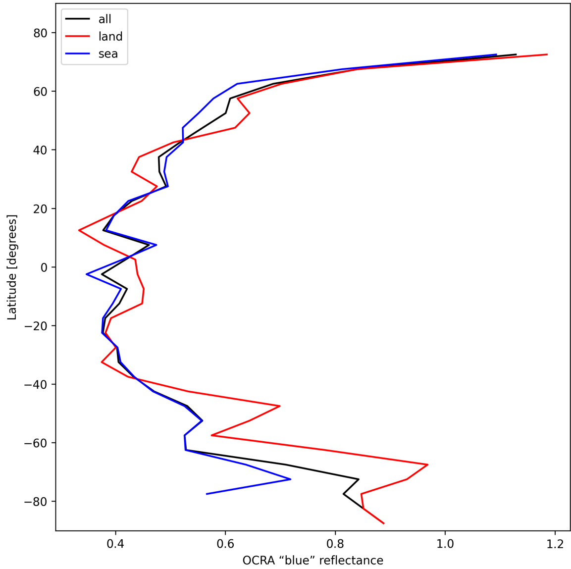
Figure 35: Zonal average of "OCRA "blue" reflectance" for 2025-01-25 to 2025-01-27.
