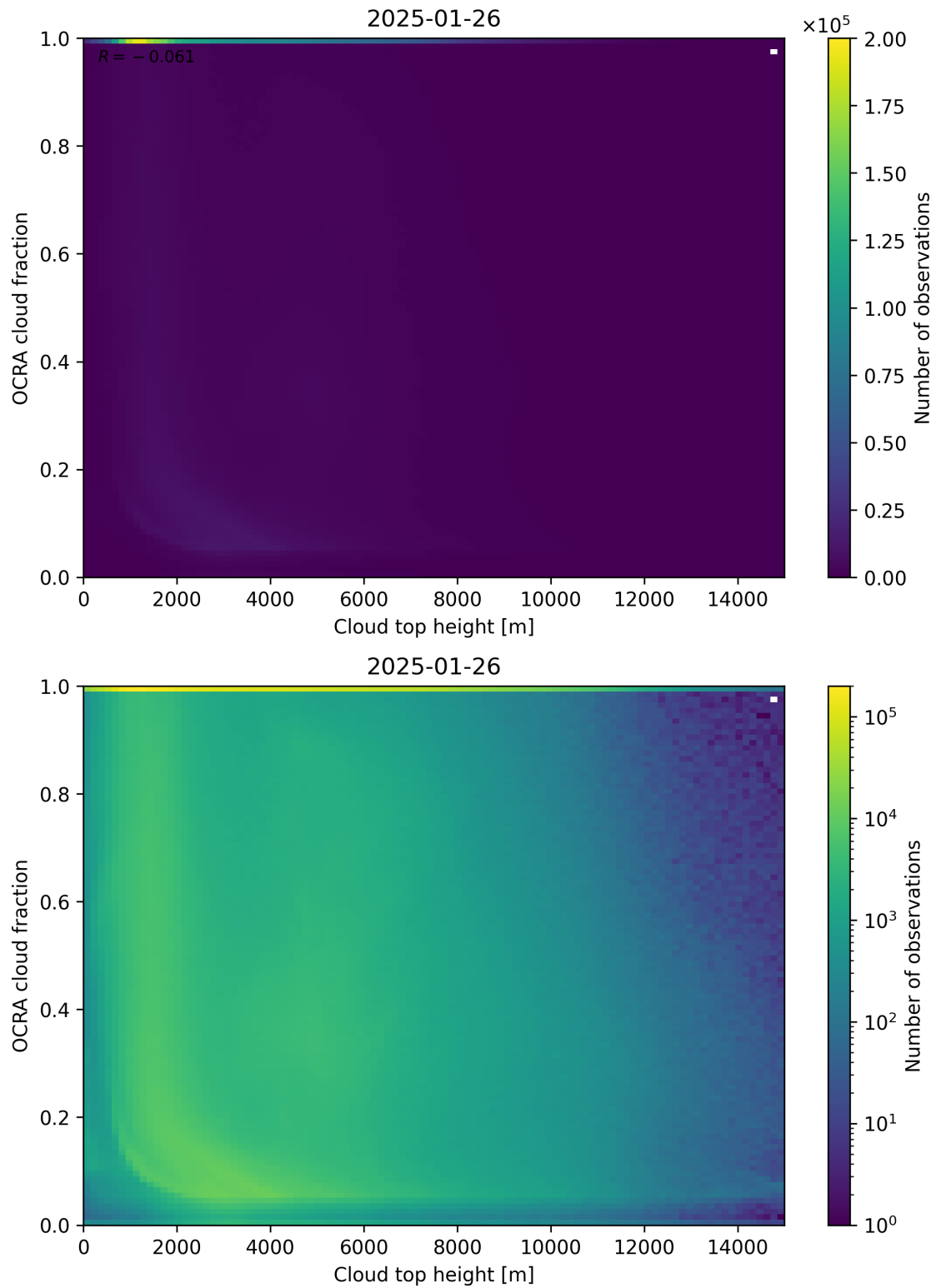
Figure 87: Scatter density plot of “Cloud top height” against “OCRA cloud fraction” for 2025-01-25 to 2025-01-27.
