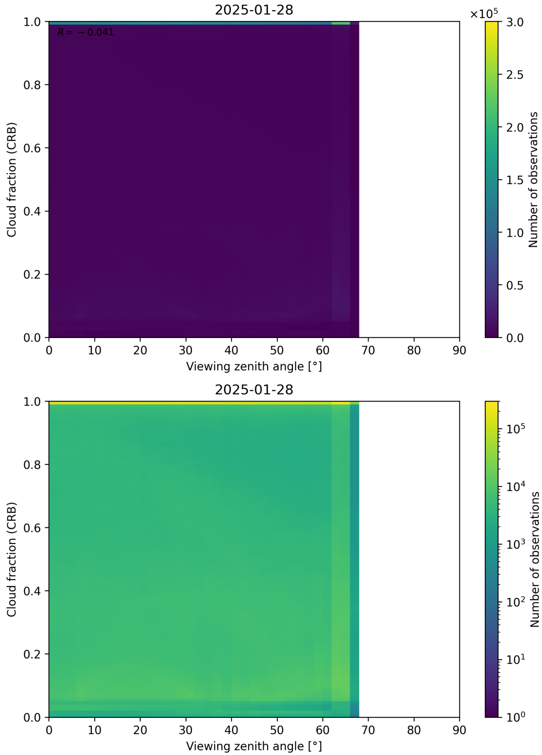
Figure 109: Scatter density plot of “Viewing zenith angle” against “Cloud fraction (CRB)” for 2025-01-28 to 2025-01-29.
