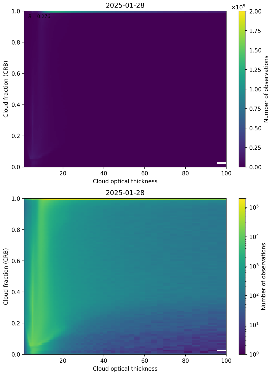
Figure 84: Scatter density plot of “Cloud optical thickness” against “Cloud fraction (CRB)” for 2025-01-28 to 2025-01-29.
