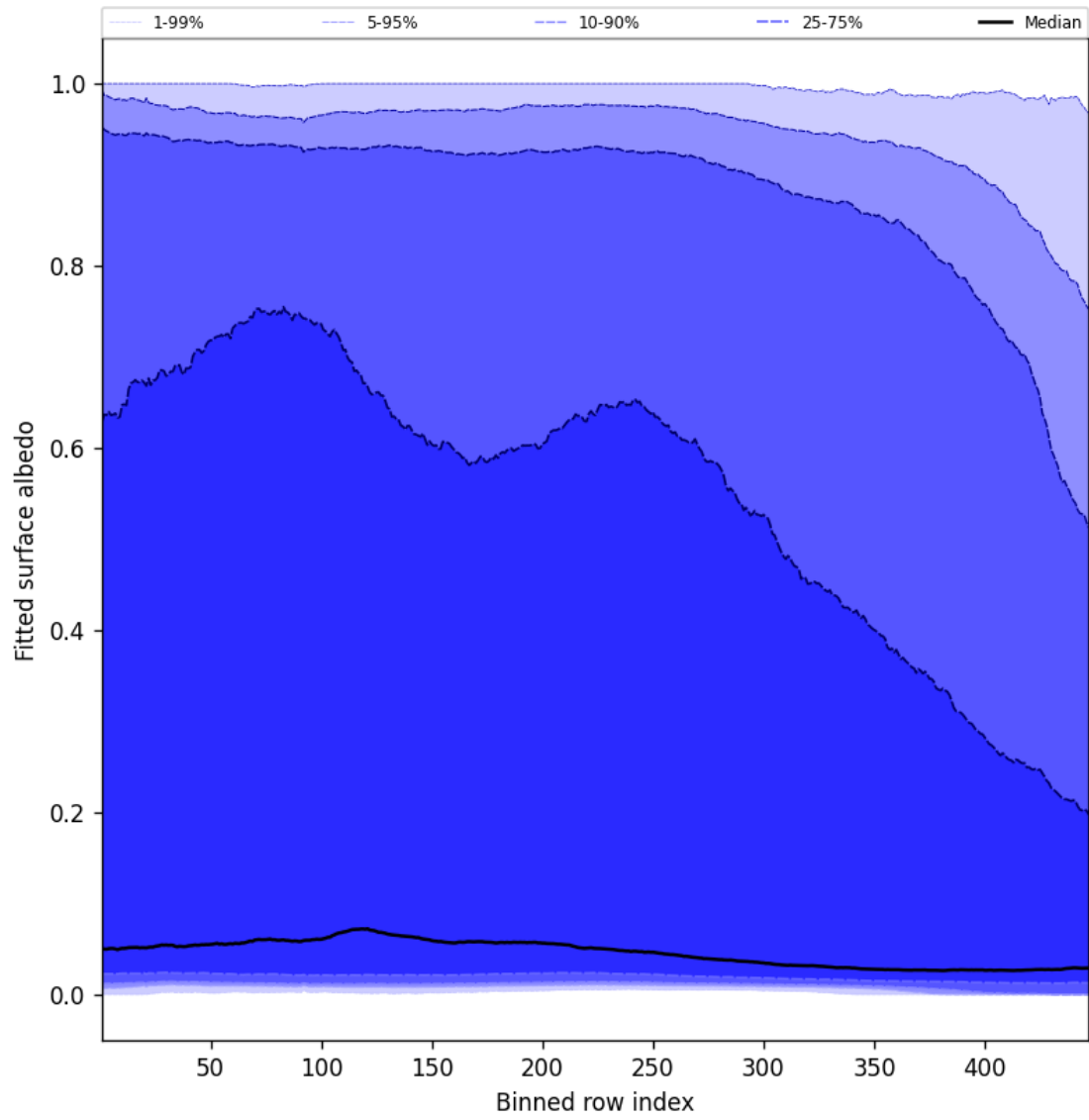
Figure 61: Along track statistics of “Fitted surface albedo” for 2025-01-28 to 2025-01-29
