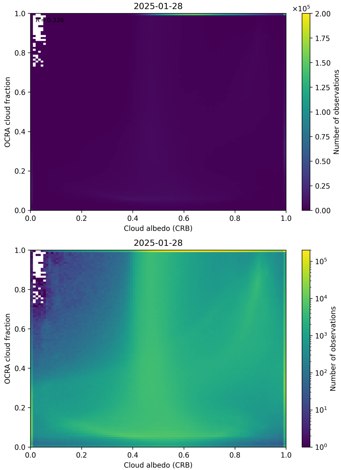
Figure 70: Scatter density plot of “Cloud albedo (CRB)” against “OCRA cloud fraction” for 2025-01-28 to 2025-01-29.
