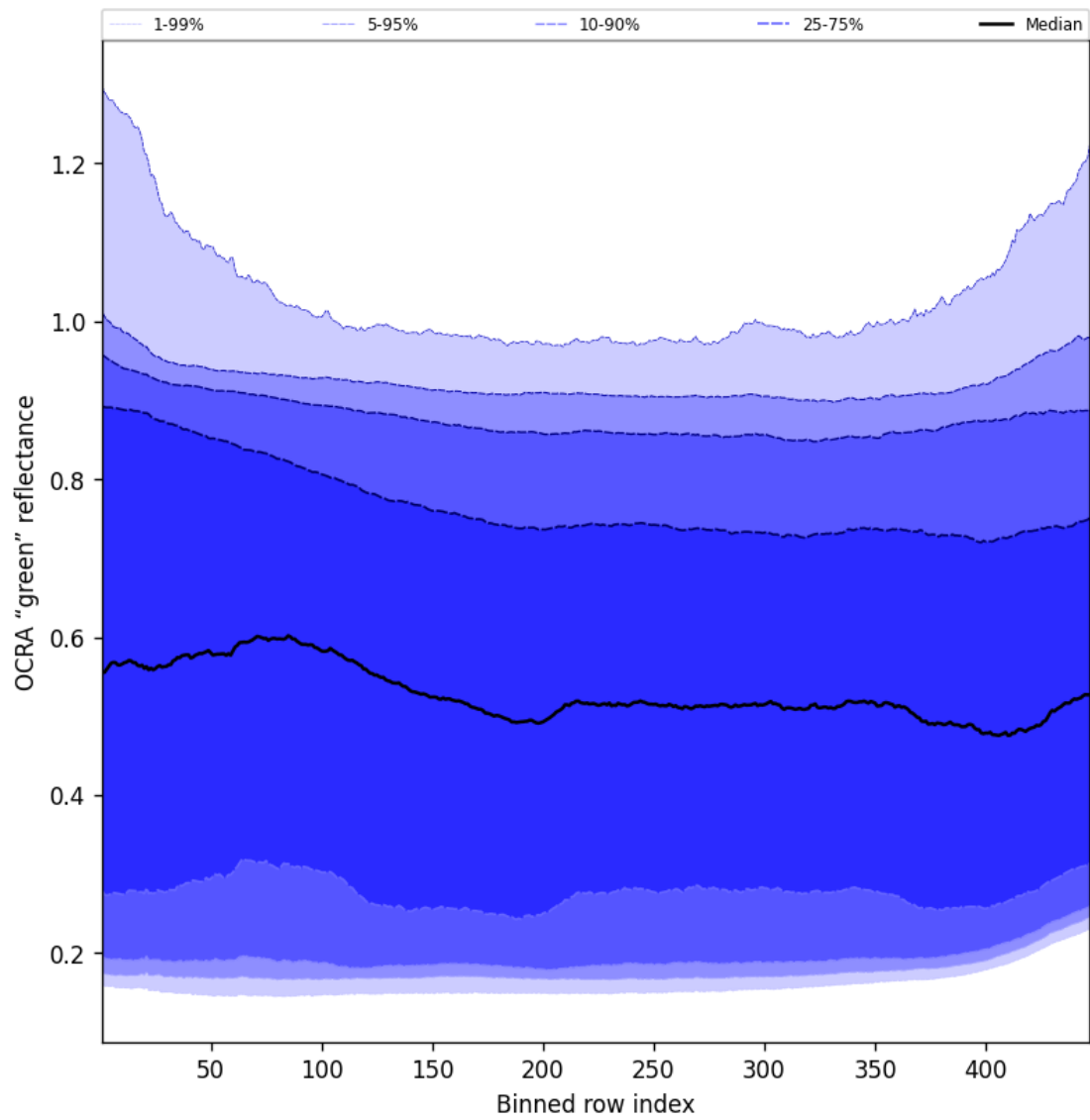
Figure 68: Along track statistics of "OCRA "green" reflectance" for 2025-01-28 to 2025-01-29
