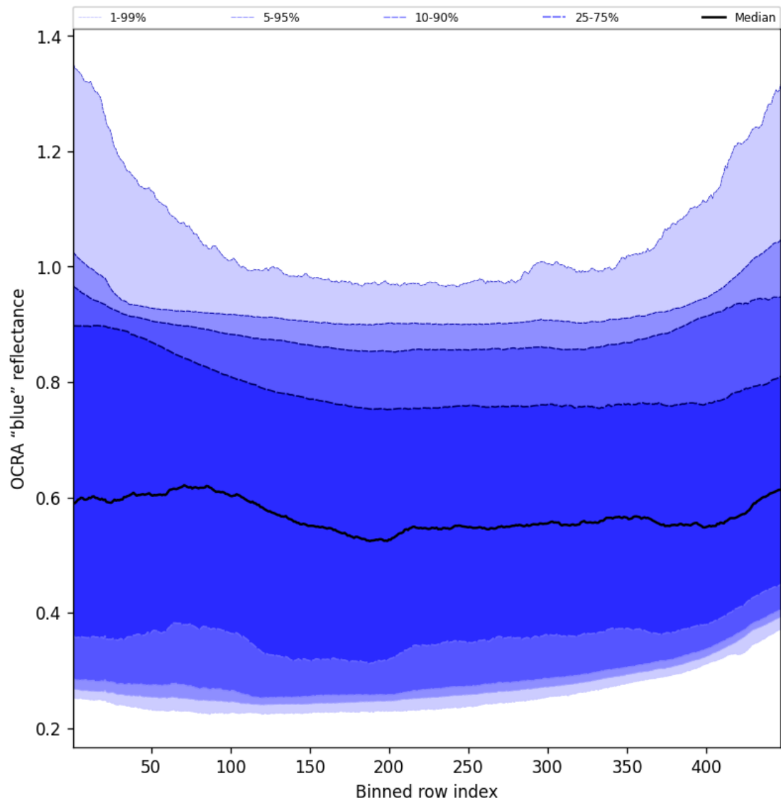
Figure 67: Along track statistics of “OCRA “blue” reflectance” for 2025-01-28 to 2025-01-29
