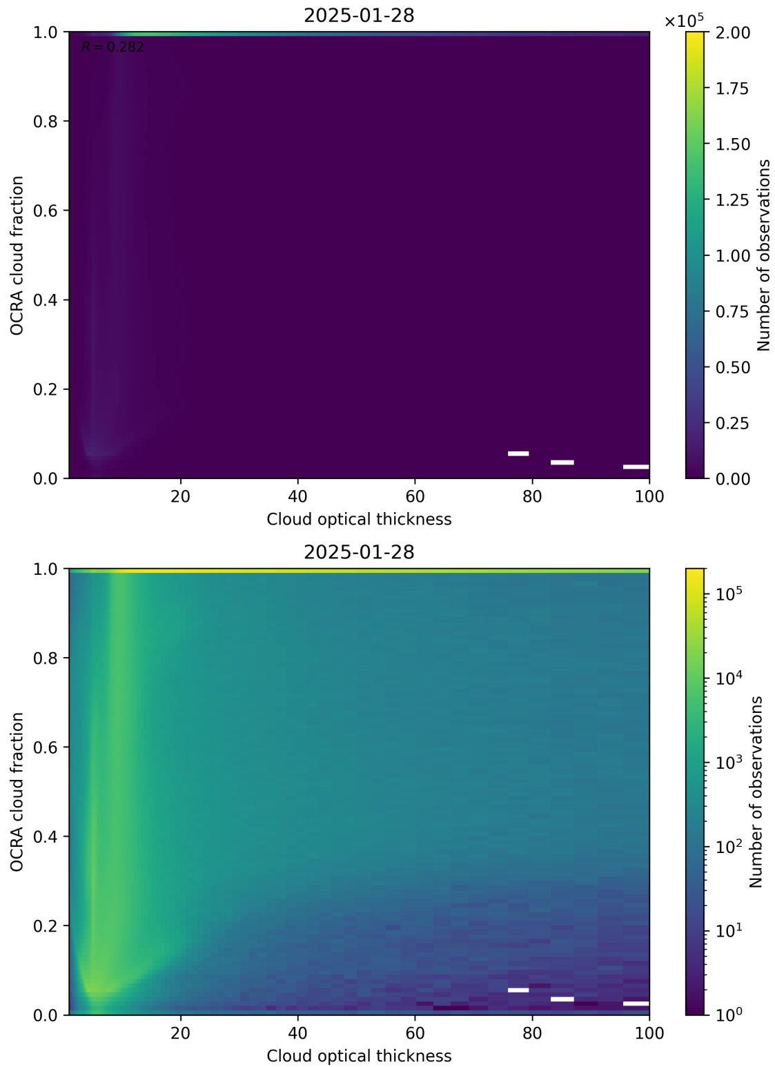
Figure 83: Scatter density plot of “Cloud optical thickness” against “OCRA cloud fraction” for 2025-01-28 to 2025-01-29.
