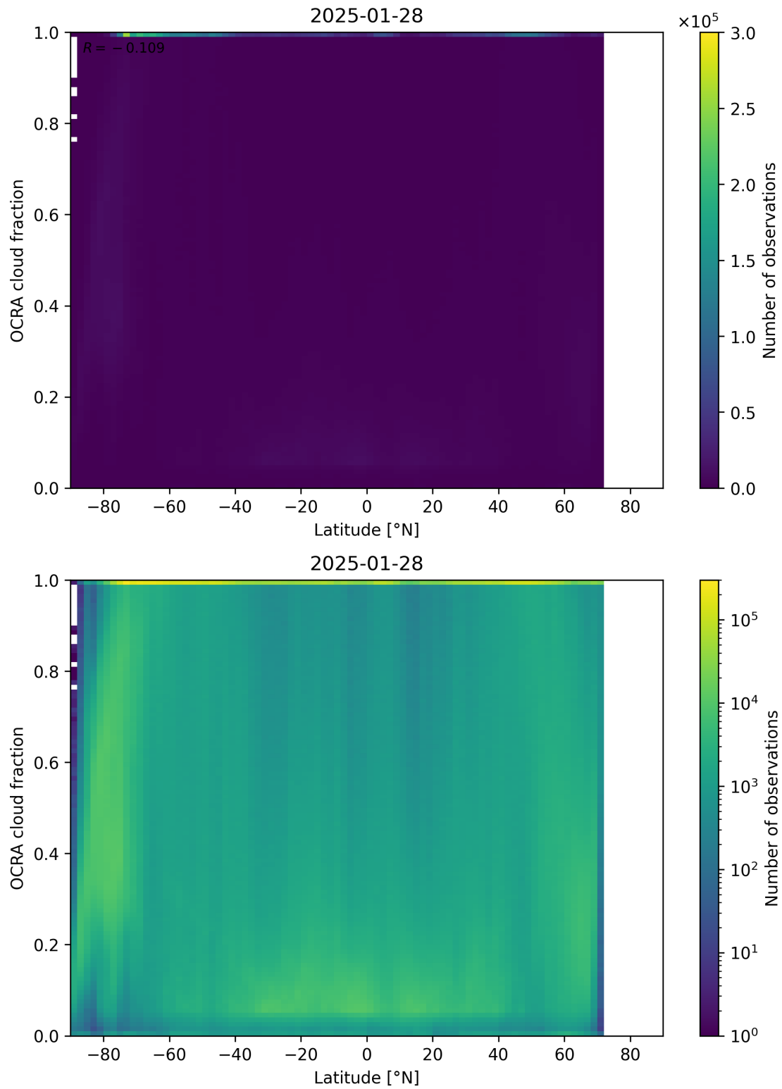
Figure 93: Scatter density plot of “Latitude” against “OCRA cloud fraction” for 2025-01-28 to 2025-01-29.
