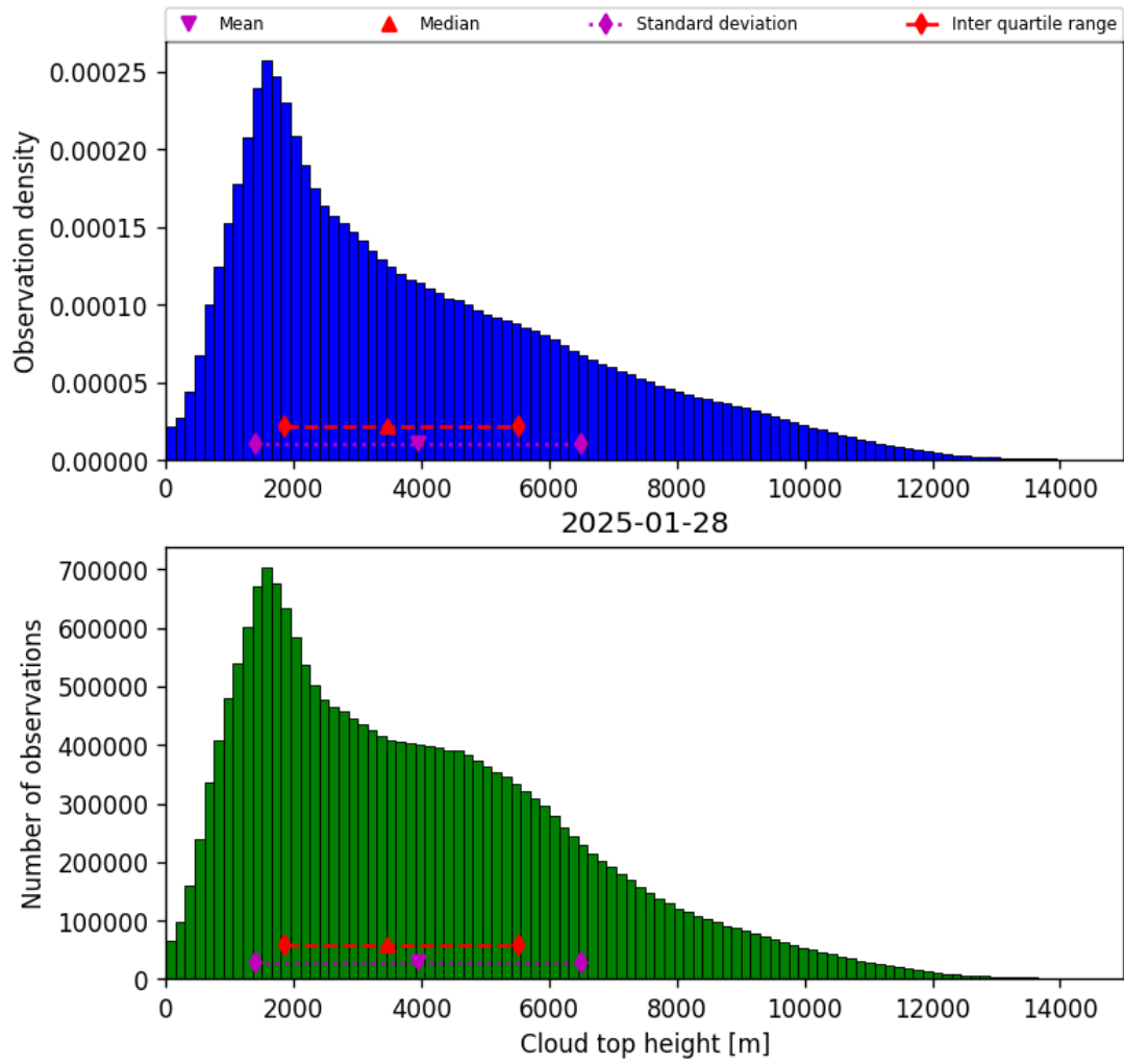
Figure 40: Histogram of “Cloud top height” for 2025-01-28 to 2025-01-29
