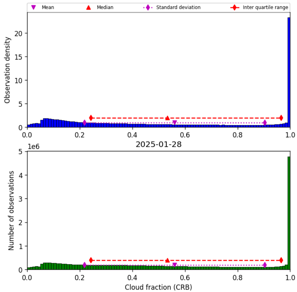
Figure 42: Histogram of “Cloud fraction (CRB)” for 2025-01-28 to 2025-01-29
