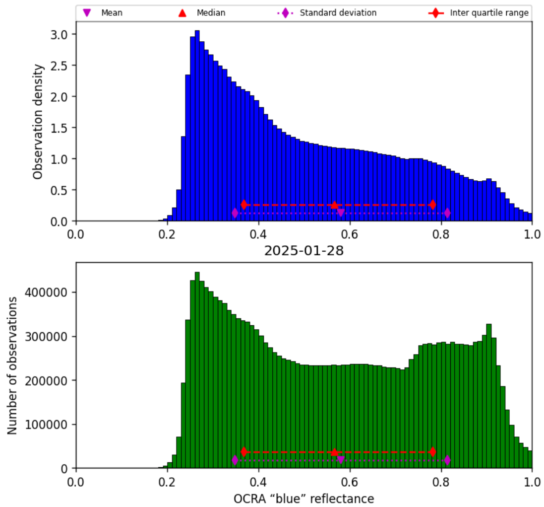
Figure 51: Histogram of “OCRA “blue” reflectance” for 2025-01-28 to 2025-01-29
