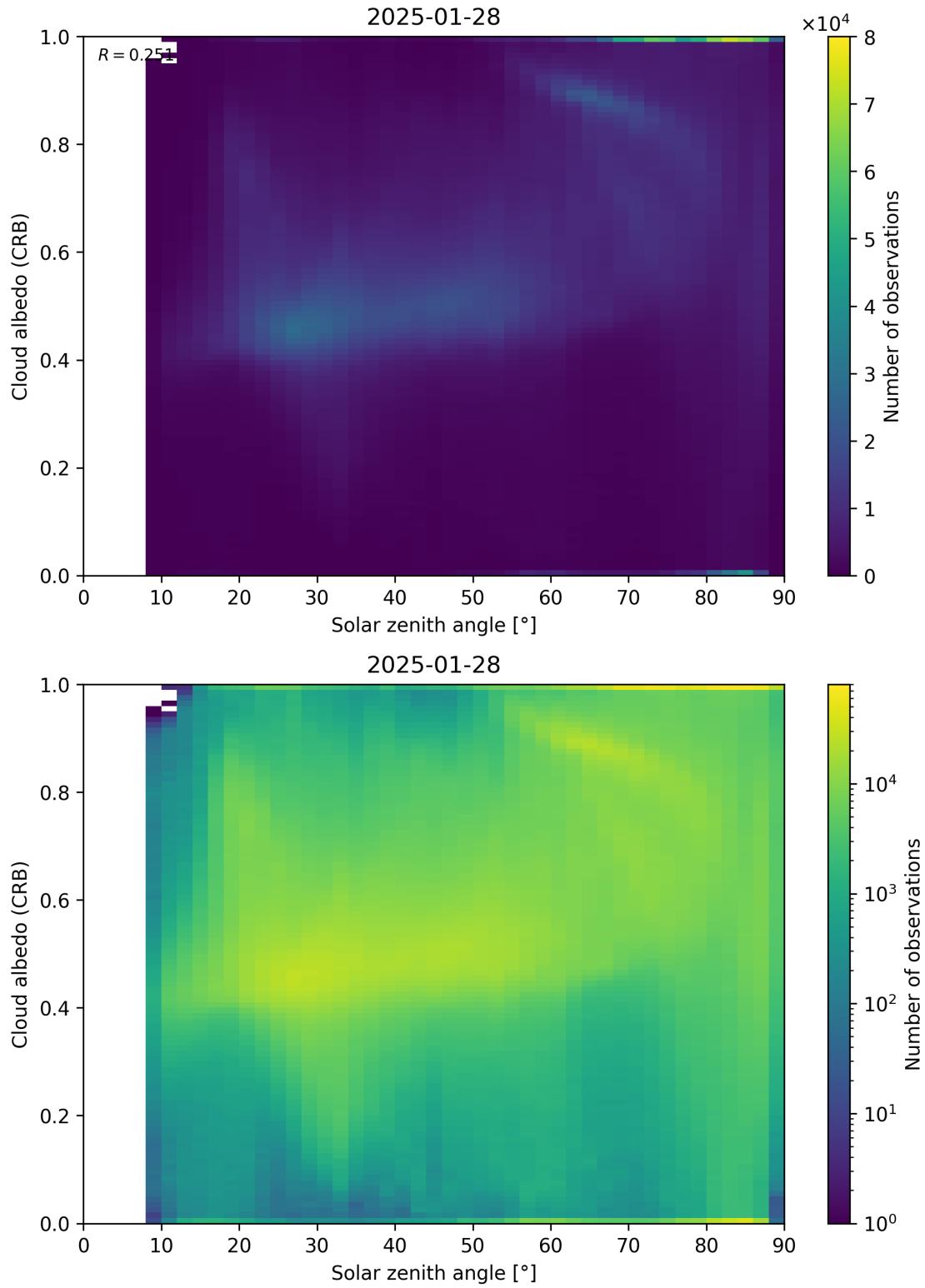
Figure 98: Scatter density plot of “Solar zenith angle” against “Cloud albedo (CRB)” for 2025-01-28 to 2025-01-29.
