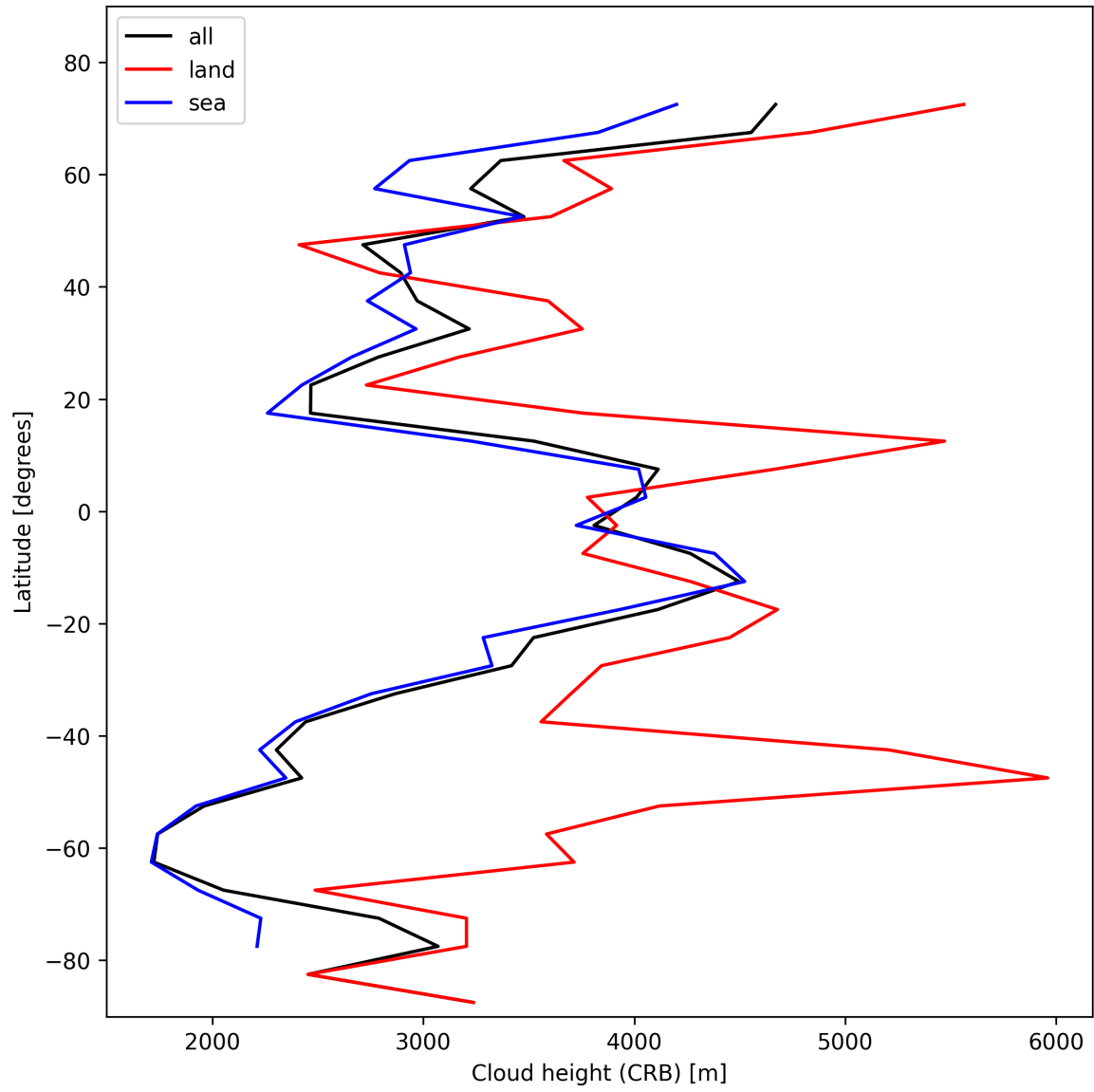
Figure 27: Zonal average of “Cloud height (CRB)” for 2025-01-28 to 2025-01-29.
