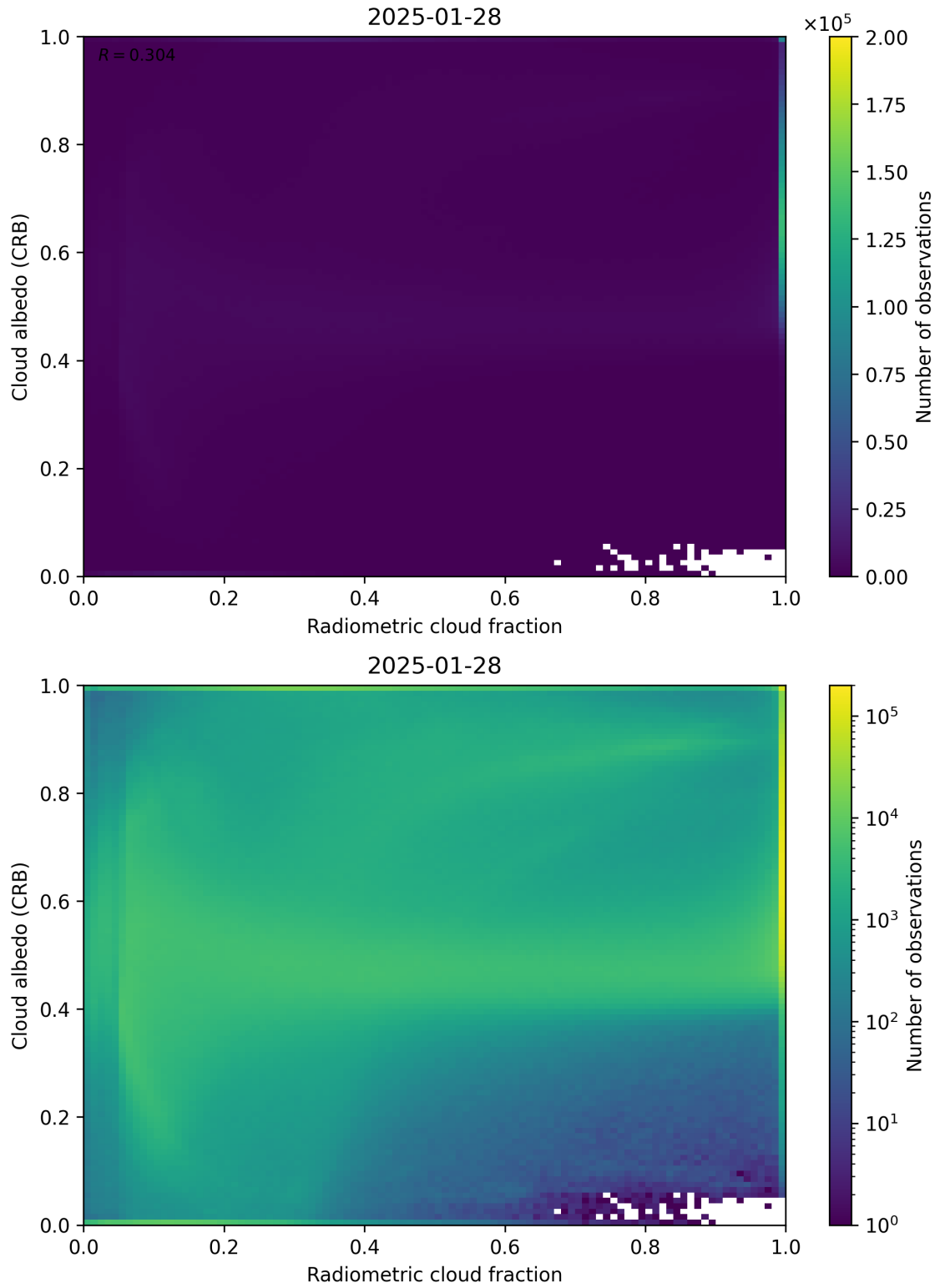
Figure 71: Scatter density plot of “Radiometric cloud fraction” against “Cloud albedo (CRB)” for 2025-01-28 to 2025-01-29.
