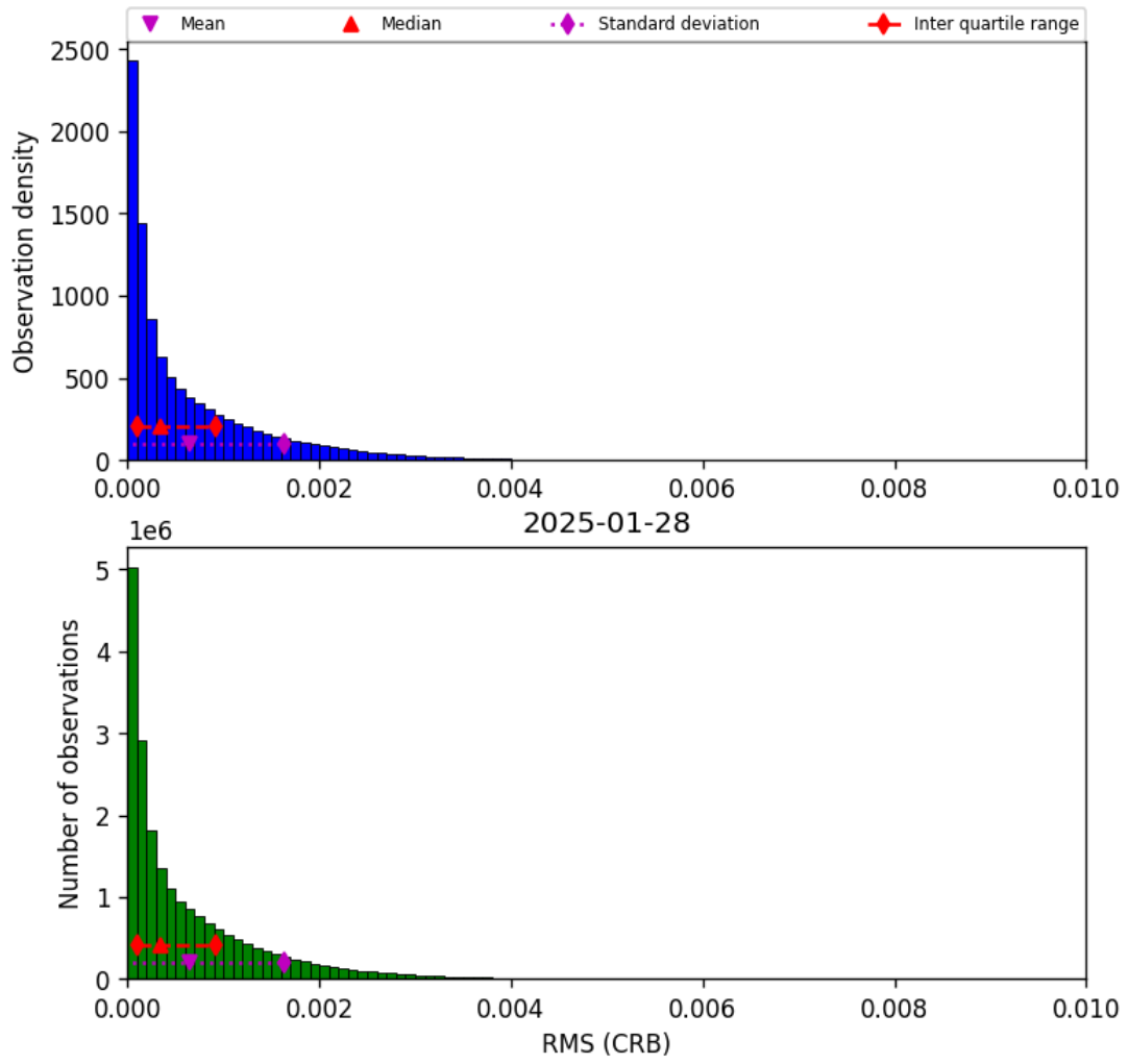
Figure 48: Histogram of "RMS (CRB)" for 2025-01-28 to 2025-01-29
