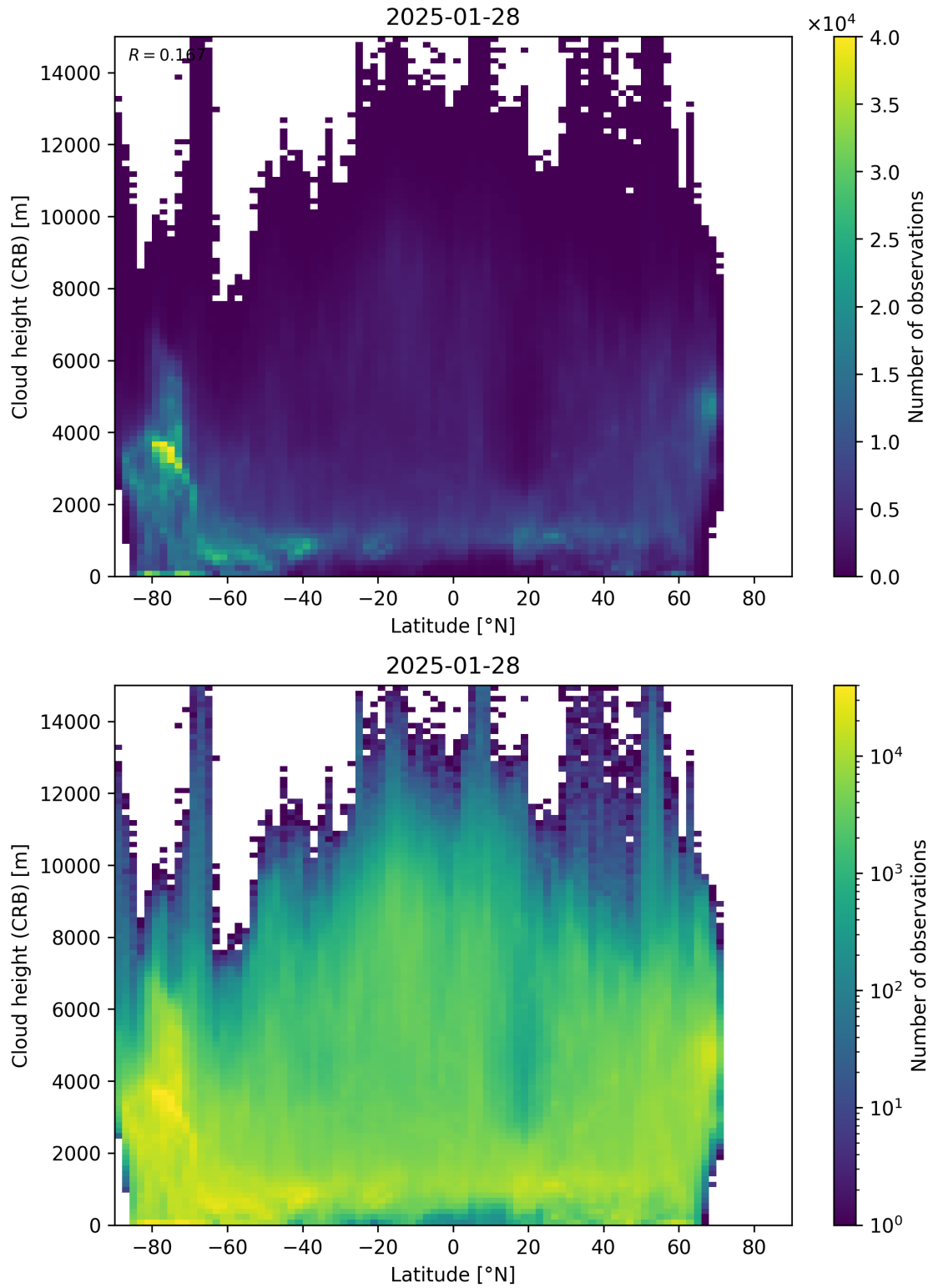
Figure 95: Scatter density plot of “Latitude” against “Cloud height (CRB)” for 2025-01-28 to 2025-01-29.
