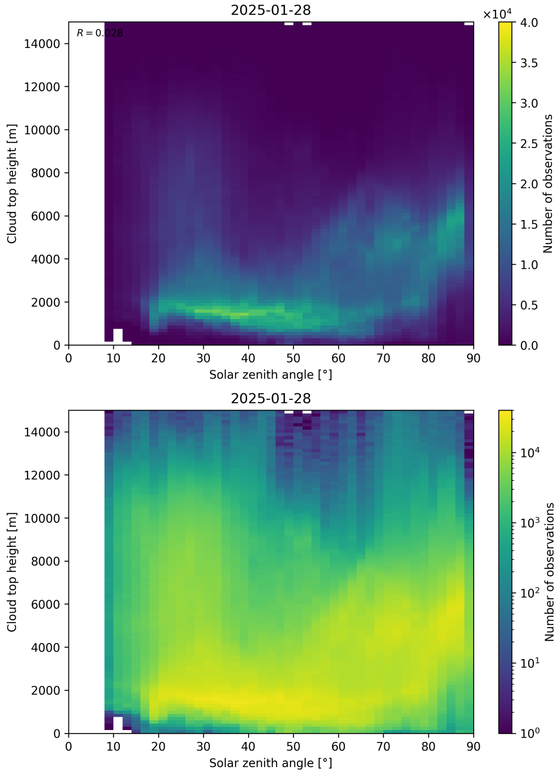
Figure 104: Scatter density plot of “Solar zenith angle” against “Cloud top height” for 2025-01-28 to 2025-01-29.
