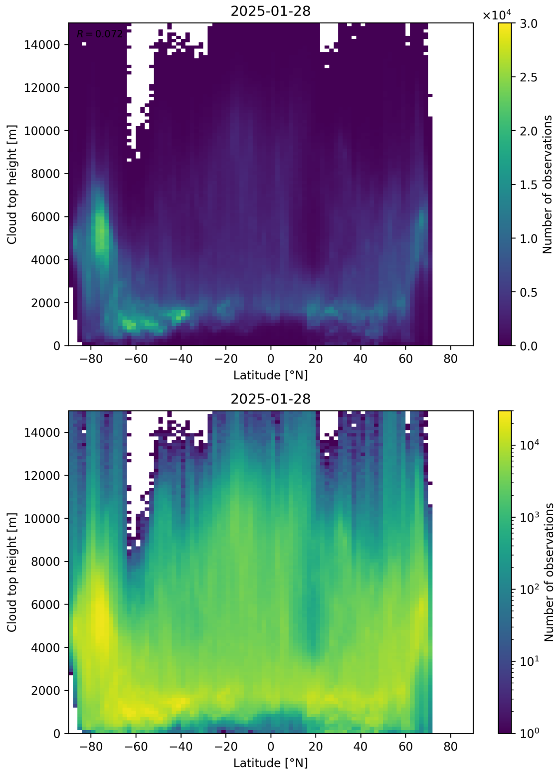
Figure 97: Scatter density plot of “Latitude” against “Cloud top height” for 2025-01-28 to 2025-01-29.
