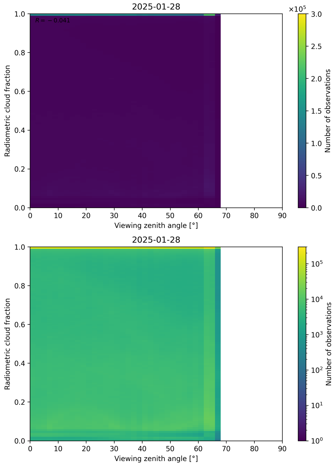
Figure 107: Scatter density plot of “Viewing zenith angle” against “Radiometric cloud fraction” for 2025-01-28 to 2025-01-29.
