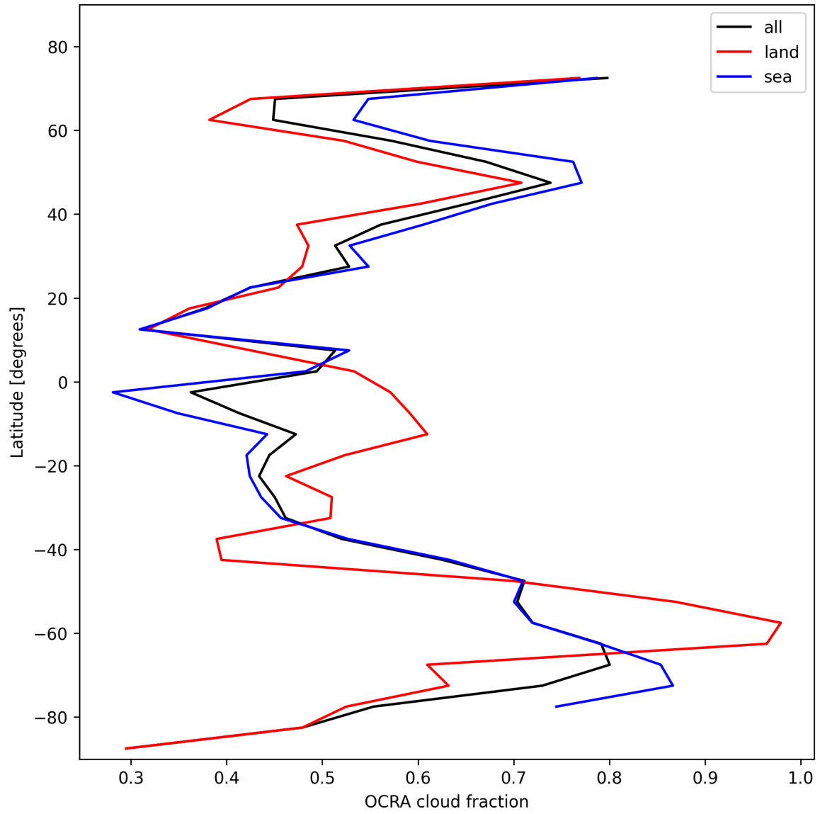
Figure 34: Zonal average of “OCRA cloud fraction” for 2025-01-28 to 2025-01-29.
