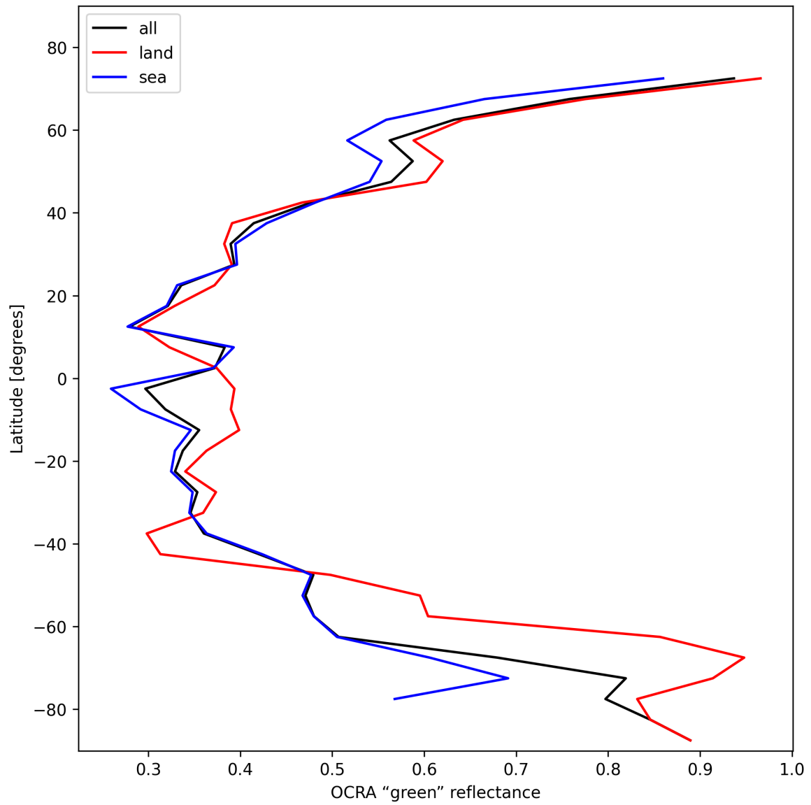
Figure 36: Zonal average of “OCRA “green” reflectance” for 2025-01-28 to 2025-01-29.
