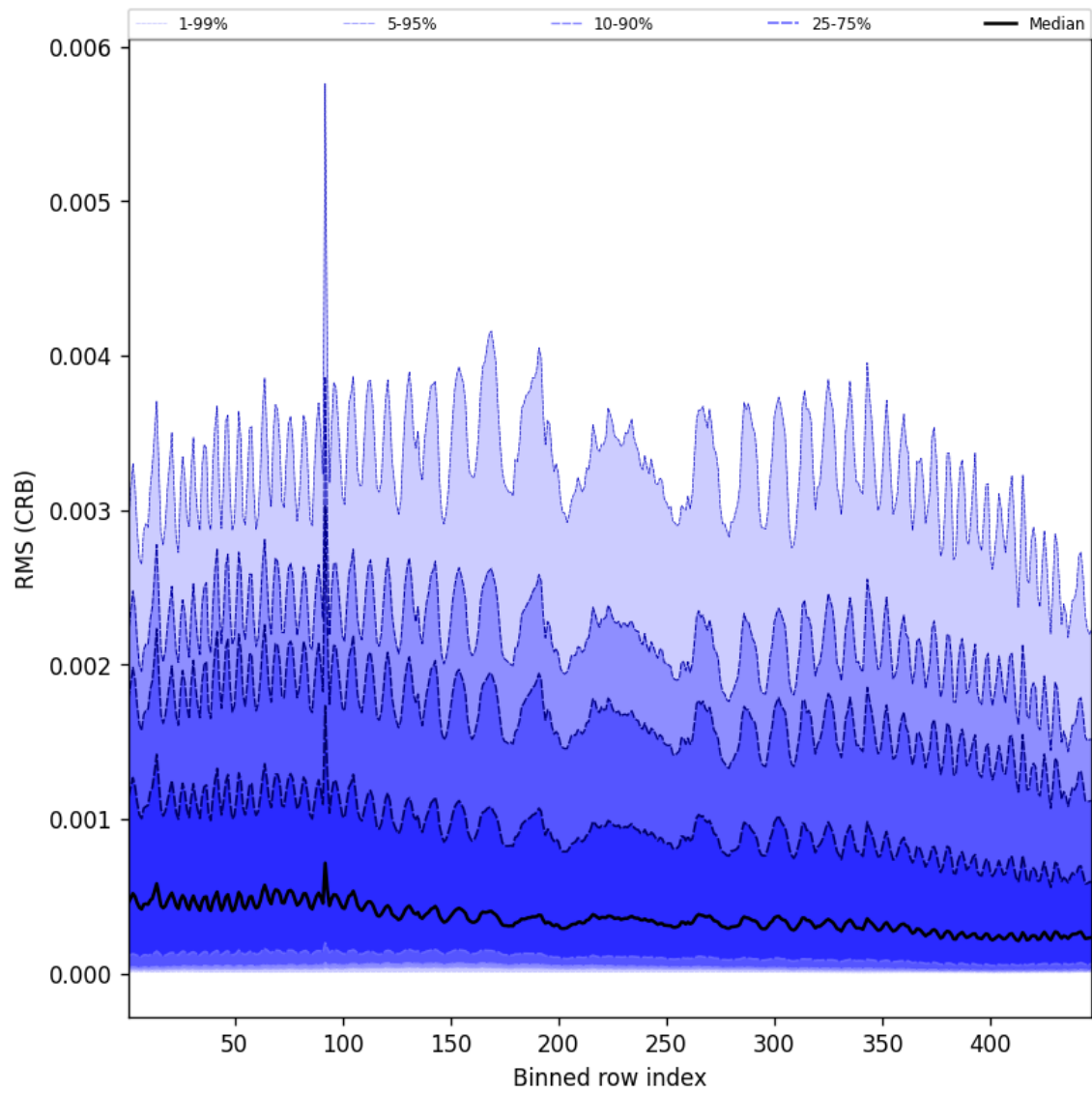
Figure 64: Along track statistics of “RMS (CRB)” for 2025-01-28 to 2025-01-29
