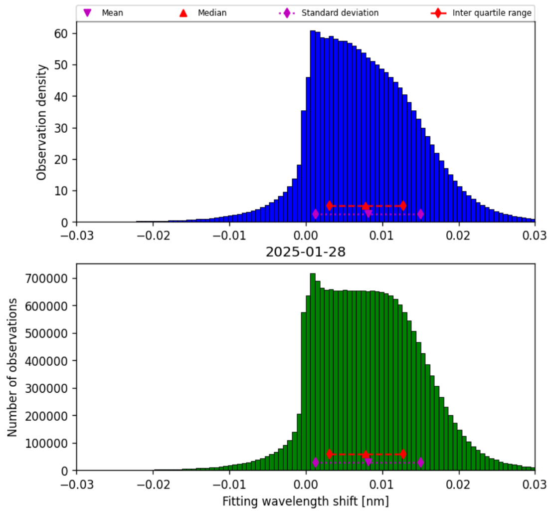
Figure 49: Histogram of “Fitting wavelength shift” for 2025-01-28 to 2025-01-29
