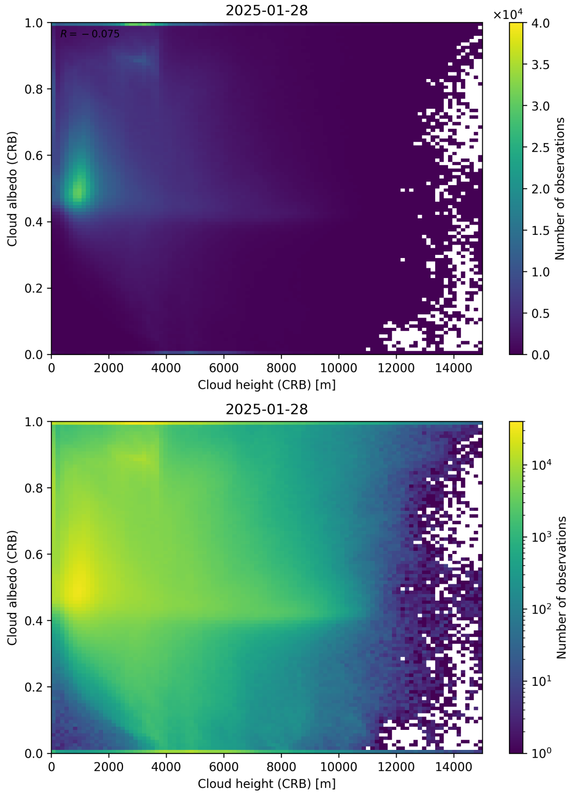
Figure 80: Scatter density plot of “Cloud height (CRB)” against “Cloud albedo (CRB)” for 2025-01-28 to 2025-01-29.
