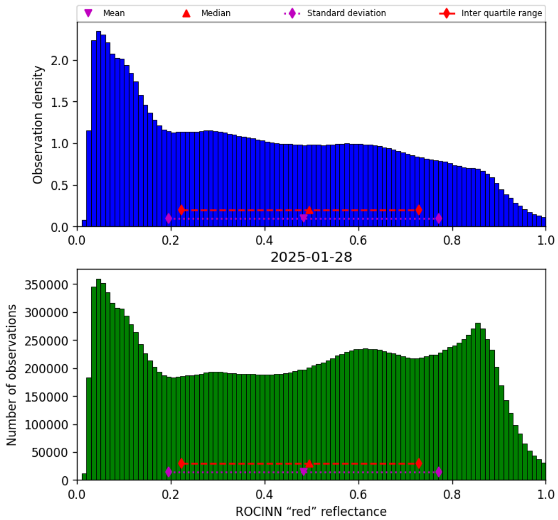
Figure 53: Histogram of “ROCINN “red” reflectance” for 2025-01-28 to 2025-01-29
