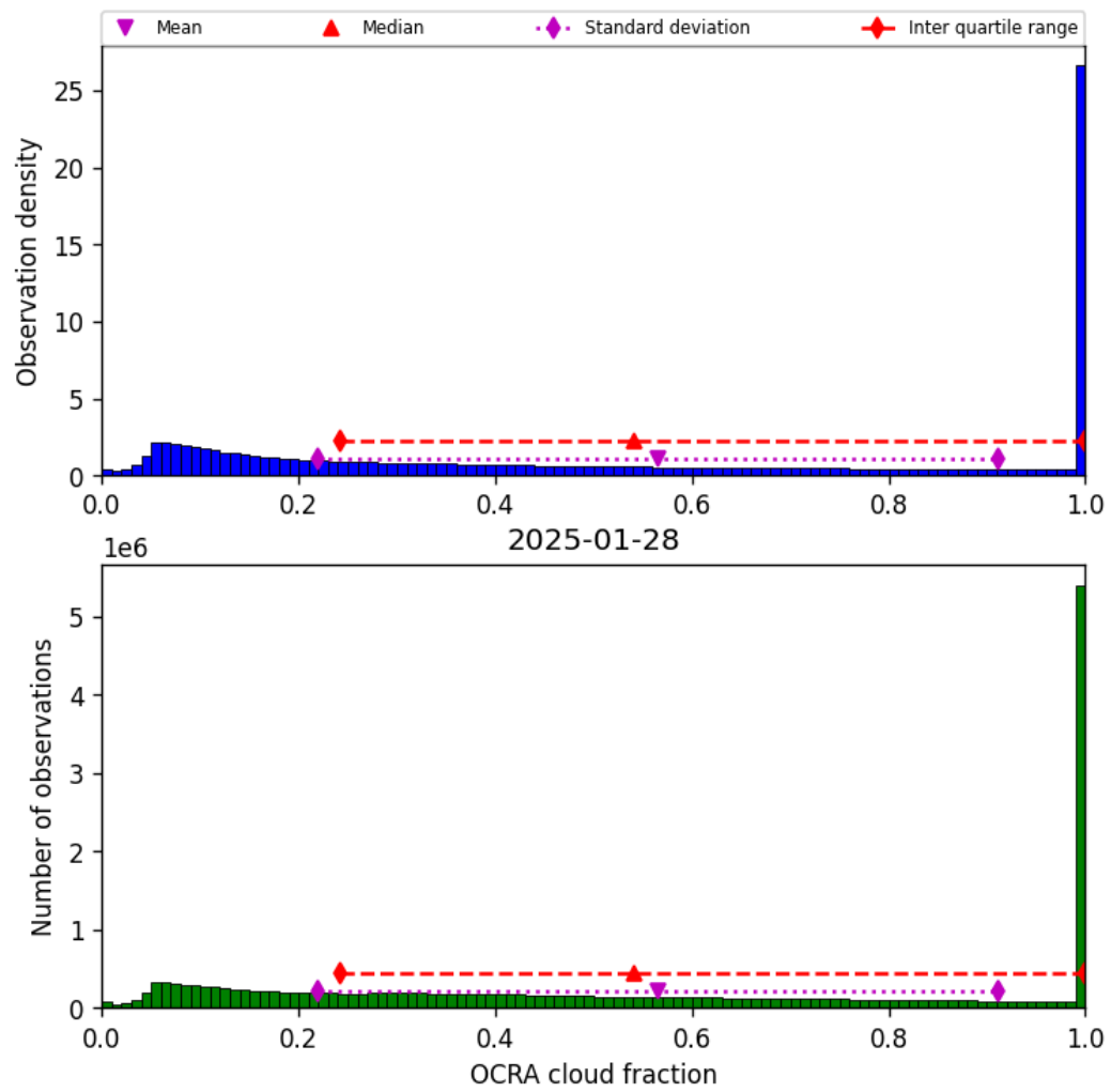
Figure 50: Histogram of “OCRA cloud fraction” for 2025-01-28 to 2025-01-29
