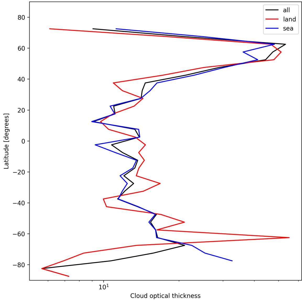
Figure 25: Zonal average of “Cloud optical thickness” for 2025-01-28 to 2025-01-29.
