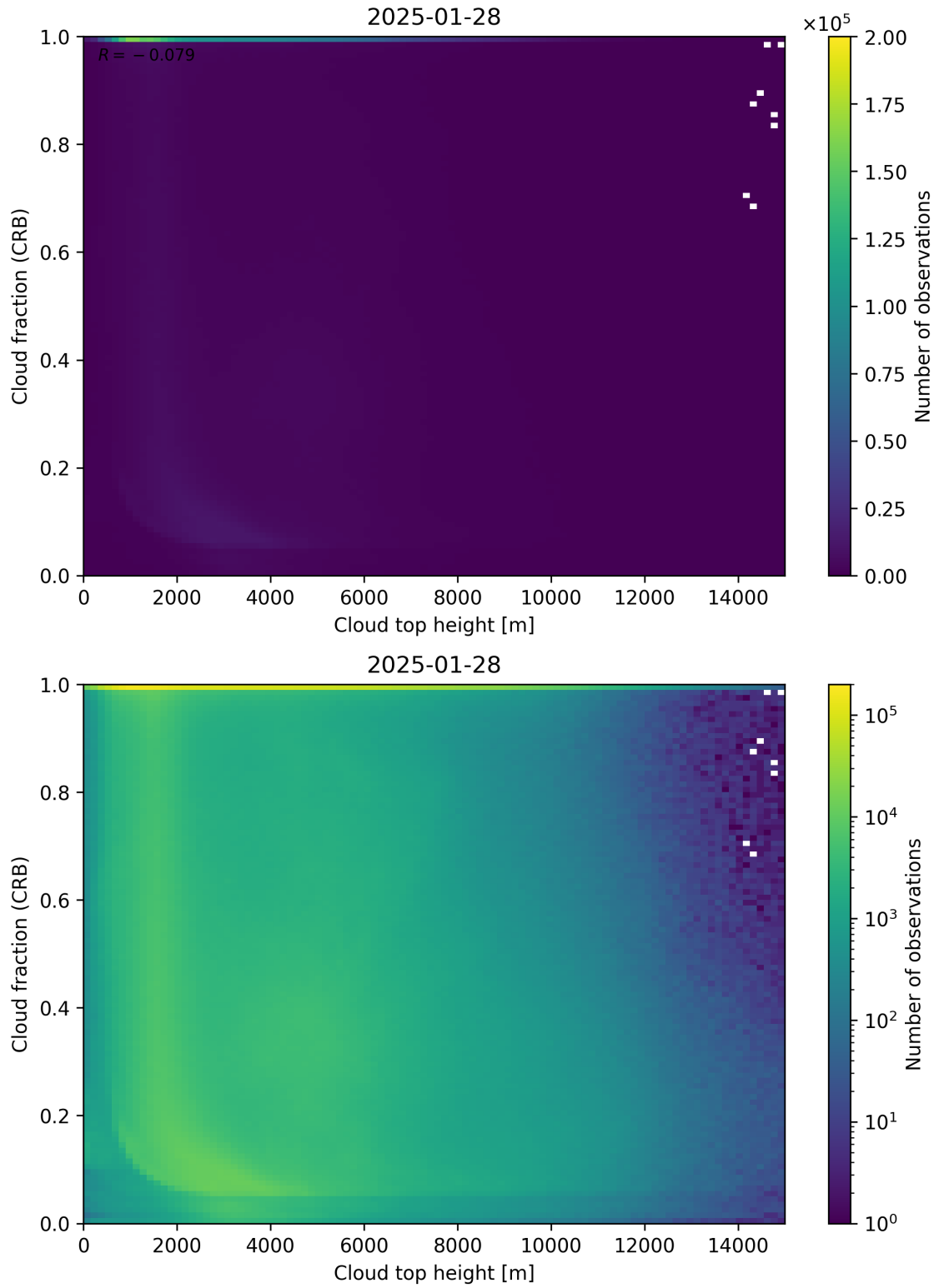
Figure 88: Scatter density plot of “Cloud top height” against “Cloud fraction (CRB)” for 2025-01-28 to 2025-01-29.
