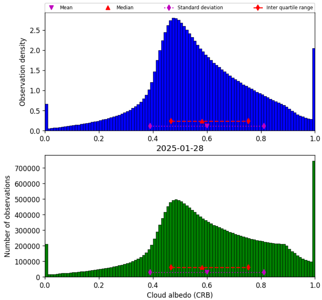
Figure 44: Histogram of “Cloud albedo (CRB)” for 2025-01-28 to 2025-01-29
