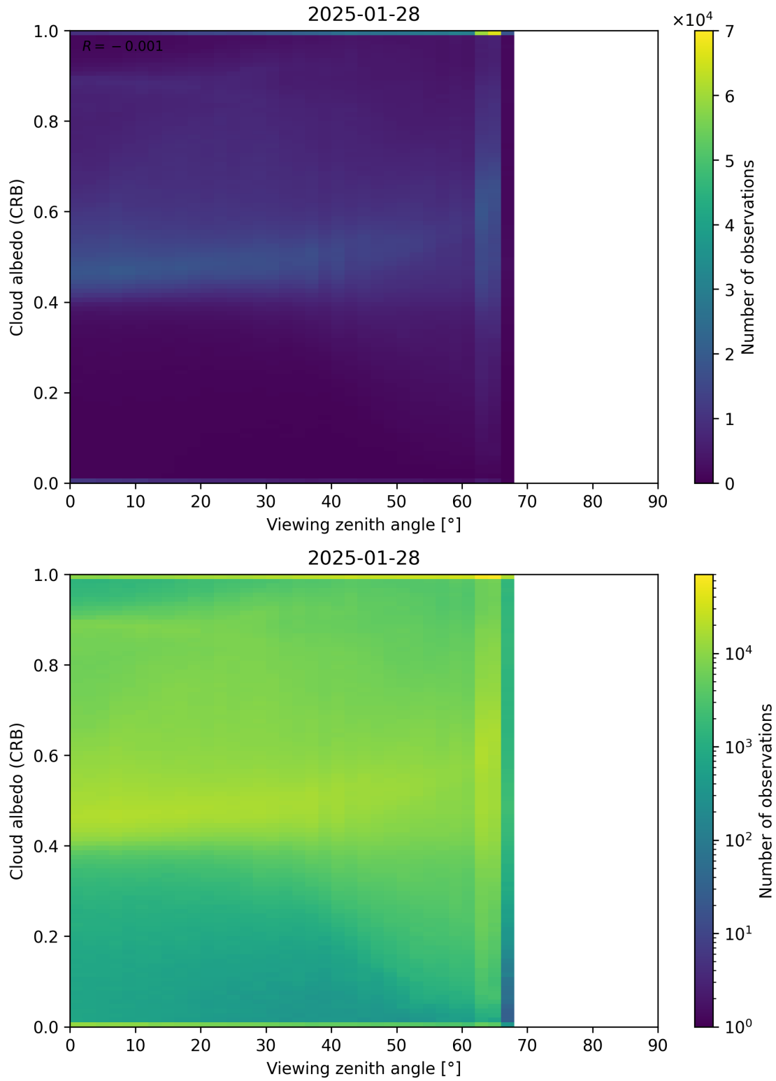
Figure 106: Scatter density plot of “Viewing zenith angle” against “Cloud albedo (CRB)” for 2025-01-28 to 2025-01-29.
