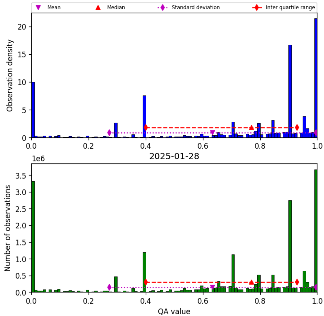
Figure 38: Histogram of “QA value” for 2025-01-28 to 2025-01-29
