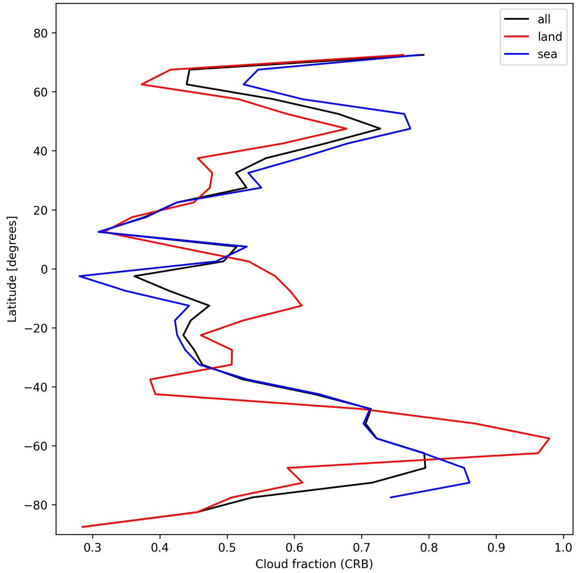
Figure 26: Zonal average of “Cloud fraction (CRB)” for 2025-01-28 to 2025-01-29.
