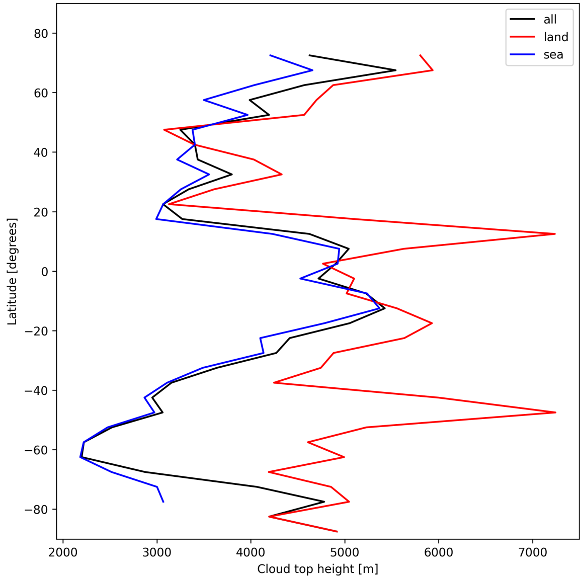
Figure 24: Zonal average of “Cloud top height” for 2025-01-28 to 2025-01-29.
