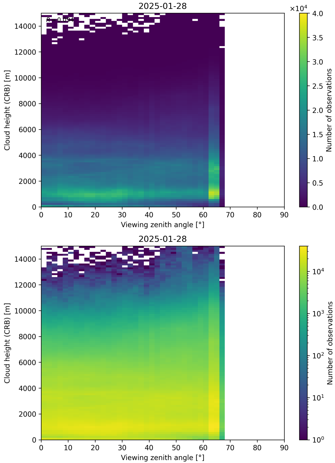
Figure 110: Scatter density plot of “Viewing zenith angle” against “Cloud height (CRB)” for 2025-01-28 to 2025-01-29.
