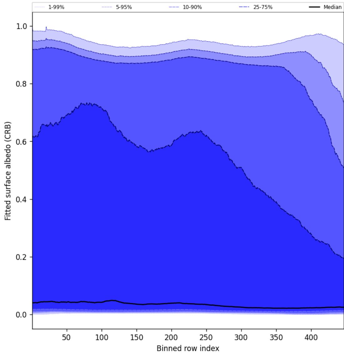
Figure 62: Along track statistics of “Fitted surface albedo (CRB)” for 2025-01-28 to 2025-01-29
