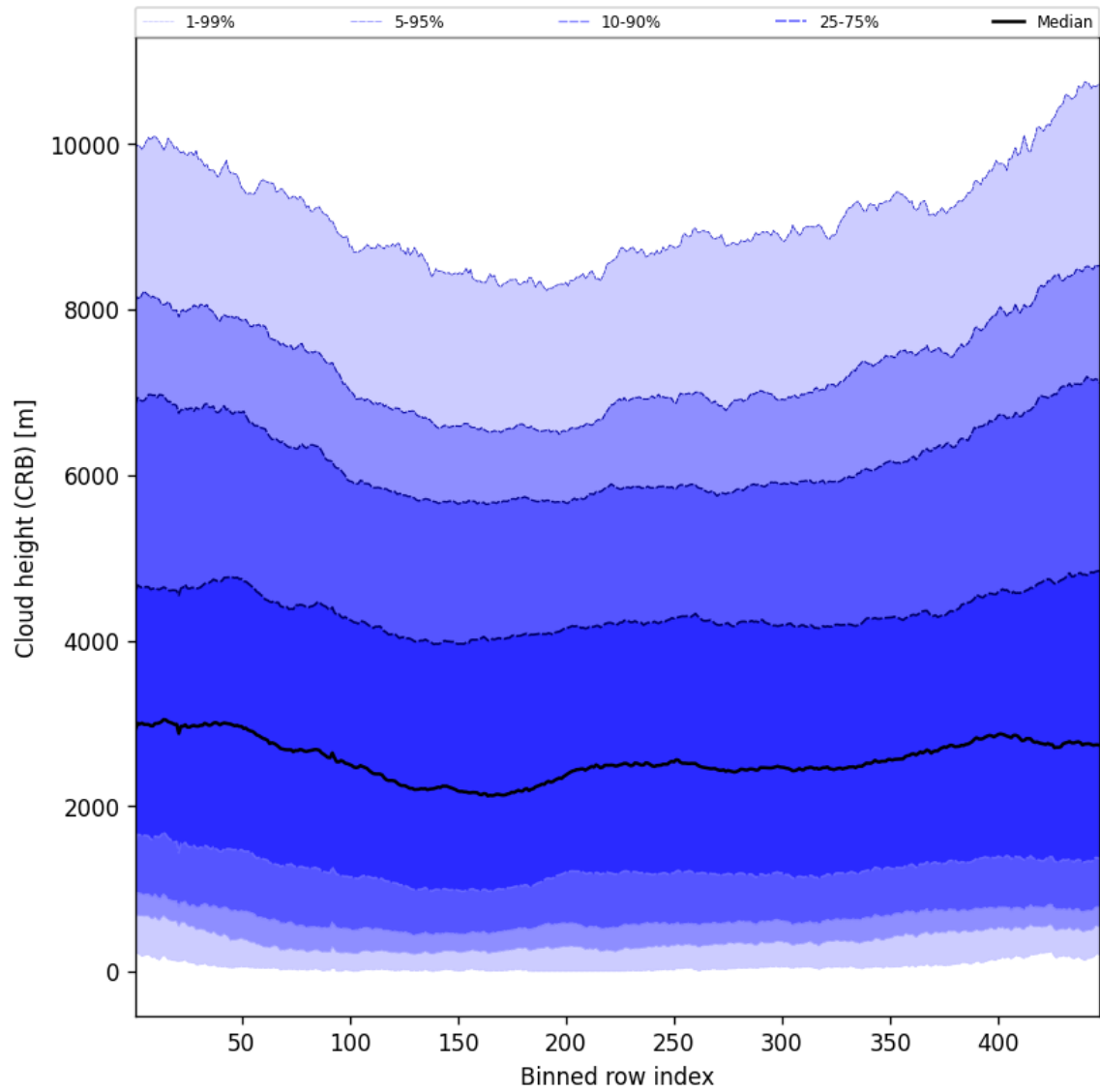
Figure 59: Along track statistics of “Cloud height (CRB)” for 2025-01-28 to 2025-01-29
