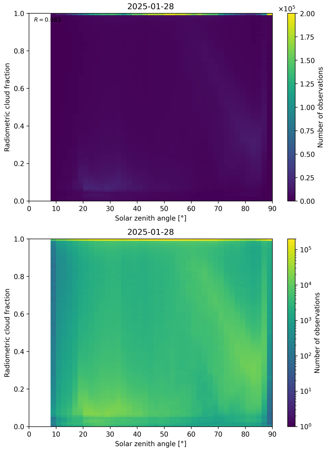
Figure 99: Scatter density plot of “Solar zenith angle” against “Radiometric cloud fraction” for 2025-01-28 to 2025-01-29.
