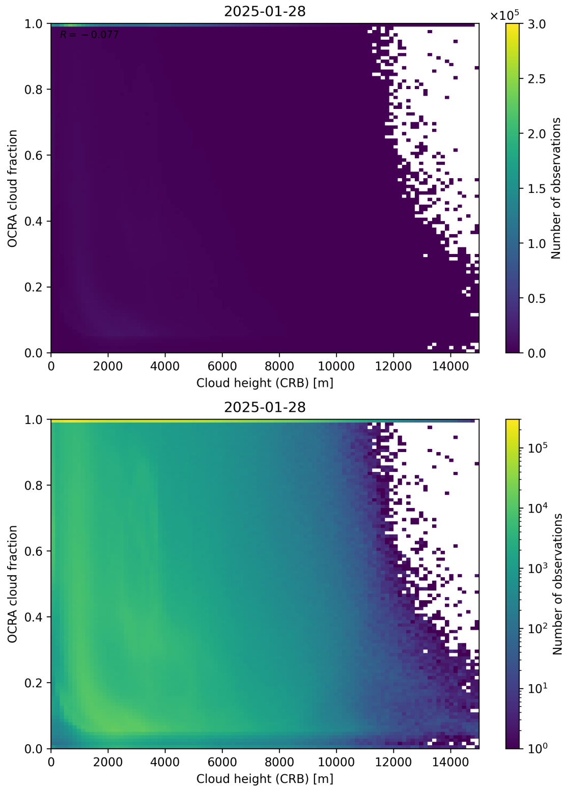
Figure 81: Scatter density plot of “Cloud height (CRB)” against “OCRA cloud fraction” for 2025-01-28 to 2025-01-29.
