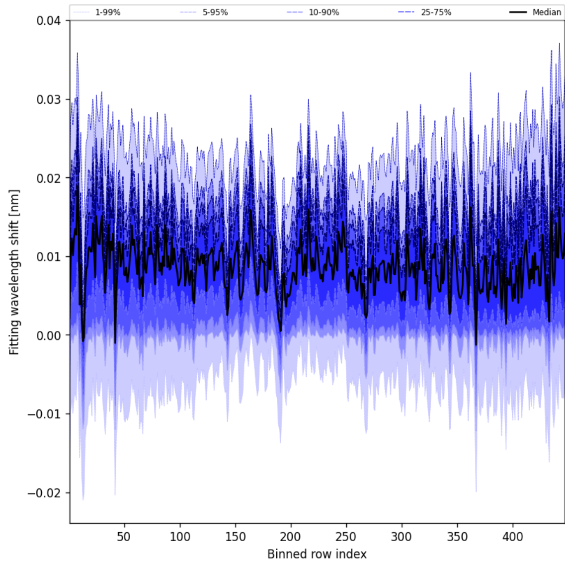
Figure 65: Along track statistics of “Fitting wavelength shift” for 2025-01-28 to 2025-01-29
