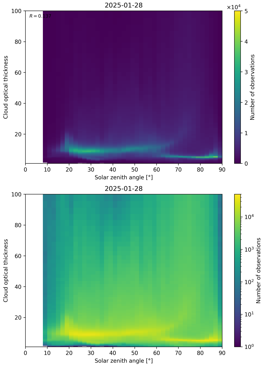
Figure 103: Scatter density plot of “Solar zenith angle” against “Cloud optical thickness” for 2025-01-28 to 2025-01-29.
