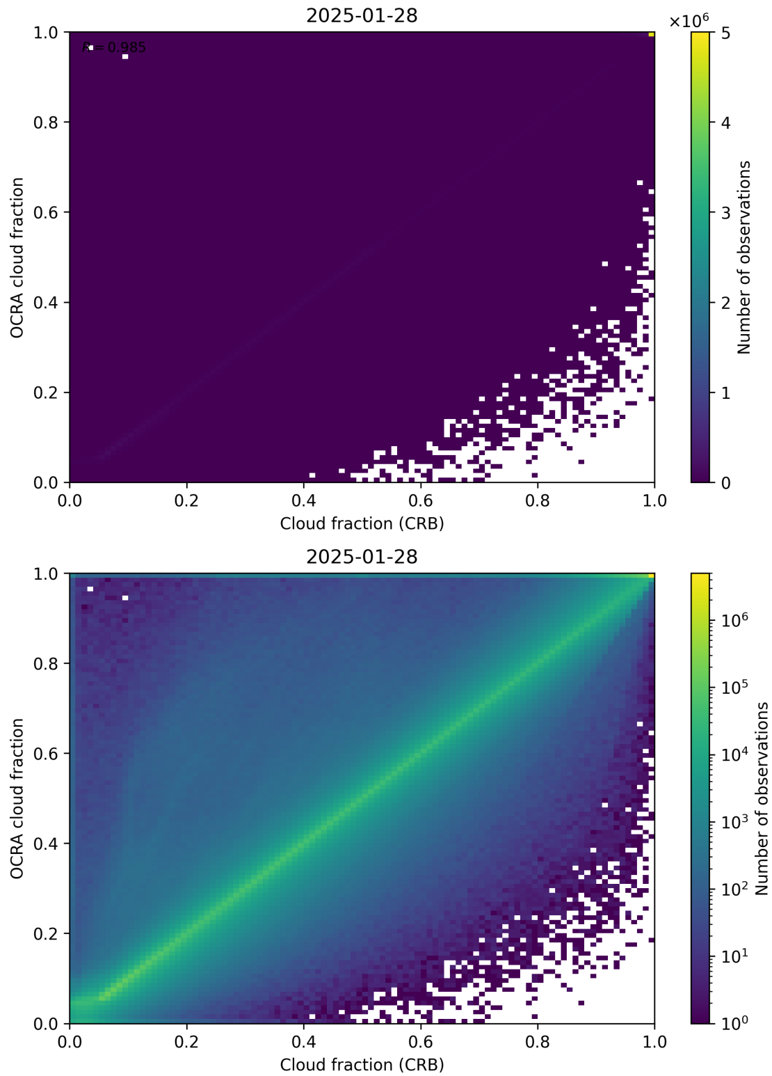
Figure 78: Scatter density plot of “Cloud fraction (CRB)” against “OCRA cloud fraction” for 2025-01-28 to 2025-01-29.
