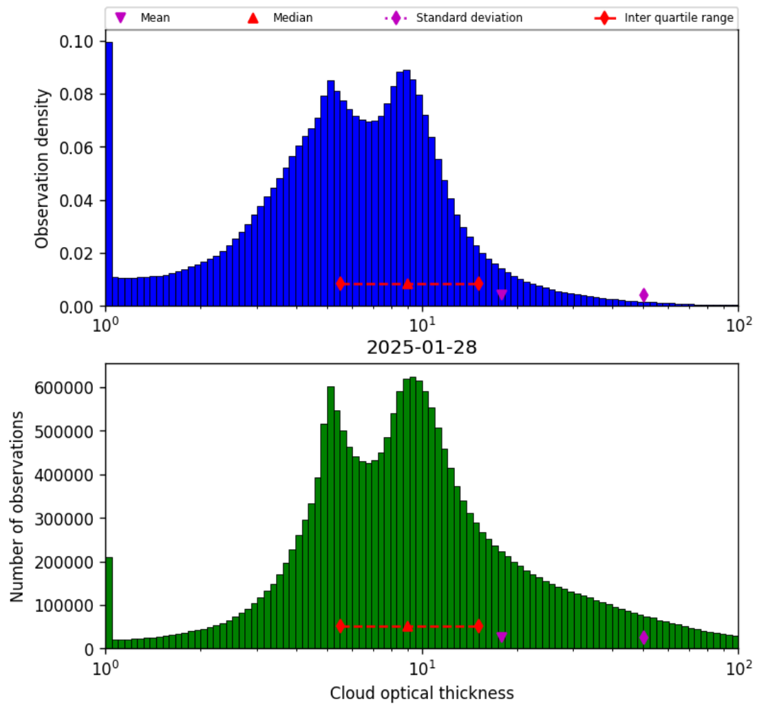
Figure 41: Histogram of “Cloud optical thickness” for 2025-01-28 to 2025-01-29
