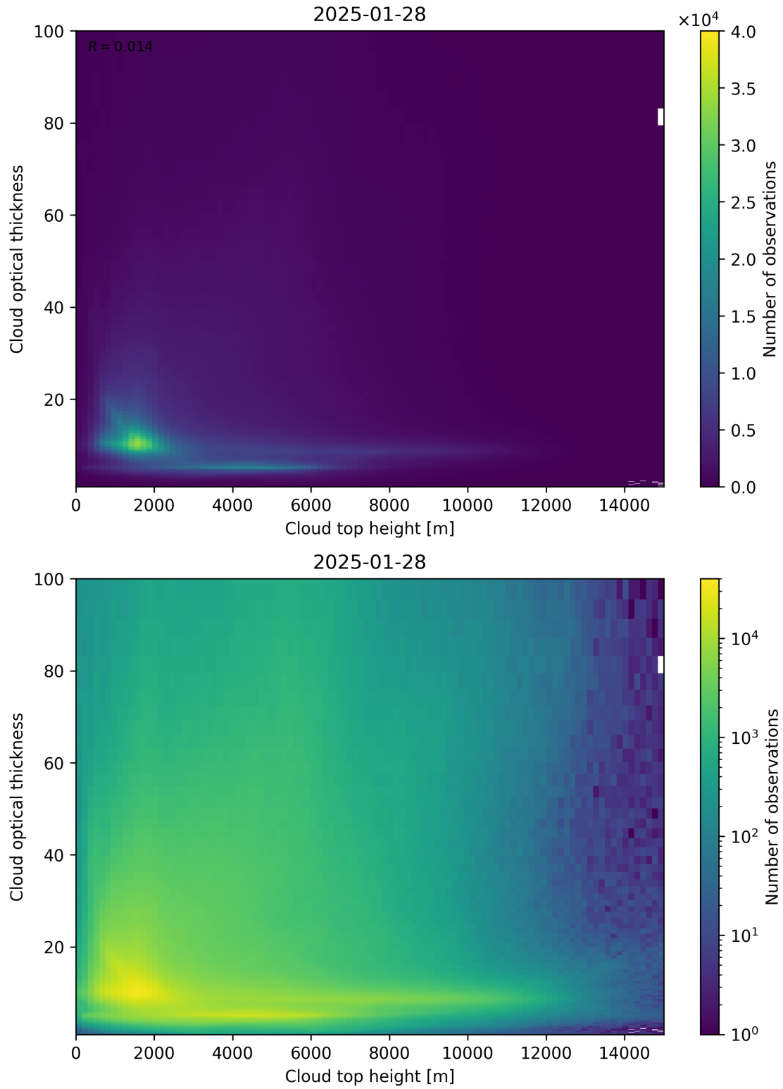
Figure 90: Scatter density plot of “Cloud top height” against “Cloud optical thickness” for 2025-01-28 to 2025-01-29.
