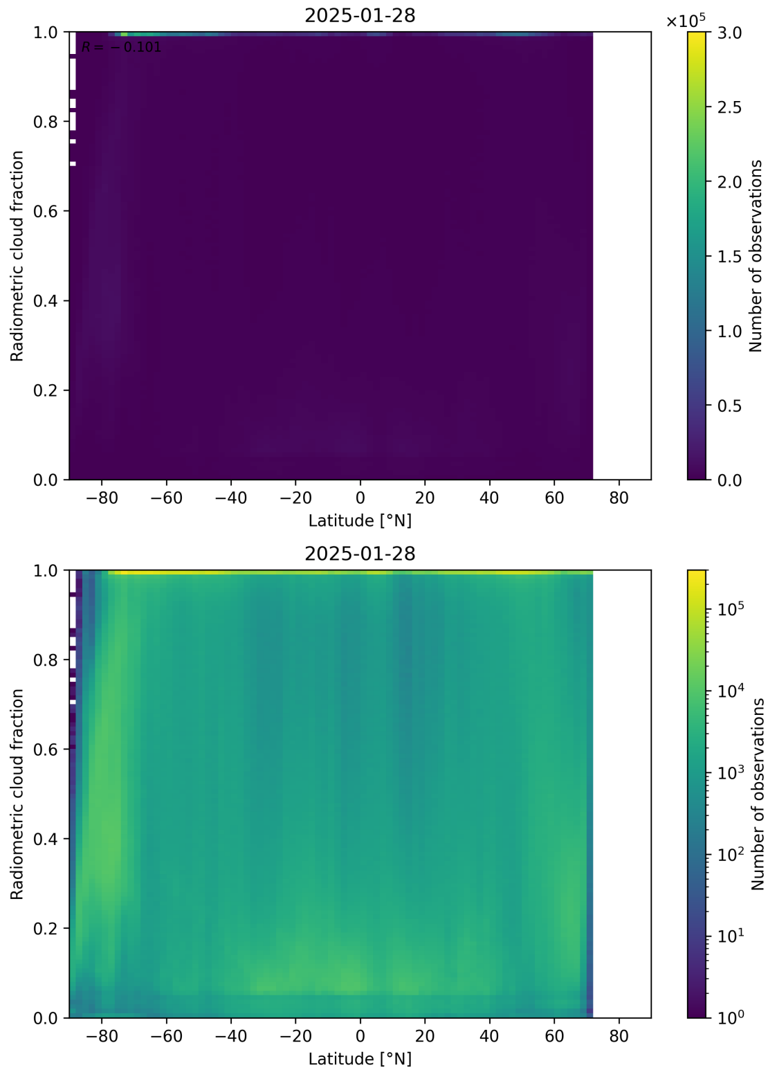
Figure 92: Scatter density plot of “Latitude” against “Radiometric cloud fraction” for 2025-01-28 to 2025-01-29.
