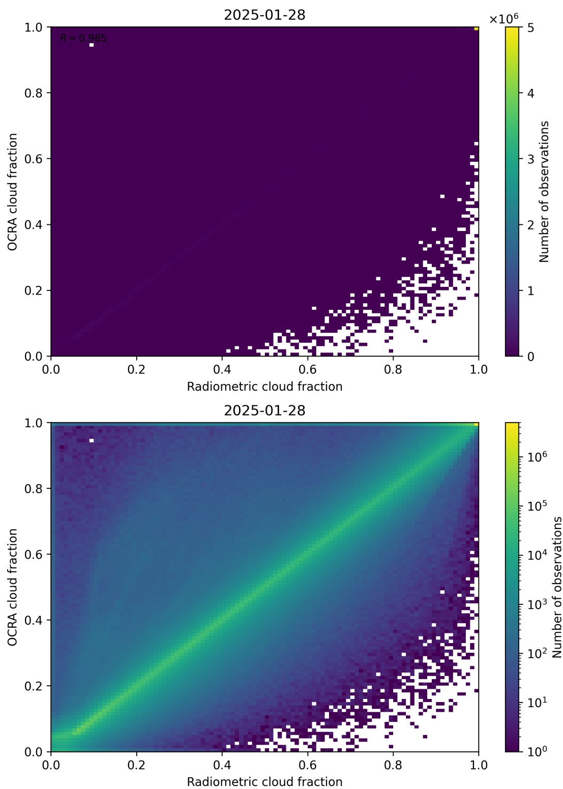
Figure 72: Scatter density plot of “Radiometric cloud fraction” against “OCRA cloud fraction” for 2025-01-28 to 2025-01-29.
