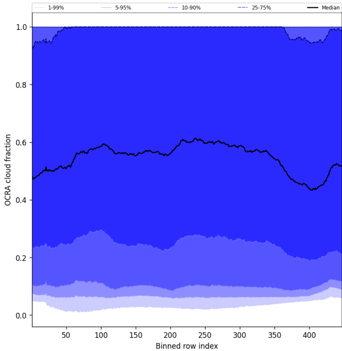
Figure 66: Along track statistics of “OCRA cloud fraction” for 2025-01-28 to 2025-01-29
