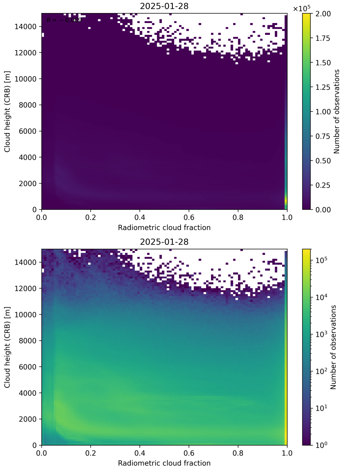
Figure 74: Scatter density plot of “Radiometric cloud fraction” against “Cloud height (CRB)” for 2025-01-28 to 2025-01-29.
