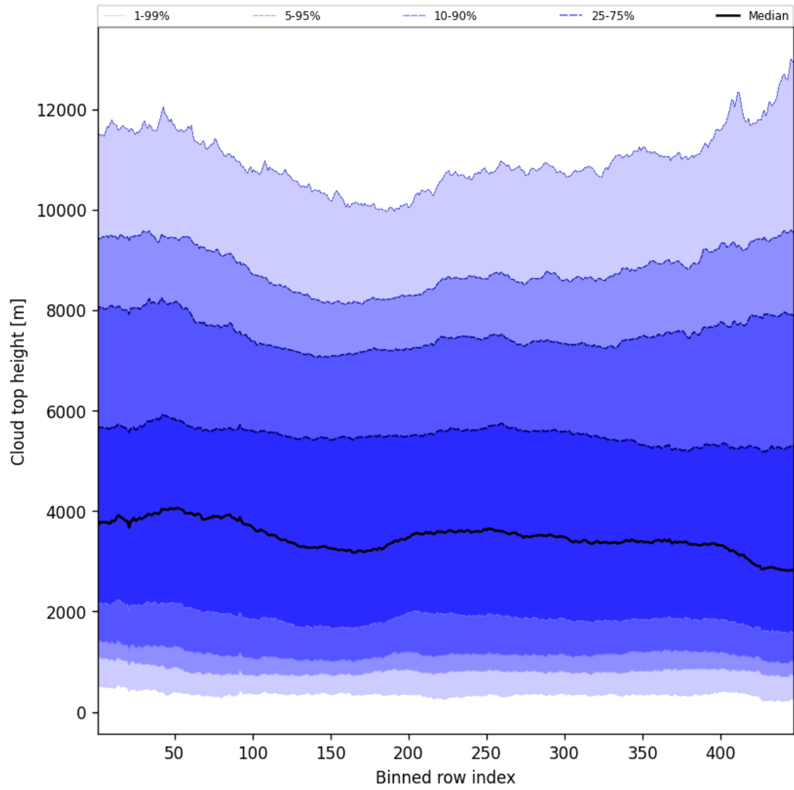
Figure 56: Along track statistics of “Cloud top height” for 2025-01-28 to 2025-01-29
