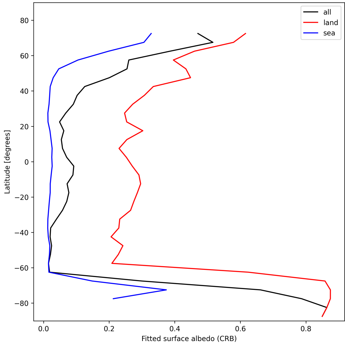
Figure 30: Zonal average of “Fitted surface albedo (CRB)” for 2025-01-28 to 2025-01-29.
