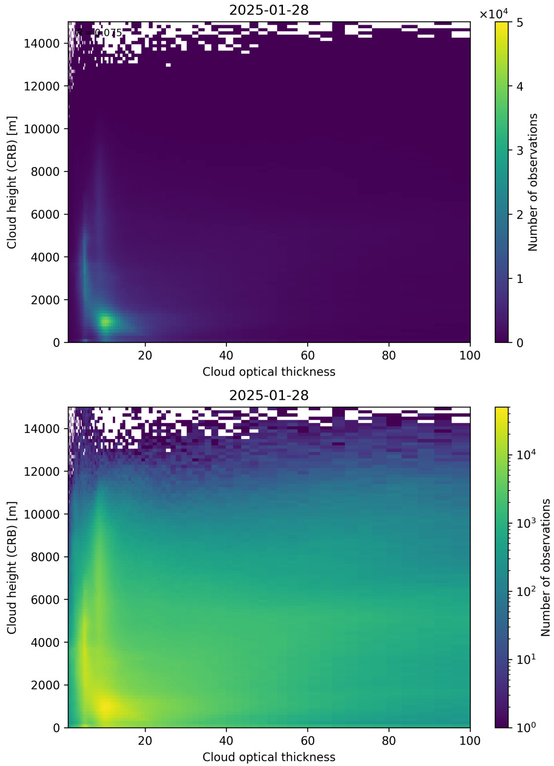
Figure 85: Scatter density plot of “Cloud optical thickness” against “Cloud height (CRB)” for 2025-01-28 to 2025-01-29.
