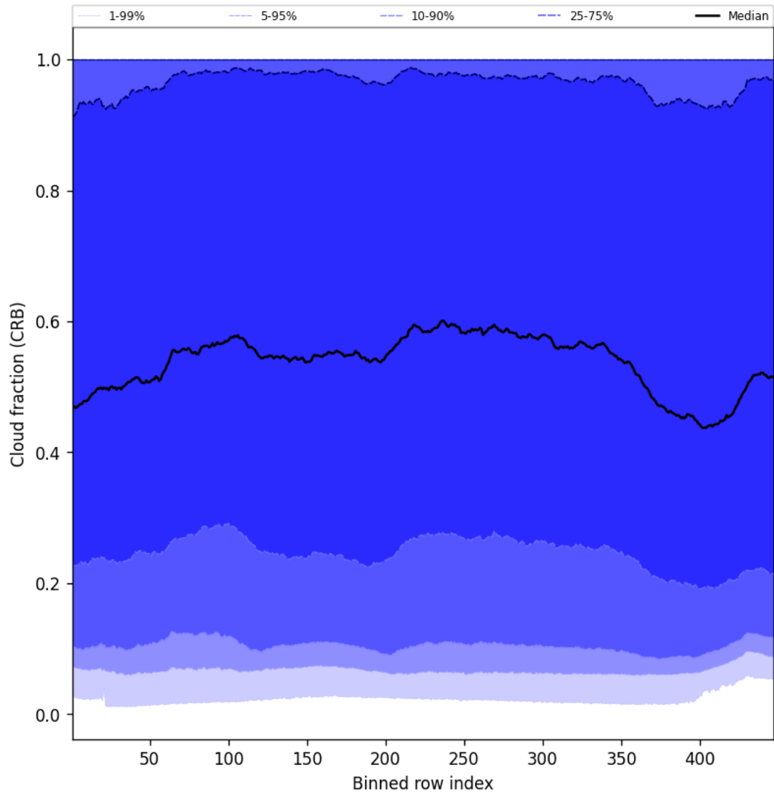
Figure 58: Along track statistics of “Cloud fraction (CRB)” for 2025-01-28 to 2025-01-29
