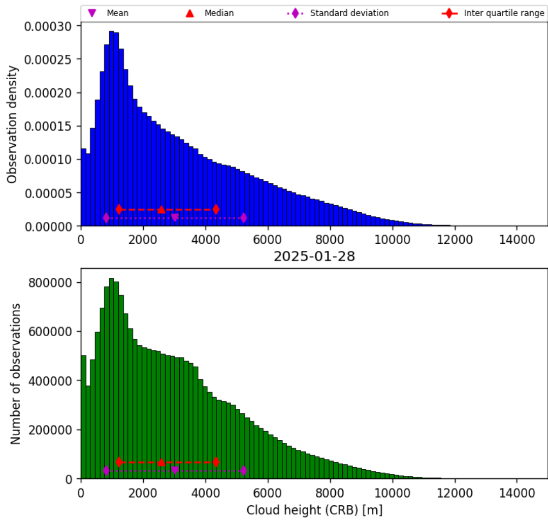
Figure 43: Histogram of “Cloud height (CRB)” for 2025-01-28 to 2025-01-29
