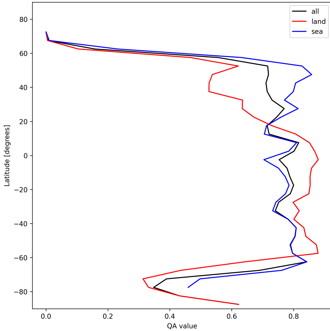
Figure 22: Zonal average of “QA value” for 2025-01-28 to 2025-01-29.
