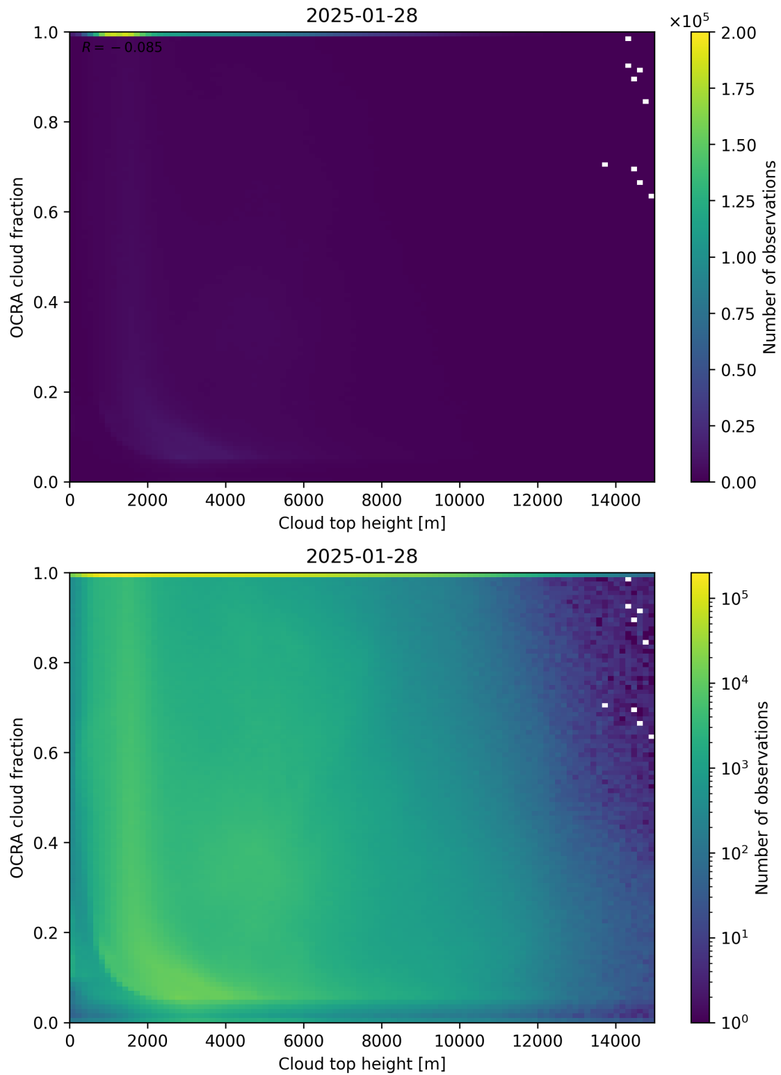
Figure 87: Scatter density plot of “Cloud top height” against “OCRA cloud fraction” for 2025-01-28 to 2025-01-29.
