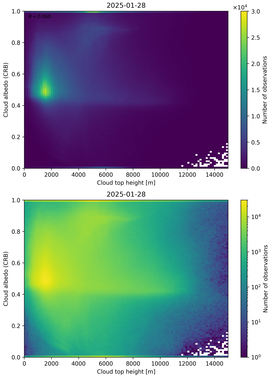
Figure 86: Scatter density plot of “Cloud top height” against “Cloud albedo (CRB)” for 2025-01-28 to 2025-01-29.
