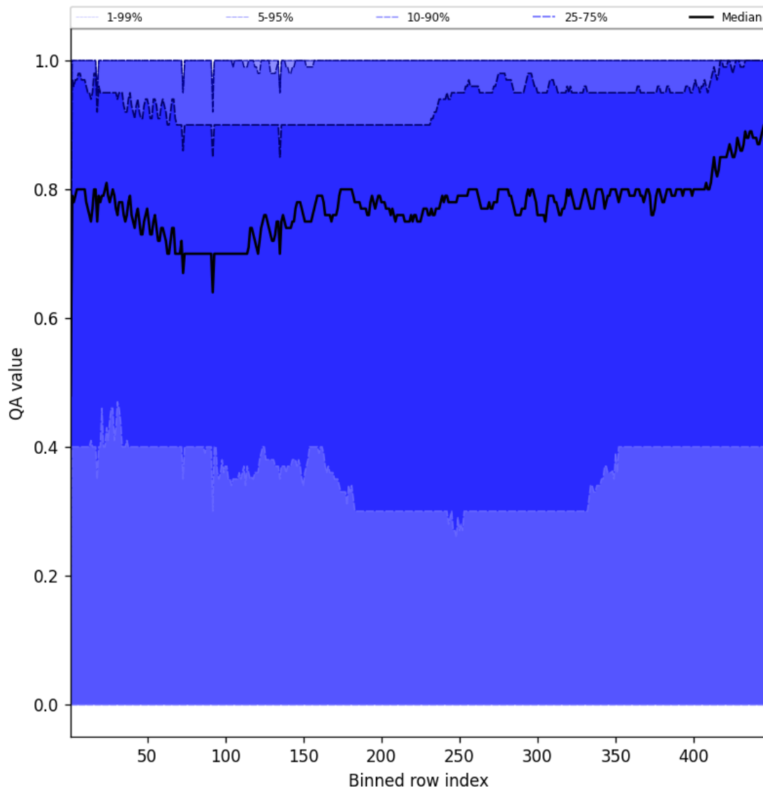
Figure 54: Along track statistics of “QA value” for 2025-01-28 to 2025-01-29
