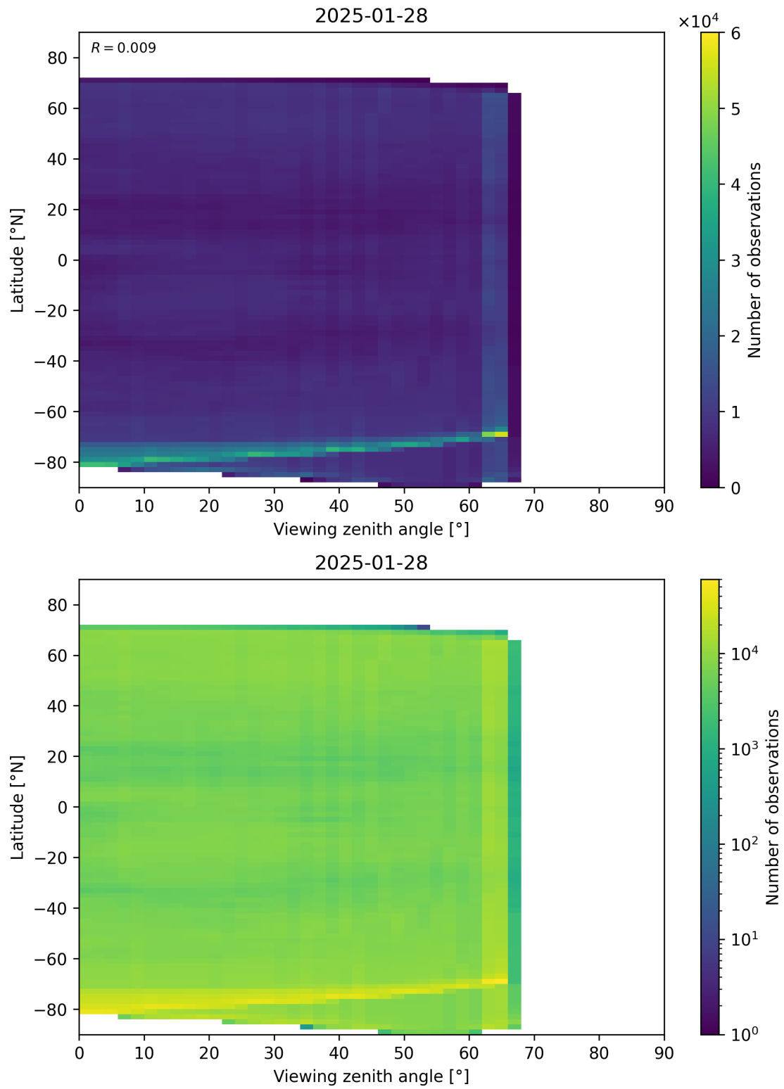
Figure 113: Scatter density plot of “Viewing zenith angle” against “Latitude” for 2025-01-28 to 2025-01-29.
