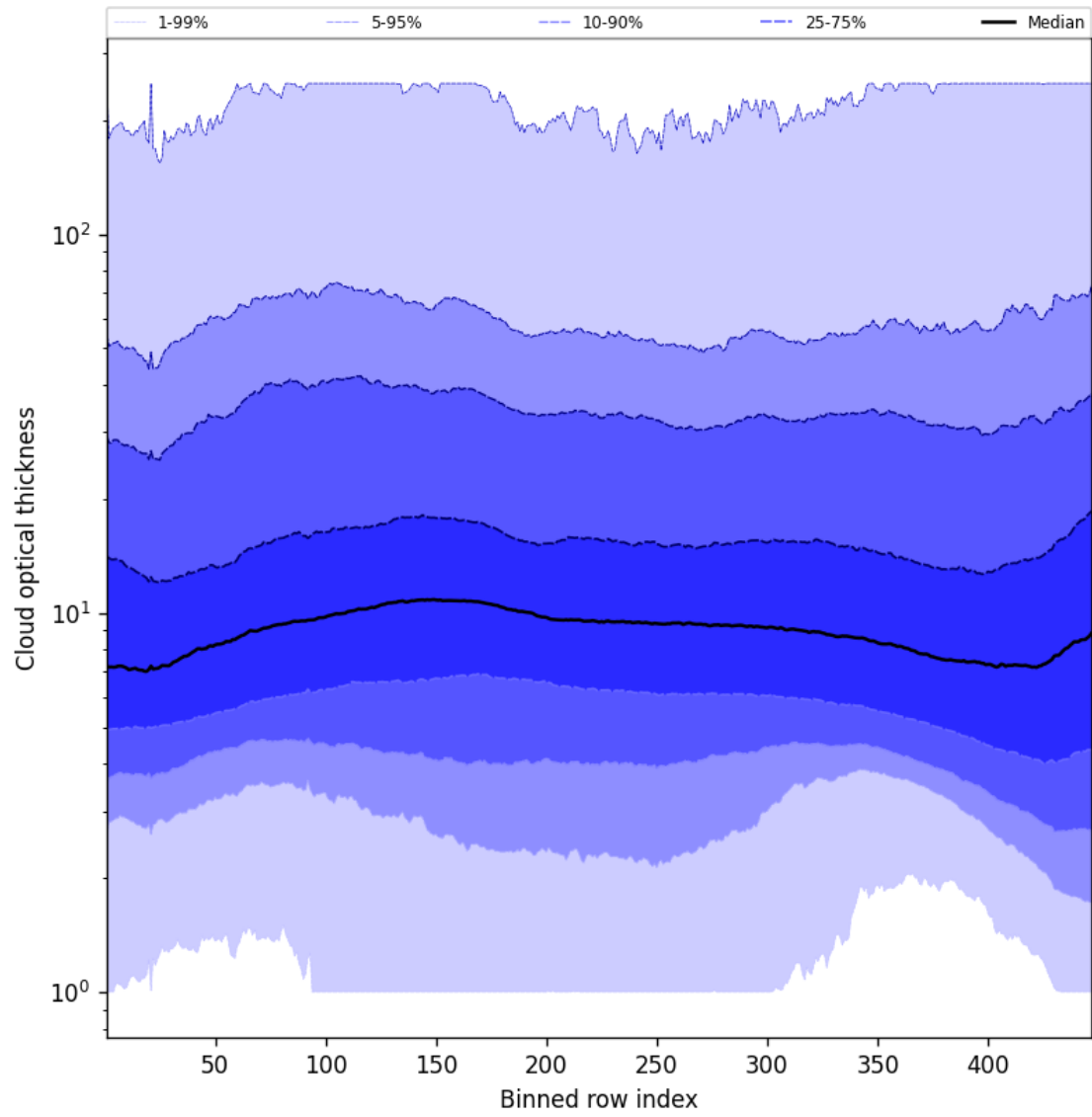
Figure 57: Along track statistics of “Cloud optical thickness” for 2025-01-28 to 2025-01-29
