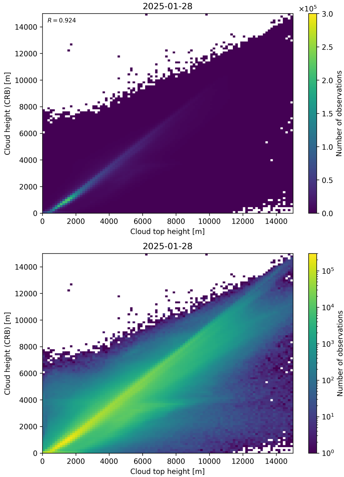
Figure 89: Scatter density plot of “Cloud top height” against “Cloud height (CRB)” for 2025-01-28 to 2025-01-29.
