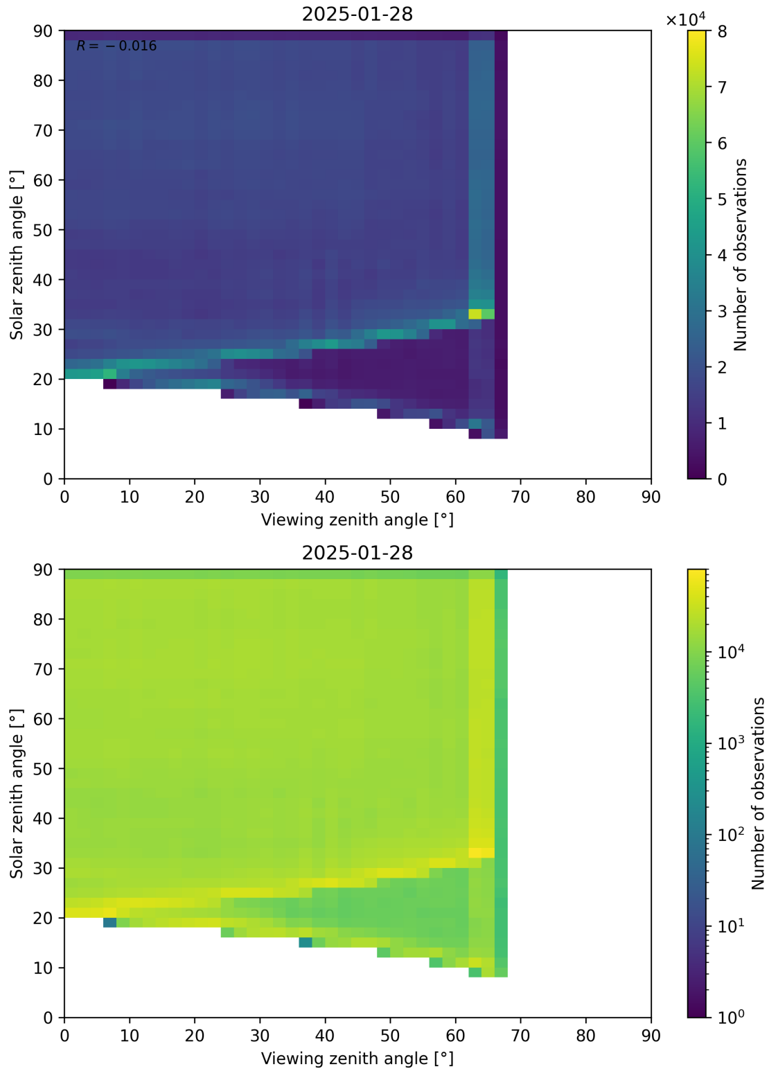
Figure 114: Scatter density plot of “Viewing zenith angle” against “Solar zenith angle” for 2025-01-28 to 2025-01-29.
