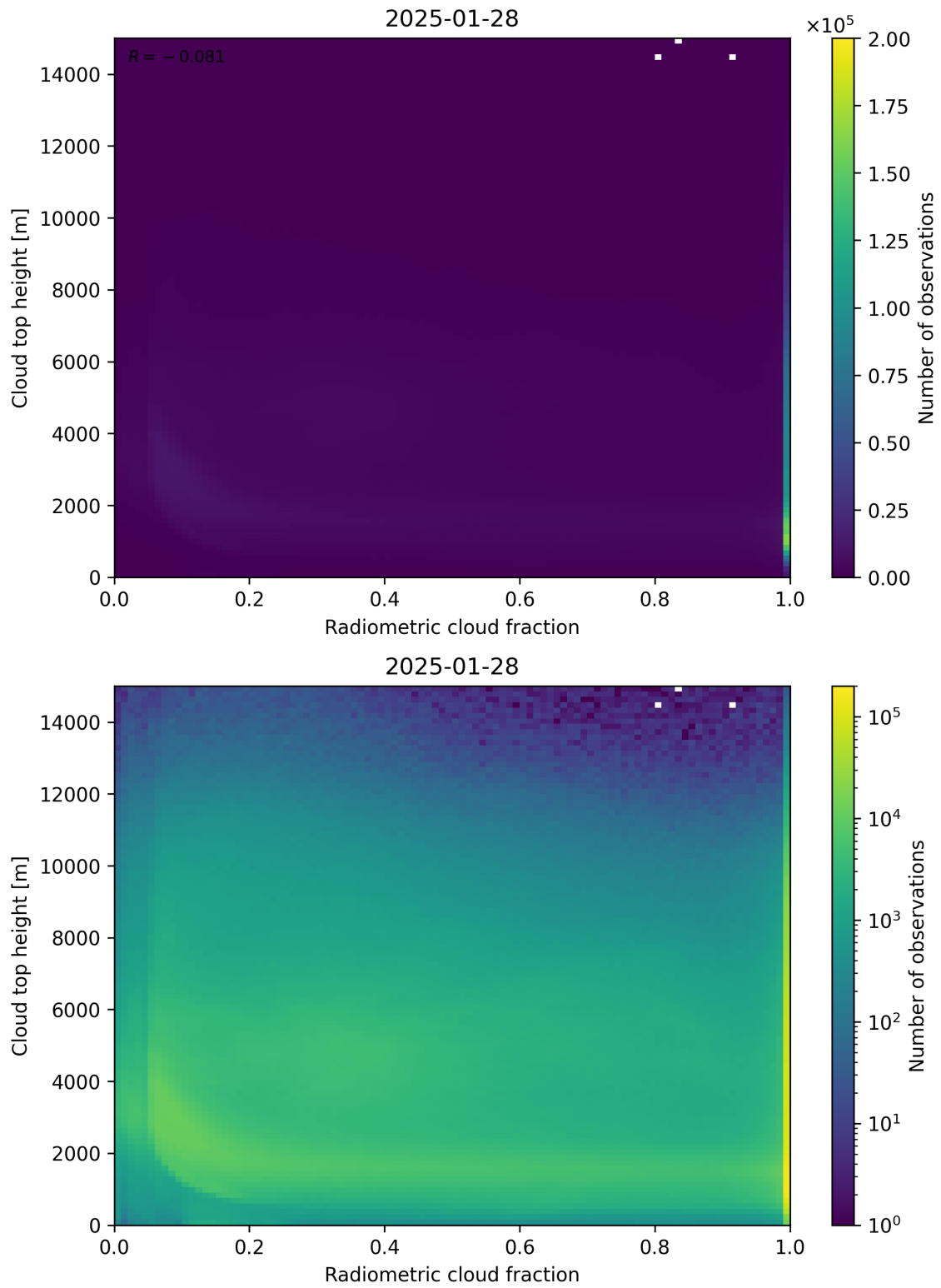
Figure 76: Scatter density plot of “Radiometric cloud fraction” against “Cloud top height” for 2025-01-28 to 2025-01-29.
