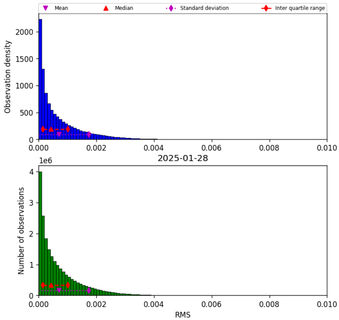
Figure 47: Histogram of “RMS” for 2025-01-28 to 2025-01-29
