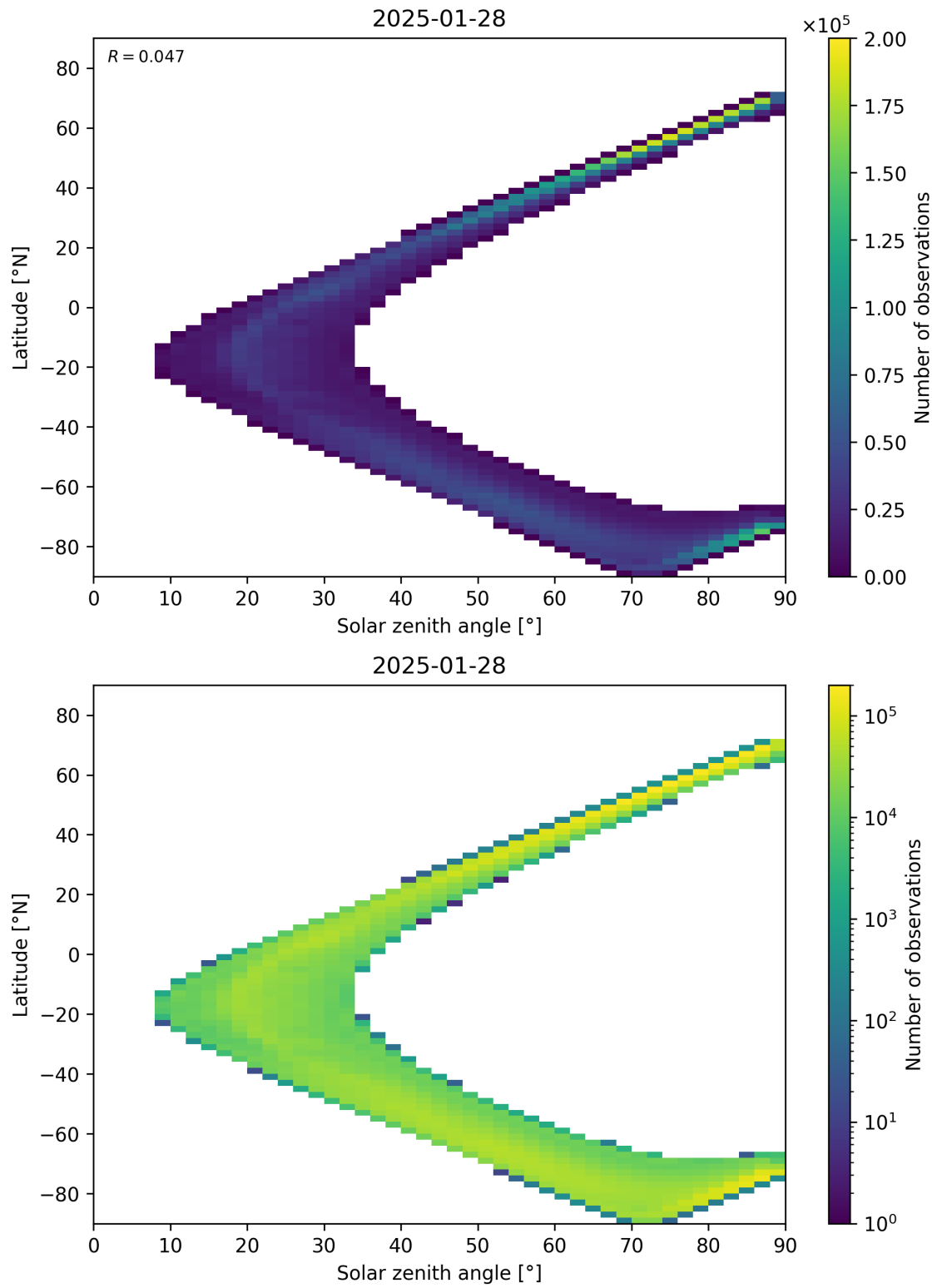
Figure 105: Scatter density plot of “Solar zenith angle” against “Latitude” for 2025-01-28 to 2025-01-29.
