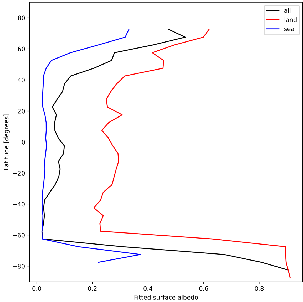
Figure 29: Zonal average of “Fitted surface albedo” for 2025-01-28 to 2025-01-29.
