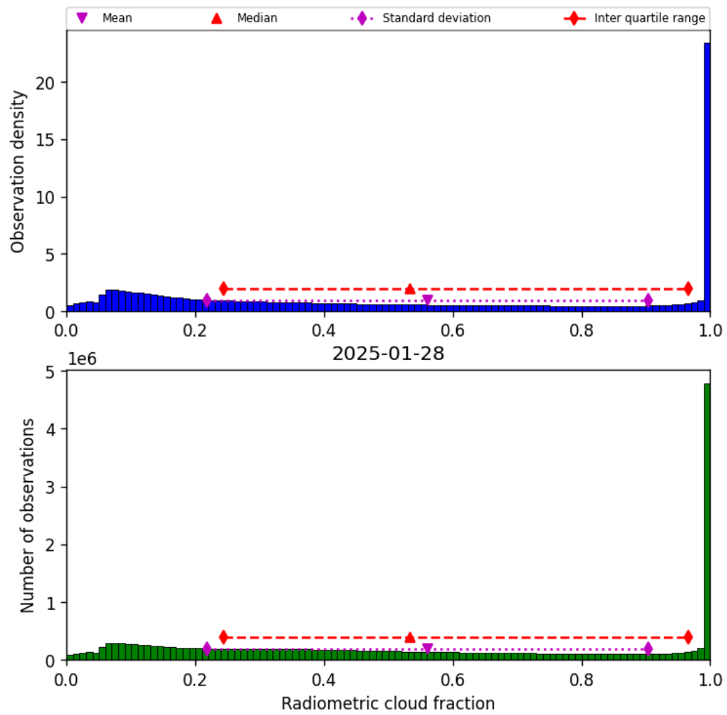
Figure 39: Histogram of “Radiometric cloud fraction” for 2025-01-28 to 2025-01-29
