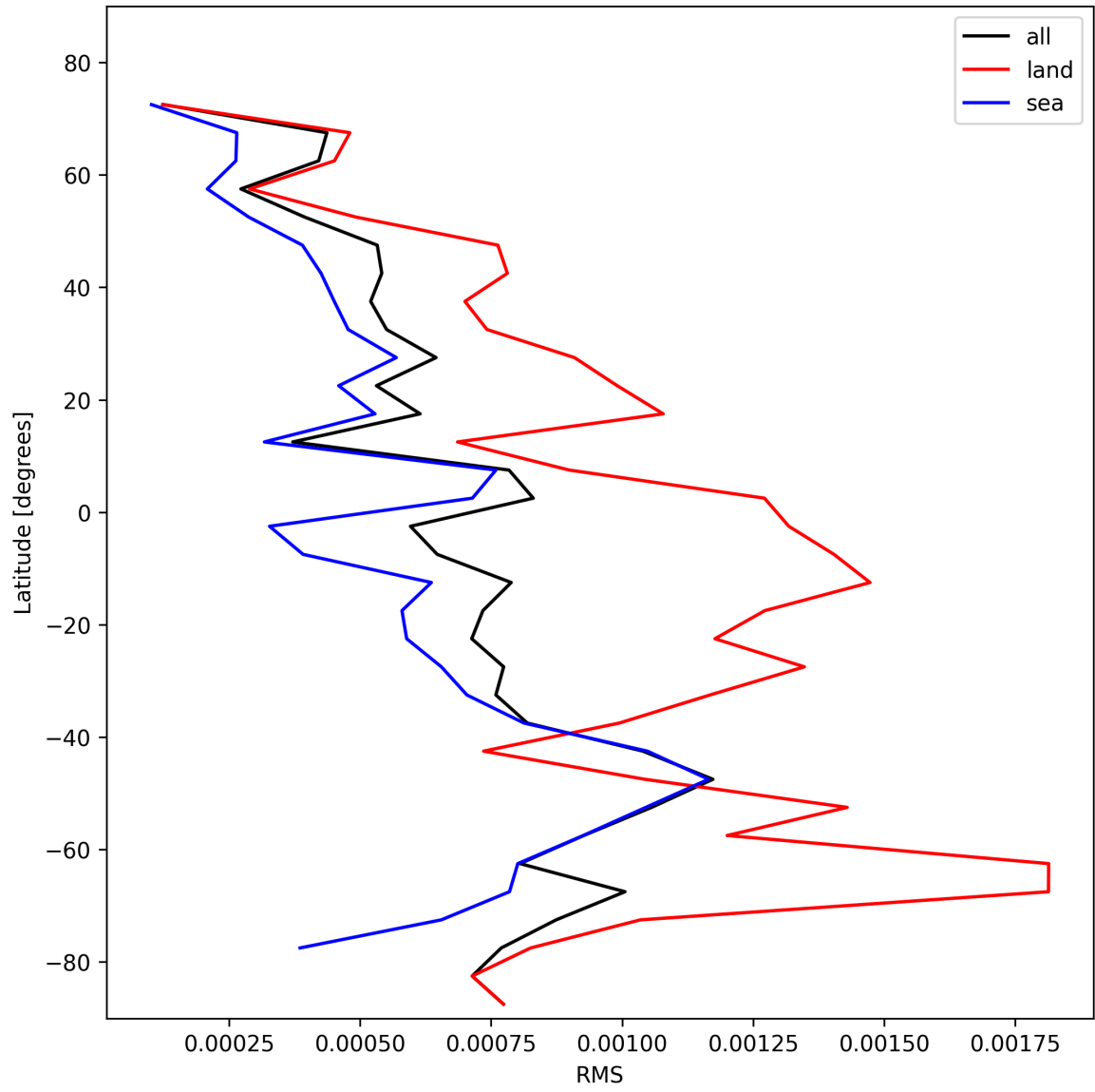
Figure 31: Zonal average of “RMS” for 2025-01-28 to 2025-01-29.
