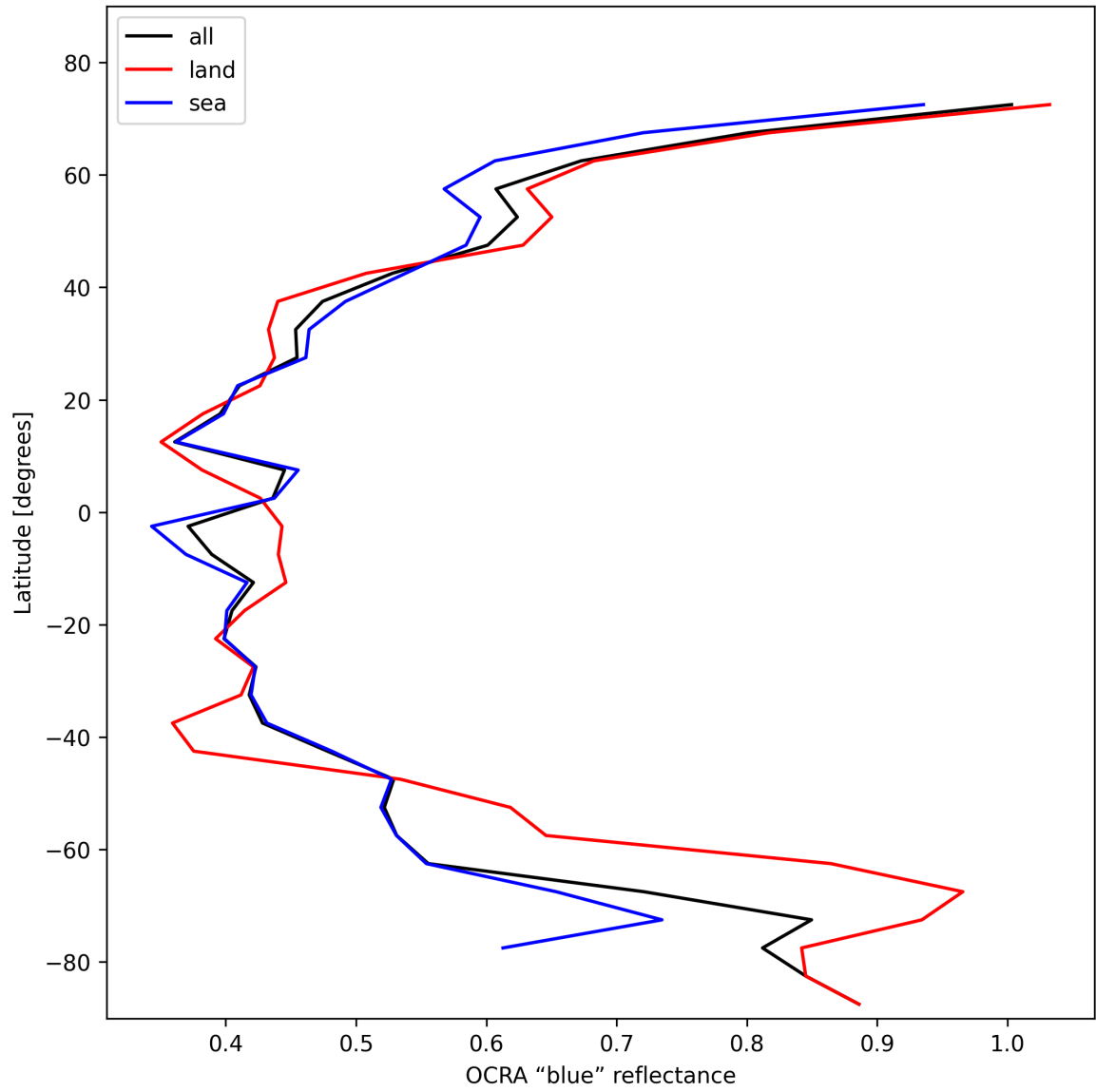
Figure 35: Zonal average of “OCRA “blue” reflectance” for 2025-01-28 to 2025-01-29.
