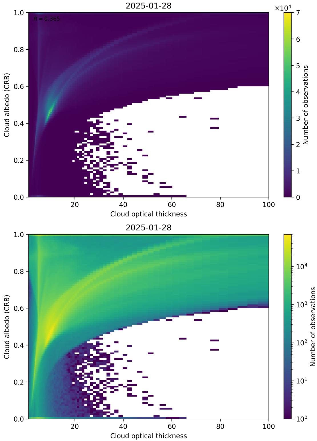
Figure 82: Scatter density plot of “Cloud optical thickness” against “Cloud albedo (CRB)” for 2025-01-28 to 2025-01-29.
