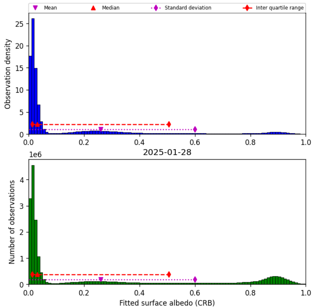
Figure 46: Histogram of "Fitted surface albedo (CRB)" for 2025-01-28 to 2025-01-29
