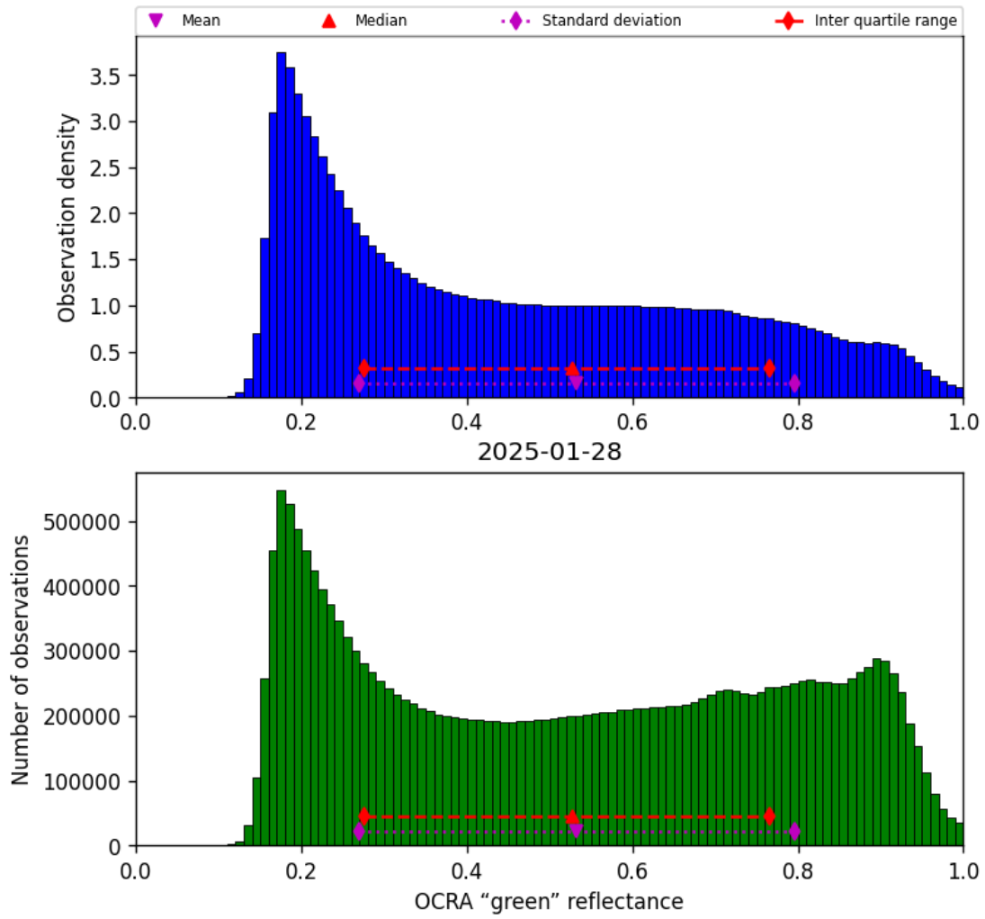
Figure 52: Histogram of “OCRA “green” reflectance” for 2025-01-28 to 2025-01-29
