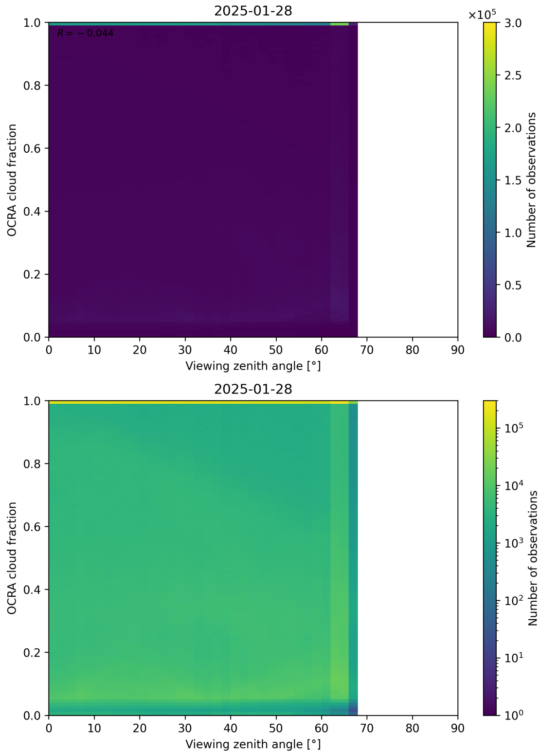
Figure 108: Scatter density plot of “Viewing zenith angle” against “OCRA cloud fraction” for 2025-01-28 to 2025-01-29.
