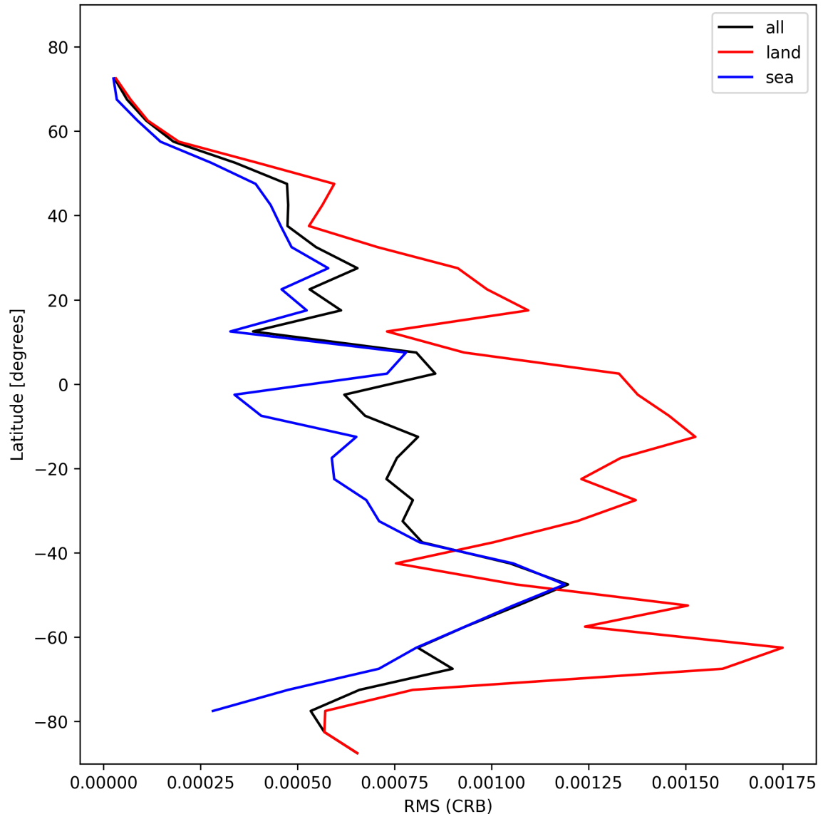
Figure 32: Zonal average of “RMS (CRB)” for 2025-01-28 to 2025-01-29.
