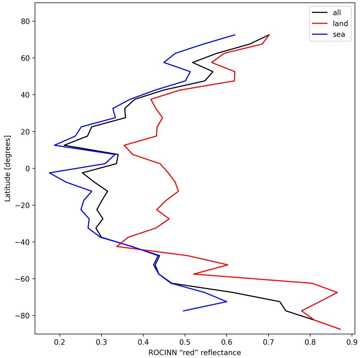
Figure 37: Zonal average of “ROCINN “red” reflectance” for 2025-01-28 to 2025-01-29.
