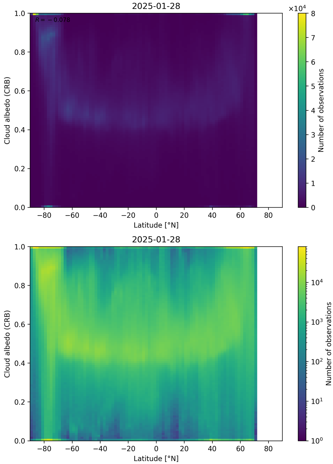
Figure 91: Scatter density plot of “Latitude” against “Cloud albedo (CRB)” for 2025-01-28 to 2025-01-29.
