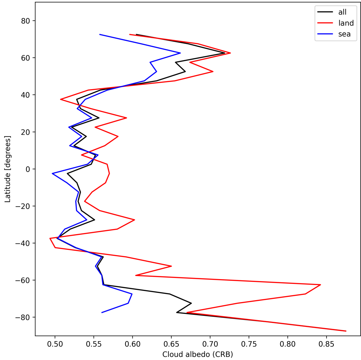
Figure 28: Zonal average of “Cloud albedo (CRB)” for 2025-01-28 to 2025-01-29.
