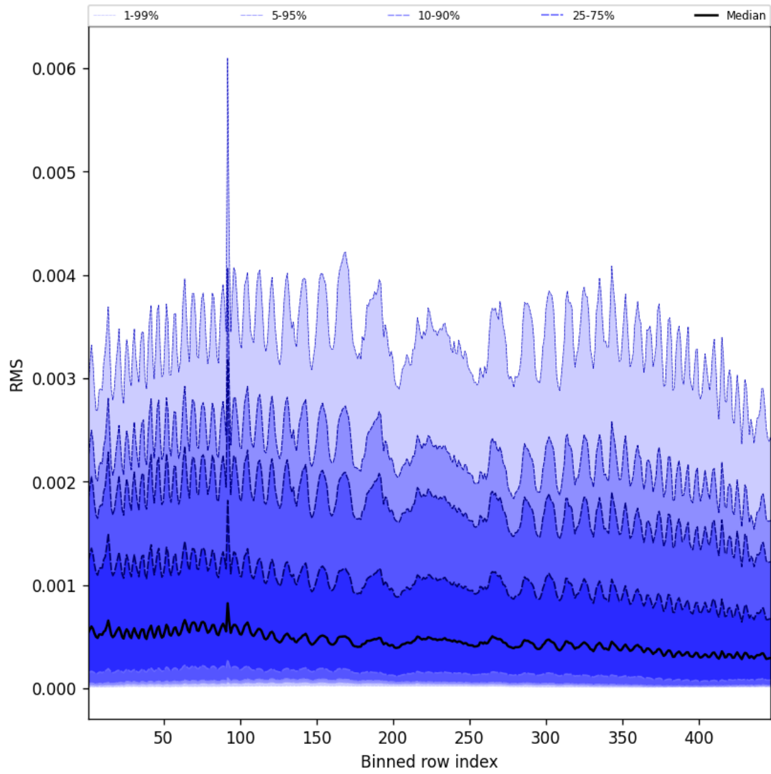
Figure 63: Along track statistics of “RMS” for 2025-01-28 to 2025-01-29
