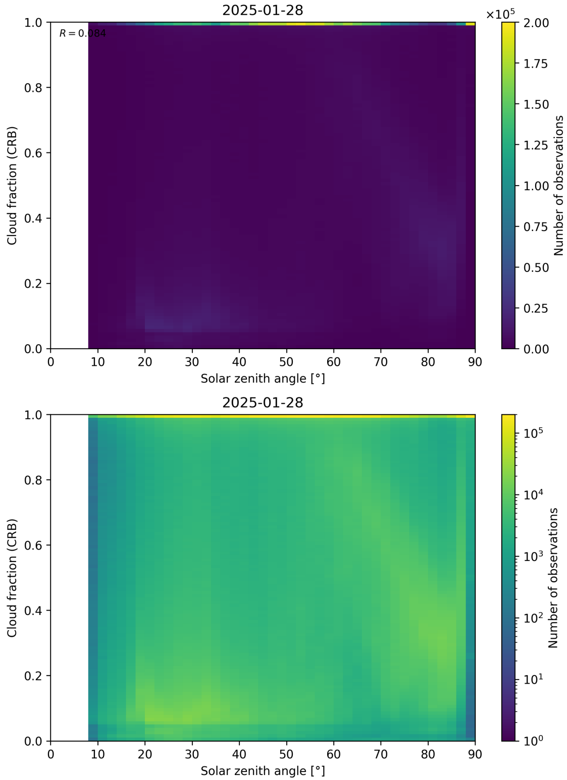
Figure 101: Scatter density plot of “Solar zenith angle” against “Cloud fraction (CRB)” for 2025-01-28 to 2025-01-29.
