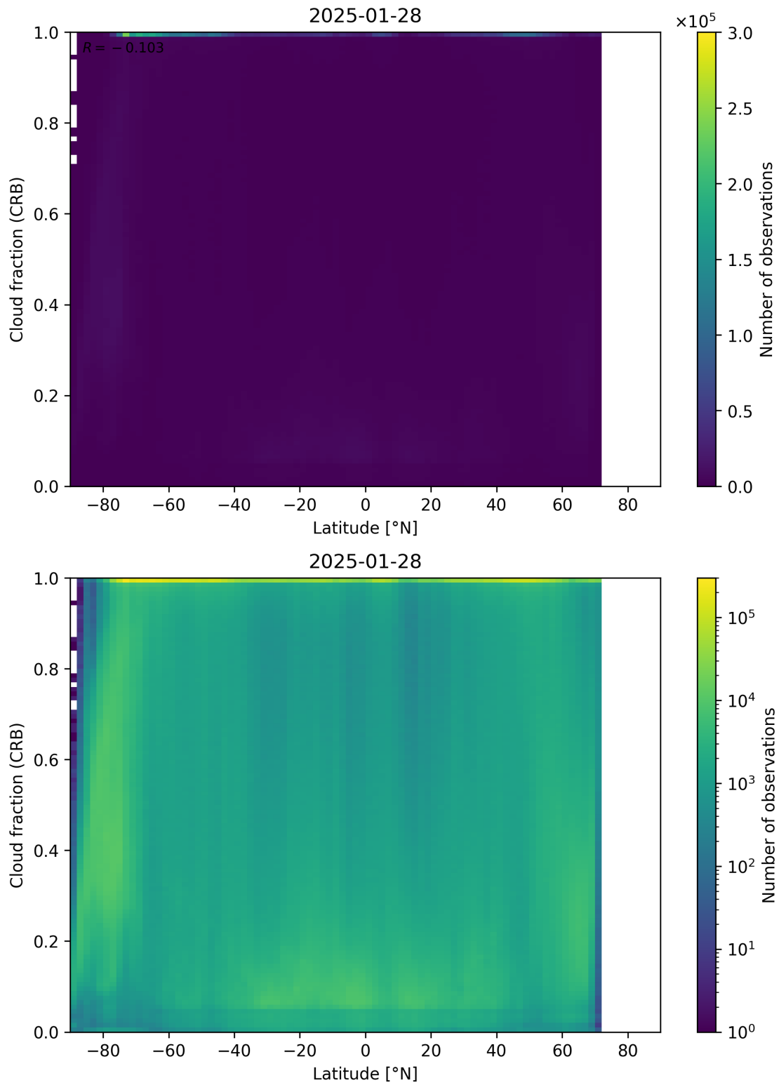
Figure 94: Scatter density plot of “Latitude” against “Cloud fraction (CRB)” for 2025-01-28 to 2025-01-29.
