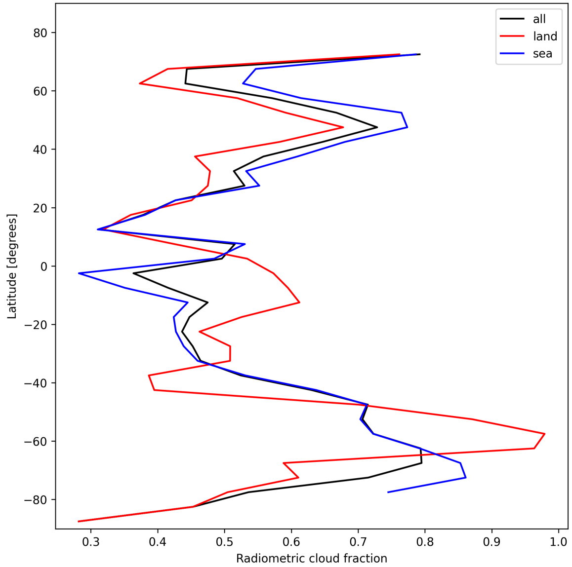
Figure 23: Zonal average of “Radiometric cloud fraction” for 2025-01-28 to 2025-01-29.
