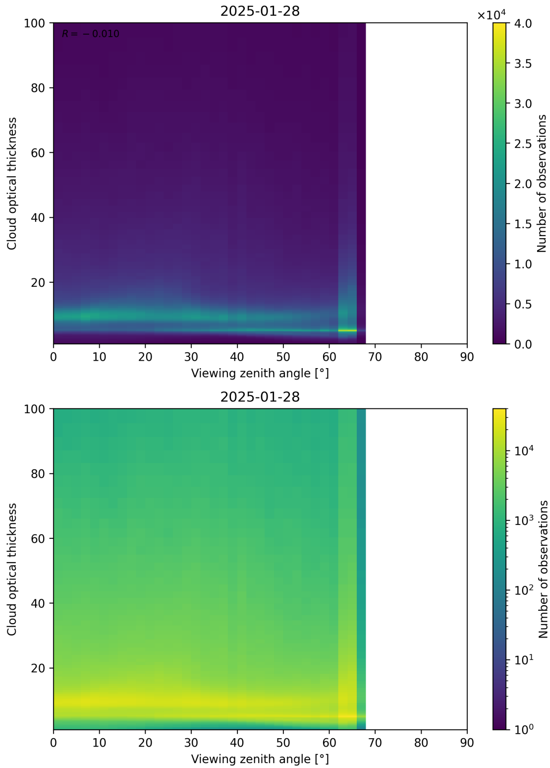
Figure 111: Scatter density plot of “Viewing zenith angle” against “Cloud optical thickness” for 2025-01-28 to 2025-01-29.
