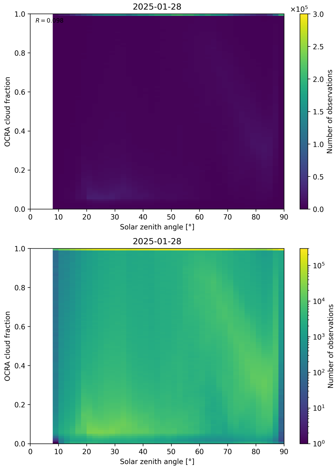
Figure 100: Scatter density plot of “Solar zenith angle” against “OCRA cloud fraction” for 2025-01-28 to 2025-01-29.
