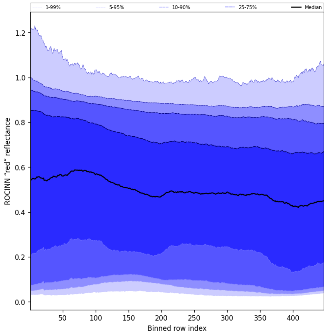
Figure 69: Along track statistics of "ROCINN "red" reflectance" for 2025-01-28 to 2025-01-29
