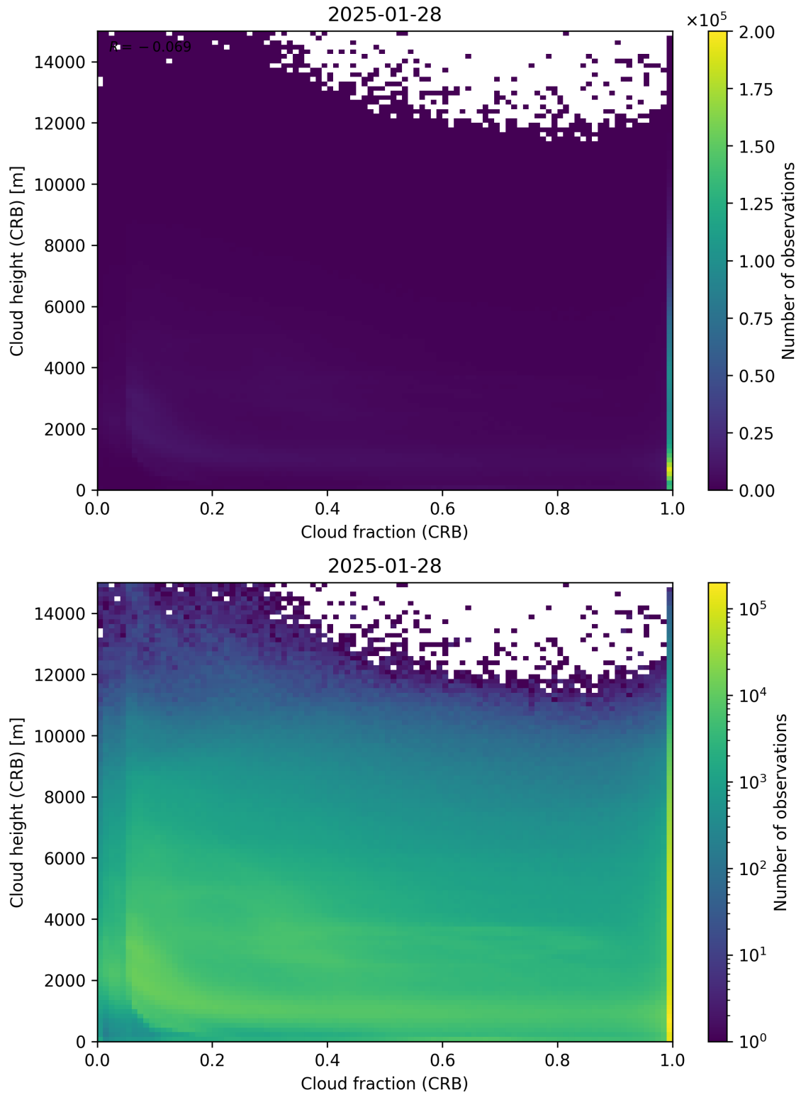
Figure 79: Scatter density plot of “Cloud fraction (CRB)” against “Cloud height (CRB)” for 2025-01-28 to 2025-01-29.
