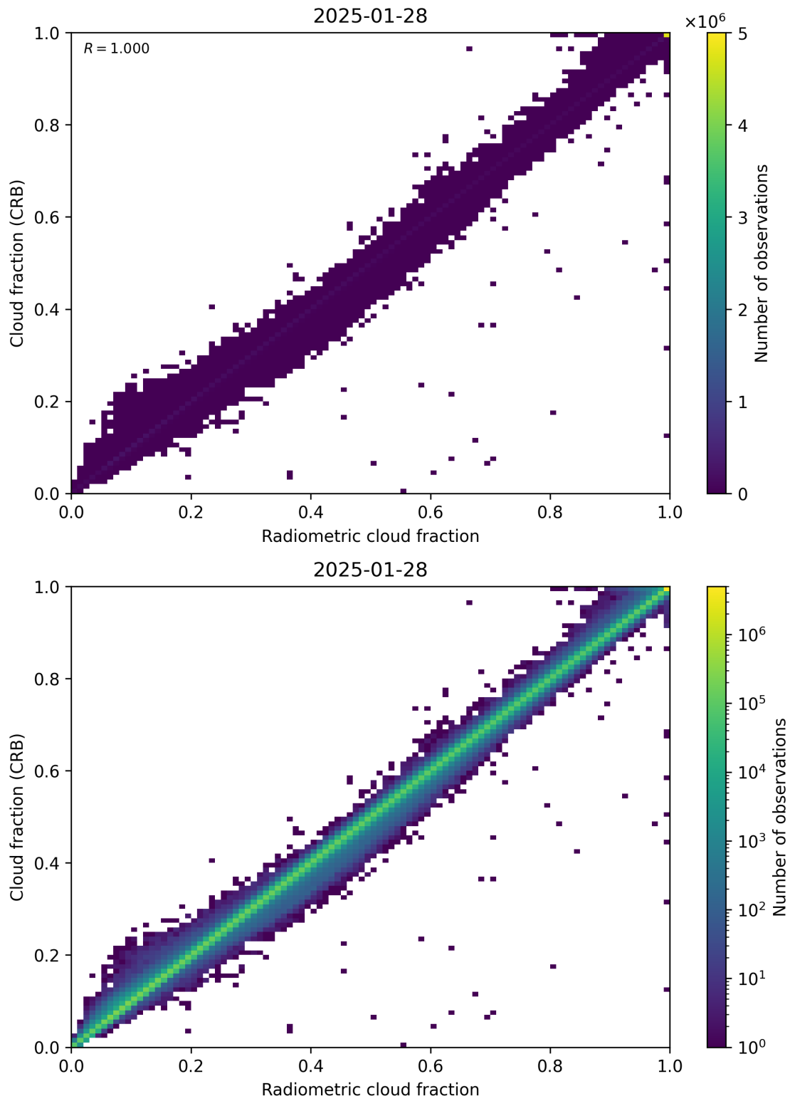
Figure 73: Scatter density plot of “Radiometric cloud fraction” against “Cloud fraction (CRB)” for 2025-01-28 to 2025-01-29.
