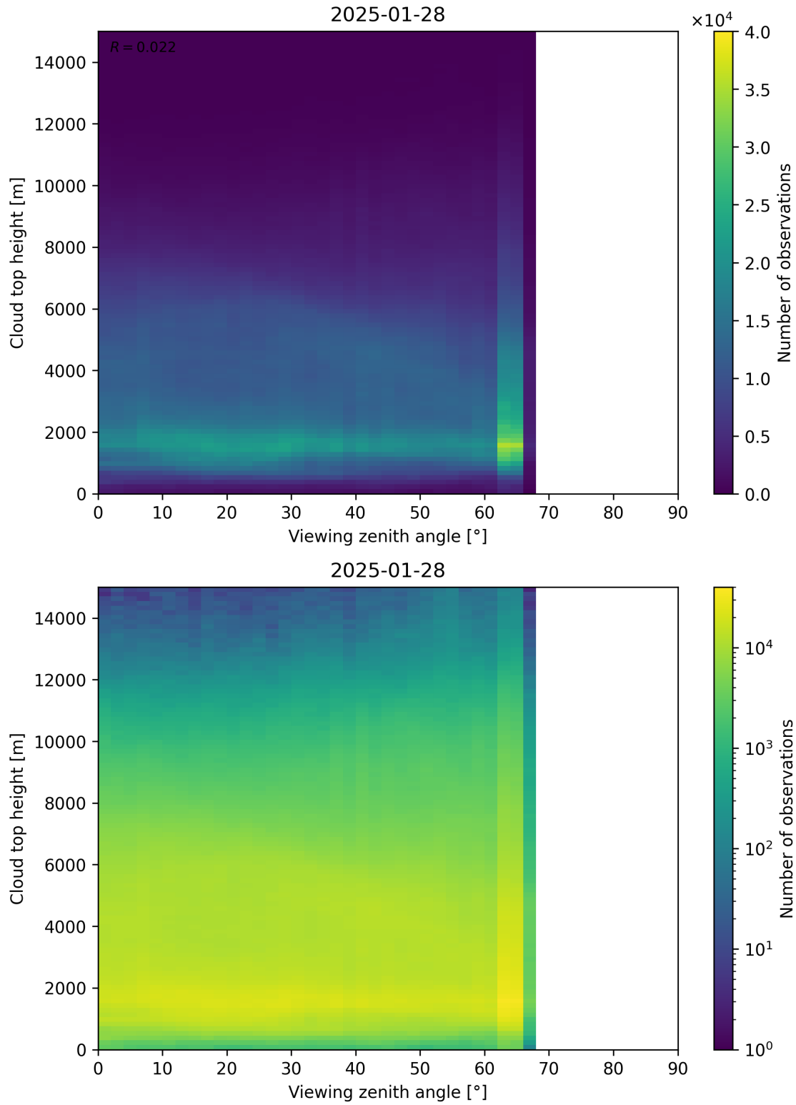
Figure 112: Scatter density plot of “Viewing zenith angle” against “Cloud top height” for 2025-01-28 to 2025-01-29.
