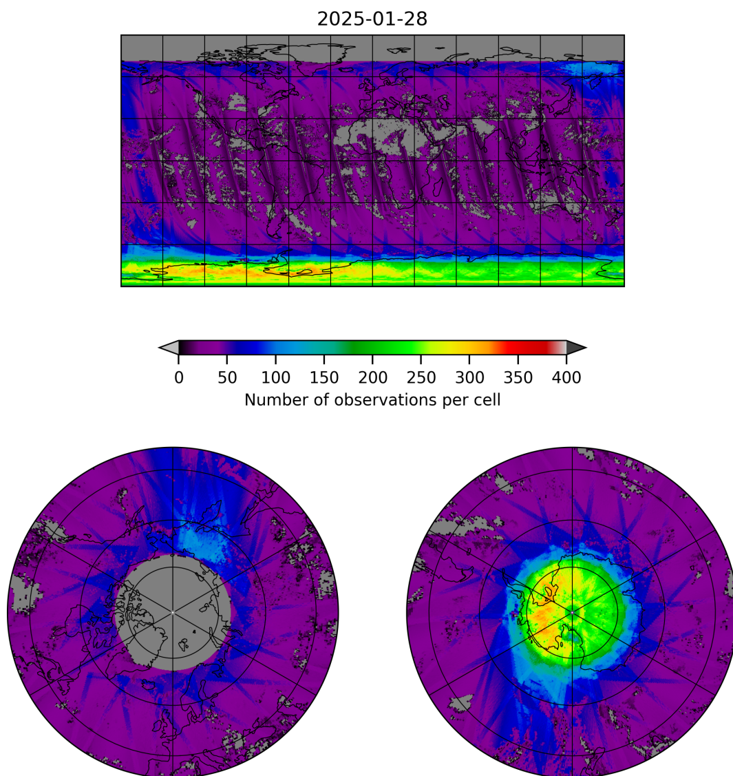
Figure 21: Map of the number of observations for 2025-01-28 to 2025-01-29
