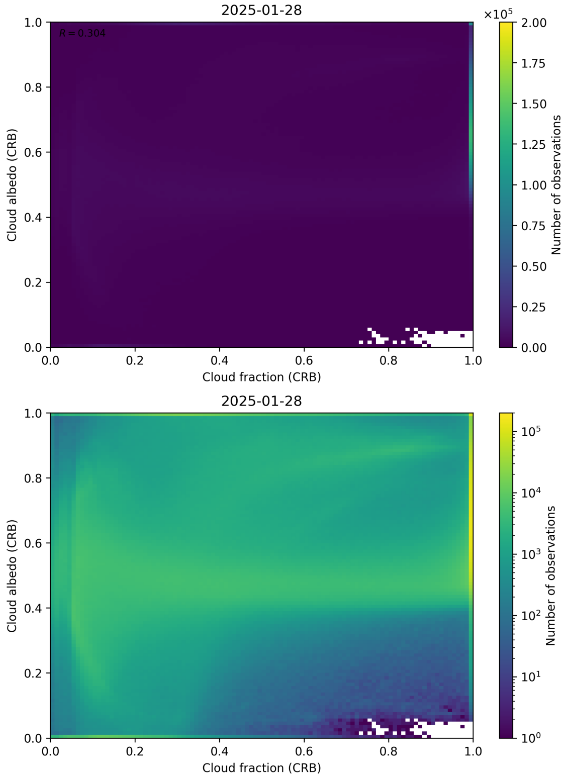
Figure 77: Scatter density plot of “Cloud fraction (CRB)” against “Cloud albedo (CRB)” for 2025-01-28 to 2025-01-29.
