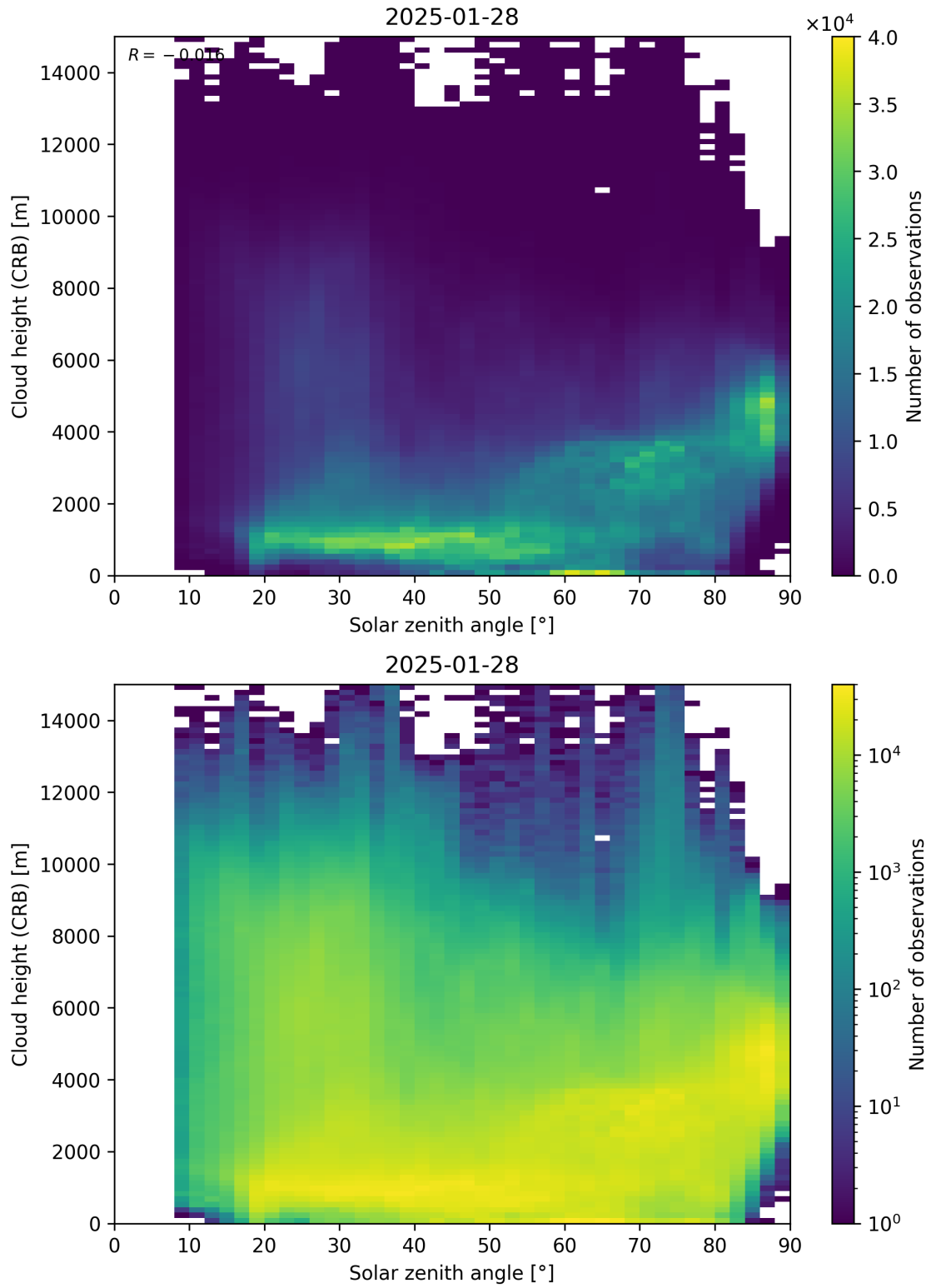
Figure 102: Scatter density plot of “Solar zenith angle” against “Cloud height (CRB)” for 2025-01-28 to 2025-01-29.
