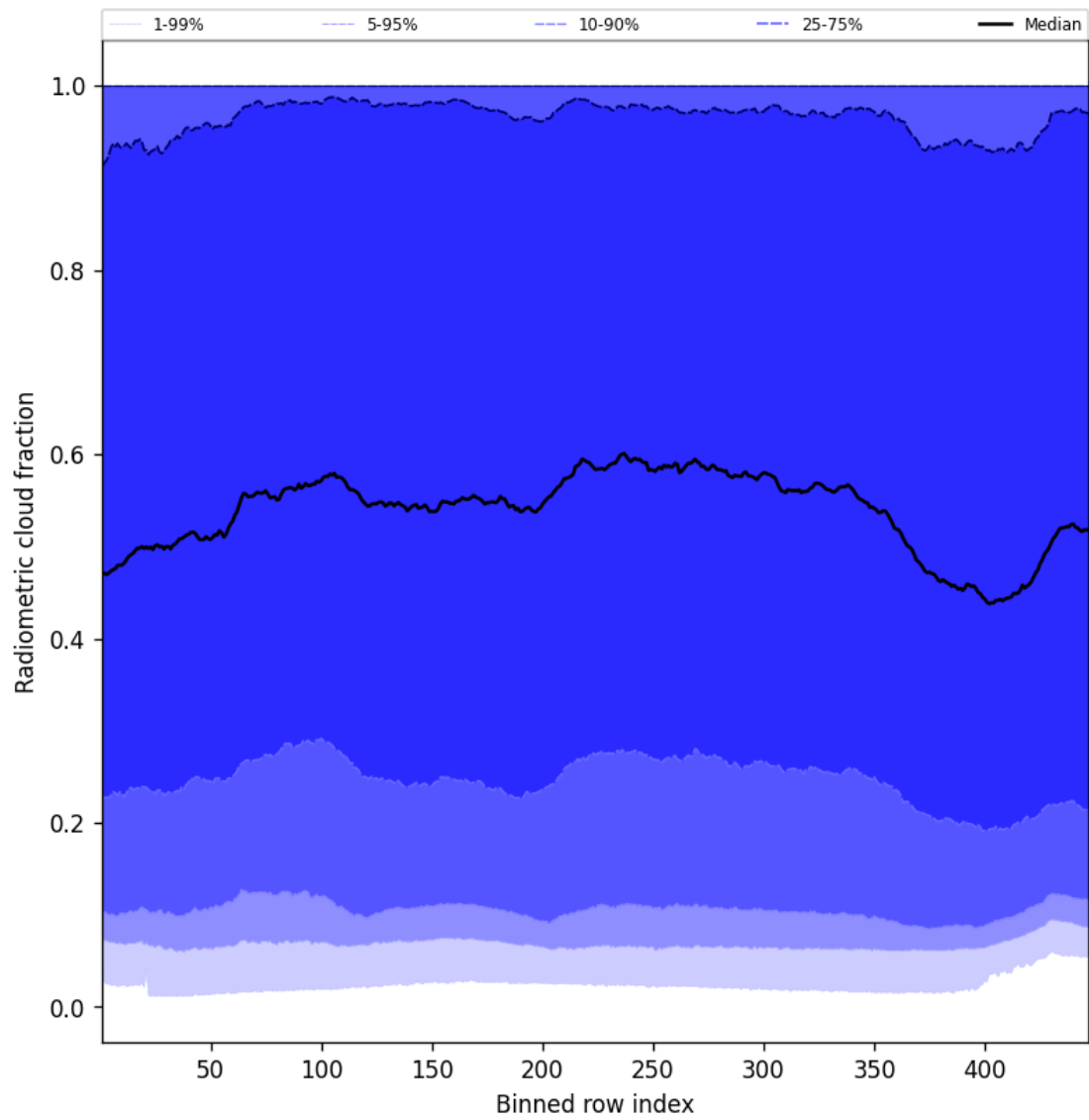
Figure 55: Along track statistics of “Radiometric cloud fraction” for 2025-01-28 to 2025-01-29
