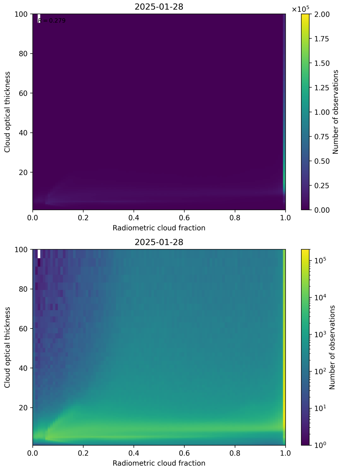
Figure 75: Scatter density plot of “Radiometric cloud fraction” against “Cloud optical thickness” for 2025-01-28 to 2025-01-29.
