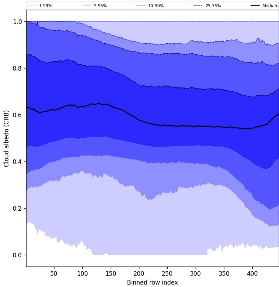
Figure 60: Along track statistics of “Cloud albedo (CRB)” for 2025-01-28 to 2025-01-29
