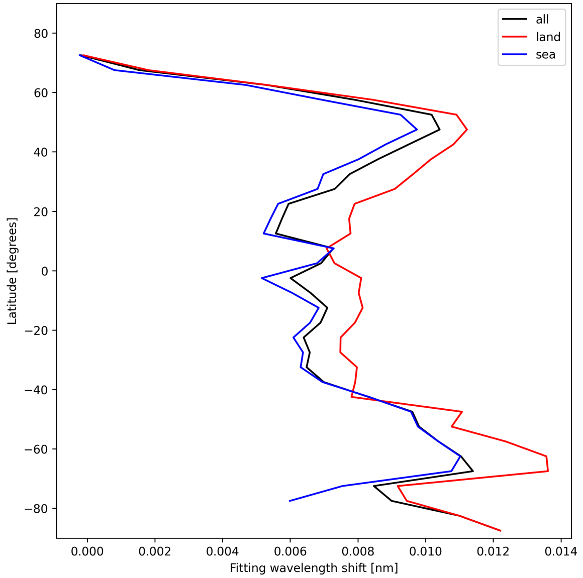
Figure 33: Zonal average of “Fitting wavelength shift” for 2025-01-28 to 2025-01-29.
