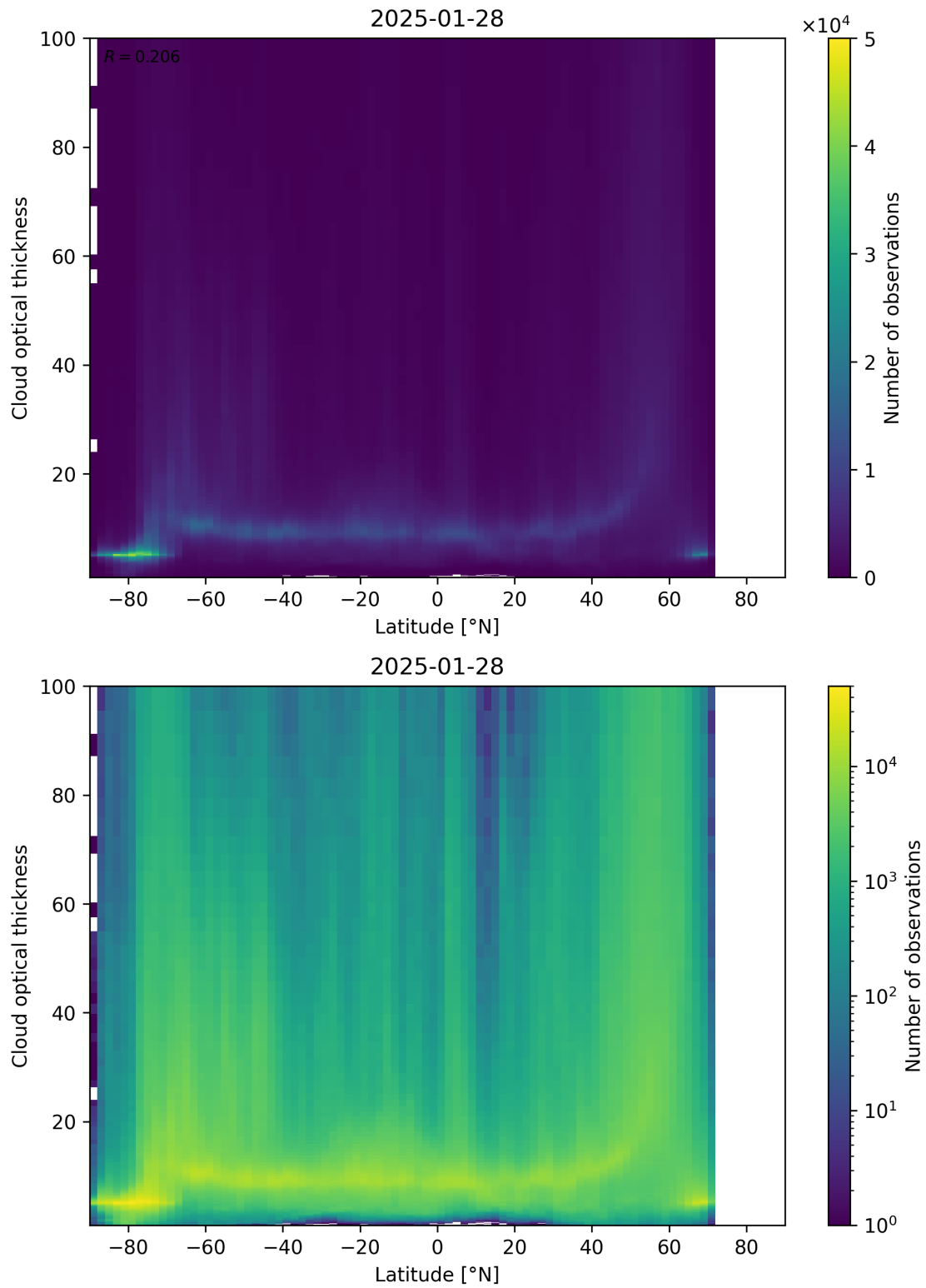
Figure 96: Scatter density plot of “Latitude” against “Cloud optical thickness” for 2025-01-28 to 2025-01-29.
