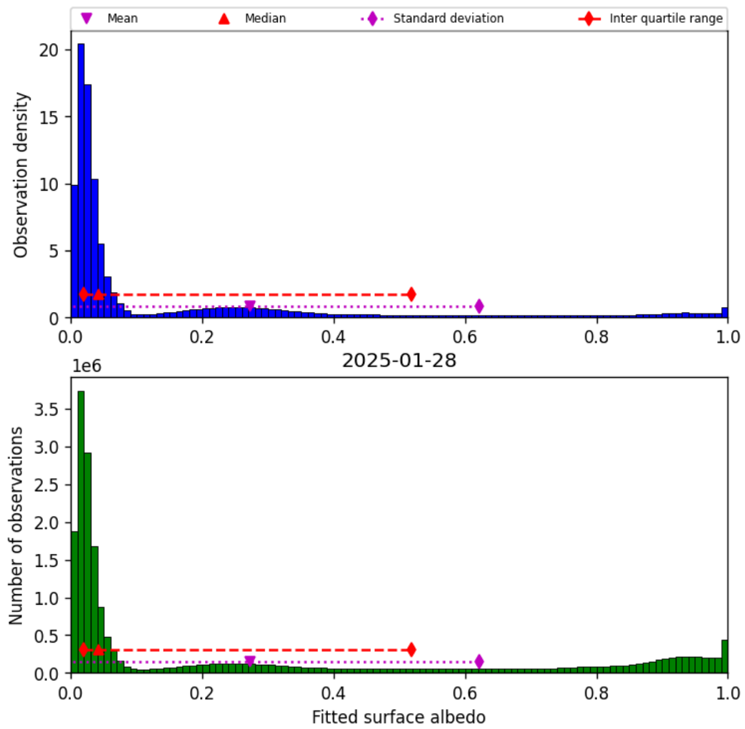
Figure 45: Histogram of “Fitted surface albedo” for 2025-01-28 to 2025-01-29
