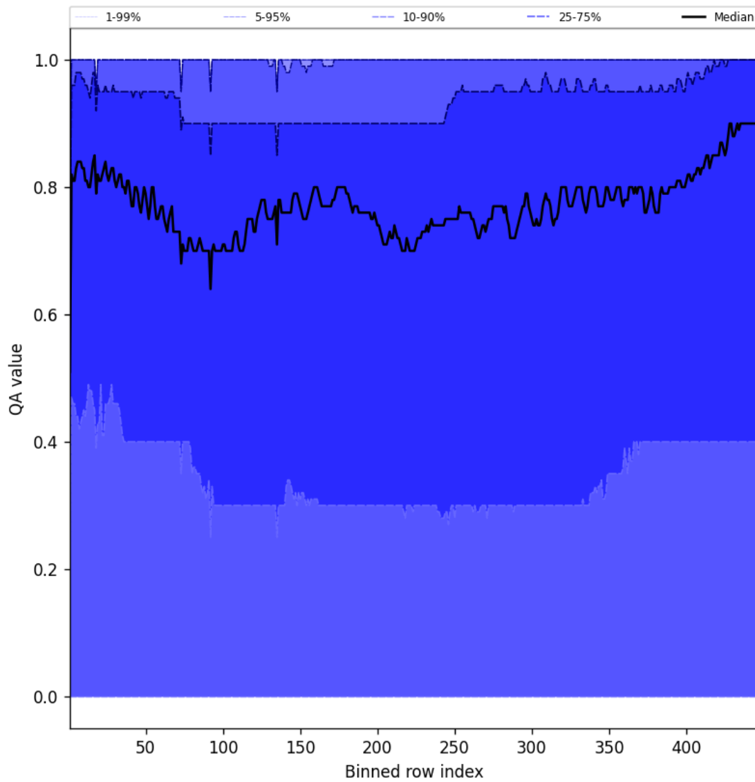
Figure 54: Along track statistics of “QA value” for 2025-01-29 to 2025-01-31
