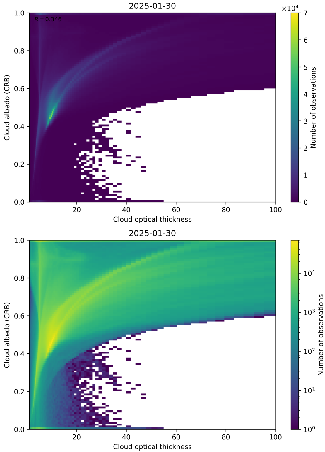
Figure 82: Scatter density plot of “Cloud optical thickness” against “Cloud albedo (CRB)” for 2025-01-29 to 2025-01-31.
