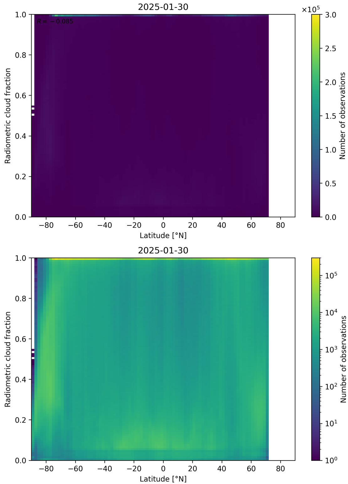
Figure 92: Scatter density plot of “Latitude” against “Radiometric cloud fraction” for 2025-01-29 to 2025-01-31.
