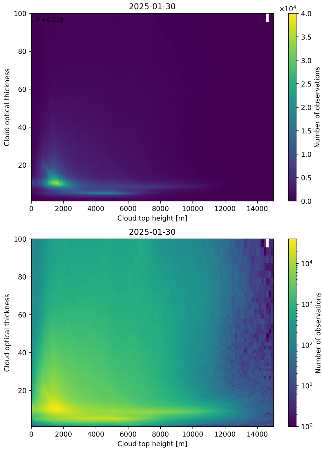
Figure 90: Scatter density plot of “Cloud top height” against “Cloud optical thickness” for 2025-01-29 to 2025-01-31.
