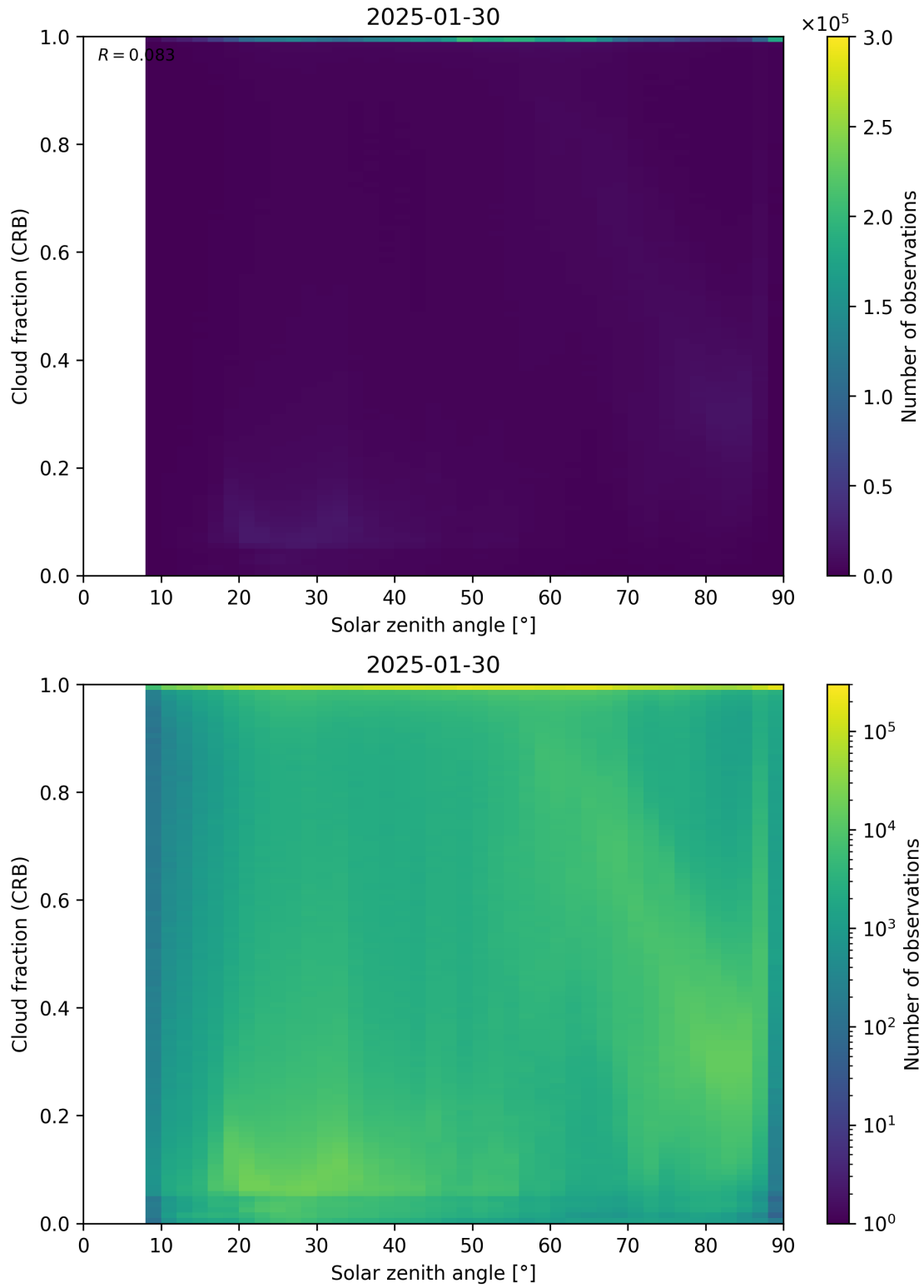
Figure 101: Scatter density plot of “Solar zenith angle” against “Cloud fraction (CRB)” for 2025-01-29 to 2025-01-31.
