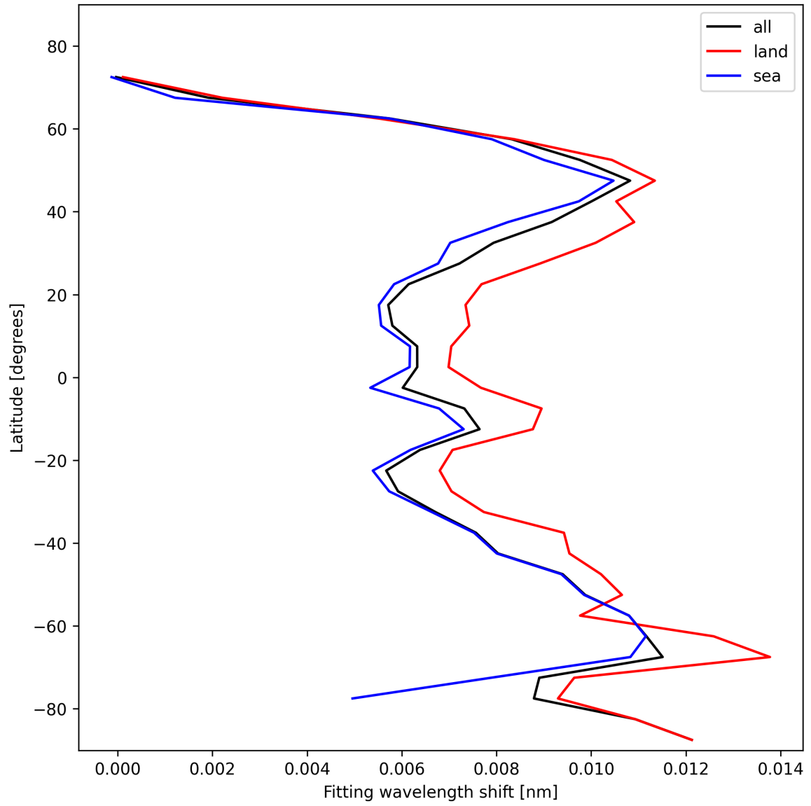
Figure 33: Zonal average of “Fitting wavelength shift” for 2025-01-29 to 2025-01-31.
