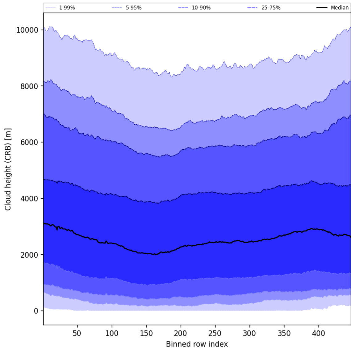
Figure 59: Along track statistics of “Cloud height (CRB)” for 2025-01-29 to 2025-01-31
