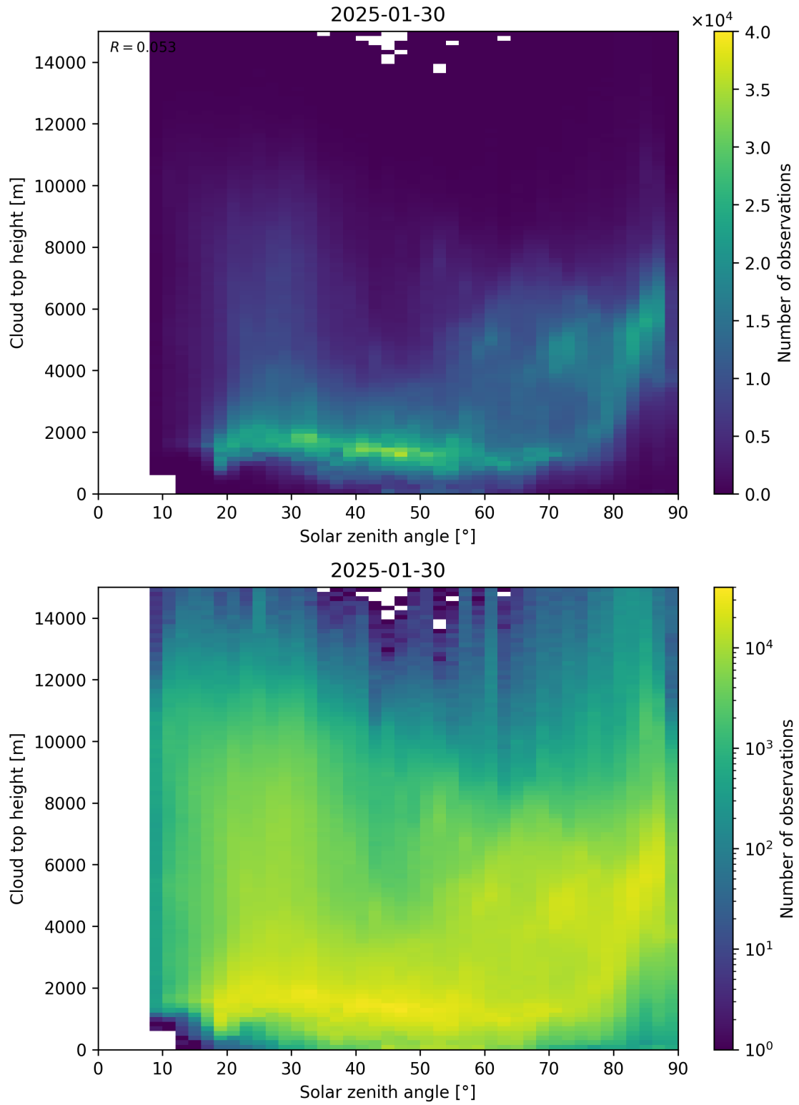
Figure 104: Scatter density plot of “Solar zenith angle” against “Cloud top height” for 2025-01-29 to 2025-01-31.
