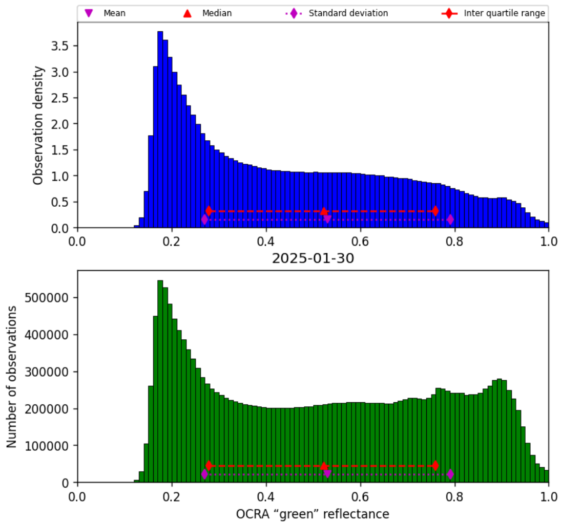
Figure 52: Histogram of “OCRA “green” reflectance” for 2025-01-29 to 2025-01-31
