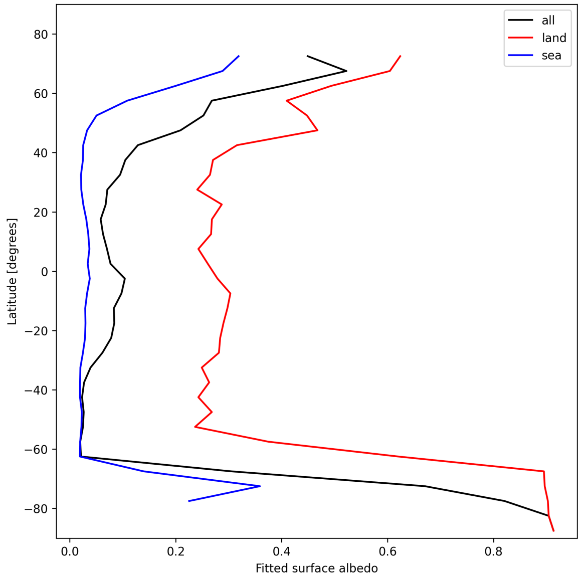
Figure 29: Zonal average of “Fitted surface albedo” for 2025-01-29 to 2025-01-31.
