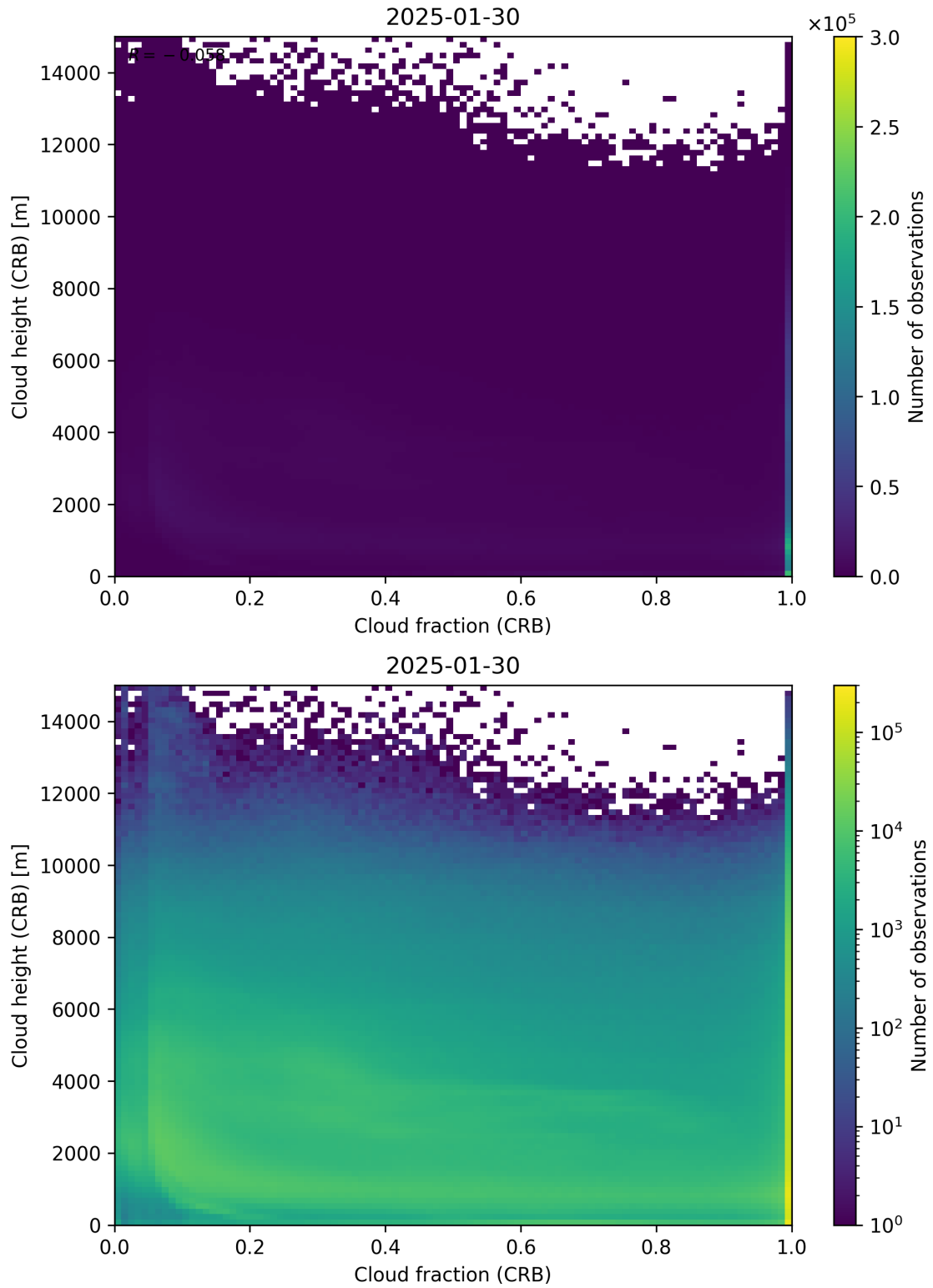
Figure 79: Scatter density plot of “Cloud fraction (CRB)” against “Cloud height (CRB)” for 2025-01-29 to 2025-01-31.
