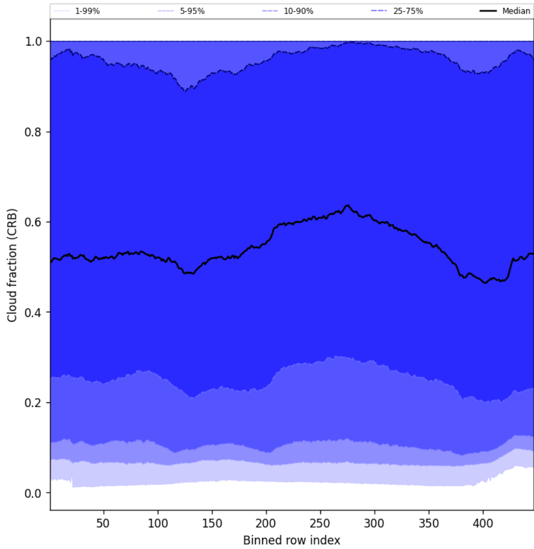
Figure 58: Along track statistics of “Cloud fraction (CRB)” for 2025-01-29 to 2025-01-31
