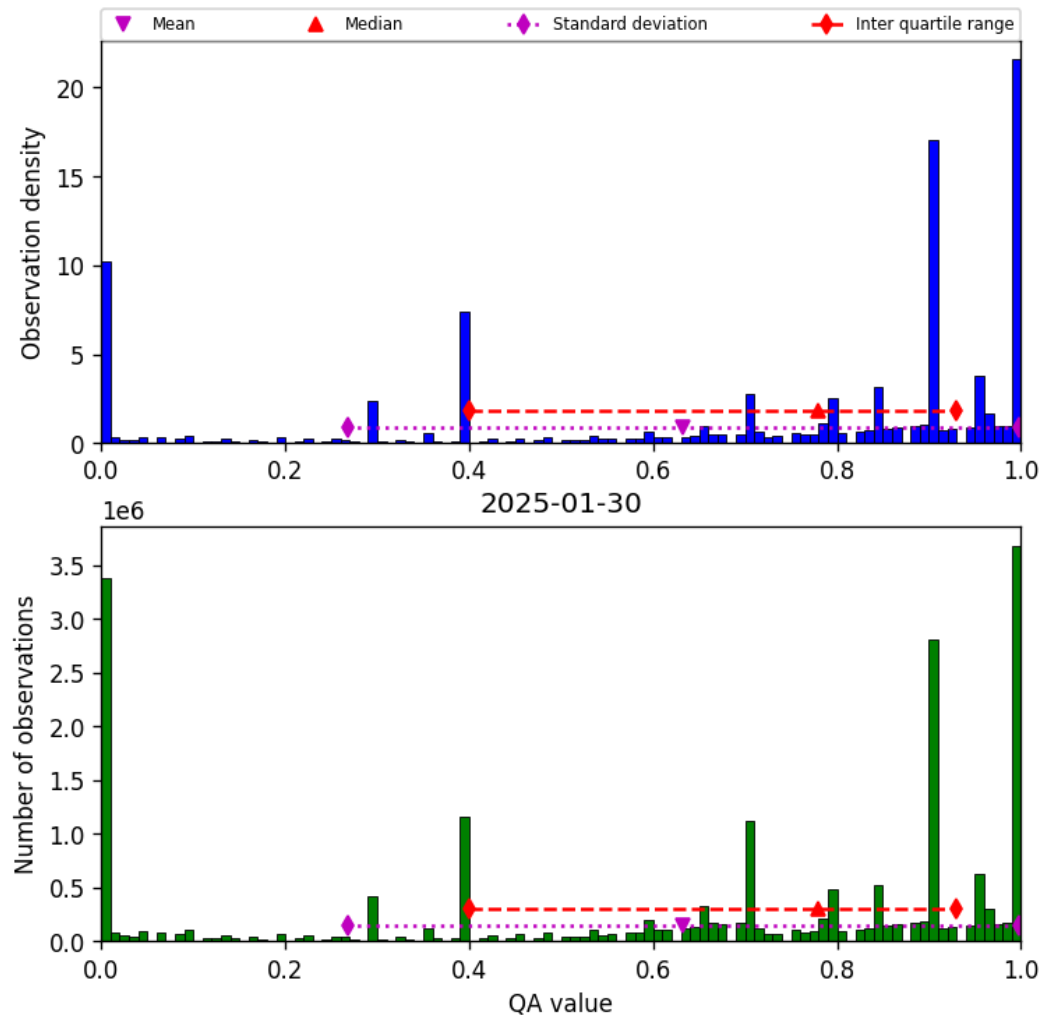
Figure 38: Histogram of “QA value” for 2025-01-29 to 2025-01-31
