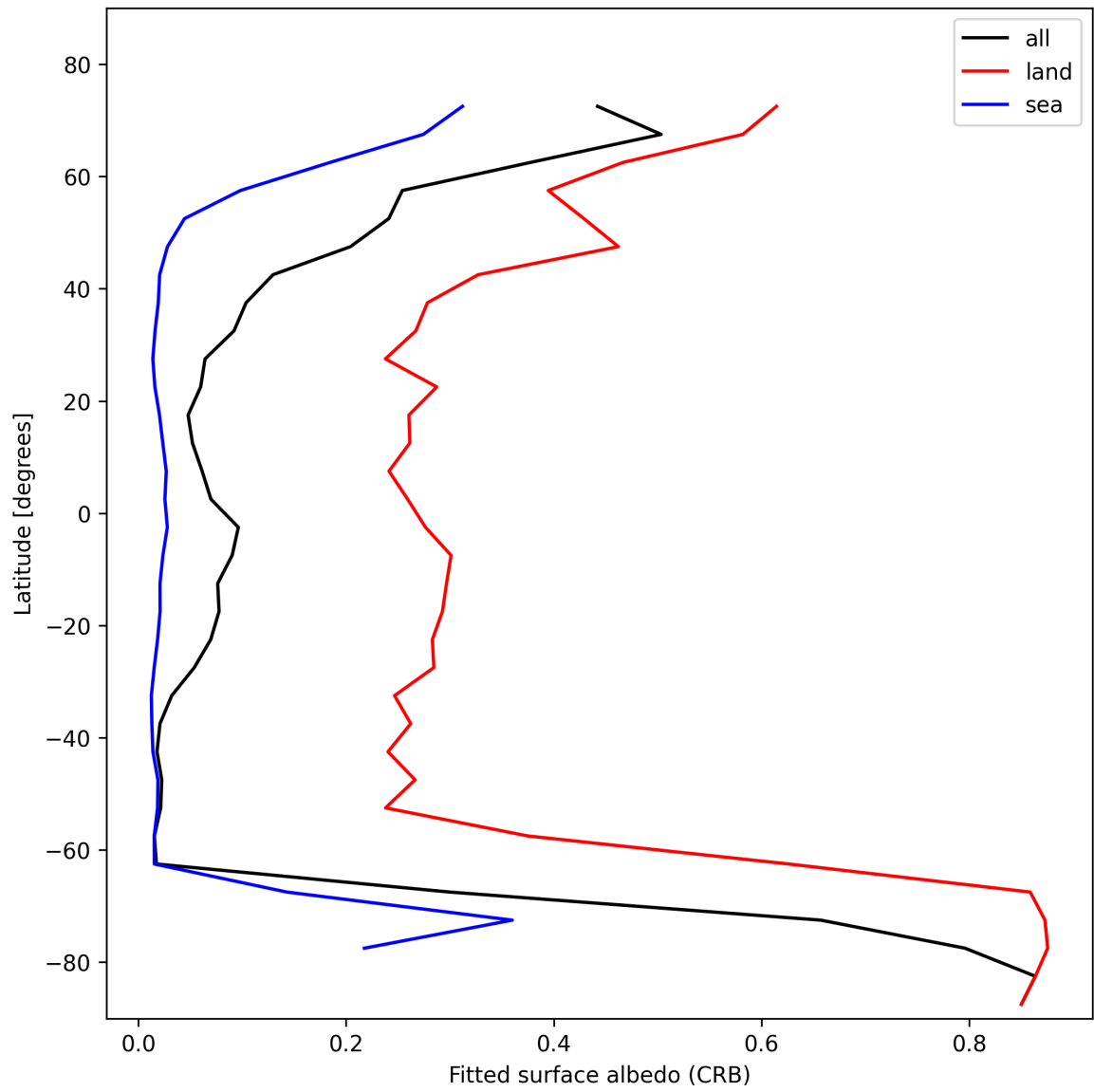
Figure 30: Zonal average of “Fitted surface albedo (CRB)” for 2025-01-29 to 2025-01-31.
