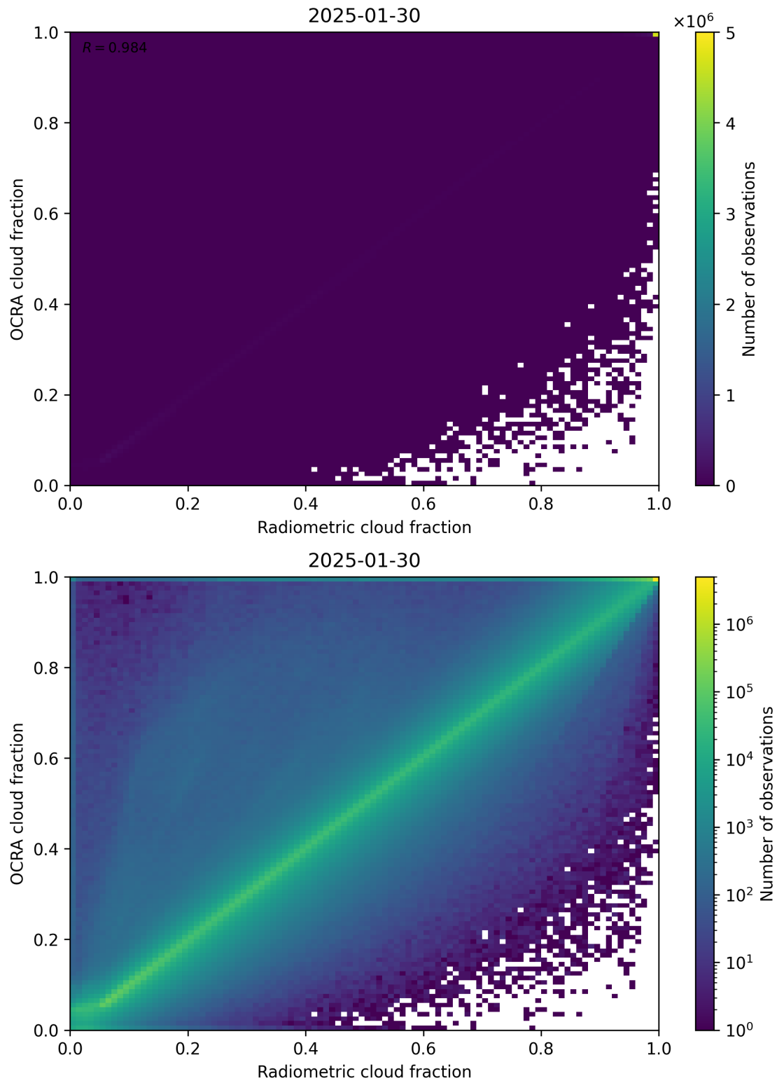
Figure 72: Scatter density plot of “Radiometric cloud fraction” against “OCRA cloud fraction” for 2025-01-29 to 2025-01-31.
