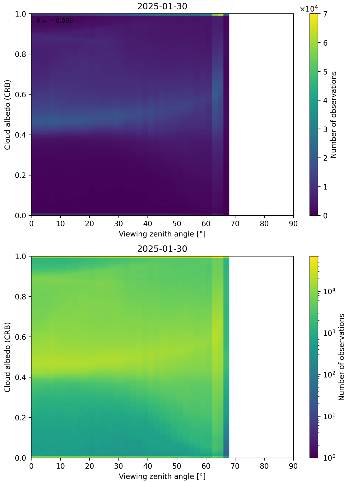
Figure 106: Scatter density plot of “Viewing zenith angle” against “Cloud albedo (CRB)” for 2025-01-29 to 2025-01-31.
