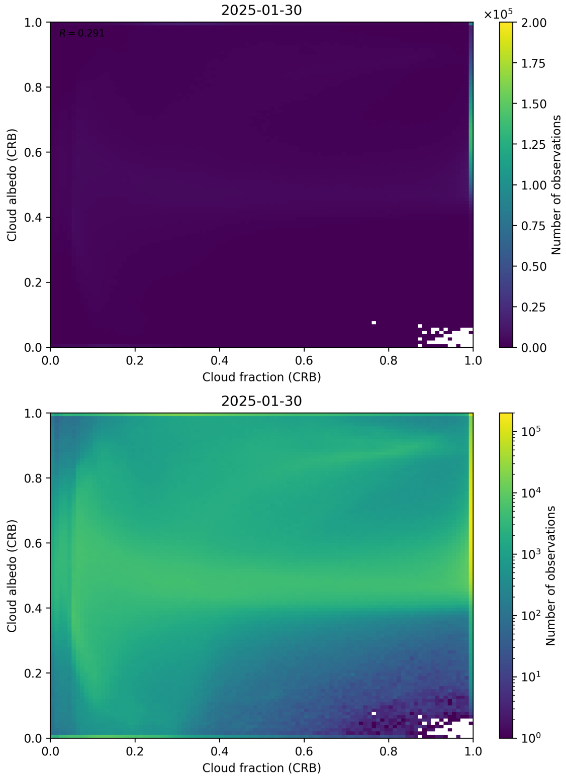
Figure 77: Scatter density plot of “Cloud fraction (CRB)” against “Cloud albedo (CRB)” for 2025-01-29 to 2025-01-31.
