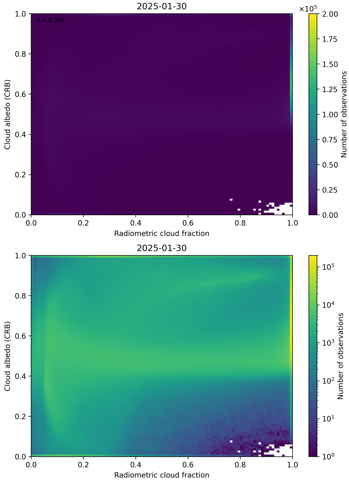
Figure 71: Scatter density plot of “Radiometric cloud fraction” against “Cloud albedo (CRB)” for 2025-01-29 to 2025-01-31.
