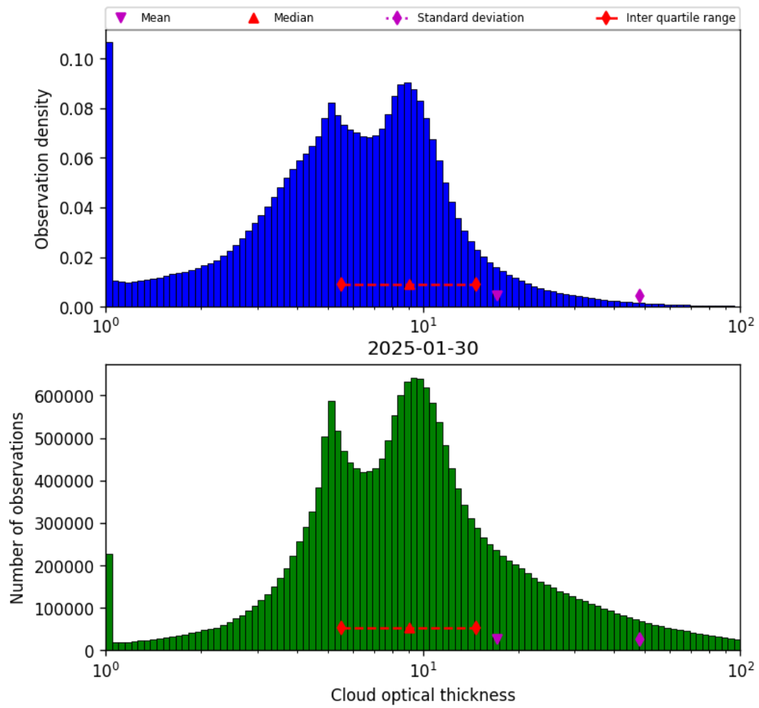
Figure 41: Histogram of “Cloud optical thickness” for 2025-01-29 to 2025-01-31
