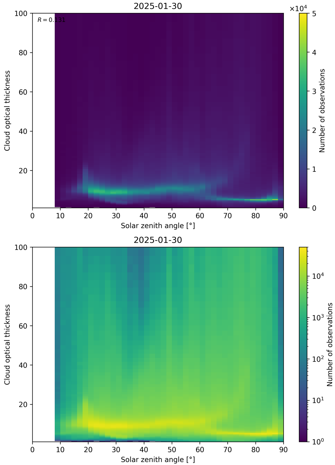
Figure 103: Scatter density plot of “Solar zenith angle” against “Cloud optical thickness” for 2025-01-29 to 2025-01-31.
