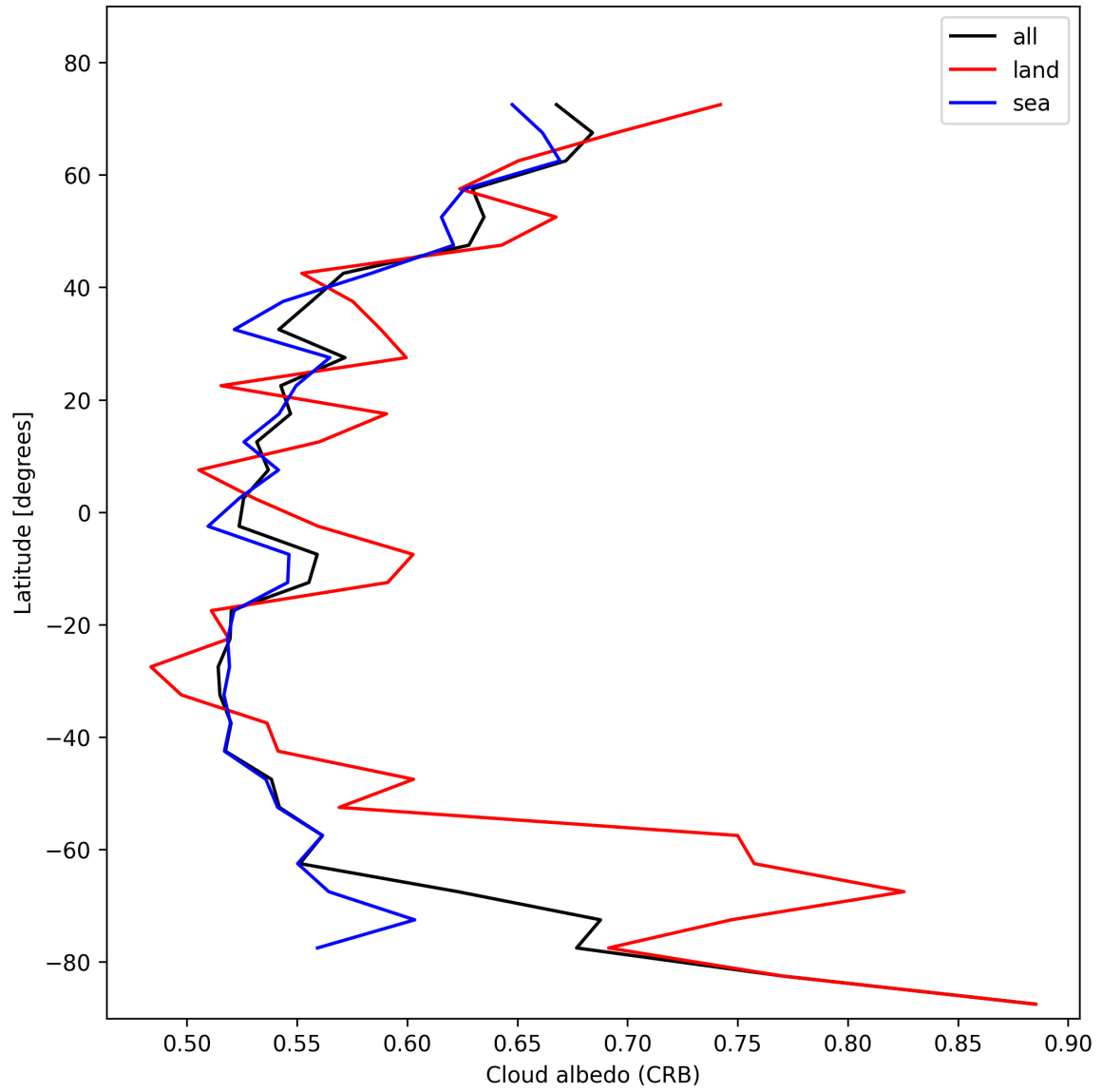
Figure 28: Zonal average of “Cloud albedo (CRB)” for 2025-01-29 to 2025-01-31.
