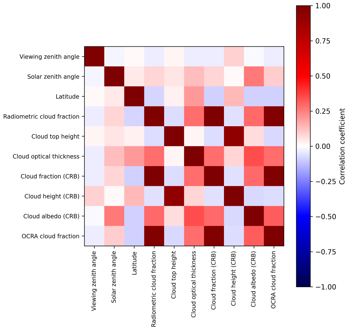
Figure 2: Map of correlation matrix for 2025-01-29 to 2025-01-31.
