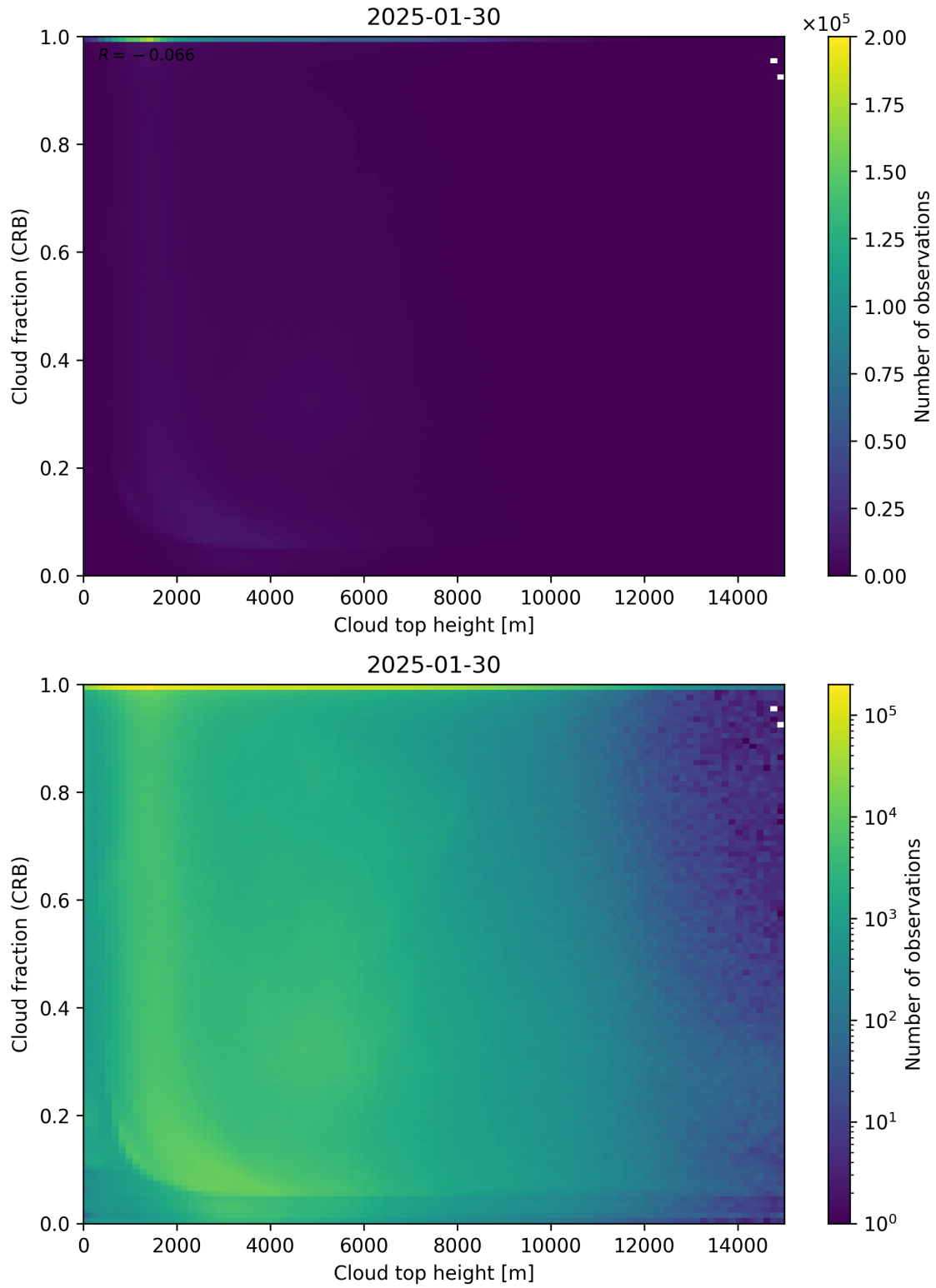
Figure 88: Scatter density plot of “Cloud top height” against “Cloud fraction (CRB)” for 2025-01-29 to 2025-01-31.
