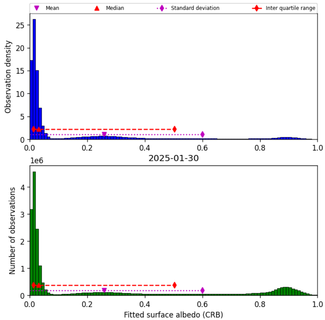
Figure 46: Histogram of “Fitted surface albedo (CRB)” for 2025-01-29 to 2025-01-31
