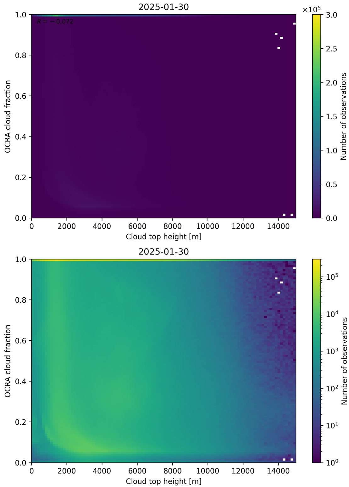
Figure 87: Scatter density plot of “Cloud top height” against “OCRA cloud fraction” for 2025-01-29 to 2025-01-31.
