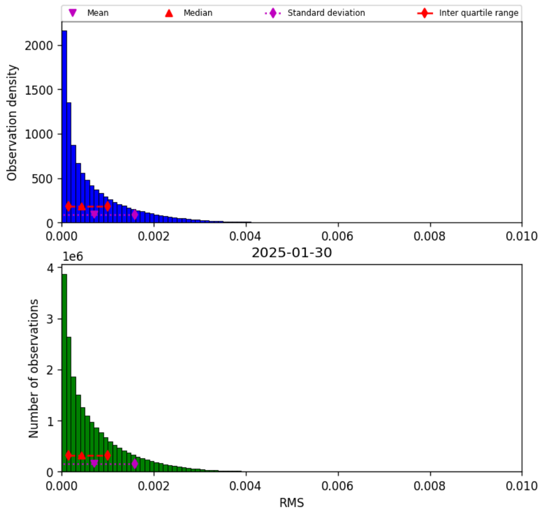
Figure 47: Histogram of “RMS” for 2025-01-29 to 2025-01-31
