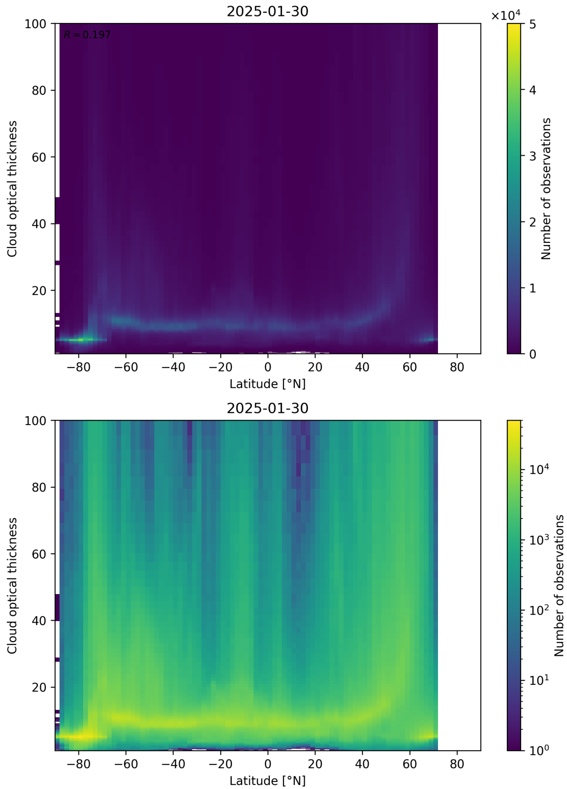
Figure 96: Scatter density plot of “Latitude” against “Cloud optical thickness” for 2025-01-29 to 2025-01-31.
