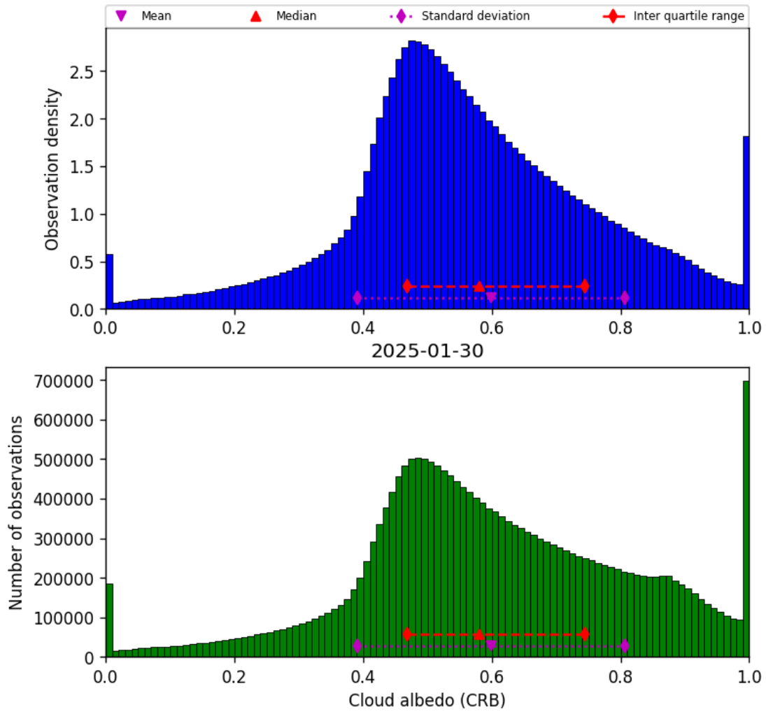
Figure 44: Histogram of “Cloud albedo (CRB)” for 2025-01-29 to 2025-01-31
