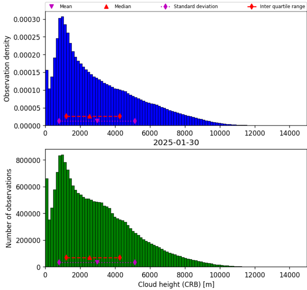
Figure 43: Histogram of “Cloud height (CRB)” for 2025-01-29 to 2025-01-31
