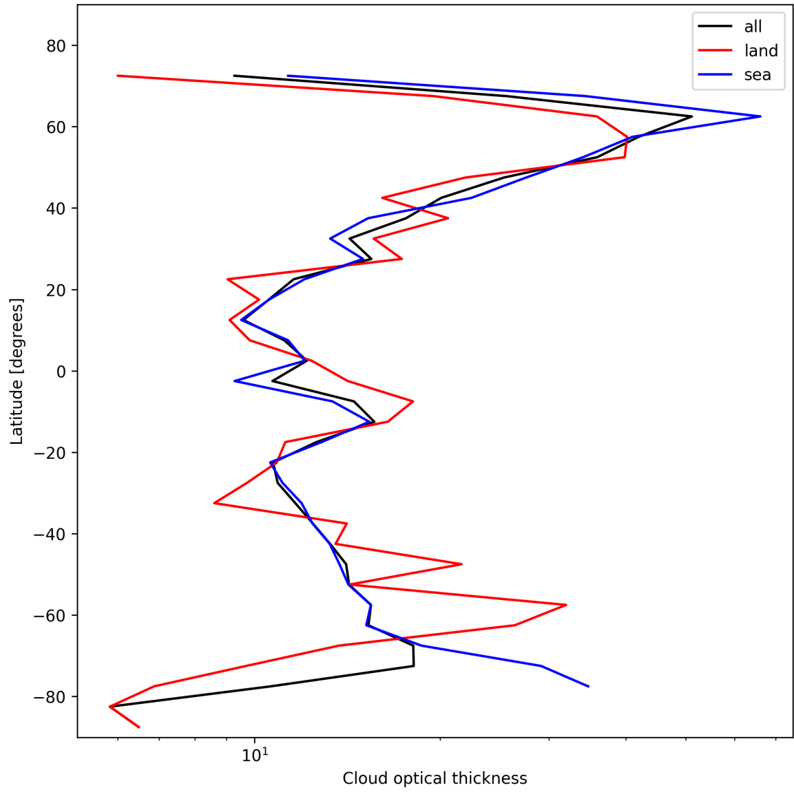
Figure 25: Zonal average of “Cloud optical thickness” for 2025-01-29 to 2025-01-31.
