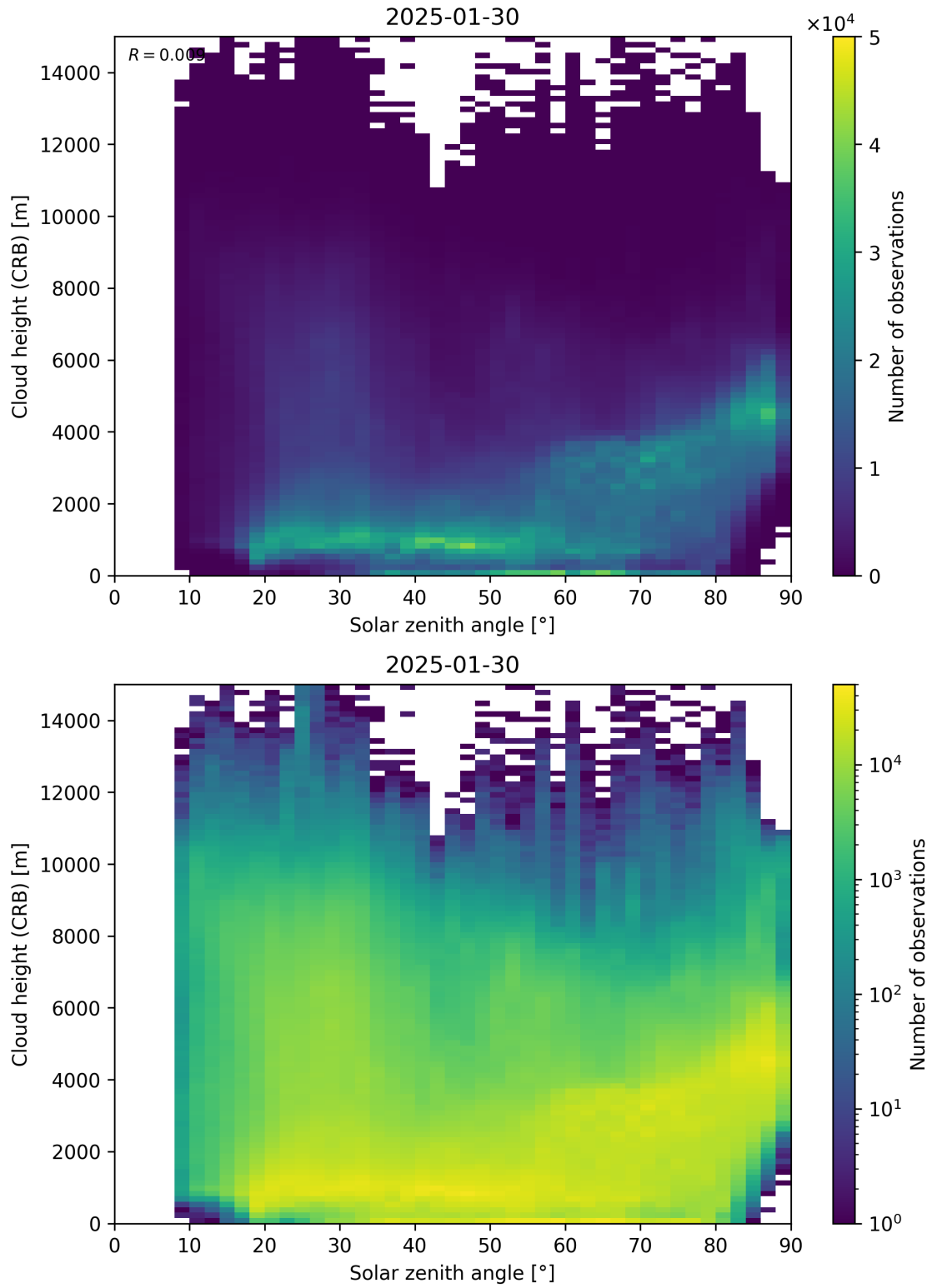
Figure 102: Scatter density plot of “Solar zenith angle” against “Cloud height (CRB)” for 2025-01-29 to 2025-01-31.
