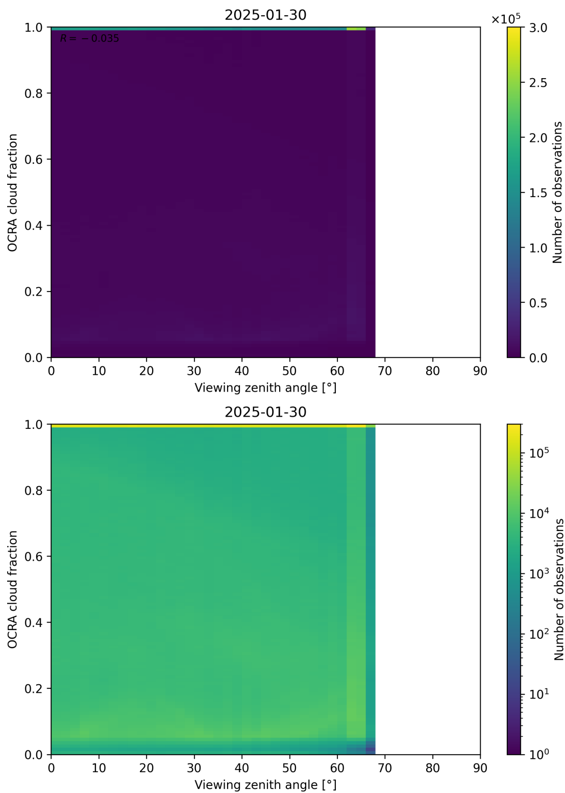
Figure 108: Scatter density plot of “Viewing zenith angle” against “OCRA cloud fraction” for 2025-01-29 to 2025-01-31.
