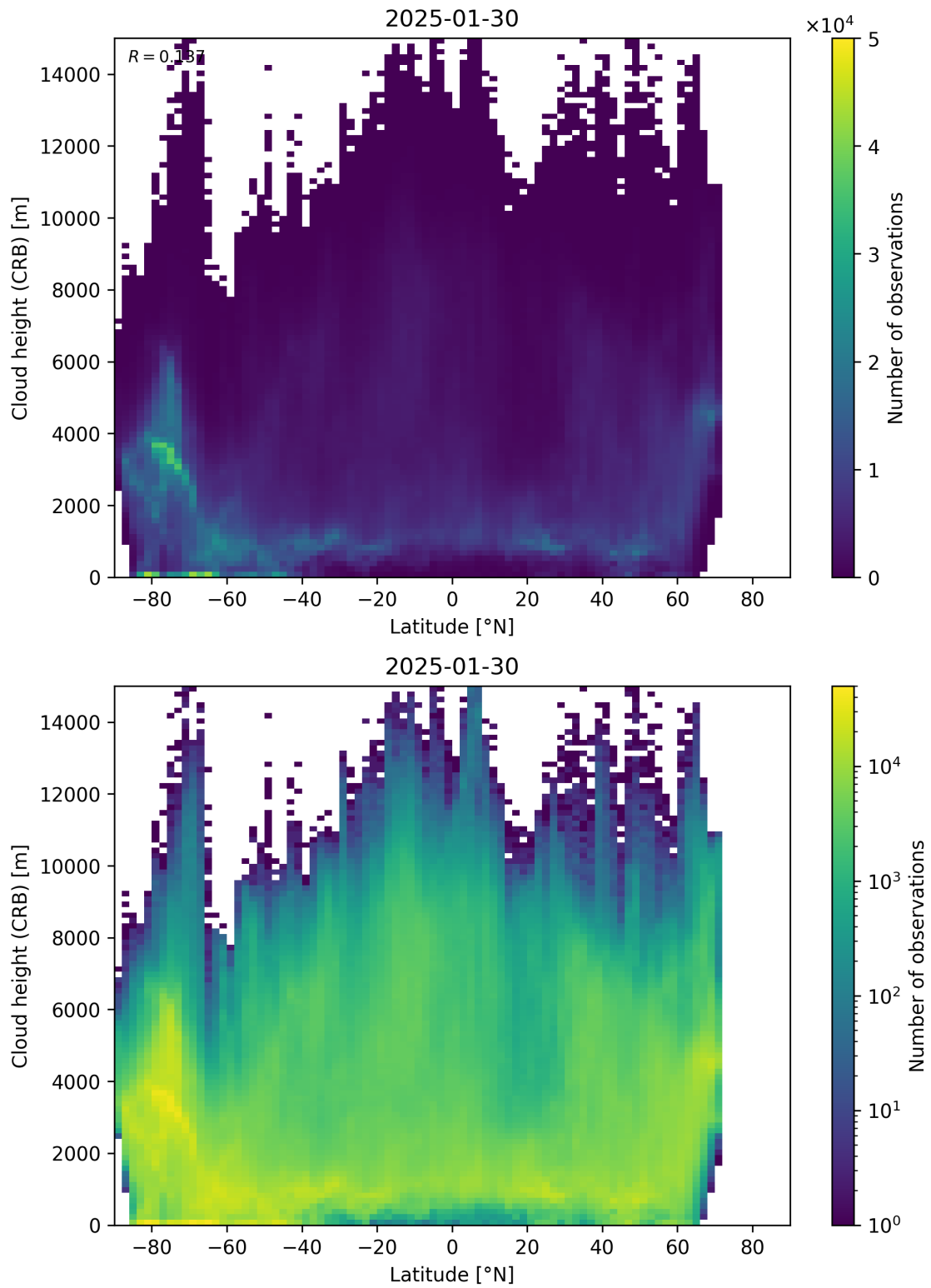
Figure 95: Scatter density plot of “Latitude” against “Cloud height (CRB)” for 2025-01-29 to 2025-01-31.
