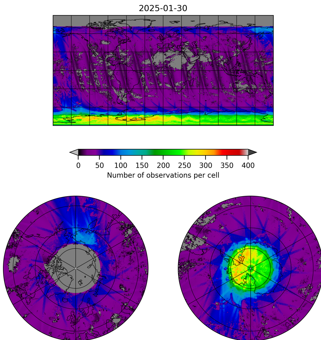
Figure 21: Map of the number of observations for 2025-01-29 to 2025-01-31
