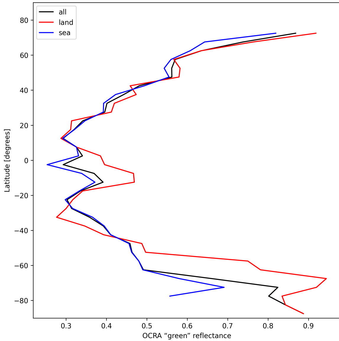
Figure 36: Zonal average of “OCRA “green” reflectance” for 2025-01-29 to 2025-01-31.
