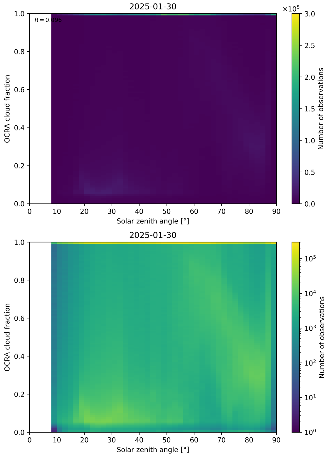
Figure 100: Scatter density plot of “Solar zenith angle” against “OCRA cloud fraction” for 2025-01-29 to 2025-01-31.
