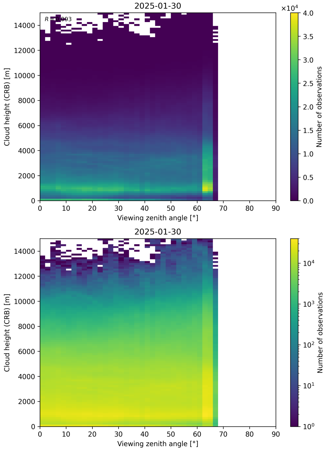
Figure 110: Scatter density plot of “Viewing zenith angle” against “Cloud height (CRB)” for 2025-01-29 to 2025-01-31.
