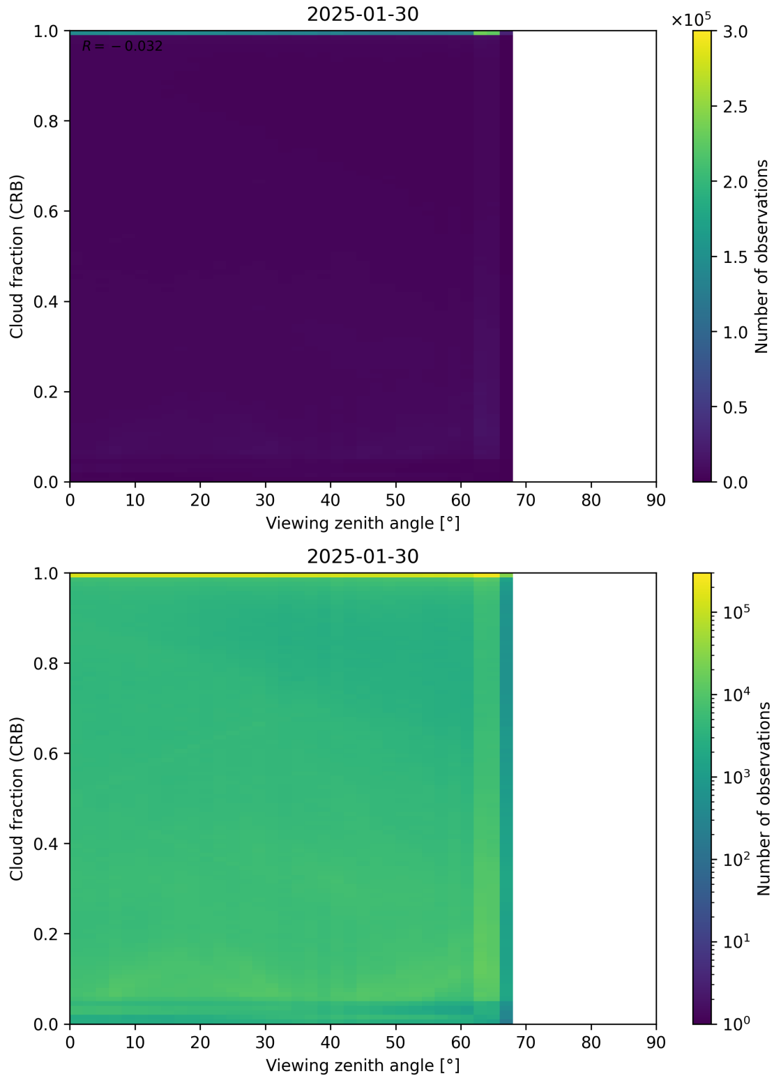
Figure 109: Scatter density plot of “Viewing zenith angle” against “Cloud fraction (CRB)” for 2025-01-29 to 2025-01-31.
