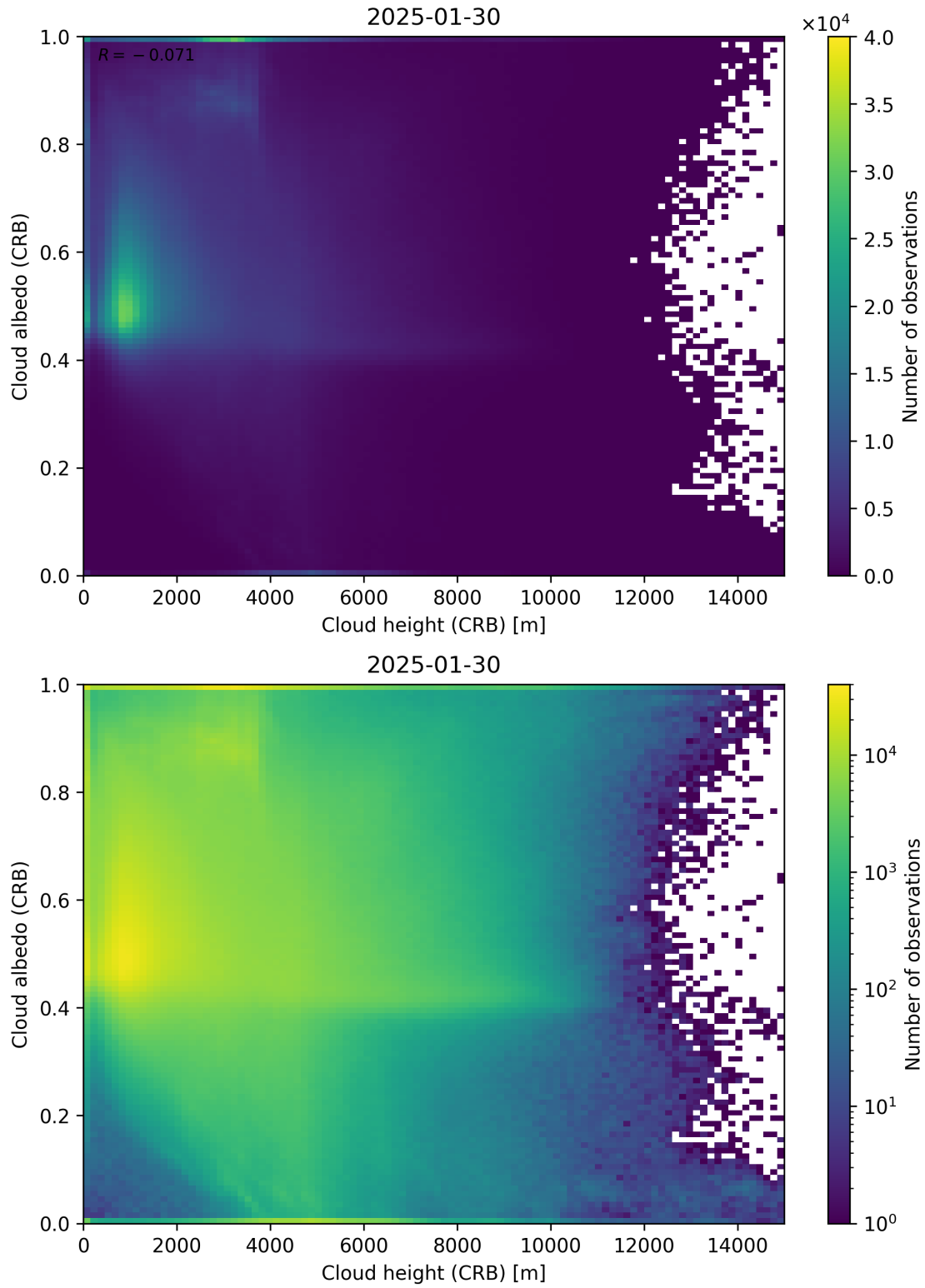
Figure 80: Scatter density plot of “Cloud height (CRB)” against “Cloud albedo (CRB)” for 2025-01-29 to 2025-01-31.
