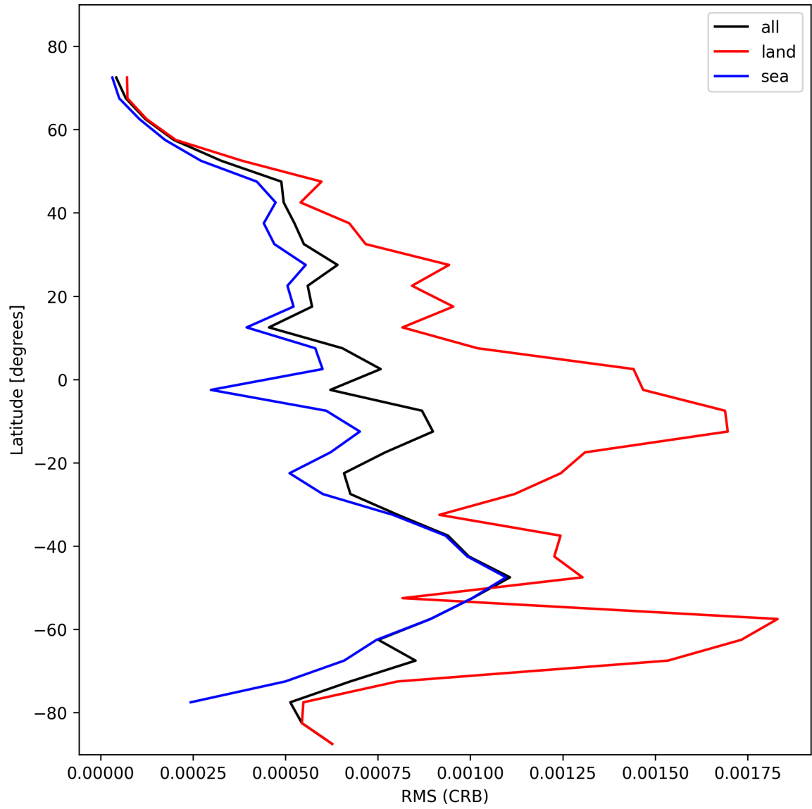
Figure 32: Zonal average of “RMS (CRB)” for 2025-01-29 to 2025-01-31.
