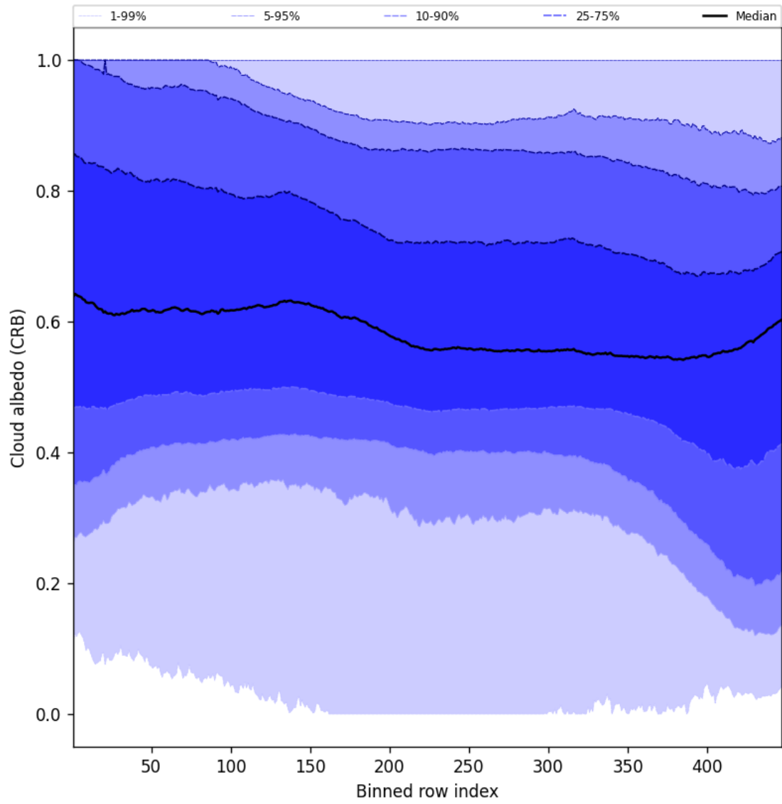
Figure 60: Along track statistics of “Cloud albedo (CRB)” for 2025-01-29 to 2025-01-31
