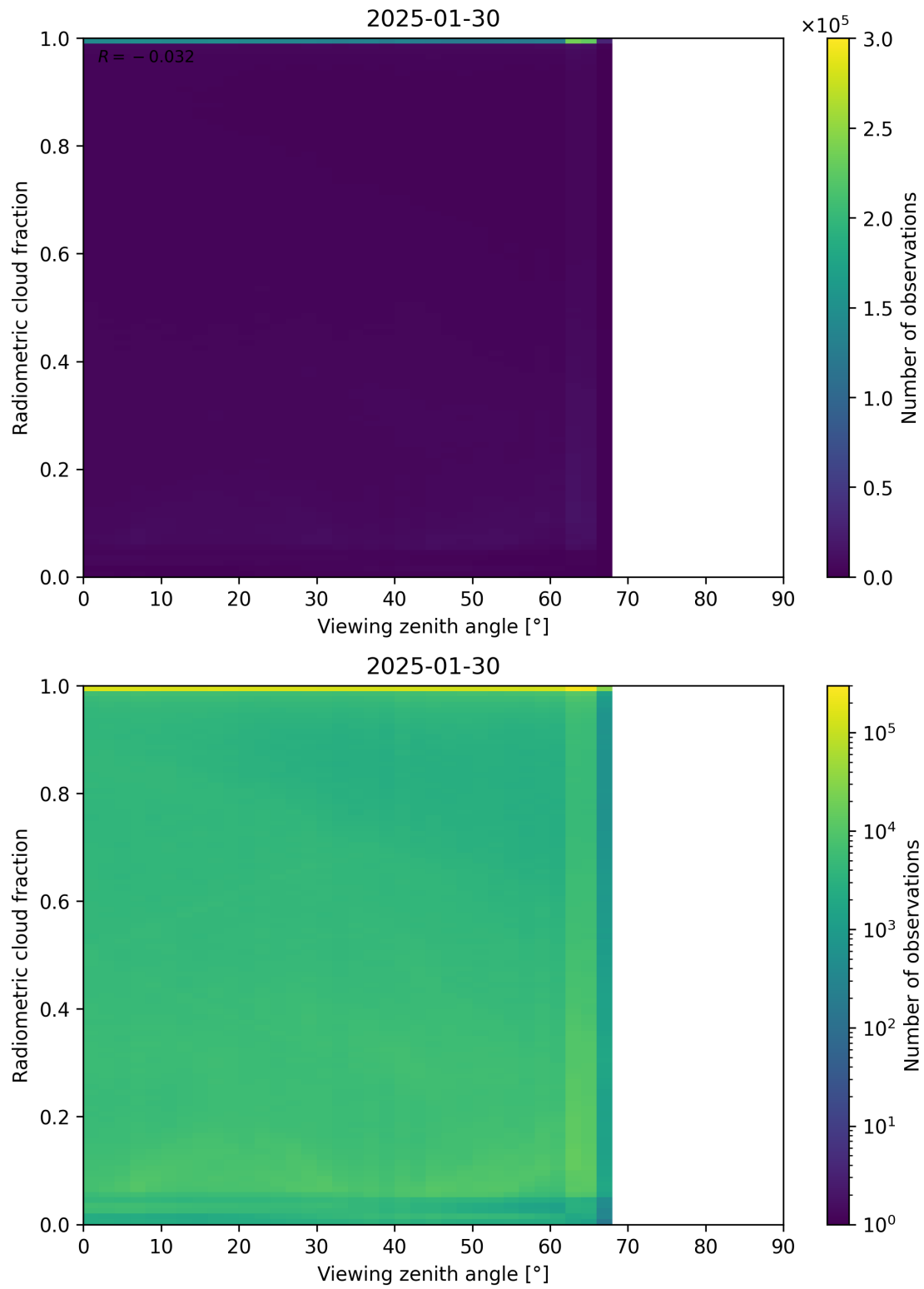
Figure 107: Scatter density plot of “Viewing zenith angle” against “Radiometric cloud fraction” for 2025-01-29 to 2025-01-31.
