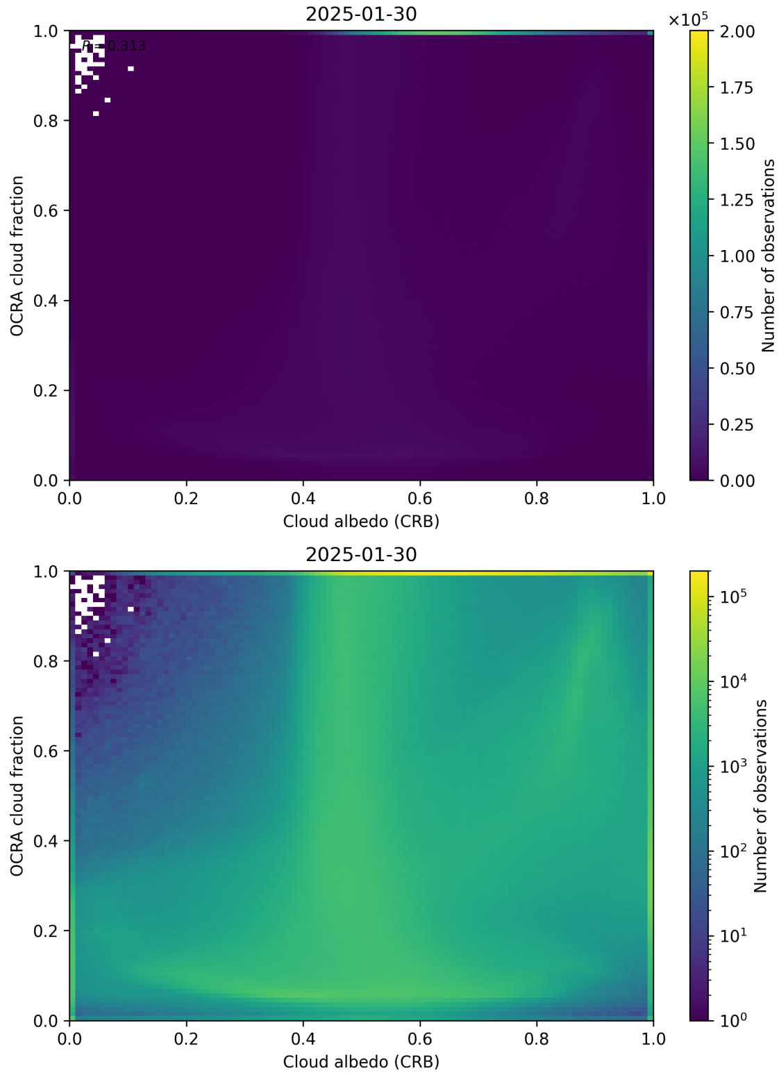
Figure 70: Scatter density plot of “Cloud albedo (CRB)” against “OCRA cloud fraction” for 2025-01-29 to 2025-01-31.
