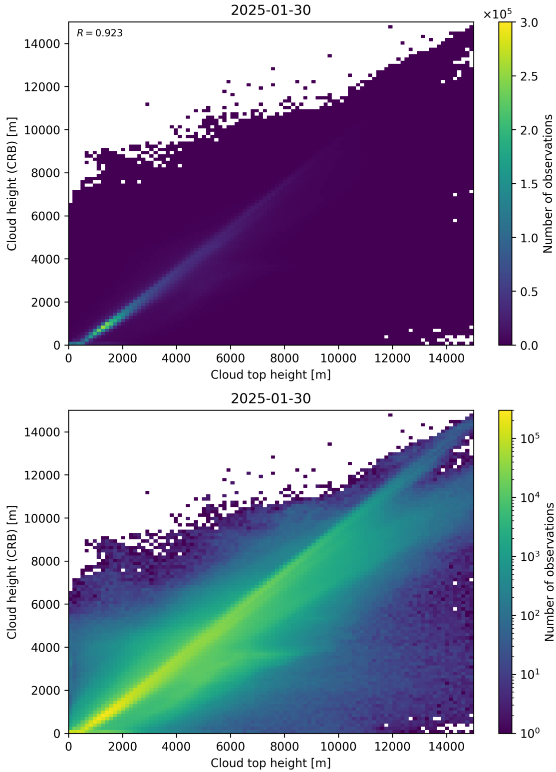
Figure 89: Scatter density plot of “Cloud top height” against “Cloud height (CRB)” for 2025-01-29 to 2025-01-31.
