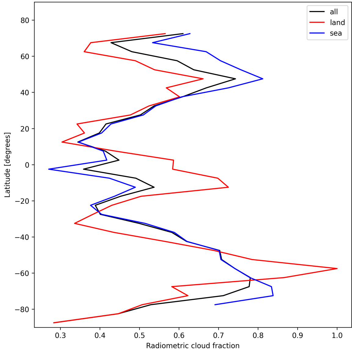
Figure 23: Zonal average of “Radiometric cloud fraction” for 2025-01-29 to 2025-01-31.
