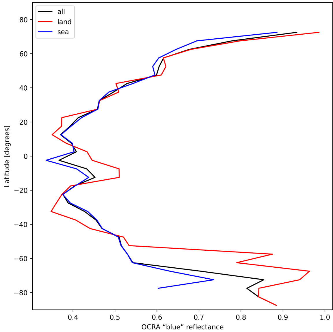
Figure 35: Zonal average of “OCRA “blue” reflectance” for 2025-01-29 to 2025-01-31.
