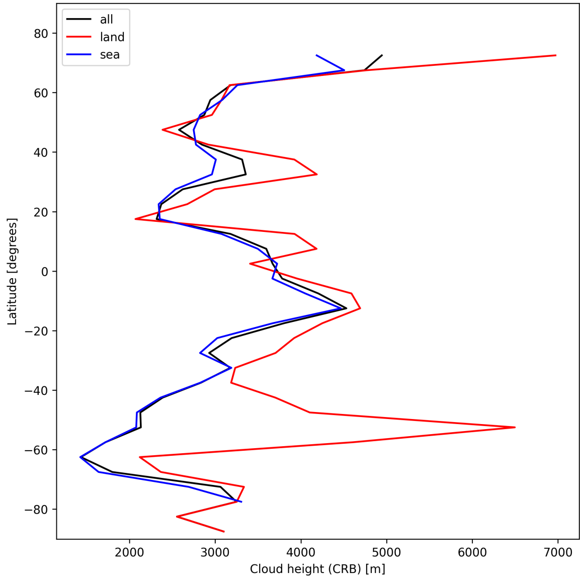
Figure 27: Zonal average of “Cloud height (CRB)” for 2025-01-29 to 2025-01-31.
