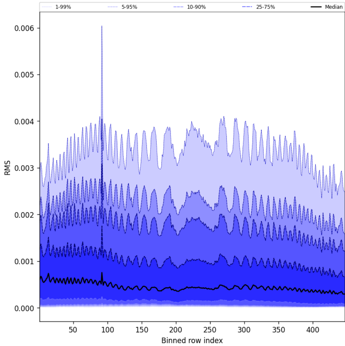
Figure 63: Along track statistics of “RMS” for 2025-01-29 to 2025-01-31
