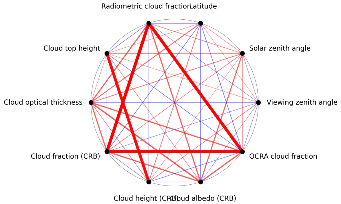
Figure 1: Map of correlation graph for 2025-01-29 to 2025-01-31.
