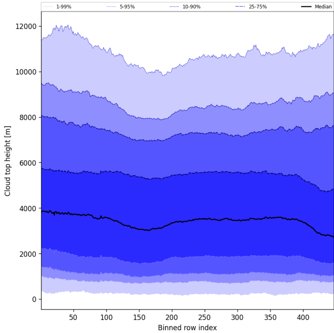
Figure 56: Along track statistics of “Cloud top height” for 2025-01-29 to 2025-01-31
