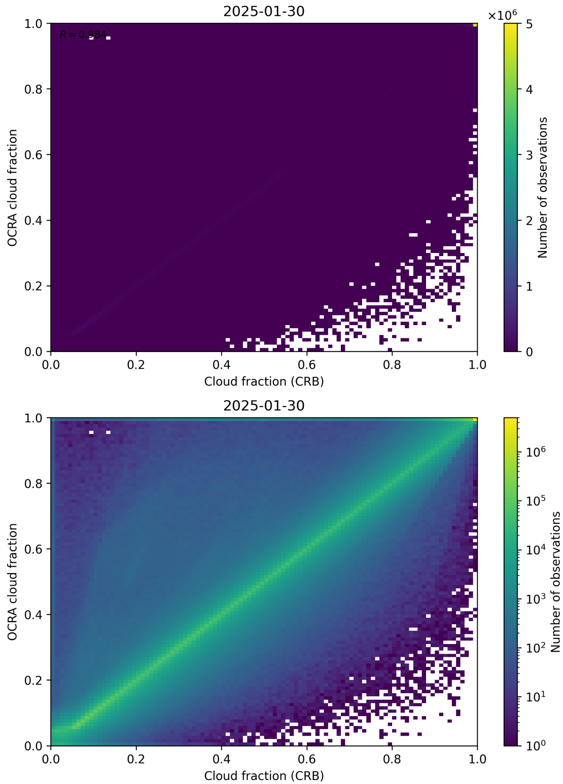
Figure 78: Scatter density plot of “Cloud fraction (CRB)” against “OCRA cloud fraction” for 2025-01-29 to 2025-01-31.
