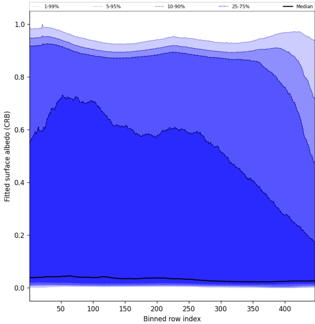
Figure 62: Along track statistics of “Fitted surface albedo (CRB)” for 2025-01-29 to 2025-01-31
