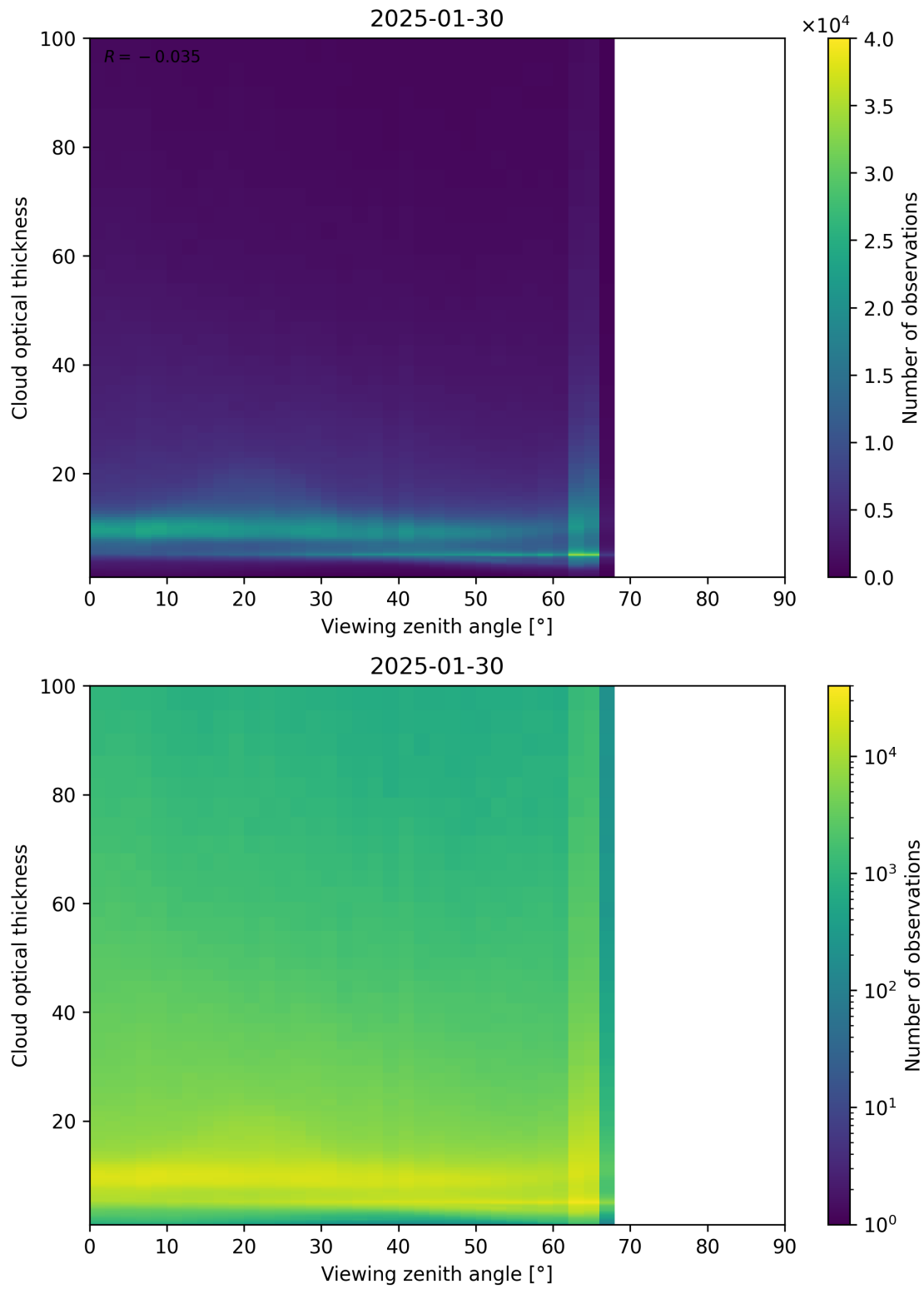
Figure 111: Scatter density plot of “Viewing zenith angle” against “Cloud optical thickness” for 2025-01-29 to 2025-01-31.
