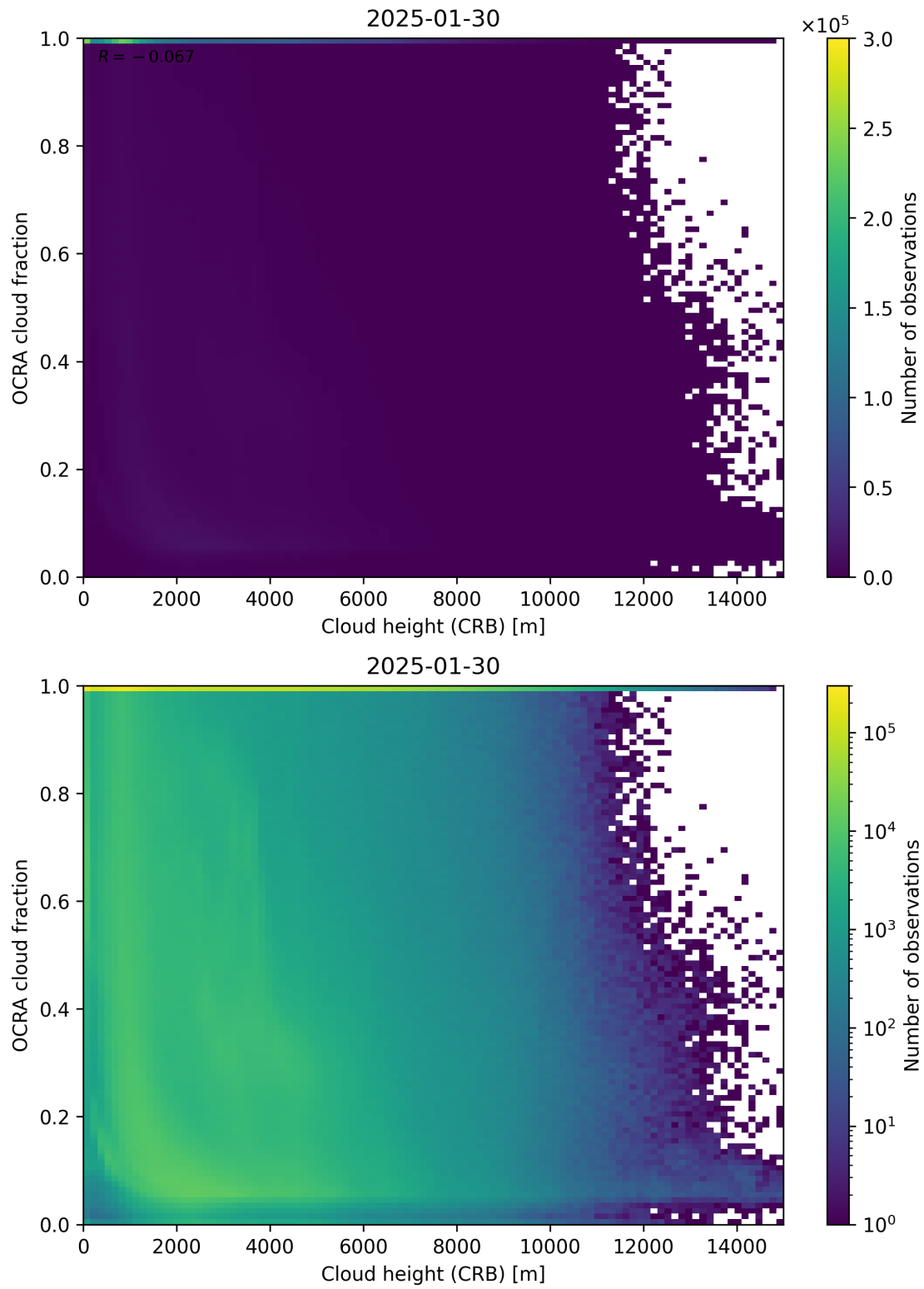
Figure 81: Scatter density plot of “Cloud height (CRB)” against “OCRA cloud fraction” for 2025-01-29 to 2025-01-31.
