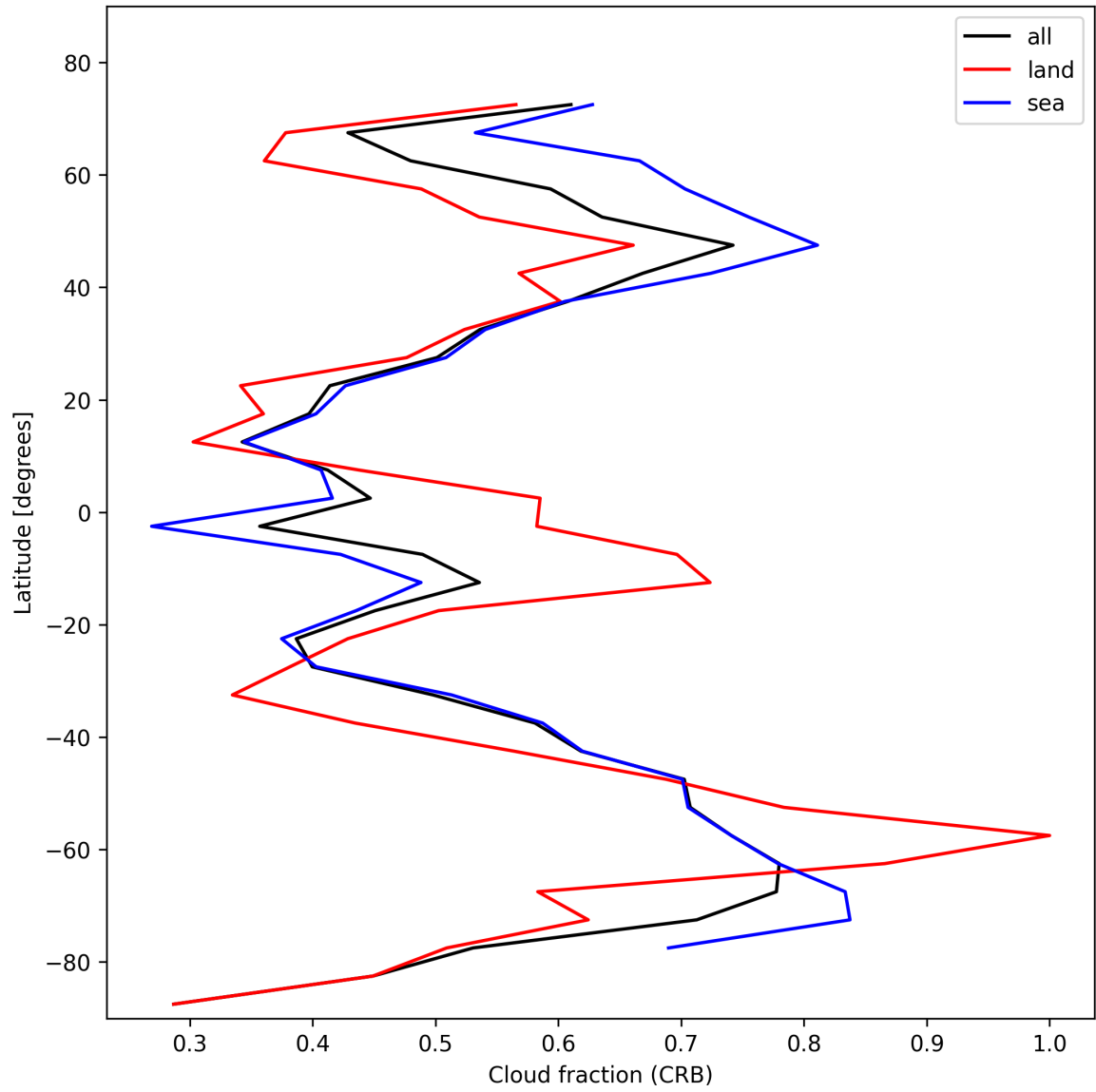
Figure 26: Zonal average of “Cloud fraction (CRB)” for 2025-01-29 to 2025-01-31.
