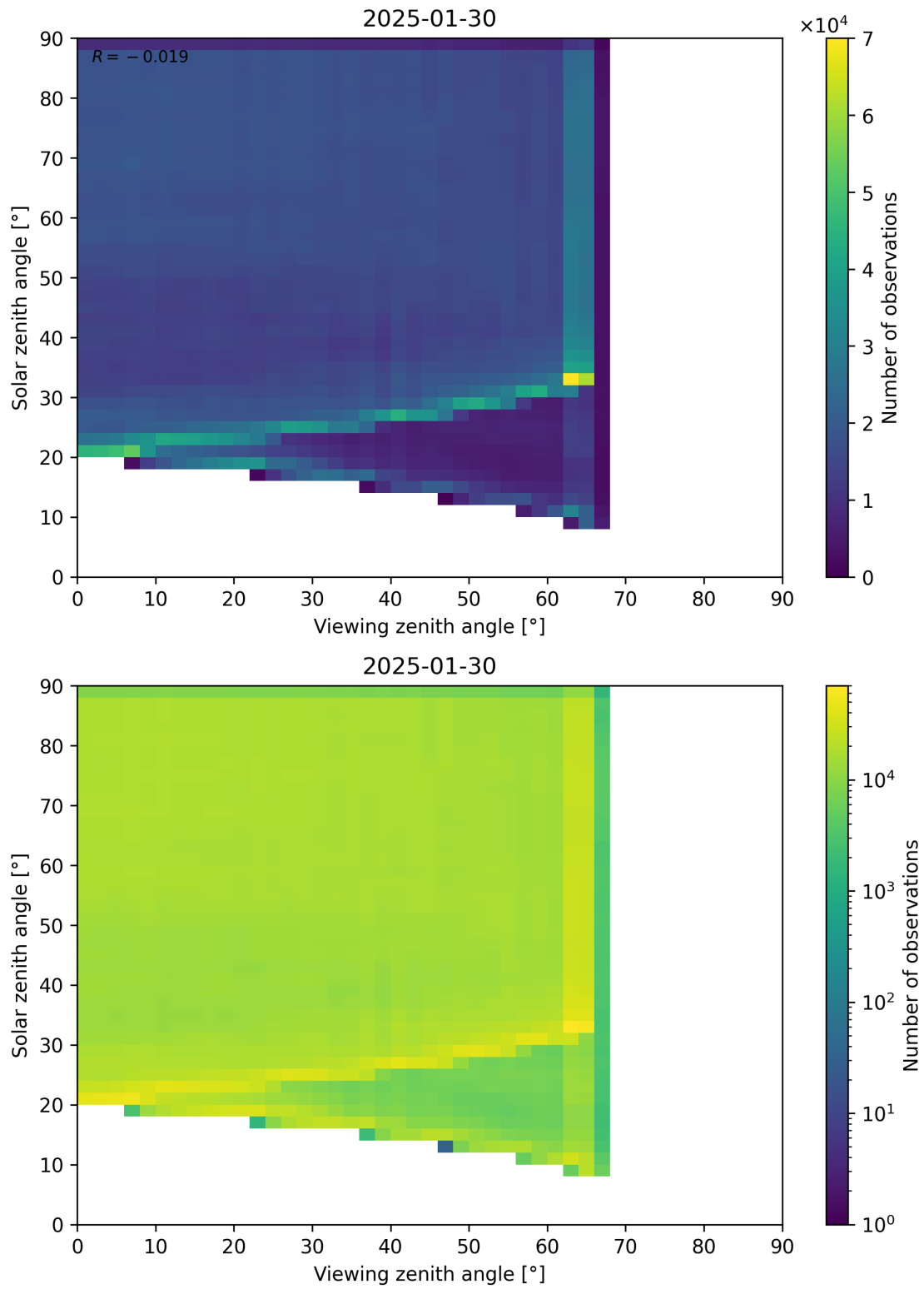
Figure 114: Scatter density plot of “Viewing zenith angle” against “Solar zenith angle” for 2025-01-29 to 2025-01-31.
