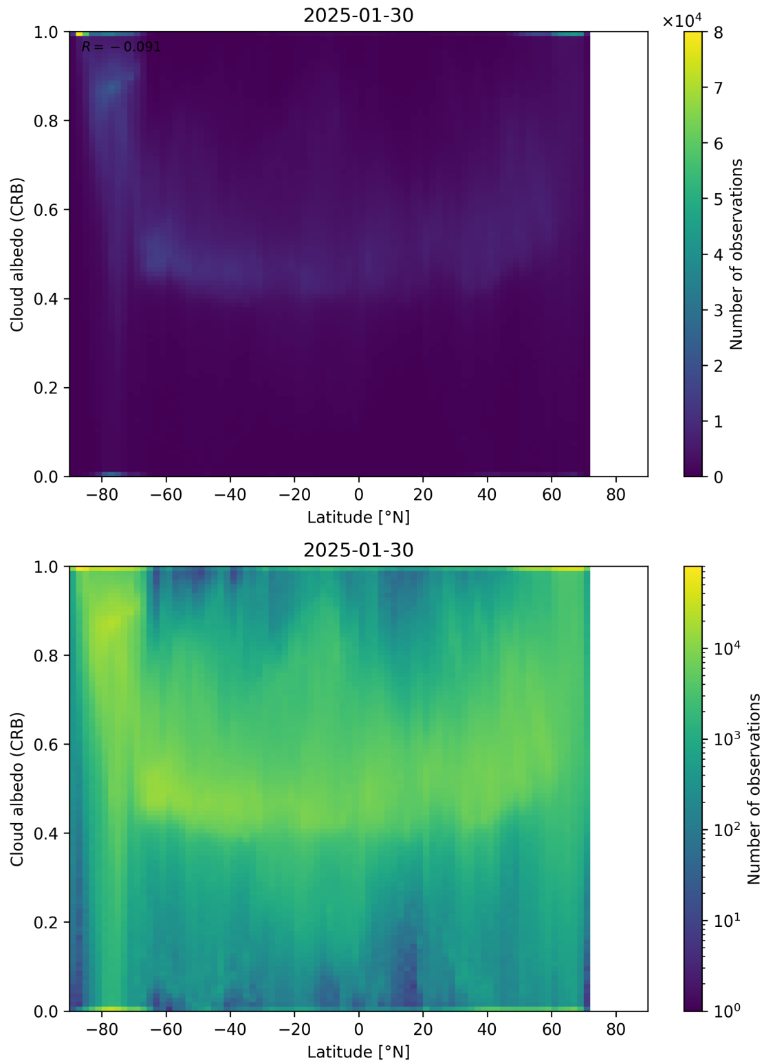
Figure 91: Scatter density plot of “Latitude” against “Cloud albedo (CRB)” for 2025-01-29 to 2025-01-31.
