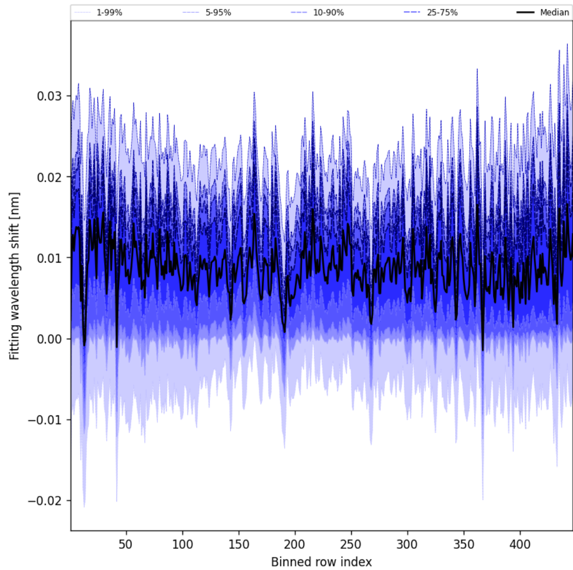
Figure 65: Along track statistics of “Fitting wavelength shift” for 2025-01-29 to 2025-01-31
