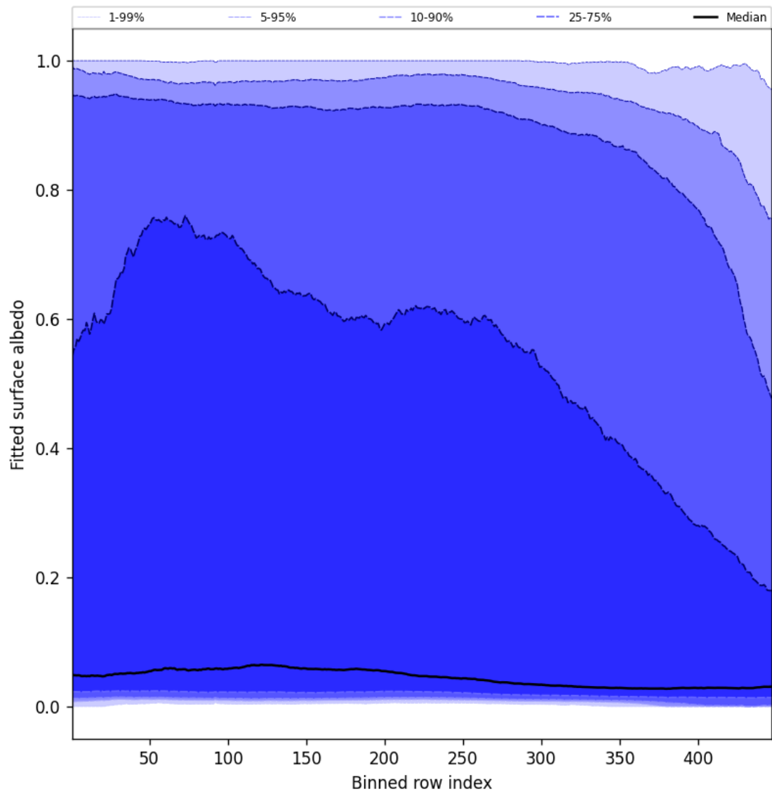
Figure 61: Along track statistics of “Fitted surface albedo” for 2025-01-29 to 2025-01-31
