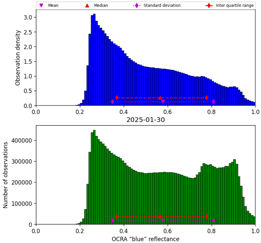
Figure 51: Histogram of “OCRA “blue” reflectance” for 2025-01-29 to 2025-01-31
