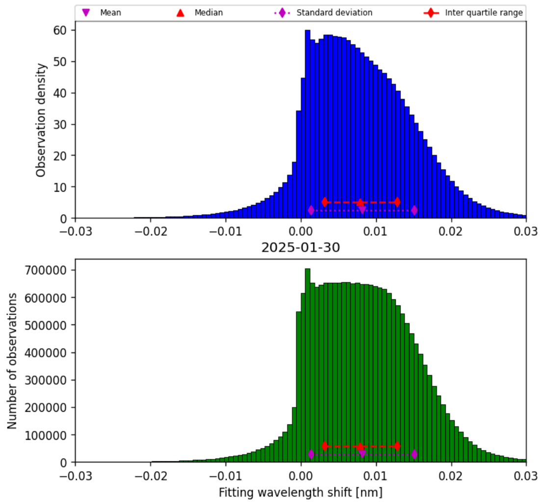
Figure 49: Histogram of “Fitting wavelength shift” for 2025-01-29 to 2025-01-31
