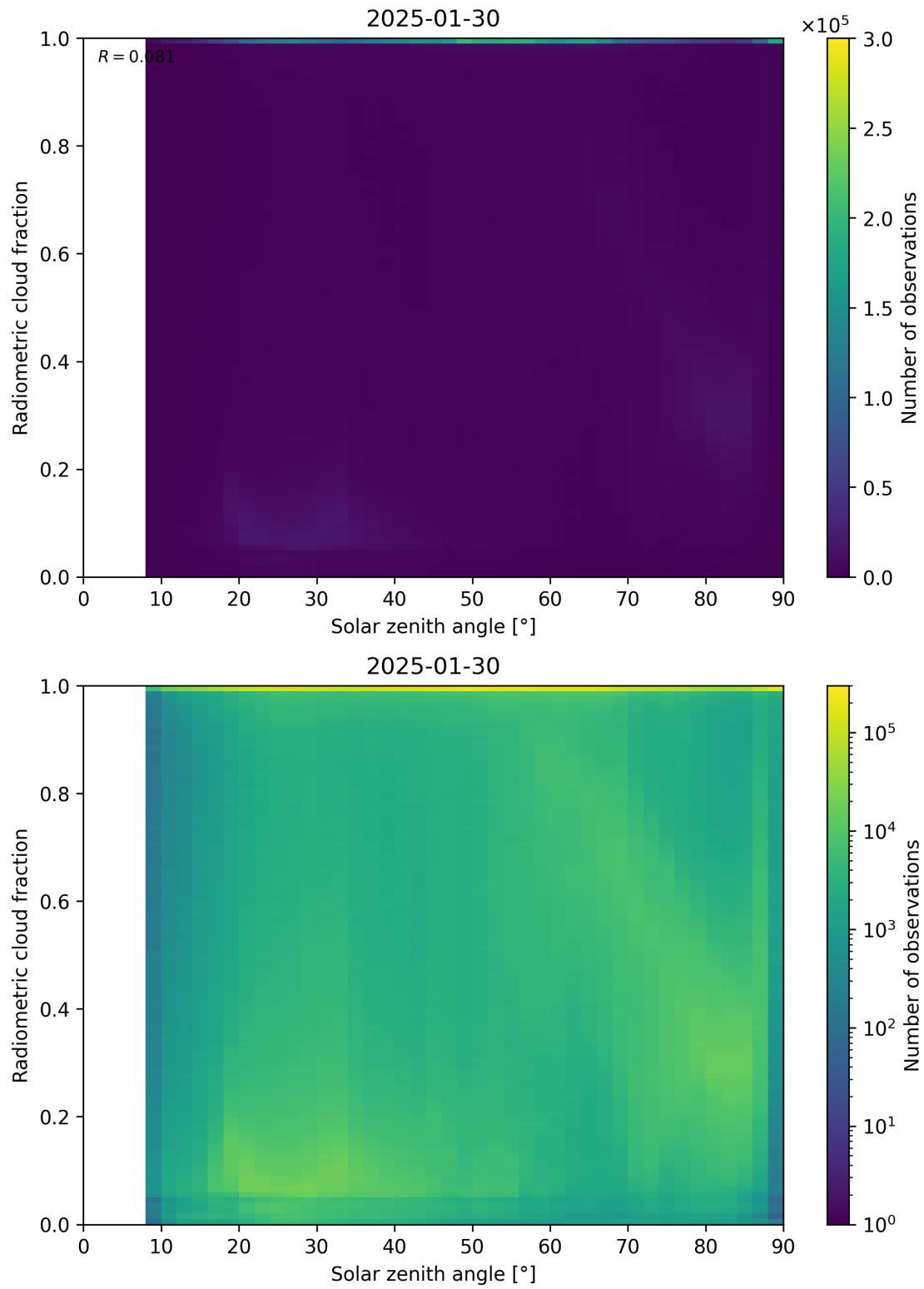
Figure 99: Scatter density plot of “Solar zenith angle” against “Radiometric cloud fraction” for 2025-01-29 to 2025-01-31.
