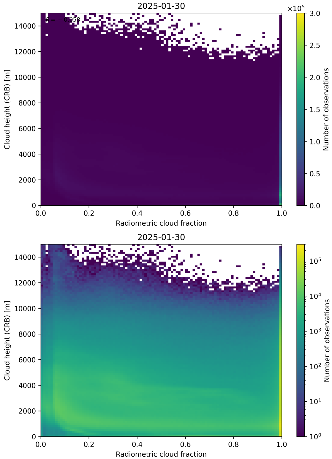
Figure 74: Scatter density plot of “Radiometric cloud fraction” against “Cloud height (CRB)” for 2025-01-29 to 2025-01-31.
