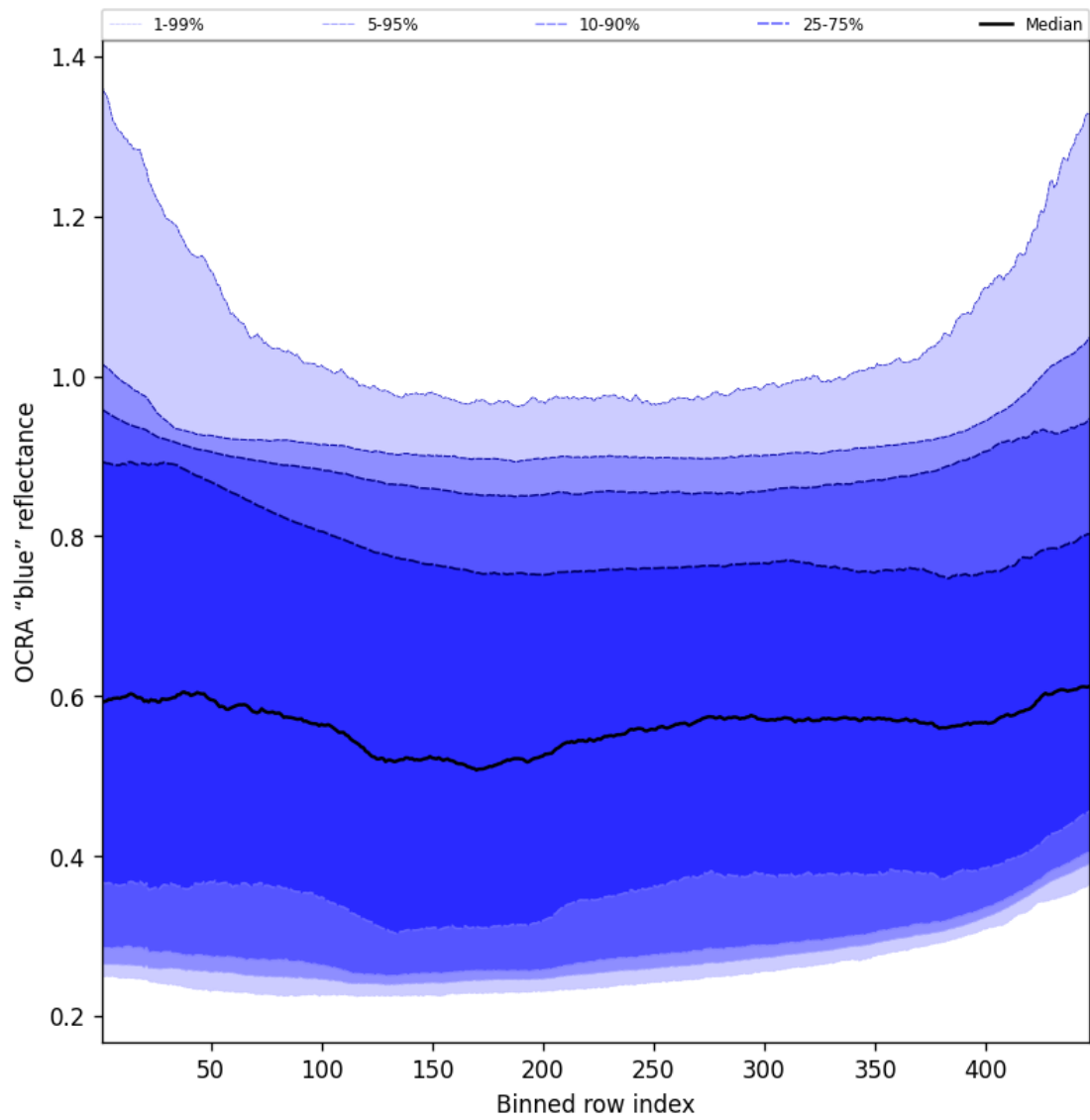
Figure 67: Along track statistics of "OCRA "blue" reflectance" for 2025-01-29 to 2025-01-31
