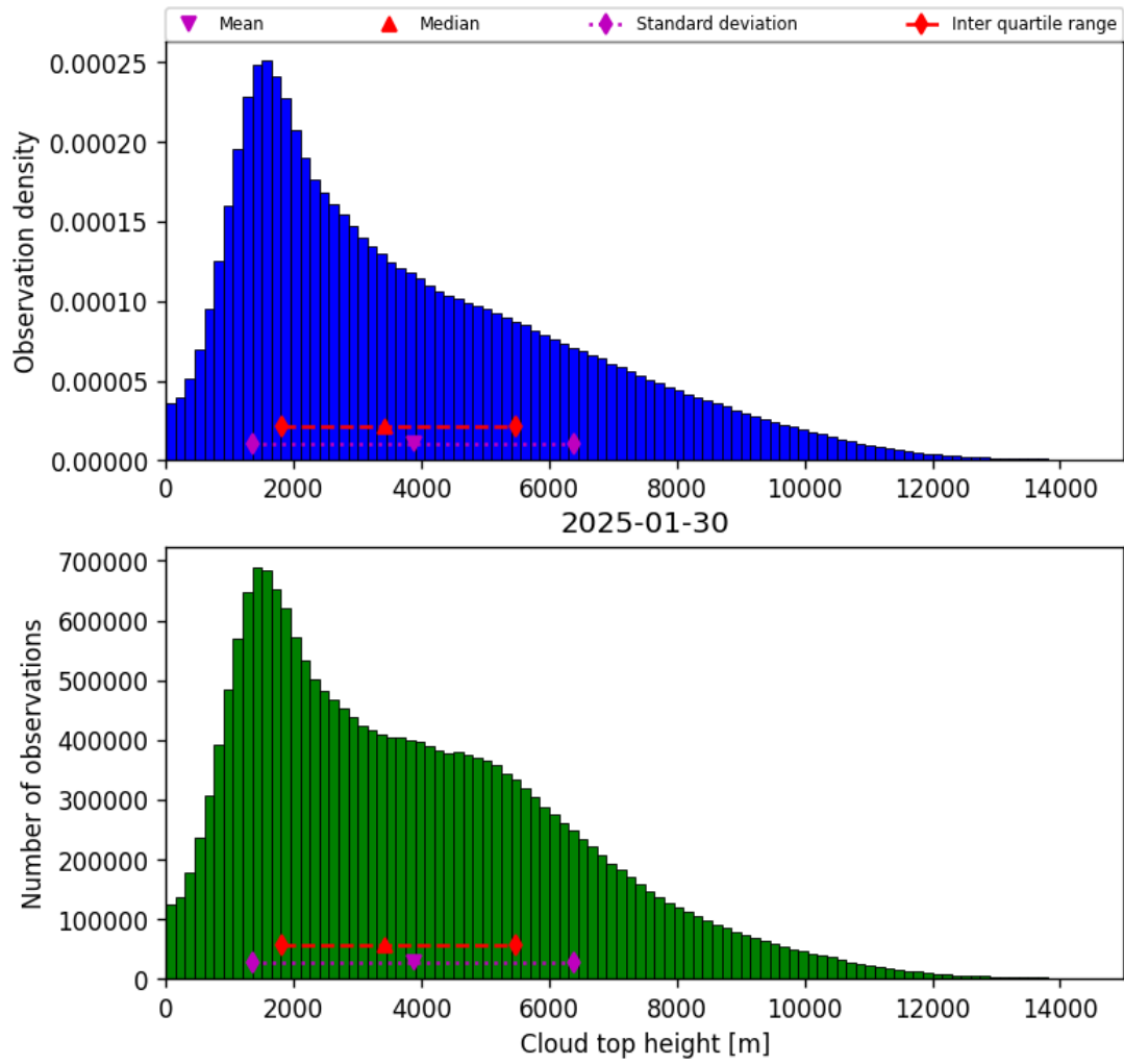
Figure 40: Histogram of “Cloud top height” for 2025-01-29 to 2025-01-31
