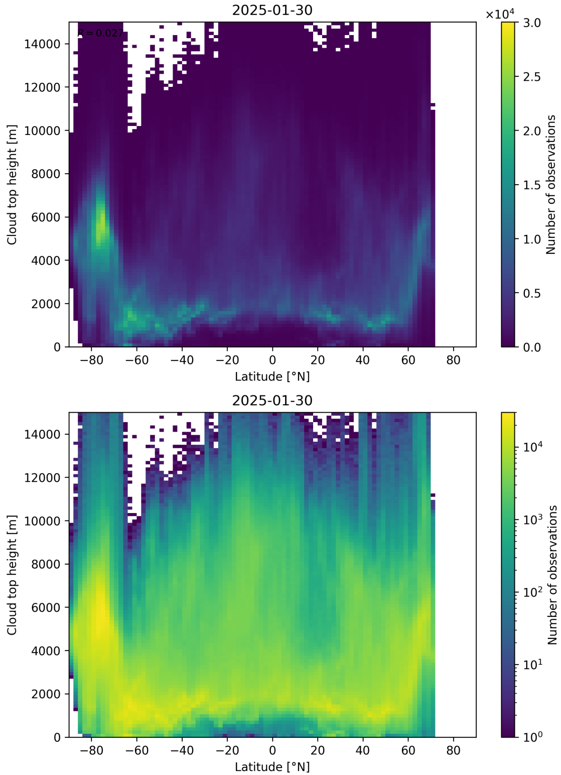
Figure 97: Scatter density plot of “Latitude” against “Cloud top height” for 2025-01-29 to 2025-01-31.
