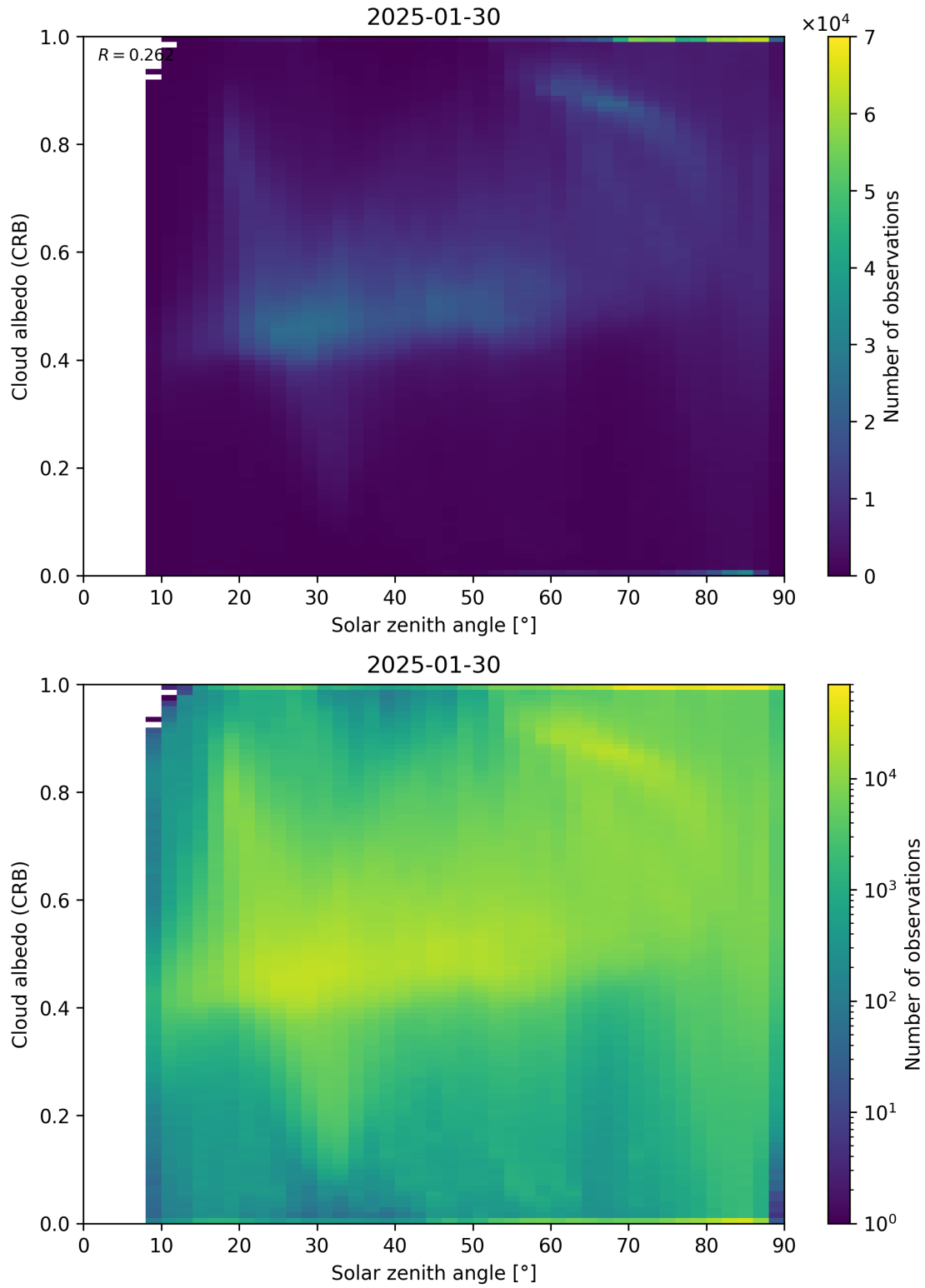
Figure 98: Scatter density plot of “Solar zenith angle” against “Cloud albedo (CRB)” for 2025-01-29 to 2025-01-31.
