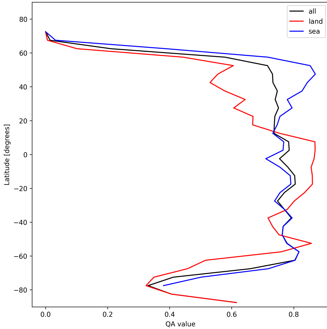
Figure 22: Zonal average of “QA value” for 2025-01-29 to 2025-01-31.
