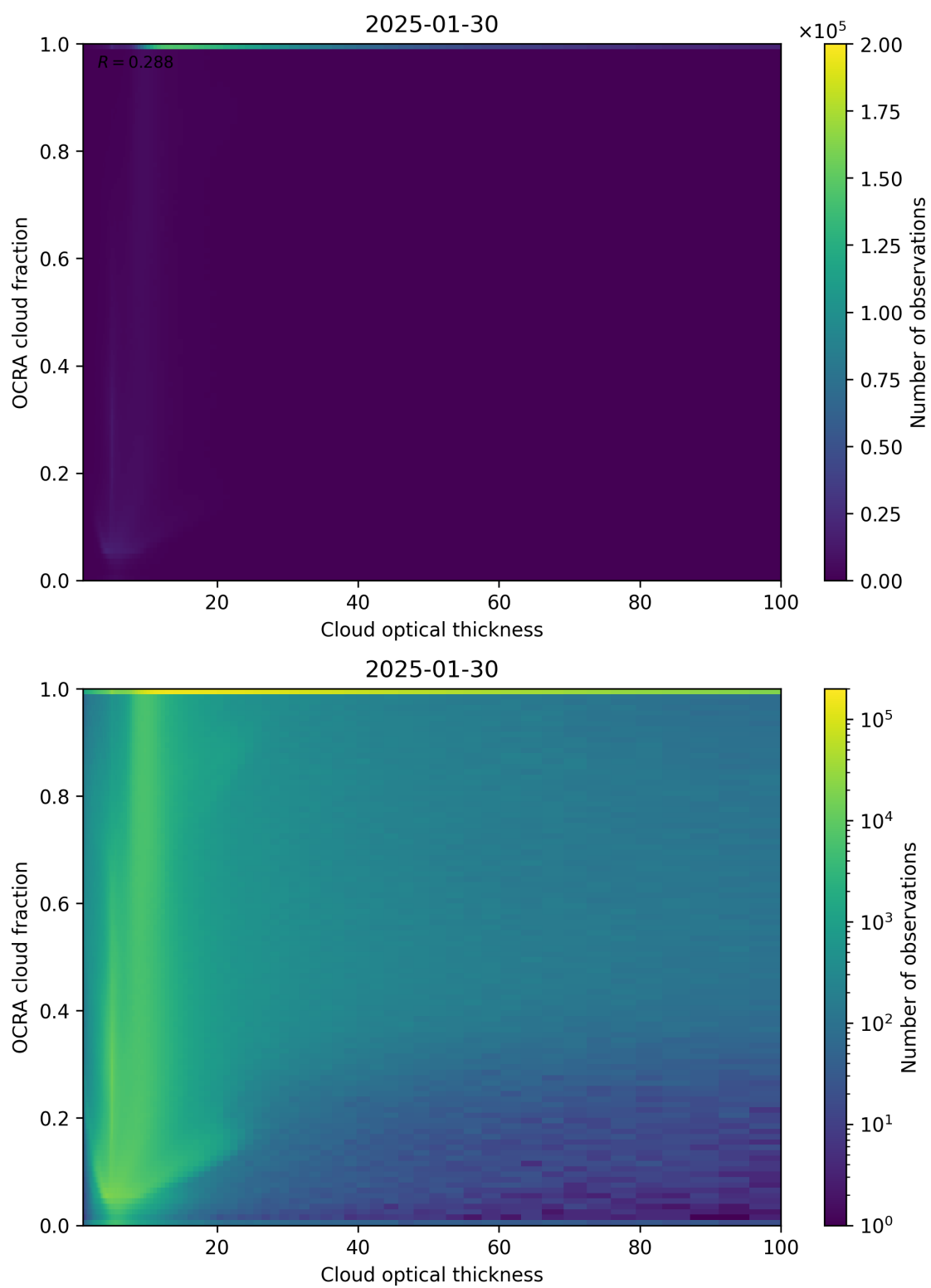
Figure 83: Scatter density plot of “Cloud optical thickness” against “OCRA cloud fraction” for 2025-01-29 to 2025-01-31.
