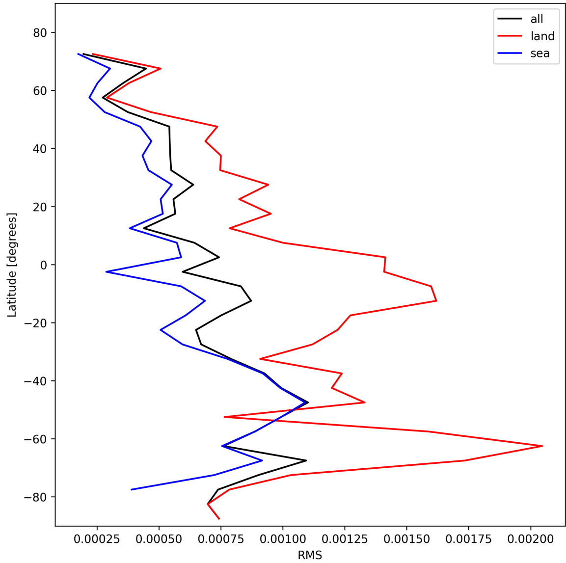
Figure 31: Zonal average of “RMS” for 2025-01-29 to 2025-01-31.
