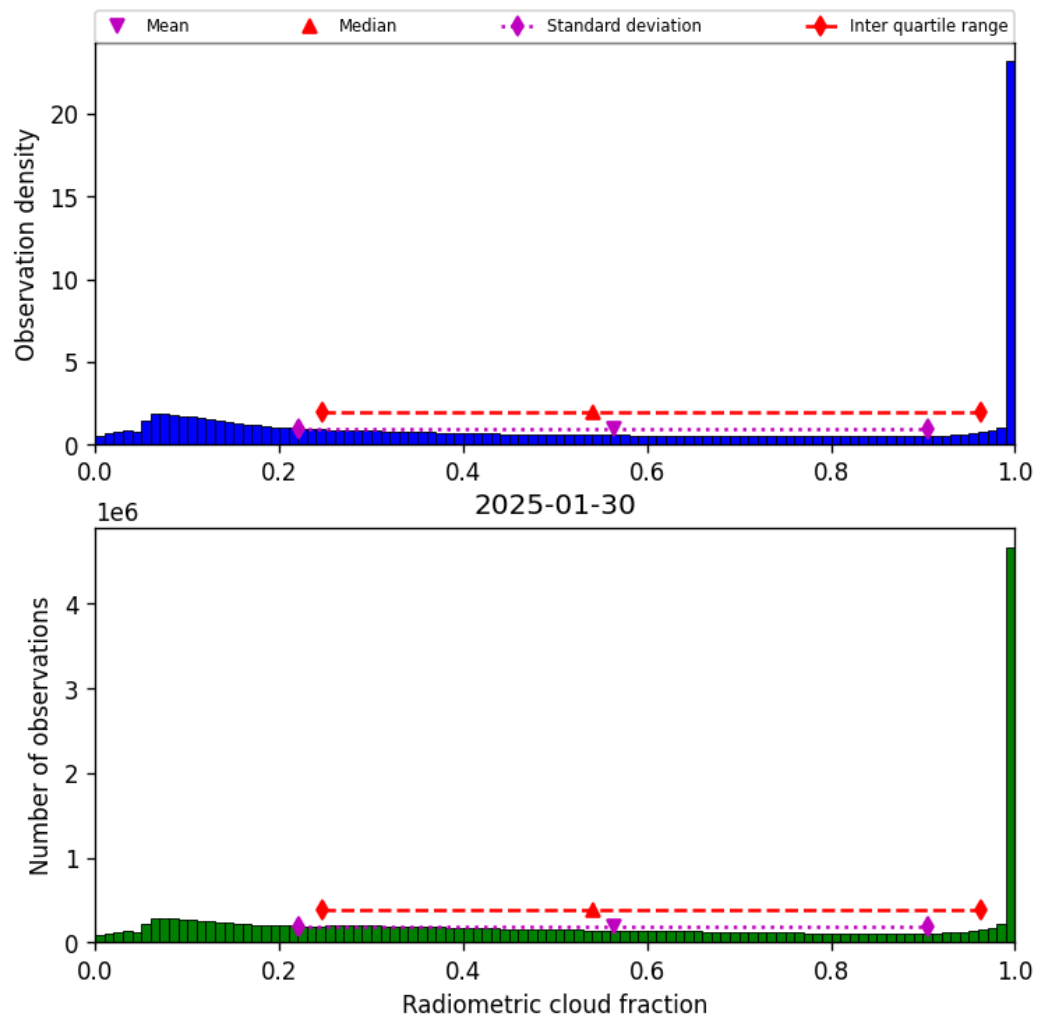
Figure 39: Histogram of “Radiometric cloud fraction” for 2025-01-29 to 2025-01-31
