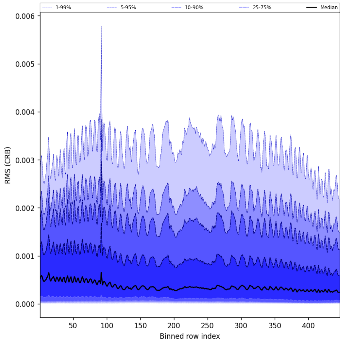
Figure 64: Along track statistics of “RMS (CRB)” for 2025-01-29 to 2025-01-31
