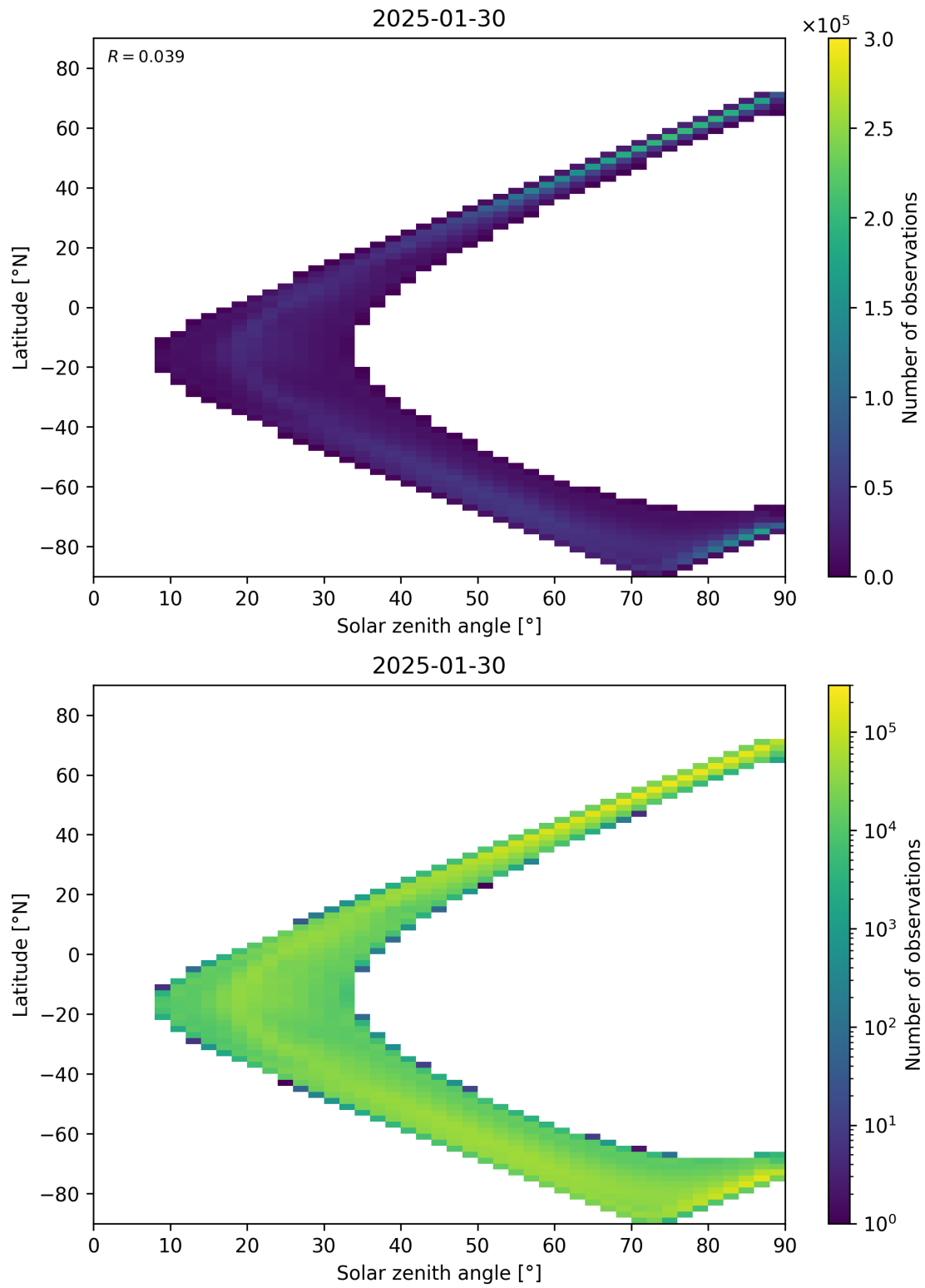
Figure 105: Scatter density plot of “Solar zenith angle” against “Latitude” for 2025-01-29 to 2025-01-31.
