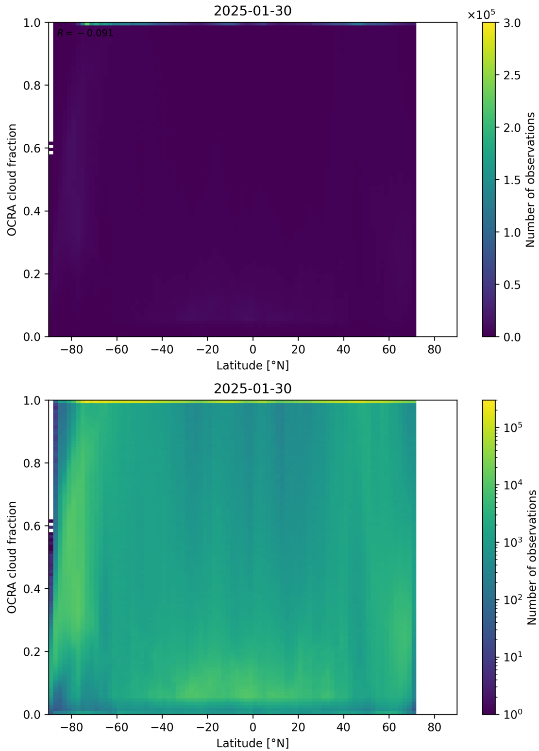
Figure 93: Scatter density plot of “Latitude” against “OCRA cloud fraction” for 2025-01-29 to 2025-01-31.
