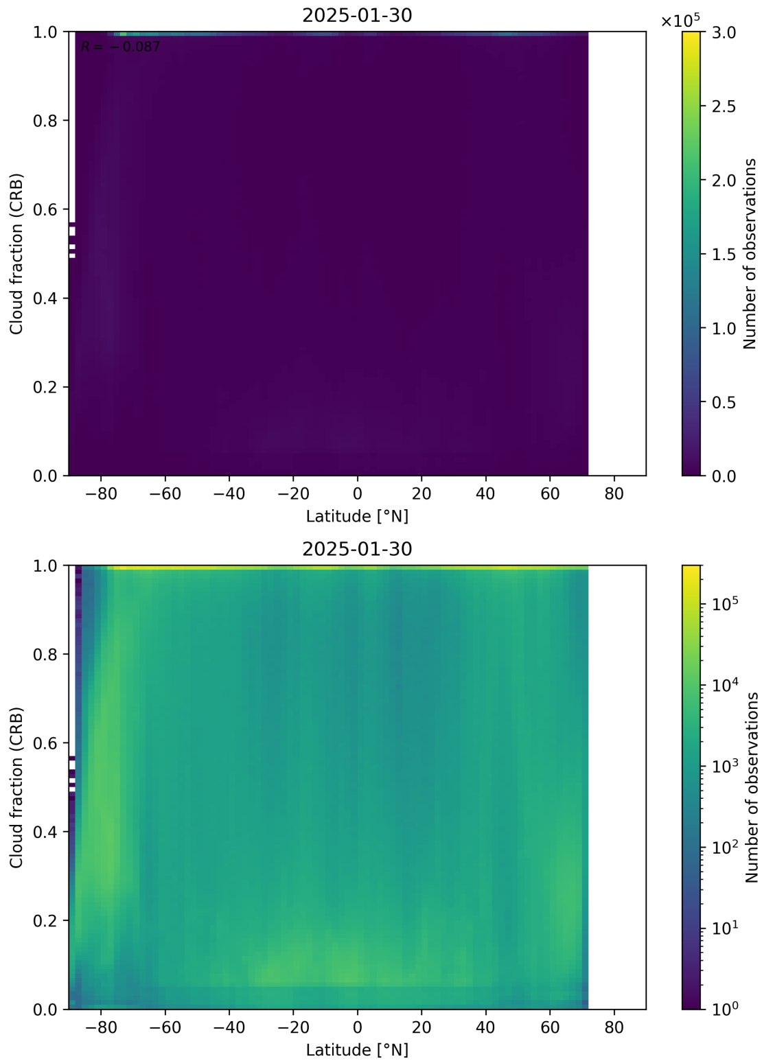
Figure 94: Scatter density plot of “Latitude” against “Cloud fraction (CRB)” for 2025-01-29 to 2025-01-31.
