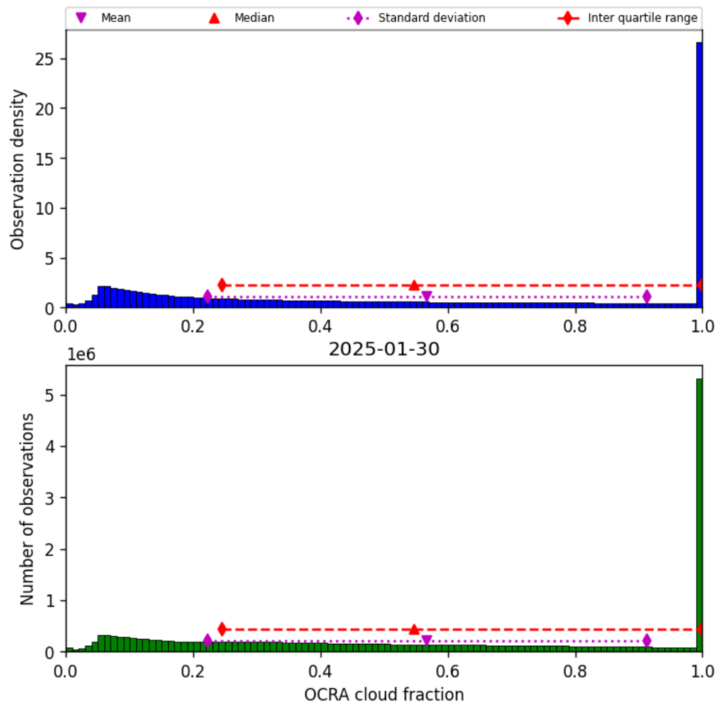
Figure 50: Histogram of “OCRA cloud fraction” for 2025-01-29 to 2025-01-31
