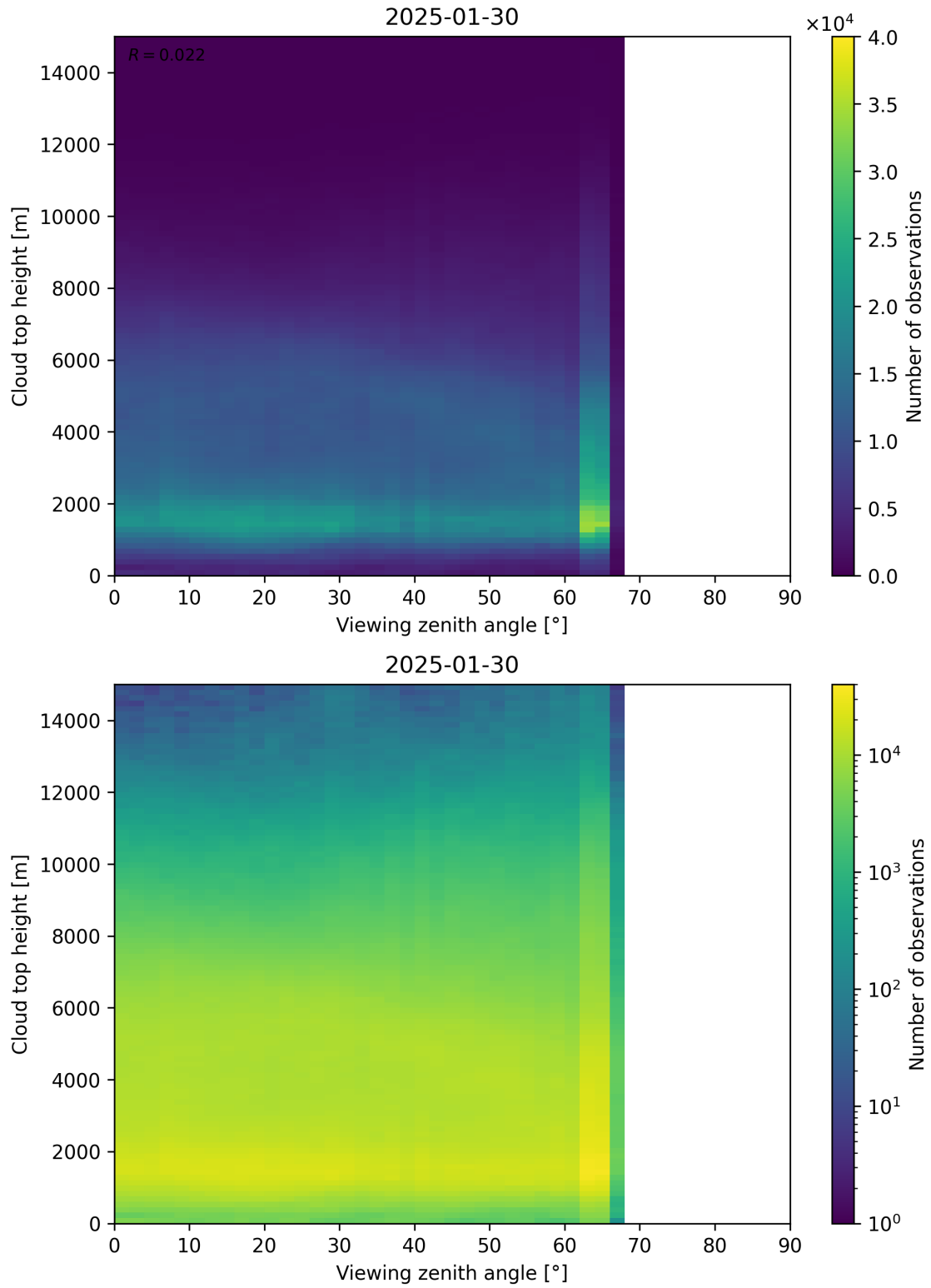
Figure 112: Scatter density plot of “Viewing zenith angle” against “Cloud top height” for 2025-01-29 to 2025-01-31.
