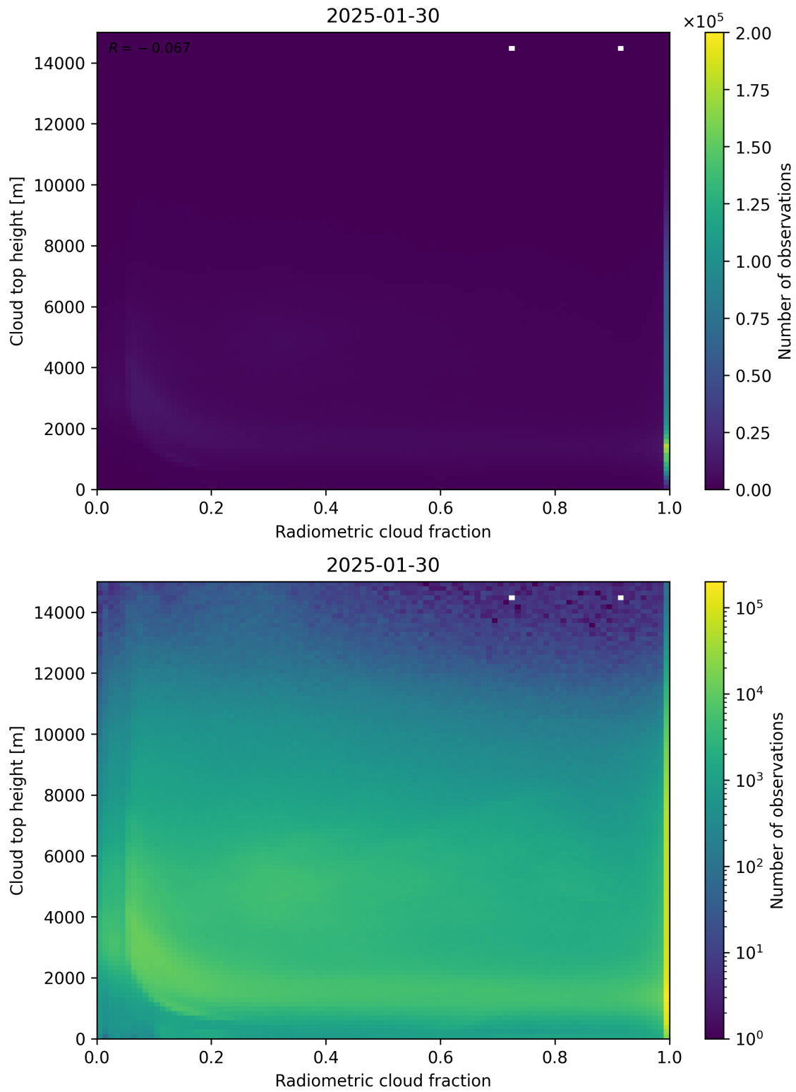
Figure 76: Scatter density plot of “Radiometric cloud fraction” against “Cloud top height” for 2025-01-29 to 2025-01-31.
