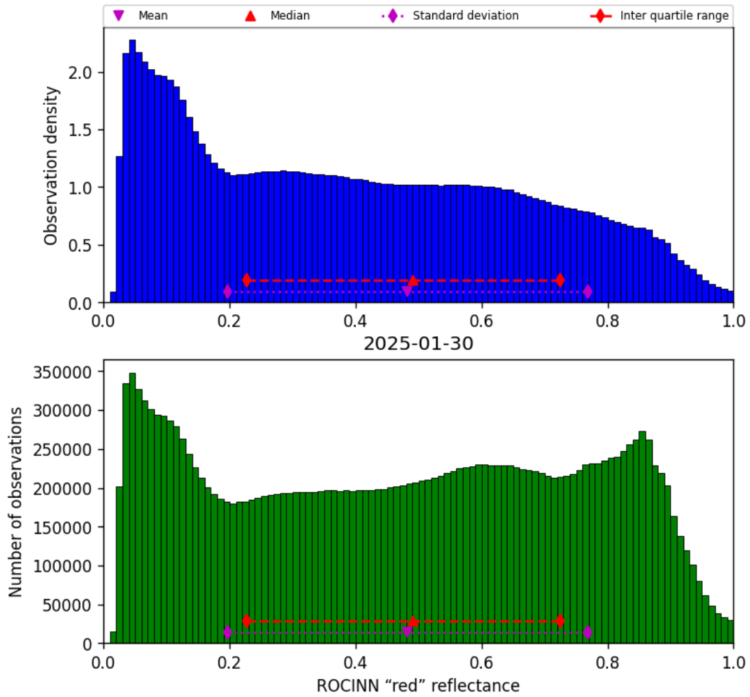
Figure 53: Histogram of “ROCINN “red” reflectance” for 2025-01-29 to 2025-01-31
