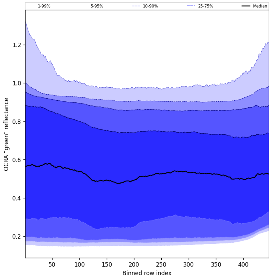
Figure 68: Along track statistics of “OCRA “green” reflectance” for 2025-01-29 to 2025-01-31
