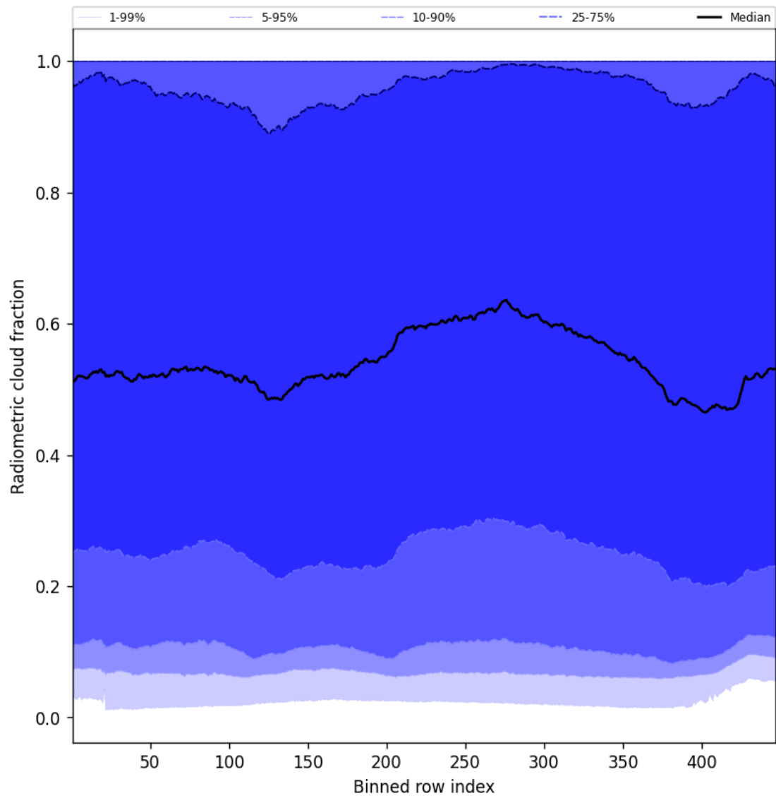
Figure 55: Along track statistics of “Radiometric cloud fraction” for 2025-01-29 to 2025-01-31
