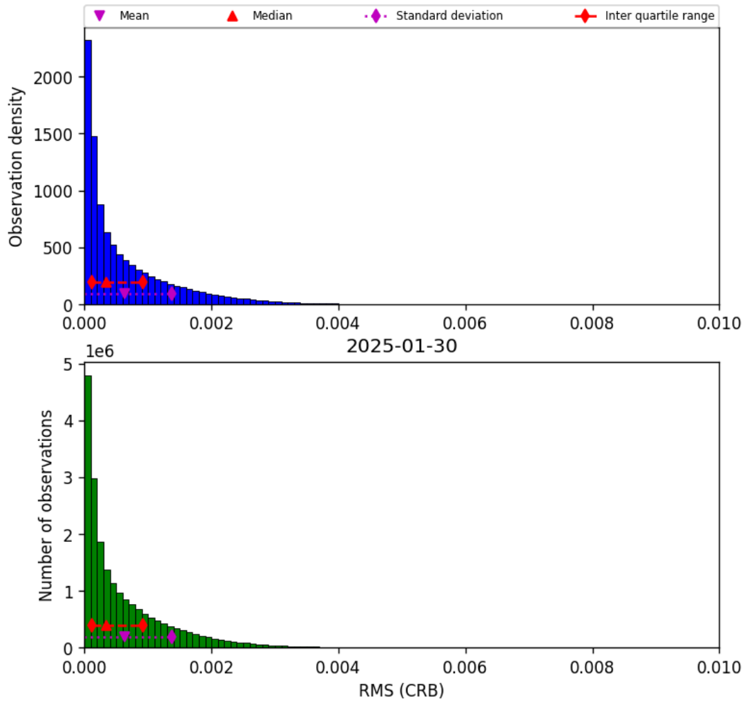
Figure 48: Histogram of “RMS (CRB)” for 2025-01-29 to 2025-01-31
