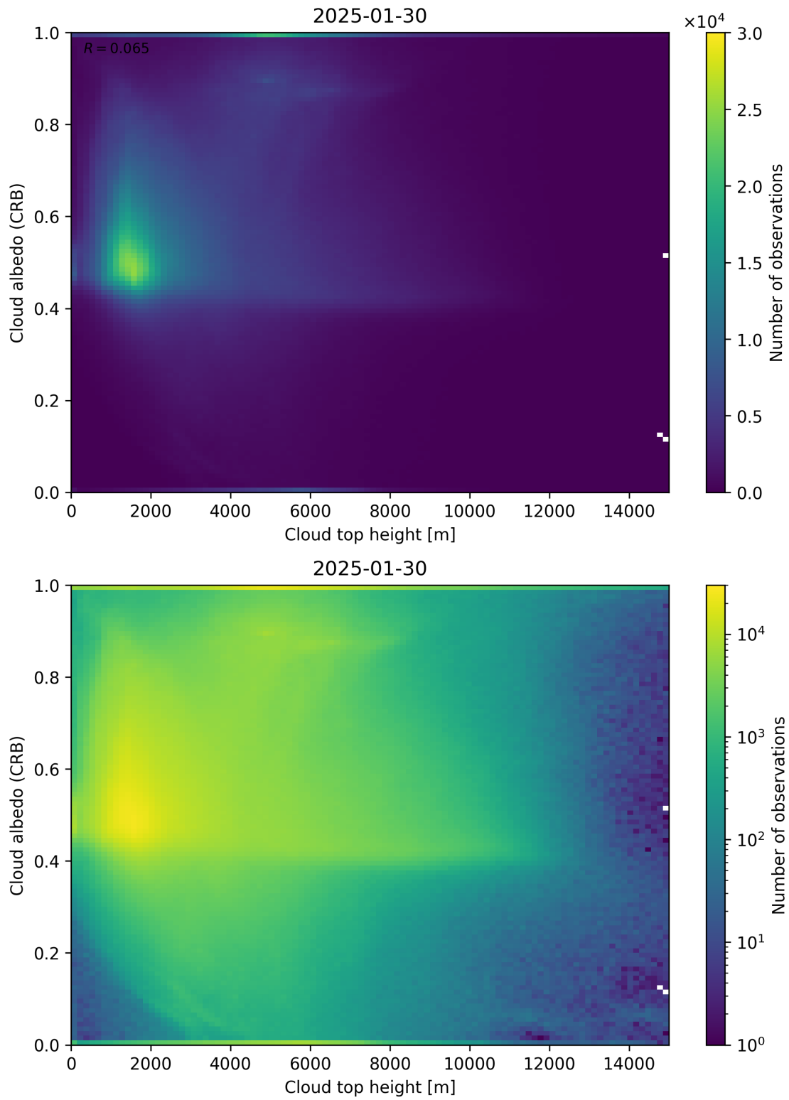
Figure 86: Scatter density plot of “Cloud top height” against “Cloud albedo (CRB)” for 2025-01-29 to 2025-01-31.
