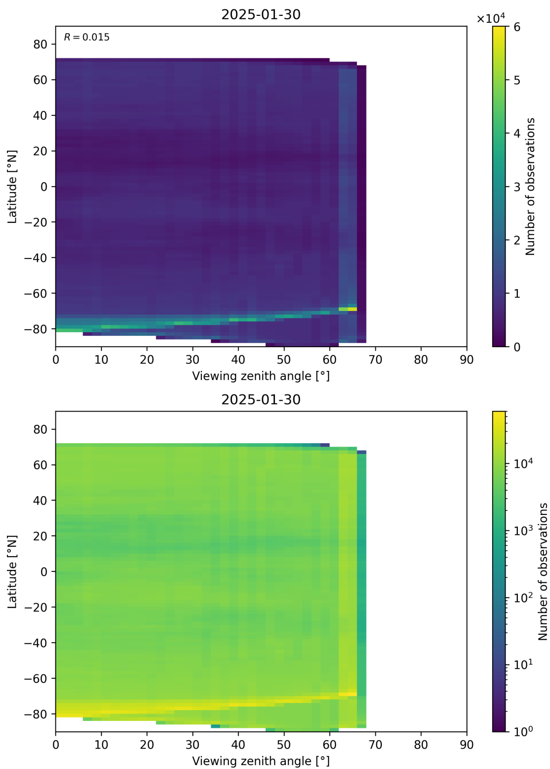
Figure 113: Scatter density plot of “Viewing zenith angle” against “Latitude” for 2025-01-29 to 2025-01-31.
