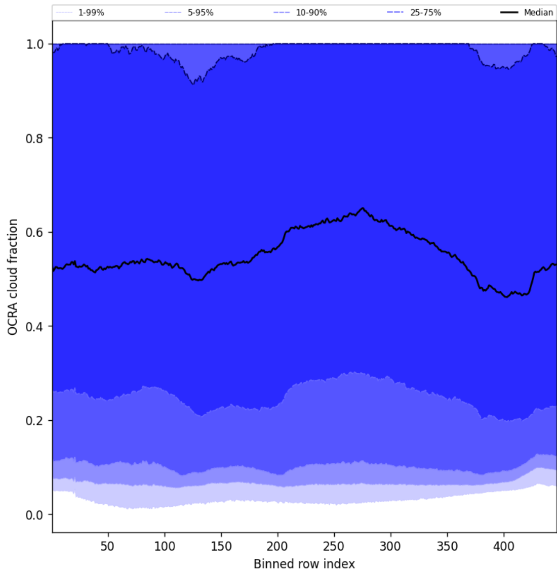
Figure 66: Along track statistics of “OCRA cloud fraction” for 2025-01-29 to 2025-01-31
