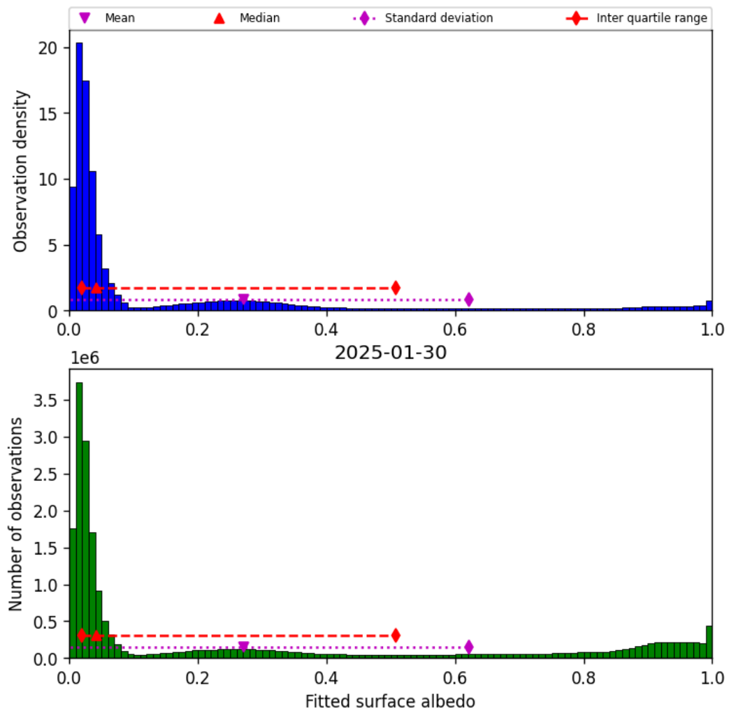
Figure 45: Histogram of “Fitted surface albedo” for 2025-01-29 to 2025-01-31
