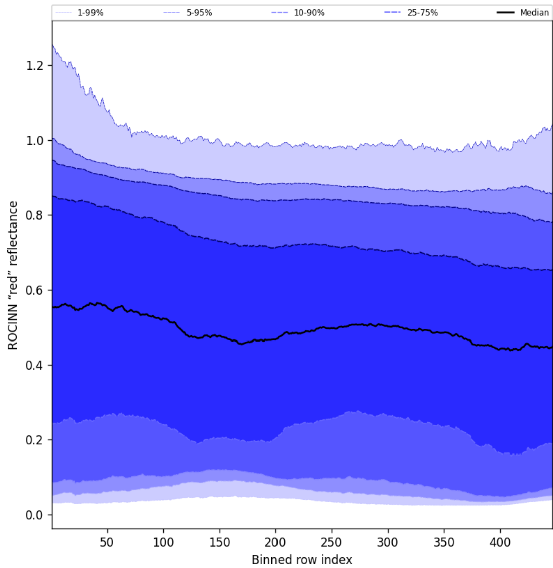
Figure 69: Along track statistics of “ROCINN “red” reflectance” for 2025-01-29 to 2025-01-31
