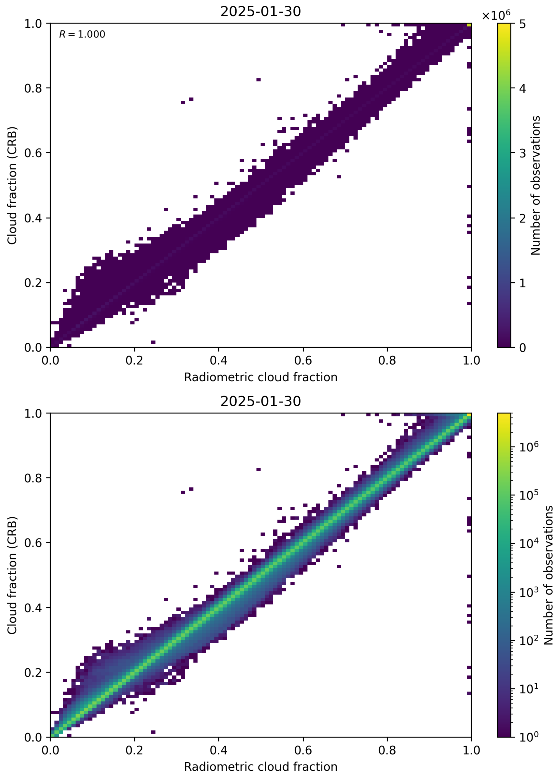
Figure 73: Scatter density plot of “Radiometric cloud fraction” against “Cloud fraction (CRB)” for 2025-01-29 to 2025-01-31.
