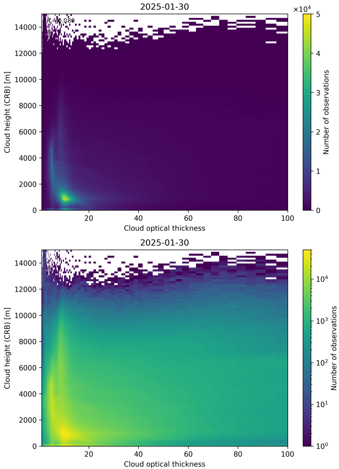
Figure 85: Scatter density plot of “Cloud optical thickness” against “Cloud height (CRB)” for 2025-01-29 to 2025-01-31.
