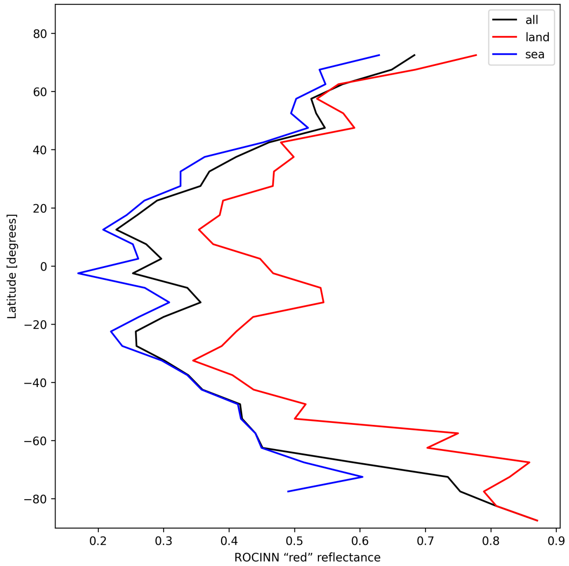
Figure 37: Zonal average of “ROCINN “red” reflectance” for 2025-01-29 to 2025-01-31.
