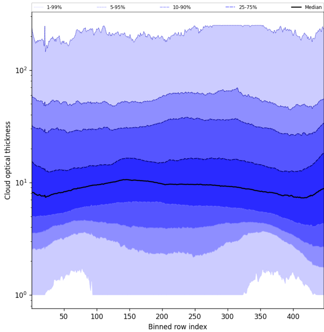
Figure 57: Along track statistics of “Cloud optical thickness” for 2025-01-29 to 2025-01-31
