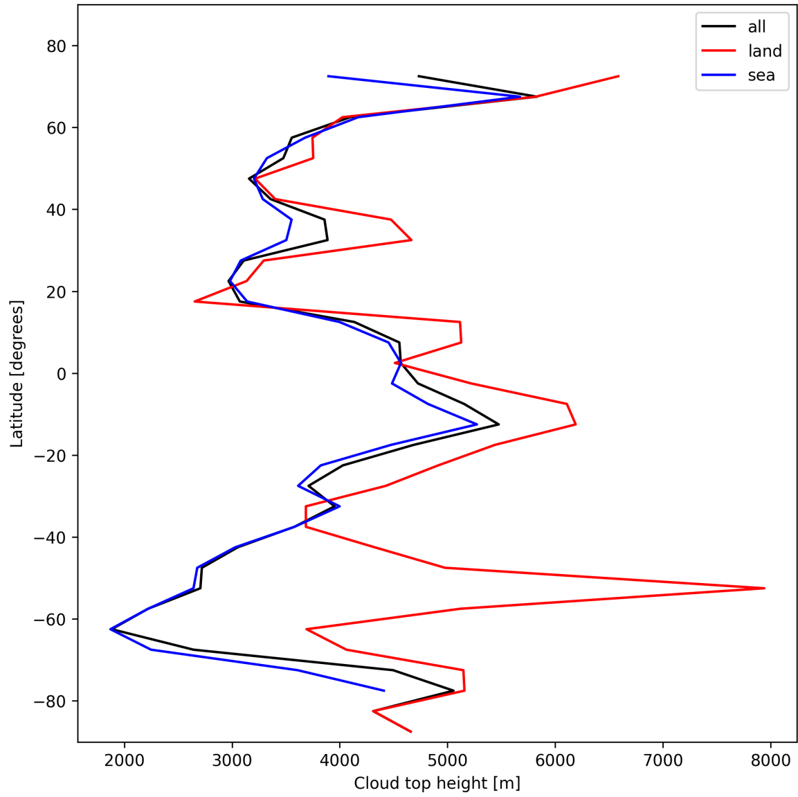
Figure 24: Zonal average of “Cloud top height” for 2025-01-29 to 2025-01-31.
