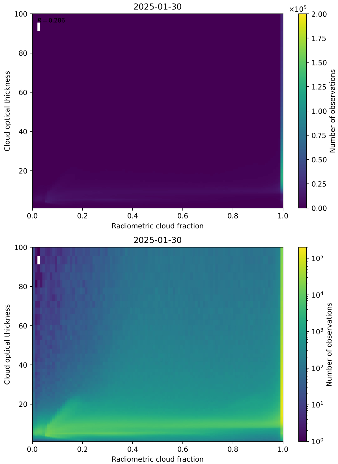
Figure 75: Scatter density plot of “Radiometric cloud fraction” against “Cloud optical thickness” for 2025-01-29 to 2025-01-31.
