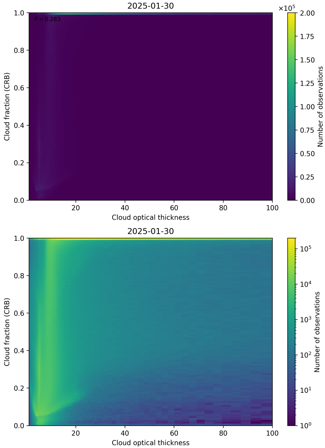
Figure 84: Scatter density plot of “Cloud optical thickness” against “Cloud fraction (CRB)” for 2025-01-29 to 2025-01-31.
