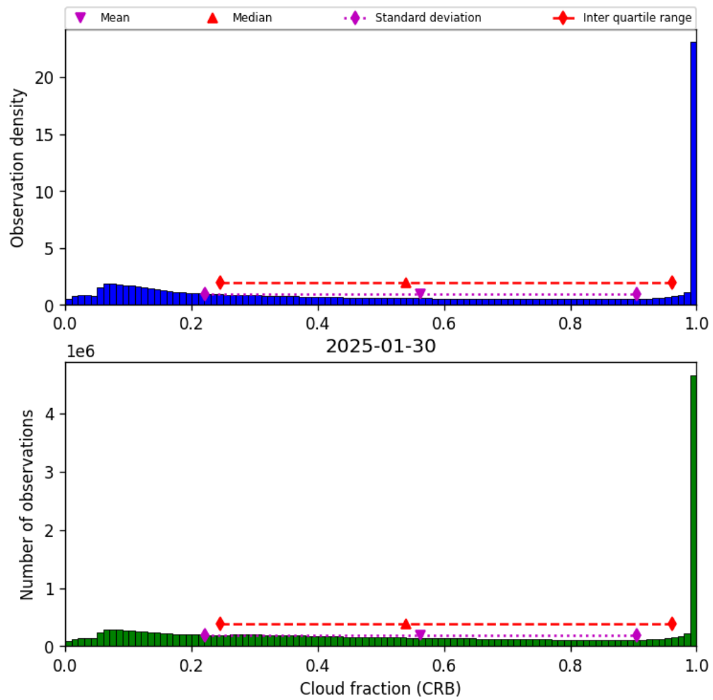
Figure 42: Histogram of “Cloud fraction (CRB)” for 2025-01-29 to 2025-01-31
