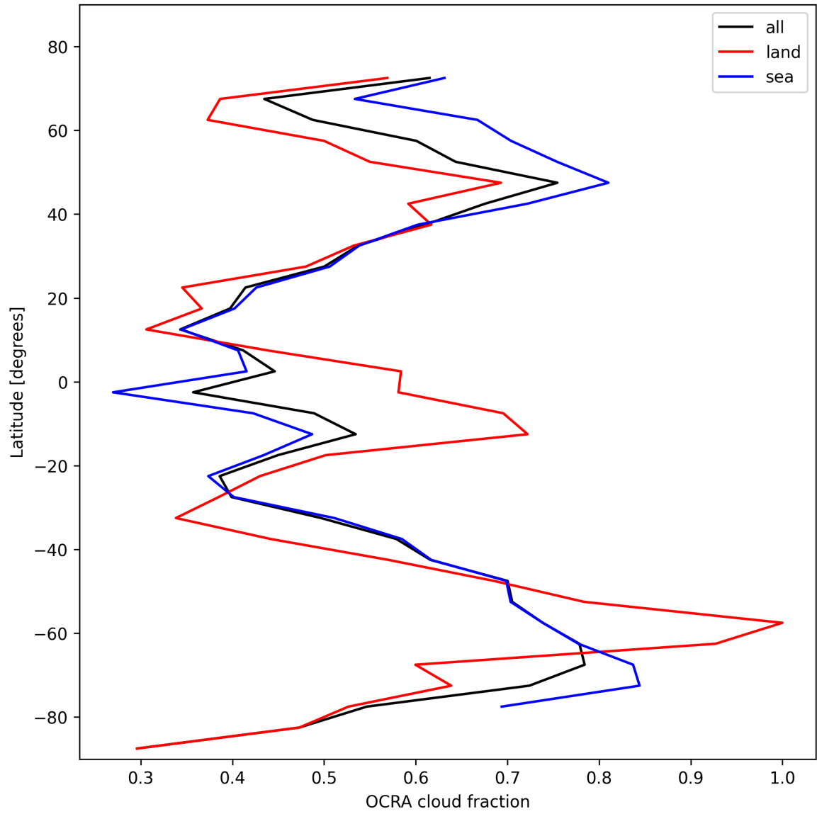
Figure 34: Zonal average of “OCRA cloud fraction” for 2025-01-29 to 2025-01-31.
