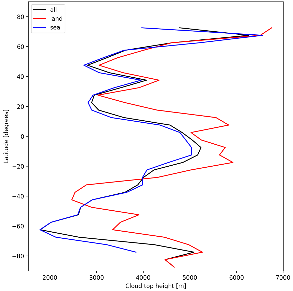
Figure 24: Zonal average of “Cloud top height” for 2025-01-30 to 2025-02-01.
