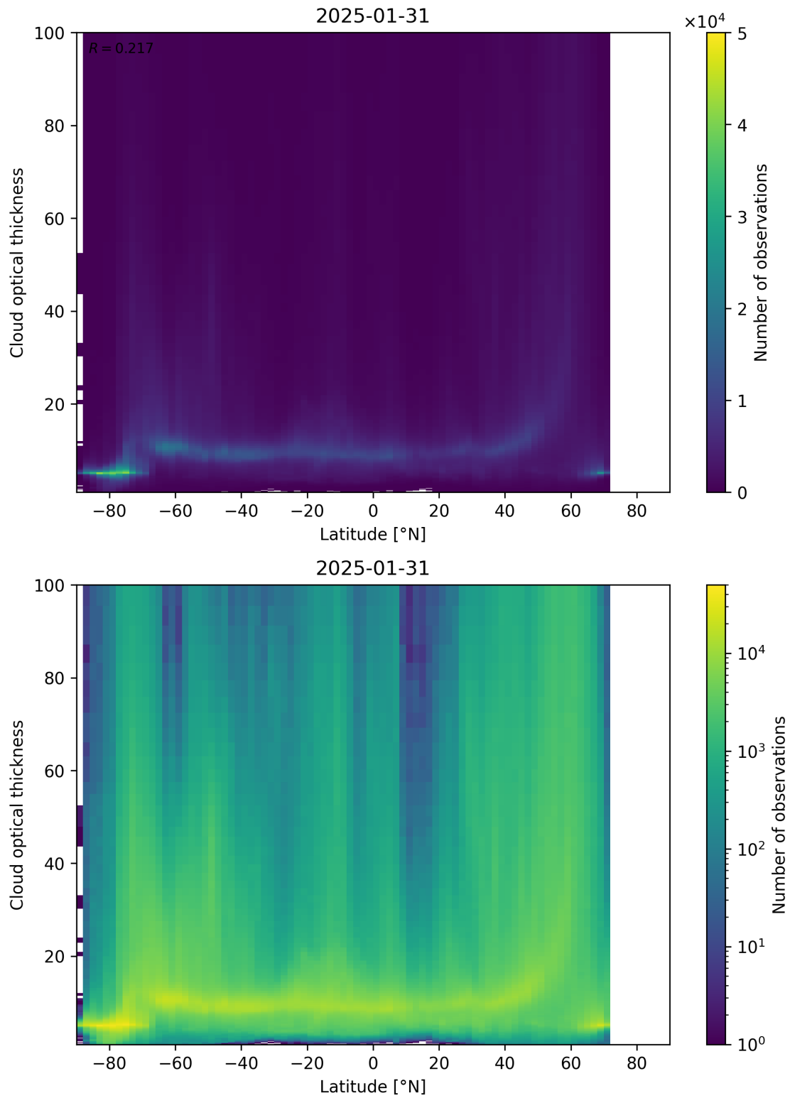
Figure 96: Scatter density plot of “Latitude” against “Cloud optical thickness” for 2025-01-30 to 2025-02-01.
