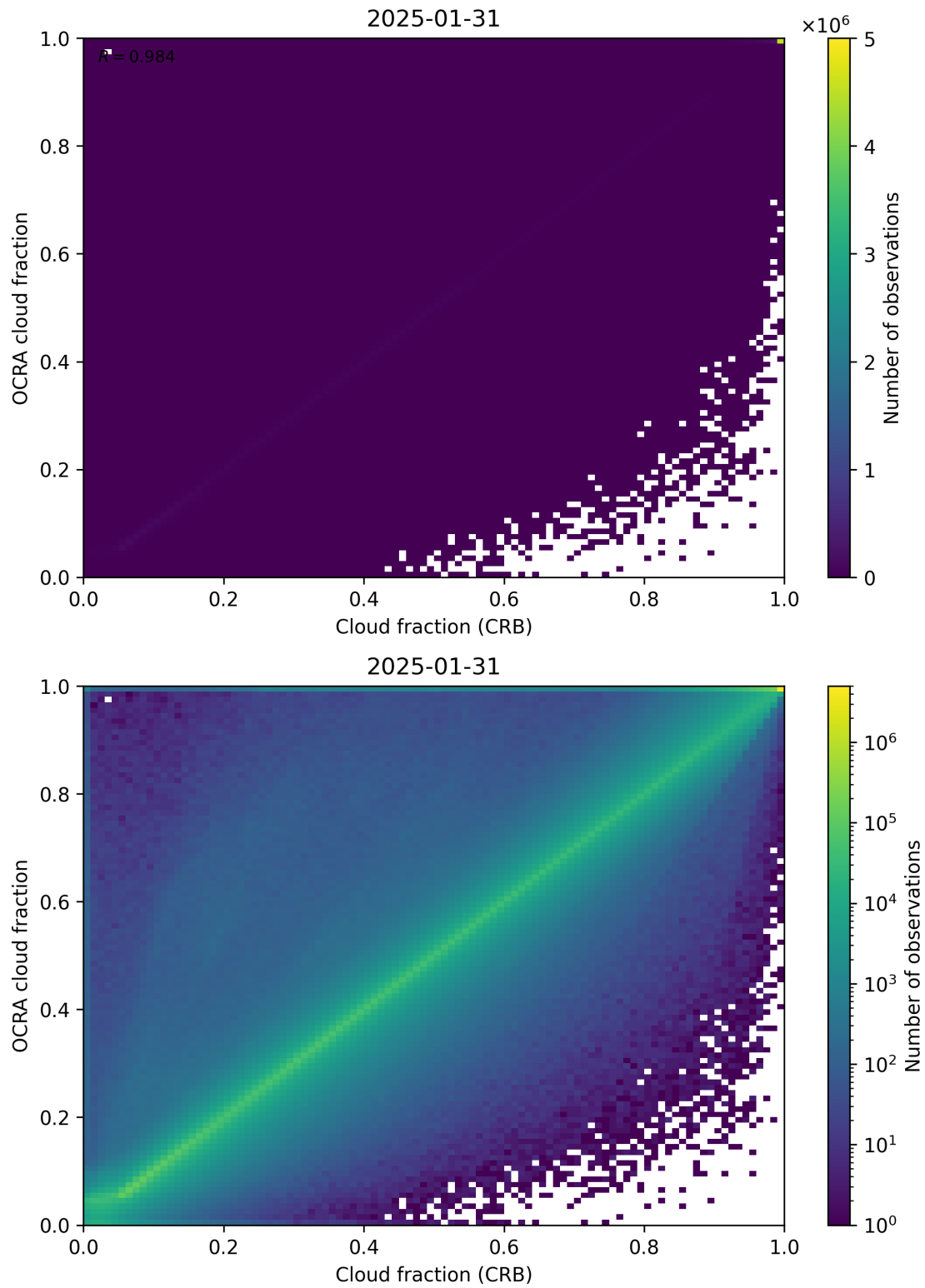
Figure 78: Scatter density plot of “Cloud fraction (CRB)” against “OCRA cloud fraction” for 2025-01-30 to 2025-02-01.
