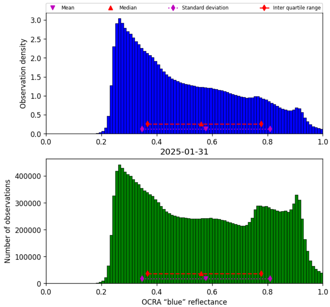
Figure 51: Histogram of “OCRA “blue” reflectance” for 2025-01-30 to 2025-02-01
