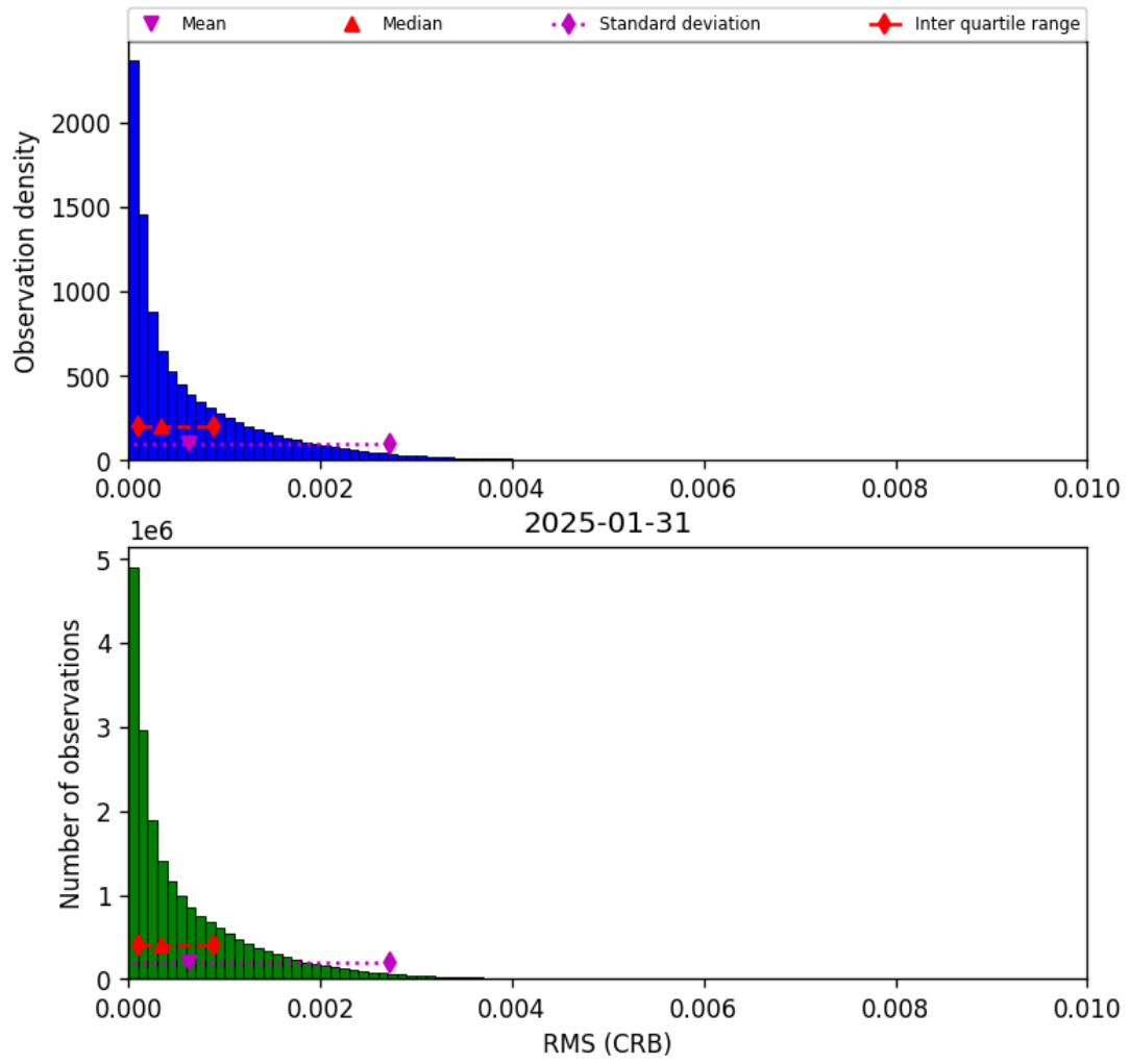
Figure 48: Histogram of “RMS (CRB)” for 2025-01-30 to 2025-02-01
