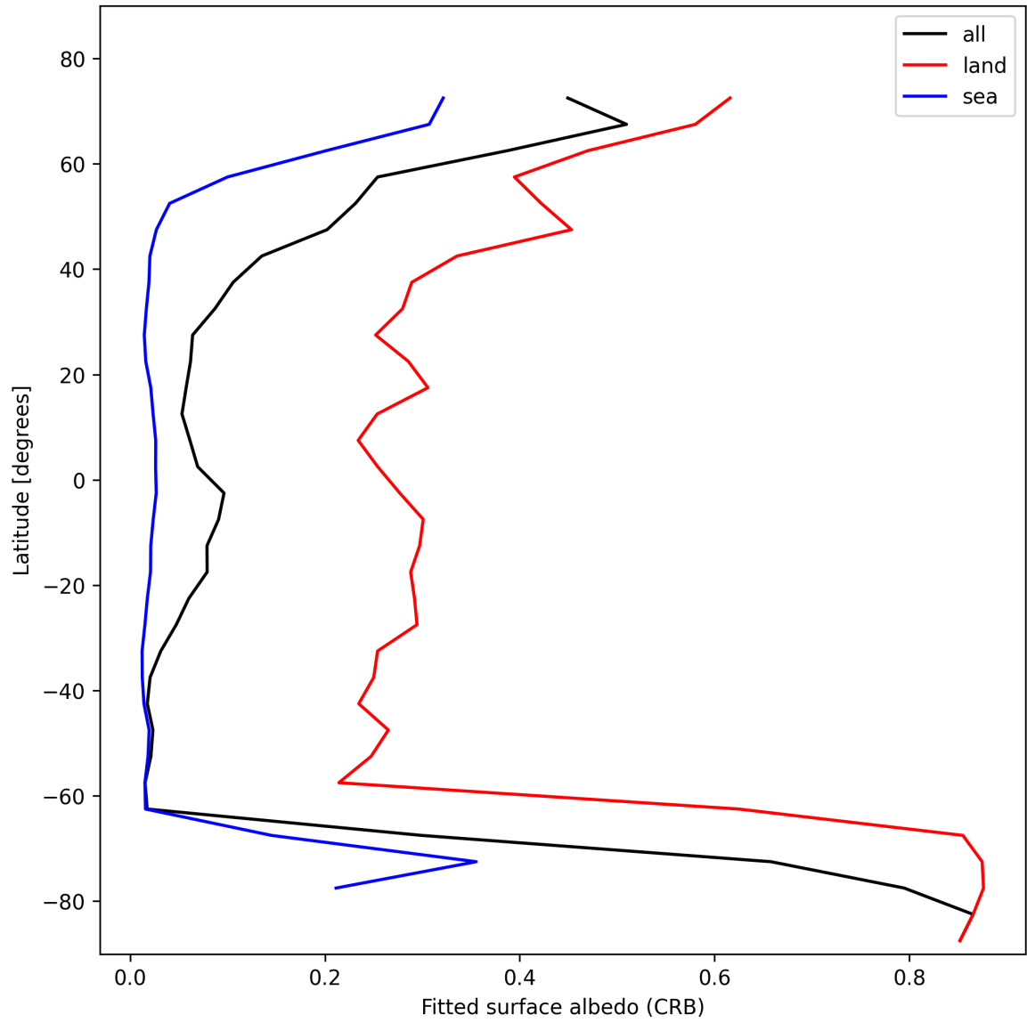
Figure 30: Zonal average of “Fitted surface albedo (CRB)” for 2025-01-30 to 2025-02-01.
