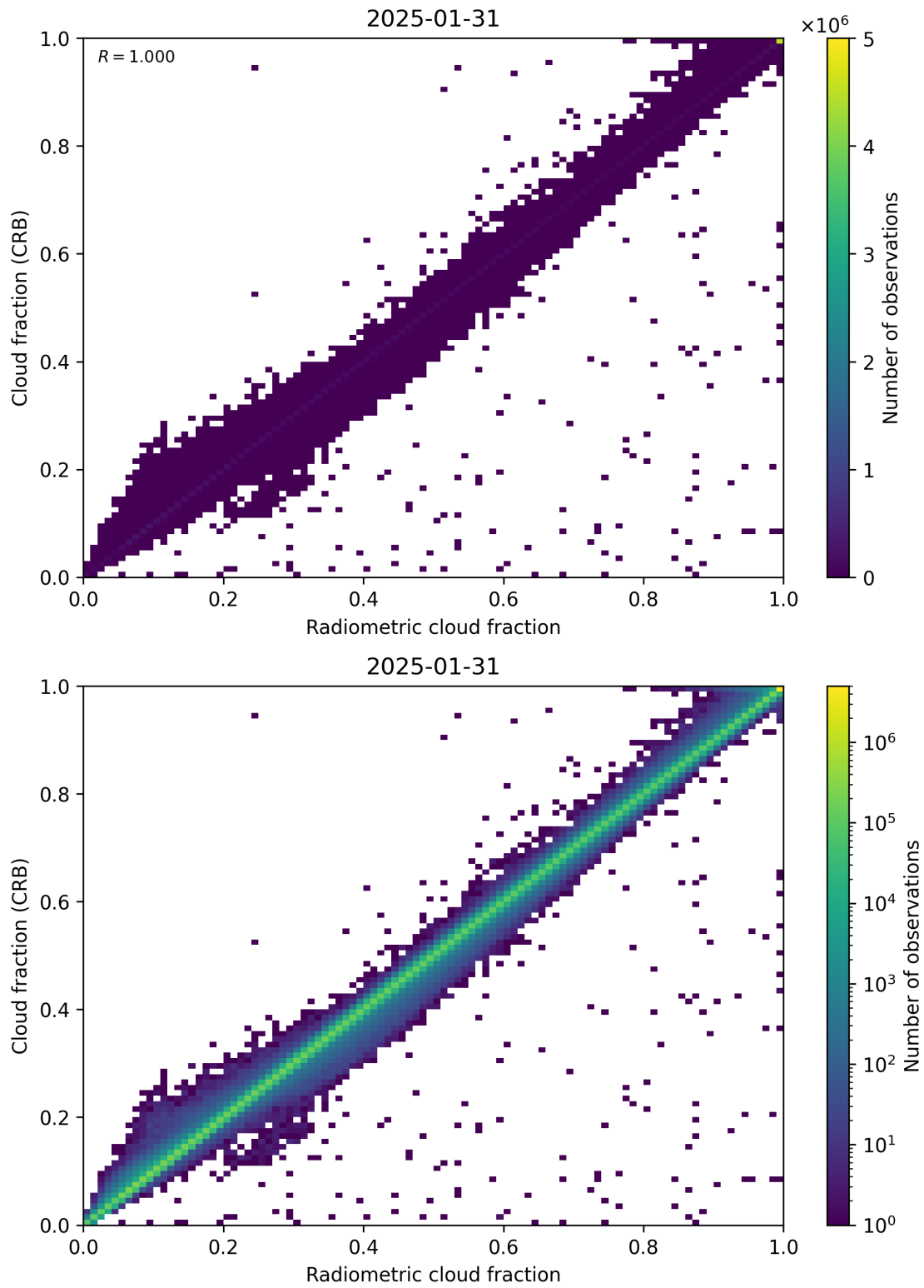
Figure 73: Scatter density plot of “Radiometric cloud fraction” against “Cloud fraction (CRB)” for 2025-01-30 to 2025-02-01.
