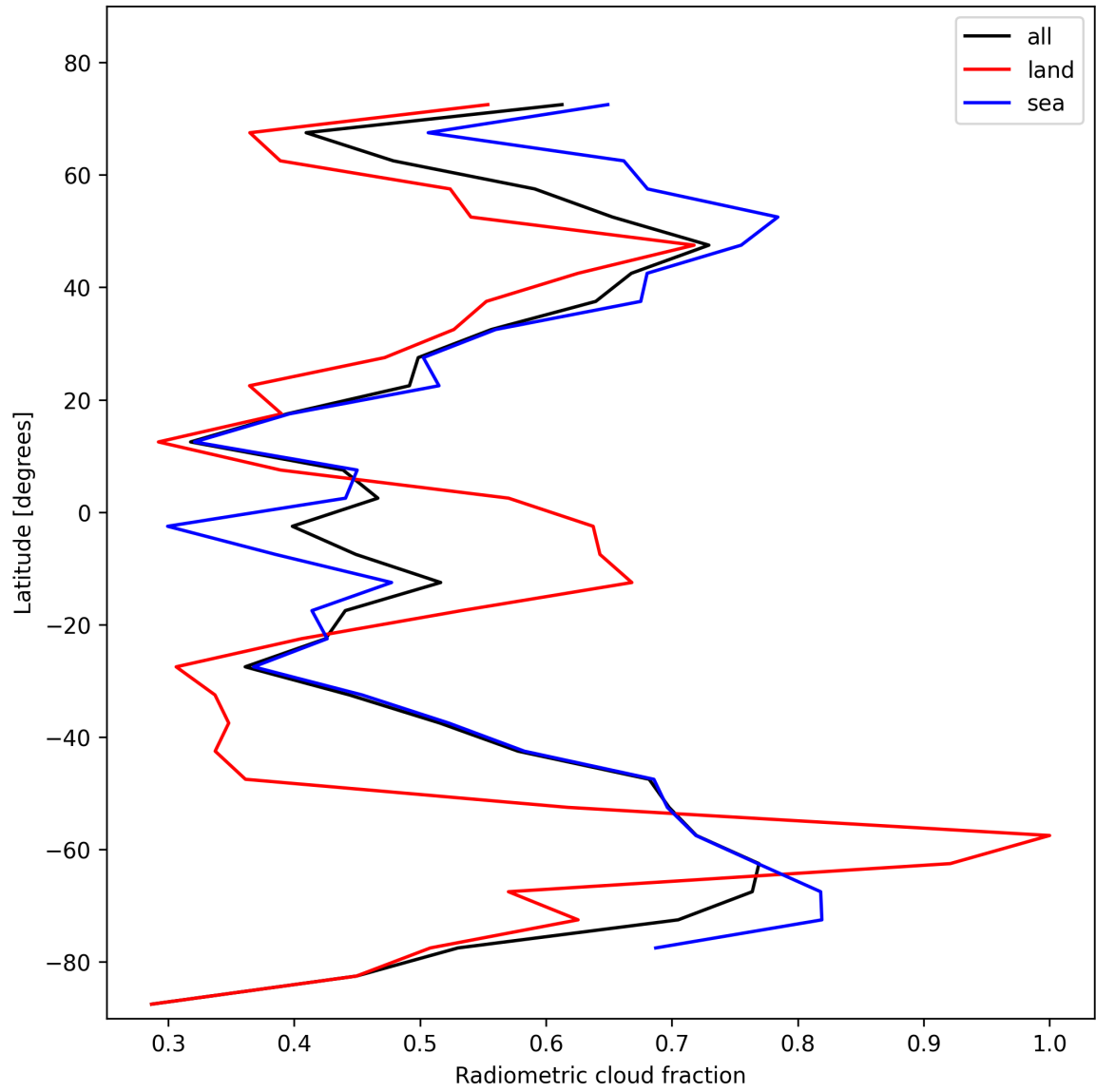
Figure 23: Zonal average of “Radiometric cloud fraction” for 2025-01-30 to 2025-02-01.
