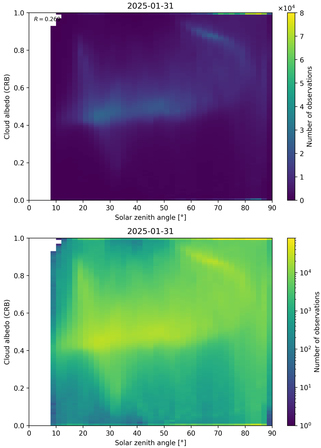
Figure 98: Scatter density plot of “Solar zenith angle” against “Cloud albedo (CRB)” for 2025-01-30 to 2025-02-01.
