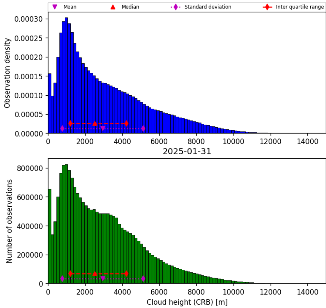
Figure 43: Histogram of “Cloud height (CRB)” for 2025-01-30 to 2025-02-01
