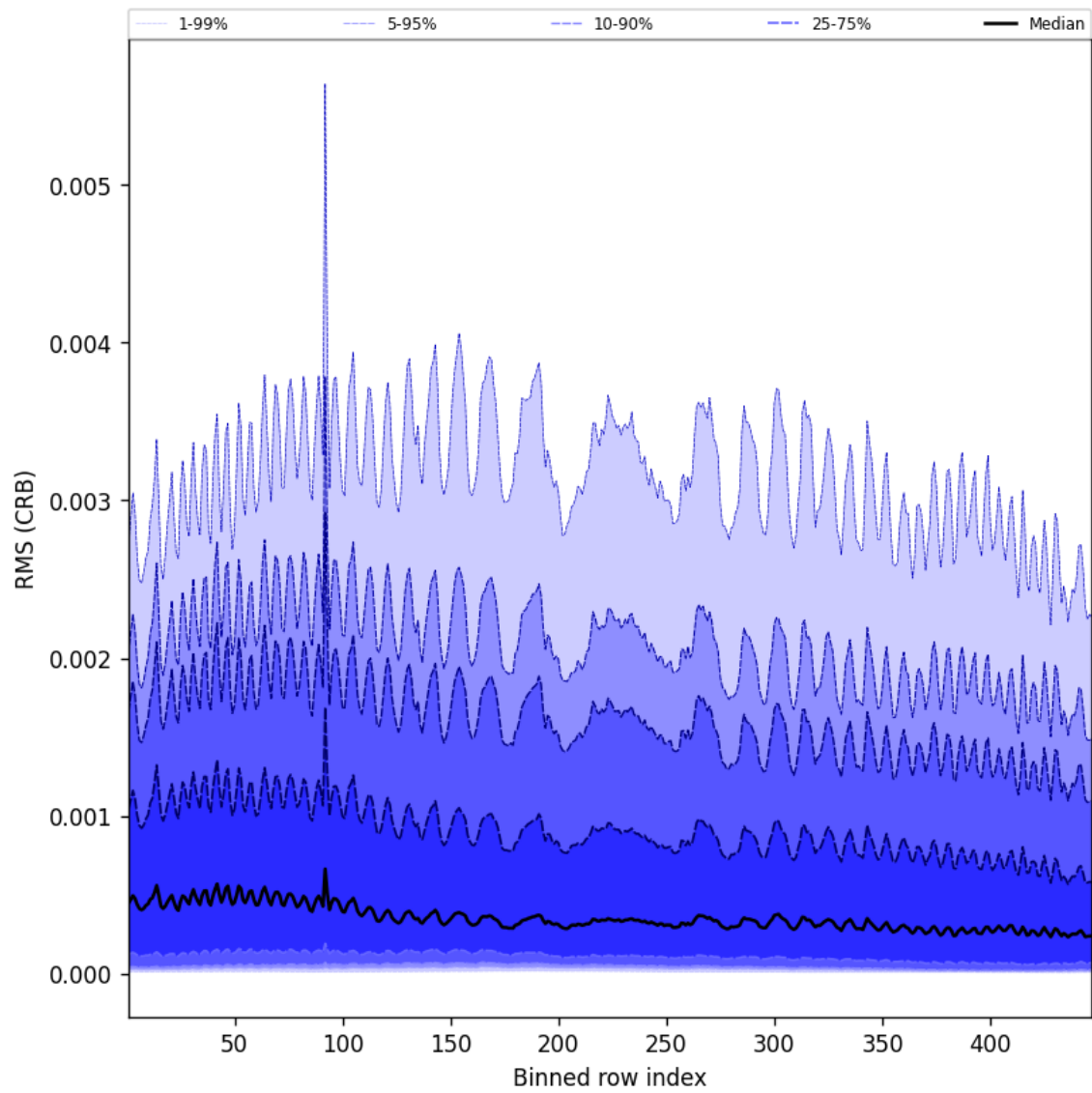
Figure 64: Along track statistics of “RMS (CRB)” for 2025-01-30 to 2025-02-01
