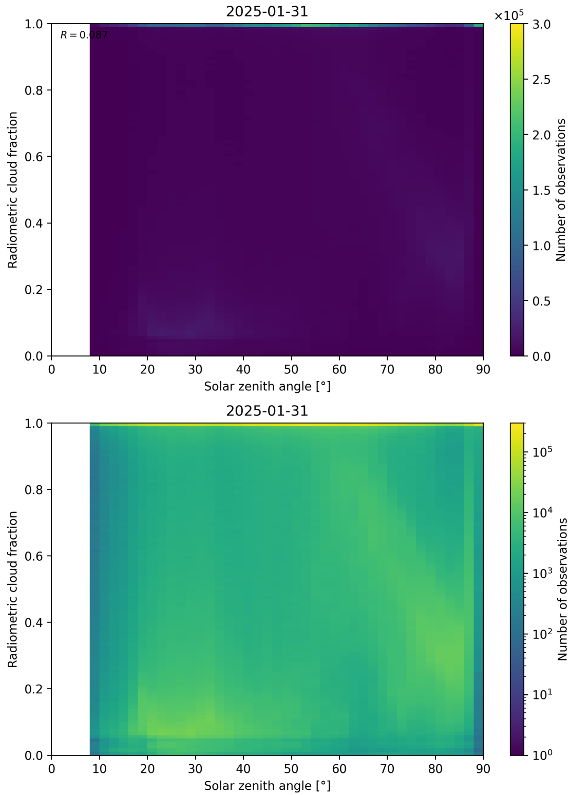
Figure 99: Scatter density plot of “Solar zenith angle” against “Radiometric cloud fraction” for 2025-01-30 to 2025-02-01.
