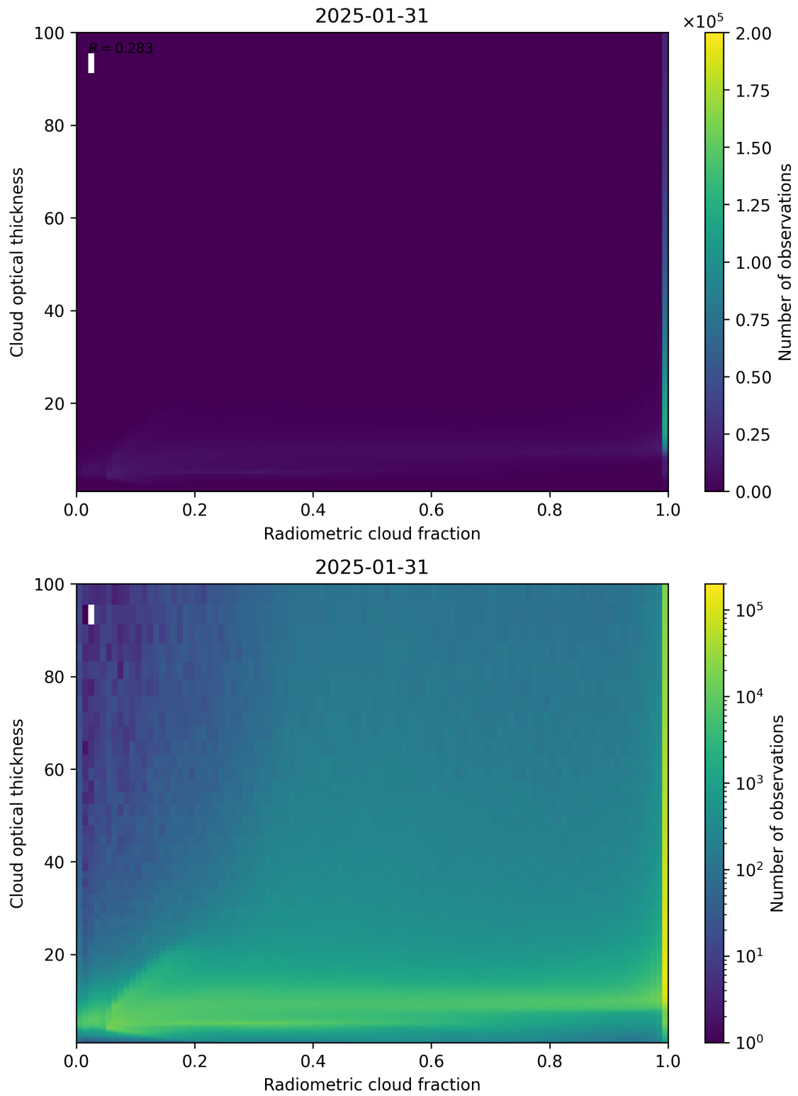
Figure 75: Scatter density plot of “Radiometric cloud fraction” against “Cloud optical thickness” for 2025-01-30 to 2025-02-01.
