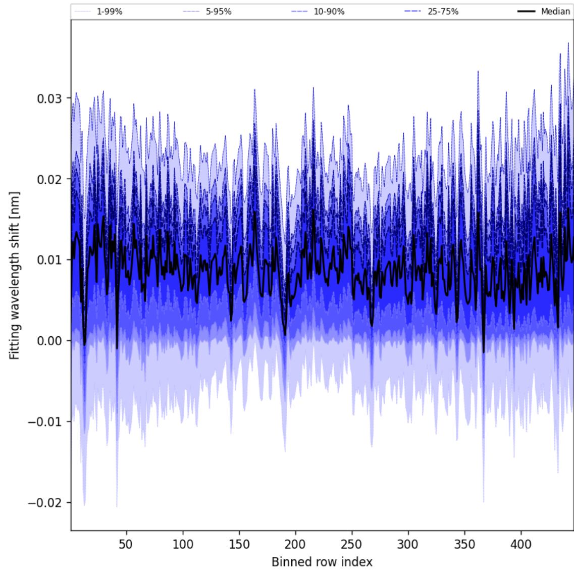
Figure 65: Along track statistics of “Fitting wavelength shift” for 2025-01-30 to 2025-02-01
