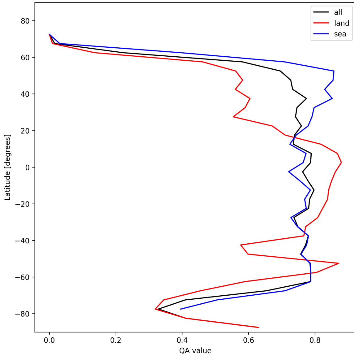
Figure 22: Zonal average of “QA value” for 2025-01-30 to 2025-02-01.
