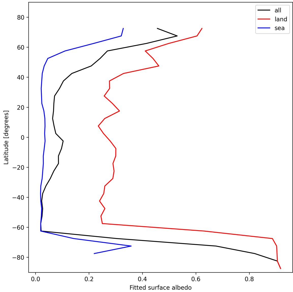
Figure 29: Zonal average of “Fitted surface albedo” for 2025-01-30 to 2025-02-01.
