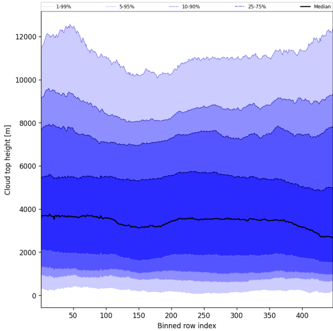
Figure 56: Along track statistics of “Cloud top height” for 2025-01-30 to 2025-02-01
