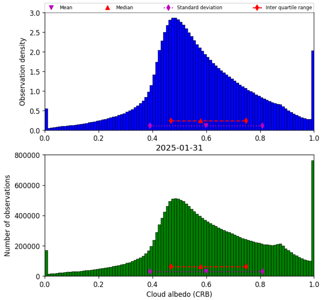
Figure 44: Histogram of “Cloud albedo (CRB)” for 2025-01-30 to 2025-02-01
