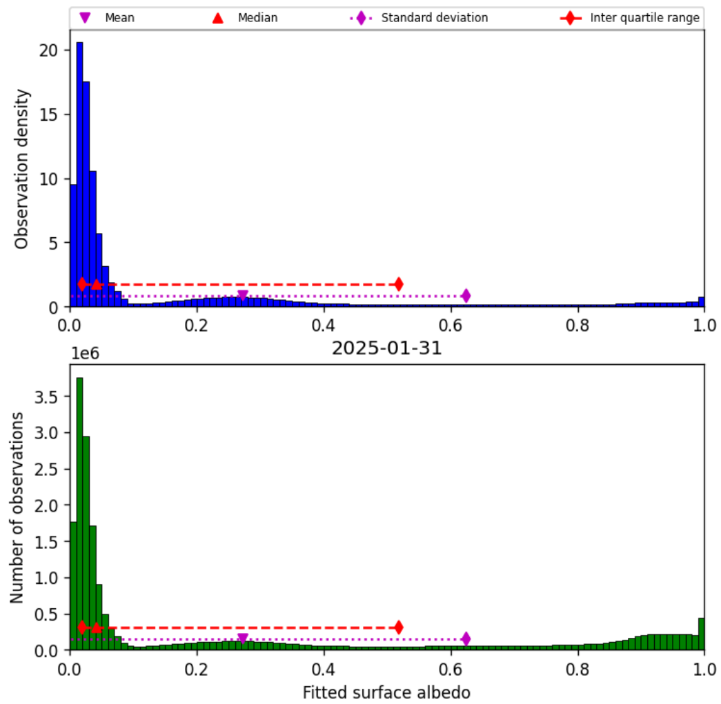
Figure 45: Histogram of “Fitted surface albedo” for 2025-01-30 to 2025-02-01
