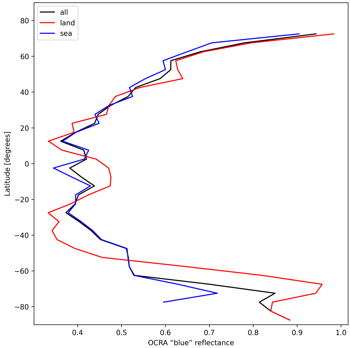
Figure 35: Zonal average of "OCRA "blue" reflectance" for 2025-01-30 to 2025-02-01.
