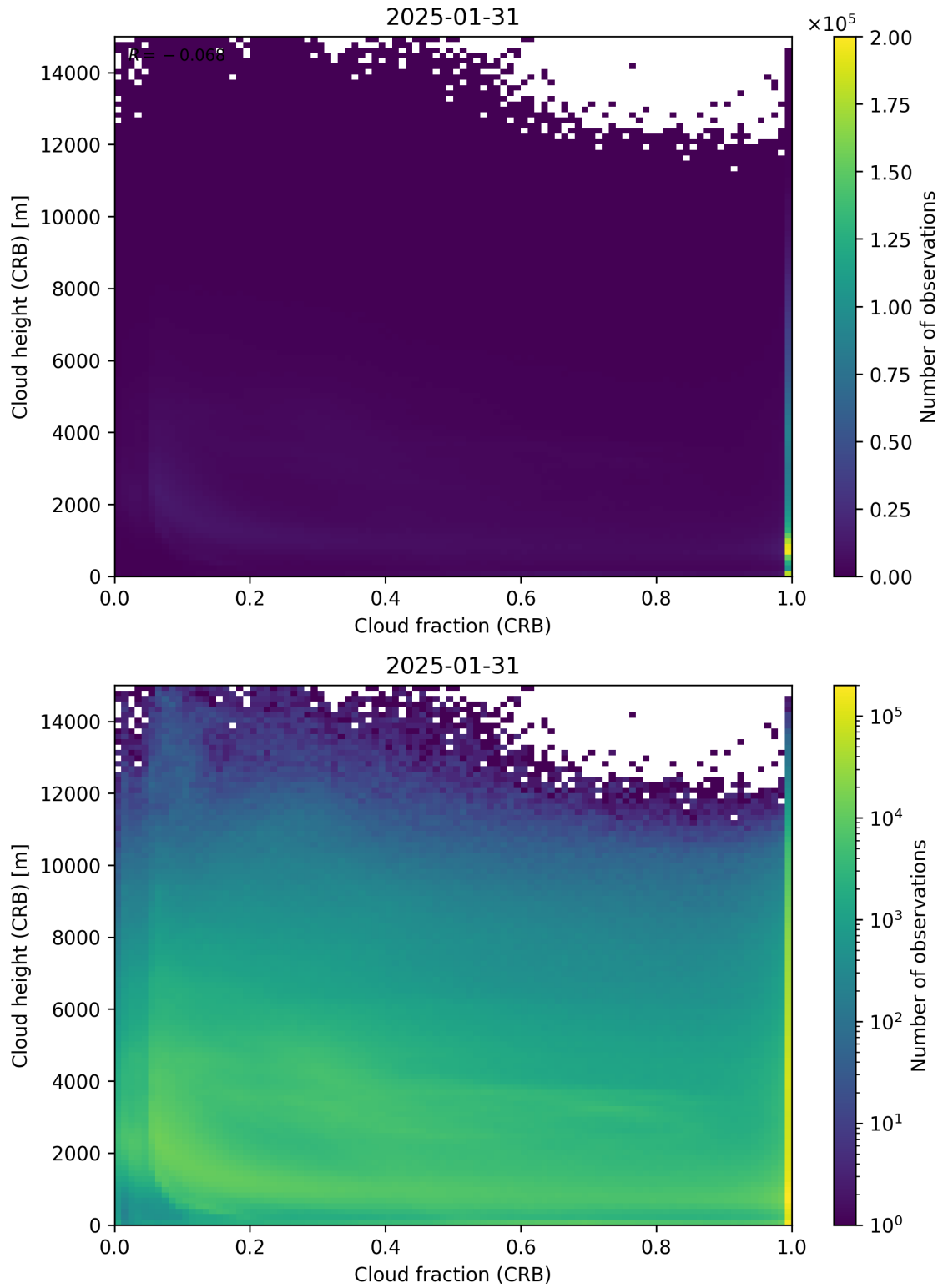
Figure 79: Scatter density plot of “Cloud fraction (CRB)” against “Cloud height (CRB)” for 2025-01-30 to 2025-02-01.
