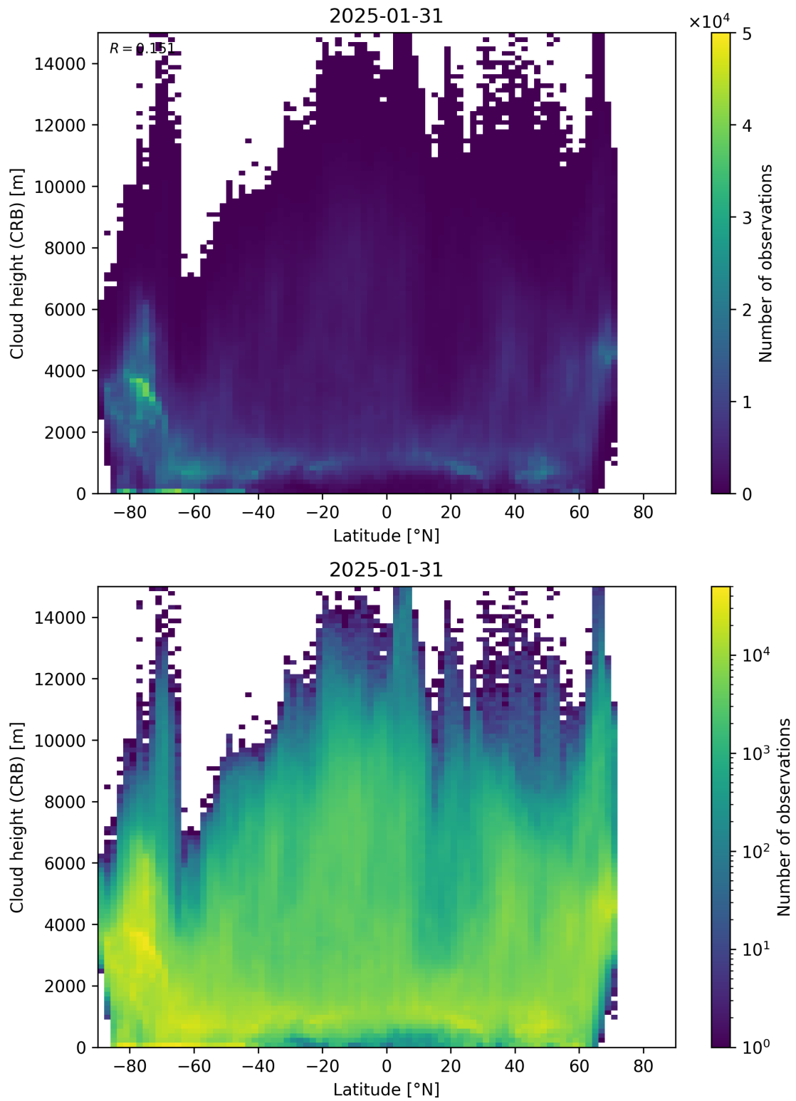
Figure 95: Scatter density plot of “Latitude” against “Cloud height (CRB)” for 2025-01-30 to 2025-02-01.
