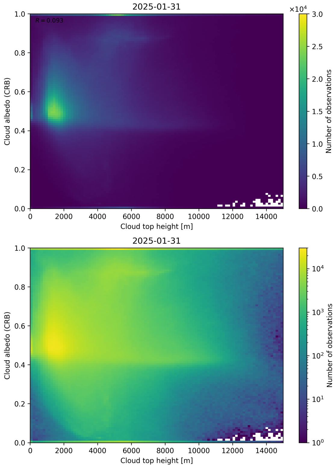
Figure 86: Scatter density plot of “Cloud top height” against “Cloud albedo (CRB)” for 2025-01-30 to 2025-02-01.
