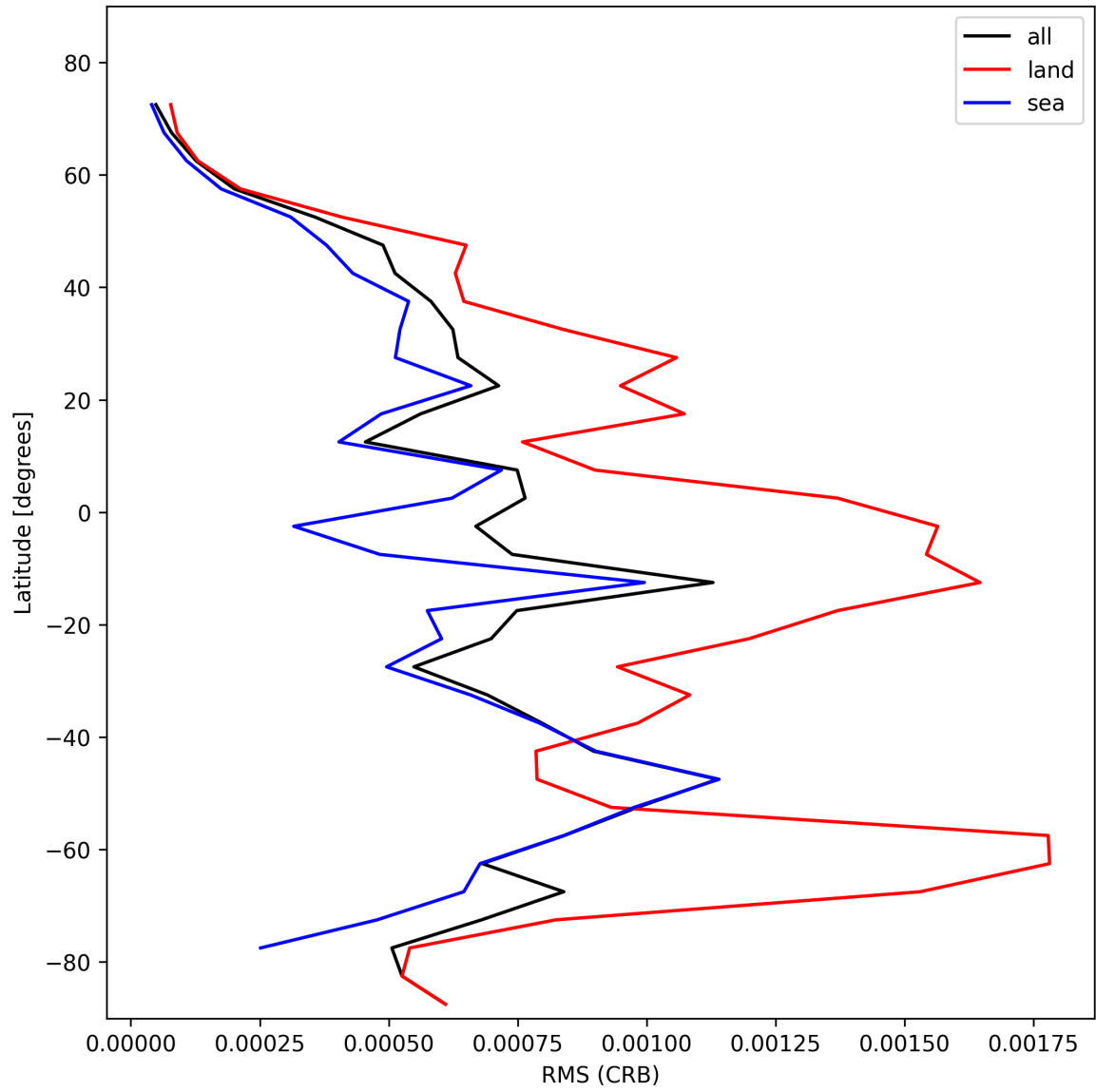
Figure 32: Zonal average of “RMS (CRB)” for 2025-01-30 to 2025-02-01.
