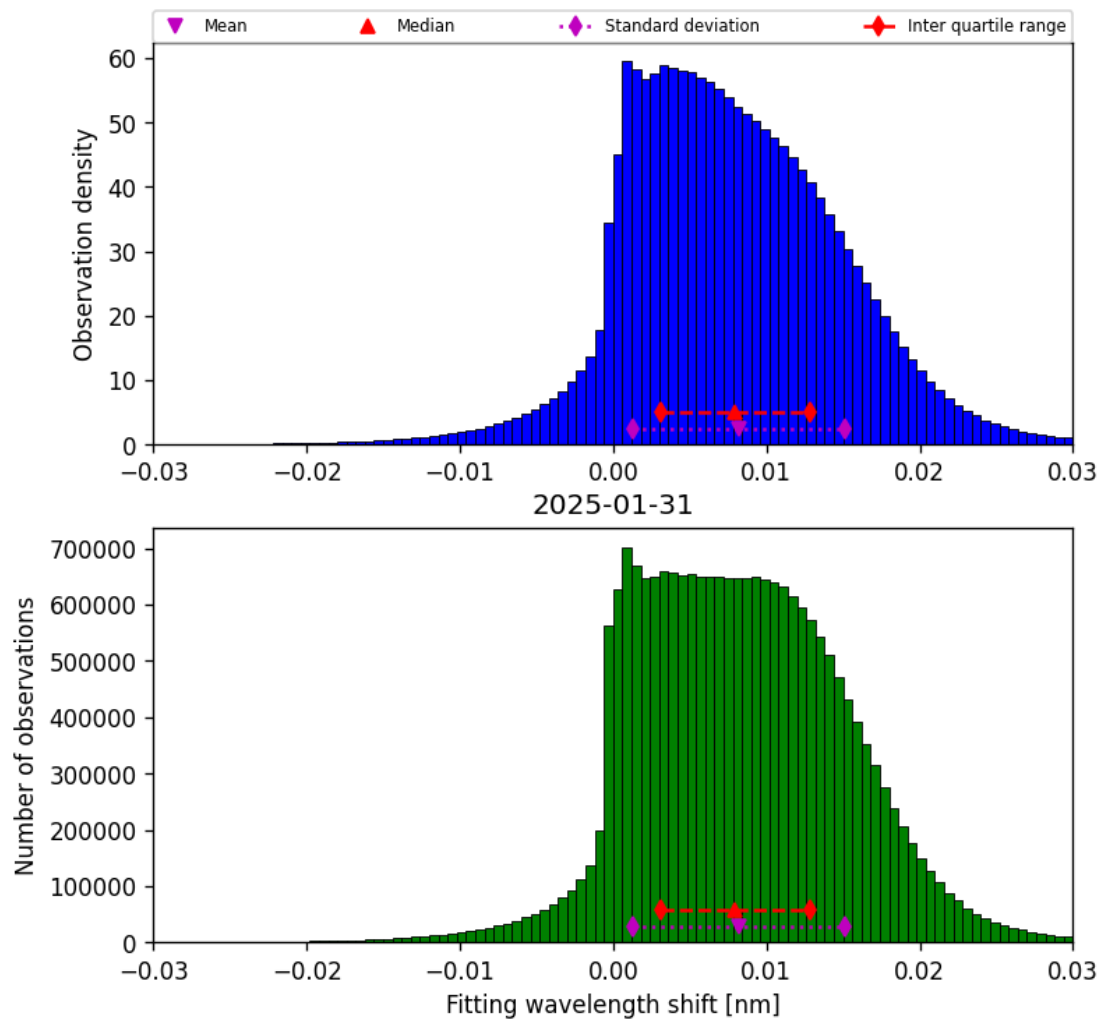
Figure 49: Histogram of “Fitting wavelength shift” for 2025-01-30 to 2025-02-01
