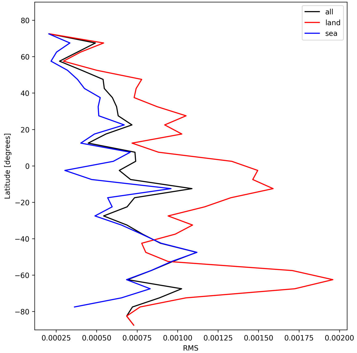
Figure 31: Zonal average of “RMS” for 2025-01-30 to 2025-02-01.
