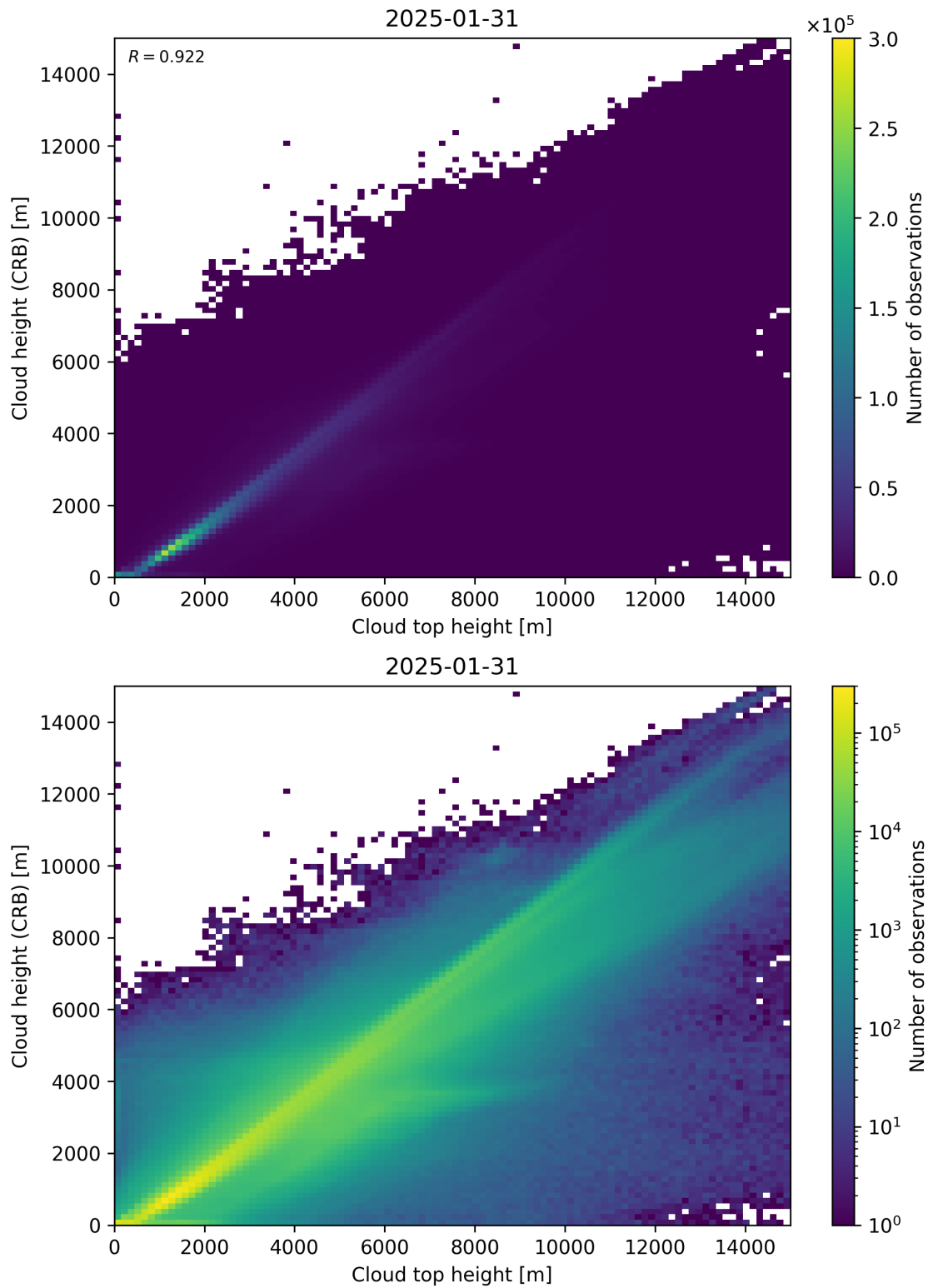
Figure 89: Scatter density plot of “Cloud top height” against “Cloud height (CRB)” for 2025-01-30 to 2025-02-01.
