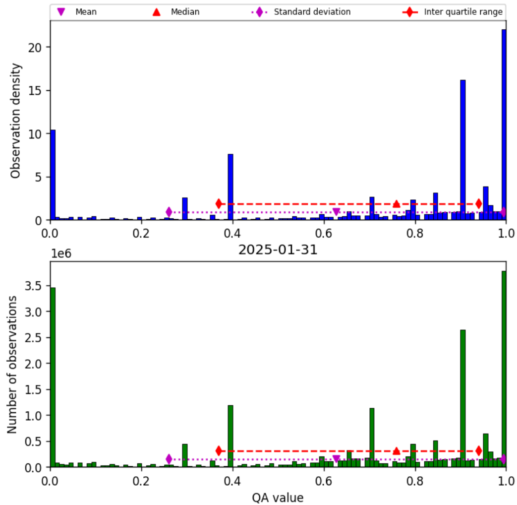
Figure 38: Histogram of “QA value” for 2025-01-30 to 2025-02-01
