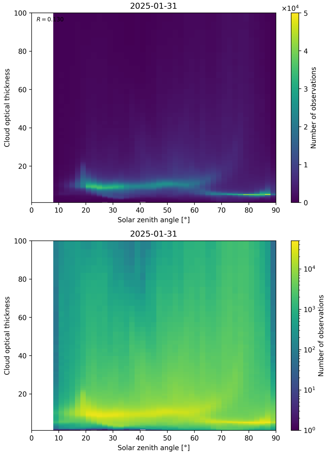
Figure 103: Scatter density plot of “Solar zenith angle” against “Cloud optical thickness” for 2025-01-30 to 2025-02-01.
