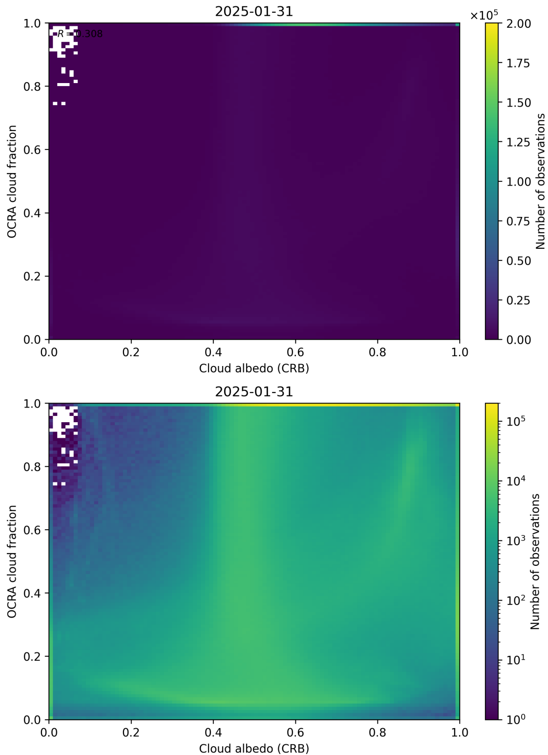
Figure 70: Scatter density plot of “Cloud albedo (CRB)” against “OCRA cloud fraction” for 2025-01-30 to 2025-02-01.
