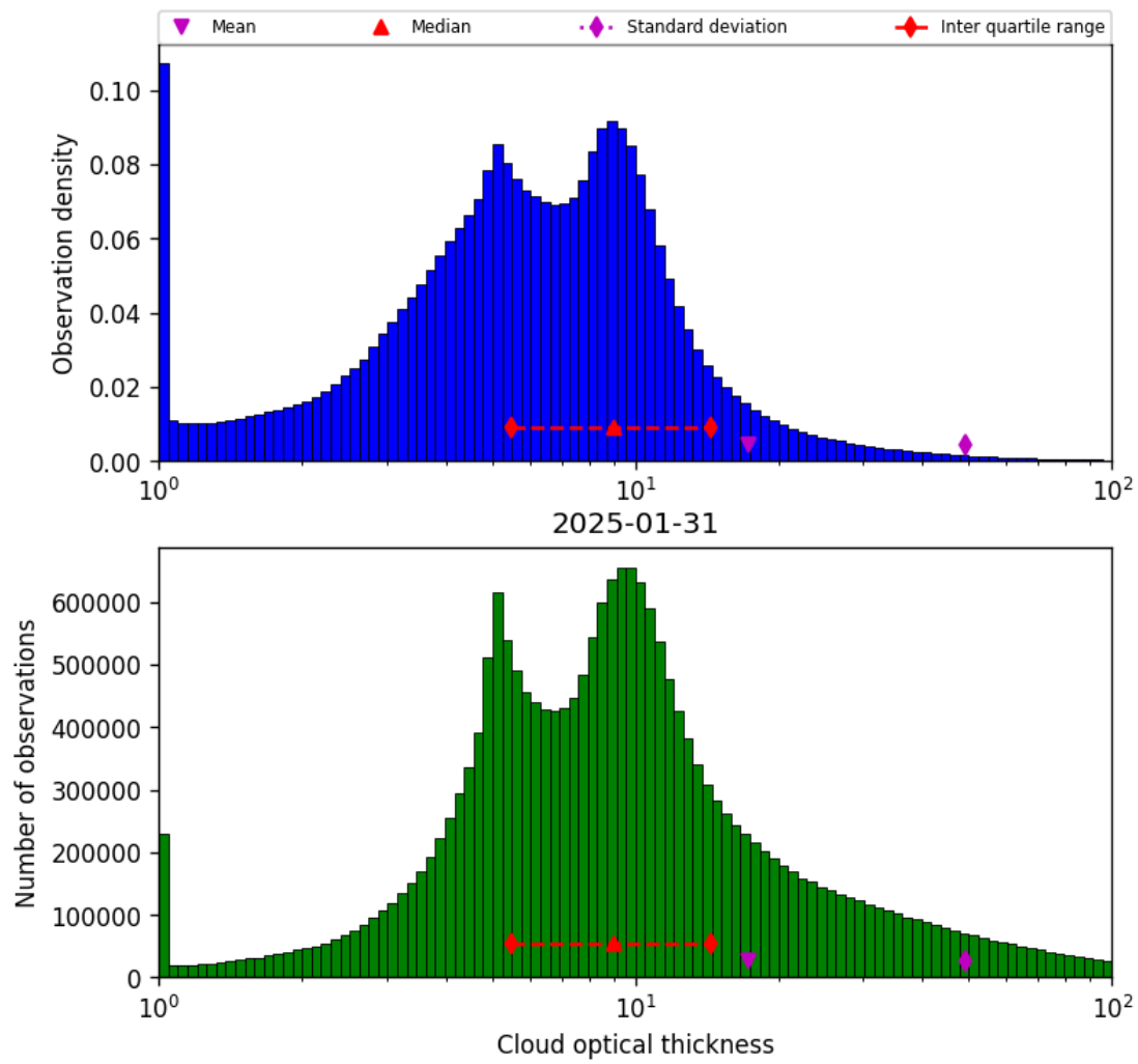
Figure 41: Histogram of “Cloud optical thickness” for 2025-01-30 to 2025-02-01
