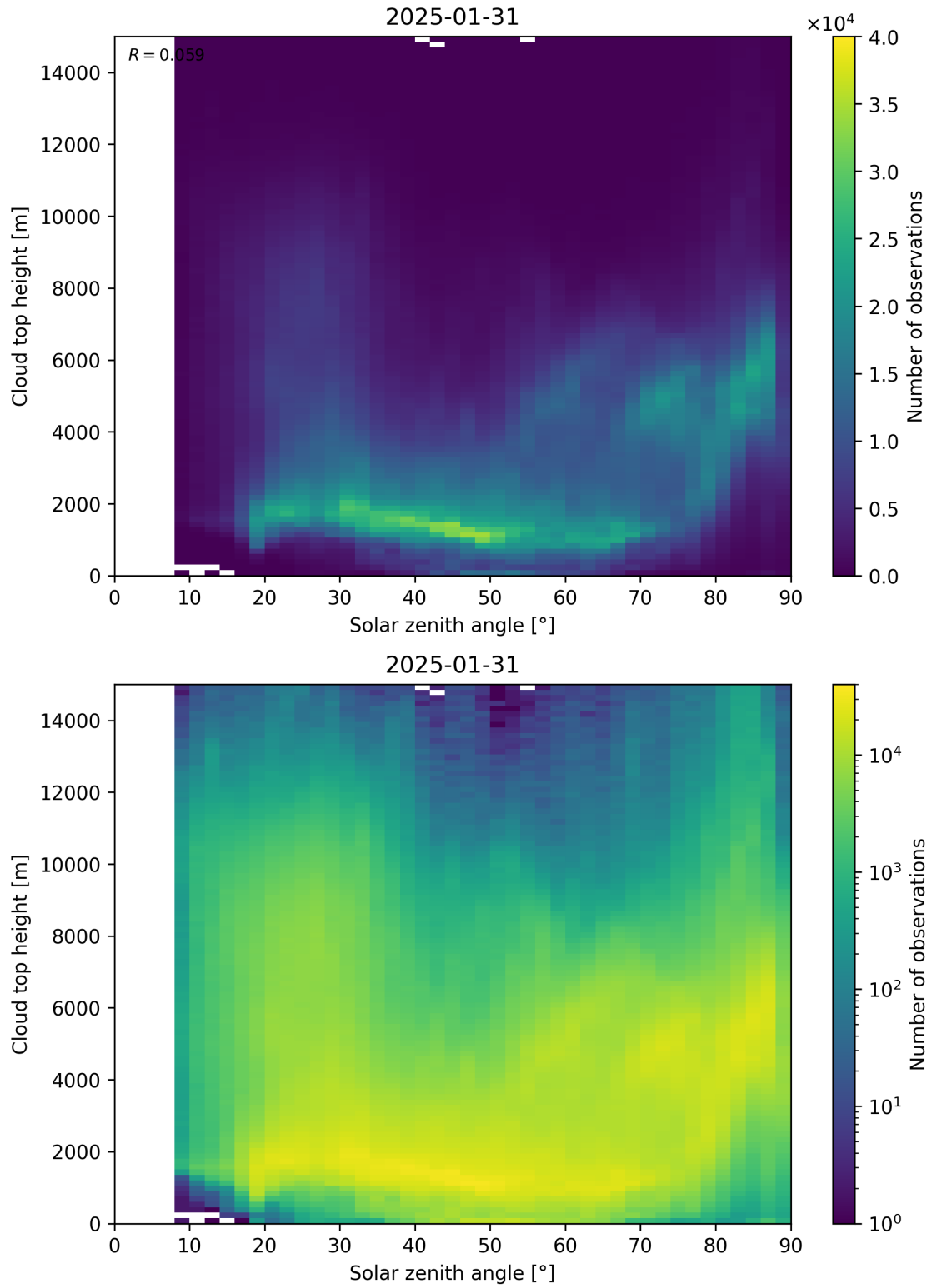
Figure 104: Scatter density plot of “Solar zenith angle” against “Cloud top height” for 2025-01-30 to 2025-02-01.
