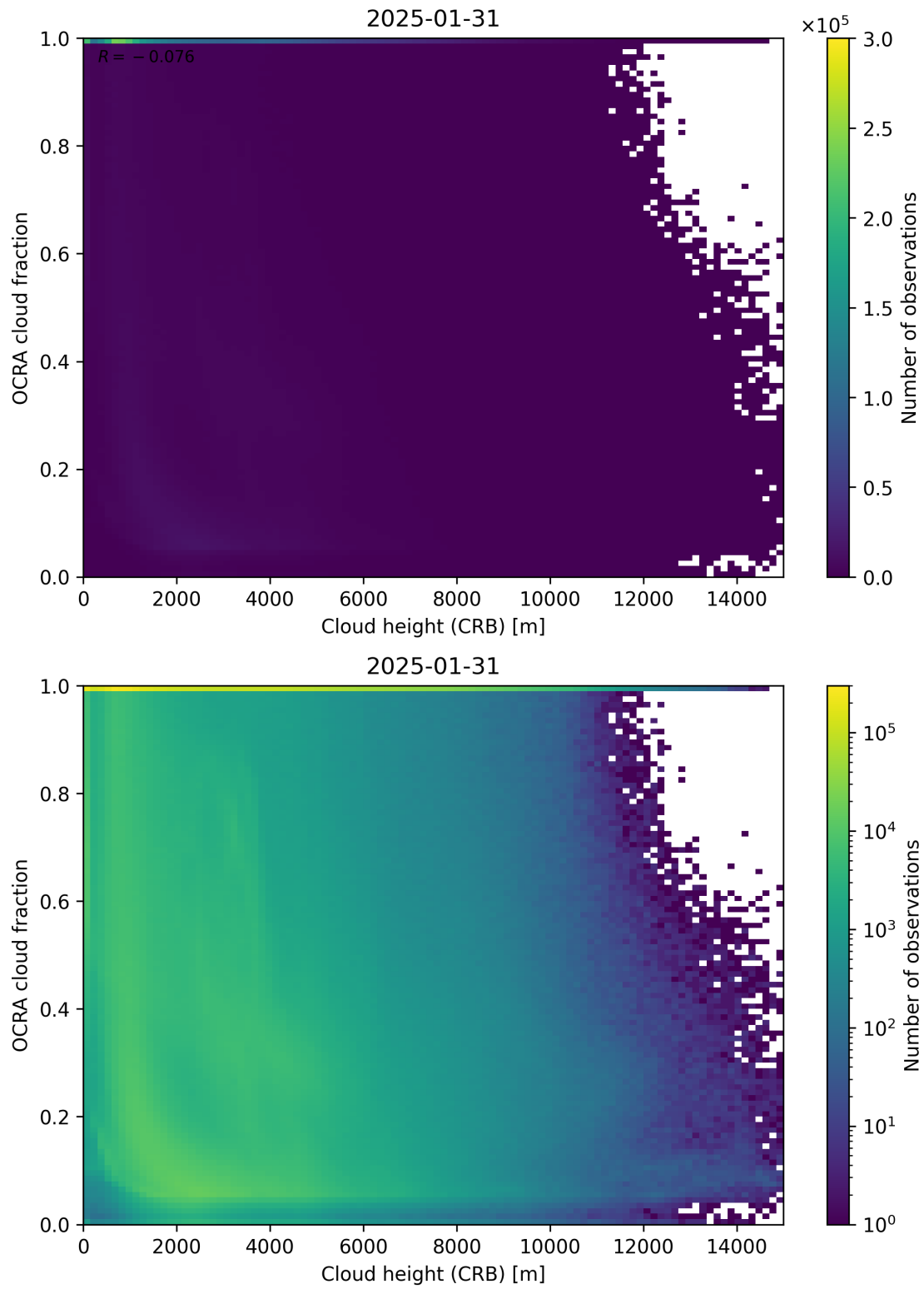
Figure 81: Scatter density plot of “Cloud height (CRB)” against “OCRA cloud fraction” for 2025-01-30 to 2025-02-01.
