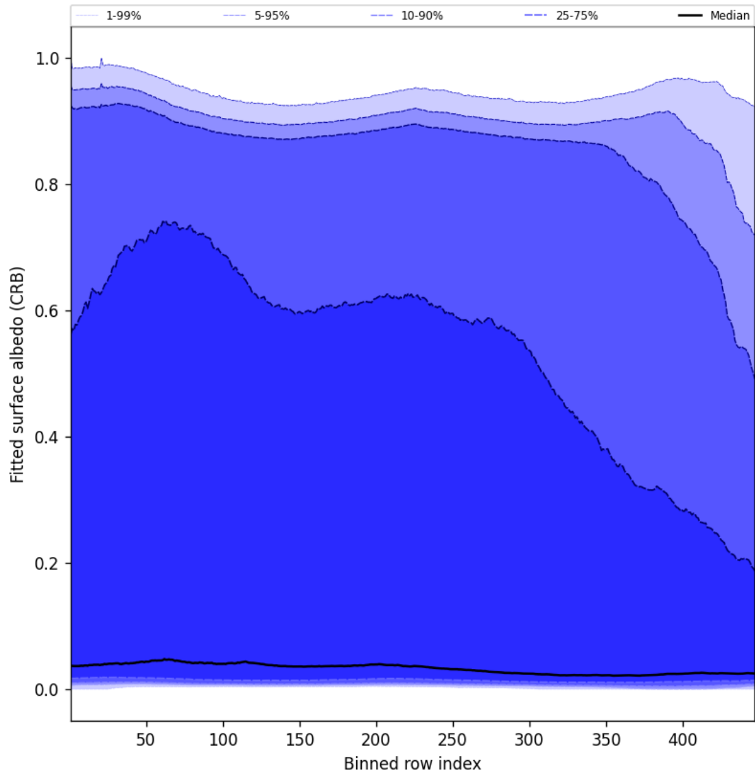
Figure 62: Along track statistics of “Fitted surface albedo (CRB)” for 2025-01-30 to 2025-02-01
