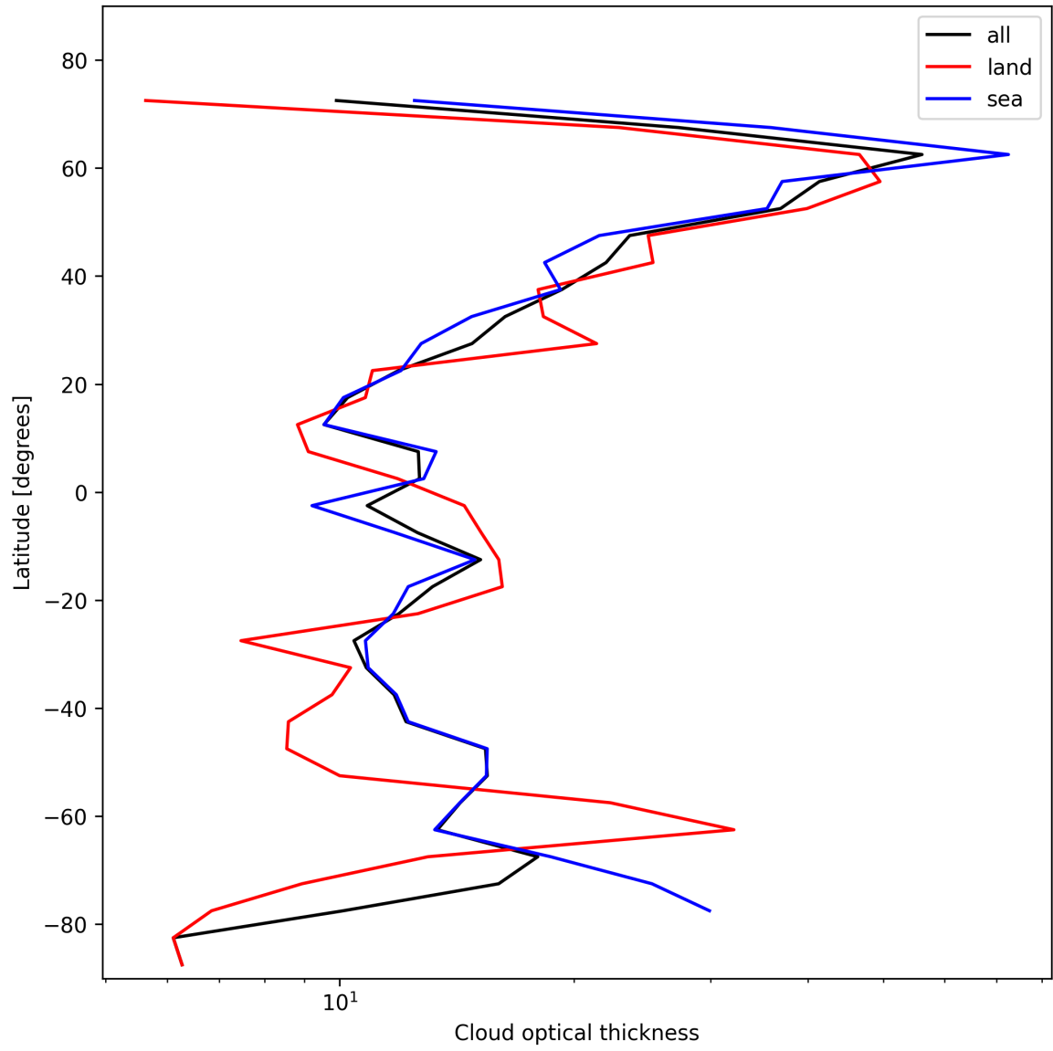
Figure 25: Zonal average of “Cloud optical thickness” for 2025-01-30 to 2025-02-01.
