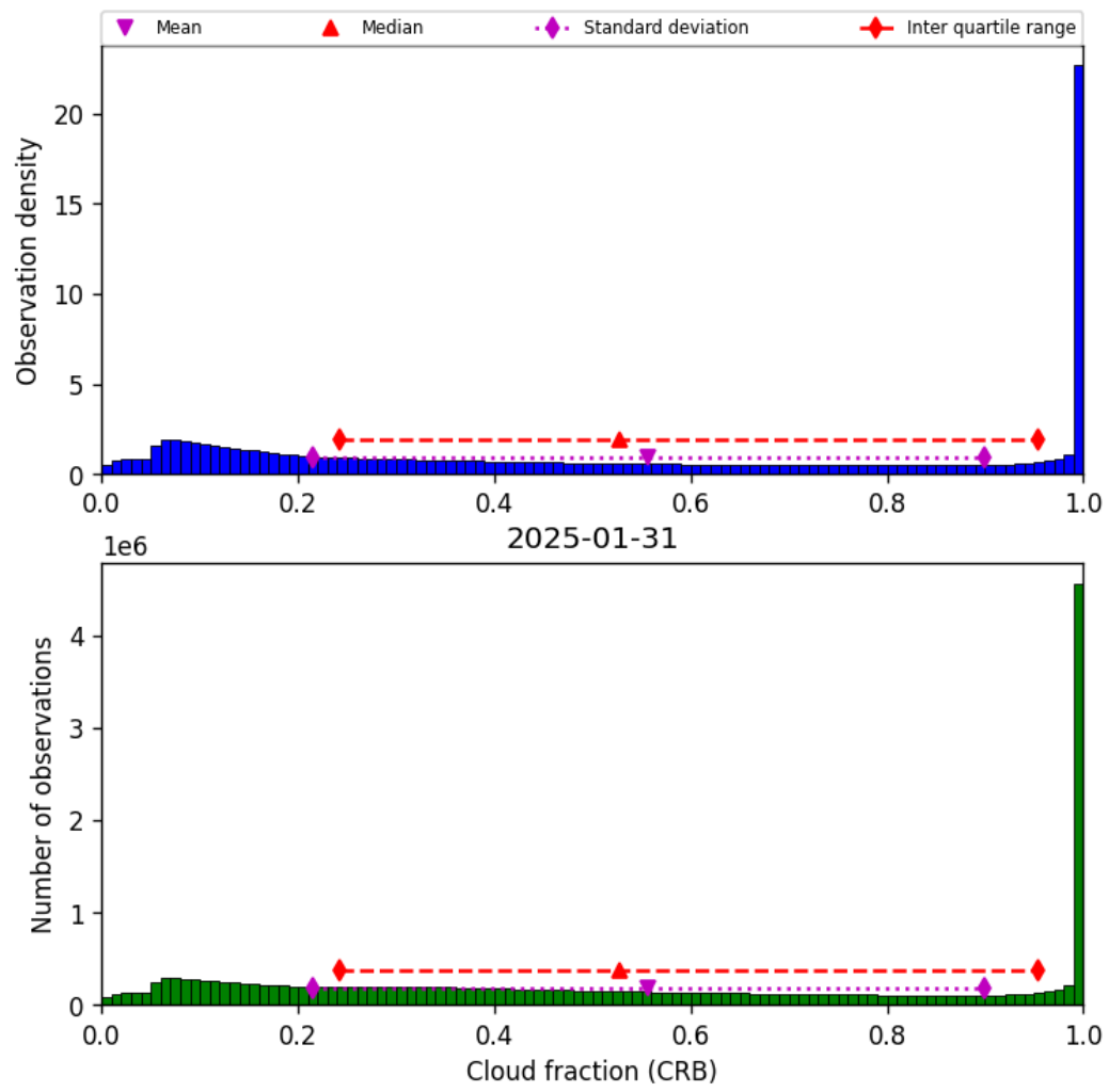
Figure 42: Histogram of “Cloud fraction (CRB)” for 2025-01-30 to 2025-02-01
