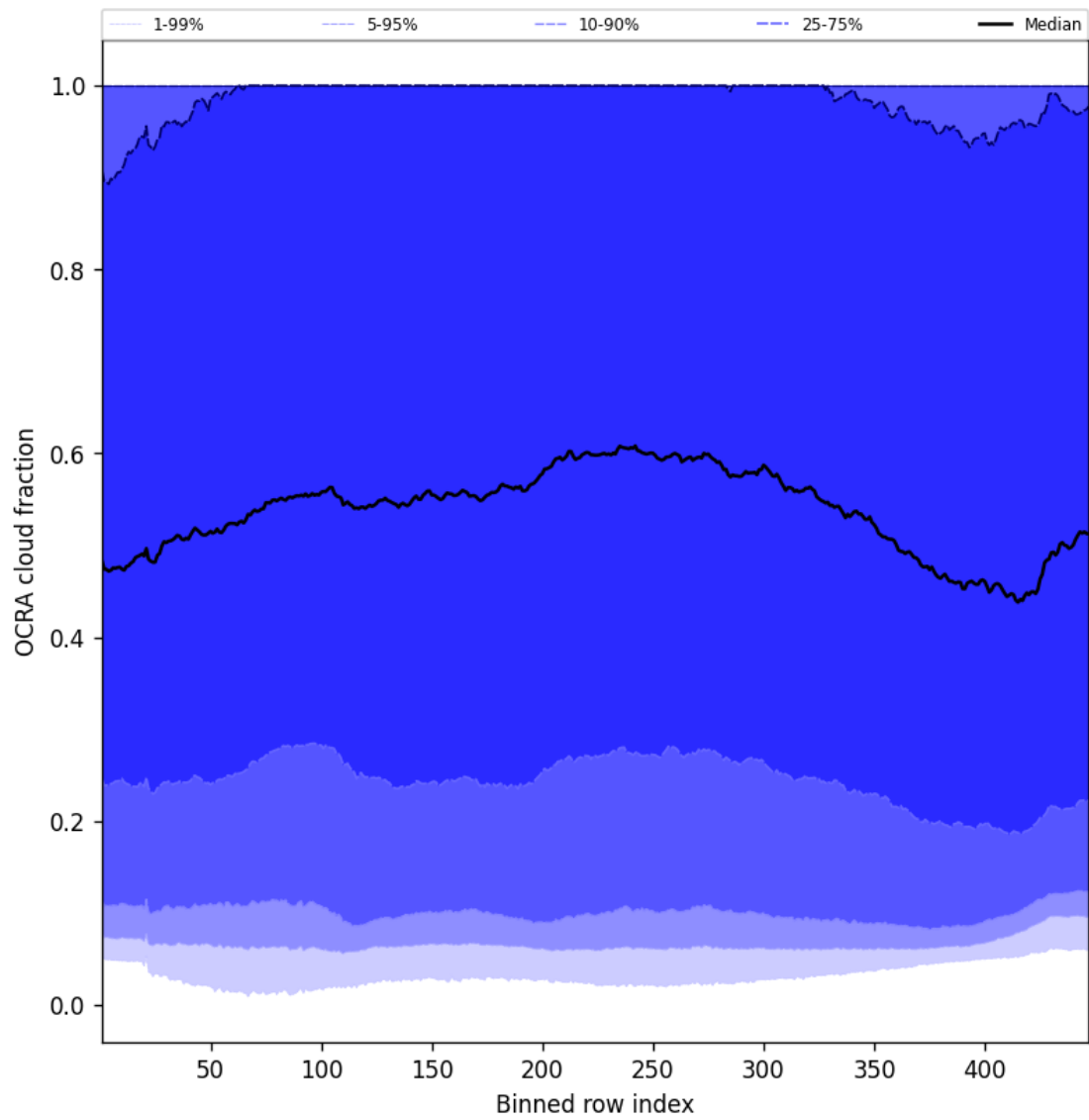
Figure 66: Along track statistics of “OCRA cloud fraction” for 2025-01-30 to 2025-02-01
