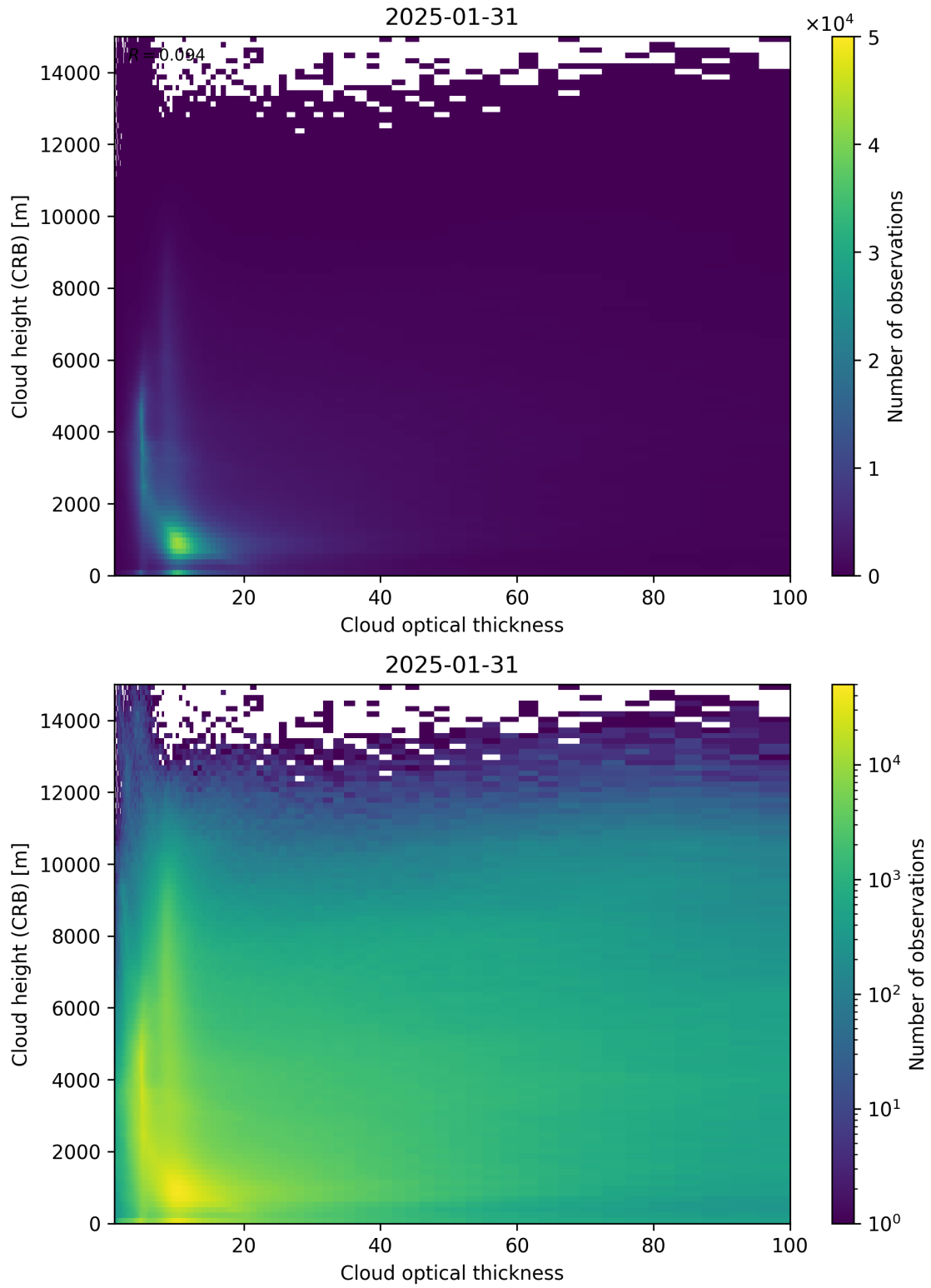
Figure 85: Scatter density plot of “Cloud optical thickness” against “Cloud height (CRB)” for 2025-01-30 to 2025-02-01.
