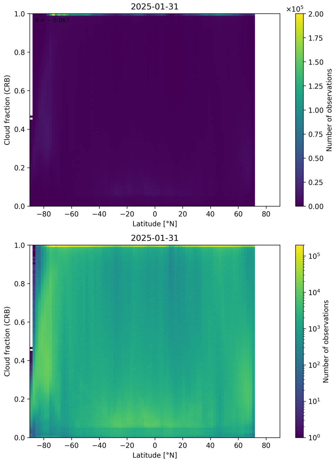
Figure 94: Scatter density plot of “Latitude” against “Cloud fraction (CRB)” for 2025-01-30 to 2025-02-01.
