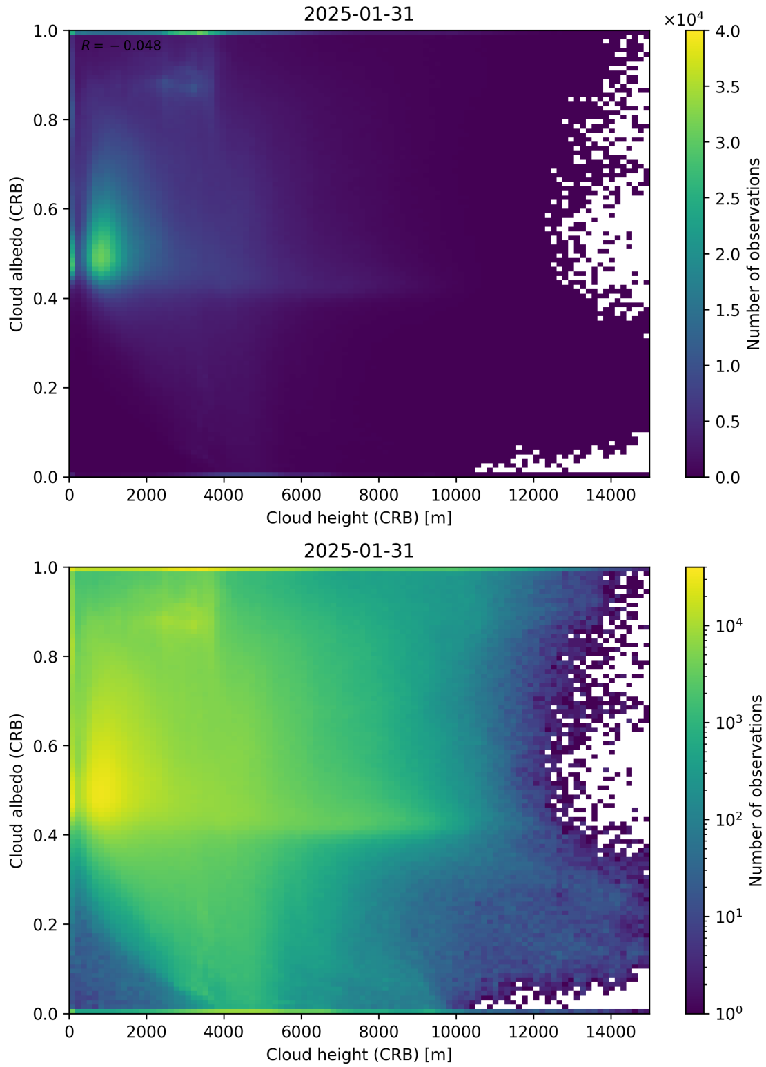
Figure 80: Scatter density plot of “Cloud height (CRB)” against “Cloud albedo (CRB)” for 2025-01-30 to 2025-02-01.
