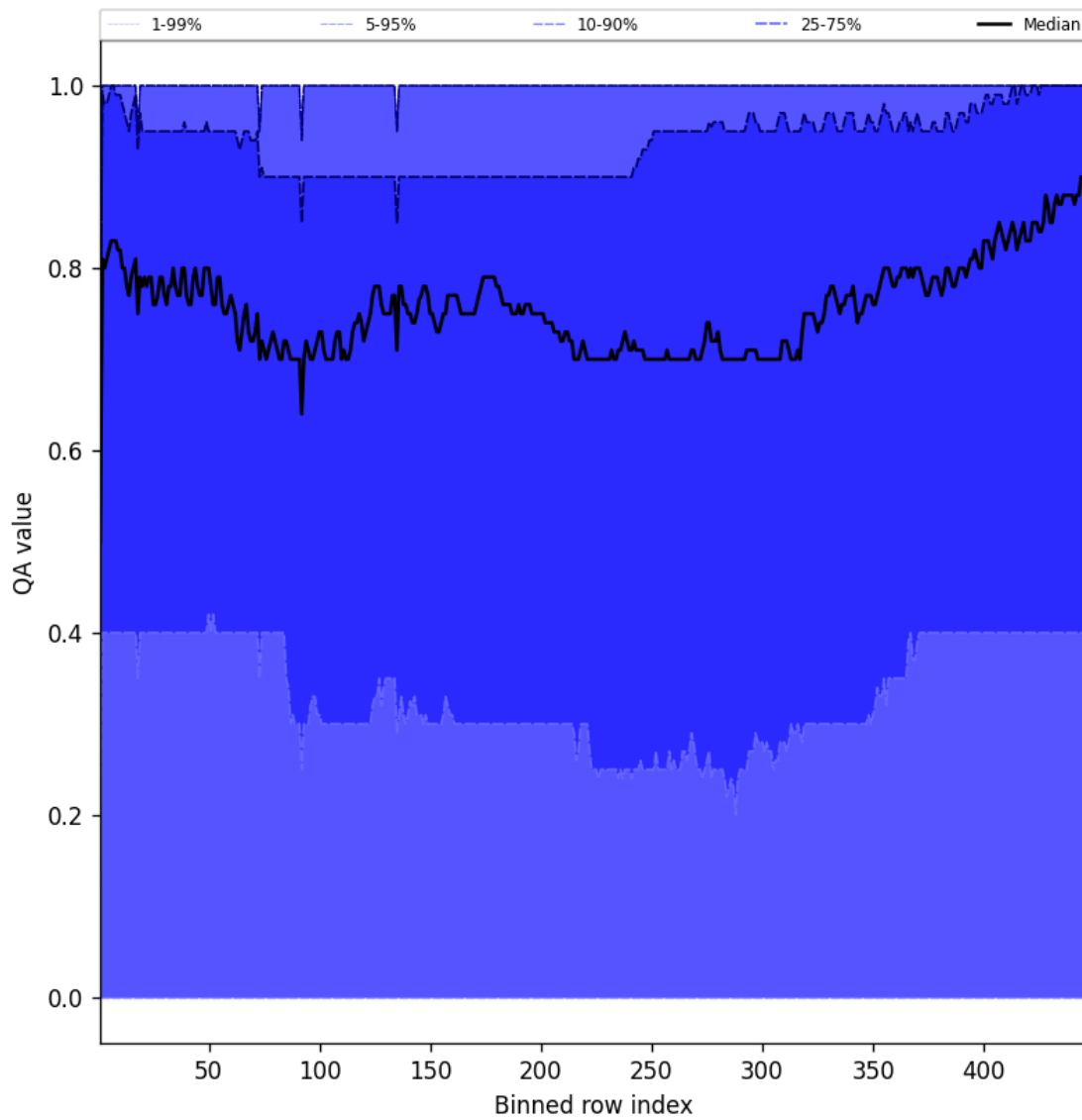
Figure 54: Along track statistics of “QA value” for 2025-01-30 to 2025-02-01
