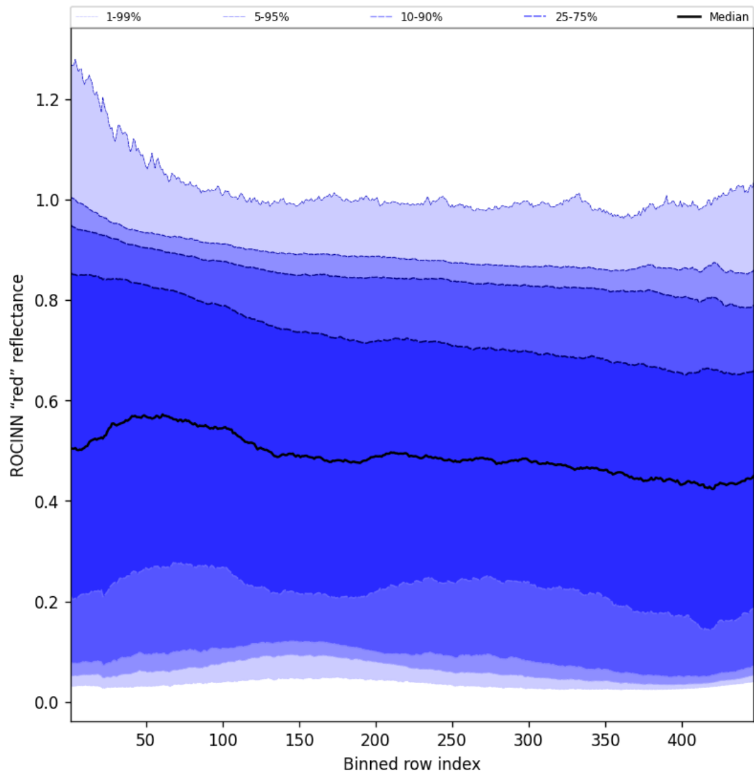
Figure 69: Along track statistics of "ROCINN "red" reflectance" for 2025-01-30 to 2025-02-01
