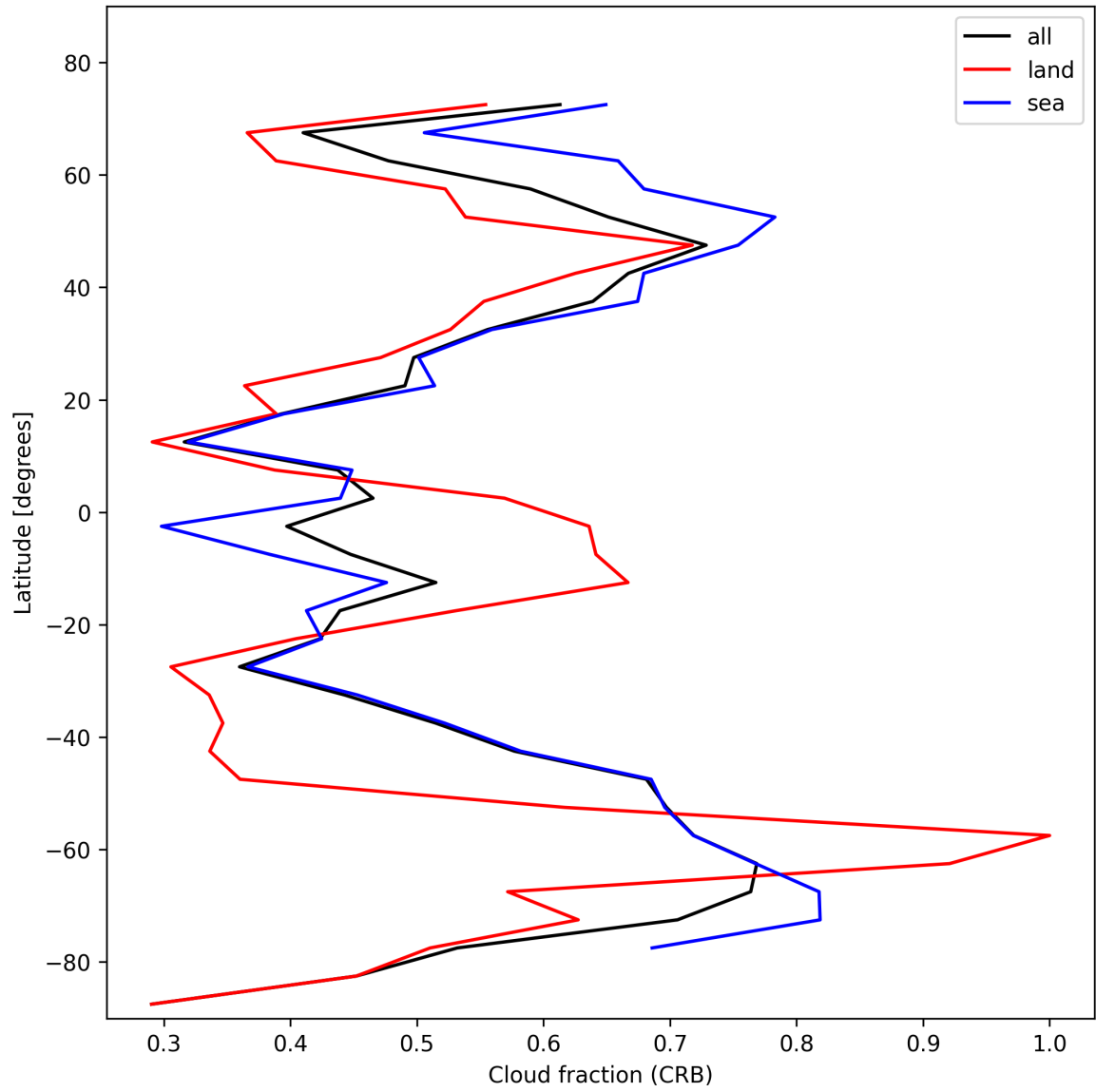
Figure 26: Zonal average of “Cloud fraction (CRB)” for 2025-01-30 to 2025-02-01.
