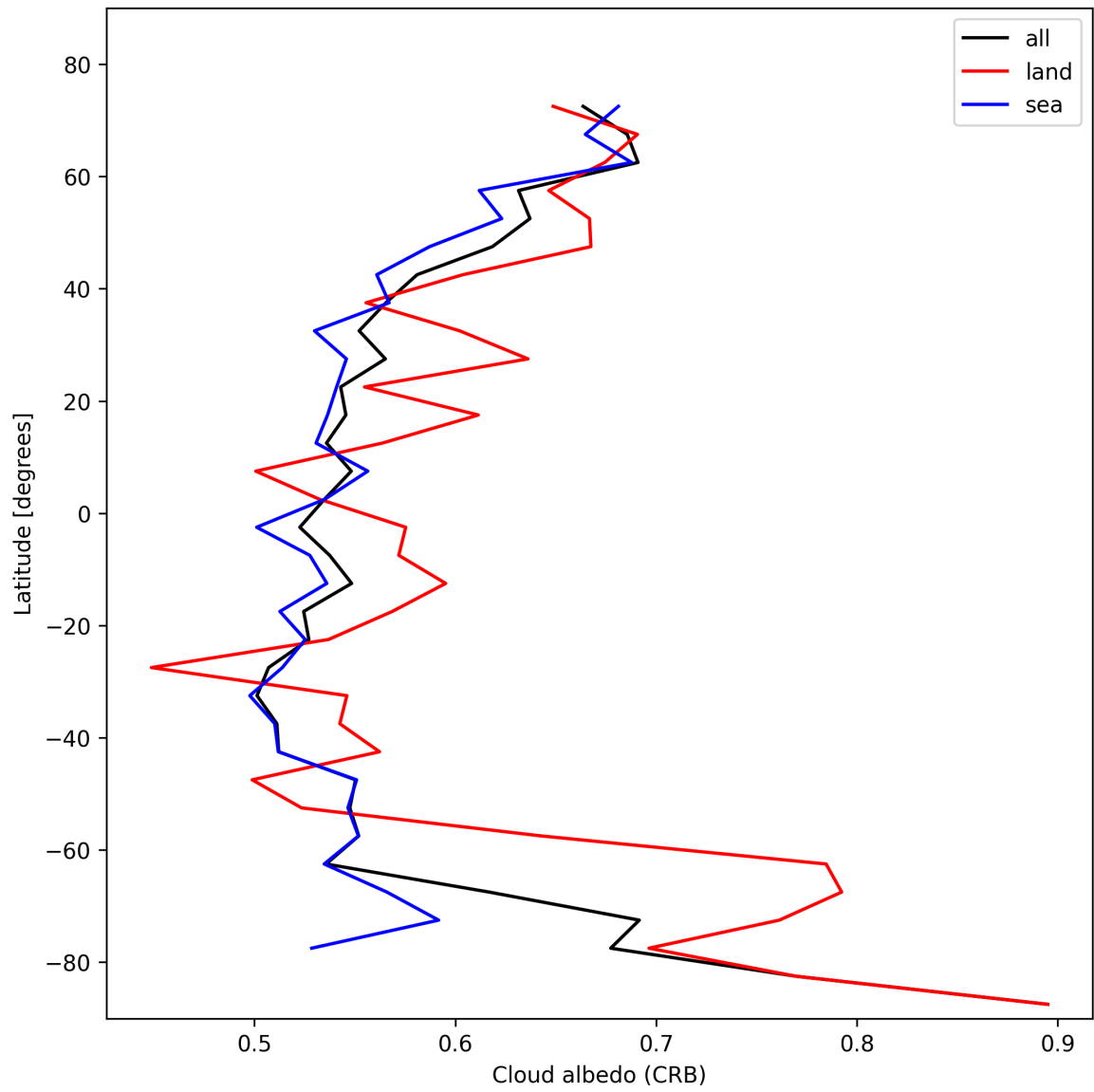
Figure 28: Zonal average of “Cloud albedo (CRB)” for 2025-01-30 to 2025-02-01.
