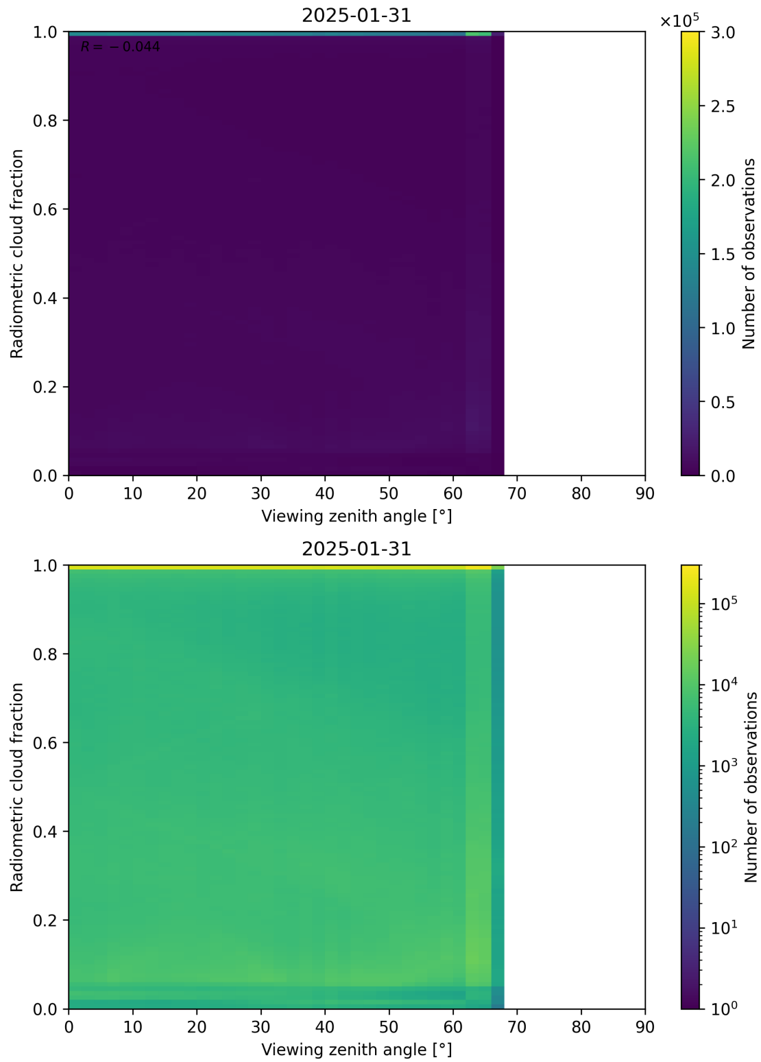
Figure 107: Scatter density plot of “Viewing zenith angle” against “Radiometric cloud fraction” for 2025-01-30 to 2025-02-01.
