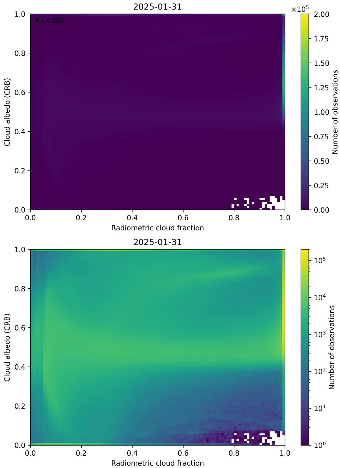
Figure 71: Scatter density plot of “Radiometric cloud fraction” against “Cloud albedo (CRB)” for 2025-01-30 to 2025-02-01.
