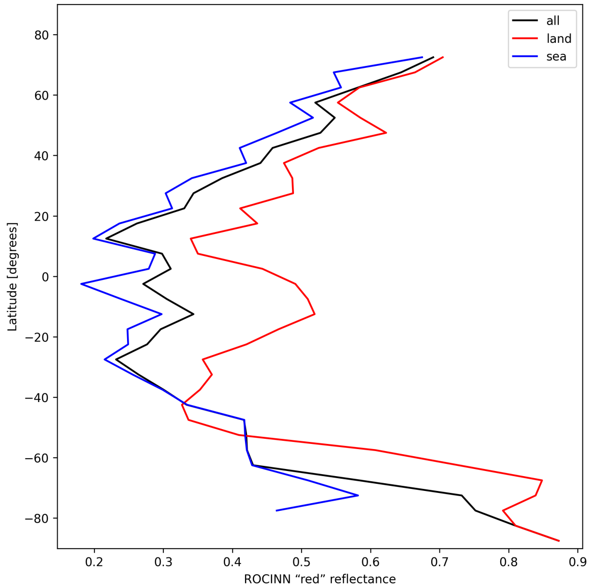
Figure 37: Zonal average of “ROCINN “red” reflectance” for 2025-01-30 to 2025-02-01.
