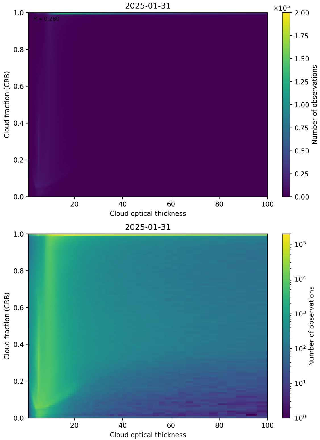
Figure 84: Scatter density plot of “Cloud optical thickness” against “Cloud fraction (CRB)” for 2025-01-30 to 2025-02-01.
