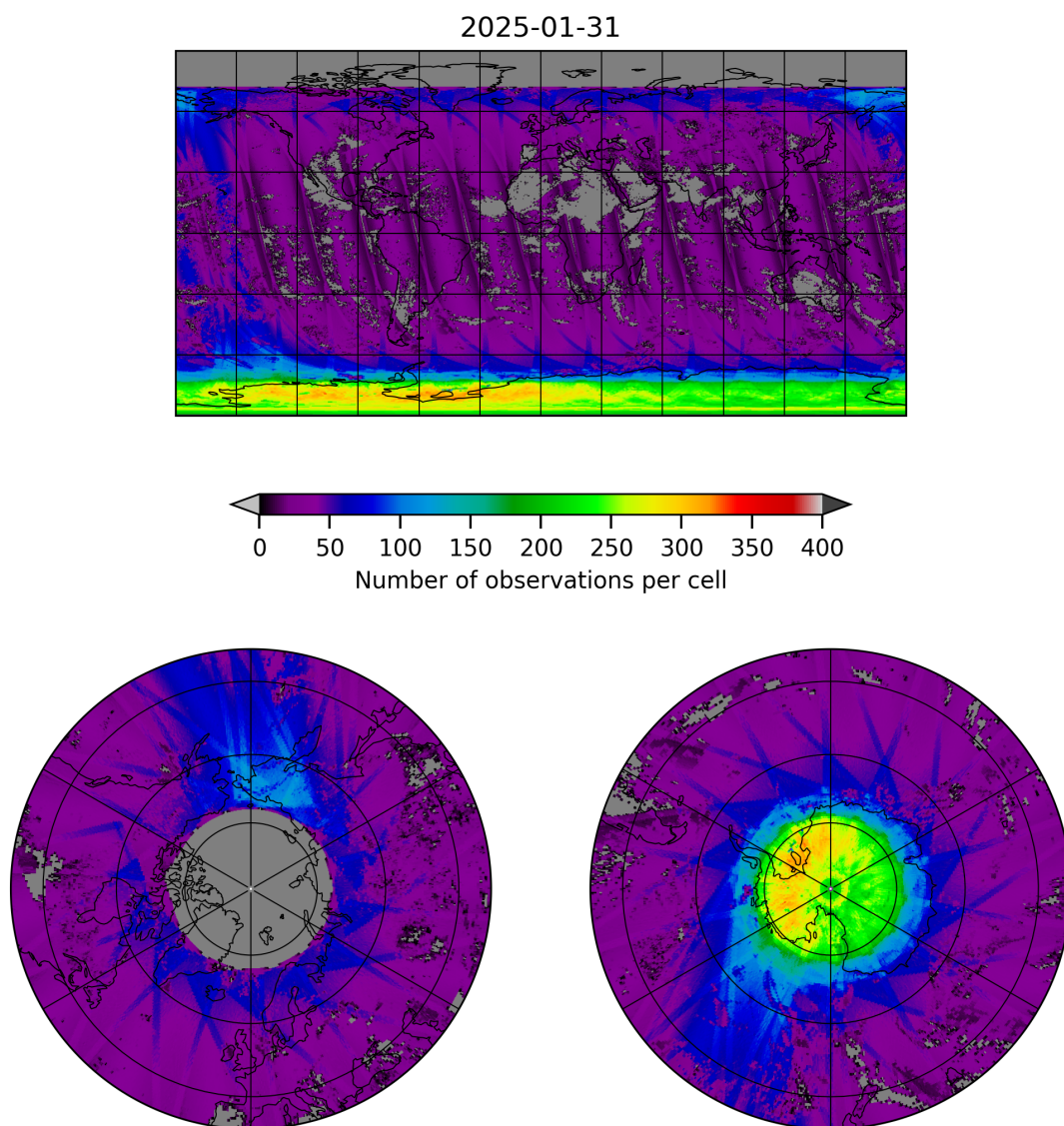
Figure 21: Map of the number of observations for 2025-01-30 to 2025-02-01
