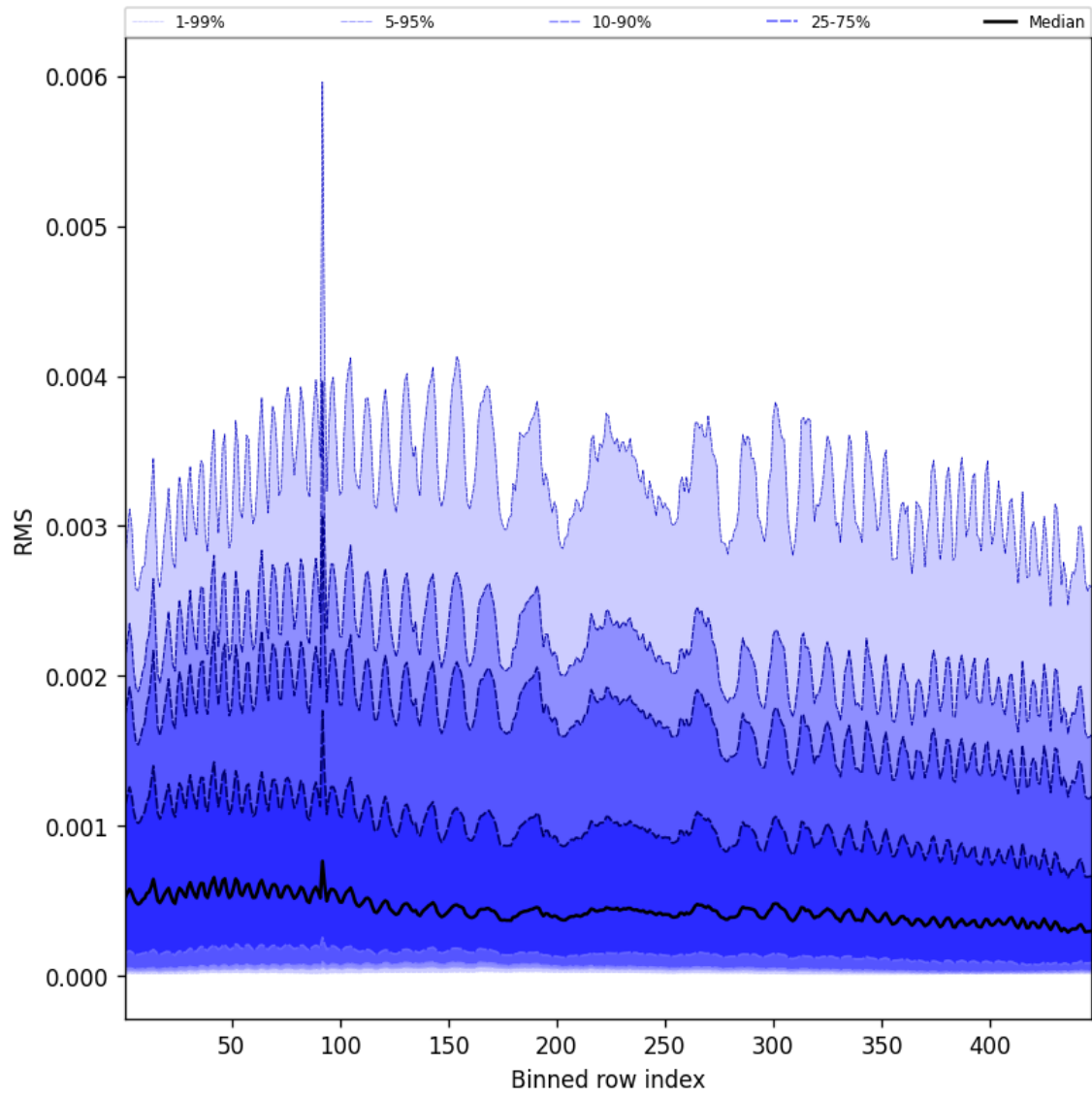
Figure 63: Along track statistics of “RMS” for 2025-01-30 to 2025-02-01
