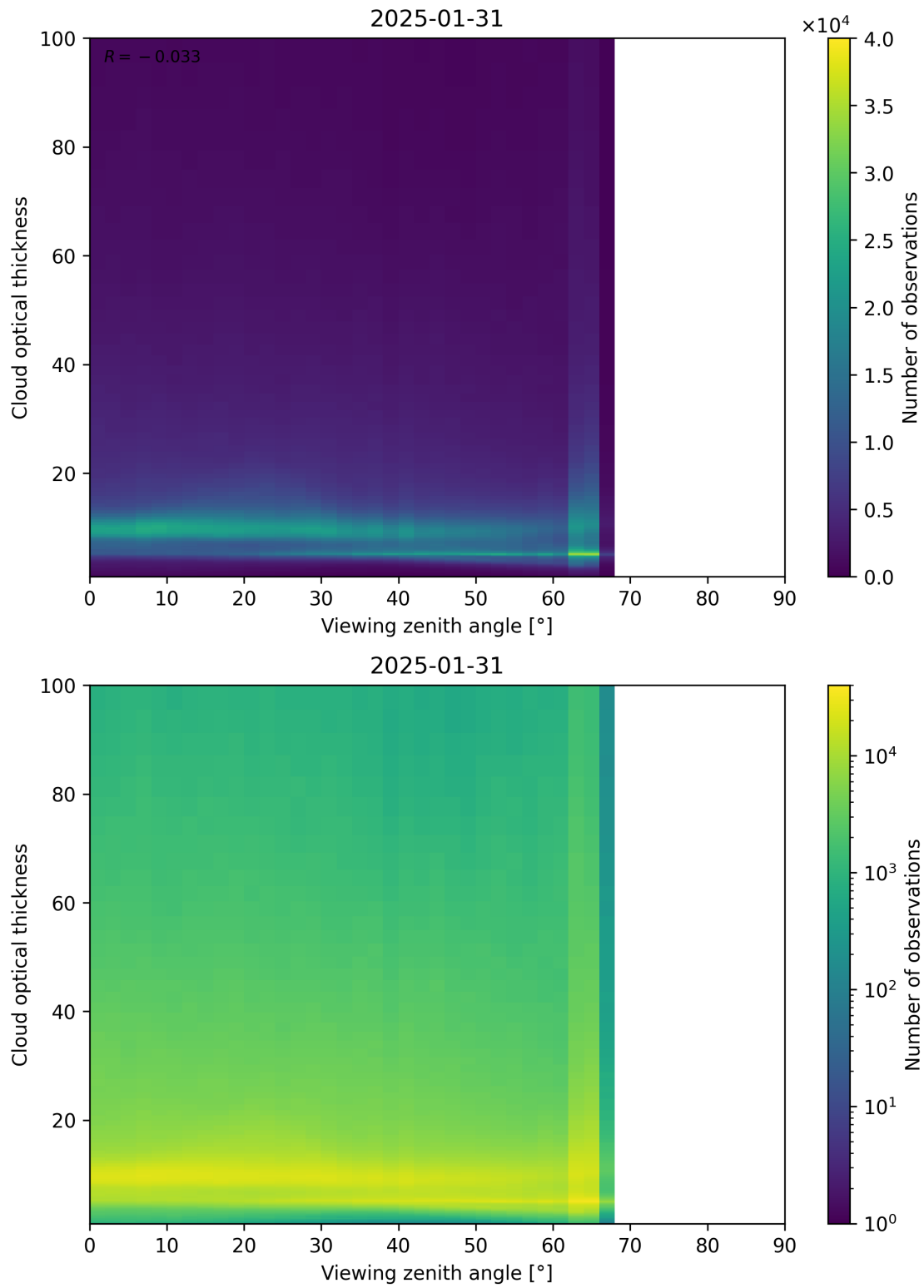
Figure 111: Scatter density plot of “Viewing zenith angle” against “Cloud optical thickness” for 2025-01-30 to 2025-02-01.
