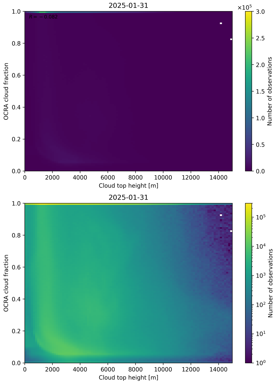
Figure 87: Scatter density plot of “Cloud top height” against “OCRA cloud fraction” for 2025-01-30 to 2025-02-01.
