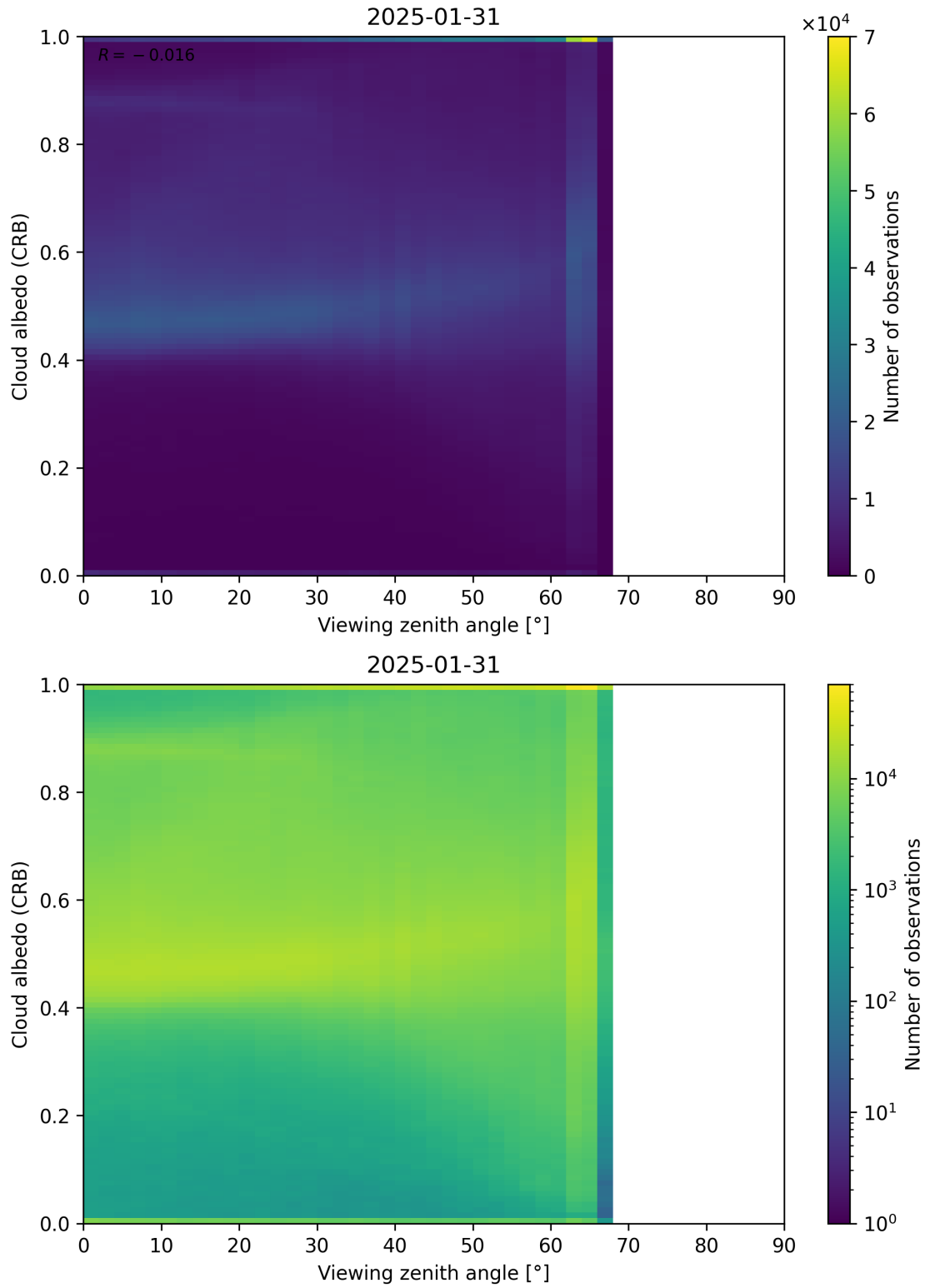
Figure 106: Scatter density plot of “Viewing zenith angle” against “Cloud albedo (CRB)” for 2025-01-30 to 2025-02-01.
