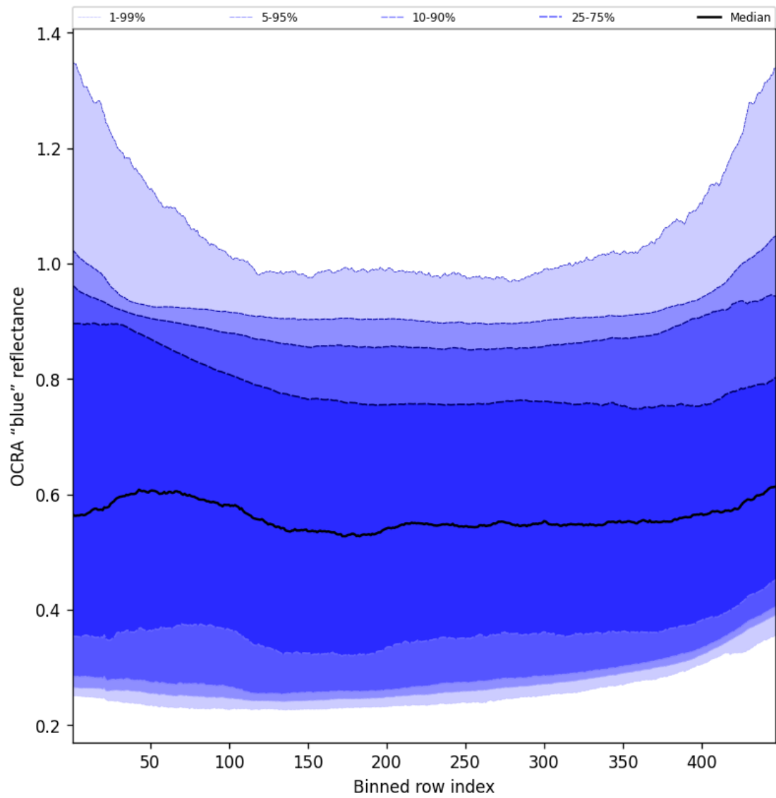
Figure 67: Along track statistics of “OCRA “blue” reflectance” for 2025-01-30 to 2025-02-01
