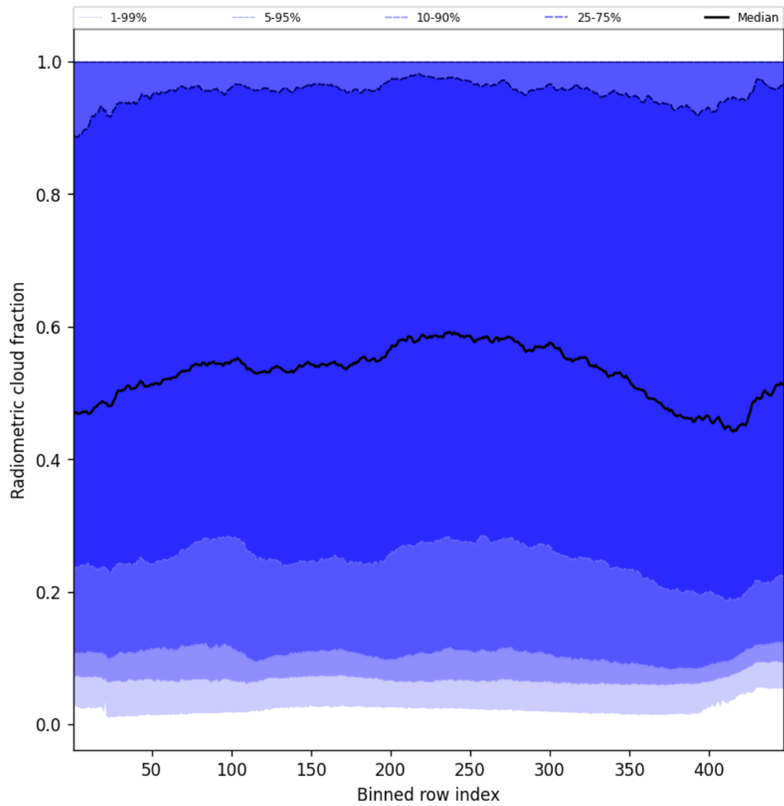
Figure 55: Along track statistics of “Radiometric cloud fraction” for 2025-01-30 to 2025-02-01
