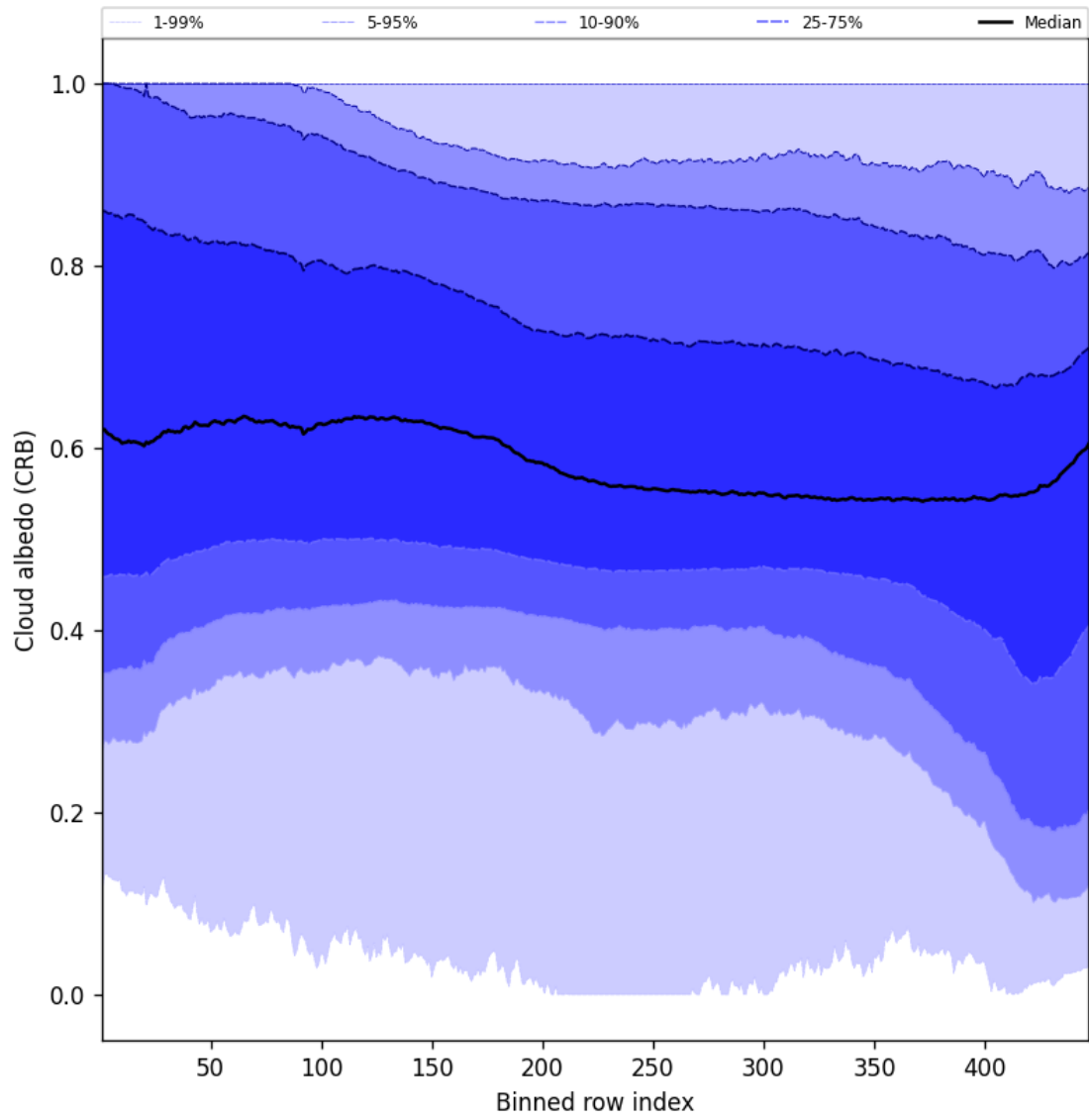
Figure 60: Along track statistics of “Cloud albedo (CRB)” for 2025-01-30 to 2025-02-01
