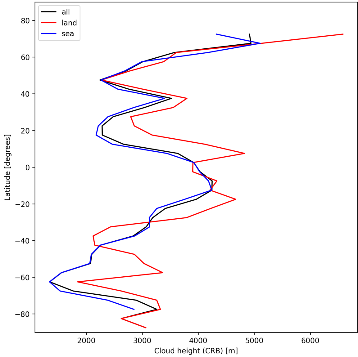
Figure 27: Zonal average of “Cloud height (CRB)” for 2025-01-30 to 2025-02-01.
