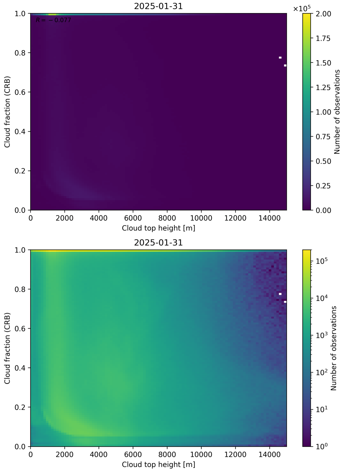
Figure 88: Scatter density plot of “Cloud top height” against “Cloud fraction (CRB)” for 2025-01-30 to 2025-02-01.
