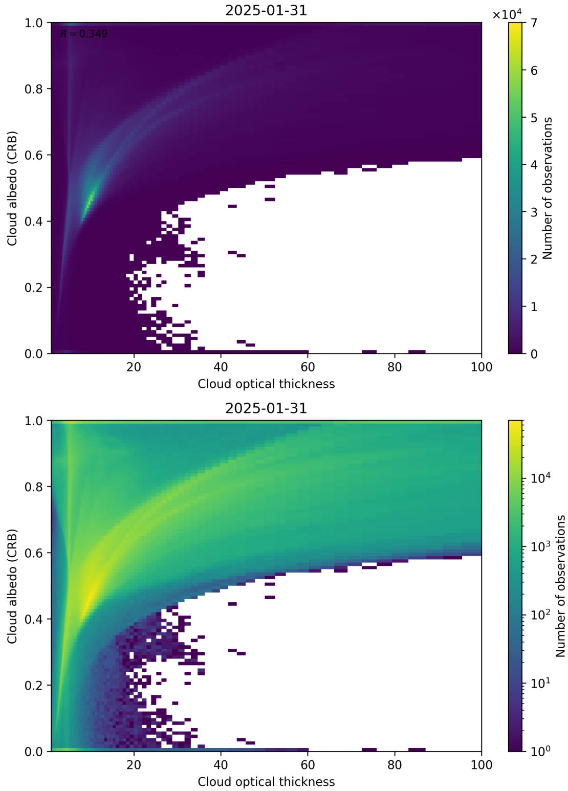
Figure 82: Scatter density plot of “Cloud optical thickness” against “Cloud albedo (CRB)” for 2025-01-30 to 2025-02-01.
