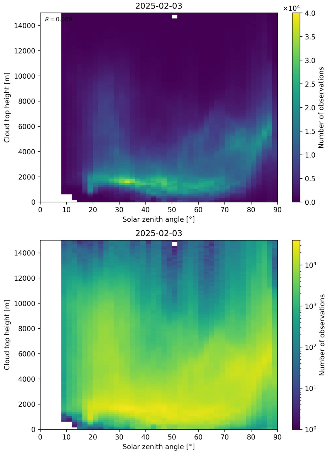
Figure 104: Scatter density plot of “Solar zenith angle” against “Cloud top height” for 2025-02-03 to 2025-02-04.
