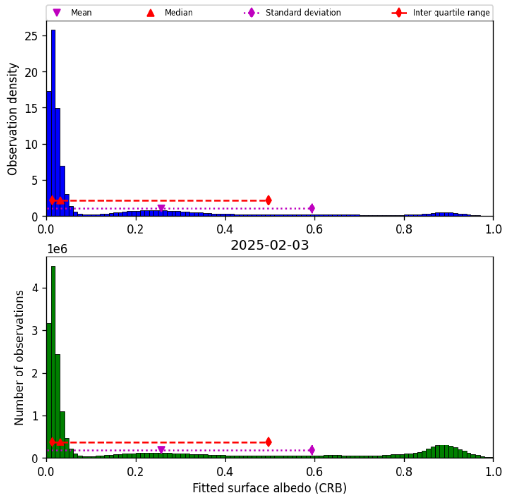
Figure 46: Histogram of “Fitted surface albedo (CRB)” for 2025-02-03 to 2025-02-04
