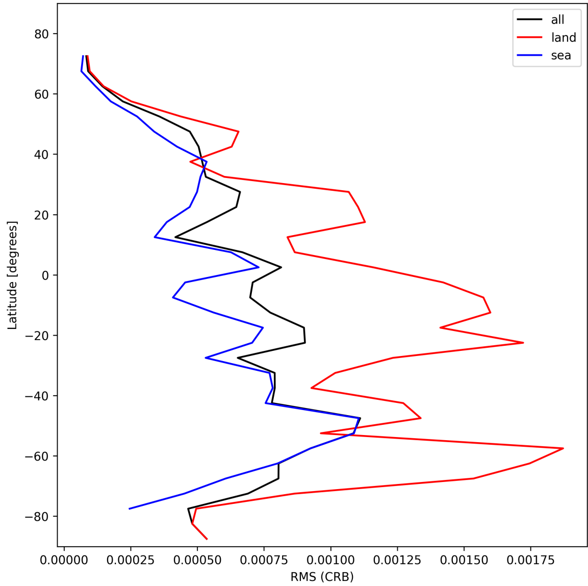
Figure 32: Zonal average of “RMS (CRB)” for 2025-02-03 to 2025-02-04.
