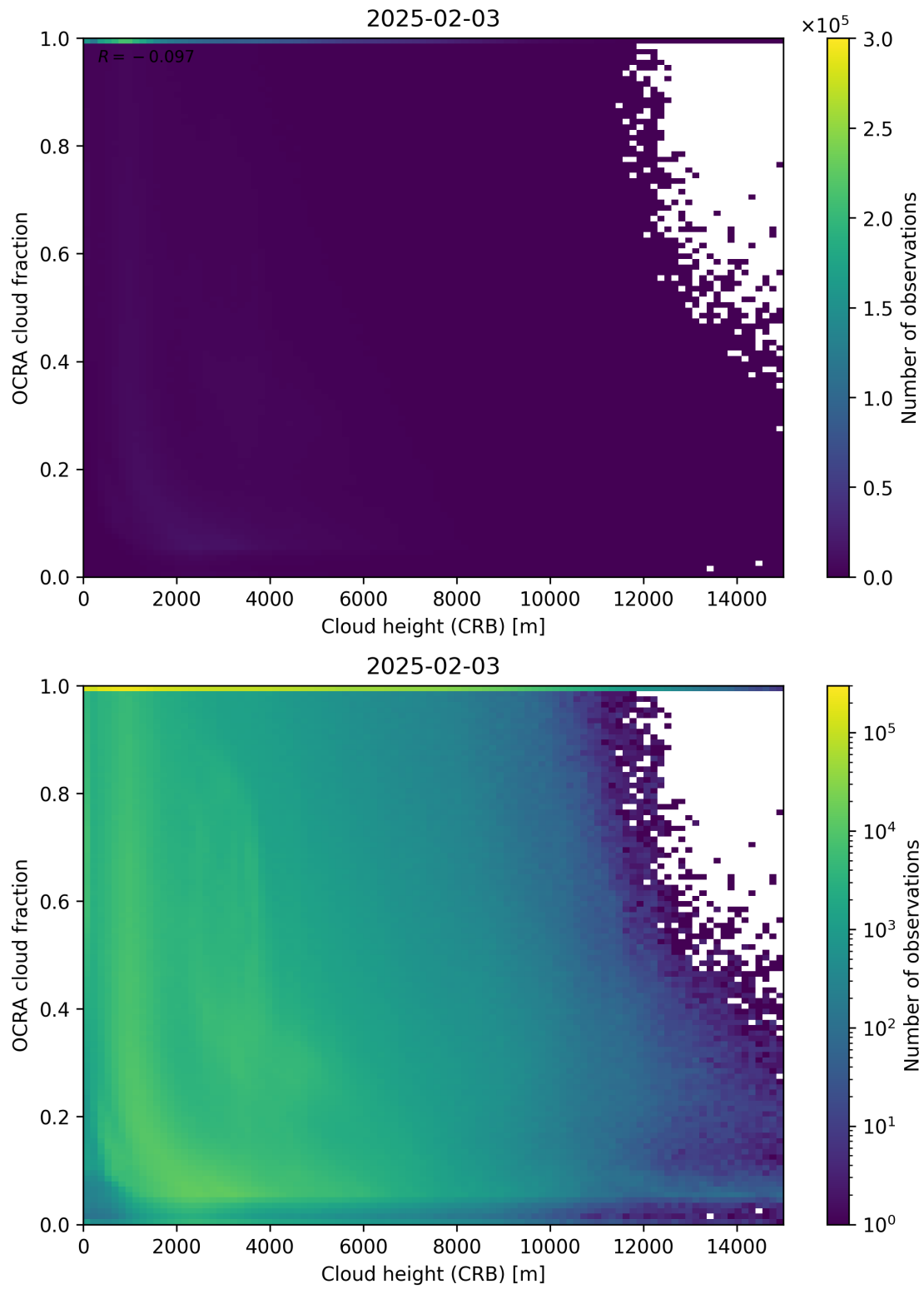
Figure 81: Scatter density plot of “Cloud height (CRB)” against “OCRA cloud fraction” for 2025-02-03 to 2025-02-04.
