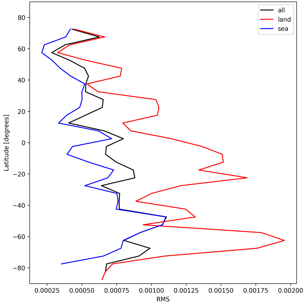
Figure 31: Zonal average of “RMS” for 2025-02-03 to 2025-02-04.
