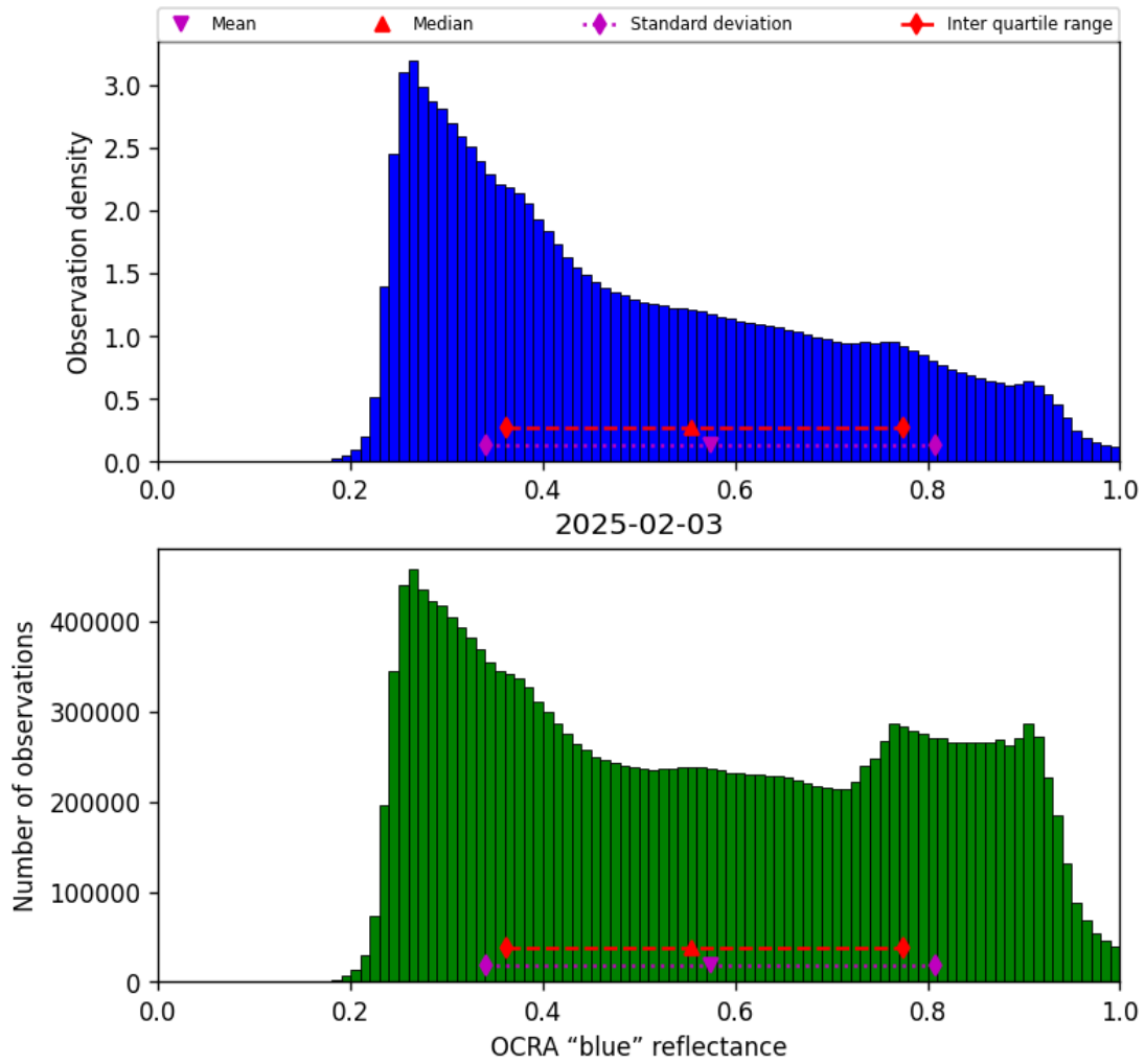
Figure 51: Histogram of “OCRA “blue” reflectance” for 2025-02-03 to 2025-02-04
