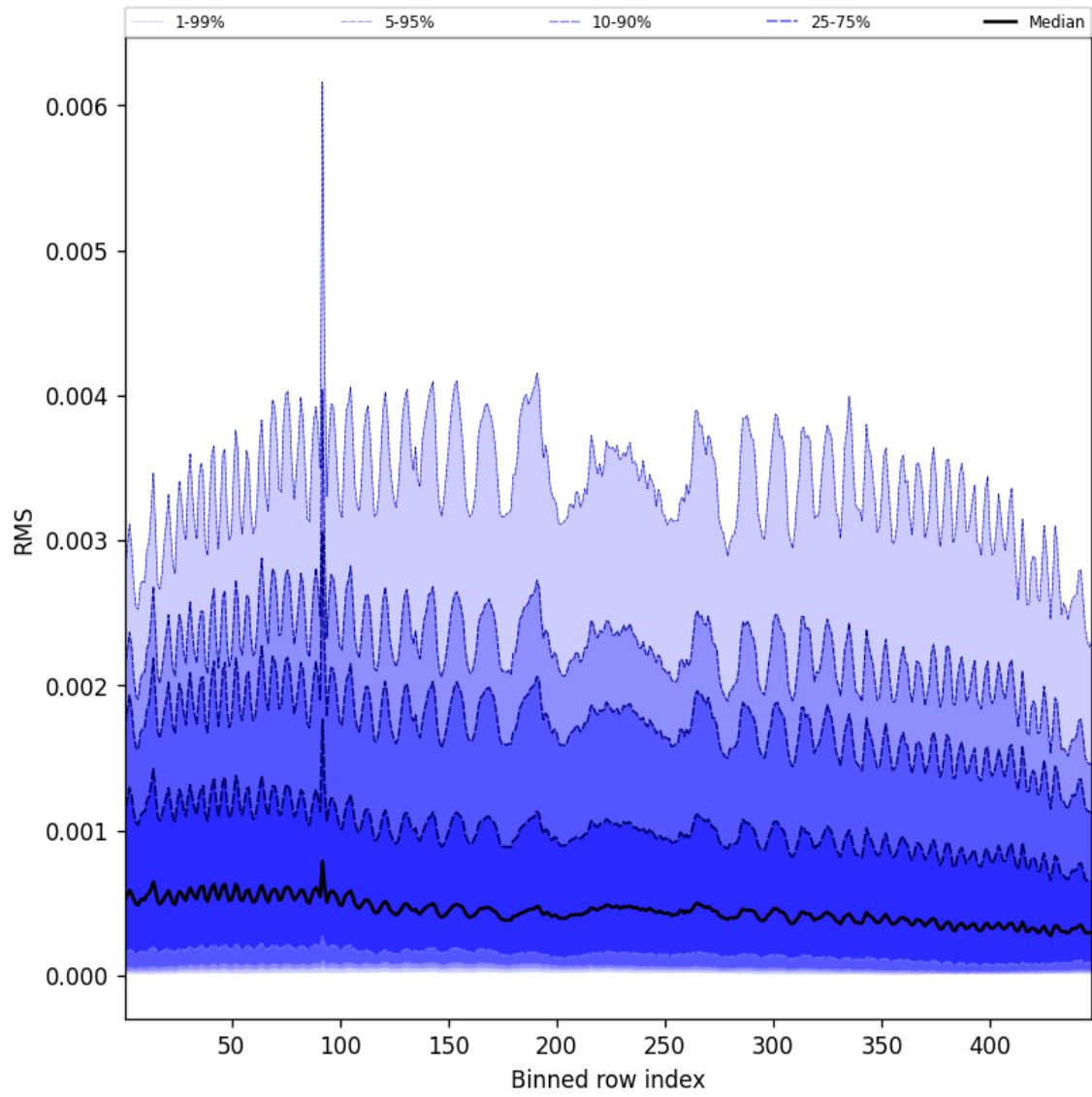
Figure 63: Along track statistics of “RMS” for 2025-02-03 to 2025-02-04
