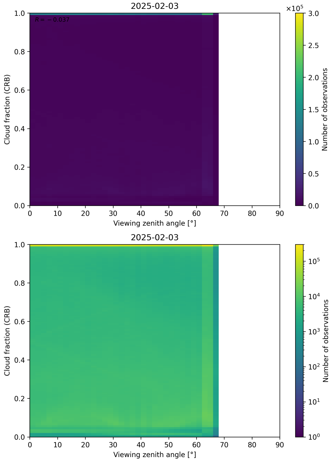
Figure 109: Scatter density plot of “Viewing zenith angle” against “Cloud fraction (CRB)” for 2025-02-03 to 2025-02-04.
