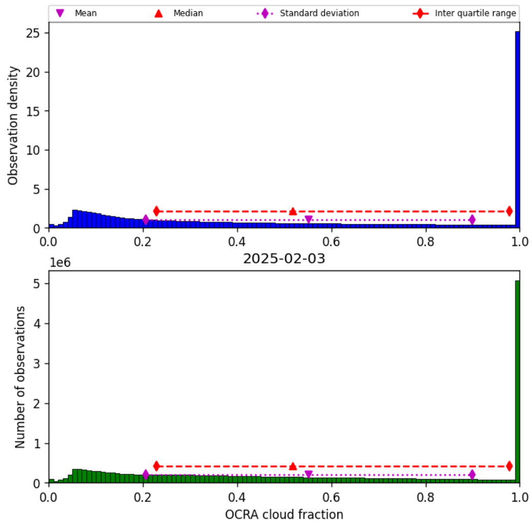
Figure 50: Histogram of “OCRA cloud fraction” for 2025-02-03 to 2025-02-04
