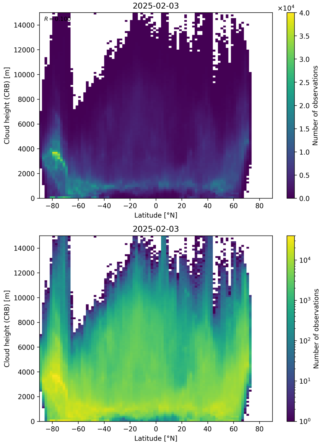
Figure 95: Scatter density plot of “Latitude” against “Cloud height (CRB)” for 2025-02-03 to 2025-02-04.
