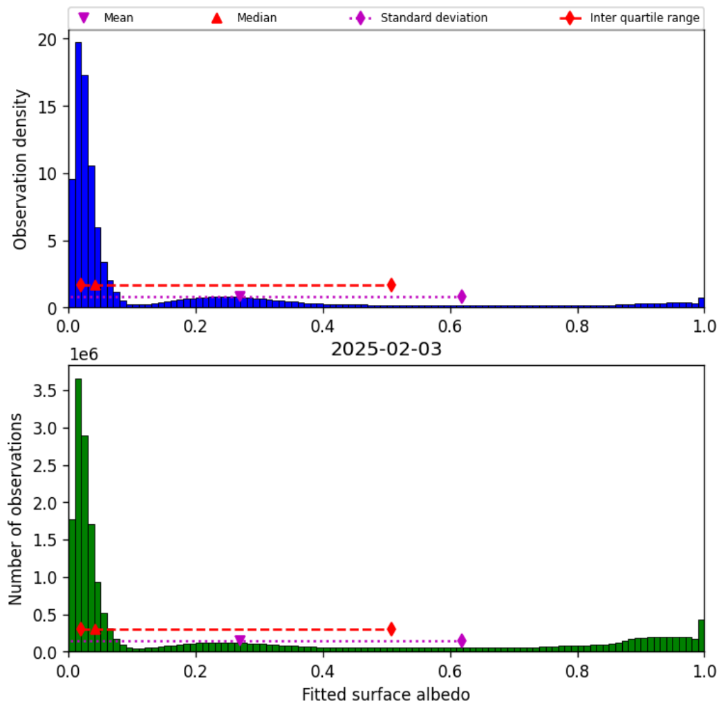
Figure 45: Histogram of “Fitted surface albedo” for 2025-02-03 to 2025-02-04
