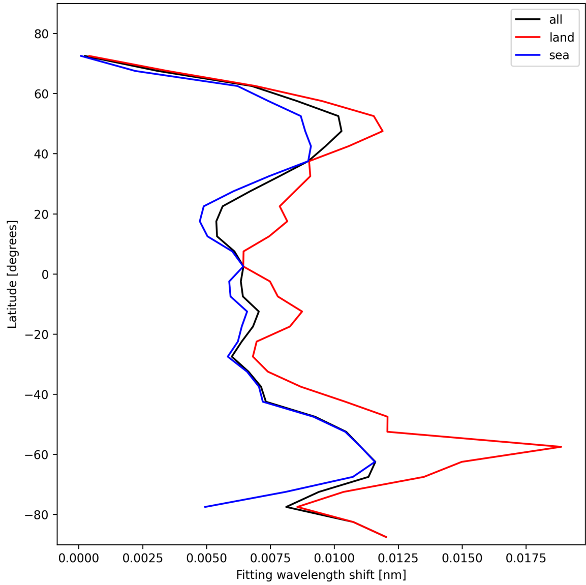
Figure 33: Zonal average of “Fitting wavelength shift” for 2025-02-03 to 2025-02-04.
