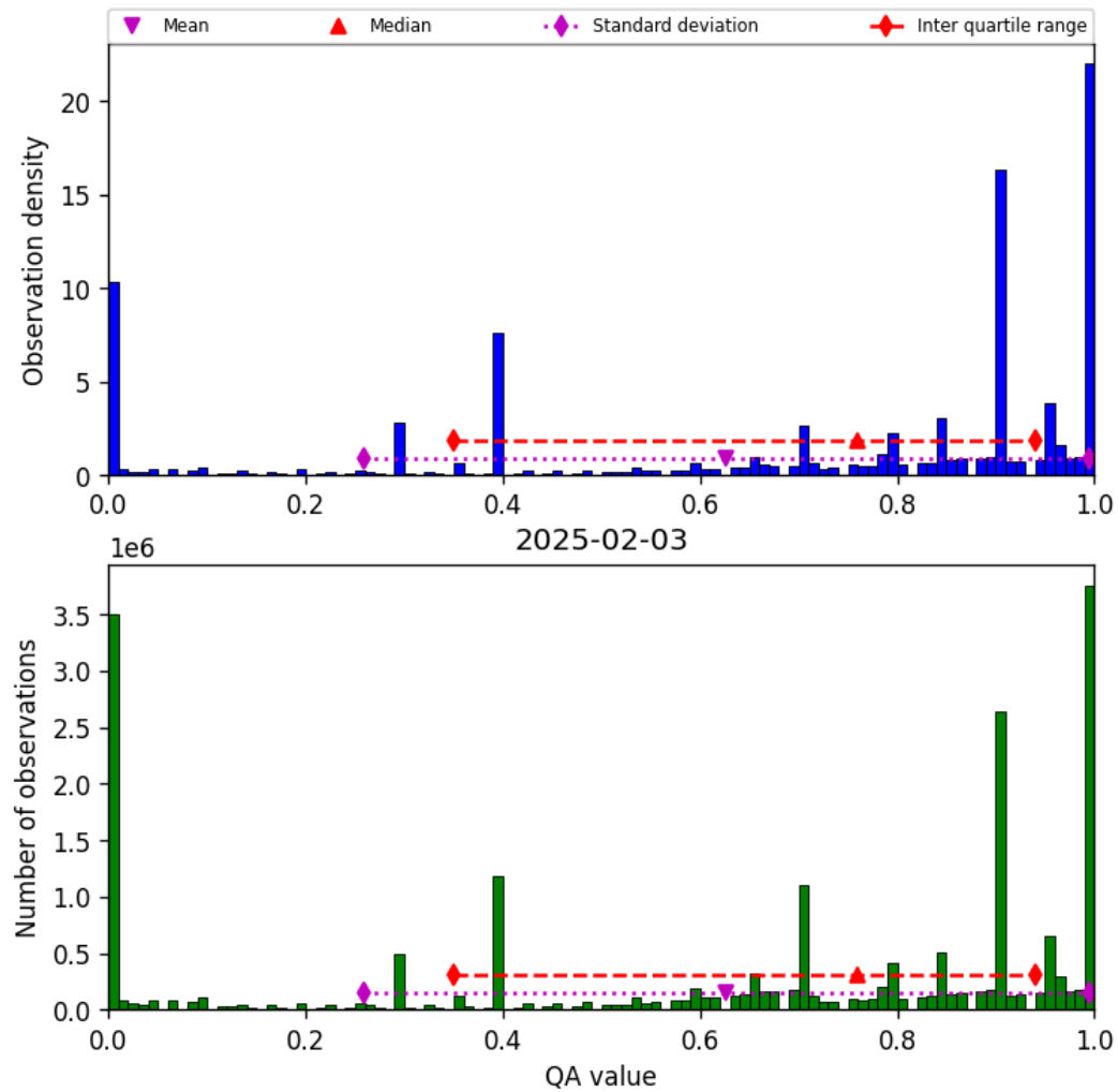
Figure 38: Histogram of “QA value” for 2025-02-03 to 2025-02-04
