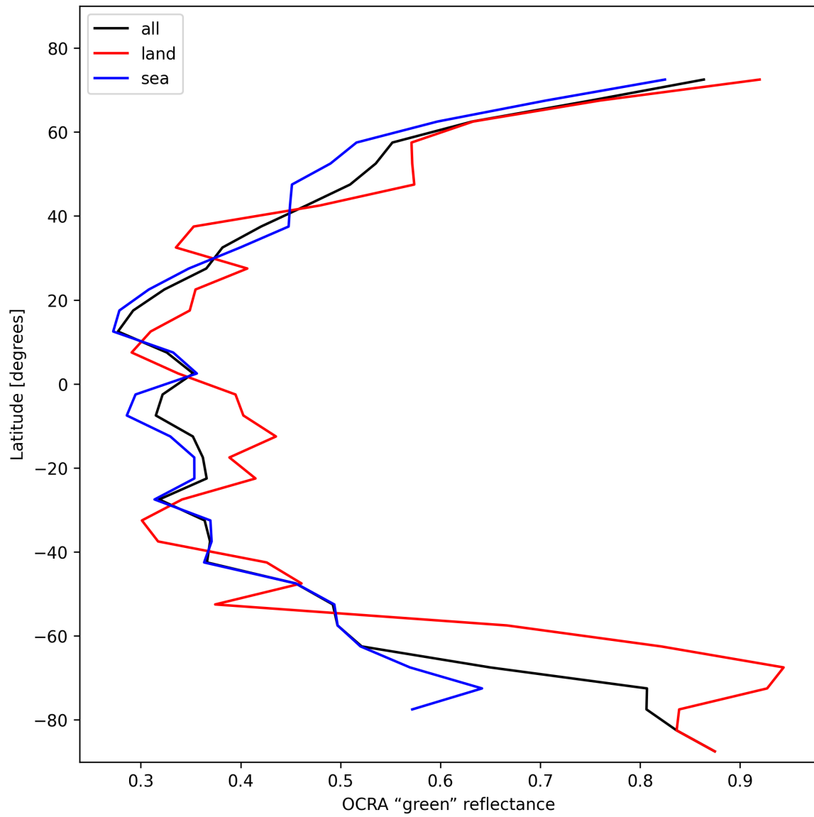
Figure 36: Zonal average of “OCRA “green” reflectance” for 2025-02-03 to 2025-02-04.
