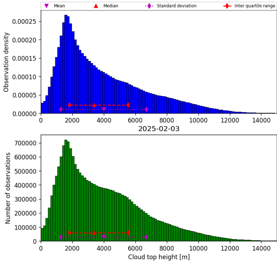
Figure 40: Histogram of “Cloud top height” for 2025-02-03 to 2025-02-04
