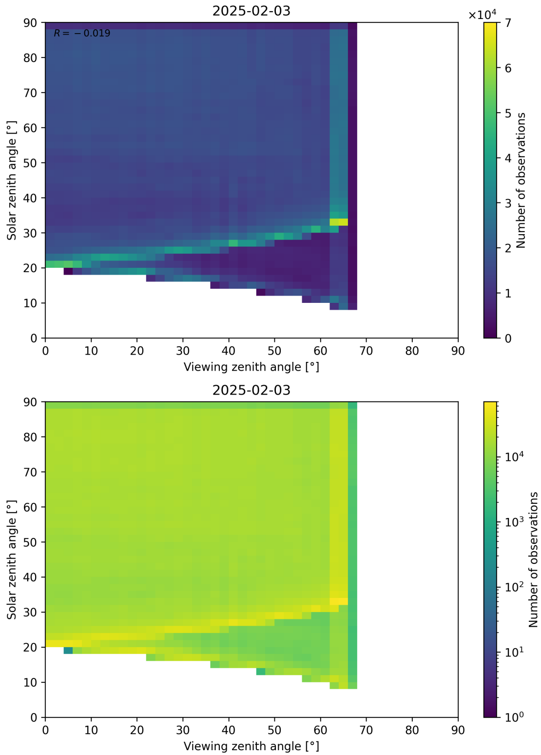
Figure 114: Scatter density plot of “Viewing zenith angle” against “Solar zenith angle” for 2025-02-03 to 2025-02-04.
