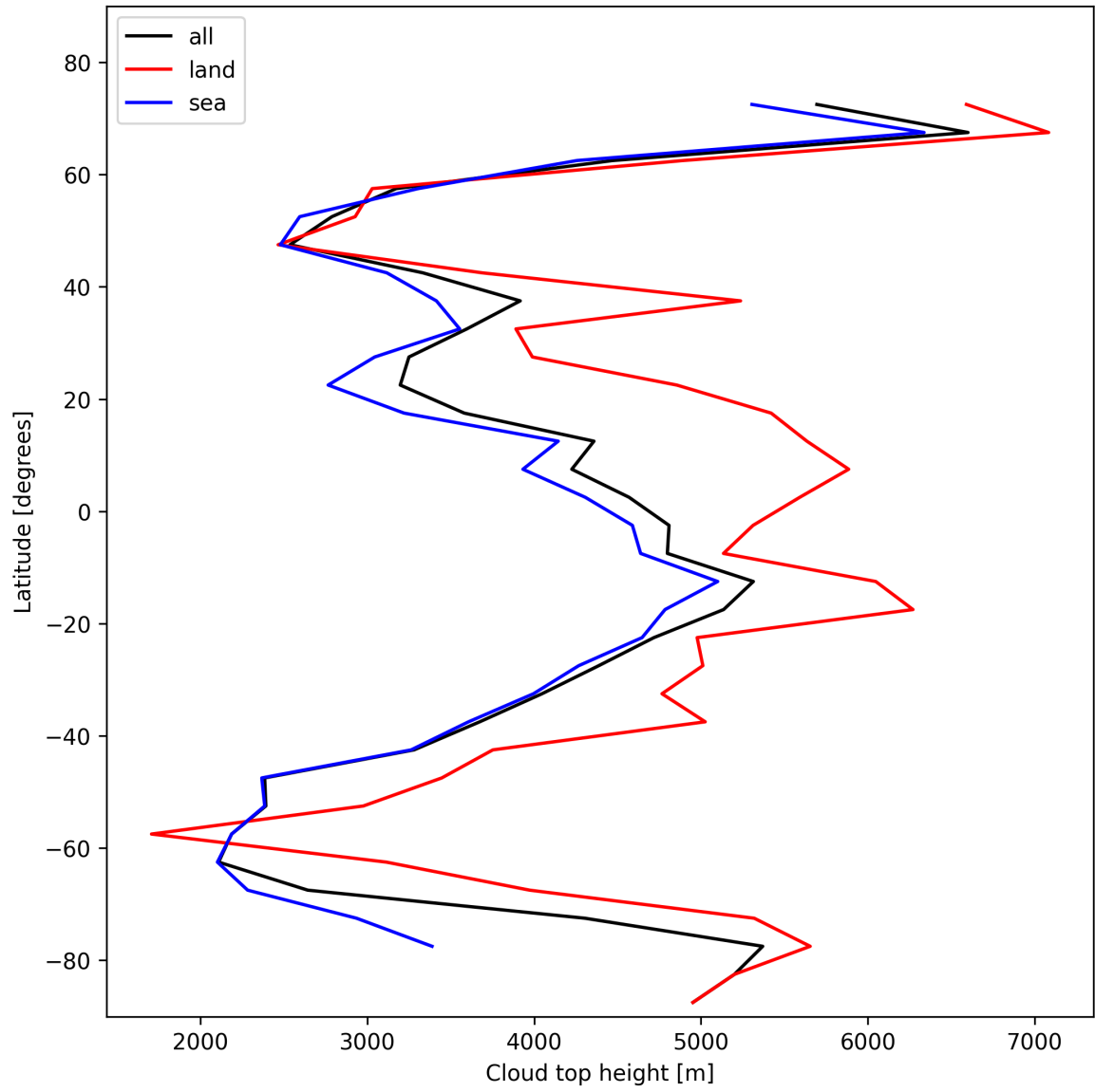
Figure 24: Zonal average of “Cloud top height” for 2025-02-03 to 2025-02-04.
