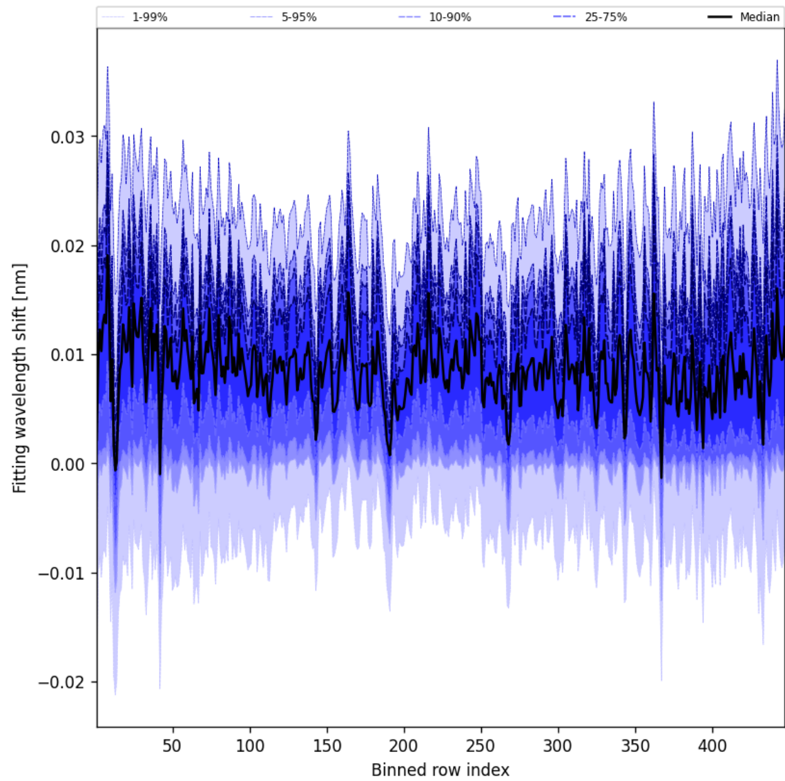
Figure 65: Along track statistics of “Fitting wavelength shift” for 2025-02-03 to 2025-02-04
