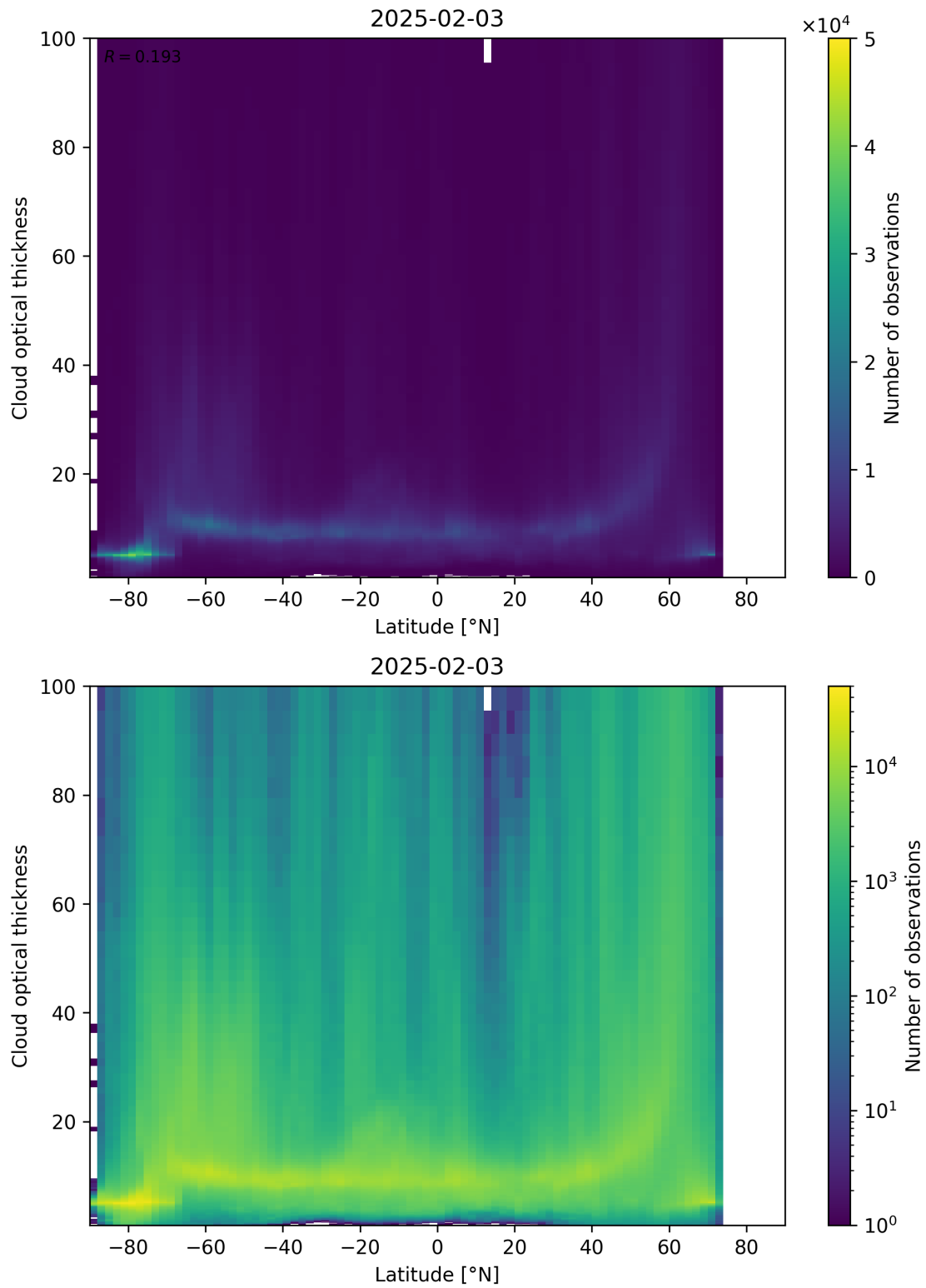
Figure 96: Scatter density plot of “Latitude” against “Cloud optical thickness” for 2025-02-03 to 2025-02-04.
