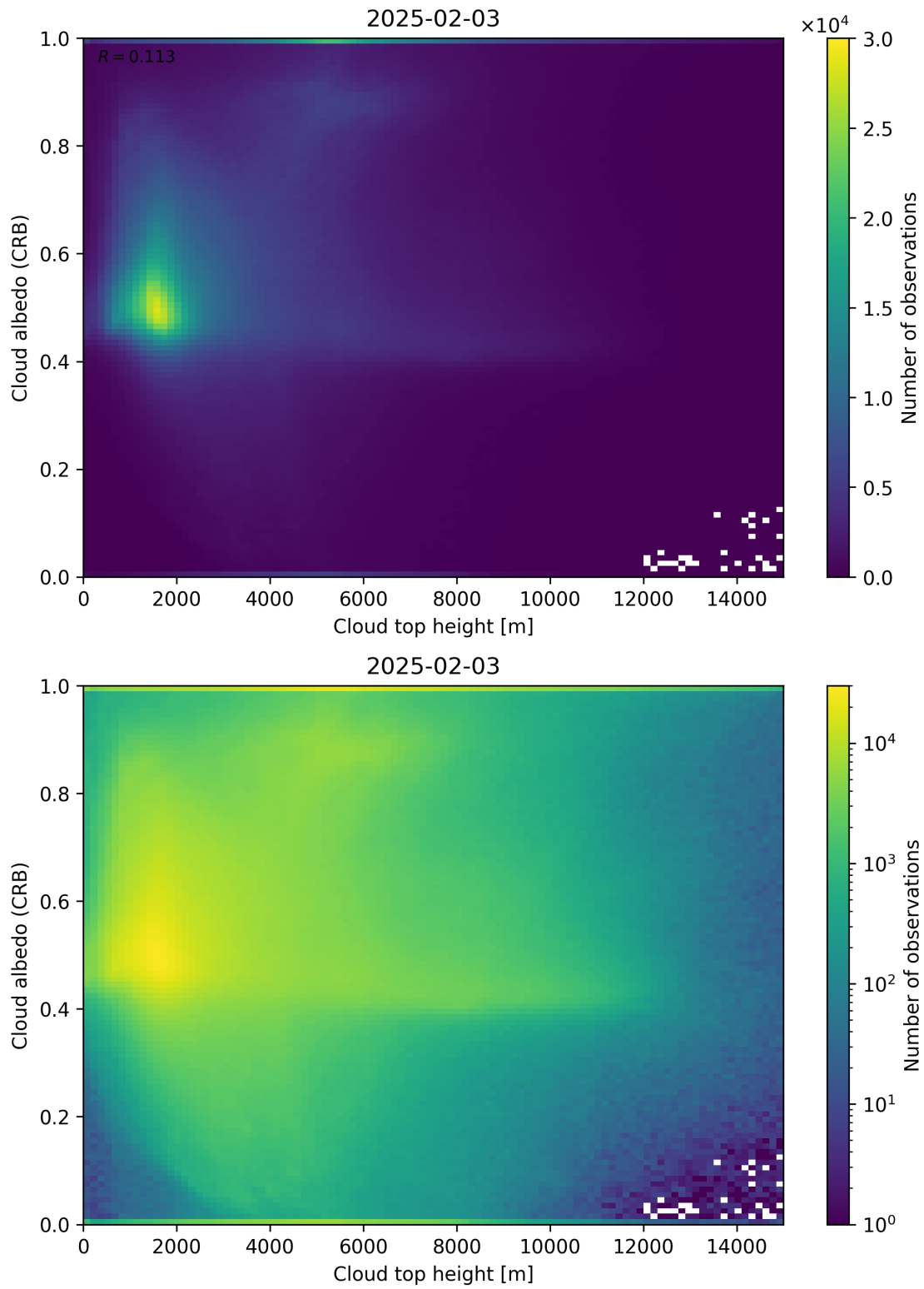
Figure 86: Scatter density plot of “Cloud top height” against “Cloud albedo (CRB)” for 2025-02-03 to 2025-02-04.
