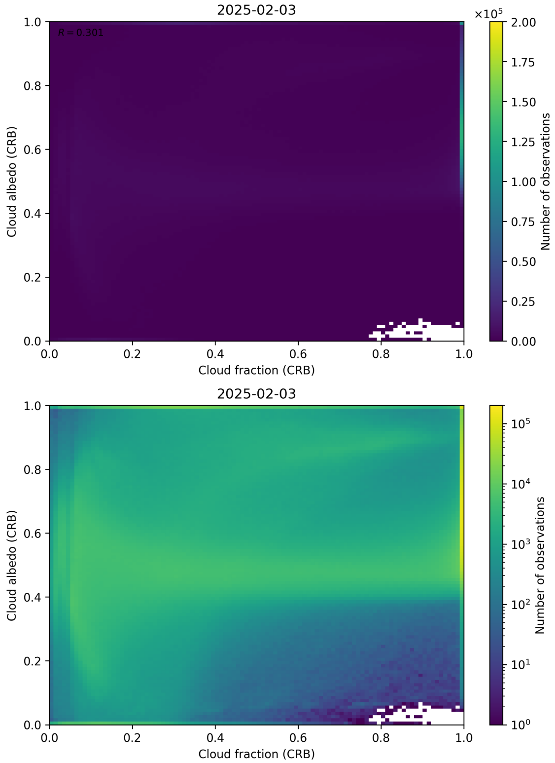
Figure 77: Scatter density plot of “Cloud fraction (CRB)” against “Cloud albedo (CRB)” for 2025-02-03 to 2025-02-04.
