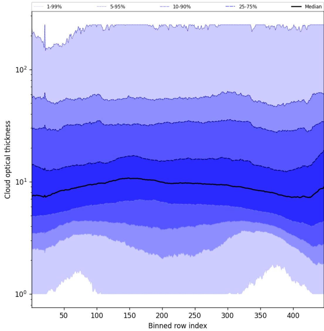
Figure 57: Along track statistics of “Cloud optical thickness” for 2025-02-03 to 2025-02-04
