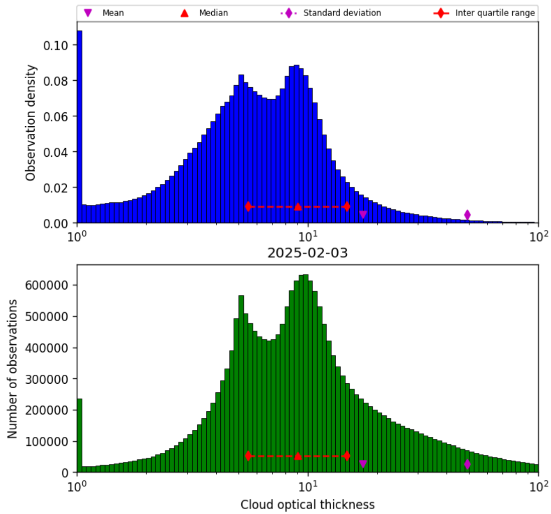
Figure 41: Histogram of “Cloud optical thickness” for 2025-02-03 to 2025-02-04
