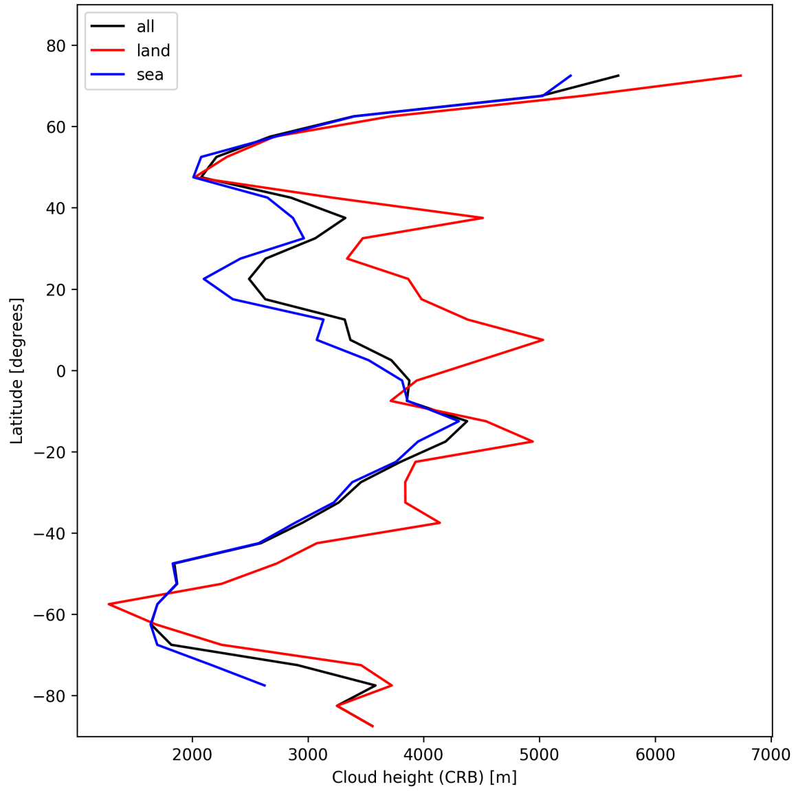
Figure 27: Zonal average of “Cloud height (CRB)” for 2025-02-03 to 2025-02-04.
