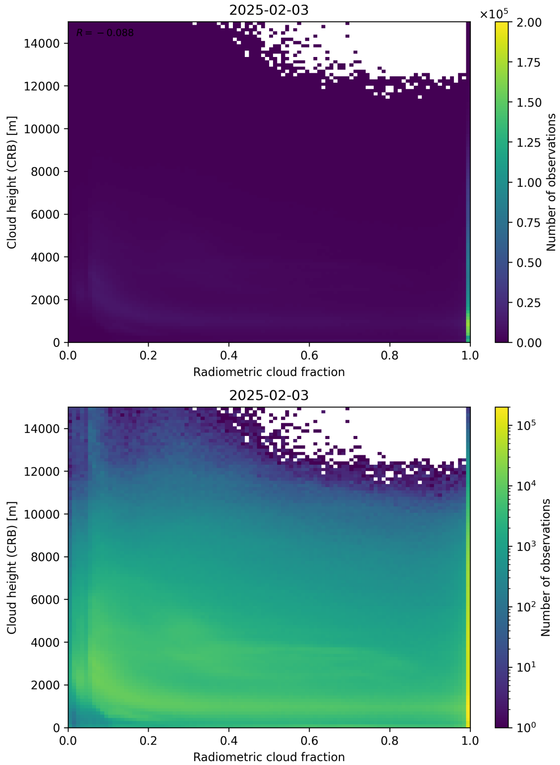
Figure 74: Scatter density plot of “Radiometric cloud fraction” against “Cloud height (CRB)” for 2025-02-03 to 2025-02-04.
