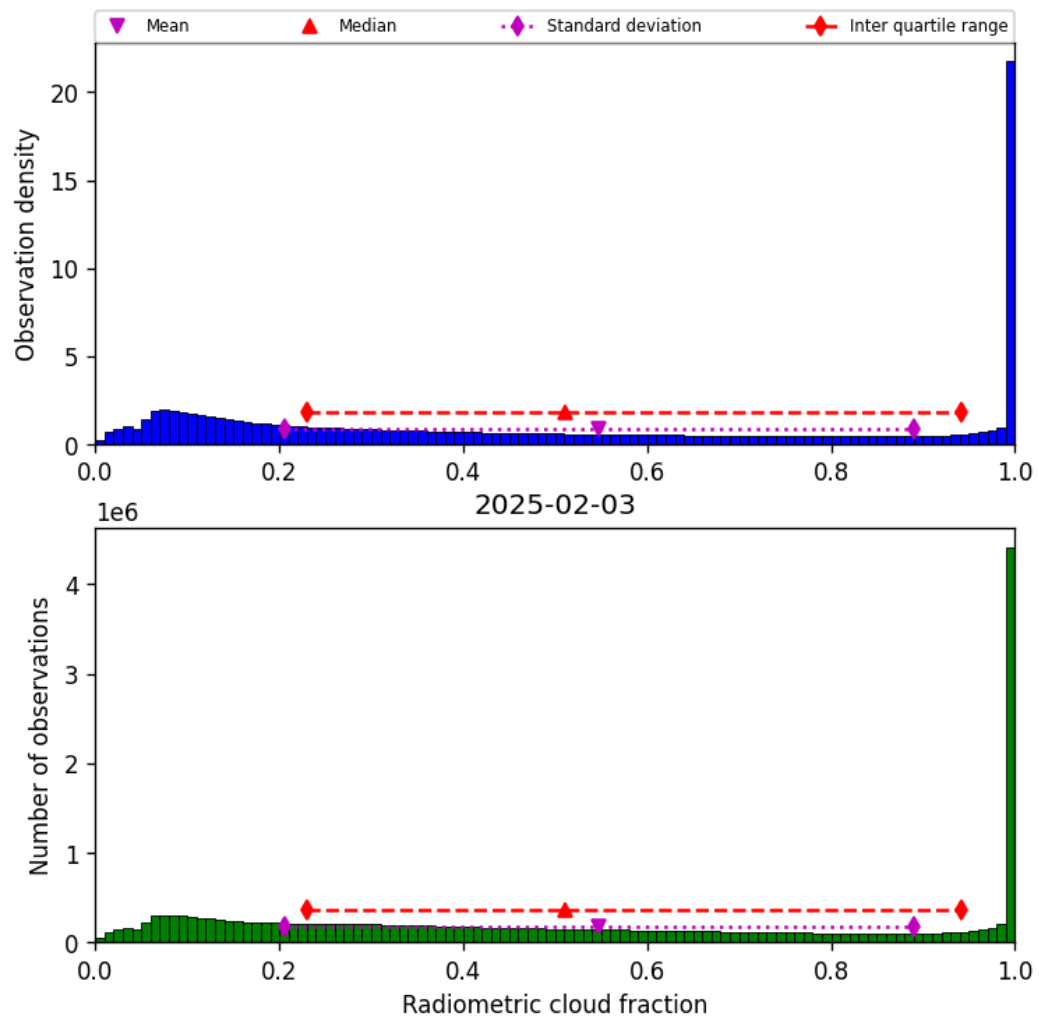
Figure 39: Histogram of “Radiometric cloud fraction” for 2025-02-03 to 2025-02-04
