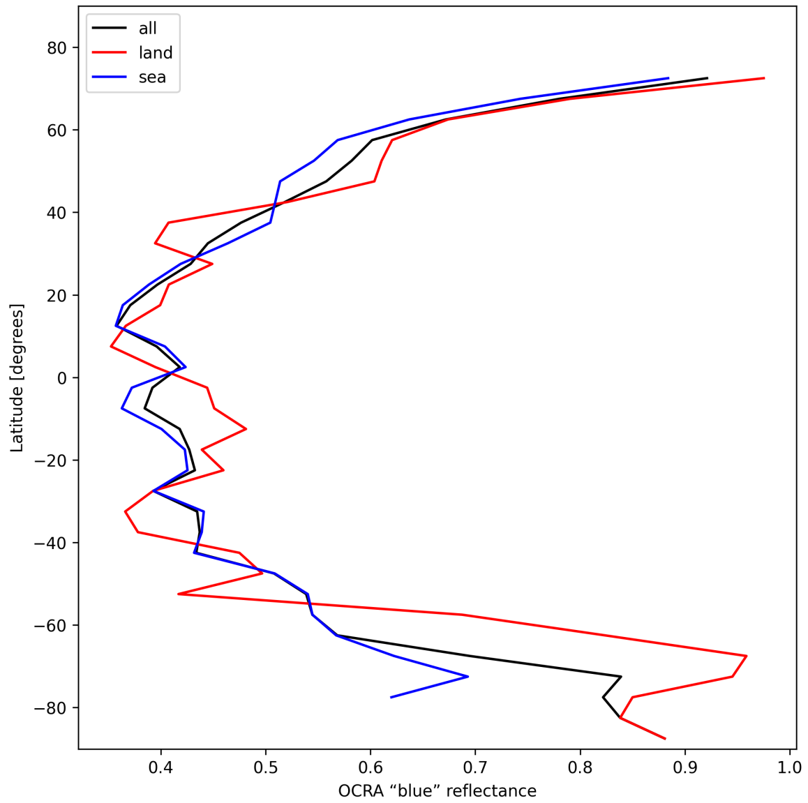
Figure 35: Zonal average of “OCRA “blue” reflectance” for 2025-02-03 to 2025-02-04.
