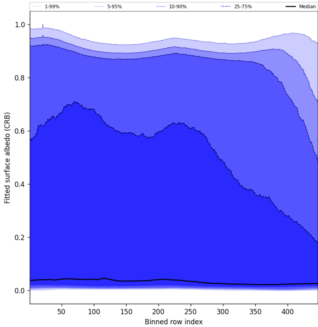
Figure 62: Along track statistics of “Fitted surface albedo (CRB)” for 2025-02-03 to 2025-02-04
