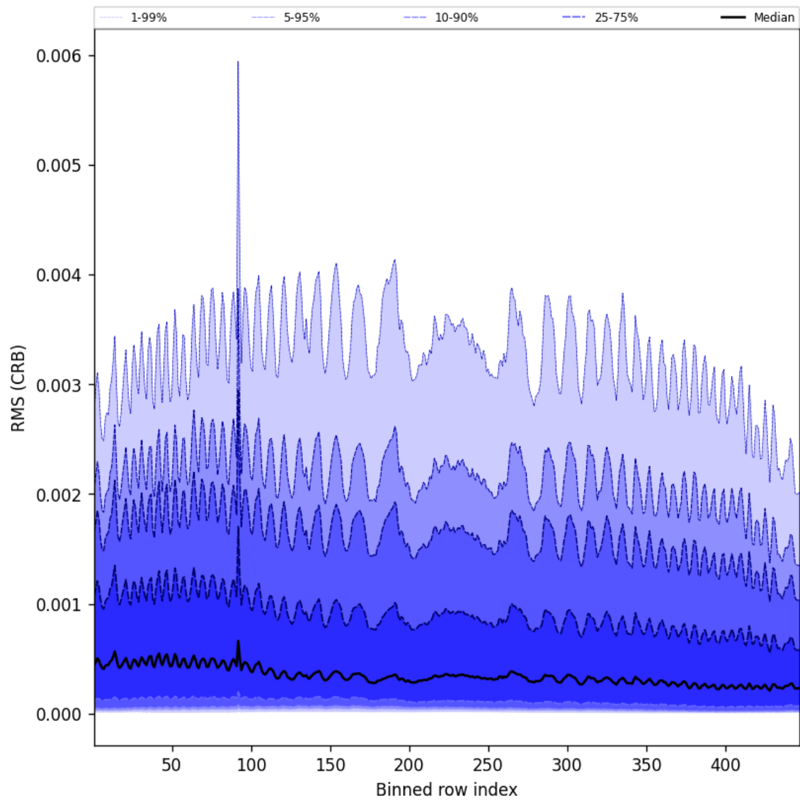
Figure 64: Along track statistics of “RMS (CRB)” for 2025-02-03 to 2025-02-04
