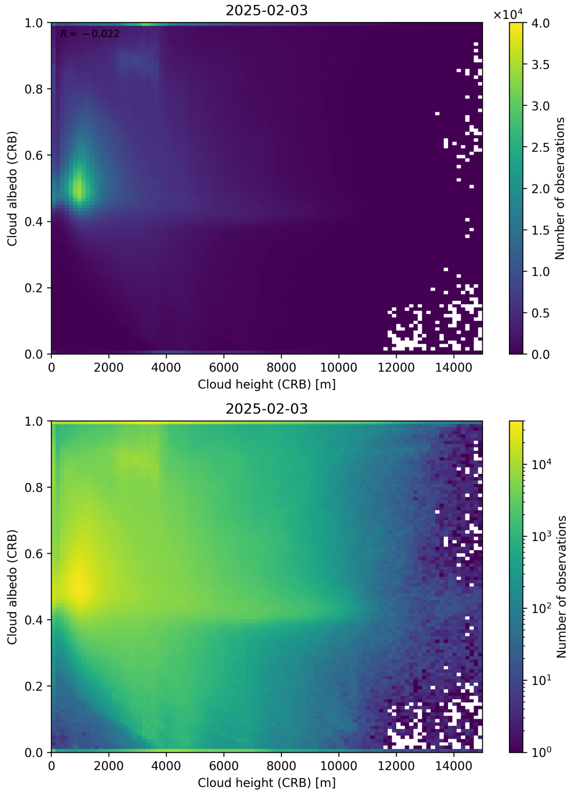
Figure 80: Scatter density plot of “Cloud height (CRB)” against “Cloud albedo (CRB)” for 2025-02-03 to 2025-02-04.
