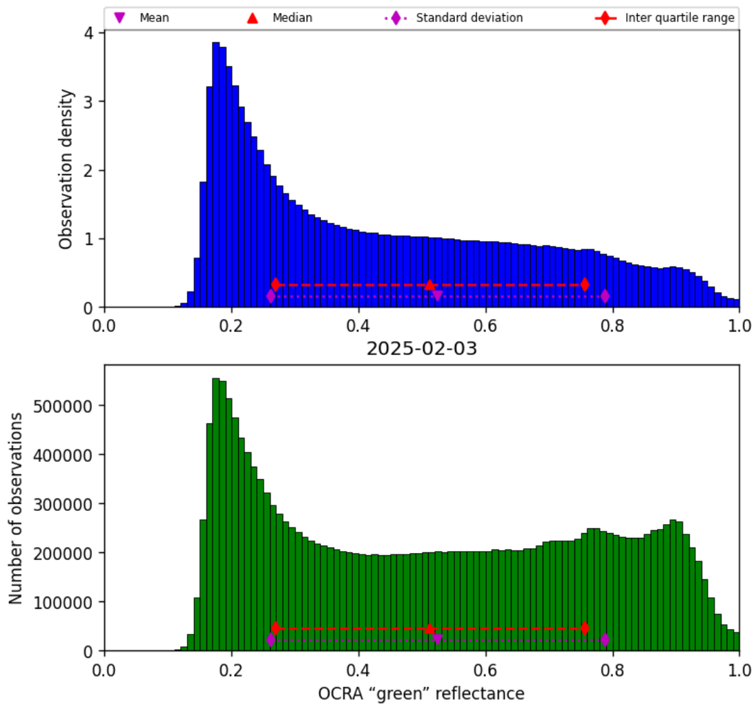
Figure 52: Histogram of “OCRA “green” reflectance” for 2025-02-03 to 2025-02-04
