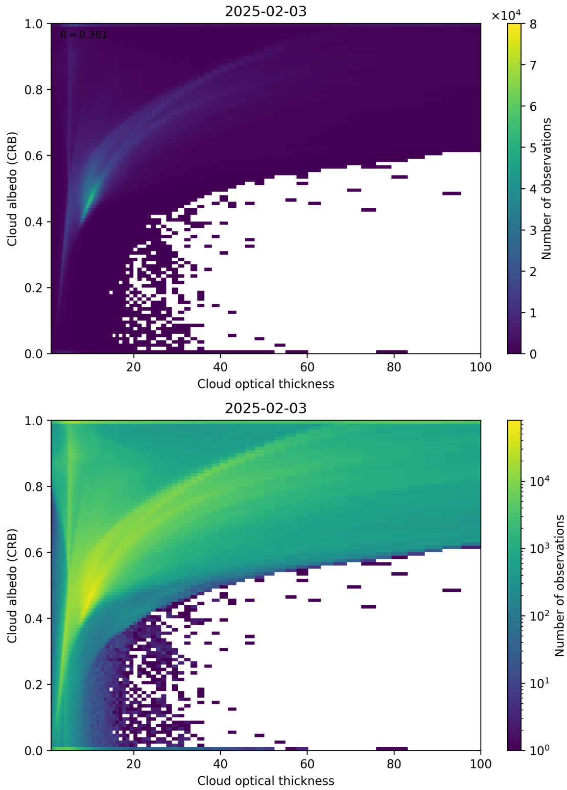
Figure 82: Scatter density plot of “Cloud optical thickness” against “Cloud albedo (CRB)” for 2025-02-03 to 2025-02-04.
