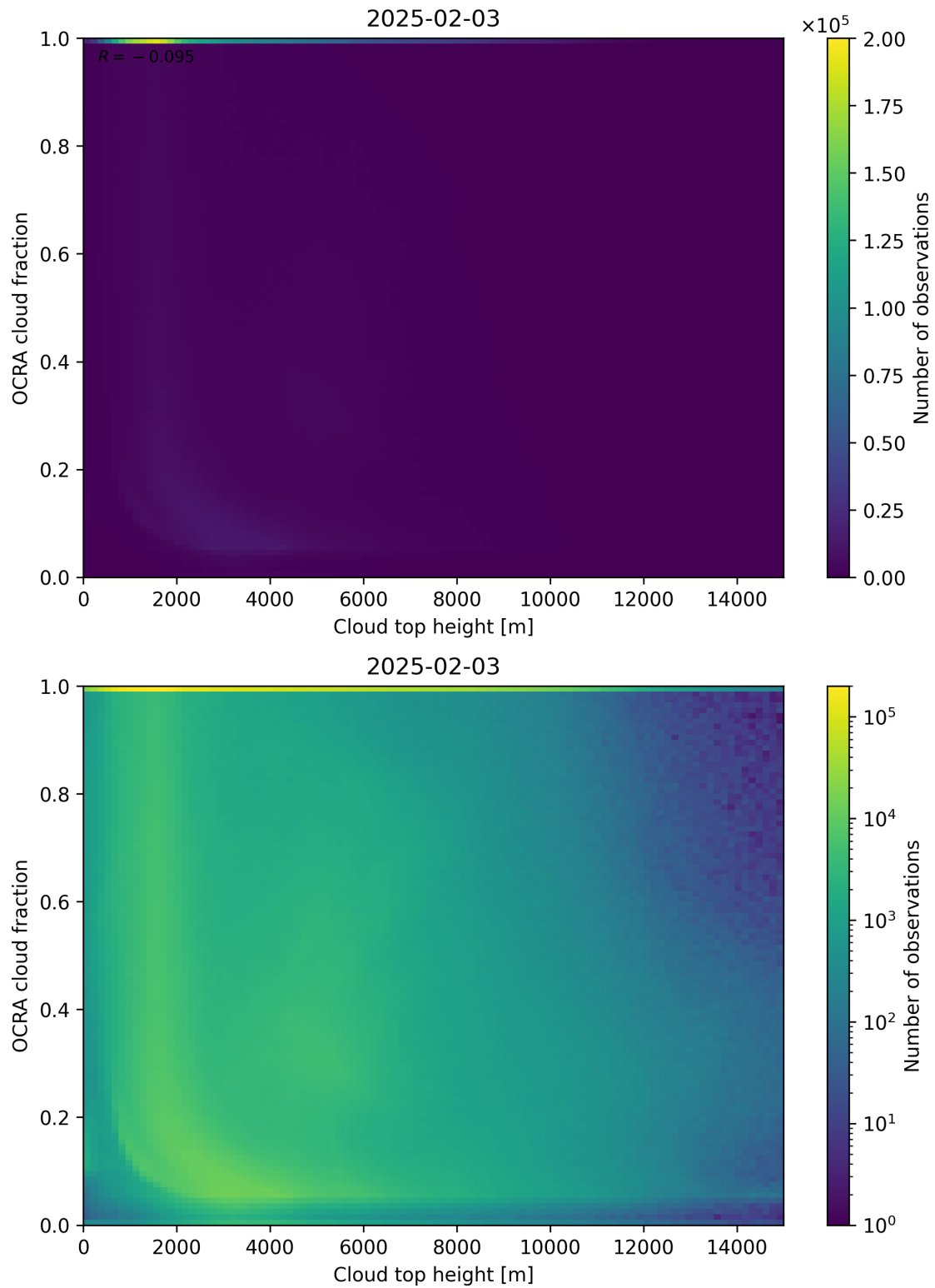
Figure 87: Scatter density plot of “Cloud top height” against “OCRA cloud fraction” for 2025-02-03 to 2025-02-04.
