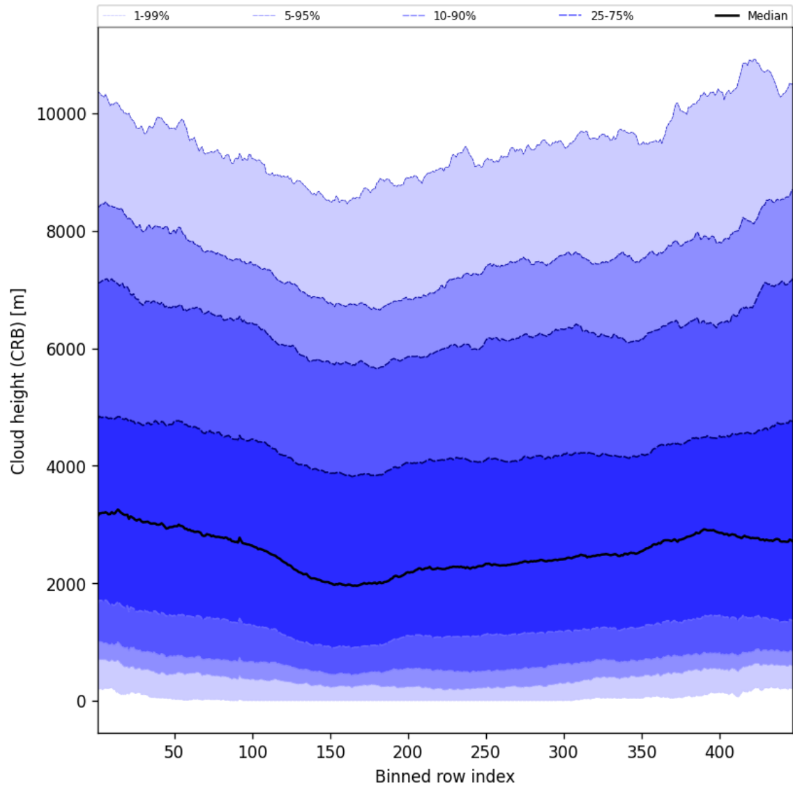
Figure 59: Along track statistics of “Cloud height (CRB)” for 2025-02-03 to 2025-02-04
