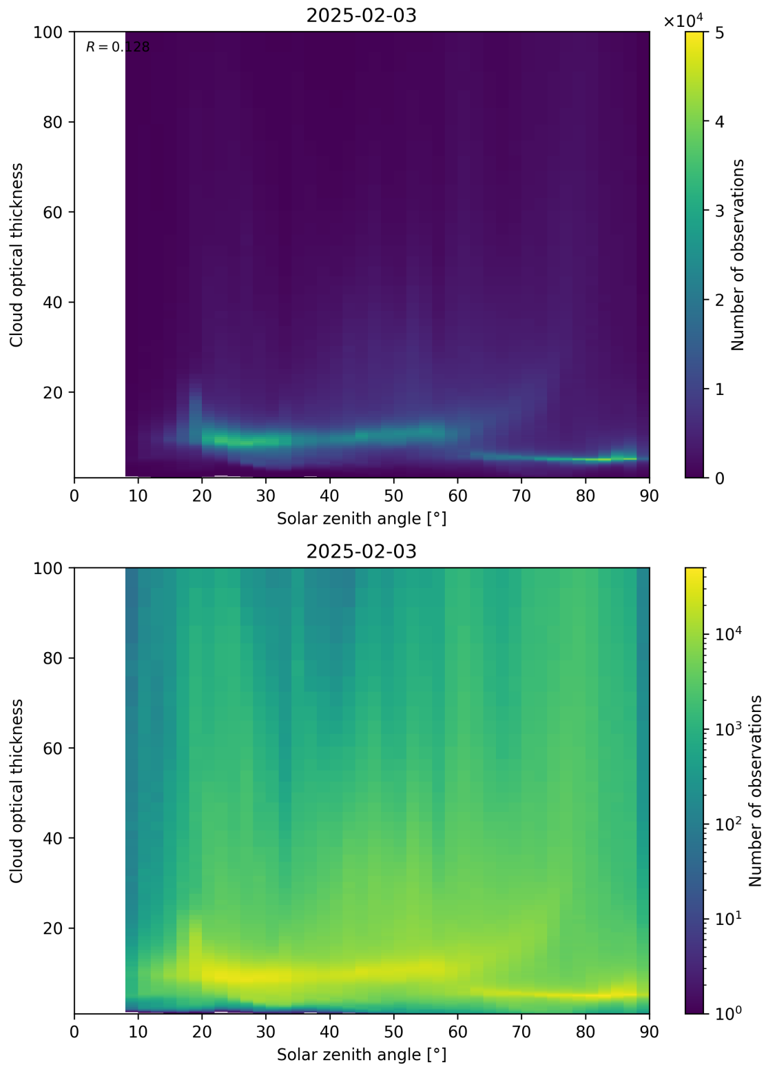
Figure 103: Scatter density plot of “Solar zenith angle” against “Cloud optical thickness” for 2025-02-03 to 2025-02-04.
