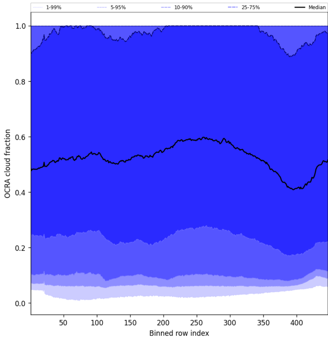
Figure 66: Along track statistics of “OCRA cloud fraction” for 2025-02-03 to 2025-02-04
