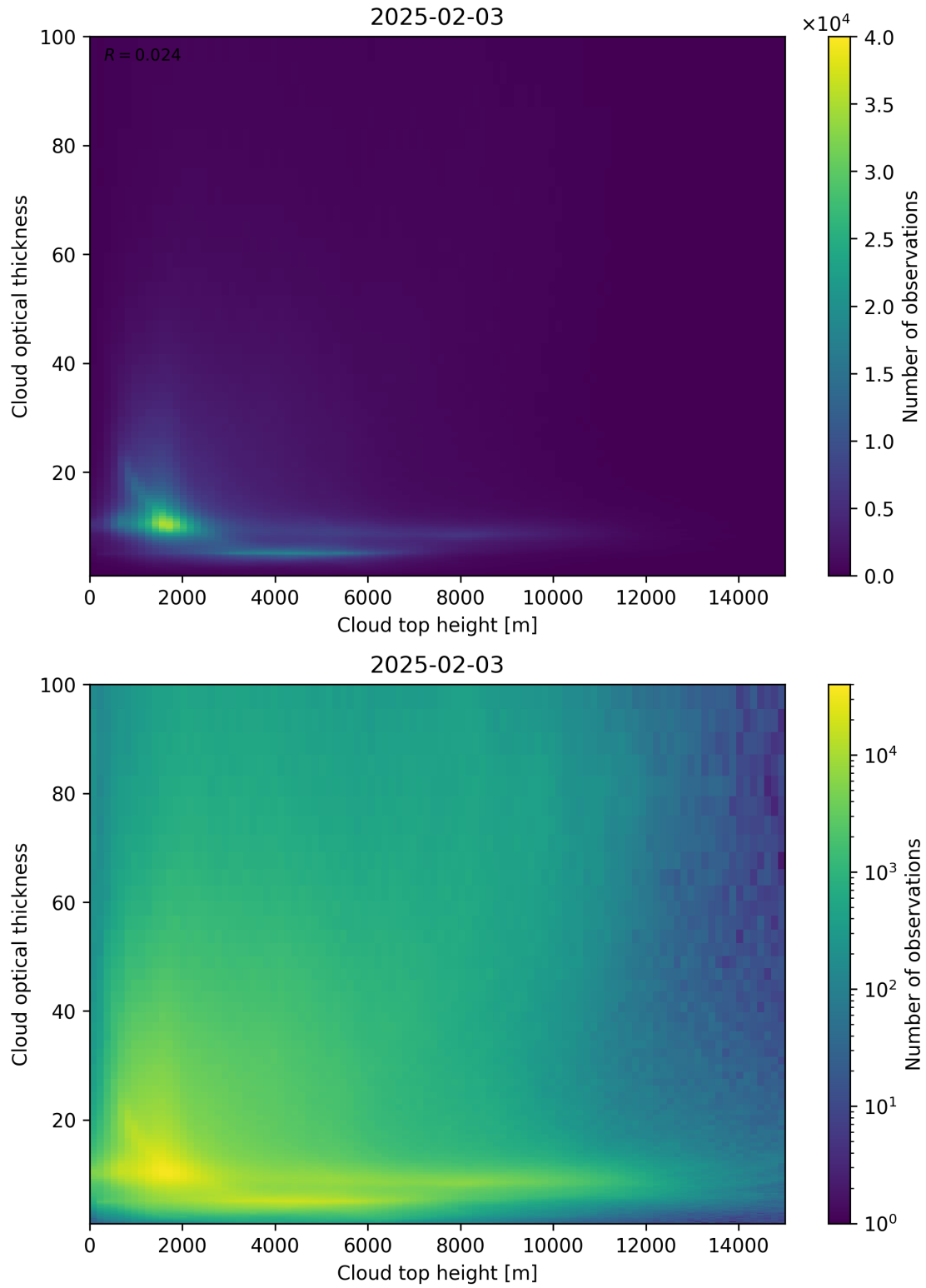
Figure 90: Scatter density plot of “Cloud top height” against “Cloud optical thickness” for 2025-02-03 to 2025-02-04.
