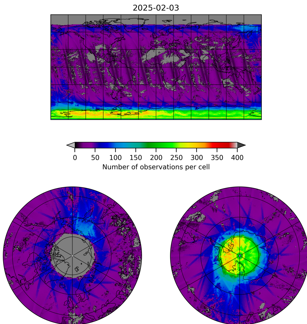
Figure 21: Map of the number of observations for 2025-02-03 to 2025-02-04
