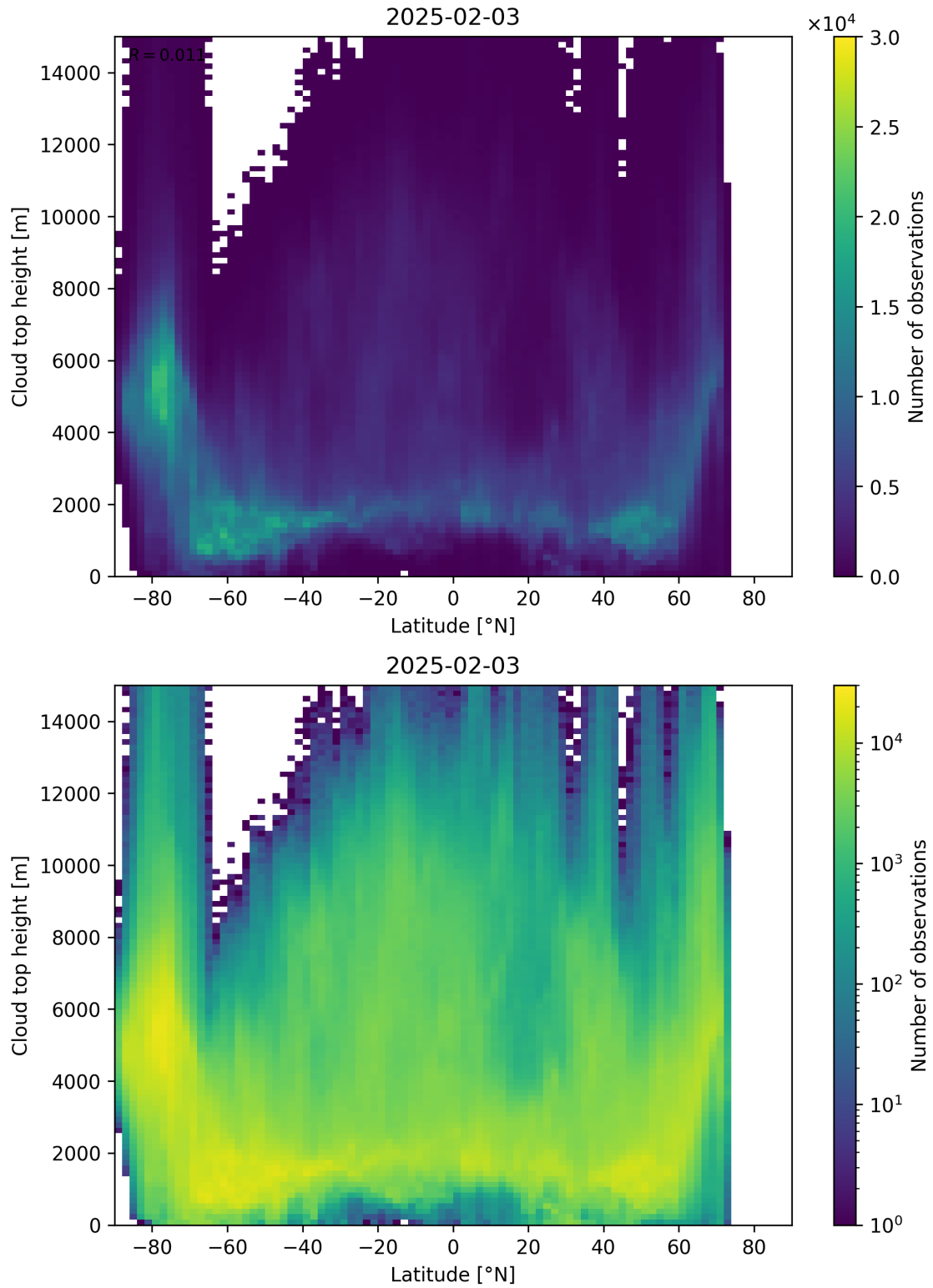
Figure 97: Scatter density plot of “Latitude” against “Cloud top height” for 2025-02-03 to 2025-02-04.
