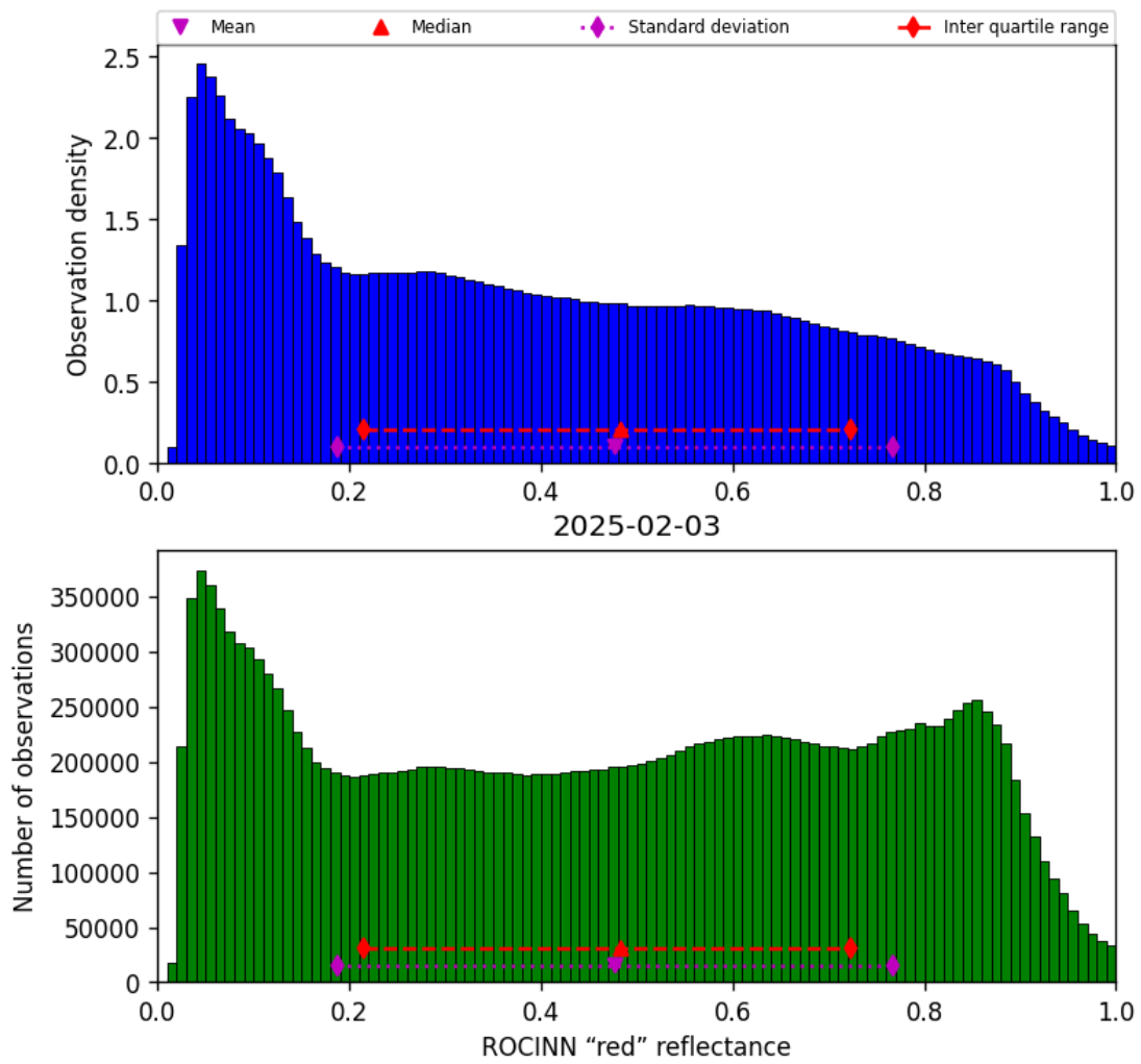
Figure 53: Histogram of “ROCINN “red” reflectance” for 2025-02-03 to 2025-02-04
