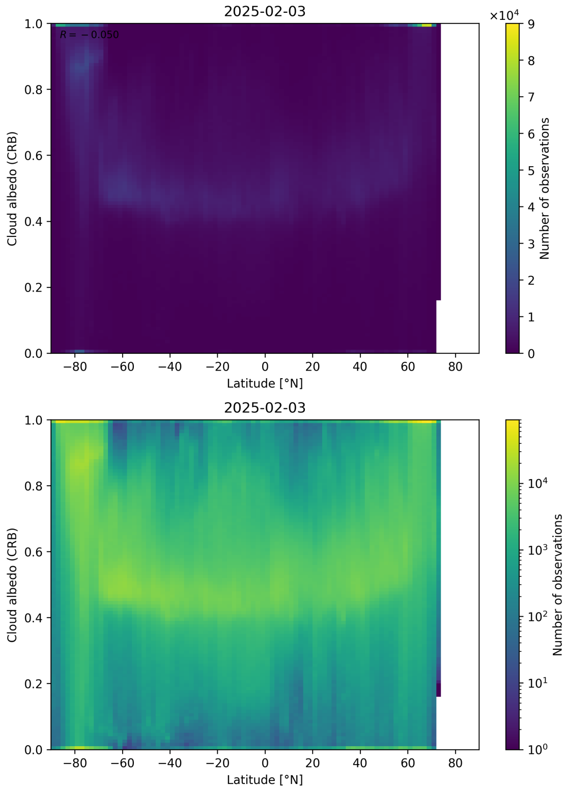
Figure 91: Scatter density plot of “Latitude” against “Cloud albedo (CRB)” for 2025-02-03 to 2025-02-04.
