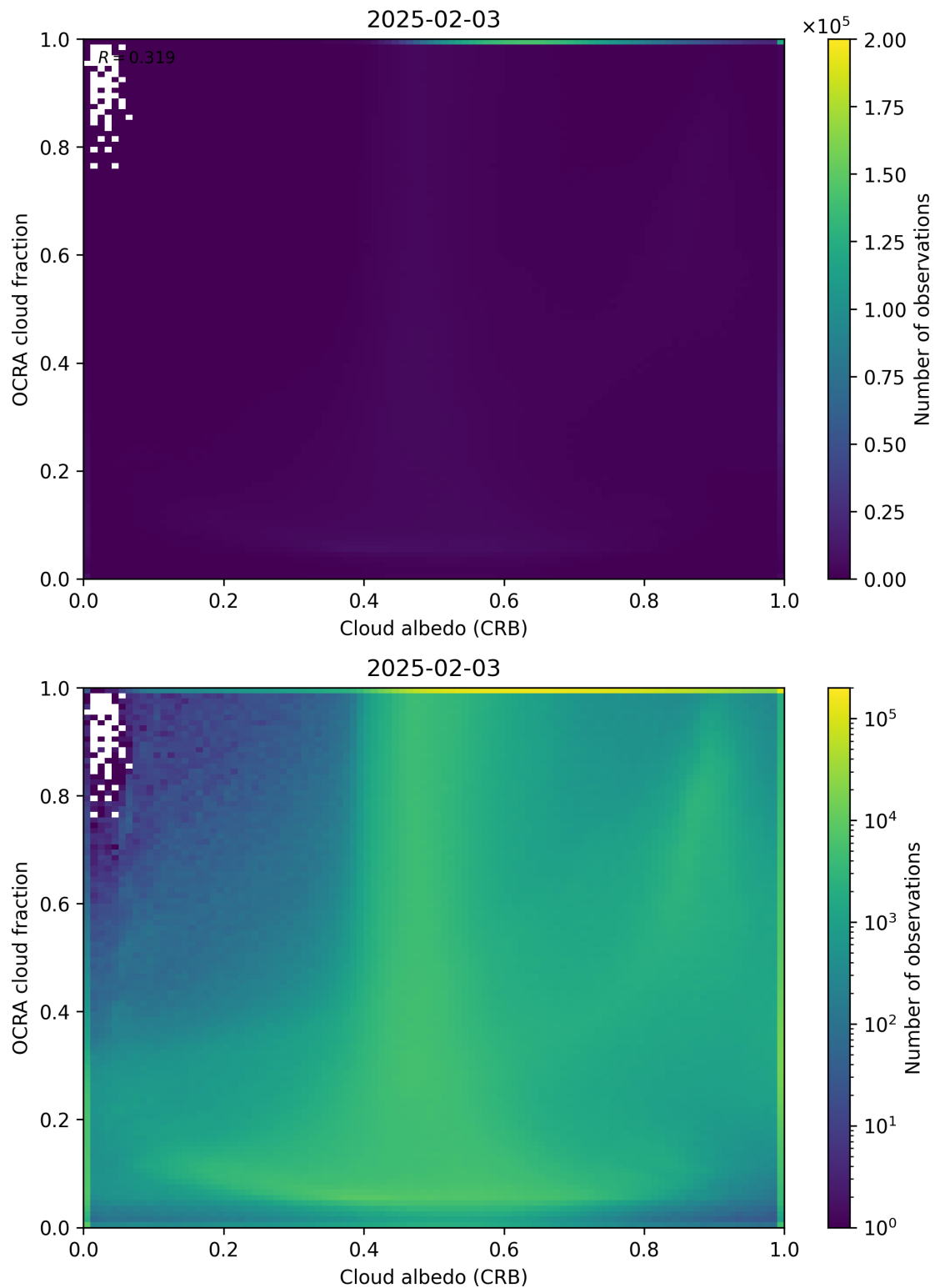
Figure 70: Scatter density plot of “Cloud albedo (CRB)” against “OCRA cloud fraction” for 2025-02-03 to 2025-02-04.
