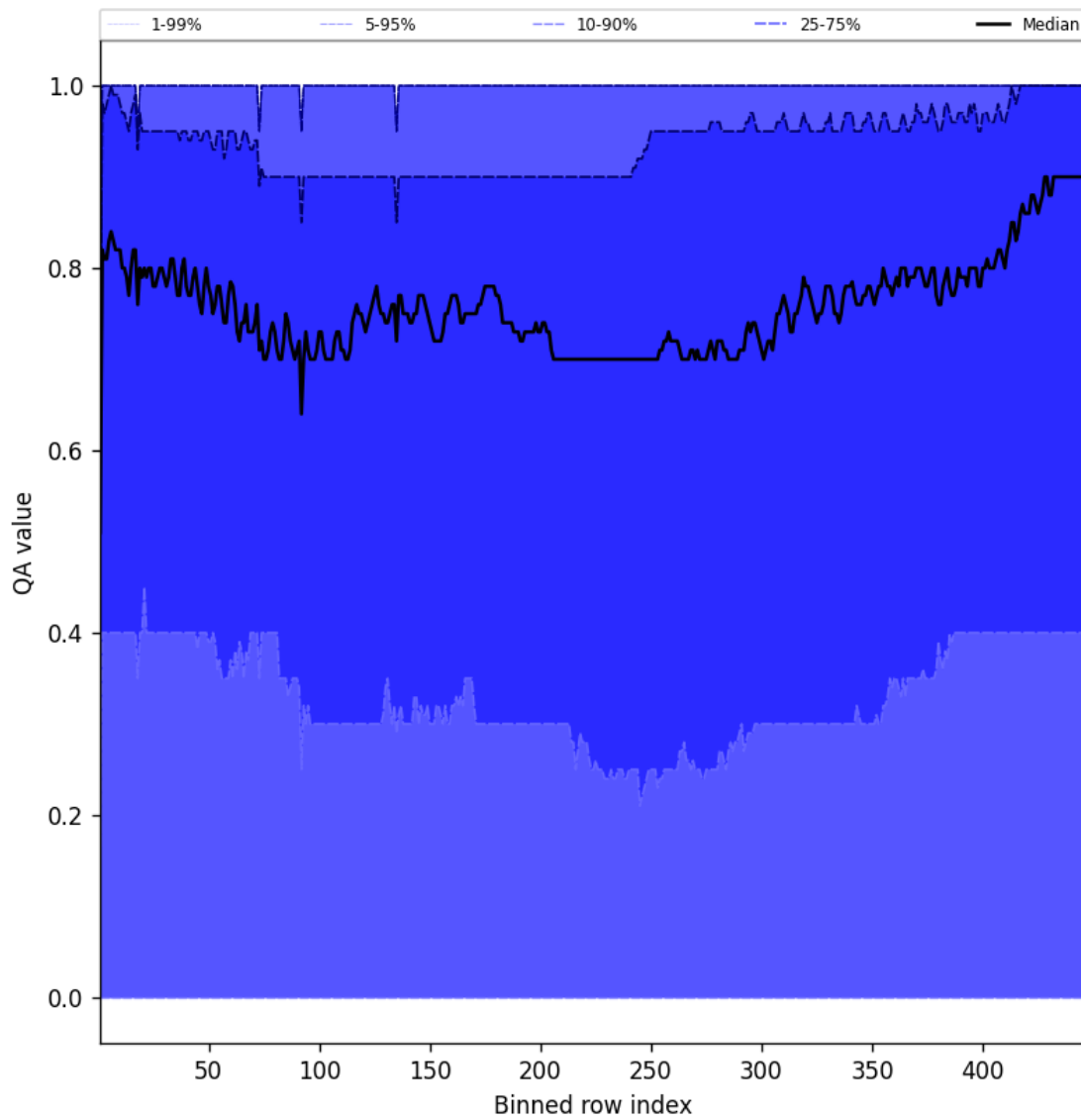
Figure 54: Along track statistics of “QA value” for 2025-02-03 to 2025-02-04
