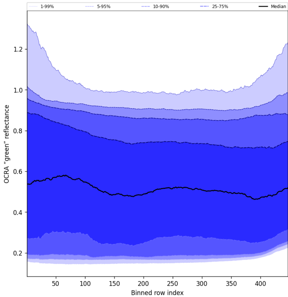
Figure 68: Along track statistics of "OCRA "green" reflectance" for 2025-02-03 to 2025-02-04
