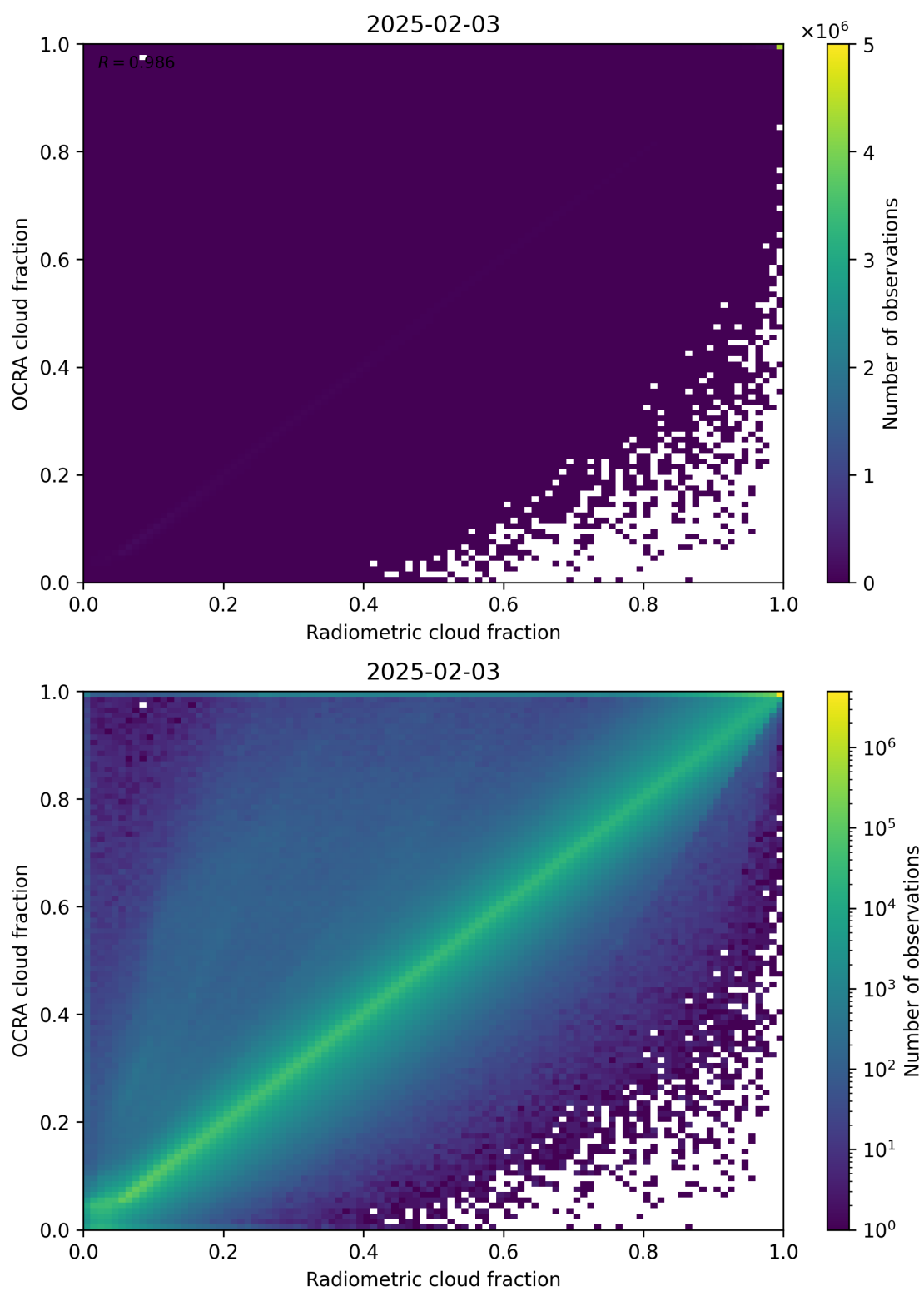
Figure 72: Scatter density plot of “Radiometric cloud fraction” against “OCRA cloud fraction” for 2025-02-03 to 2025-02-04.
