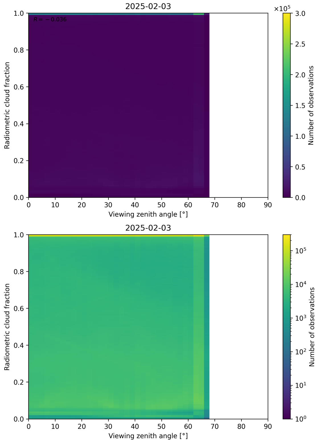
Figure 107: Scatter density plot of “Viewing zenith angle” against “Radiometric cloud fraction” for 2025-02-03 to 2025-02-04.
