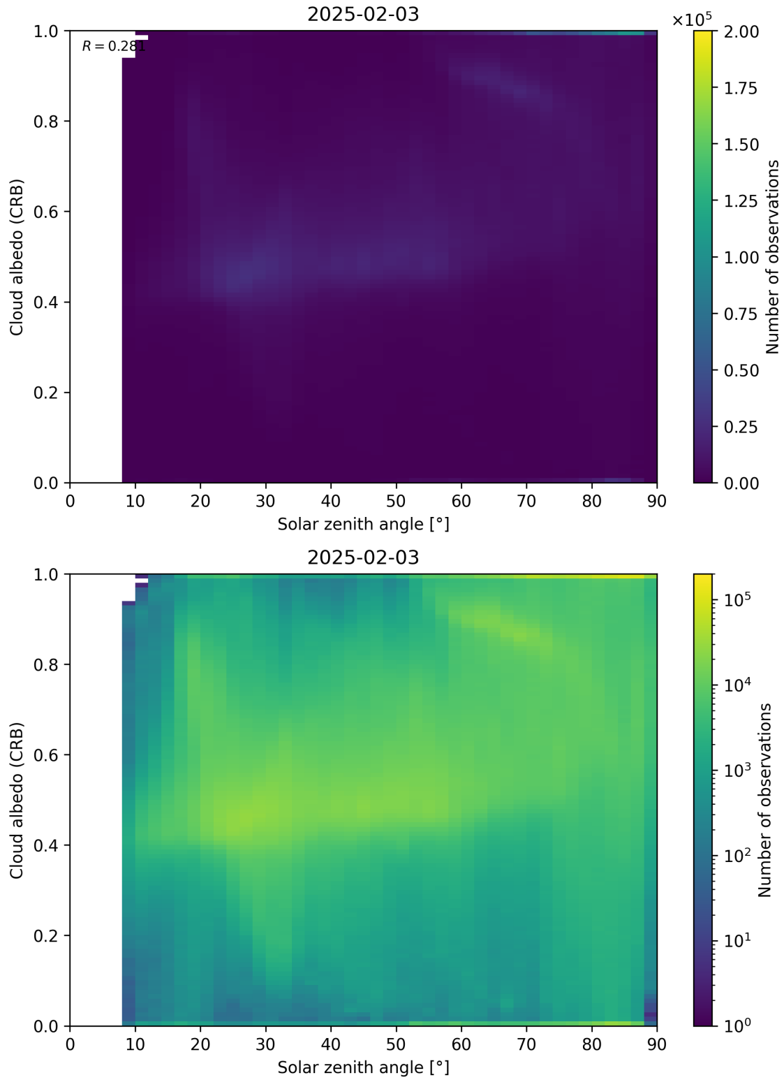
Figure 98: Scatter density plot of “Solar zenith angle” against “Cloud albedo (CRB)” for 2025-02-03 to 2025-02-04.
