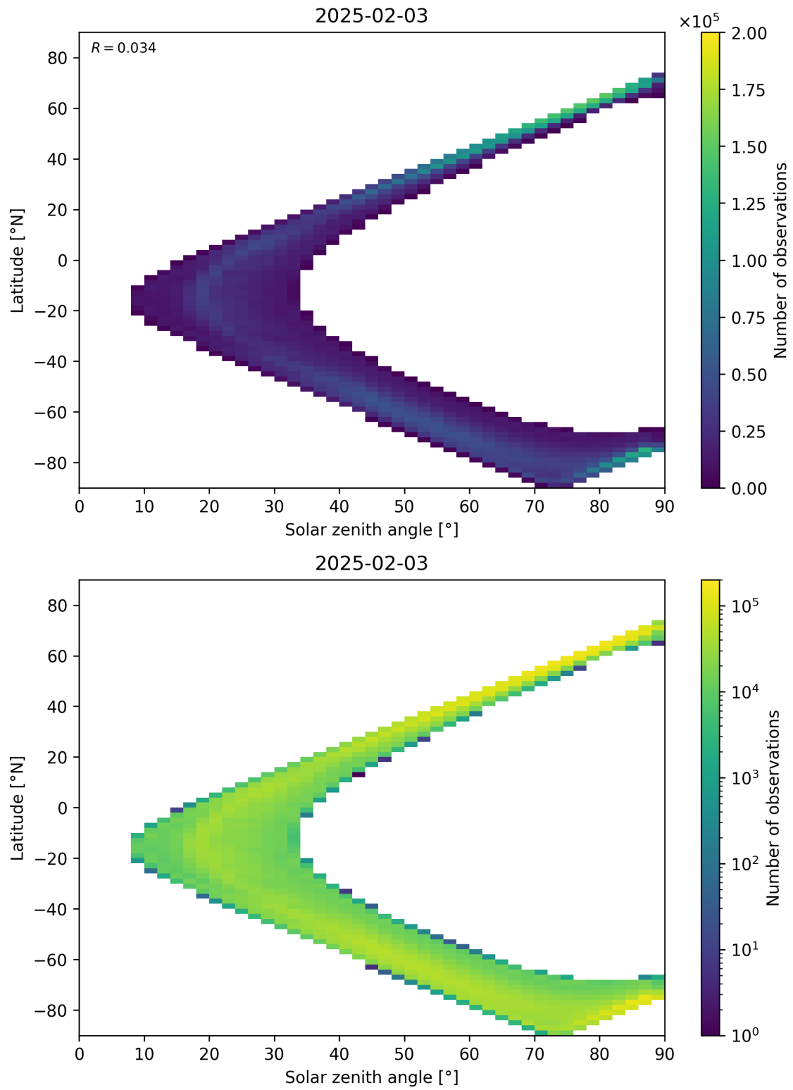
Figure 105: Scatter density plot of “Solar zenith angle” against “Latitude” for 2025-02-03 to 2025-02-04.
