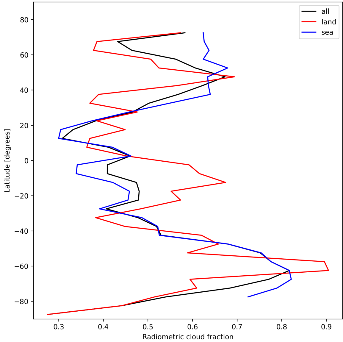
Figure 23: Zonal average of “Radiometric cloud fraction” for 2025-02-03 to 2025-02-04.
