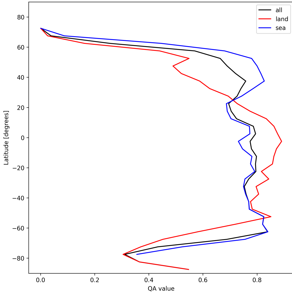
Figure 22: Zonal average of “QA value” for 2025-02-03 to 2025-02-04.
