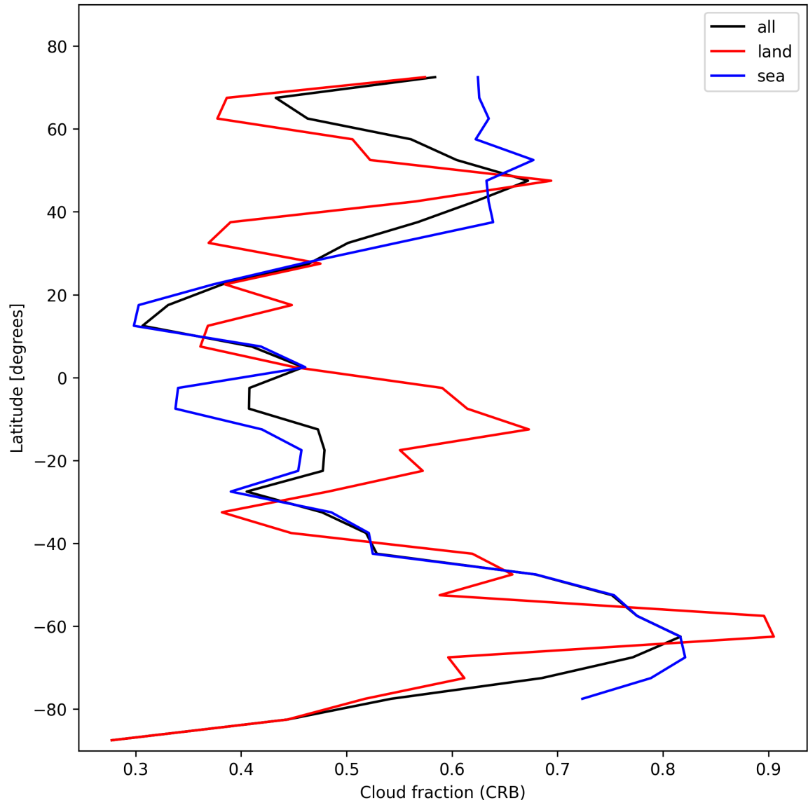
Figure 26: Zonal average of “Cloud fraction (CRB)” for 2025-02-03 to 2025-02-04.
