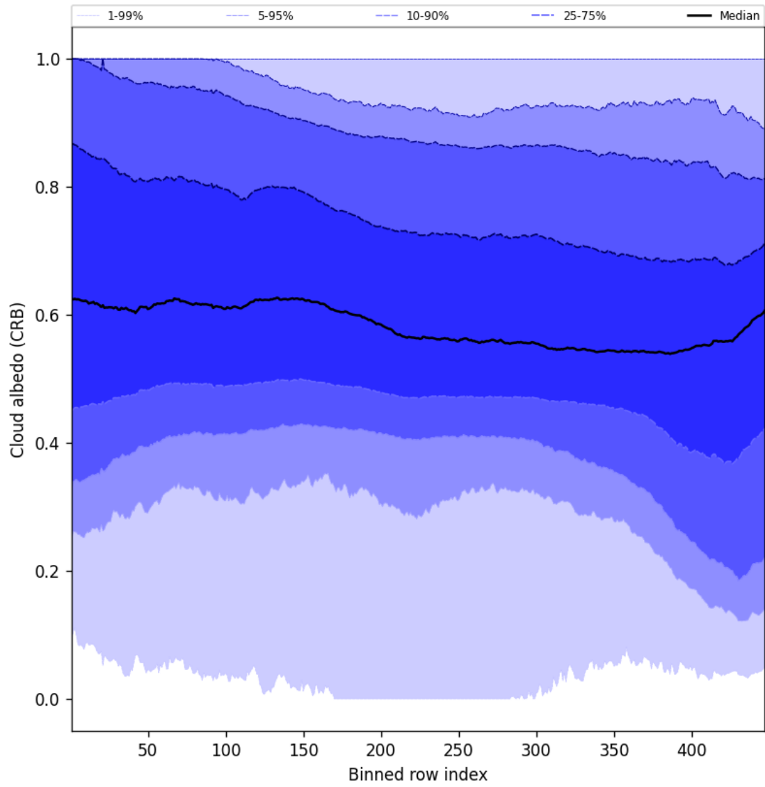
Figure 60: Along track statistics of “Cloud albedo (CRB)” for 2025-02-03 to 2025-02-04
