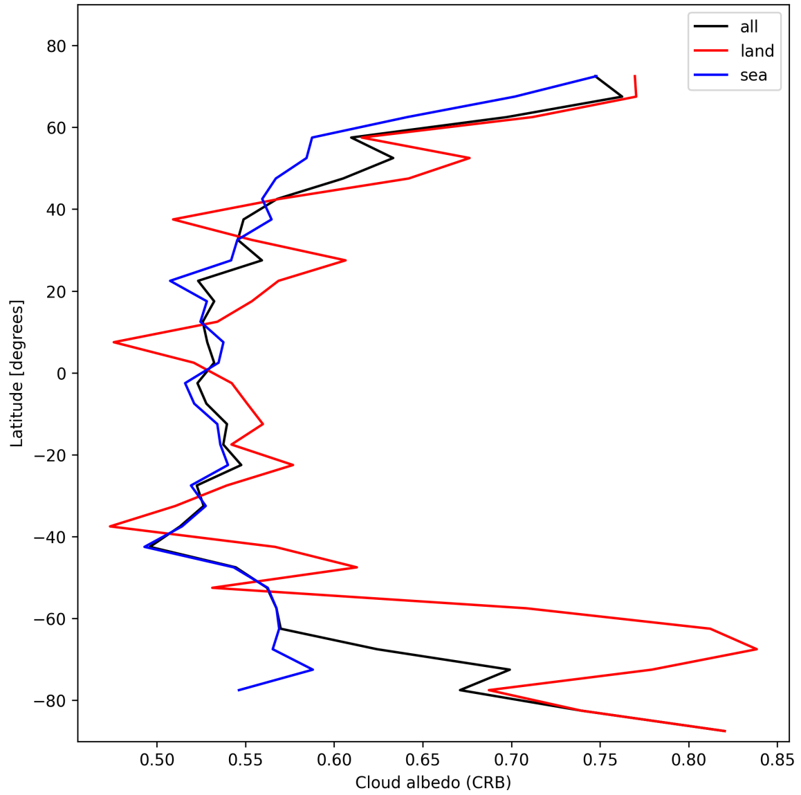
Figure 28: Zonal average of “Cloud albedo (CRB)” for 2025-02-03 to 2025-02-04.
