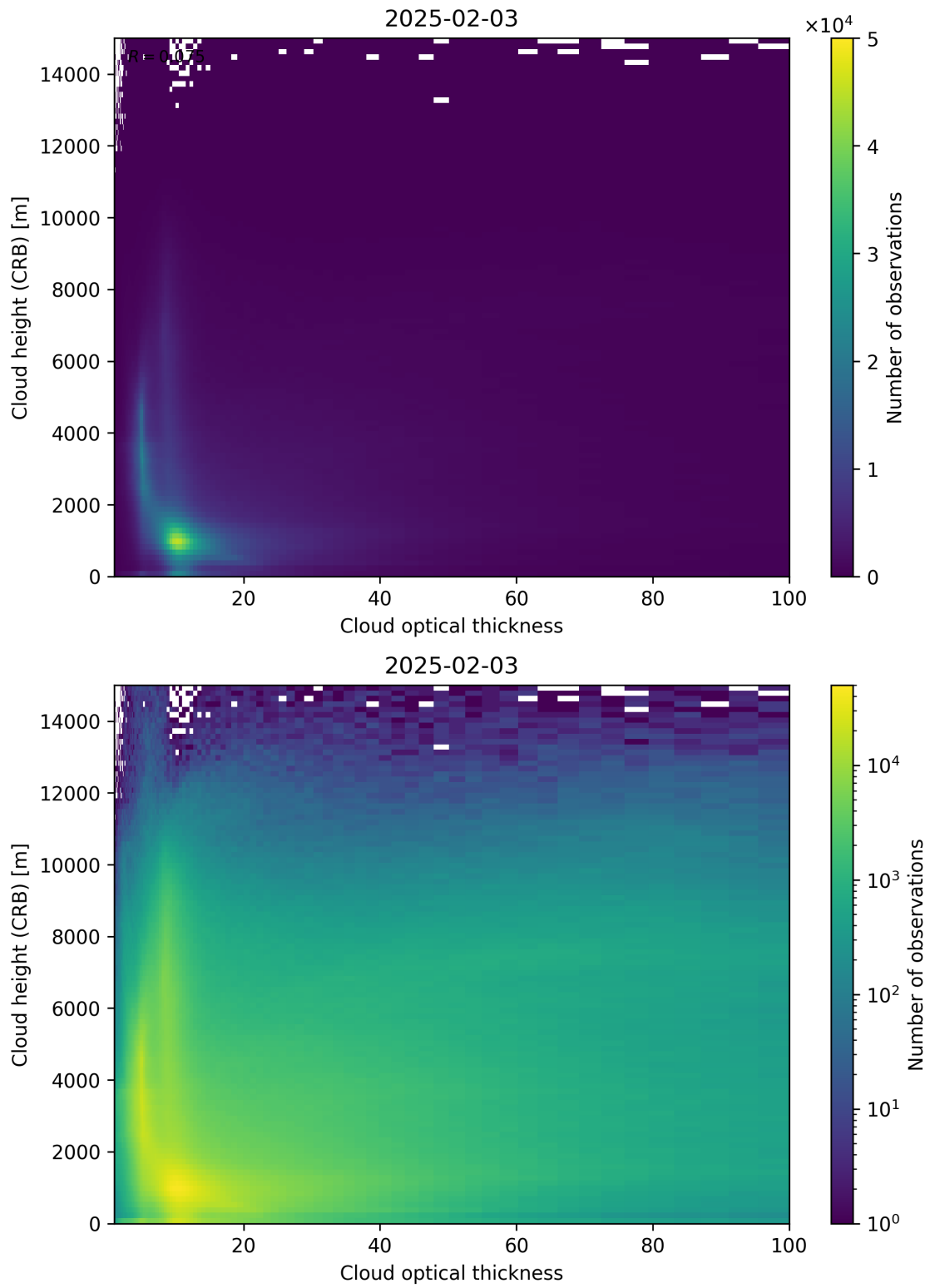
Figure 85: Scatter density plot of “Cloud optical thickness” against “Cloud height (CRB)” for 2025-02-03 to 2025-02-04.
