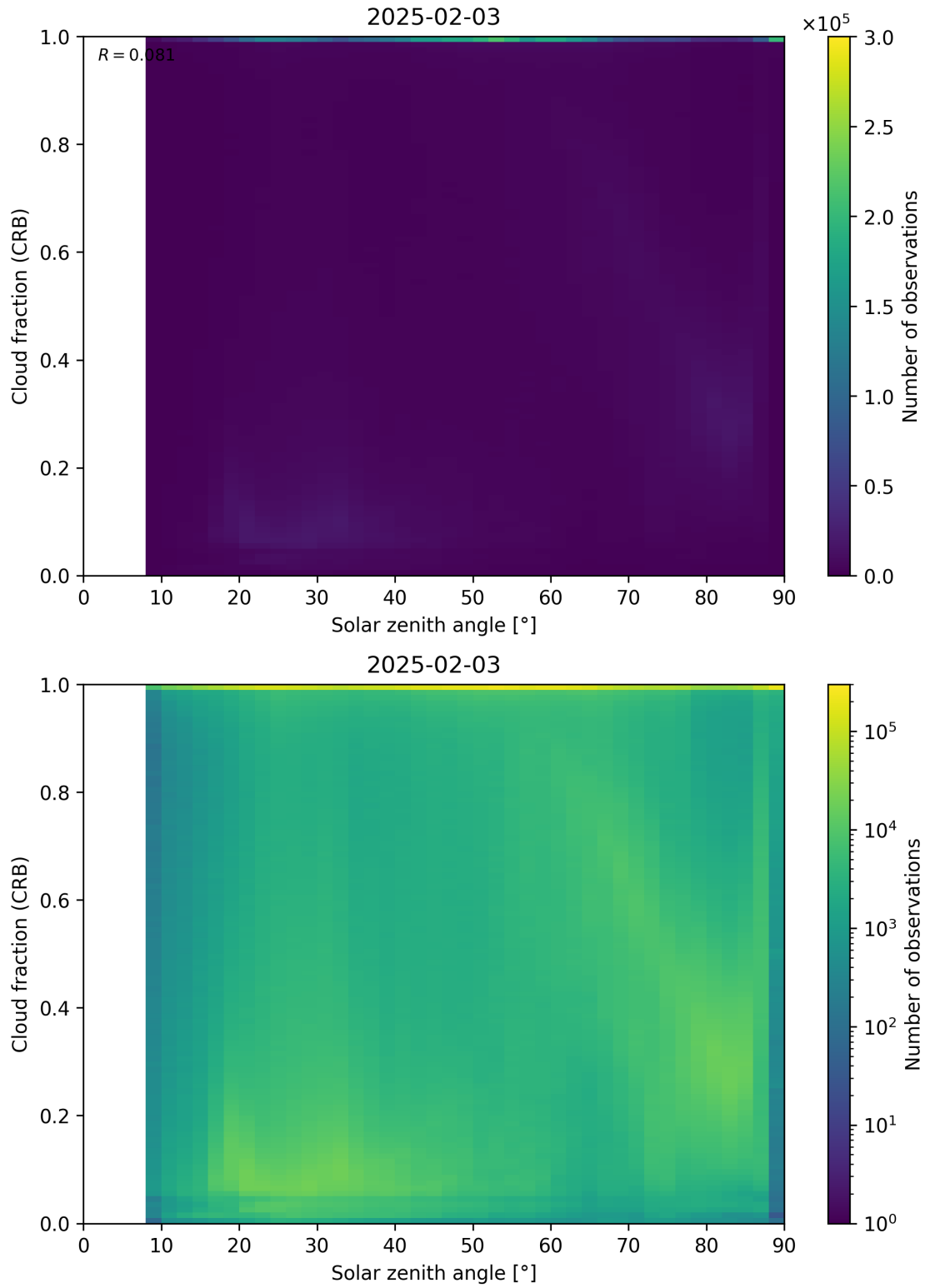
Figure 101: Scatter density plot of “Solar zenith angle” against “Cloud fraction (CRB)” for 2025-02-03 to 2025-02-04.
