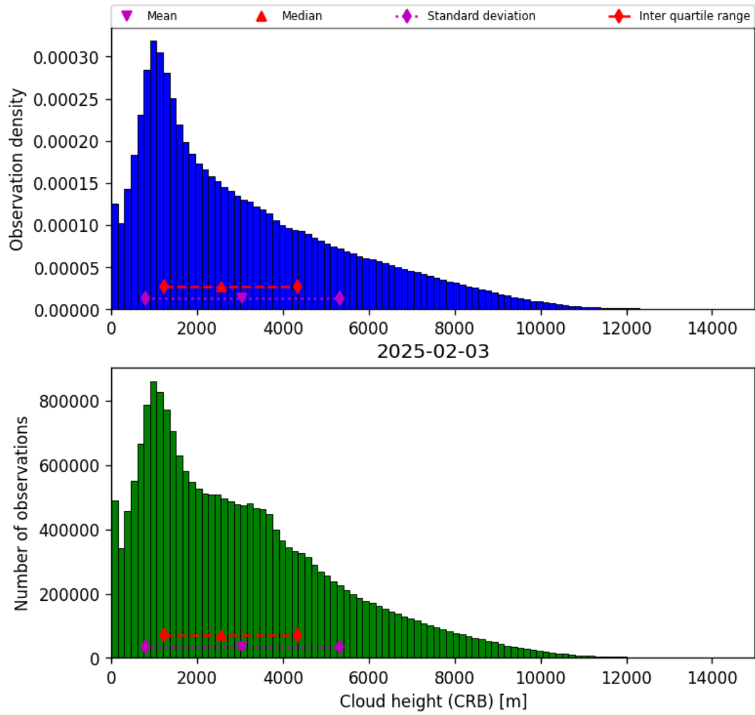
Figure 43: Histogram of “Cloud height (CRB)” for 2025-02-03 to 2025-02-04
