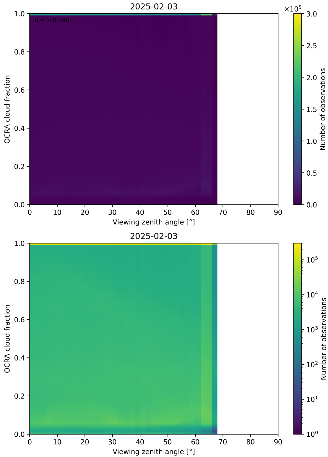
Figure 108: Scatter density plot of “Viewing zenith angle” against “OCRA cloud fraction” for 2025-02-03 to 2025-02-04.
