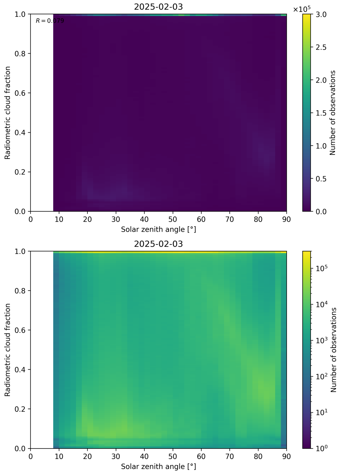
Figure 99: Scatter density plot of “Solar zenith angle” against “Radiometric cloud fraction” for 2025-02-03 to 2025-02-04.
