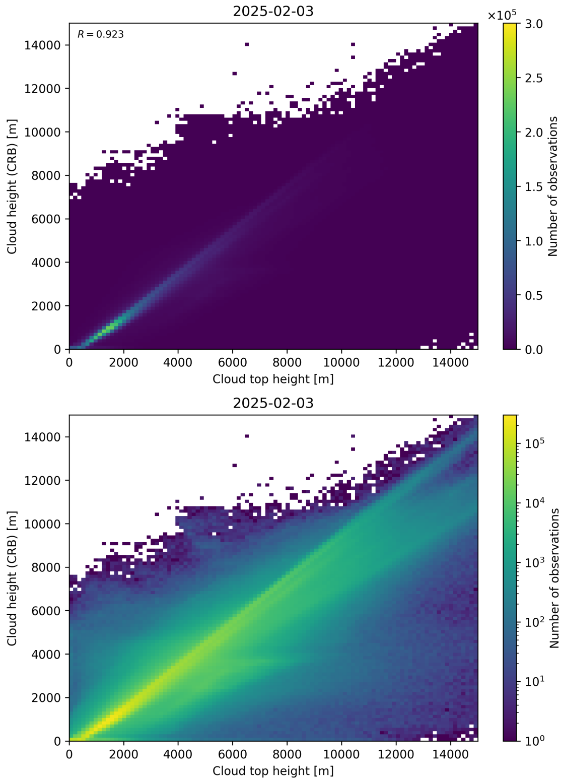
Figure 89: Scatter density plot of “Cloud top height” against “Cloud height (CRB)” for 2025-02-03 to 2025-02-04.
