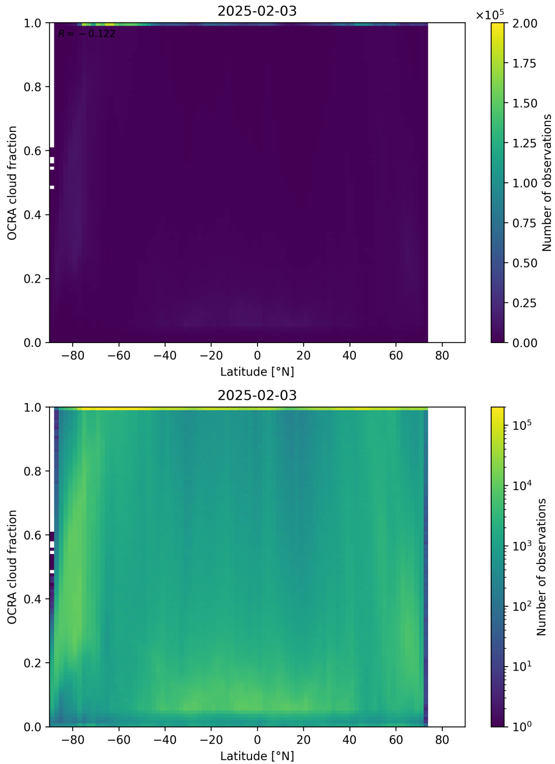
Figure 93: Scatter density plot of “Latitude” against “OCRA cloud fraction” for 2025-02-03 to 2025-02-04.
