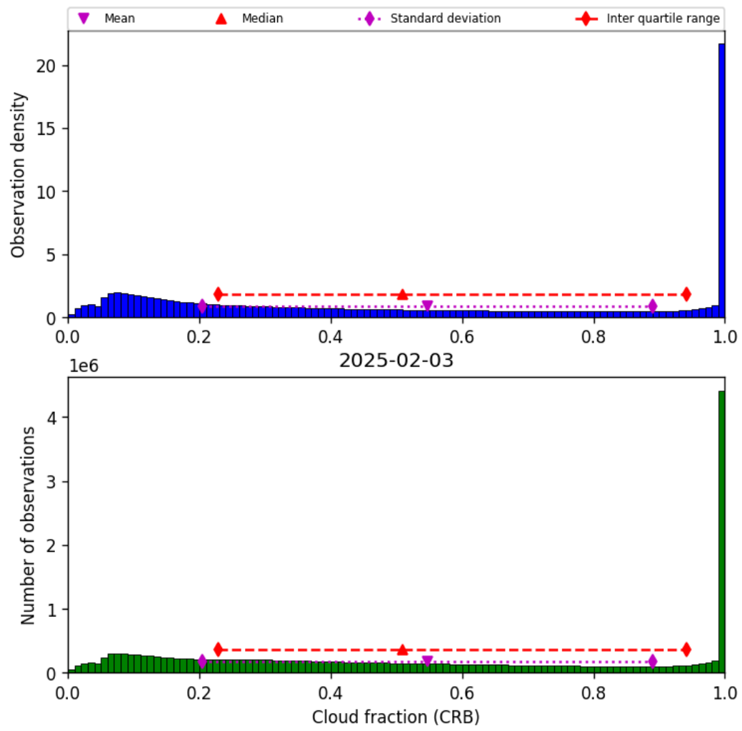
Figure 42: Histogram of “Cloud fraction (CRB)” for 2025-02-03 to 2025-02-04
