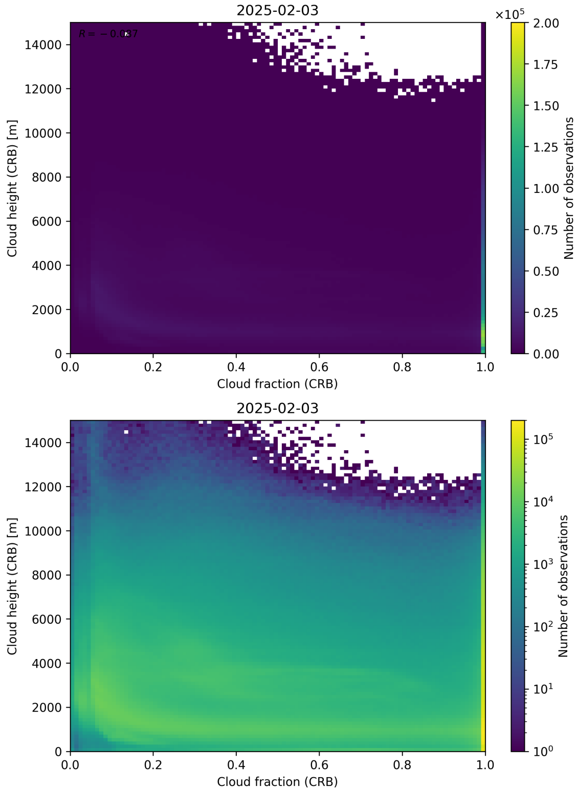
Figure 79: Scatter density plot of “Cloud fraction (CRB)” against “Cloud height (CRB)” for 2025-02-03 to 2025-02-04.
