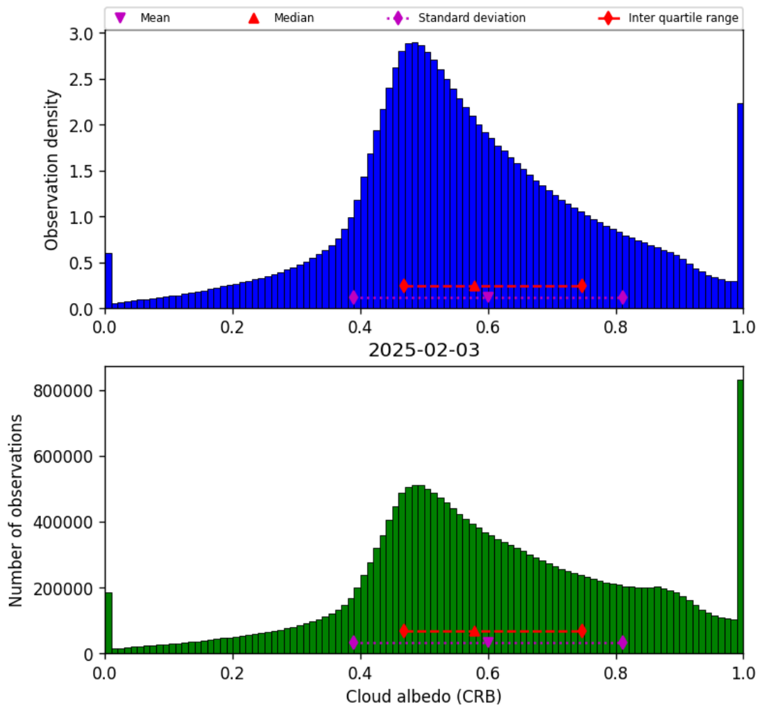
Figure 44: Histogram of “Cloud albedo (CRB)” for 2025-02-03 to 2025-02-04
