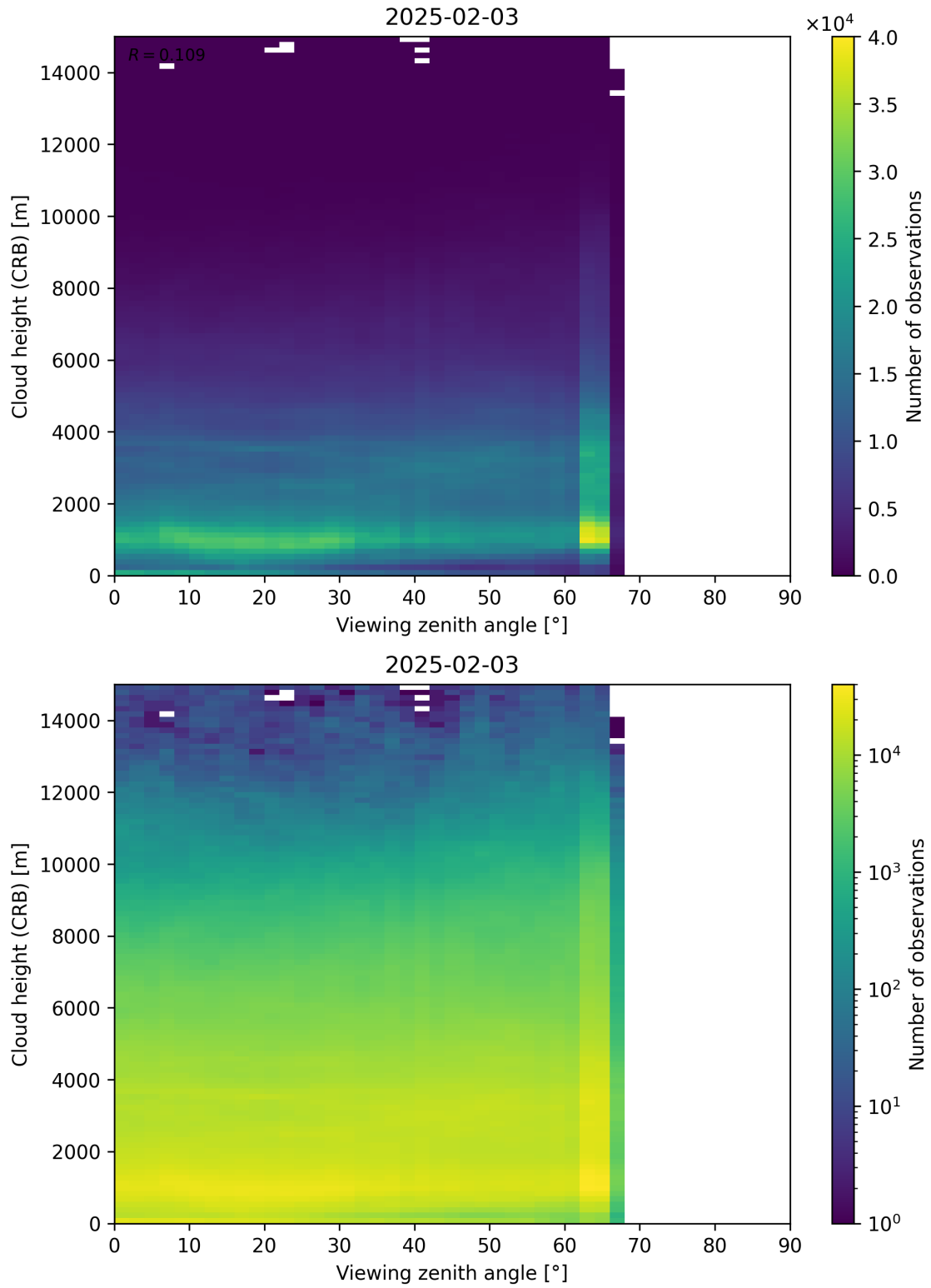
Figure 110: Scatter density plot of “Viewing zenith angle” against “Cloud height (CRB)” for 2025-02-03 to 2025-02-04.
