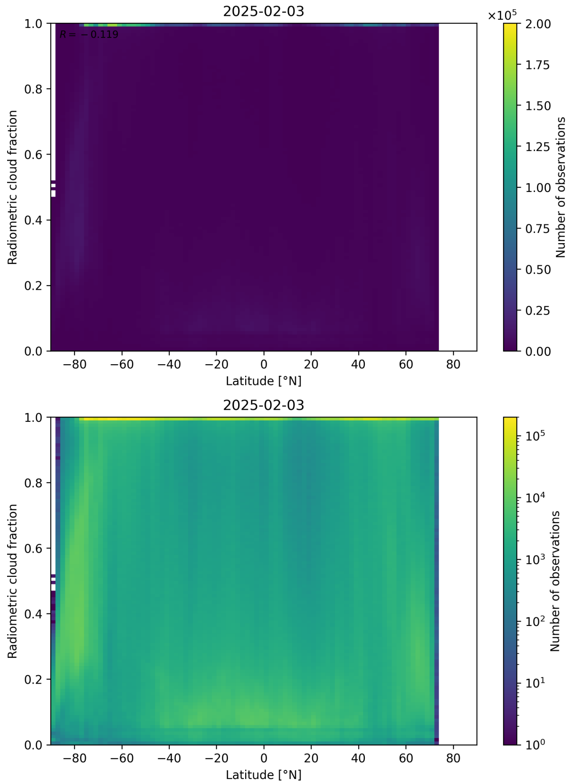
Figure 92: Scatter density plot of “Latitude” against “Radiometric cloud fraction” for 2025-02-03 to 2025-02-04.
