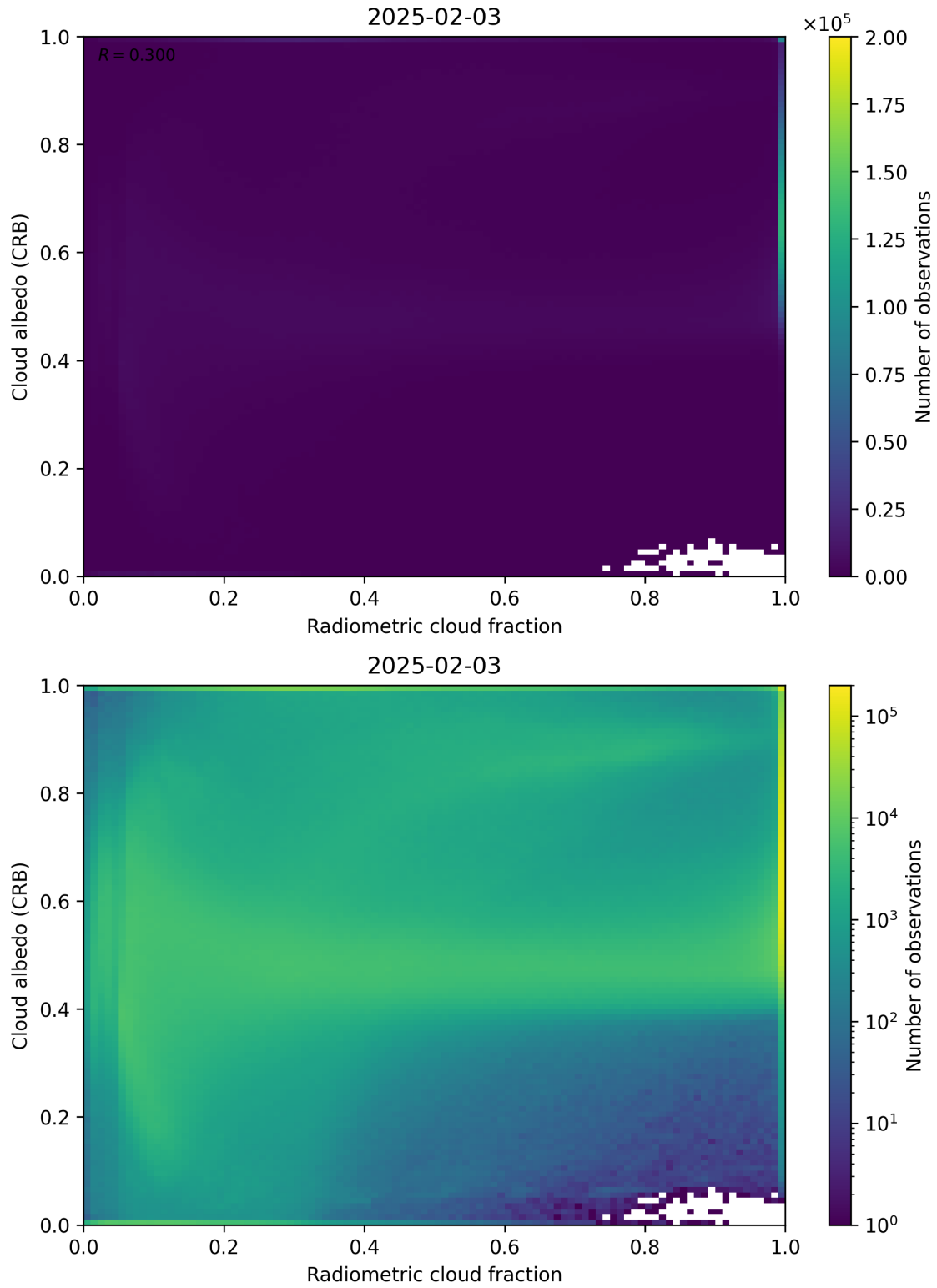
Figure 71: Scatter density plot of “Radiometric cloud fraction” against “Cloud albedo (CRB)” for 2025-02-03 to 2025-02-04.
