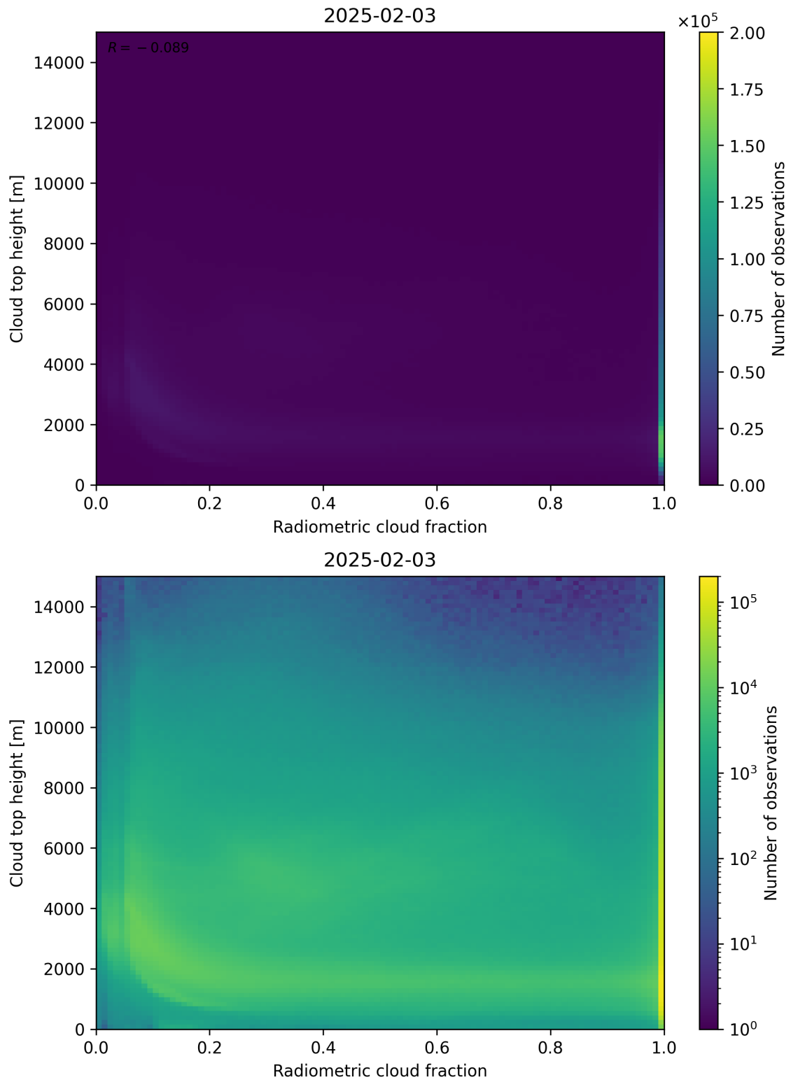
Figure 76: Scatter density plot of “Radiometric cloud fraction” against “Cloud top height” for 2025-02-03 to 2025-02-04.
