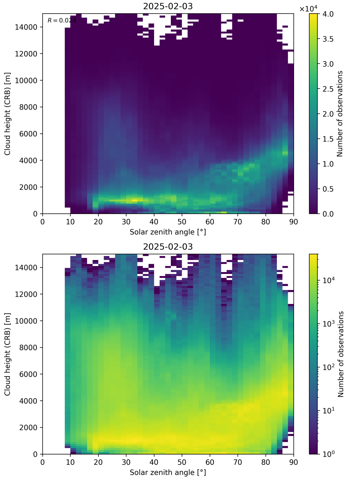
Figure 102: Scatter density plot of “Solar zenith angle” against “Cloud height (CRB)” for 2025-02-03 to 2025-02-04.
