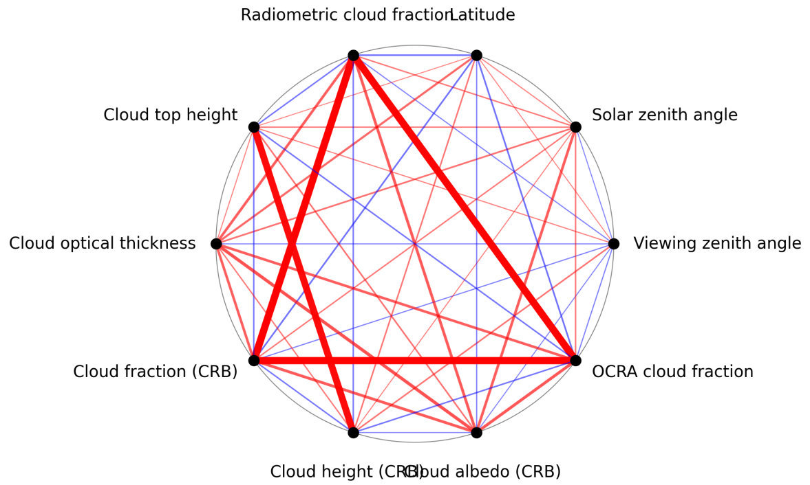
Figure 1: Map of correlation graph for 2025-02-03 to 2025-02-04.
