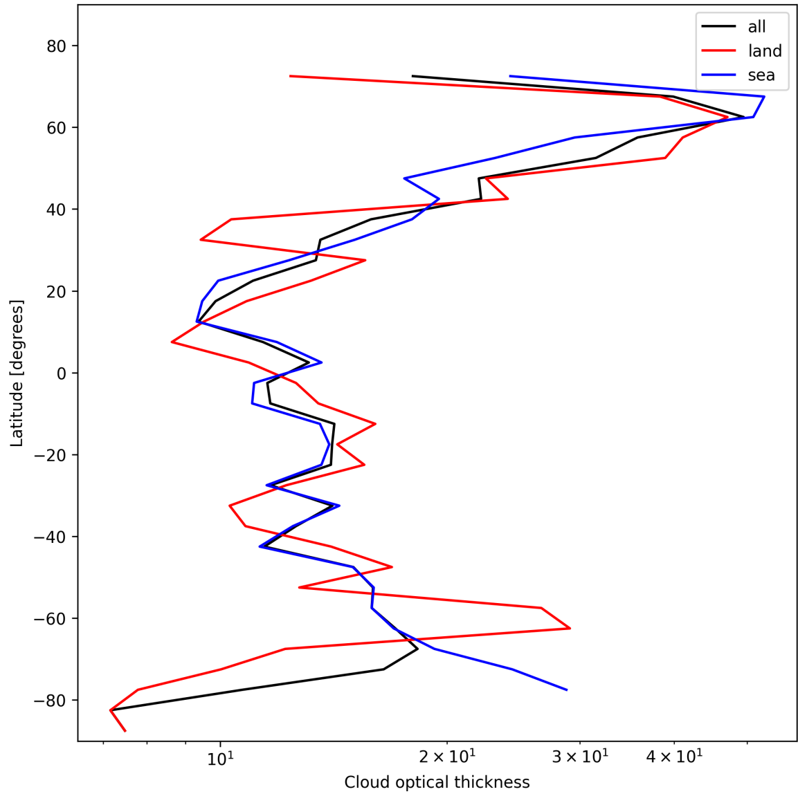
Figure 25: Zonal average of “Cloud optical thickness” for 2025-02-03 to 2025-02-04.
