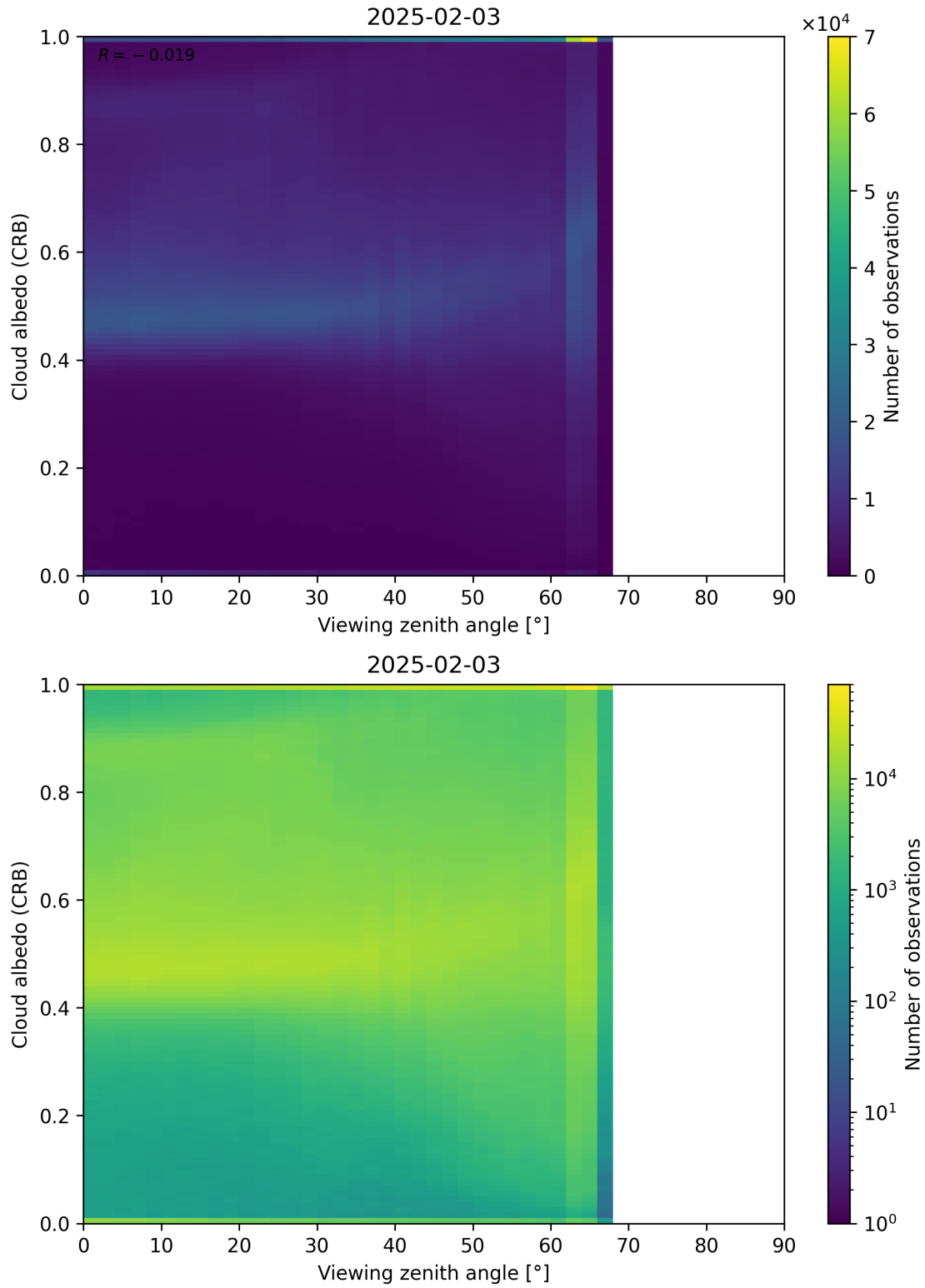
Figure 106: Scatter density plot of “Viewing zenith angle” against “Cloud albedo (CRB)” for 2025-02-03 to 2025-02-04.
