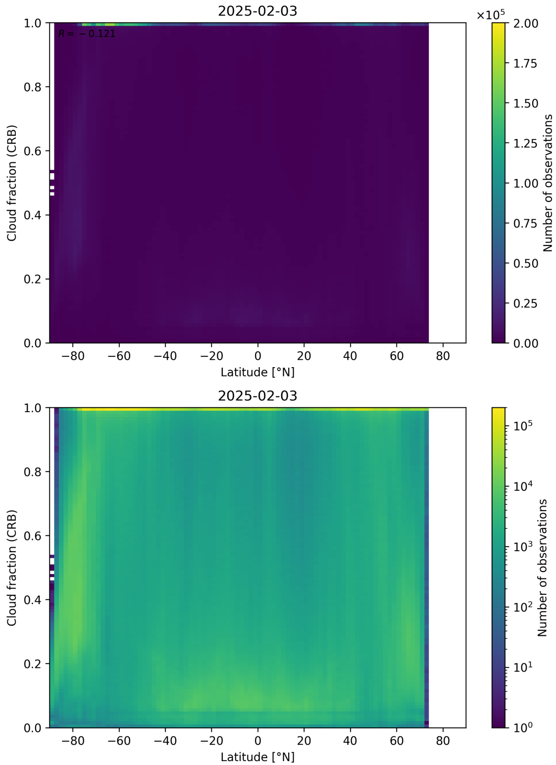
Figure 94: Scatter density plot of “Latitude” against “Cloud fraction (CRB)” for 2025-02-03 to 2025-02-04.
