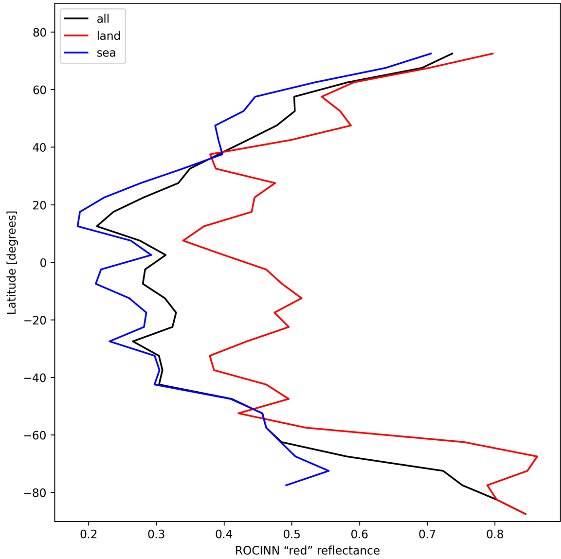
Figure 37: Zonal average of “ROCINN “red” reflectance” for 2025-02-03 to 2025-02-04.
