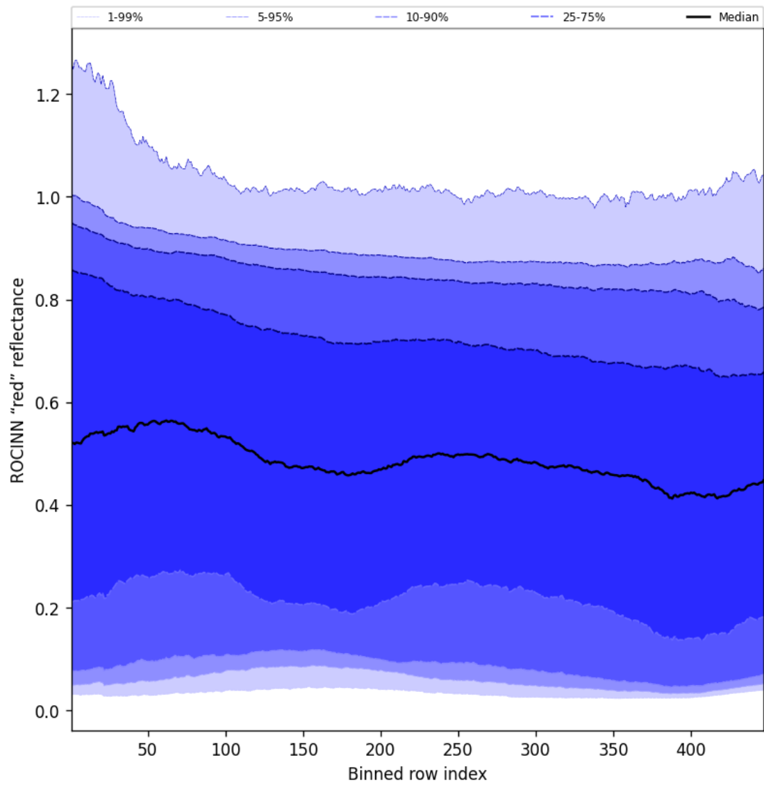
Figure 69: Along track statistics of “ROCINN “red” reflectance” for 2025-02-03 to 2025-02-04
