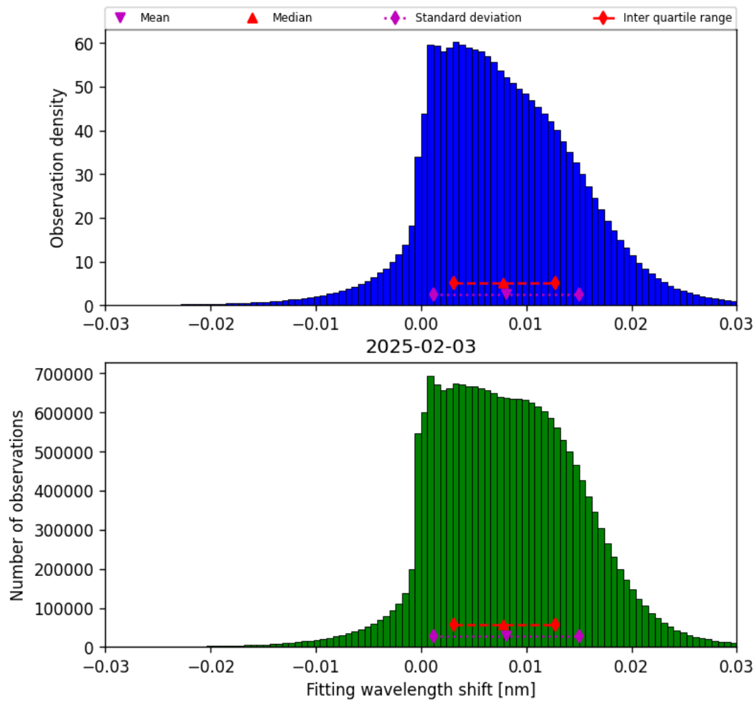
Figure 49: Histogram of “Fitting wavelength shift” for 2025-02-03 to 2025-02-04
