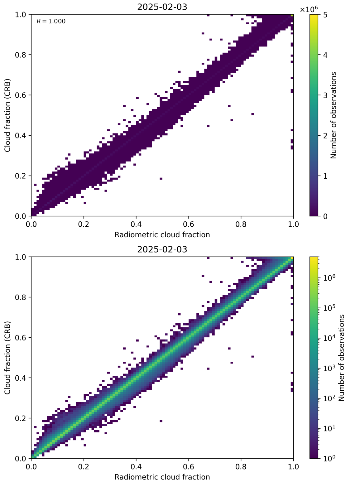
Figure 73: Scatter density plot of “Radiometric cloud fraction” against “Cloud fraction (CRB)” for 2025-02-03 to 2025-02-04.
