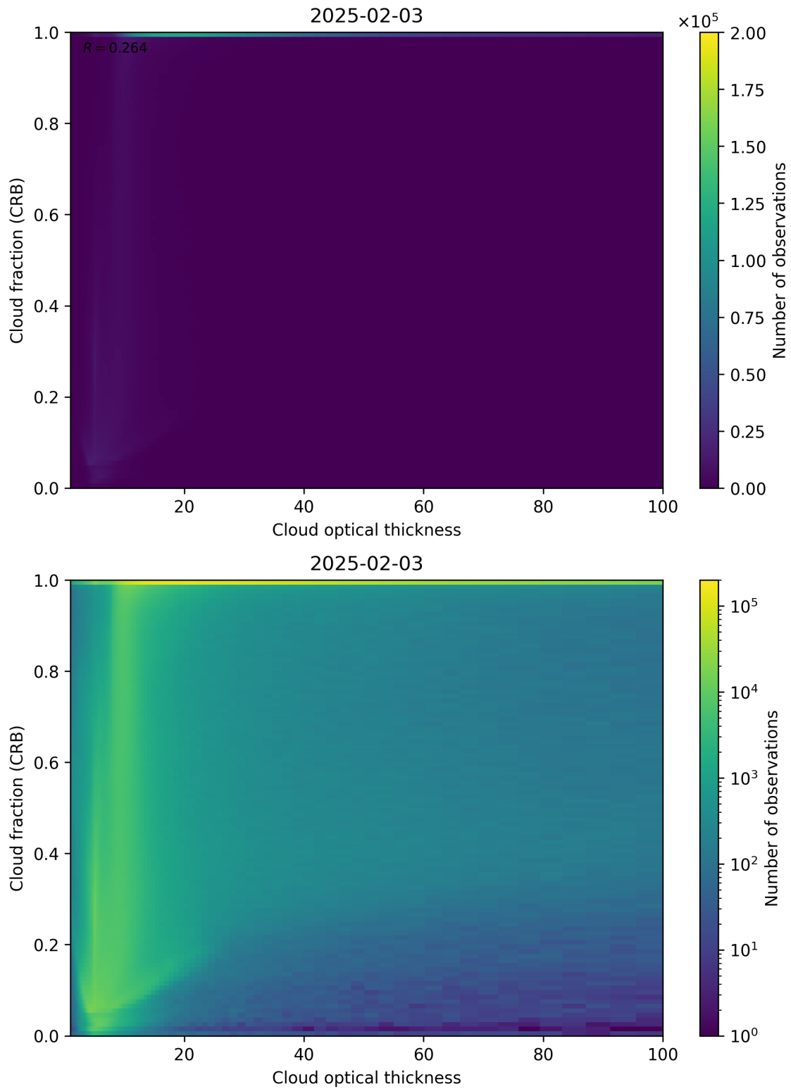
Figure 84: Scatter density plot of “Cloud optical thickness” against “Cloud fraction (CRB)” for 2025-02-03 to 2025-02-04.
