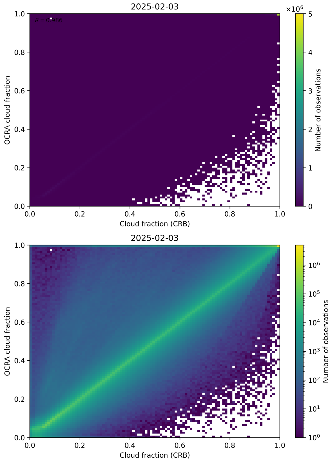
Figure 78: Scatter density plot of “Cloud fraction (CRB)” against “OCRA cloud fraction” for 2025-02-03 to 2025-02-04.
