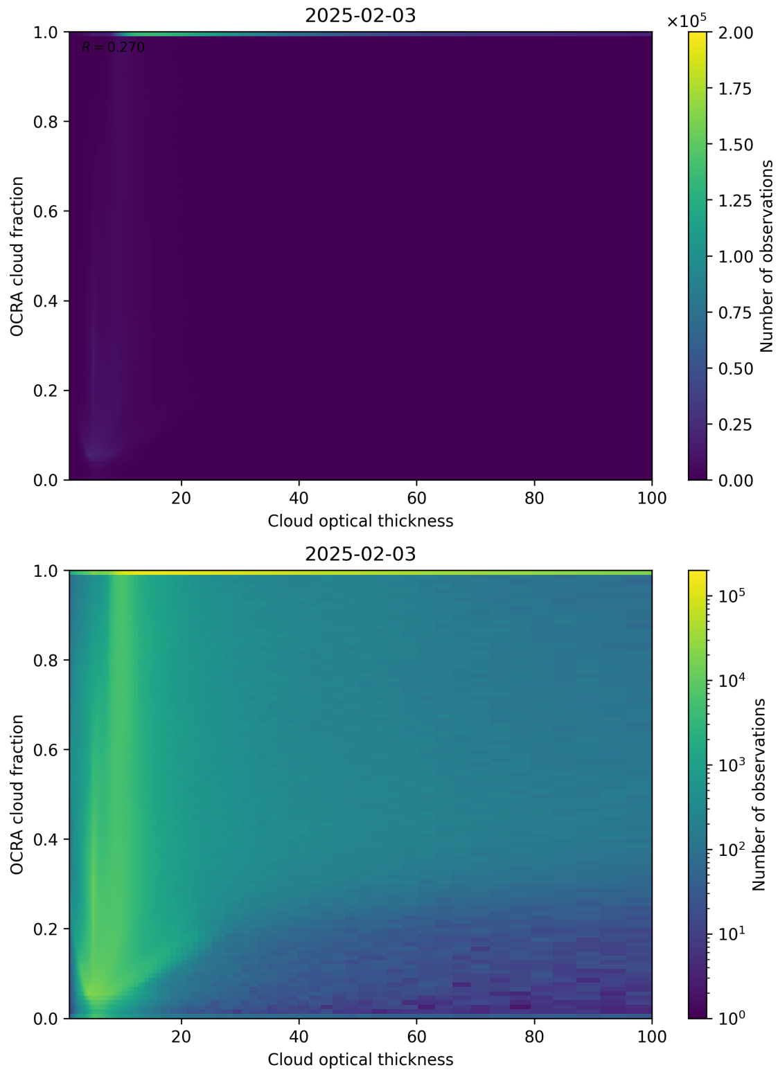
Figure 83: Scatter density plot of “Cloud optical thickness” against “OCRA cloud fraction” for 2025-02-03 to 2025-02-04.
