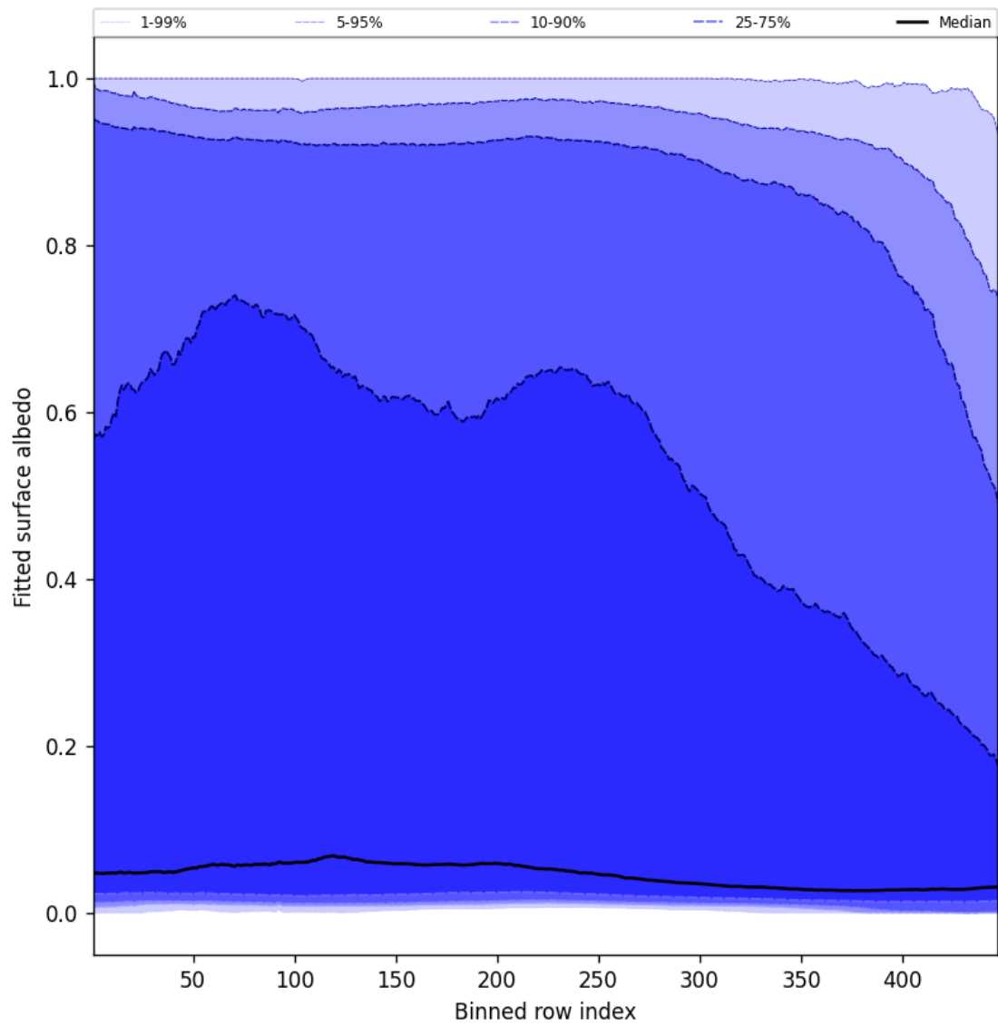
Figure 61: Along track statistics of “Fitted surface albedo” for 2025-02-03 to 2025-02-04
