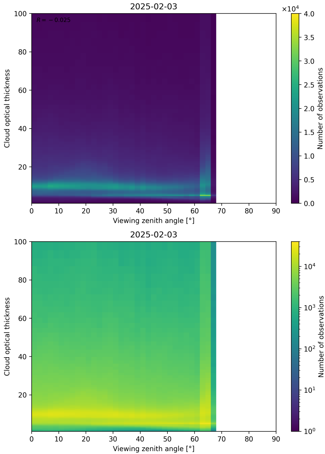
Figure 111: Scatter density plot of “Viewing zenith angle” against “Cloud optical thickness” for 2025-02-03 to 2025-02-04.
