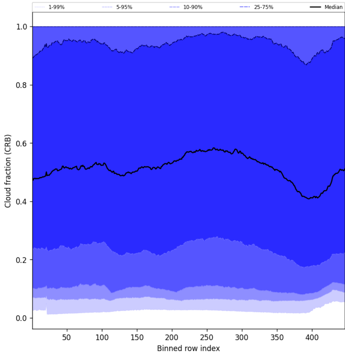
Figure 58: Along track statistics of “Cloud fraction (CRB)” for 2025-02-03 to 2025-02-04
