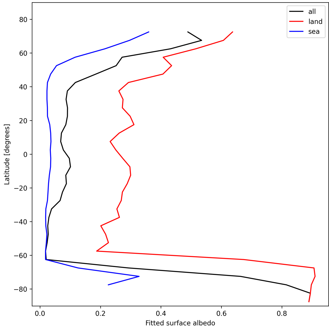
Figure 29: Zonal average of “Fitted surface albedo” for 2025-02-03 to 2025-02-04.
