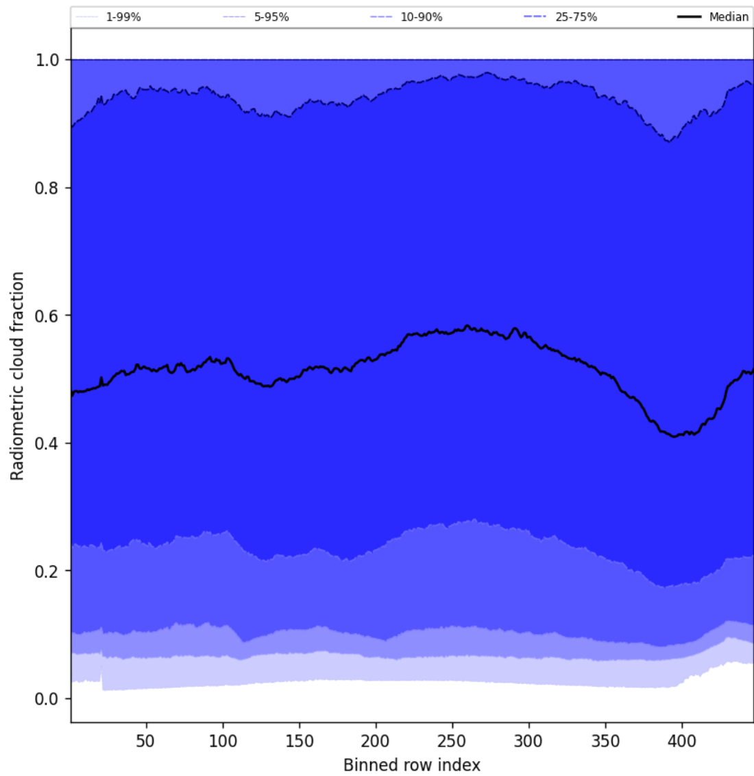
Figure 55: Along track statistics of “Radiometric cloud fraction” for 2025-02-03 to 2025-02-04
