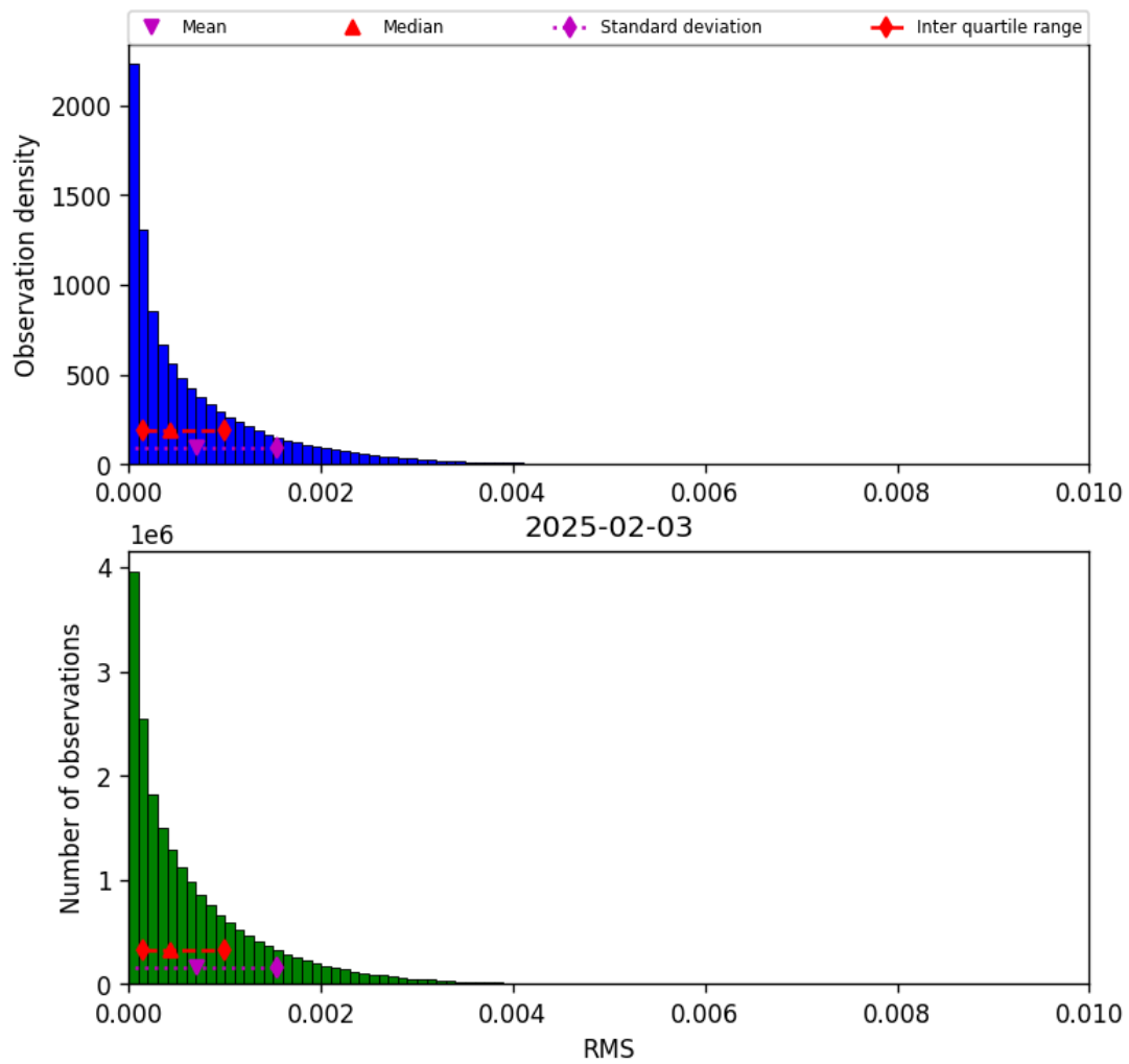
Figure 47: Histogram of “RMS” for 2025-02-03 to 2025-02-04
