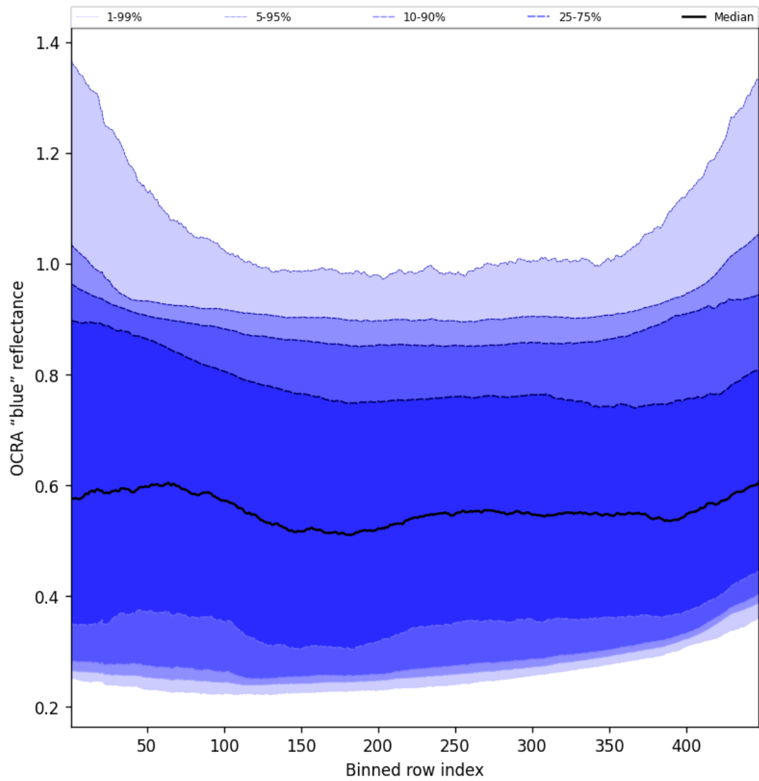
Figure 67: Along track statistics of "OCRA "blue" reflectance" for 2025-02-03 to 2025-02-04
