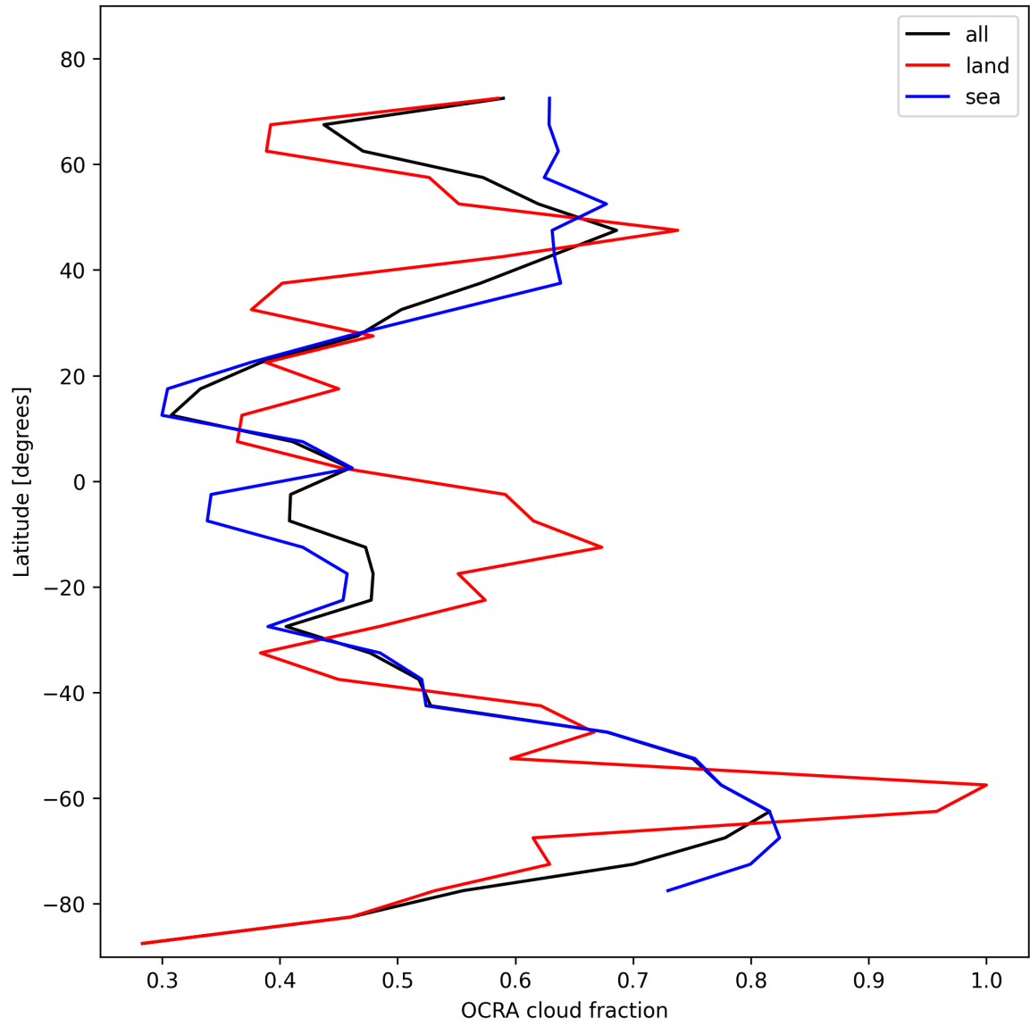
Figure 34: Zonal average of “OCRA cloud fraction” for 2025-02-03 to 2025-02-04.
