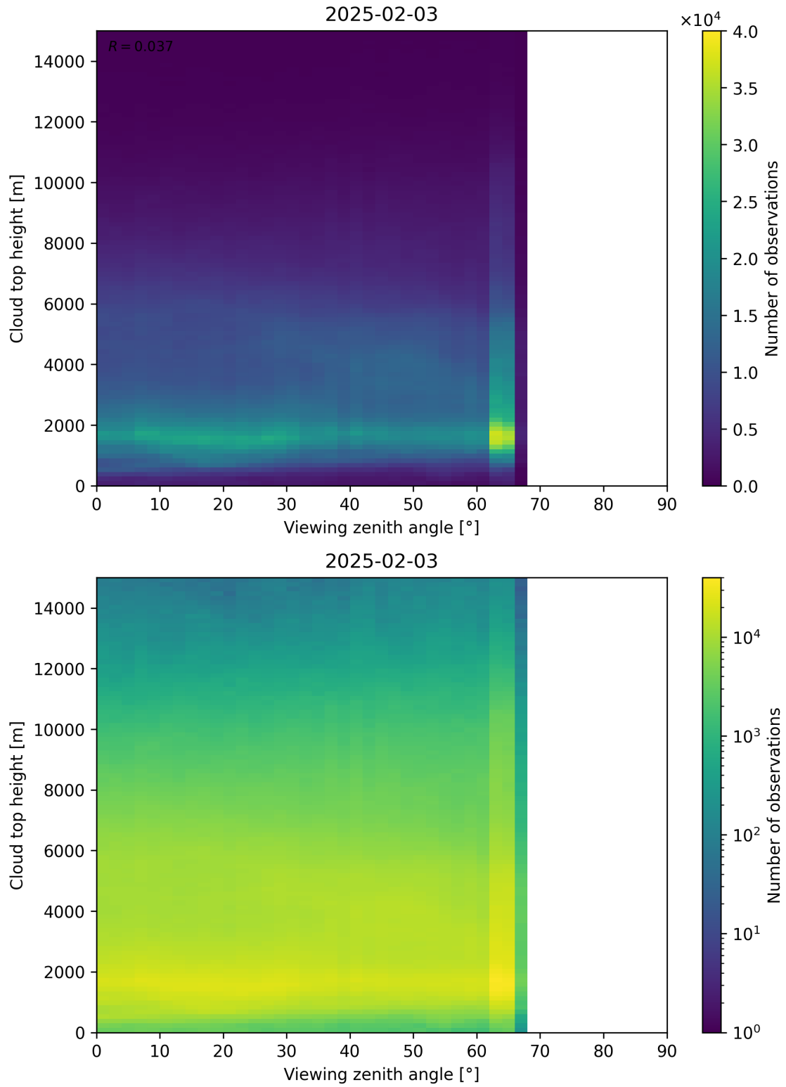
Figure 112: Scatter density plot of “Viewing zenith angle” against “Cloud top height” for 2025-02-03 to 2025-02-04.
