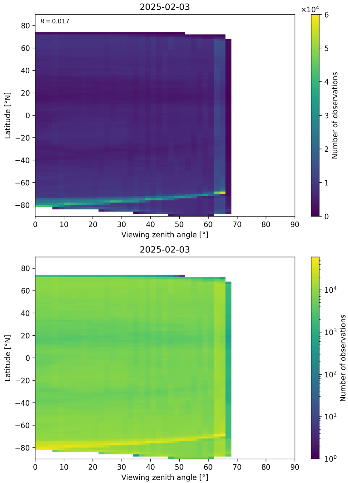
Figure 113: Scatter density plot of “Viewing zenith angle” against “Latitude” for 2025-02-03 to 2025-02-04.
