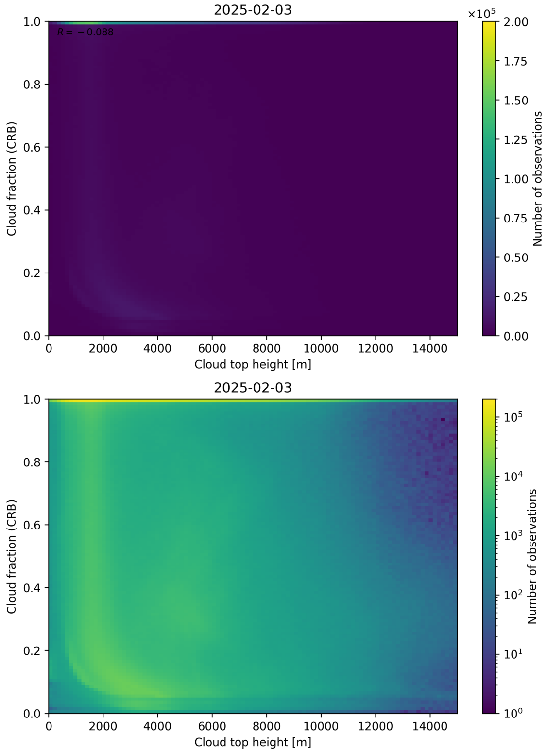
Figure 88: Scatter density plot of “Cloud top height” against “Cloud fraction (CRB)” for 2025-02-03 to 2025-02-04.
