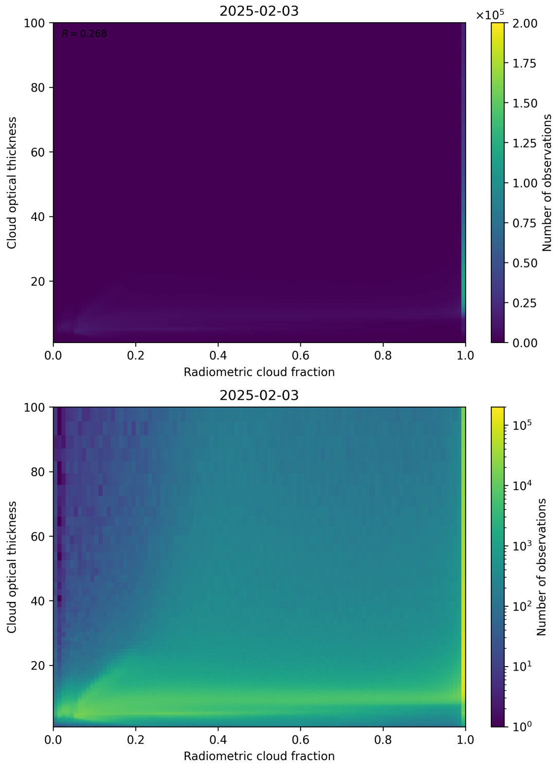
Figure 75: Scatter density plot of “Radiometric cloud fraction” against “Cloud optical thickness” for 2025-02-03 to 2025-02-04.
