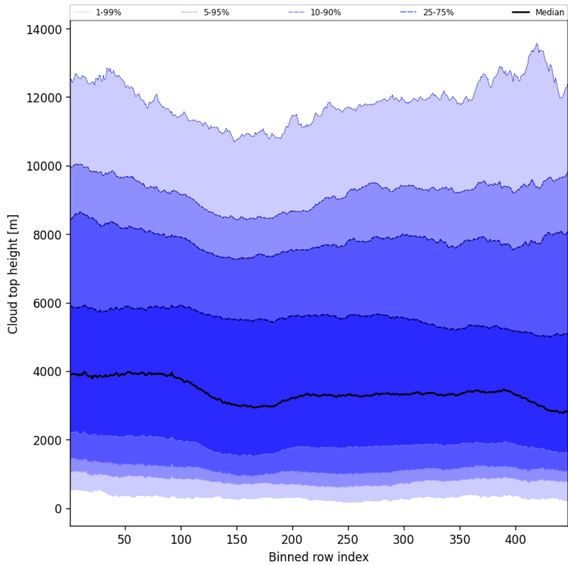
Figure 56: Along track statistics of “Cloud top height” for 2025-02-03 to 2025-02-04
