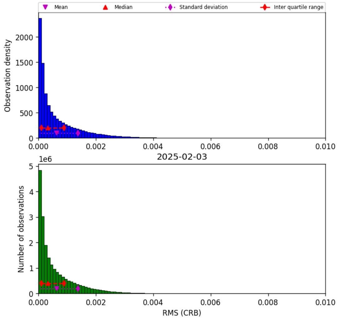
Figure 48: Histogram of “RMS (CRB)” for 2025-02-03 to 2025-02-04
