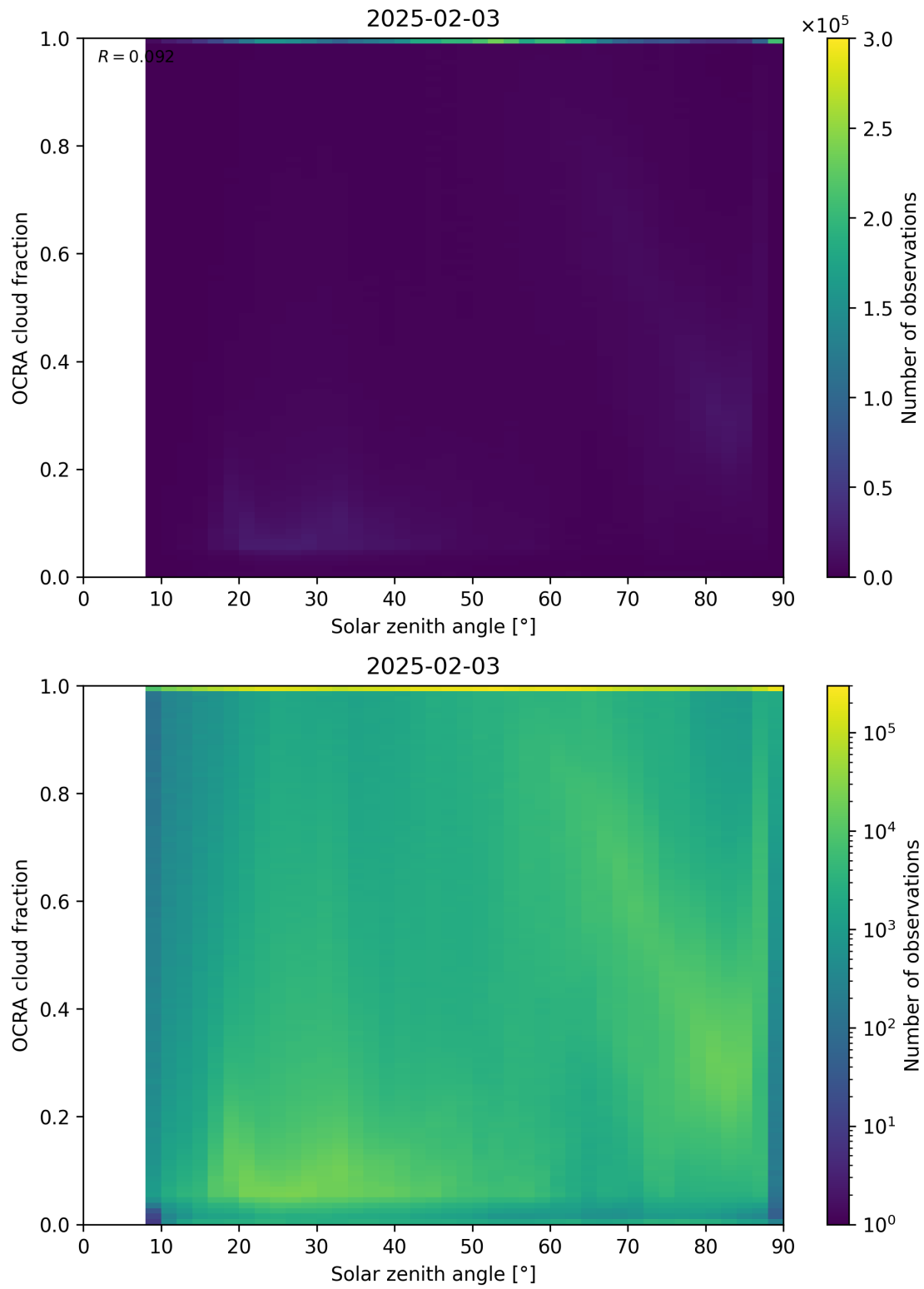
Figure 100: Scatter density plot of “Solar zenith angle” against “OCRA cloud fraction” for 2025-02-03 to 2025-02-04.
