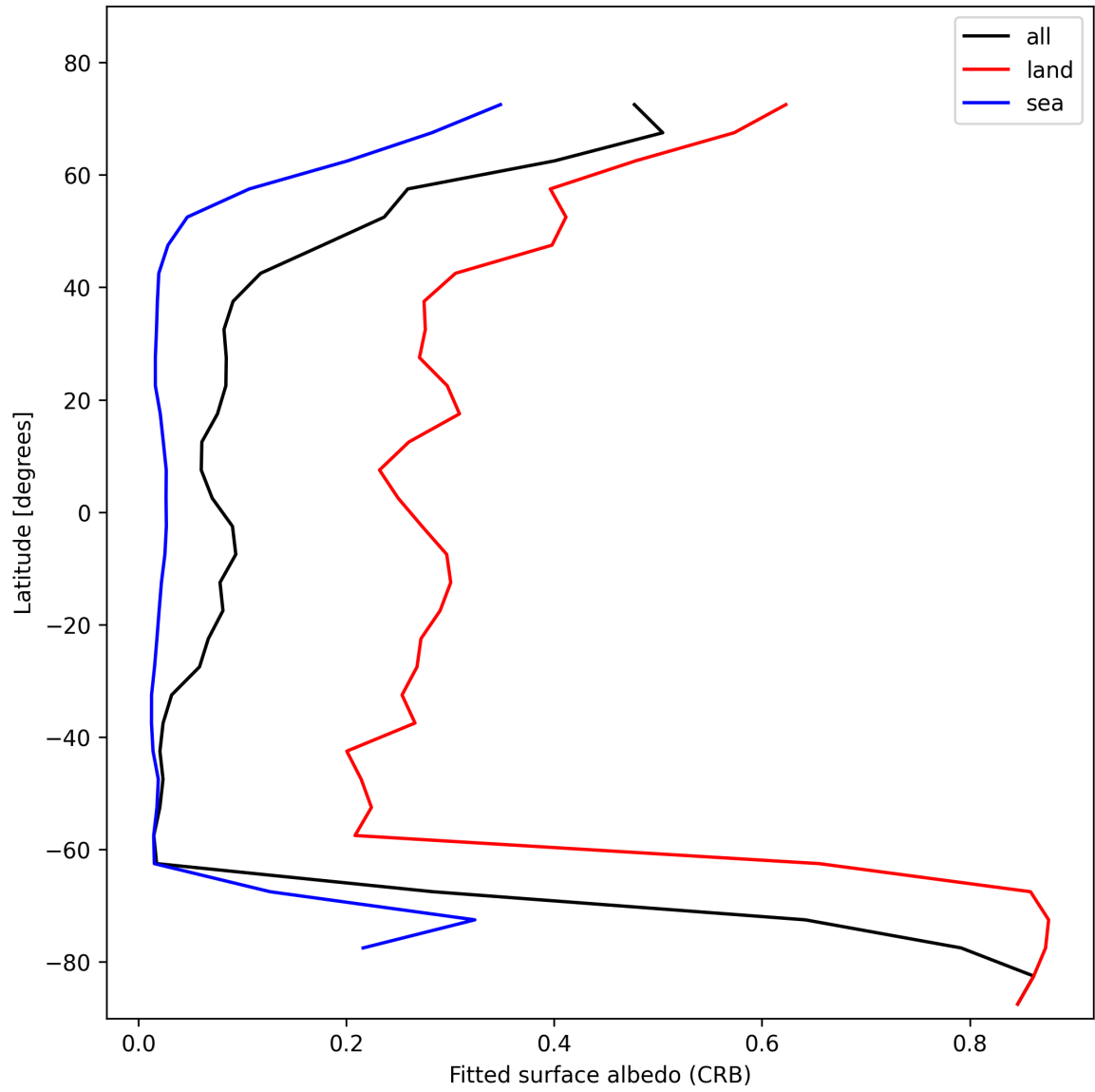
Figure 30: Zonal average of “Fitted surface albedo (CRB)” for 2025-02-03 to 2025-02-04.
