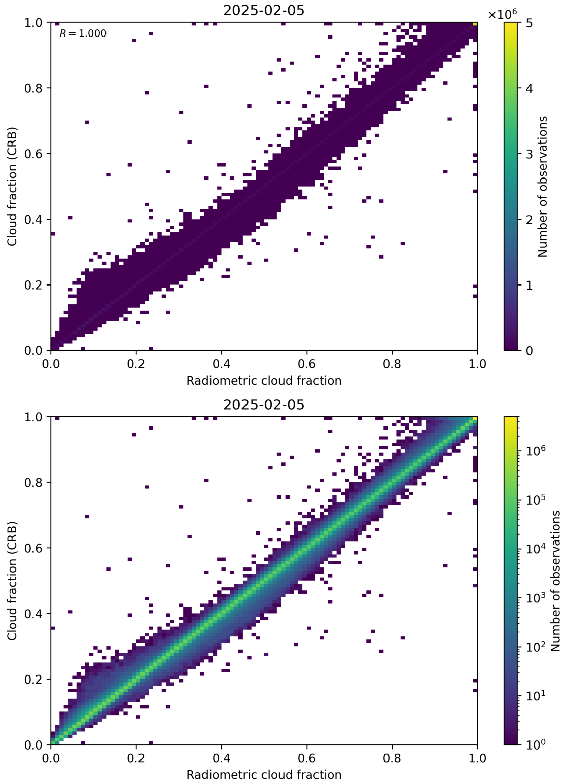
Figure 73: Scatter density plot of “Radiometric cloud fraction” against “Cloud fraction (CRB)” for 2025-02-04 to 2025-02-06.
