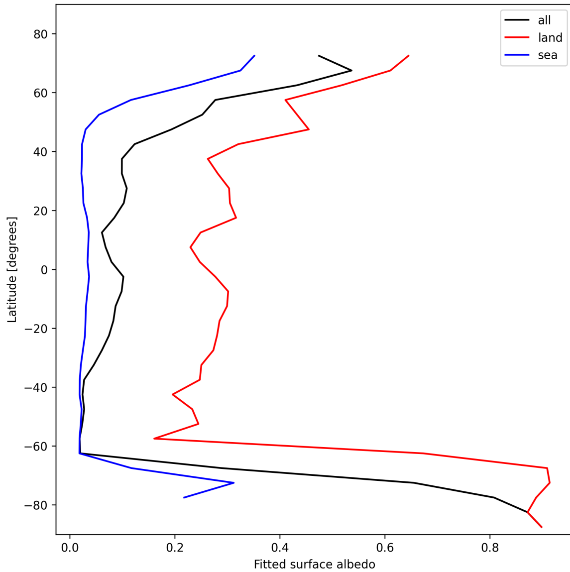
Figure 29: Zonal average of “Fitted surface albedo” for 2025-02-04 to 2025-02-06.
