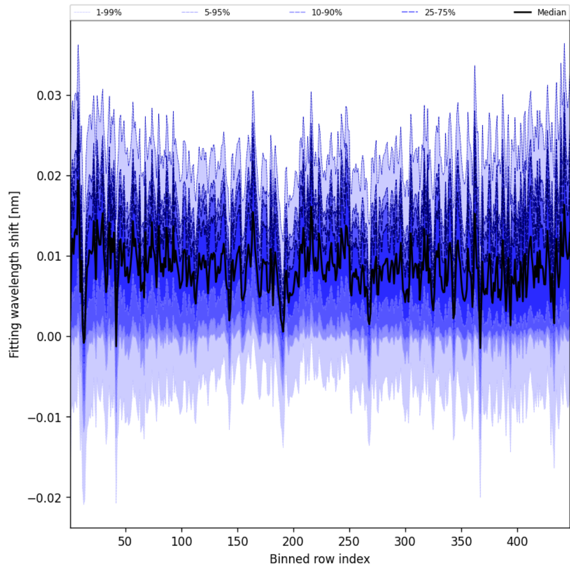
Figure 65: Along track statistics of “Fitting wavelength shift” for 2025-02-04 to 2025-02-06
