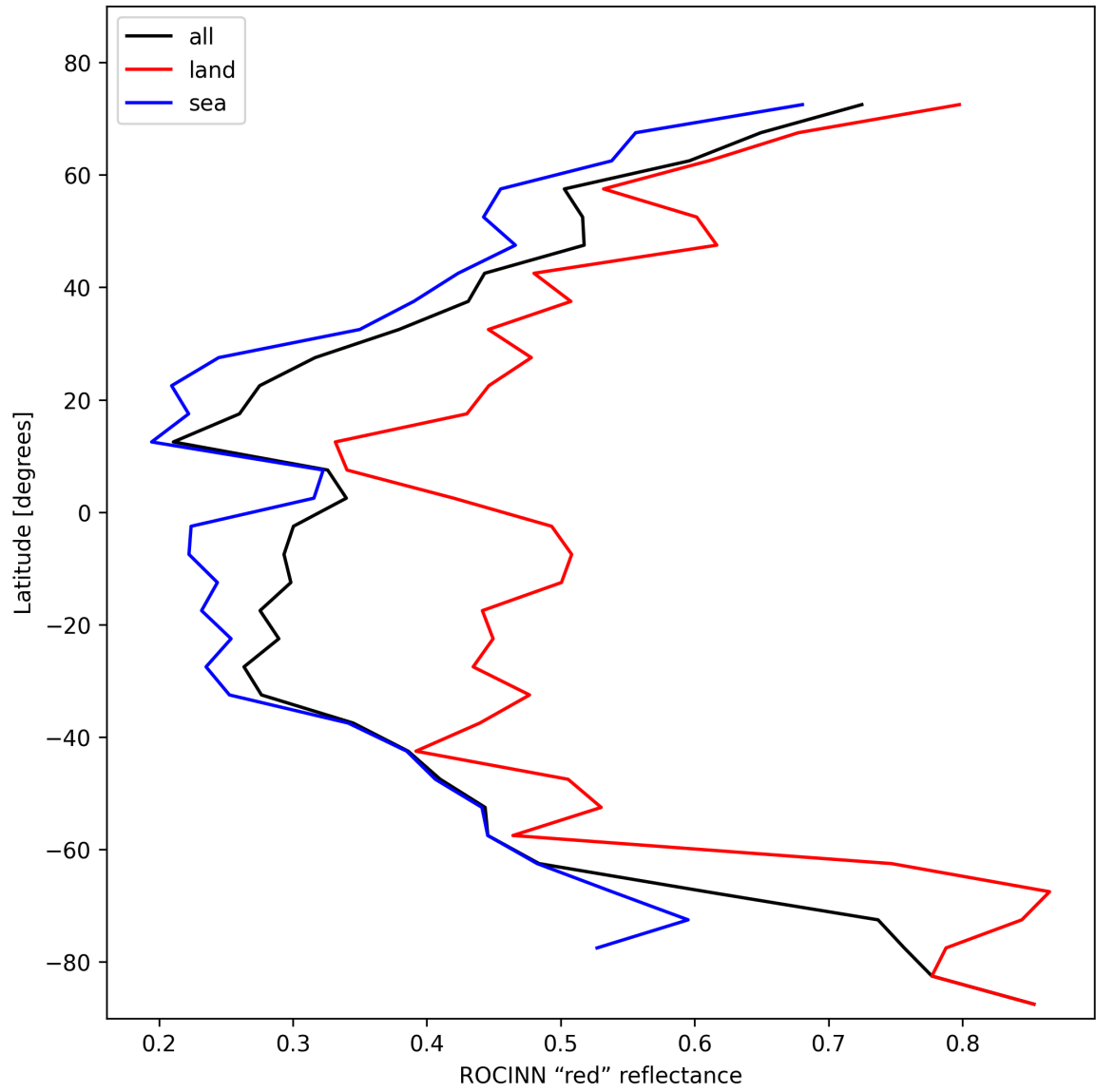
Figure 37: Zonal average of “ROCINN “red” reflectance” for 2025-02-04 to 2025-02-06.
