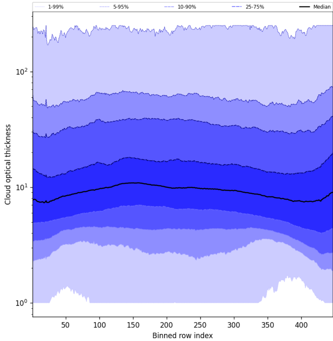
Figure 57: Along track statistics of “Cloud optical thickness” for 2025-02-04 to 2025-02-06
