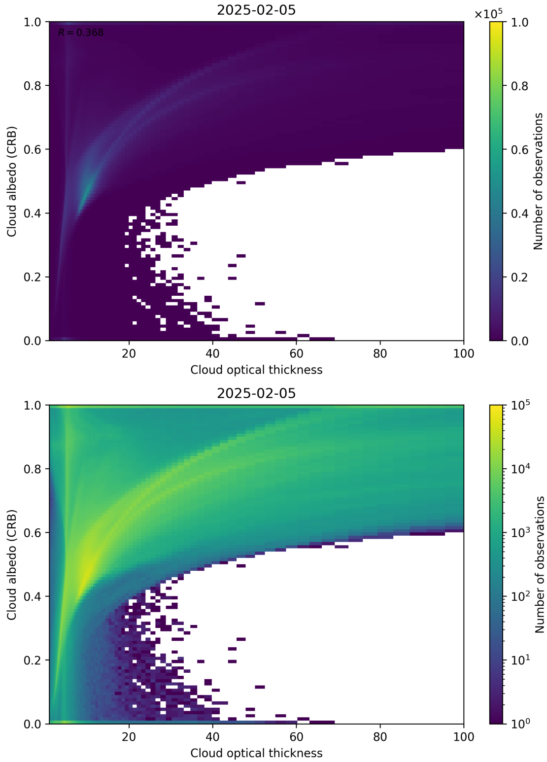
Figure 82: Scatter density plot of “Cloud optical thickness” against “Cloud albedo (CRB)” for 2025-02-04 to 2025-02-06.
