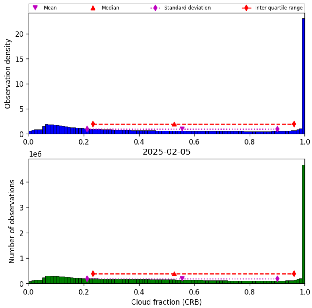
Figure 42: Histogram of “Cloud fraction (CRB)” for 2025-02-04 to 2025-02-06
