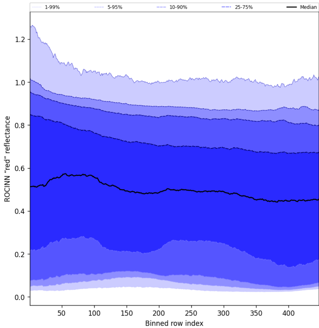
Figure 69: Along track statistics of "ROCINN "red" reflectance" for 2025-02-04 to 2025-02-06
