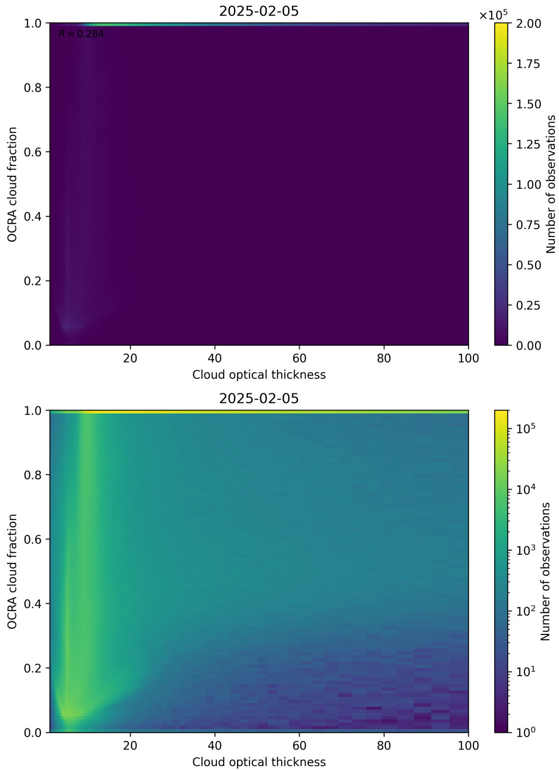
Figure 83: Scatter density plot of “Cloud optical thickness” against “OCRA cloud fraction” for 2025-02-04 to 2025-02-06.
