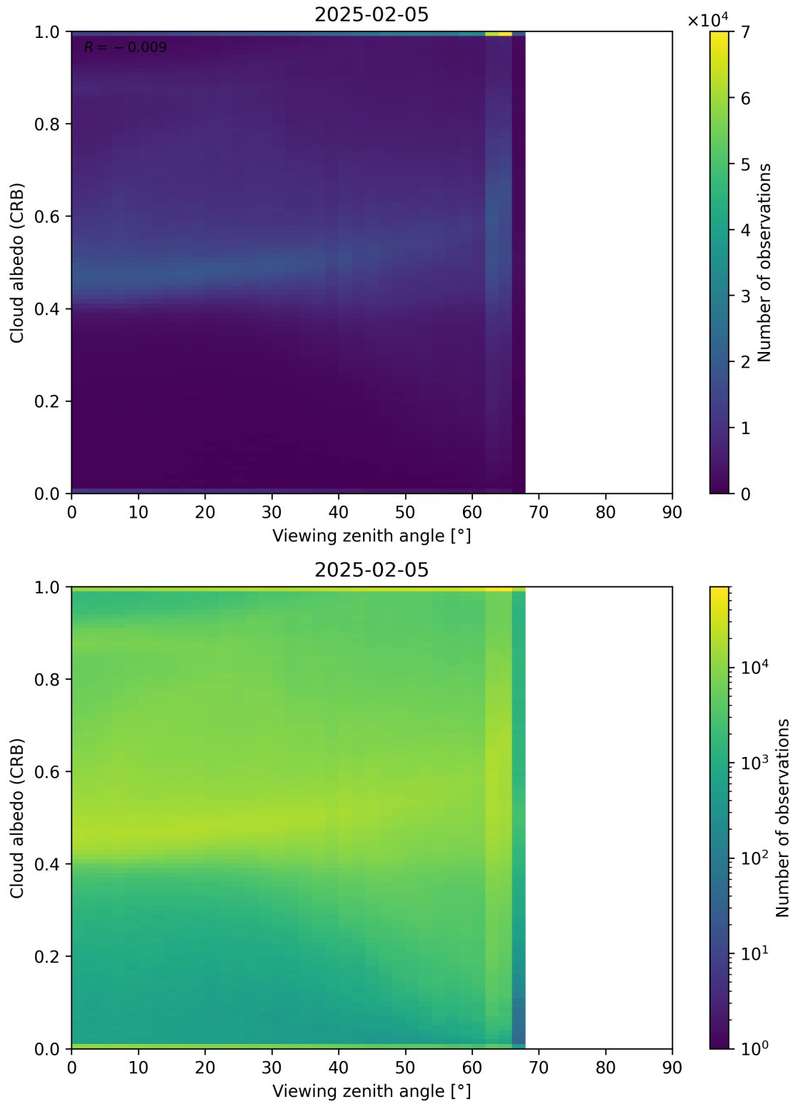
Figure 106: Scatter density plot of “Viewing zenith angle” against “Cloud albedo (CRB)” for 2025-02-04 to 2025-02-06.
