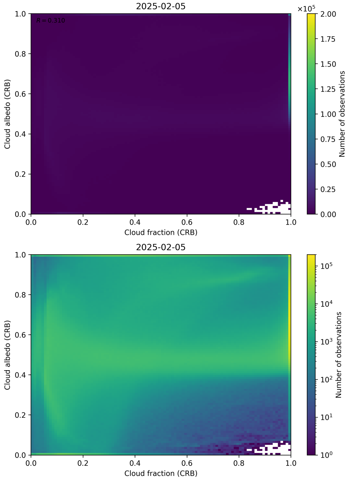
Figure 77: Scatter density plot of “Cloud fraction (CRB)” against “Cloud albedo (CRB)” for 2025-02-04 to 2025-02-06.
