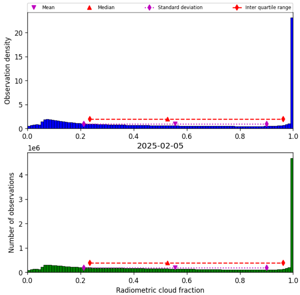
Figure 39: Histogram of “Radiometric cloud fraction” for 2025-02-04 to 2025-02-06
