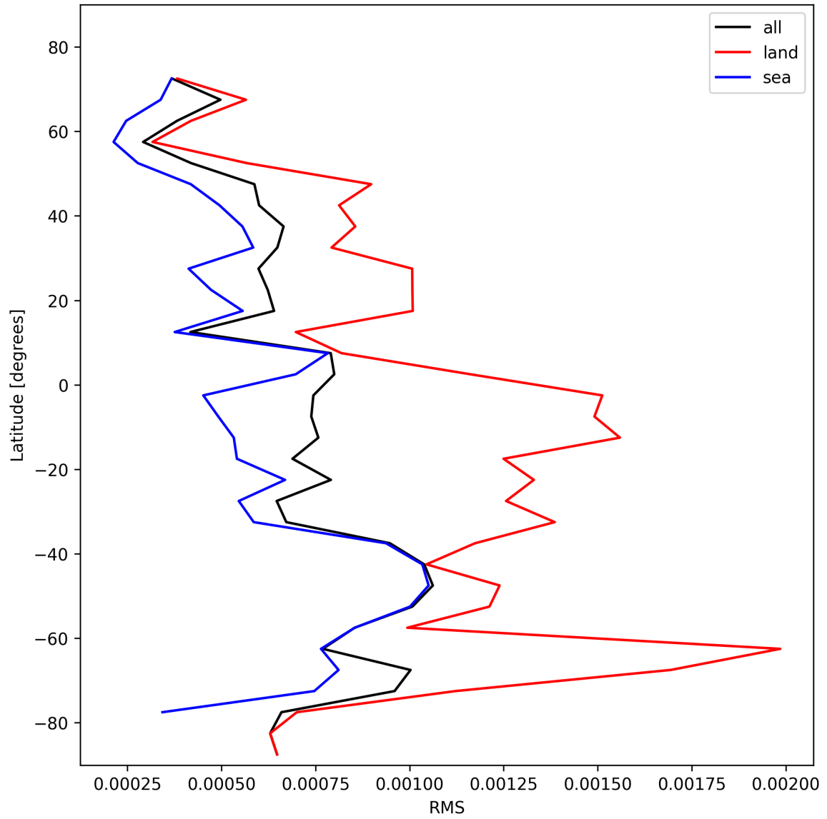
Figure 31: Zonal average of “RMS” for 2025-02-04 to 2025-02-06.
