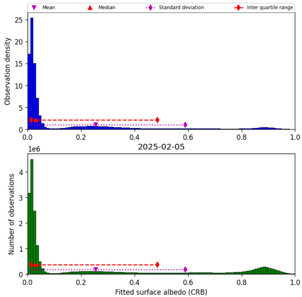
Figure 46: Histogram of “Fitted surface albedo (CRB)” for 2025-02-04 to 2025-02-06
