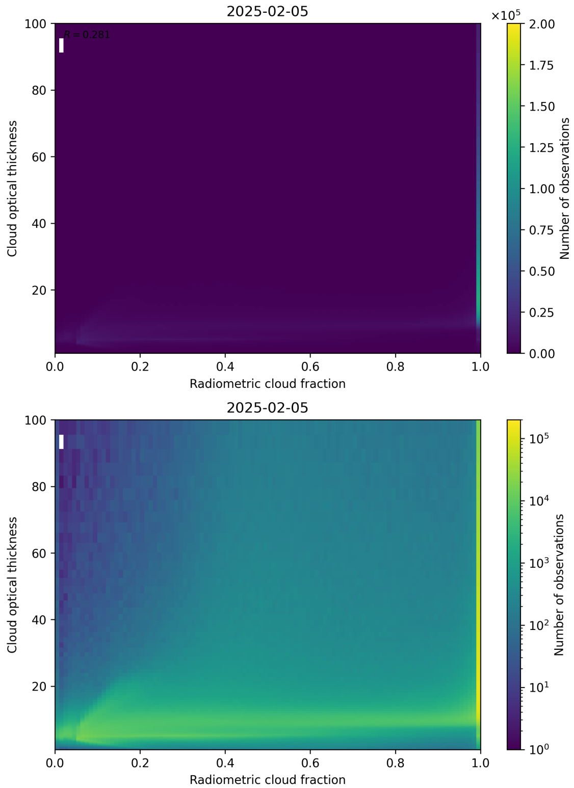
Figure 75: Scatter density plot of “Radiometric cloud fraction” against “Cloud optical thickness” for 2025-02-04 to 2025-02-06.
