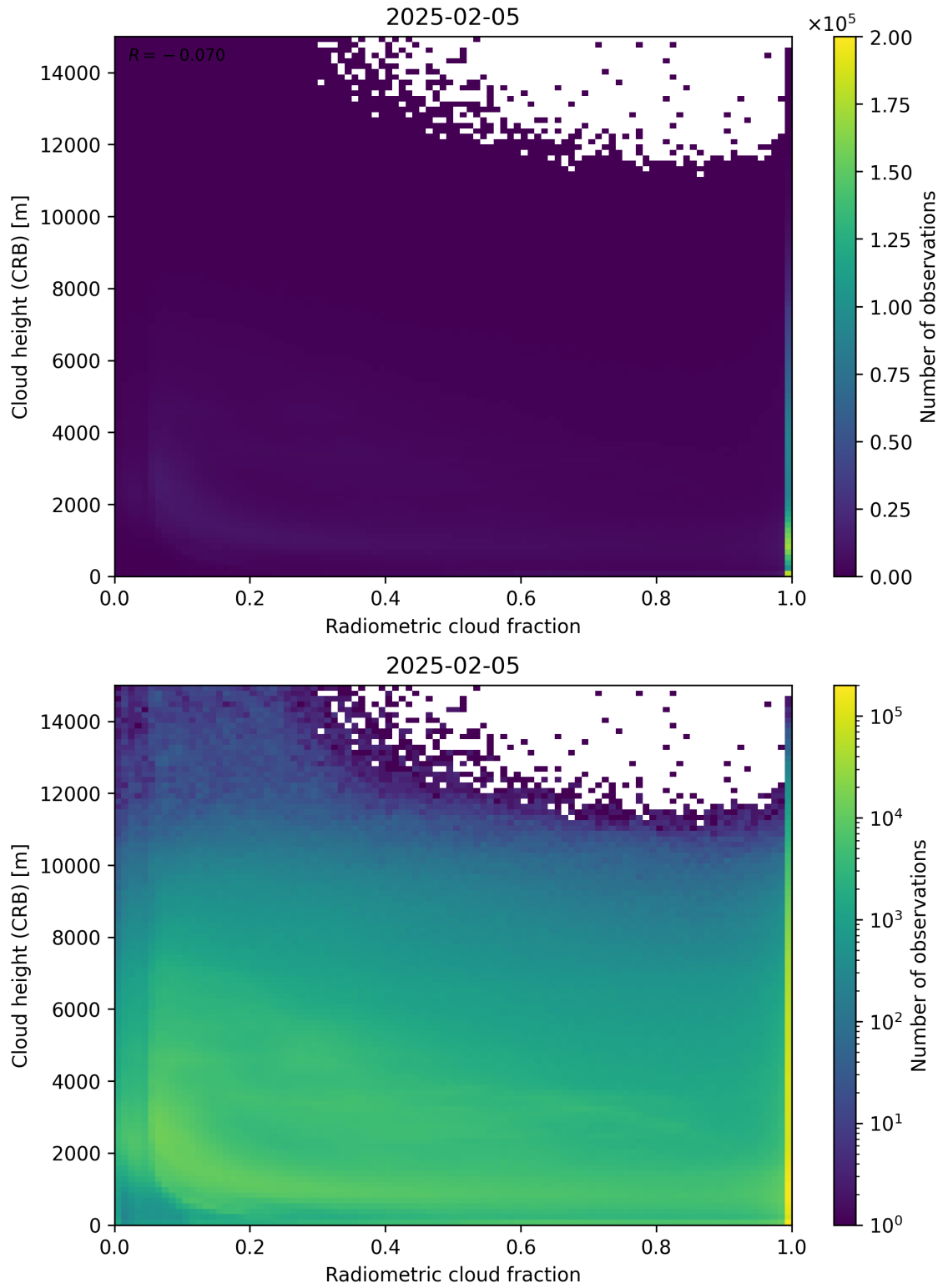
Figure 74: Scatter density plot of “Radiometric cloud fraction” against “Cloud height (CRB)” for 2025-02-04 to 2025-02-06.
