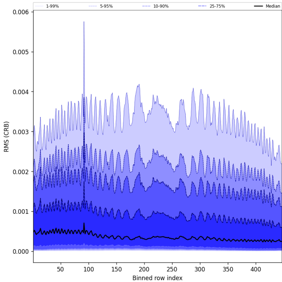
Figure 64: Along track statistics of “RMS (CRB)” for 2025-02-04 to 2025-02-06
