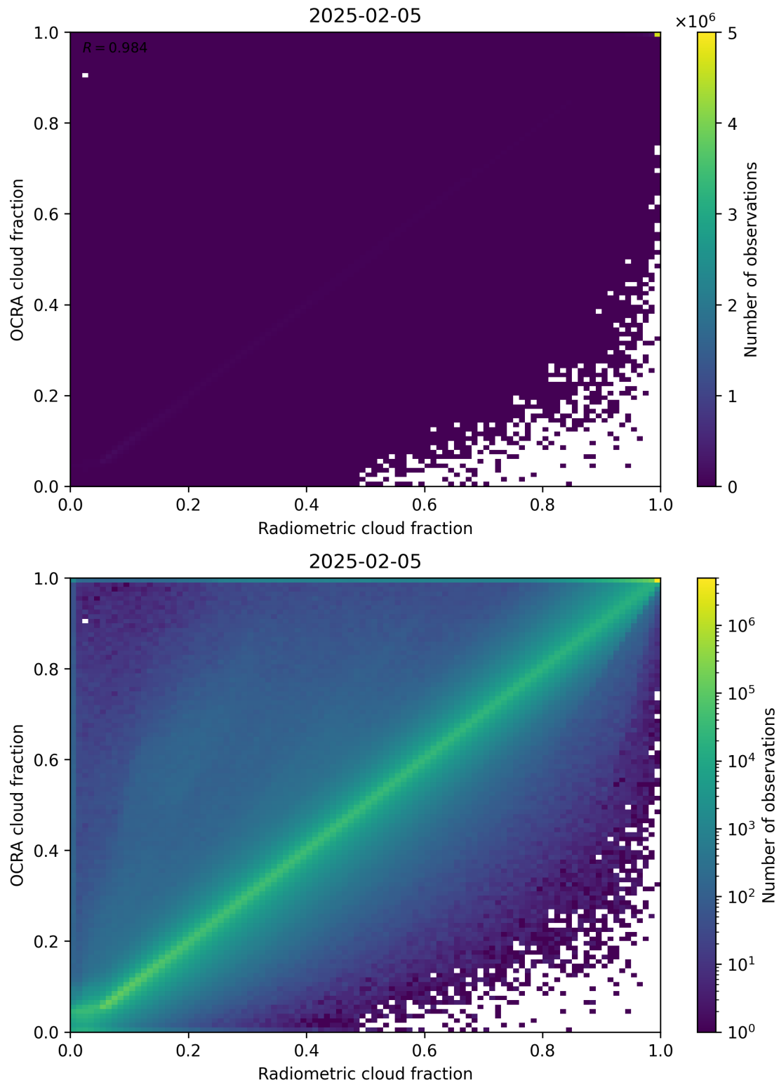
Figure 72: Scatter density plot of “Radiometric cloud fraction” against “OCRA cloud fraction” for 2025-02-04 to 2025-02-06.
