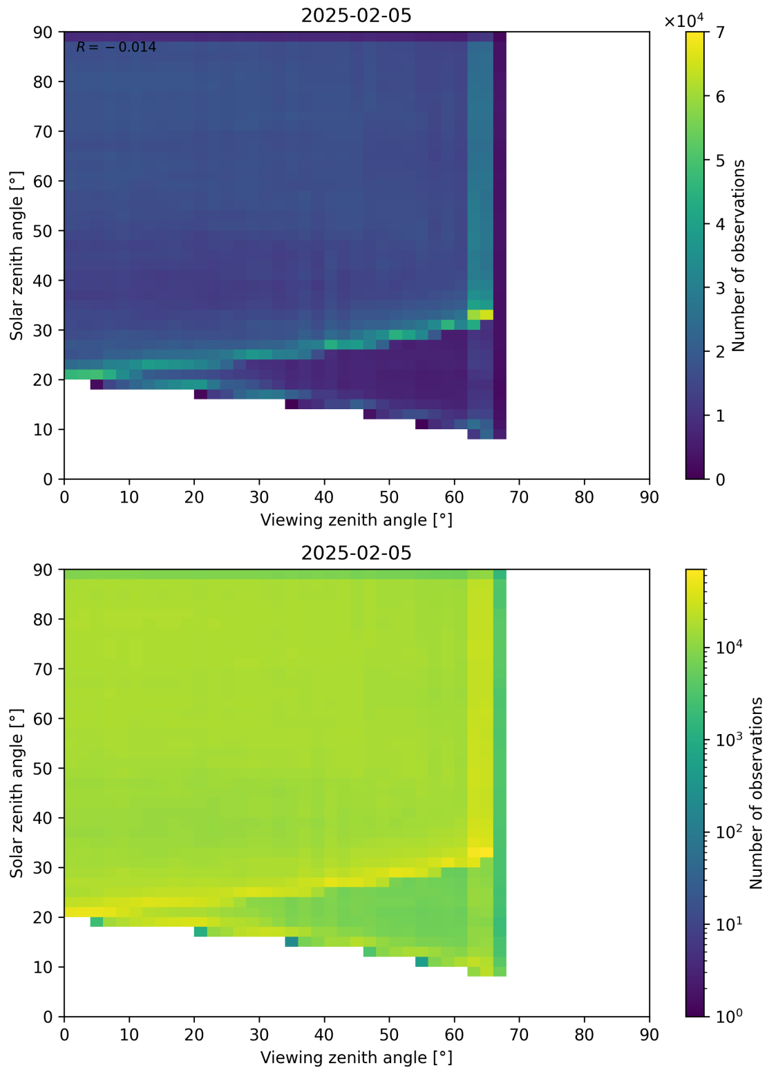
Figure 114: Scatter density plot of “Viewing zenith angle” against “Solar zenith angle” for 2025-02-04 to 2025-02-06.
