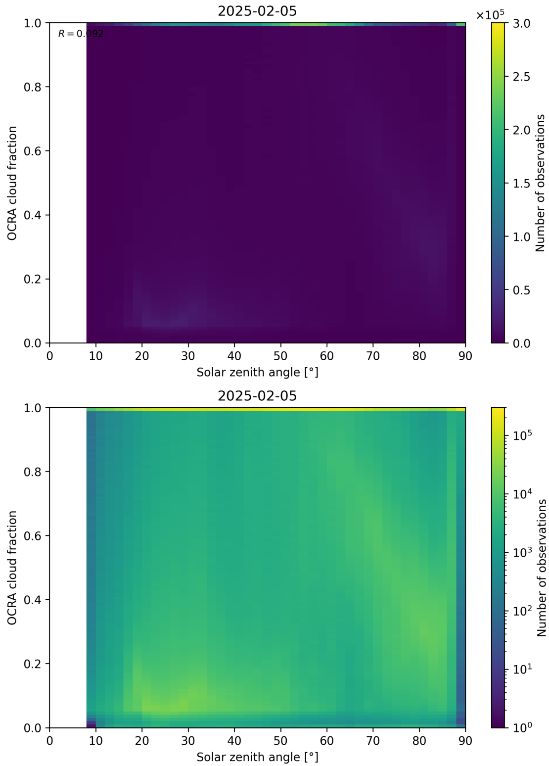
Figure 100: Scatter density plot of “Solar zenith angle” against “OCRA cloud fraction” for 2025-02-04 to 2025-02-06.
