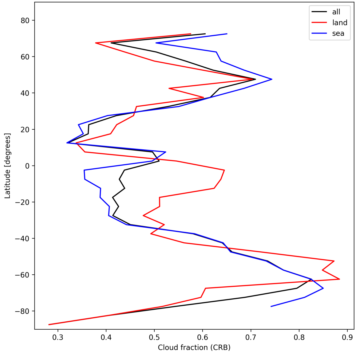
Figure 26: Zonal average of “Cloud fraction (CRB)” for 2025-02-04 to 2025-02-06.
