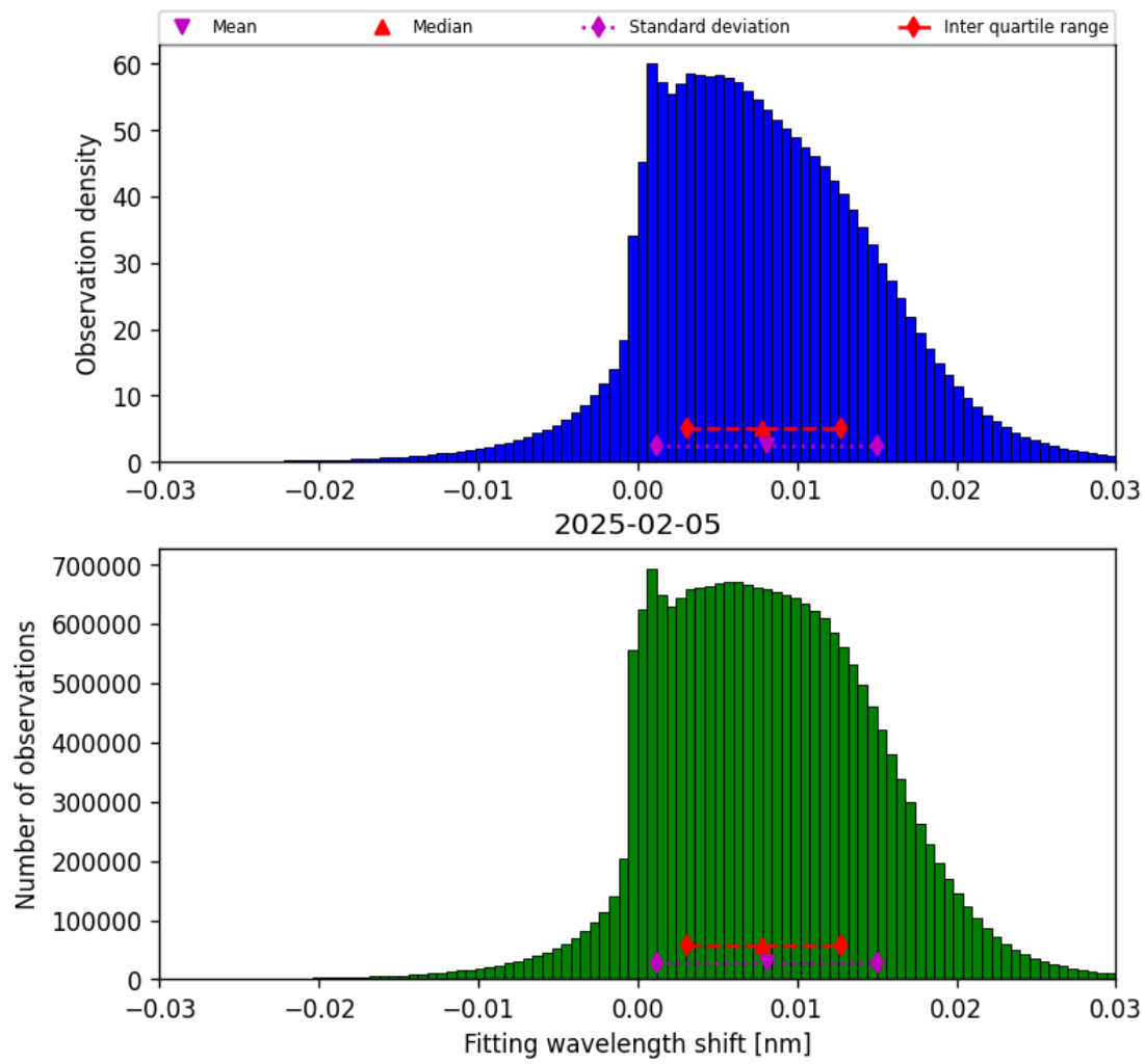
Figure 49: Histogram of “Fitting wavelength shift” for 2025-02-04 to 2025-02-06
