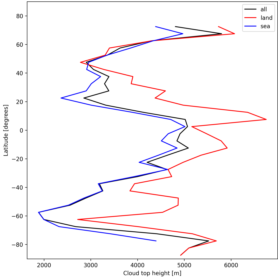
Figure 24: Zonal average of “Cloud top height” for 2025-02-04 to 2025-02-06.
