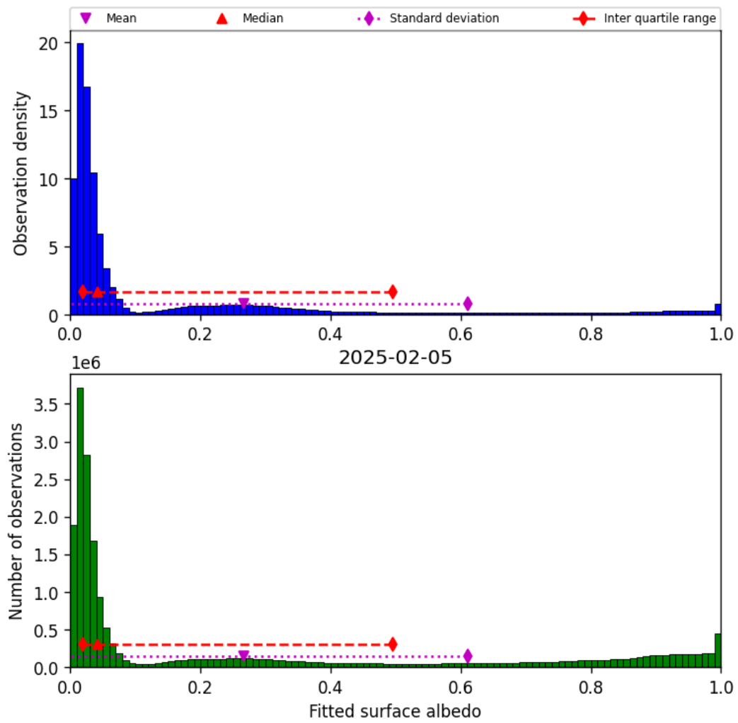
Figure 45: Histogram of “Fitted surface albedo” for 2025-02-04 to 2025-02-06
