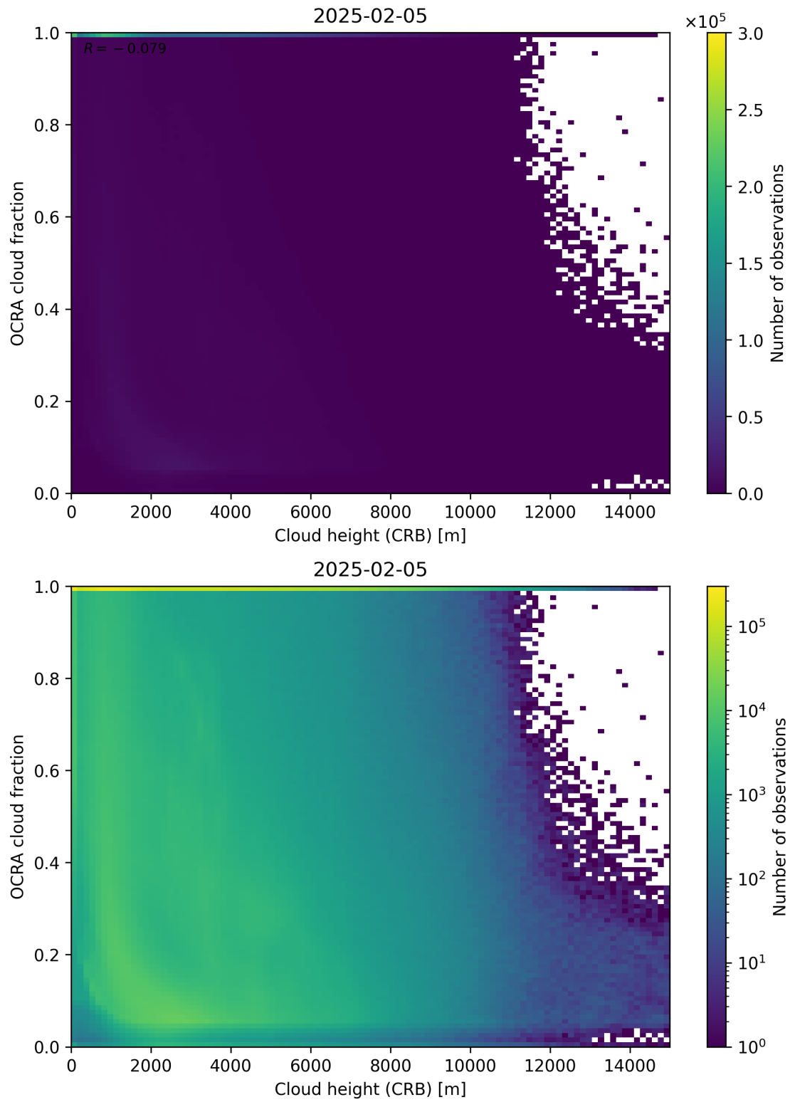
Figure 81: Scatter density plot of “Cloud height (CRB)” against “OCRA cloud fraction” for 2025-02-04 to 2025-02-06.
