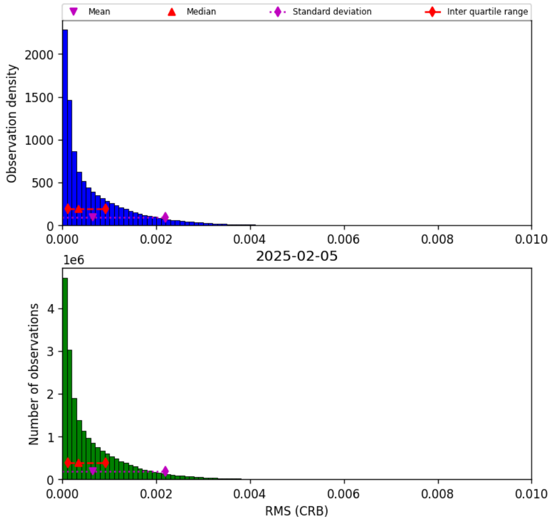
Figure 48: Histogram of “RMS (CRB)” for 2025-02-04 to 2025-02-06
