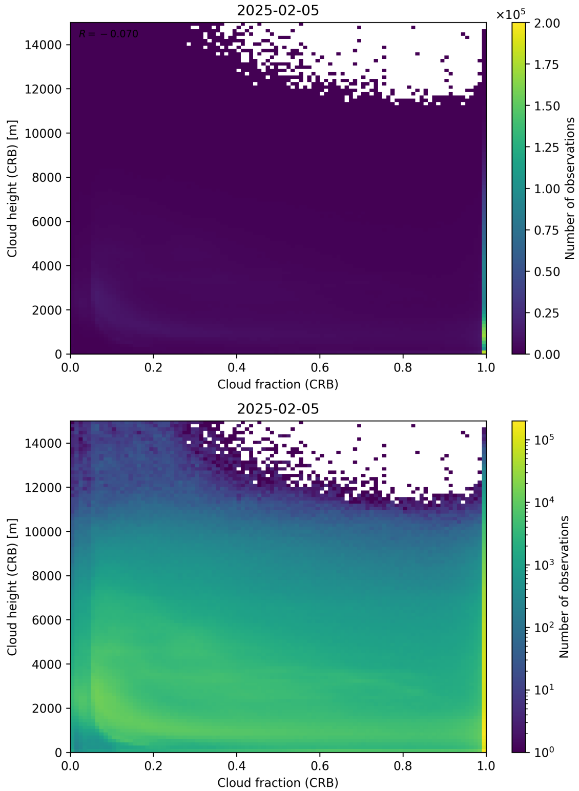
Figure 79: Scatter density plot of “Cloud fraction (CRB)” against “Cloud height (CRB)” for 2025-02-04 to 2025-02-06.
