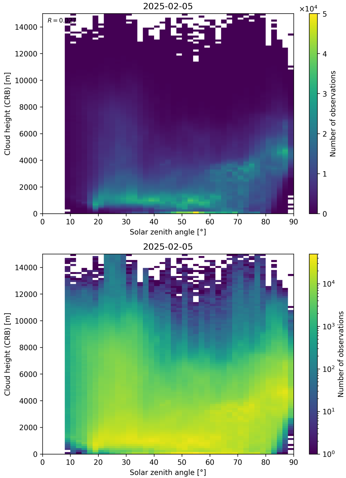
Figure 102: Scatter density plot of “Solar zenith angle” against “Cloud height (CRB)” for 2025-02-04 to 2025-02-06.
