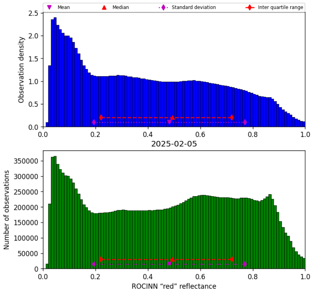
Figure 53: Histogram of “ROCINN “red” reflectance” for 2025-02-04 to 2025-02-06
