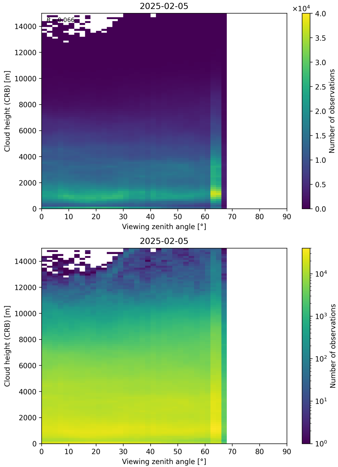
Figure 110: Scatter density plot of “Viewing zenith angle” against “Cloud height (CRB)” for 2025-02-04 to 2025-02-06.
