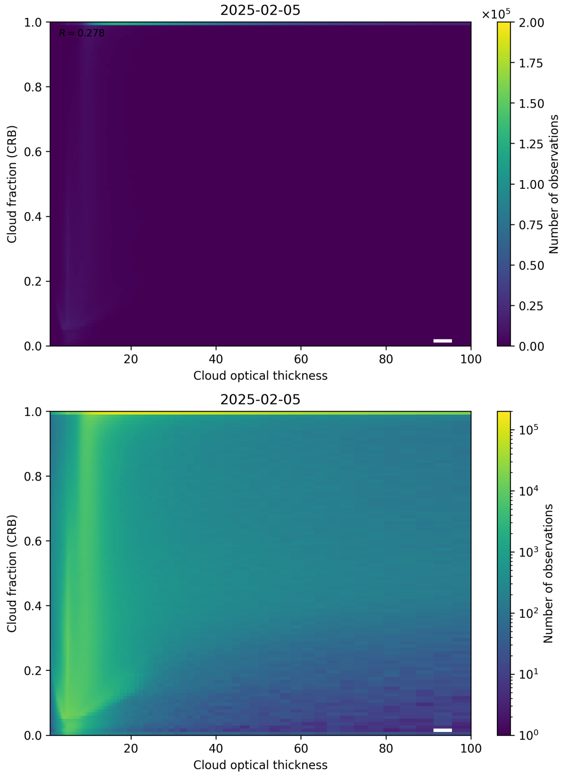
Figure 84: Scatter density plot of “Cloud optical thickness” against “Cloud fraction (CRB)” for 2025-02-04 to 2025-02-06.
