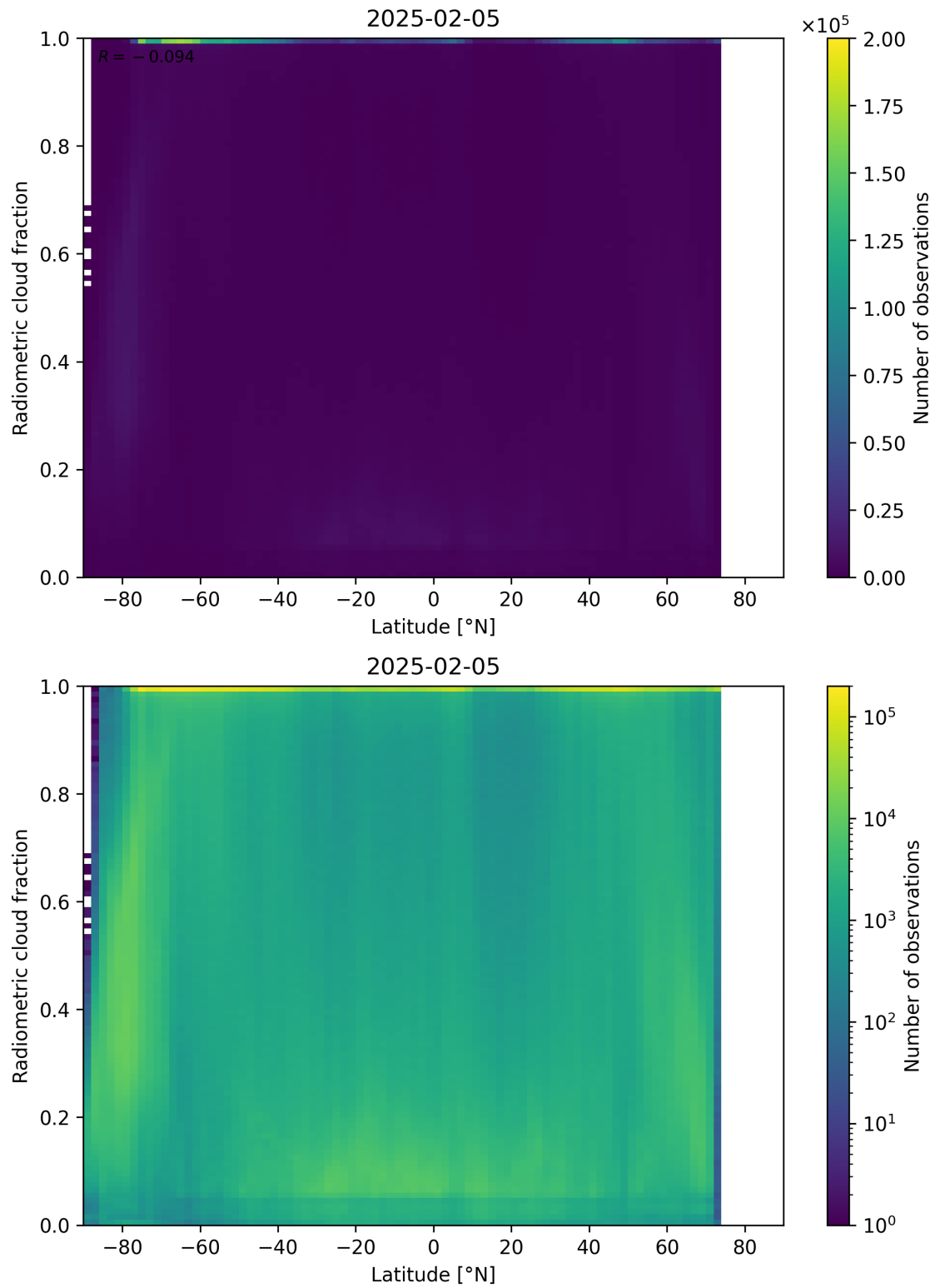
Figure 92: Scatter density plot of “Latitude” against “Radiometric cloud fraction” for 2025-02-04 to 2025-02-06.
