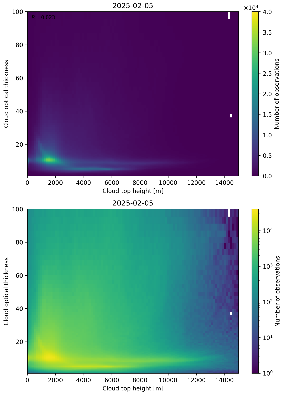
Figure 90: Scatter density plot of “Cloud top height” against “Cloud optical thickness” for 2025-02-04 to 2025-02-06.
