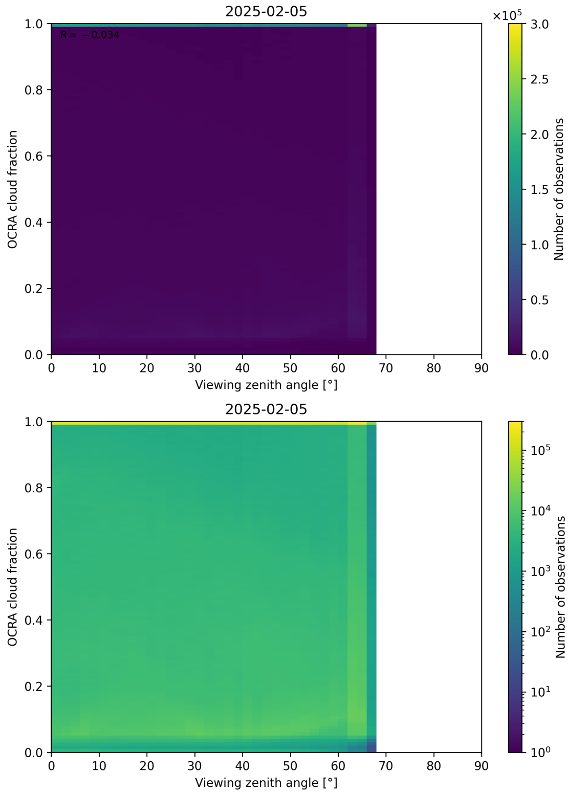
Figure 108: Scatter density plot of “Viewing zenith angle” against “OCRA cloud fraction” for 2025-02-04 to 2025-02-06.
