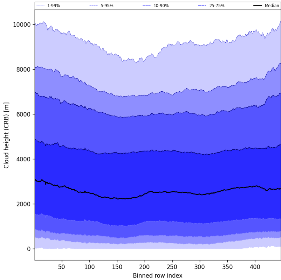
Figure 59: Along track statistics of “Cloud height (CRB)” for 2025-02-04 to 2025-02-06
