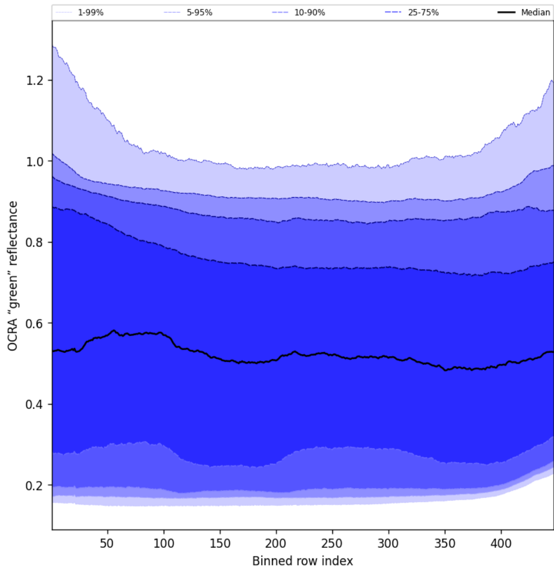
Figure 68: Along track statistics of “OCRA “green” reflectance” for 2025-02-04 to 2025-02-06
