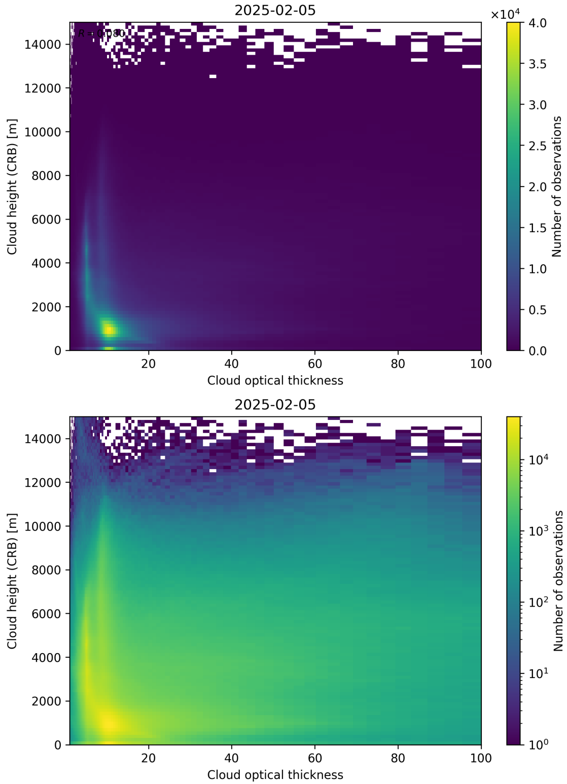
Figure 85: Scatter density plot of “Cloud optical thickness” against “Cloud height (CRB)” for 2025-02-04 to 2025-02-06.
