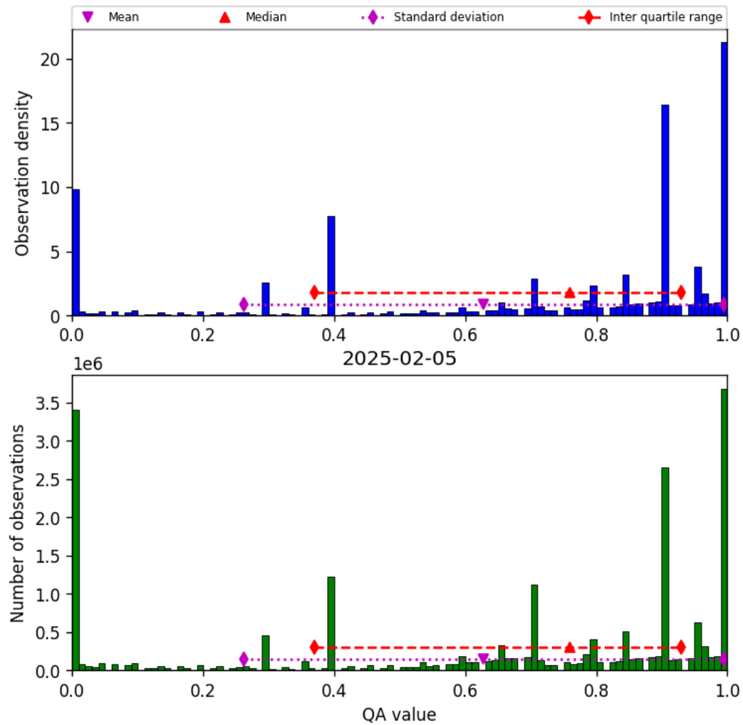
Figure 38: Histogram of “QA value” for 2025-02-04 to 2025-02-06
