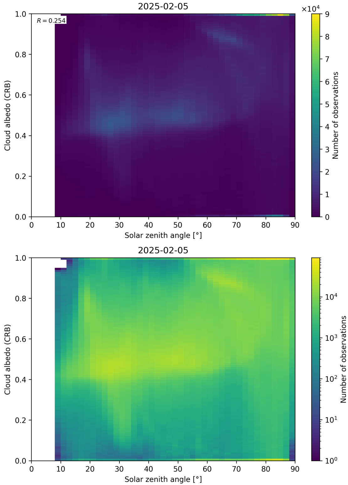
Figure 98: Scatter density plot of “Solar zenith angle” against “Cloud albedo (CRB)” for 2025-02-04 to 2025-02-06.
