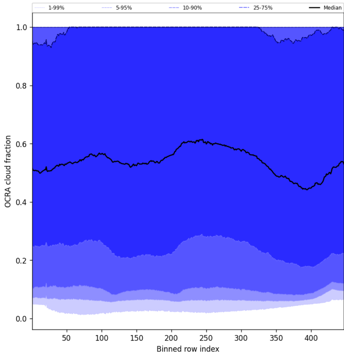
Figure 66: Along track statistics of “OCRA cloud fraction” for 2025-02-04 to 2025-02-06
