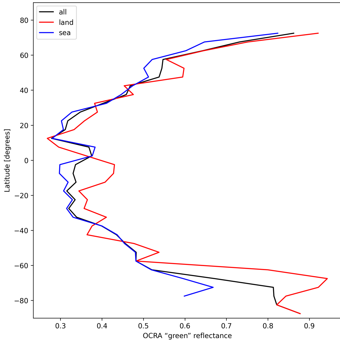
Figure 36: Zonal average of “OCRA “green” reflectance” for 2025-02-04 to 2025-02-06.
