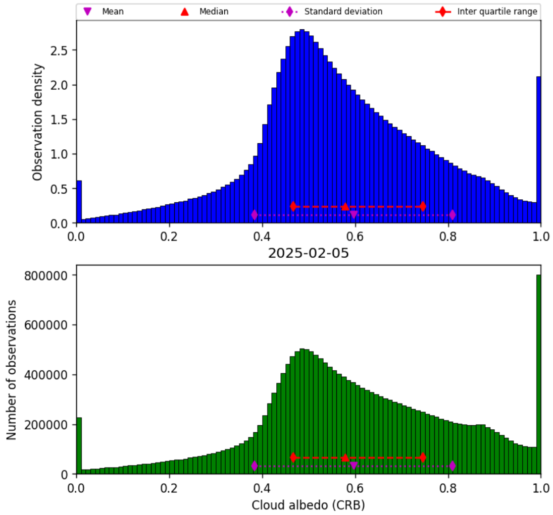
Figure 44: Histogram of “Cloud albedo (CRB)” for 2025-02-04 to 2025-02-06
