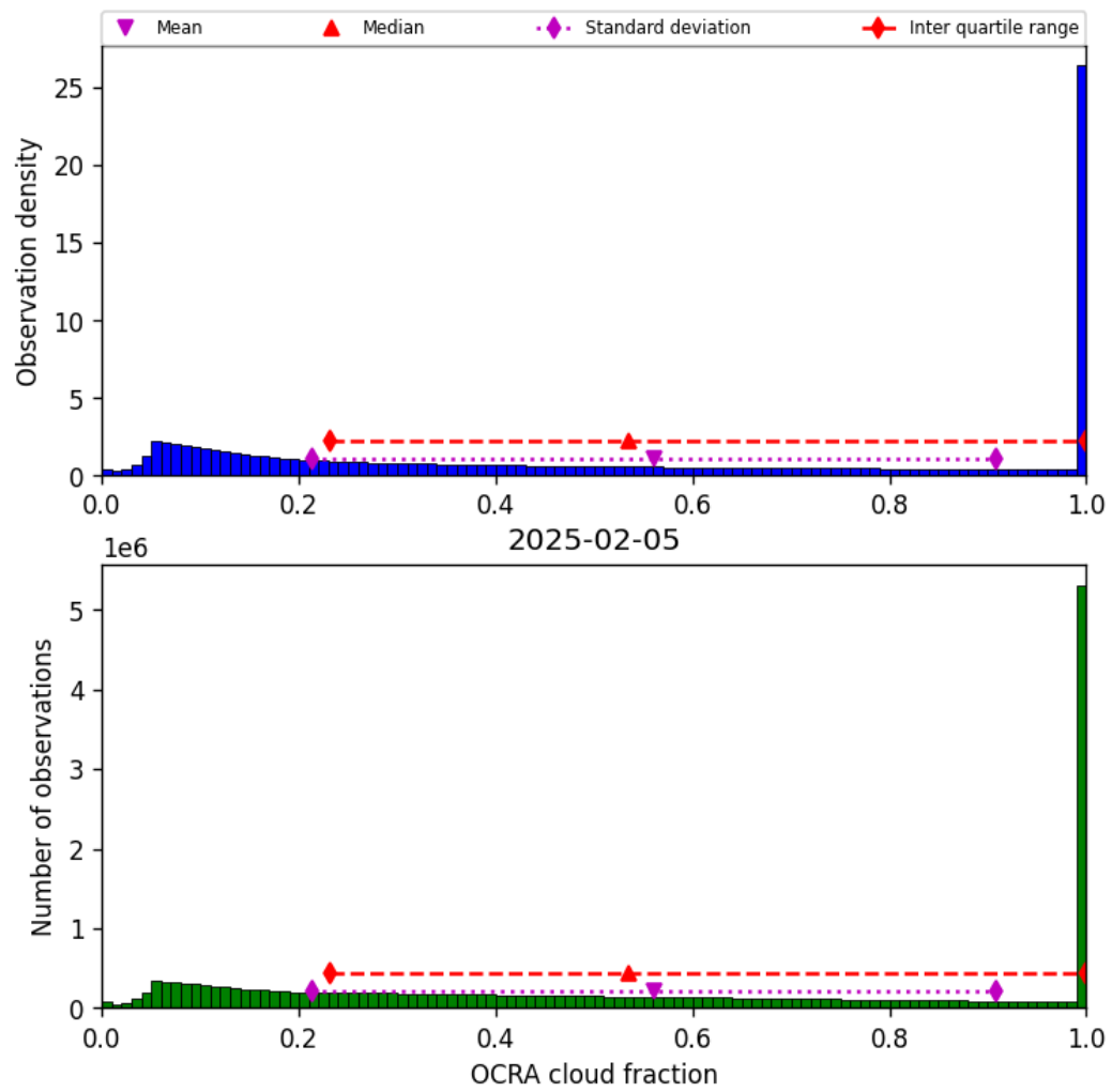
Figure 50: Histogram of “OCRA cloud fraction” for 2025-02-04 to 2025-02-06
