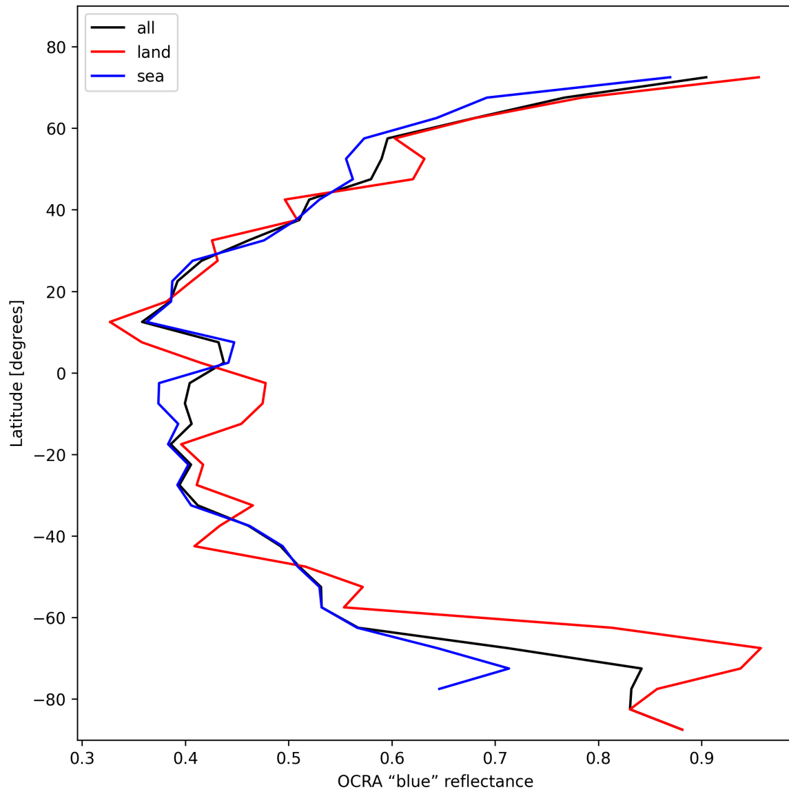
Figure 35: Zonal average of “OCRA “blue” reflectance” for 2025-02-04 to 2025-02-06.
