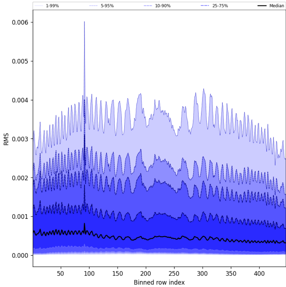
Figure 63: Along track statistics of “RMS” for 2025-02-04 to 2025-02-06
