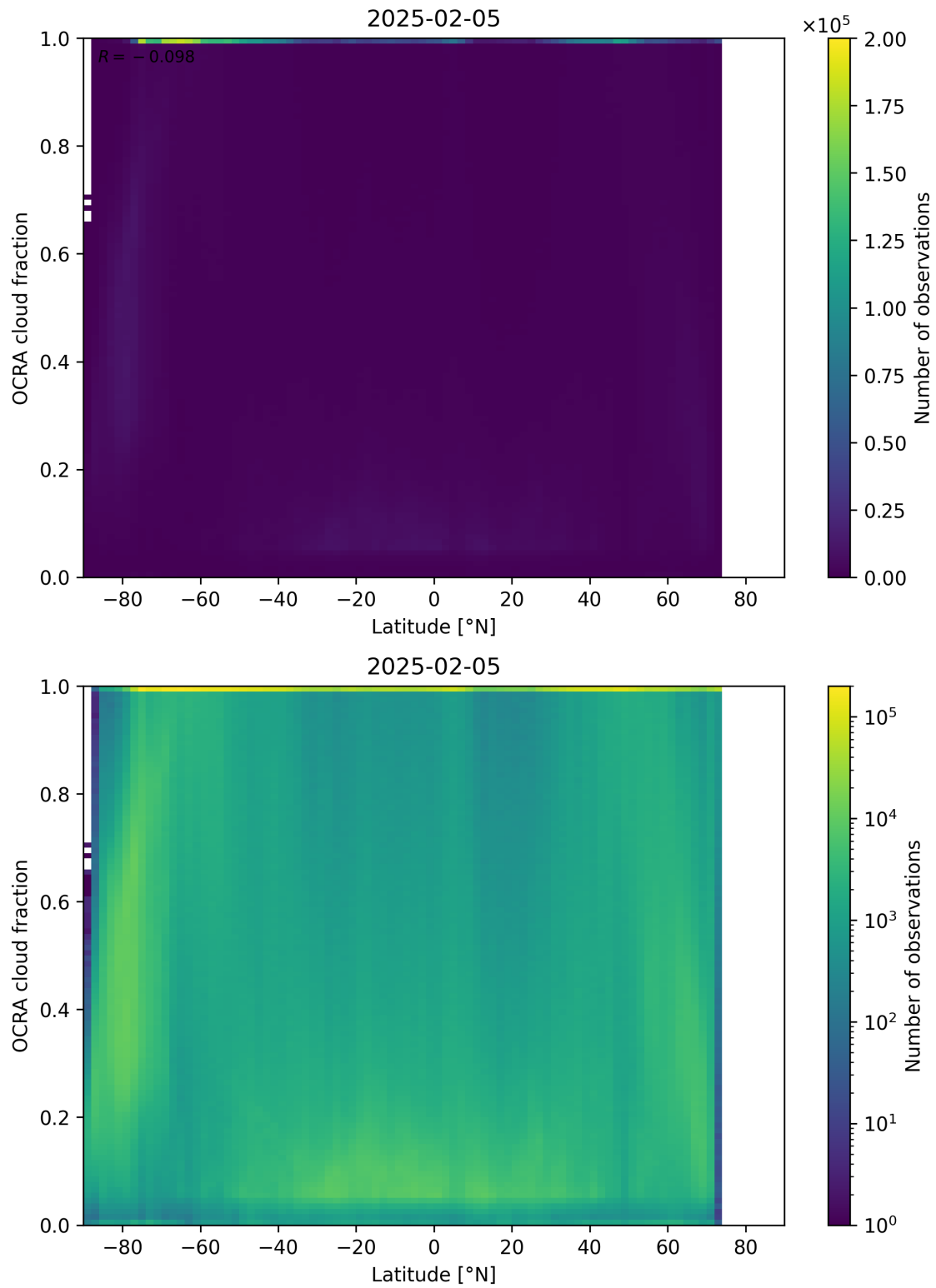
Figure 93: Scatter density plot of “Latitude” against “OCRA cloud fraction” for 2025-02-04 to 2025-02-06.
