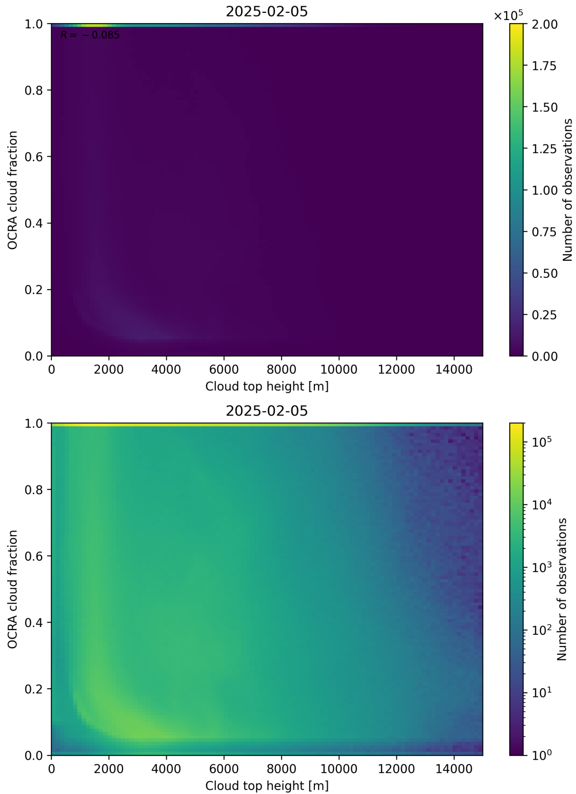
Figure 87: Scatter density plot of “Cloud top height” against “OCRA cloud fraction” for 2025-02-04 to 2025-02-06.
