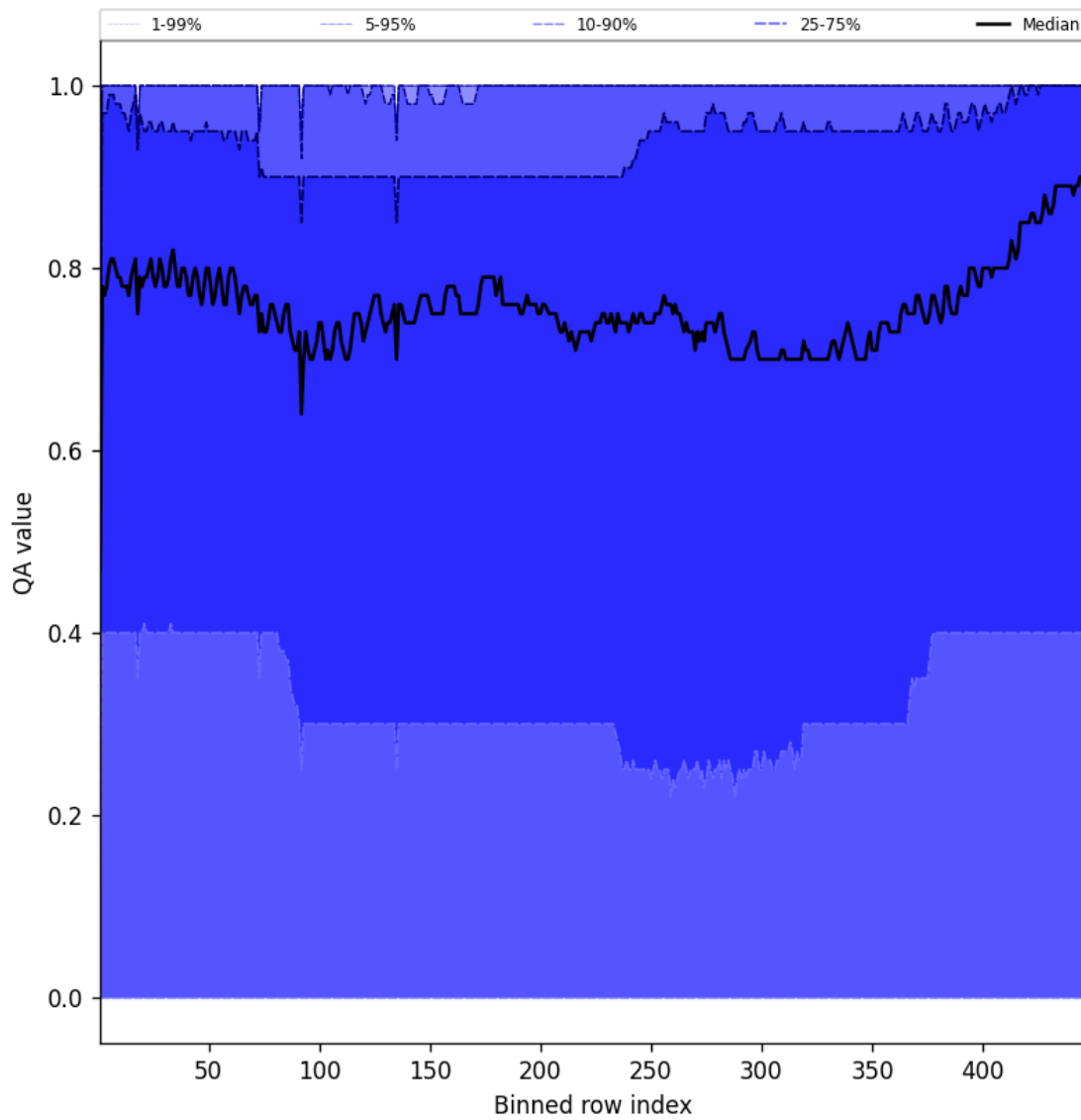
Figure 54: Along track statistics of “QA value” for 2025-02-04 to 2025-02-06
