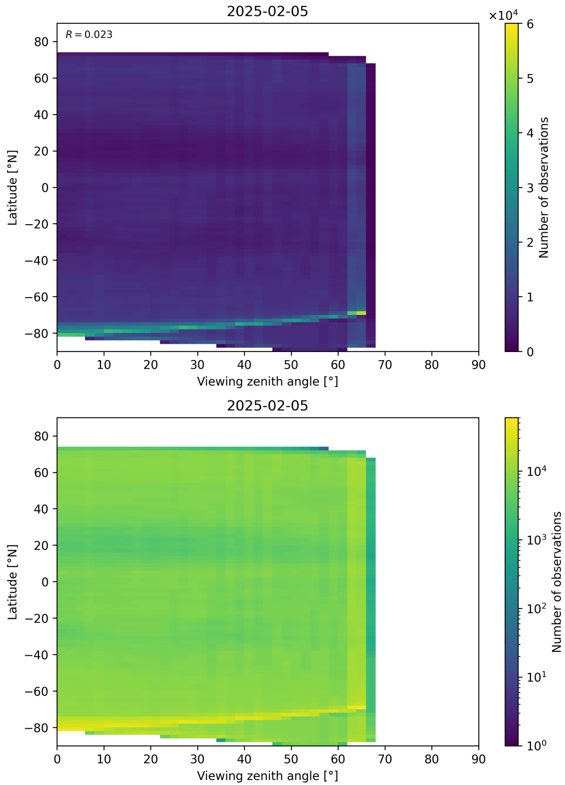
Figure 113: Scatter density plot of “Viewing zenith angle” against “Latitude” for 2025-02-04 to 2025-02-06.
