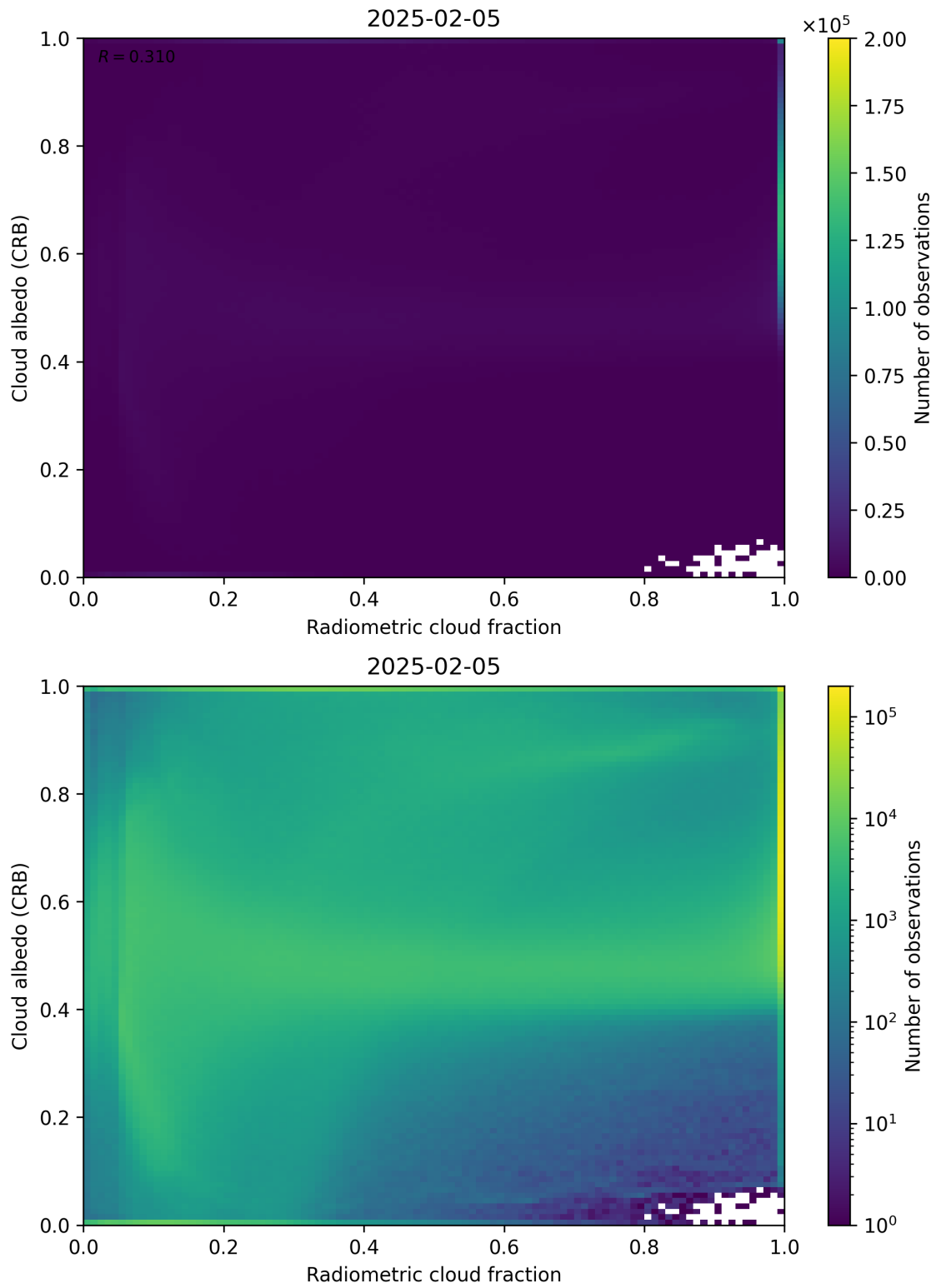
Figure 71: Scatter density plot of “Radiometric cloud fraction” against “Cloud albedo (CRB)” for 2025-02-04 to 2025-02-06.
