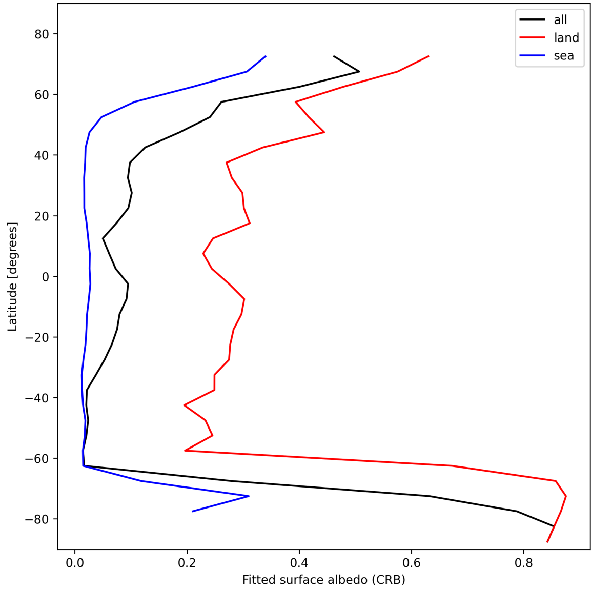
Figure 30: Zonal average of “Fitted surface albedo (CRB)” for 2025-02-04 to 2025-02-06.
