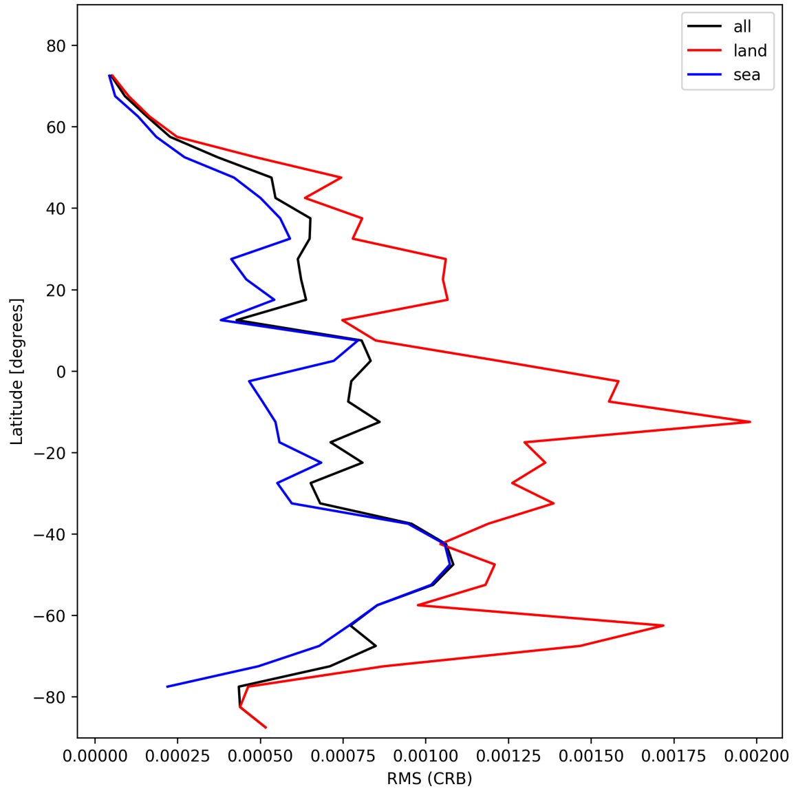
Figure 32: Zonal average of “RMS (CRB)” for 2025-02-04 to 2025-02-06.
