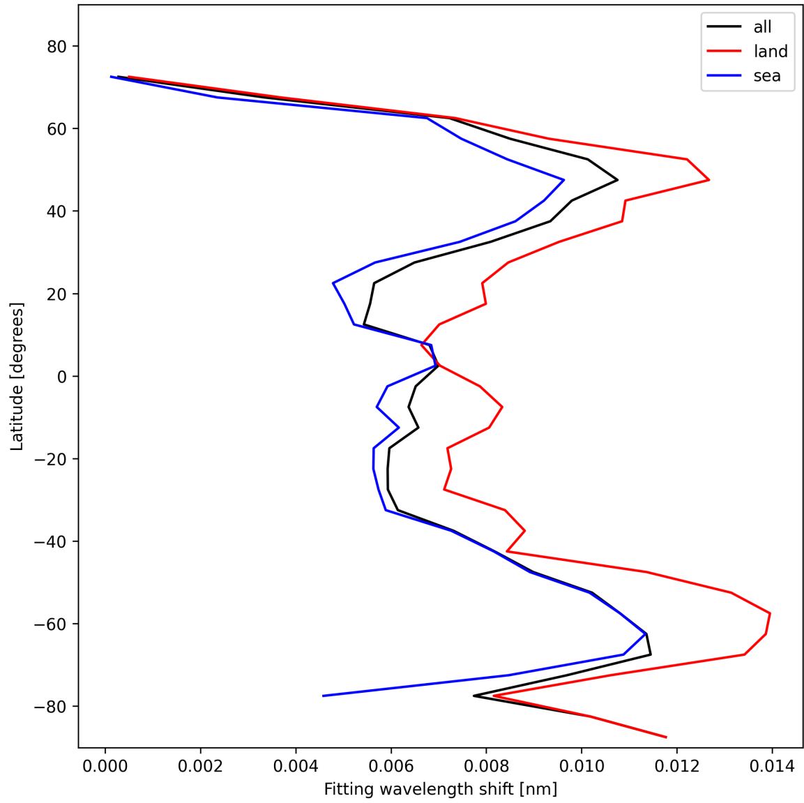
Figure 33: Zonal average of “Fitting wavelength shift” for 2025-02-04 to 2025-02-06.
