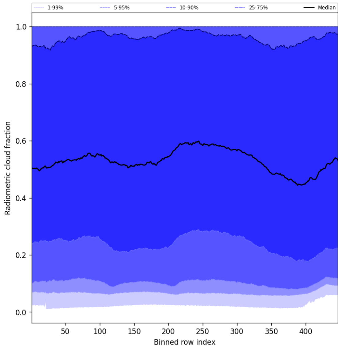
Figure 55: Along track statistics of “Radiometric cloud fraction” for 2025-02-04 to 2025-02-06
