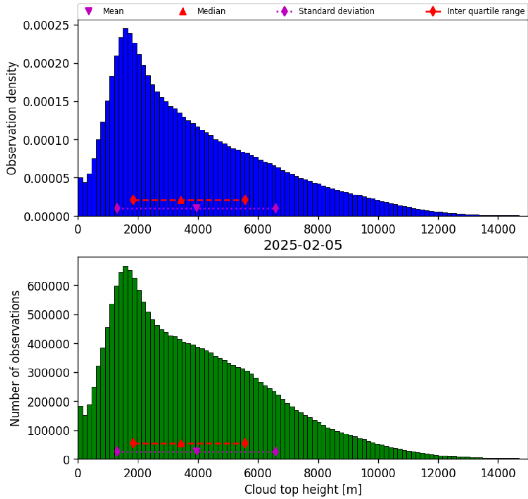
Figure 40: Histogram of “Cloud top height” for 2025-02-04 to 2025-02-06
