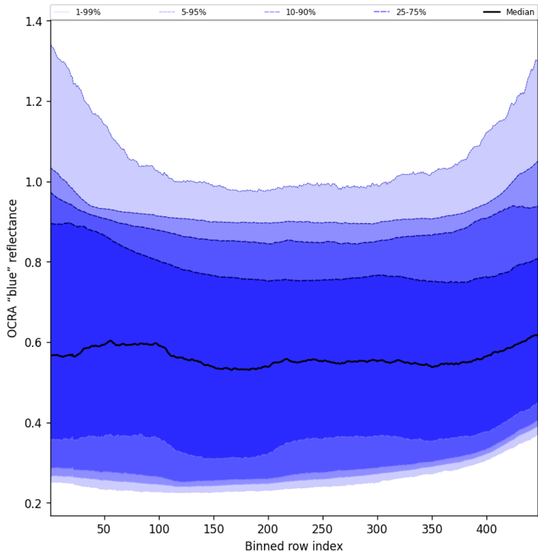
Figure 67: Along track statistics of "OCRA "blue" reflectance" for 2025-02-04 to 2025-02-06
