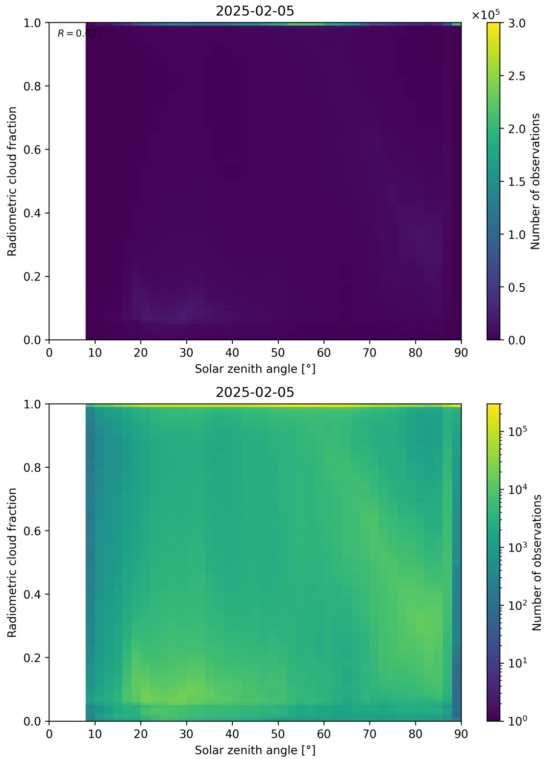
Figure 99: Scatter density plot of “Solar zenith angle” against “Radiometric cloud fraction” for 2025-02-04 to 2025-02-06.
