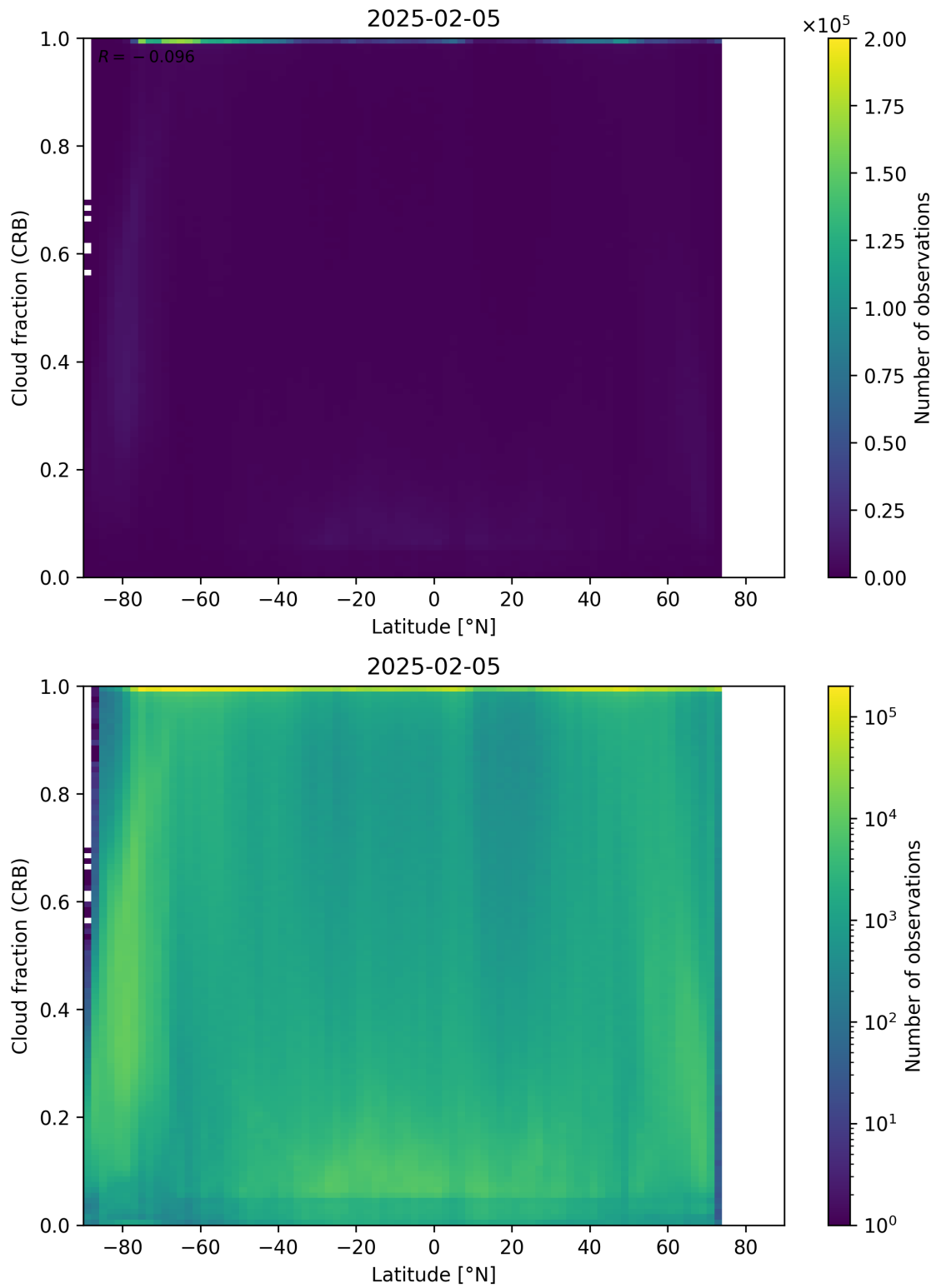
Figure 94: Scatter density plot of “Latitude” against “Cloud fraction (CRB)” for 2025-02-04 to 2025-02-06.
