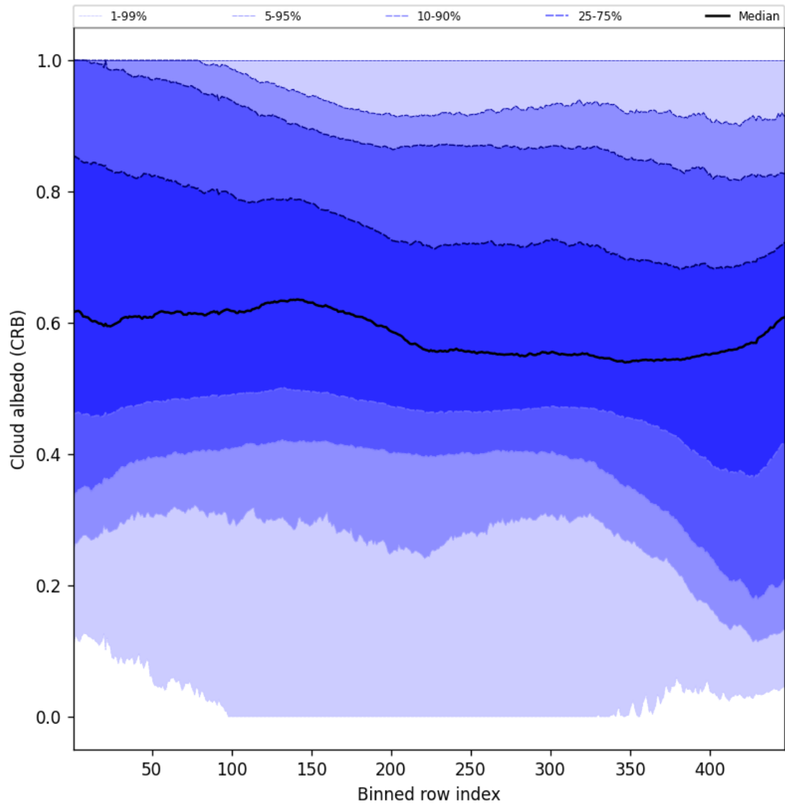
Figure 60: Along track statistics of “Cloud albedo (CRB)” for 2025-02-04 to 2025-02-06
