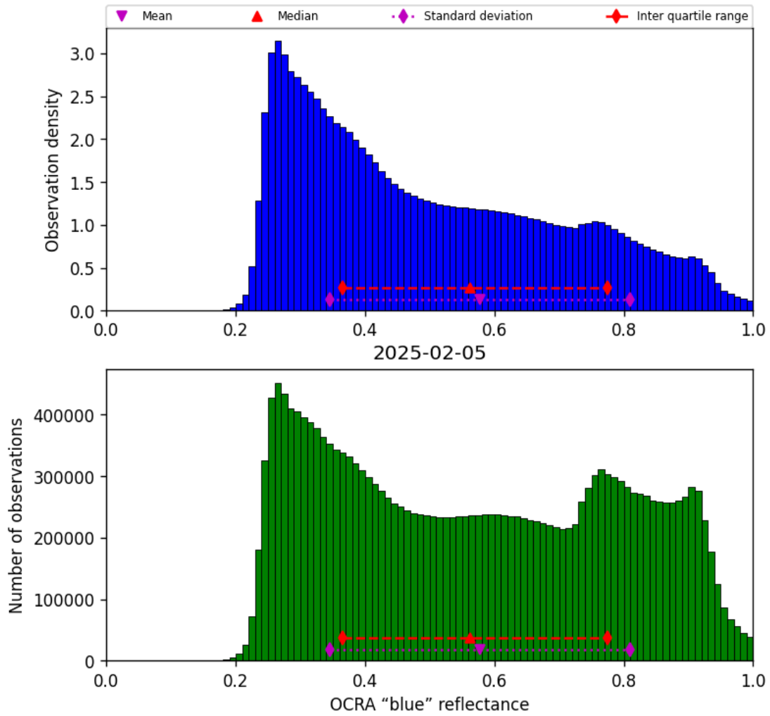
Figure 51: Histogram of “OCRA “blue” reflectance” for 2025-02-04 to 2025-02-06
