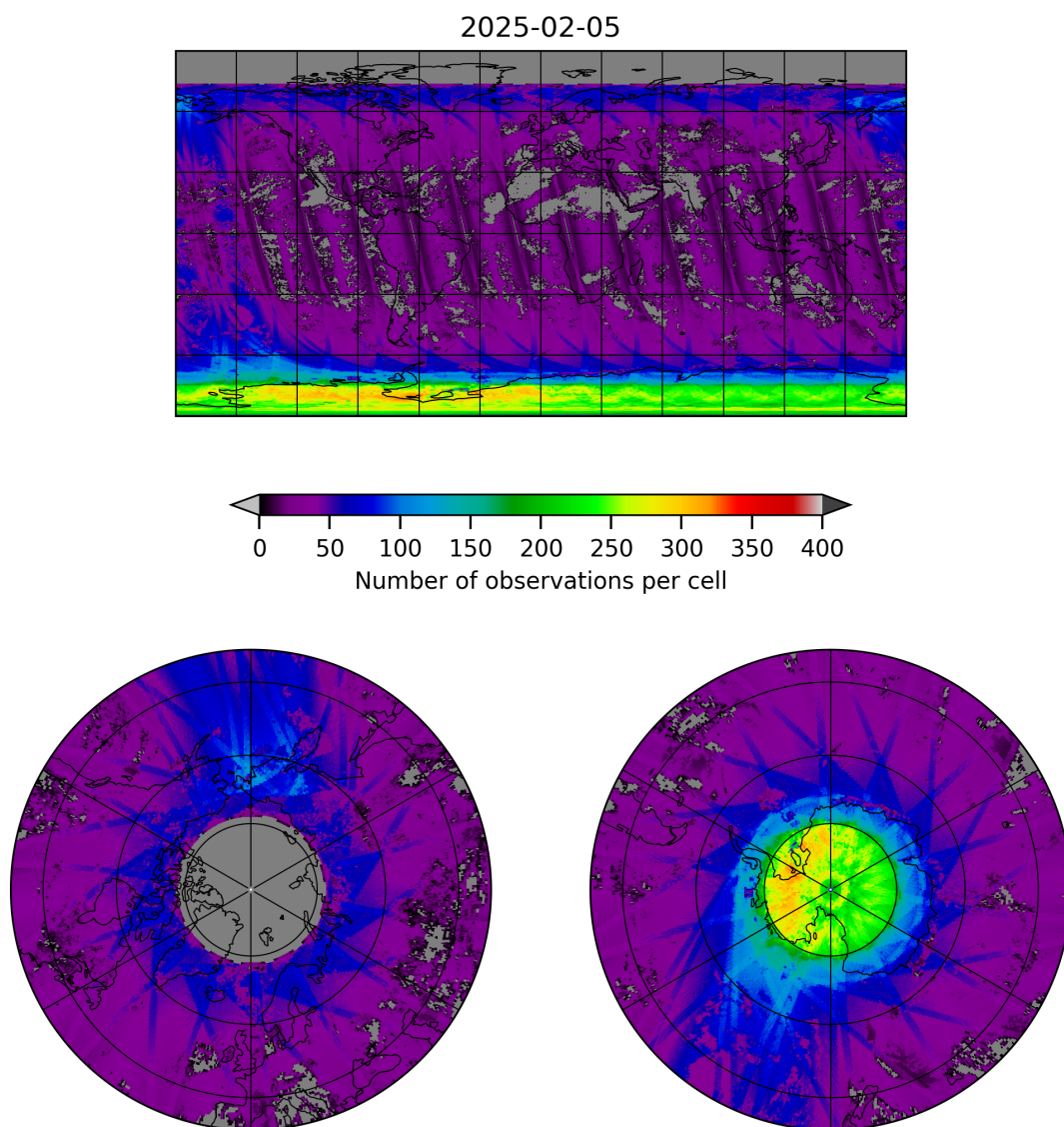
Figure 21: Map of the number of observations for 2025-02-04 to 2025-02-06
