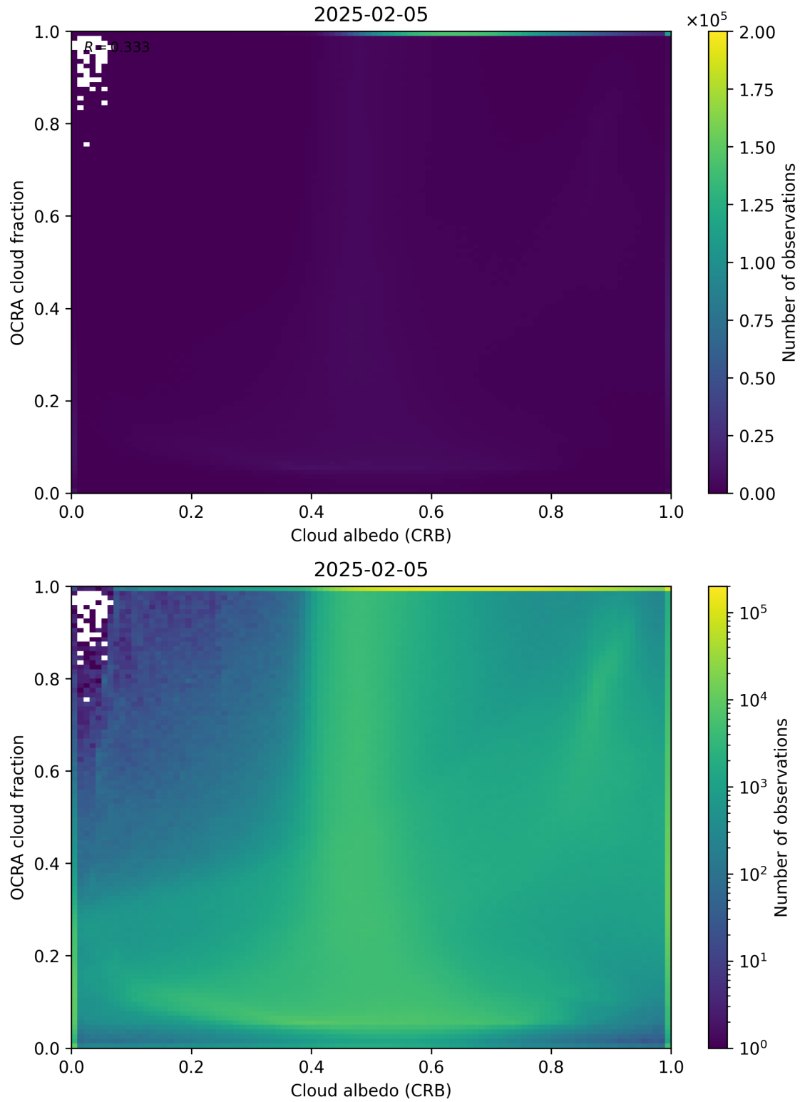
Figure 70: Scatter density plot of “Cloud albedo (CRB)” against “OCRA cloud fraction” for 2025-02-04 to 2025-02-06.
