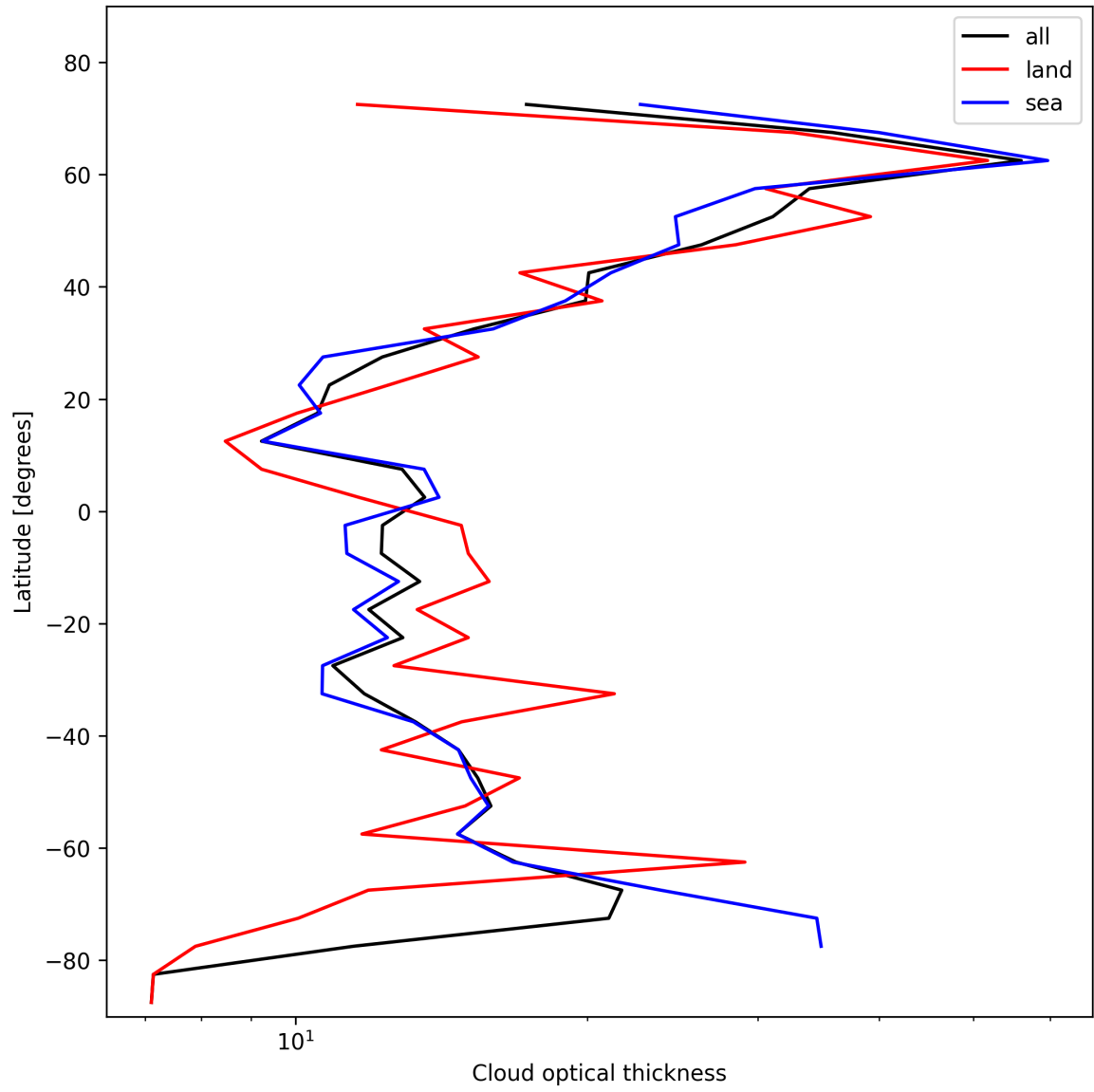
Figure 25: Zonal average of “Cloud optical thickness” for 2025-02-04 to 2025-02-06.
