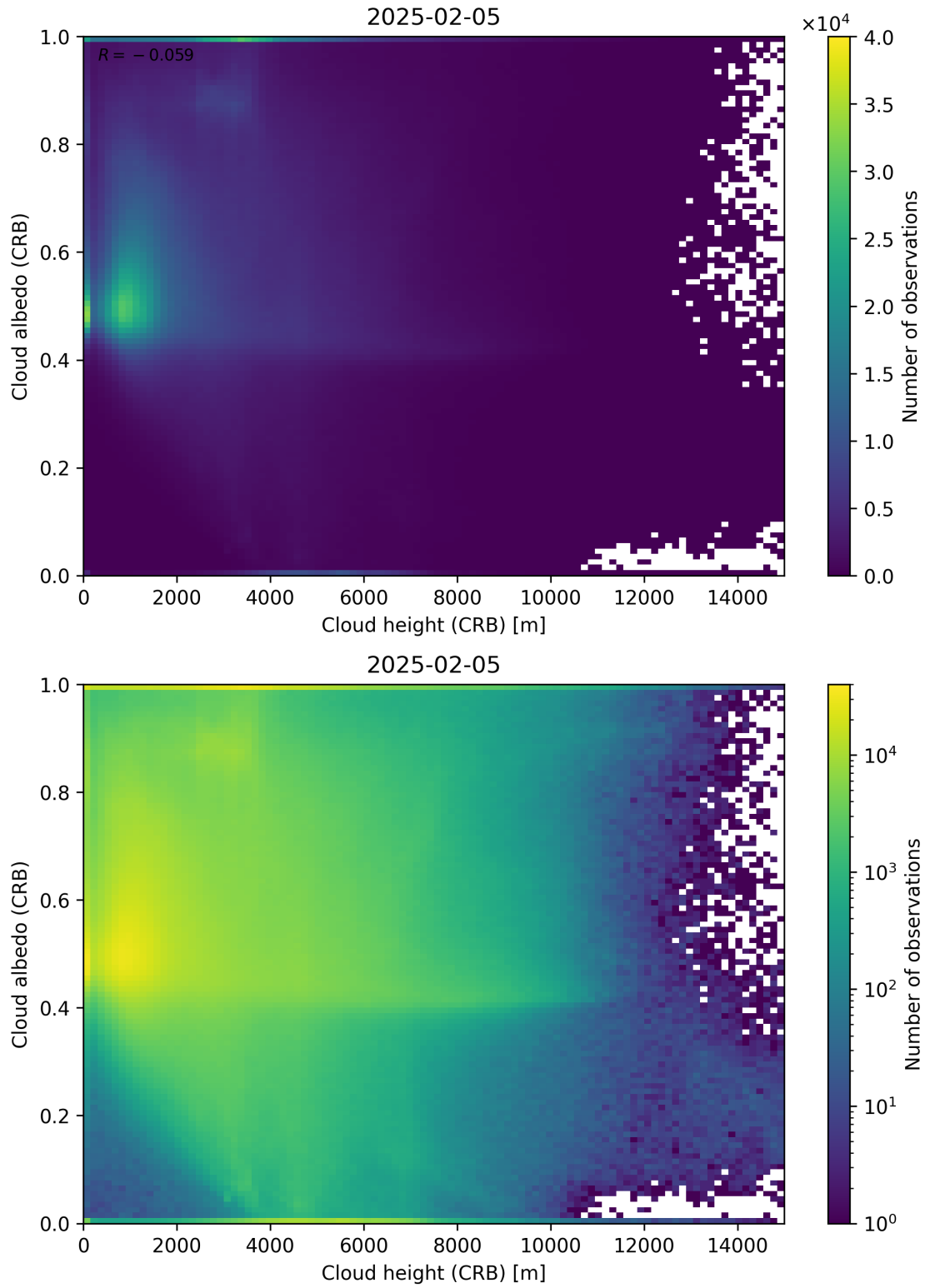
Figure 80: Scatter density plot of “Cloud height (CRB)” against “Cloud albedo (CRB)” for 2025-02-04 to 2025-02-06.
