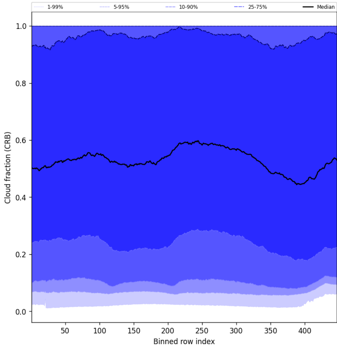
Figure 58: Along track statistics of “Cloud fraction (CRB)” for 2025-02-04 to 2025-02-06
