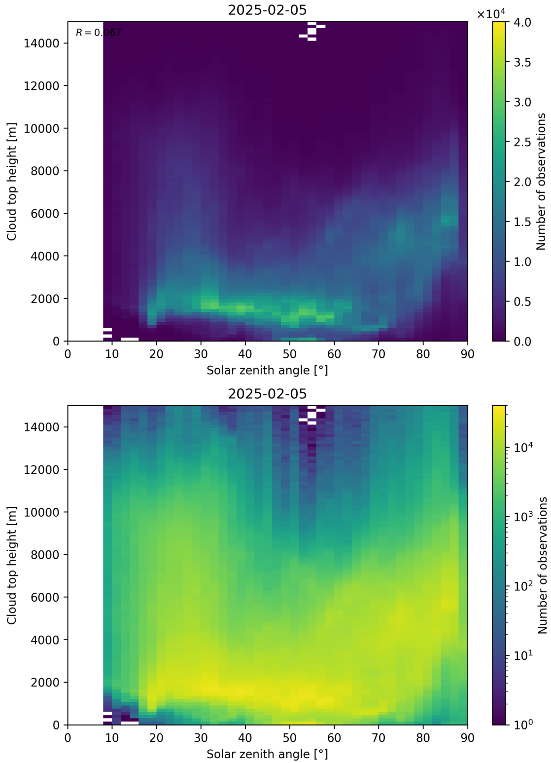
Figure 104: Scatter density plot of “Solar zenith angle” against “Cloud top height” for 2025-02-04 to 2025-02-06.
