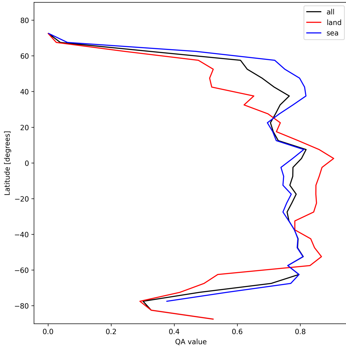
Figure 22: Zonal average of “QA value” for 2025-02-04 to 2025-02-06.
