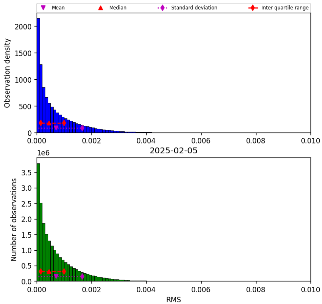
Figure 47: Histogram of “RMS” for 2025-02-04 to 2025-02-06
