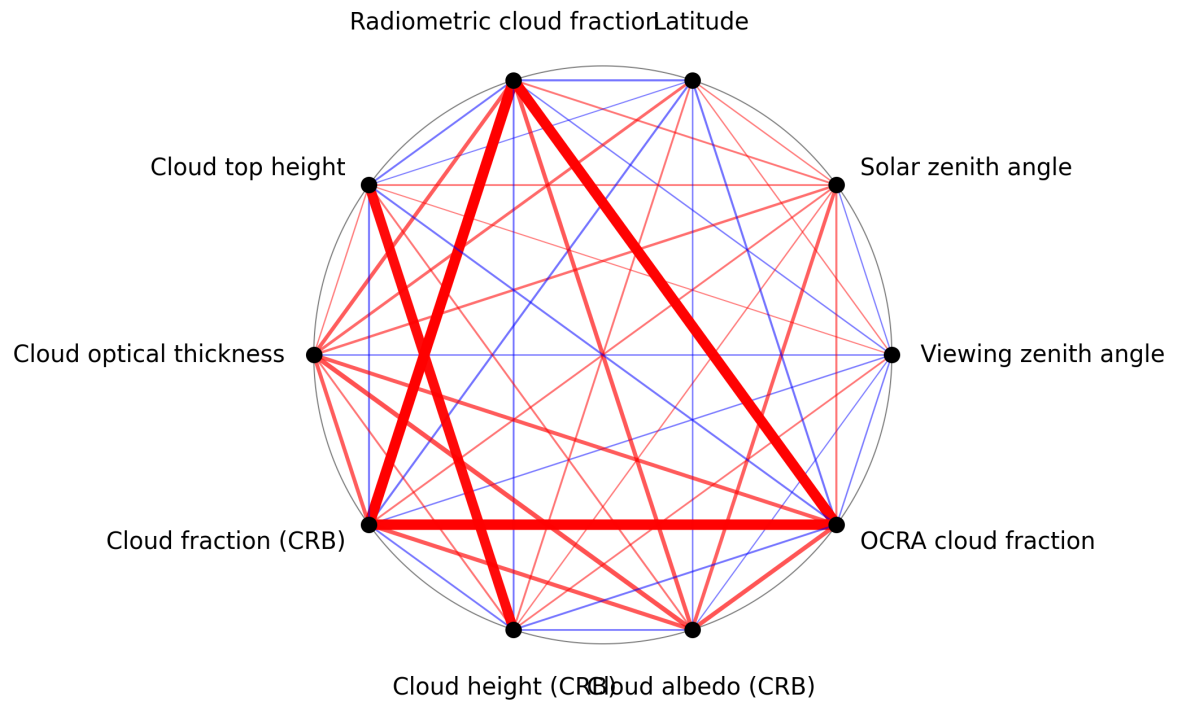
Figure 1: Map of correlation graph for 2025-02-04 to 2025-02-06.
