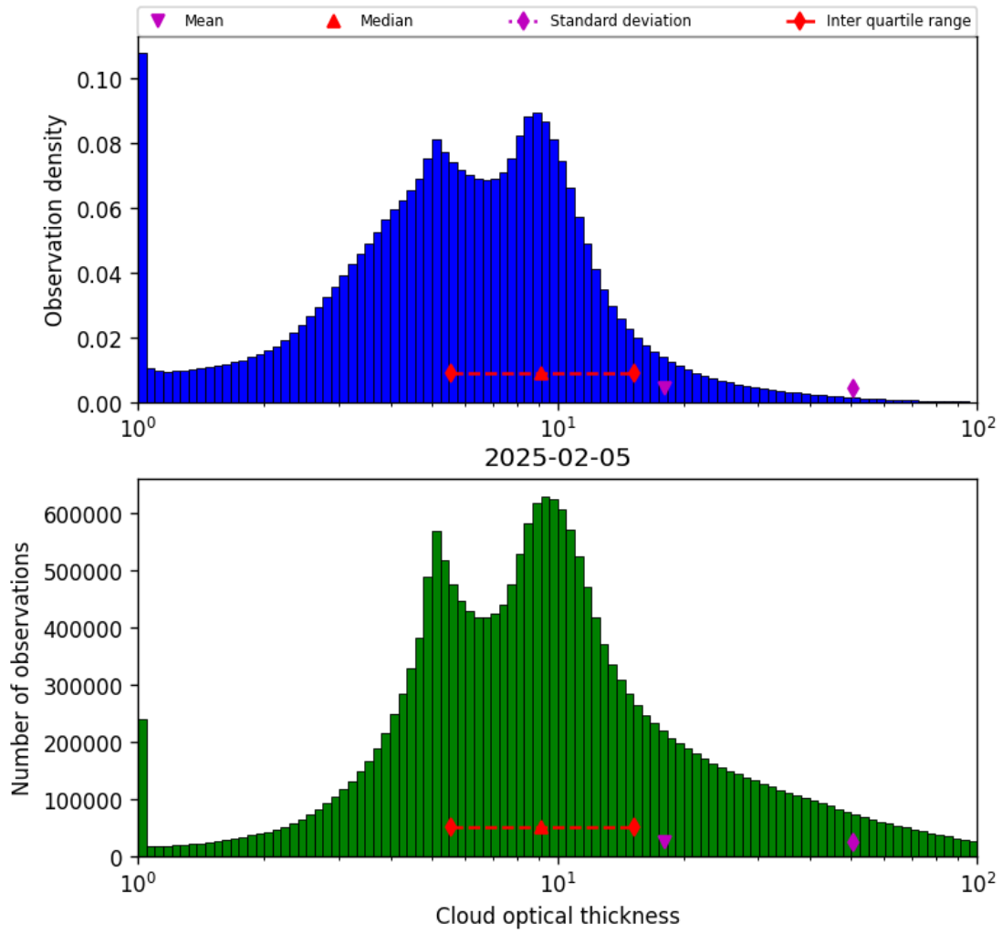
Figure 41: Histogram of “Cloud optical thickness” for 2025-02-04 to 2025-02-06
