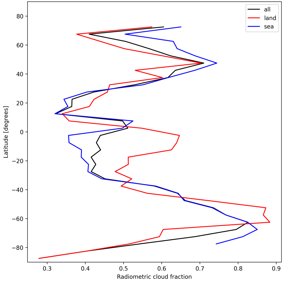
Figure 23: Zonal average of “Radiometric cloud fraction” for 2025-02-04 to 2025-02-06.
