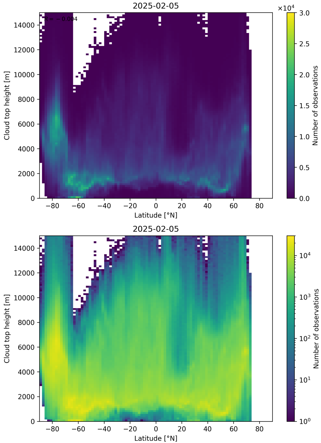
Figure 97: Scatter density plot of “Latitude” against “Cloud top height” for 2025-02-04 to 2025-02-06.
