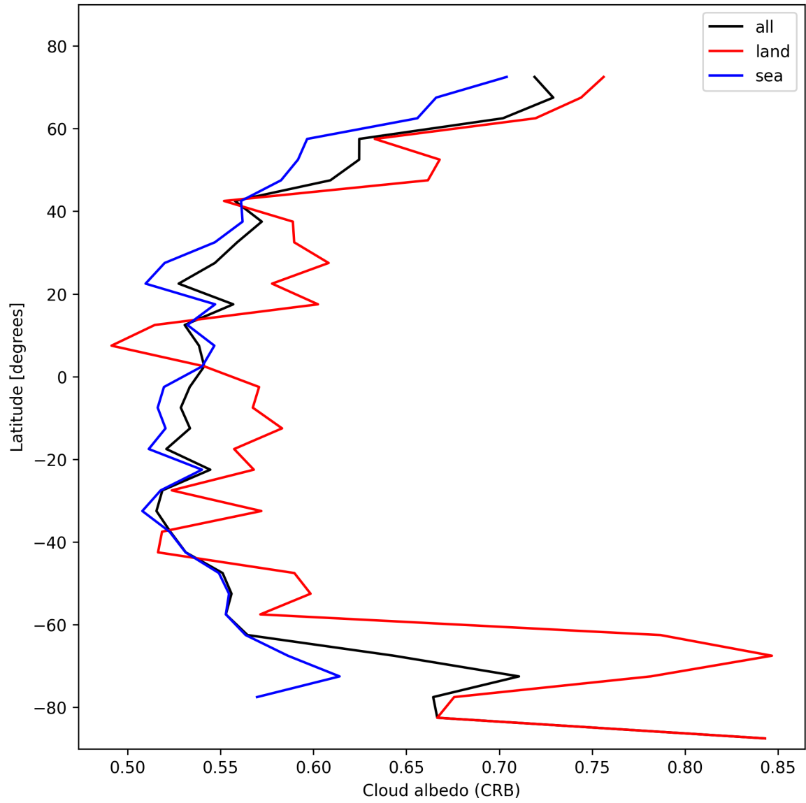
Figure 28: Zonal average of “Cloud albedo (CRB)” for 2025-02-04 to 2025-02-06.
