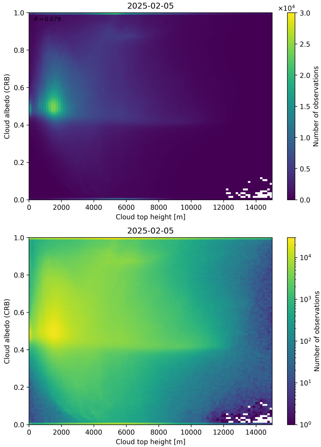
Figure 86: Scatter density plot of “Cloud top height” against “Cloud albedo (CRB)” for 2025-02-04 to 2025-02-06.
