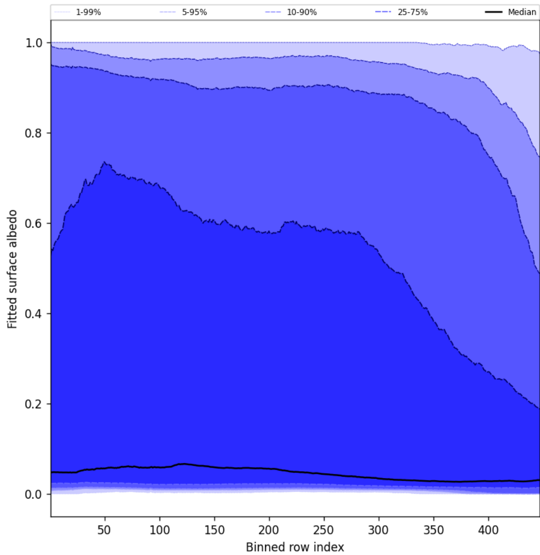
Figure 61: Along track statistics of “Fitted surface albedo” for 2025-02-04 to 2025-02-06
