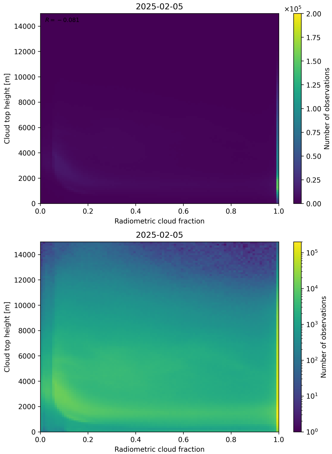
Figure 76: Scatter density plot of “Radiometric cloud fraction” against “Cloud top height” for 2025-02-04 to 2025-02-06.
