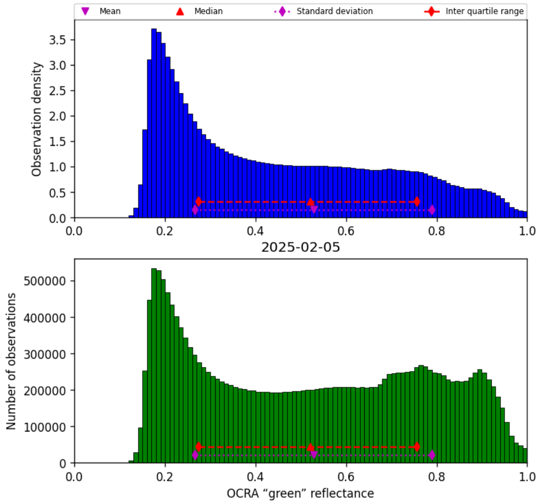
Figure 52: Histogram of “OCRA “green” reflectance” for 2025-02-04 to 2025-02-06
