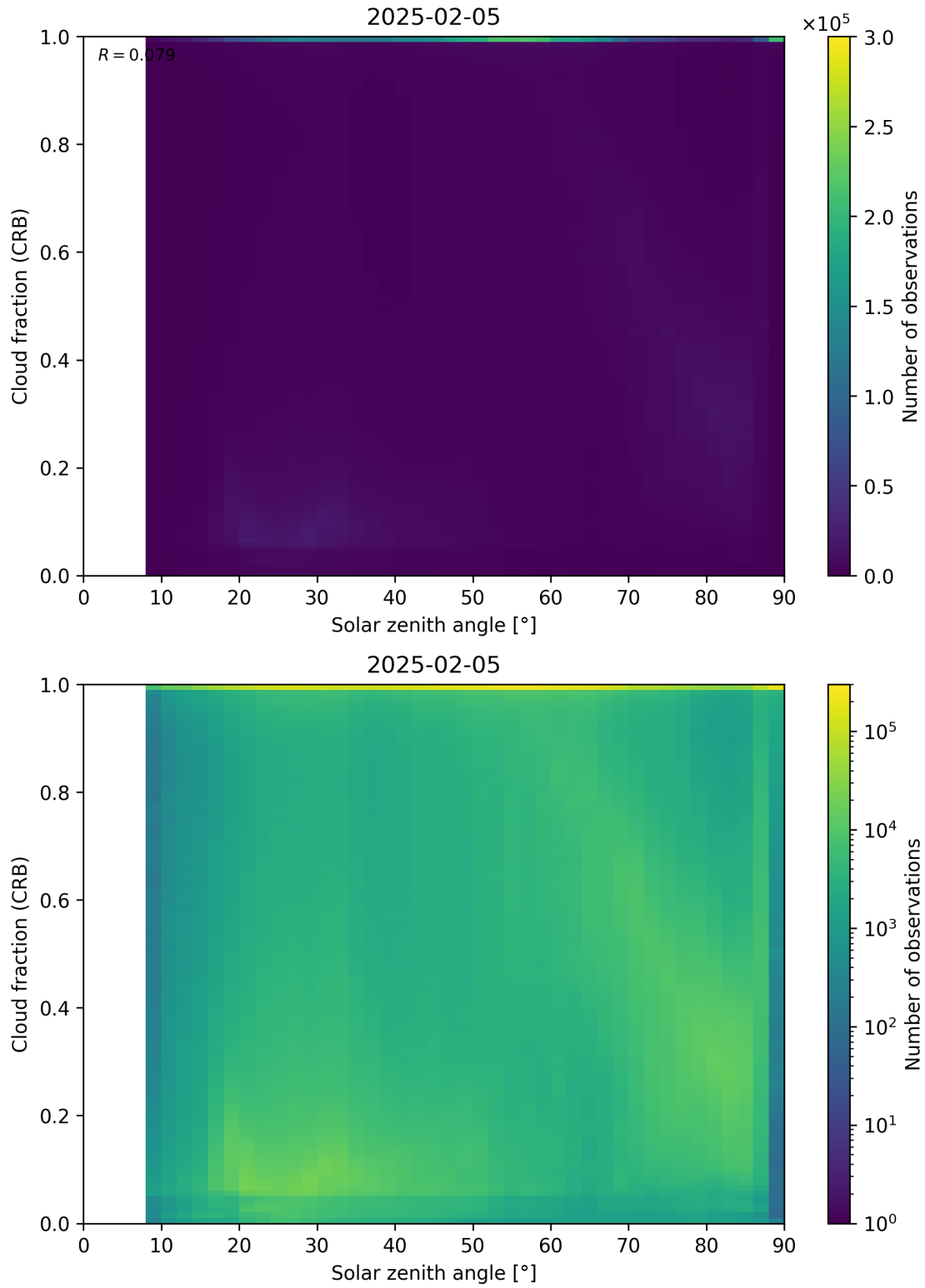
Figure 101: Scatter density plot of “Solar zenith angle” against “Cloud fraction (CRB)” for 2025-02-04 to 2025-02-06.
