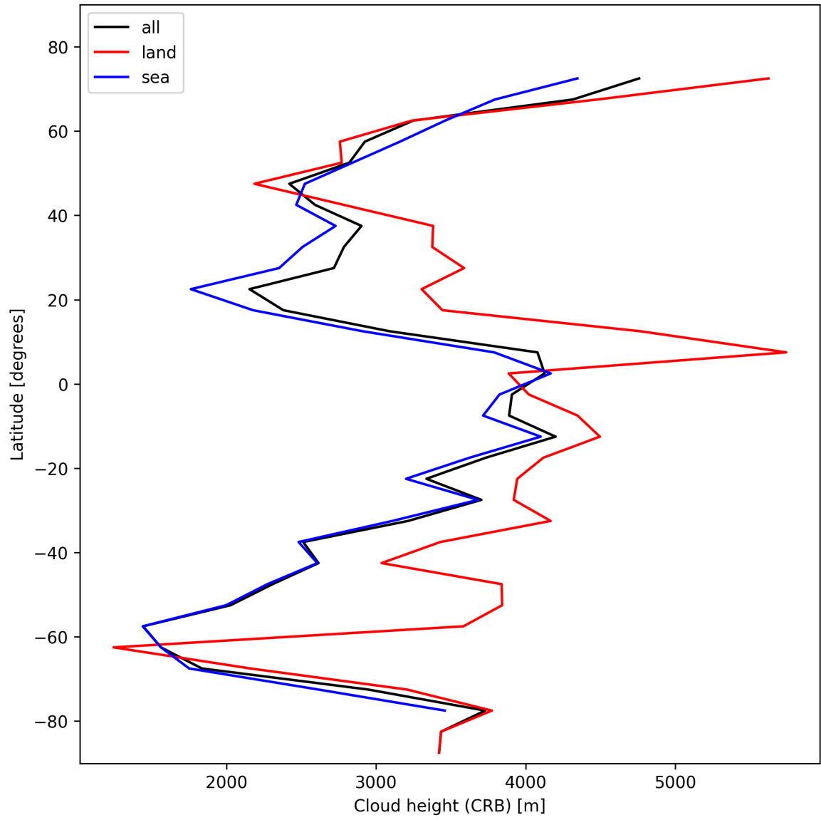
Figure 27: Zonal average of “Cloud height (CRB)” for 2025-02-04 to 2025-02-06.
