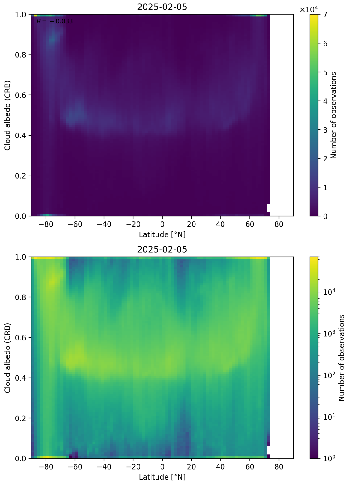
Figure 91: Scatter density plot of “Latitude” against “Cloud albedo (CRB)” for 2025-02-04 to 2025-02-06.
