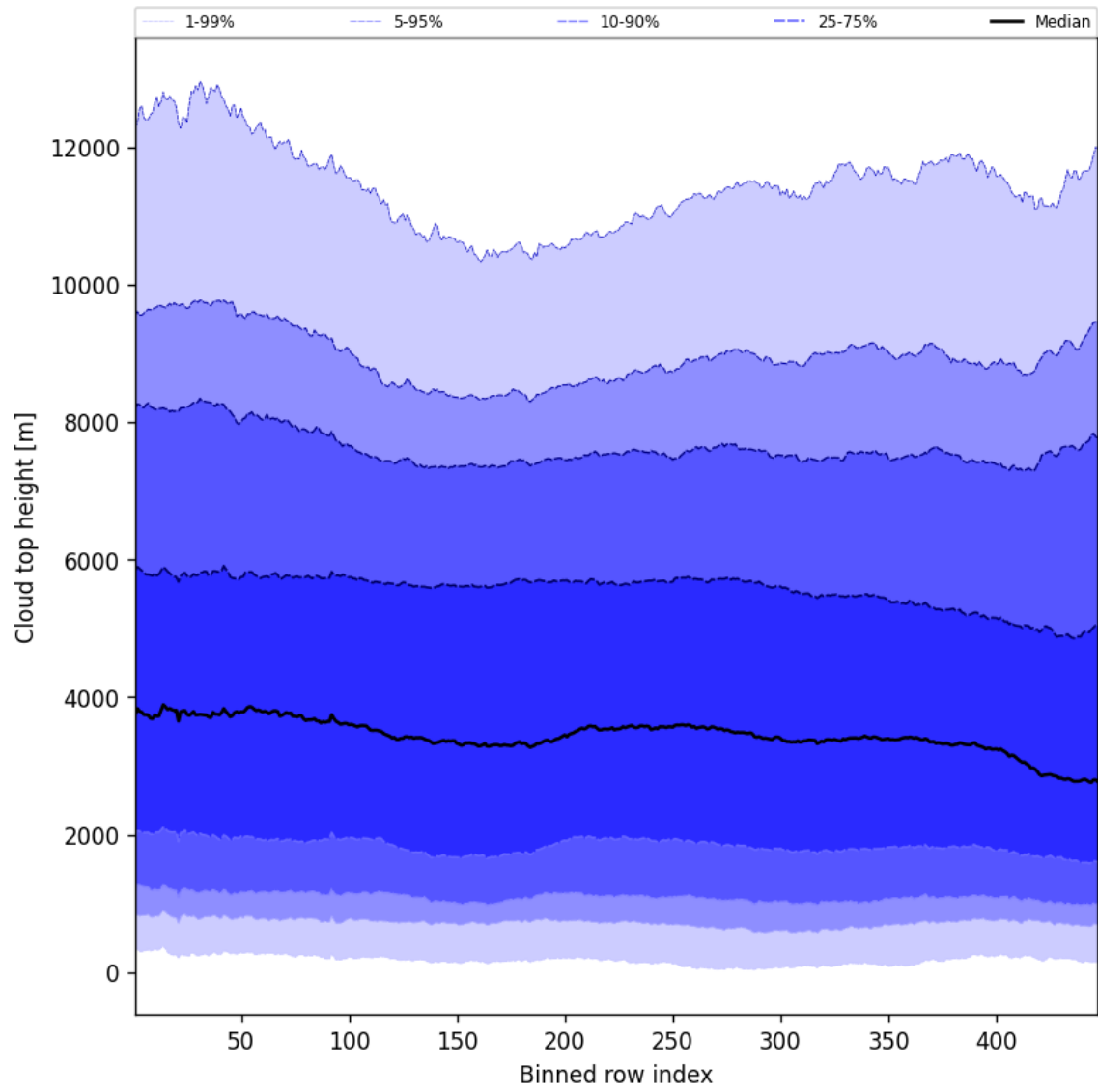
Figure 56: Along track statistics of “Cloud top height” for 2025-02-04 to 2025-02-06
