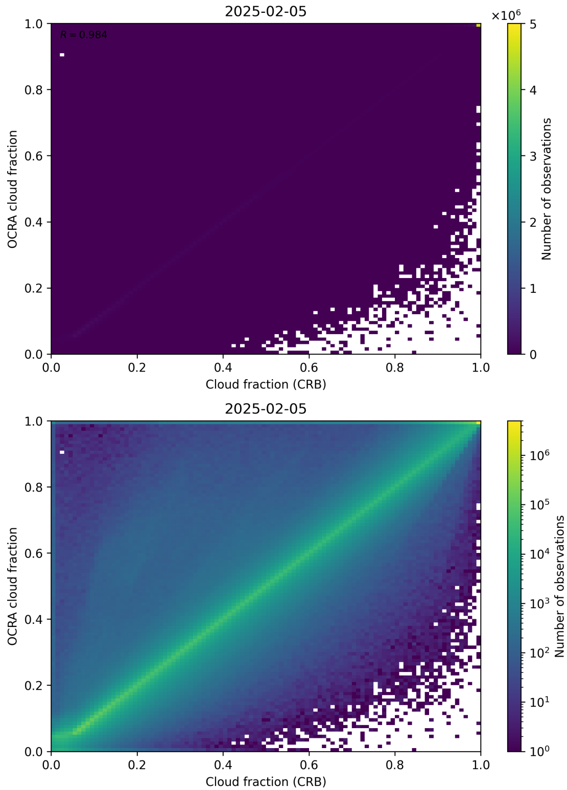
Figure 78: Scatter density plot of “Cloud fraction (CRB)” against “OCRA cloud fraction” for 2025-02-04 to 2025-02-06.
