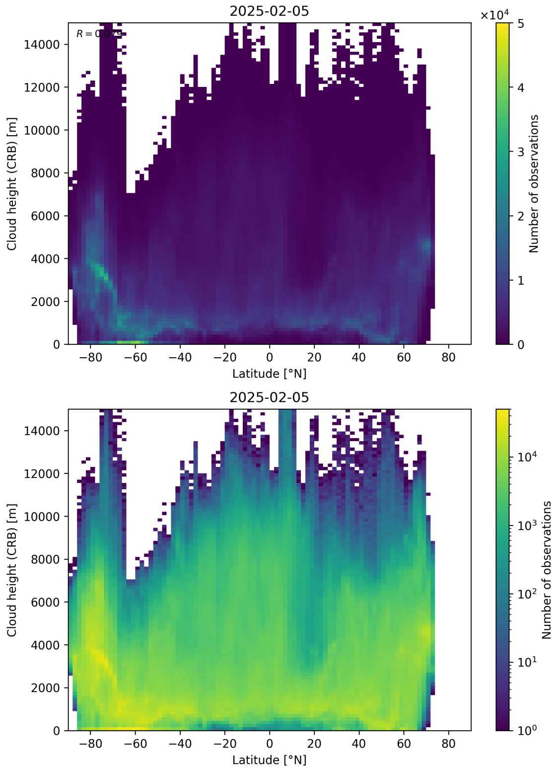
Figure 95: Scatter density plot of “Latitude” against “Cloud height (CRB)” for 2025-02-04 to 2025-02-06.
