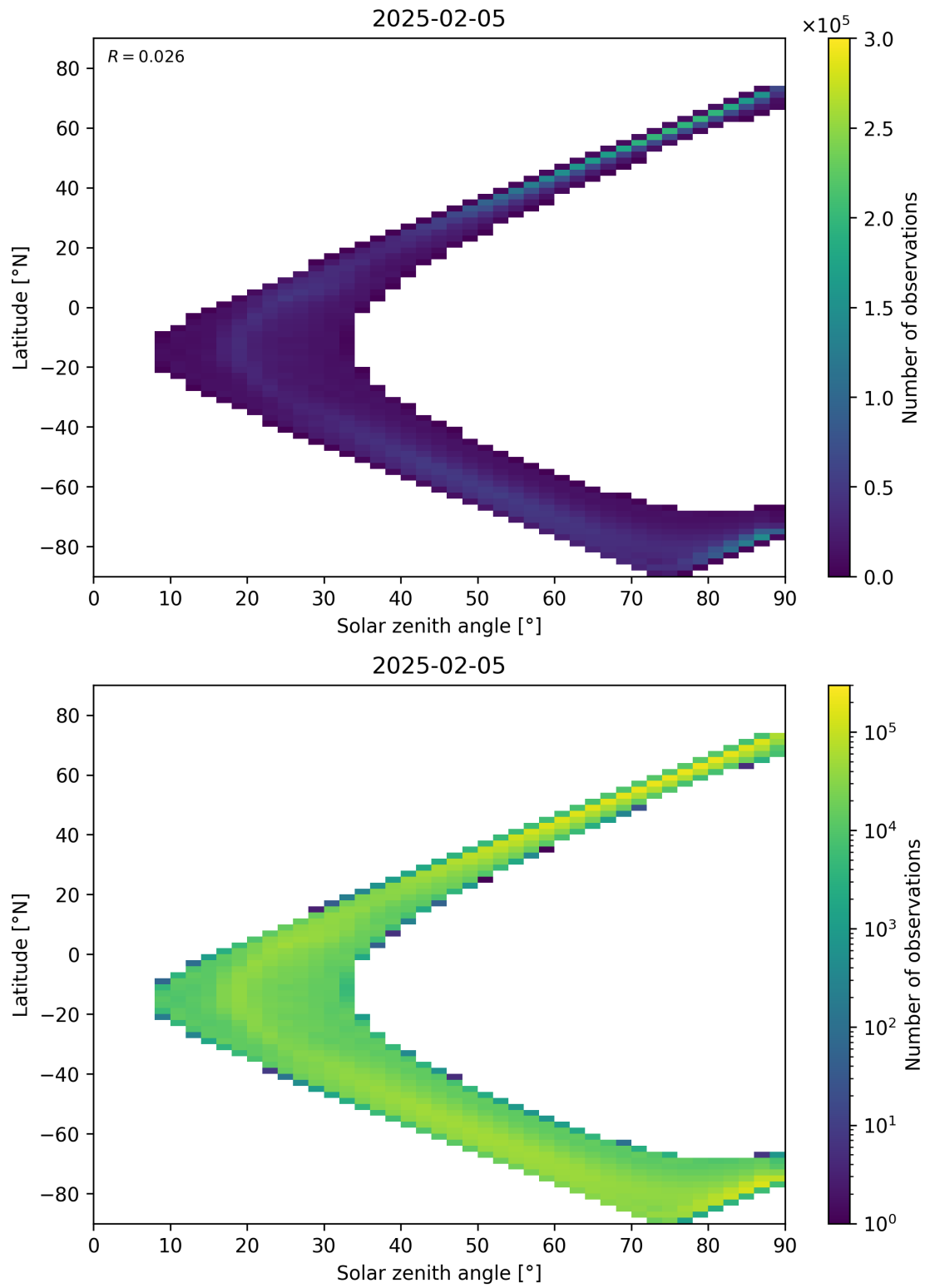
Figure 105: Scatter density plot of “Solar zenith angle” against “Latitude” for 2025-02-04 to 2025-02-06.
