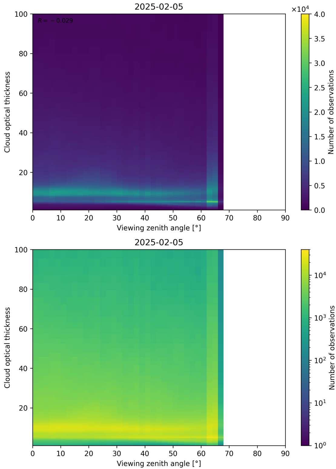
Figure 111: Scatter density plot of “Viewing zenith angle” against “Cloud optical thickness” for 2025-02-04 to 2025-02-06.
