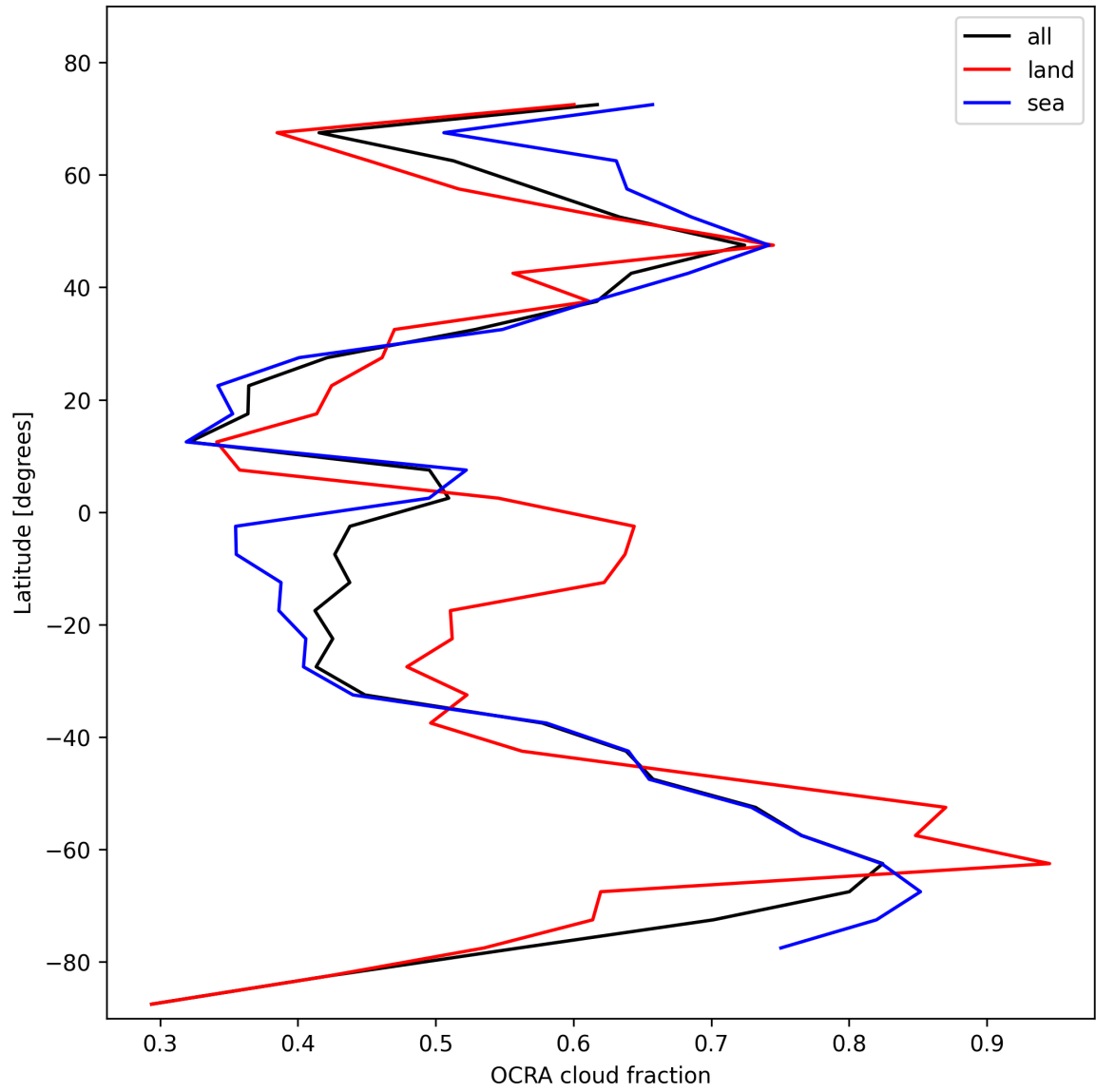
Figure 34: Zonal average of “OCRA cloud fraction” for 2025-02-04 to 2025-02-06.
