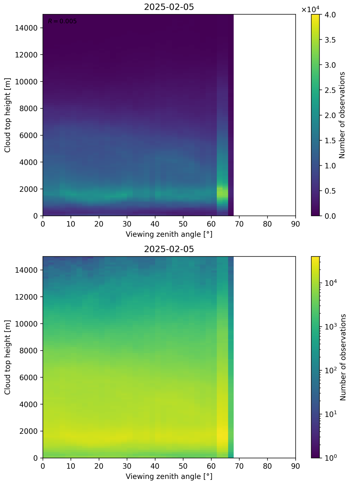
Figure 112: Scatter density plot of “Viewing zenith angle” against “Cloud top height” for 2025-02-04 to 2025-02-06.
