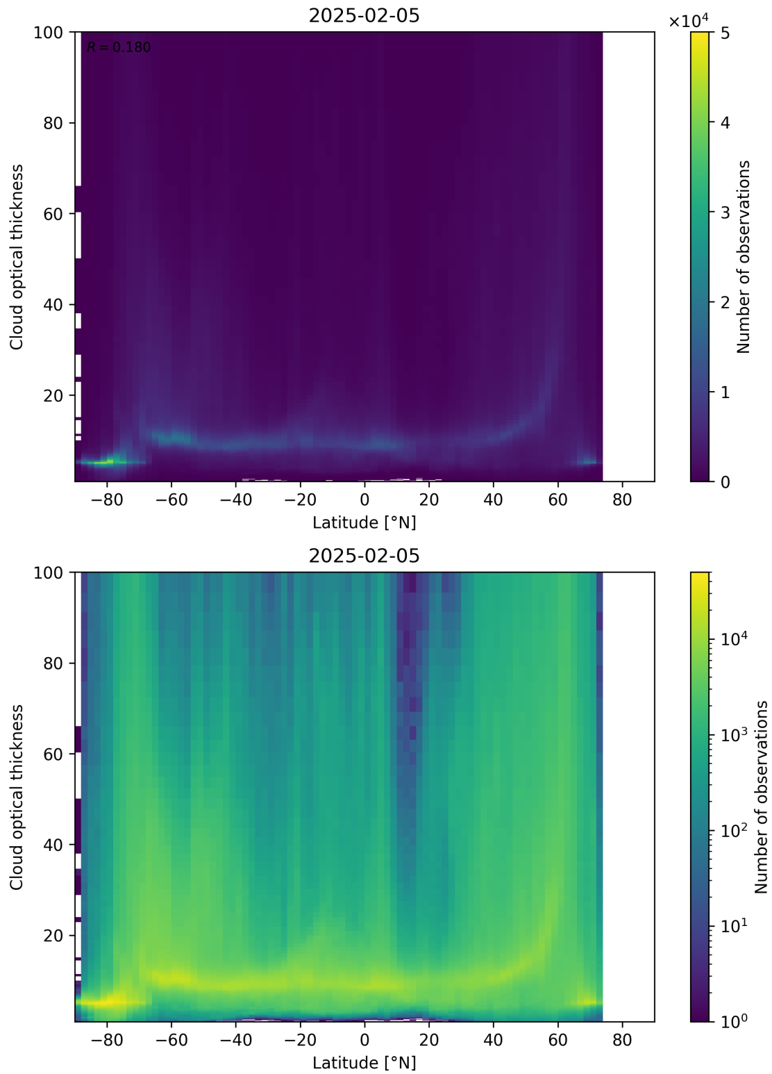
Figure 96: Scatter density plot of “Latitude” against “Cloud optical thickness” for 2025-02-04 to 2025-02-06.
