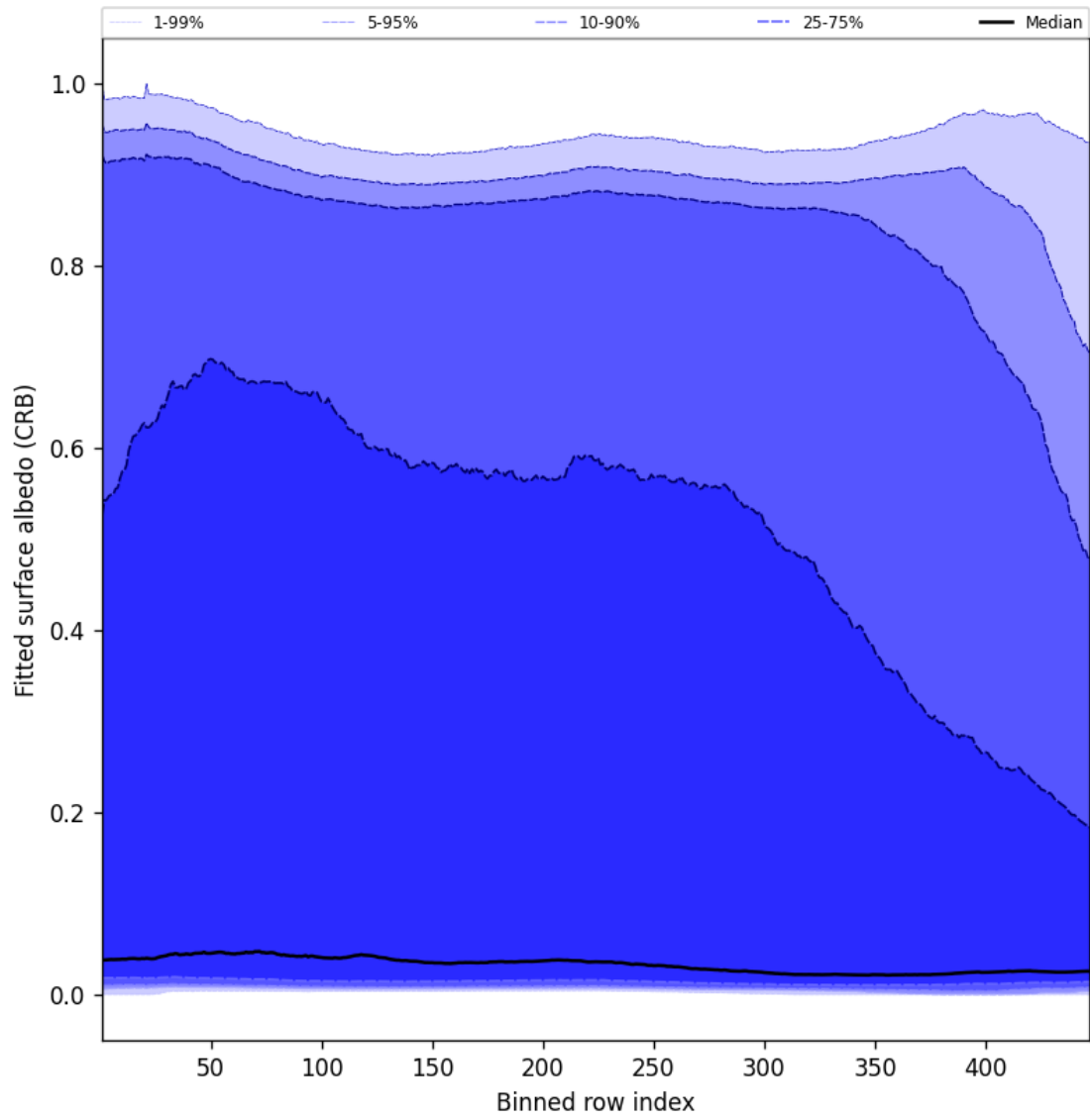
Figure 62: Along track statistics of “Fitted surface albedo (CRB)” for 2025-02-04 to 2025-02-06
