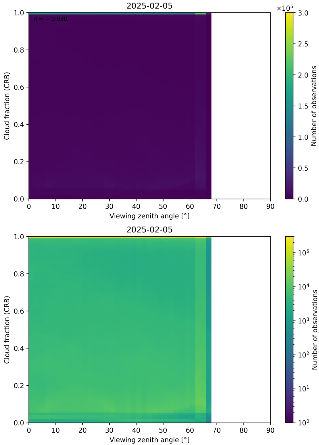
Figure 109: Scatter density plot of “Viewing zenith angle” against “Cloud fraction (CRB)” for 2025-02-04 to 2025-02-06.
