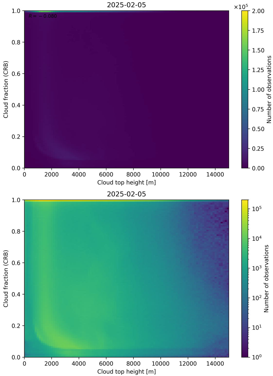
Figure 88: Scatter density plot of “Cloud top height” against “Cloud fraction (CRB)” for 2025-02-04 to 2025-02-06.
