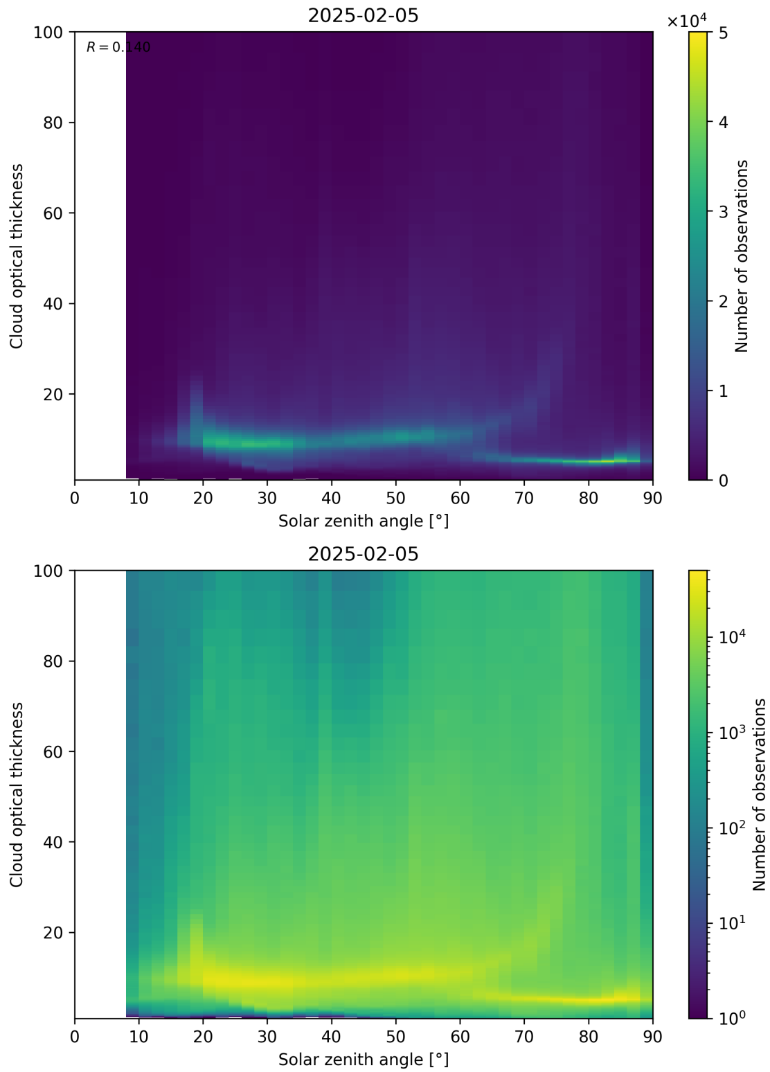
Figure 103: Scatter density plot of “Solar zenith angle” against “Cloud optical thickness” for 2025-02-04 to 2025-02-06.
