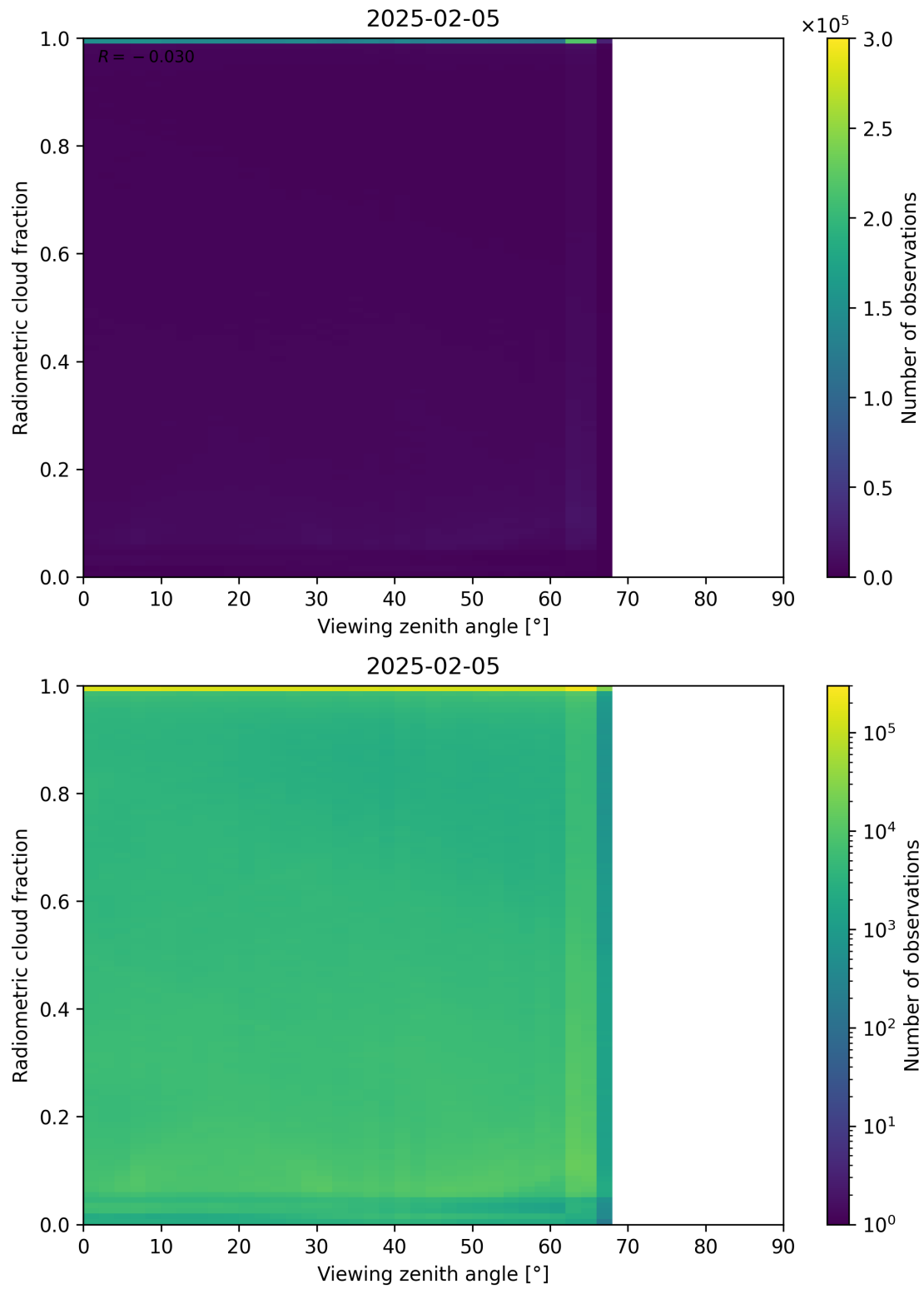
Figure 107: Scatter density plot of “Viewing zenith angle” against “Radiometric cloud fraction” for 2025-02-04 to 2025-02-06.
