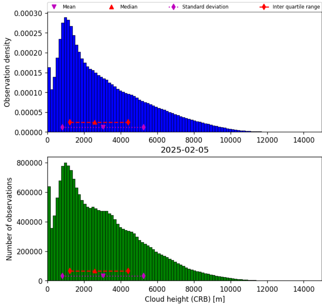
Figure 43: Histogram of “Cloud height (CRB)” for 2025-02-04 to 2025-02-06
