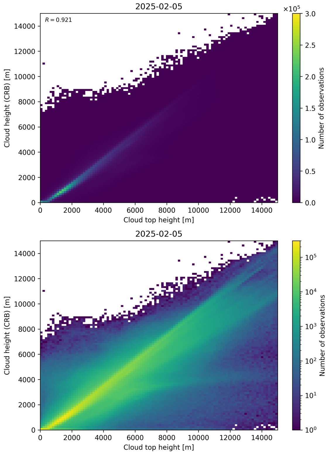
Figure 89: Scatter density plot of “Cloud top height” against “Cloud height (CRB)” for 2025-02-04 to 2025-02-06.
