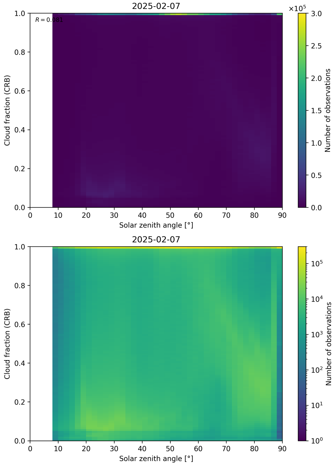
Figure 101: Scatter density plot of “Solar zenith angle” against “Cloud fraction (CRB)” for 2025-02-06 to 2025-02-08.
