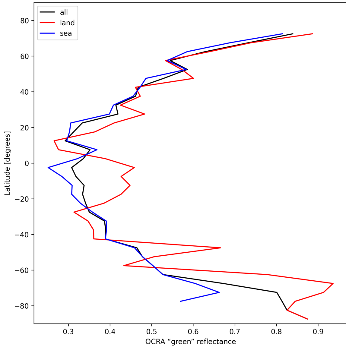
Figure 36: Zonal average of “OCRA “green” reflectance” for 2025-02-06 to 2025-02-08.
