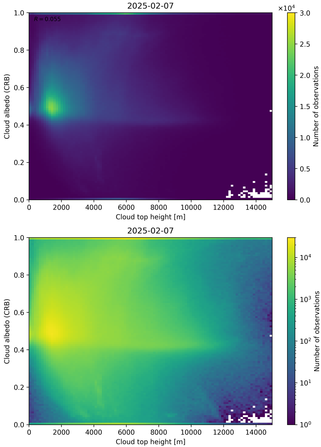
Figure 86: Scatter density plot of “Cloud top height” against “Cloud albedo (CRB)” for 2025-02-06 to 2025-02-08.
