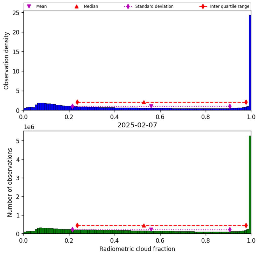
Figure 39: Histogram of “Radiometric cloud fraction” for 2025-02-06 to 2025-02-08
