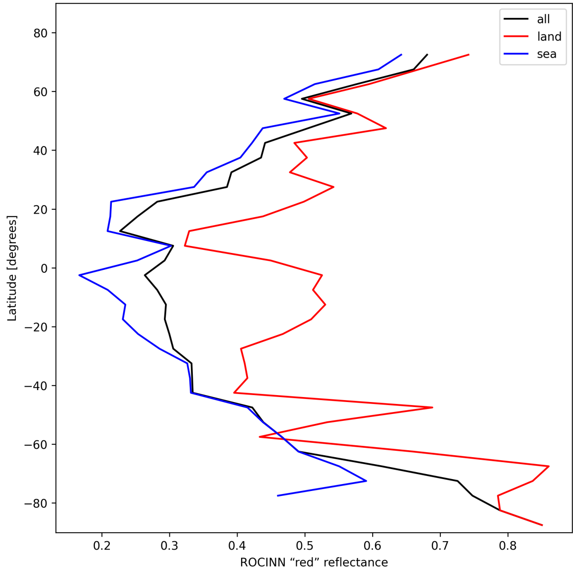
Figure 37: Zonal average of “ROCINN “red” reflectance” for 2025-02-06 to 2025-02-08.
