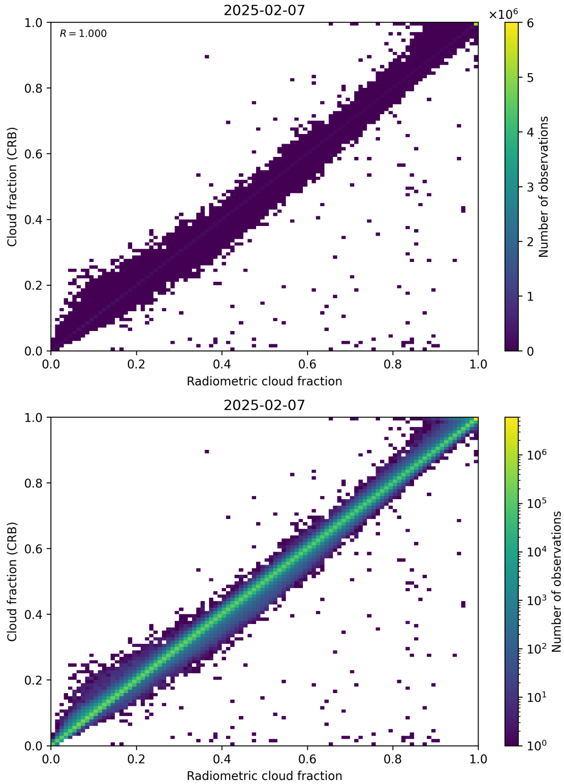
Figure 73: Scatter density plot of “Radiometric cloud fraction” against “Cloud fraction (CRB)” for 2025-02-06 to 2025-02-08.
