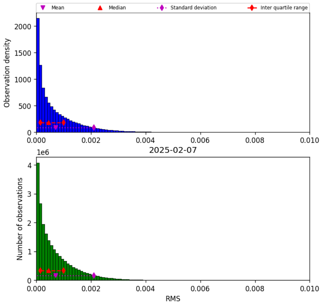
Figure 47: Histogram of “RMS” for 2025-02-06 to 2025-02-08
