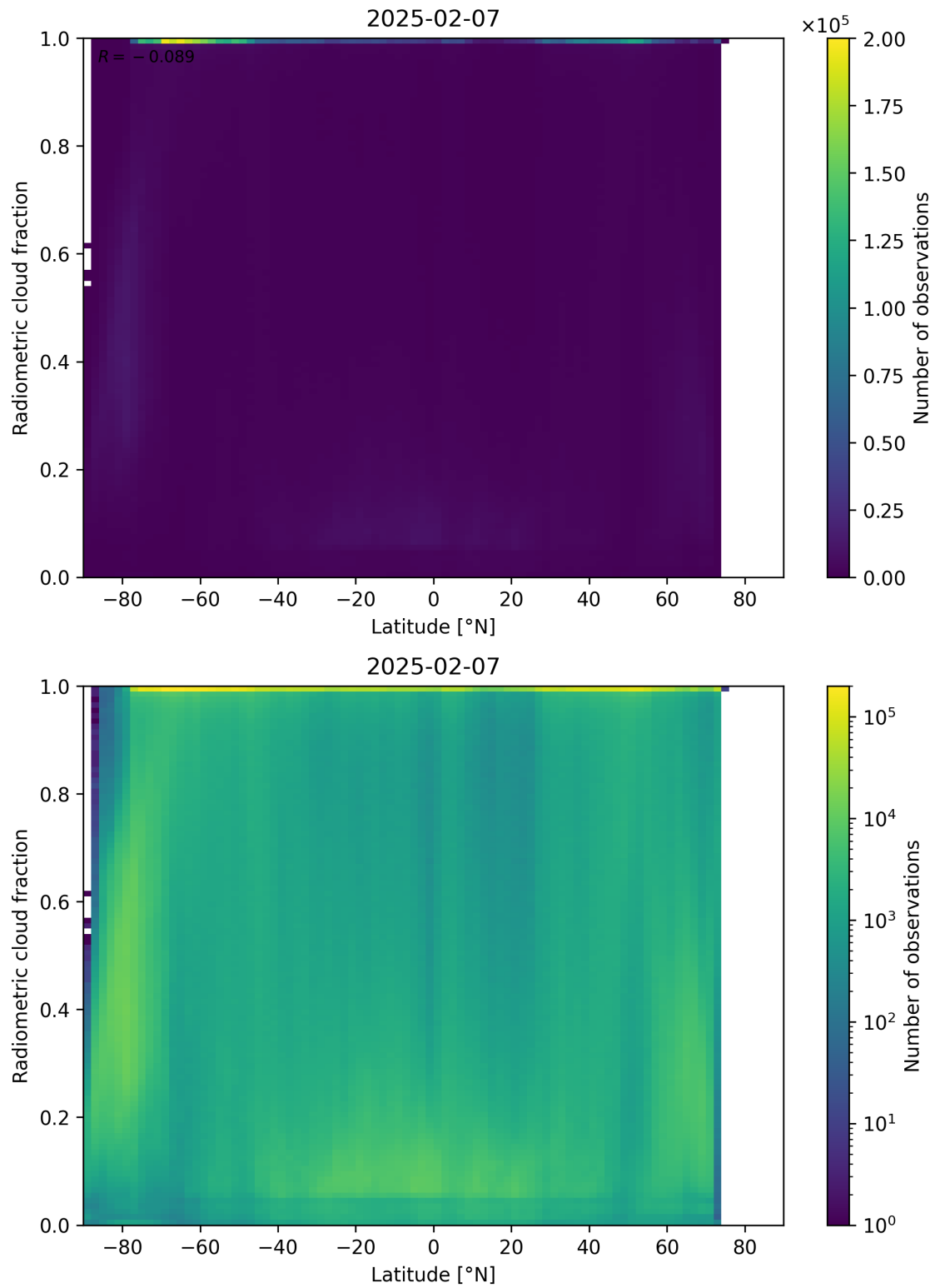
Figure 92: Scatter density plot of “Latitude” against “Radiometric cloud fraction” for 2025-02-06 to 2025-02-08.
