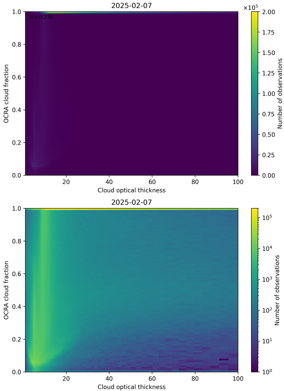
Figure 83: Scatter density plot of “Cloud optical thickness” against “OCRA cloud fraction” for 2025-02-06 to 2025-02-08.
