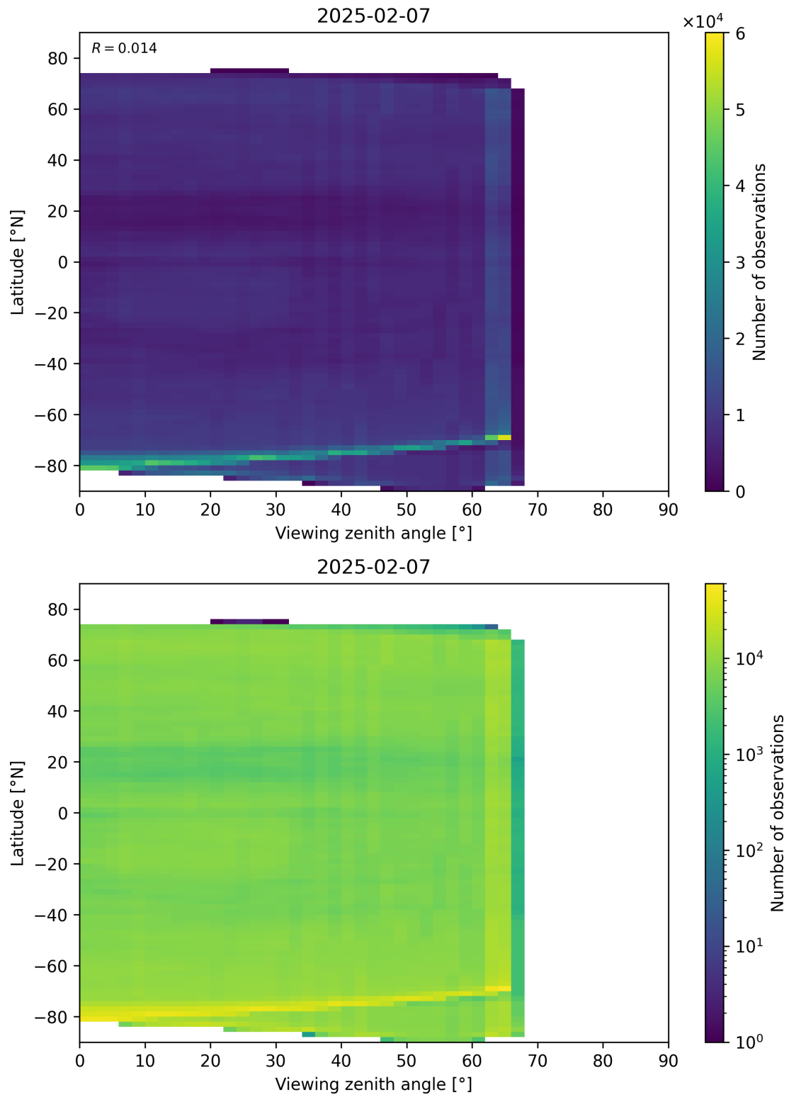
Figure 113: Scatter density plot of “Viewing zenith angle” against “Latitude” for 2025-02-06 to 2025-02-08.
