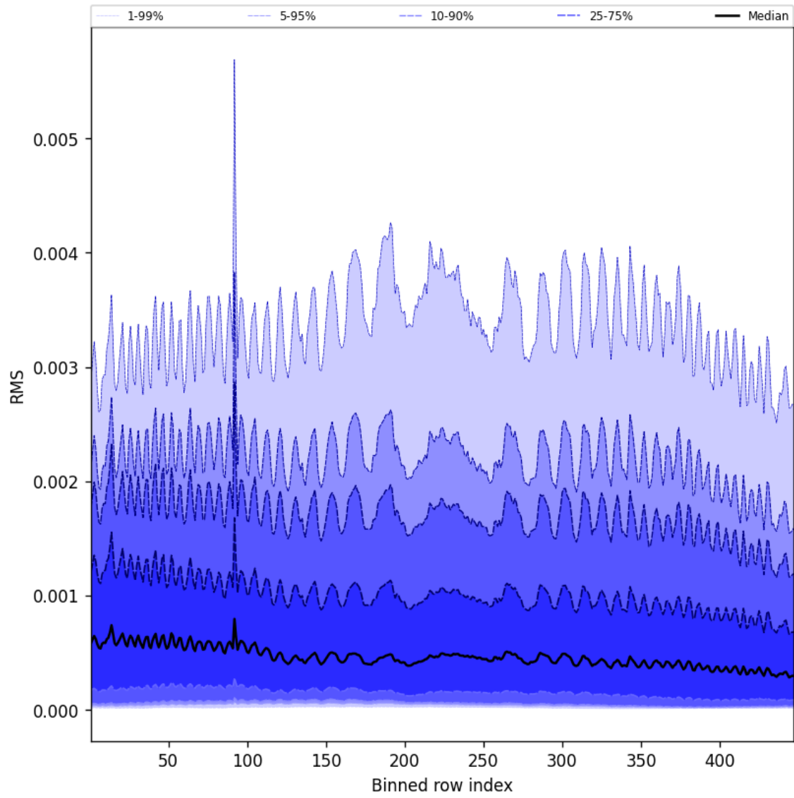
Figure 63: Along track statistics of “RMS” for 2025-02-06 to 2025-02-08
