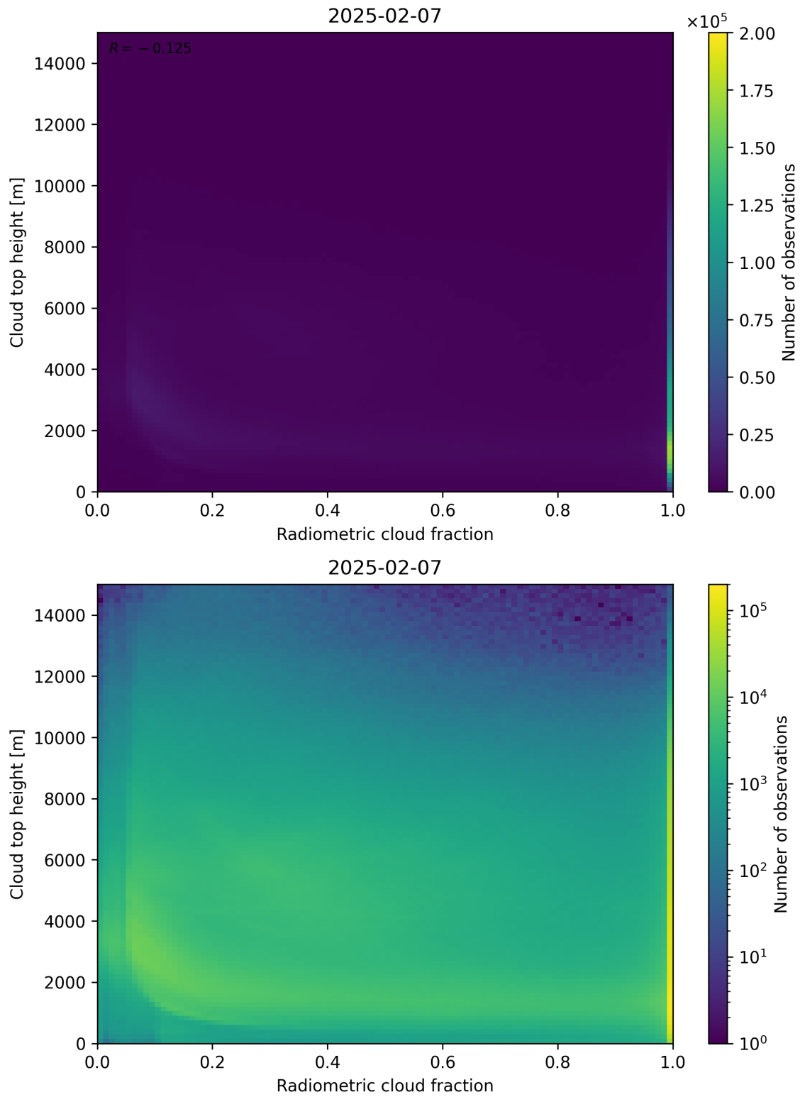
Figure 76: Scatter density plot of “Radiometric cloud fraction” against “Cloud top height” for 2025-02-06 to 2025-02-08.
