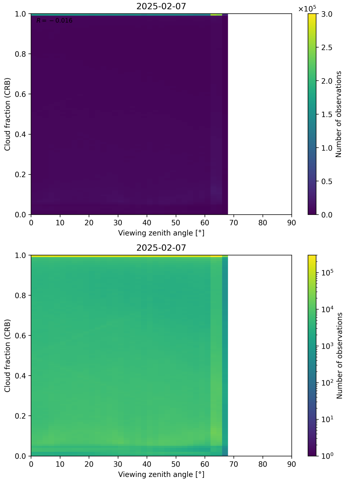
Figure 109: Scatter density plot of “Viewing zenith angle” against “Cloud fraction (CRB)” for 2025-02-06 to 2025-02-08.
