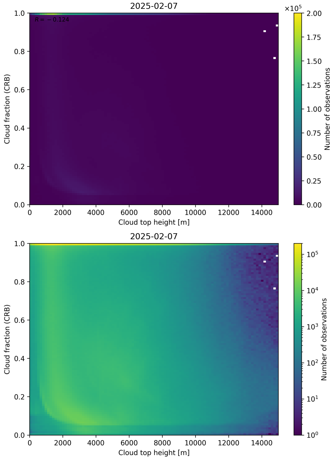
Figure 88: Scatter density plot of “Cloud top height” against “Cloud fraction (CRB)” for 2025-02-06 to 2025-02-08.
