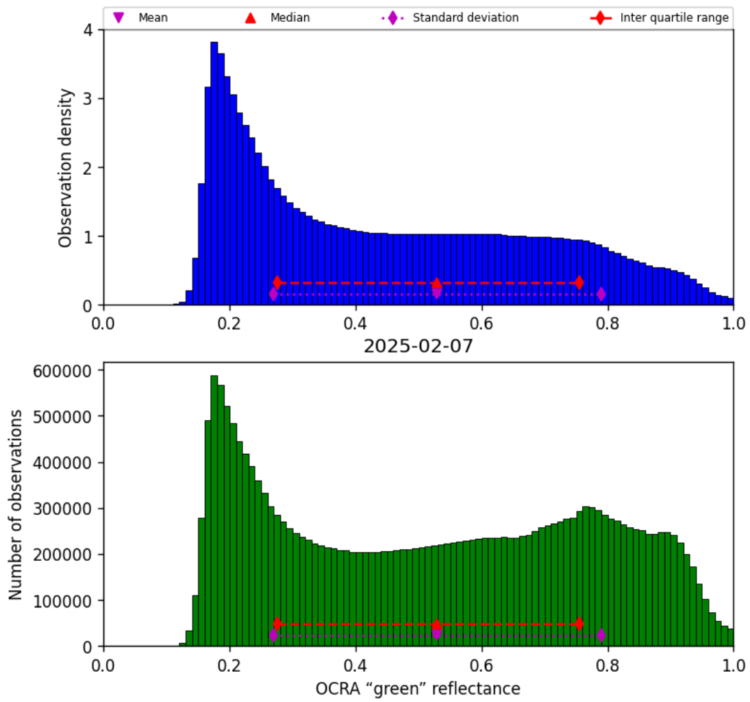
Figure 52: Histogram of “OCRA “green” reflectance” for 2025-02-06 to 2025-02-08
