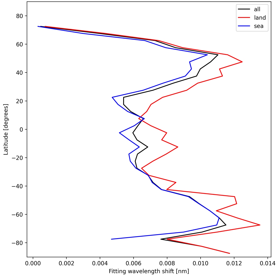
Figure 33: Zonal average of “Fitting wavelength shift” for 2025-02-06 to 2025-02-08.
