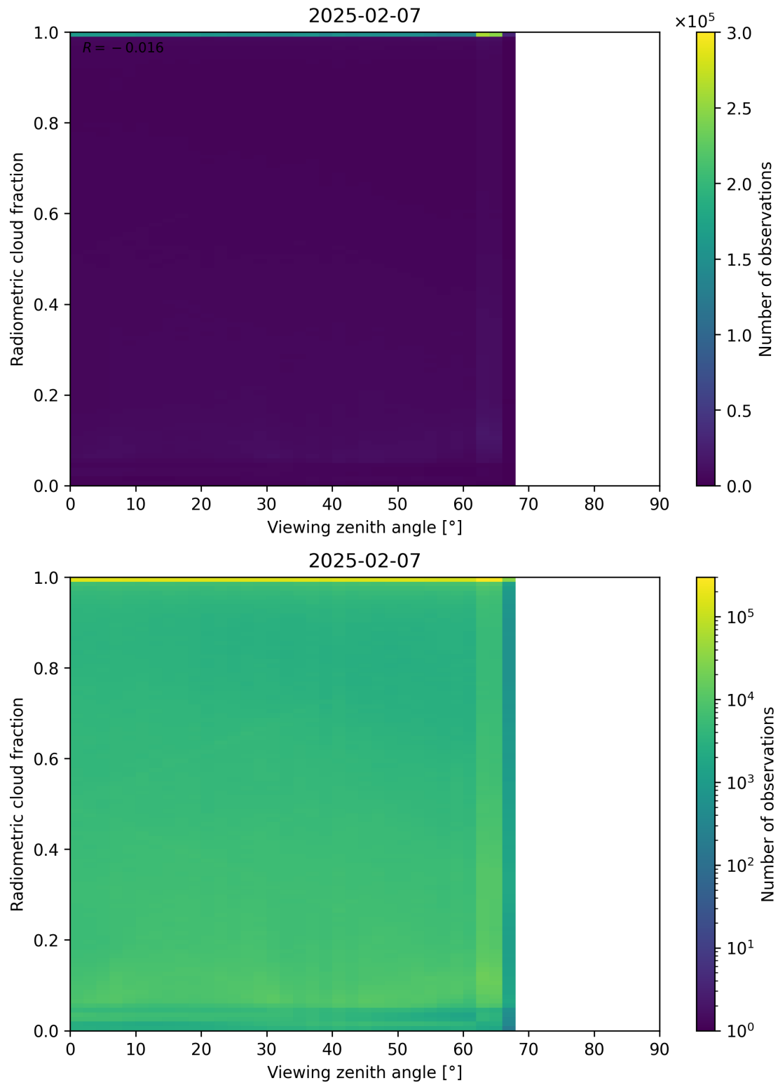
Figure 107: Scatter density plot of “Viewing zenith angle” against “Radiometric cloud fraction” for 2025-02-06 to 2025-02-08.
