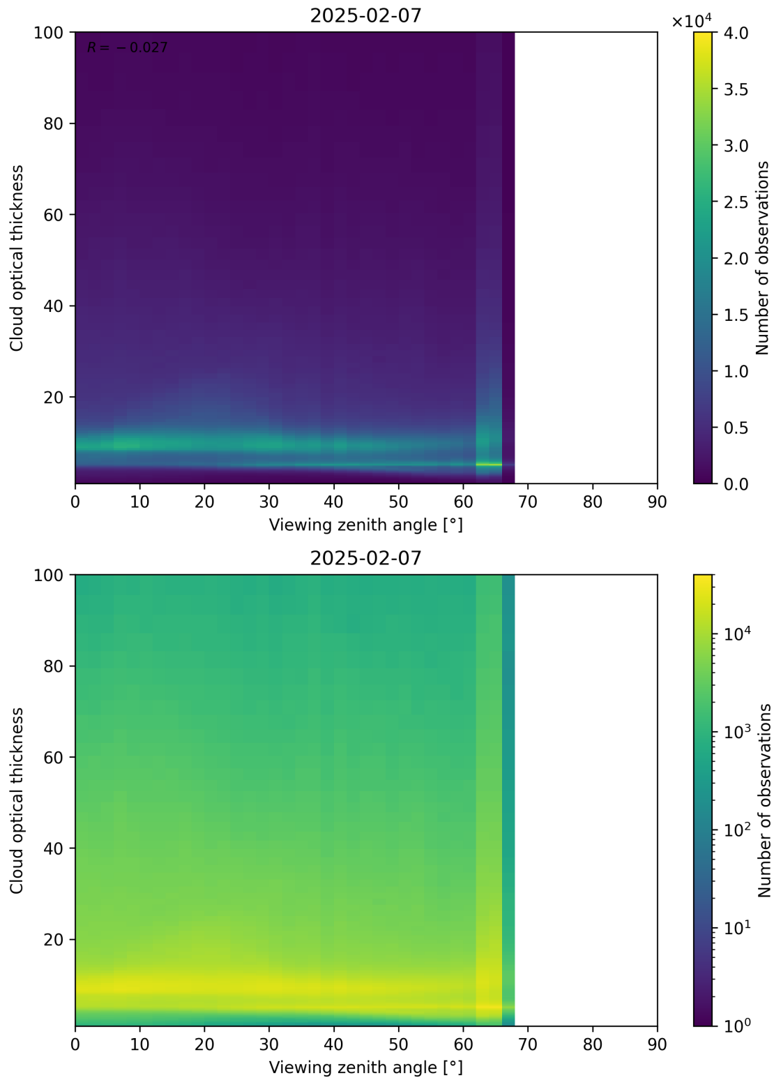
Figure 111: Scatter density plot of “Viewing zenith angle” against “Cloud optical thickness” for 2025-02-06 to 2025-02-08.
