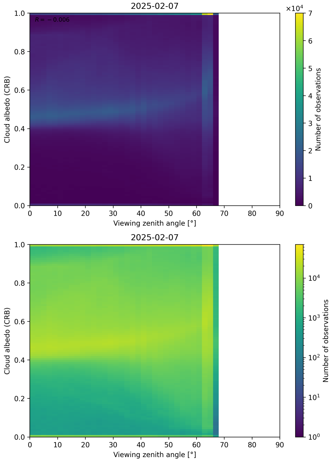
Figure 106: Scatter density plot of “Viewing zenith angle” against “Cloud albedo (CRB)” for 2025-02-06 to 2025-02-08.
