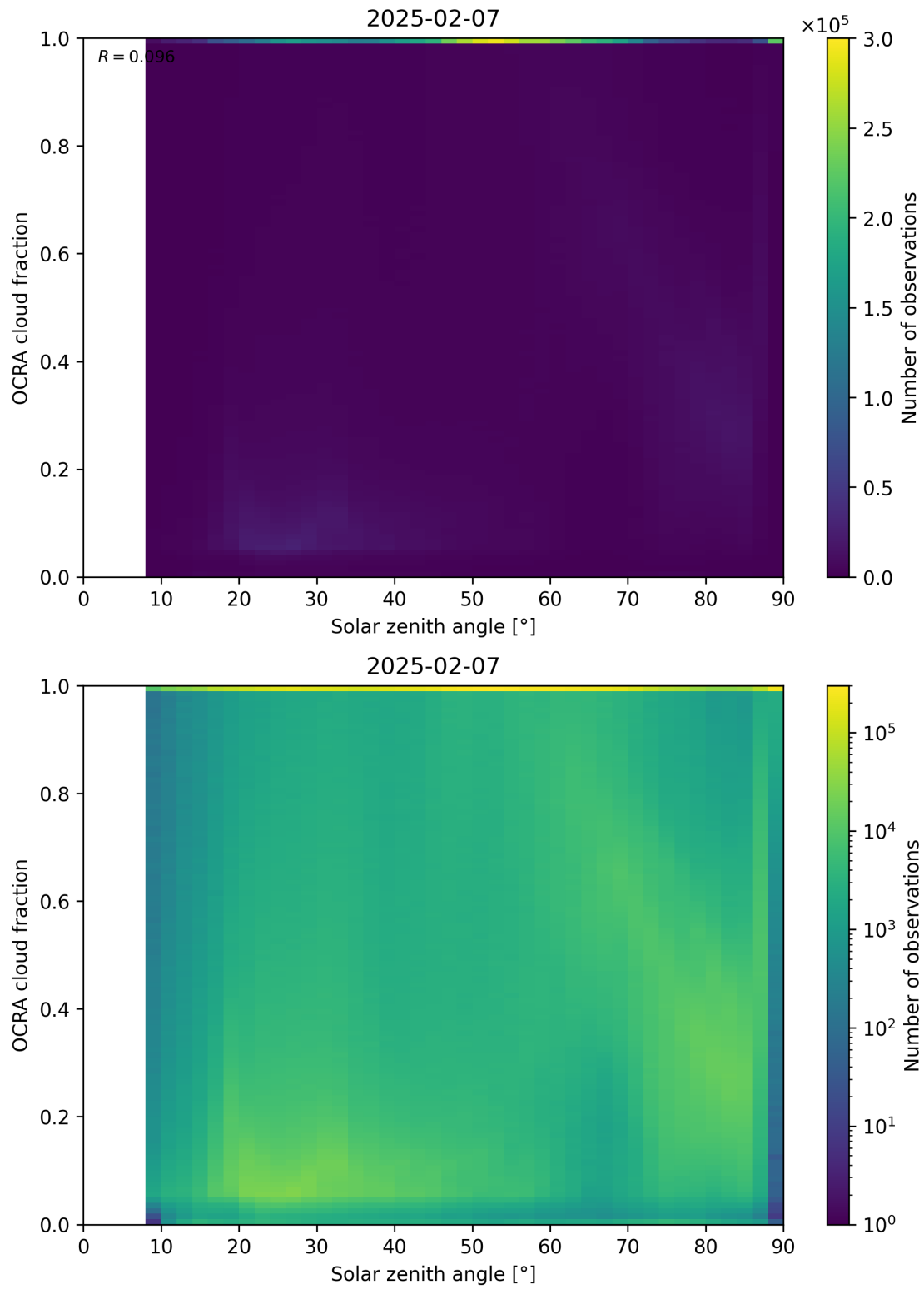
Figure 100: Scatter density plot of “Solar zenith angle” against “OCRA cloud fraction” for 2025-02-06 to 2025-02-08.
