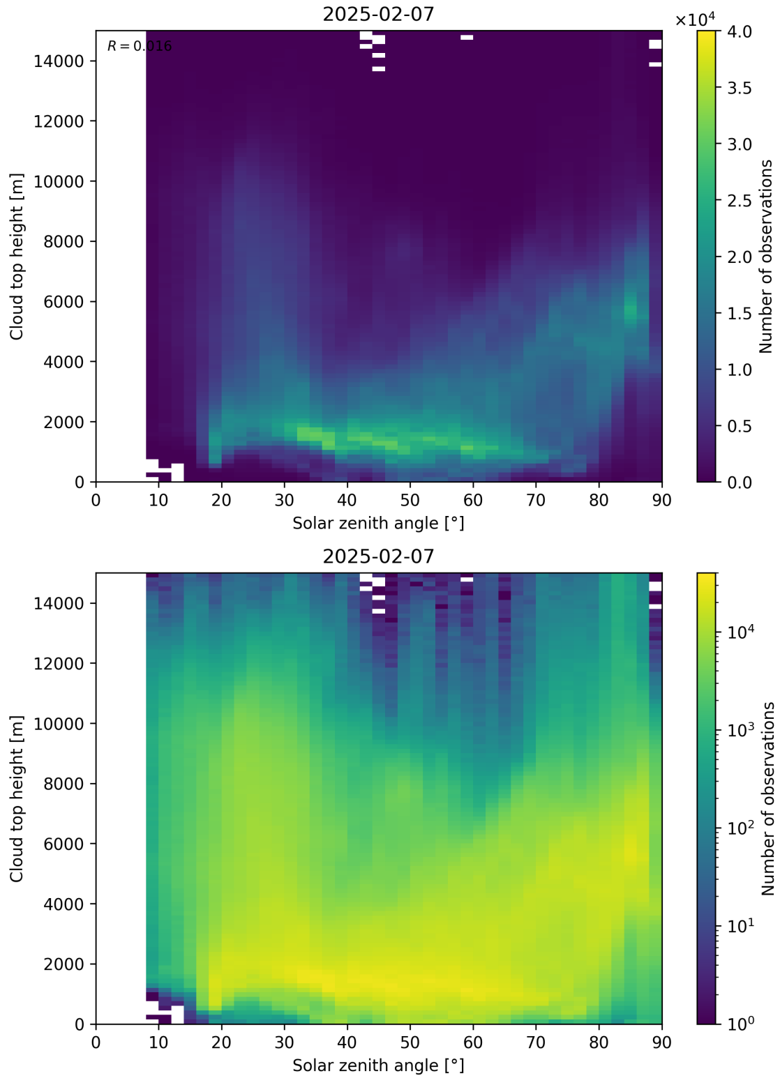
Figure 104: Scatter density plot of “Solar zenith angle” against “Cloud top height” for 2025-02-06 to 2025-02-08.
