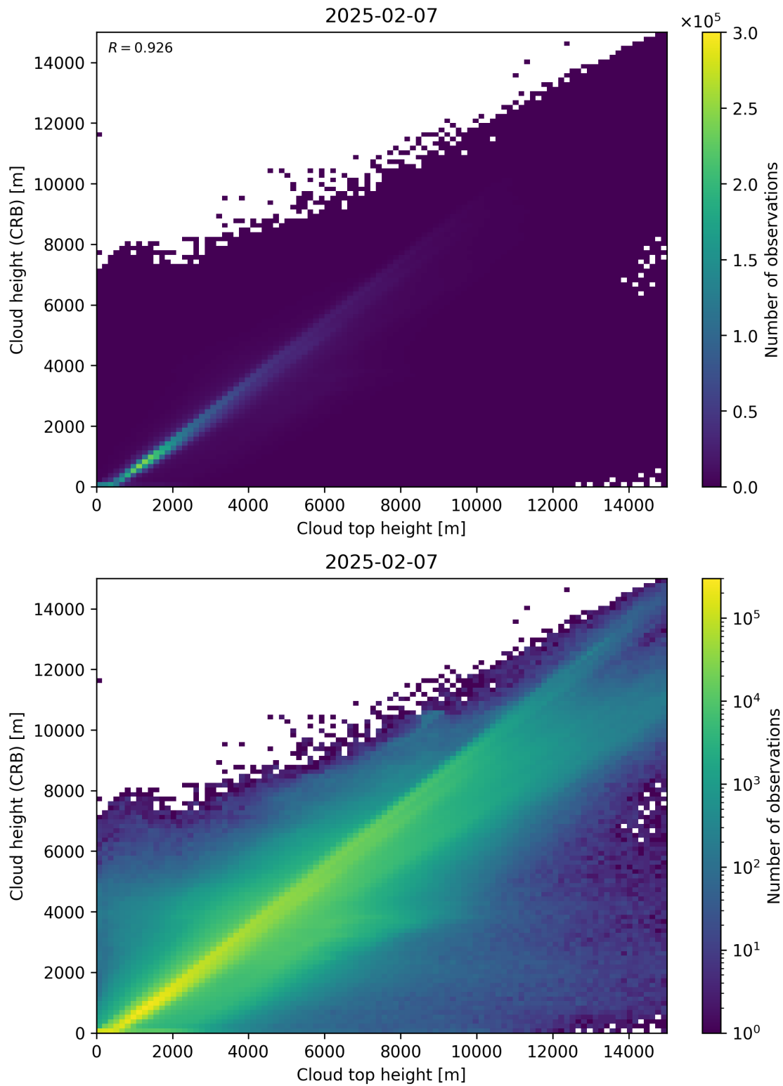
Figure 89: Scatter density plot of “Cloud top height” against “Cloud height (CRB)” for 2025-02-06 to 2025-02-08.
