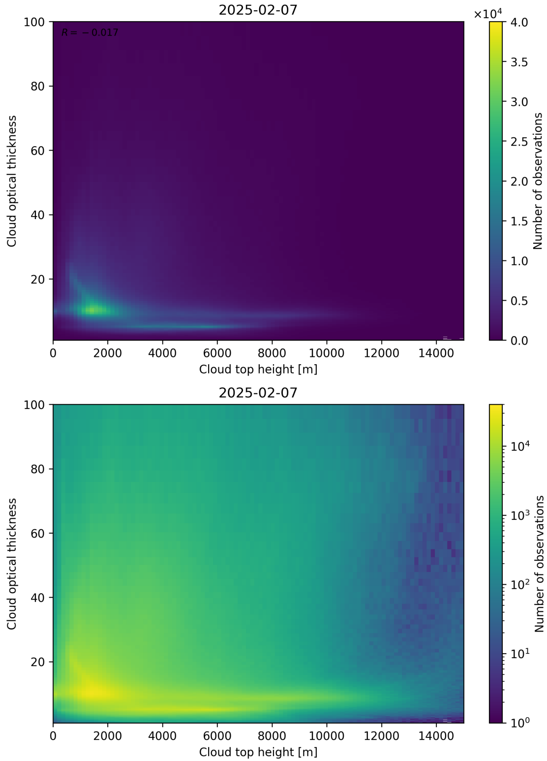
Figure 90: Scatter density plot of “Cloud top height” against “Cloud optical thickness” for 2025-02-06 to 2025-02-08.
