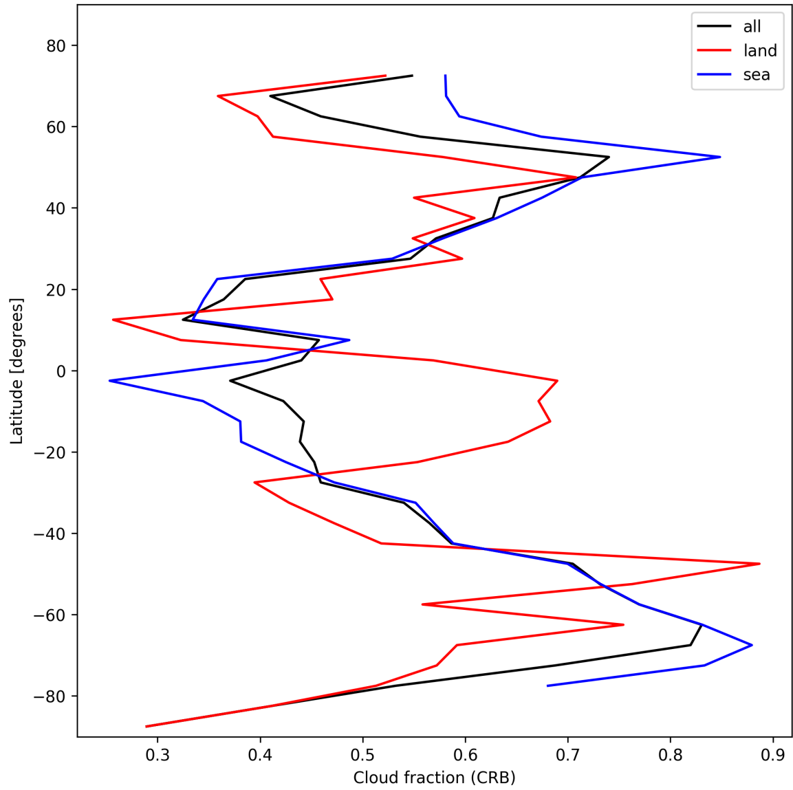
Figure 26: Zonal average of “Cloud fraction (CRB)” for 2025-02-06 to 2025-02-08.
