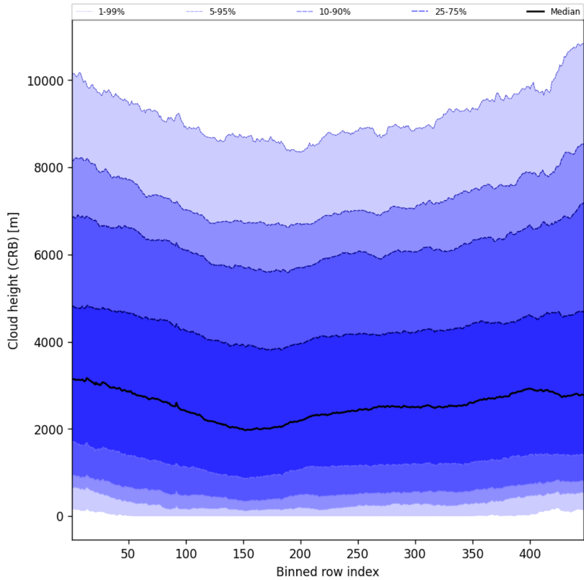
Figure 59: Along track statistics of “Cloud height (CRB)” for 2025-02-06 to 2025-02-08
