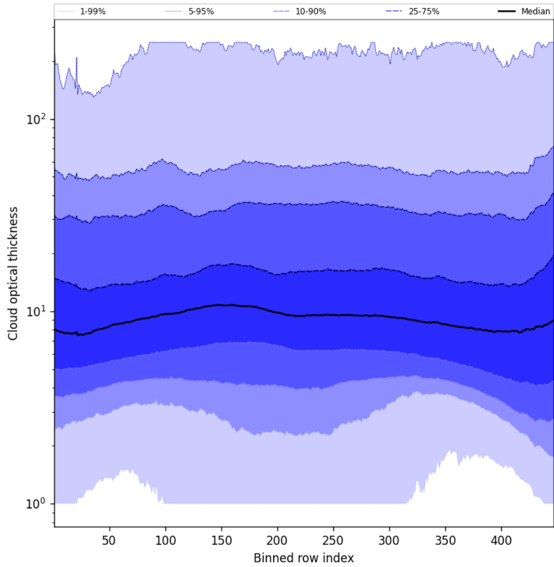
Figure 57: Along track statistics of “Cloud optical thickness” for 2025-02-06 to 2025-02-08
