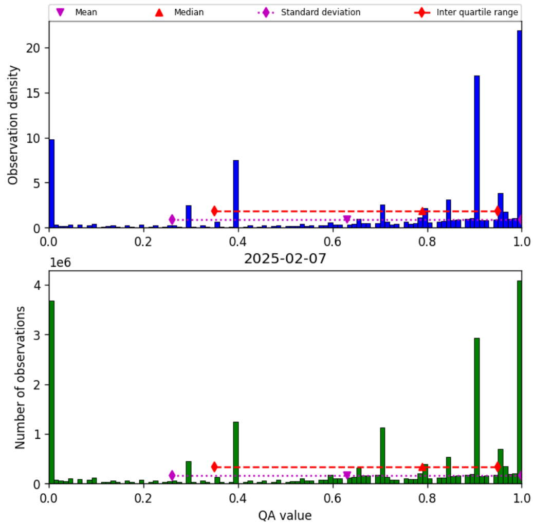
Figure 38: Histogram of “QA value” for 2025-02-06 to 2025-02-08
