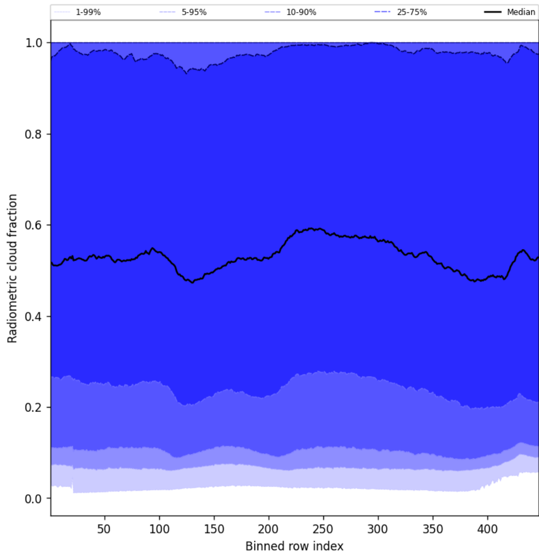
Figure 55: Along track statistics of “Radiometric cloud fraction” for 2025-02-06 to 2025-02-08
