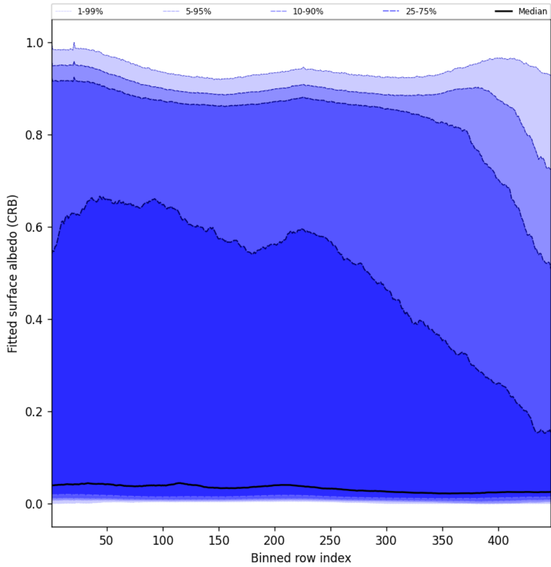
Figure 62: Along track statistics of “Fitted surface albedo (CRB)” for 2025-02-06 to 2025-02-08
