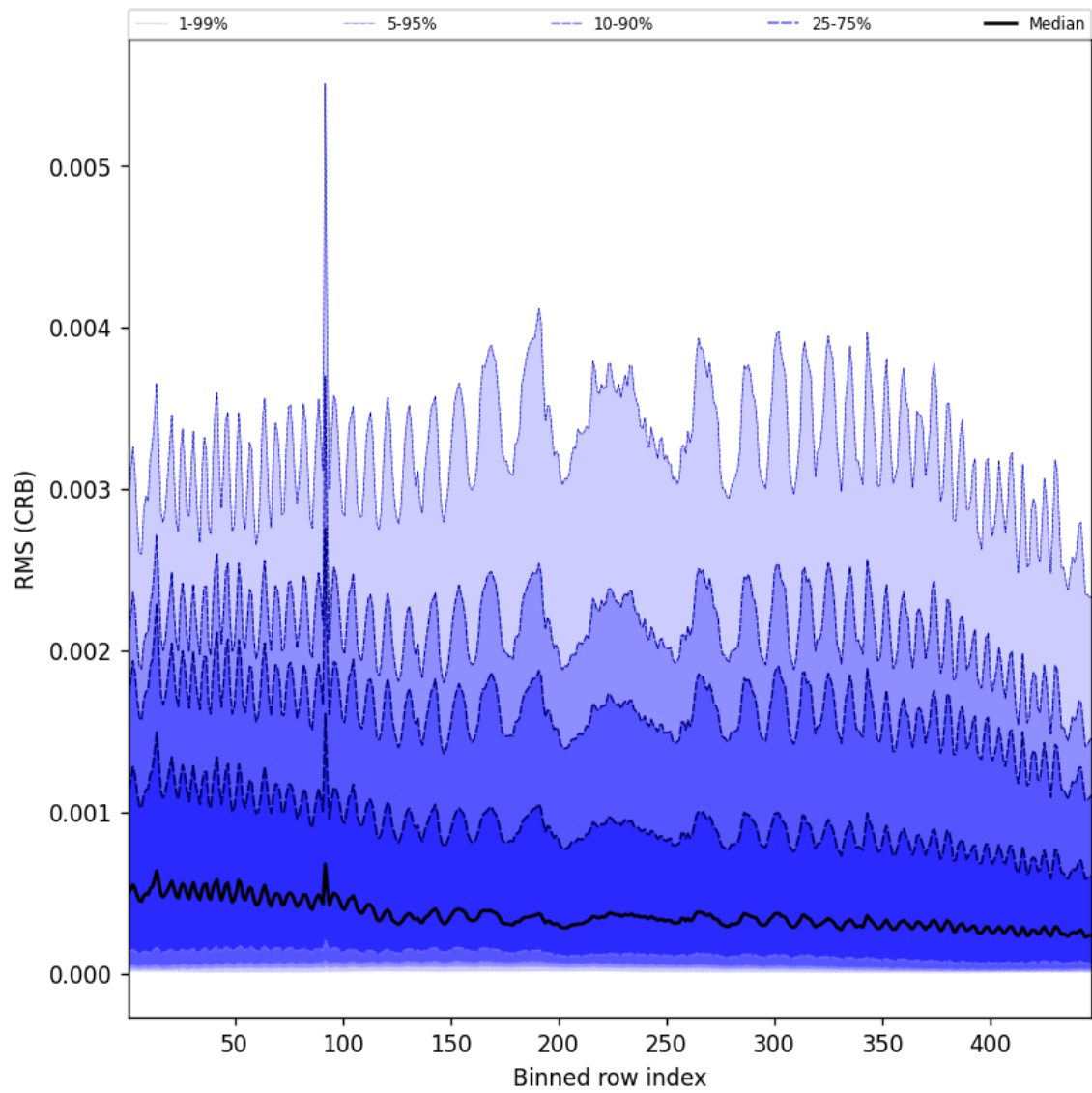
Figure 64: Along track statistics of “RMS (CRB)” for 2025-02-06 to 2025-02-08
