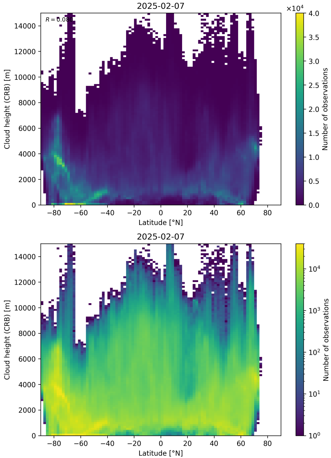
Figure 95: Scatter density plot of “Latitude” against “Cloud height (CRB)” for 2025-02-06 to 2025-02-08.
