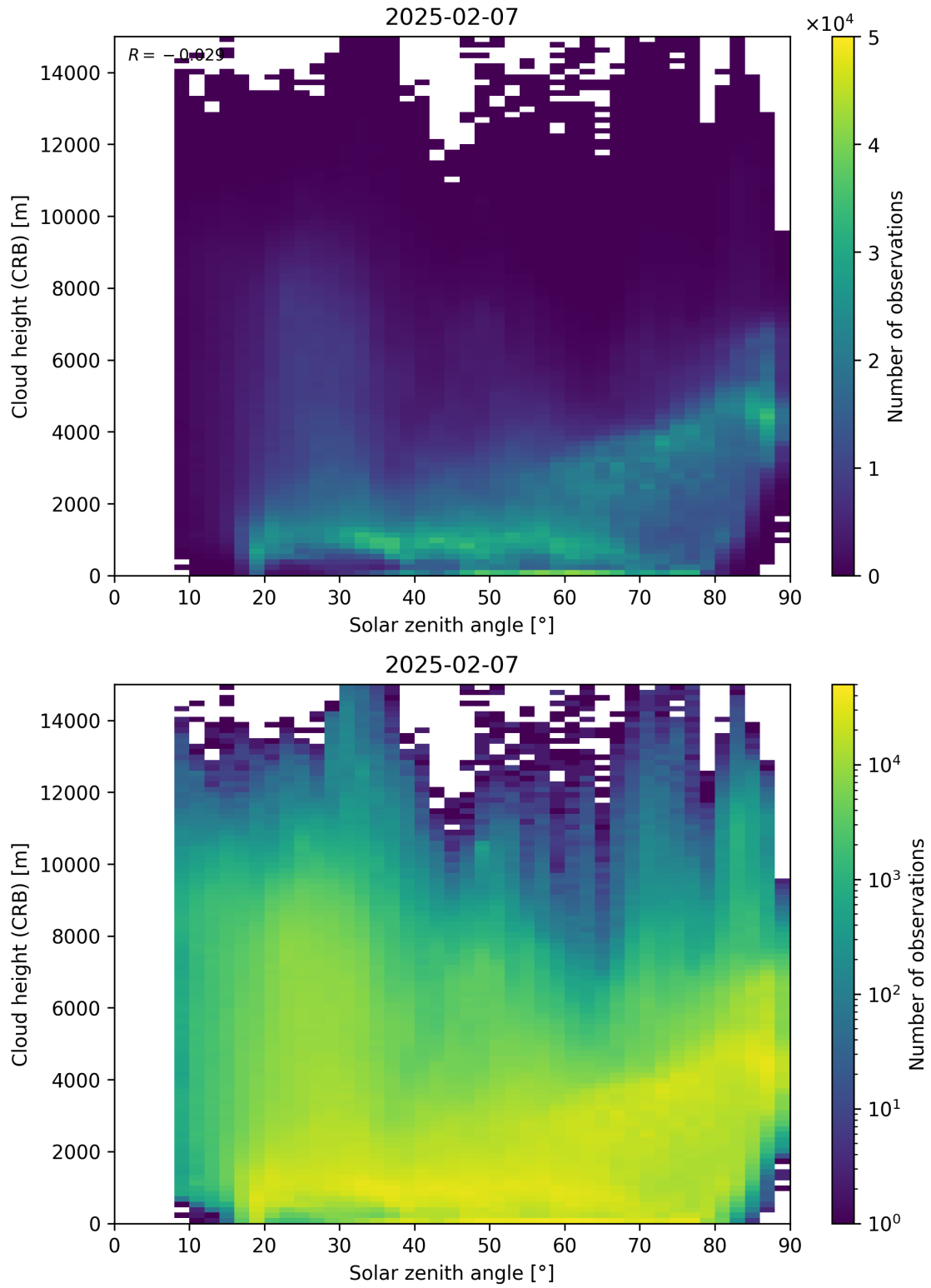
Figure 102: Scatter density plot of “Solar zenith angle” against “Cloud height (CRB)” for 2025-02-06 to 2025-02-08.
