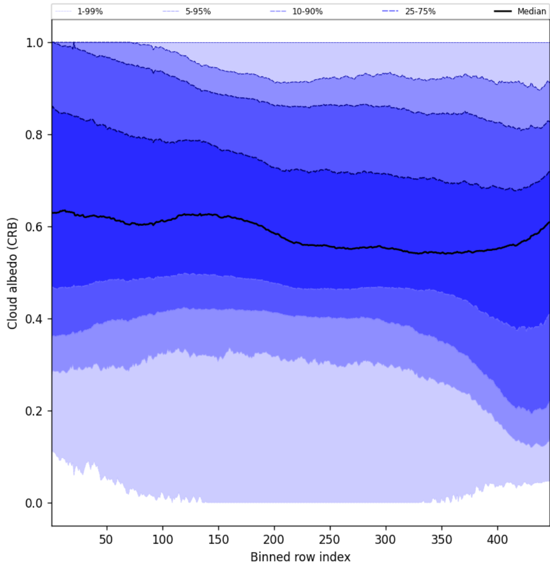
Figure 60: Along track statistics of “Cloud albedo (CRB)” for 2025-02-06 to 2025-02-08
