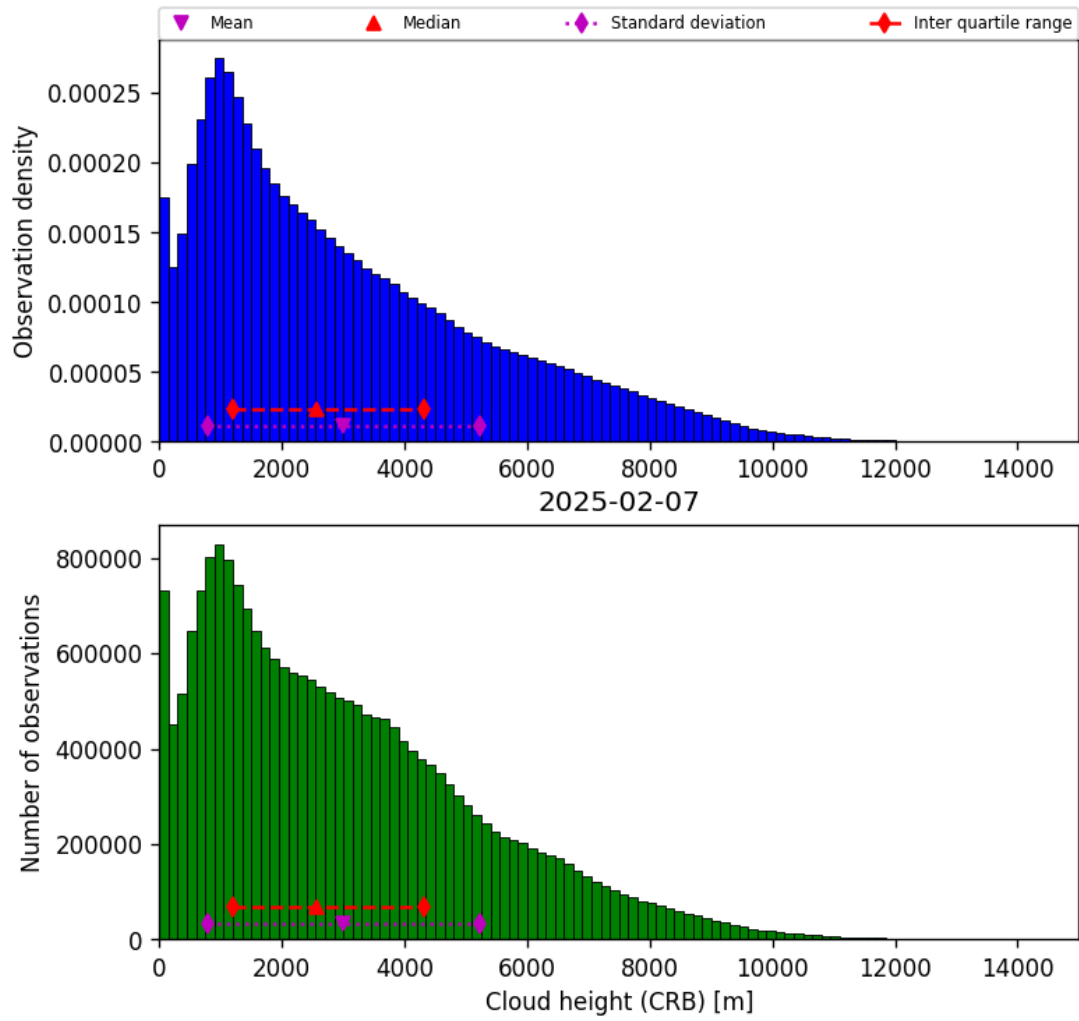
Figure 43: Histogram of “Cloud height (CRB)” for 2025-02-06 to 2025-02-08
