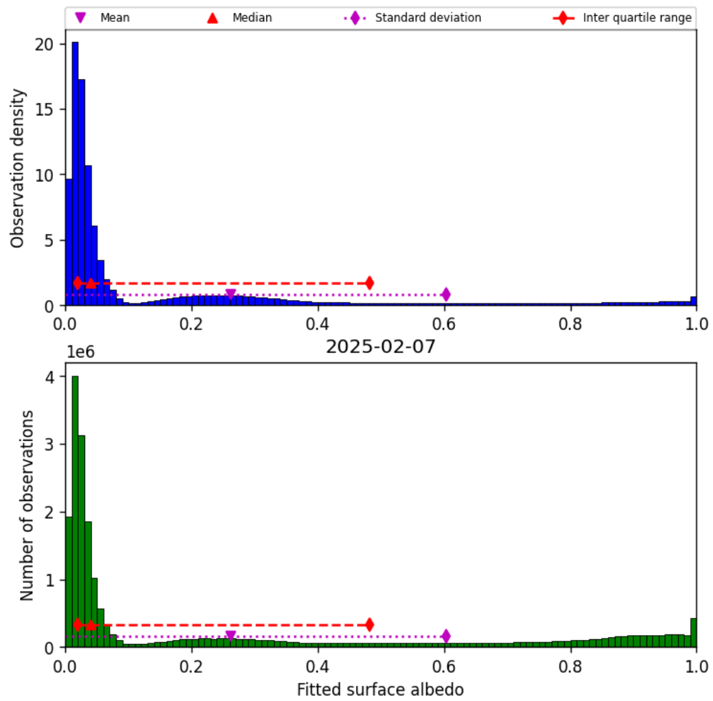
Figure 45: Histogram of “Fitted surface albedo” for 2025-02-06 to 2025-02-08
