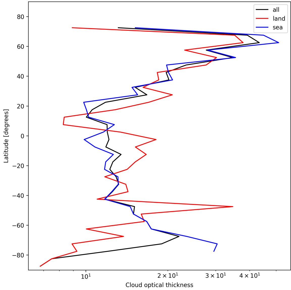
Figure 25: Zonal average of “Cloud optical thickness” for 2025-02-06 to 2025-02-08.
