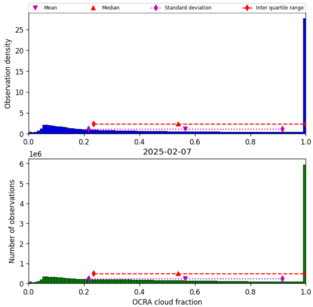
Figure 50: Histogram of “OCRA cloud fraction” for 2025-02-06 to 2025-02-08
