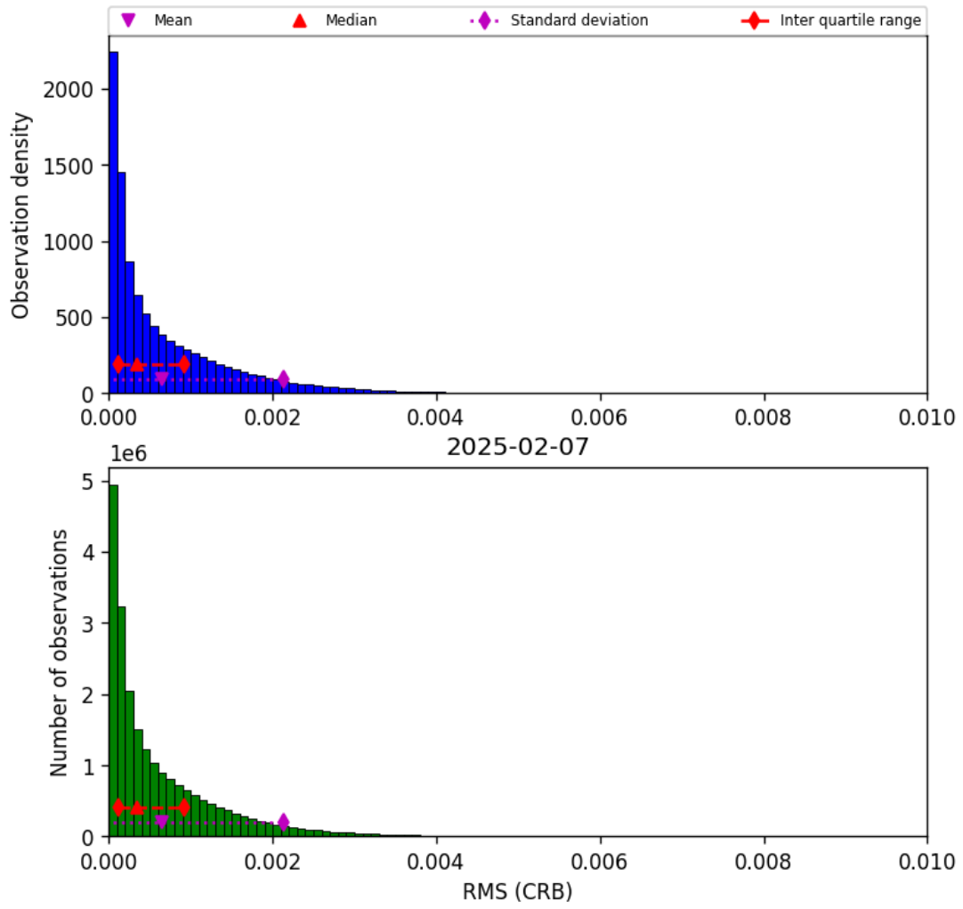
Figure 48: Histogram of “RMS (CRB)” for 2025-02-06 to 2025-02-08
