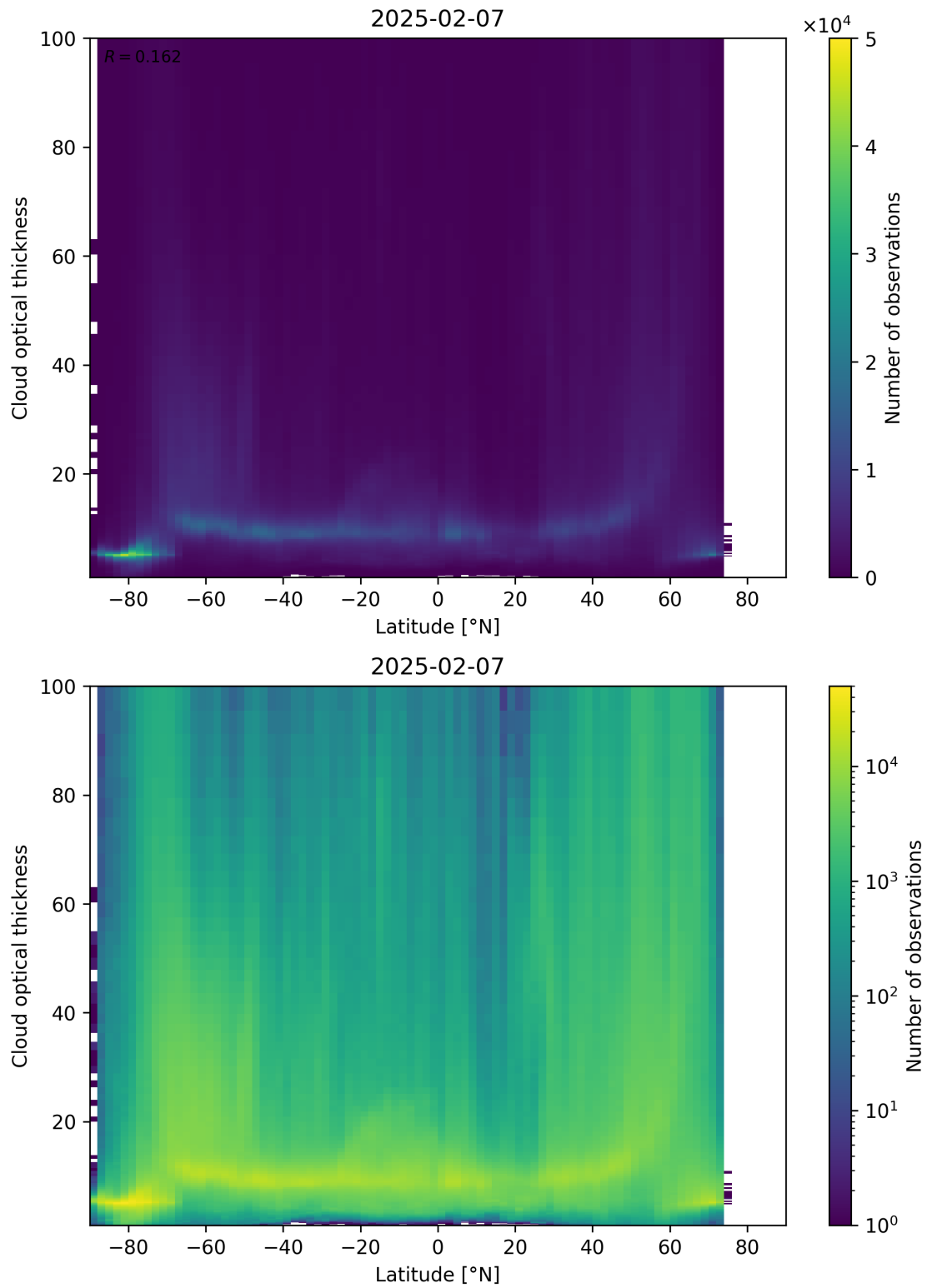
Figure 96: Scatter density plot of “Latitude” against “Cloud optical thickness” for 2025-02-06 to 2025-02-08.
