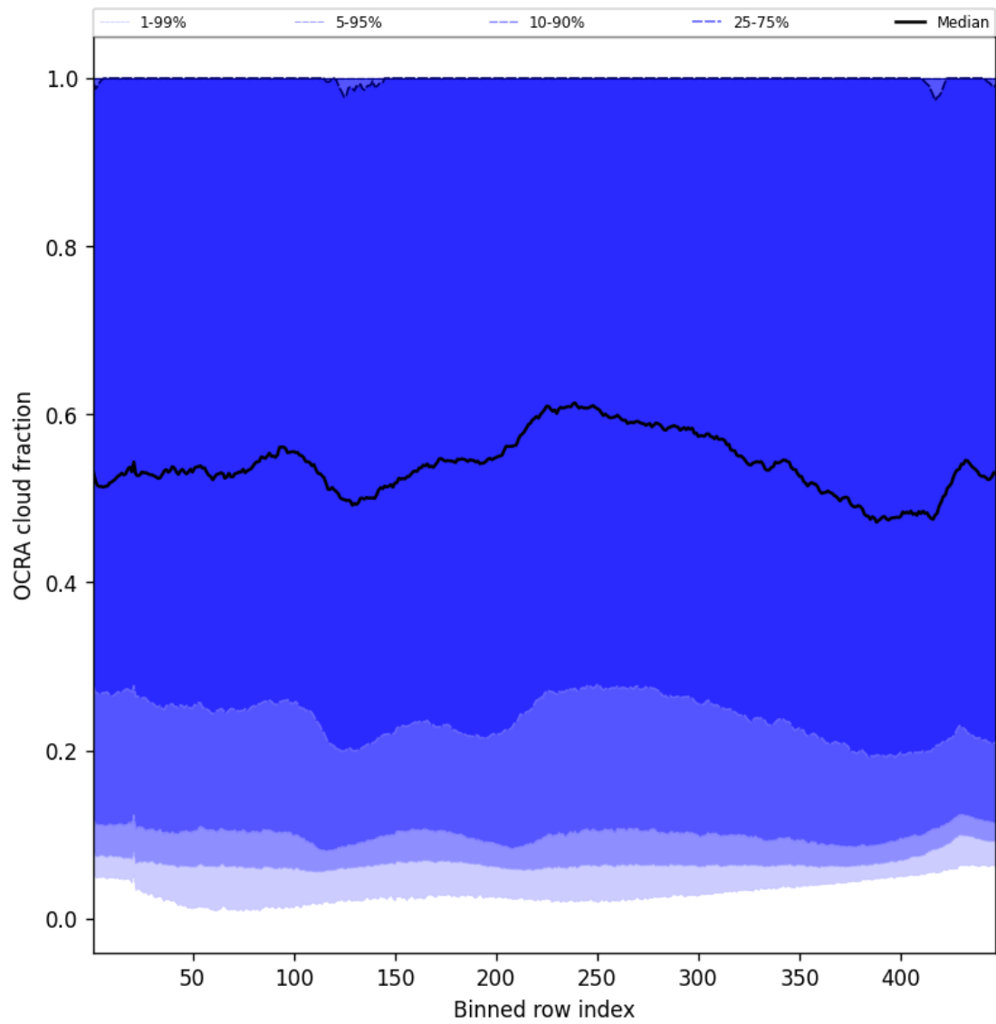
Figure 66: Along track statistics of “OCRA cloud fraction” for 2025-02-06 to 2025-02-08
