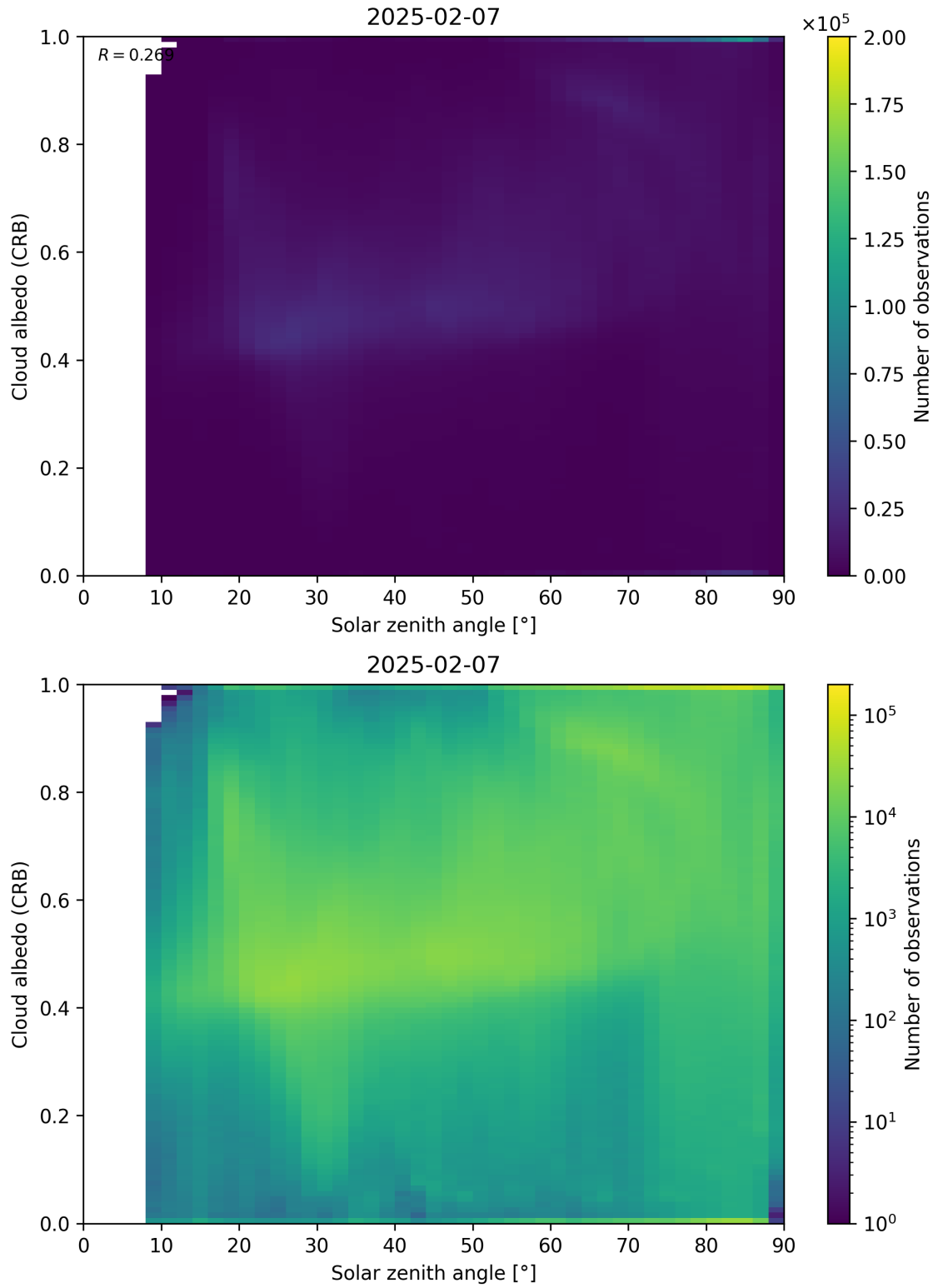
Figure 98: Scatter density plot of “Solar zenith angle” against “Cloud albedo (CRB)” for 2025-02-06 to 2025-02-08.
