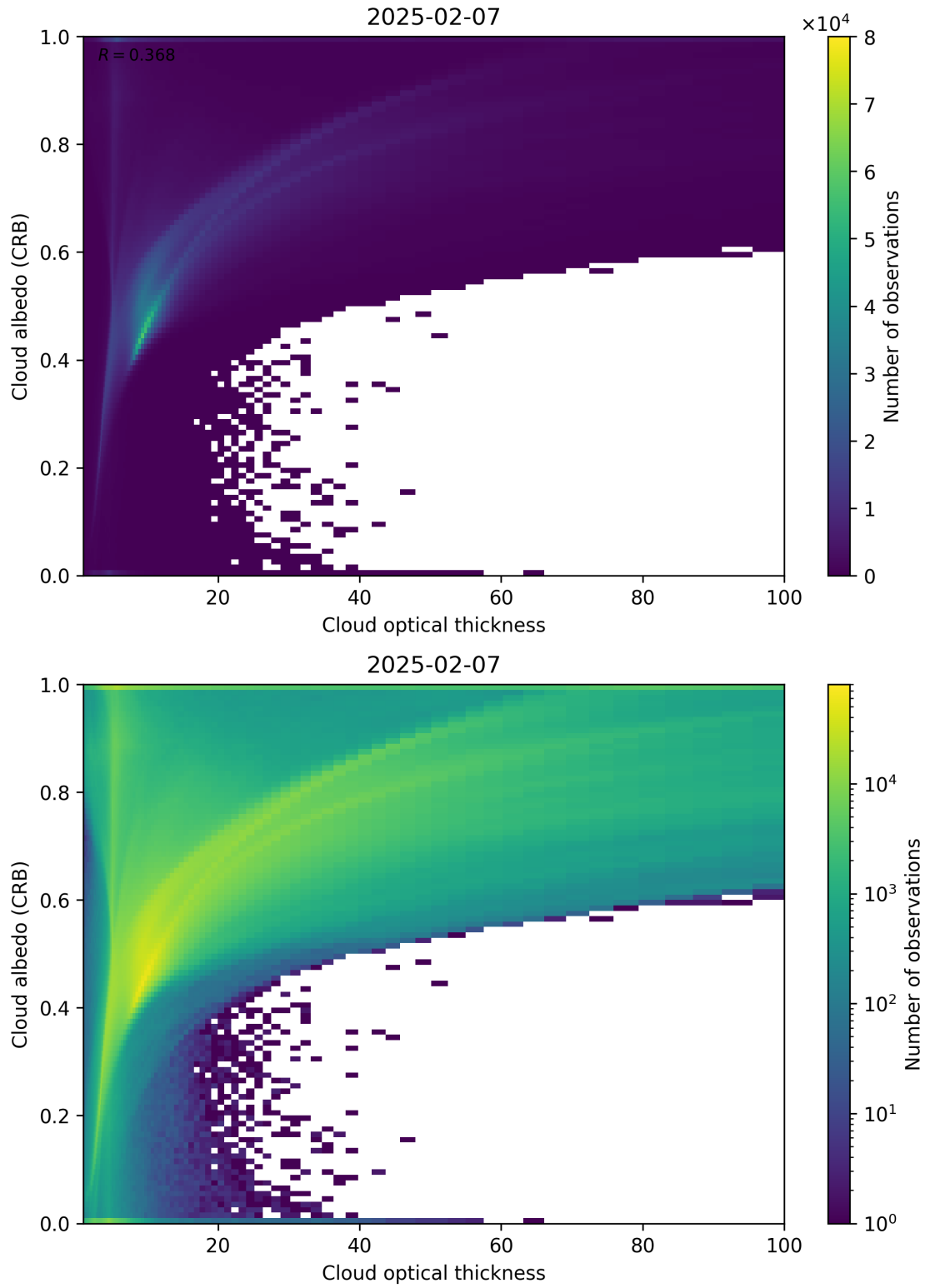
Figure 82: Scatter density plot of “Cloud optical thickness” against “Cloud albedo (CRB)” for 2025-02-06 to 2025-02-08.
