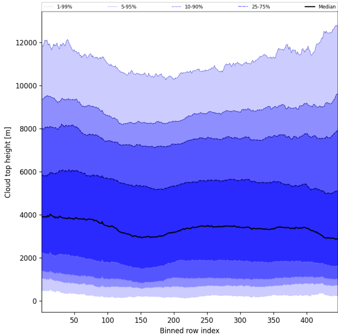
Figure 56: Along track statistics of “Cloud top height” for 2025-02-06 to 2025-02-08
