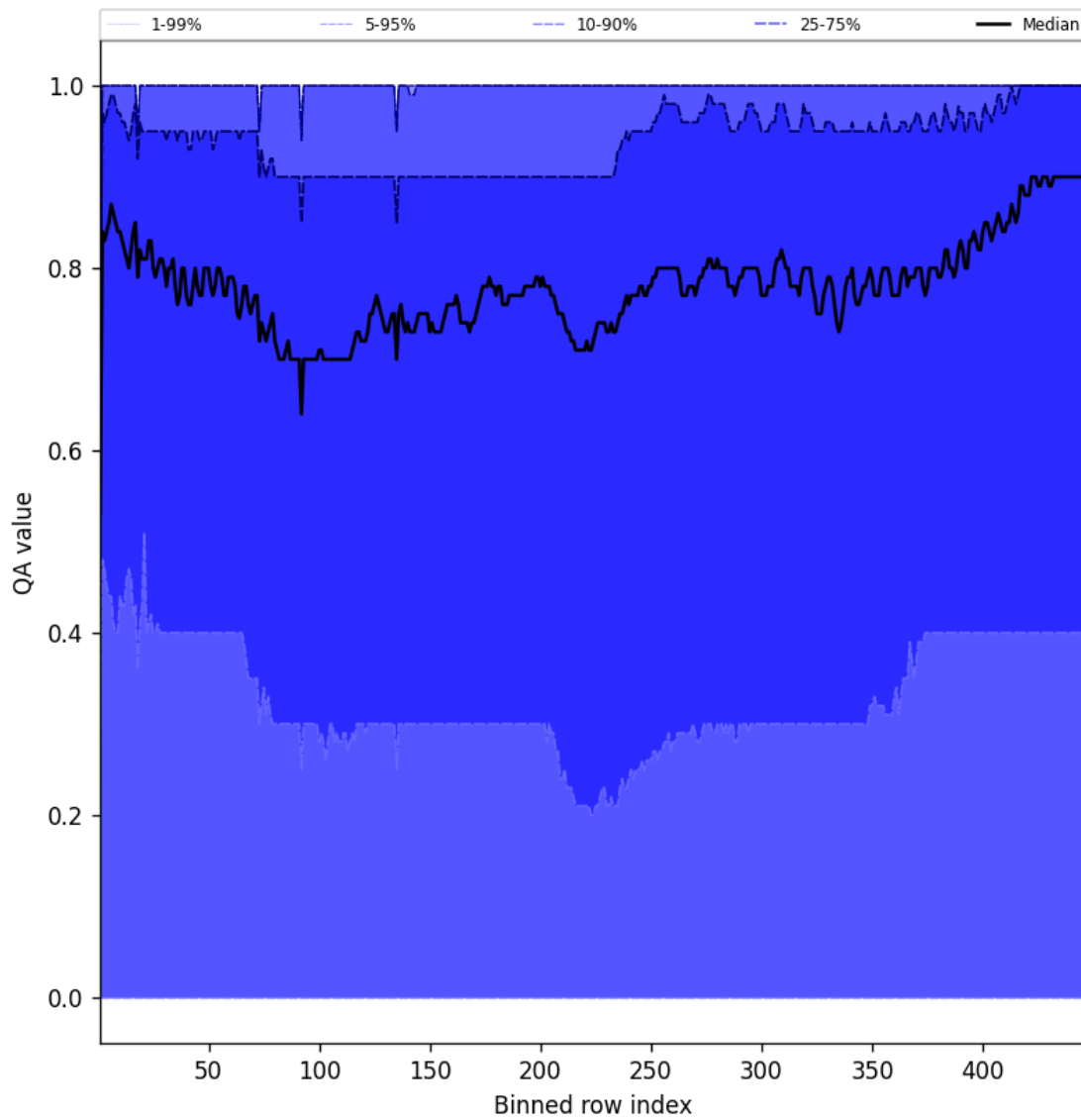
Figure 54: Along track statistics of “QA value” for 2025-02-06 to 2025-02-08
