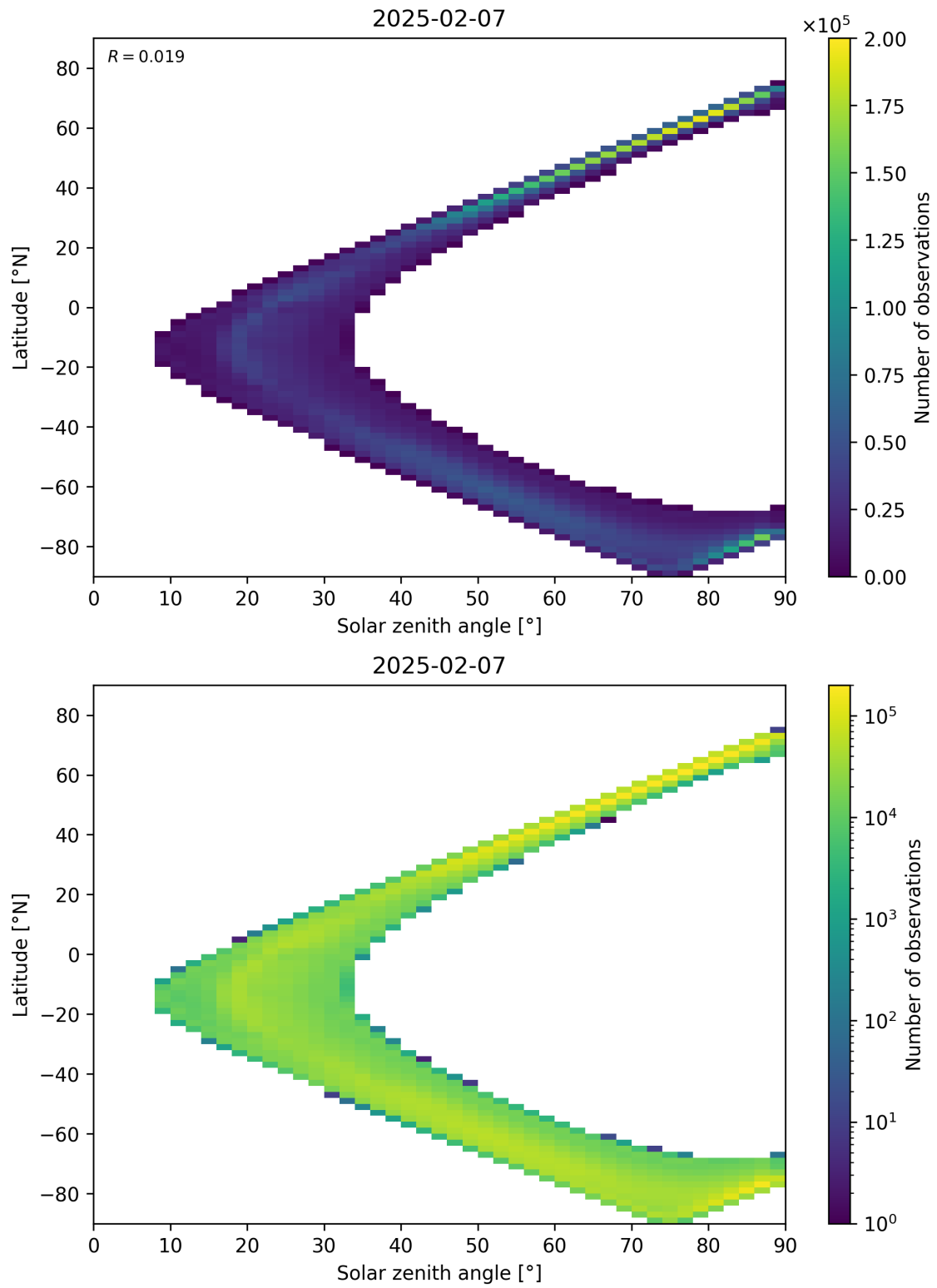
Figure 105: Scatter density plot of “Solar zenith angle” against “Latitude” for 2025-02-06 to 2025-02-08.
