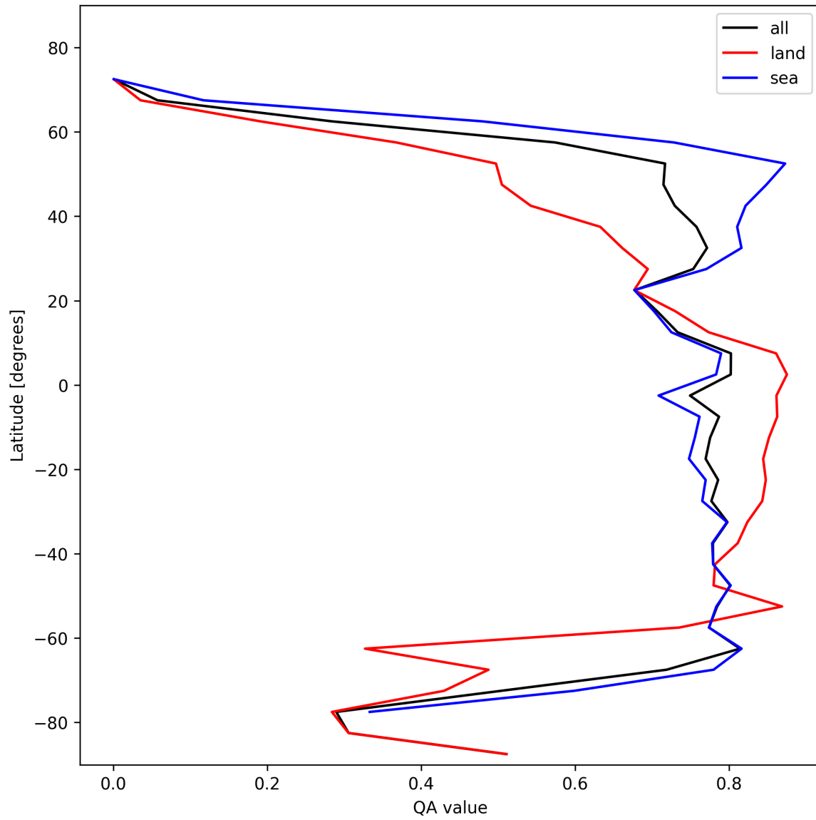
Figure 22: Zonal average of “QA value” for 2025-02-06 to 2025-02-08.
