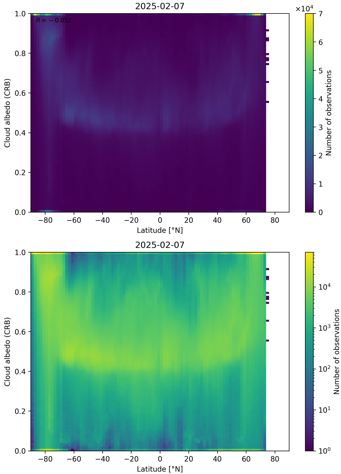
Figure 91: Scatter density plot of “Latitude” against “Cloud albedo (CRB)” for 2025-02-06 to 2025-02-08.
