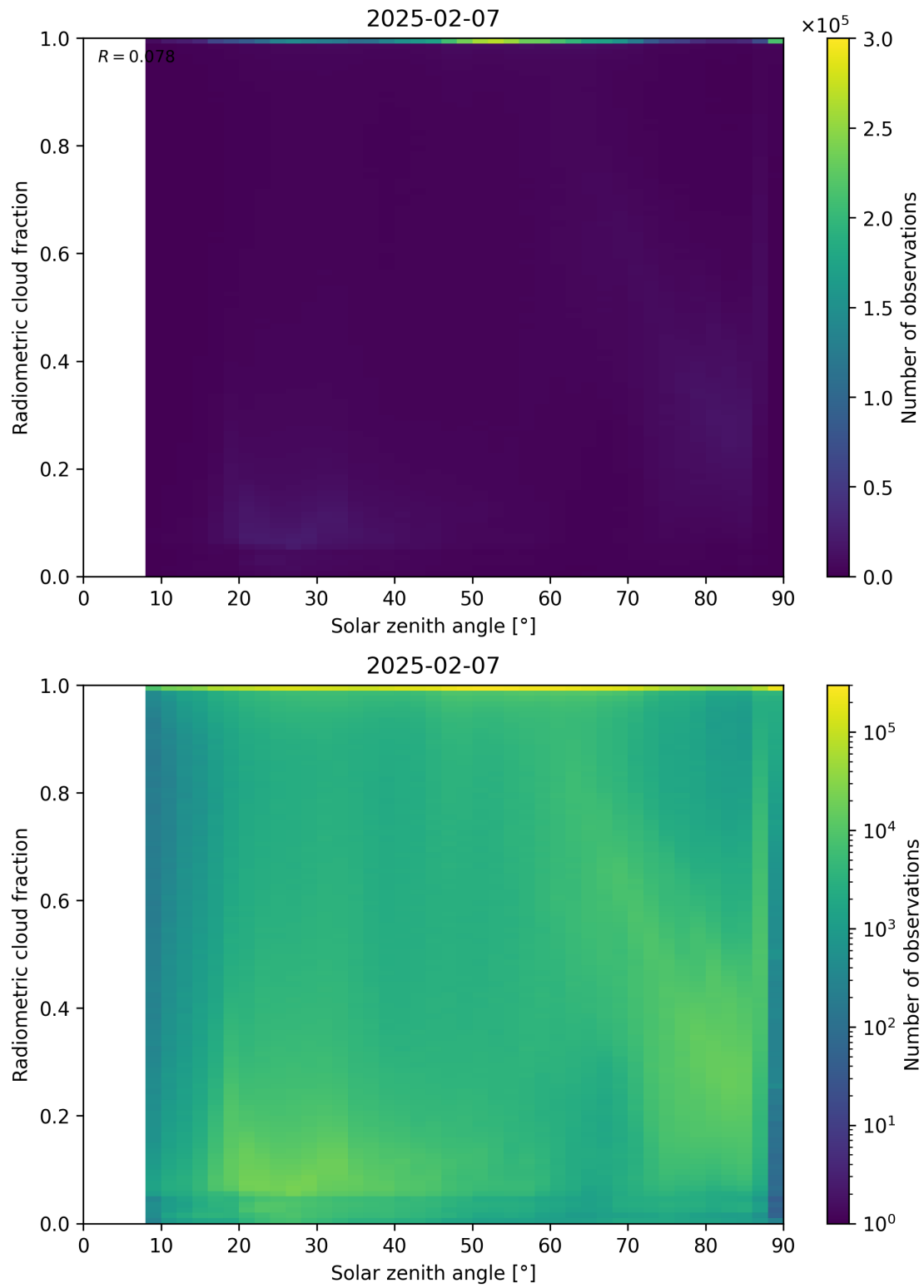
Figure 99: Scatter density plot of “Solar zenith angle” against “Radiometric cloud fraction” for 2025-02-06 to 2025-02-08.
