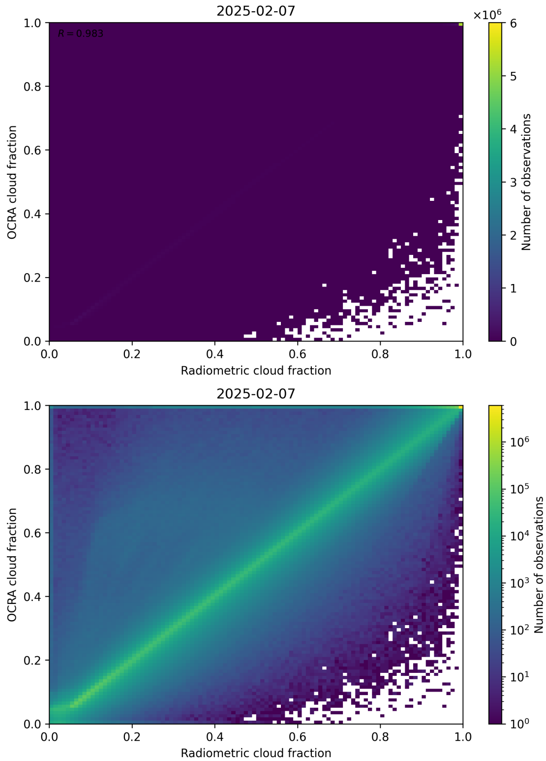
Figure 72: Scatter density plot of “Radiometric cloud fraction” against “OCRA cloud fraction” for 2025-02-06 to 2025-02-08.
