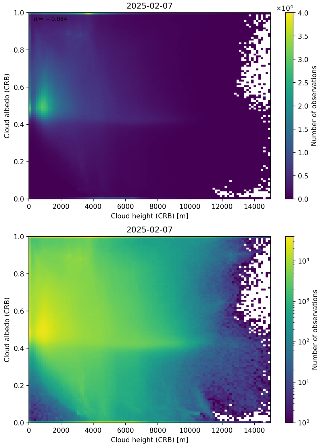
Figure 80: Scatter density plot of “Cloud height (CRB)” against “Cloud albedo (CRB)” for 2025-02-06 to 2025-02-08.
