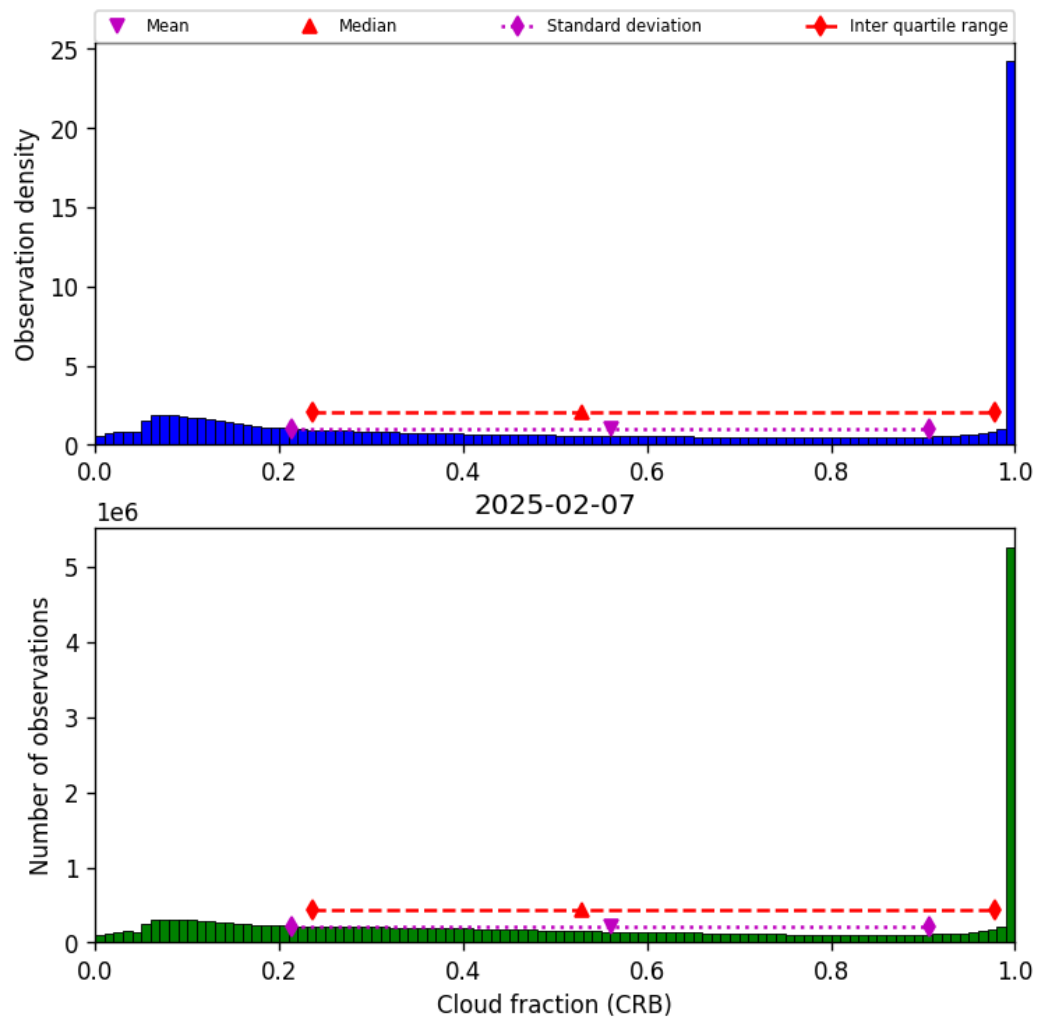
Figure 42: Histogram of “Cloud fraction (CRB)” for 2025-02-06 to 2025-02-08
