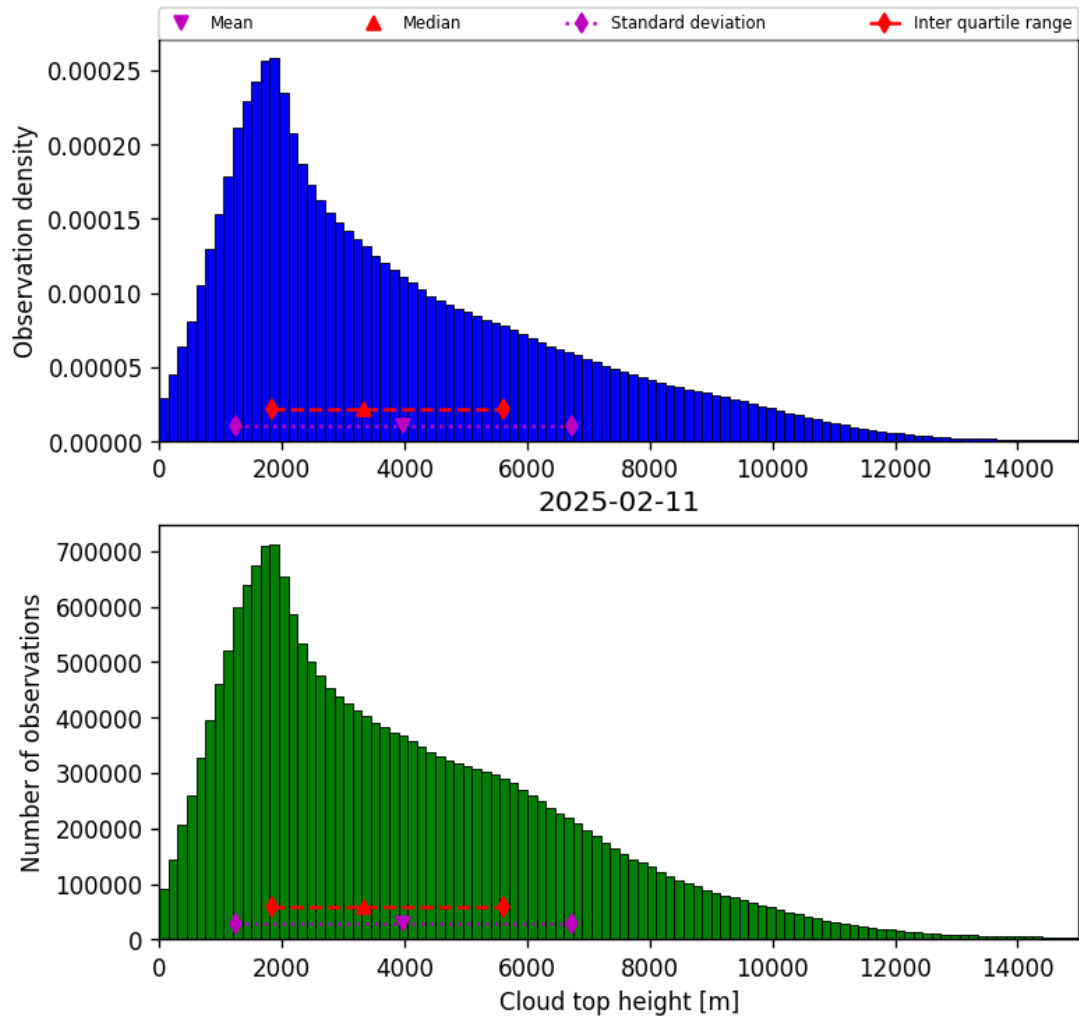
Figure 40: Histogram of “Cloud top height” for 2025-02-10 to 2025-02-12
