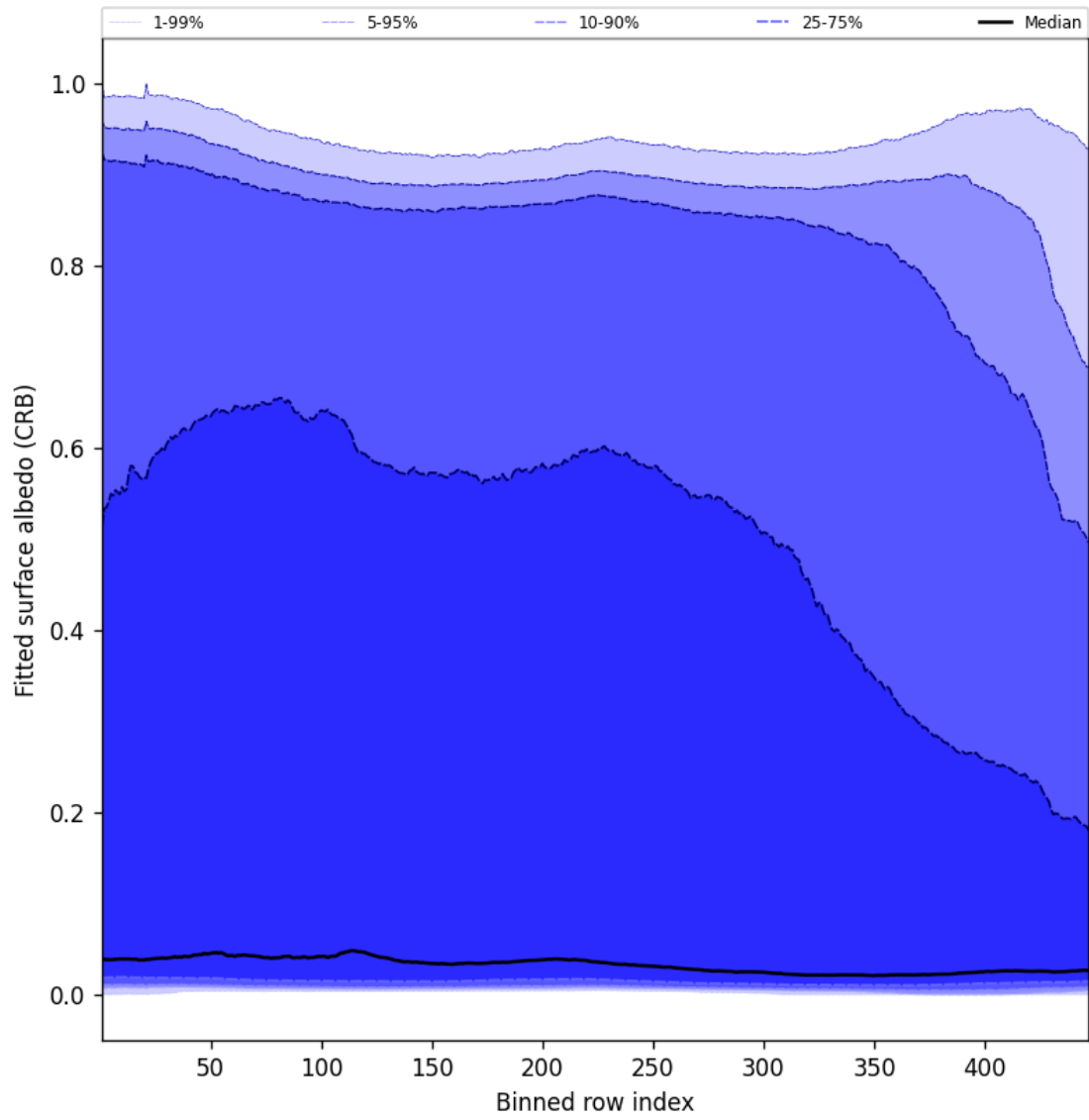
Figure 62: Along track statistics of “Fitted surface albedo (CRB)” for 2025-02-10 to 2025-02-12
