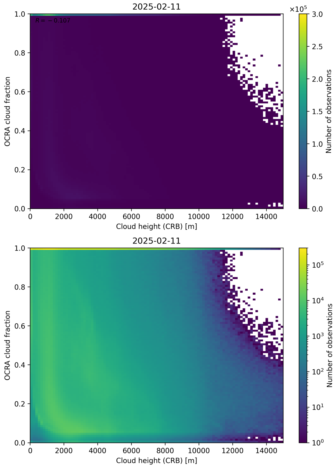
Figure 81: Scatter density plot of “Cloud height (CRB)” against “OCRA cloud fraction” for 2025-02-10 to 2025-02-12.
