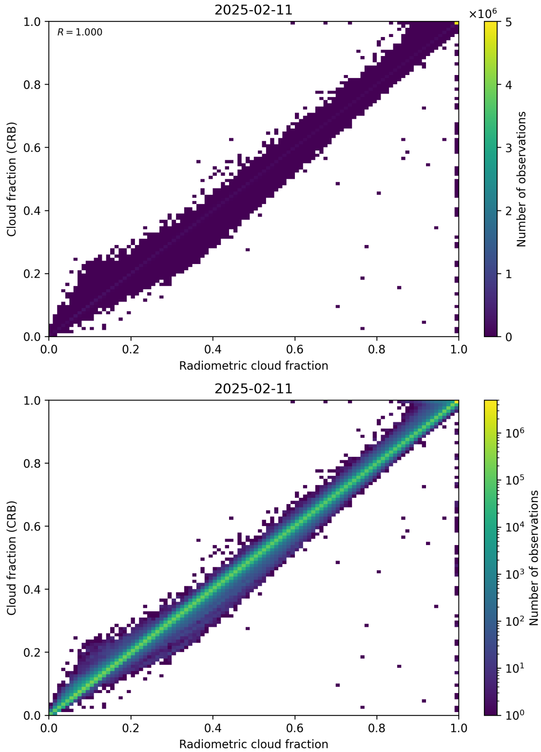
Figure 73: Scatter density plot of “Radiometric cloud fraction” against “Cloud fraction (CRB)” for 2025-02-10 to 2025-02-12.
