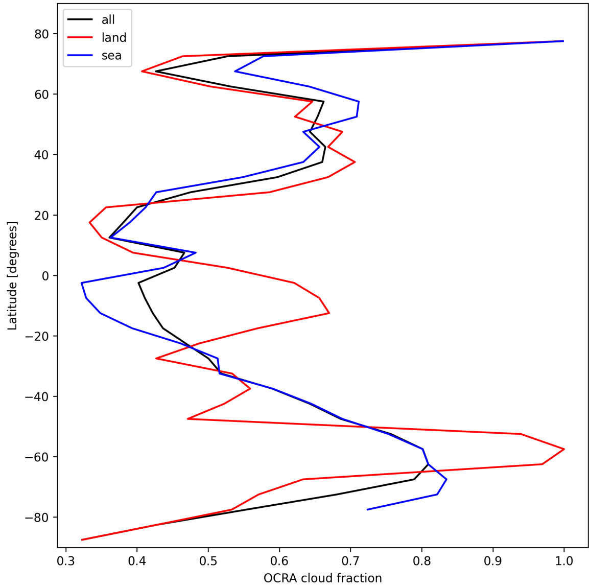
Figure 34: Zonal average of “OCRA cloud fraction” for 2025-02-10 to 2025-02-12.
