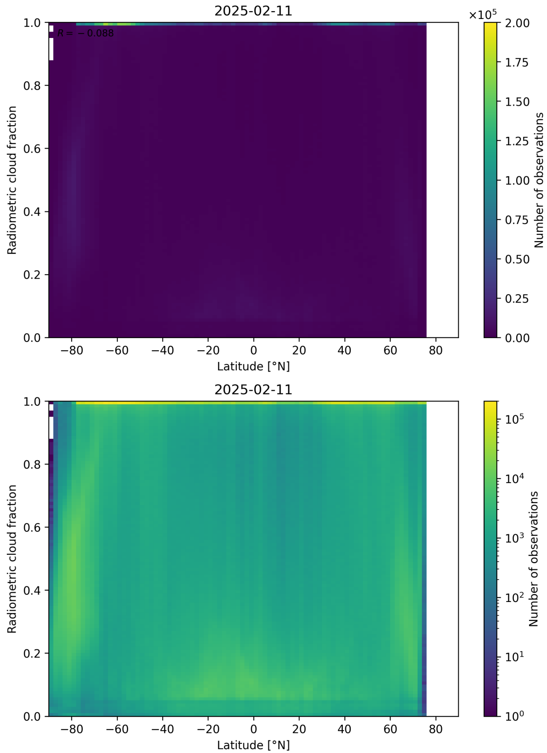
Figure 92: Scatter density plot of “Latitude” against “Radiometric cloud fraction” for 2025-02-10 to 2025-02-12.
