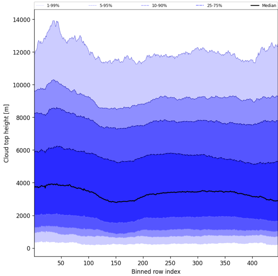
Figure 56: Along track statistics of “Cloud top height” for 2025-02-10 to 2025-02-12
