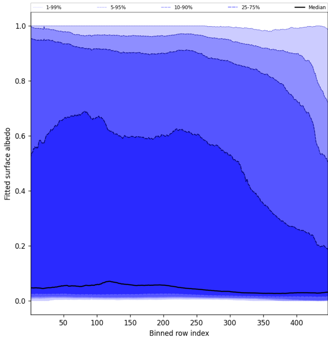
Figure 61: Along track statistics of “Fitted surface albedo” for 2025-02-10 to 2025-02-12
