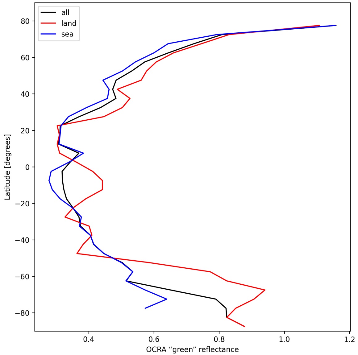
Figure 36: Zonal average of “OCRA “green” reflectance” for 2025-02-10 to 2025-02-12.
