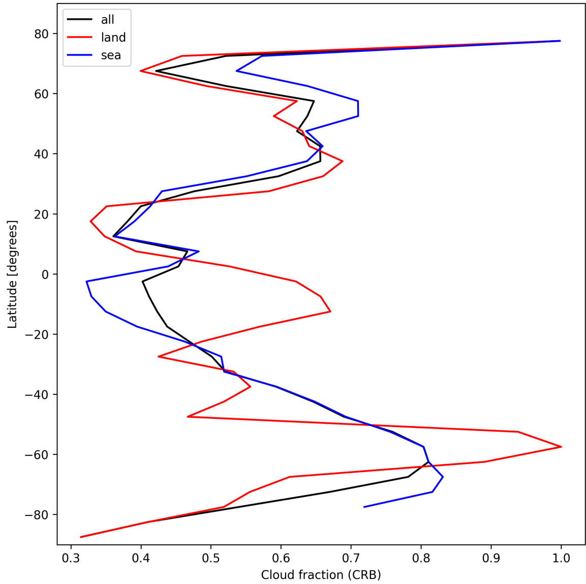
Figure 26: Zonal average of “Cloud fraction (CRB)” for 2025-02-10 to 2025-02-12.
