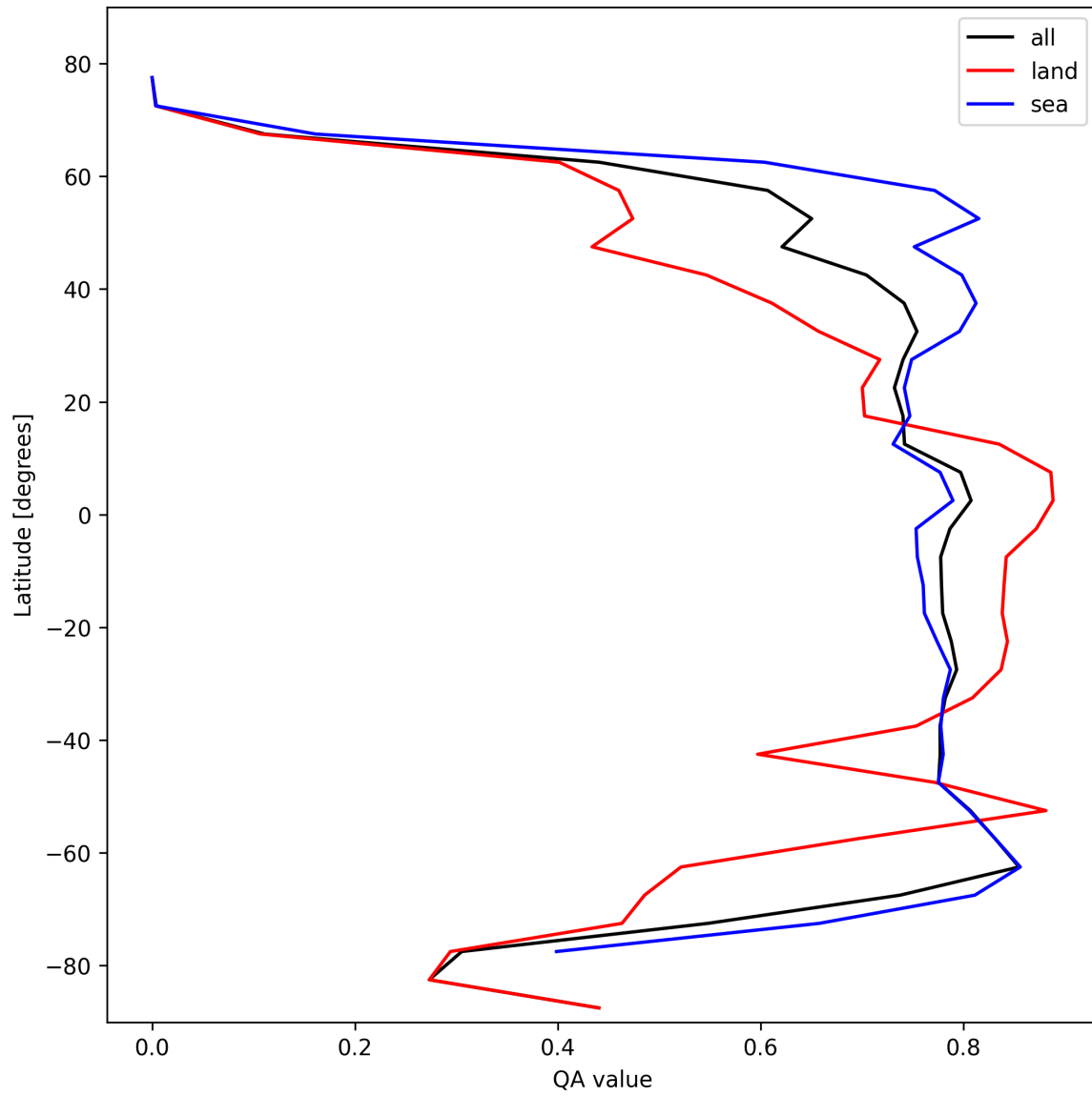
Figure 22: Zonal average of “QA value” for 2025-02-10 to 2025-02-12.
