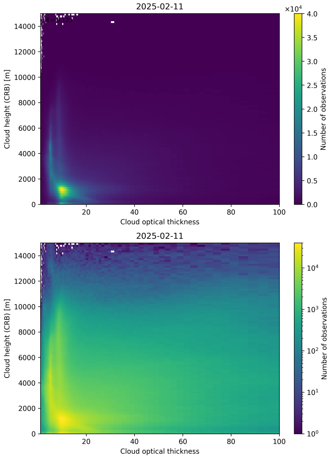
Figure 85: Scatter density plot of “Cloud optical thickness” against “Cloud height (CRB)” for 2025-02-10 to 2025-02-12.
