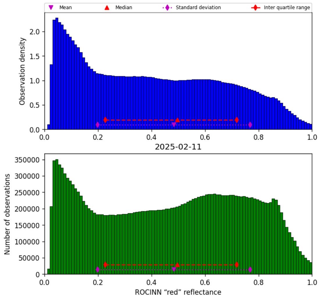
Figure 53: Histogram of “ROCINN “red” reflectance” for 2025-02-10 to 2025-02-12
