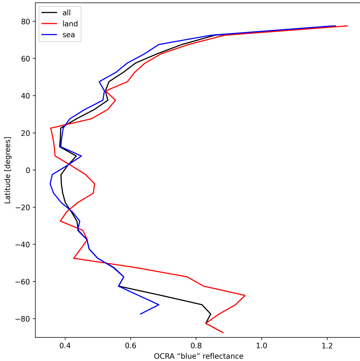
Figure 35: Zonal average of “OCRA “blue” reflectance” for 2025-02-10 to 2025-02-12.
