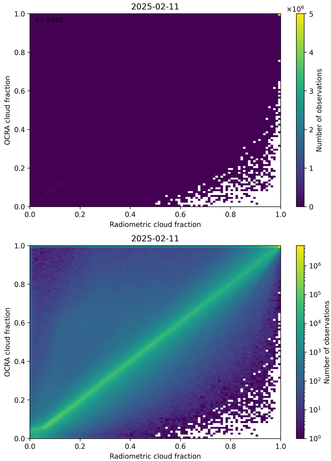
Figure 72: Scatter density plot of “Radiometric cloud fraction” against “OCRA cloud fraction” for 2025-02-10 to 2025-02-12.
