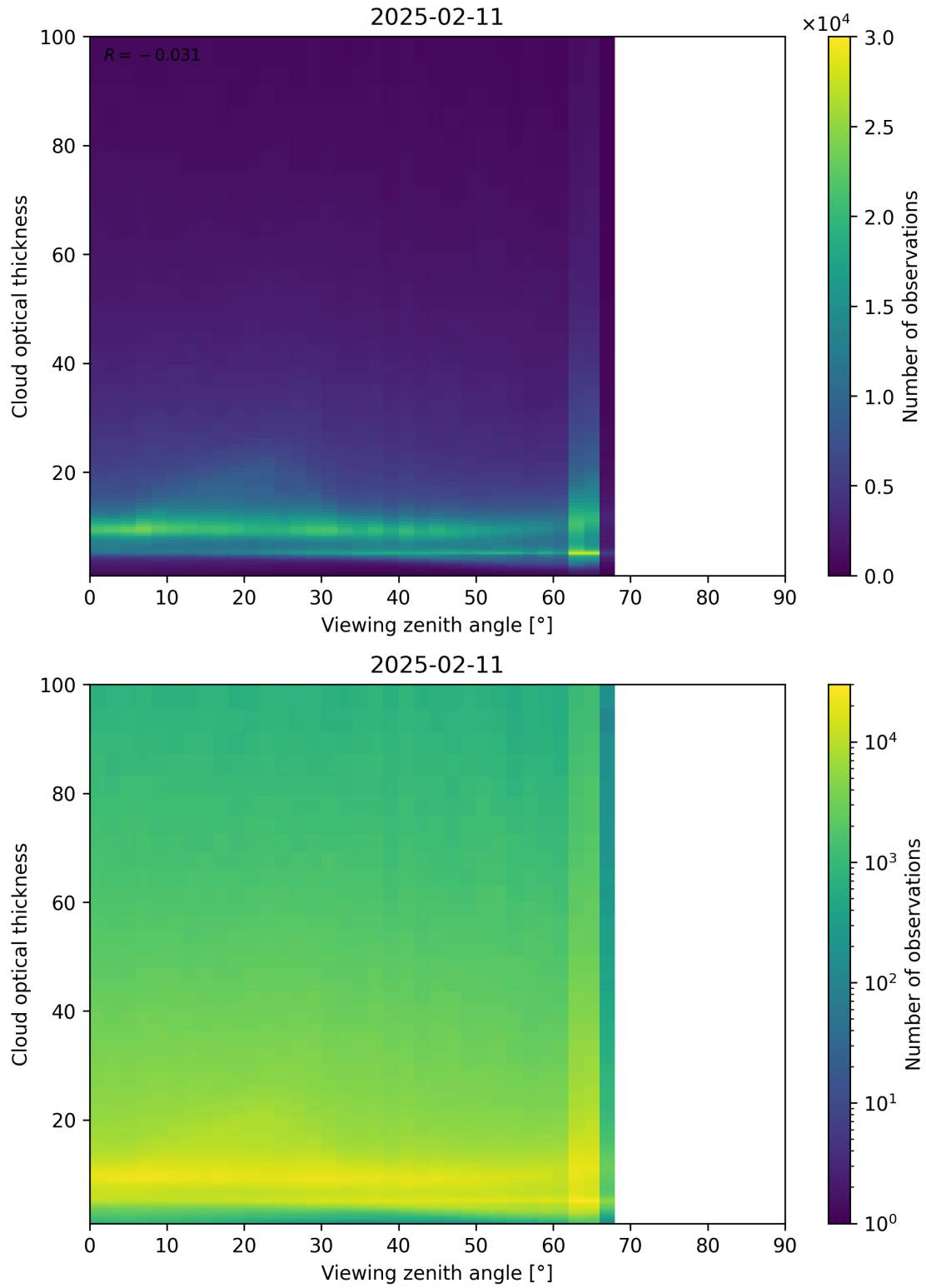
Figure 111: Scatter density plot of “Viewing zenith angle” against “Cloud optical thickness” for 2025-02-10 to 2025-02-12.
