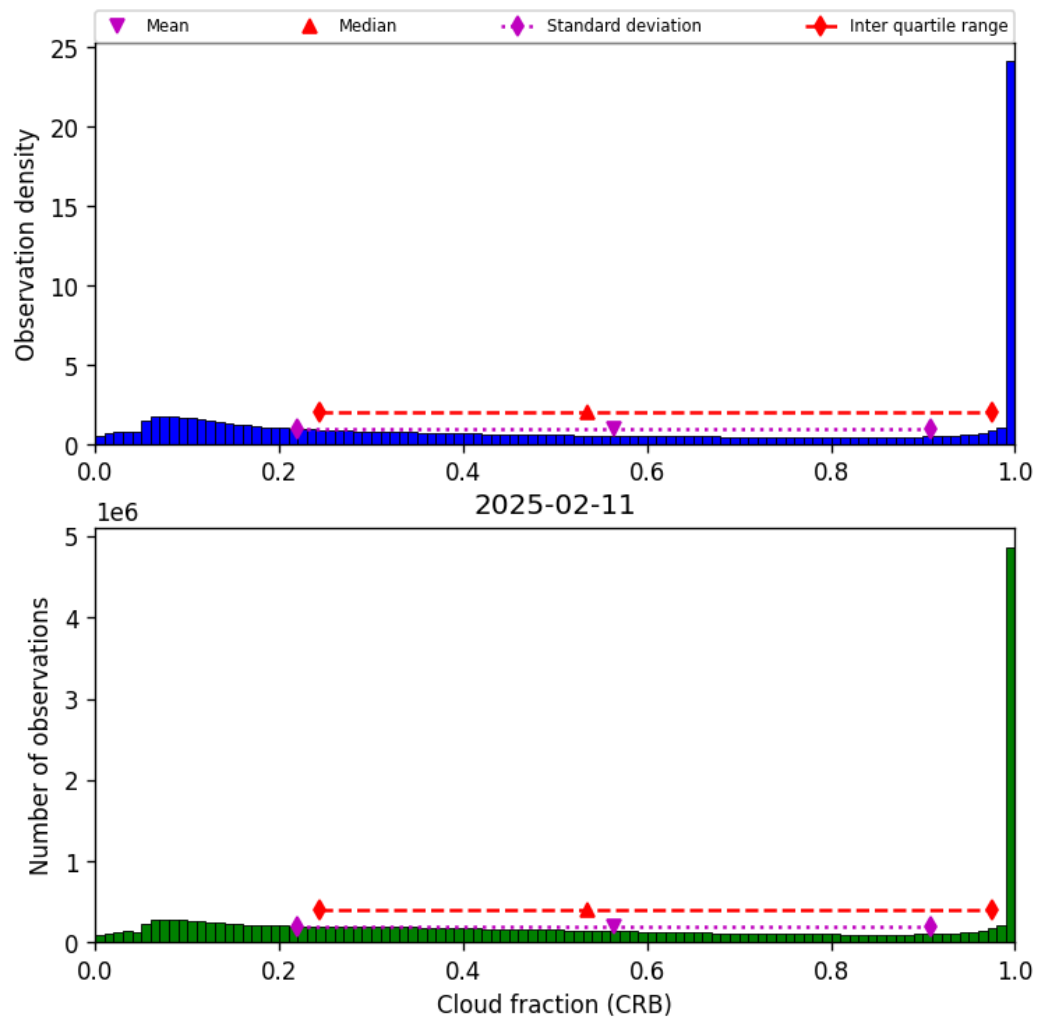
Figure 42: Histogram of “Cloud fraction (CRB)” for 2025-02-10 to 2025-02-12
