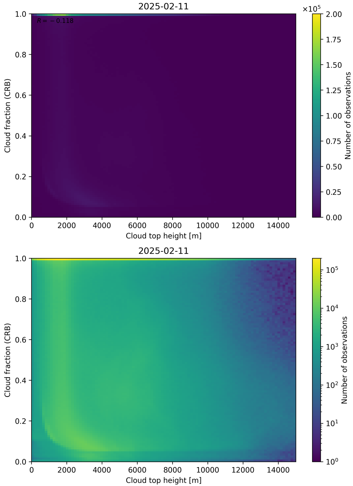
Figure 88: Scatter density plot of “Cloud top height” against “Cloud fraction (CRB)” for 2025-02-10 to 2025-02-12.
