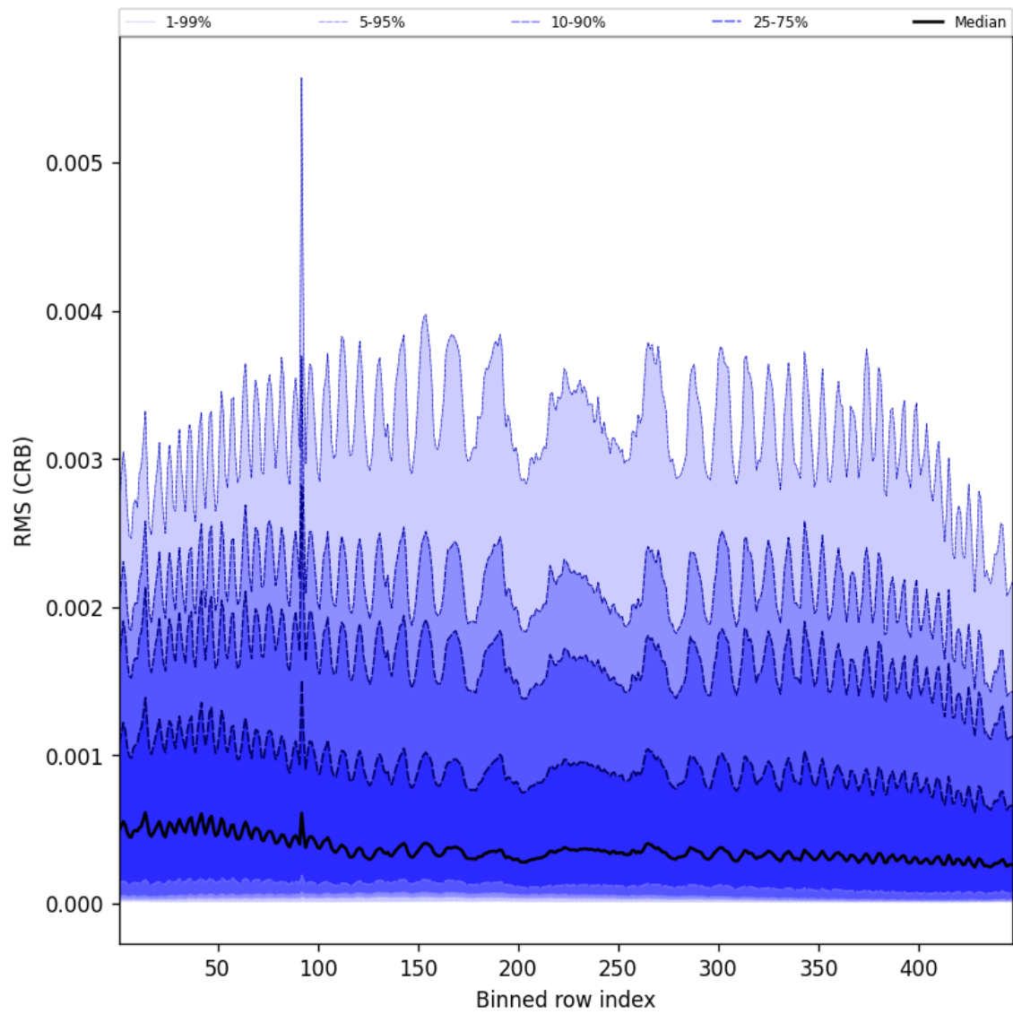
Figure 64: Along track statistics of “RMS (CRB)” for 2025-02-10 to 2025-02-12
