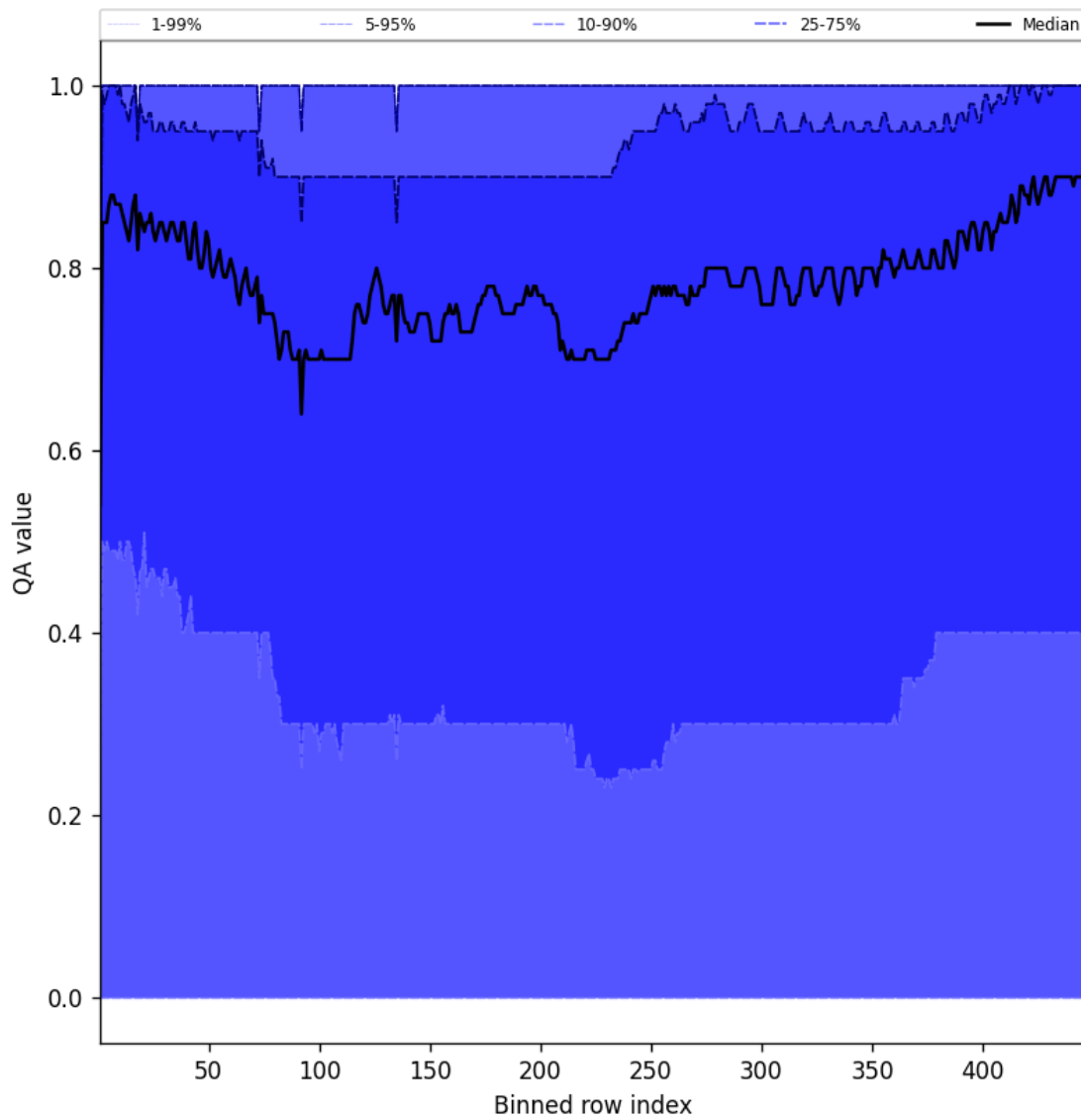
Figure 54: Along track statistics of “QA value” for 2025-02-10 to 2025-02-12
