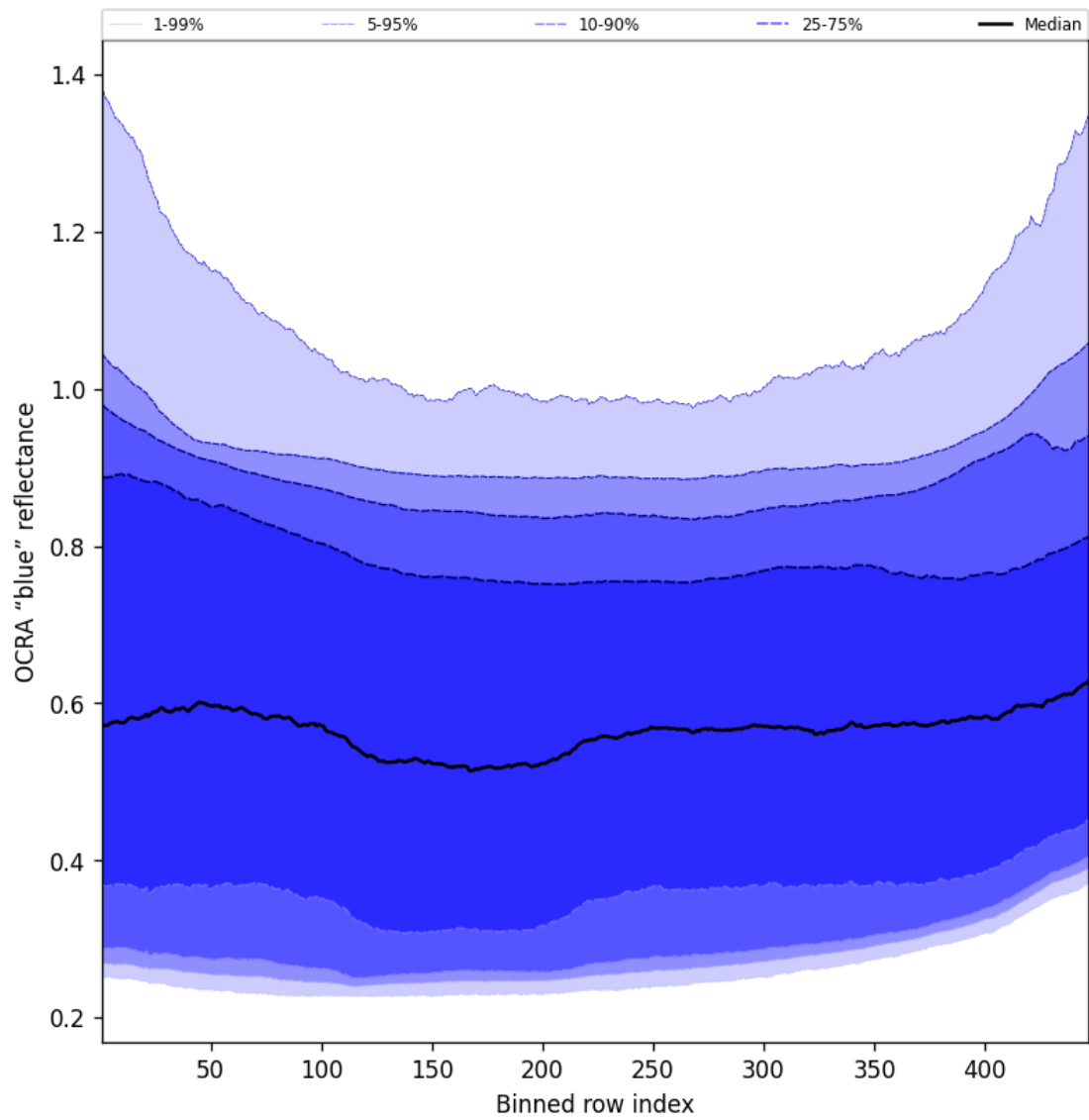
Figure 67: Along track statistics of “OCRA “blue” reflectance” for 2025-02-10 to 2025-02-12
