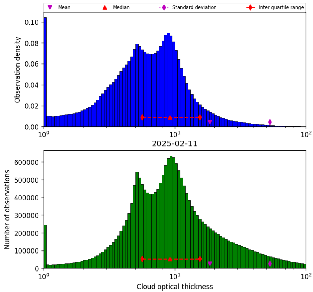
Figure 41: Histogram of “Cloud optical thickness” for 2025-02-10 to 2025-02-12
