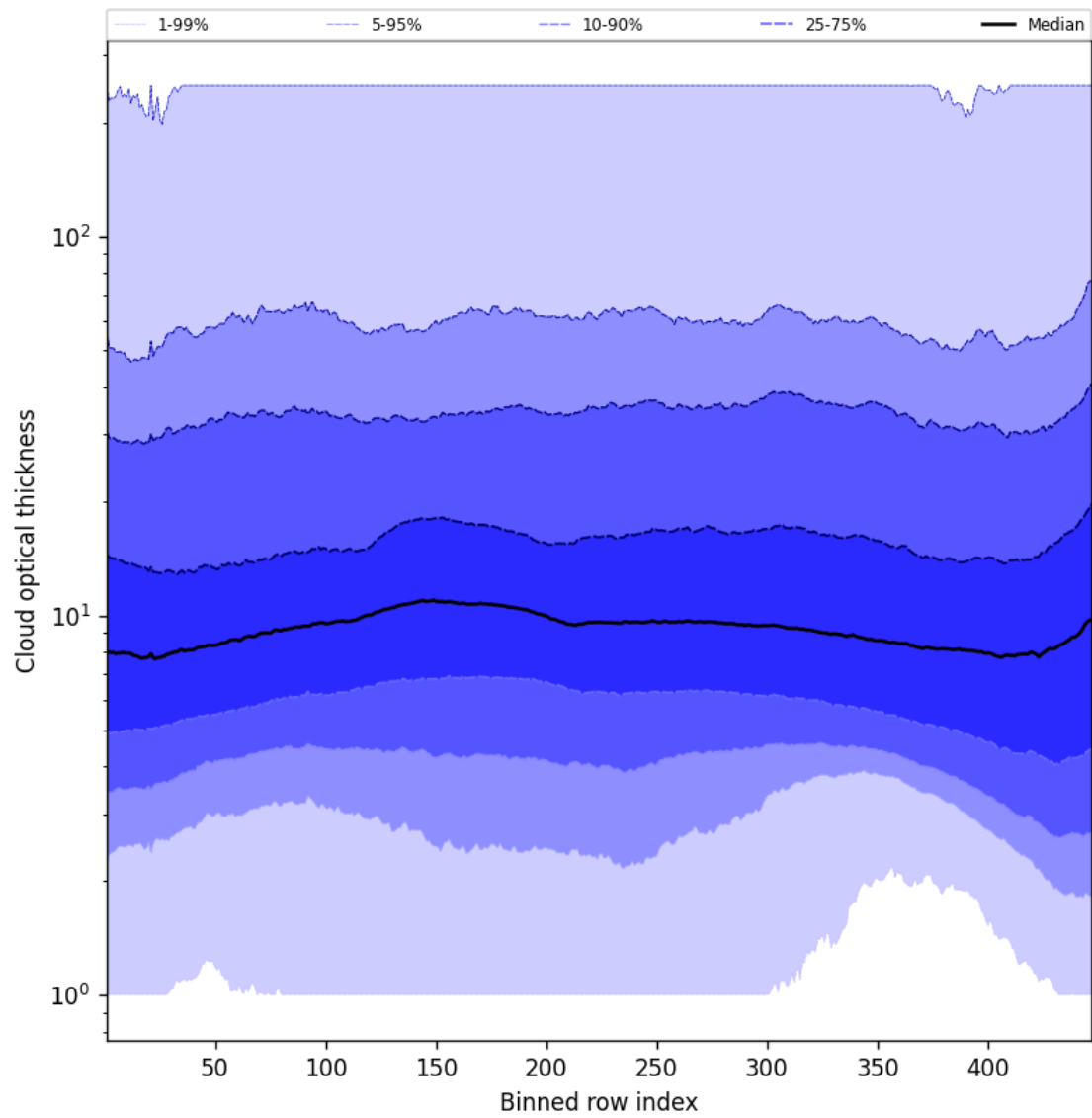
Figure 57: Along track statistics of “Cloud optical thickness” for 2025-02-10 to 2025-02-12
