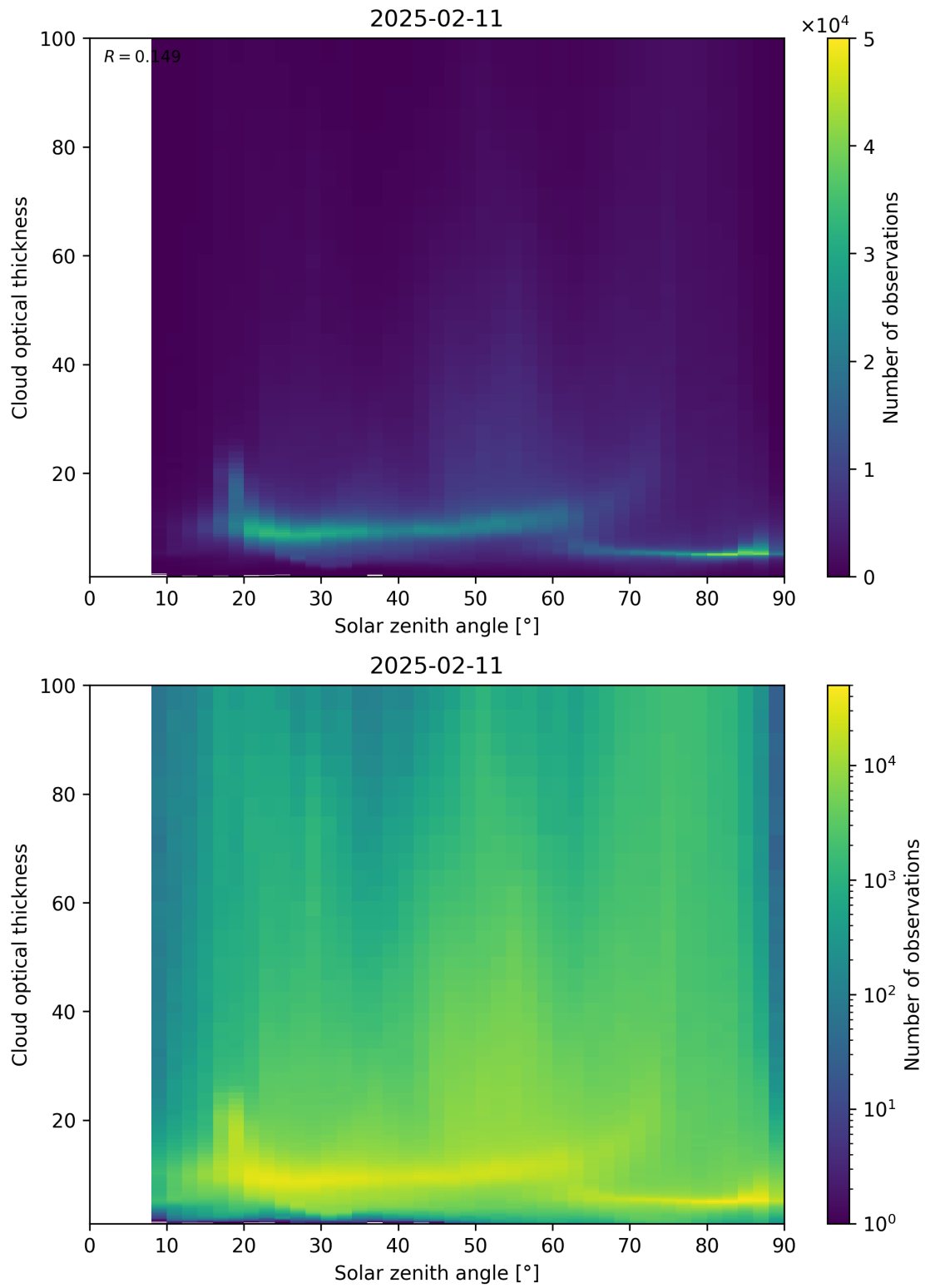
Figure 103: Scatter density plot of “Solar zenith angle” against “Cloud optical thickness” for 2025-02-10 to 2025-02-12.
