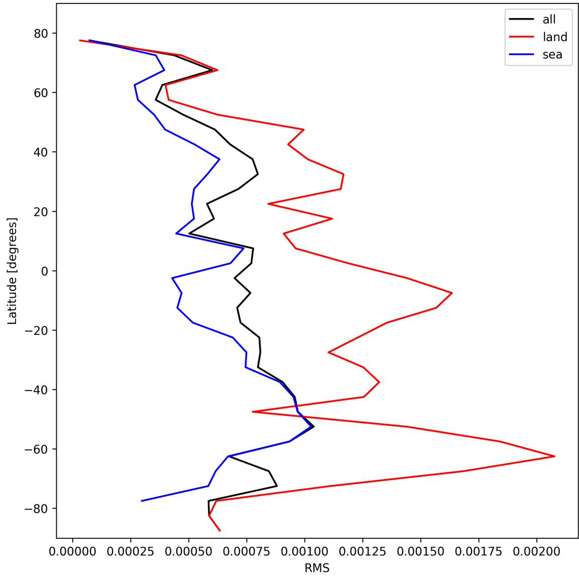
Figure 31: Zonal average of “RMS” for 2025-02-10 to 2025-02-12.
