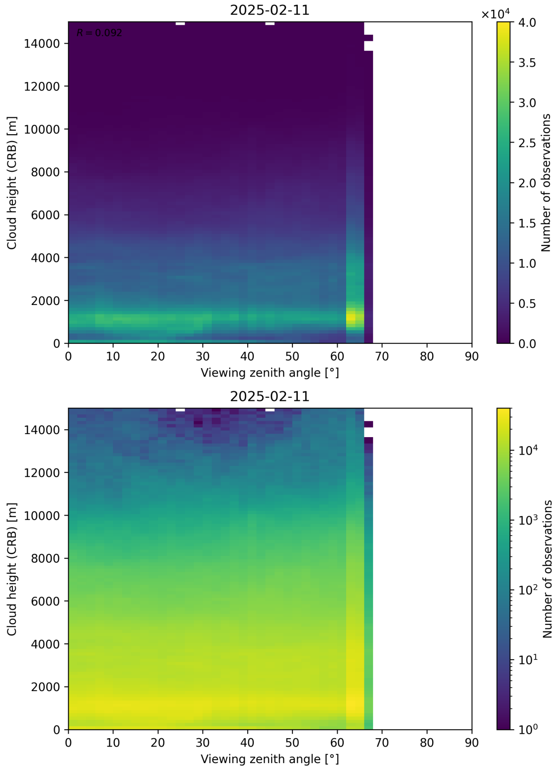
Figure 110: Scatter density plot of “Viewing zenith angle” against “Cloud height (CRB)” for 2025-02-10 to 2025-02-12.
