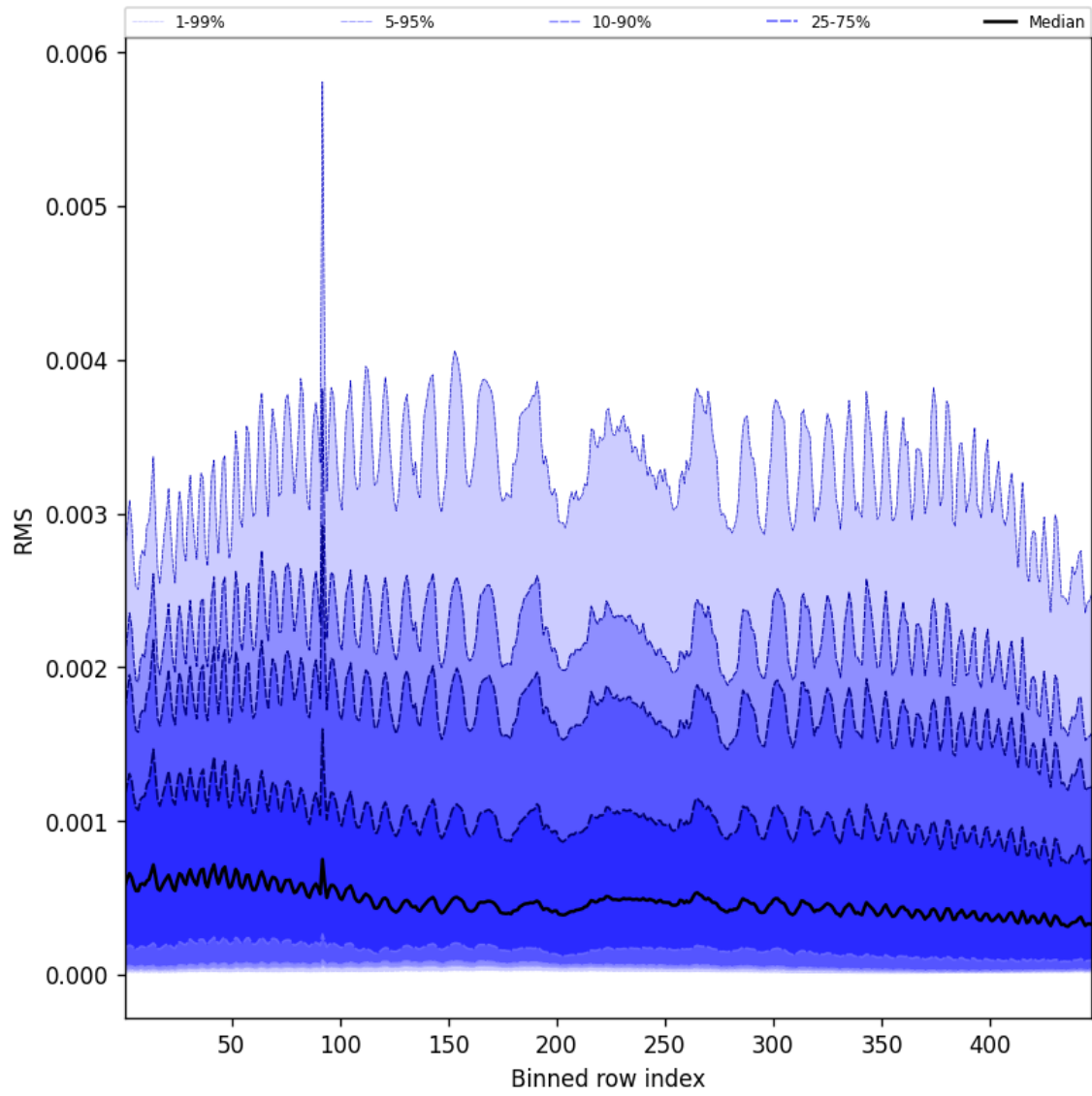
Figure 63: Along track statistics of “RMS” for 2025-02-10 to 2025-02-12
