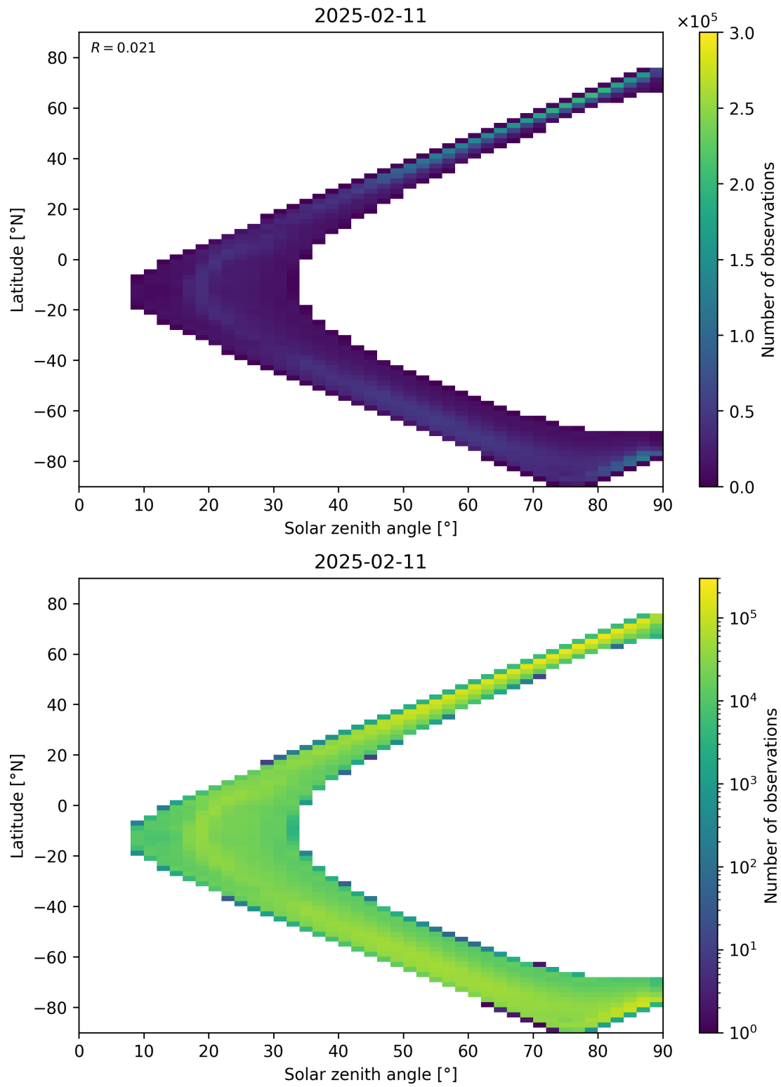
Figure 105: Scatter density plot of “Solar zenith angle” against “Latitude” for 2025-02-10 to 2025-02-12.
