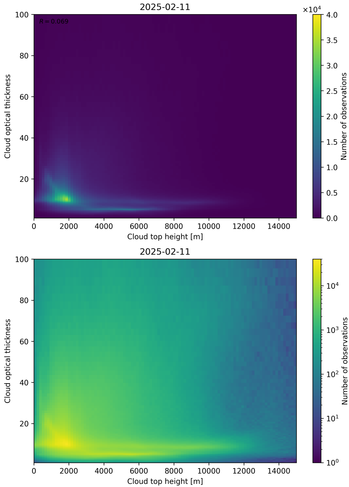
Figure 90: Scatter density plot of “Cloud top height” against “Cloud optical thickness” for 2025-02-10 to 2025-02-12.
