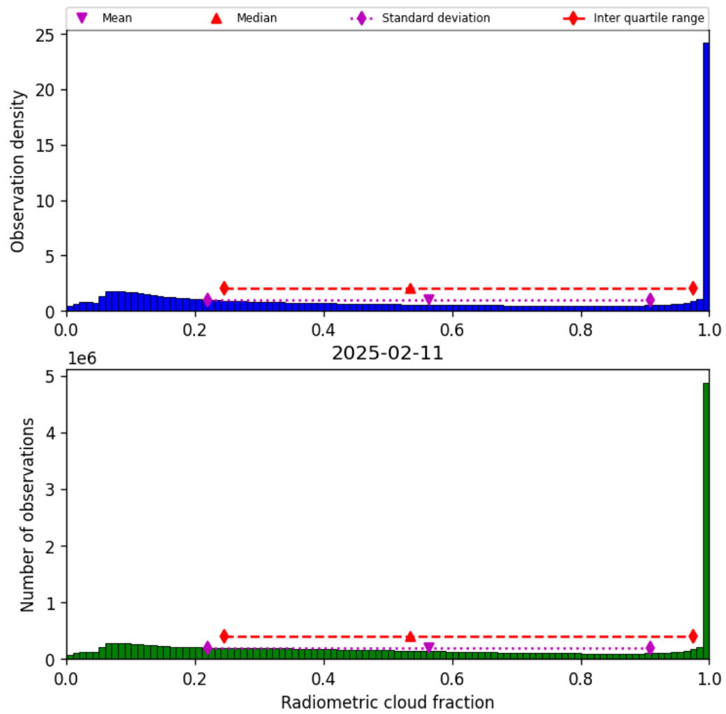
Figure 39: Histogram of “Radiometric cloud fraction” for 2025-02-10 to 2025-02-12
