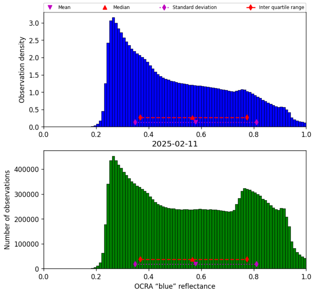
Figure 51: Histogram of “OCRA “blue” reflectance” for 2025-02-10 to 2025-02-12
