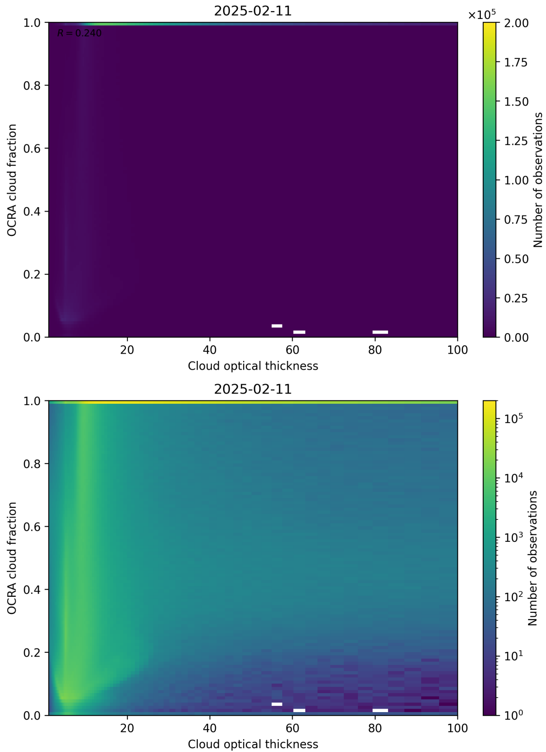
Figure 83: Scatter density plot of “Cloud optical thickness” against “OCRA cloud fraction” for 2025-02-10 to 2025-02-12.
