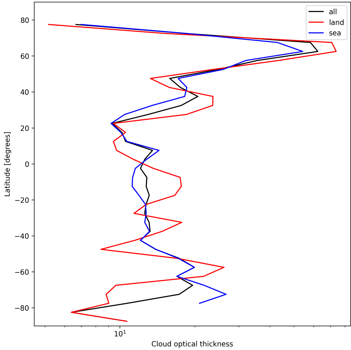
Figure 25: Zonal average of “Cloud optical thickness” for 2025-02-10 to 2025-02-12.
