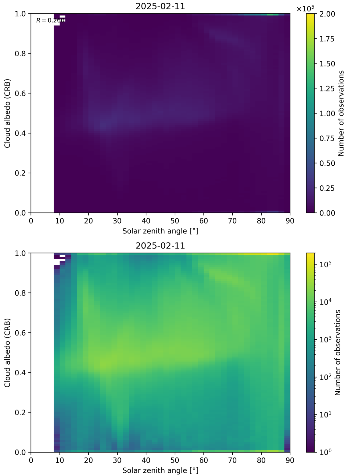
Figure 98: Scatter density plot of “Solar zenith angle” against “Cloud albedo (CRB)” for 2025-02-10 to 2025-02-12.
