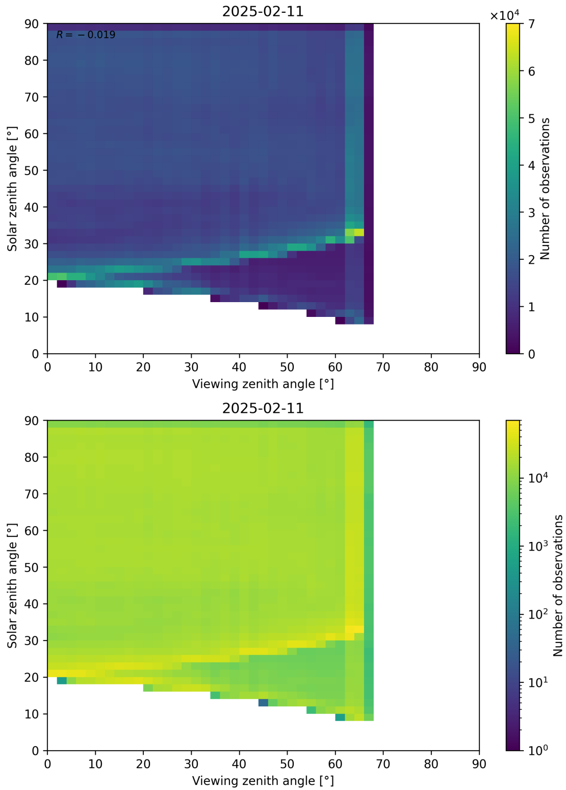
Figure 114: Scatter density plot of “Viewing zenith angle” against “Solar zenith angle” for 2025-02-10 to 2025-02-12.
