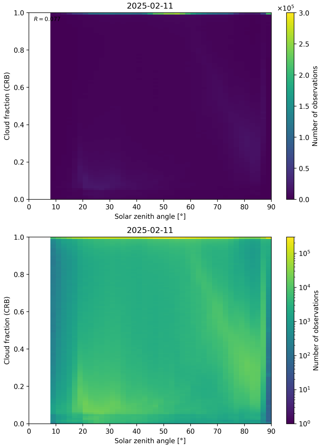
Figure 101: Scatter density plot of “Solar zenith angle” against “Cloud fraction (CRB)” for 2025-02-10 to 2025-02-12.
