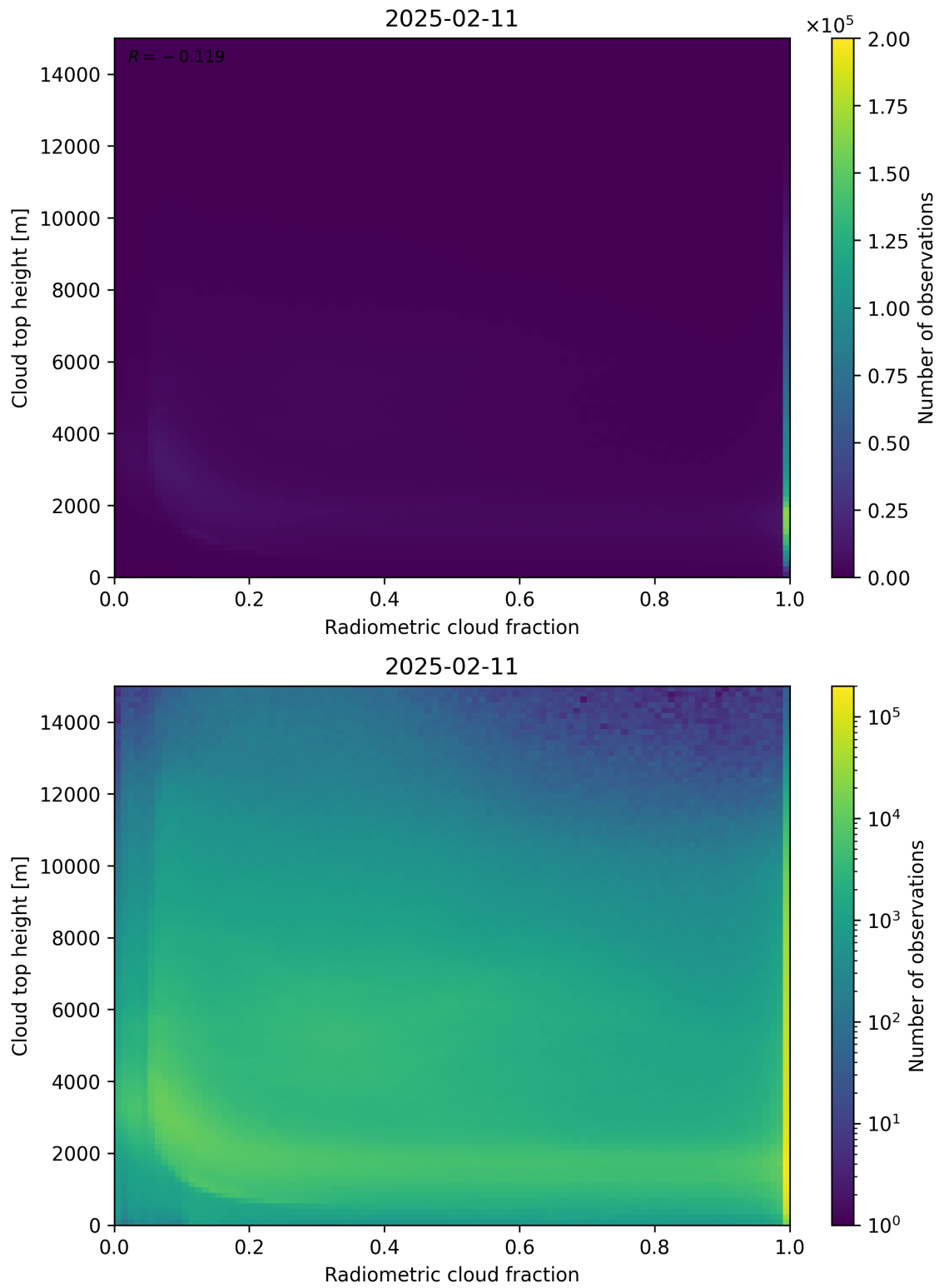
Figure 76: Scatter density plot of “Radiometric cloud fraction” against “Cloud top height” for 2025-02-10 to 2025-02-12.
