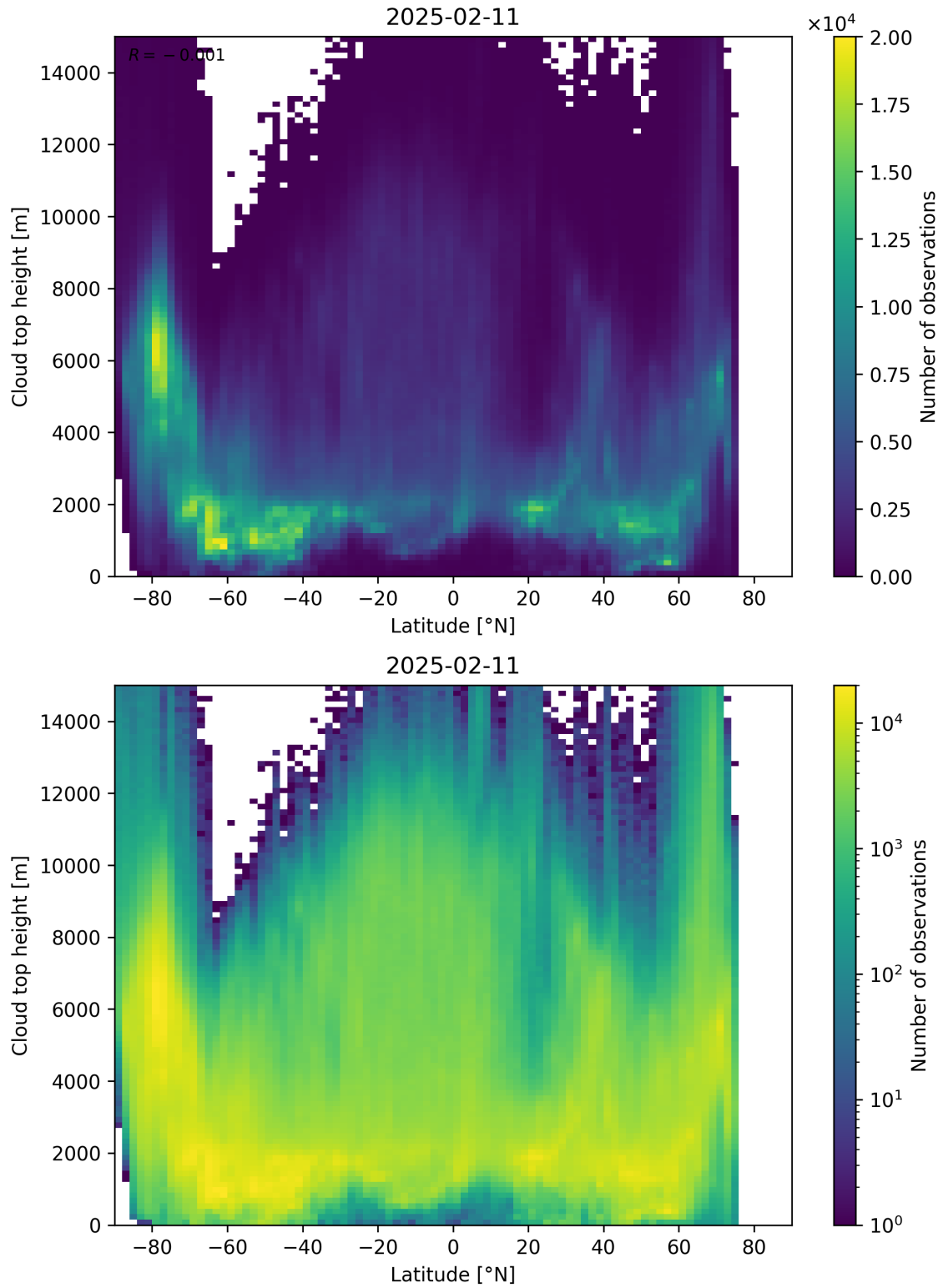
Figure 97: Scatter density plot of “Latitude” against “Cloud top height” for 2025-02-10 to 2025-02-12.
