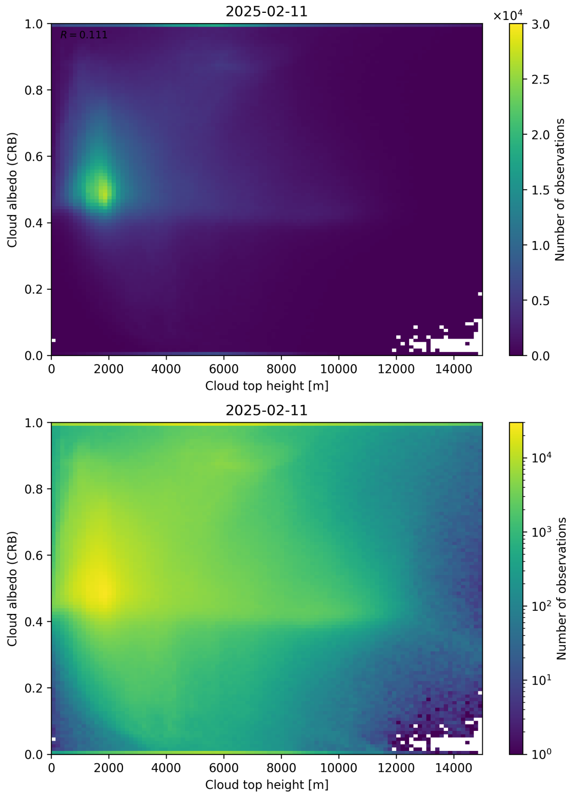
Figure 86: Scatter density plot of “Cloud top height” against “Cloud albedo (CRB)” for 2025-02-10 to 2025-02-12.
