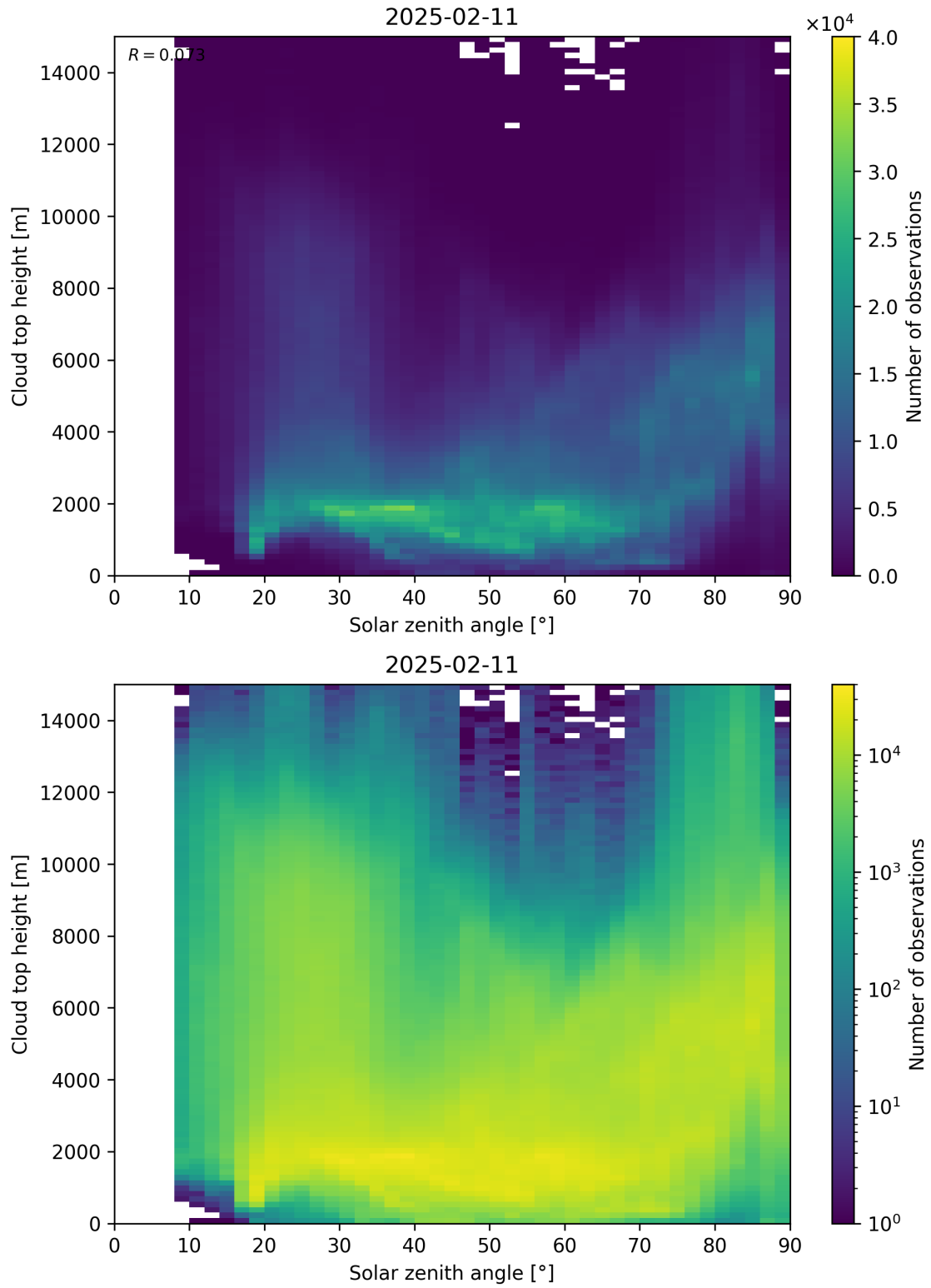
Figure 104: Scatter density plot of “Solar zenith angle” against “Cloud top height” for 2025-02-10 to 2025-02-12.
