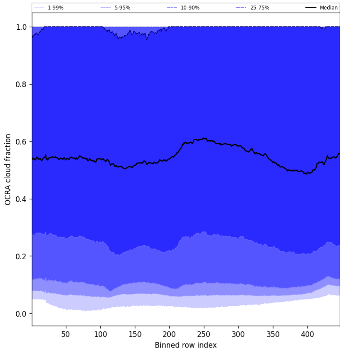
Figure 66: Along track statistics of “OCRA cloud fraction” for 2025-02-10 to 2025-02-12
