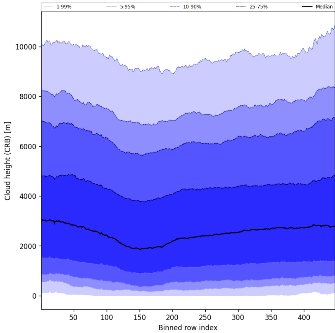
Figure 59: Along track statistics of “Cloud height (CRB)” for 2025-02-10 to 2025-02-12
