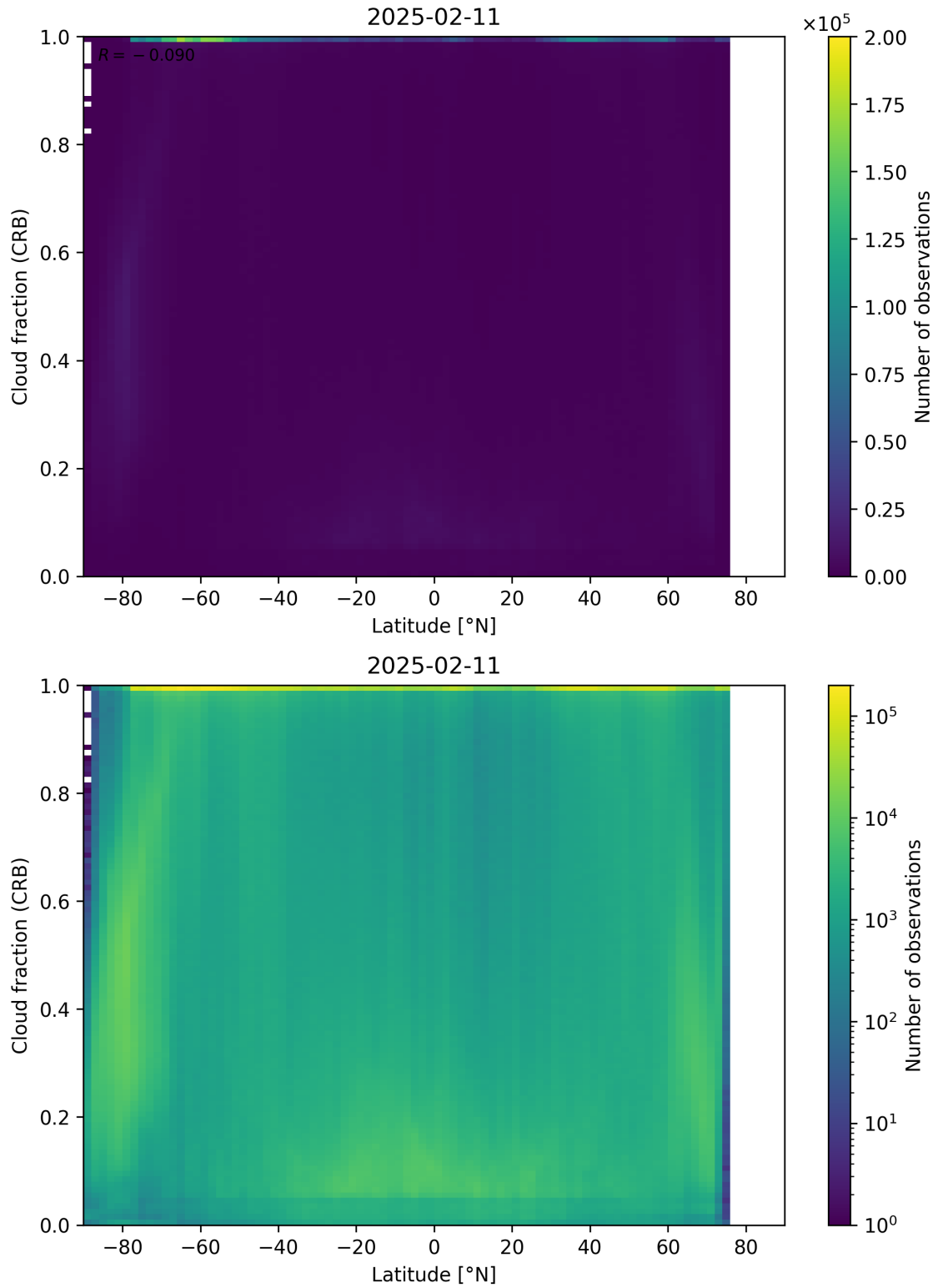
Figure 94: Scatter density plot of “Latitude” against “Cloud fraction (CRB)” for 2025-02-10 to 2025-02-12.
