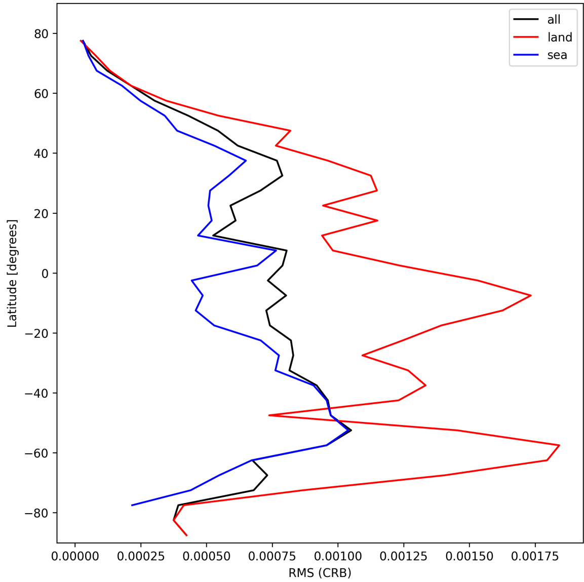
Figure 32: Zonal average of “RMS (CRB)” for 2025-02-10 to 2025-02-12.
