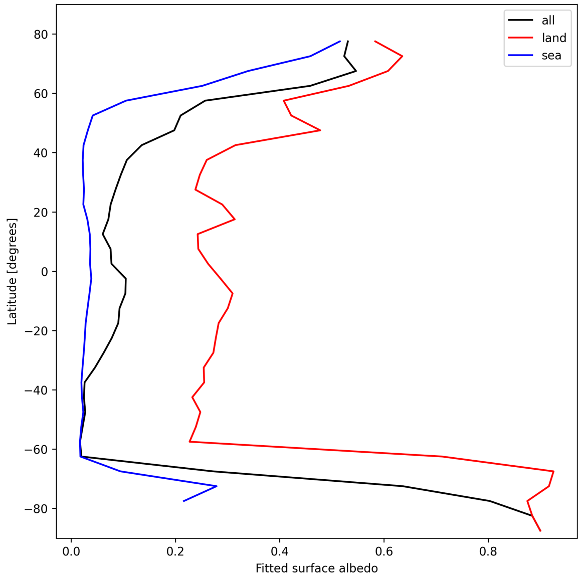
Figure 29: Zonal average of “Fitted surface albedo” for 2025-02-10 to 2025-02-12.
