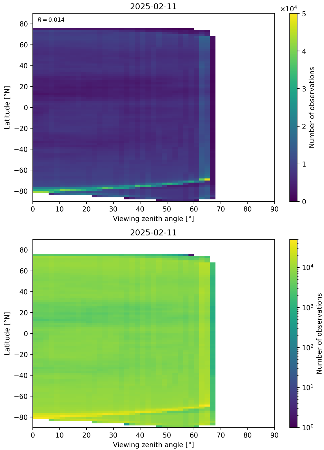
Figure 113: Scatter density plot of “Viewing zenith angle” against “Latitude” for 2025-02-10 to 2025-02-12.
