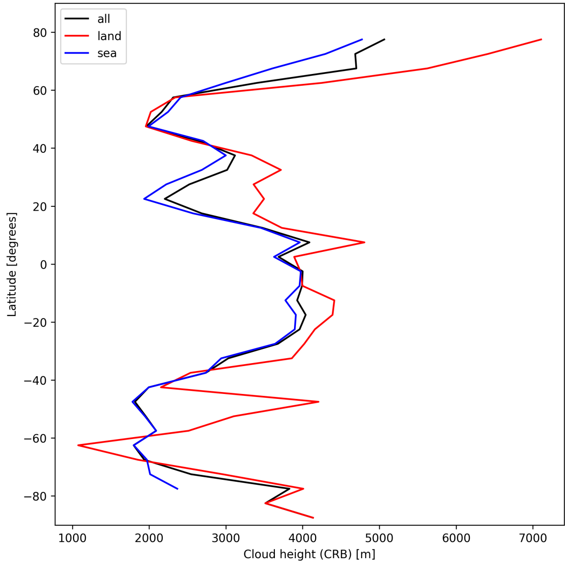
Figure 27: Zonal average of “Cloud height (CRB)” for 2025-02-10 to 2025-02-12.
