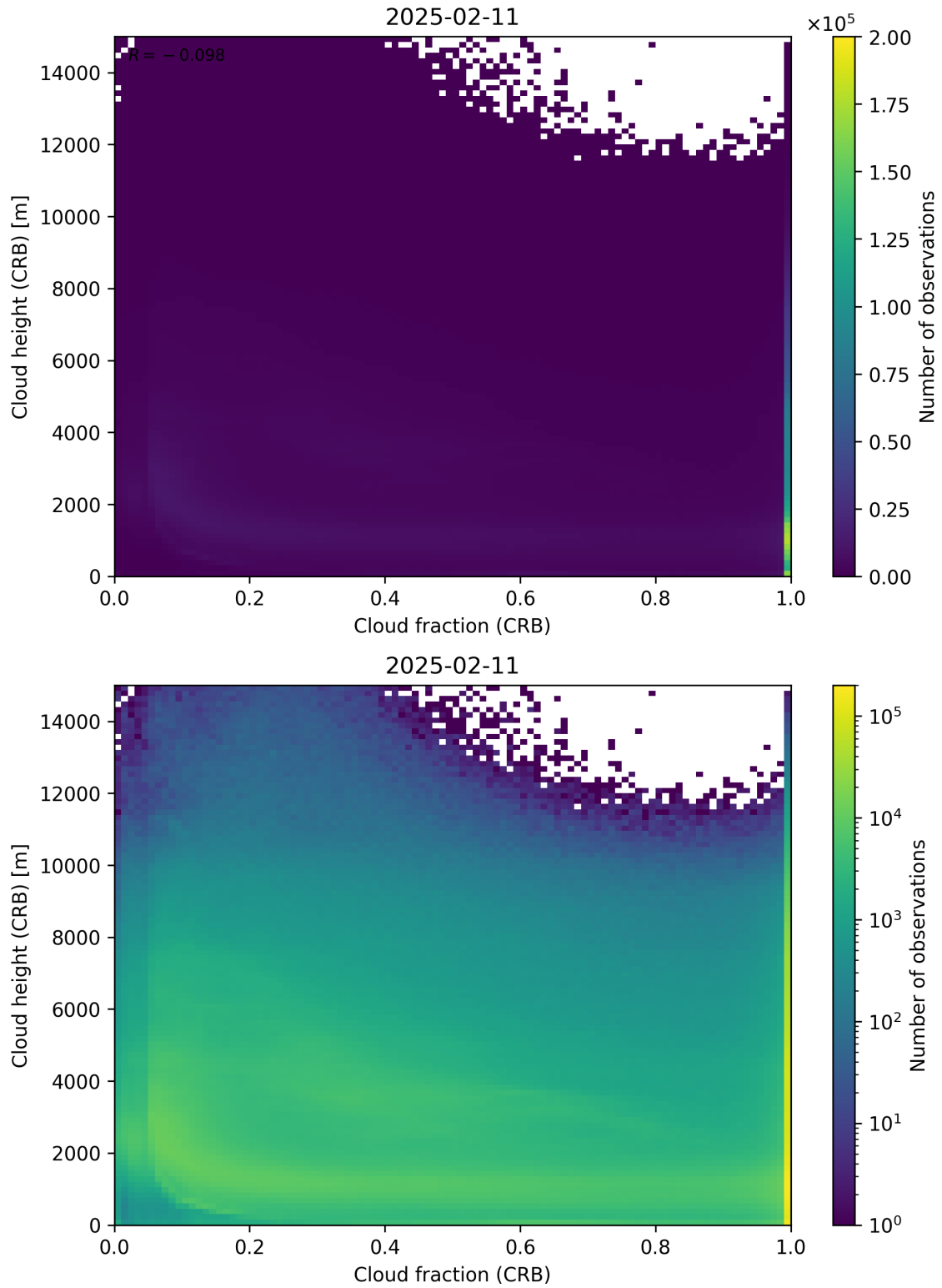
Figure 79: Scatter density plot of “Cloud fraction (CRB)” against “Cloud height (CRB)” for 2025-02-10 to 2025-02-12.
