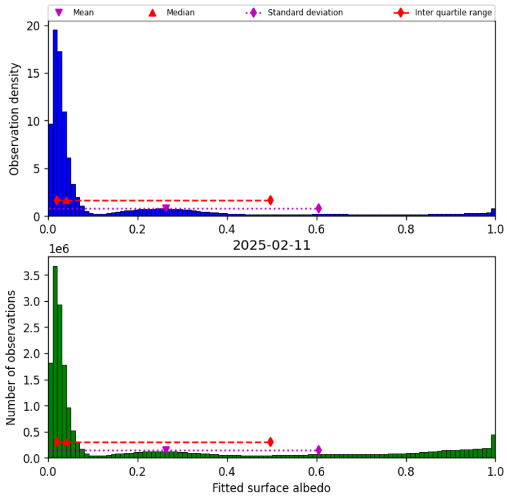
Figure 45: Histogram of “Fitted surface albedo” for 2025-02-10 to 2025-02-12
