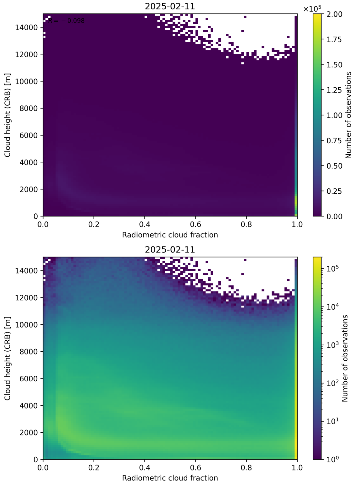
Figure 74: Scatter density plot of “Radiometric cloud fraction” against “Cloud height (CRB)” for 2025-02-10 to 2025-02-12.
