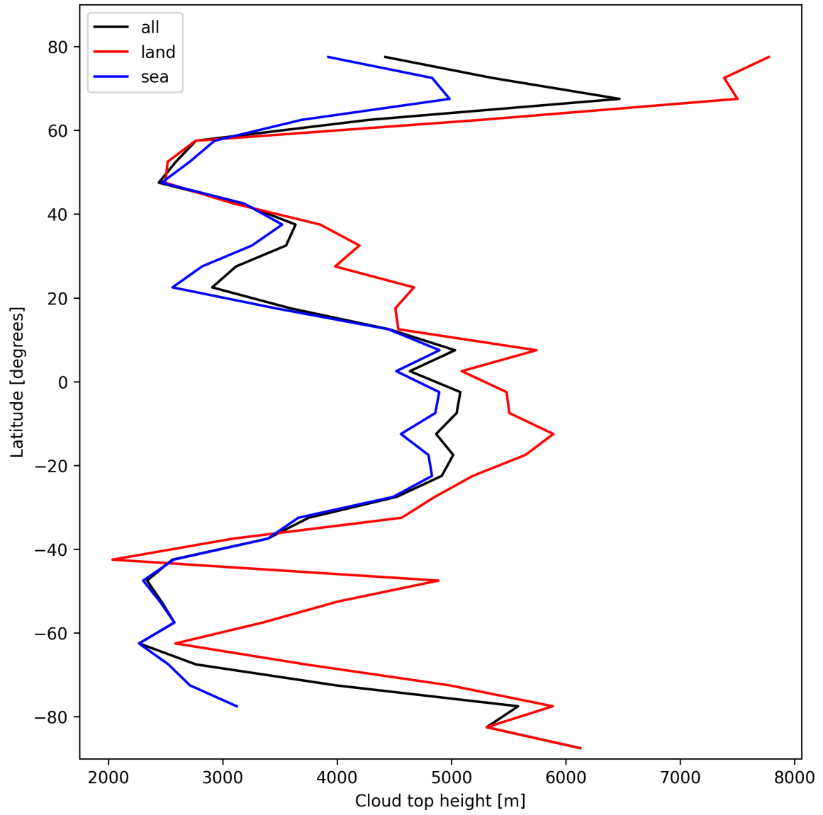
Figure 24: Zonal average of “Cloud top height” for 2025-02-10 to 2025-02-12.
