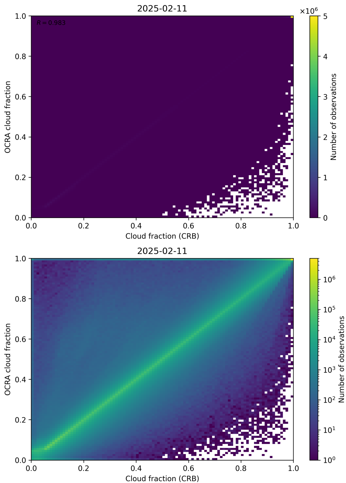
Figure 78: Scatter density plot of “Cloud fraction (CRB)” against “OCRA cloud fraction” for 2025-02-10 to 2025-02-12.
