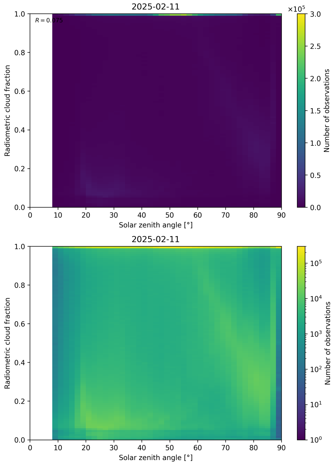
Figure 99: Scatter density plot of “Solar zenith angle” against “Radiometric cloud fraction” for 2025-02-10 to 2025-02-12.
