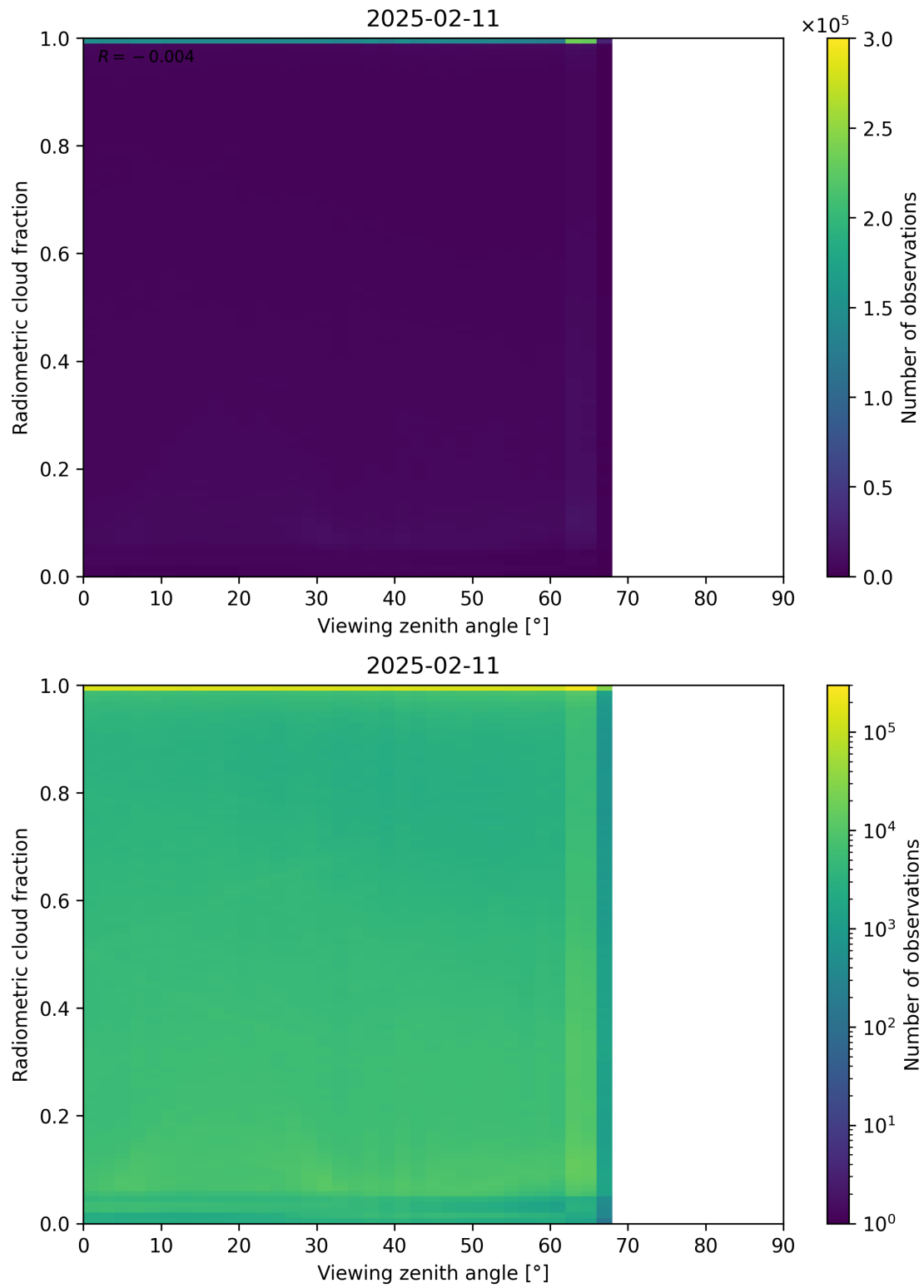
Figure 107: Scatter density plot of “Viewing zenith angle” against “Radiometric cloud fraction” for 2025-02-10 to 2025-02-12.
