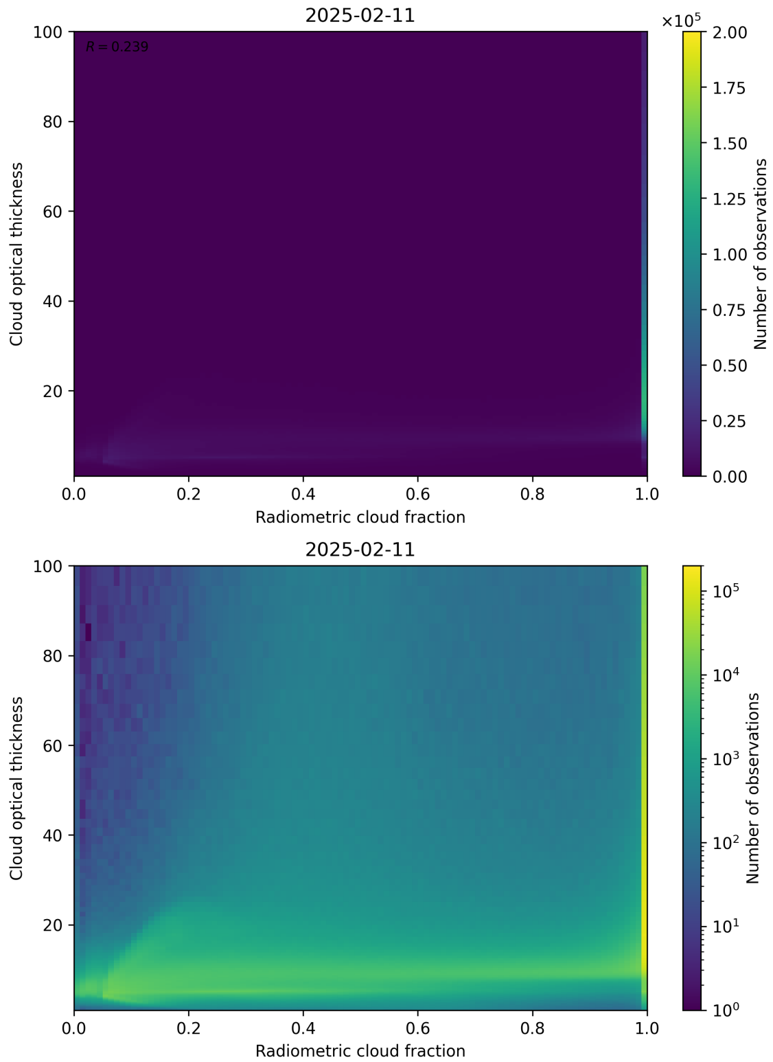
Figure 75: Scatter density plot of “Radiometric cloud fraction” against “Cloud optical thickness” for 2025-02-10 to 2025-02-12.
