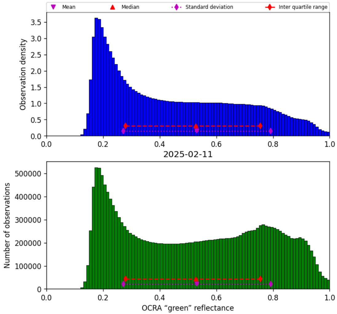
Figure 52: Histogram of “OCRA “green” reflectance” for 2025-02-10 to 2025-02-12
