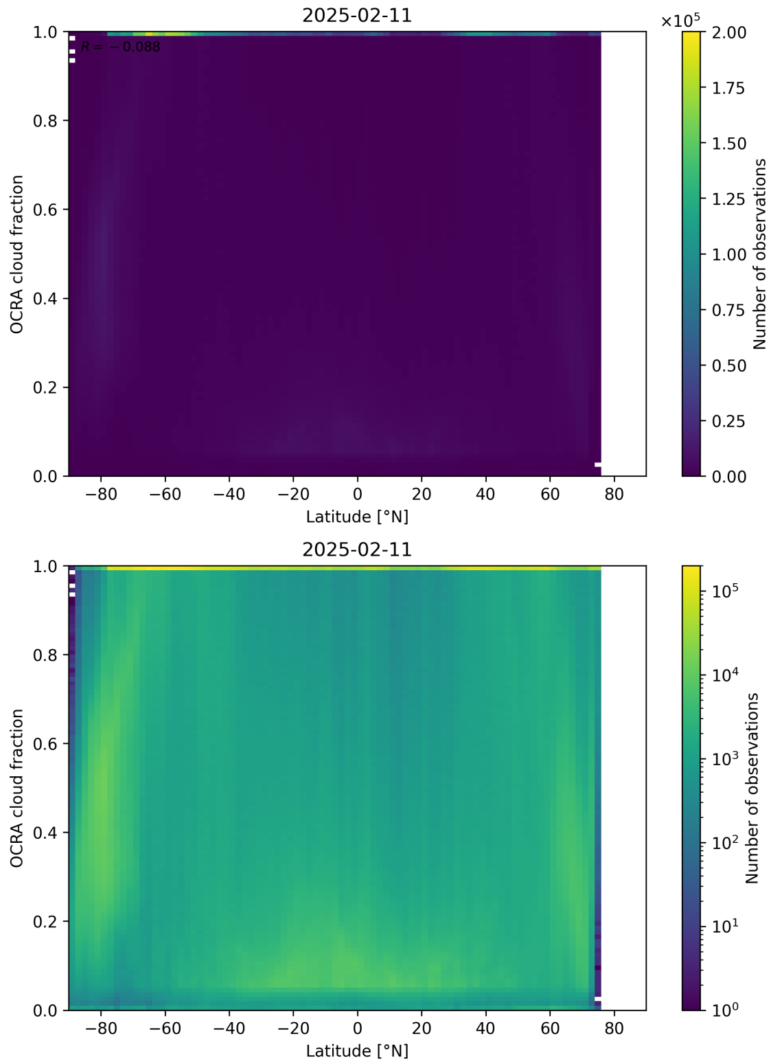
Figure 93: Scatter density plot of “Latitude” against “OCRA cloud fraction” for 2025-02-10 to 2025-02-12.
