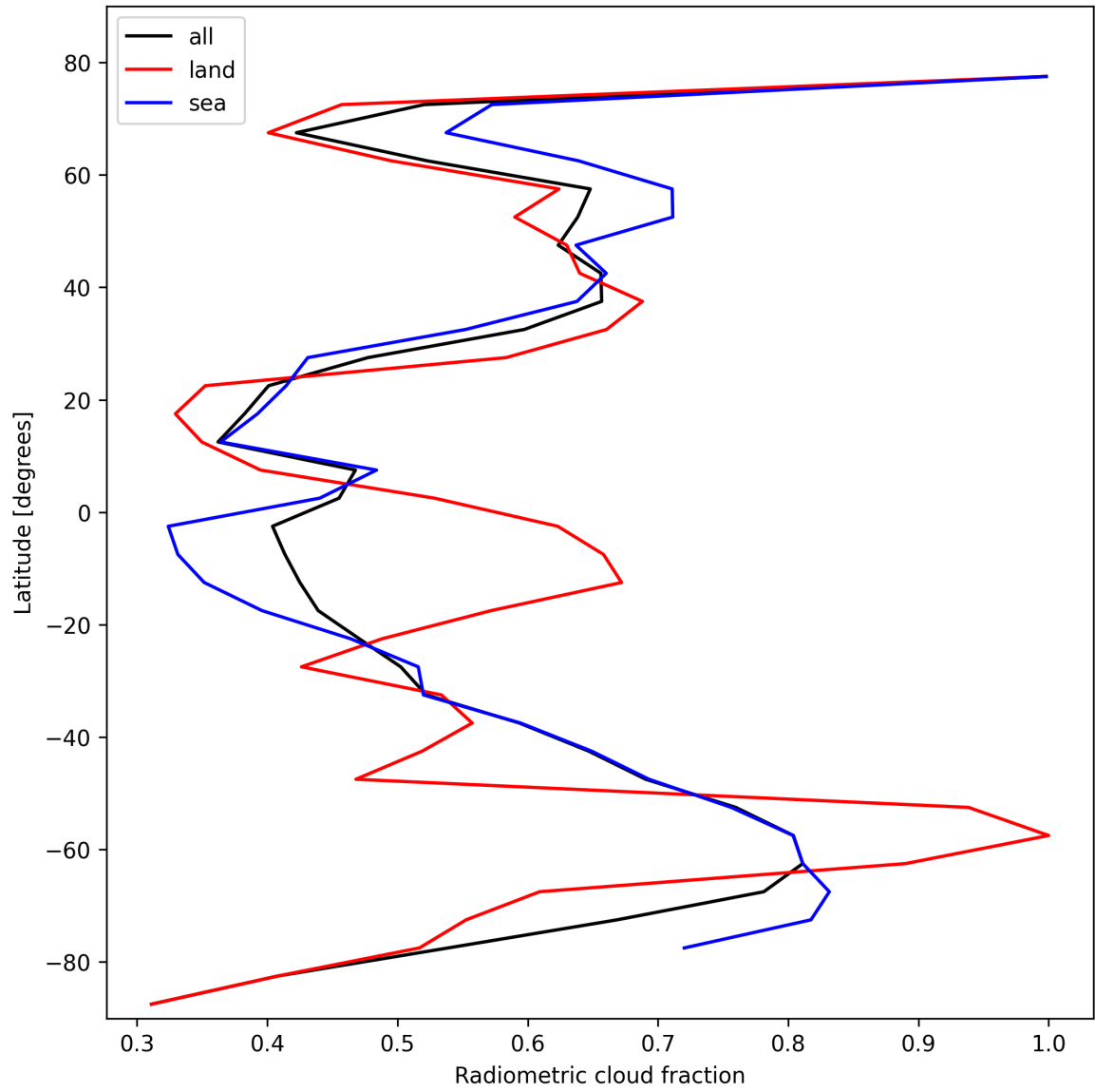
Figure 23: Zonal average of “Radiometric cloud fraction” for 2025-02-10 to 2025-02-12.
