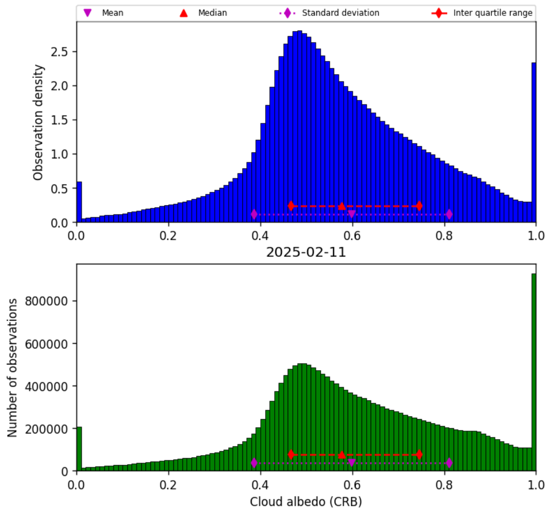
Figure 44: Histogram of “Cloud albedo (CRB)” for 2025-02-10 to 2025-02-12
