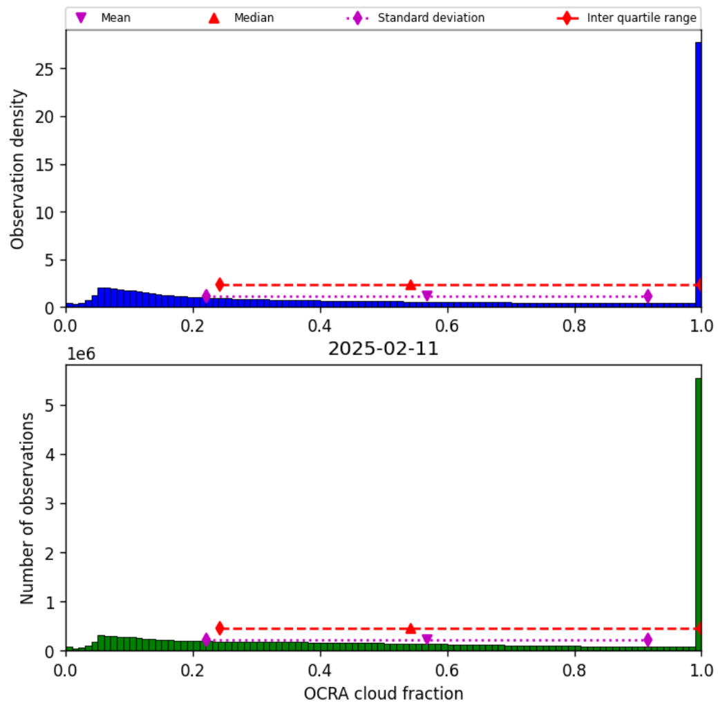
Figure 50: Histogram of “OCRA cloud fraction” for 2025-02-10 to 2025-02-12
