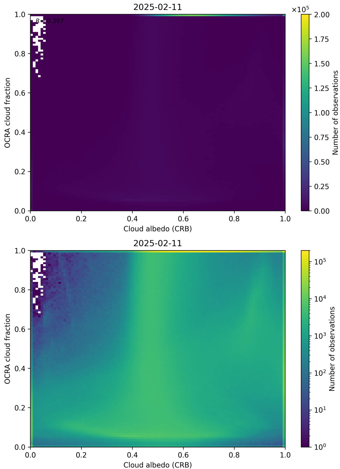
Figure 70: Scatter density plot of “Cloud albedo (CRB)” against “OCRA cloud fraction” for 2025-02-10 to 2025-02-12.
