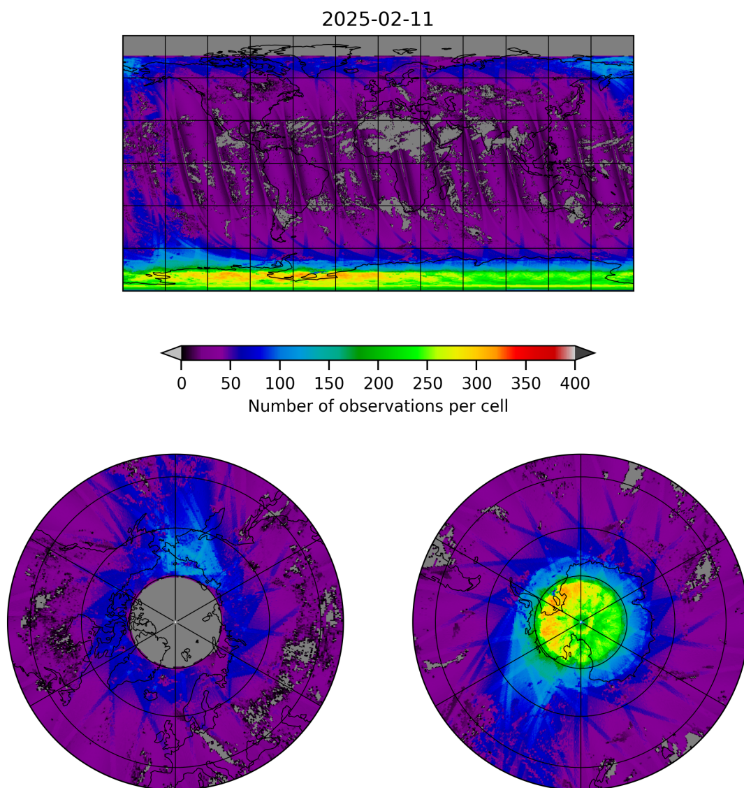
Figure 21: Map of the number of observations for 2025-02-10 to 2025-02-12
