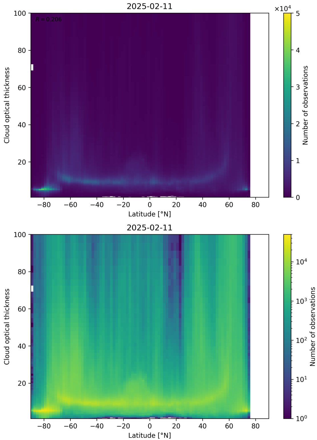
Figure 96: Scatter density plot of “Latitude” against “Cloud optical thickness” for 2025-02-10 to 2025-02-12.
