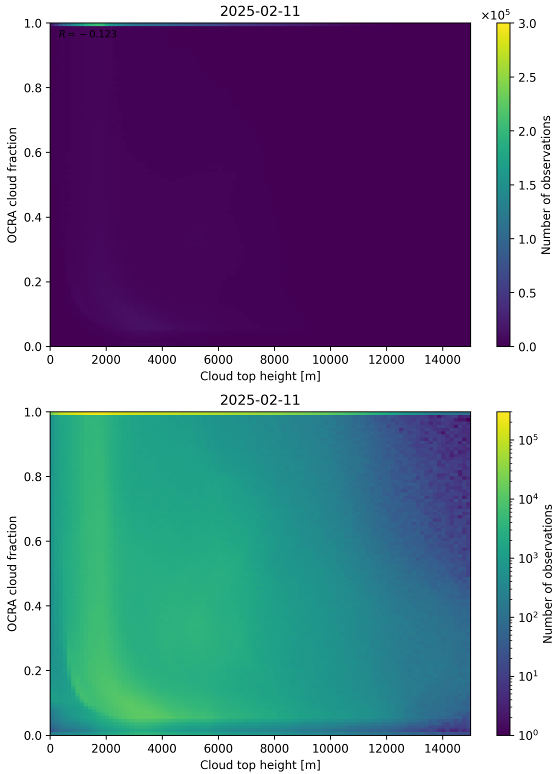
Figure 87: Scatter density plot of “Cloud top height” against “OCRA cloud fraction” for 2025-02-10 to 2025-02-12.
