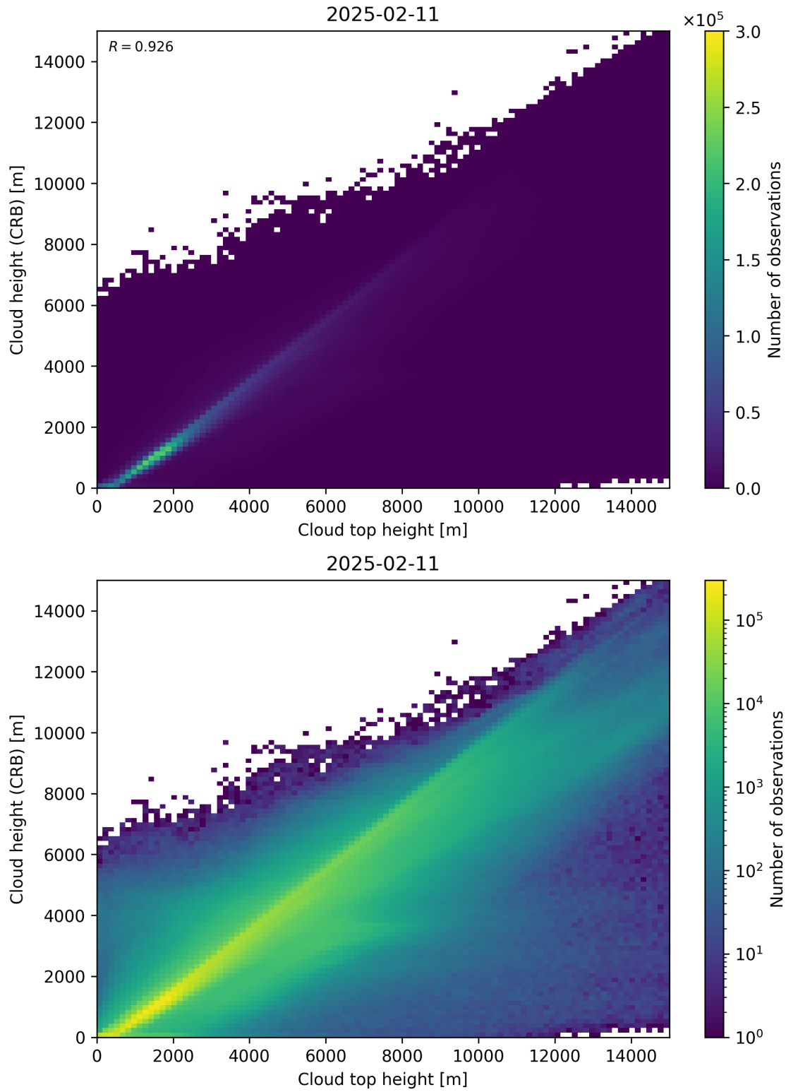
Figure 89: Scatter density plot of “Cloud top height” against “Cloud height (CRB)” for 2025-02-10 to 2025-02-12.
