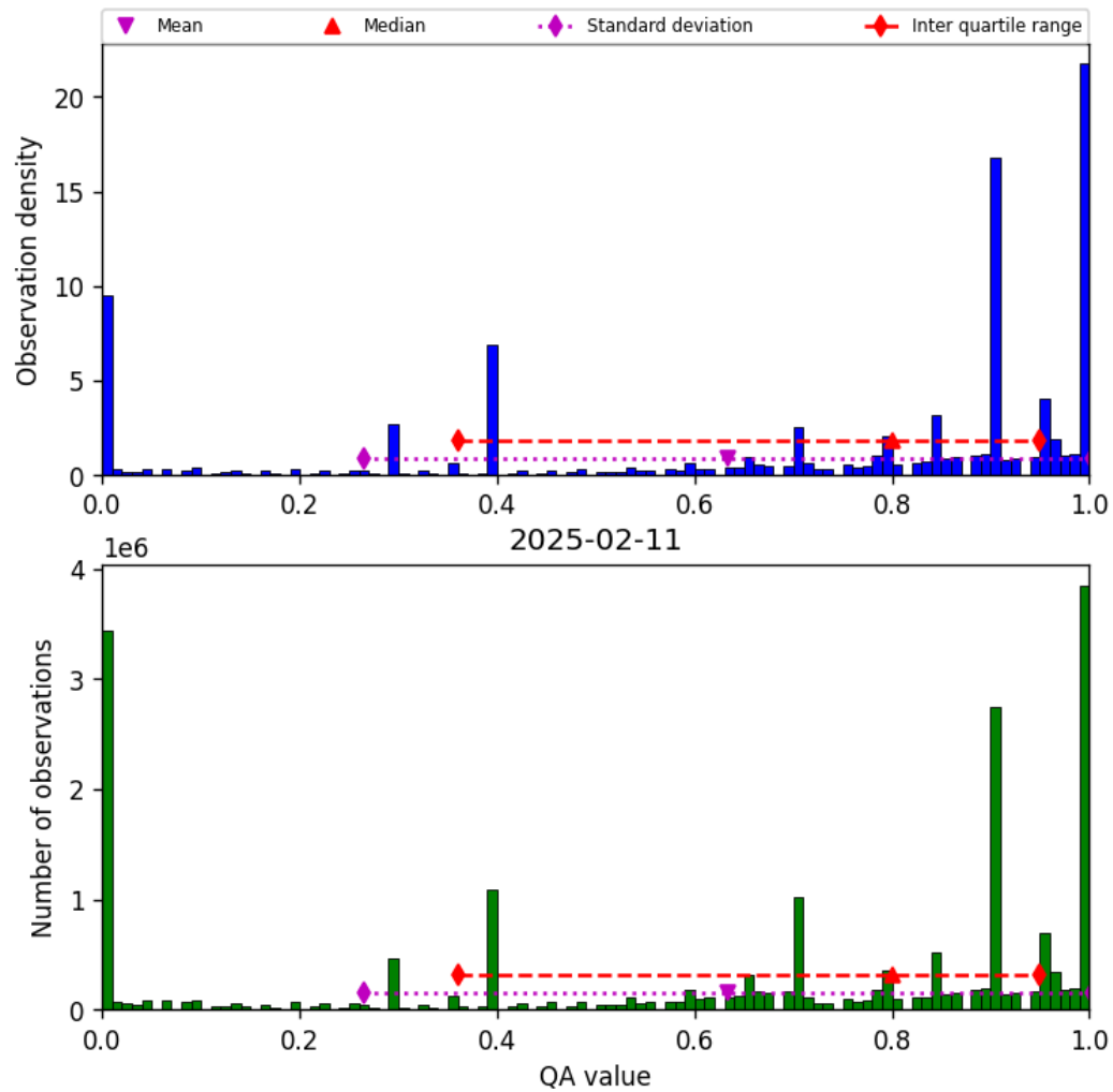
Figure 38: Histogram of “QA value” for 2025-02-10 to 2025-02-12
