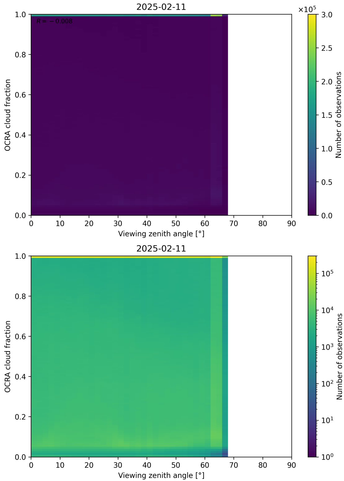
Figure 108: Scatter density plot of “Viewing zenith angle” against “OCRA cloud fraction” for 2025-02-10 to 2025-02-12.
