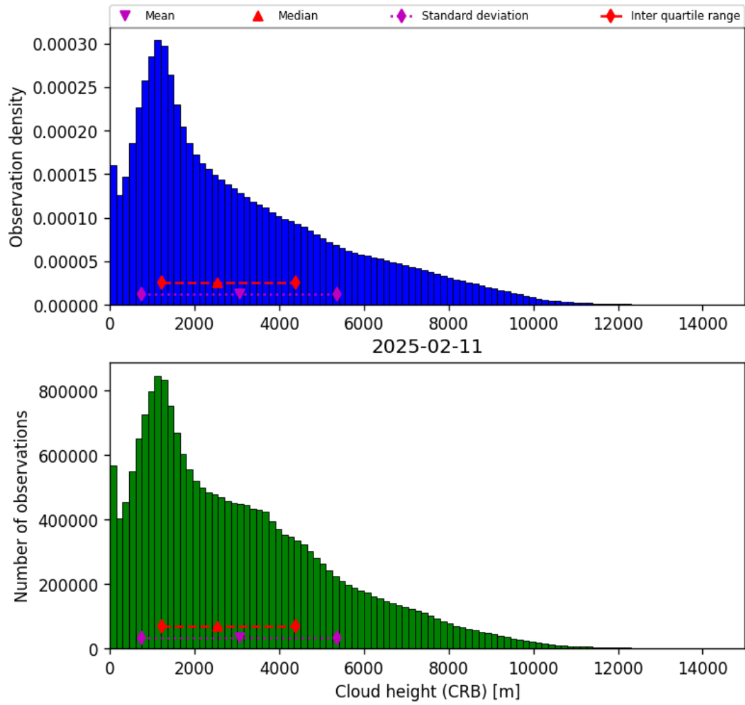
Figure 43: Histogram of “Cloud height (CRB)” for 2025-02-10 to 2025-02-12
