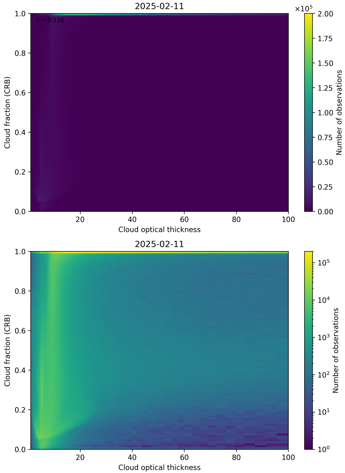
Figure 84: Scatter density plot of “Cloud optical thickness” against “Cloud fraction (CRB)” for 2025-02-10 to 2025-02-12.
