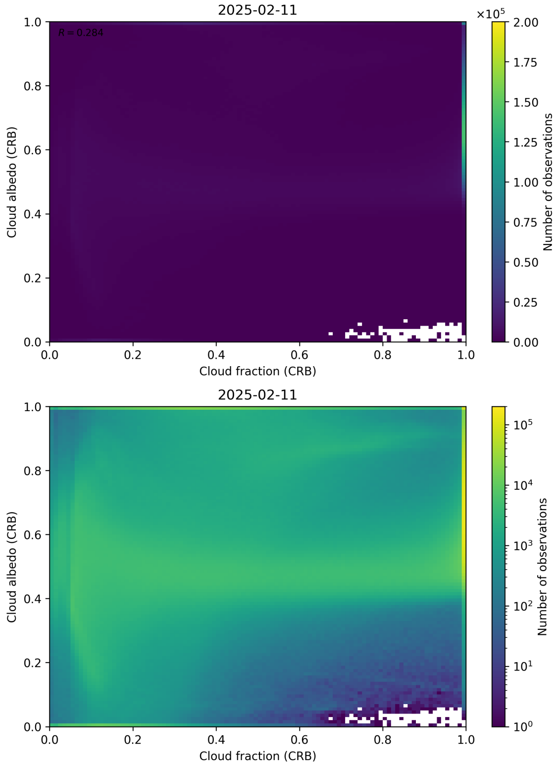
Figure 77: Scatter density plot of “Cloud fraction (CRB)” against “Cloud albedo (CRB)” for 2025-02-10 to 2025-02-12.
