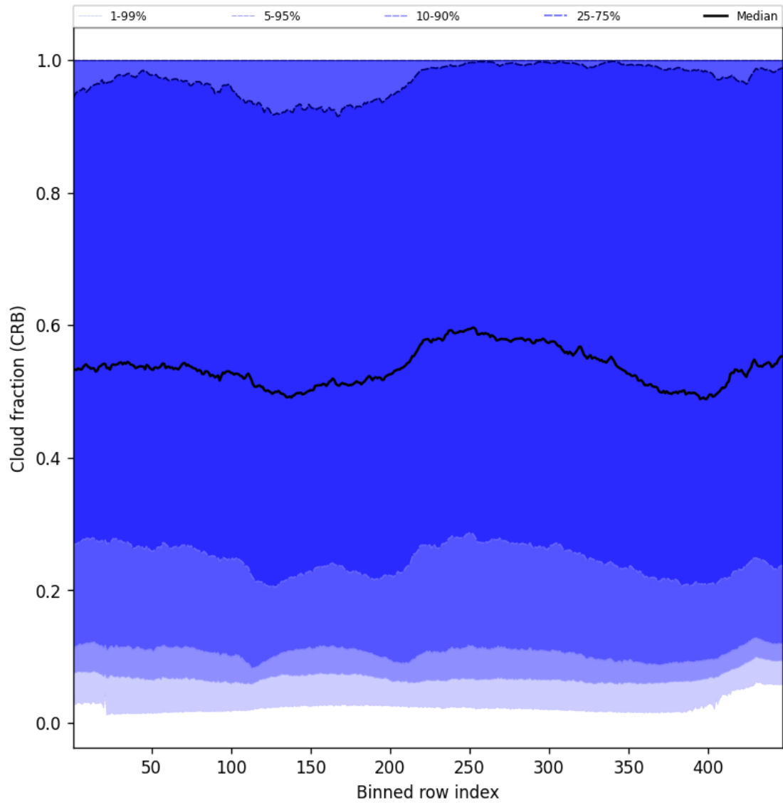
Figure 58: Along track statistics of “Cloud fraction (CRB)” for 2025-02-10 to 2025-02-12
