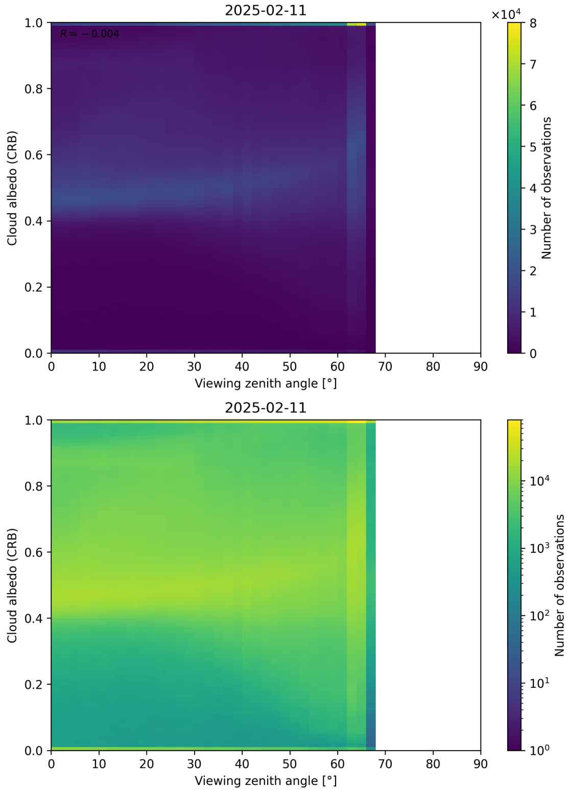
Figure 106: Scatter density plot of “Viewing zenith angle” against “Cloud albedo (CRB)” for 2025-02-10 to 2025-02-12.
