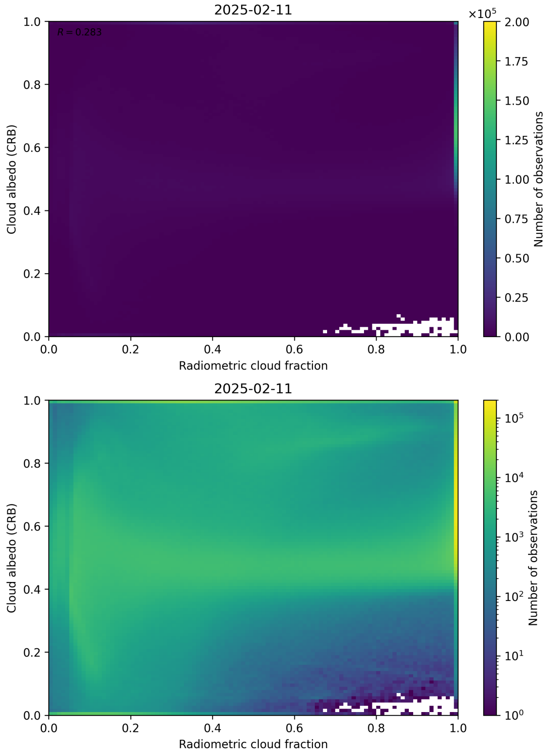
Figure 71: Scatter density plot of “Radiometric cloud fraction” against “Cloud albedo (CRB)” for 2025-02-10 to 2025-02-12.
