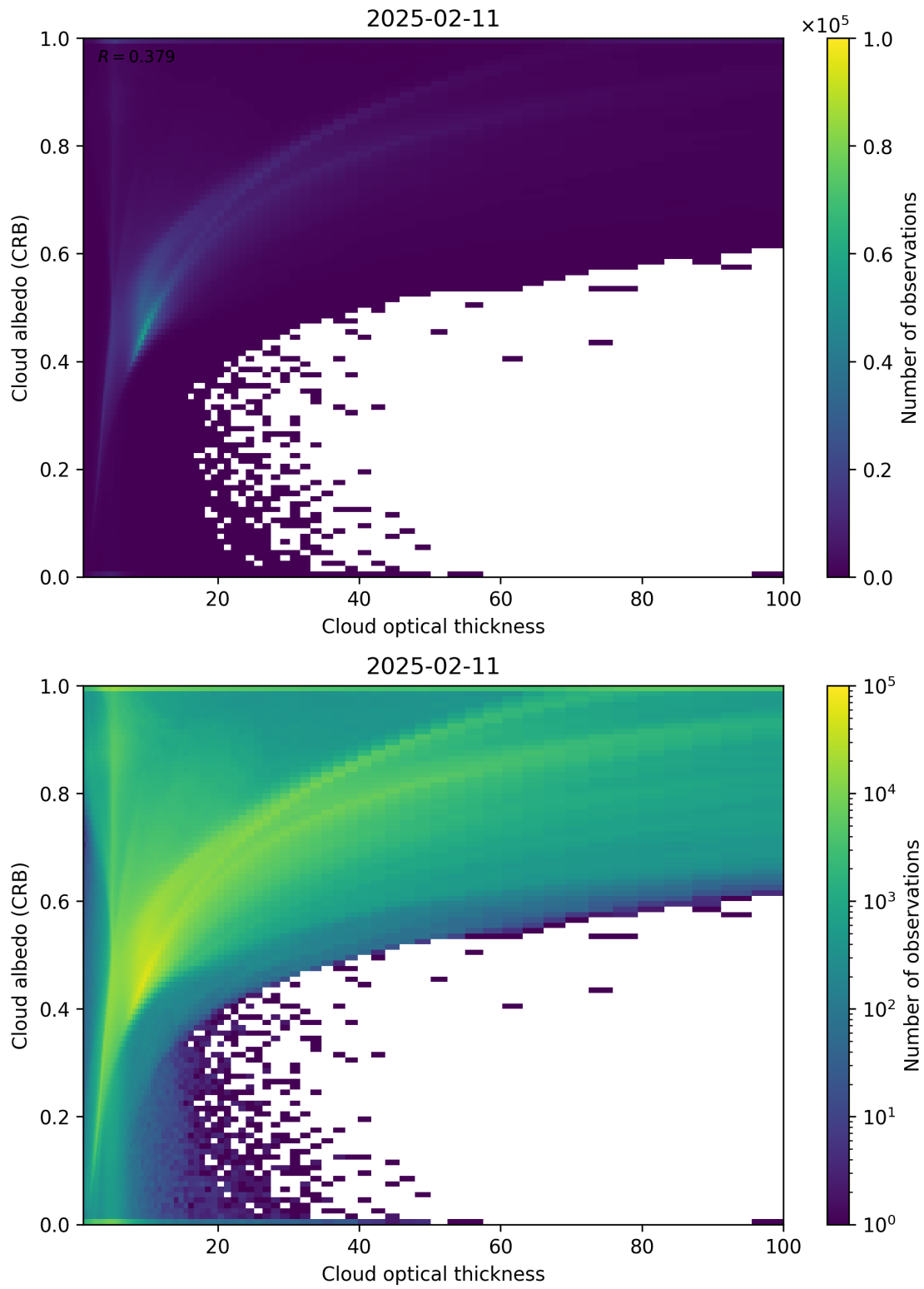
Figure 82: Scatter density plot of “Cloud optical thickness” against “Cloud albedo (CRB)” for 2025-02-10 to 2025-02-12.
