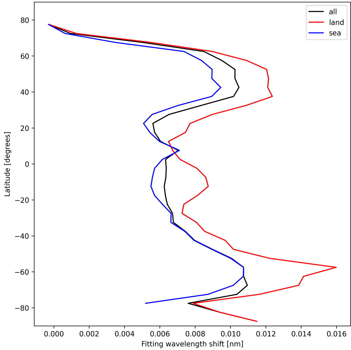
Figure 33: Zonal average of “Fitting wavelength shift” for 2025-02-10 to 2025-02-12.
