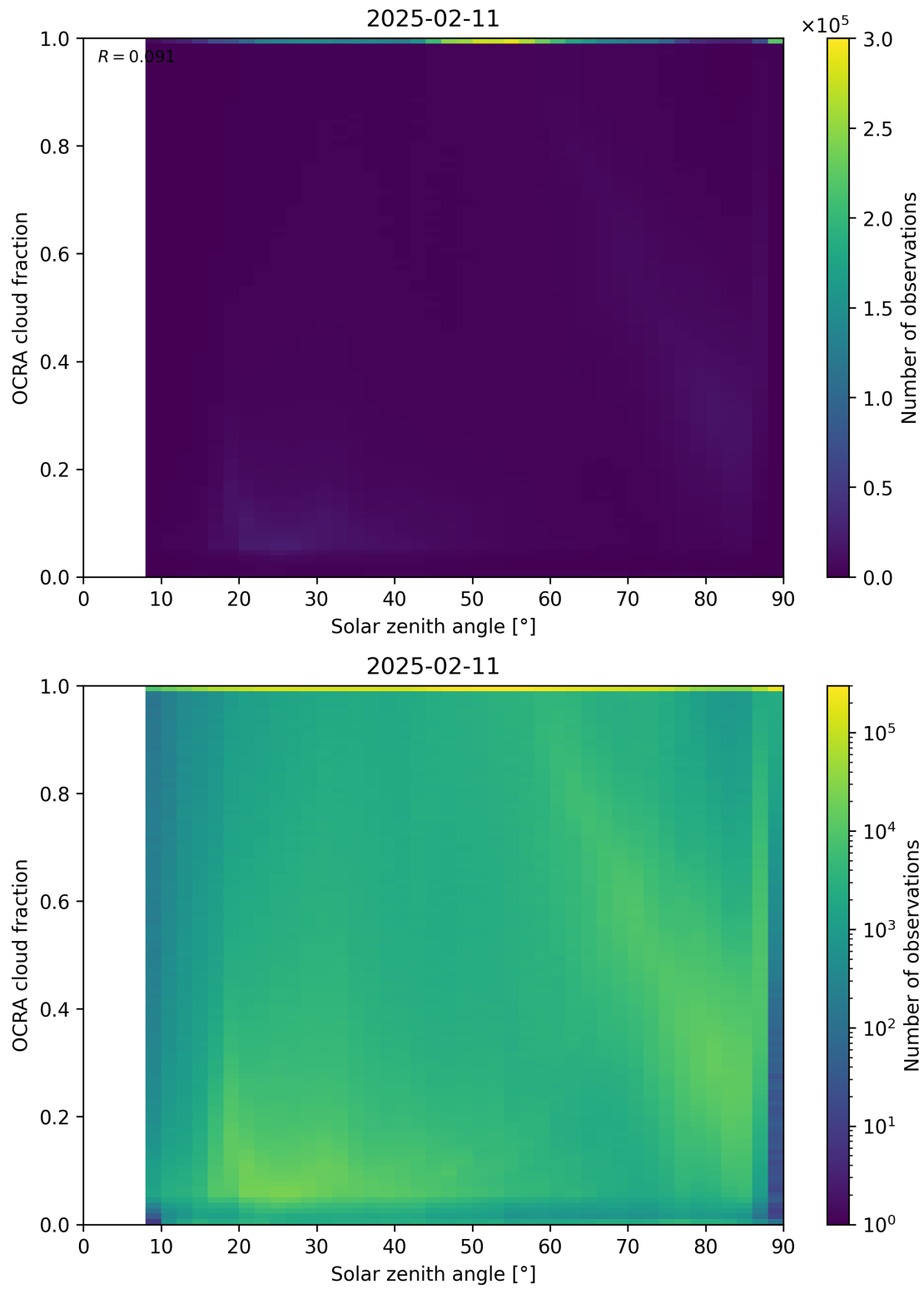
Figure 100: Scatter density plot of “Solar zenith angle” against “OCRA cloud fraction” for 2025-02-10 to 2025-02-12.
