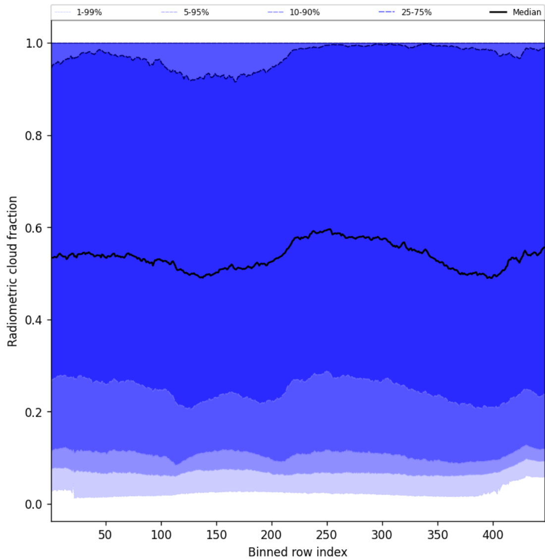
Figure 55: Along track statistics of “Radiometric cloud fraction” for 2025-02-10 to 2025-02-12
