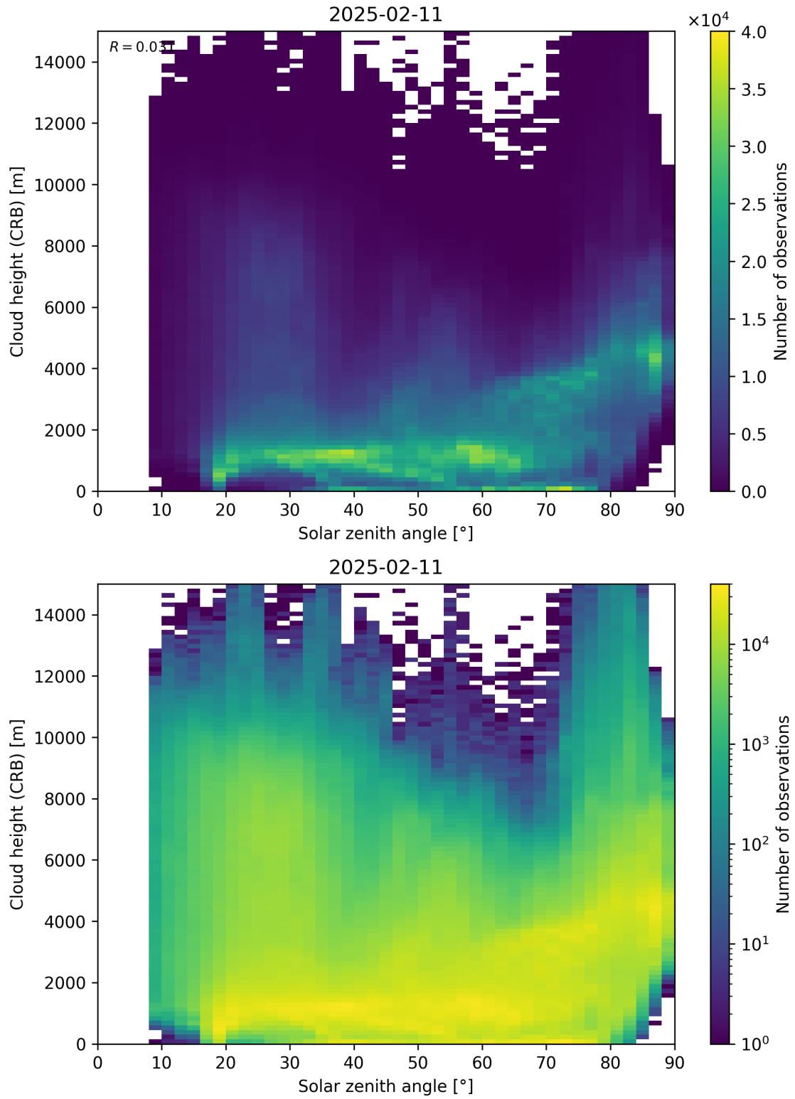
Figure 102: Scatter density plot of “Solar zenith angle” against “Cloud height (CRB)” for 2025-02-10 to 2025-02-12.
