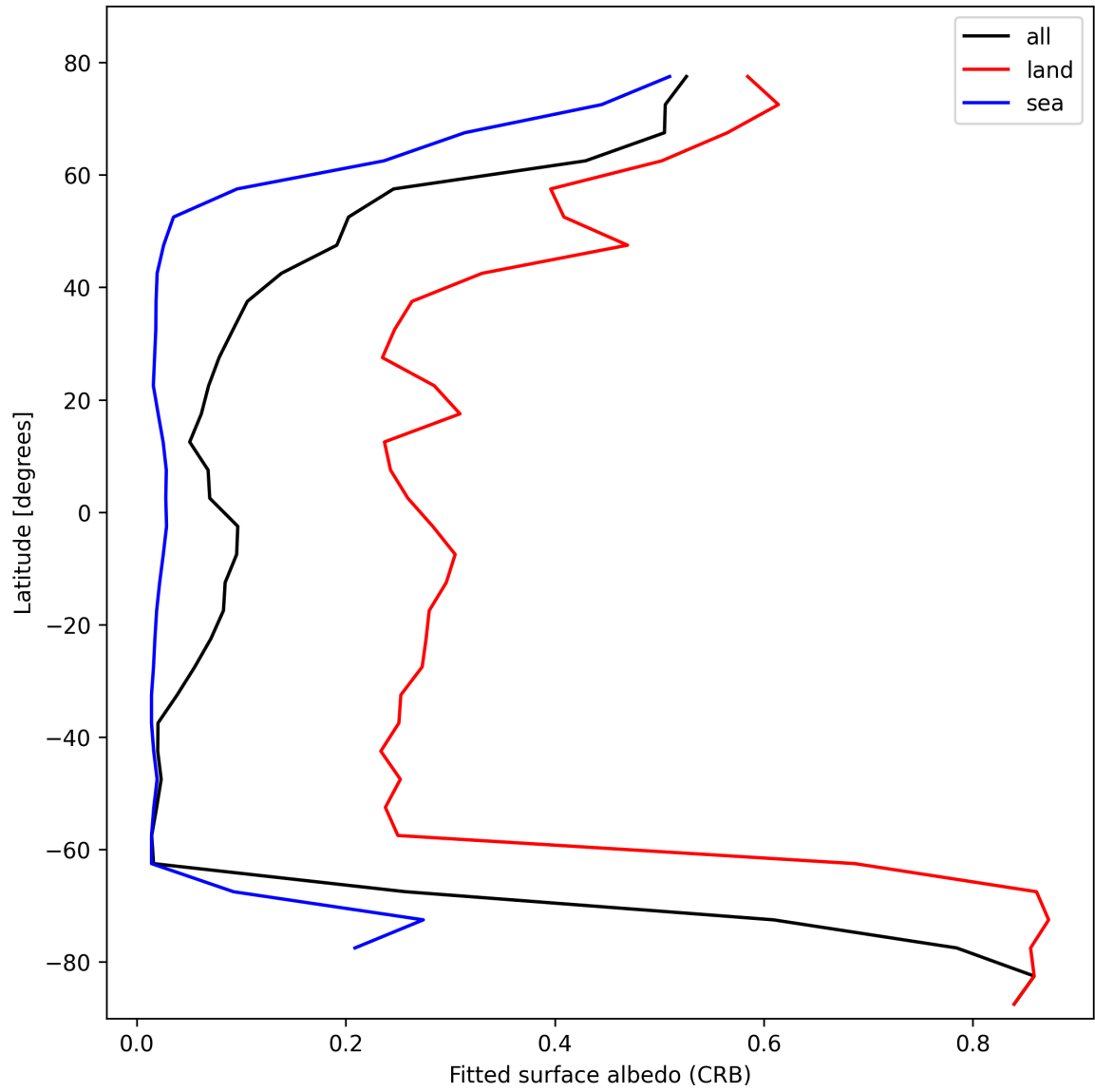
Figure 30: Zonal average of “Fitted surface albedo (CRB)” for 2025-02-10 to 2025-02-12.
