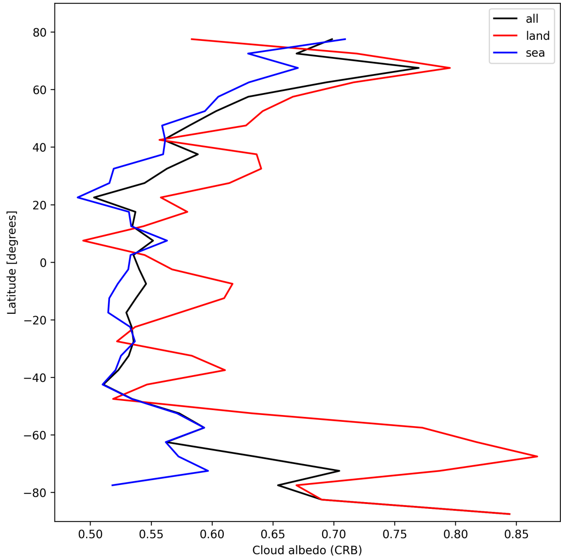
Figure 28: Zonal average of “Cloud albedo (CRB)” for 2025-02-10 to 2025-02-12.
