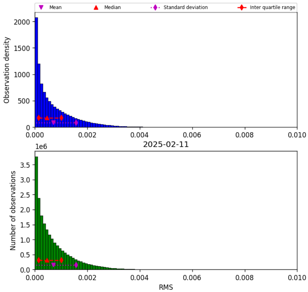
Figure 47: Histogram of “RMS” for 2025-02-10 to 2025-02-12
