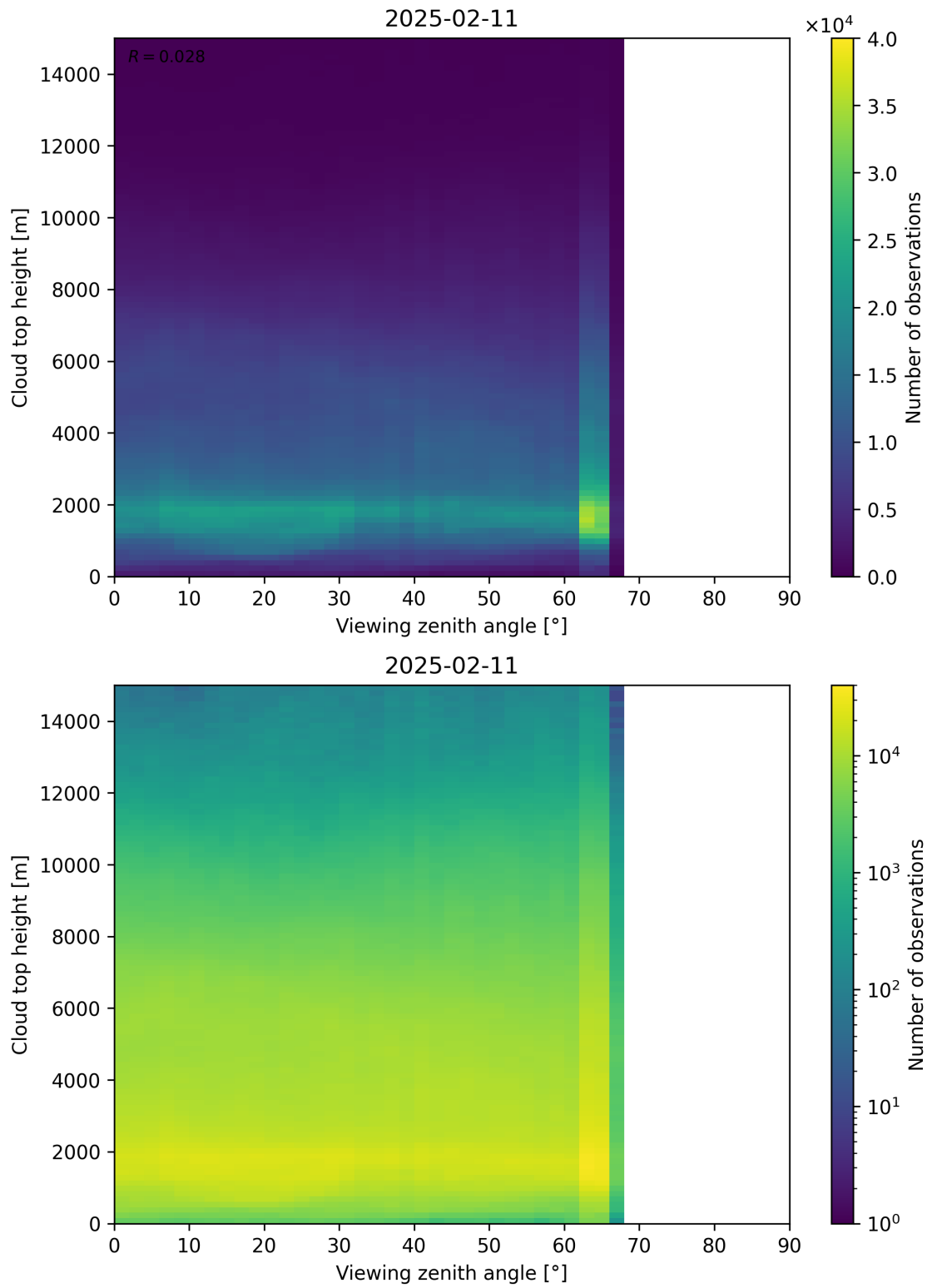
Figure 112: Scatter density plot of “Viewing zenith angle” against “Cloud top height” for 2025-02-10 to 2025-02-12.
