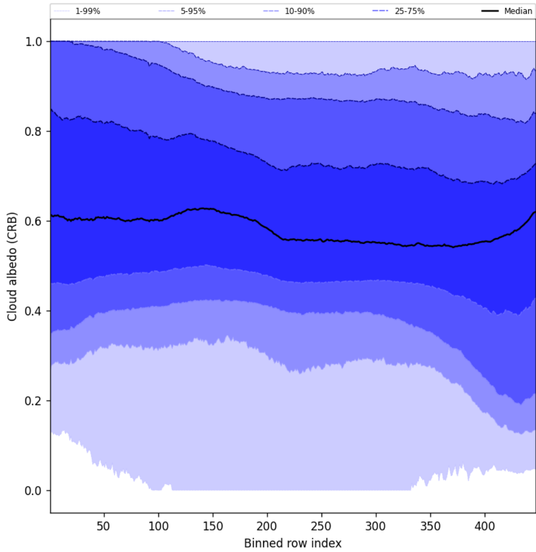
Figure 60: Along track statistics of “Cloud albedo (CRB)” for 2025-02-10 to 2025-02-12
