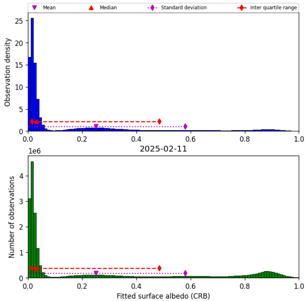
Figure 46: Histogram of “Fitted surface albedo (CRB)” for 2025-02-10 to 2025-02-12
