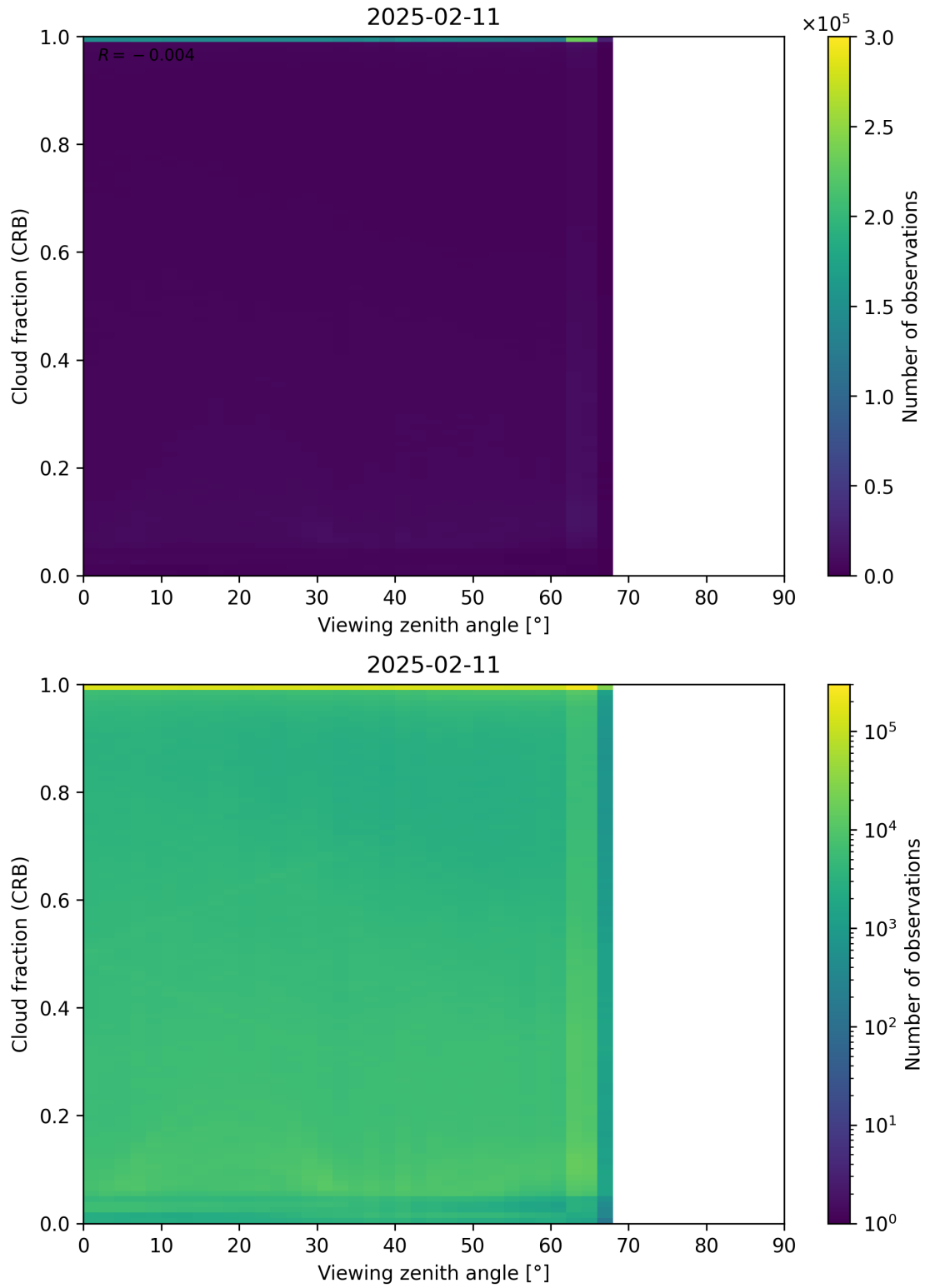
Figure 109: Scatter density plot of “Viewing zenith angle” against “Cloud fraction (CRB)” for 2025-02-10 to 2025-02-12.
