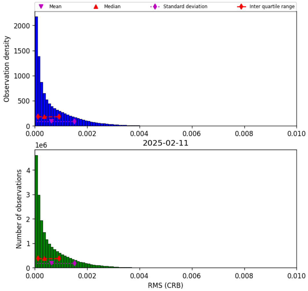
Figure 48: Histogram of “RMS (CRB)” for 2025-02-10 to 2025-02-12
