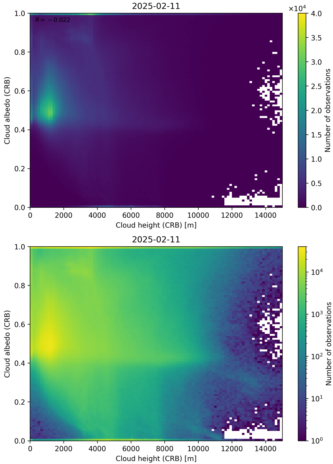
Figure 80: Scatter density plot of “Cloud height (CRB)” against “Cloud albedo (CRB)” for 2025-02-10 to 2025-02-12.
