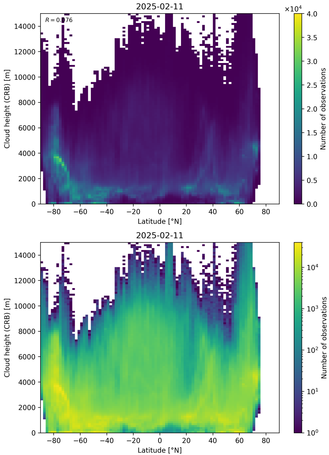
Figure 95: Scatter density plot of “Latitude” against “Cloud height (CRB)” for 2025-02-10 to 2025-02-12.
