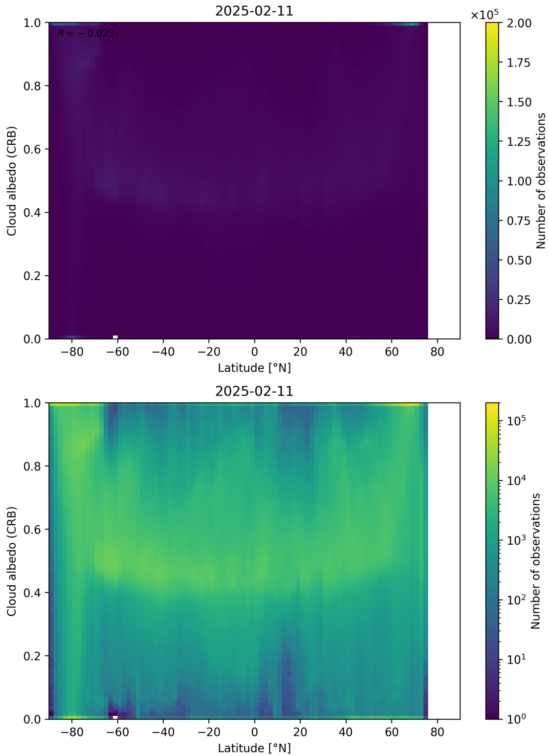
Figure 91: Scatter density plot of “Latitude” against “Cloud albedo (CRB)” for 2025-02-10 to 2025-02-12.
