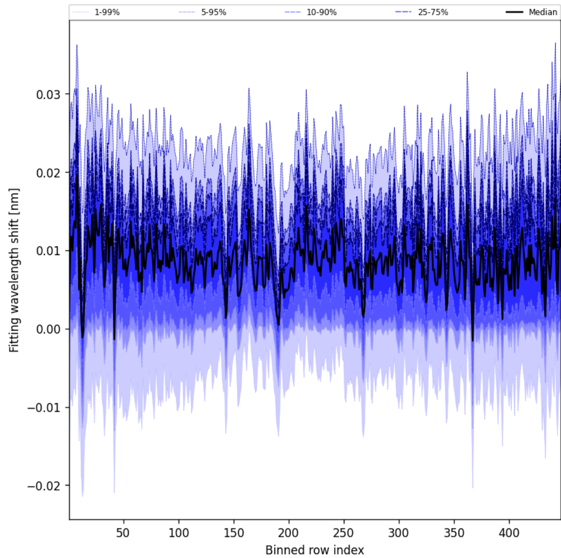
Figure 65: Along track statistics of “Fitting wavelength shift” for 2025-02-10 to 2025-02-12
