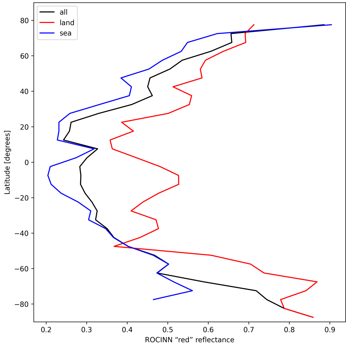
Figure 37: Zonal average of “ROCINN “red” reflectance” for 2025-02-10 to 2025-02-12.
