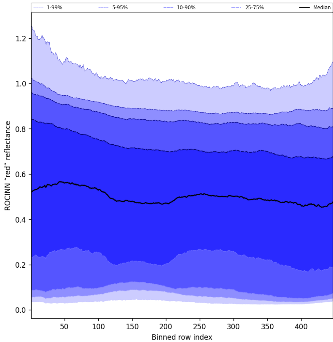
Figure 69: Along track statistics of “ROCINN “red” reflectance” for 2025-02-10 to 2025-02-12
