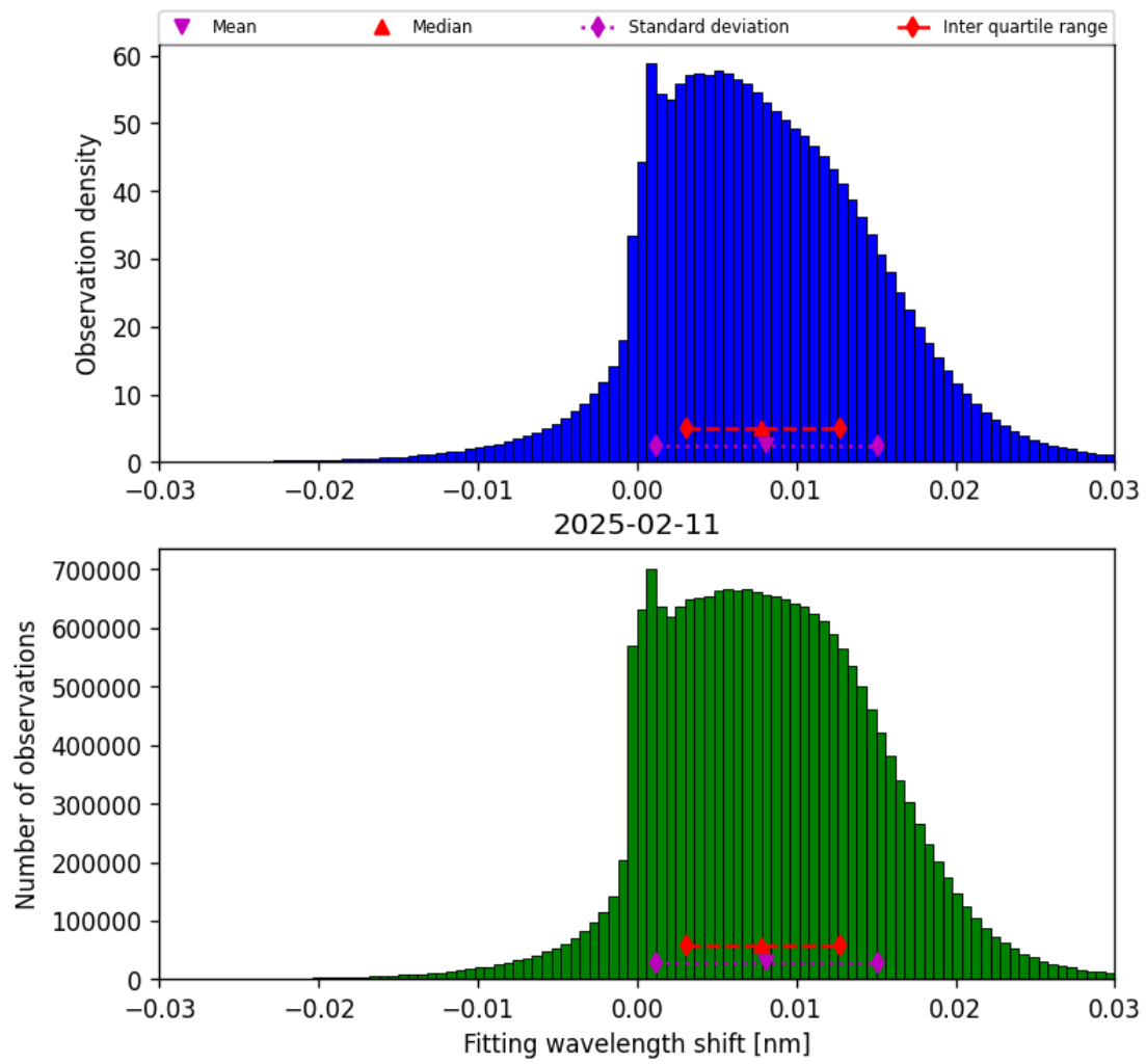
Figure 49: Histogram of “Fitting wavelength shift” for 2025-02-10 to 2025-02-12
