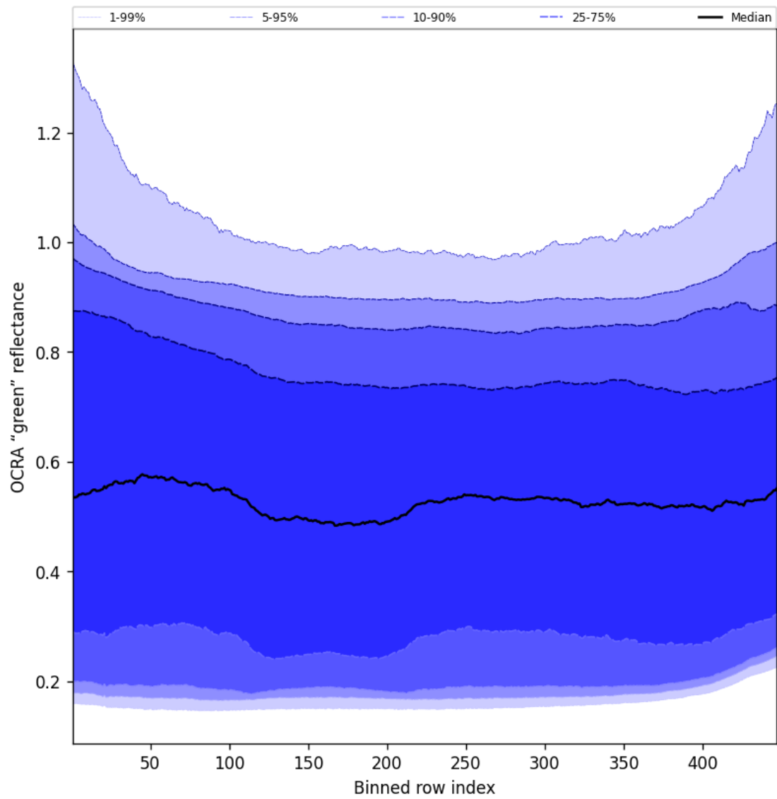
Figure 68: Along track statistics of "OCRA "green" reflectance" for 2025-02-10 to 2025-02-12
