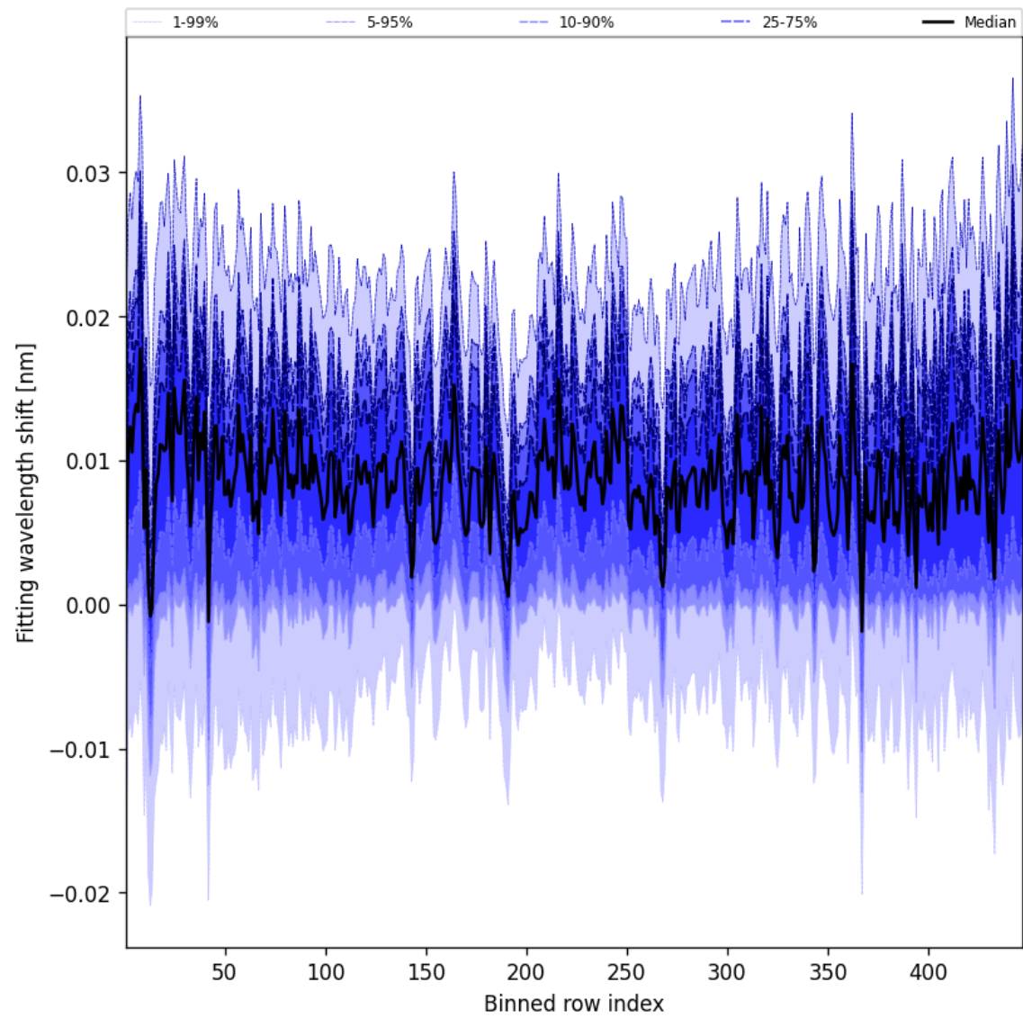
Figure 65: Along track statistics of “Fitting wavelength shift” for 2025-02-11 to 2025-02-13
