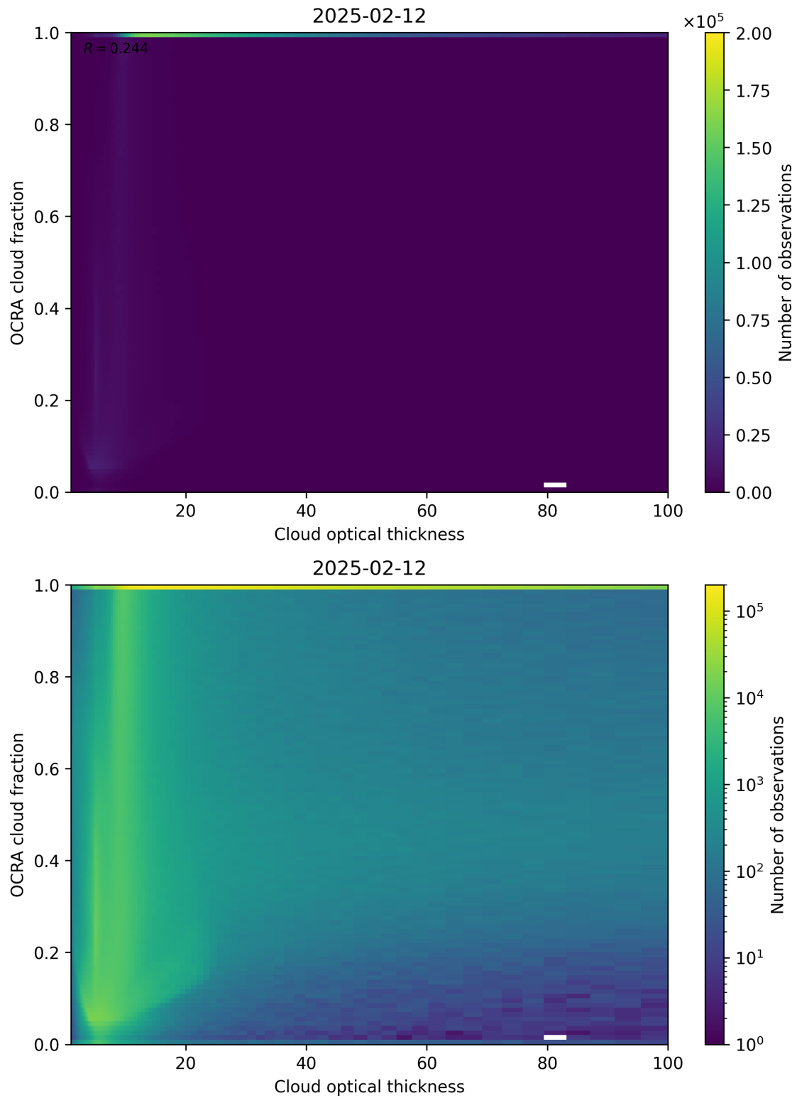
Figure 83: Scatter density plot of “Cloud optical thickness” against “OCRA cloud fraction” for 2025-02-11 to 2025-02-13.
