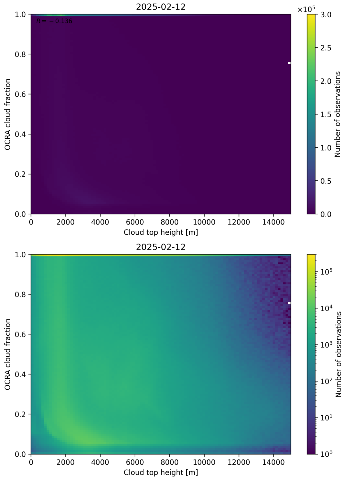
Figure 87: Scatter density plot of “Cloud top height” against “OCRA cloud fraction” for 2025-02-11 to 2025-02-13.
