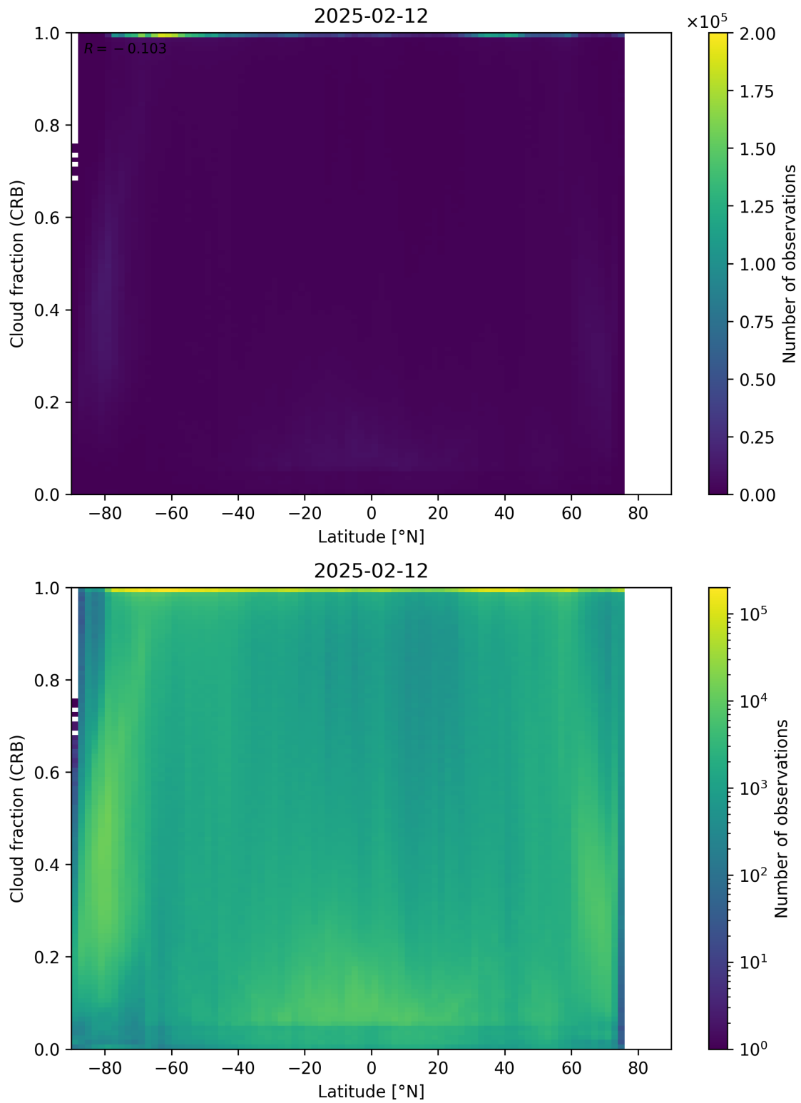
Figure 94: Scatter density plot of “Latitude” against “Cloud fraction (CRB)” for 2025-02-11 to 2025-02-13.
