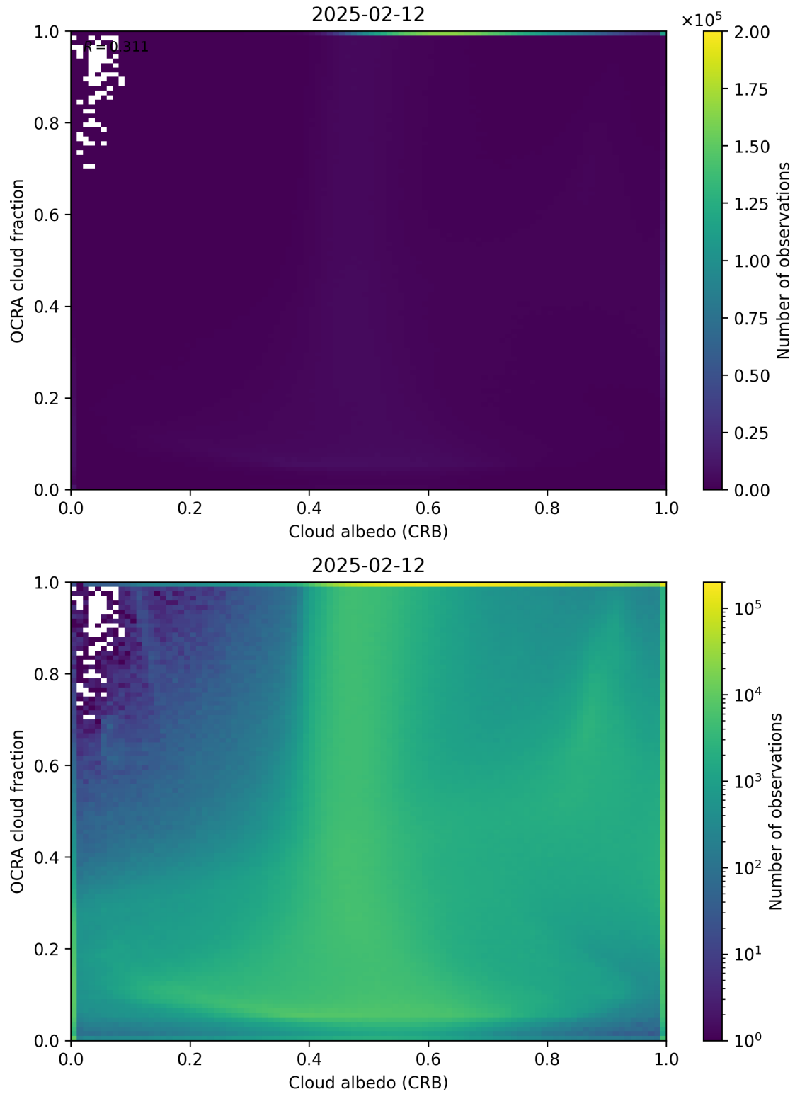
Figure 70: Scatter density plot of “Cloud albedo (CRB)” against “OCRA cloud fraction” for 2025-02-11 to 2025-02-13.
