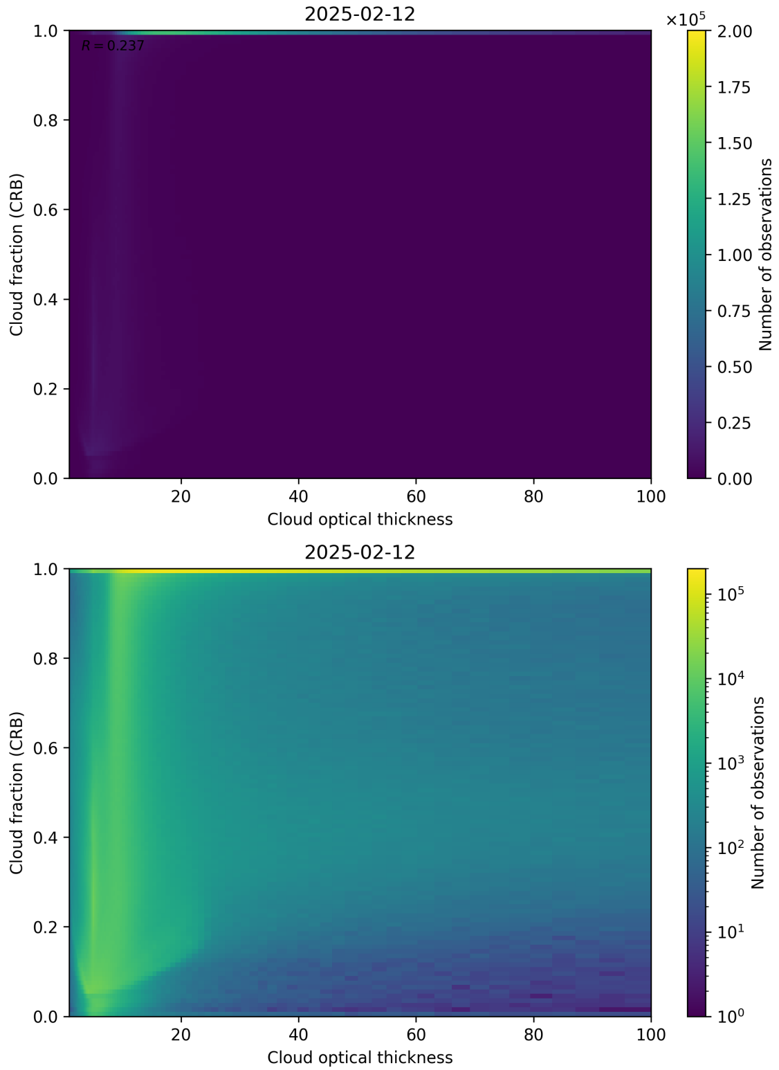
Figure 84: Scatter density plot of “Cloud optical thickness” against “Cloud fraction (CRB)” for 2025-02-11 to 2025-02-13.
