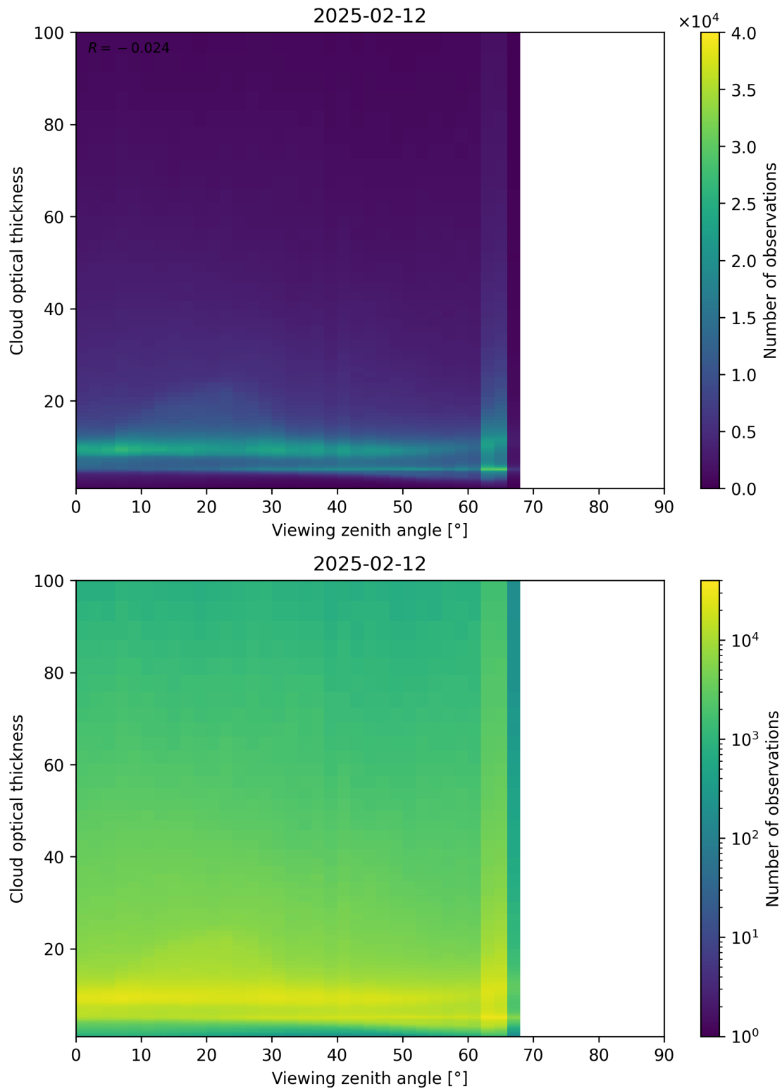
Figure 111: Scatter density plot of “Viewing zenith angle” against “Cloud optical thickness” for 2025-02-11 to 2025-02-13.
