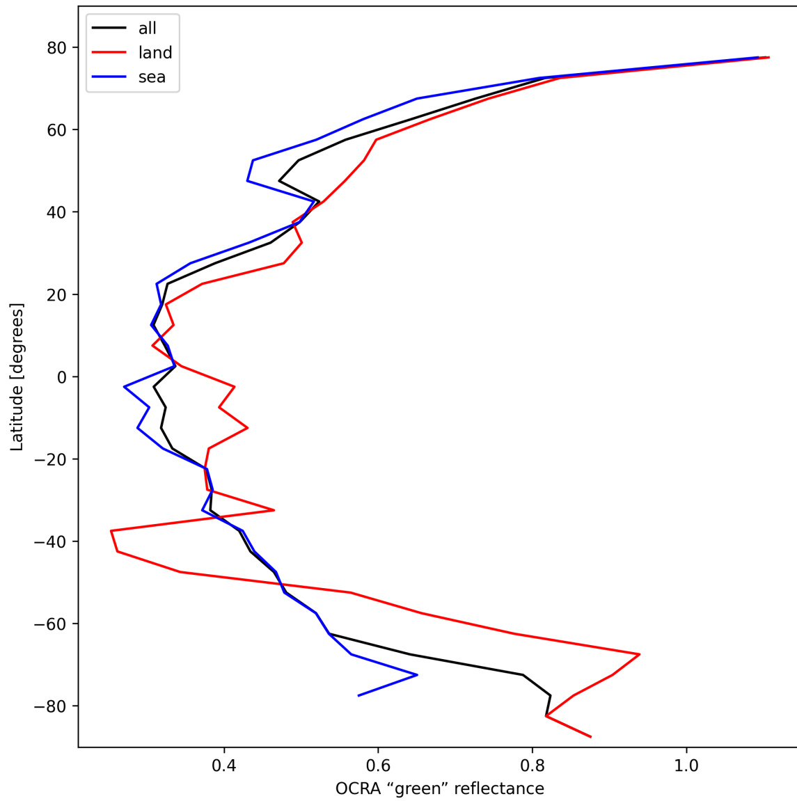
Figure 36: Zonal average of “OCRA “green” reflectance” for 2025-02-11 to 2025-02-13.
