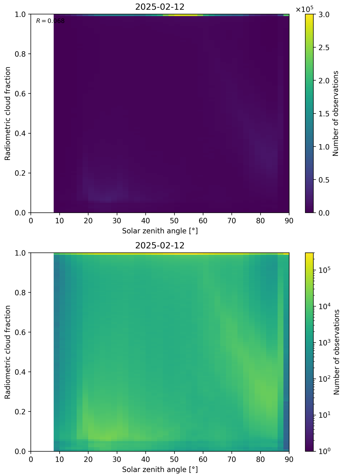
Figure 99: Scatter density plot of “Solar zenith angle” against “Radiometric cloud fraction” for 2025-02-11 to 2025-02-13.
