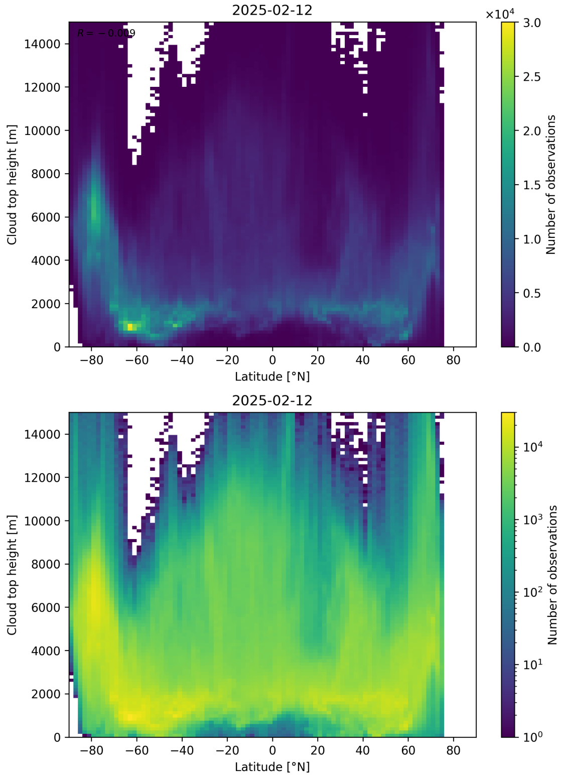
Figure 97: Scatter density plot of “Latitude” against “Cloud top height” for 2025-02-11 to 2025-02-13.
