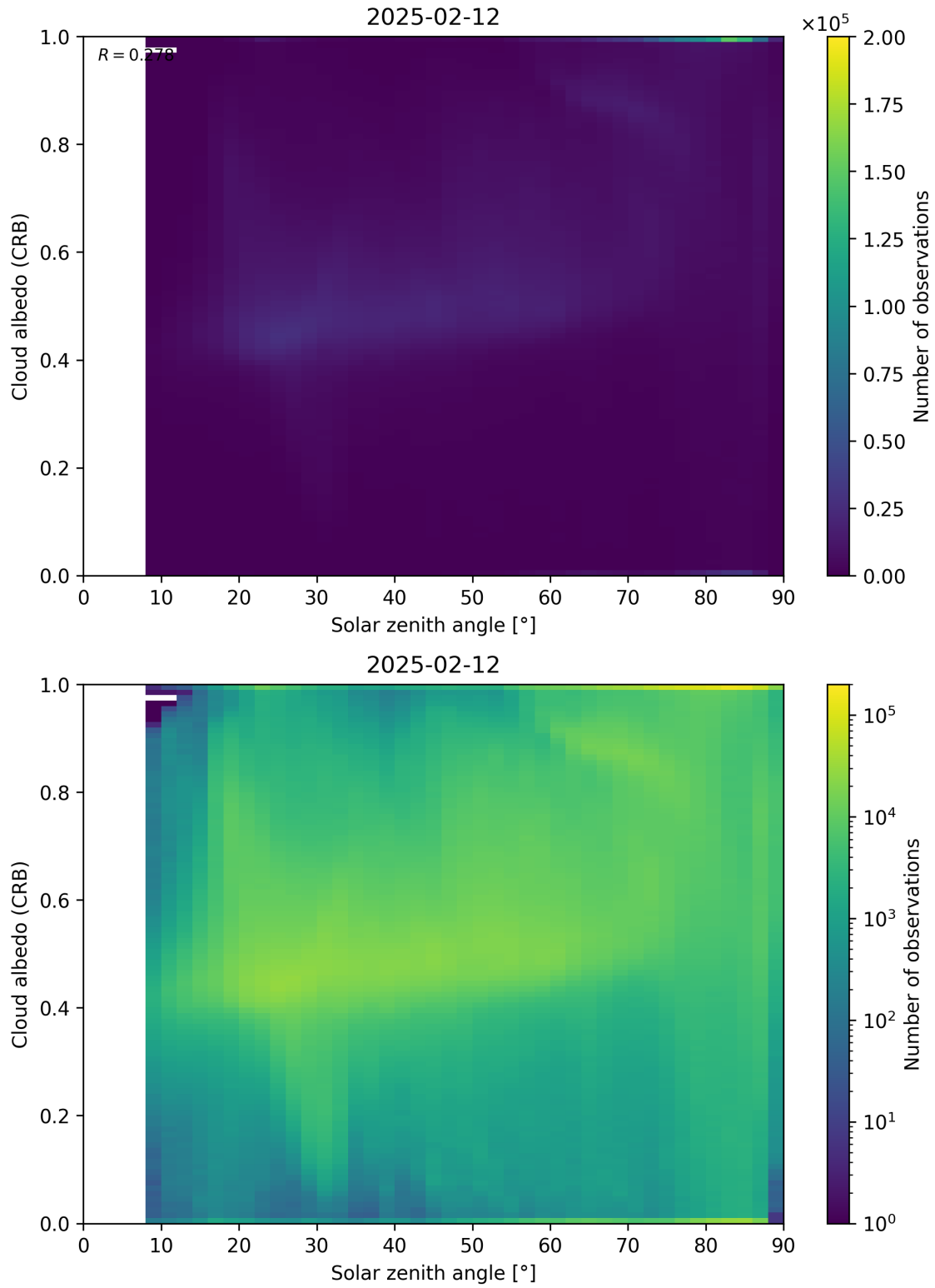
Figure 98: Scatter density plot of “Solar zenith angle” against “Cloud albedo (CRB)” for 2025-02-11 to 2025-02-13.
