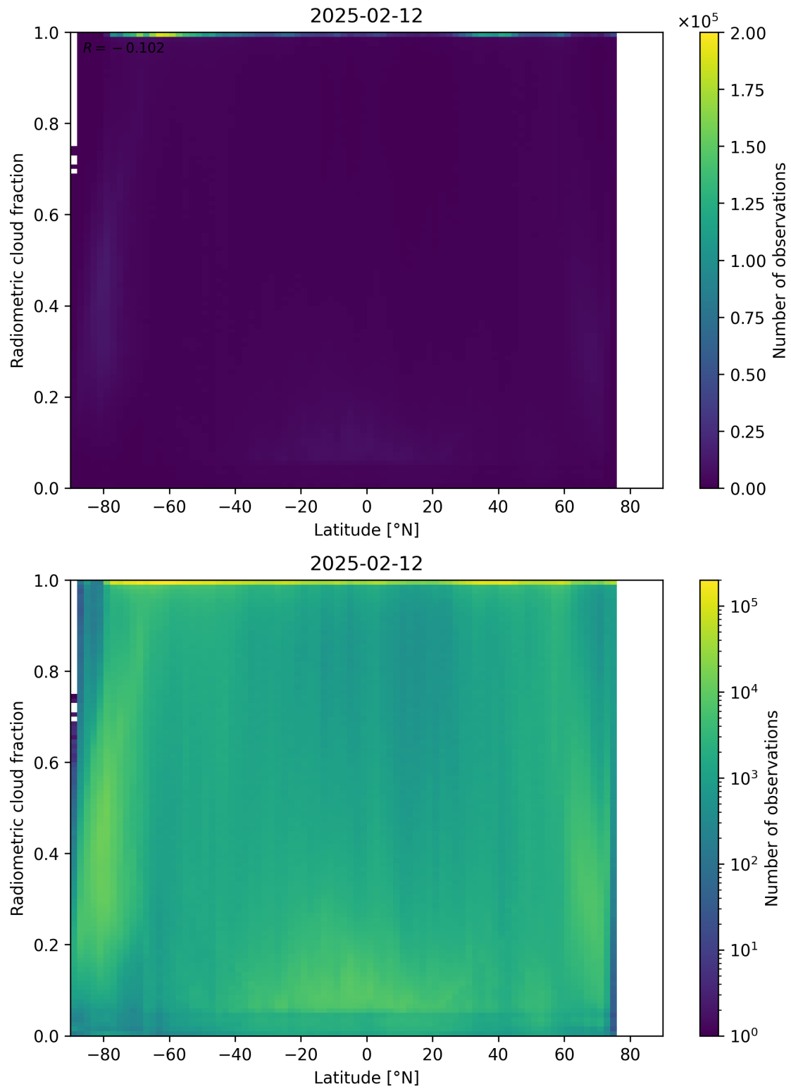
Figure 92: Scatter density plot of “Latitude” against “Radiometric cloud fraction” for 2025-02-11 to 2025-02-13.
