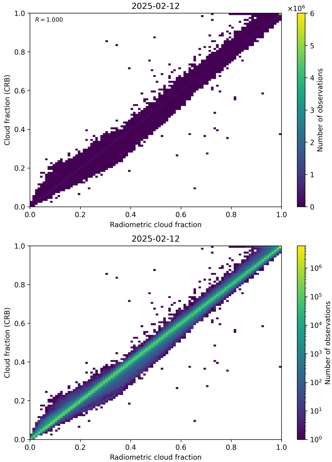
Figure 73: Scatter density plot of “Radiometric cloud fraction” against “Cloud fraction (CRB)” for 2025-02-11 to 2025-02-13.
