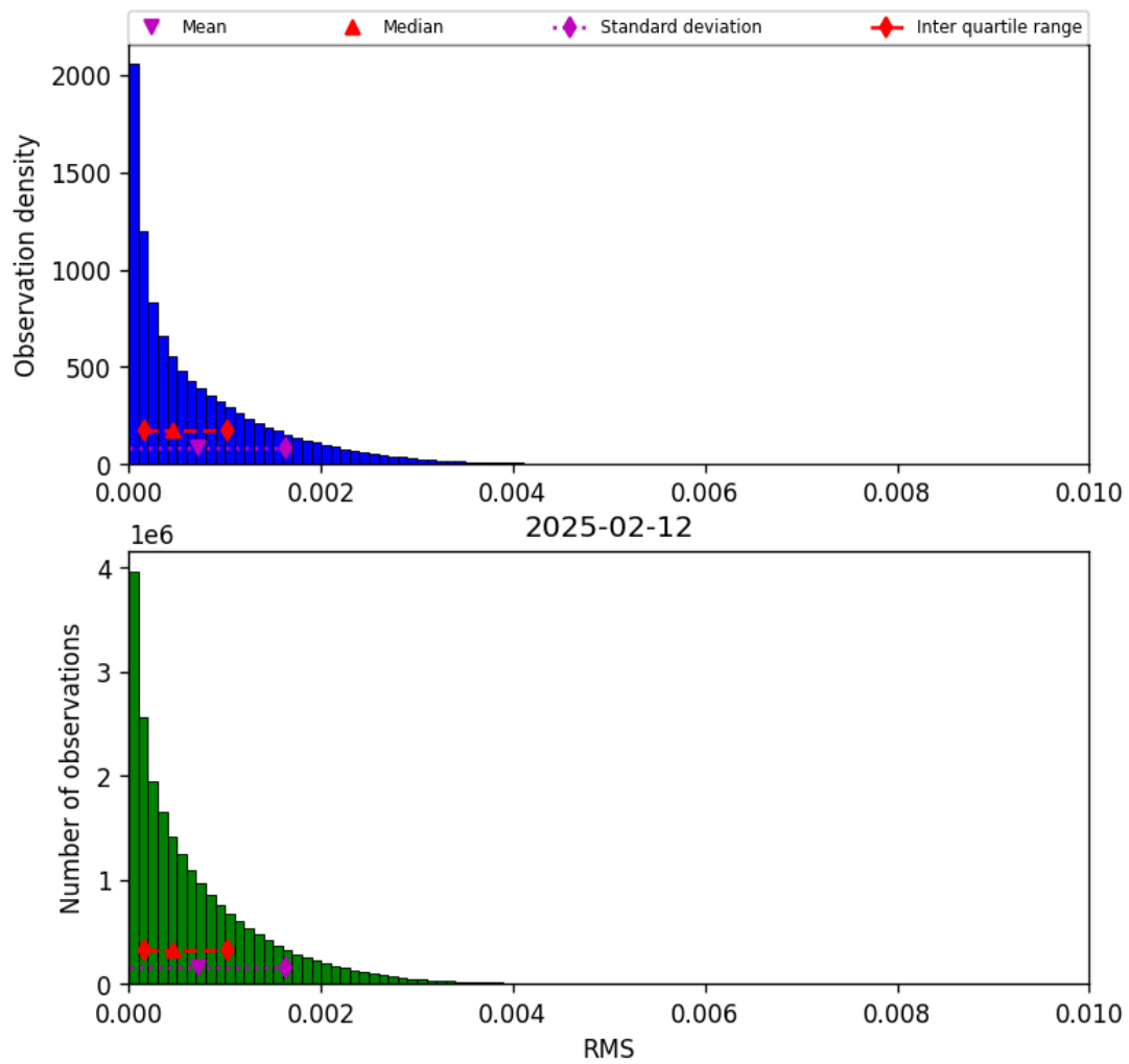
Figure 47: Histogram of “RMS” for 2025-02-11 to 2025-02-13
