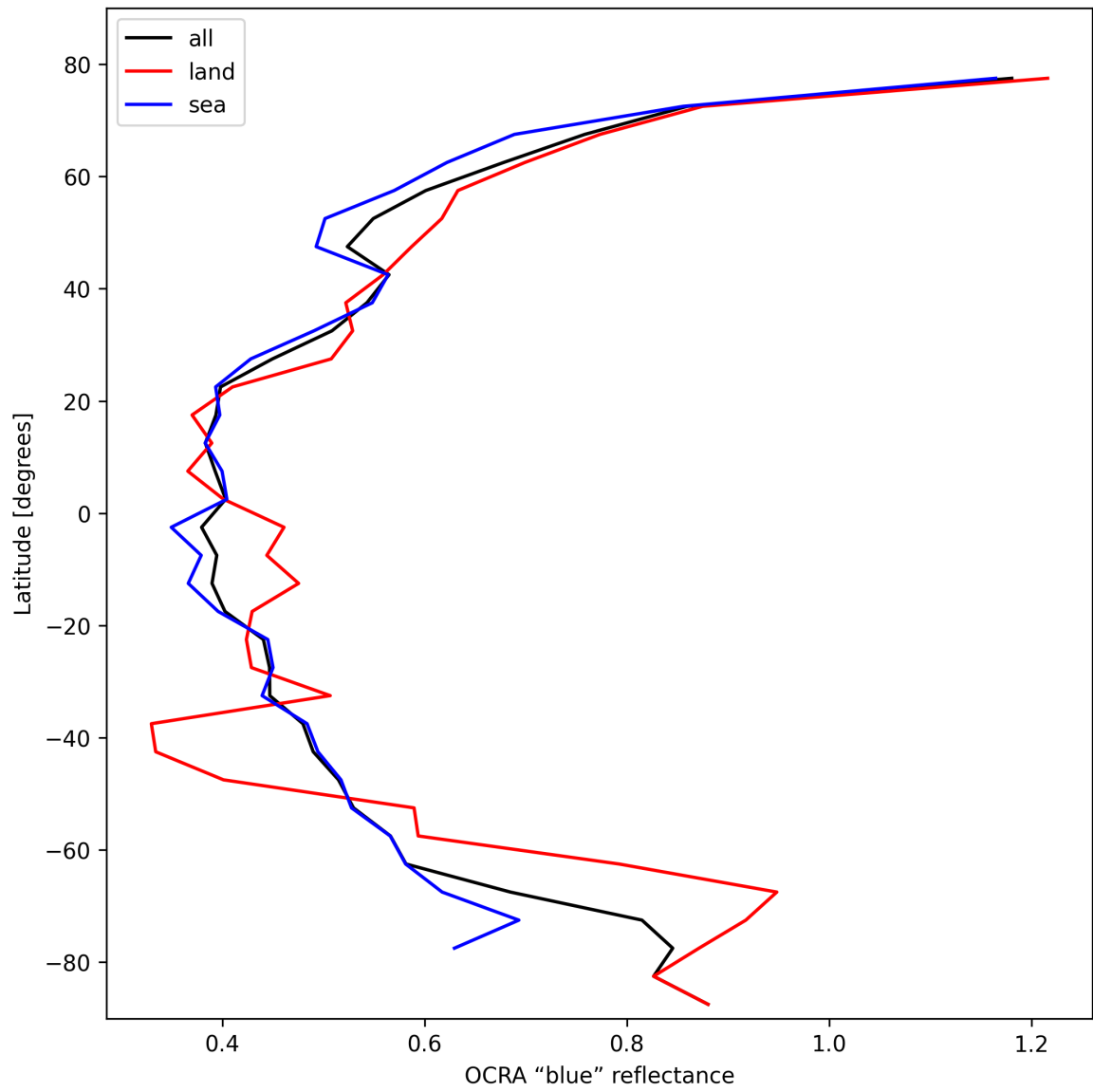
Figure 35: Zonal average of "OCRA "blue" reflectance" for 2025-02-11 to 2025-02-13.
