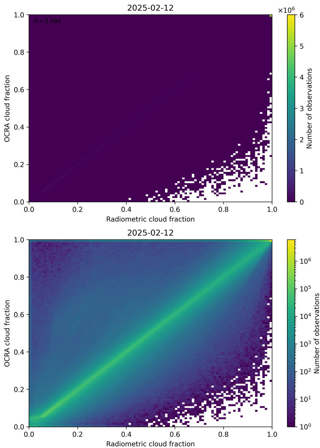
Figure 72: Scatter density plot of “Radiometric cloud fraction” against “OCRA cloud fraction” for 2025-02-11 to 2025-02-13.
