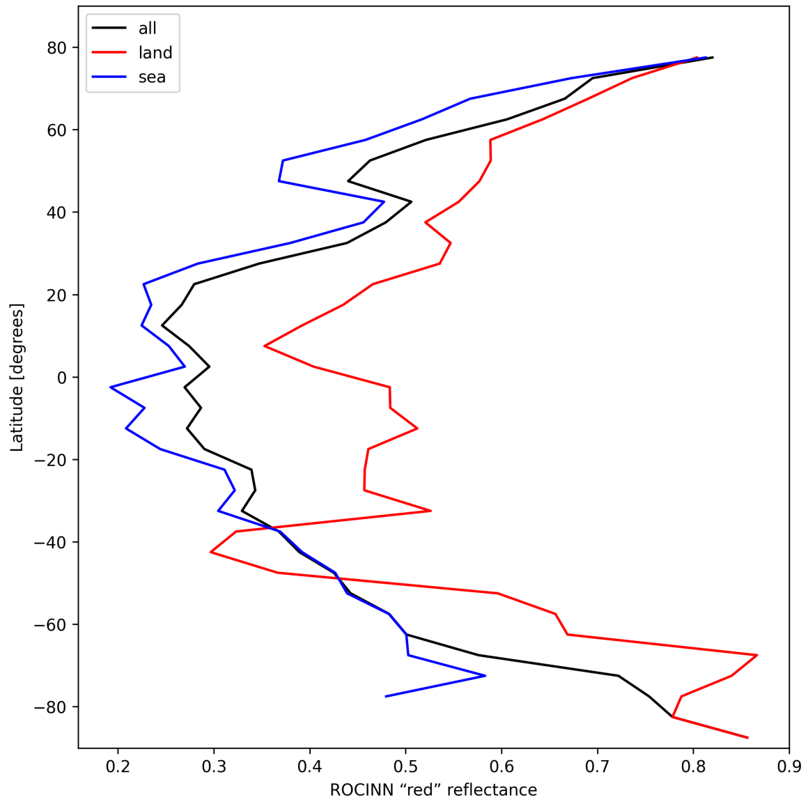
Figure 37: Zonal average of “ROCINN “red” reflectance” for 2025-02-11 to 2025-02-13.
