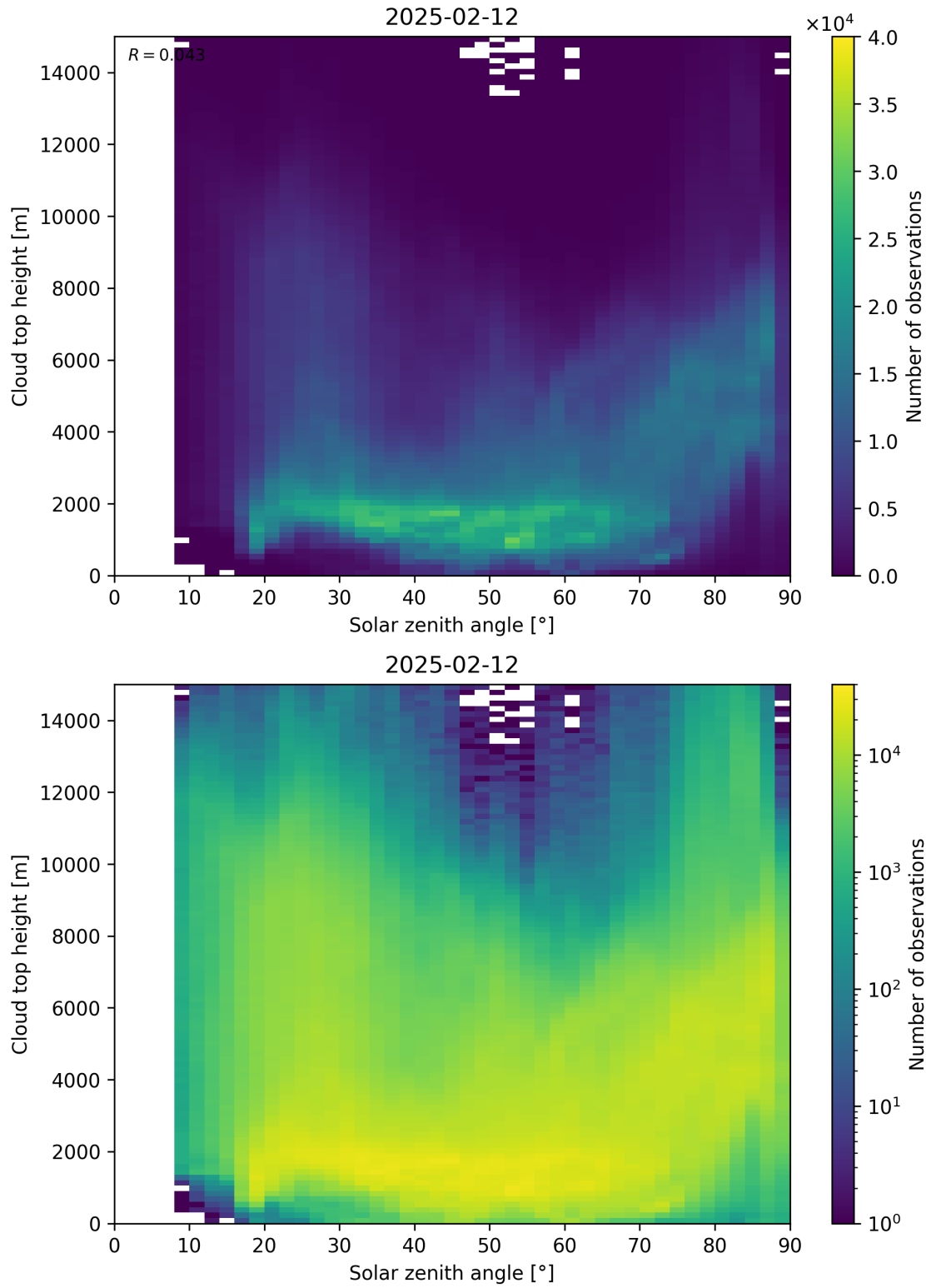
Figure 104: Scatter density plot of “Solar zenith angle” against “Cloud top height” for 2025-02-11 to 2025-02-13.
