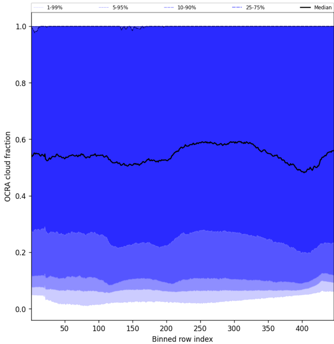
Figure 66: Along track statistics of “OCRA cloud fraction” for 2025-02-11 to 2025-02-13
