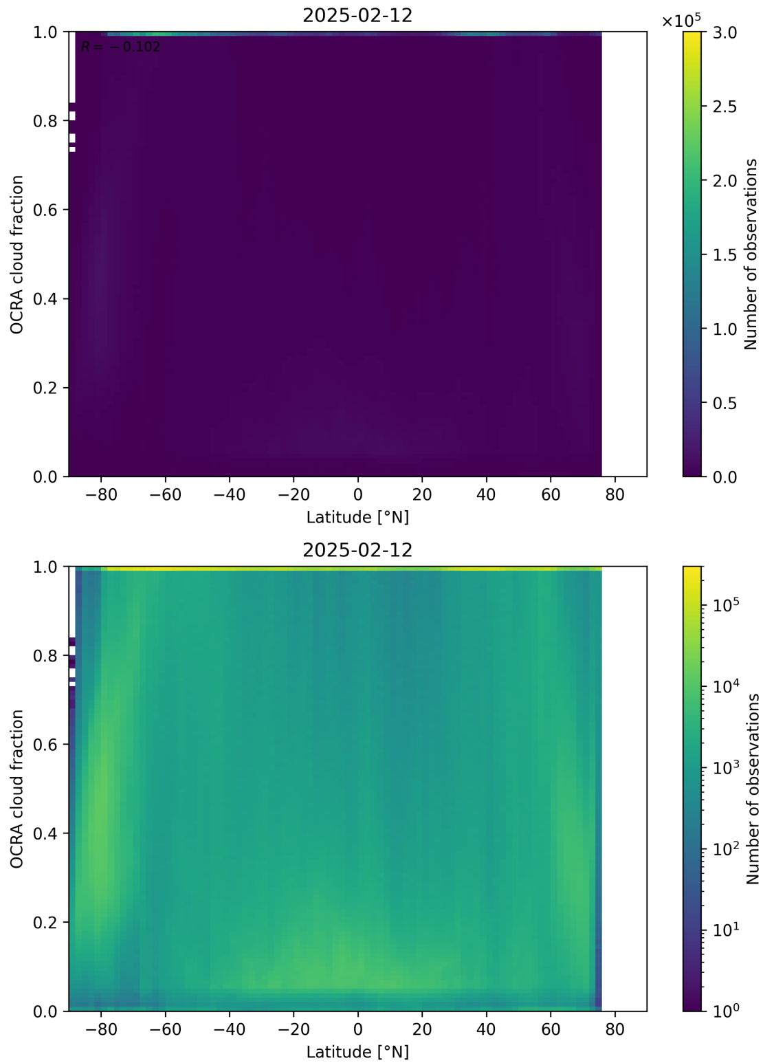
Figure 93: Scatter density plot of “Latitude” against “OCRA cloud fraction” for 2025-02-11 to 2025-02-13.
