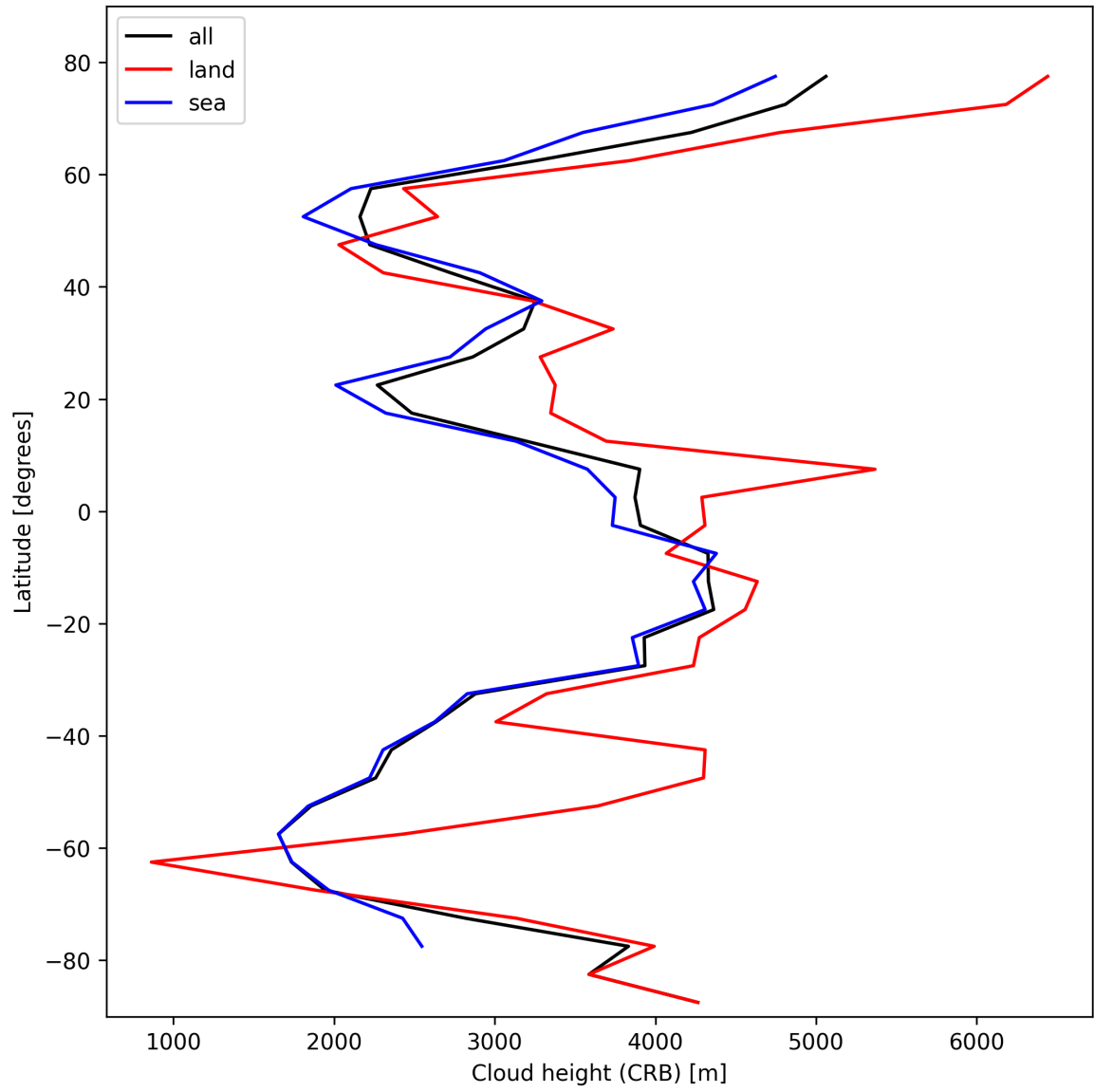
Figure 27: Zonal average of “Cloud height (CRB)” for 2025-02-11 to 2025-02-13.
