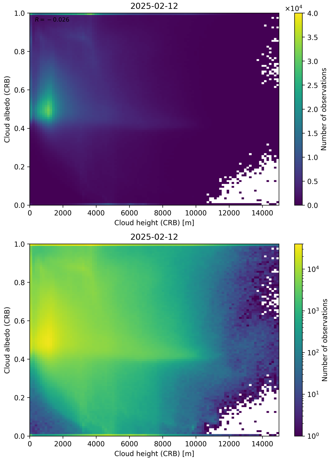
Figure 80: Scatter density plot of “Cloud height (CRB)” against “Cloud albedo (CRB)” for 2025-02-11 to 2025-02-13.
