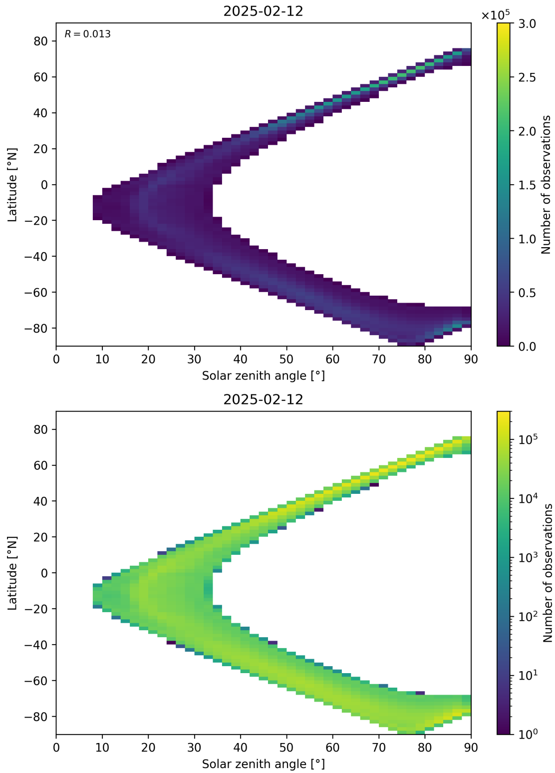
Figure 105: Scatter density plot of “Solar zenith angle” against “Latitude” for 2025-02-11 to 2025-02-13.
