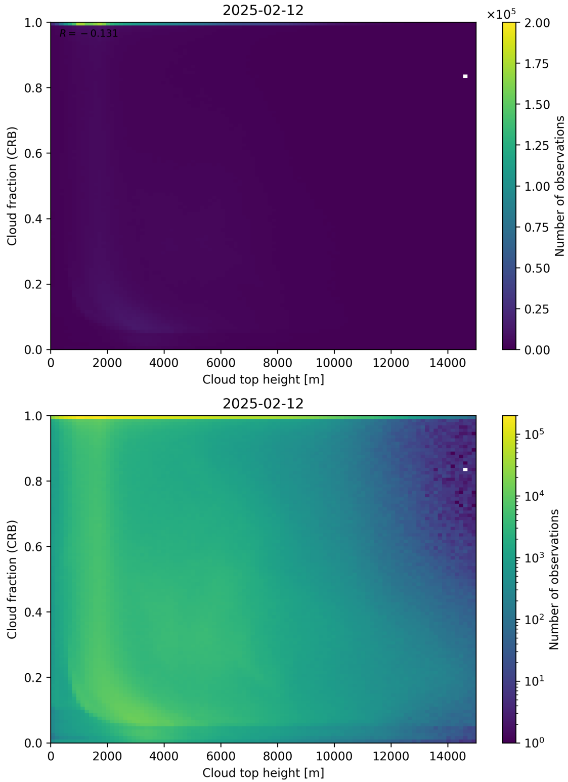
Figure 88: Scatter density plot of “Cloud top height” against “Cloud fraction (CRB)” for 2025-02-11 to 2025-02-13.
