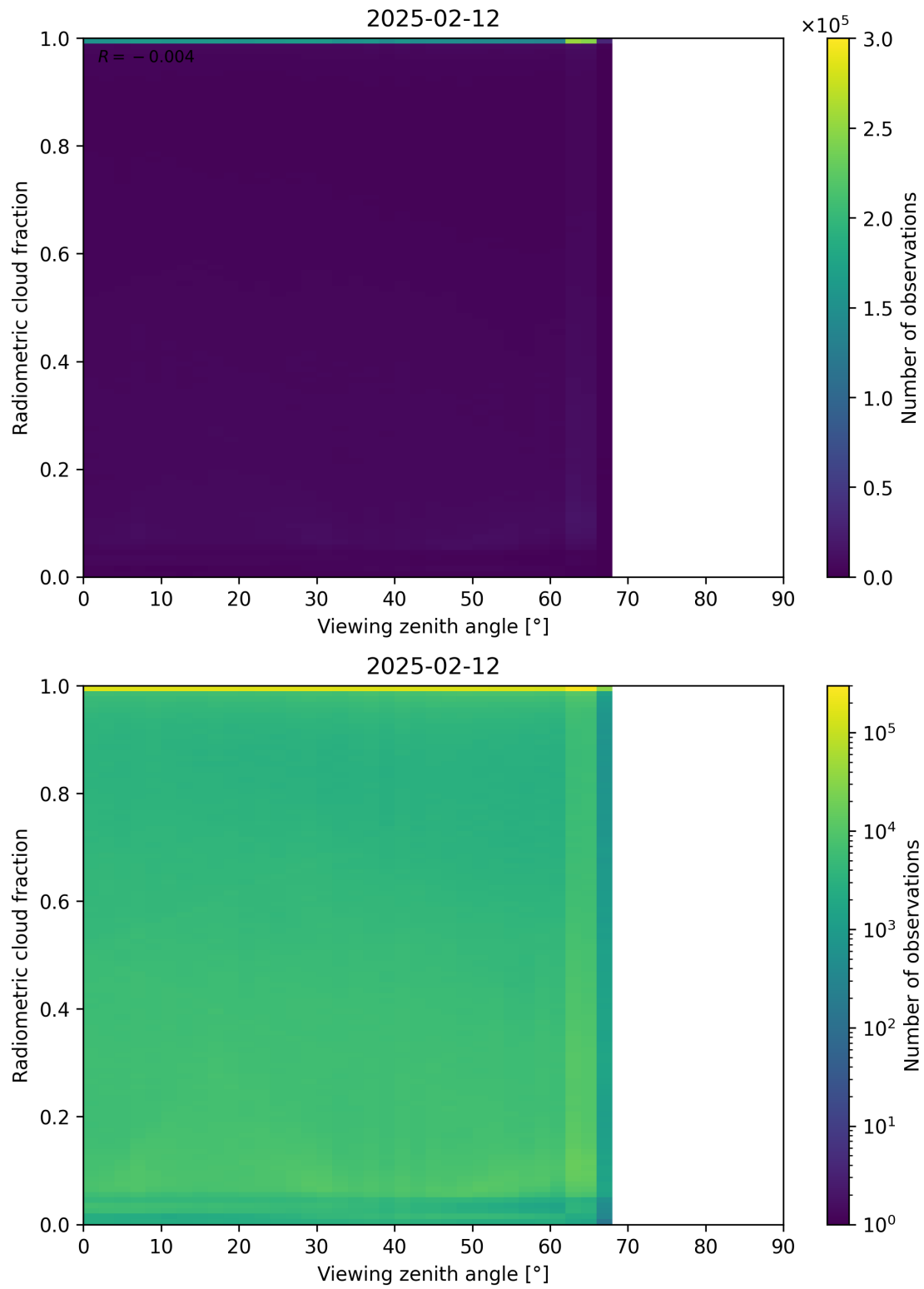
Figure 107: Scatter density plot of “Viewing zenith angle” against “Radiometric cloud fraction” for 2025-02-11 to 2025-02-13.
