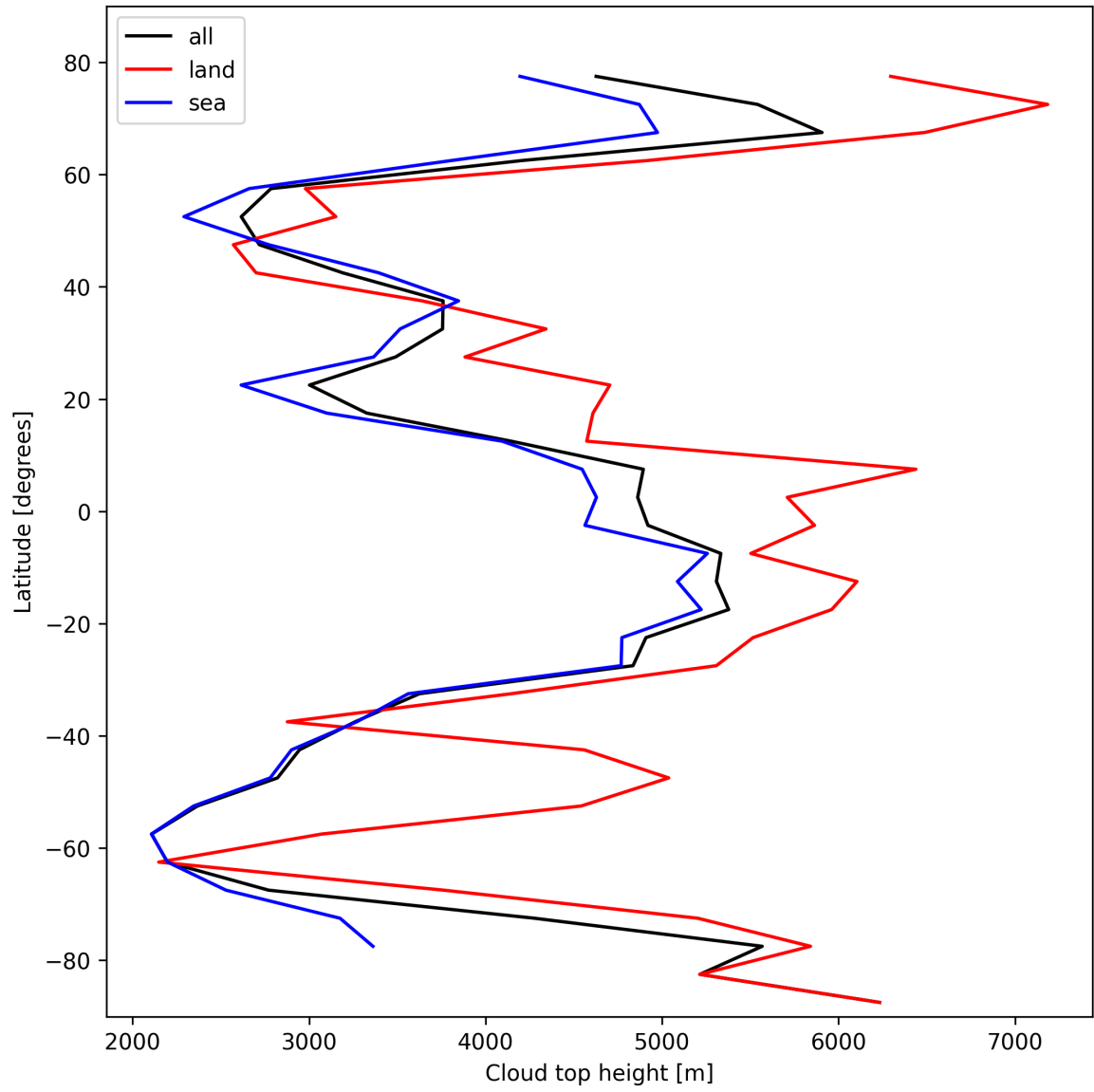
Figure 24: Zonal average of “Cloud top height” for 2025-02-11 to 2025-02-13.
