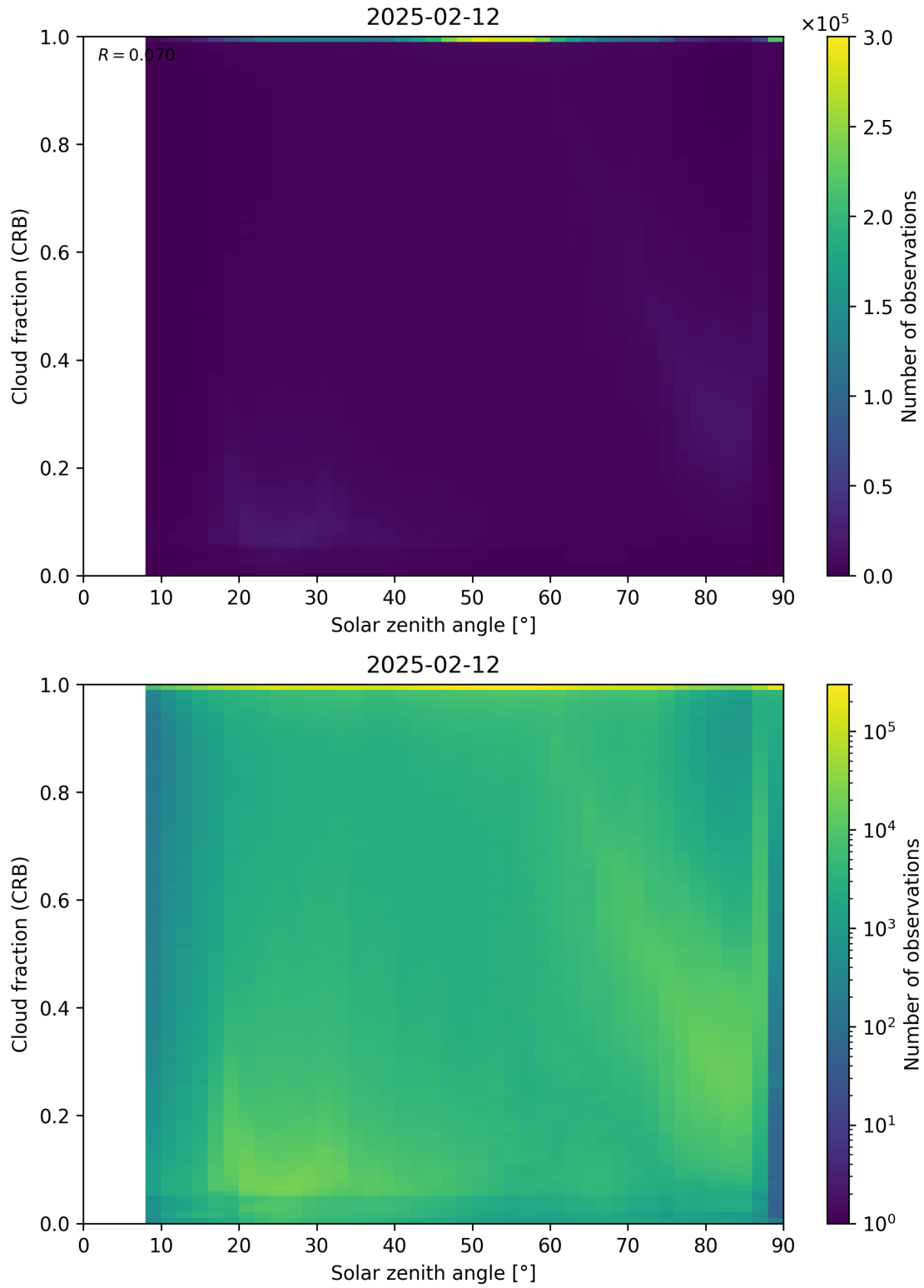
Figure 101: Scatter density plot of “Solar zenith angle” against “Cloud fraction (CRB)” for 2025-02-11 to 2025-02-13.
