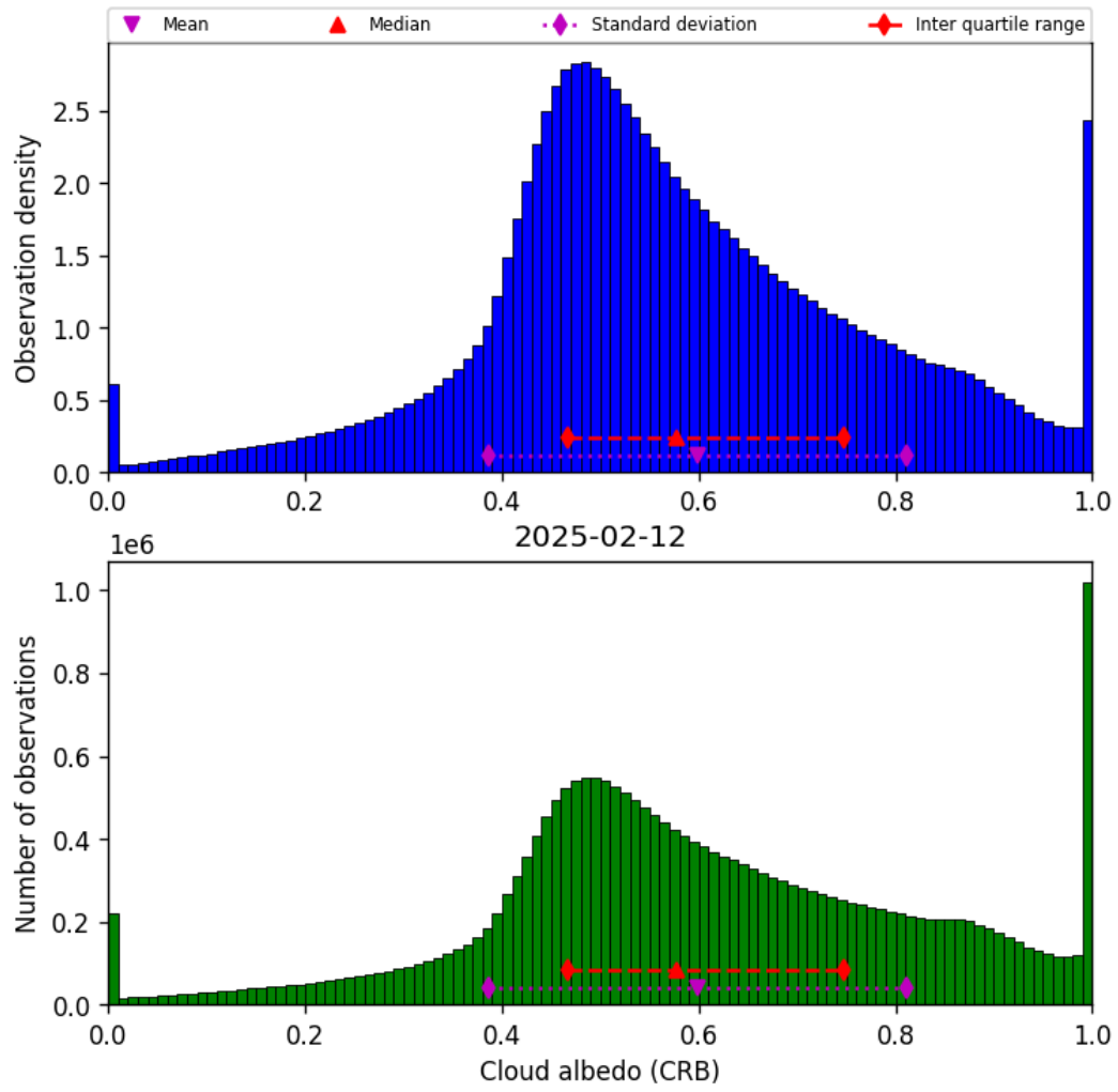
Figure 44: Histogram of “Cloud albedo (CRB)” for 2025-02-11 to 2025-02-13
