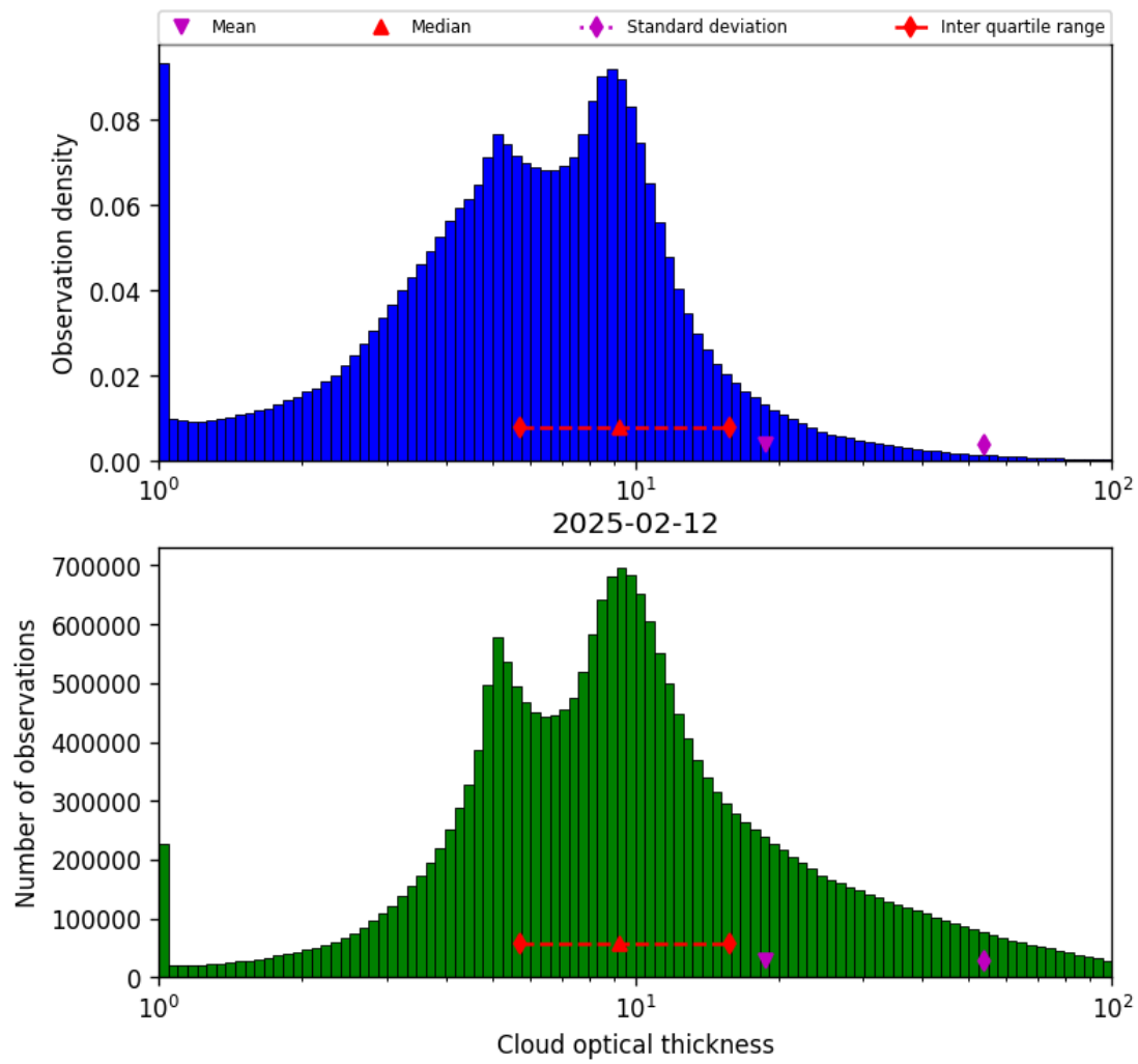
Figure 41: Histogram of “Cloud optical thickness” for 2025-02-11 to 2025-02-13
