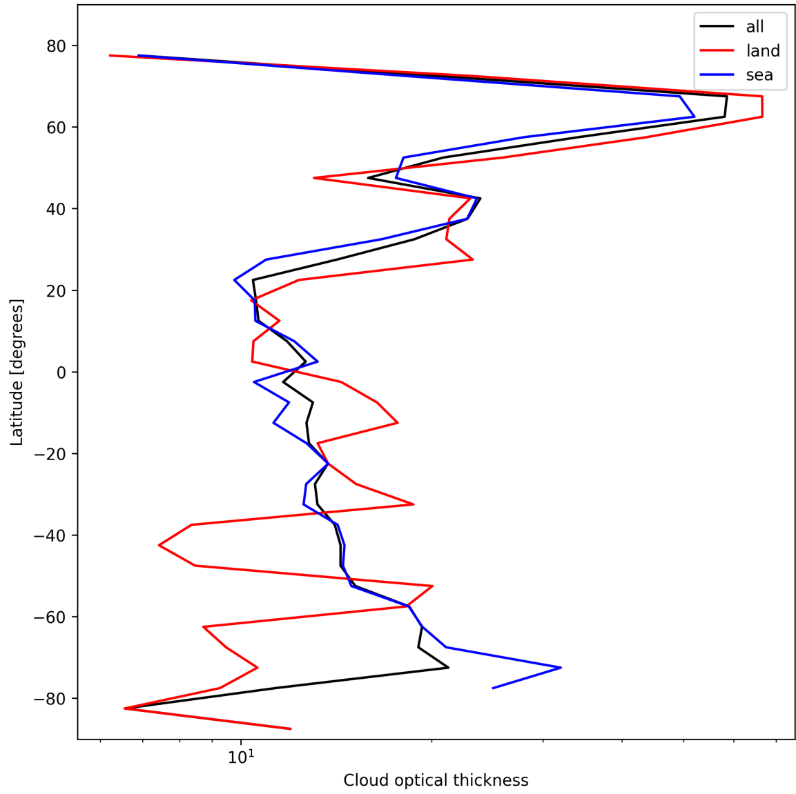
Figure 25: Zonal average of “Cloud optical thickness” for 2025-02-11 to 2025-02-13.
