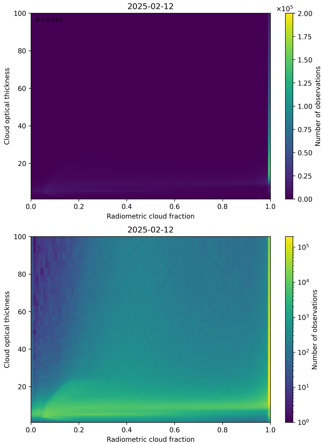
Figure 75: Scatter density plot of “Radiometric cloud fraction” against “Cloud optical thickness” for 2025-02-11 to 2025-02-13.
