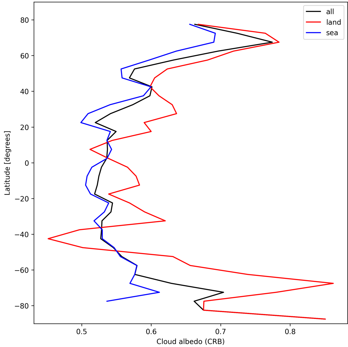
Figure 28: Zonal average of “Cloud albedo (CRB)” for 2025-02-11 to 2025-02-13.
