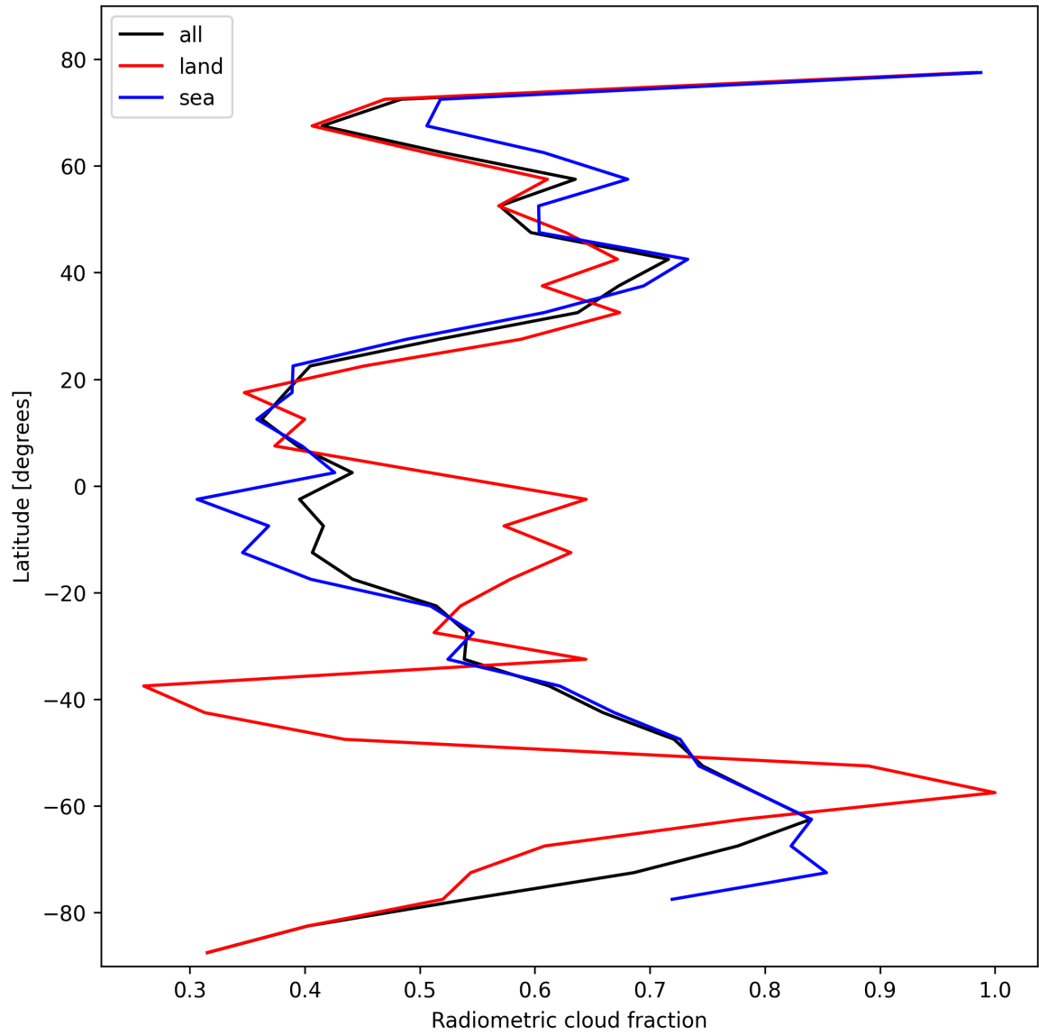
Figure 23: Zonal average of “Radiometric cloud fraction” for 2025-02-11 to 2025-02-13.
