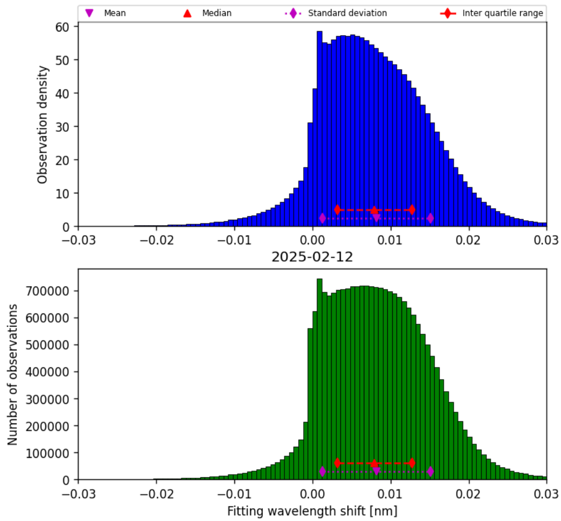
Figure 49: Histogram of “Fitting wavelength shift” for 2025-02-11 to 2025-02-13
