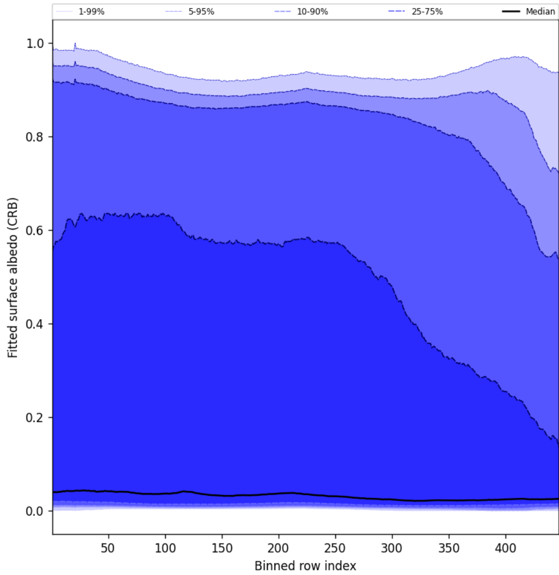
Figure 62: Along track statistics of “Fitted surface albedo (CRB)” for 2025-02-11 to 2025-02-13
