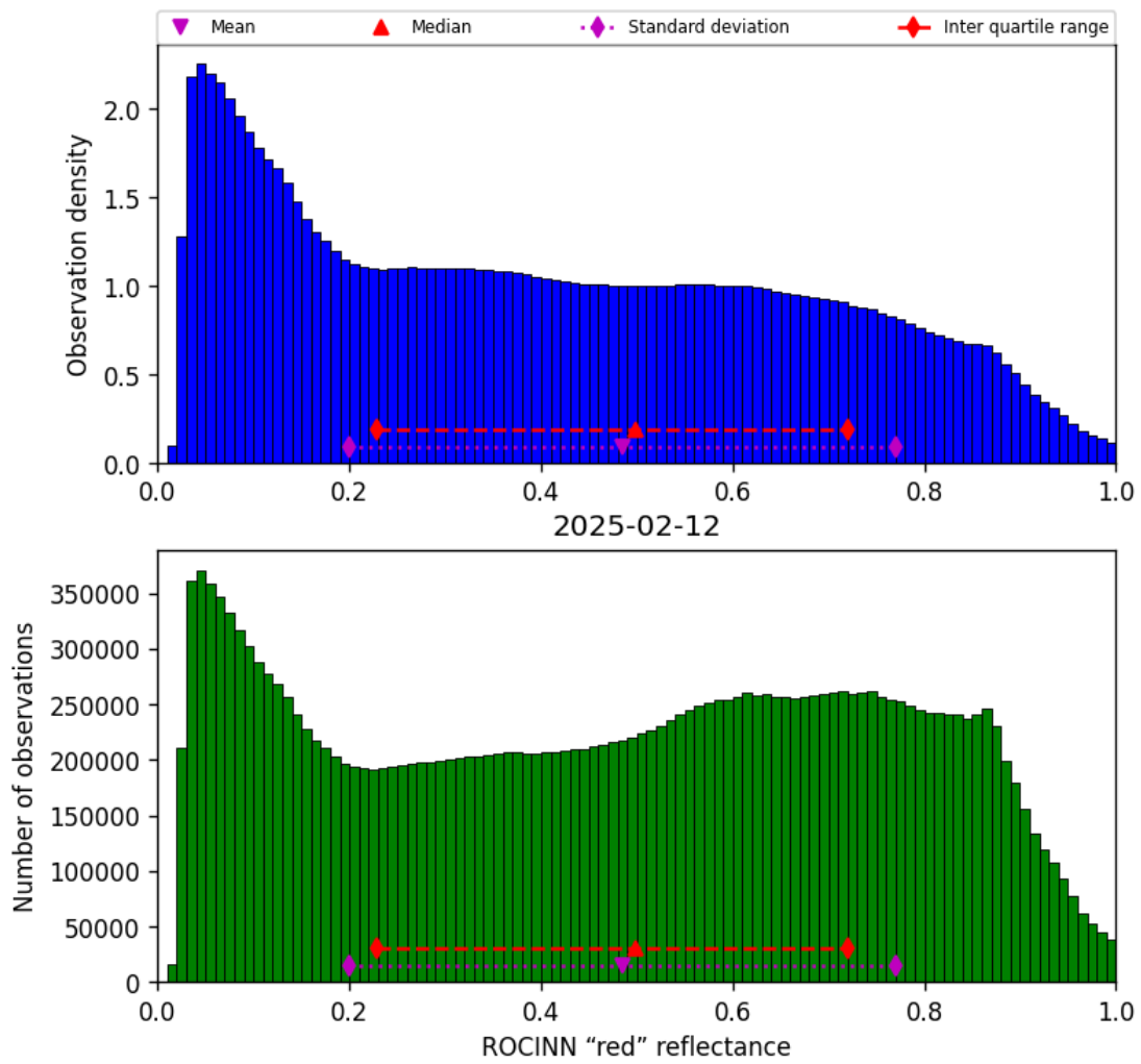
Figure 53: Histogram of “ROCINN “red” reflectance” for 2025-02-11 to 2025-02-13
