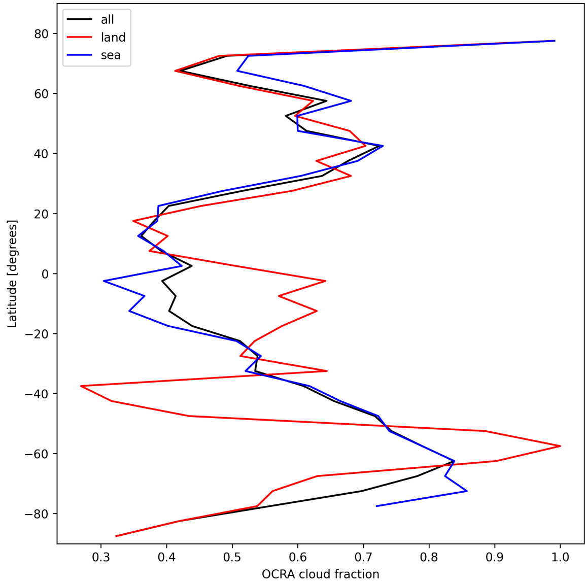
Figure 34: Zonal average of “OCRA cloud fraction” for 2025-02-11 to 2025-02-13.
