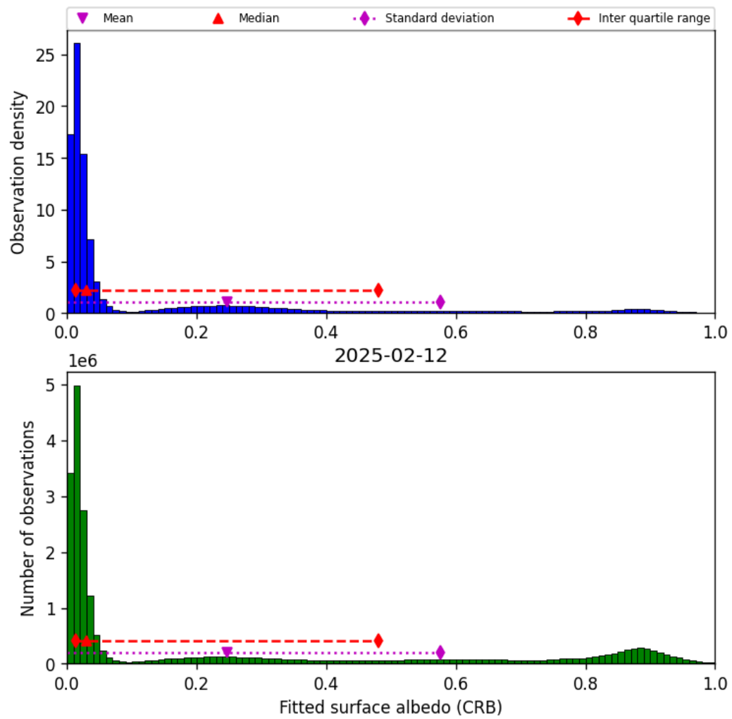
Figure 46: Histogram of “Fitted surface albedo (CRB)” for 2025-02-11 to 2025-02-13
