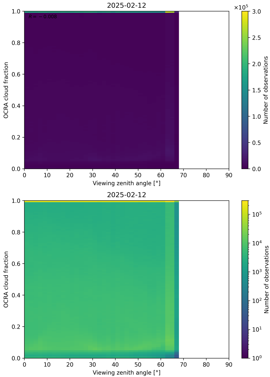
Figure 108: Scatter density plot of “Viewing zenith angle” against “OCRA cloud fraction” for 2025-02-11 to 2025-02-13.
