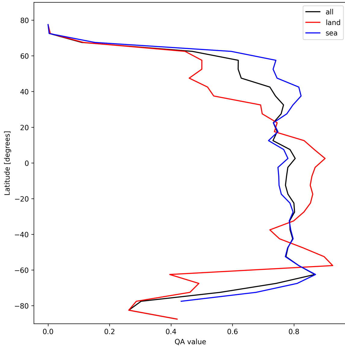
Figure 22: Zonal average of “QA value” for 2025-02-11 to 2025-02-13.
