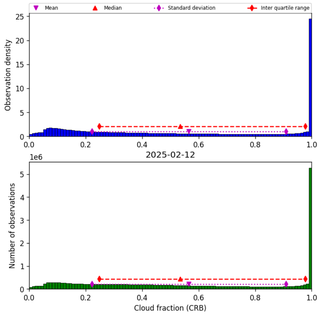
Figure 42: Histogram of “Cloud fraction (CRB)” for 2025-02-11 to 2025-02-13
