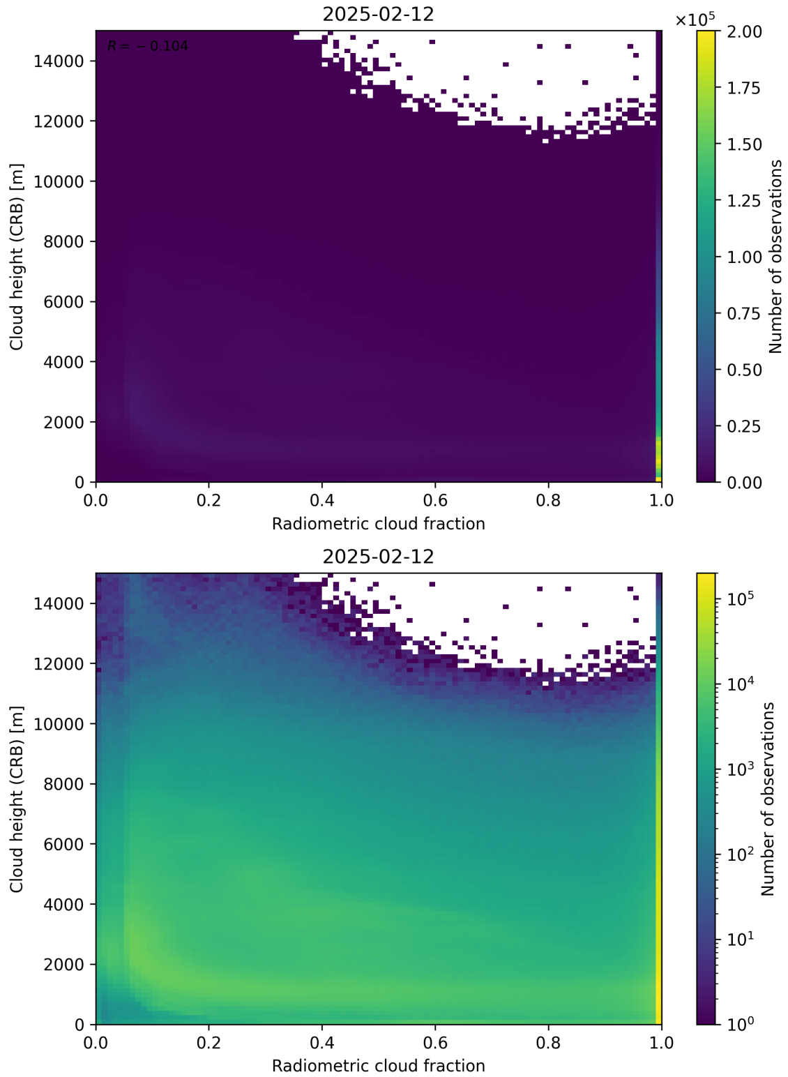
Figure 74: Scatter density plot of “Radiometric cloud fraction” against “Cloud height (CRB)” for 2025-02-11 to 2025-02-13.
