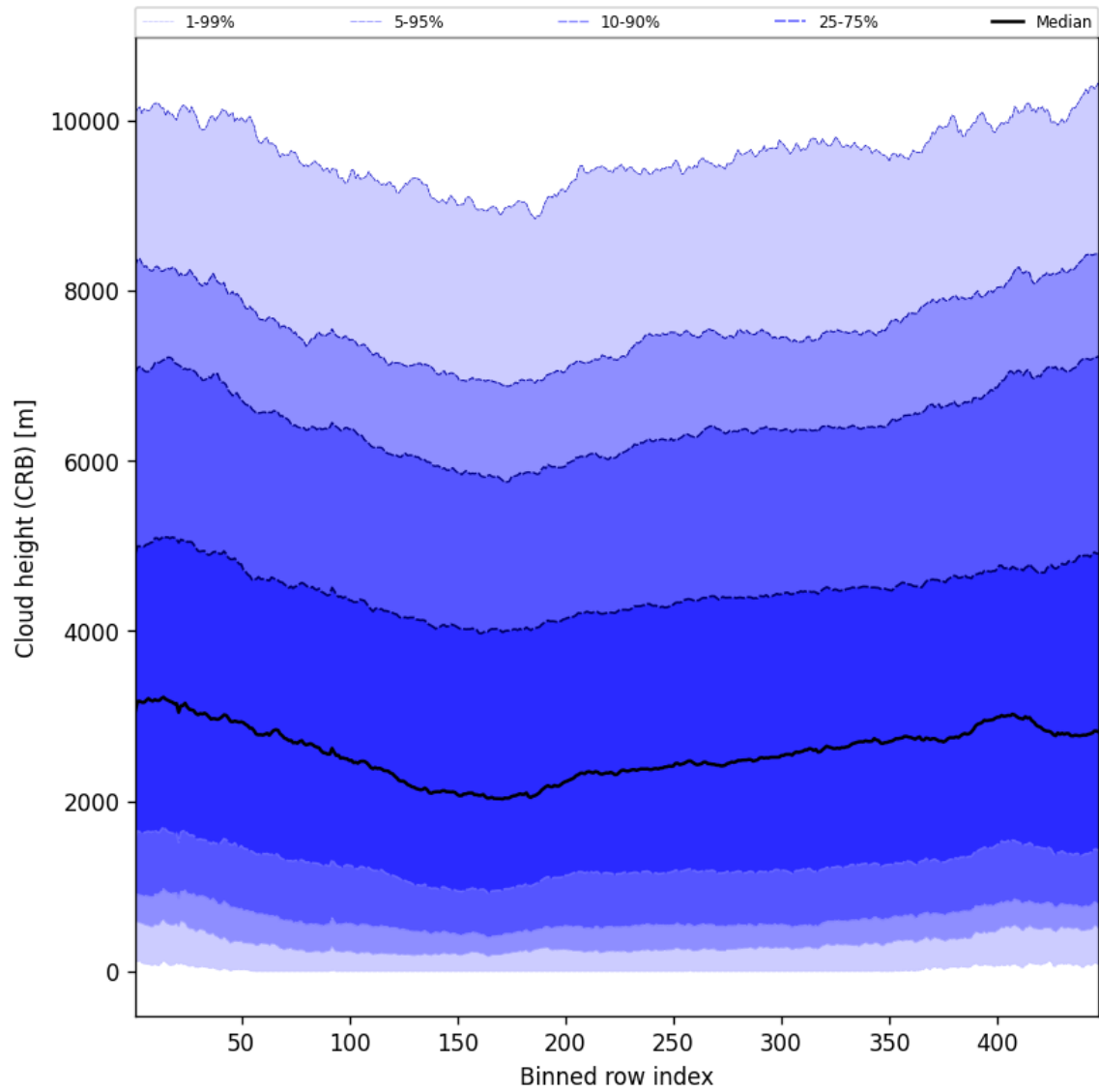
Figure 59: Along track statistics of “Cloud height (CRB)” for 2025-02-11 to 2025-02-13
