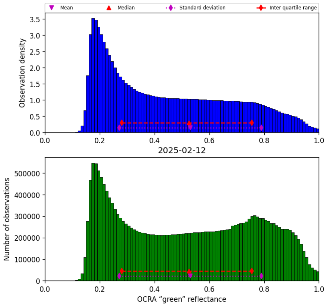
Figure 52: Histogram of “OCRA “green” reflectance” for 2025-02-11 to 2025-02-13
