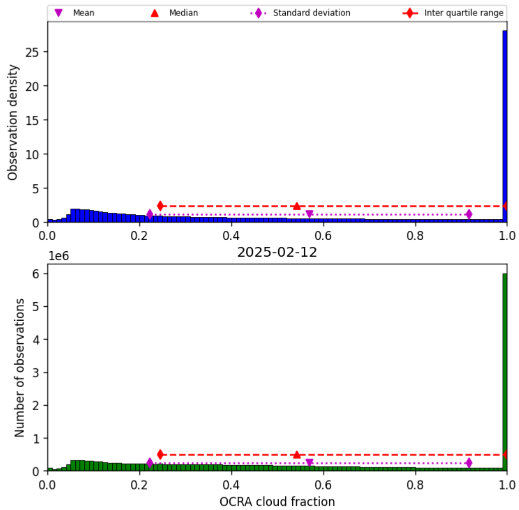
Figure 50: Histogram of “OCRA cloud fraction” for 2025-02-11 to 2025-02-13
