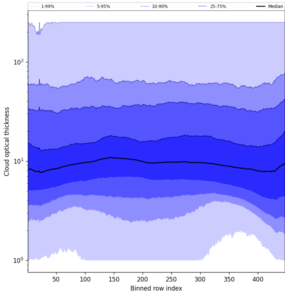
Figure 57: Along track statistics of “Cloud optical thickness” for 2025-02-11 to 2025-02-13
