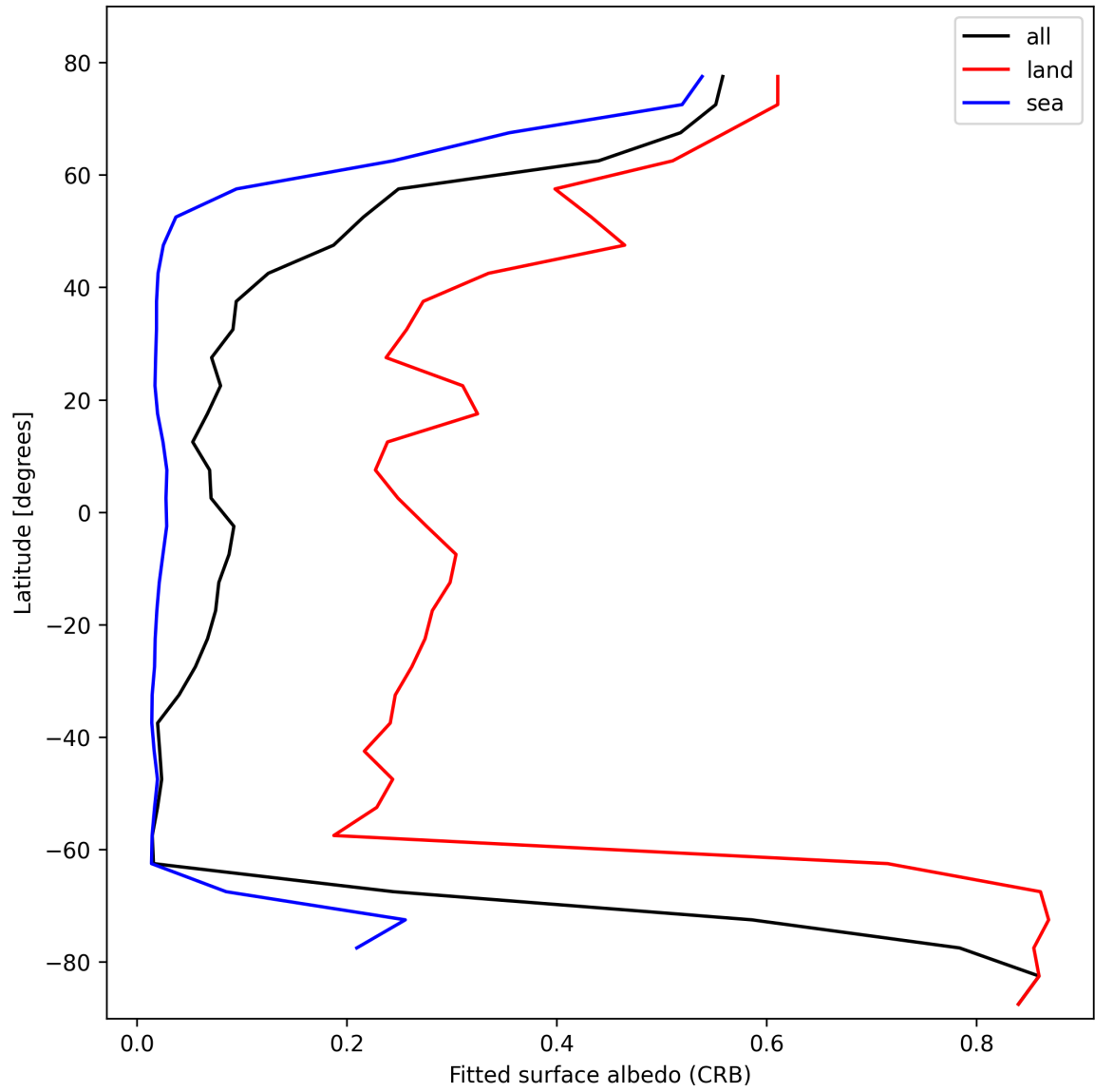
Figure 30: Zonal average of “Fitted surface albedo (CRB)” for 2025-02-11 to 2025-02-13.
