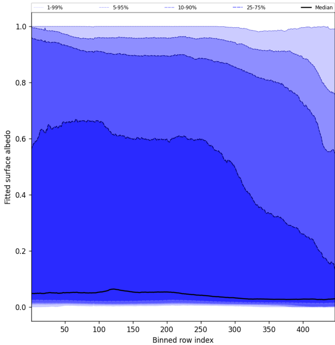
Figure 61: Along track statistics of “Fitted surface albedo” for 2025-02-11 to 2025-02-13
