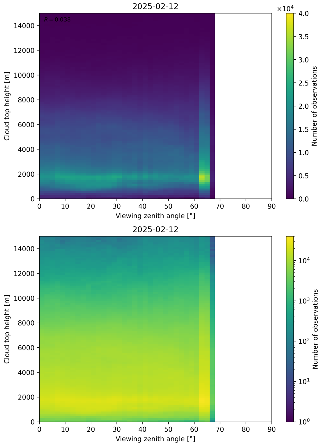
Figure 112: Scatter density plot of “Viewing zenith angle” against “Cloud top height” for 2025-02-11 to 2025-02-13.
