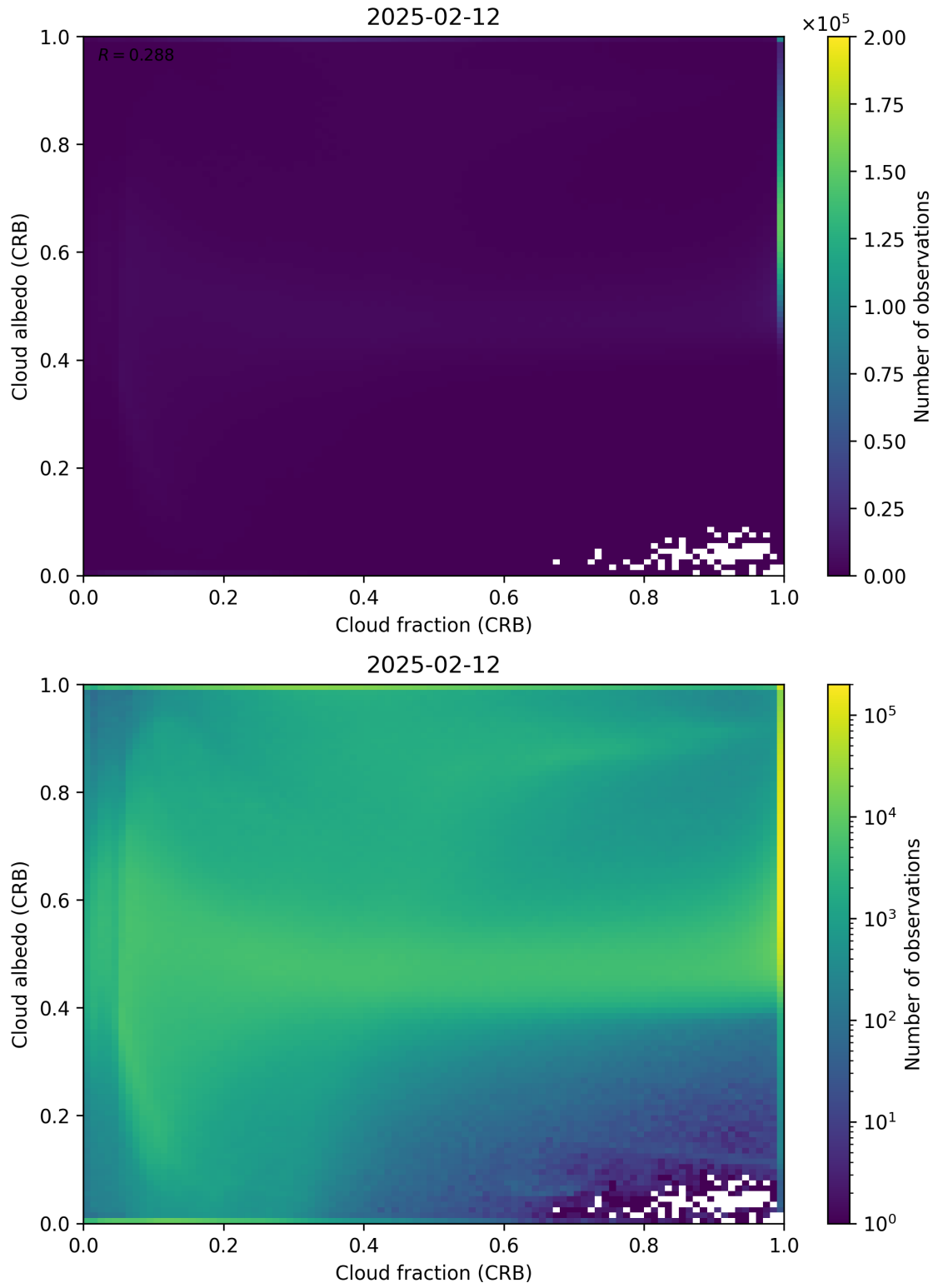
Figure 77: Scatter density plot of “Cloud fraction (CRB)” against “Cloud albedo (CRB)” for 2025-02-11 to 2025-02-13.
