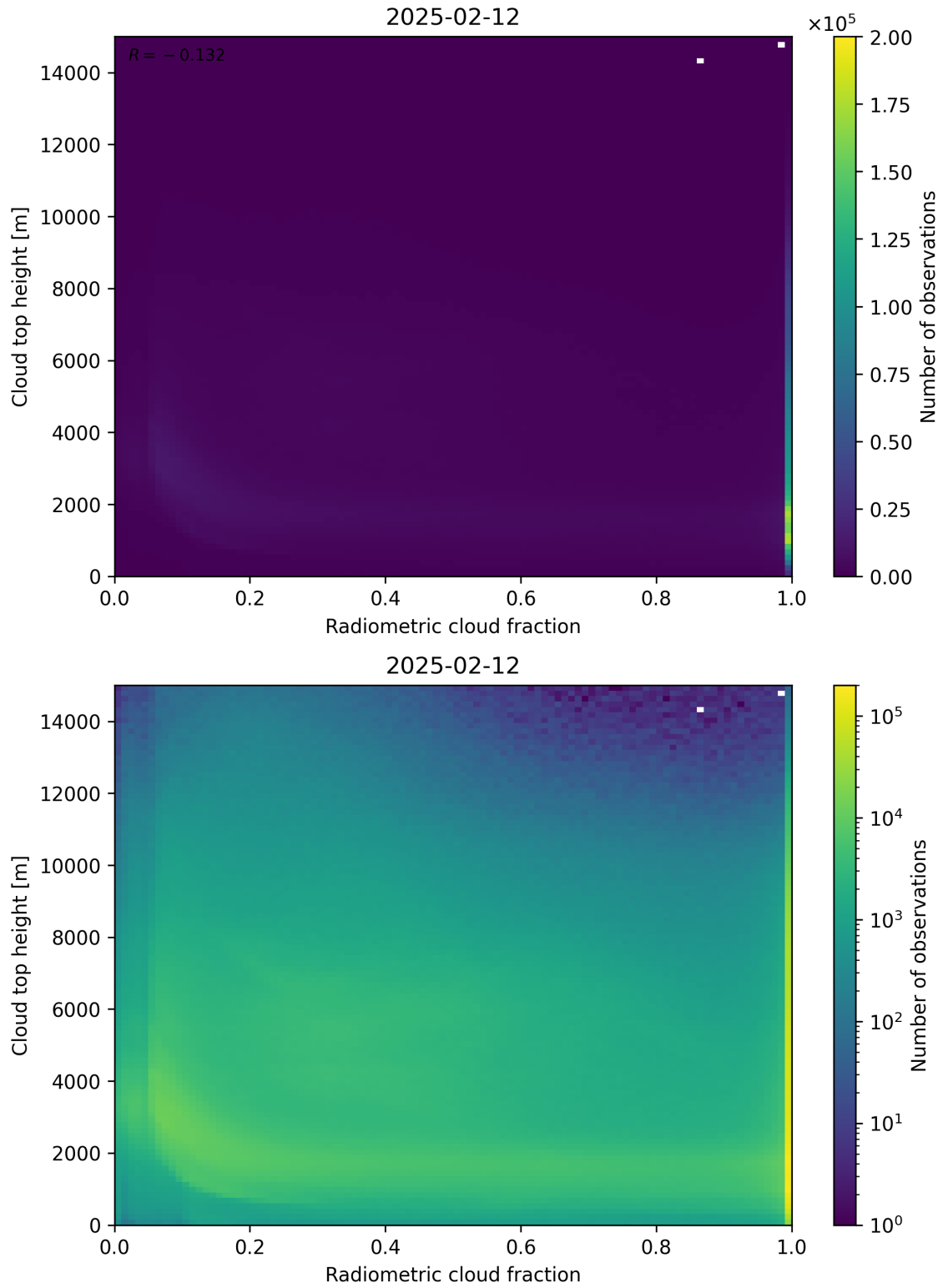
Figure 76: Scatter density plot of “Radiometric cloud fraction” against “Cloud top height” for 2025-02-11 to 2025-02-13.
