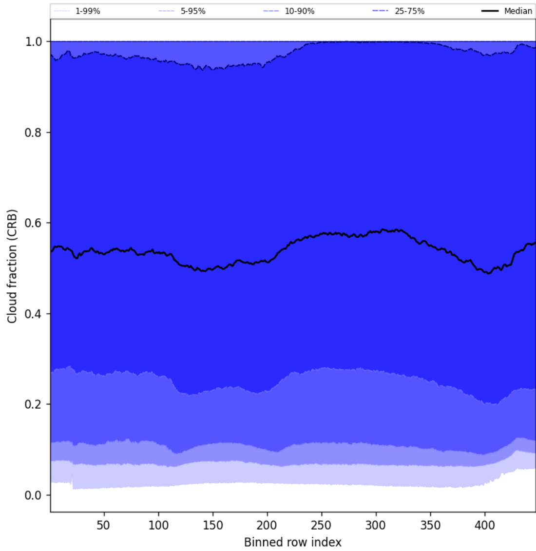
Figure 58: Along track statistics of “Cloud fraction (CRB)” for 2025-02-11 to 2025-02-13
