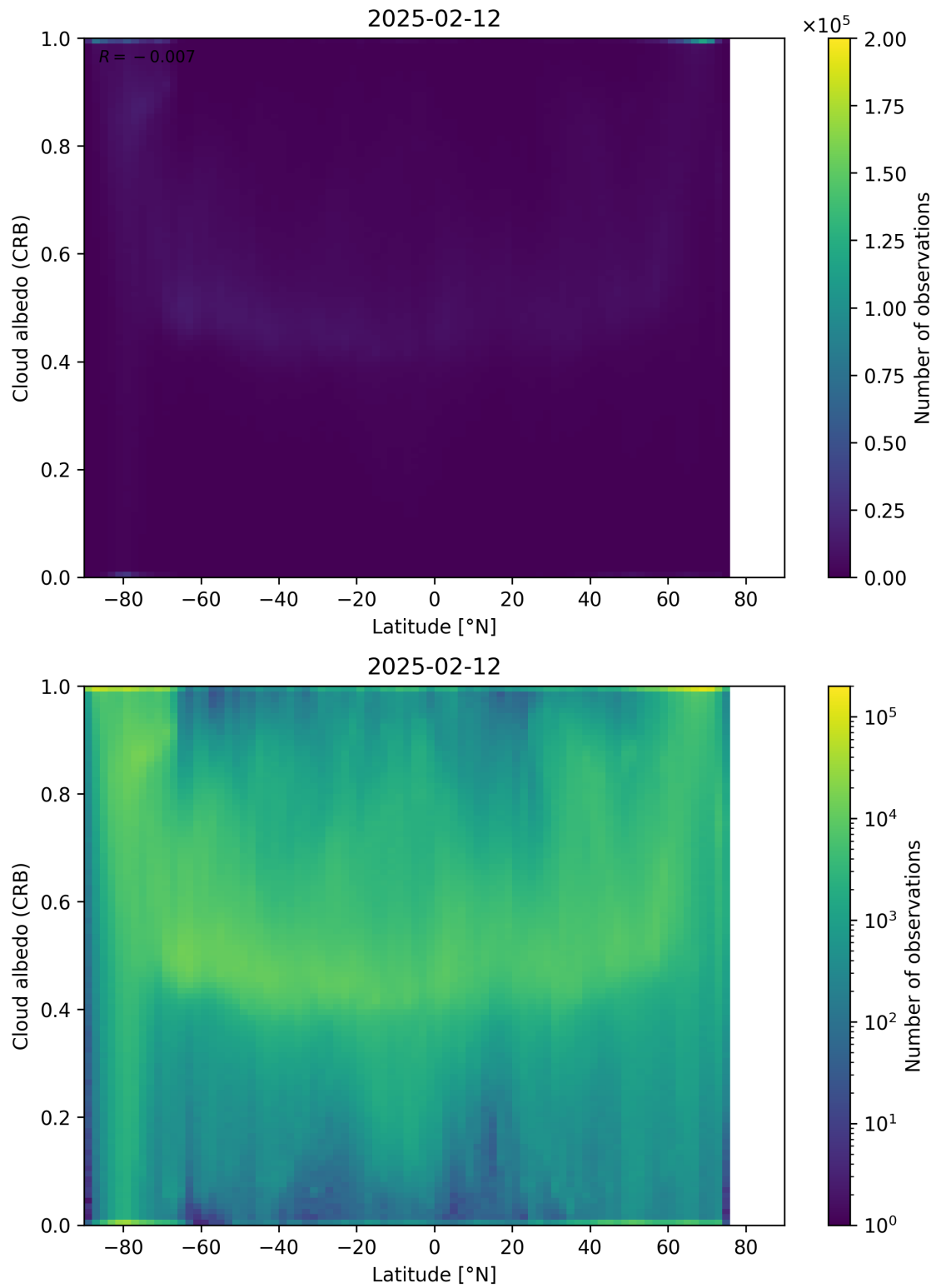
Figure 91: Scatter density plot of “Latitude” against “Cloud albedo (CRB)” for 2025-02-11 to 2025-02-13.
