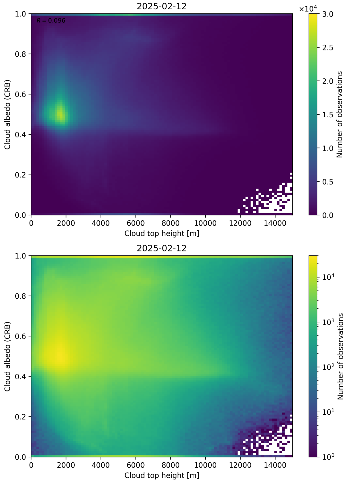
Figure 86: Scatter density plot of “Cloud top height” against “Cloud albedo (CRB)” for 2025-02-11 to 2025-02-13.
