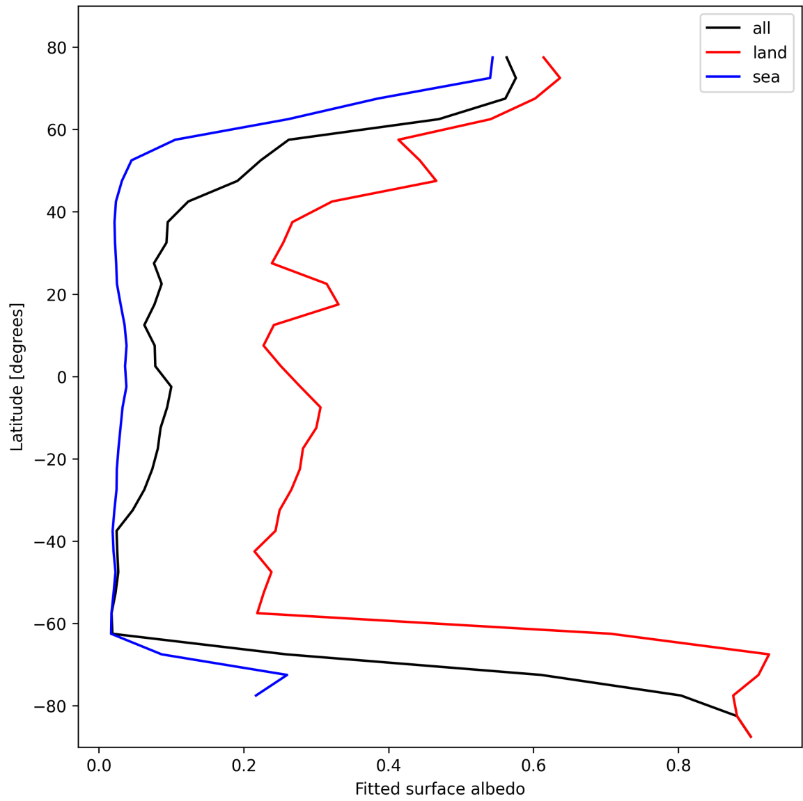
Figure 29: Zonal average of “Fitted surface albedo” for 2025-02-11 to 2025-02-13.
