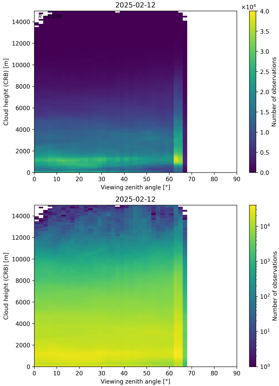
Figure 110: Scatter density plot of “Viewing zenith angle” against “Cloud height (CRB)” for 2025-02-11 to 2025-02-13.
