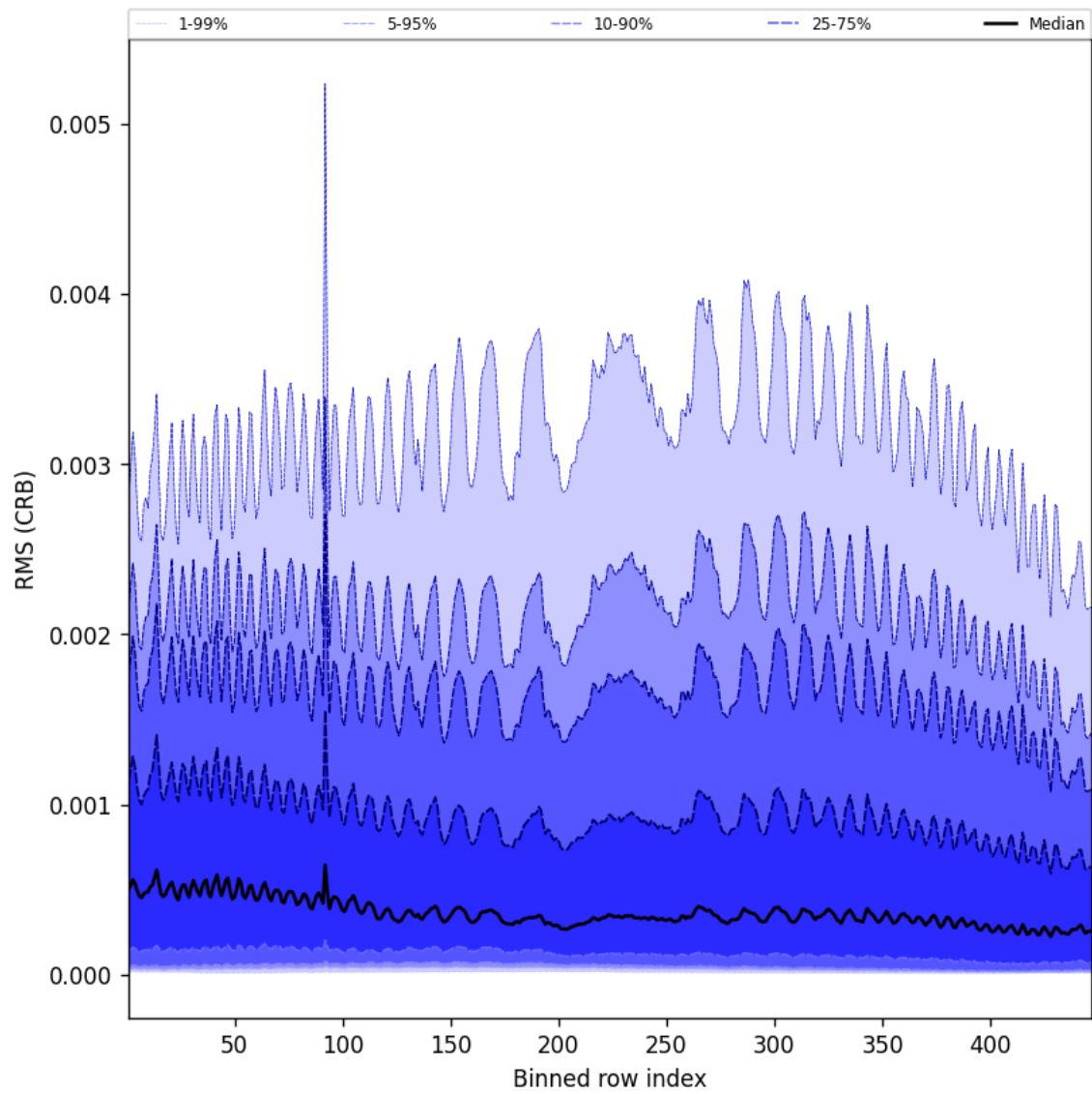
Figure 64: Along track statistics of “RMS (CRB)” for 2025-02-11 to 2025-02-13
