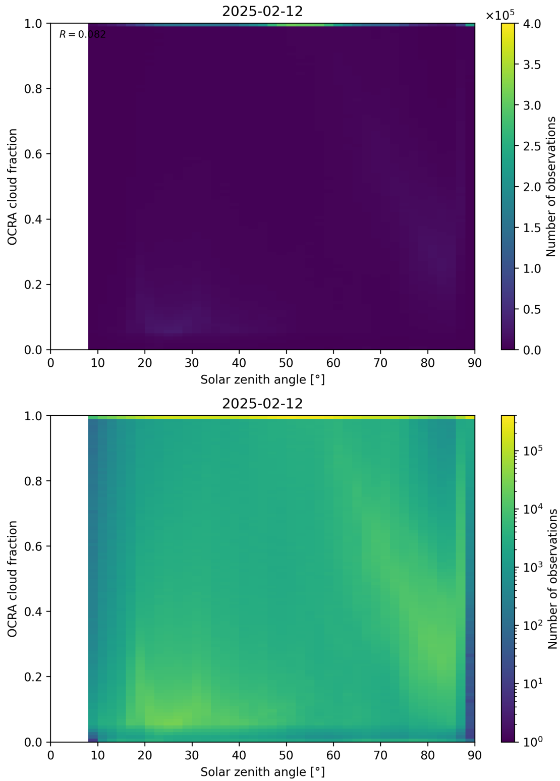
Figure 100: Scatter density plot of “Solar zenith angle” against “OCRA cloud fraction” for 2025-02-11 to 2025-02-13.
