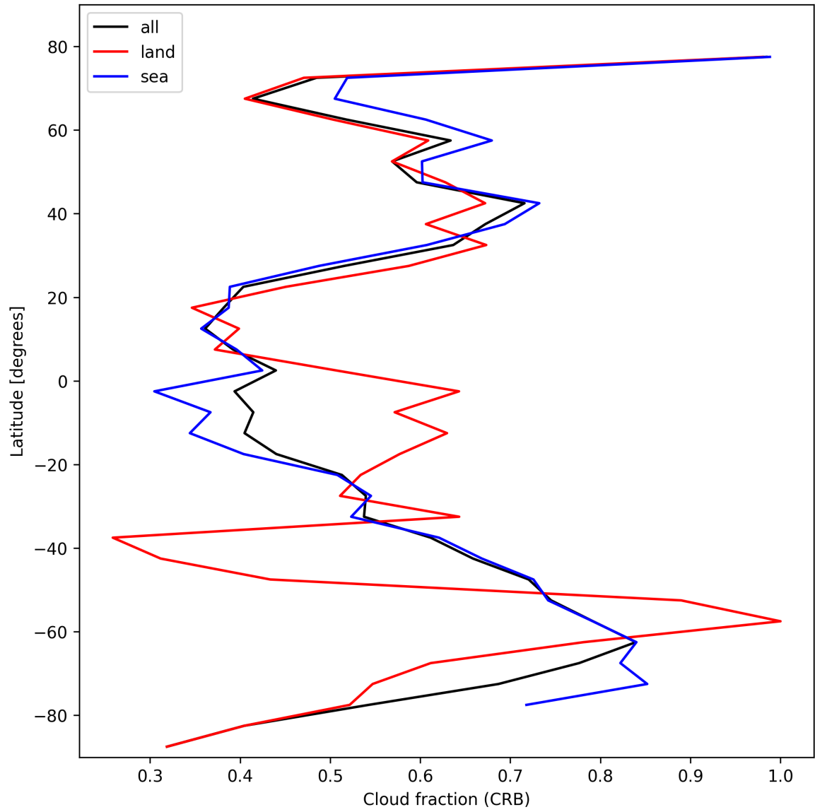
Figure 26: Zonal average of “Cloud fraction (CRB)” for 2025-02-11 to 2025-02-13.
