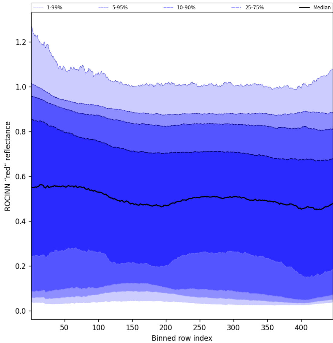
Figure 69: Along track statistics of “ROCINN “red” reflectance” for 2025-02-11 to 2025-02-13
