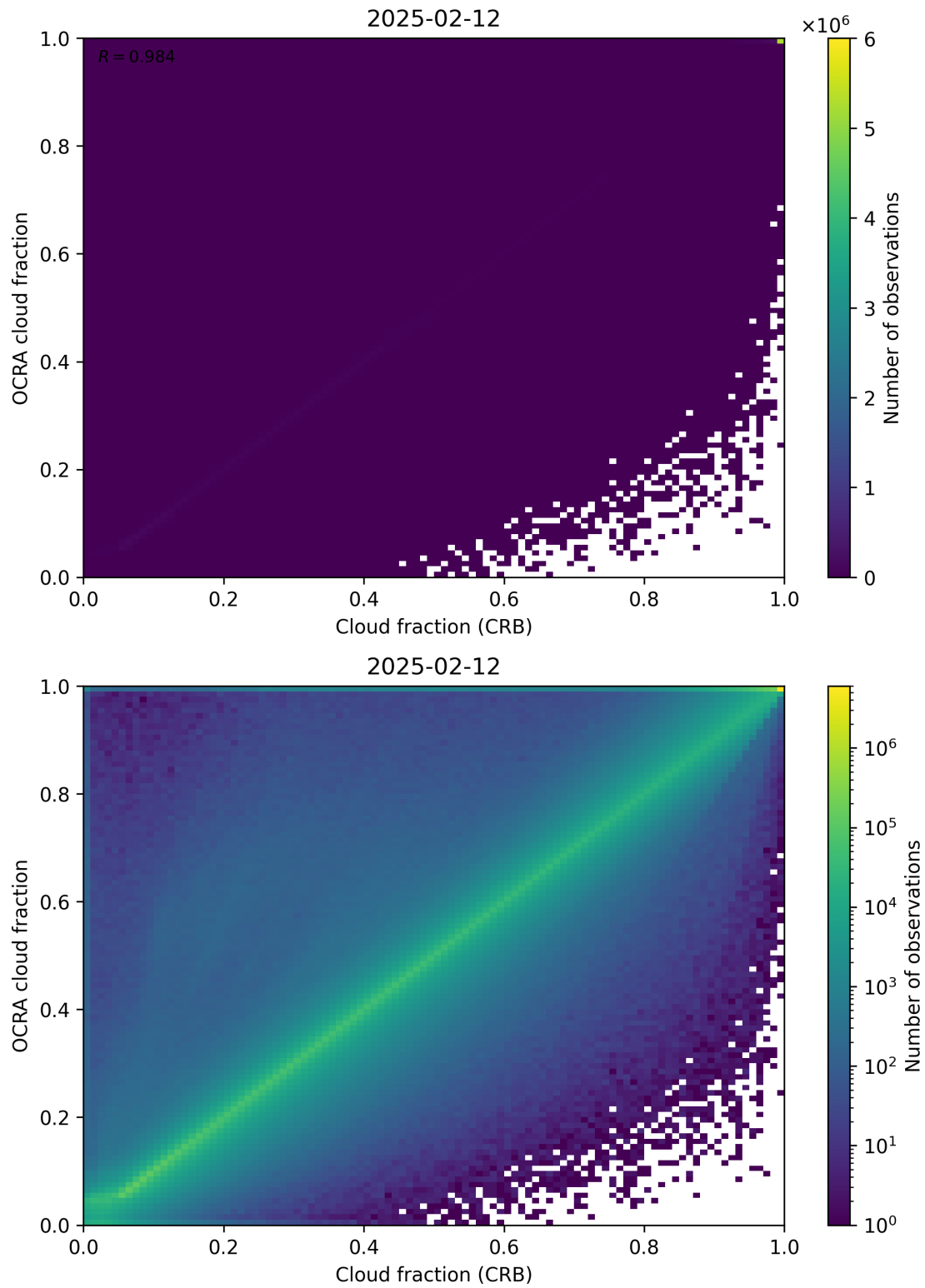
Figure 78: Scatter density plot of “Cloud fraction (CRB)” against “OCRA cloud fraction” for 2025-02-11 to 2025-02-13.
