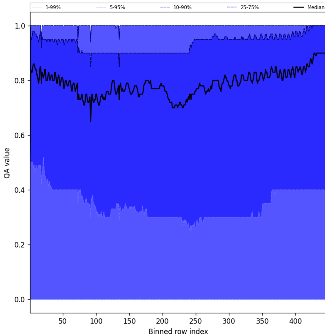
Figure 54: Along track statistics of “QA value” for 2025-02-11 to 2025-02-13
