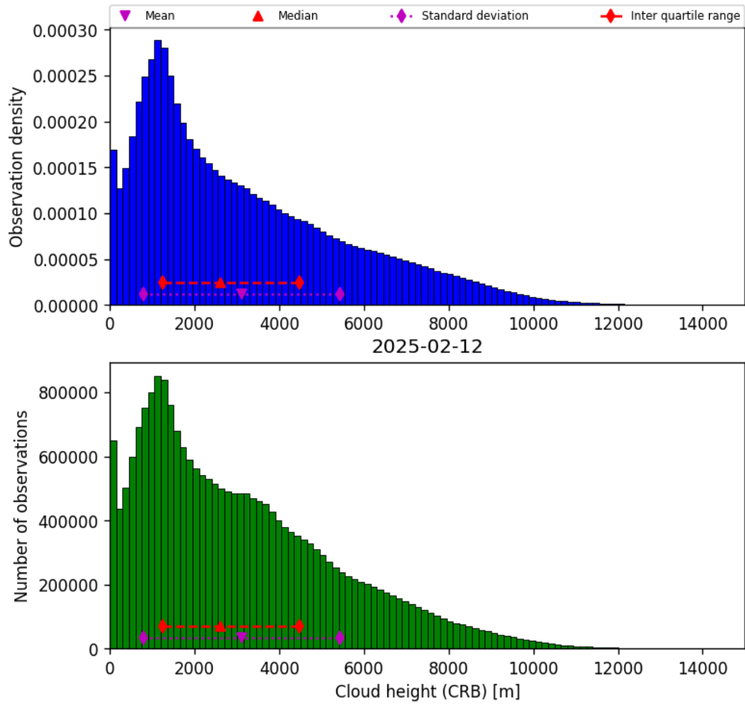
Figure 43: Histogram of “Cloud height (CRB)” for 2025-02-11 to 2025-02-13
