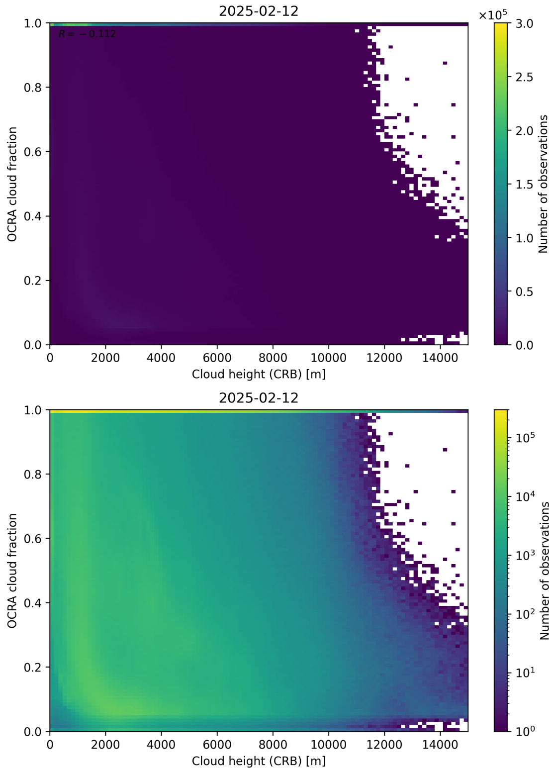
Figure 81: Scatter density plot of “Cloud height (CRB)” against “OCRA cloud fraction” for 2025-02-11 to 2025-02-13.
