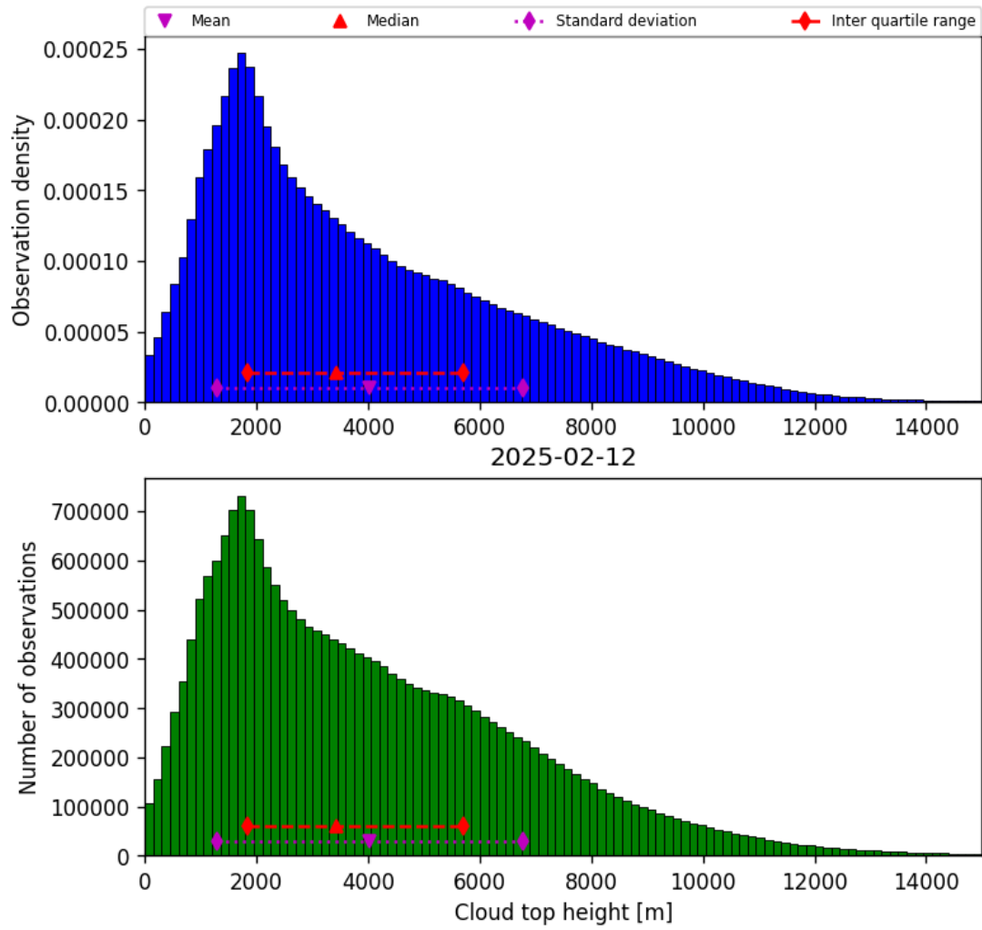
Figure 40: Histogram of “Cloud top height” for 2025-02-11 to 2025-02-13
