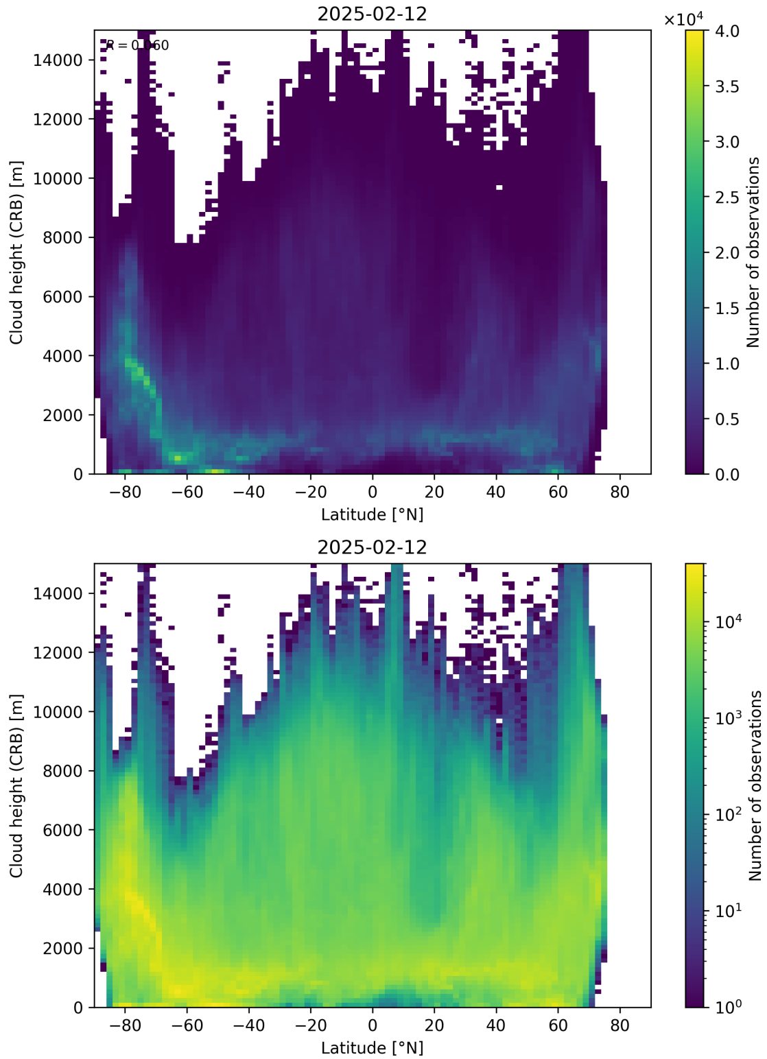
Figure 95: Scatter density plot of “Latitude” against “Cloud height (CRB)” for 2025-02-11 to 2025-02-13.
