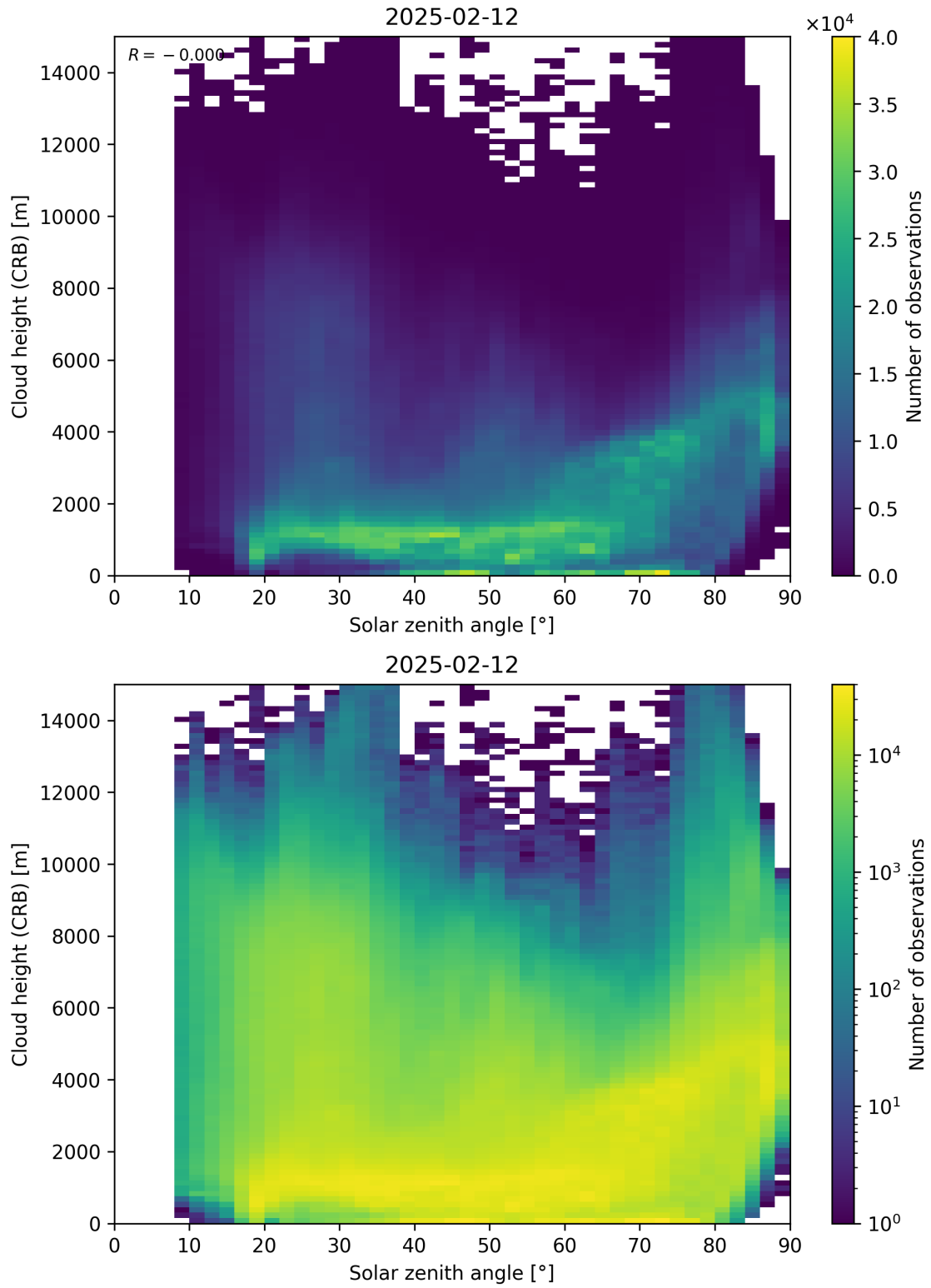
Figure 102: Scatter density plot of “Solar zenith angle” against “Cloud height (CRB)” for 2025-02-11 to 2025-02-13.
