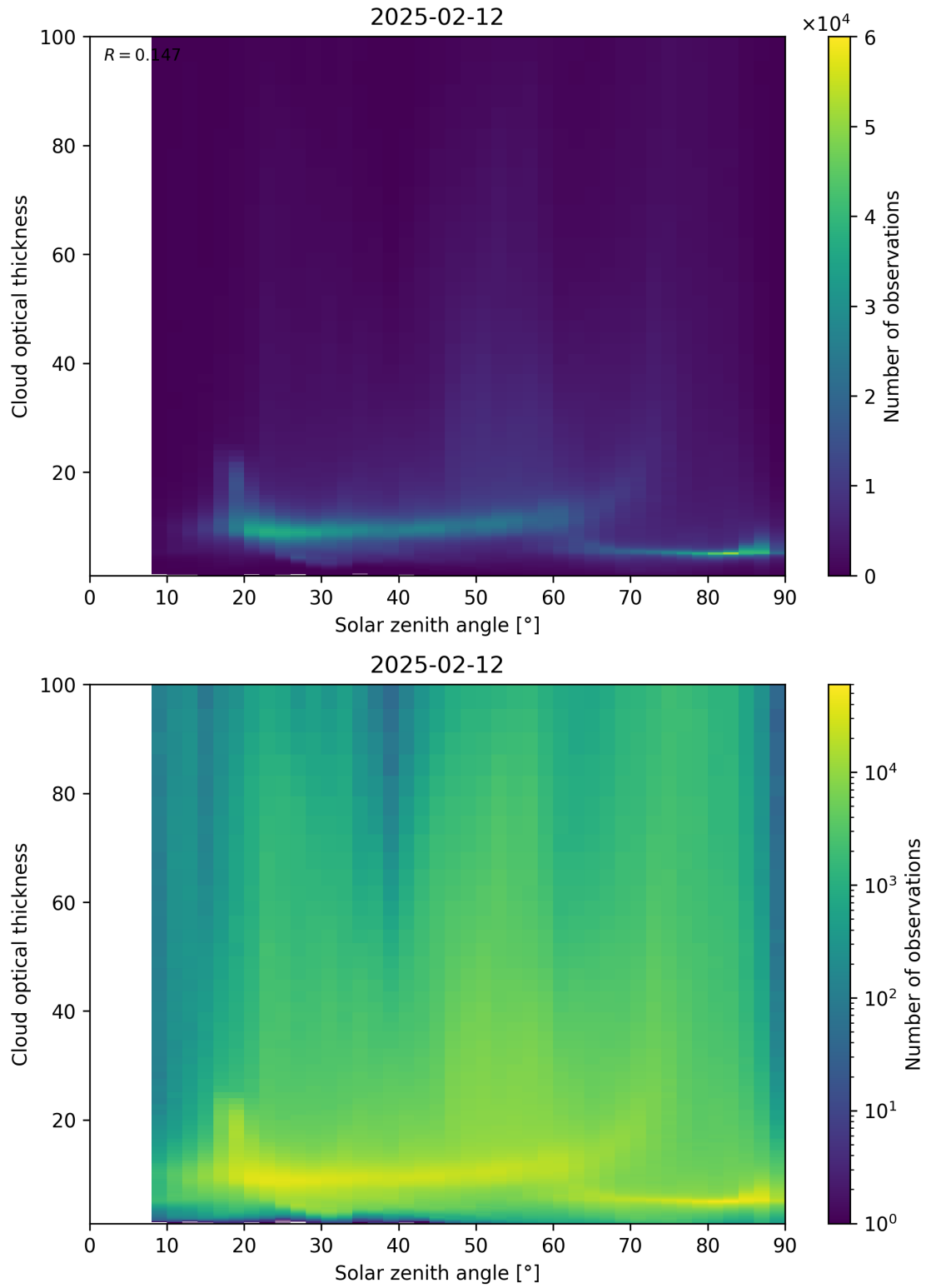
Figure 103: Scatter density plot of “Solar zenith angle” against “Cloud optical thickness” for 2025-02-11 to 2025-02-13.
