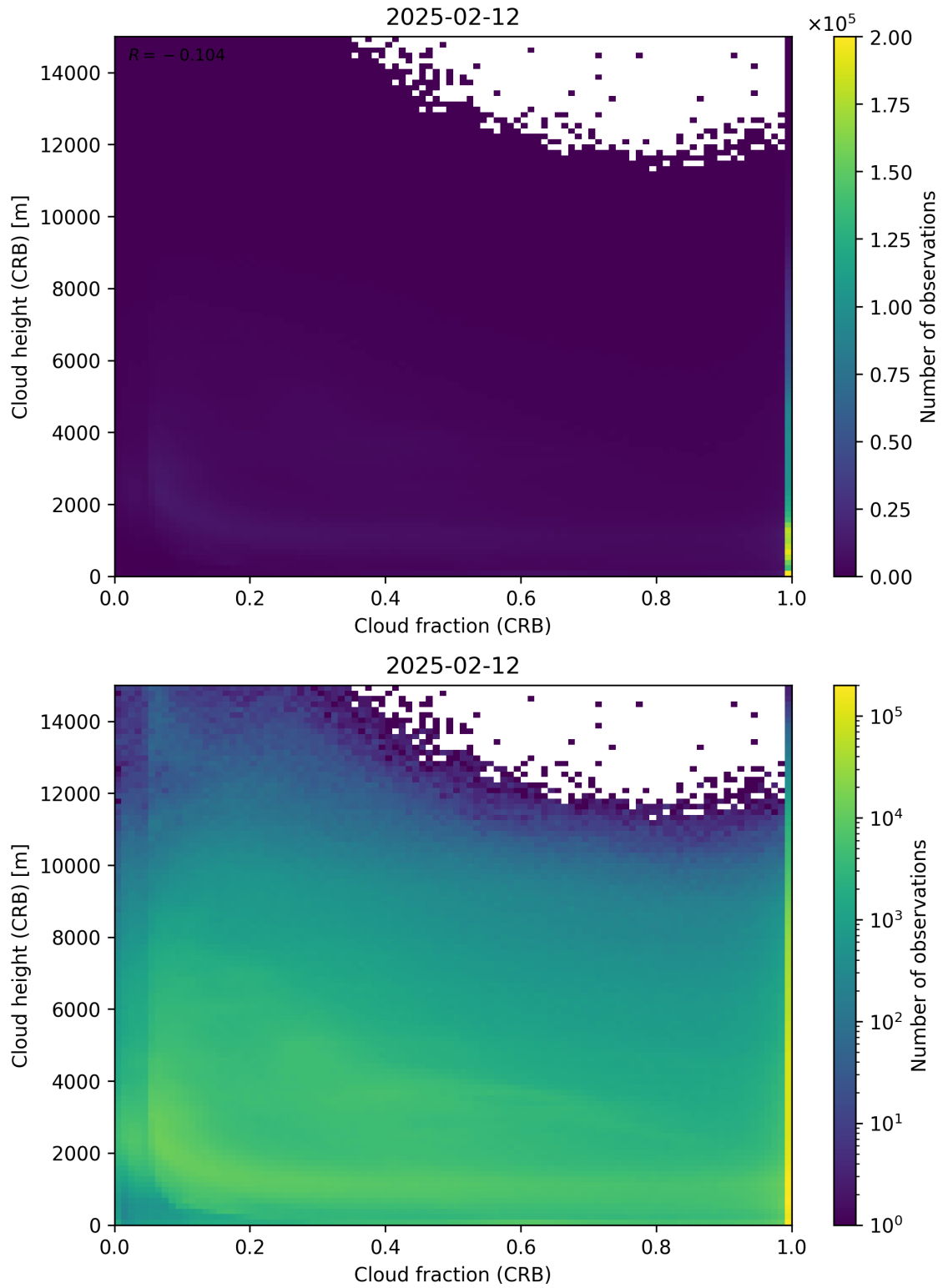
Figure 79: Scatter density plot of “Cloud fraction (CRB)” against “Cloud height (CRB)” for 2025-02-11 to 2025-02-13.
