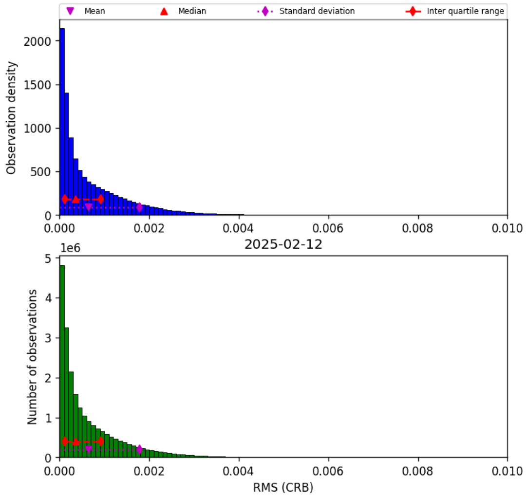
Figure 48: Histogram of “RMS (CRB)” for 2025-02-11 to 2025-02-13
