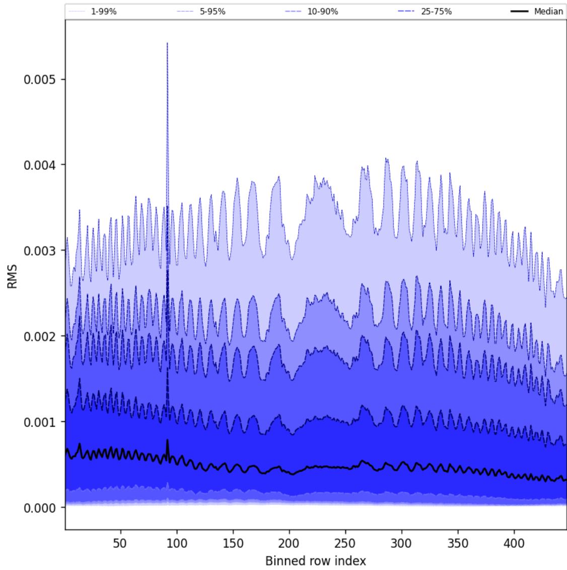
Figure 63: Along track statistics of “RMS” for 2025-02-11 to 2025-02-13
