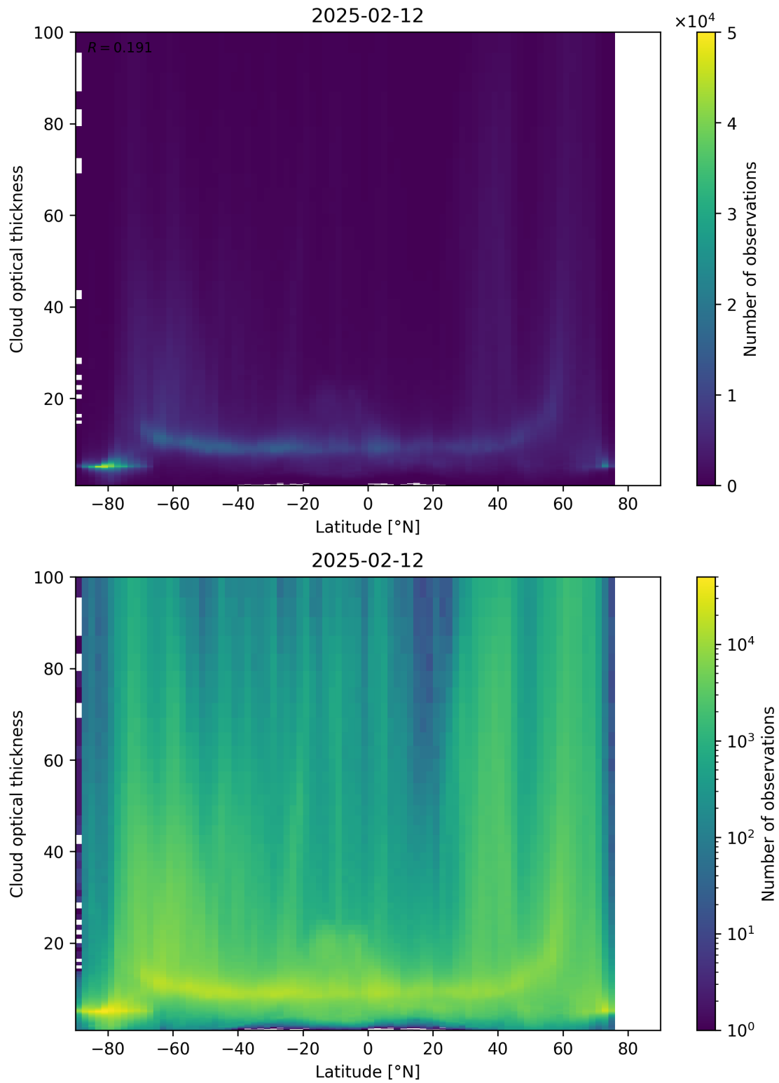
Figure 96: Scatter density plot of “Latitude” against “Cloud optical thickness” for 2025-02-11 to 2025-02-13.
