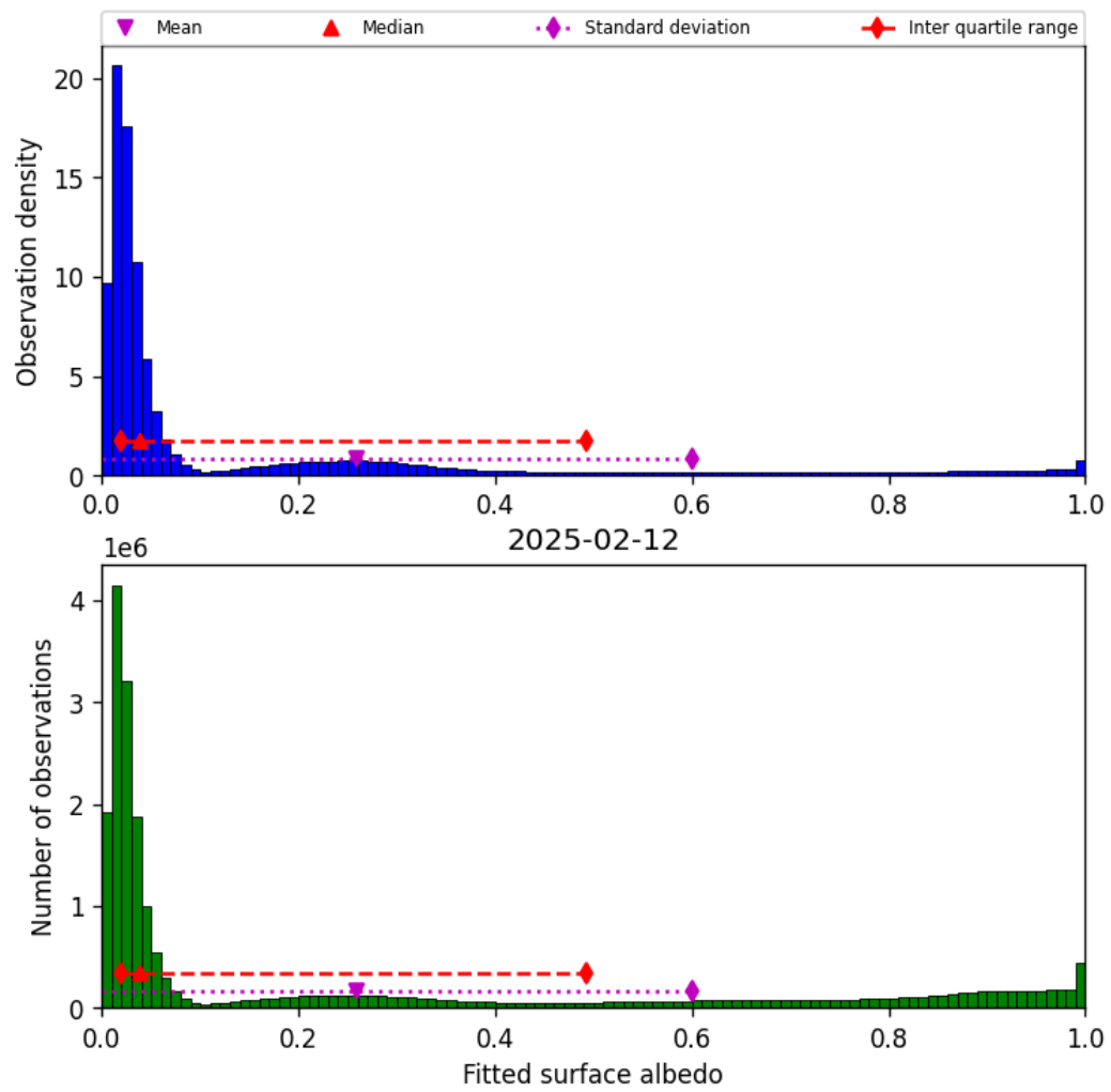
Figure 45: Histogram of “Fitted surface albedo” for 2025-02-11 to 2025-02-13
