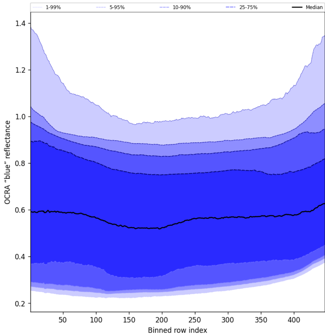
Figure 67: Along track statistics of “OCRA “blue” reflectance” for 2025-02-11 to 2025-02-13
