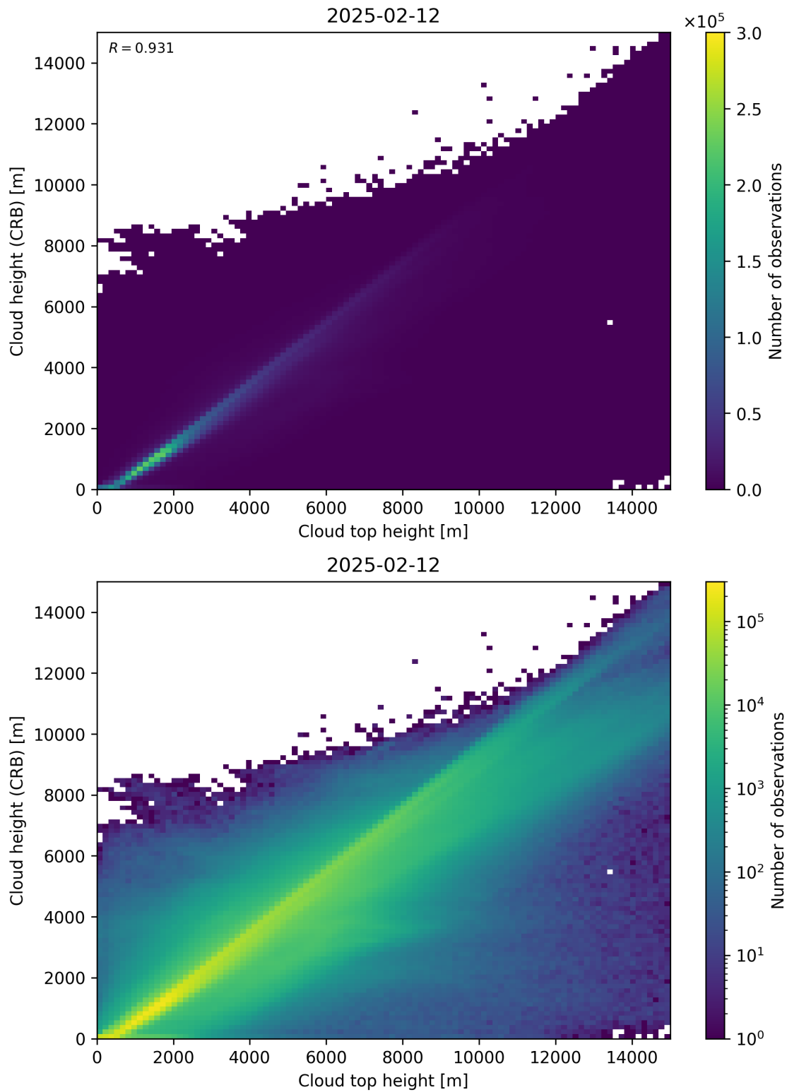
Figure 89: Scatter density plot of “Cloud top height” against “Cloud height (CRB)” for 2025-02-11 to 2025-02-13.
