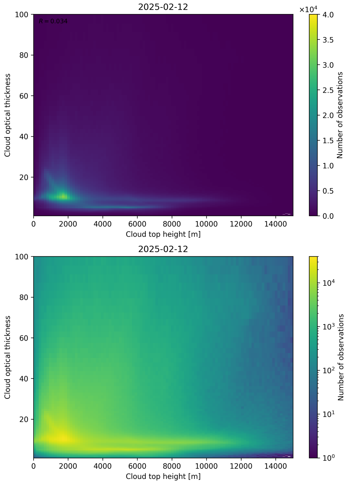
Figure 90: Scatter density plot of “Cloud top height” against “Cloud optical thickness” for 2025-02-11 to 2025-02-13.
