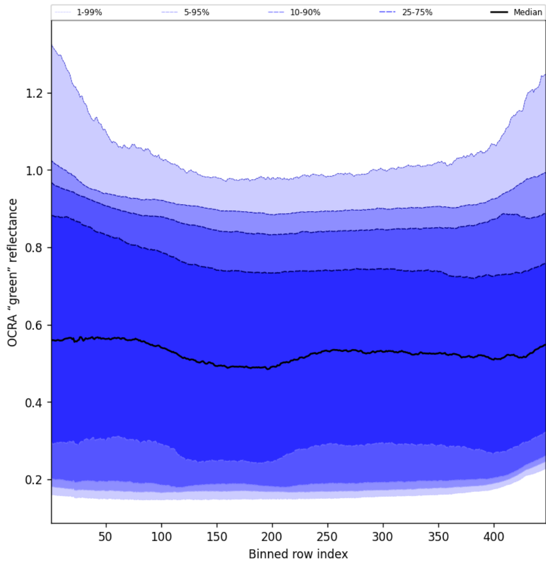
Figure 68: Along track statistics of “OCRA “green” reflectance” for 2025-02-11 to 2025-02-13
