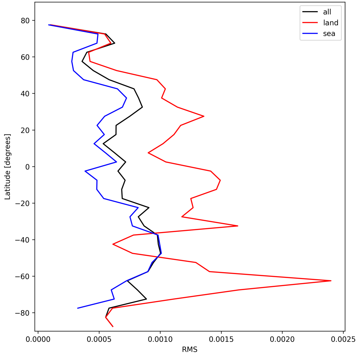
Figure 31: Zonal average of “RMS” for 2025-02-11 to 2025-02-13.
