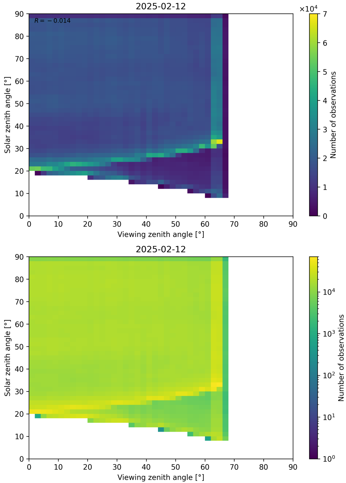
Figure 114: Scatter density plot of “Viewing zenith angle” against “Solar zenith angle” for 2025-02-11 to 2025-02-13.
