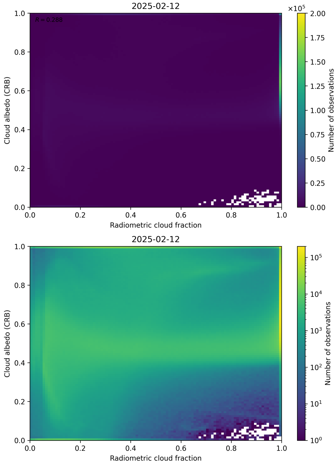
Figure 71: Scatter density plot of “Radiometric cloud fraction” against “Cloud albedo (CRB)” for 2025-02-11 to 2025-02-13.
