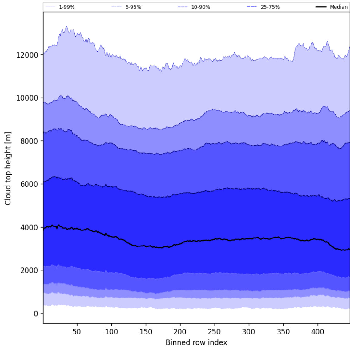
Figure 56: Along track statistics of “Cloud top height” for 2025-02-11 to 2025-02-13
