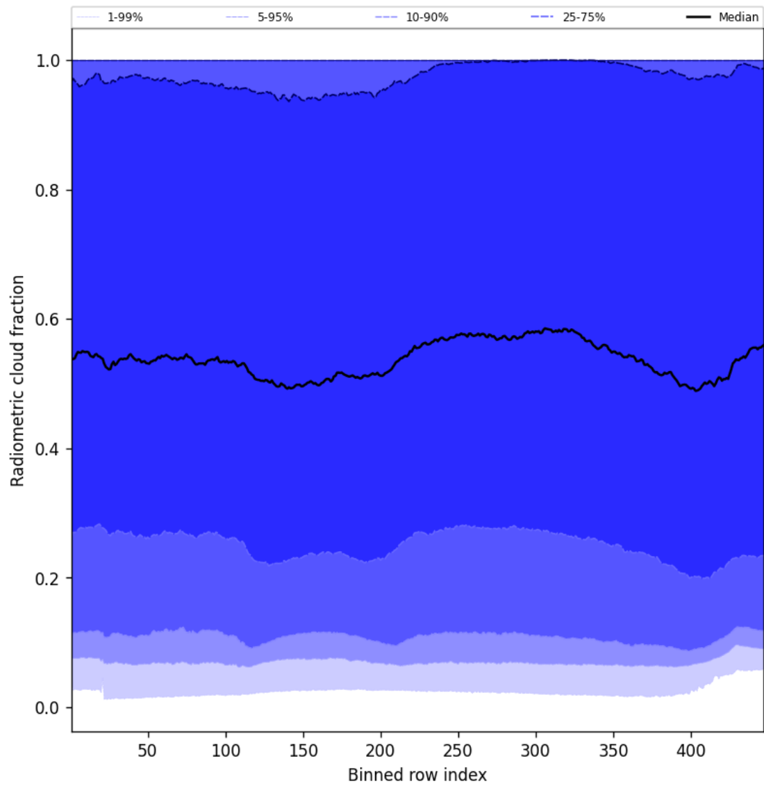
Figure 55: Along track statistics of “Radiometric cloud fraction” for 2025-02-11 to 2025-02-13
