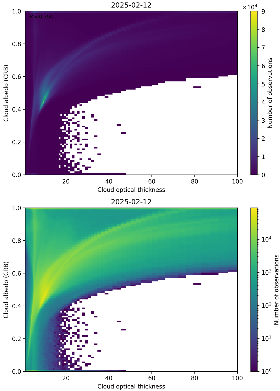
Figure 82: Scatter density plot of “Cloud optical thickness” against “Cloud albedo (CRB)” for 2025-02-11 to 2025-02-13.
