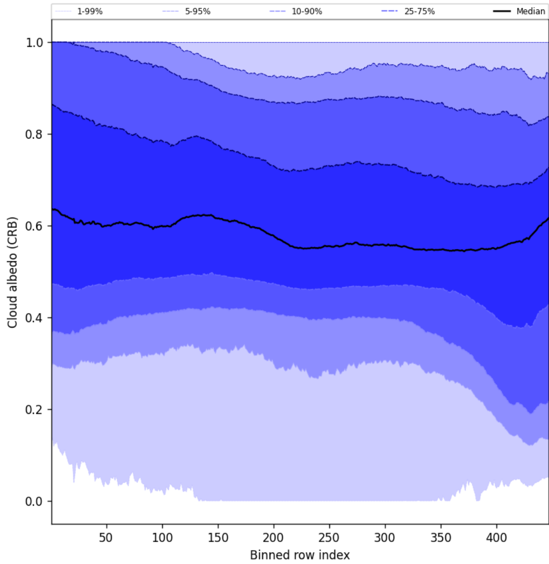
Figure 60: Along track statistics of “Cloud albedo (CRB)” for 2025-02-11 to 2025-02-13
