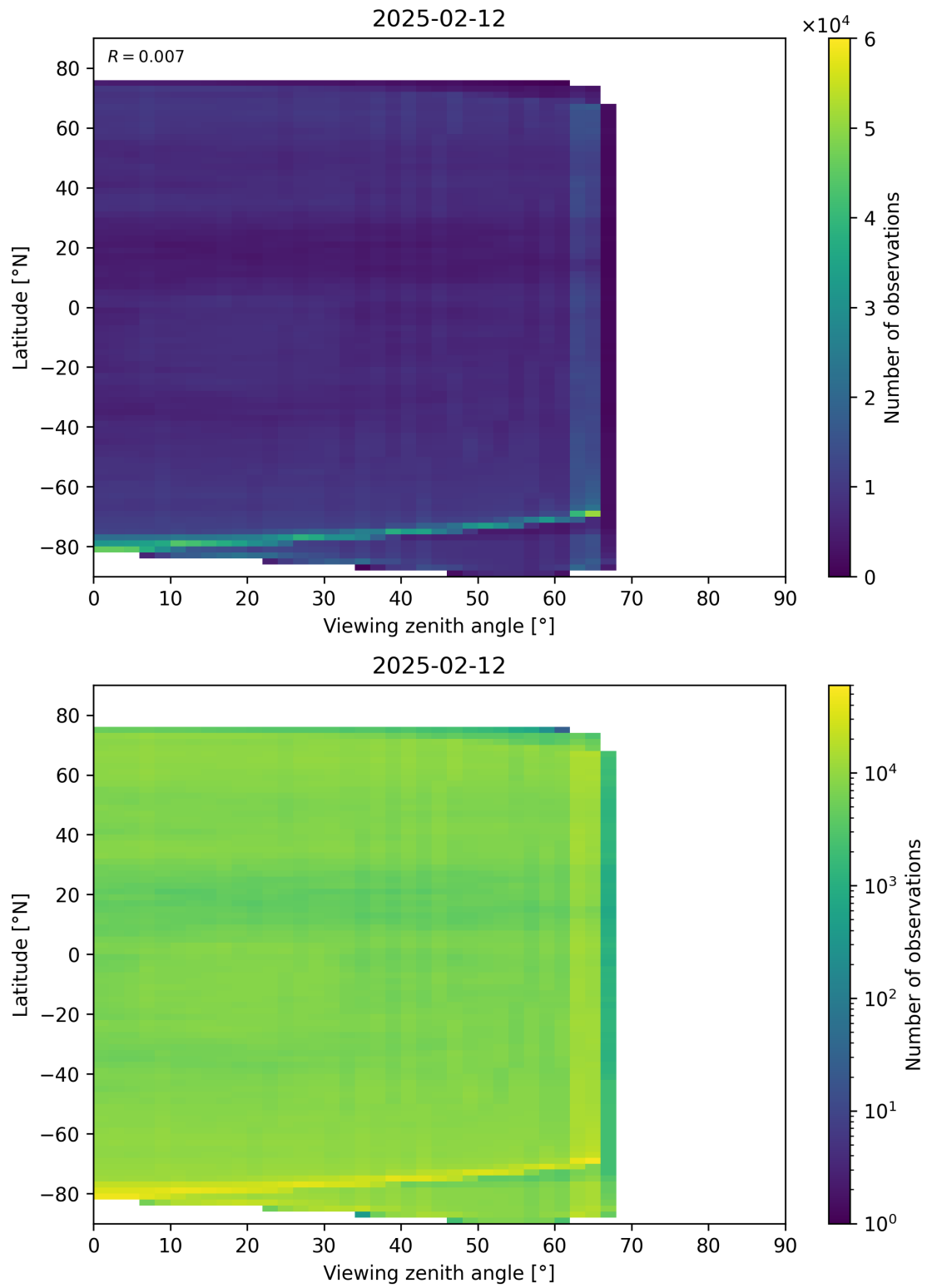
Figure 113: Scatter density plot of “Viewing zenith angle” against “Latitude” for 2025-02-11 to 2025-02-13.
