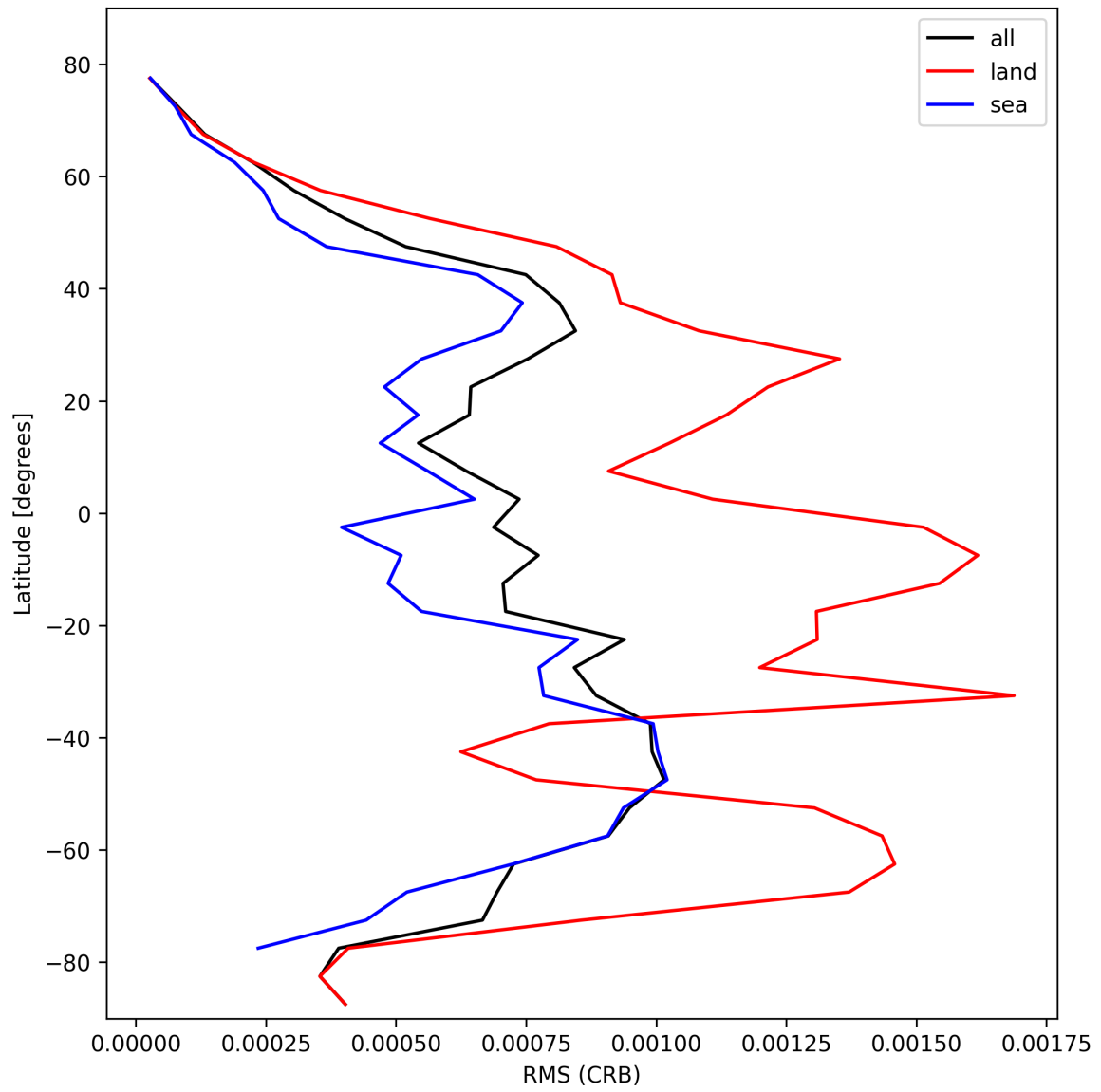
Figure 32: Zonal average of “RMS (CRB)” for 2025-02-11 to 2025-02-13.
