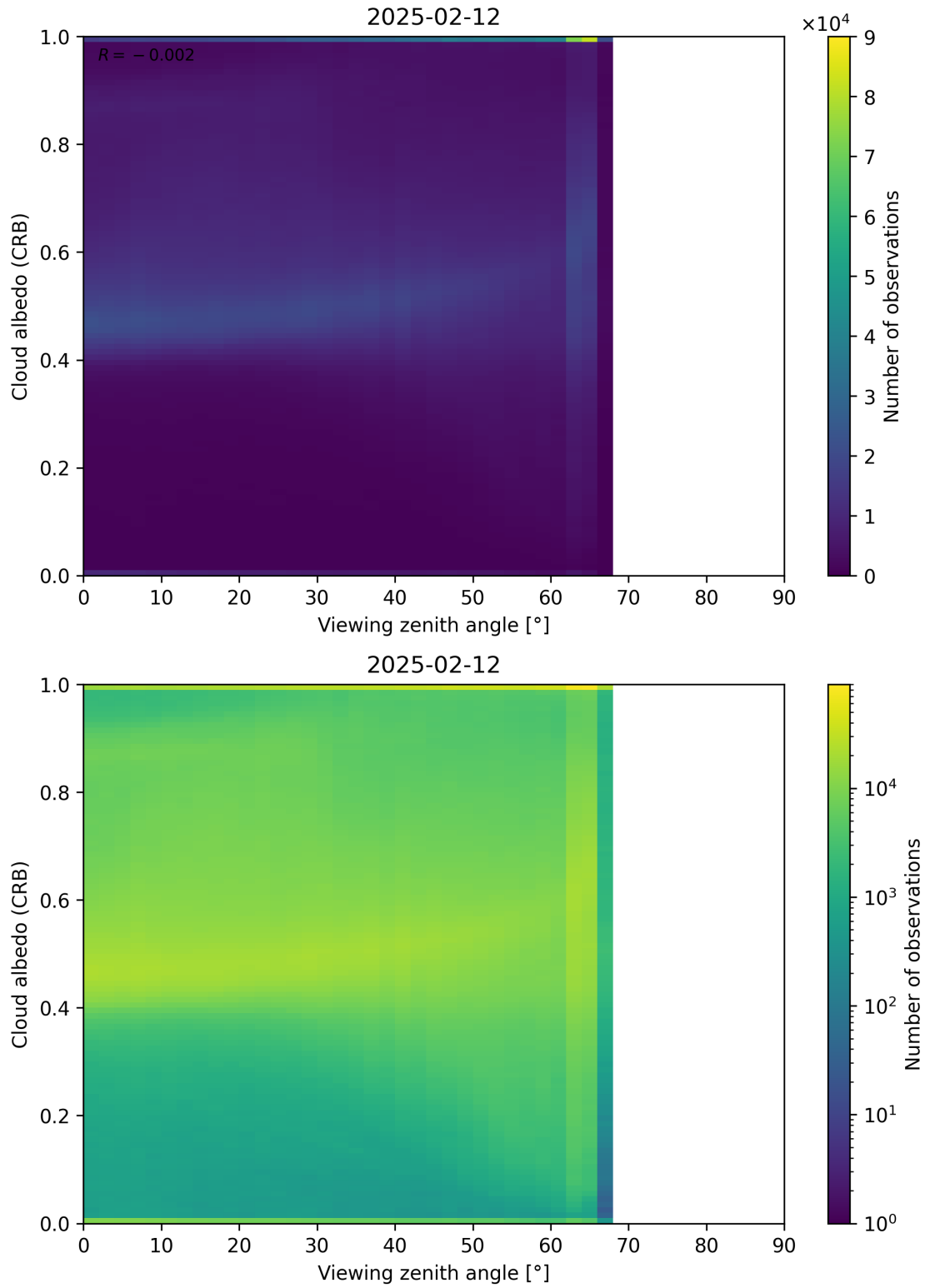
Figure 106: Scatter density plot of “Viewing zenith angle” against “Cloud albedo (CRB)” for 2025-02-11 to 2025-02-13.
