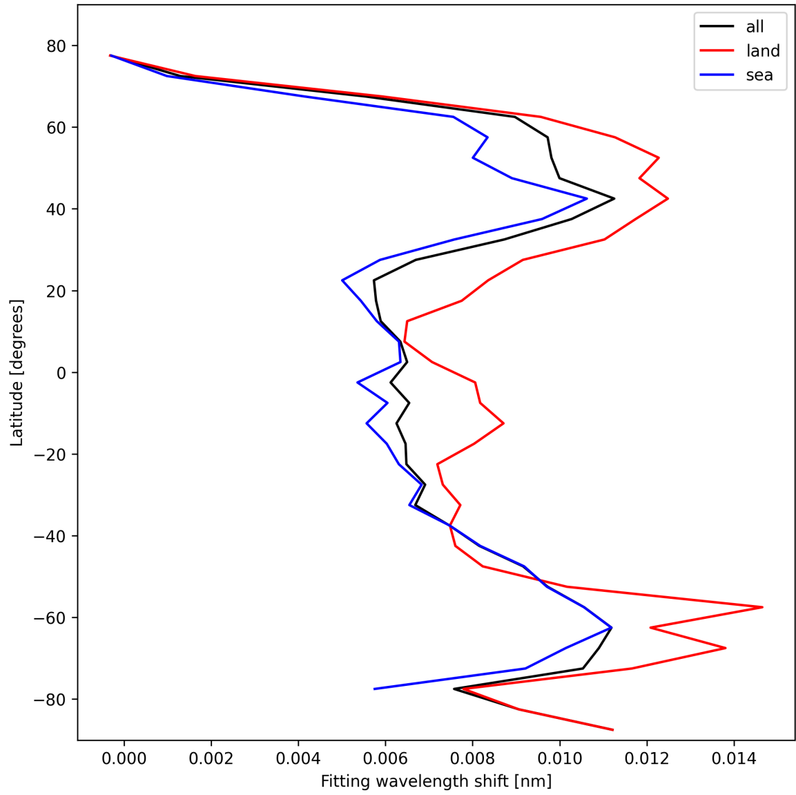
Figure 33: Zonal average of “Fitting wavelength shift” for 2025-02-11 to 2025-02-13.
