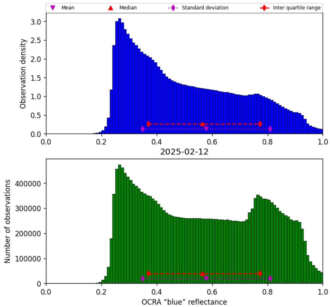
Figure 51: Histogram of “OCRA “blue” reflectance” for 2025-02-11 to 2025-02-13
