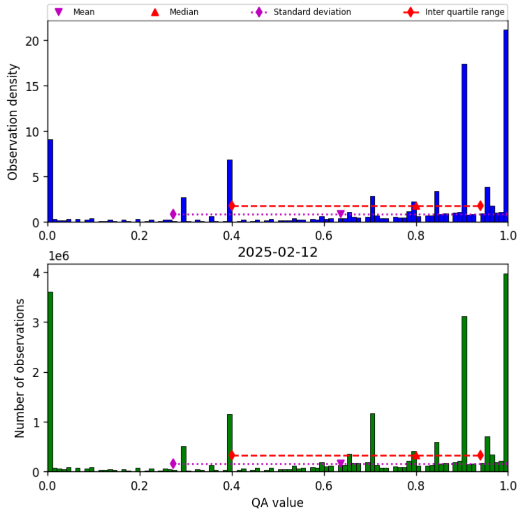
Figure 38: Histogram of “QA value” for 2025-02-11 to 2025-02-13
