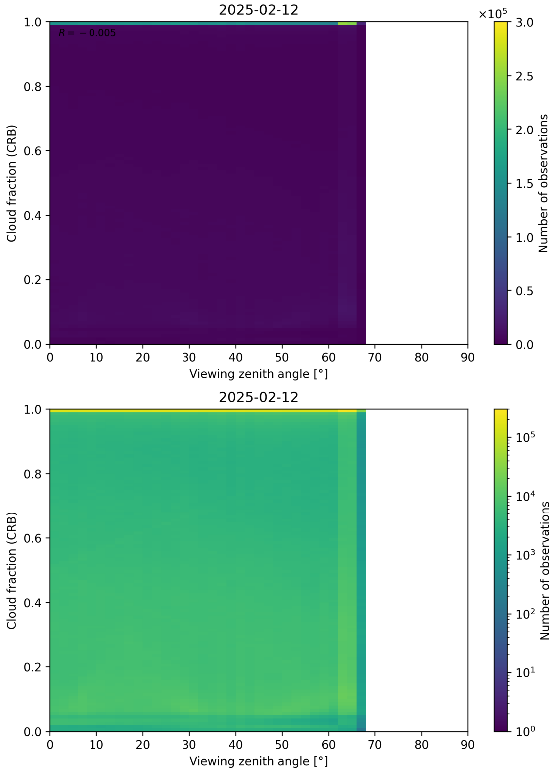
Figure 109: Scatter density plot of “Viewing zenith angle” against “Cloud fraction (CRB)” for 2025-02-11 to 2025-02-13.
