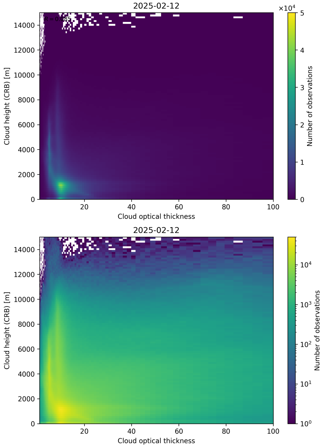
Figure 85: Scatter density plot of “Cloud optical thickness” against “Cloud height (CRB)” for 2025-02-11 to 2025-02-13.
