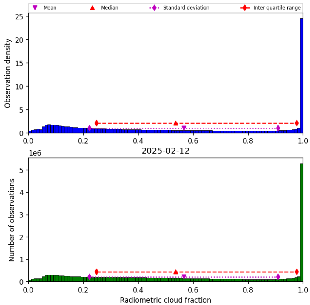
Figure 39: Histogram of “Radiometric cloud fraction” for 2025-02-11 to 2025-02-13
