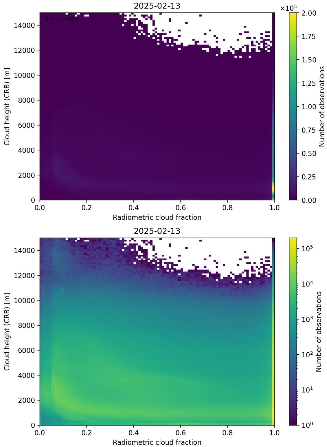
Figure 74: Scatter density plot of “Radiometric cloud fraction” against “Cloud height (CRB)” for 2025-02-13 to 2025-02-14.
