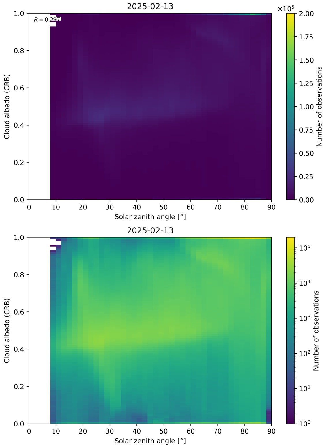
Figure 98: Scatter density plot of “Solar zenith angle” against “Cloud albedo (CRB)” for 2025-02-13 to 2025-02-14.
