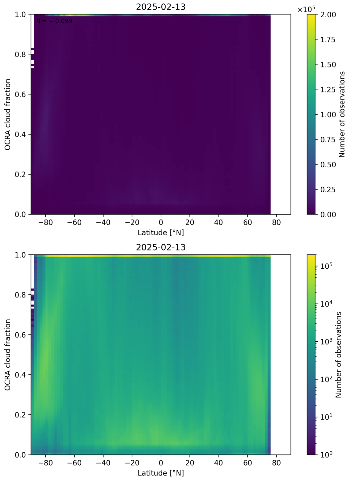
Figure 93: Scatter density plot of “Latitude” against “OCRA cloud fraction” for 2025-02-13 to 2025-02-14.
