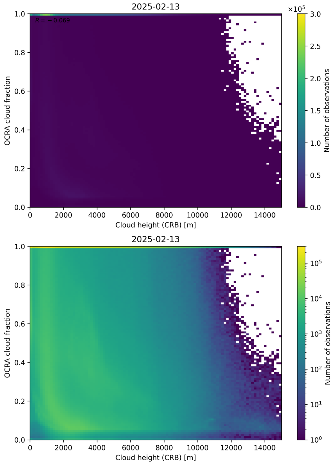
Figure 81: Scatter density plot of “Cloud height (CRB)” against “OCRA cloud fraction” for 2025-02-13 to 2025-02-14.
