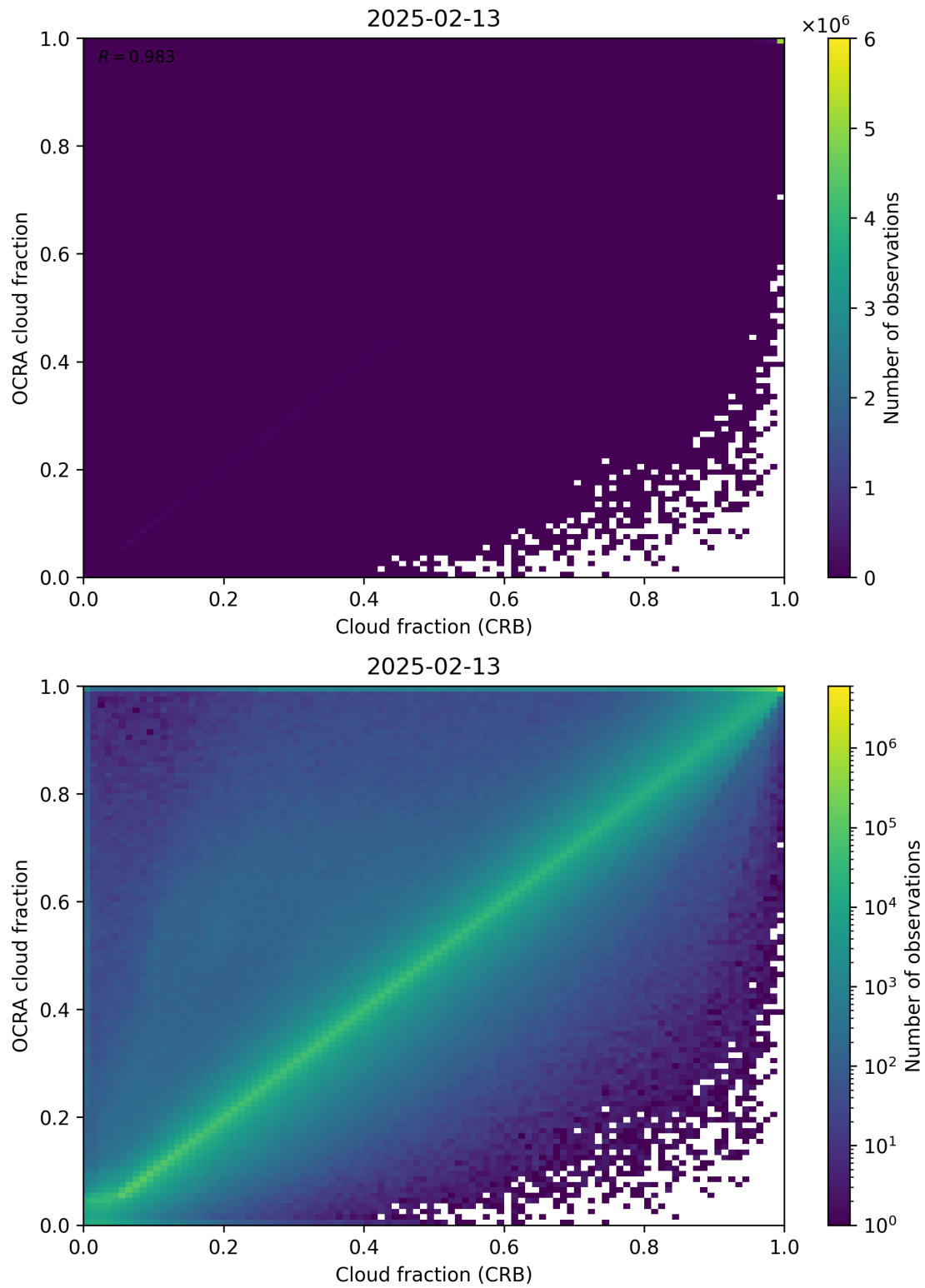
Figure 78: Scatter density plot of “Cloud fraction (CRB)” against “OCRA cloud fraction” for 2025-02-13 to 2025-02-14.
