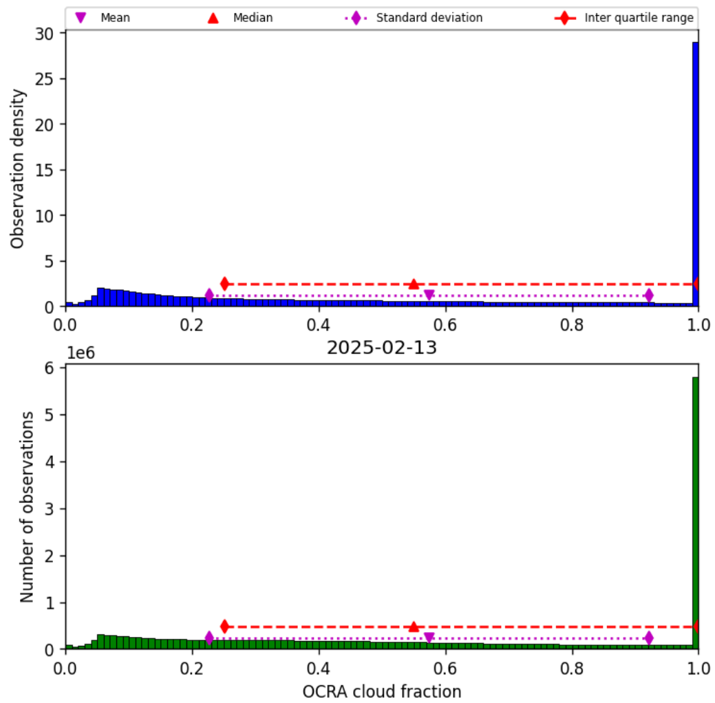
Figure 50: Histogram of “OCRA cloud fraction” for 2025-02-13 to 2025-02-14
