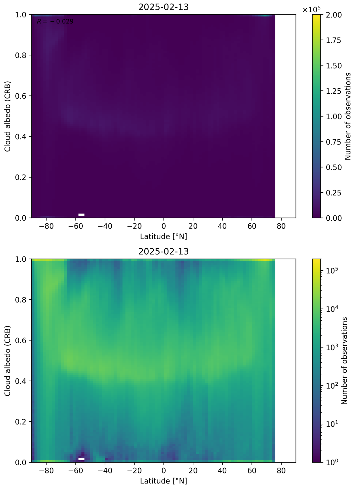
Figure 91: Scatter density plot of “Latitude” against “Cloud albedo (CRB)” for 2025-02-13 to 2025-02-14.
