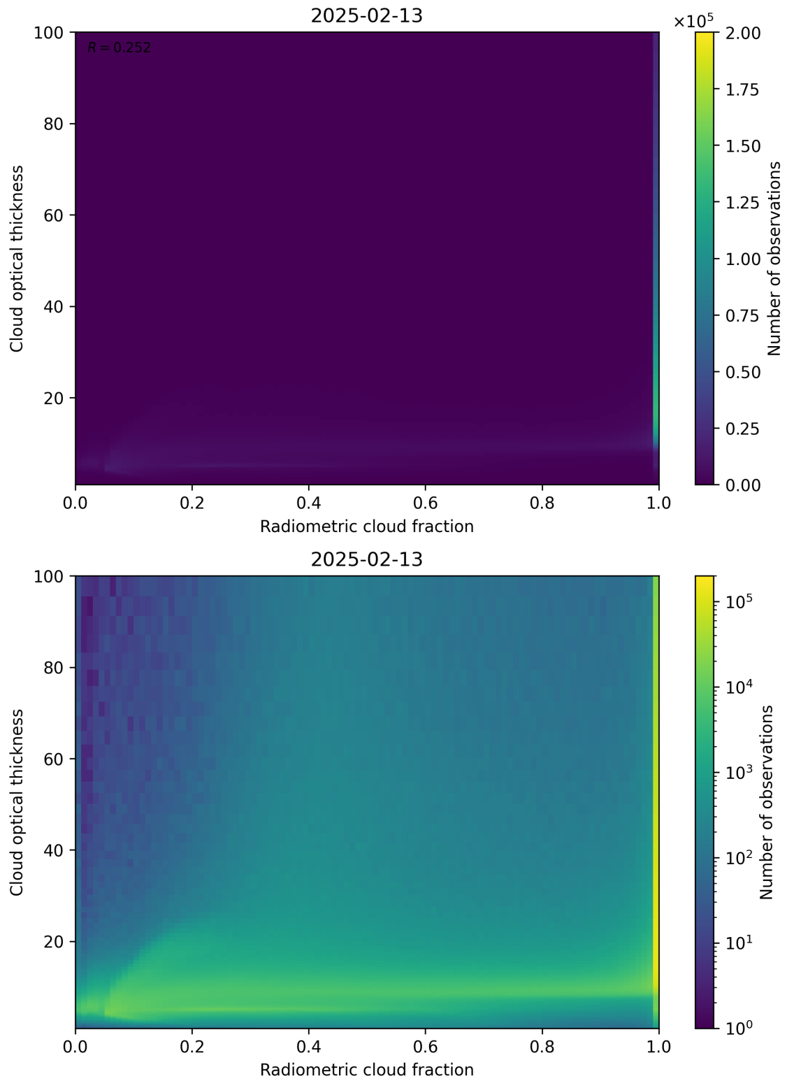
Figure 75: Scatter density plot of “Radiometric cloud fraction” against “Cloud optical thickness” for 2025-02-13 to 2025-02-14.
