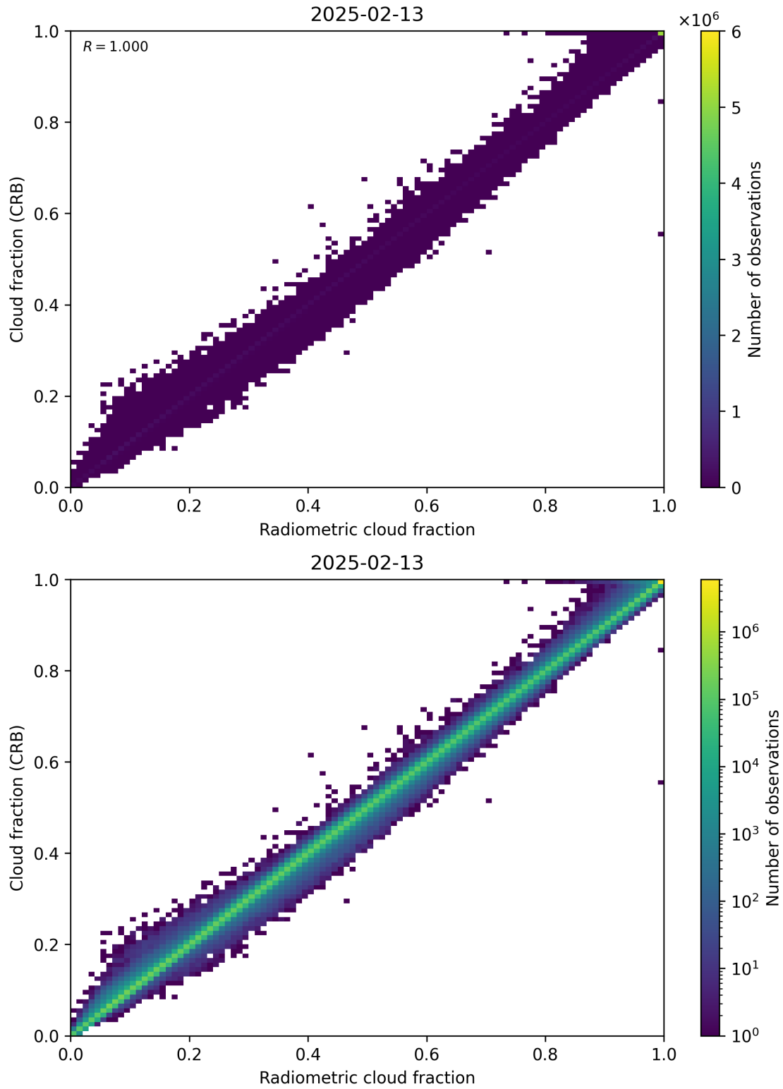
Figure 73: Scatter density plot of “Radiometric cloud fraction” against “Cloud fraction (CRB)” for 2025-02-13 to 2025-02-14.
