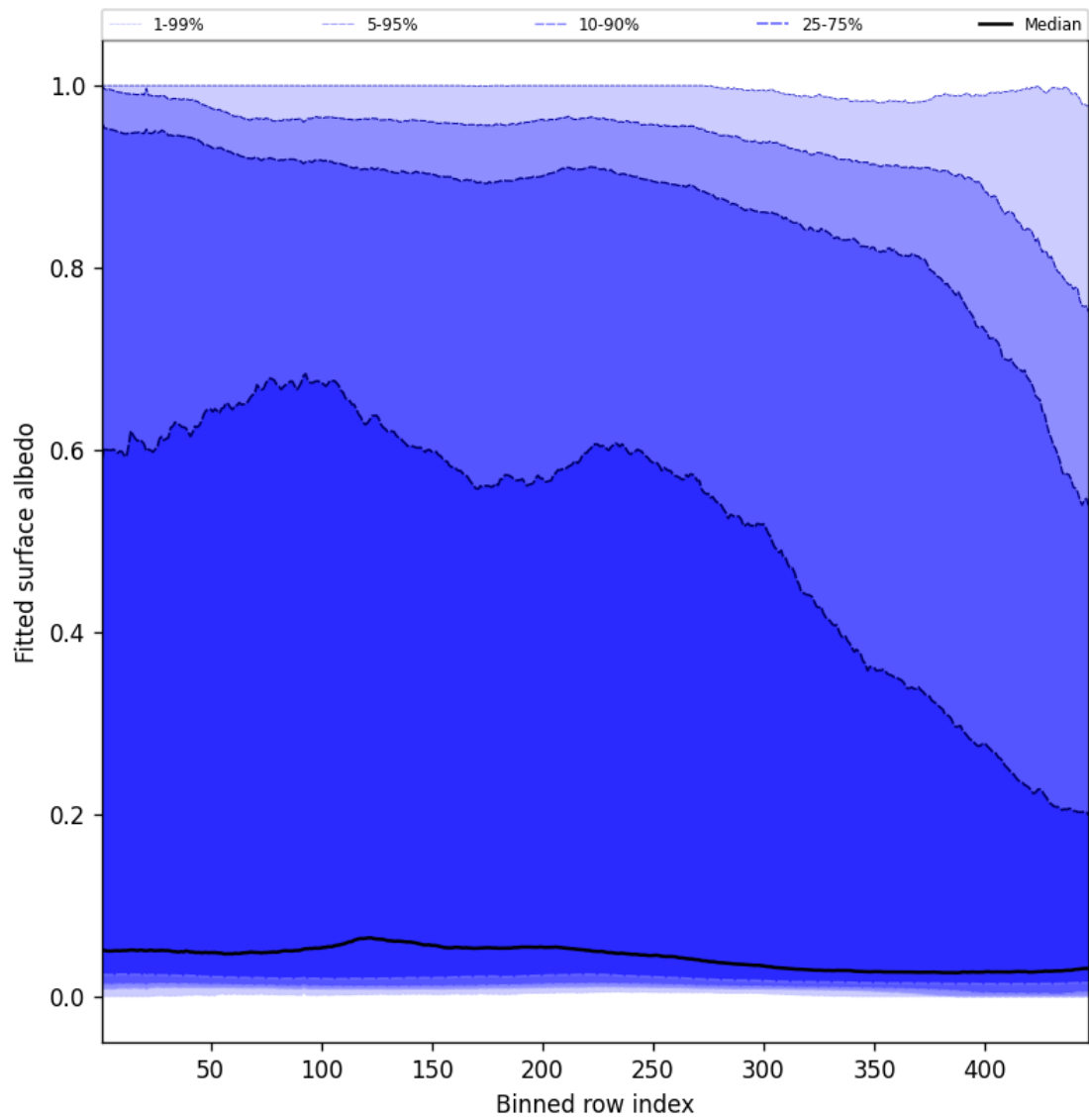
Figure 61: Along track statistics of “Fitted surface albedo” for 2025-02-13 to 2025-02-14
