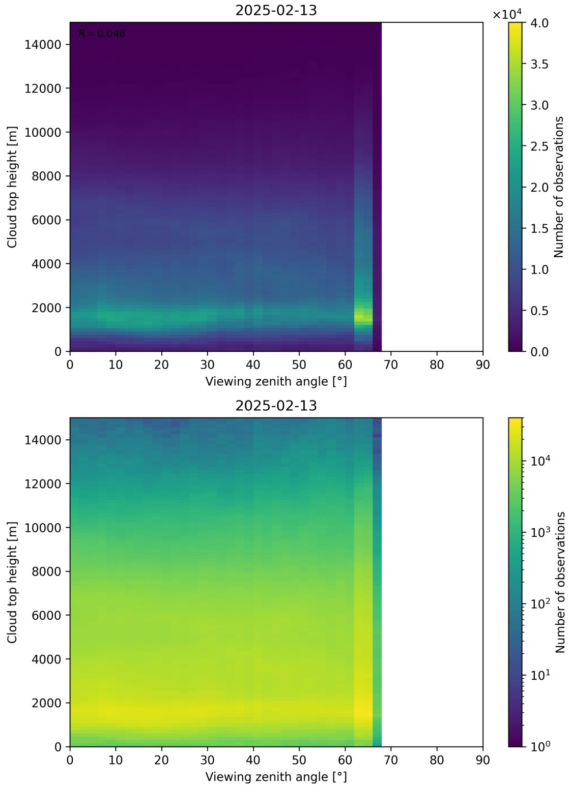
Figure 112: Scatter density plot of “Viewing zenith angle” against “Cloud top height” for 2025-02-13 to 2025-02-14.
