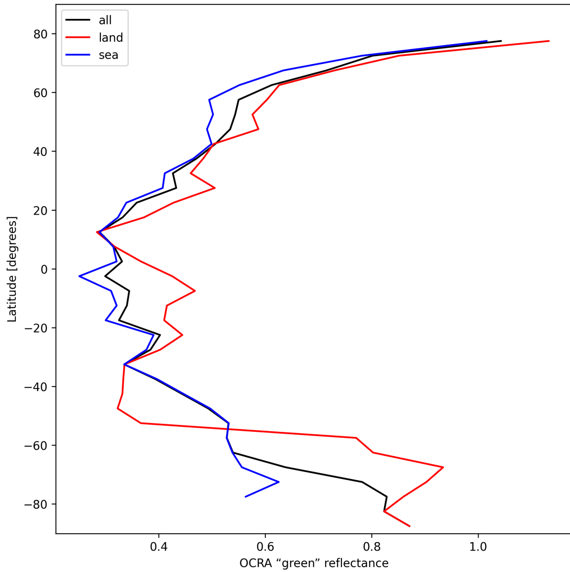
Figure 36: Zonal average of “OCRA “green” reflectance” for 2025-02-13 to 2025-02-14.
