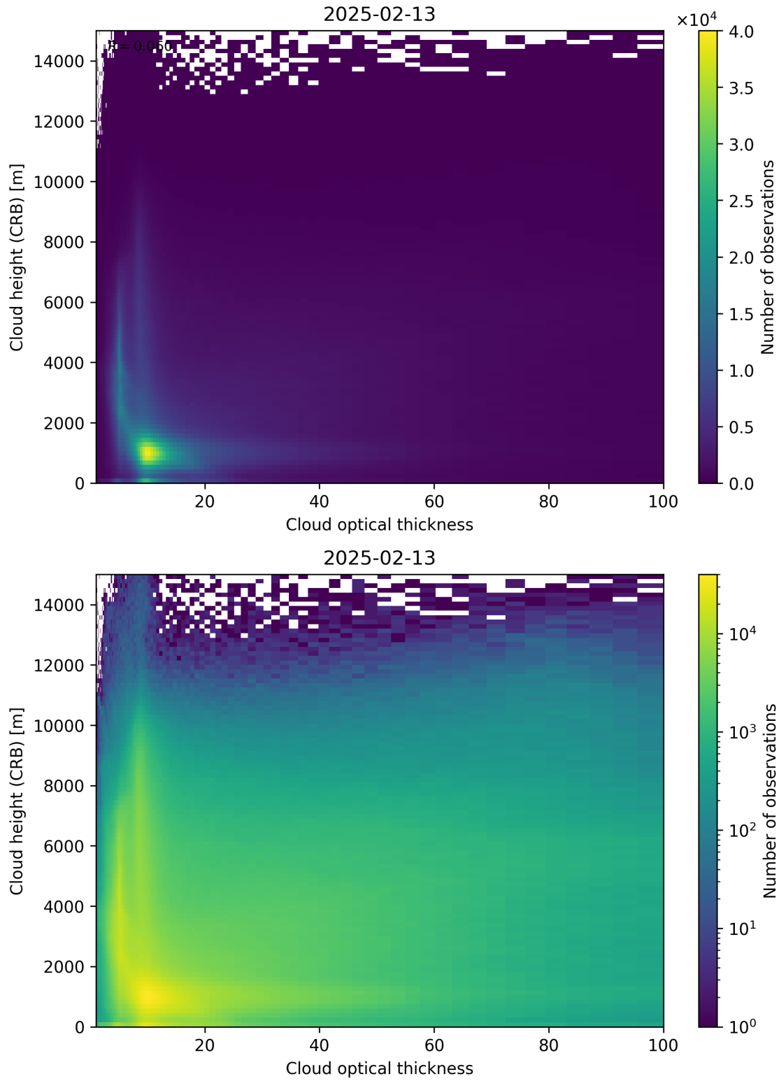
Figure 85: Scatter density plot of “Cloud optical thickness” against “Cloud height (CRB)” for 2025-02-13 to 2025-02-14.
