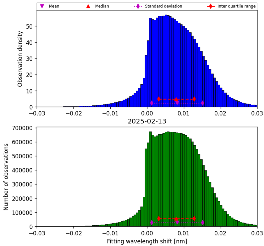
Figure 49: Histogram of “Fitting wavelength shift” for 2025-02-13 to 2025-02-14
