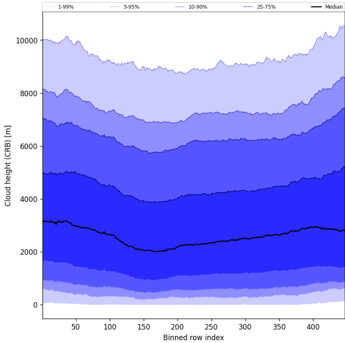
Figure 59: Along track statistics of “Cloud height (CRB)” for 2025-02-13 to 2025-02-14
