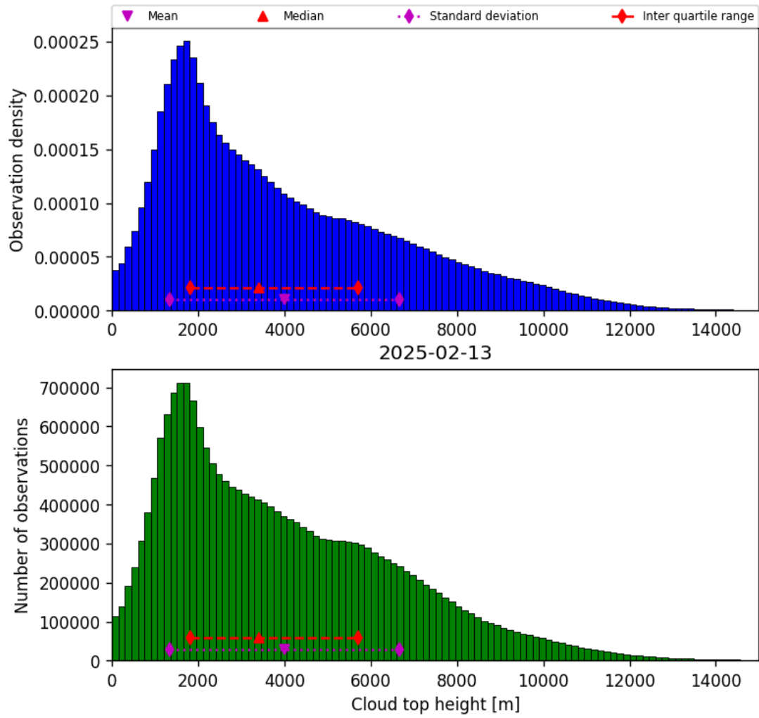
Figure 40: Histogram of “Cloud top height” for 2025-02-13 to 2025-02-14
