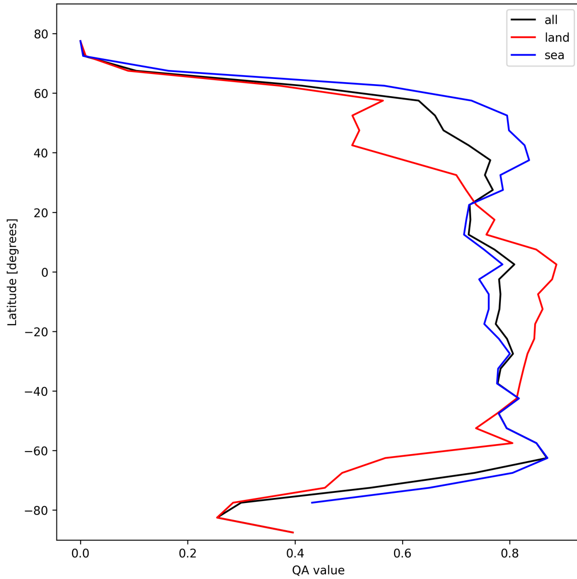
Figure 22: Zonal average of “QA value” for 2025-02-13 to 2025-02-14.
