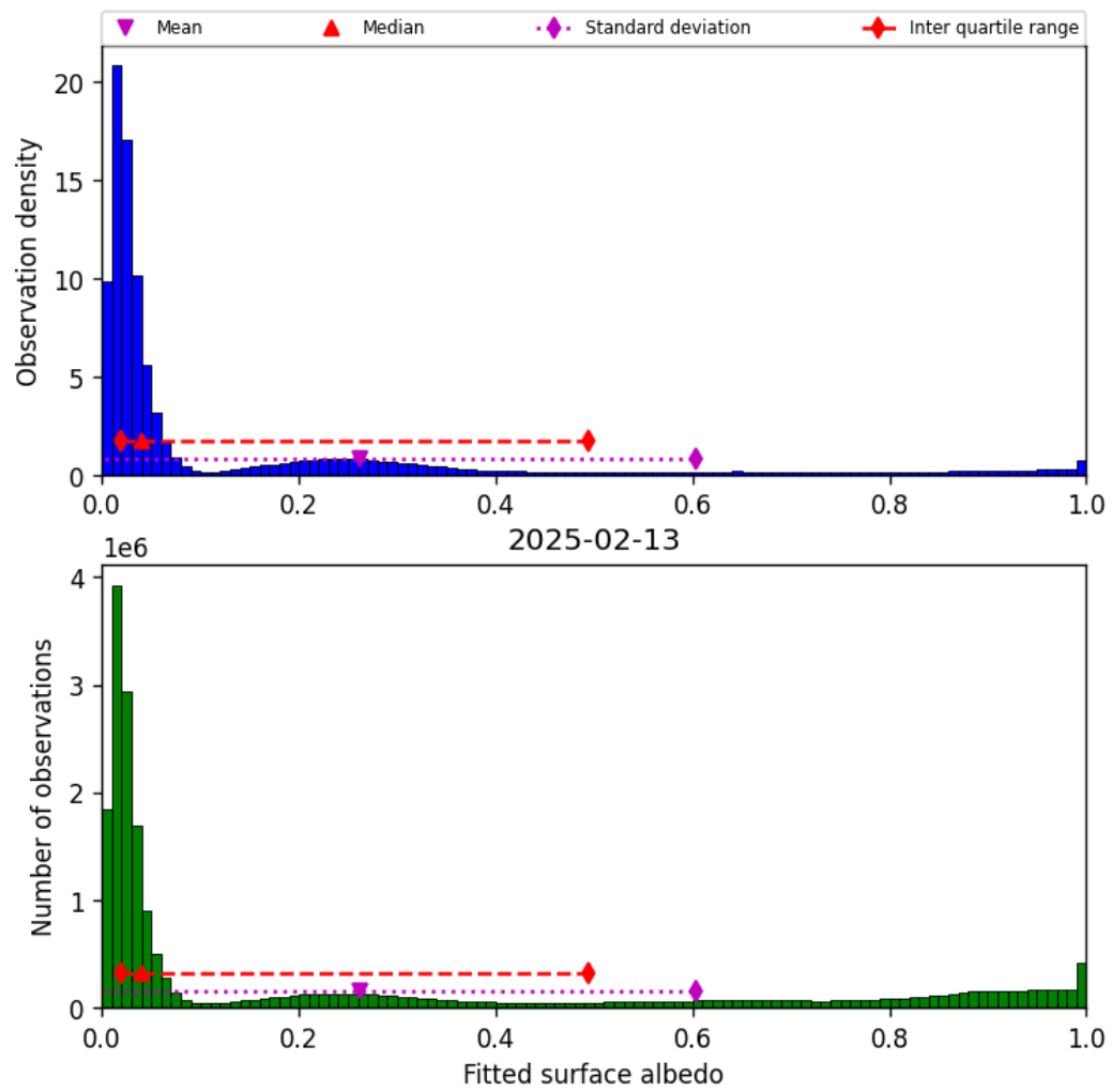
Figure 45: Histogram of “Fitted surface albedo” for 2025-02-13 to 2025-02-14
