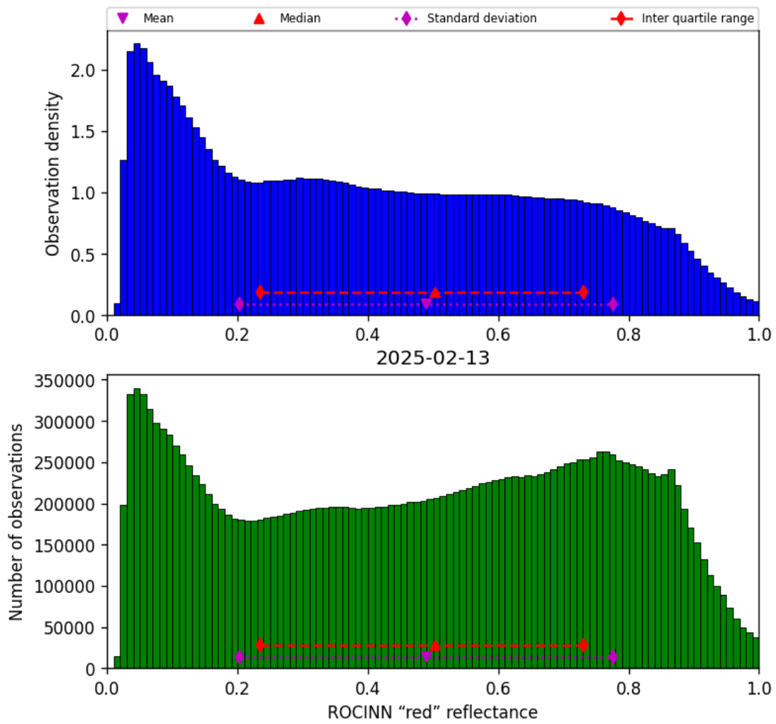
Figure 53: Histogram of “ROCINN “red” reflectance” for 2025-02-13 to 2025-02-14
