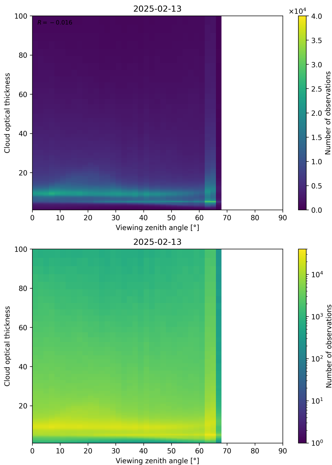
Figure 111: Scatter density plot of “Viewing zenith angle” against “Cloud optical thickness” for 2025-02-13 to 2025-02-14.
