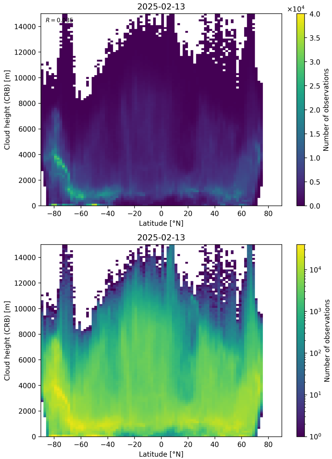
Figure 95: Scatter density plot of “Latitude” against “Cloud height (CRB)” for 2025-02-13 to 2025-02-14.
