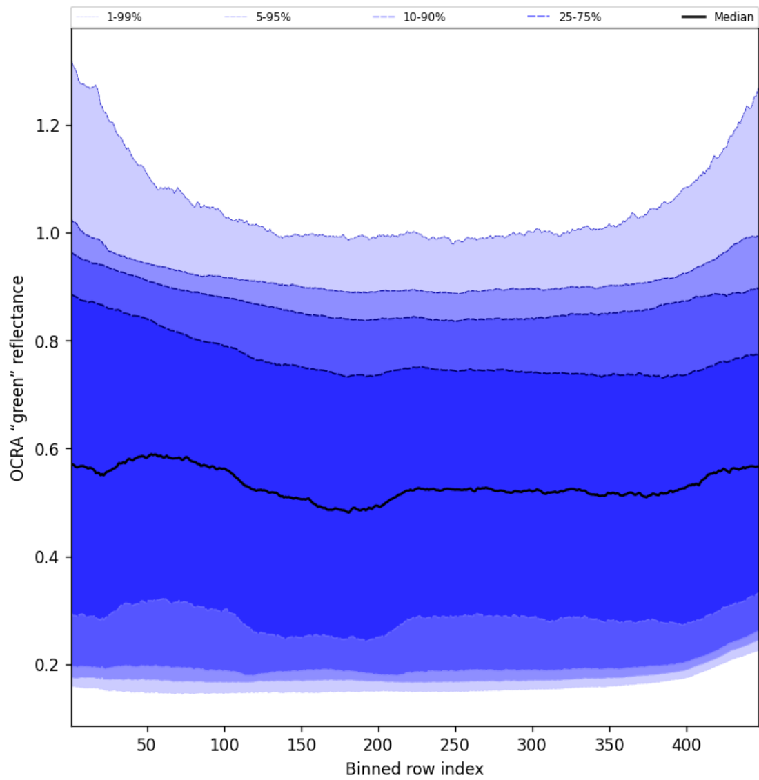
Figure 68: Along track statistics of “OCRA “green” reflectance” for 2025-02-13 to 2025-02-14
