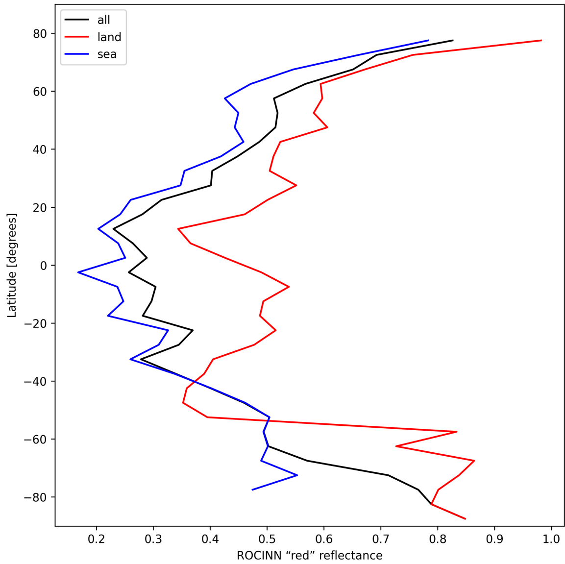
Figure 37: Zonal average of “ROCINN “red” reflectance” for 2025-02-13 to 2025-02-14.
