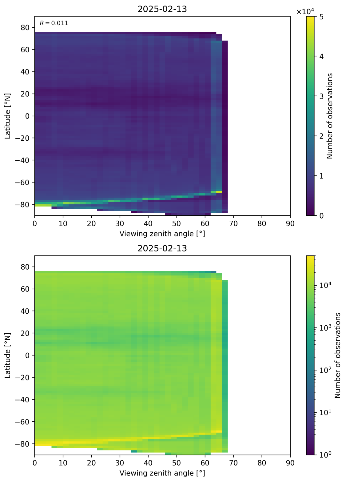
Figure 113: Scatter density plot of “Viewing zenith angle” against “Latitude” for 2025-02-13 to 2025-02-14.
