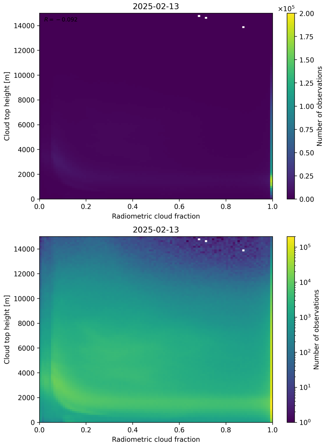
Figure 76: Scatter density plot of “Radiometric cloud fraction” against “Cloud top height” for 2025-02-13 to 2025-02-14.
