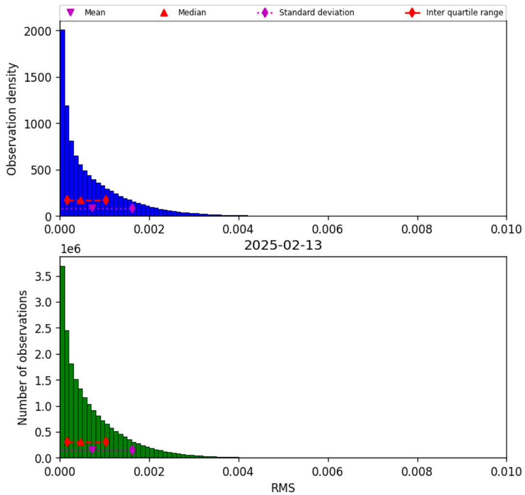
Figure 47: Histogram of “RMS” for 2025-02-13 to 2025-02-14
