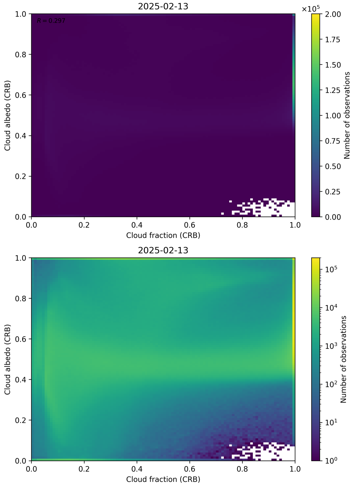
Figure 77: Scatter density plot of “Cloud fraction (CRB)” against “Cloud albedo (CRB)” for 2025-02-13 to 2025-02-14.
