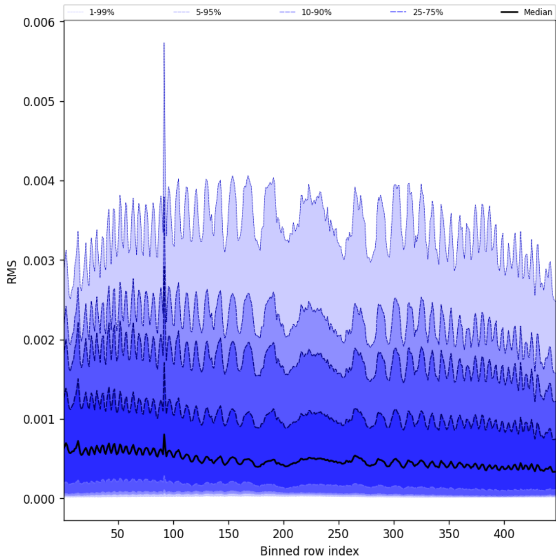
Figure 63: Along track statistics of “RMS” for 2025-02-13 to 2025-02-14
