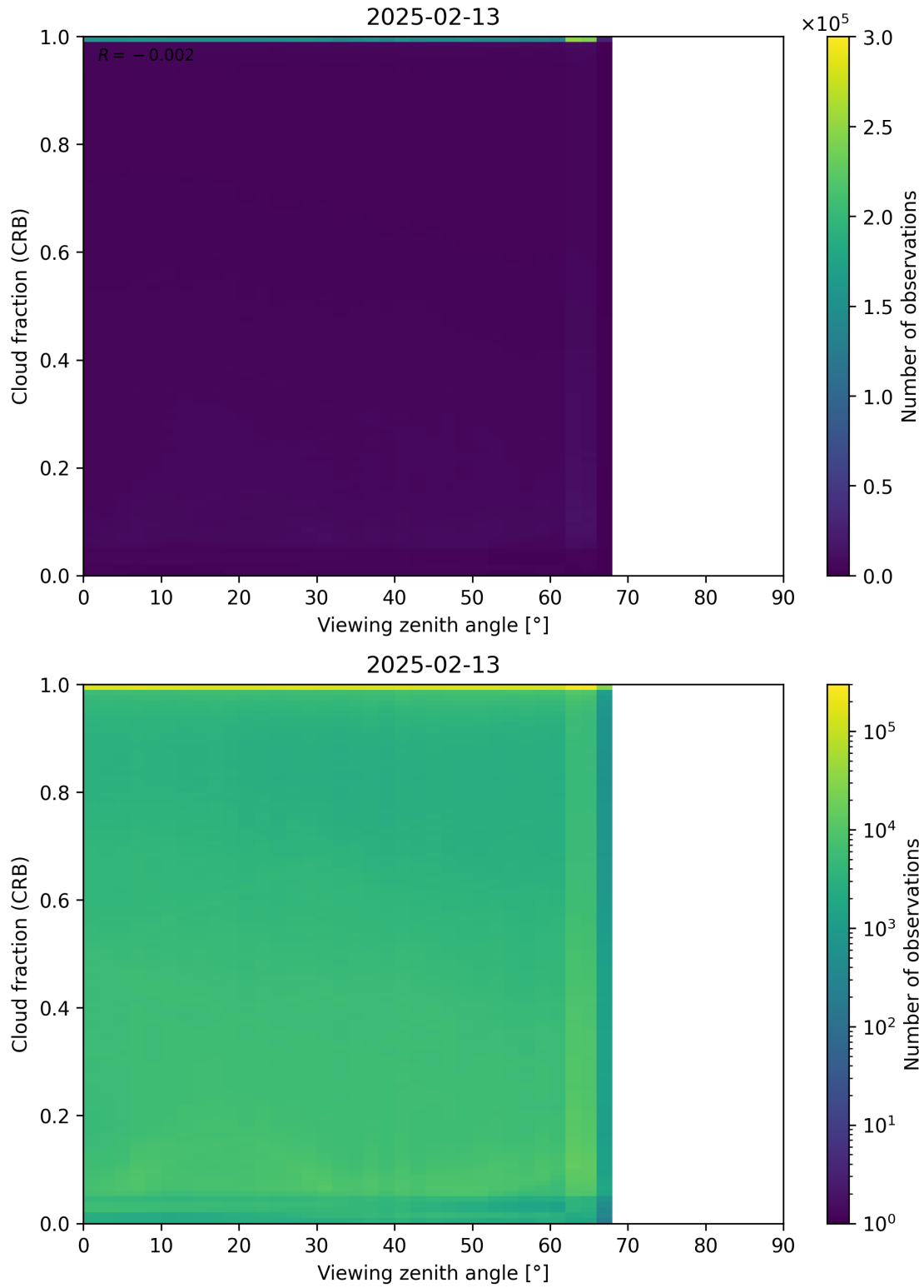
Figure 109: Scatter density plot of “Viewing zenith angle” against “Cloud fraction (CRB)” for 2025-02-13 to 2025-02-14.
