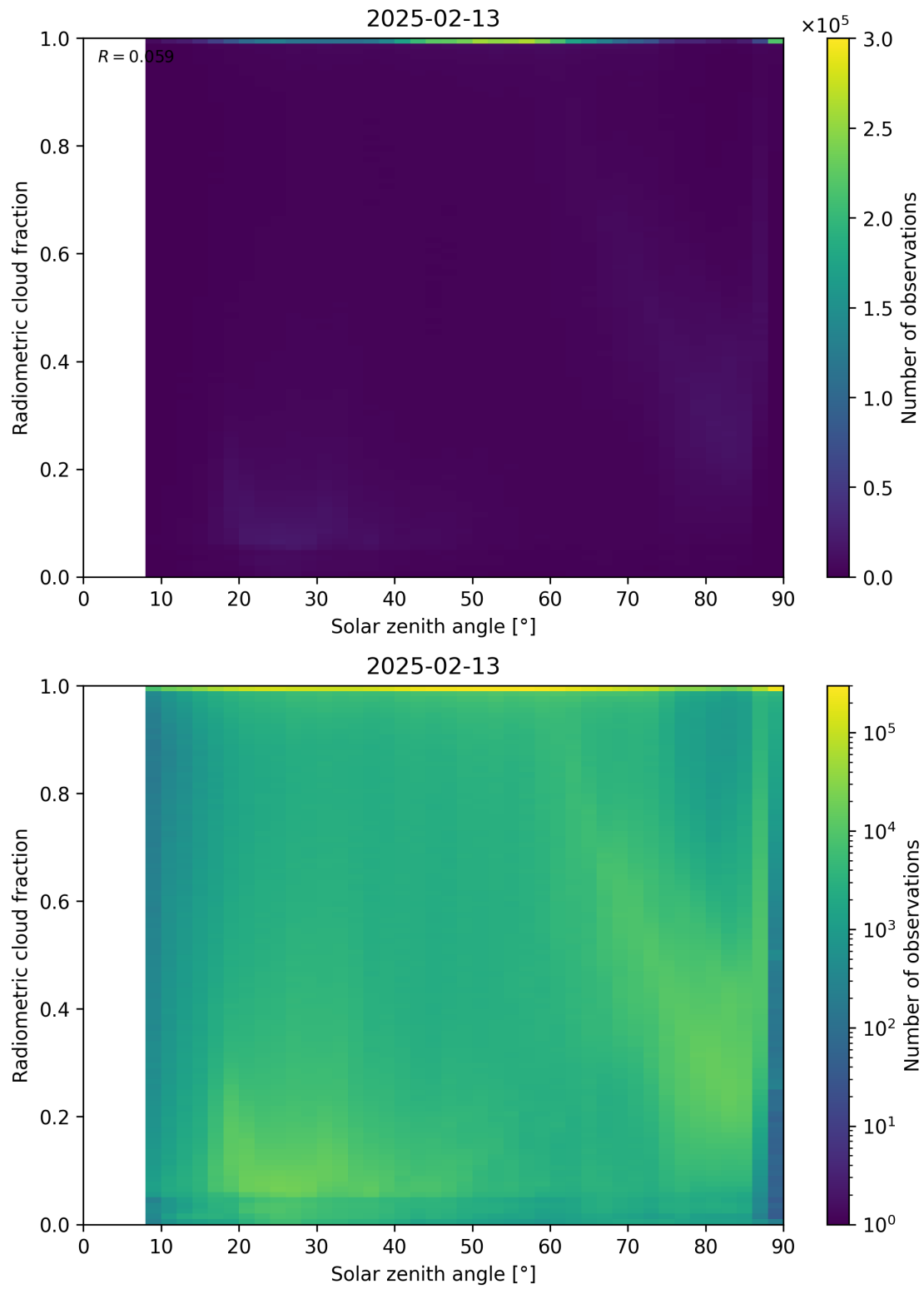
Figure 99: Scatter density plot of “Solar zenith angle” against “Radiometric cloud fraction” for 2025-02-13 to 2025-02-14.
