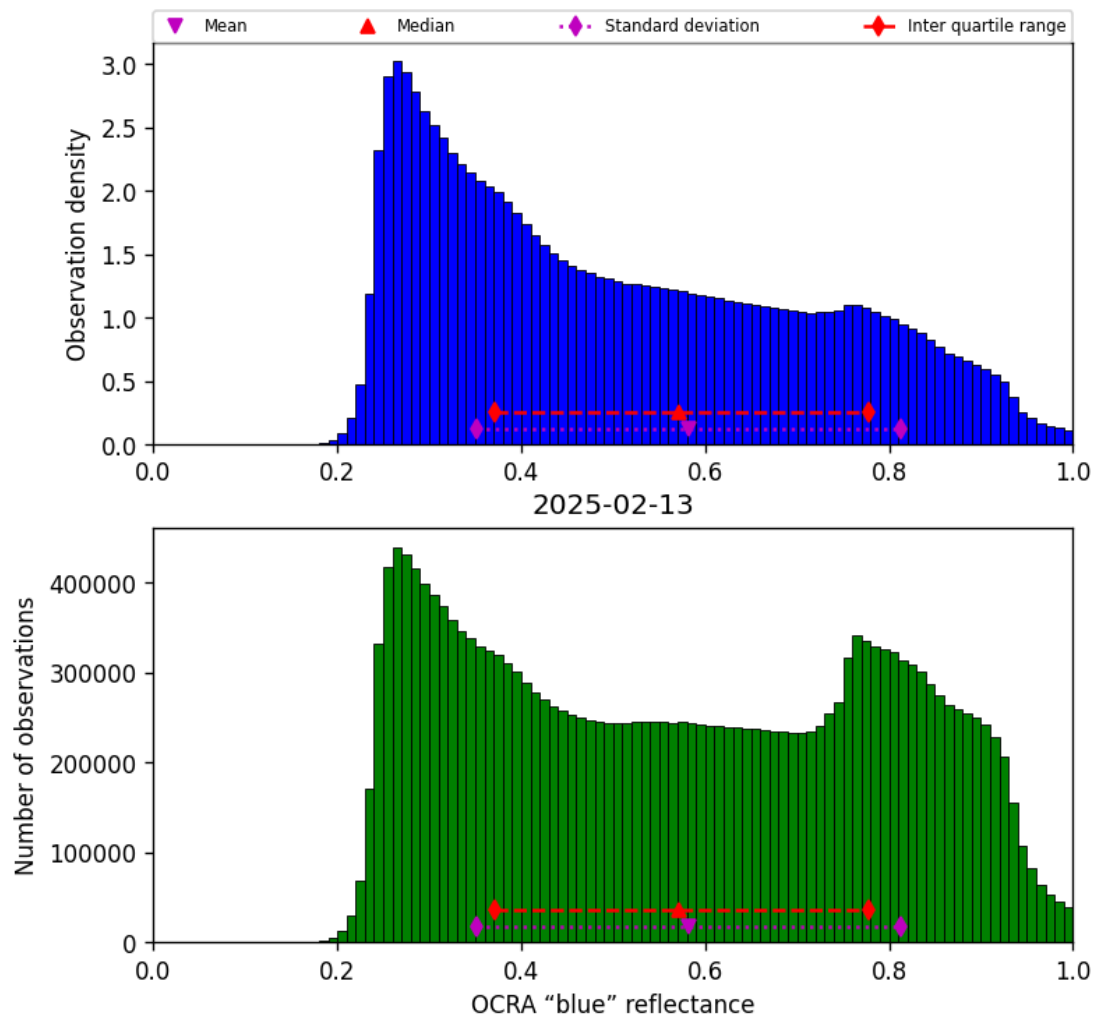
Figure 51: Histogram of “OCRA “blue” reflectance” for 2025-02-13 to 2025-02-14
