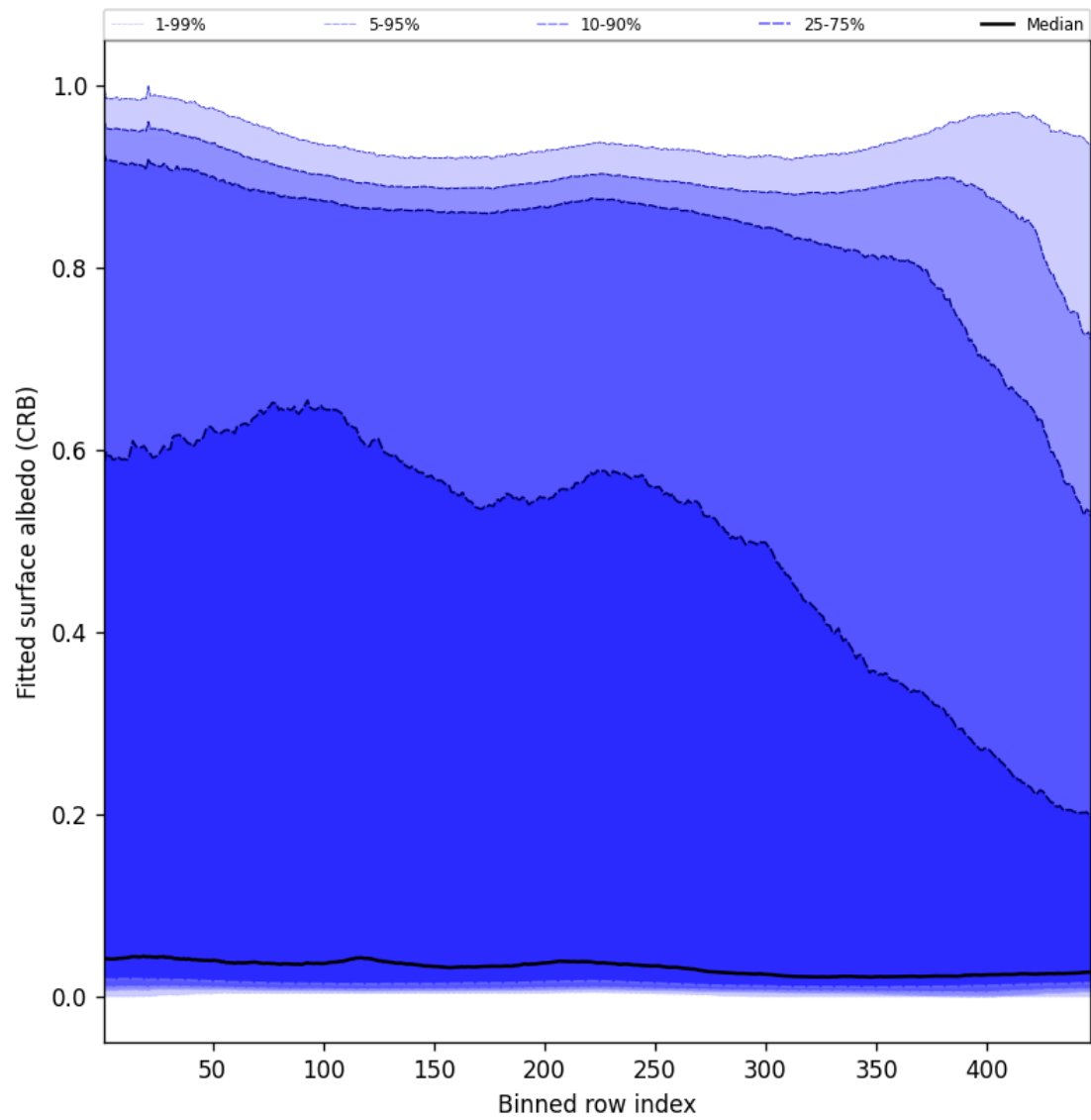
Figure 62: Along track statistics of “Fitted surface albedo (CRB)” for 2025-02-13 to 2025-02-14
