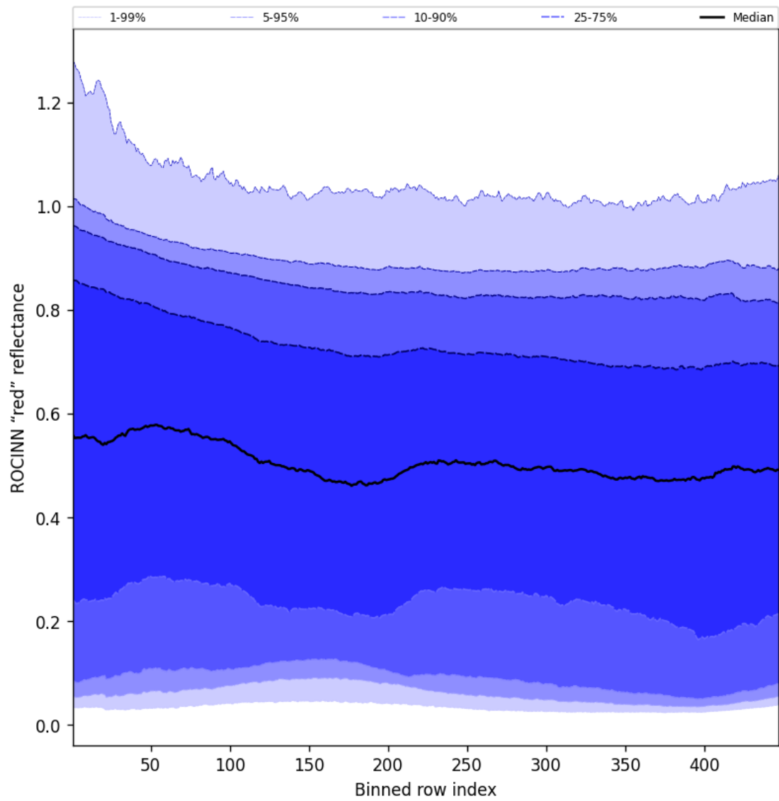
Figure 69: Along track statistics of "ROCINN "red" reflectance" for 2025-02-13 to 2025-02-14
