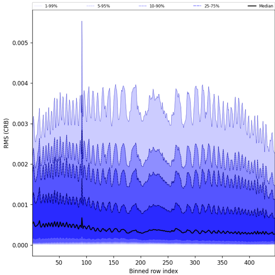
Figure 64: Along track statistics of “RMS (CRB)” for 2025-02-13 to 2025-02-14
