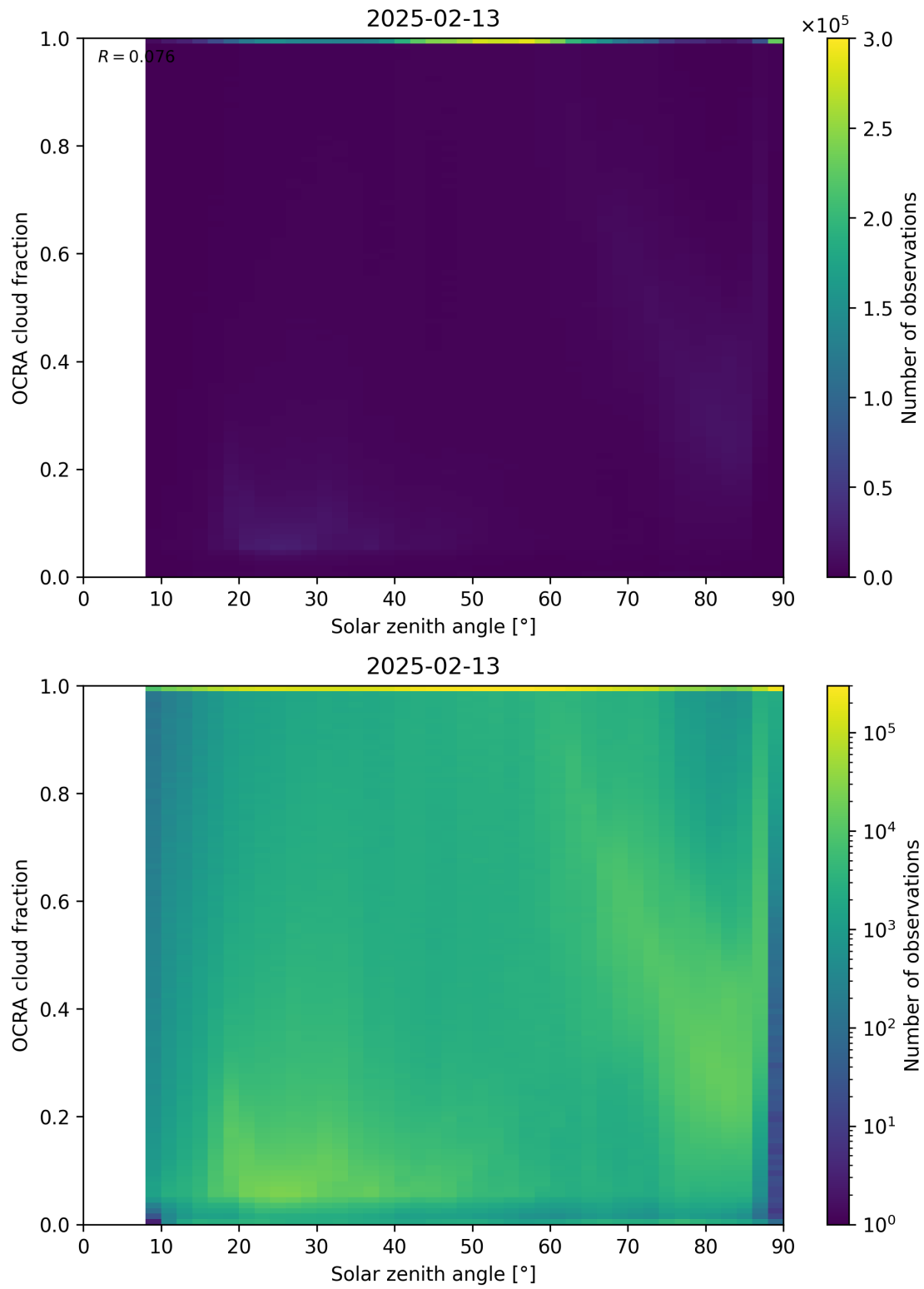
Figure 100: Scatter density plot of “Solar zenith angle” against “OCRA cloud fraction” for 2025-02-13 to 2025-02-14.
