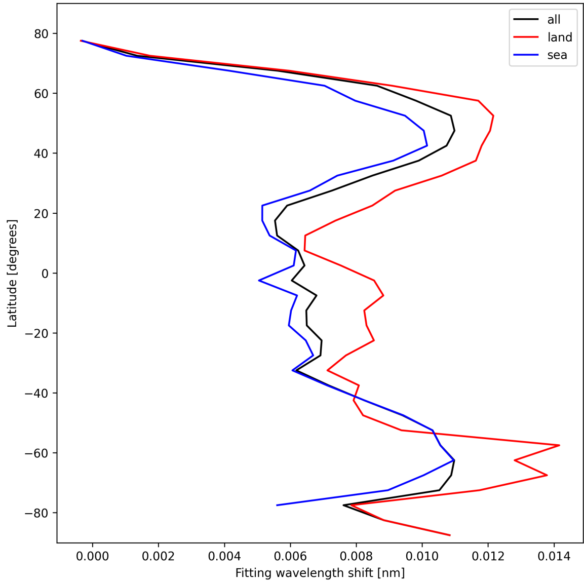
Figure 33: Zonal average of “Fitting wavelength shift” for 2025-02-13 to 2025-02-14.
