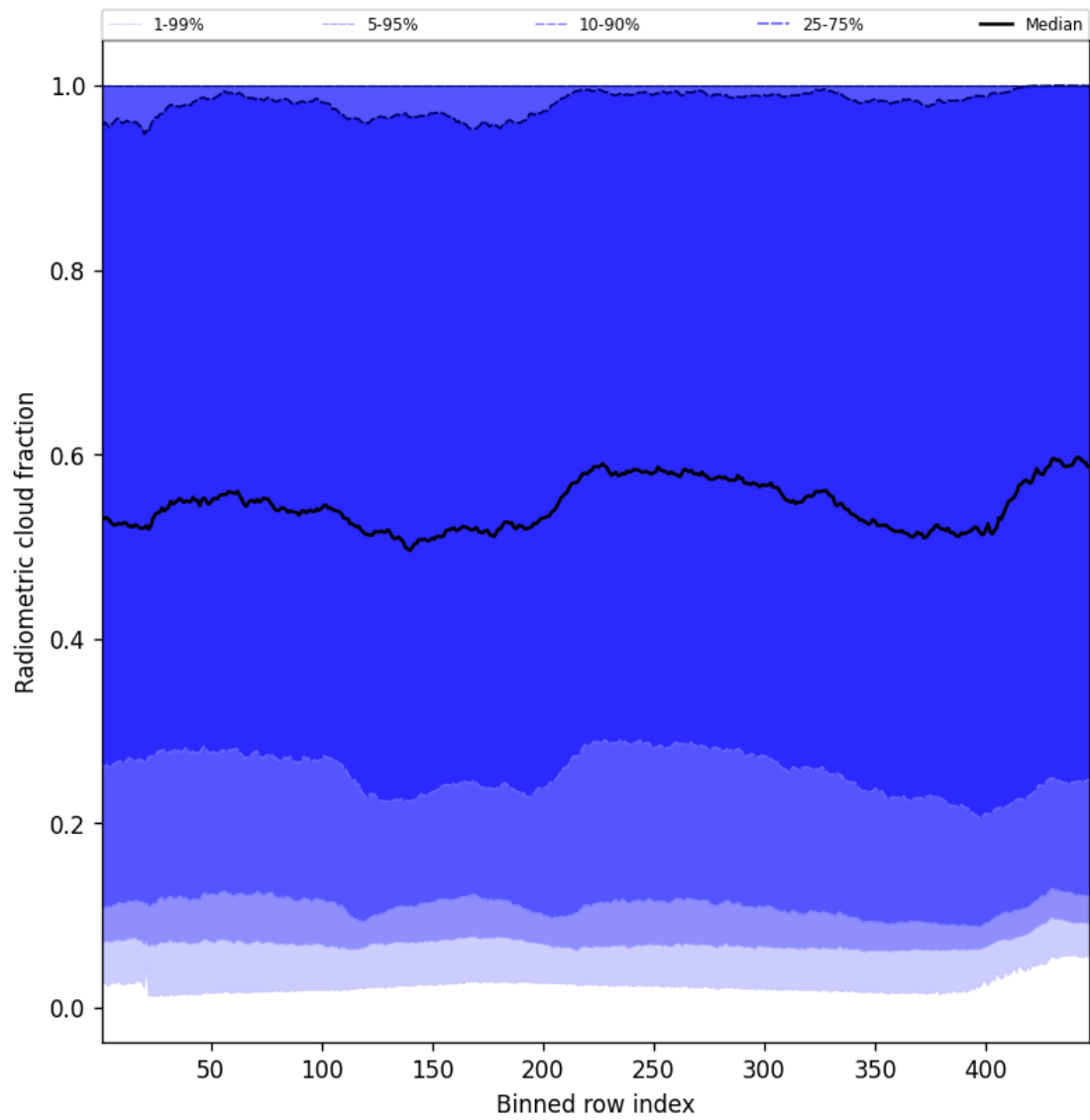
Figure 55: Along track statistics of “Radiometric cloud fraction” for 2025-02-13 to 2025-02-14
