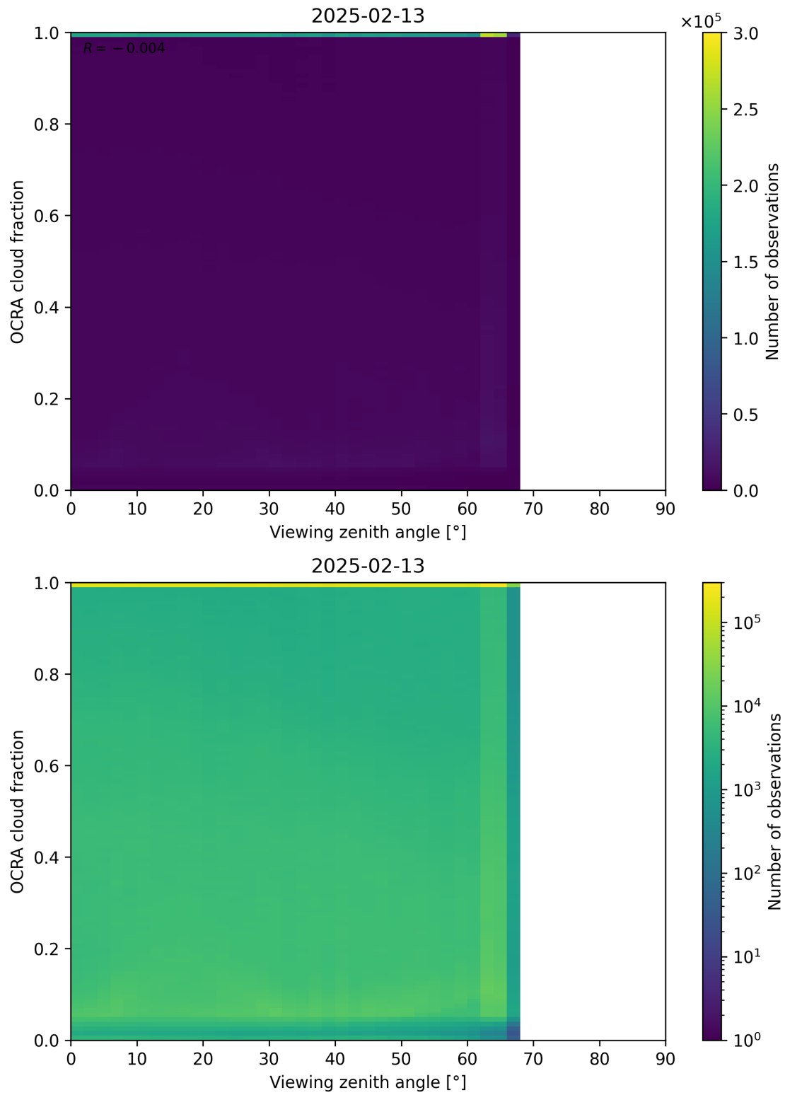
Figure 108: Scatter density plot of “Viewing zenith angle” against “OCRA cloud fraction” for 2025-02-13 to 2025-02-14.
