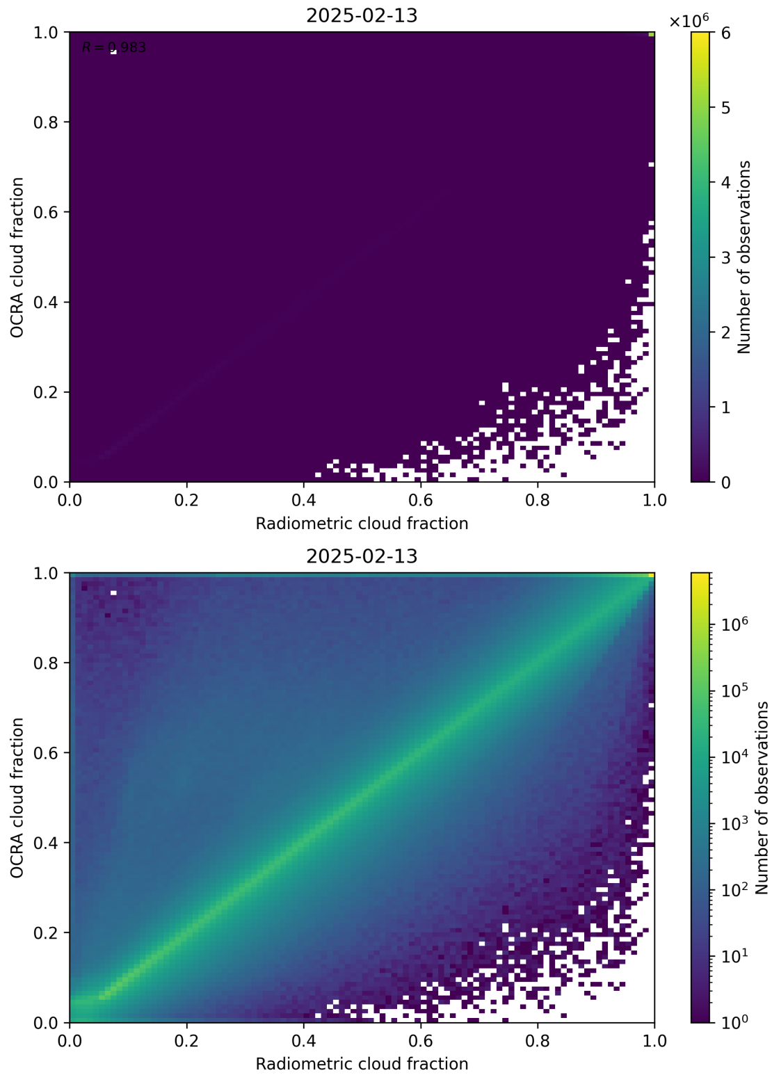
Figure 72: Scatter density plot of “Radiometric cloud fraction” against “OCRA cloud fraction” for 2025-02-13 to 2025-02-14.
