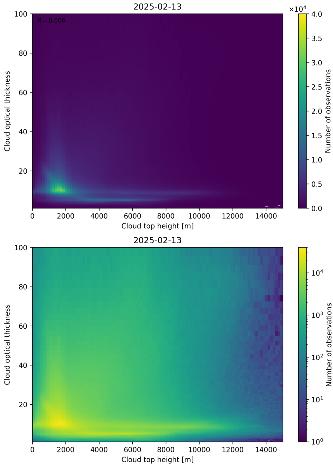
Figure 90: Scatter density plot of “Cloud top height” against “Cloud optical thickness” for 2025-02-13 to 2025-02-14.
