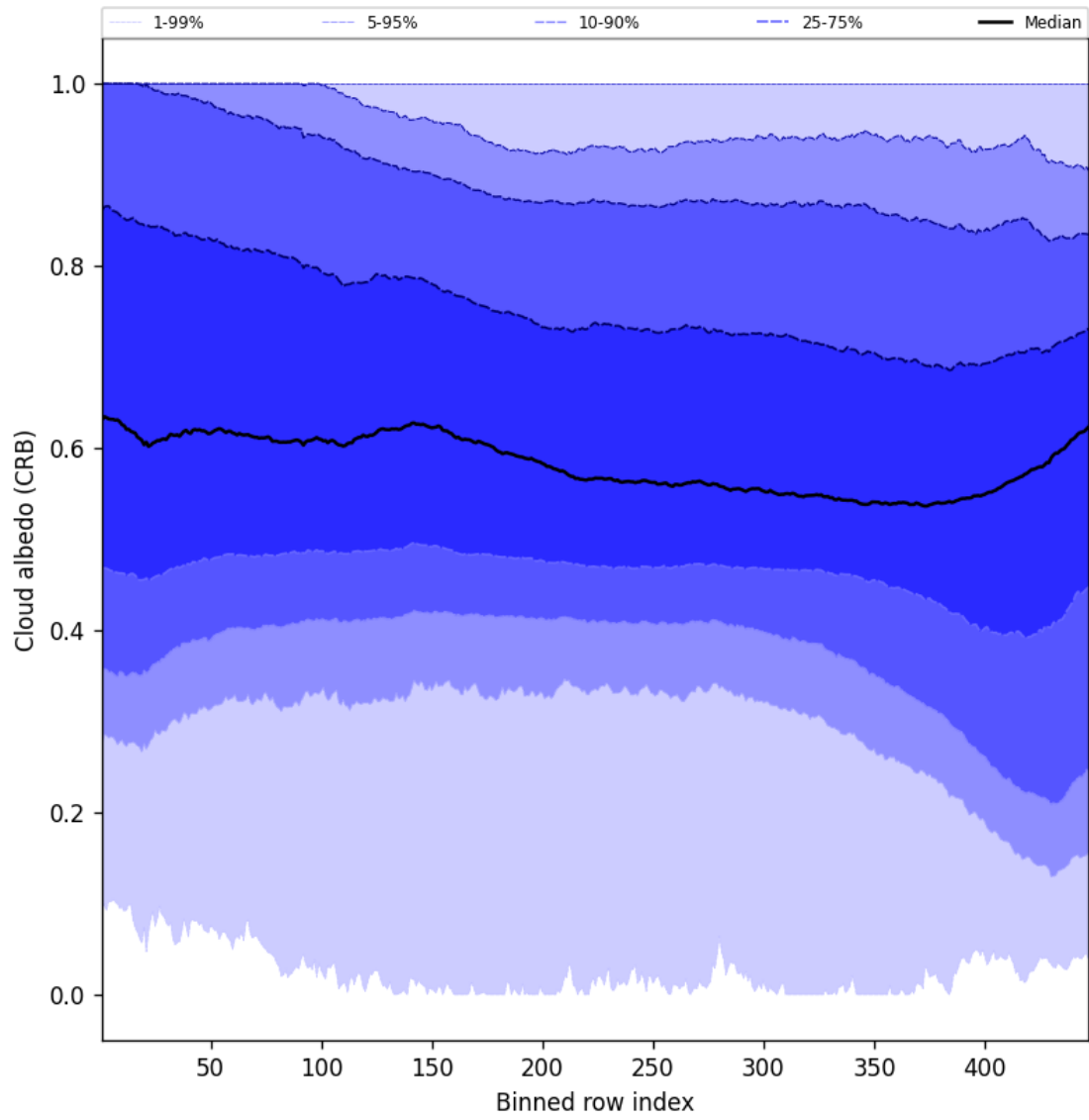
Figure 60: Along track statistics of “Cloud albedo (CRB)” for 2025-02-13 to 2025-02-14
