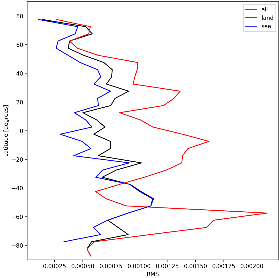
Figure 31: Zonal average of “RMS” for 2025-02-13 to 2025-02-14.
