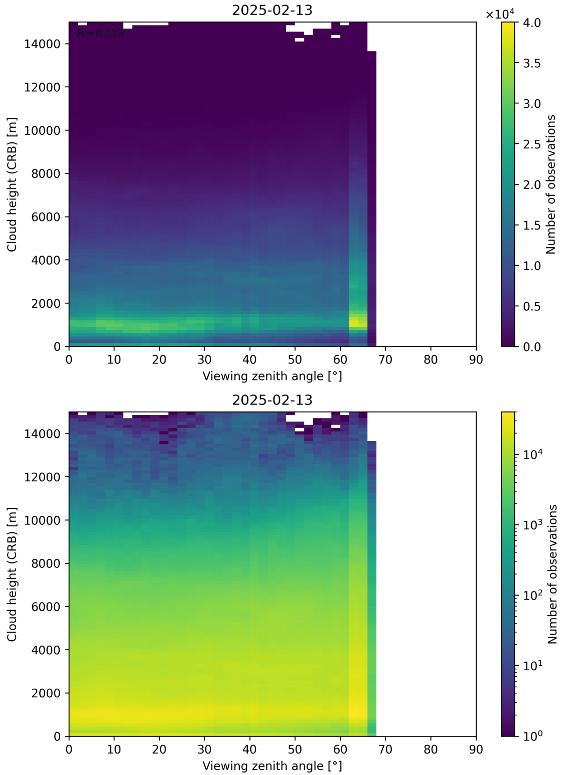
Figure 110: Scatter density plot of “Viewing zenith angle” against “Cloud height (CRB)” for 2025-02-13 to 2025-02-14.
