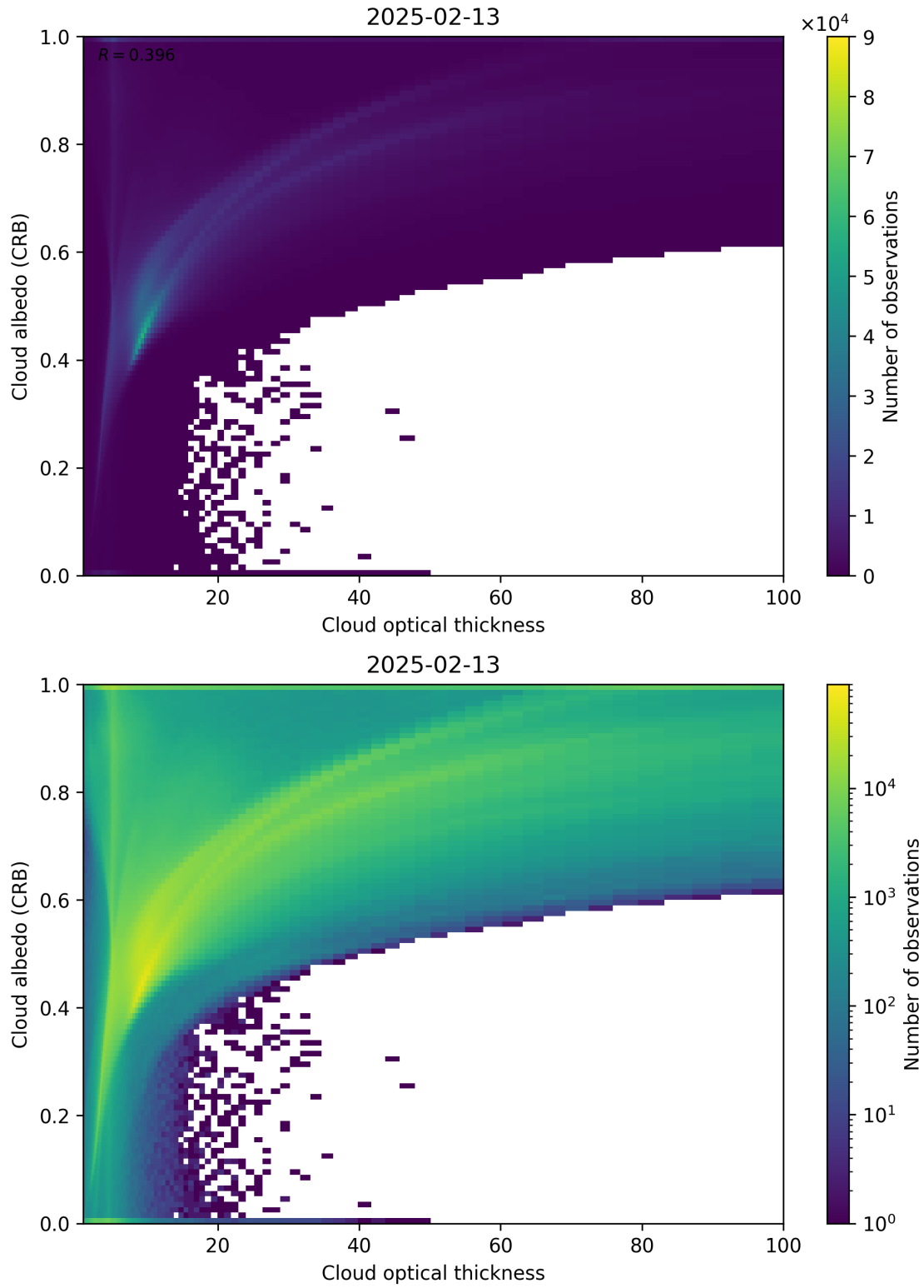
Figure 82: Scatter density plot of “Cloud optical thickness” against “Cloud albedo (CRB)” for 2025-02-13 to 2025-02-14.
