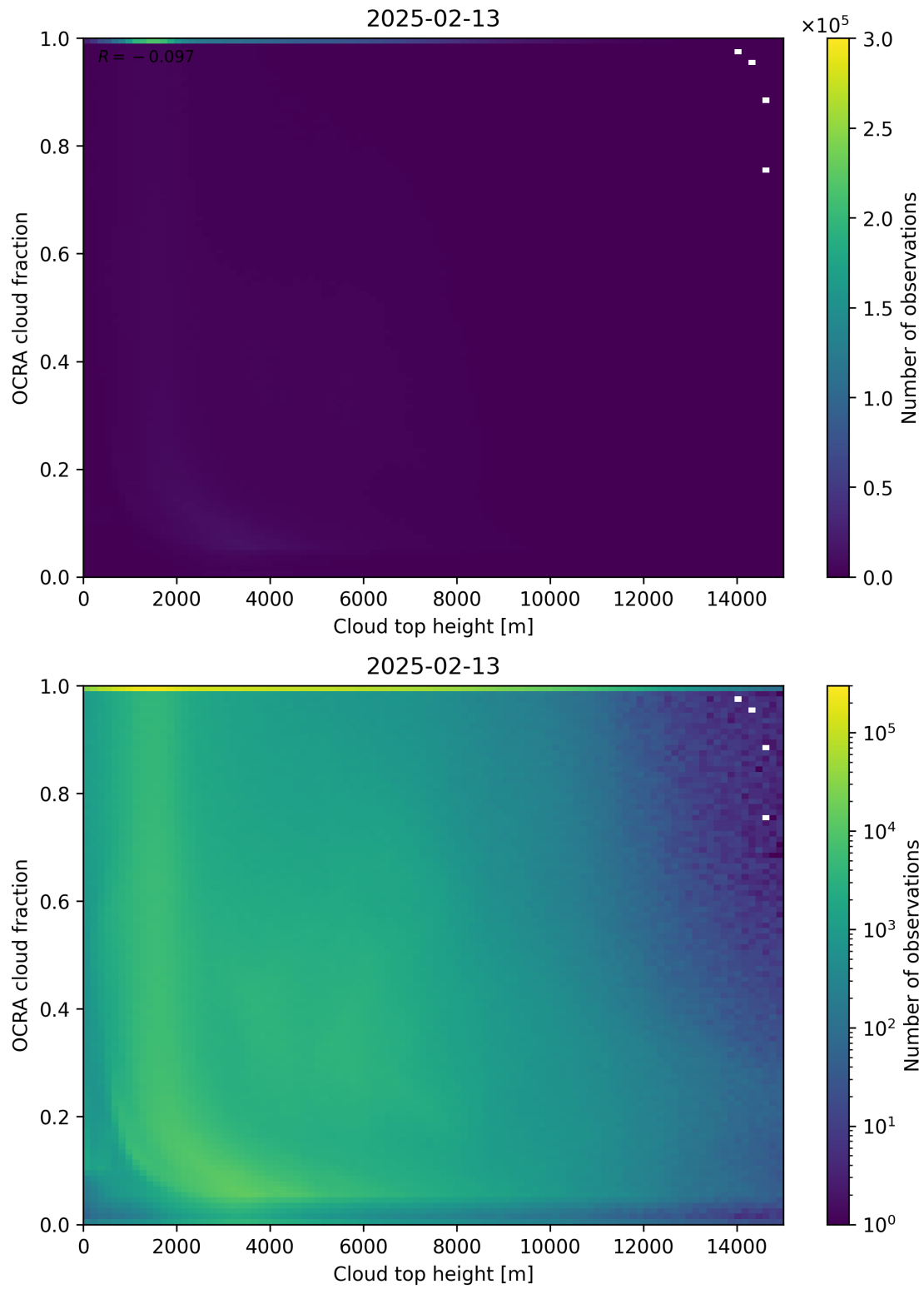
Figure 87: Scatter density plot of “Cloud top height” against “OCRA cloud fraction” for 2025-02-13 to 2025-02-14.
