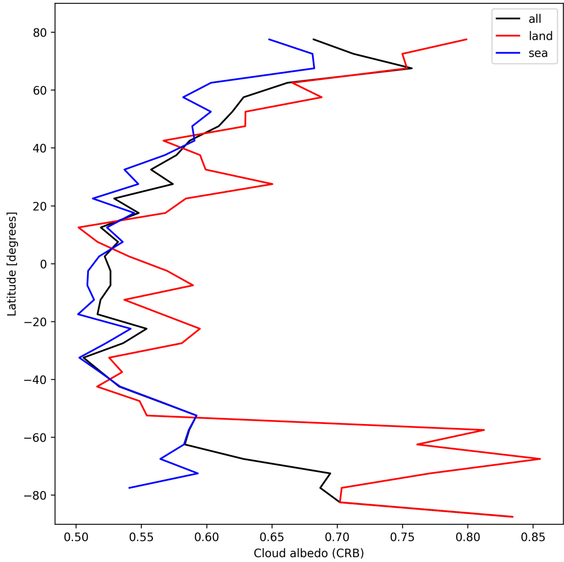
Figure 28: Zonal average of “Cloud albedo (CRB)” for 2025-02-13 to 2025-02-14.
