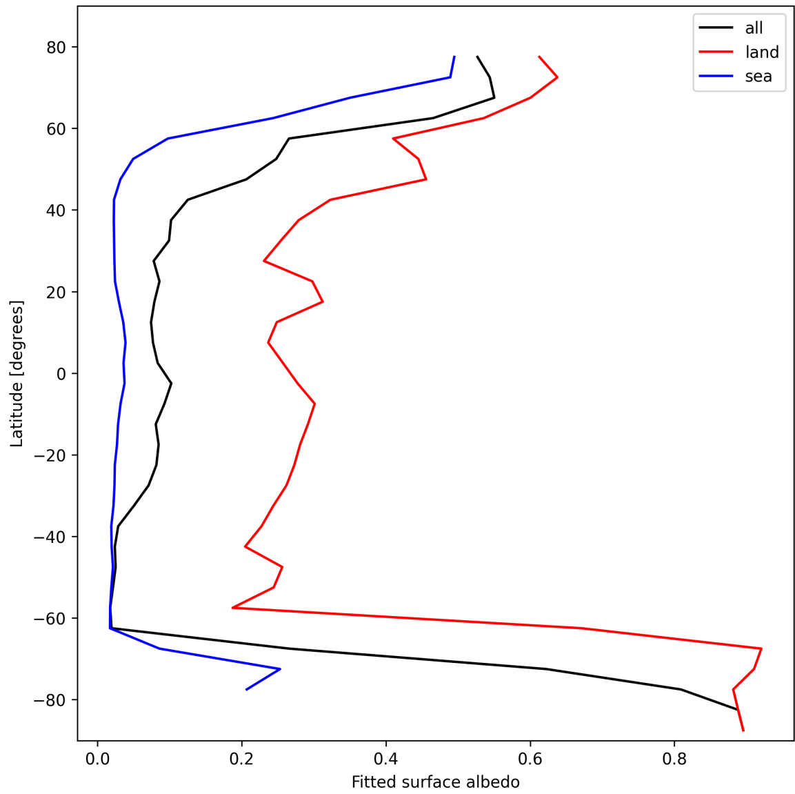
Figure 29: Zonal average of “Fitted surface albedo” for 2025-02-13 to 2025-02-14.
