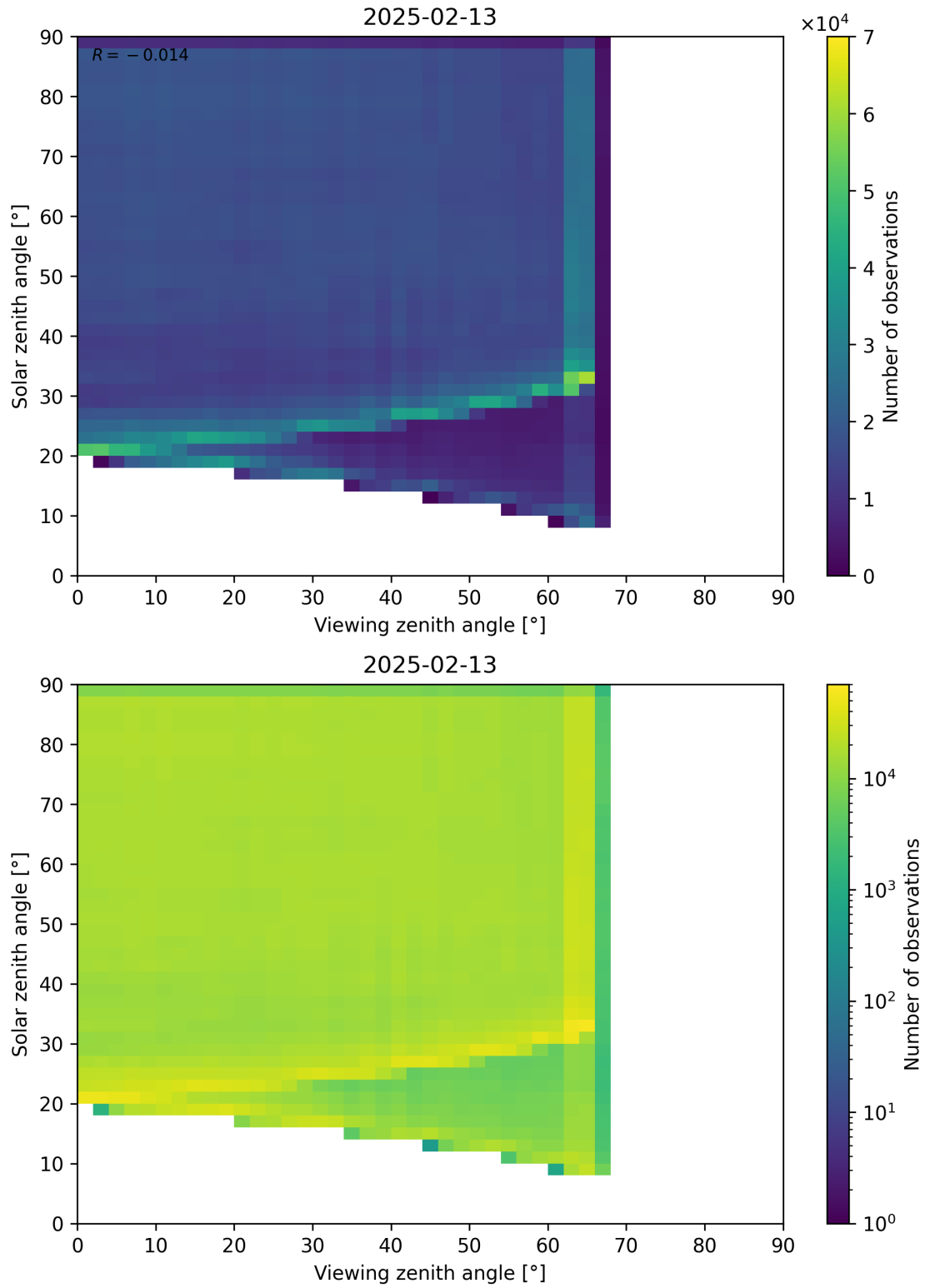
Figure 114: Scatter density plot of “Viewing zenith angle” against “Solar zenith angle” for 2025-02-13 to 2025-02-14.
