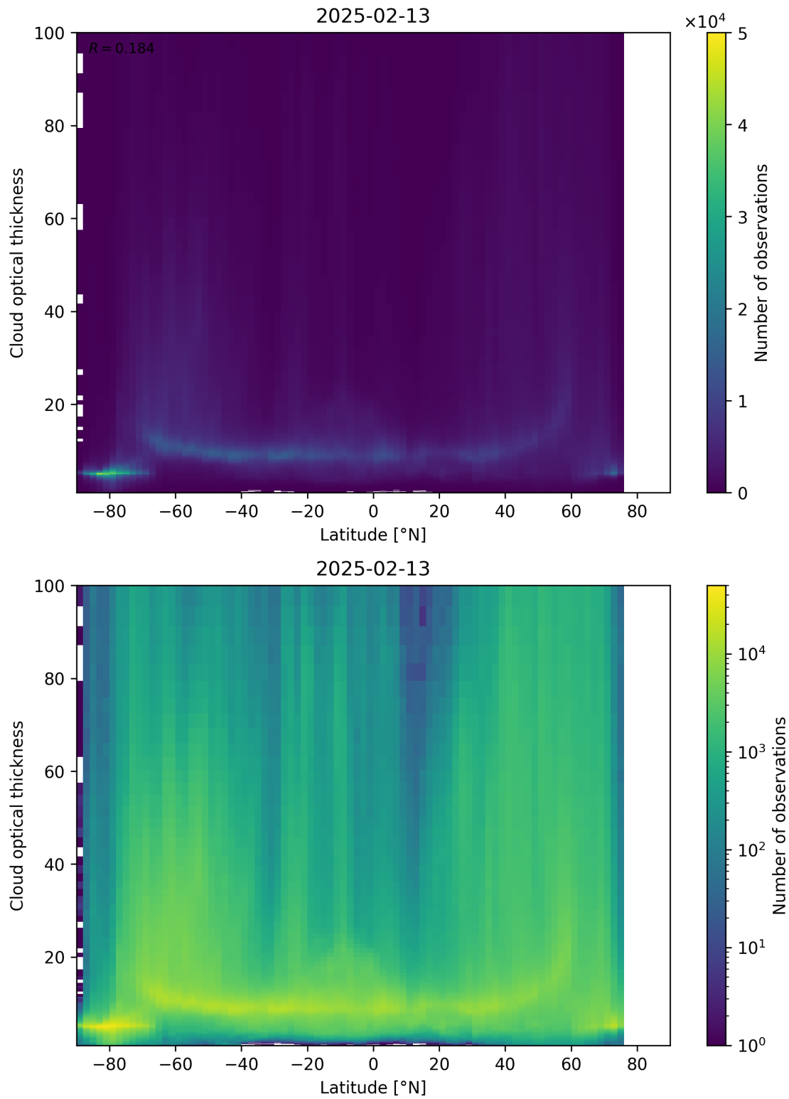
Figure 96: Scatter density plot of “Latitude” against “Cloud optical thickness” for 2025-02-13 to 2025-02-14.
