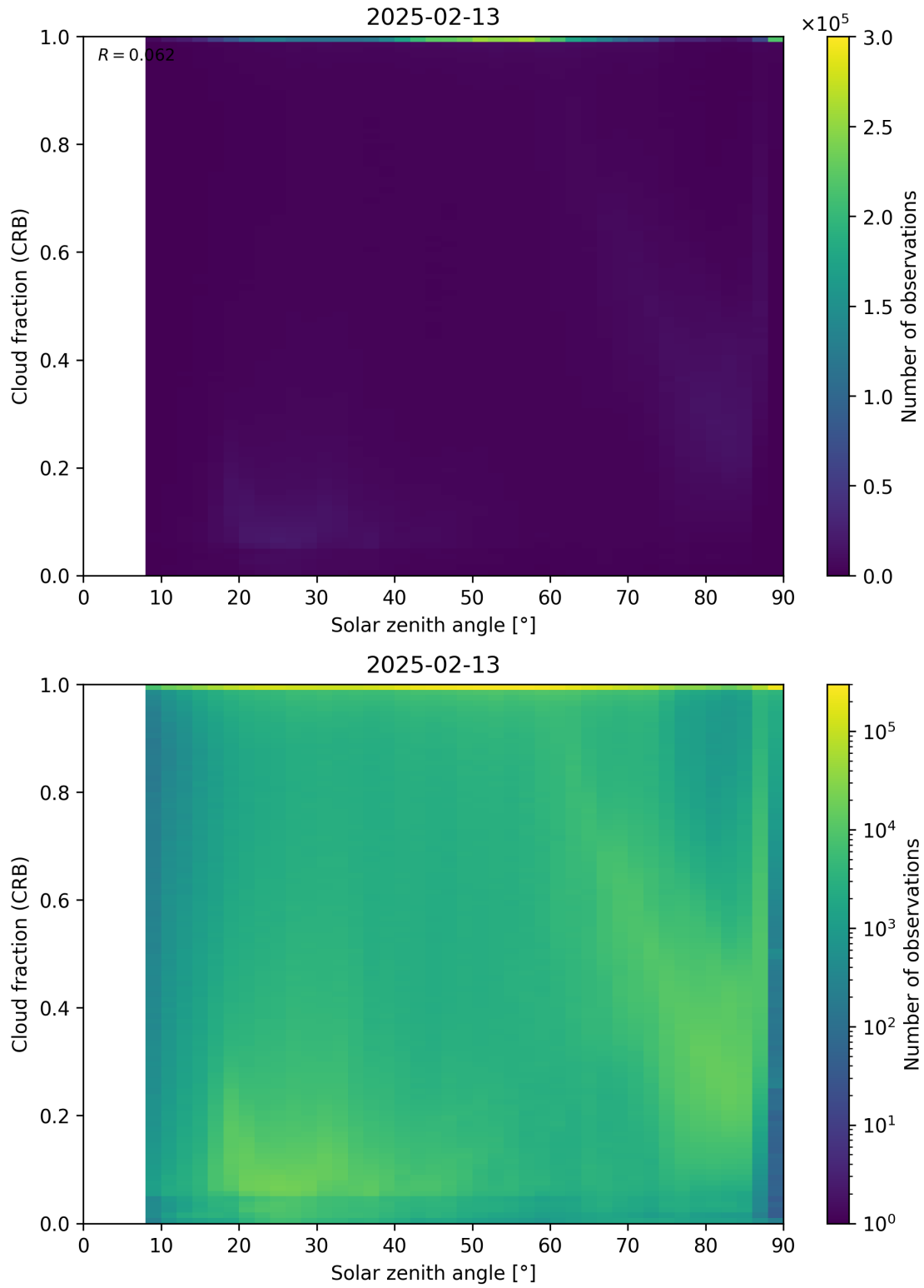
Figure 101: Scatter density plot of “Solar zenith angle” against “Cloud fraction (CRB)” for 2025-02-13 to 2025-02-14.
