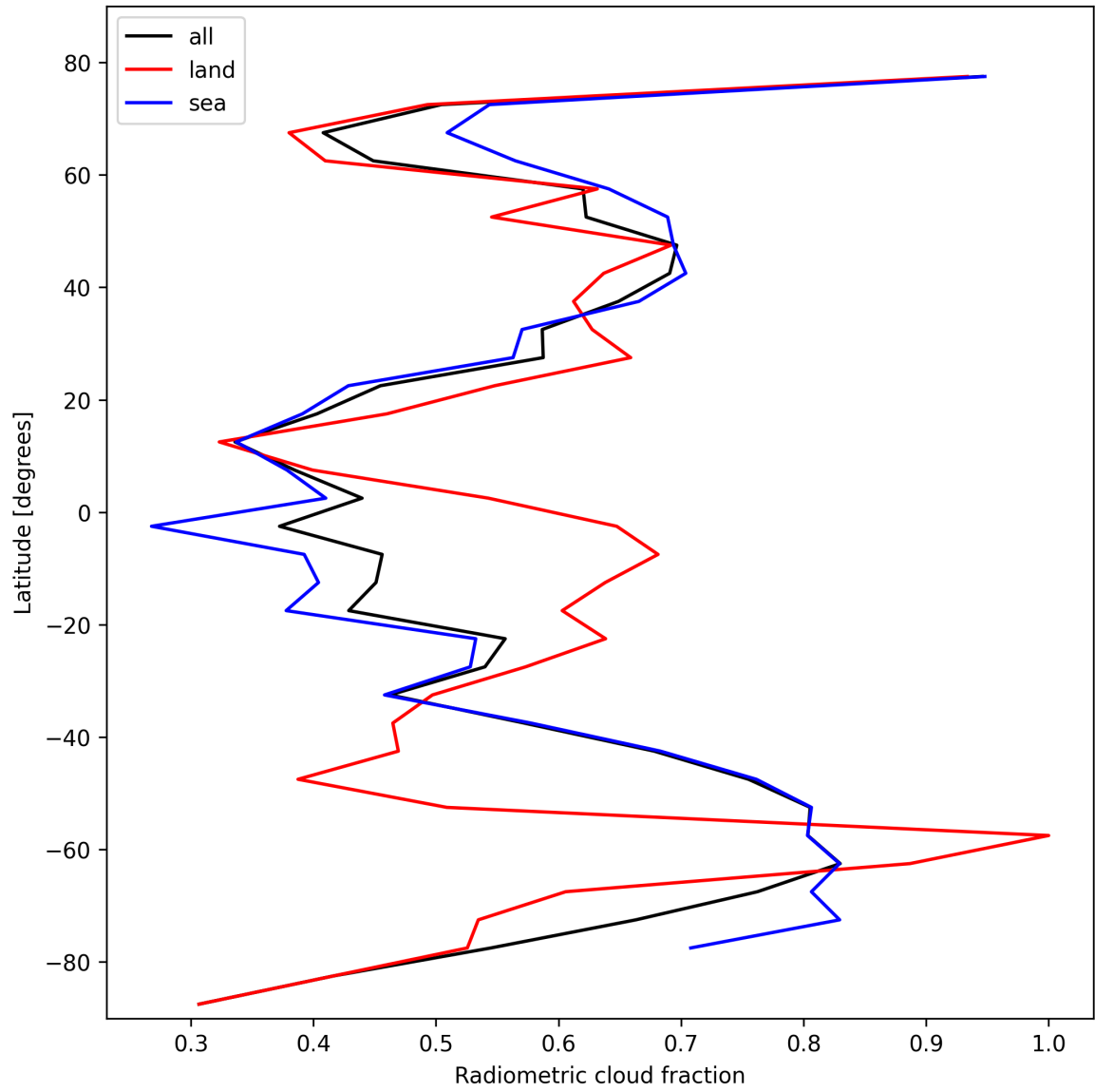
Figure 23: Zonal average of “Radiometric cloud fraction” for 2025-02-13 to 2025-02-14.
