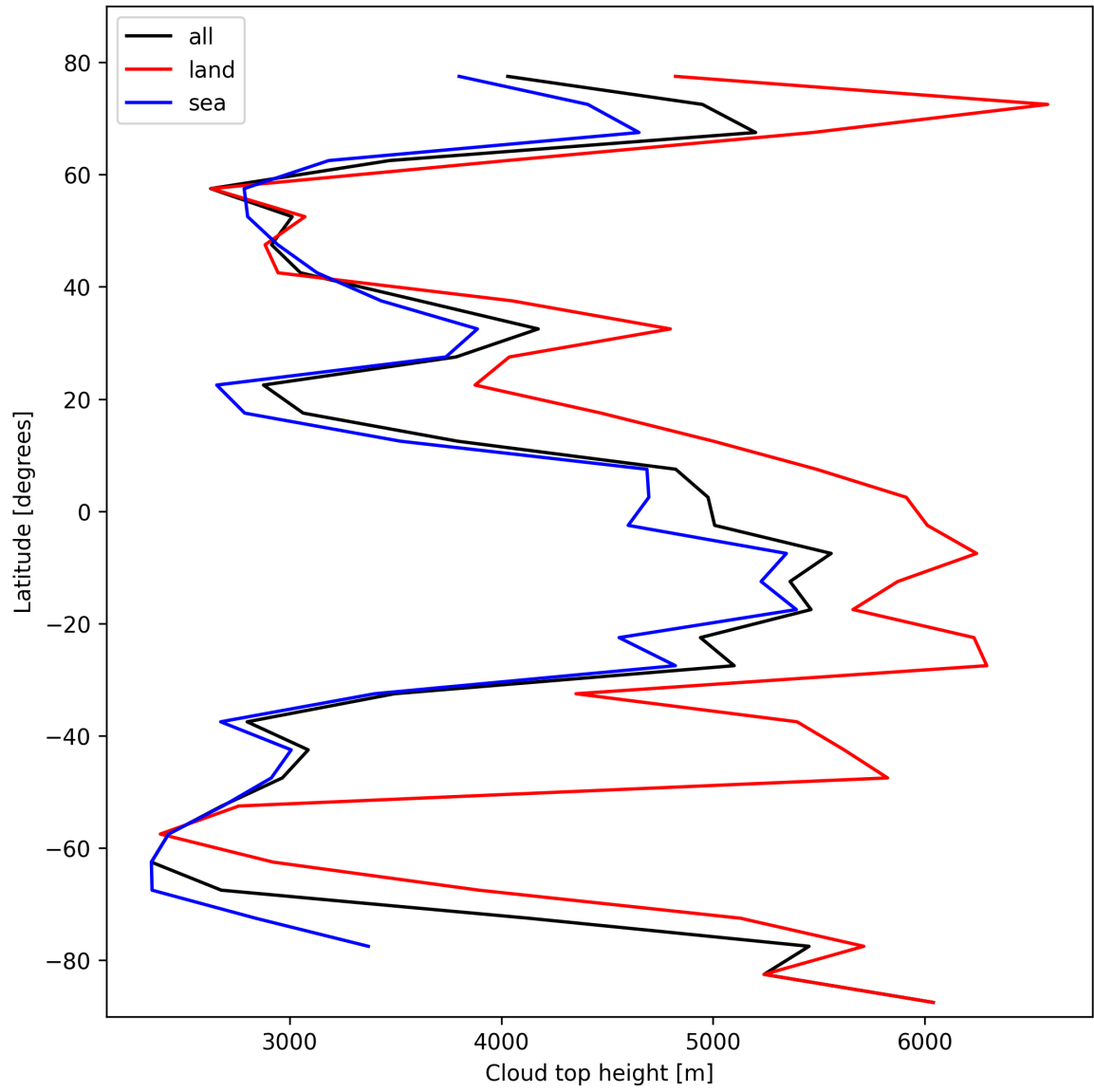
Figure 24: Zonal average of “Cloud top height” for 2025-02-13 to 2025-02-14.
