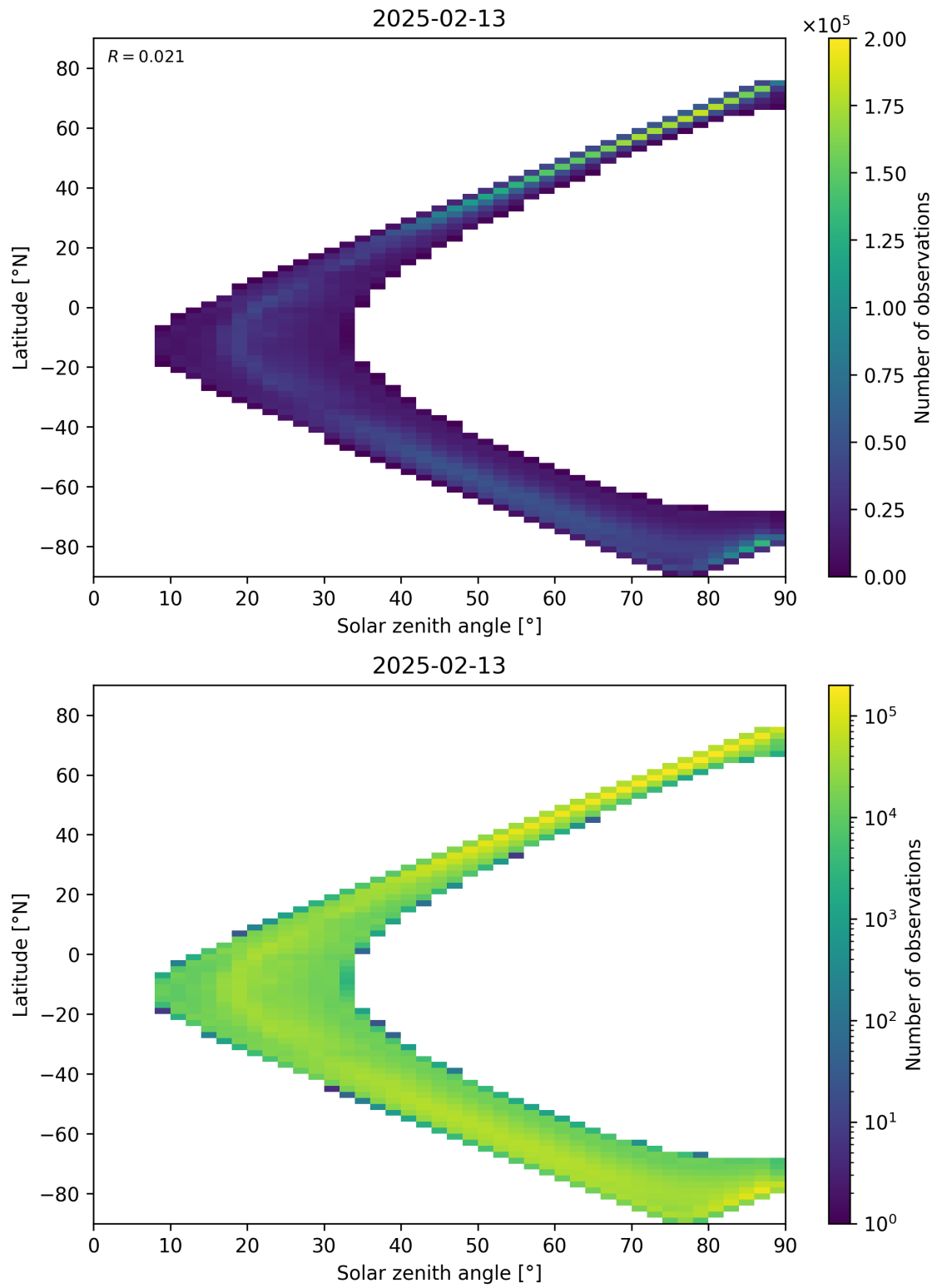
Figure 105: Scatter density plot of “Solar zenith angle” against “Latitude” for 2025-02-13 to 2025-02-14.
