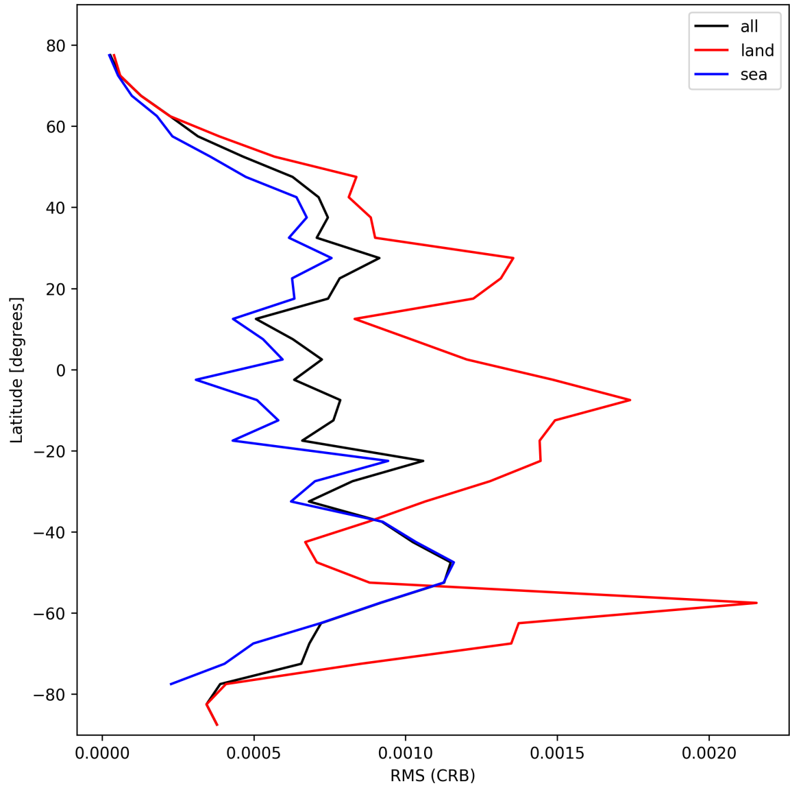
Figure 32: Zonal average of “RMS (CRB)” for 2025-02-13 to 2025-02-14.
