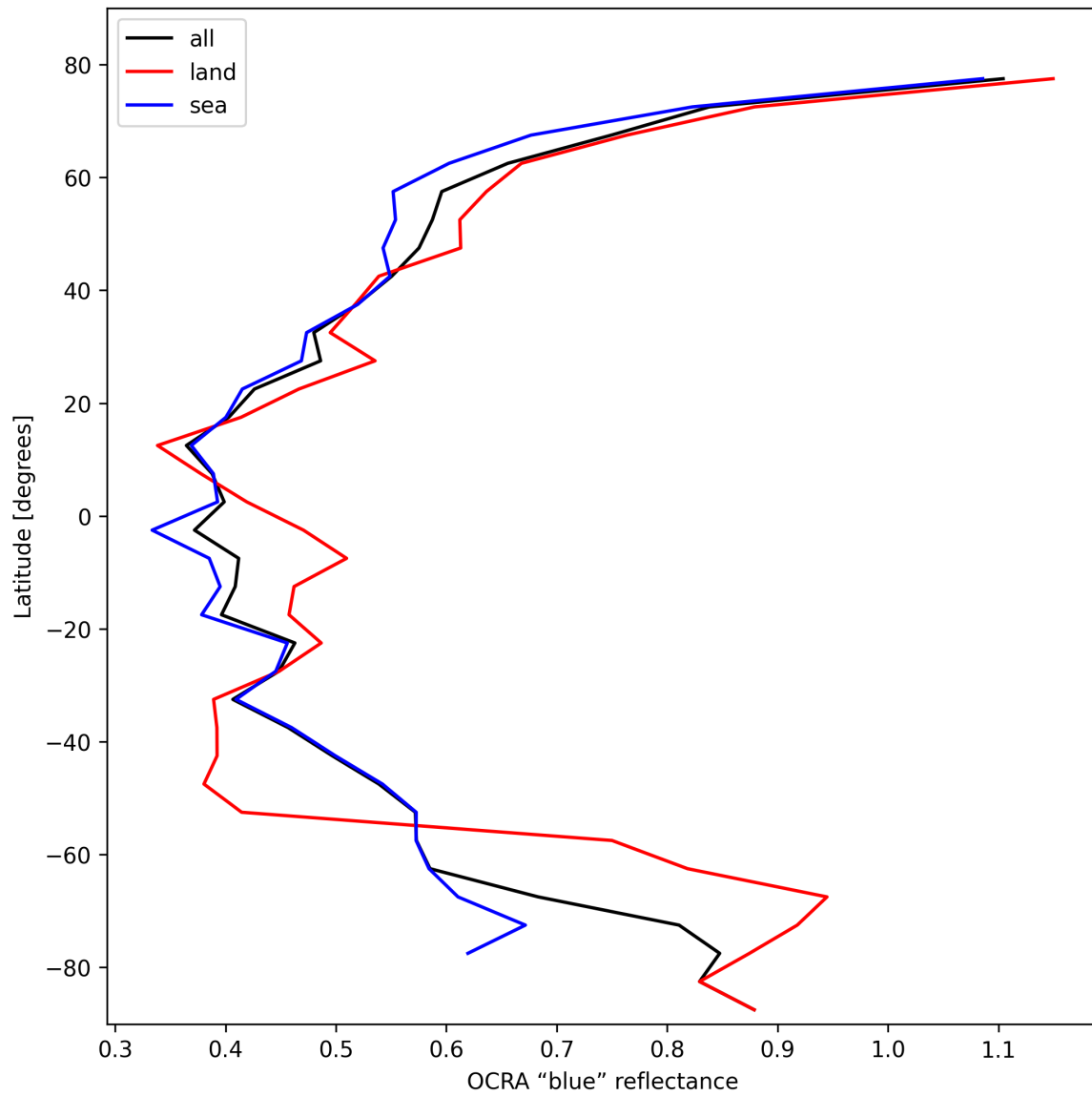
Figure 35: Zonal average of “OCRA “blue” reflectance” for 2025-02-13 to 2025-02-14.
