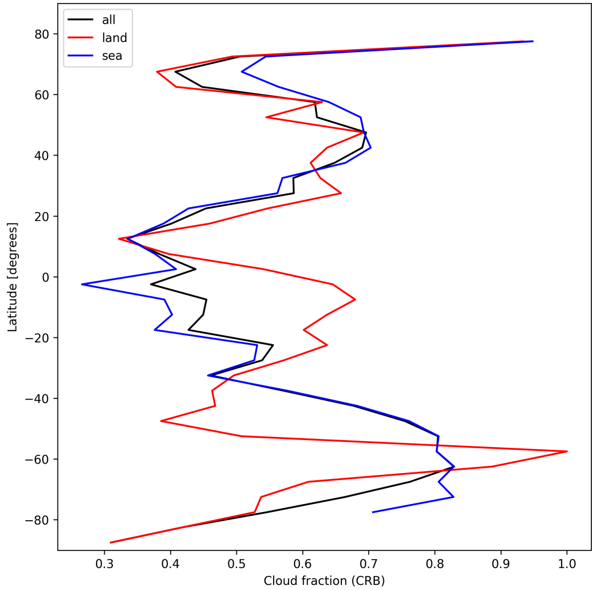
Figure 26: Zonal average of “Cloud fraction (CRB)” for 2025-02-13 to 2025-02-14.
