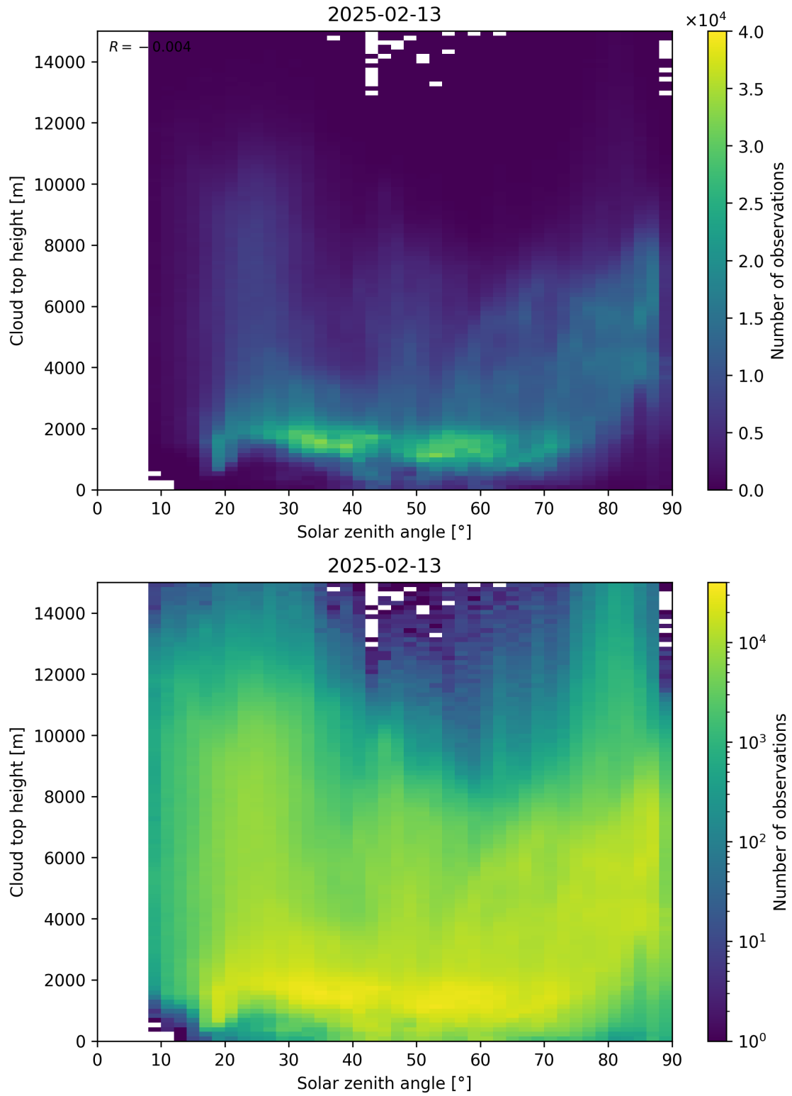
Figure 104: Scatter density plot of “Solar zenith angle” against “Cloud top height” for 2025-02-13 to 2025-02-14.
