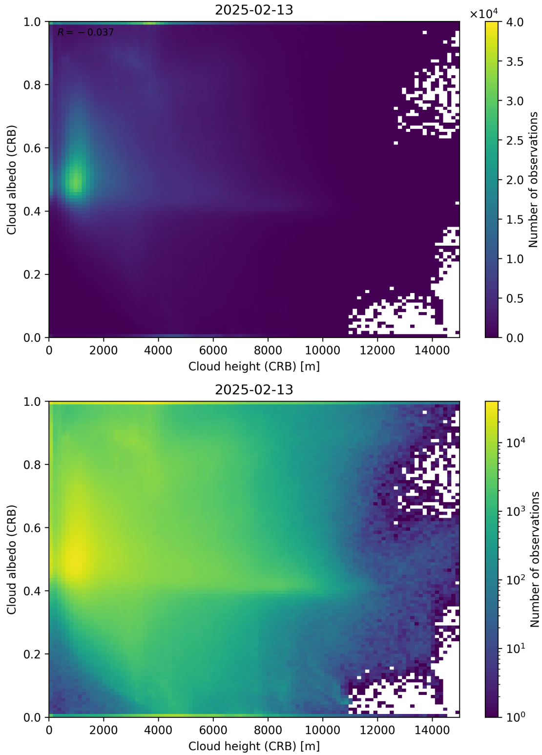
Figure 80: Scatter density plot of “Cloud height (CRB)” against “Cloud albedo (CRB)” for 2025-02-13 to 2025-02-14.
