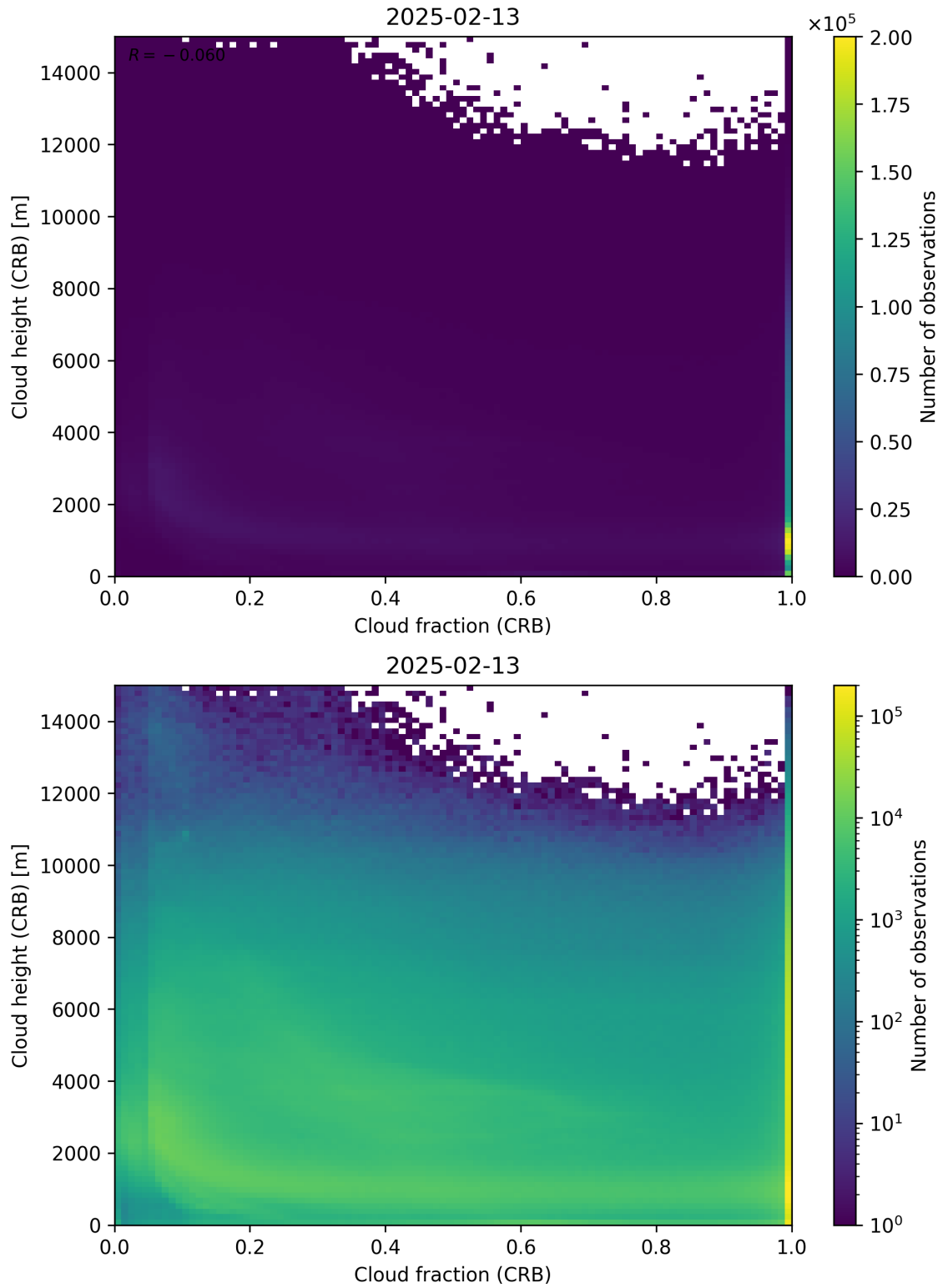
Figure 79: Scatter density plot of “Cloud fraction (CRB)” against “Cloud height (CRB)” for 2025-02-13 to 2025-02-14.
