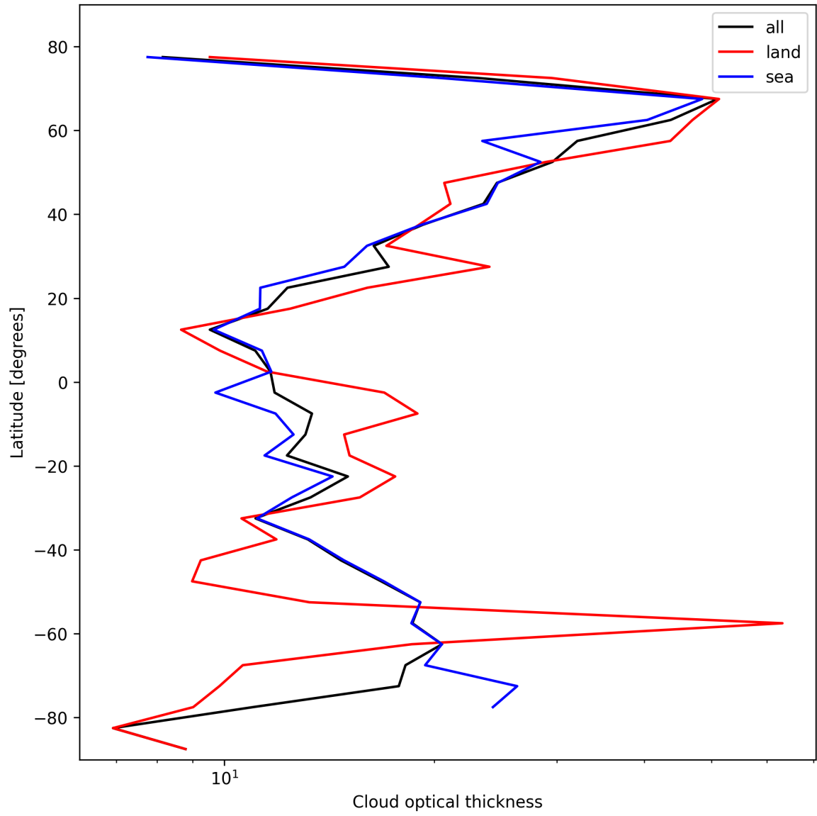
Figure 25: Zonal average of “Cloud optical thickness” for 2025-02-13 to 2025-02-14.
