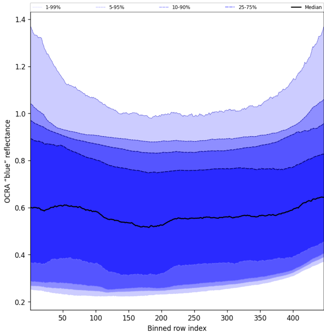
Figure 67: Along track statistics of “OCRA “blue” reflectance” for 2025-02-13 to 2025-02-14
