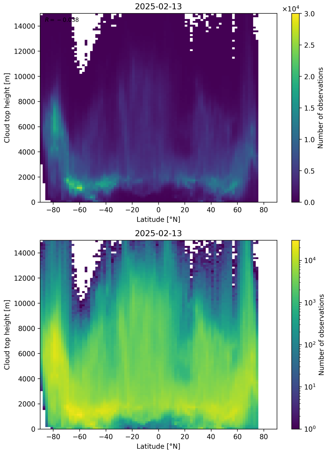
Figure 97: Scatter density plot of “Latitude” against “Cloud top height” for 2025-02-13 to 2025-02-14.
