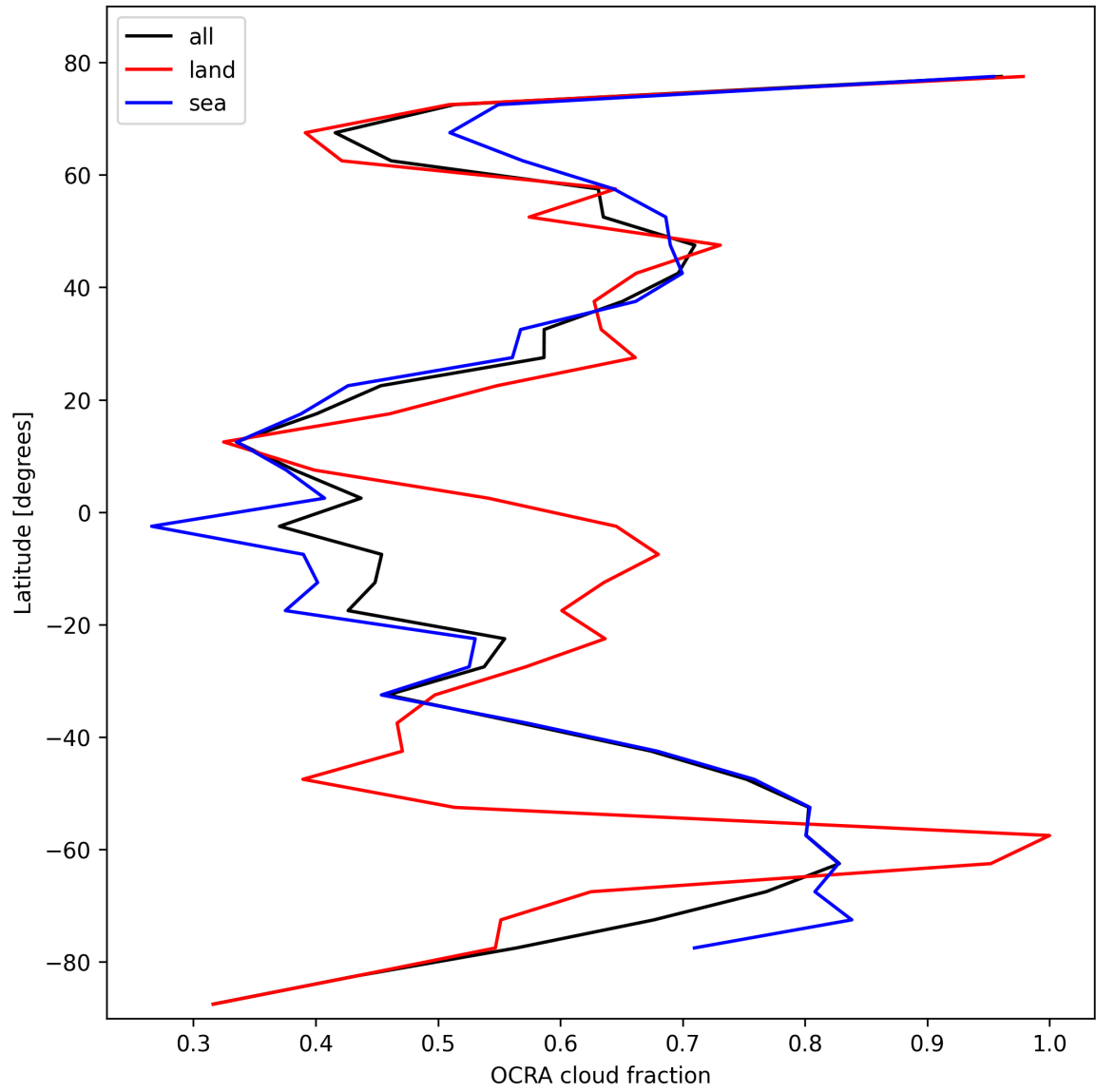
Figure 34: Zonal average of “OCRA cloud fraction” for 2025-02-13 to 2025-02-14.
