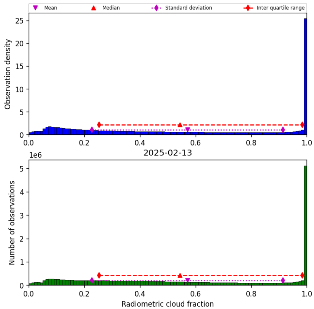
Figure 39: Histogram of “Radiometric cloud fraction” for 2025-02-13 to 2025-02-14
