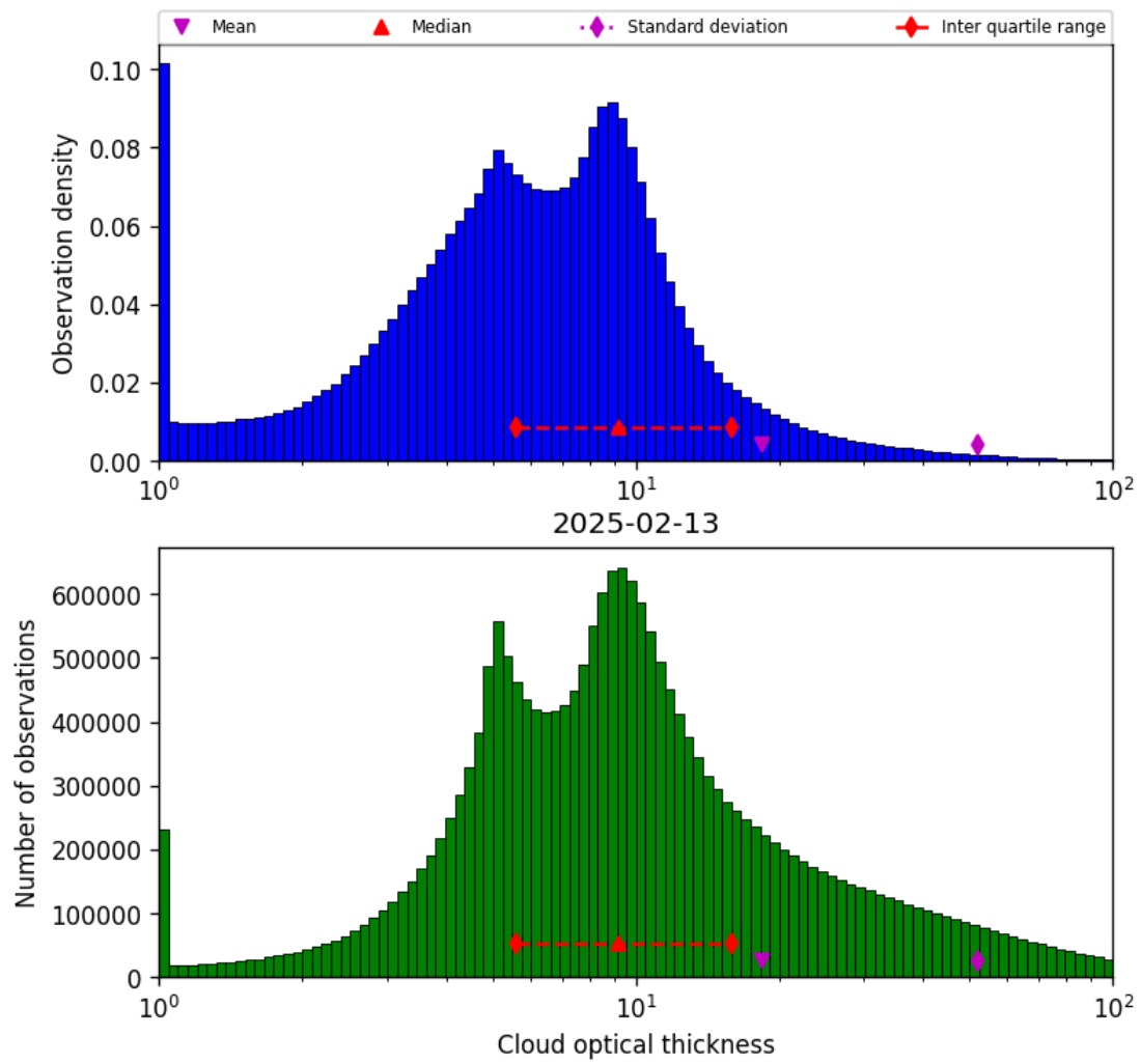
Figure 41: Histogram of “Cloud optical thickness” for 2025-02-13 to 2025-02-14
