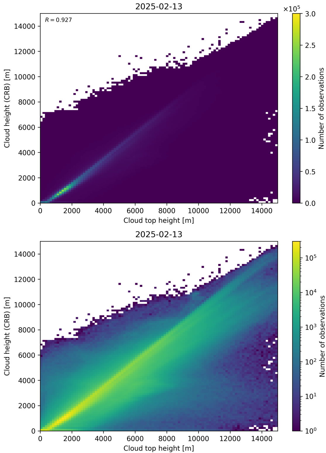
Figure 89: Scatter density plot of “Cloud top height” against “Cloud height (CRB)” for 2025-02-13 to 2025-02-14.
