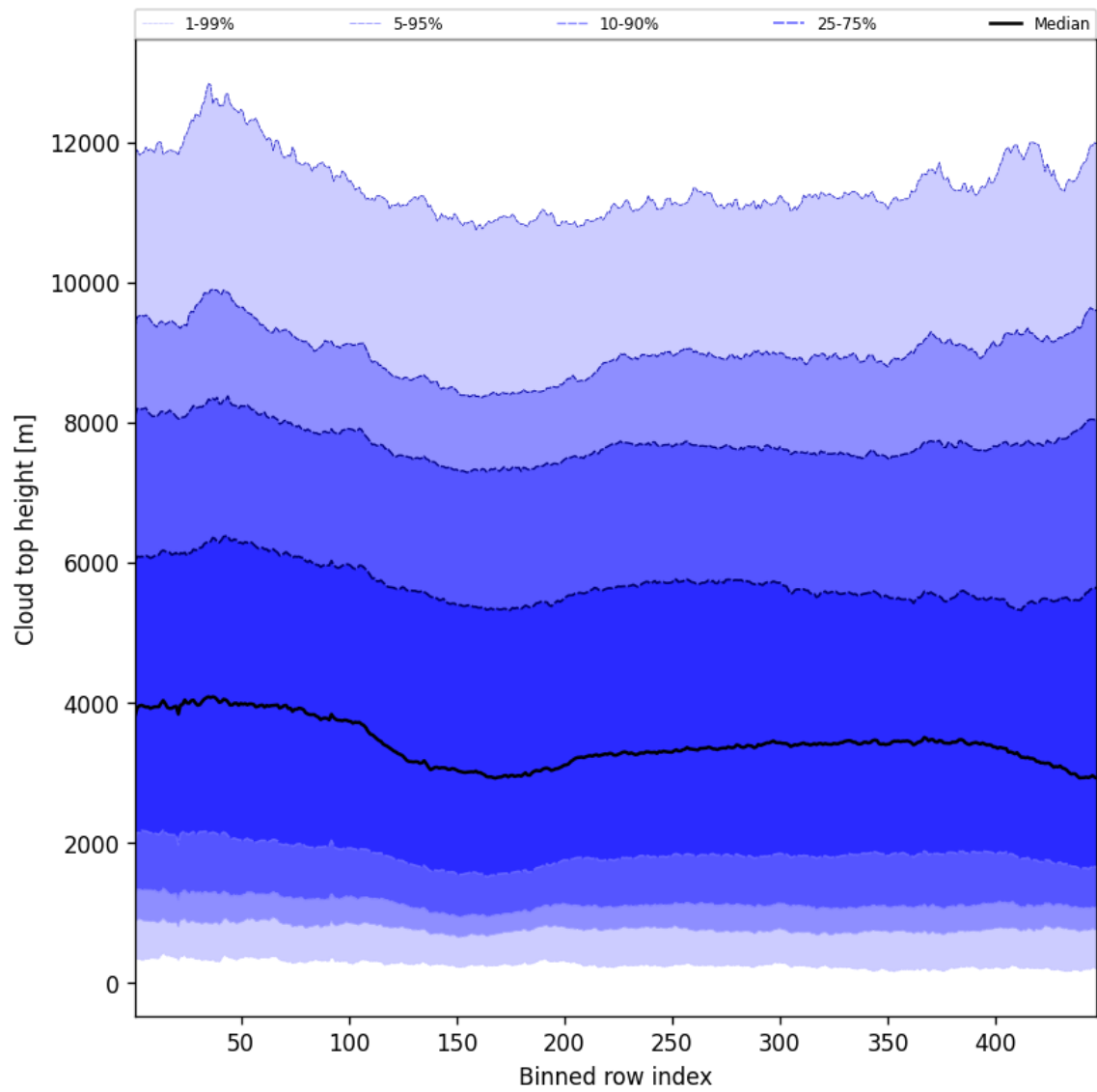
Figure 56: Along track statistics of “Cloud top height” for 2025-02-13 to 2025-02-14
