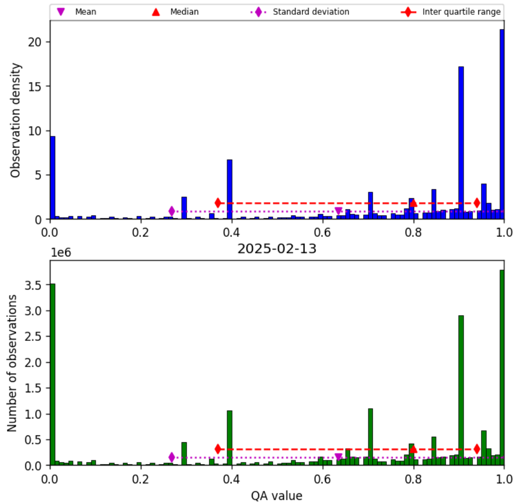
Figure 38: Histogram of “QA value” for 2025-02-13 to 2025-02-14
