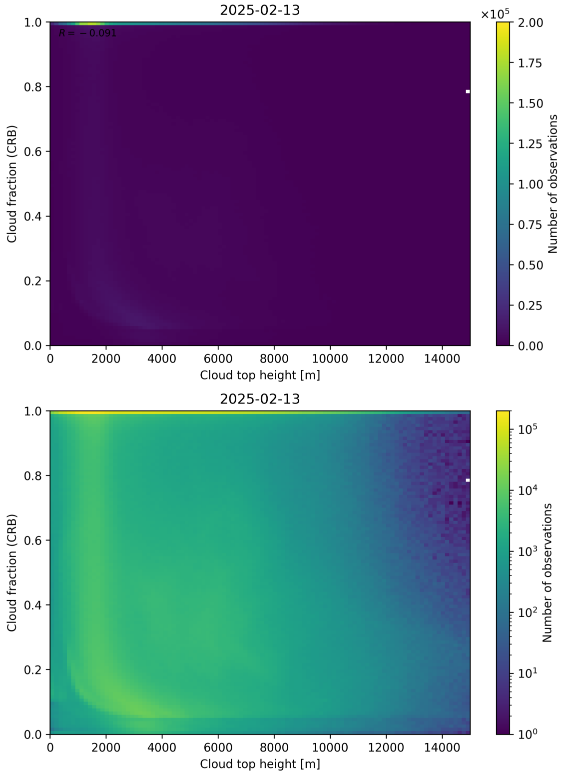
Figure 88: Scatter density plot of “Cloud top height” against “Cloud fraction (CRB)” for 2025-02-13 to 2025-02-14.
