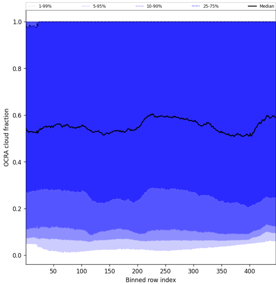
Figure 66: Along track statistics of “OCRA cloud fraction” for 2025-02-13 to 2025-02-14
