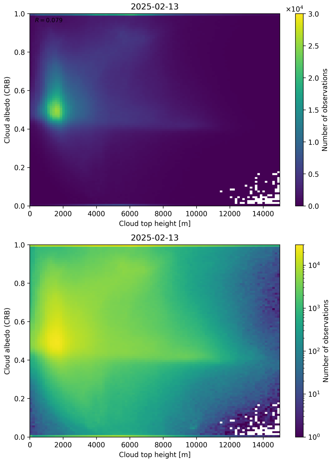
Figure 86: Scatter density plot of “Cloud top height” against “Cloud albedo (CRB)” for 2025-02-13 to 2025-02-14.
