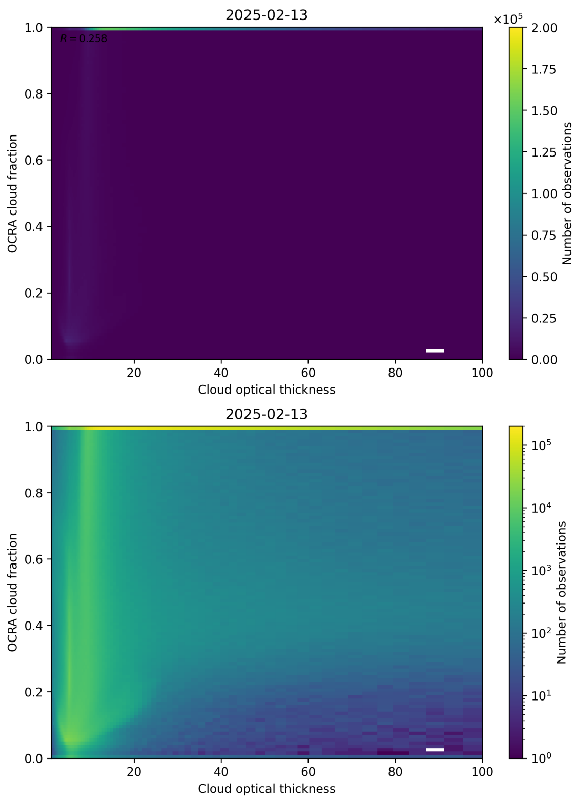
Figure 83: Scatter density plot of “Cloud optical thickness” against “OCRA cloud fraction” for 2025-02-13 to 2025-02-14.
