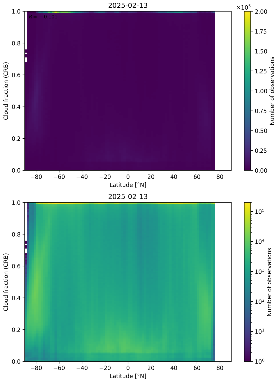
Figure 94: Scatter density plot of “Latitude” against “Cloud fraction (CRB)” for 2025-02-13 to 2025-02-14.
