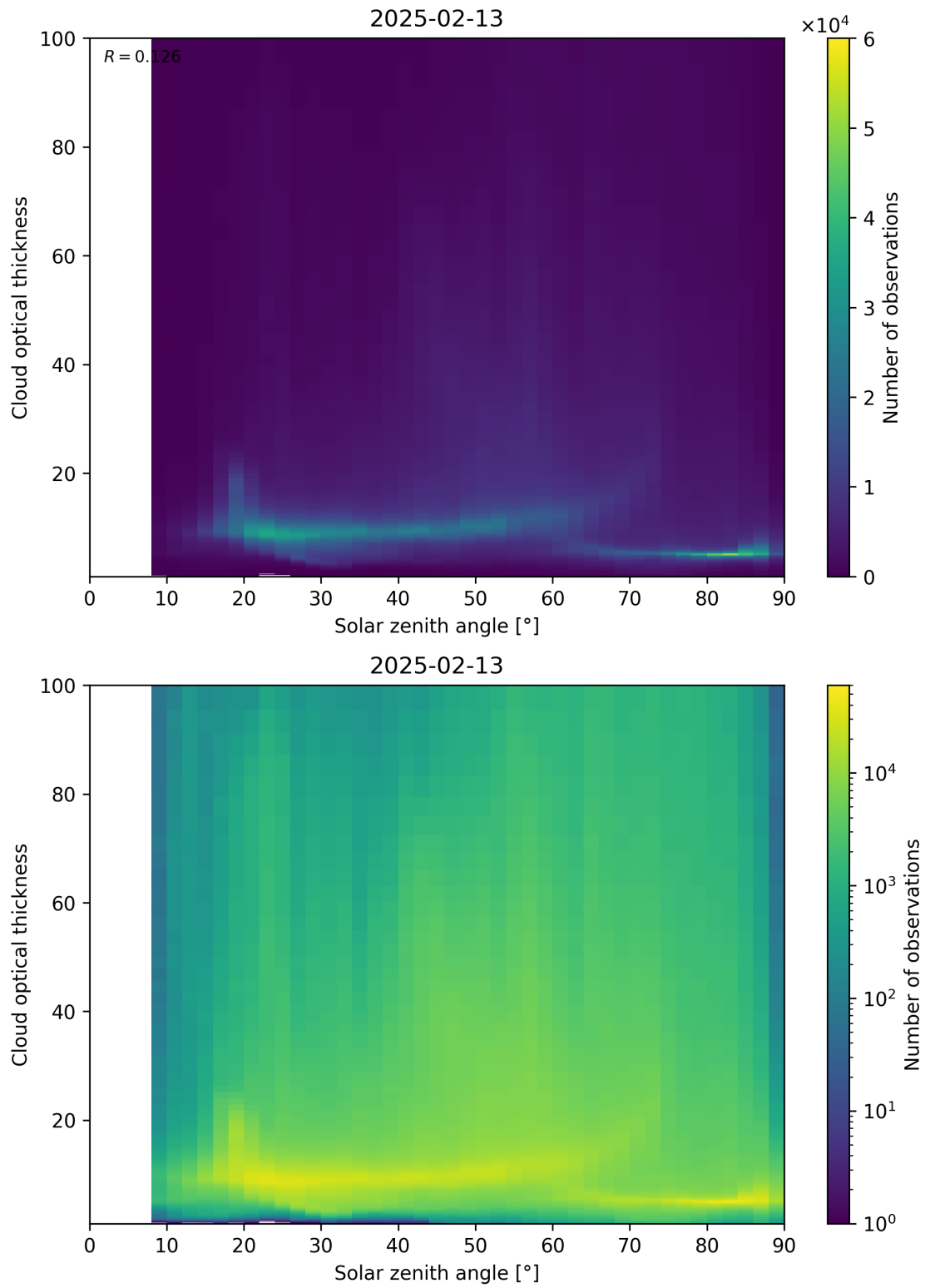
Figure 103: Scatter density plot of “Solar zenith angle” against “Cloud optical thickness” for 2025-02-13 to 2025-02-14.
