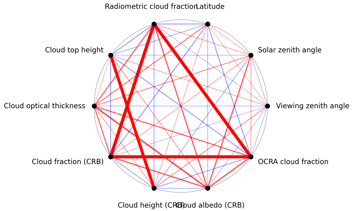
Figure 1: Map of correlation graph for 2025-02-13 to 2025-02-14.
