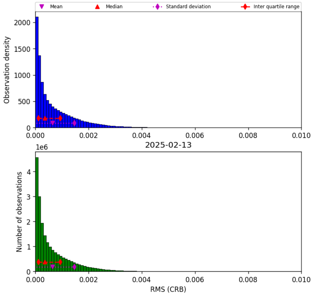
Figure 48: Histogram of “RMS (CRB)” for 2025-02-13 to 2025-02-14
