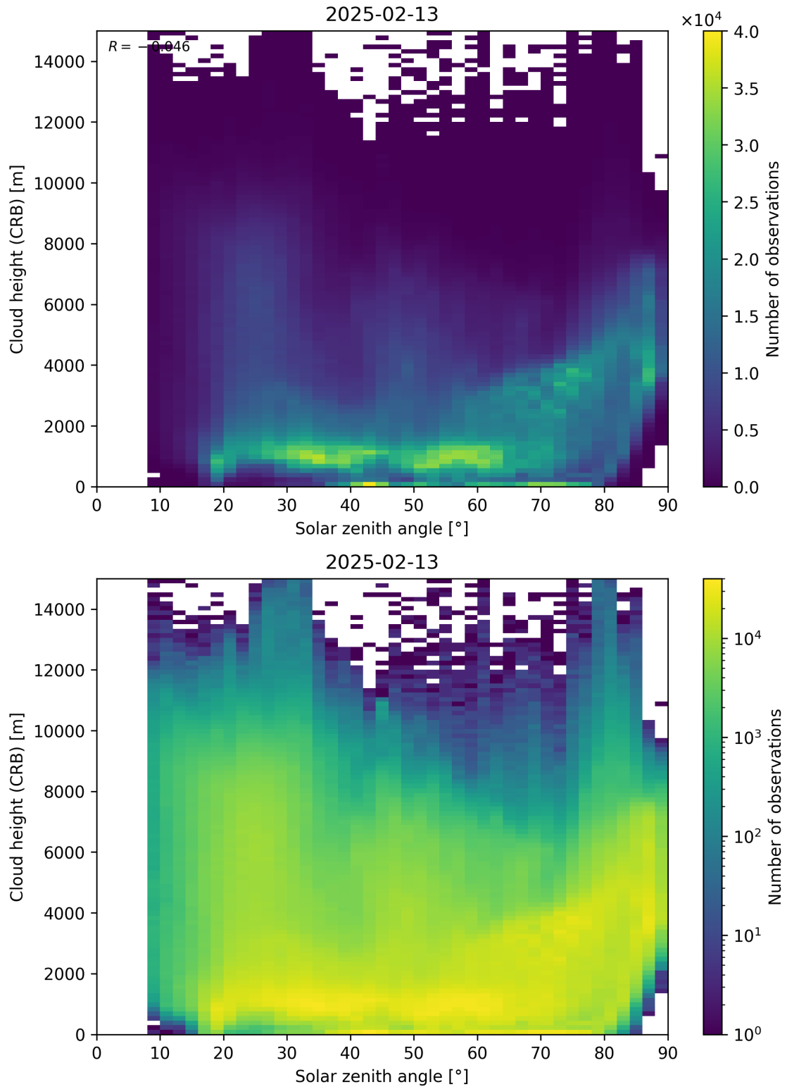
Figure 102: Scatter density plot of “Solar zenith angle” against “Cloud height (CRB)” for 2025-02-13 to 2025-02-14.
