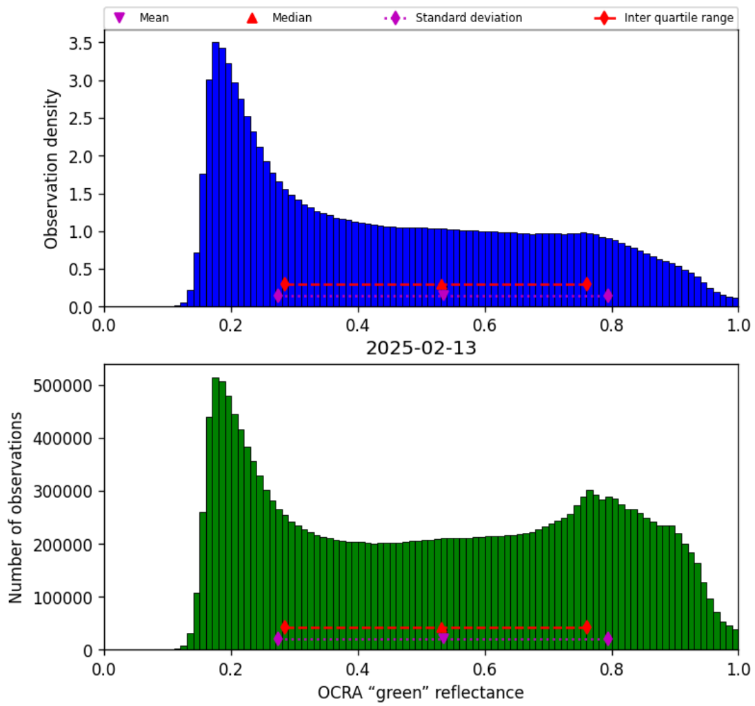
Figure 52: Histogram of “OCRA “green” reflectance” for 2025-02-13 to 2025-02-14
