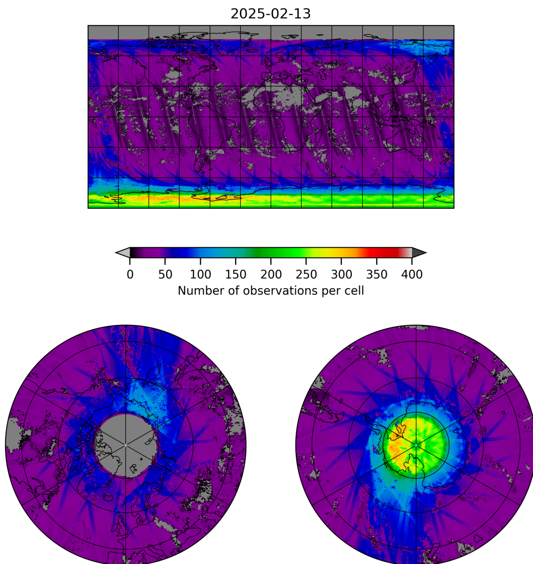
Figure 21: Map of the number of observations for 2025-02-13 to 2025-02-14
