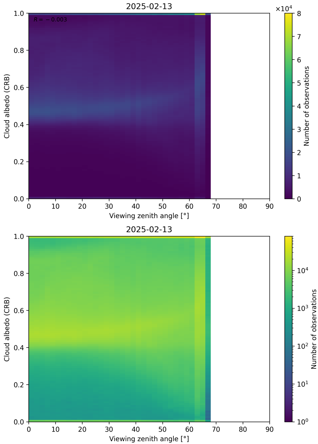
Figure 106: Scatter density plot of “Viewing zenith angle” against “Cloud albedo (CRB)” for 2025-02-13 to 2025-02-14.
