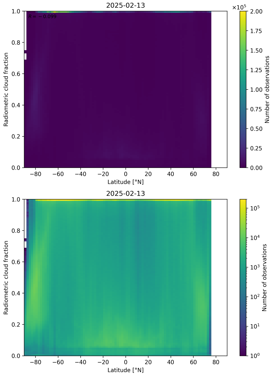
Figure 92: Scatter density plot of “Latitude” against “Radiometric cloud fraction” for 2025-02-13 to 2025-02-14.
