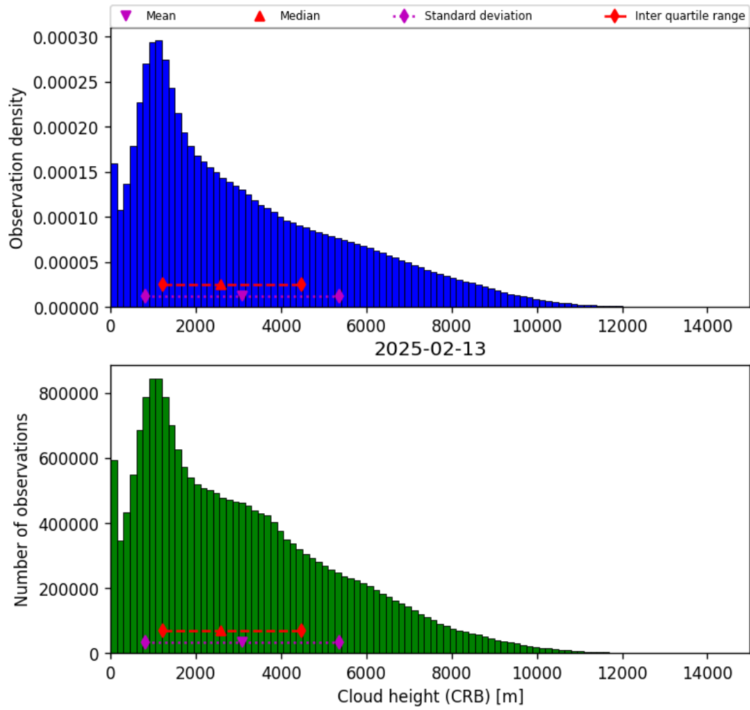
Figure 43: Histogram of “Cloud height (CRB)” for 2025-02-13 to 2025-02-14
