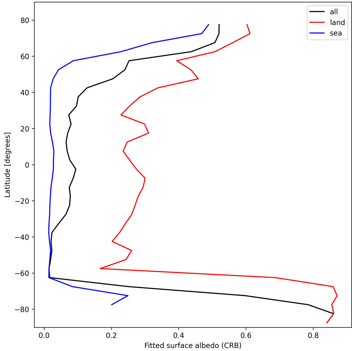
Figure 30: Zonal average of “Fitted surface albedo (CRB)” for 2025-02-13 to 2025-02-14.
