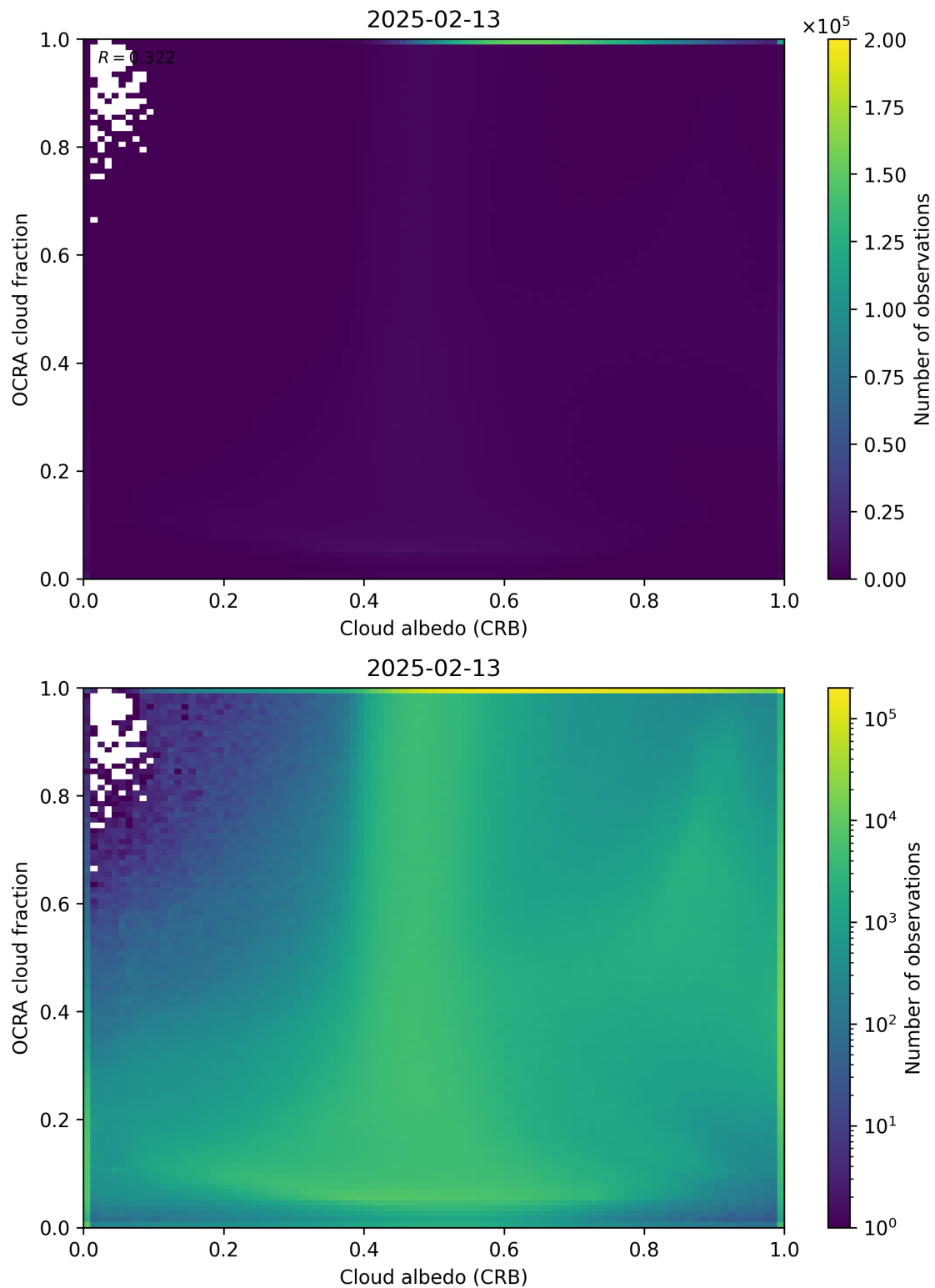
Figure 70: Scatter density plot of “Cloud albedo (CRB)” against “OCRA cloud fraction” for 2025-02-13 to 2025-02-14.
