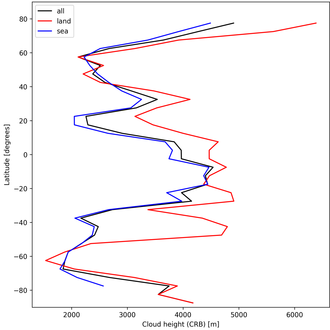
Figure 27: Zonal average of “Cloud height (CRB)” for 2025-02-13 to 2025-02-14.
