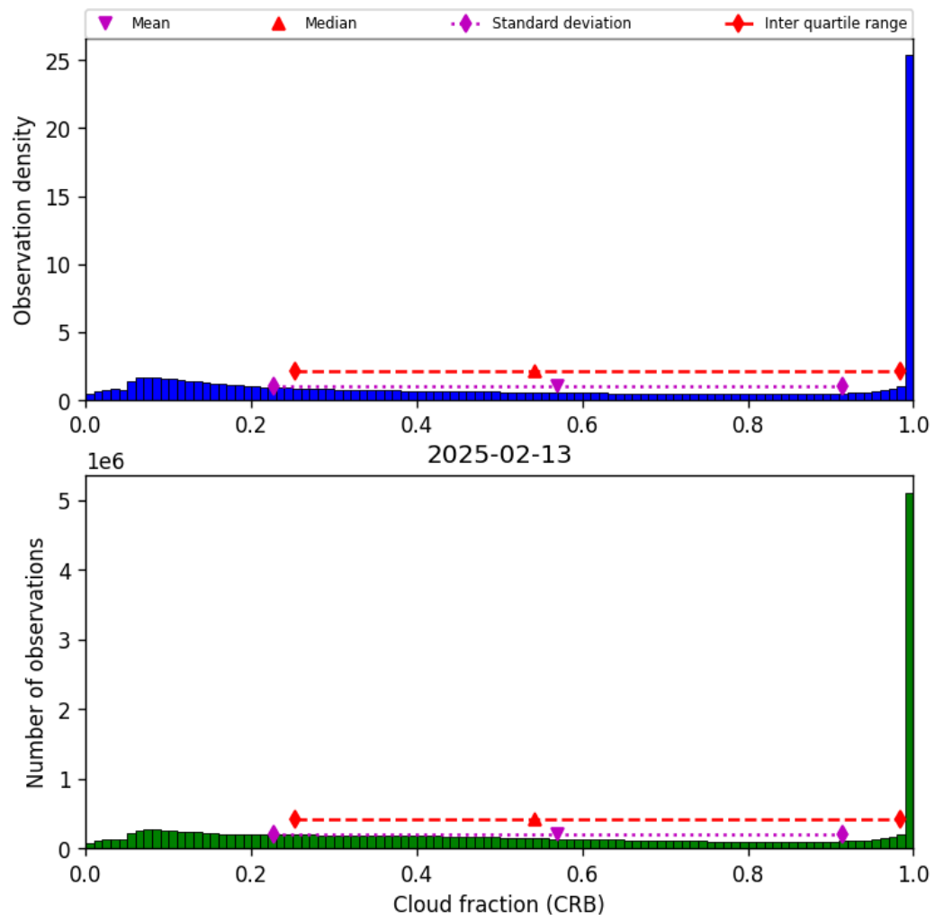
Figure 42: Histogram of “Cloud fraction (CRB)” for 2025-02-13 to 2025-02-14
