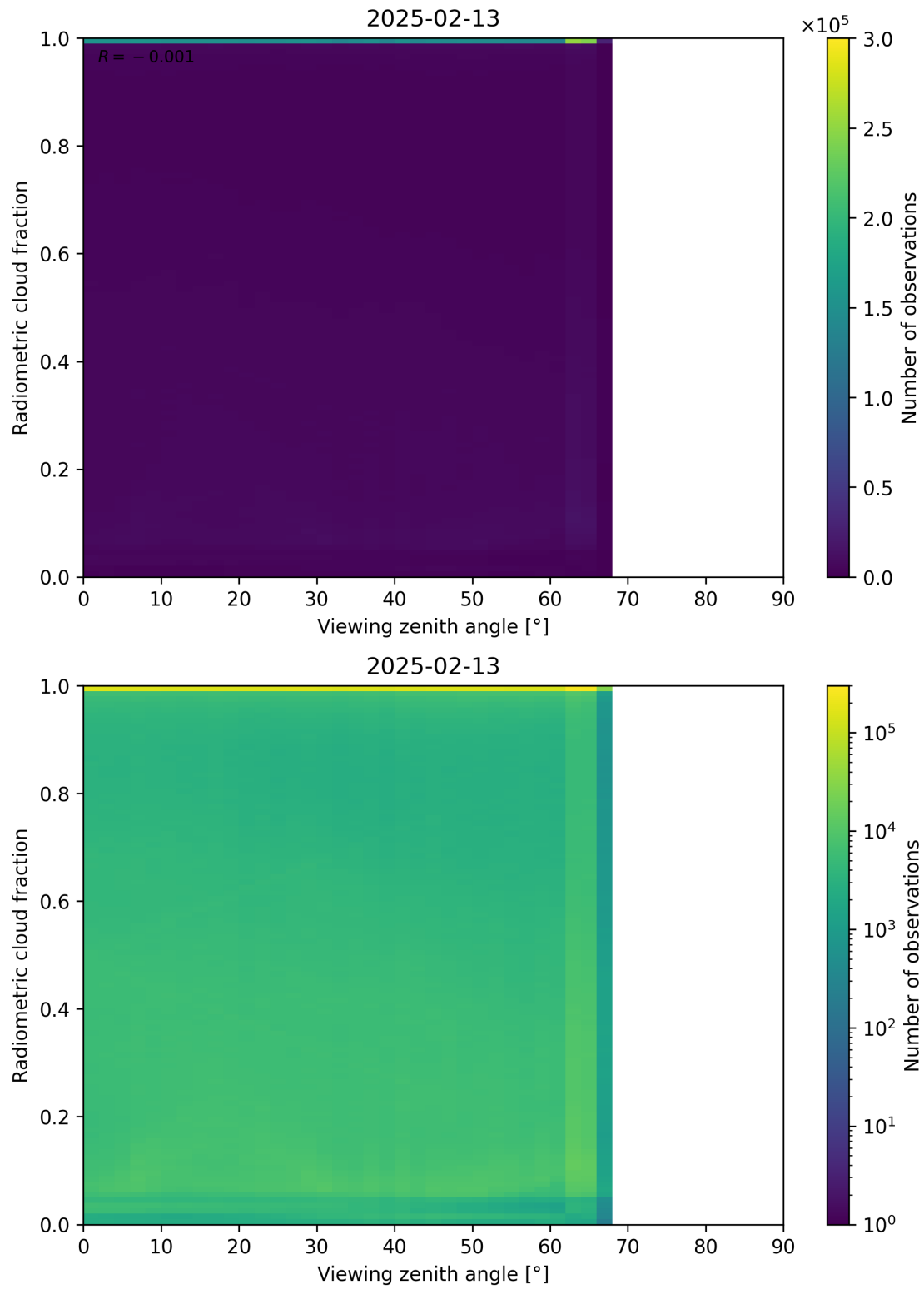
Figure 107: Scatter density plot of “Viewing zenith angle” against “Radiometric cloud fraction” for 2025-02-13 to 2025-02-14.
