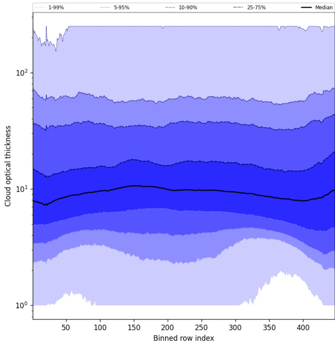
Figure 57: Along track statistics of “Cloud optical thickness” for 2025-02-13 to 2025-02-14
