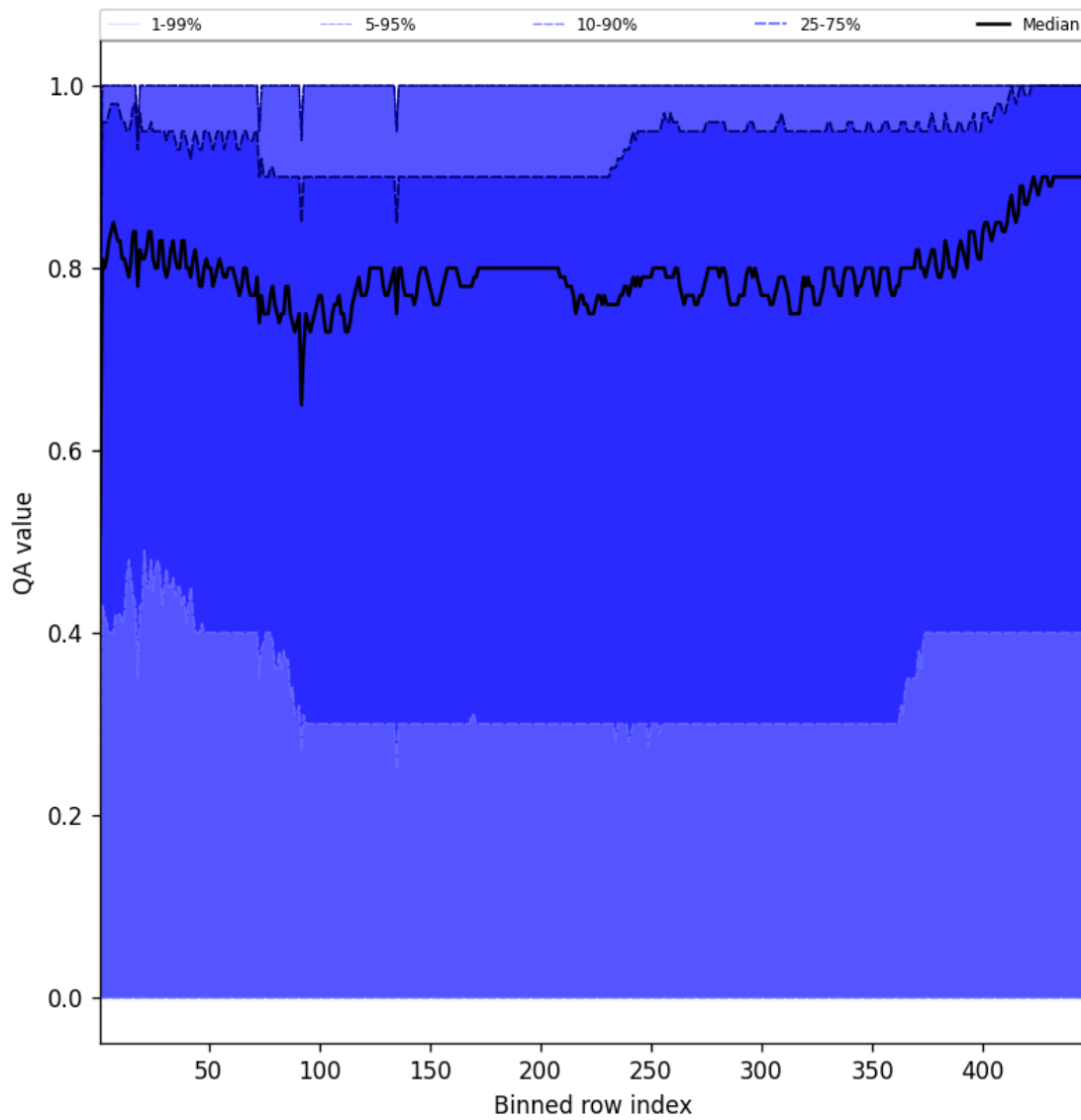
Figure 54: Along track statistics of “QA value” for 2025-02-13 to 2025-02-14
