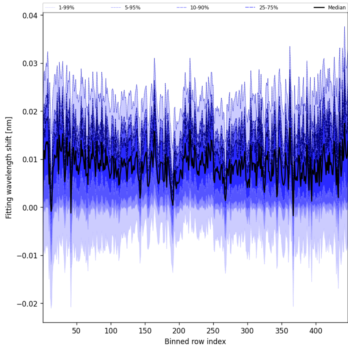
Figure 65: Along track statistics of “Fitting wavelength shift” for 2025-02-13 to 2025-02-14
