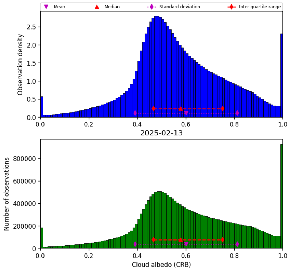
Figure 44: Histogram of “Cloud albedo (CRB)” for 2025-02-13 to 2025-02-14
