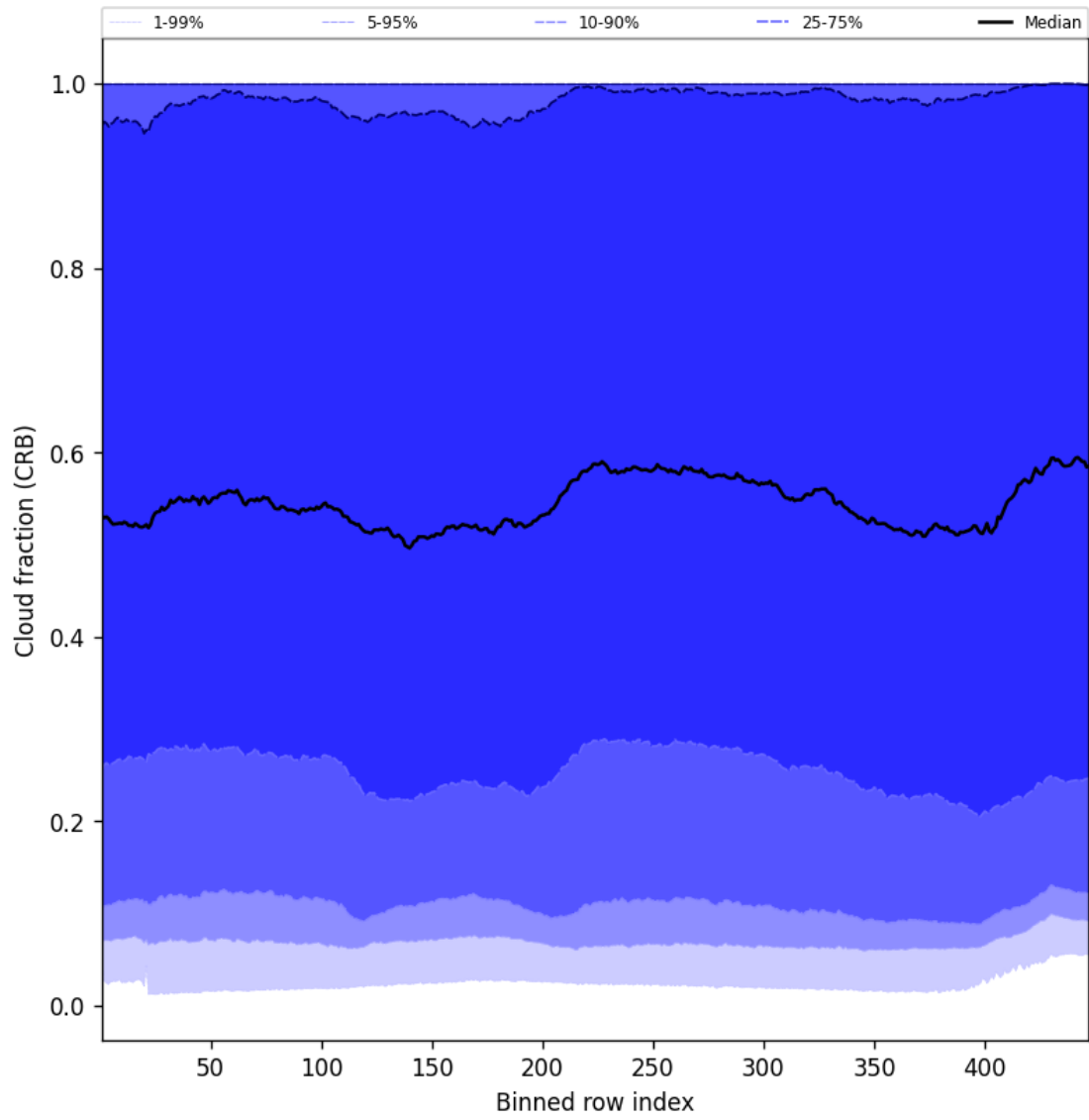
Figure 58: Along track statistics of “Cloud fraction (CRB)” for 2025-02-13 to 2025-02-14
