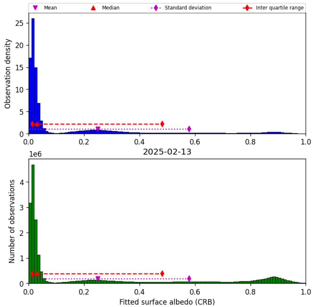
Figure 46: Histogram of “Fitted surface albedo (CRB)” for 2025-02-13 to 2025-02-14
