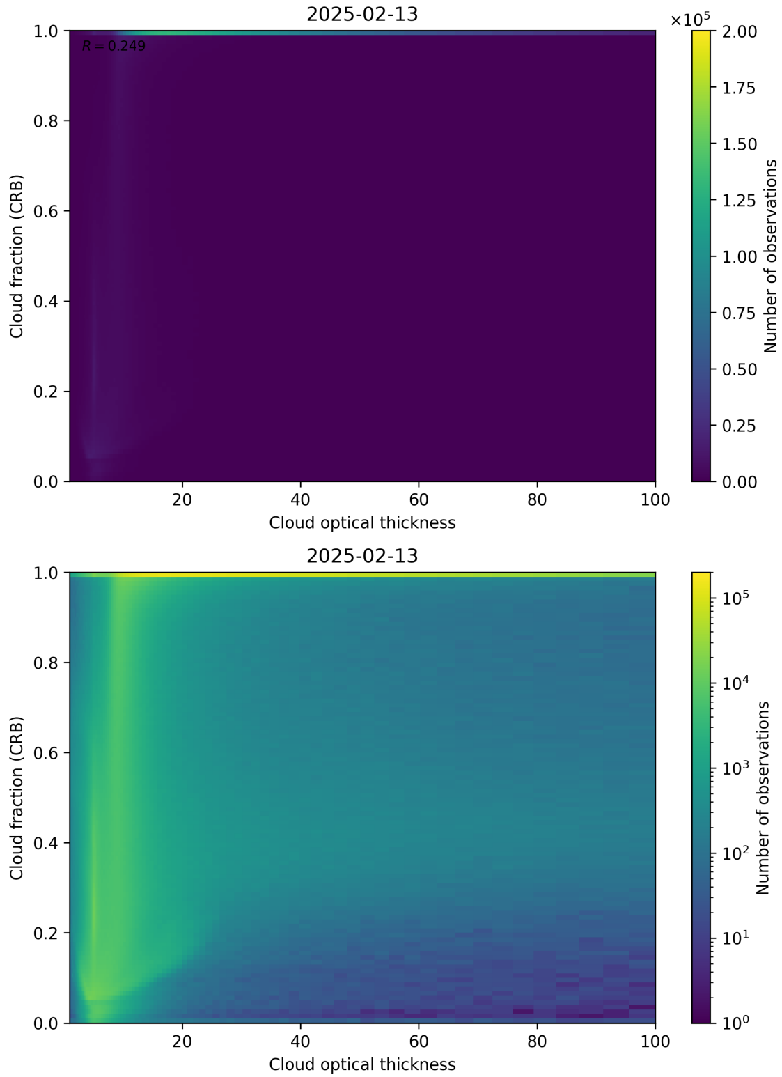
Figure 84: Scatter density plot of “Cloud optical thickness” against “Cloud fraction (CRB)” for 2025-02-13 to 2025-02-14.
