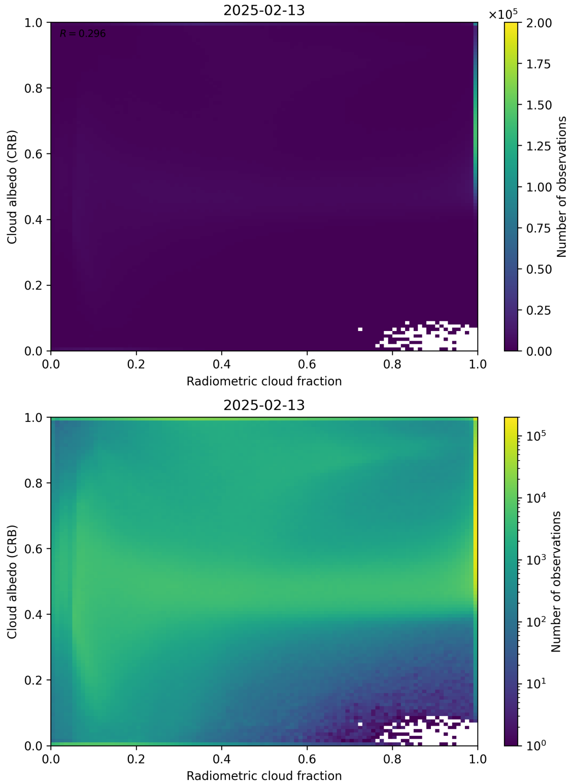
Figure 71: Scatter density plot of “Radiometric cloud fraction” against “Cloud albedo (CRB)” for 2025-02-13 to 2025-02-14.
