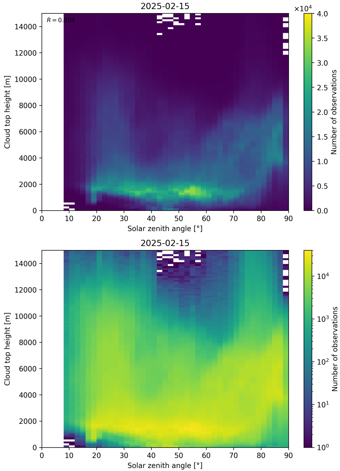
Figure 104: Scatter density plot of “Solar zenith angle” against “Cloud top height” for 2025-02-14 to 2025-02-16.
