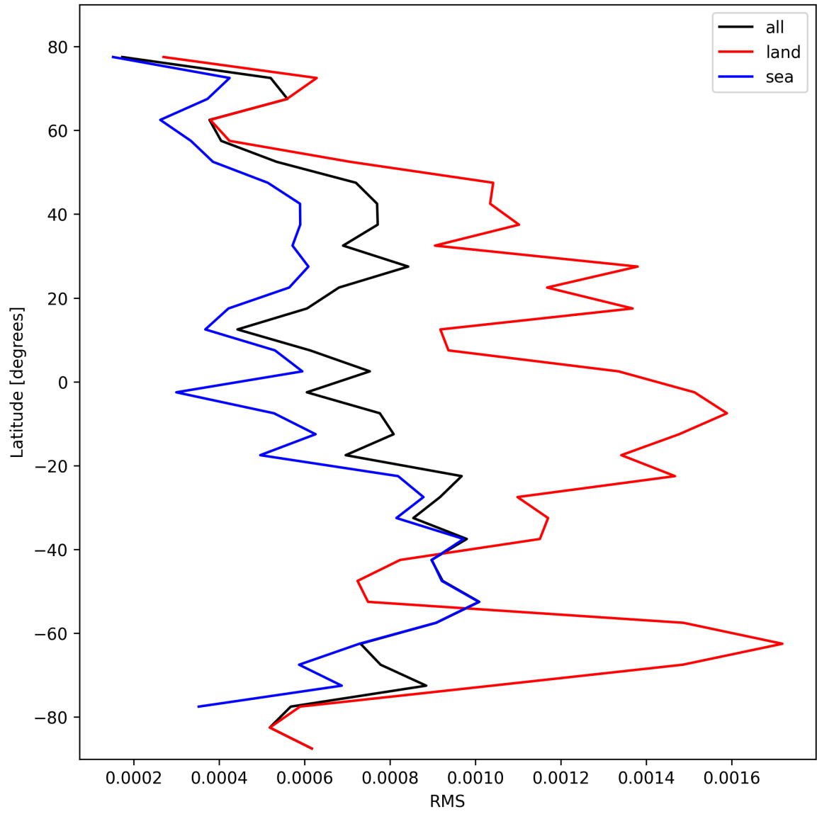
Figure 31: Zonal average of “RMS” for 2025-02-14 to 2025-02-16.
