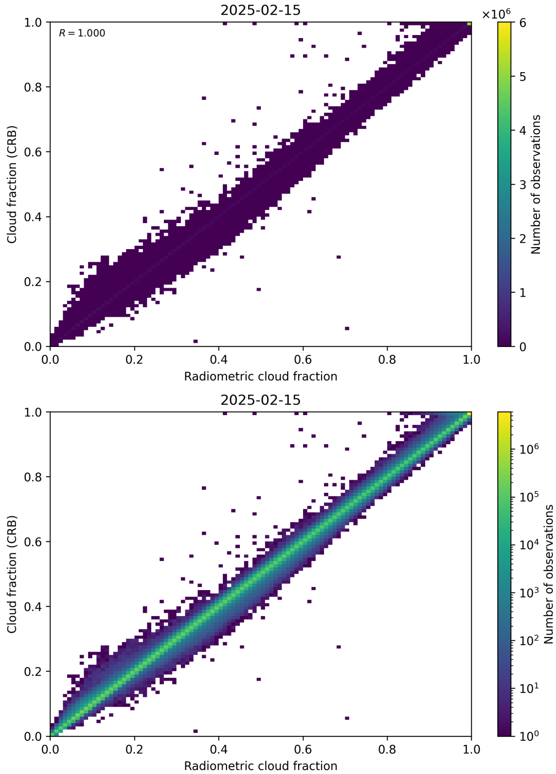
Figure 73: Scatter density plot of “Radiometric cloud fraction” against “Cloud fraction (CRB)” for 2025-02-14 to 2025-02-16.
