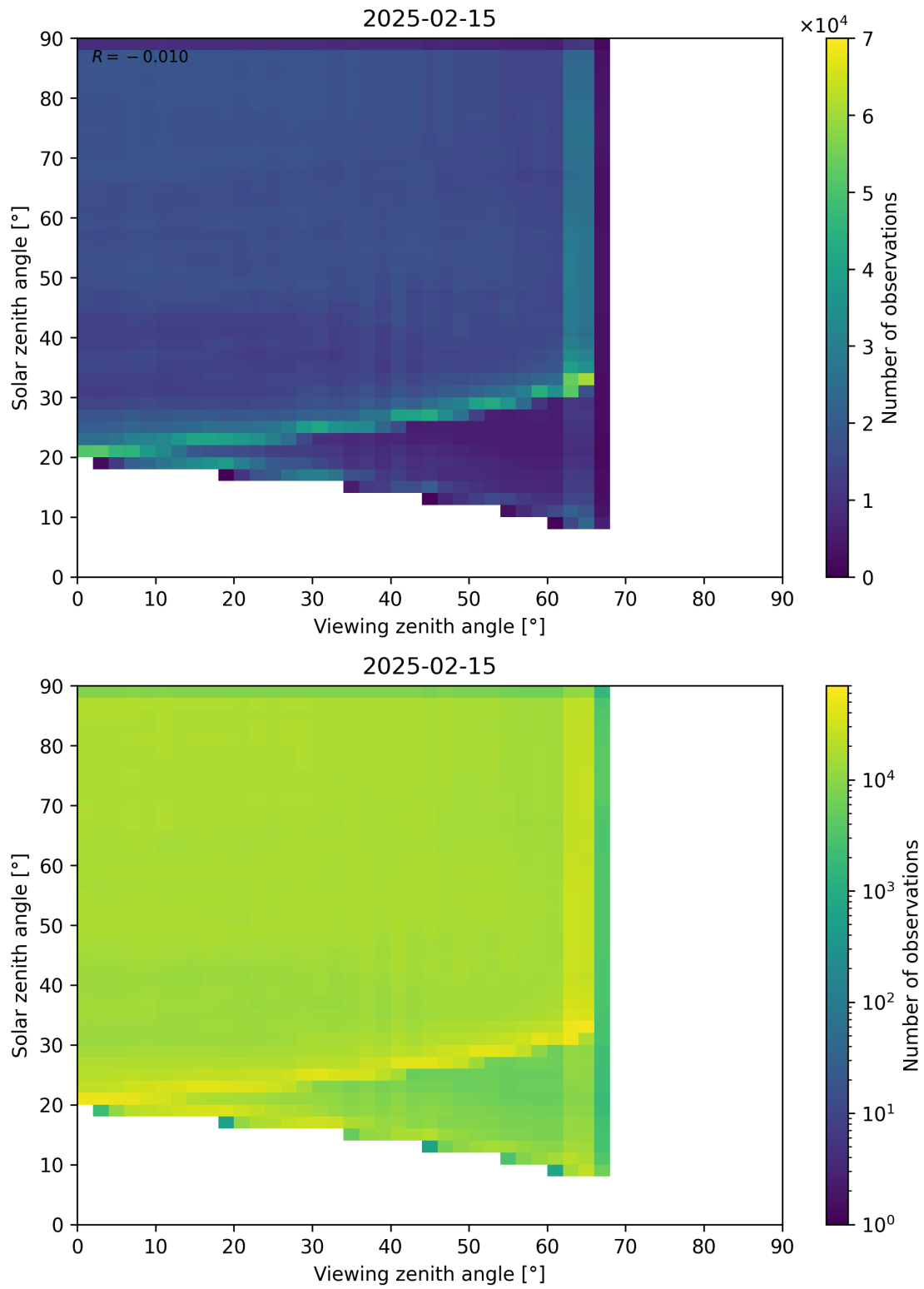
Figure 114: Scatter density plot of “Viewing zenith angle” against “Solar zenith angle” for 2025-02-14 to 2025-02-16.
