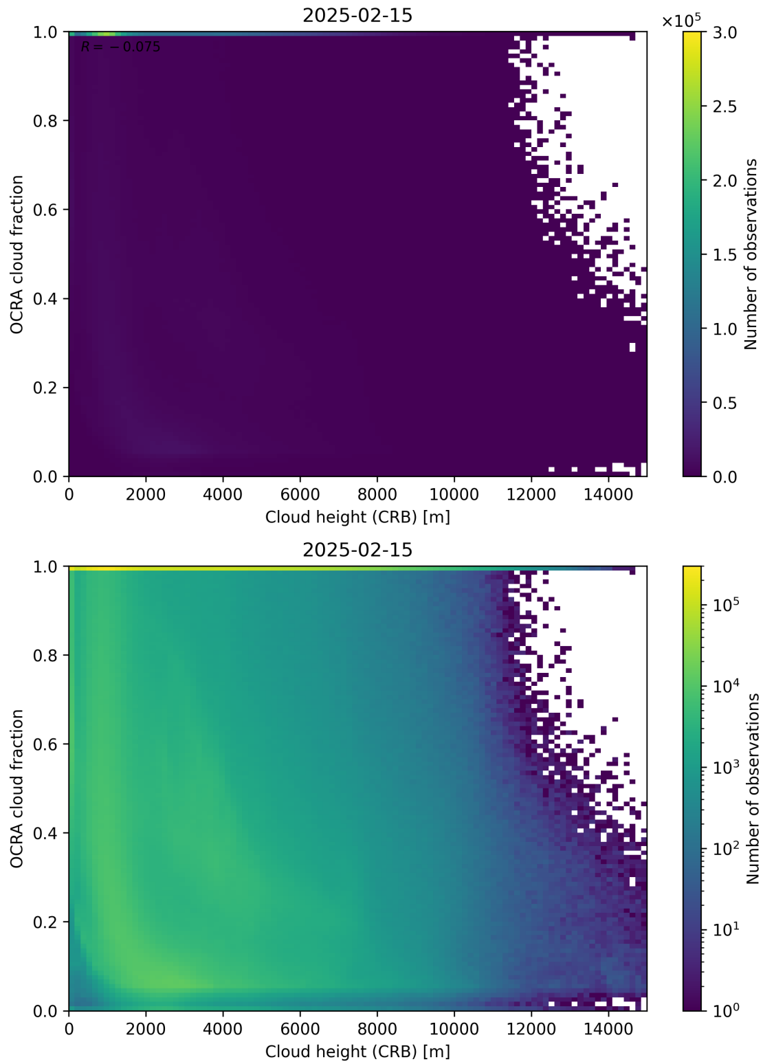
Figure 81: Scatter density plot of “Cloud height (CRB)” against “OCRA cloud fraction” for 2025-02-14 to 2025-02-16.
