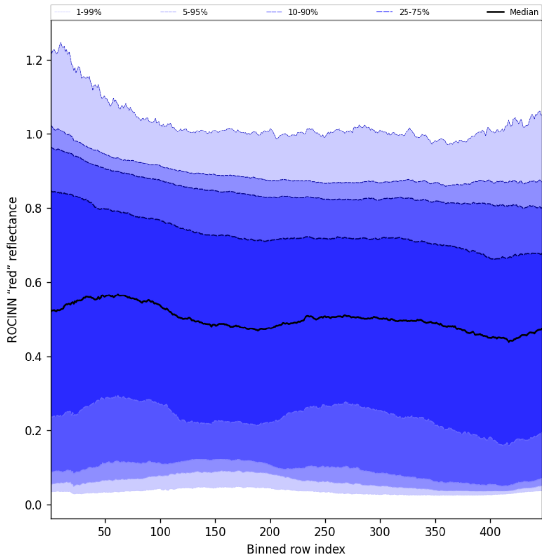
Figure 69: Along track statistics of “ROCINN “red” reflectance” for 2025-02-14 to 2025-02-16
