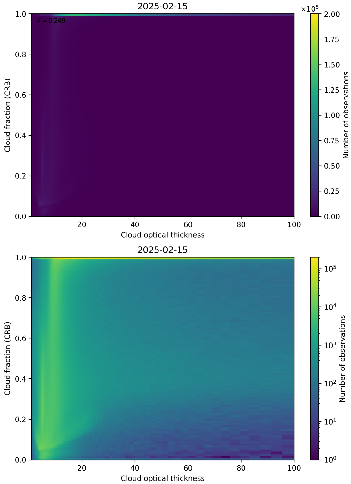
Figure 84: Scatter density plot of “Cloud optical thickness” against “Cloud fraction (CRB)” for 2025-02-14 to 2025-02-16.
