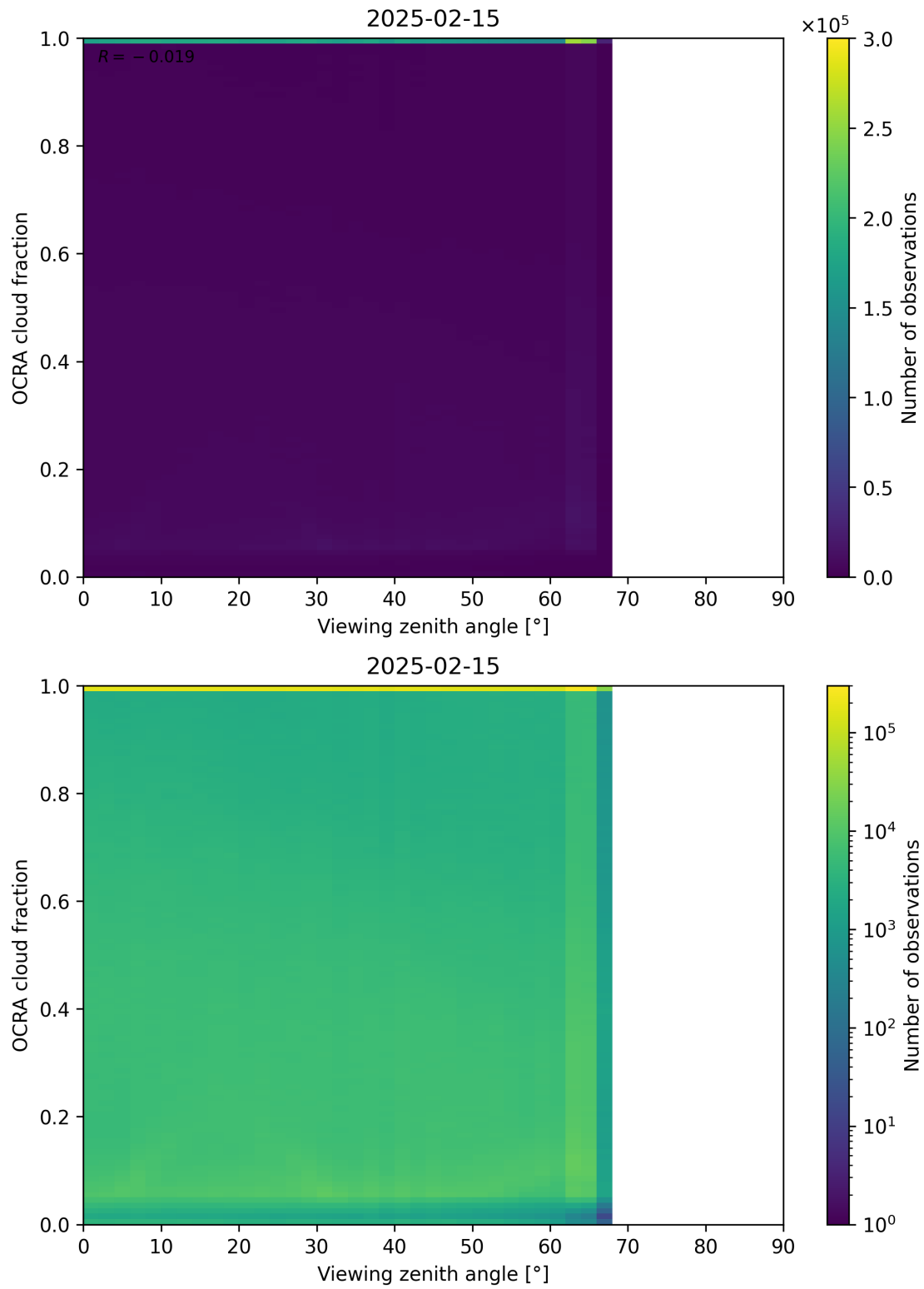
Figure 108: Scatter density plot of “Viewing zenith angle” against “OCRA cloud fraction” for 2025-02-14 to 2025-02-16.
