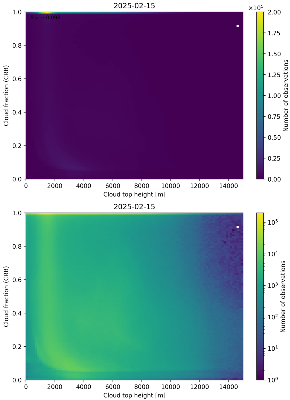
Figure 88: Scatter density plot of “Cloud top height” against “Cloud fraction (CRB)” for 2025-02-14 to 2025-02-16.
