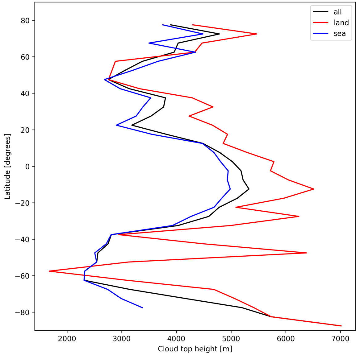
Figure 24: Zonal average of “Cloud top height” for 2025-02-14 to 2025-02-16.
