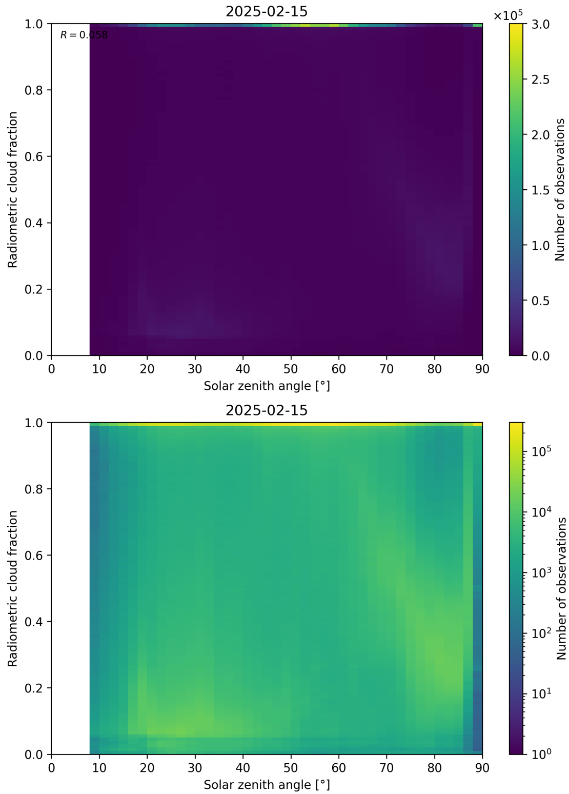
Figure 99: Scatter density plot of “Solar zenith angle” against “Radiometric cloud fraction” for 2025-02-14 to 2025-02-16.
