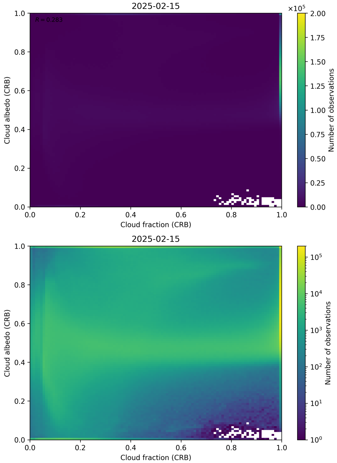
Figure 77: Scatter density plot of “Cloud fraction (CRB)” against “Cloud albedo (CRB)” for 2025-02-14 to 2025-02-16.
