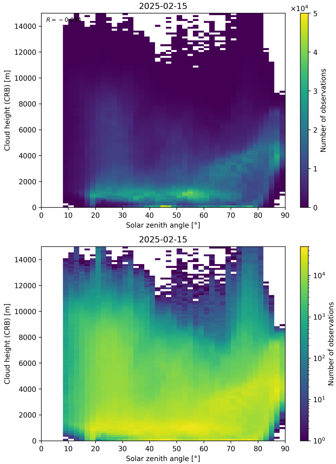
Figure 102: Scatter density plot of “Solar zenith angle” against “Cloud height (CRB)” for 2025-02-14 to 2025-02-16.
