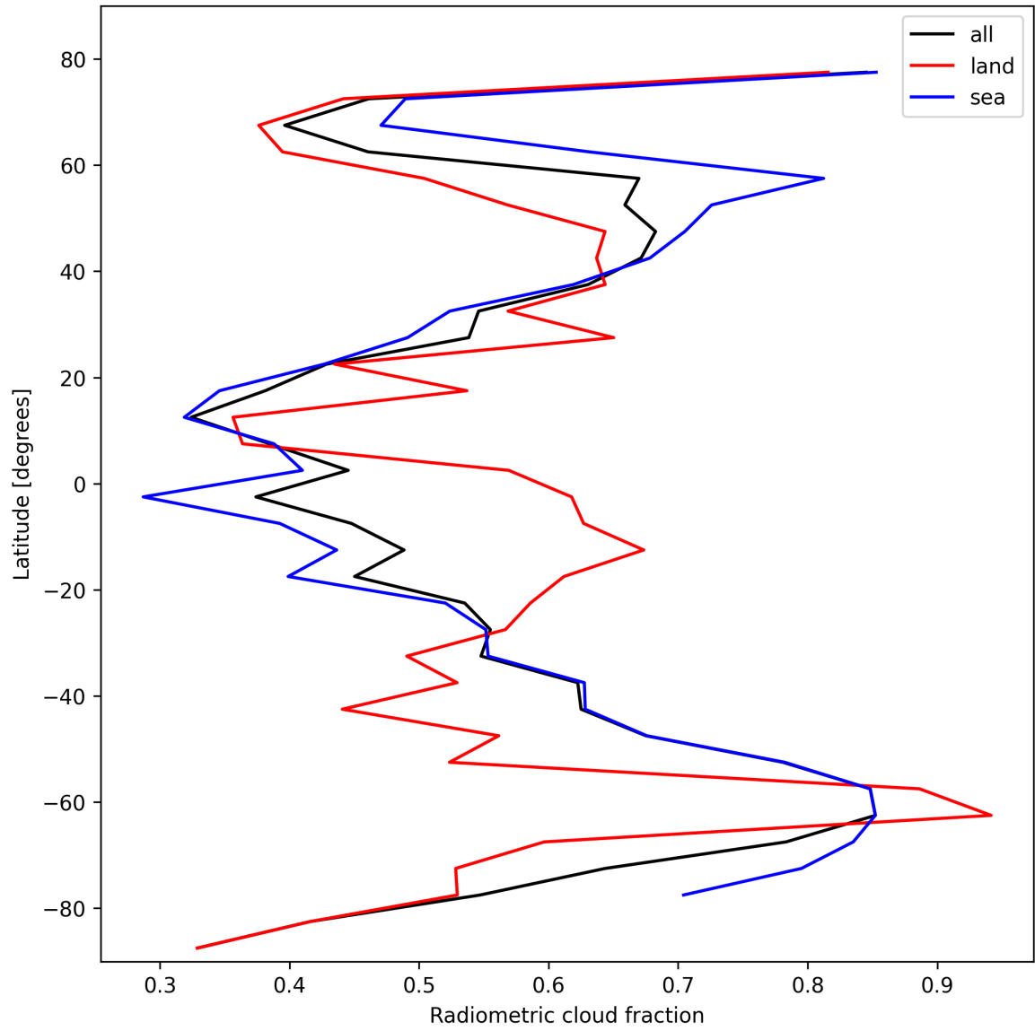
Figure 23: Zonal average of “Radiometric cloud fraction” for 2025-02-14 to 2025-02-16.
