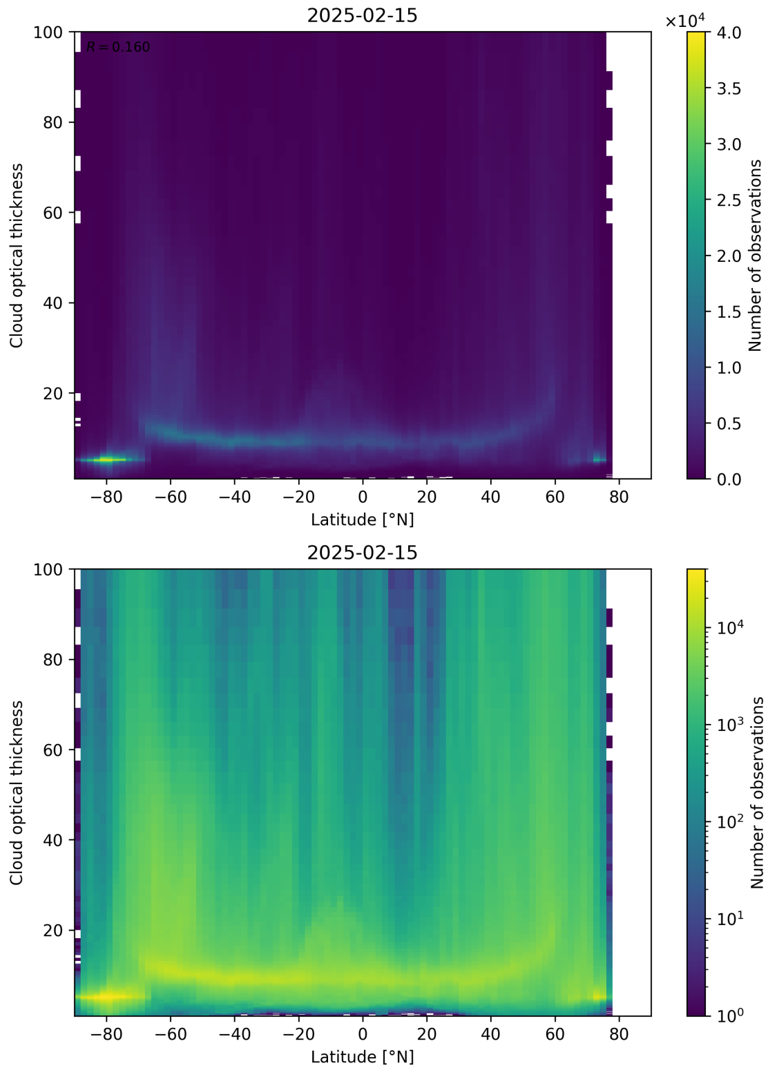
Figure 96: Scatter density plot of “Latitude” against “Cloud optical thickness” for 2025-02-14 to 2025-02-16.
