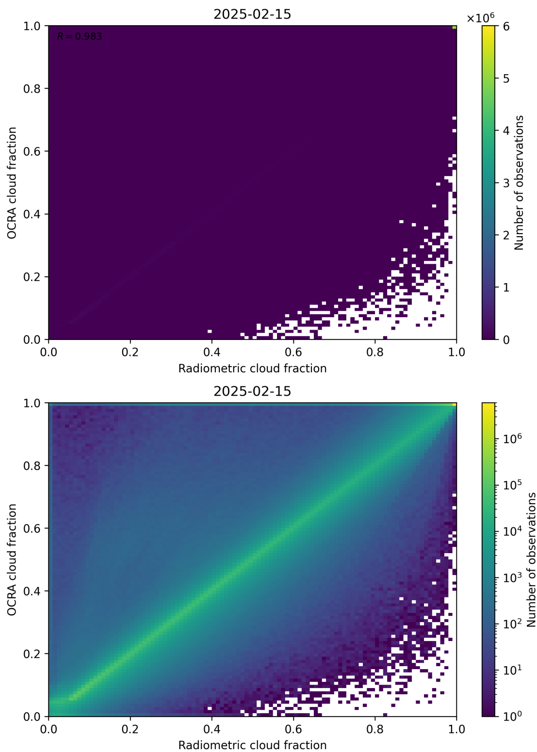
Figure 72: Scatter density plot of “Radiometric cloud fraction” against “OCRA cloud fraction” for 2025-02-14 to 2025-02-16.
