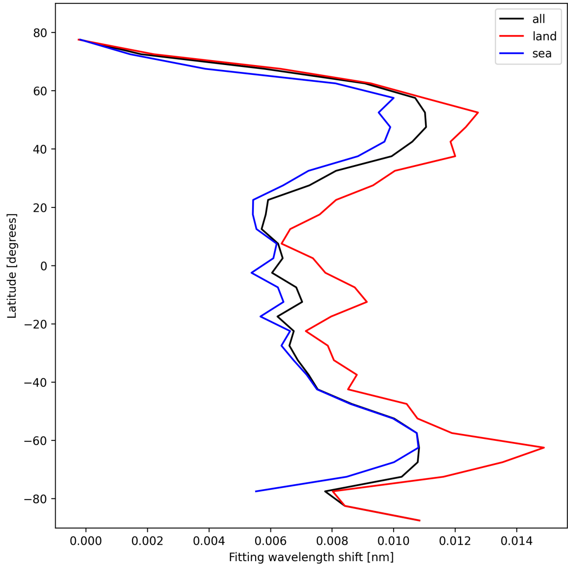
Figure 33: Zonal average of “Fitting wavelength shift” for 2025-02-14 to 2025-02-16.
