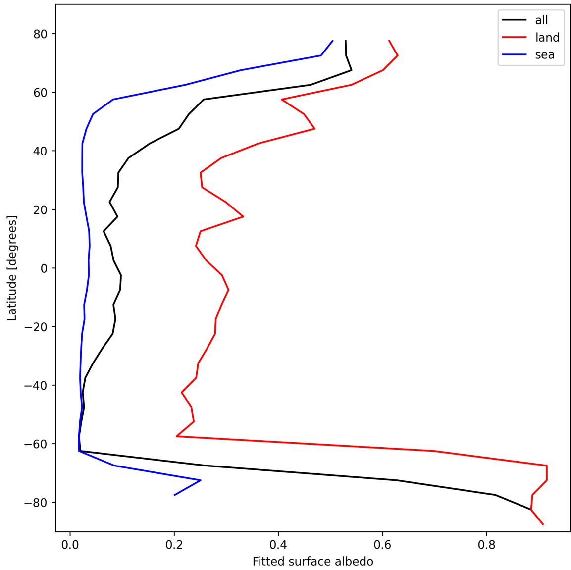
Figure 29: Zonal average of “Fitted surface albedo” for 2025-02-14 to 2025-02-16.
