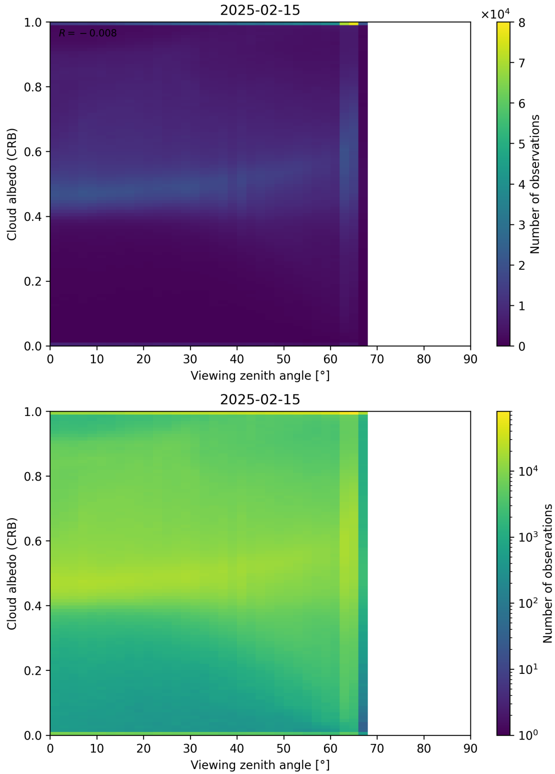
Figure 106: Scatter density plot of “Viewing zenith angle” against “Cloud albedo (CRB)” for 2025-02-14 to 2025-02-16.
