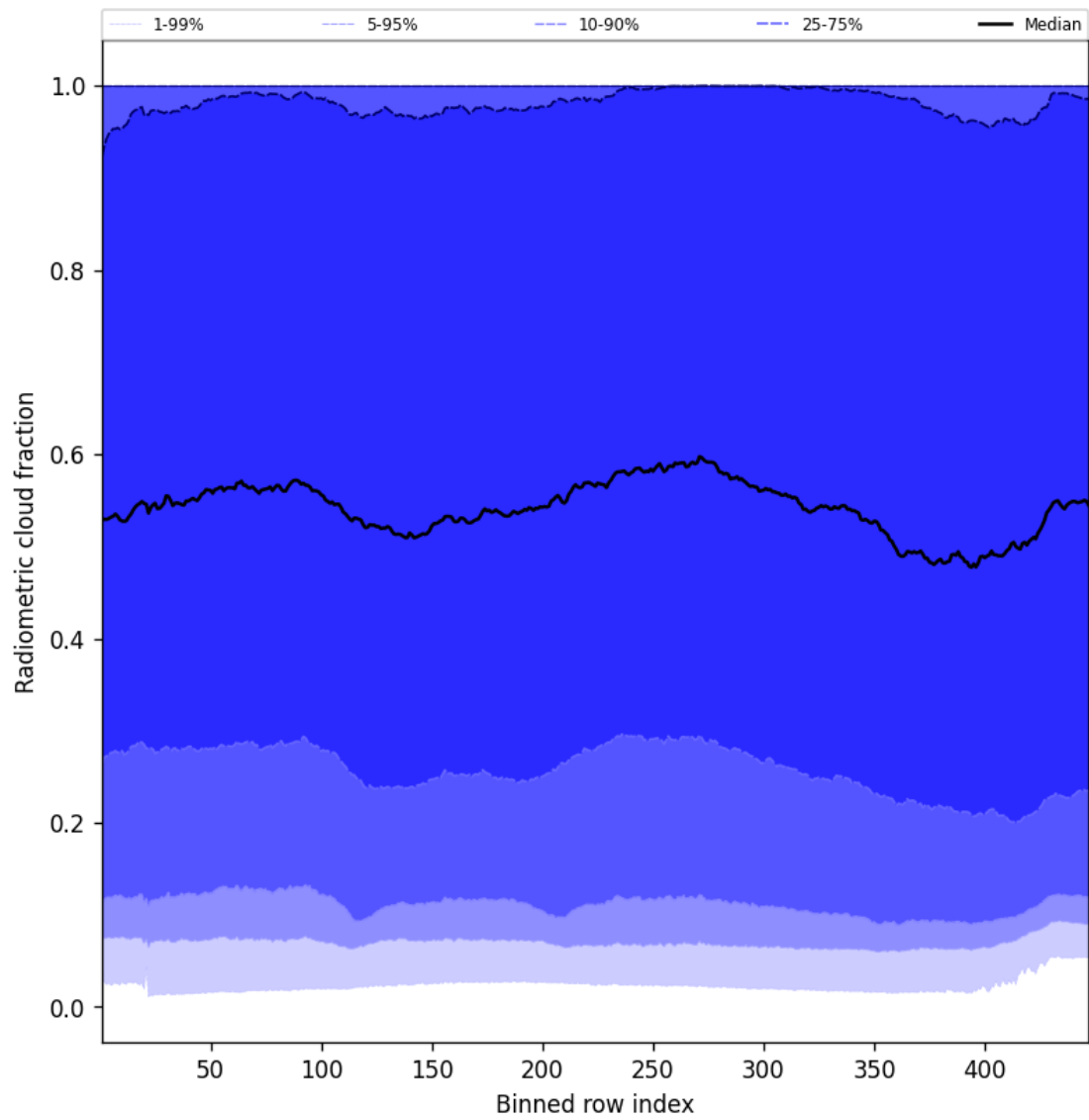
Figure 55: Along track statistics of “Radiometric cloud fraction” for 2025-02-14 to 2025-02-16
