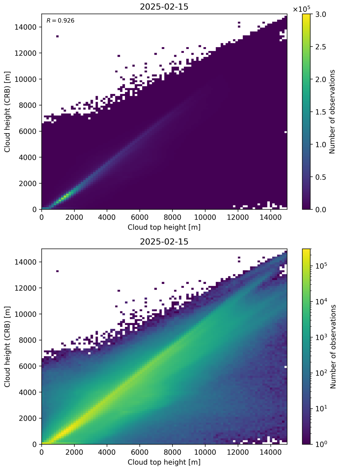
Figure 89: Scatter density plot of “Cloud top height” against “Cloud height (CRB)” for 2025-02-14 to 2025-02-16.
