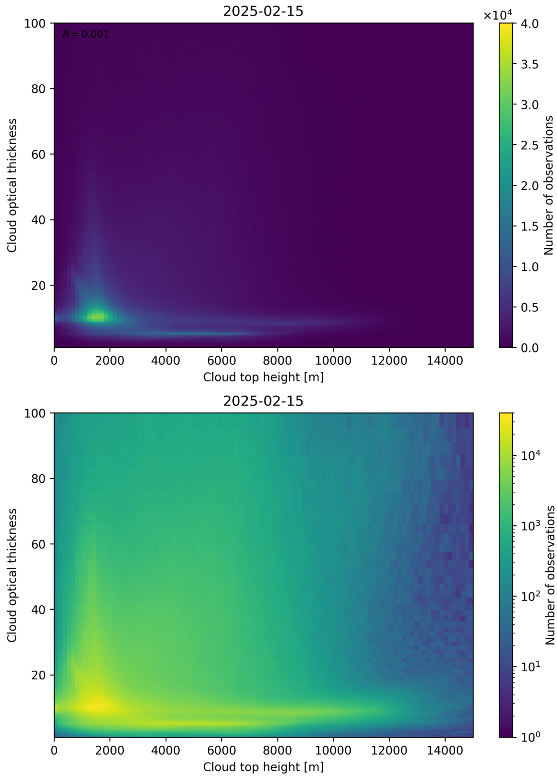
Figure 90: Scatter density plot of “Cloud top height” against “Cloud optical thickness” for 2025-02-14 to 2025-02-16.
