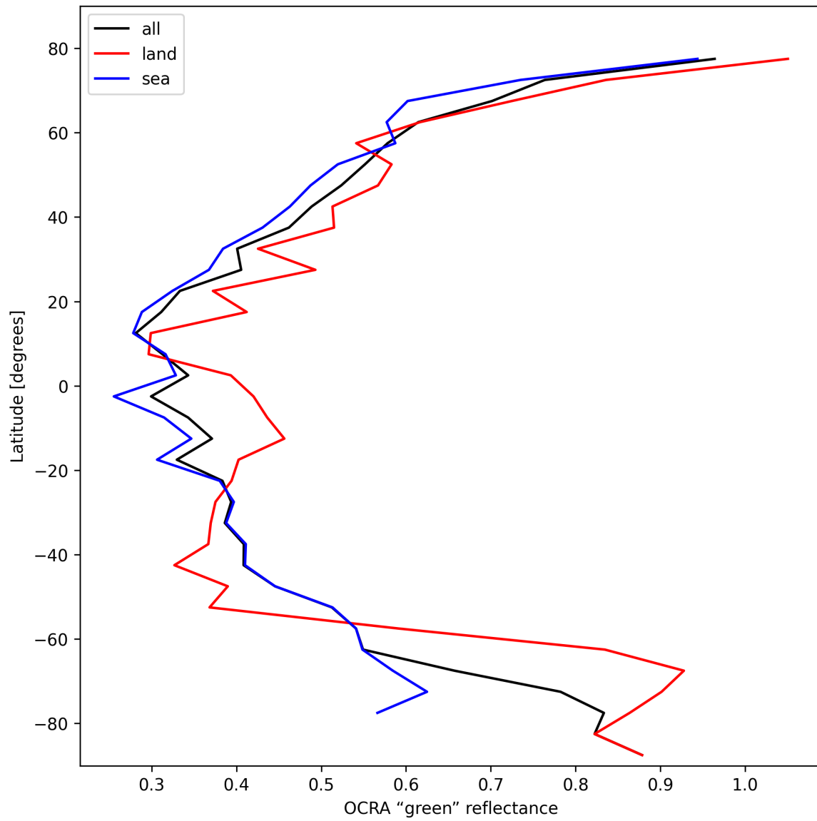
Figure 36: Zonal average of “OCRA “green” reflectance” for 2025-02-14 to 2025-02-16.
