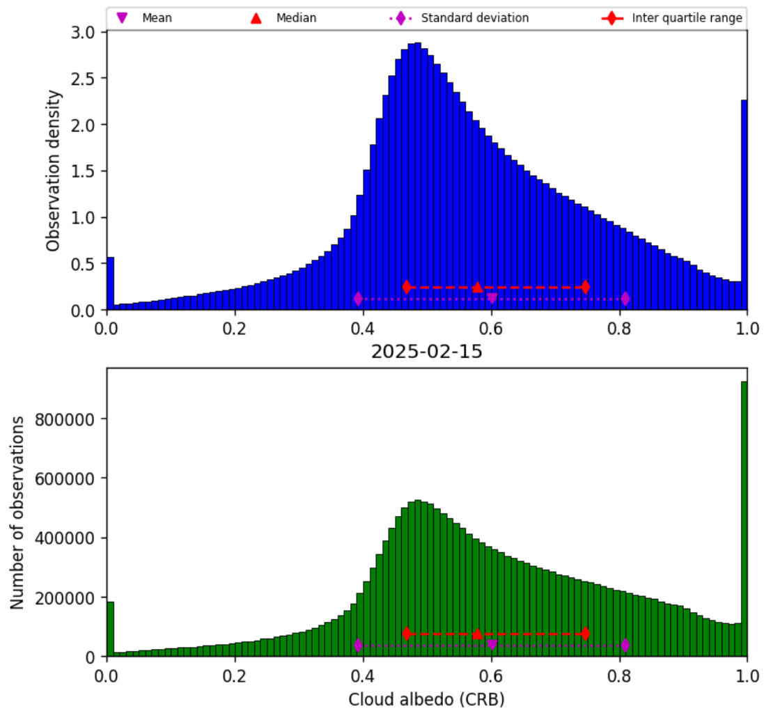
Figure 44: Histogram of “Cloud albedo (CRB)” for 2025-02-14 to 2025-02-16
