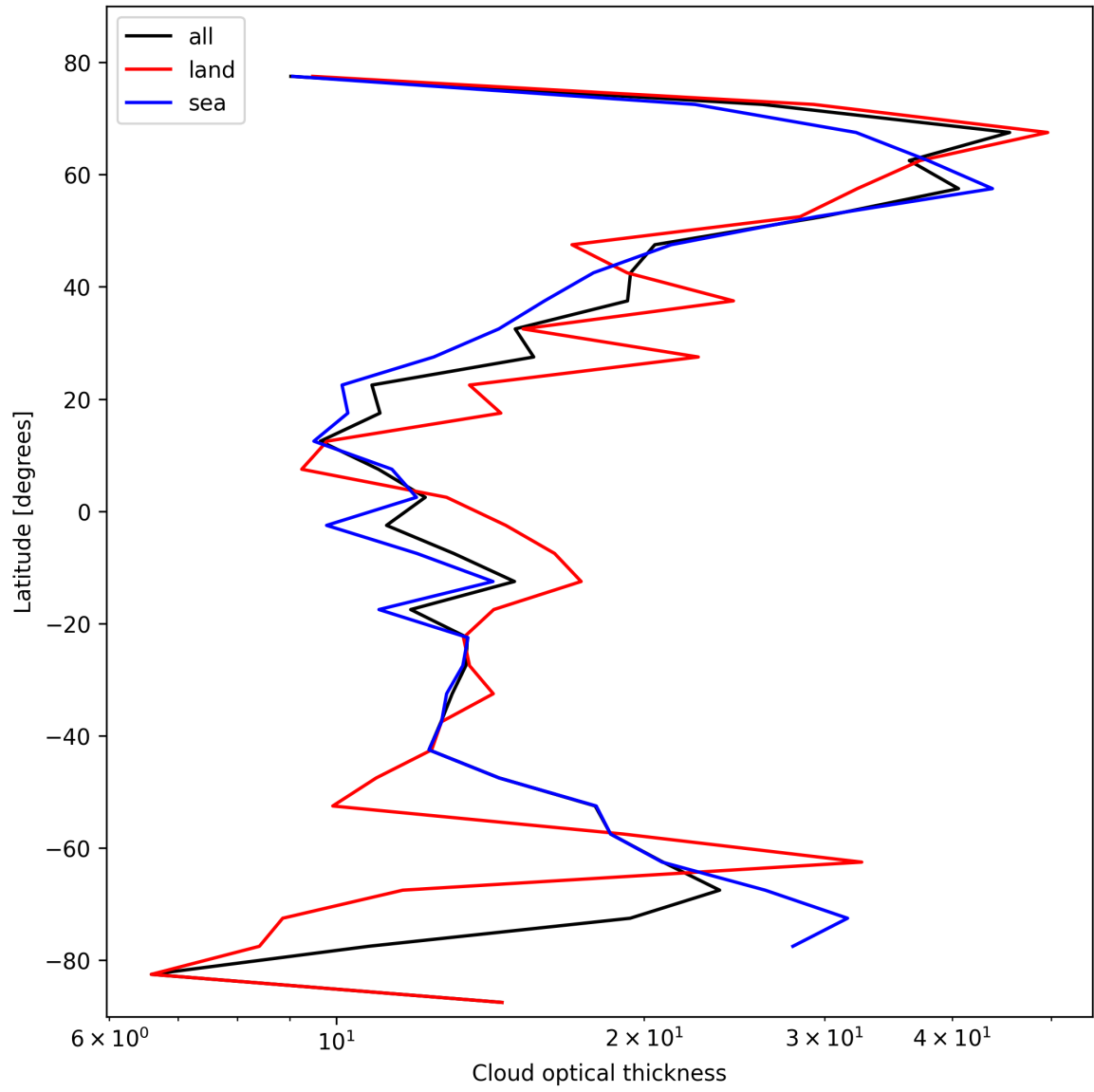
Figure 25: Zonal average of “Cloud optical thickness” for 2025-02-14 to 2025-02-16.
