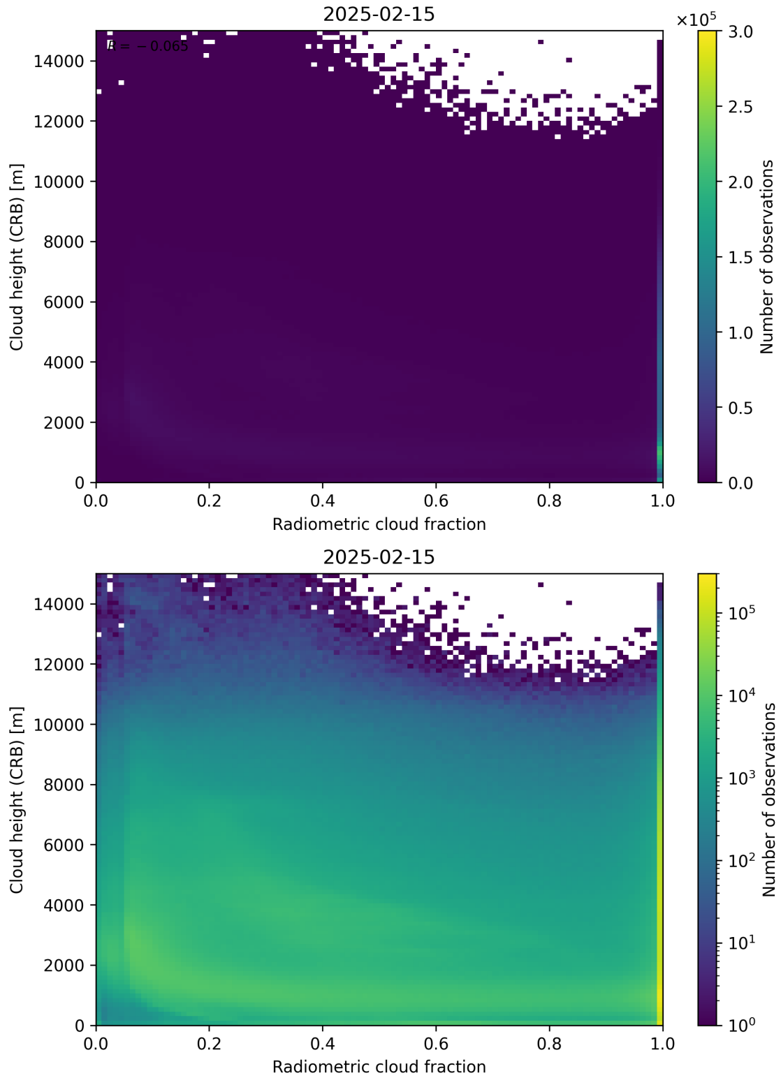
Figure 74: Scatter density plot of “Radiometric cloud fraction” against “Cloud height (CRB)” for 2025-02-14 to 2025-02-16.
