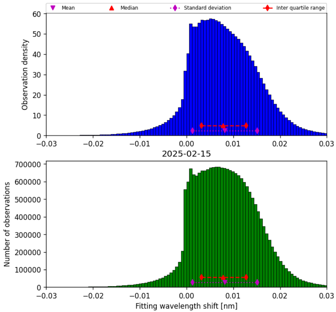
Figure 49: Histogram of “Fitting wavelength shift” for 2025-02-14 to 2025-02-16
