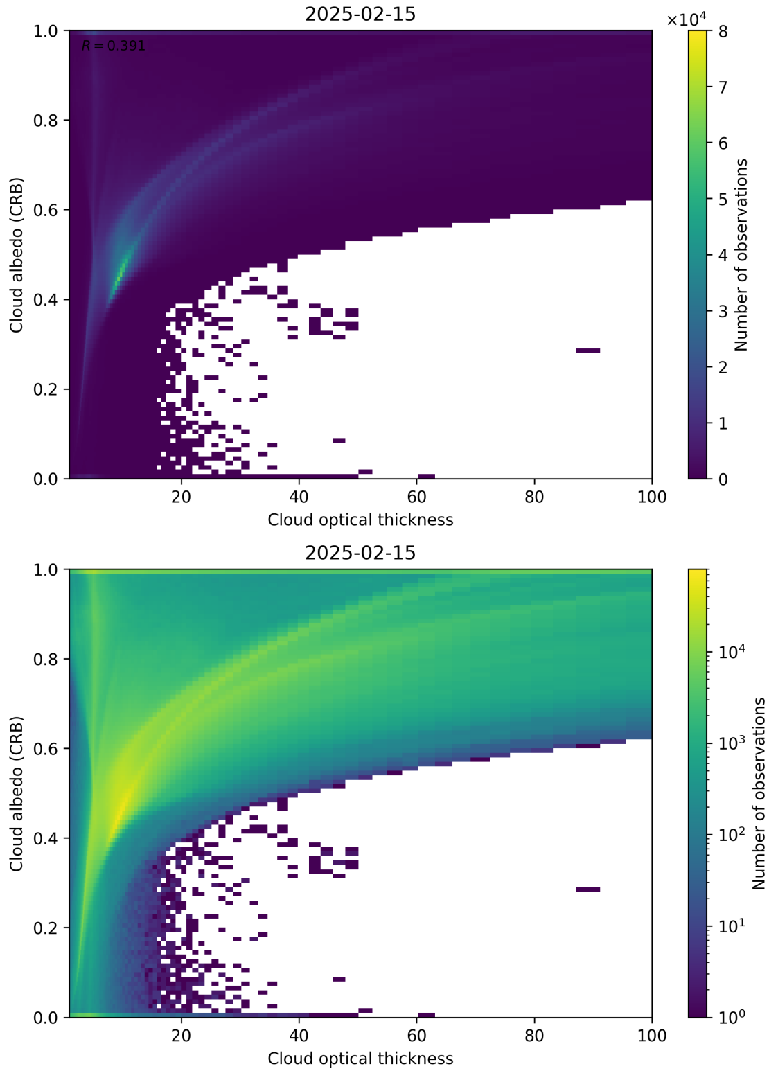
Figure 82: Scatter density plot of “Cloud optical thickness” against “Cloud albedo (CRB)” for 2025-02-14 to 2025-02-16.
