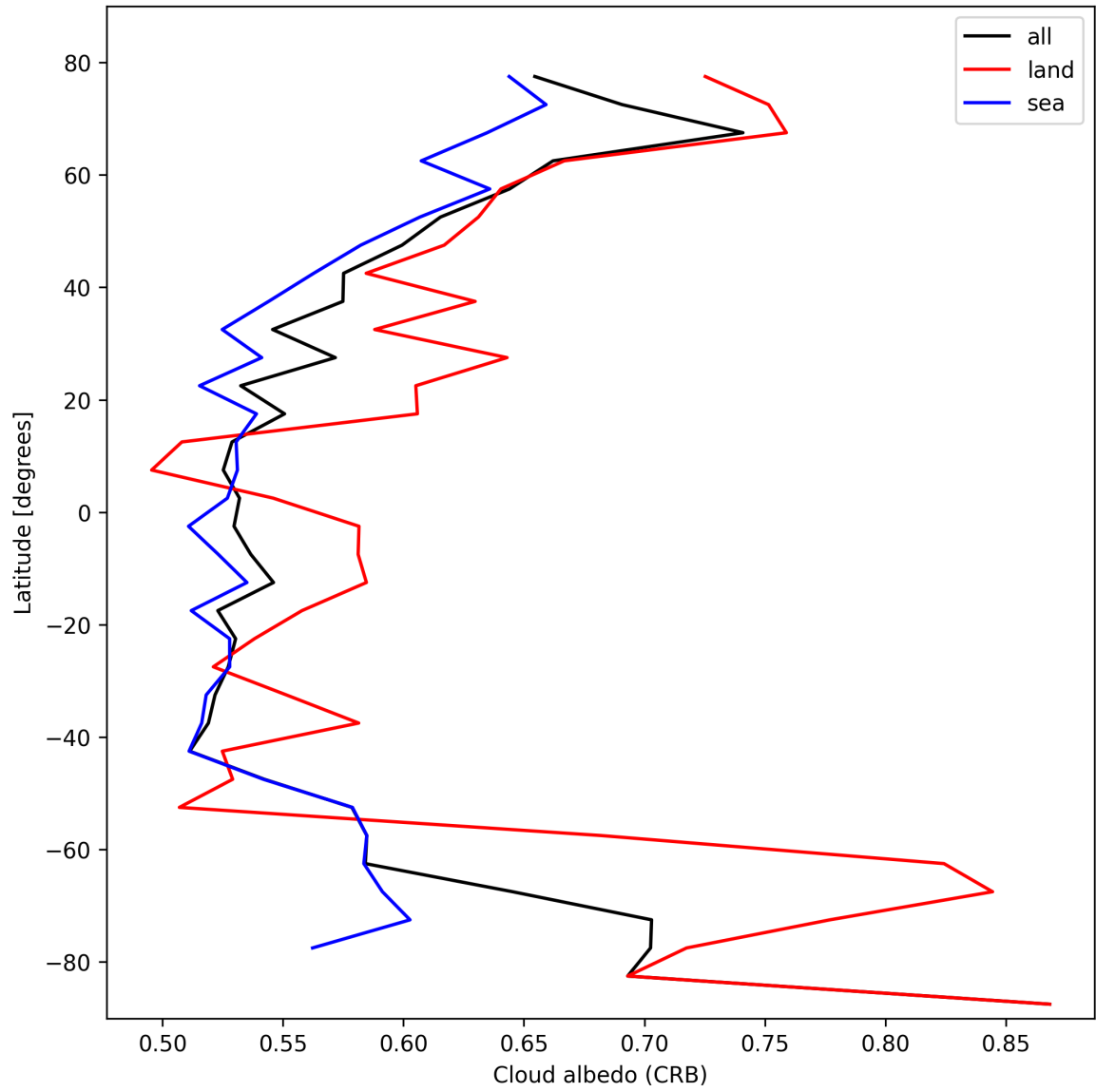
Figure 28: Zonal average of “Cloud albedo (CRB)” for 2025-02-14 to 2025-02-16.
