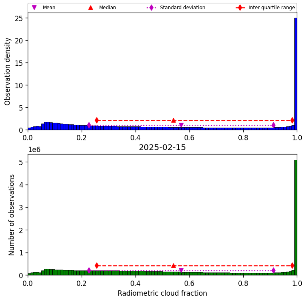
Figure 39: Histogram of “Radiometric cloud fraction” for 2025-02-14 to 2025-02-16
