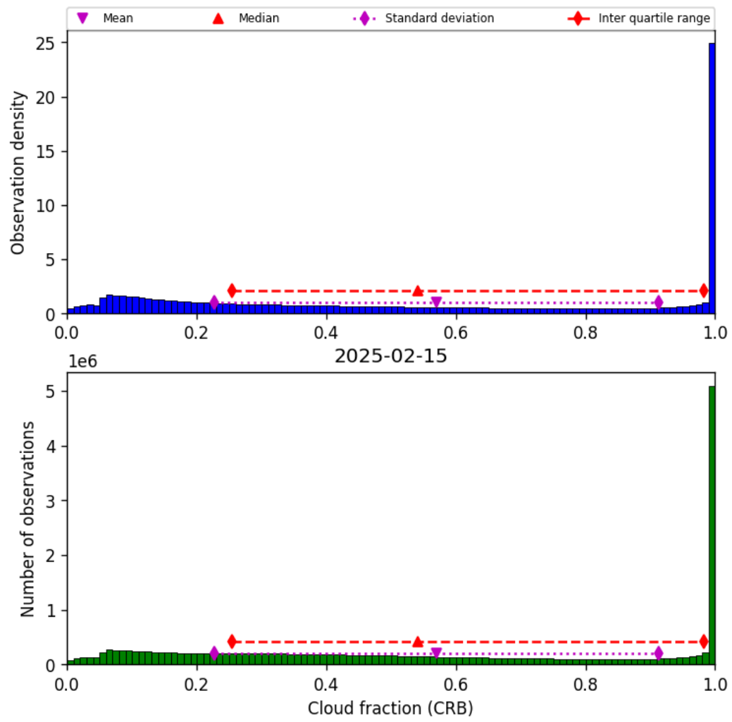
Figure 42: Histogram of “Cloud fraction (CRB)” for 2025-02-14 to 2025-02-16
