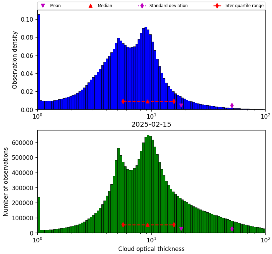
Figure 41: Histogram of “Cloud optical thickness” for 2025-02-14 to 2025-02-16
