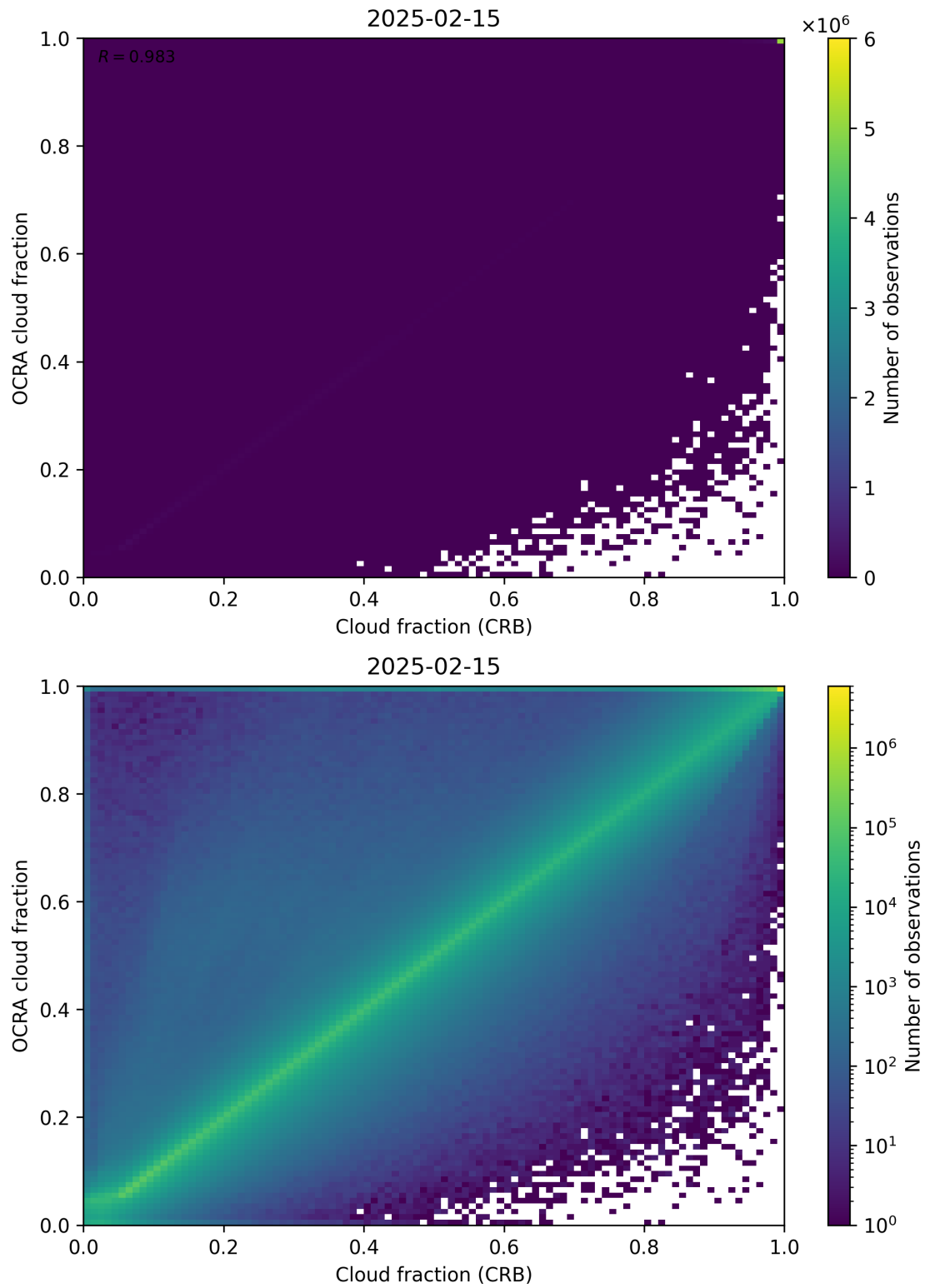
Figure 78: Scatter density plot of “Cloud fraction (CRB)” against “OCRA cloud fraction” for 2025-02-14 to 2025-02-16.
