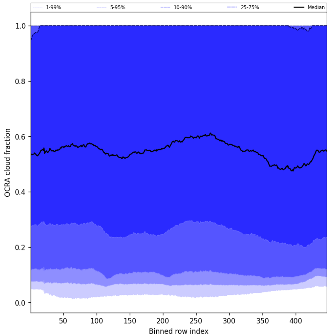
Figure 66: Along track statistics of “OCRA cloud fraction” for 2025-02-14 to 2025-02-16
