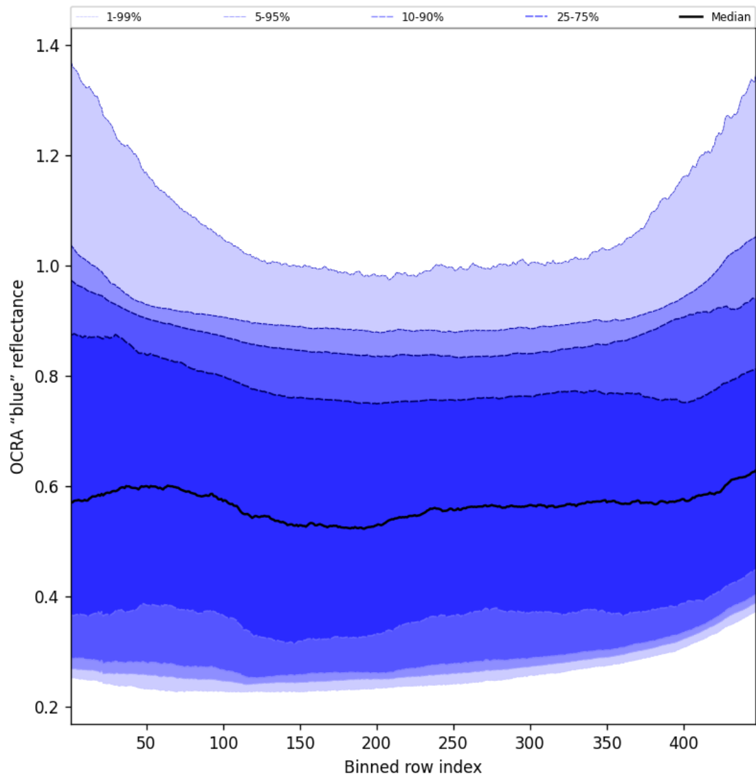
Figure 67: Along track statistics of "OCRA "blue" reflectance" for 2025-02-14 to 2025-02-16
