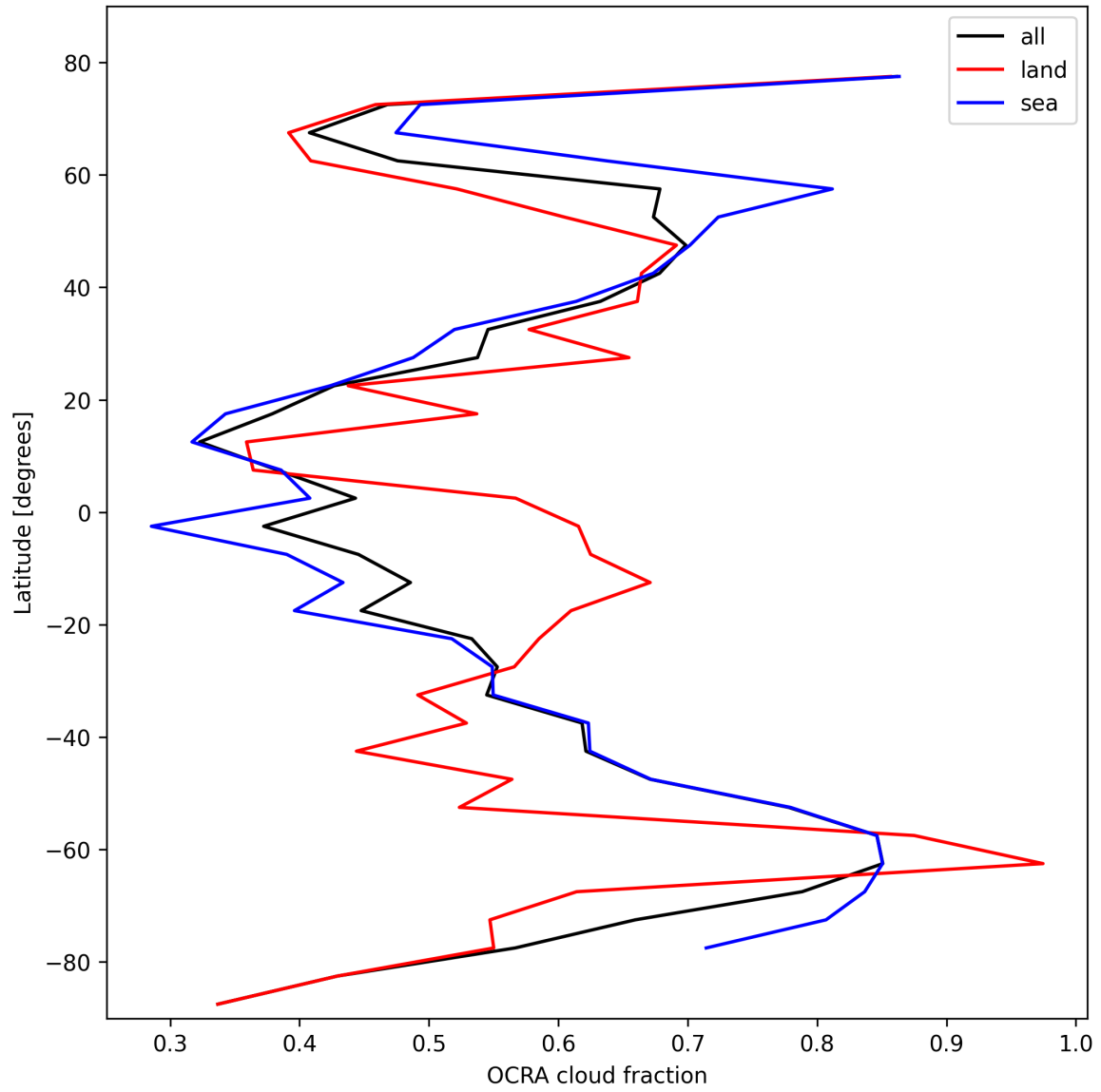
Figure 34: Zonal average of “OCRA cloud fraction” for 2025-02-14 to 2025-02-16.
