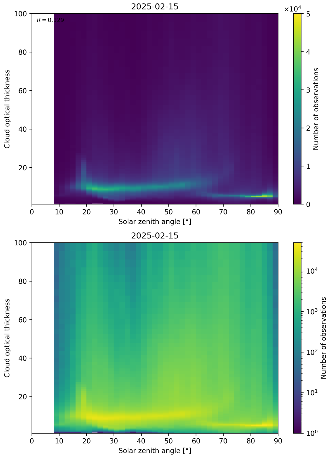
Figure 103: Scatter density plot of “Solar zenith angle” against “Cloud optical thickness” for 2025-02-14 to 2025-02-16.
