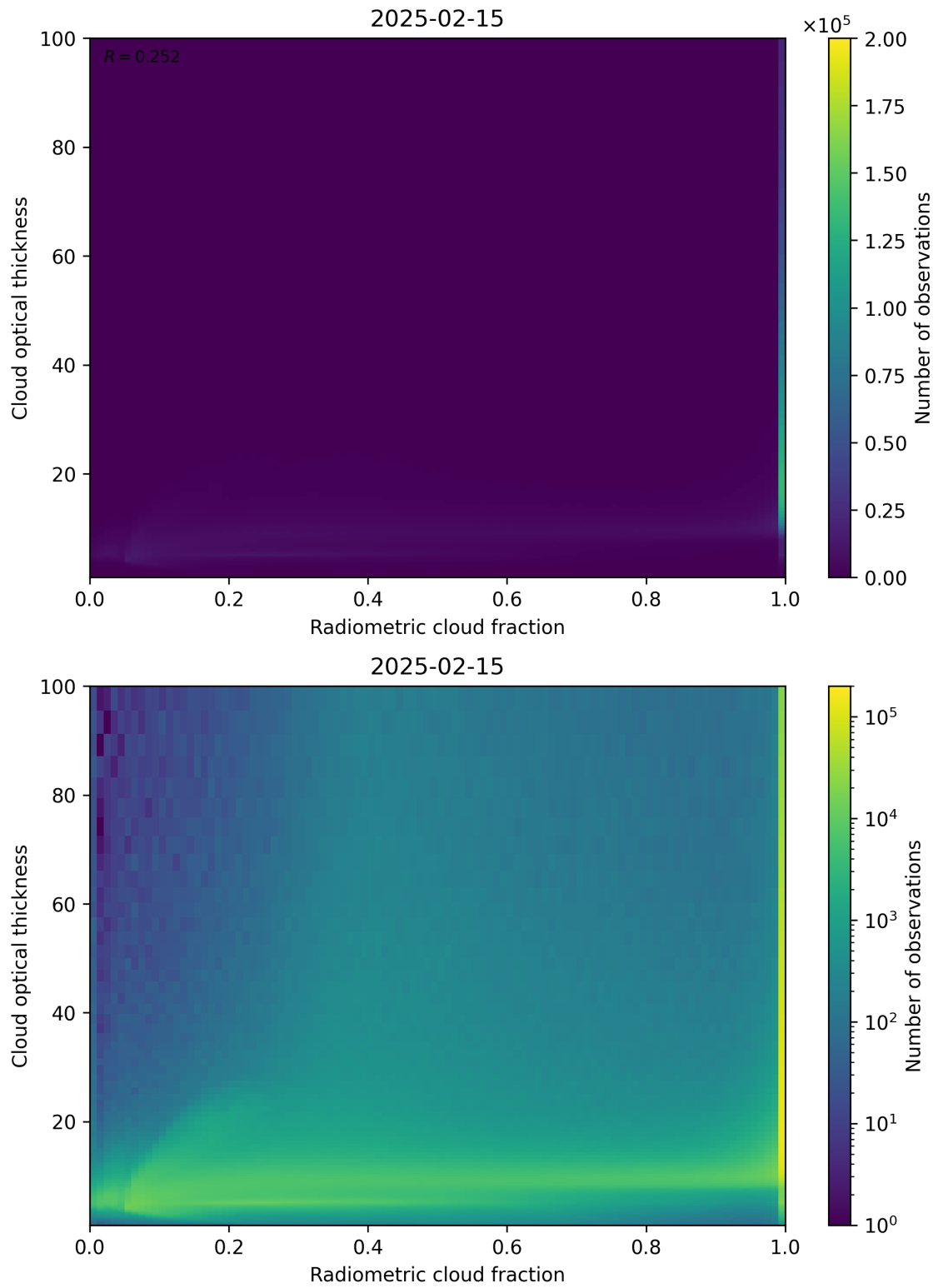
Figure 75: Scatter density plot of “Radiometric cloud fraction” against “Cloud optical thickness” for 2025-02-14 to 2025-02-16.
