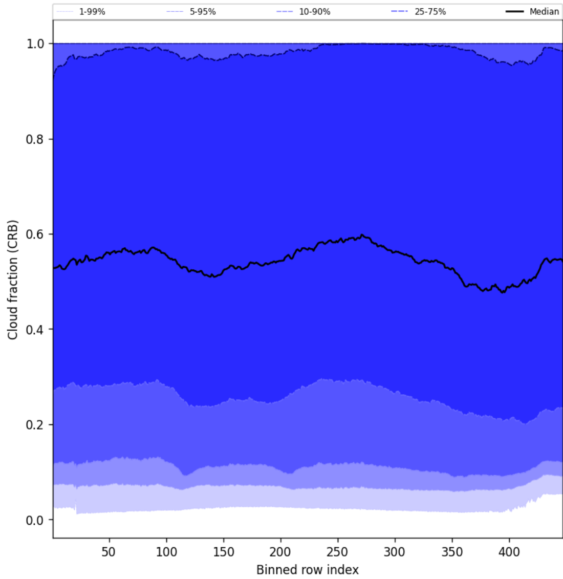
Figure 58: Along track statistics of “Cloud fraction (CRB)” for 2025-02-14 to 2025-02-16
