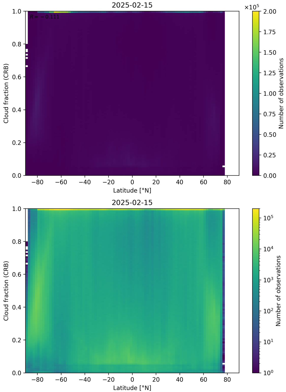
Figure 94: Scatter density plot of “Latitude” against “Cloud fraction (CRB)” for 2025-02-14 to 2025-02-16.
