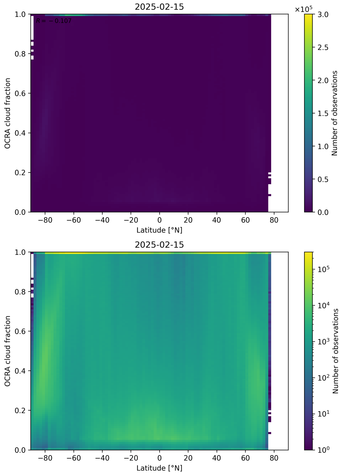
Figure 93: Scatter density plot of “Latitude” against “OCRA cloud fraction” for 2025-02-14 to 2025-02-16.
