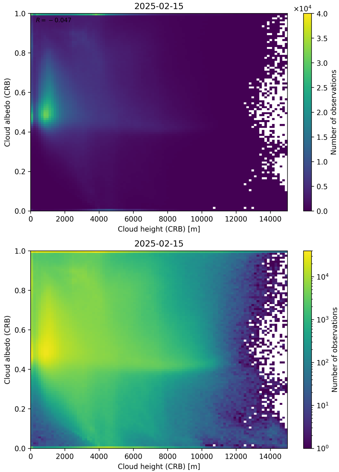
Figure 80: Scatter density plot of “Cloud height (CRB)” against “Cloud albedo (CRB)” for 2025-02-14 to 2025-02-16.
