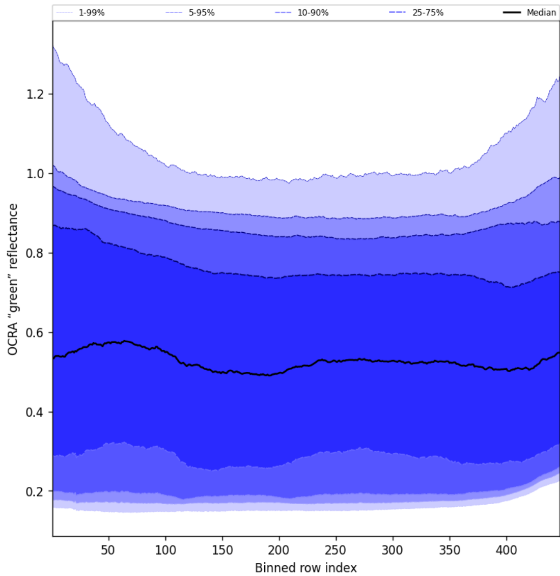
Figure 68: Along track statistics of "OCRA "green" reflectance" for 2025-02-14 to 2025-02-16
