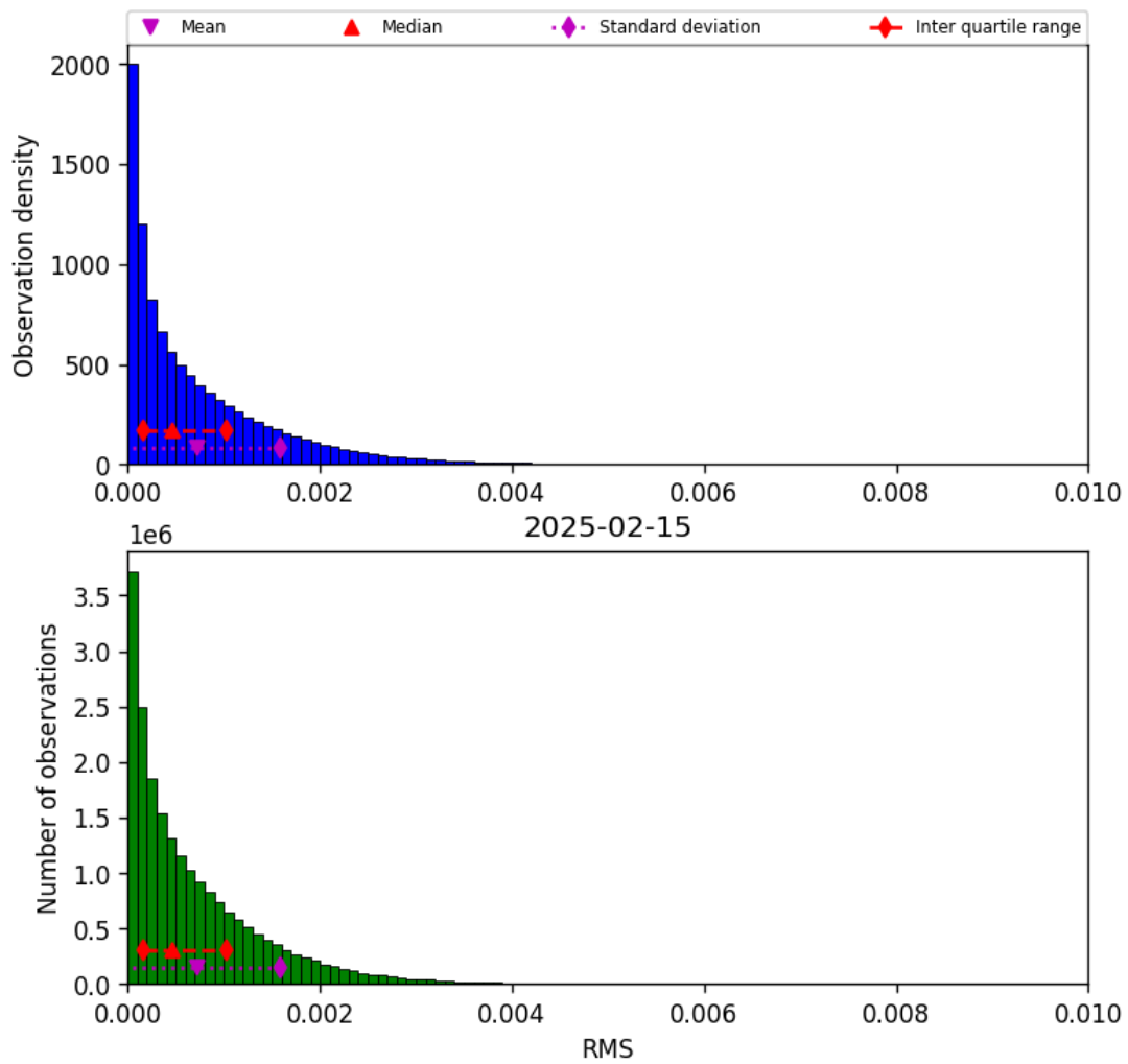
Figure 47: Histogram of “RMS” for 2025-02-14 to 2025-02-16
