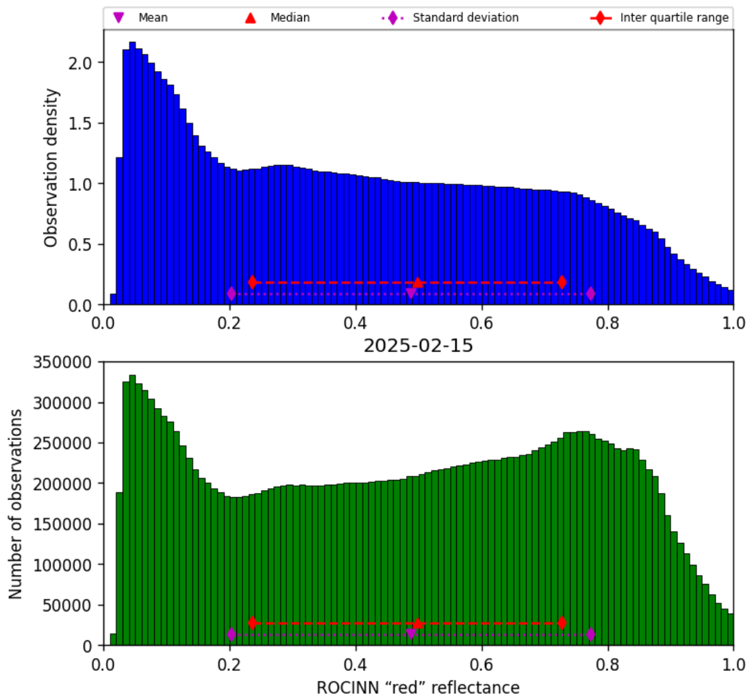
Figure 53: Histogram of “ROCINN “red” reflectance” for 2025-02-14 to 2025-02-16
