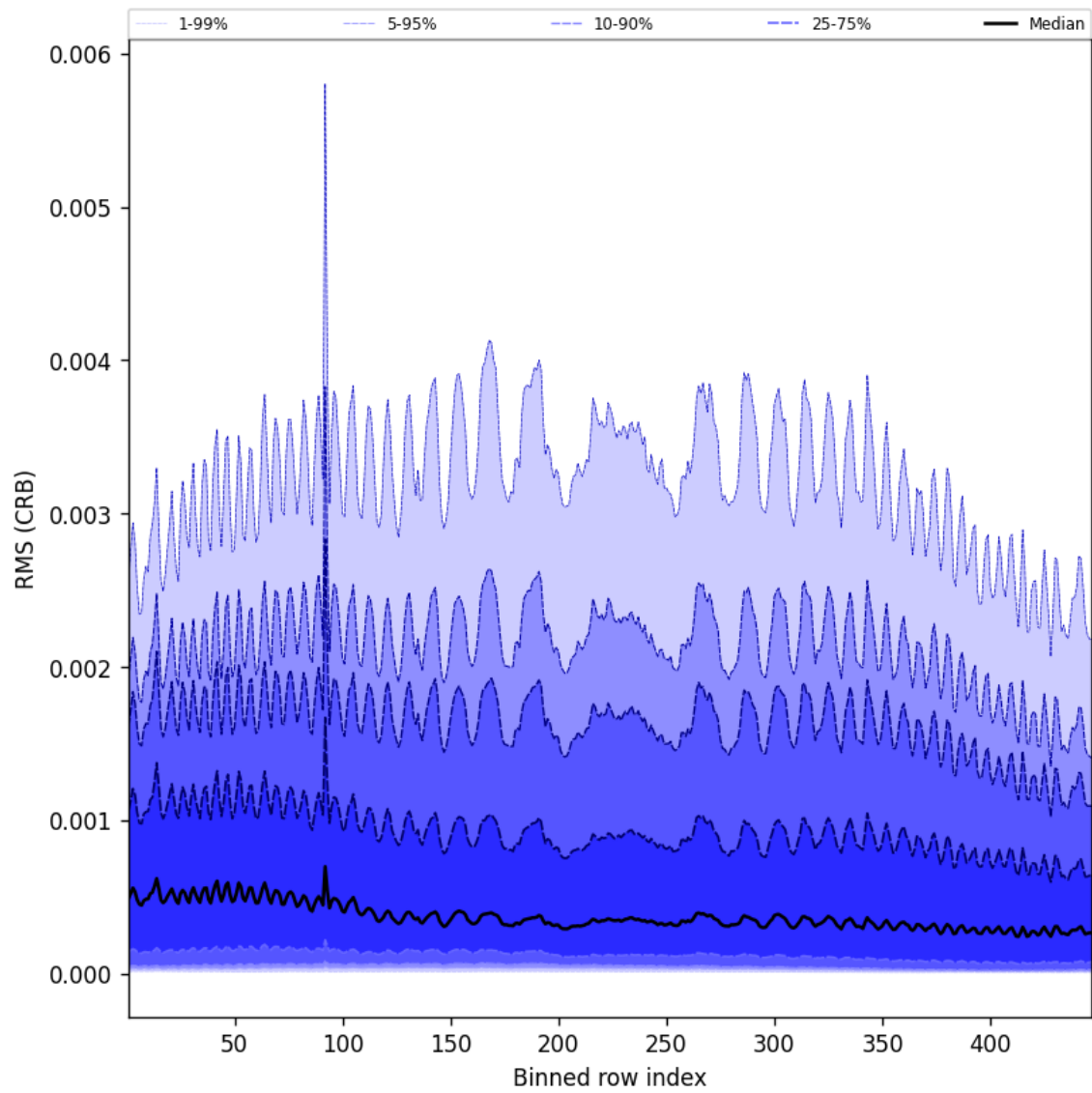
Figure 64: Along track statistics of “RMS (CRB)” for 2025-02-14 to 2025-02-16
