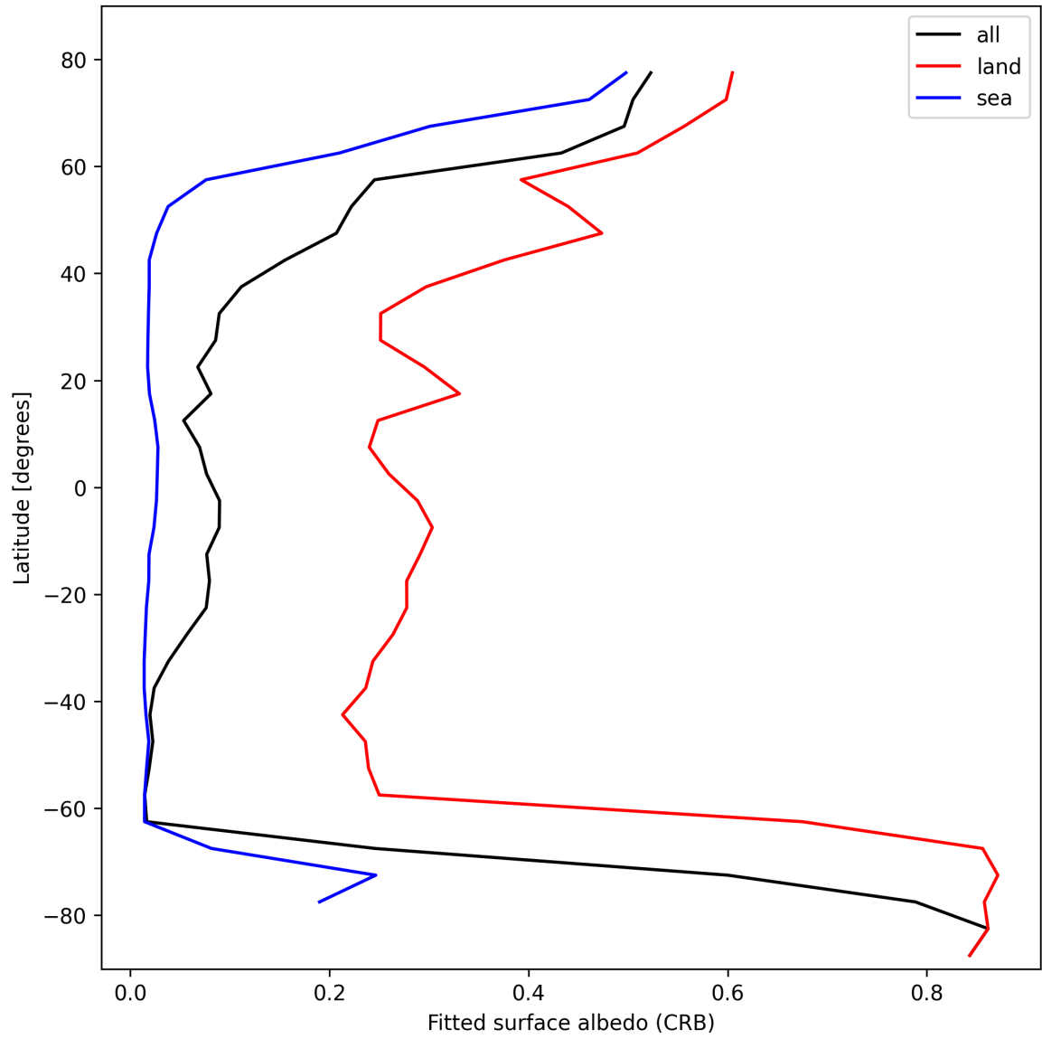
Figure 30: Zonal average of “Fitted surface albedo (CRB)” for 2025-02-14 to 2025-02-16.
