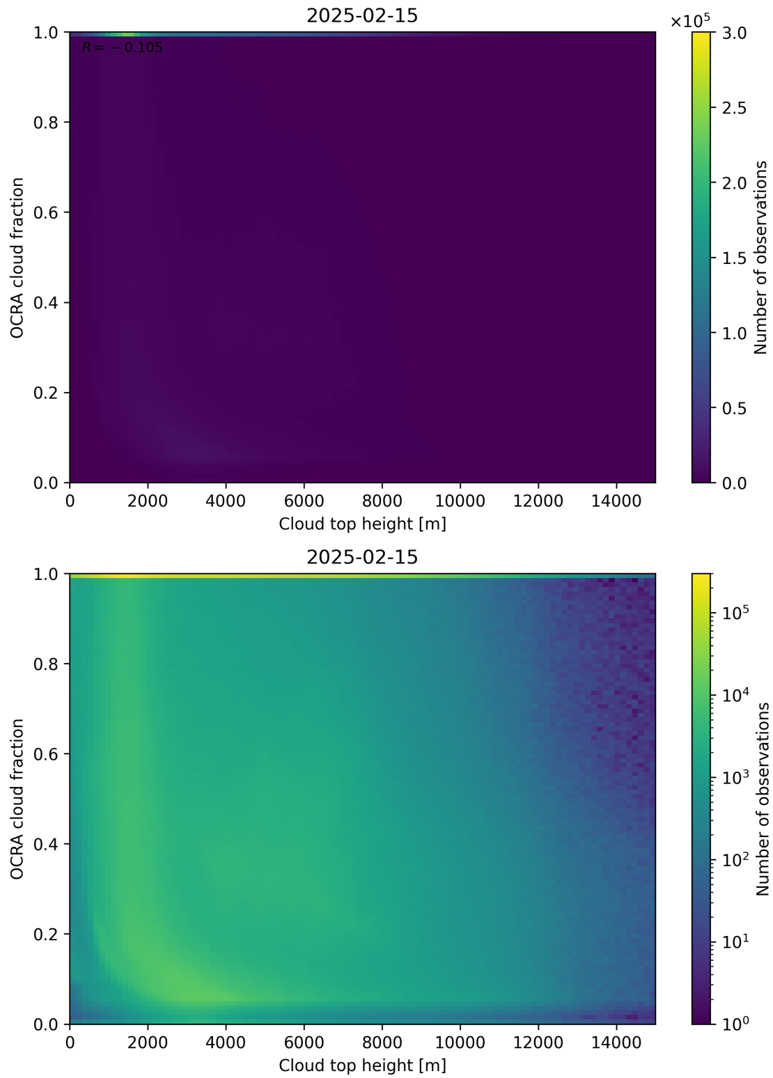
Figure 87: Scatter density plot of “Cloud top height” against “OCRA cloud fraction” for 2025-02-14 to 2025-02-16.
