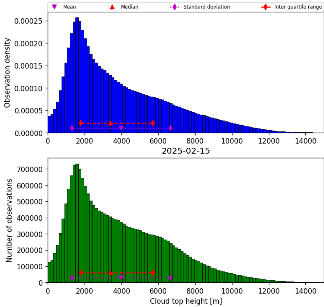
Figure 40: Histogram of “Cloud top height” for 2025-02-14 to 2025-02-16
