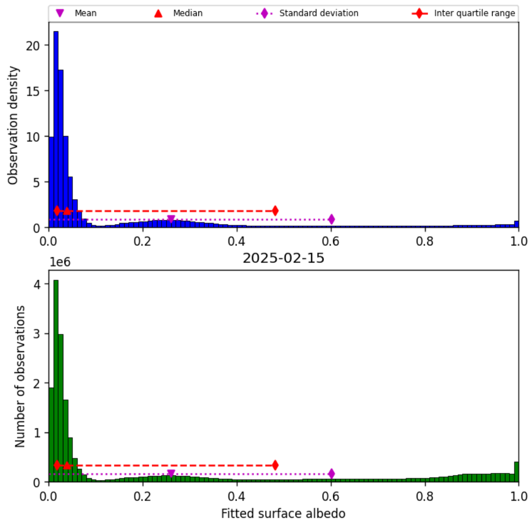
Figure 45: Histogram of “Fitted surface albedo” for 2025-02-14 to 2025-02-16
