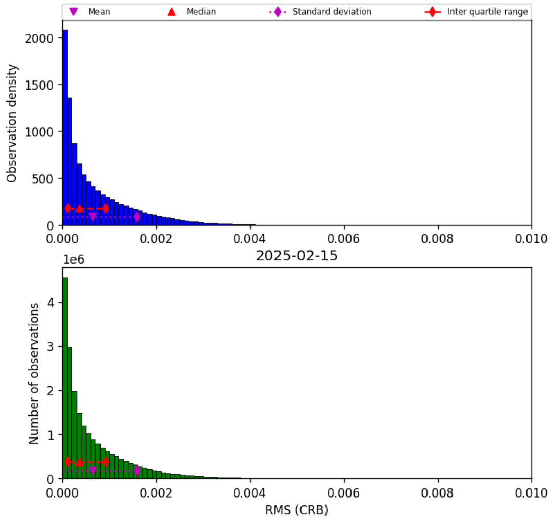
Figure 48: Histogram of “RMS (CRB)” for 2025-02-14 to 2025-02-16
