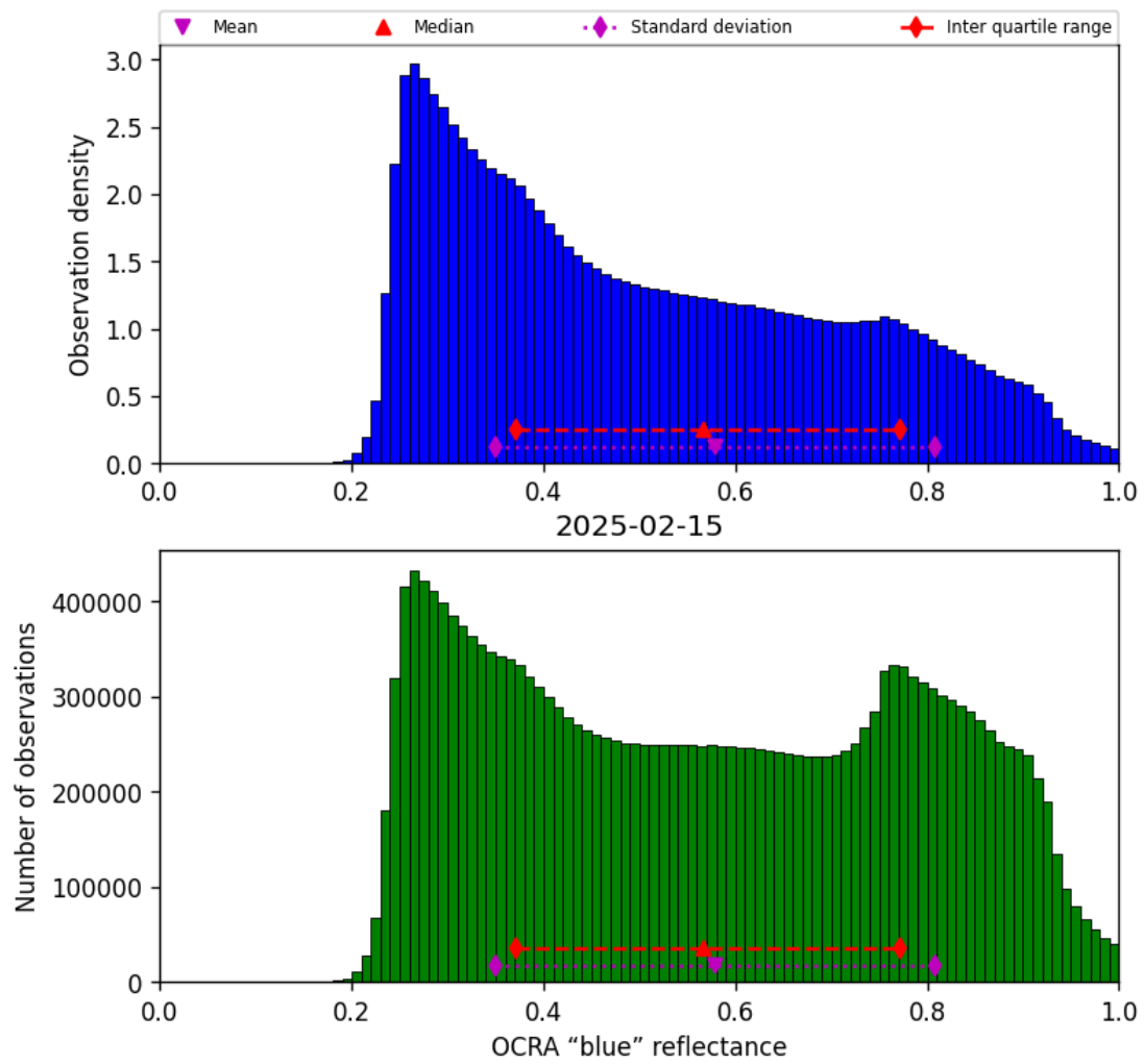
Figure 51: Histogram of “OCRA “blue” reflectance” for 2025-02-14 to 2025-02-16
