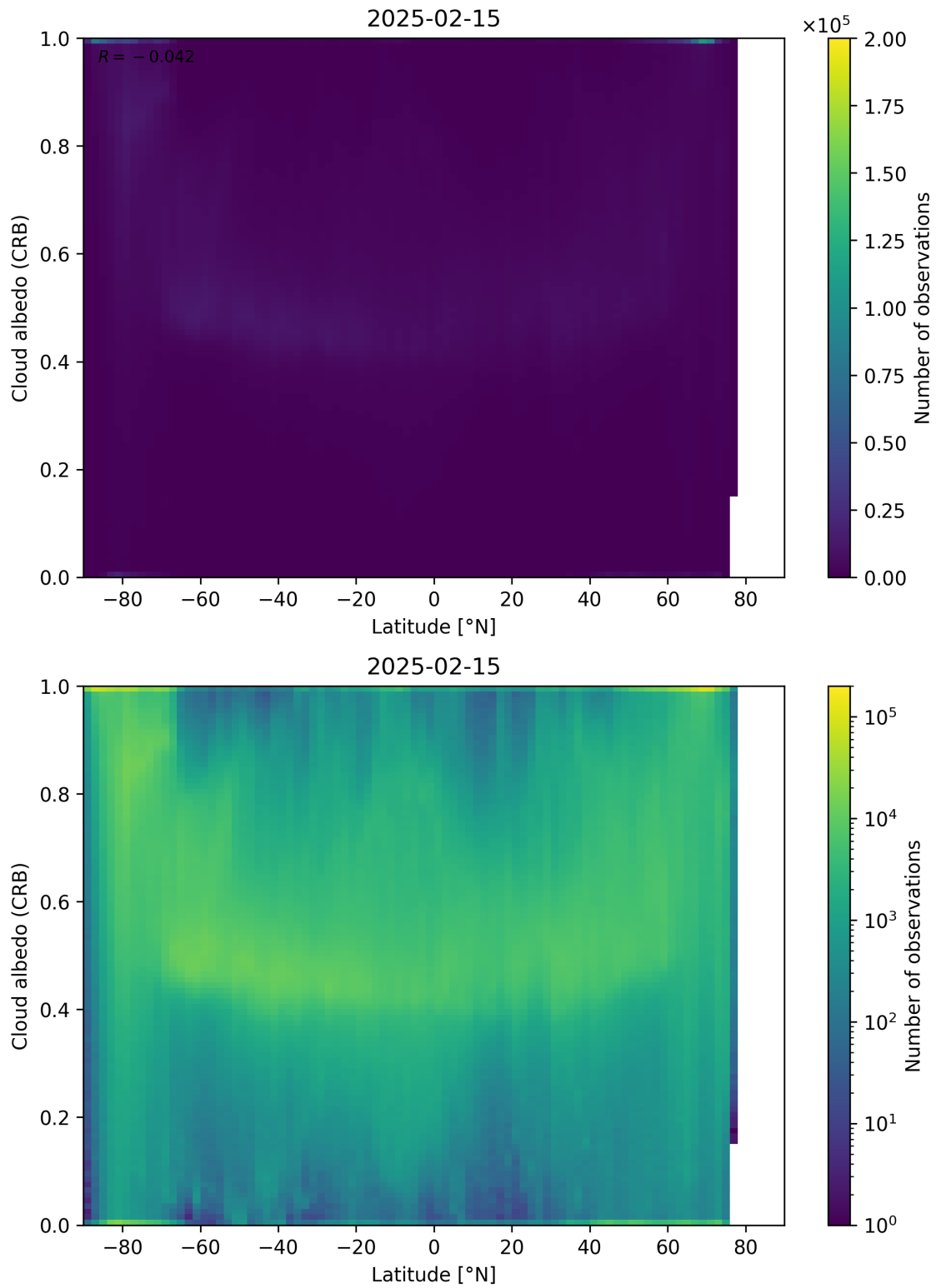
Figure 91: Scatter density plot of “Latitude” against “Cloud albedo (CRB)” for 2025-02-14 to 2025-02-16.
