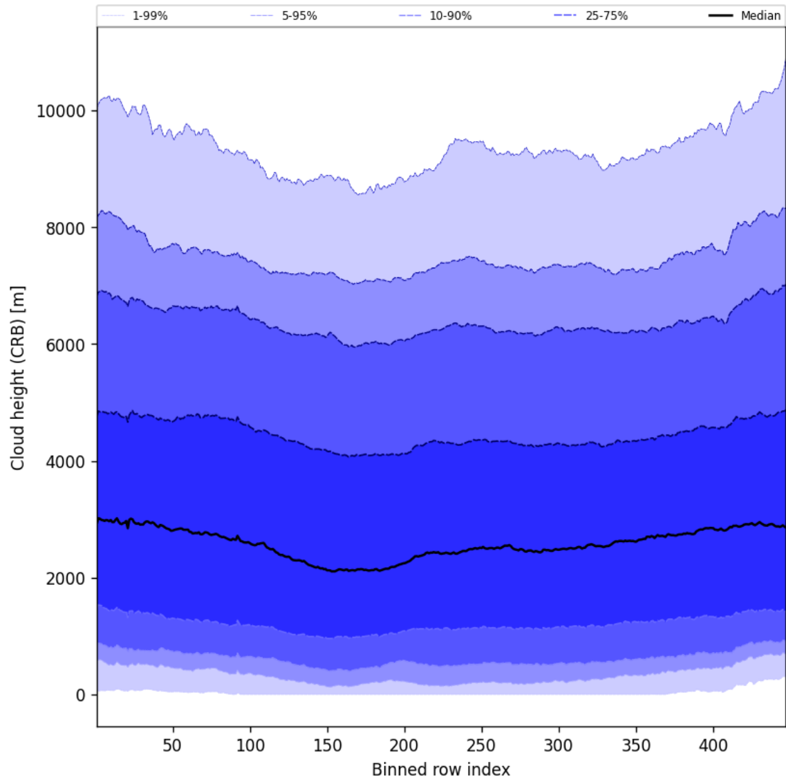
Figure 59: Along track statistics of “Cloud height (CRB)” for 2025-02-14 to 2025-02-16
