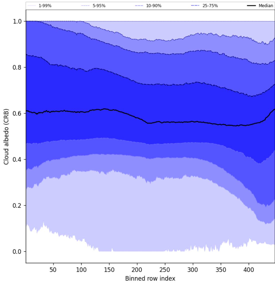
Figure 60: Along track statistics of “Cloud albedo (CRB)” for 2025-02-14 to 2025-02-16
