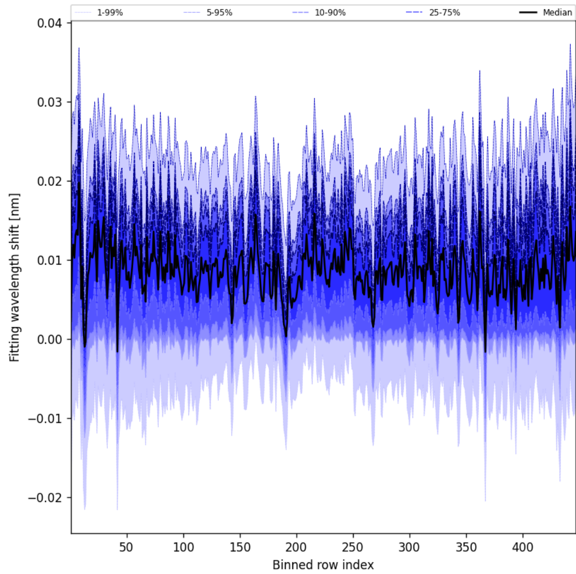
Figure 65: Along track statistics of “Fitting wavelength shift” for 2025-02-14 to 2025-02-16
