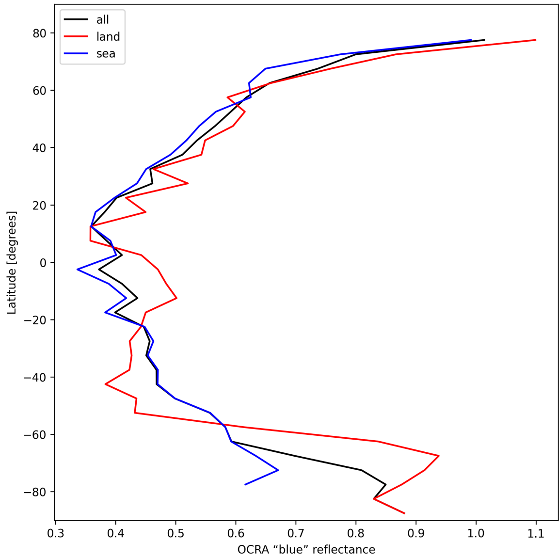
Figure 35: Zonal average of “OCRA “blue” reflectance” for 2025-02-14 to 2025-02-16.
