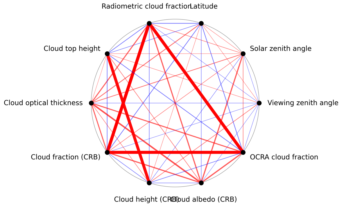
Figure 1: Map of correlation graph for 2025-02-14 to 2025-02-16.
