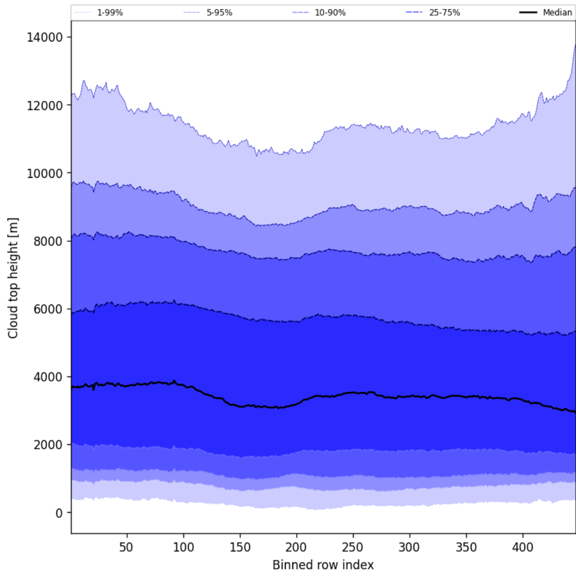
Figure 56: Along track statistics of “Cloud top height” for 2025-02-14 to 2025-02-16
