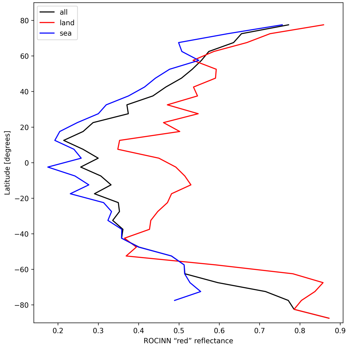
Figure 37: Zonal average of “ROCINN “red” reflectance” for 2025-02-14 to 2025-02-16.
