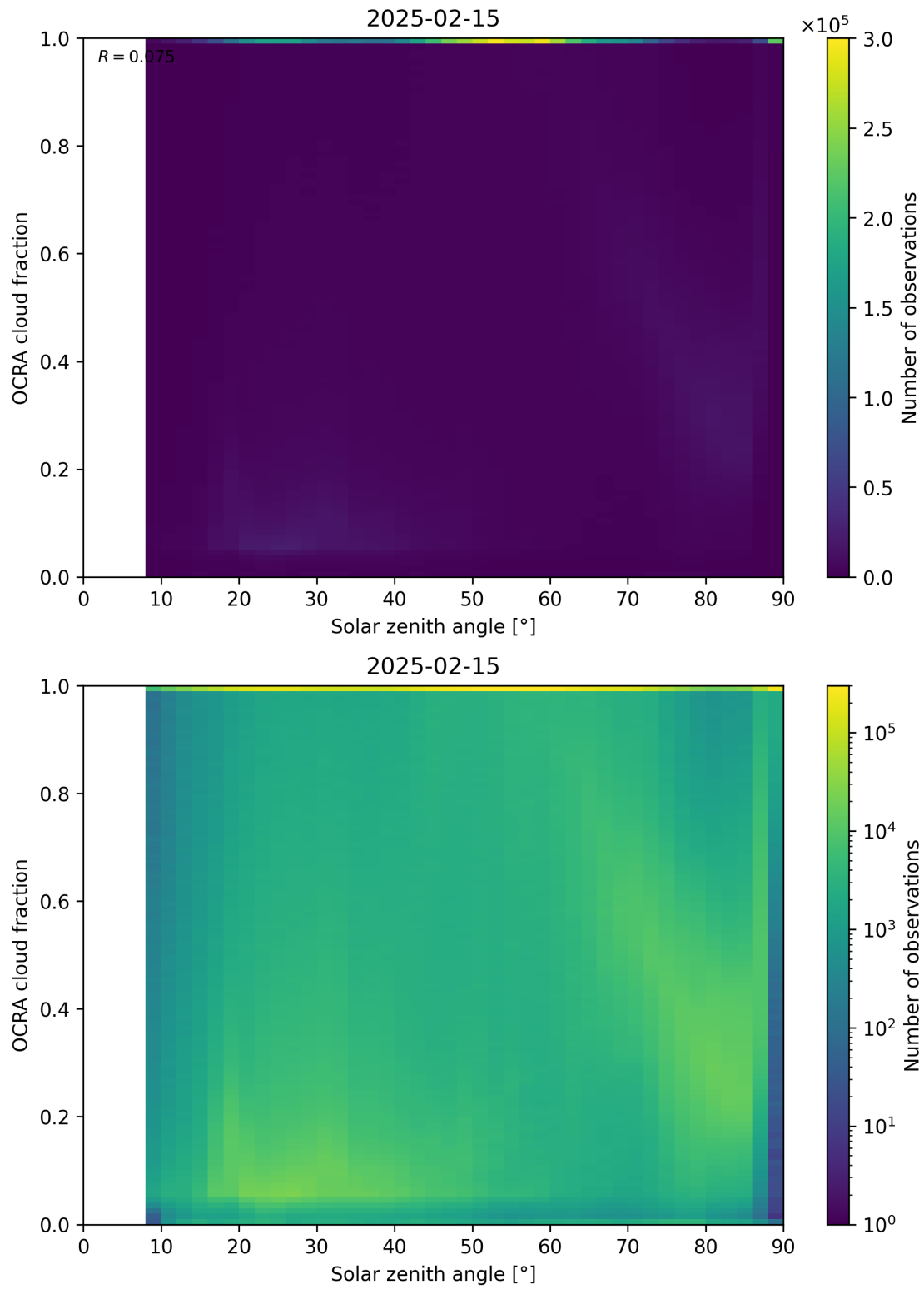
Figure 100: Scatter density plot of “Solar zenith angle” against “OCRA cloud fraction” for 2025-02-14 to 2025-02-16.
