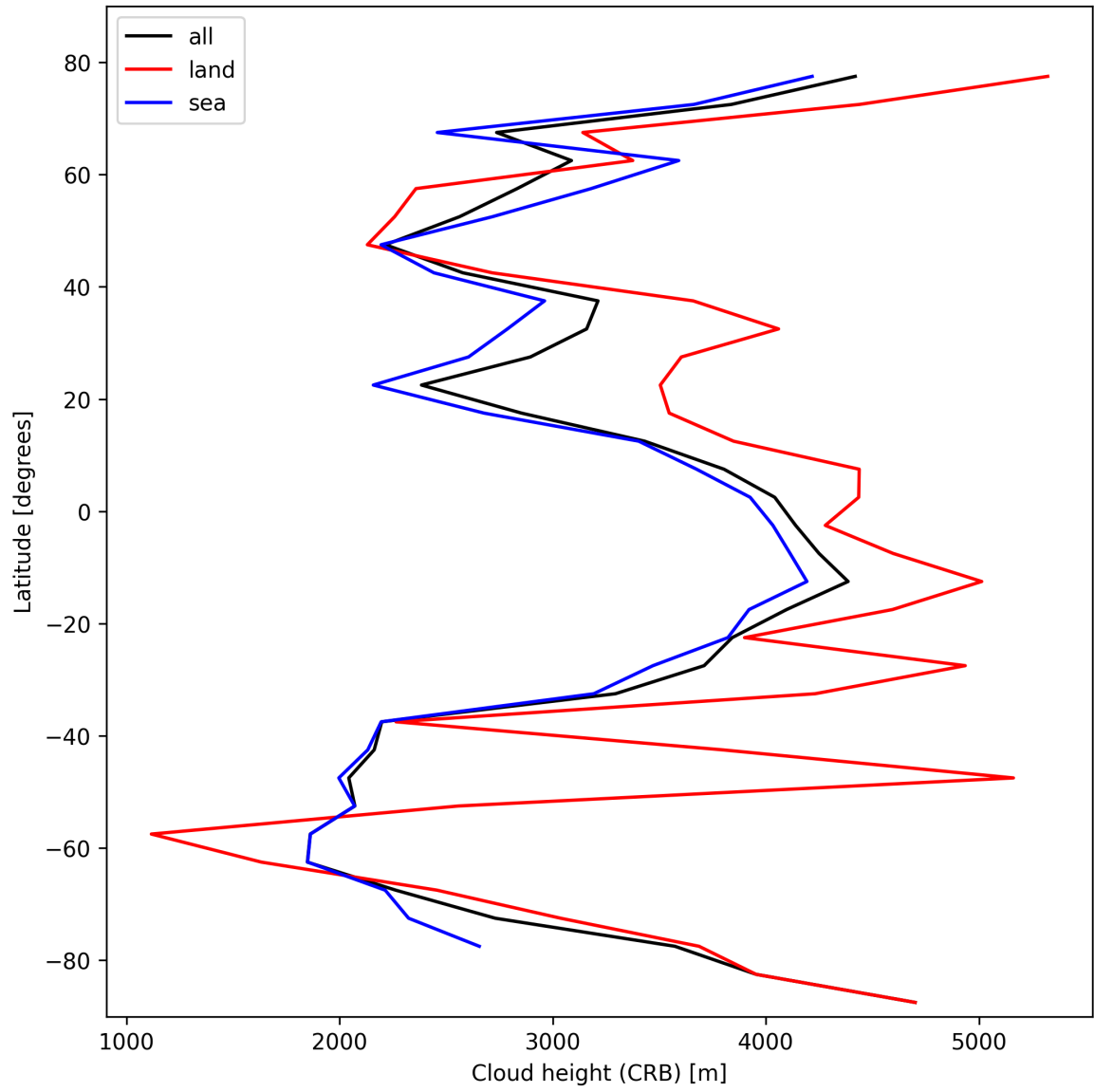
Figure 27: Zonal average of “Cloud height (CRB)” for 2025-02-14 to 2025-02-16.
