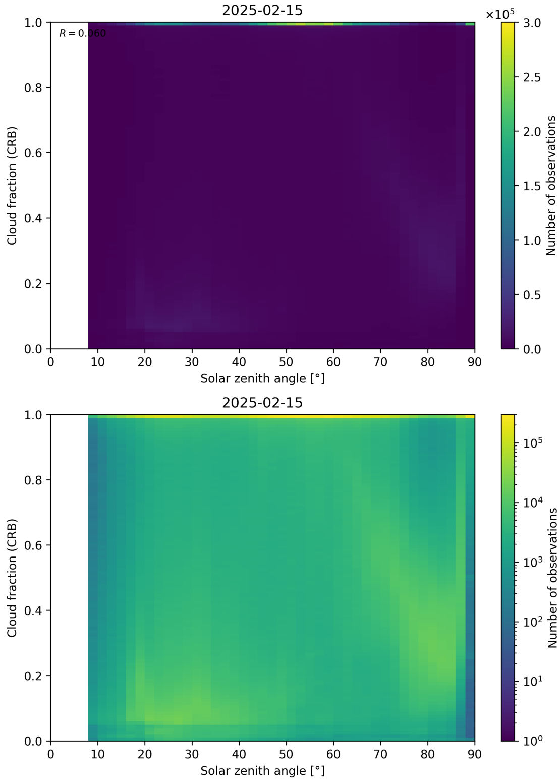
Figure 101: Scatter density plot of “Solar zenith angle” against “Cloud fraction (CRB)” for 2025-02-14 to 2025-02-16.
