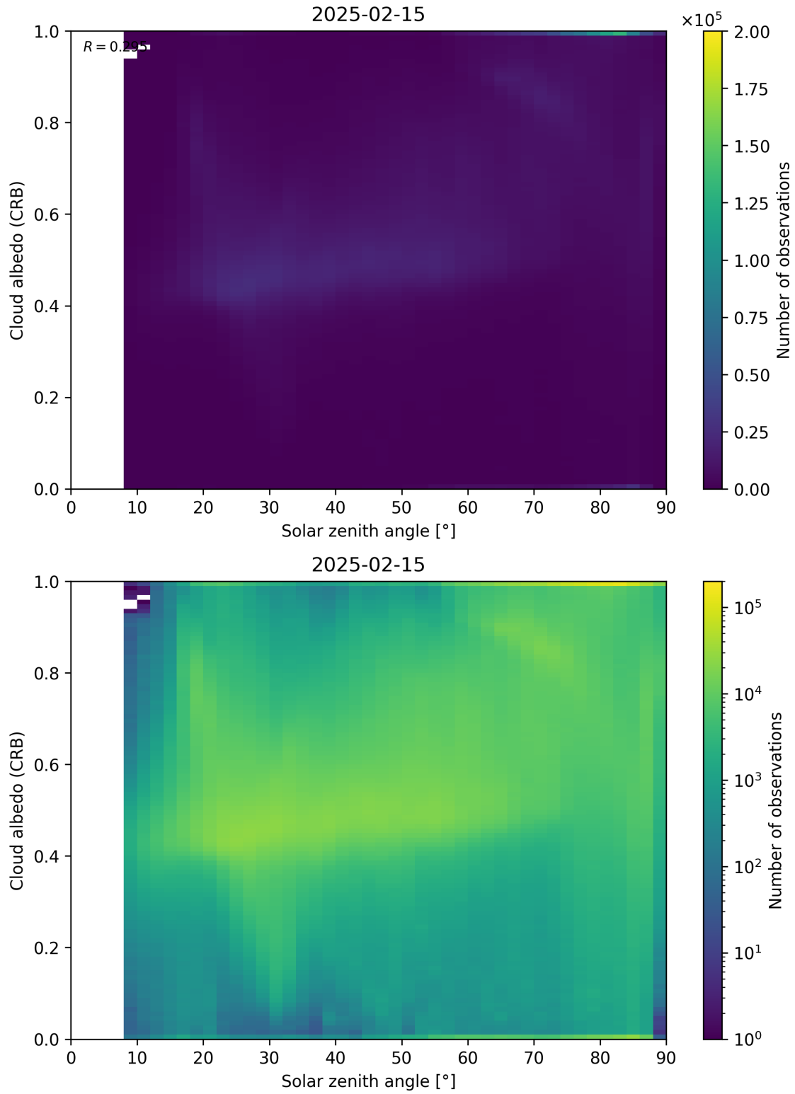
Figure 98: Scatter density plot of “Solar zenith angle” against “Cloud albedo (CRB)” for 2025-02-14 to 2025-02-16.
