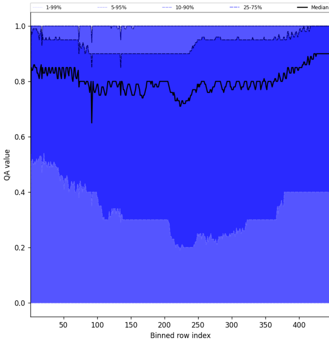
Figure 54: Along track statistics of “QA value” for 2025-02-14 to 2025-02-16
