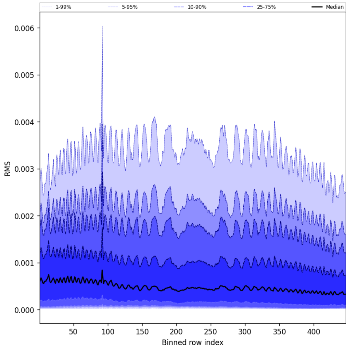
Figure 63: Along track statistics of “RMS” for 2025-02-14 to 2025-02-16
