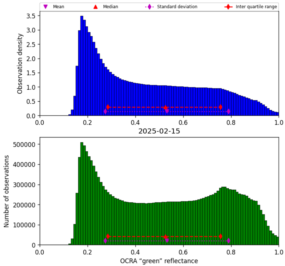
Figure 52: Histogram of “OCRA “green” reflectance” for 2025-02-14 to 2025-02-16
