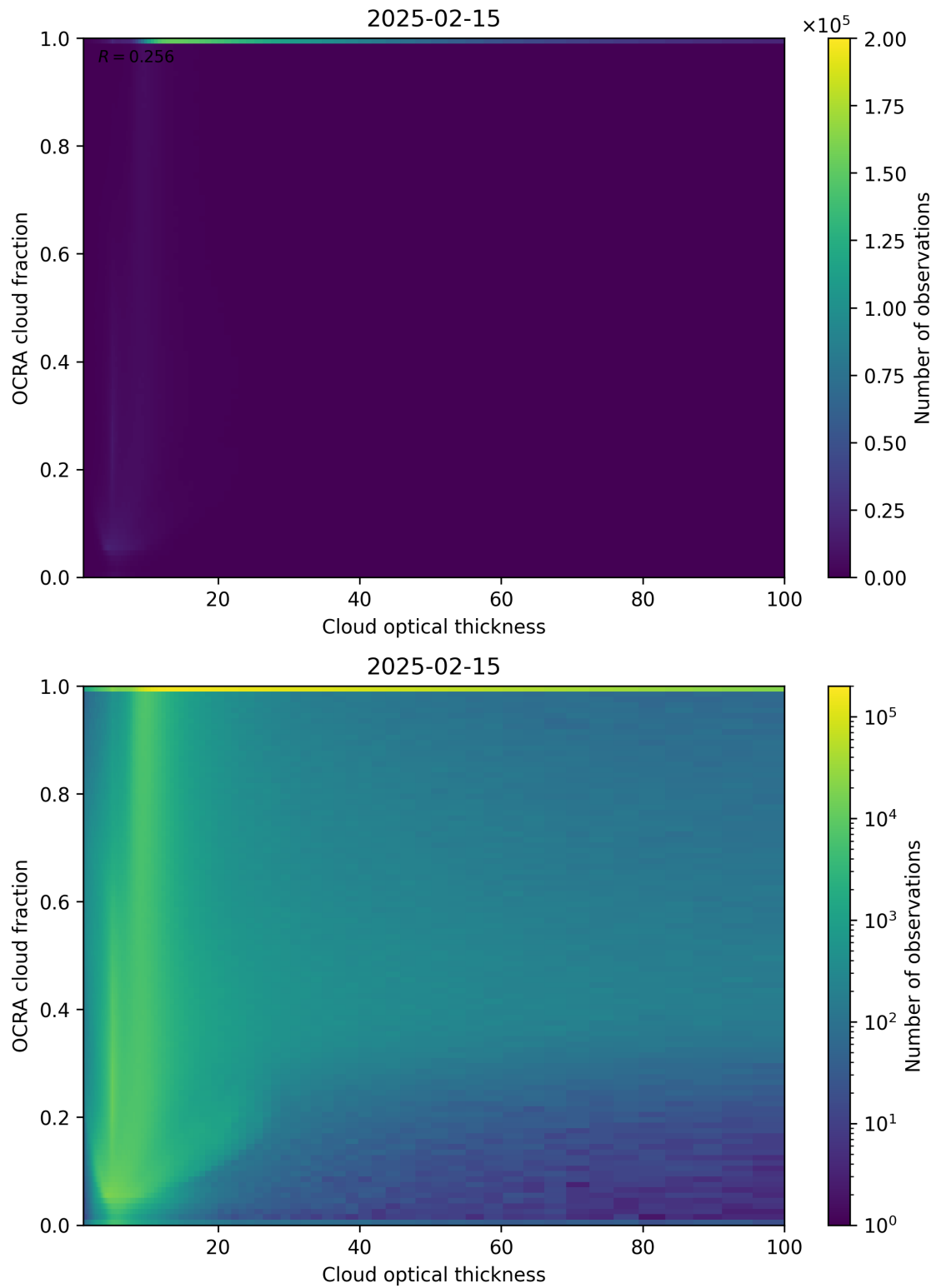
Figure 83: Scatter density plot of “Cloud optical thickness” against “OCRA cloud fraction” for 2025-02-14 to 2025-02-16.
