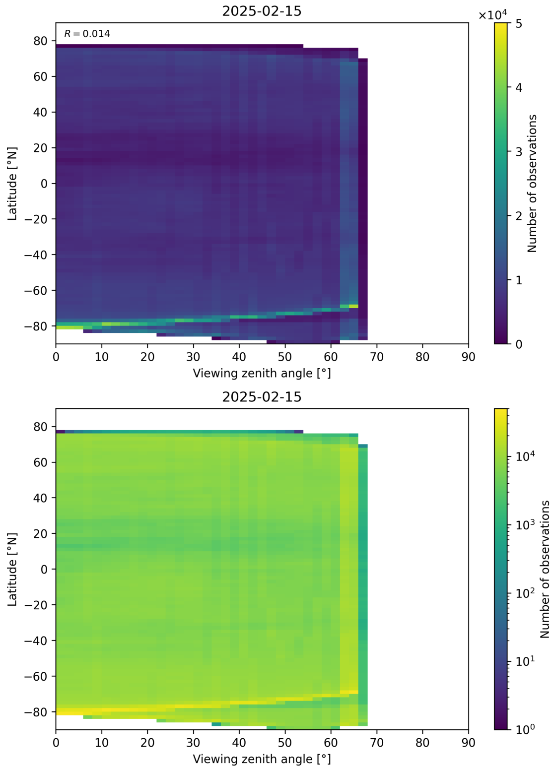
Figure 113: Scatter density plot of “Viewing zenith angle” against “Latitude” for 2025-02-14 to 2025-02-16.
