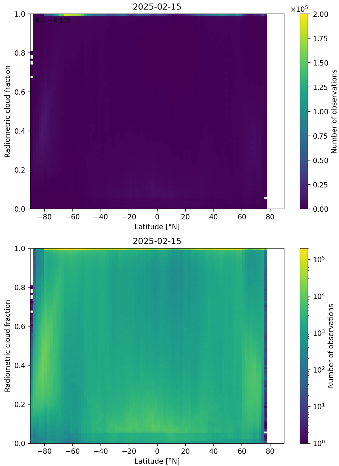
Figure 92: Scatter density plot of “Latitude” against “Radiometric cloud fraction” for 2025-02-14 to 2025-02-16.
