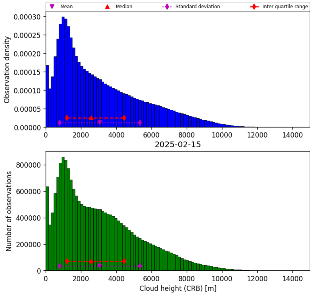
Figure 43: Histogram of “Cloud height (CRB)” for 2025-02-14 to 2025-02-16
