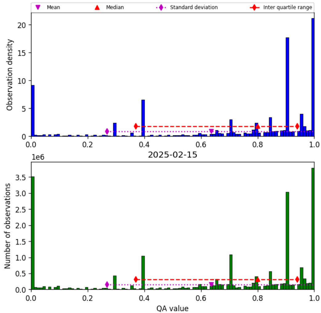
Figure 38: Histogram of “QA value” for 2025-02-14 to 2025-02-16
