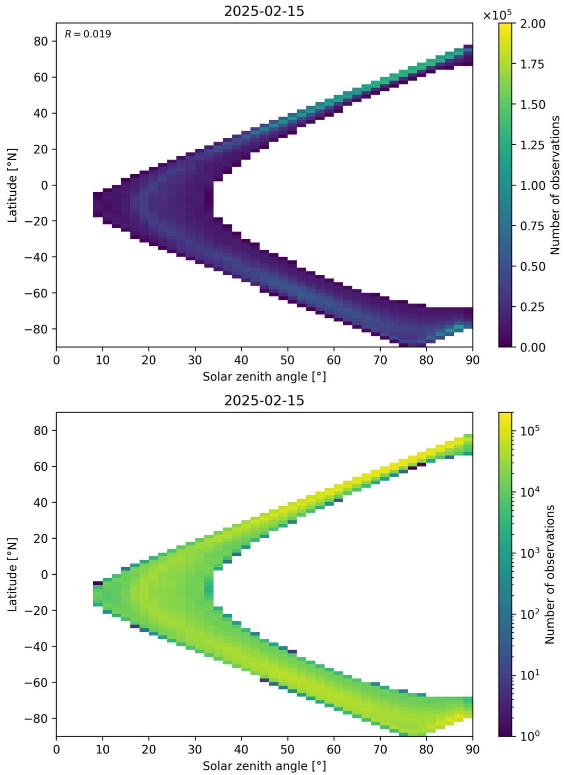
Figure 105: Scatter density plot of “Solar zenith angle” against “Latitude” for 2025-02-14 to 2025-02-16.
