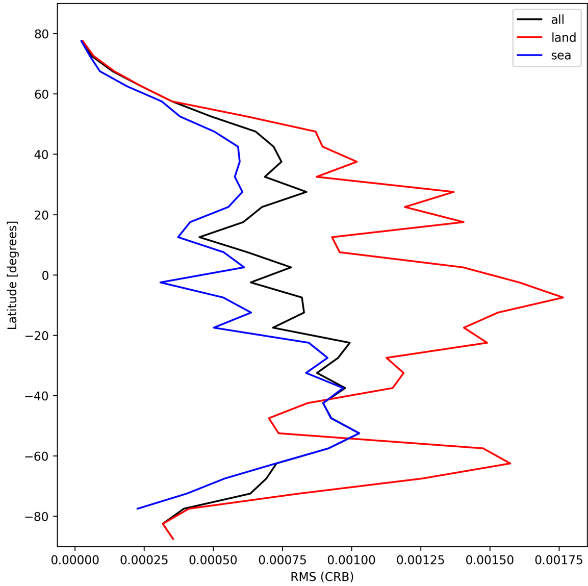
Figure 32: Zonal average of “RMS (CRB)” for 2025-02-14 to 2025-02-16.
