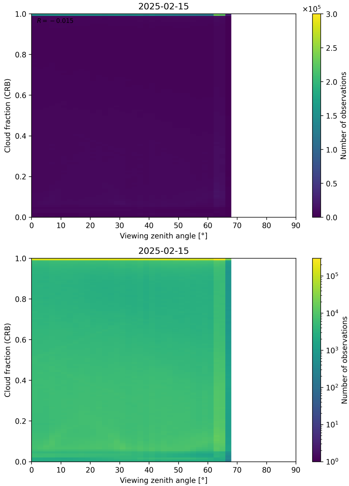
Figure 109: Scatter density plot of “Viewing zenith angle” against “Cloud fraction (CRB)” for 2025-02-14 to 2025-02-16.
