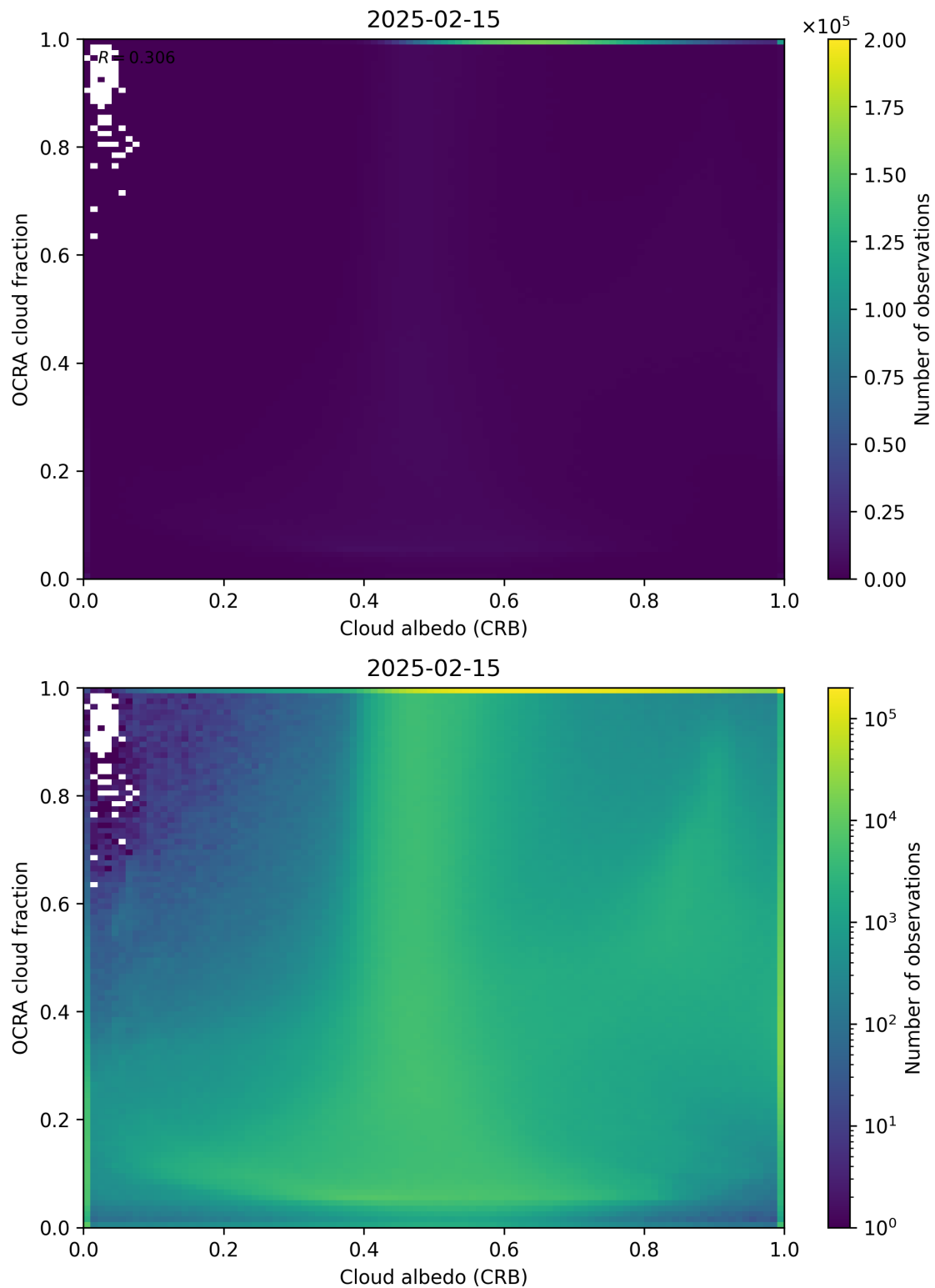
Figure 70: Scatter density plot of “Cloud albedo (CRB)” against “OCRA cloud fraction” for 2025-02-14 to 2025-02-16.
