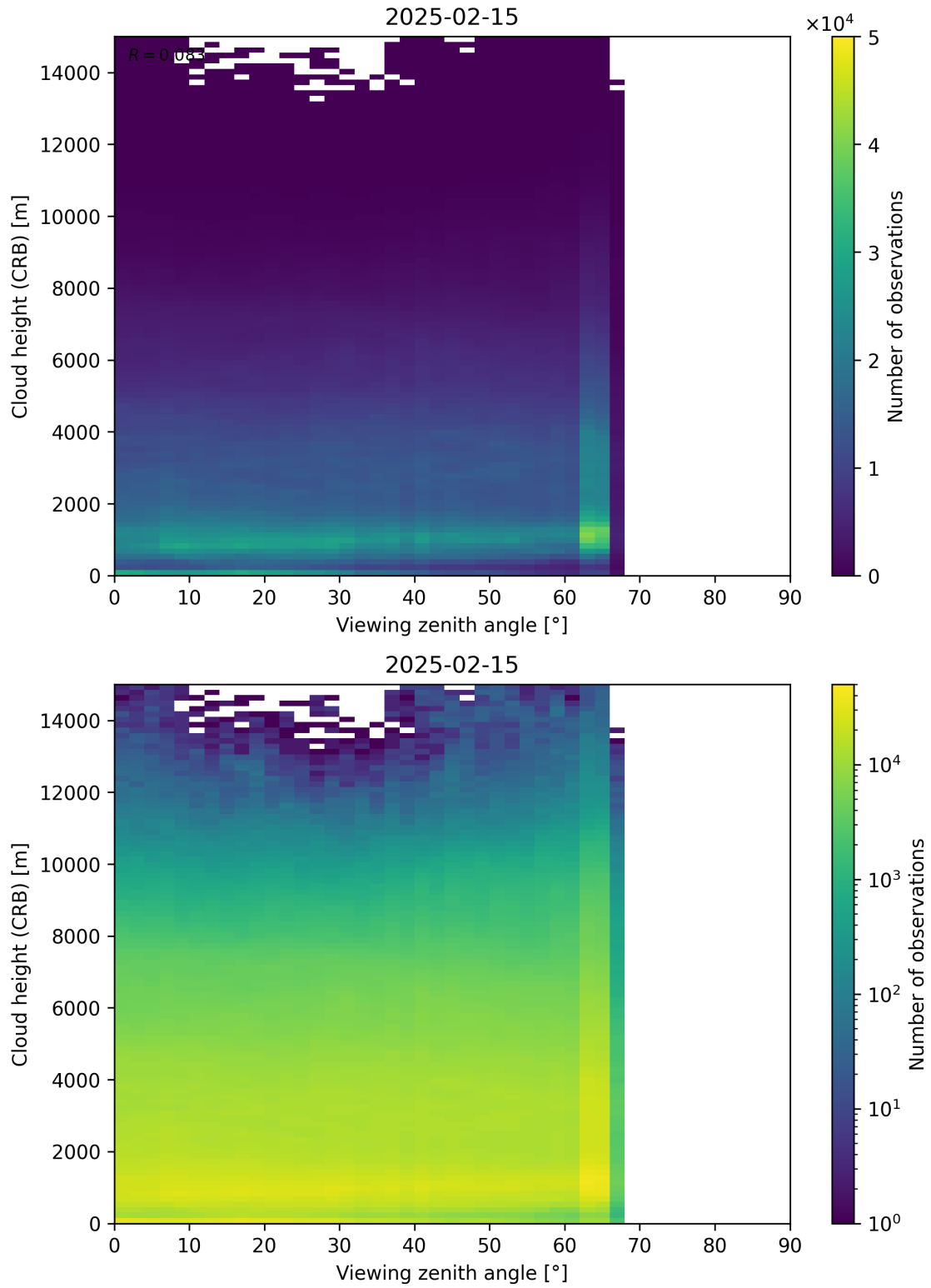
Figure 110: Scatter density plot of “Viewing zenith angle” against “Cloud height (CRB)” for 2025-02-14 to 2025-02-16.
