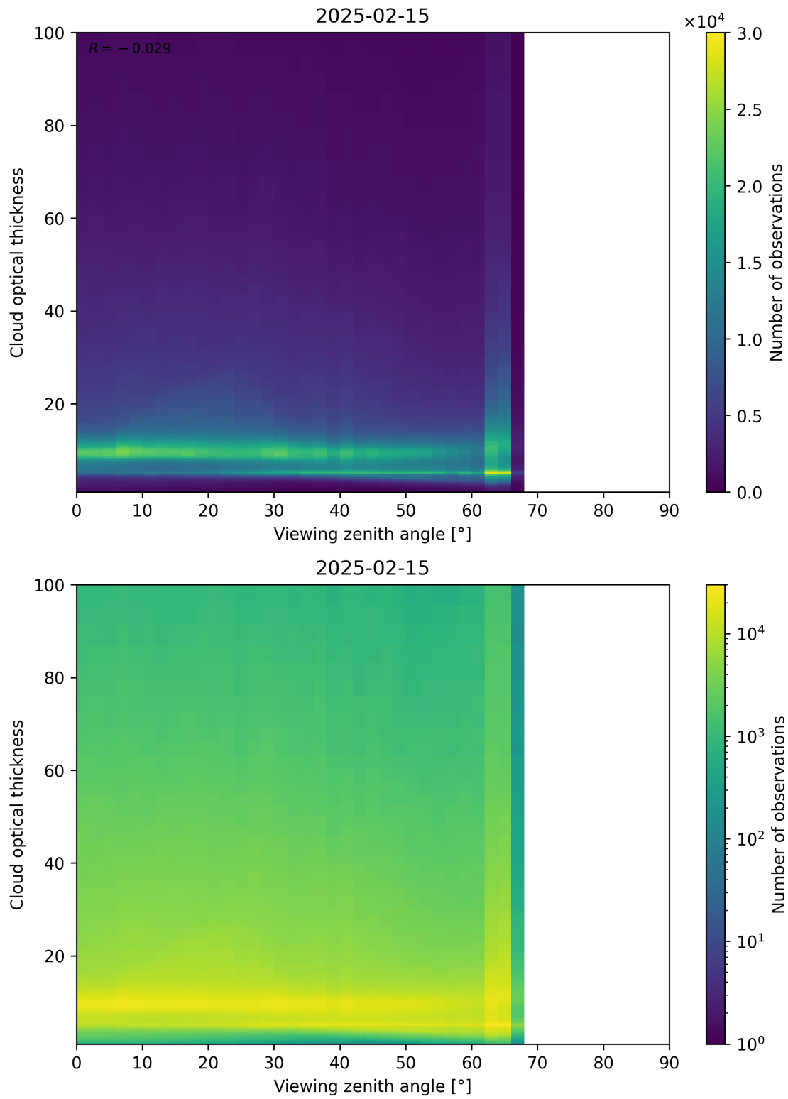
Figure 111: Scatter density plot of “Viewing zenith angle” against “Cloud optical thickness” for 2025-02-14 to 2025-02-16.
