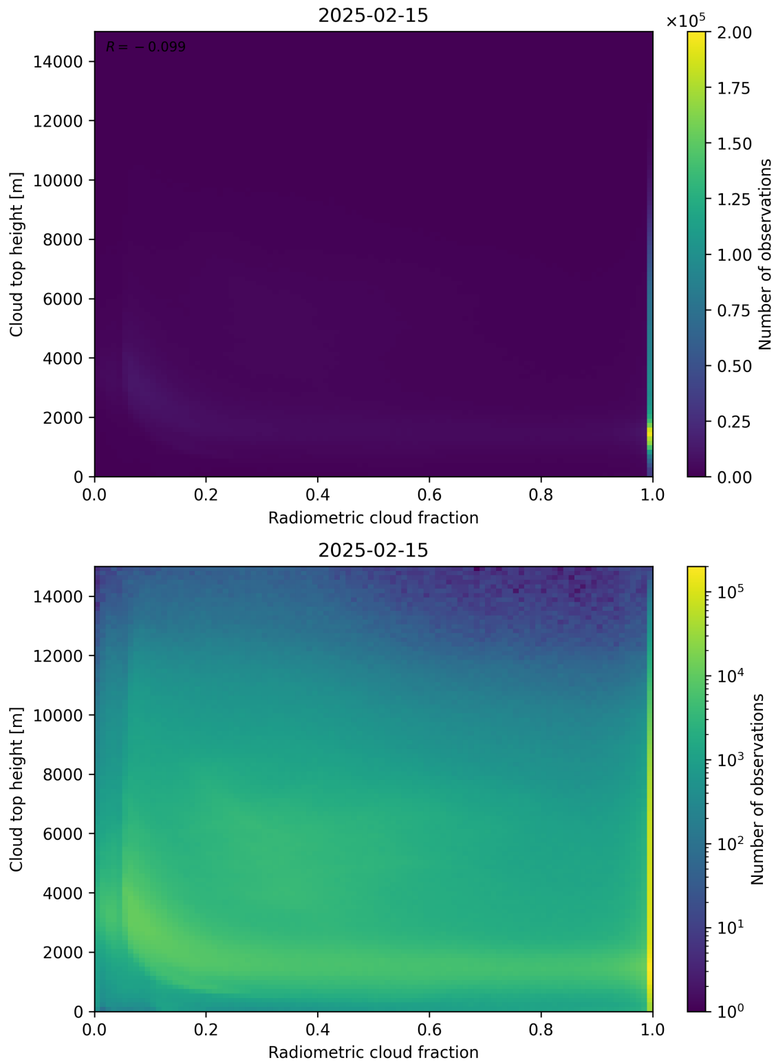
Figure 76: Scatter density plot of “Radiometric cloud fraction” against “Cloud top height” for 2025-02-14 to 2025-02-16.
