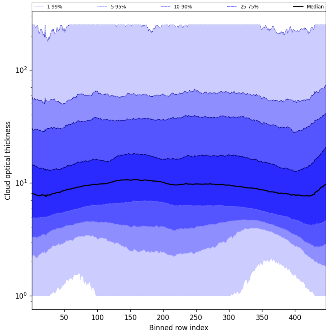
Figure 57: Along track statistics of “Cloud optical thickness” for 2025-02-14 to 2025-02-16
