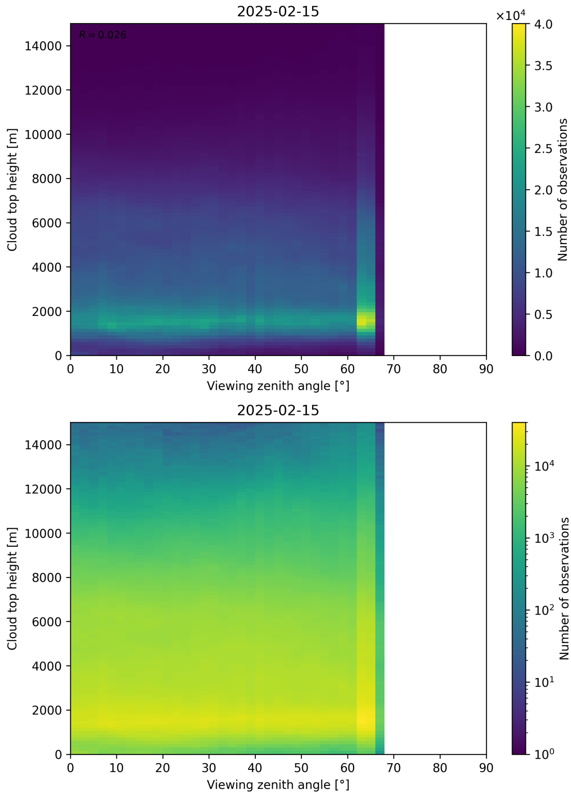
Figure 112: Scatter density plot of “Viewing zenith angle” against “Cloud top height” for 2025-02-14 to 2025-02-16.
