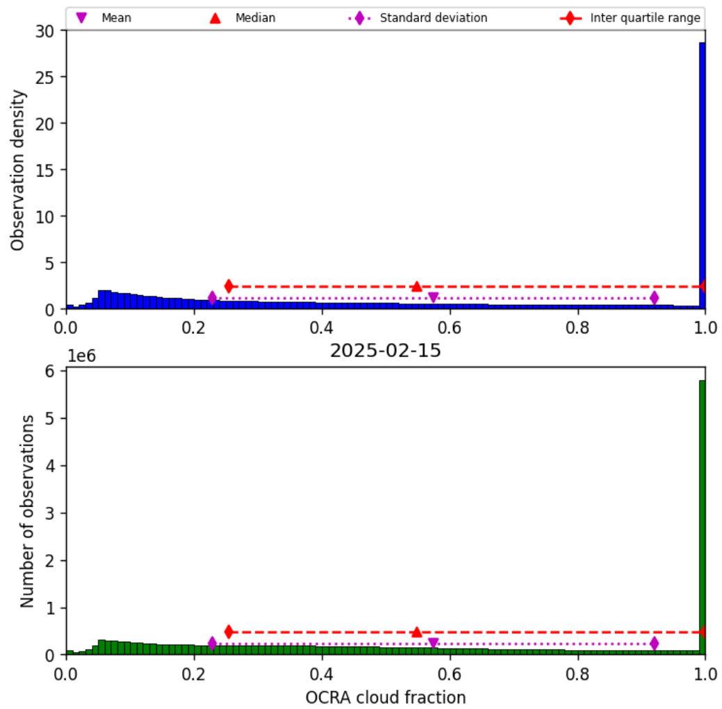
Figure 50: Histogram of “OCRA cloud fraction” for 2025-02-14 to 2025-02-16
