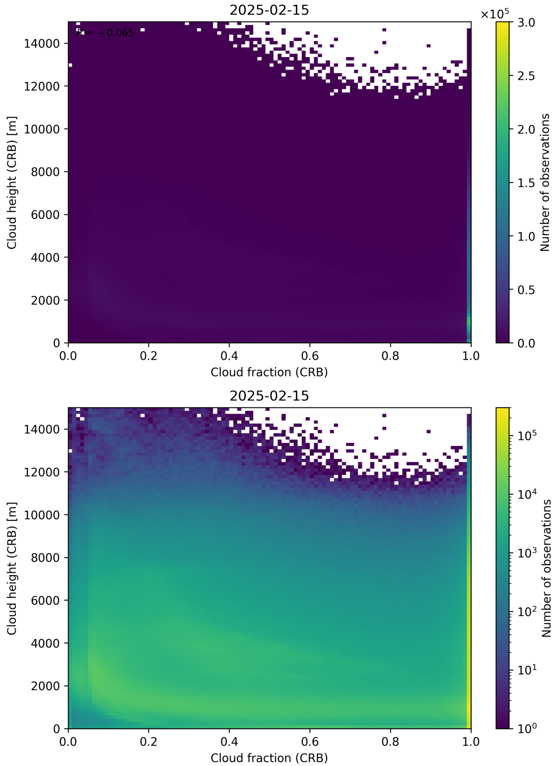
Figure 79: Scatter density plot of “Cloud fraction (CRB)” against “Cloud height (CRB)” for 2025-02-14 to 2025-02-16.
