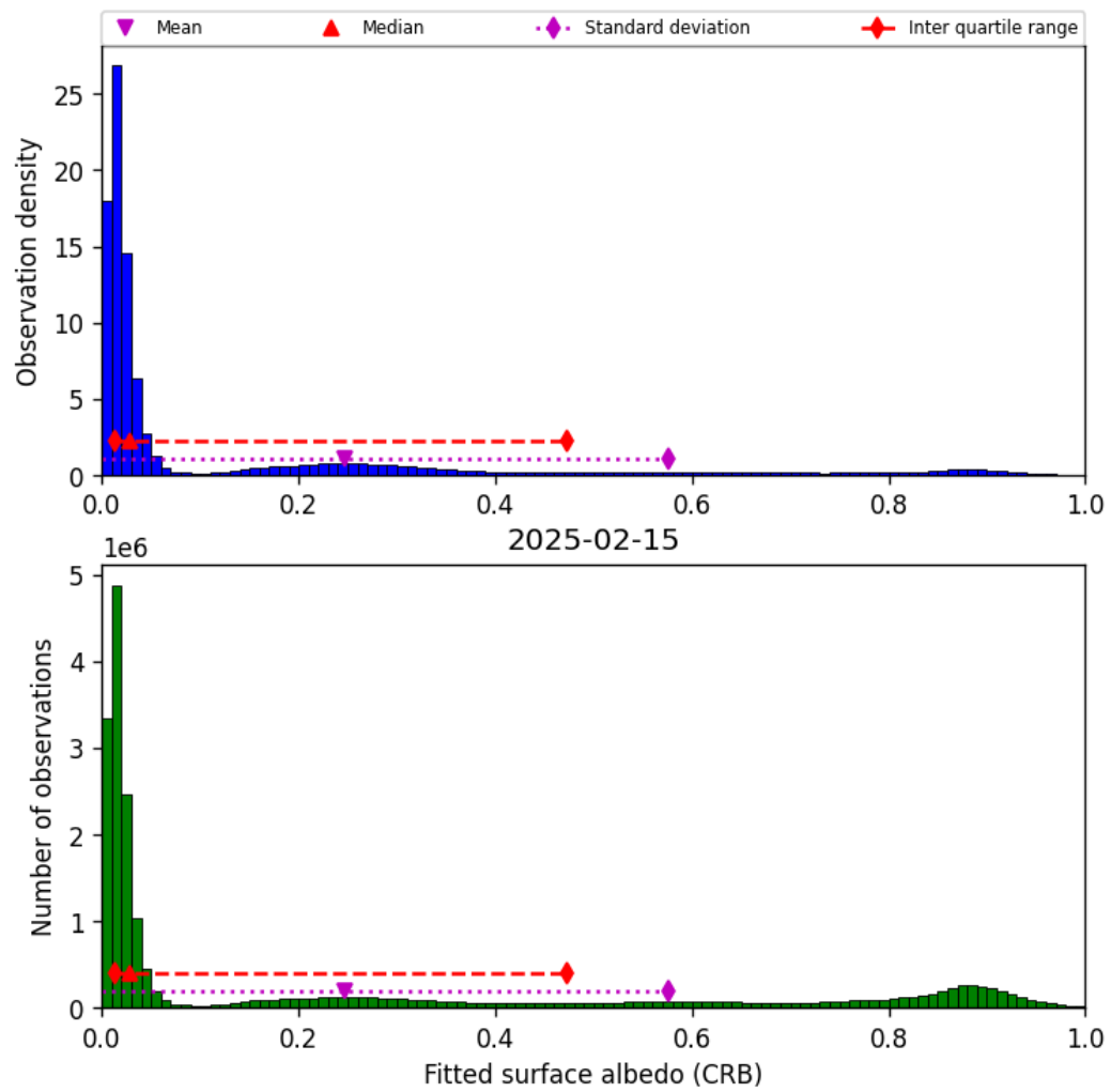
Figure 46: Histogram of “Fitted surface albedo (CRB)” for 2025-02-14 to 2025-02-16
