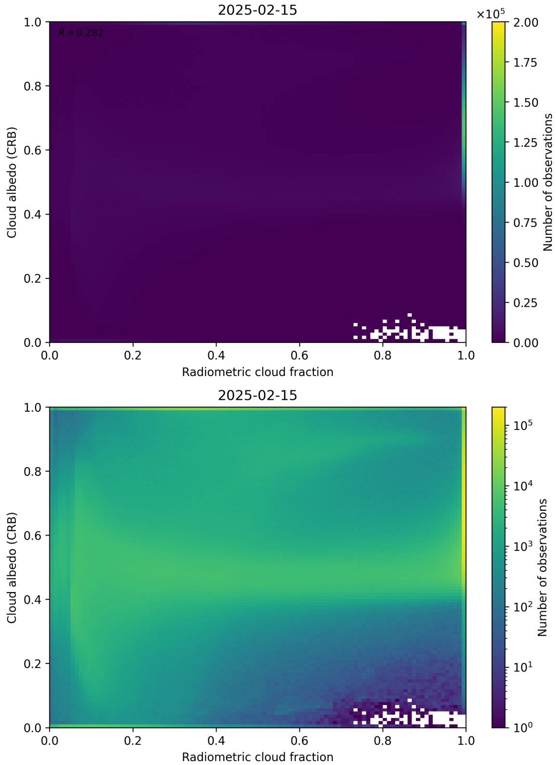
Figure 71: Scatter density plot of “Radiometric cloud fraction” against “Cloud albedo (CRB)” for 2025-02-14 to 2025-02-16.
