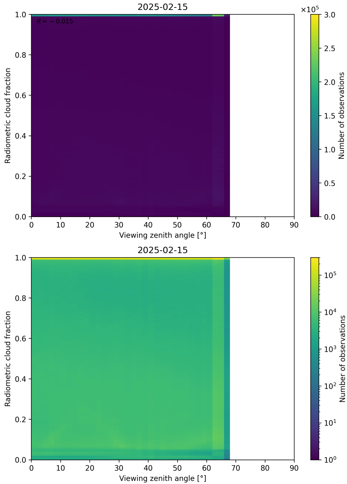
Figure 107: Scatter density plot of “Viewing zenith angle” against “Radiometric cloud fraction” for 2025-02-14 to 2025-02-16.
