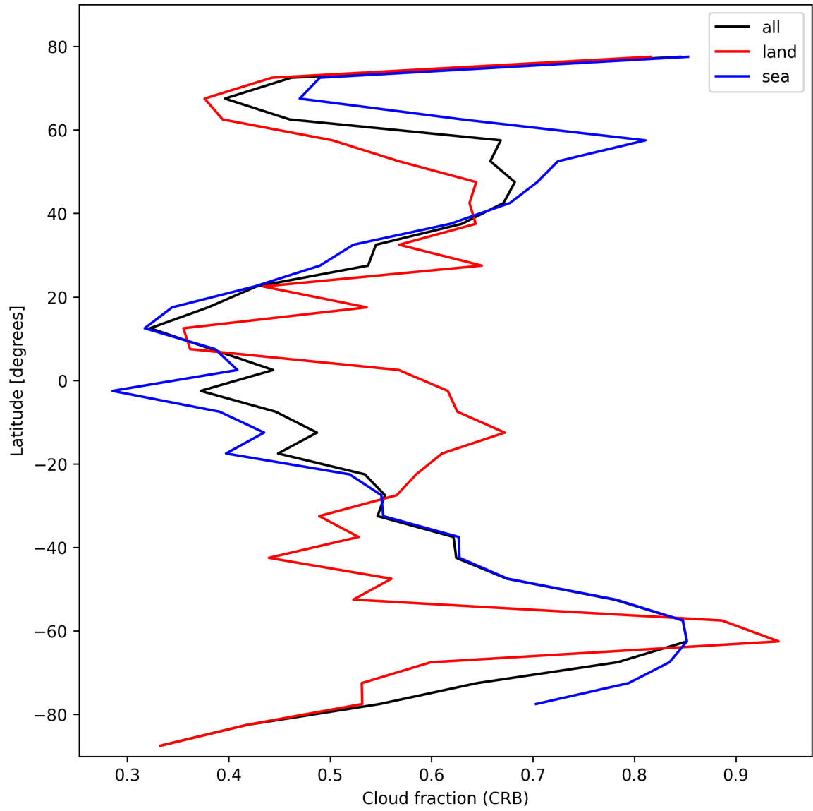
Figure 26: Zonal average of “Cloud fraction (CRB)” for 2025-02-14 to 2025-02-16.
