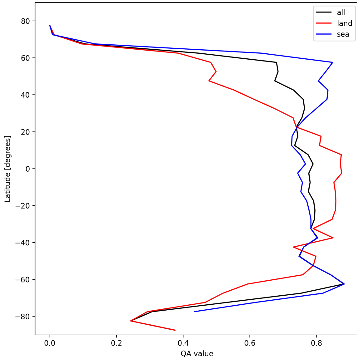
Figure 22: Zonal average of “QA value” for 2025-02-14 to 2025-02-16.
