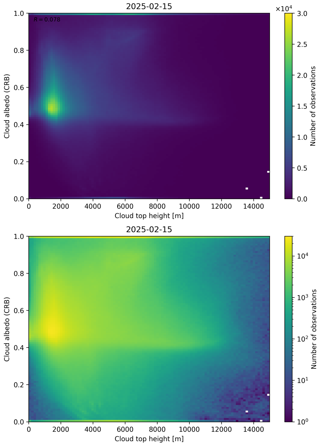
Figure 86: Scatter density plot of “Cloud top height” against “Cloud albedo (CRB)” for 2025-02-14 to 2025-02-16.
