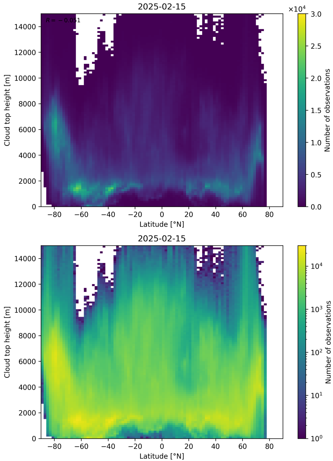
Figure 97: Scatter density plot of “Latitude” against “Cloud top height” for 2025-02-14 to 2025-02-16.
