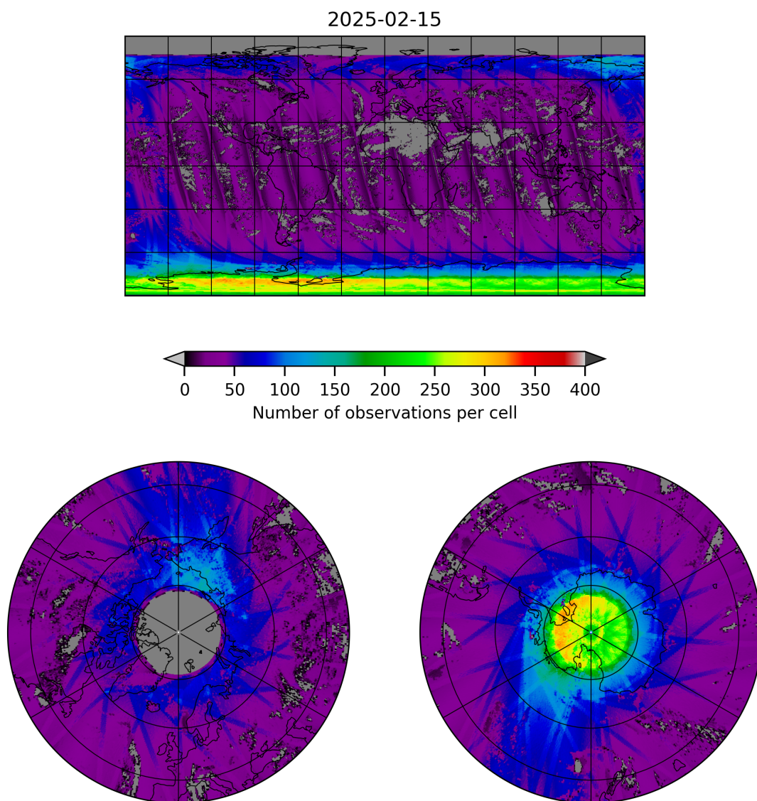
Figure 21: Map of the number of observations for 2025-02-14 to 2025-02-16
