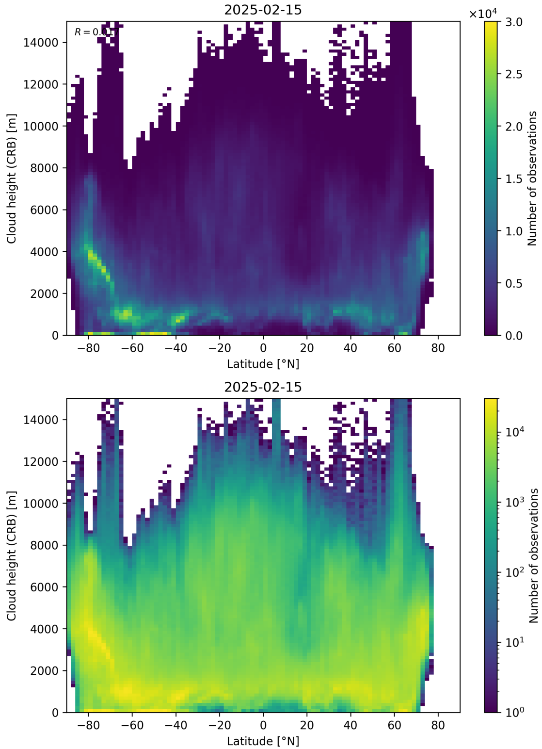
Figure 95: Scatter density plot of “Latitude” against “Cloud height (CRB)” for 2025-02-14 to 2025-02-16.
