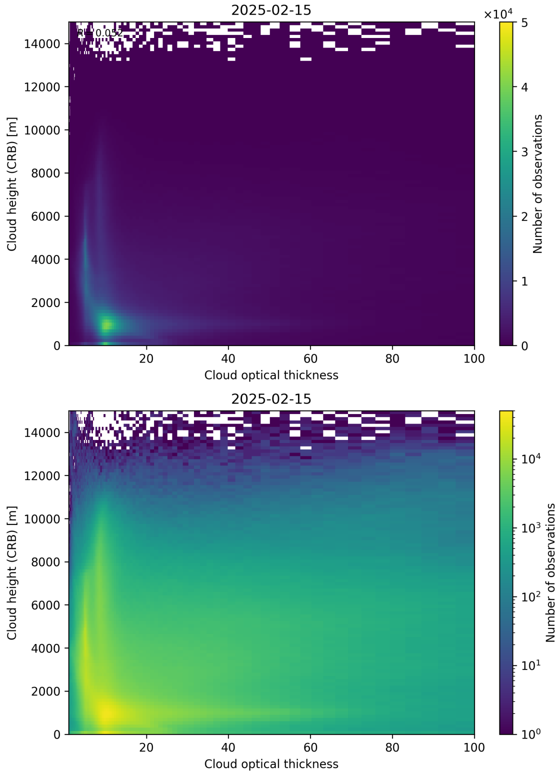
Figure 85: Scatter density plot of “Cloud optical thickness” against “Cloud height (CRB)” for 2025-02-14 to 2025-02-16.
