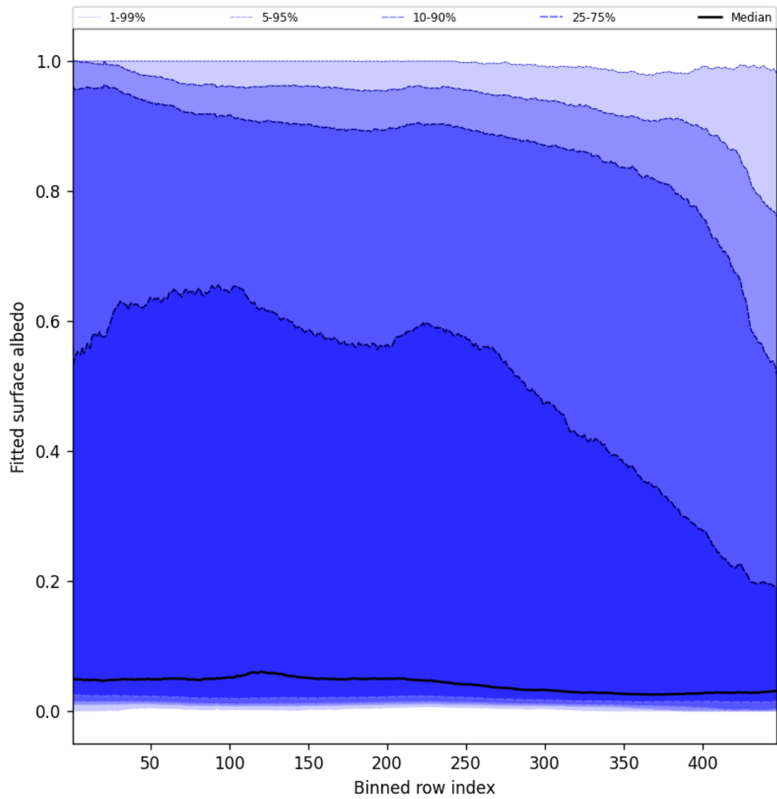
Figure 61: Along track statistics of “Fitted surface albedo” for 2025-02-14 to 2025-02-16
