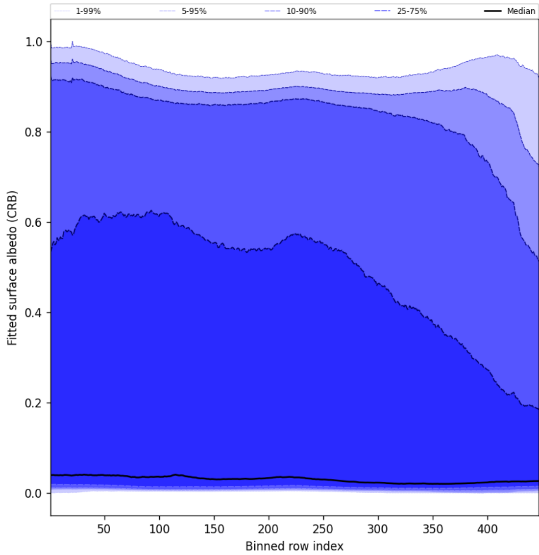
Figure 62: Along track statistics of “Fitted surface albedo (CRB)” for 2025-02-14 to 2025-02-16
