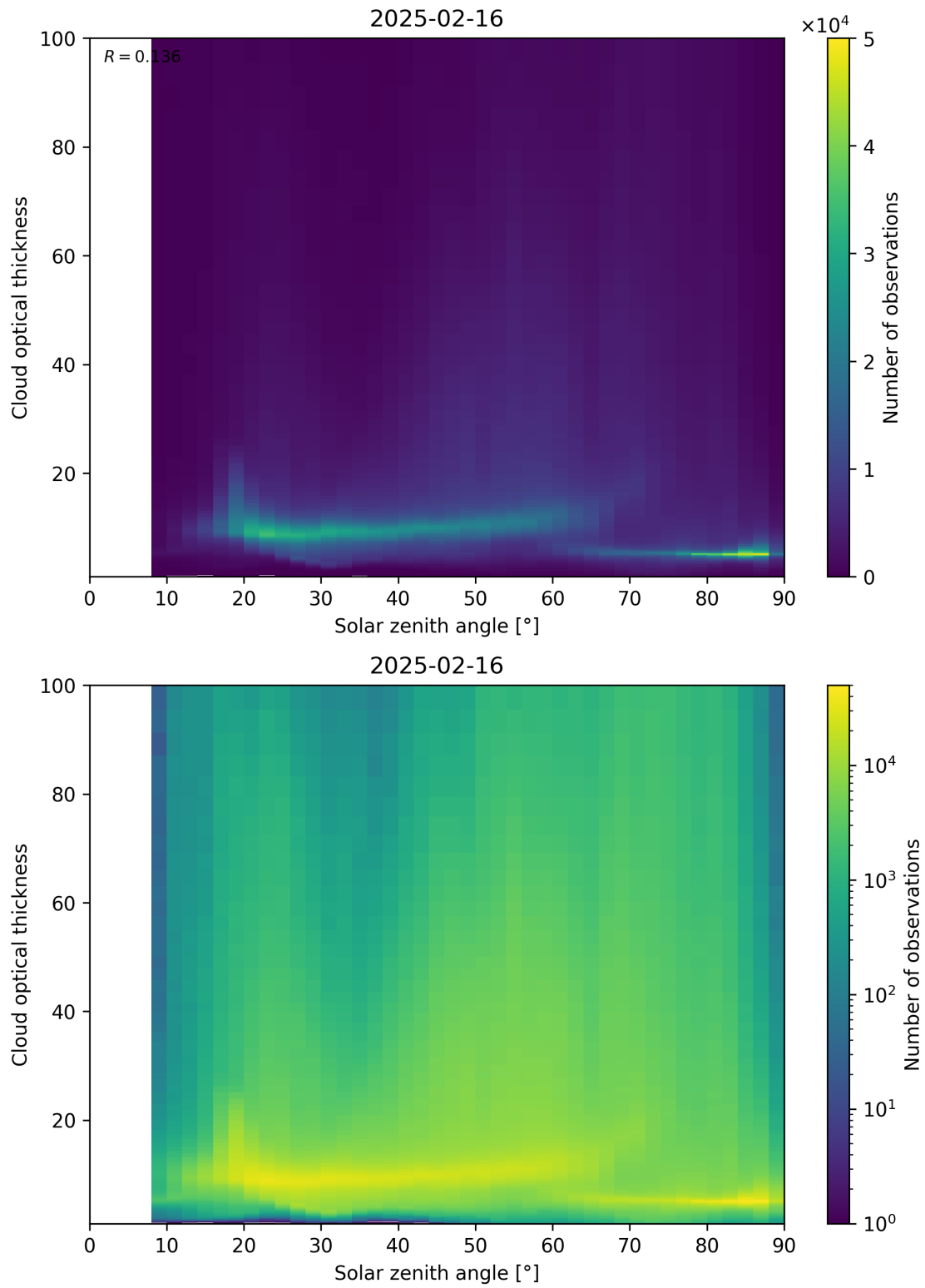
Figure 103: Scatter density plot of “Solar zenith angle” against “Cloud optical thickness” for 2025-02-15 to 2025-02-17.
