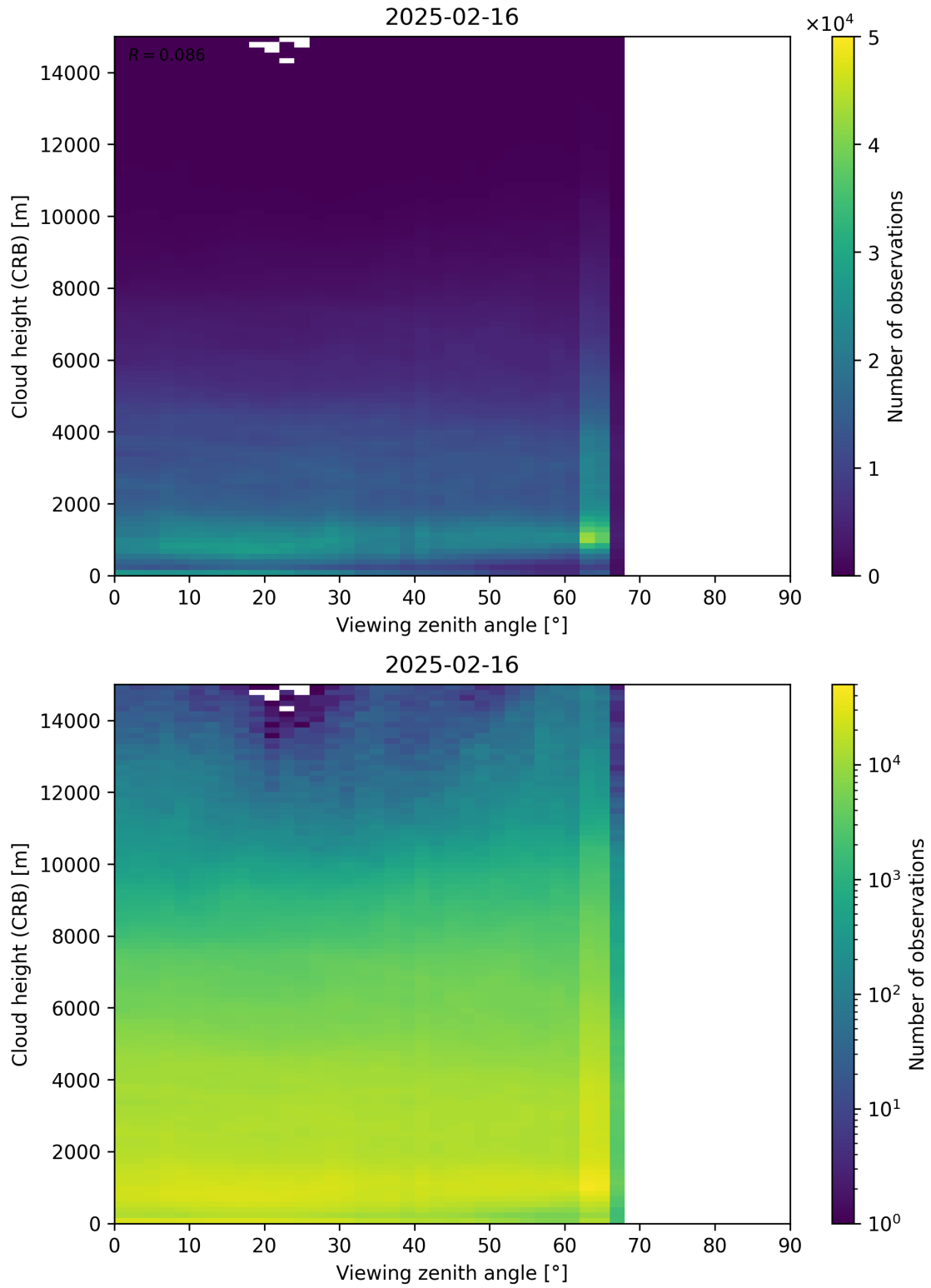
Figure 110: Scatter density plot of “Viewing zenith angle” against “Cloud height (CRB)” for 2025-02-15 to 2025-02-17.
