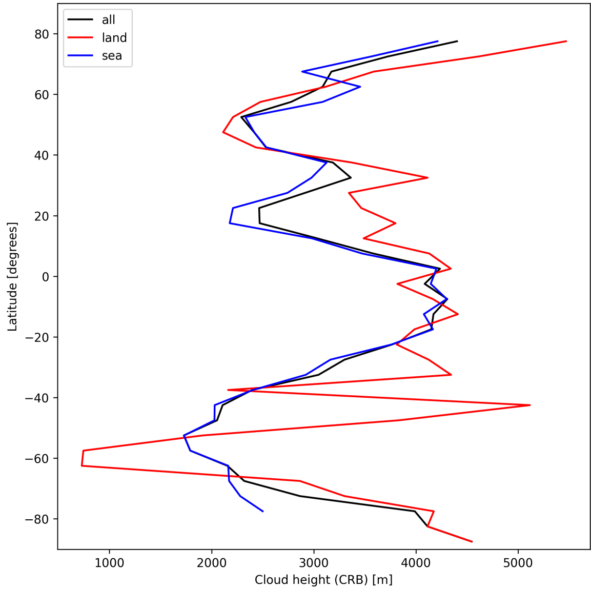
Figure 27: Zonal average of “Cloud height (CRB)” for 2025-02-15 to 2025-02-17.
