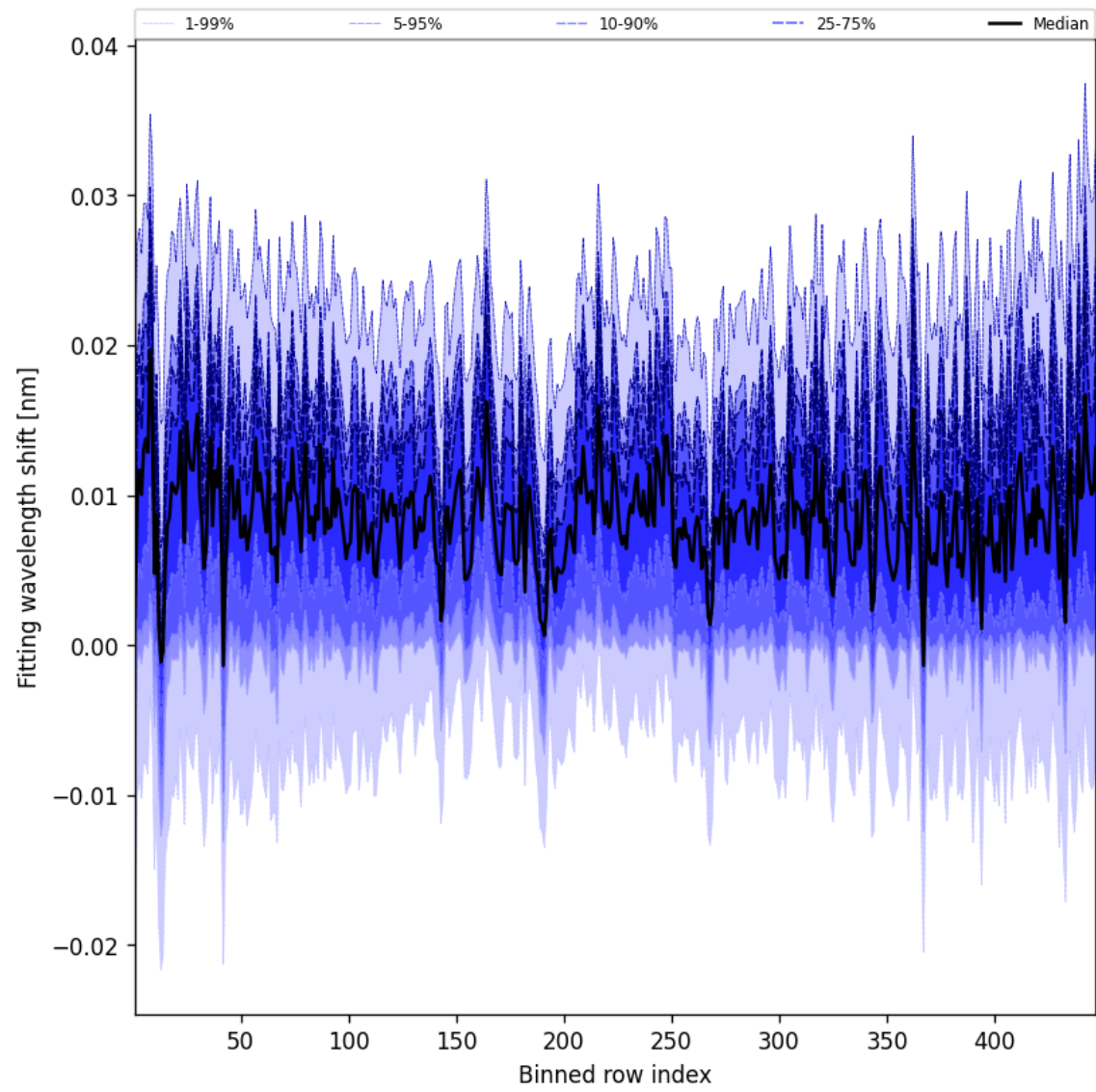
Figure 65: Along track statistics of “Fitting wavelength shift” for 2025-02-15 to 2025-02-17
