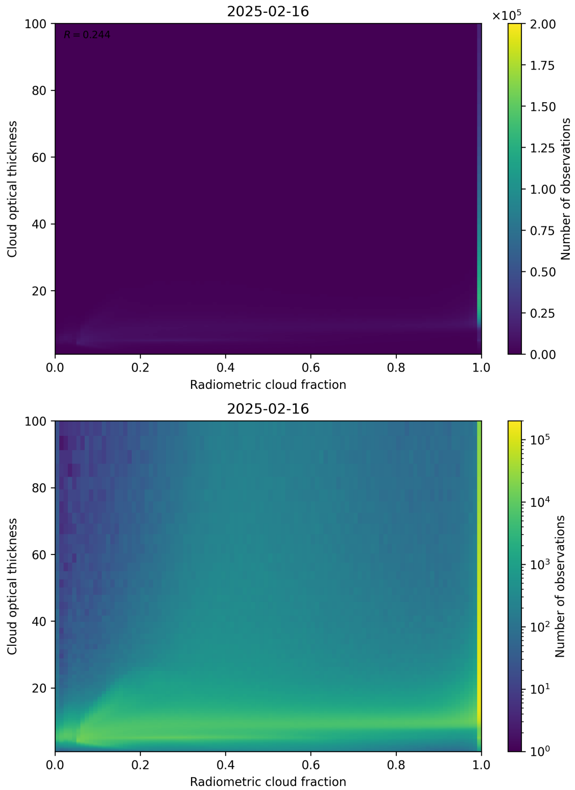
Figure 75: Scatter density plot of “Radiometric cloud fraction” against “Cloud optical thickness” for 2025-02-15 to 2025-02-17.
