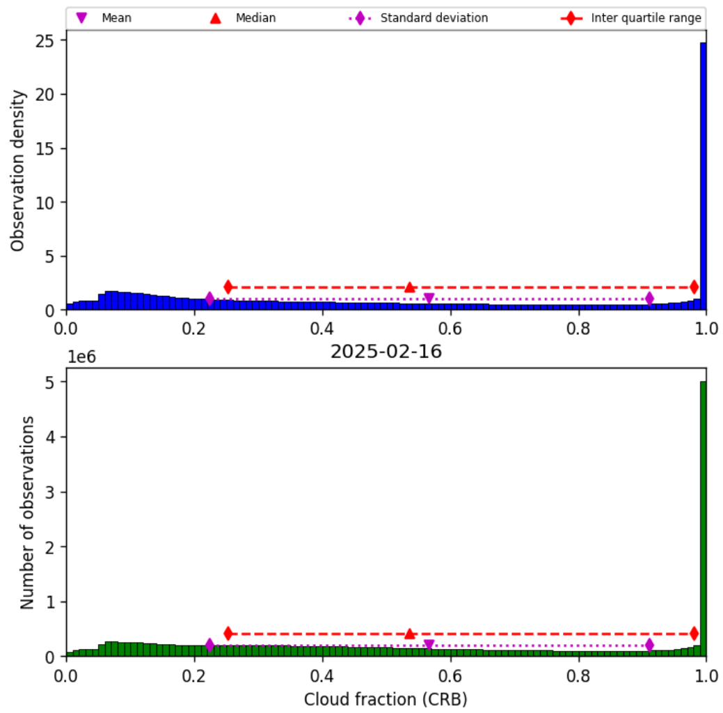
Figure 42: Histogram of “Cloud fraction (CRB)” for 2025-02-15 to 2025-02-17
