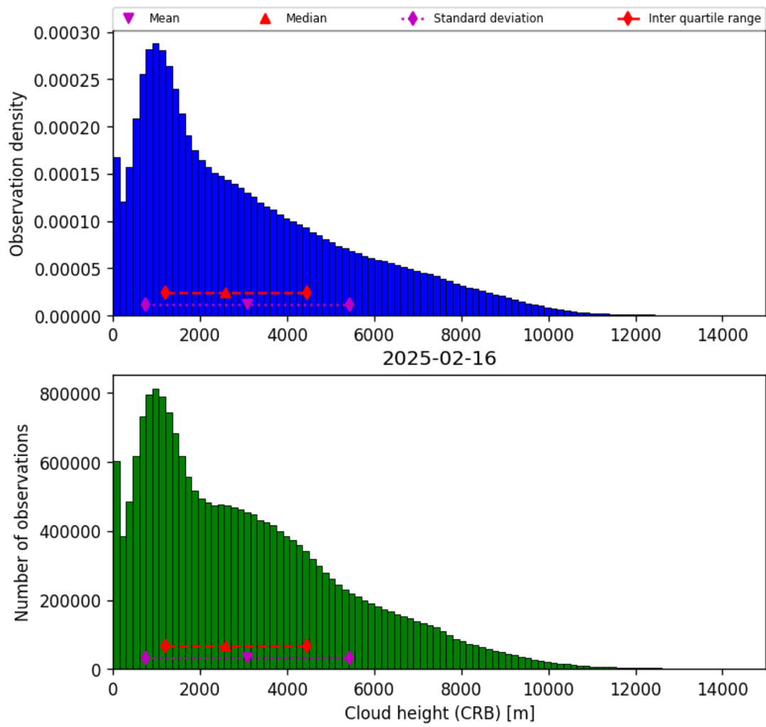
Figure 43: Histogram of “Cloud height (CRB)” for 2025-02-15 to 2025-02-17
