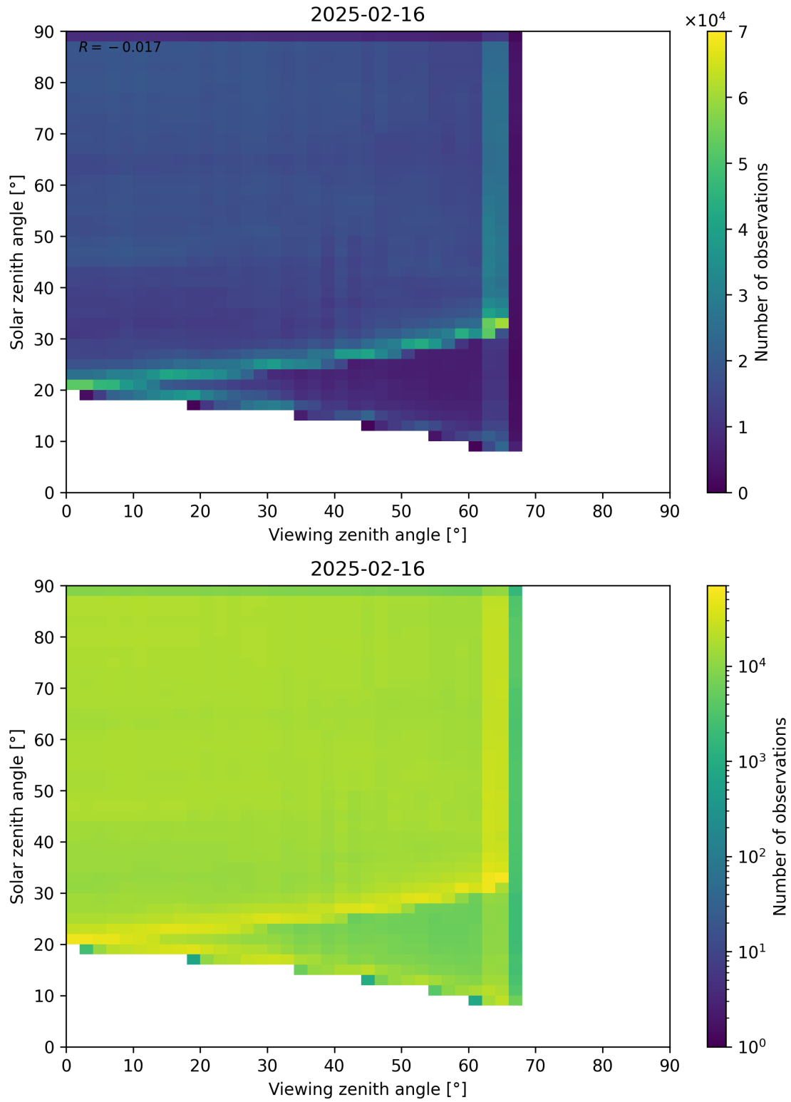
Figure 114: Scatter density plot of “Viewing zenith angle” against “Solar zenith angle” for 2025-02-15 to 2025-02-17.
