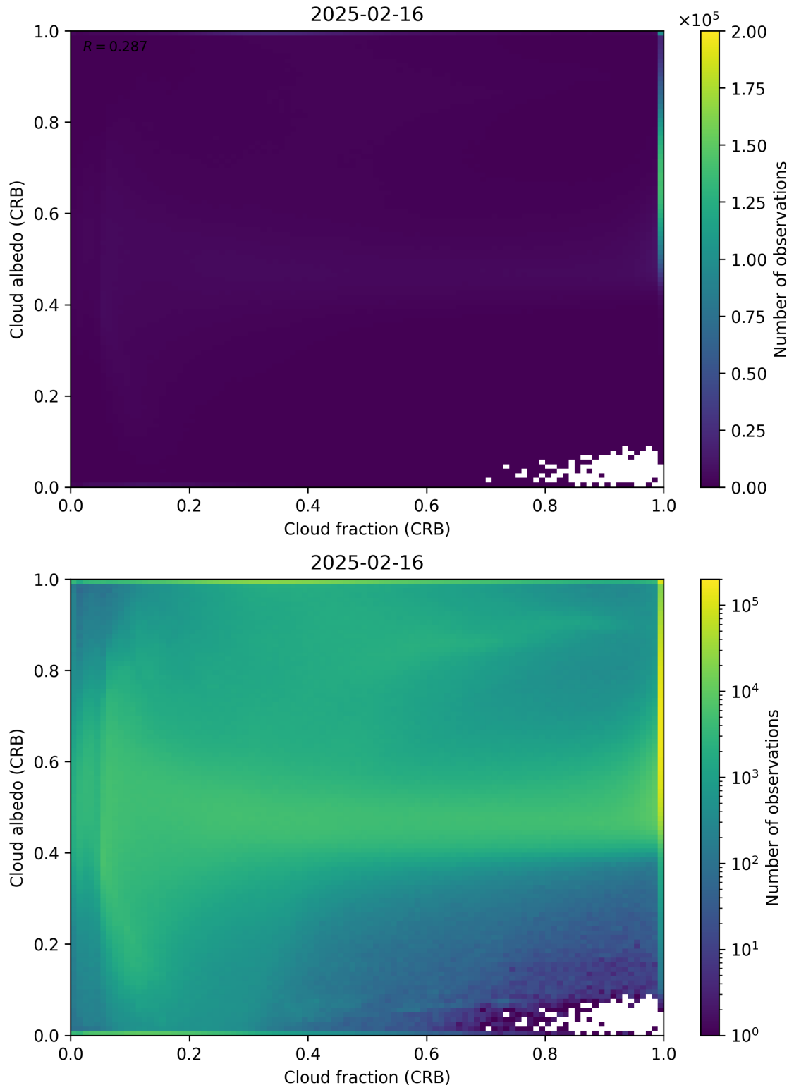
Figure 77: Scatter density plot of “Cloud fraction (CRB)” against “Cloud albedo (CRB)” for 2025-02-15 to 2025-02-17.
