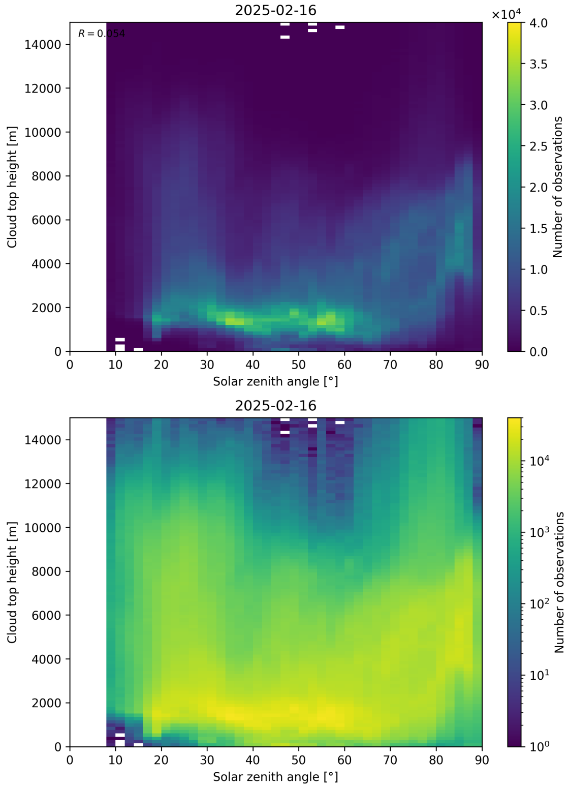
Figure 104: Scatter density plot of “Solar zenith angle” against “Cloud top height” for 2025-02-15 to 2025-02-17.
