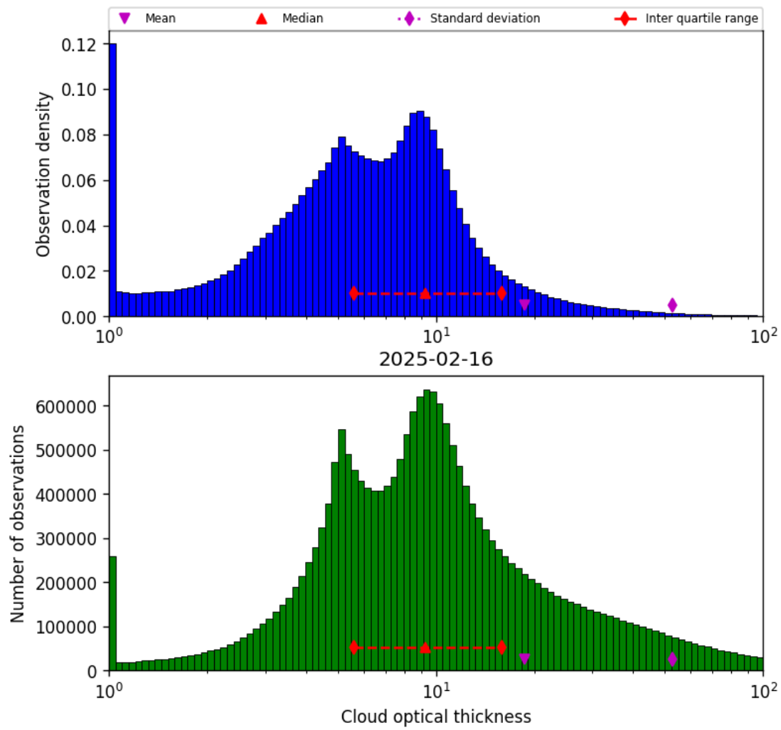
Figure 41: Histogram of “Cloud optical thickness” for 2025-02-15 to 2025-02-17
