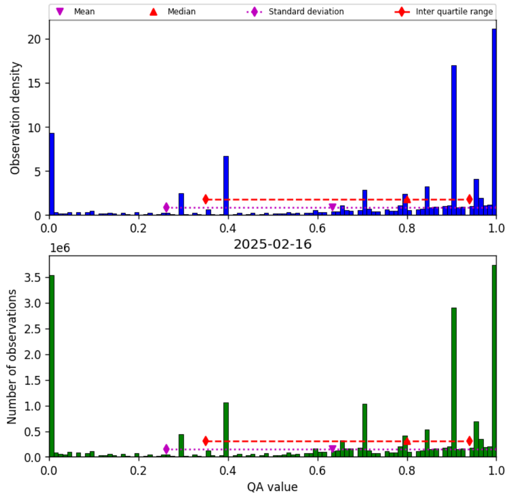
Figure 38: Histogram of “QA value” for 2025-02-15 to 2025-02-17
