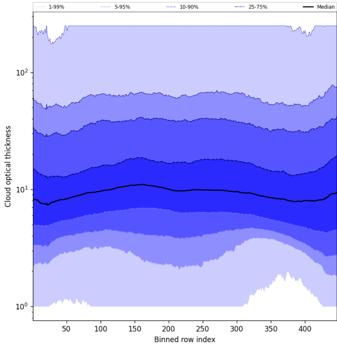
Figure 57: Along track statistics of “Cloud optical thickness” for 2025-02-15 to 2025-02-17
