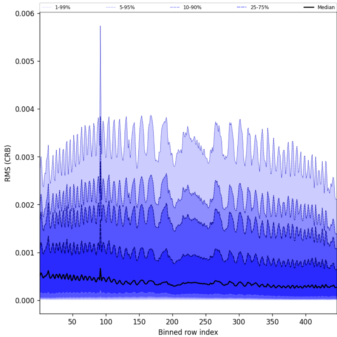
Figure 64: Along track statistics of “RMS (CRB)” for 2025-02-15 to 2025-02-17
