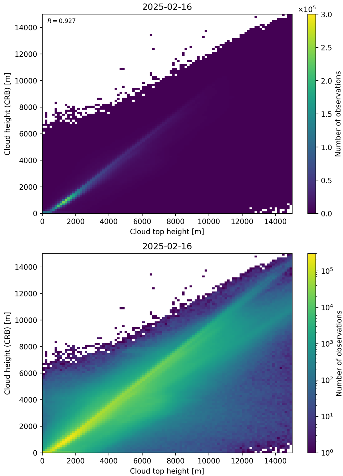
Figure 89: Scatter density plot of “Cloud top height” against “Cloud height (CRB)” for 2025-02-15 to 2025-02-17.
