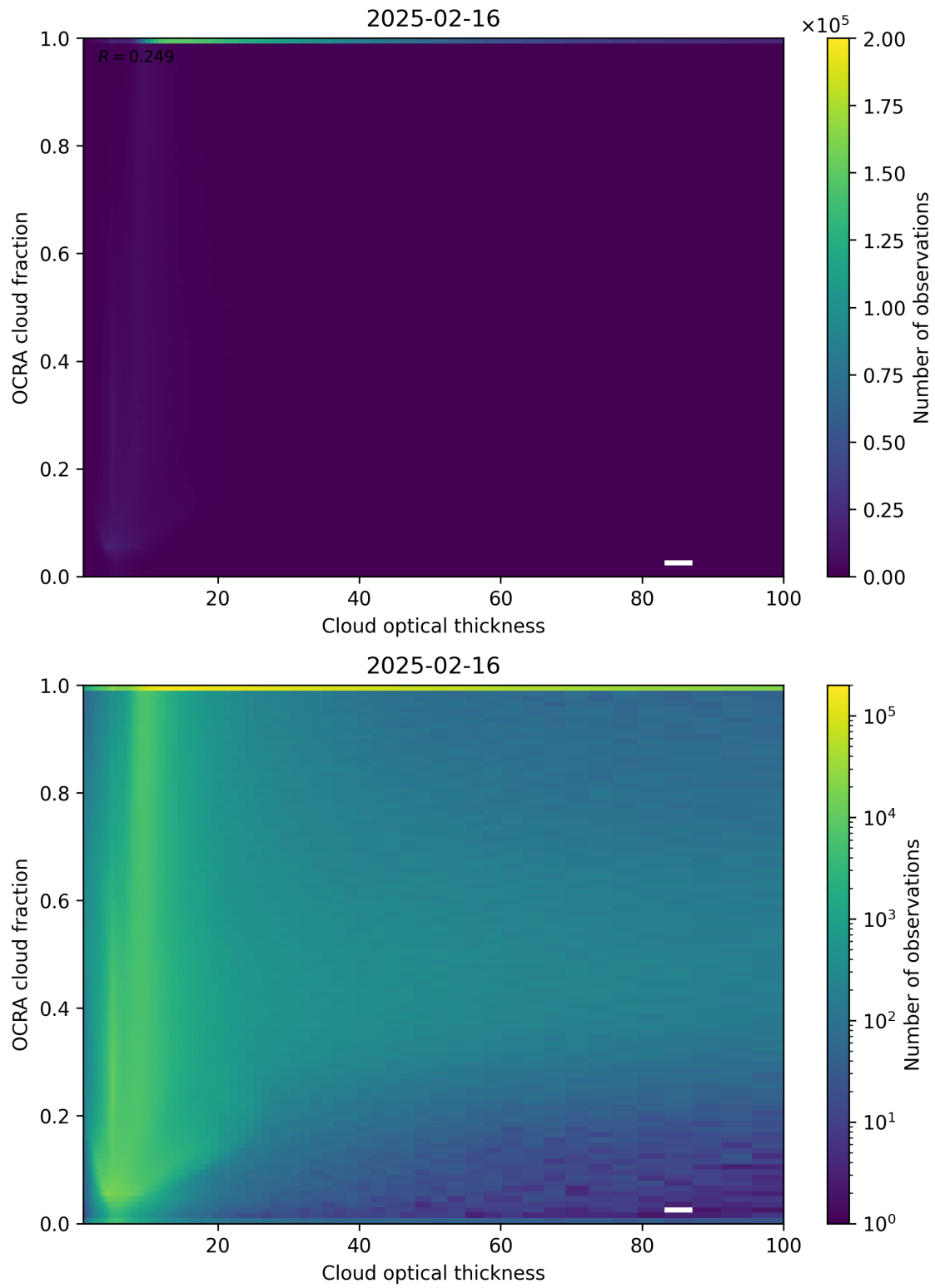
Figure 83: Scatter density plot of “Cloud optical thickness” against “OCRA cloud fraction” for 2025-02-15 to 2025-02-17.
