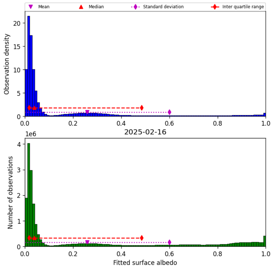
Figure 45: Histogram of “Fitted surface albedo” for 2025-02-15 to 2025-02-17
