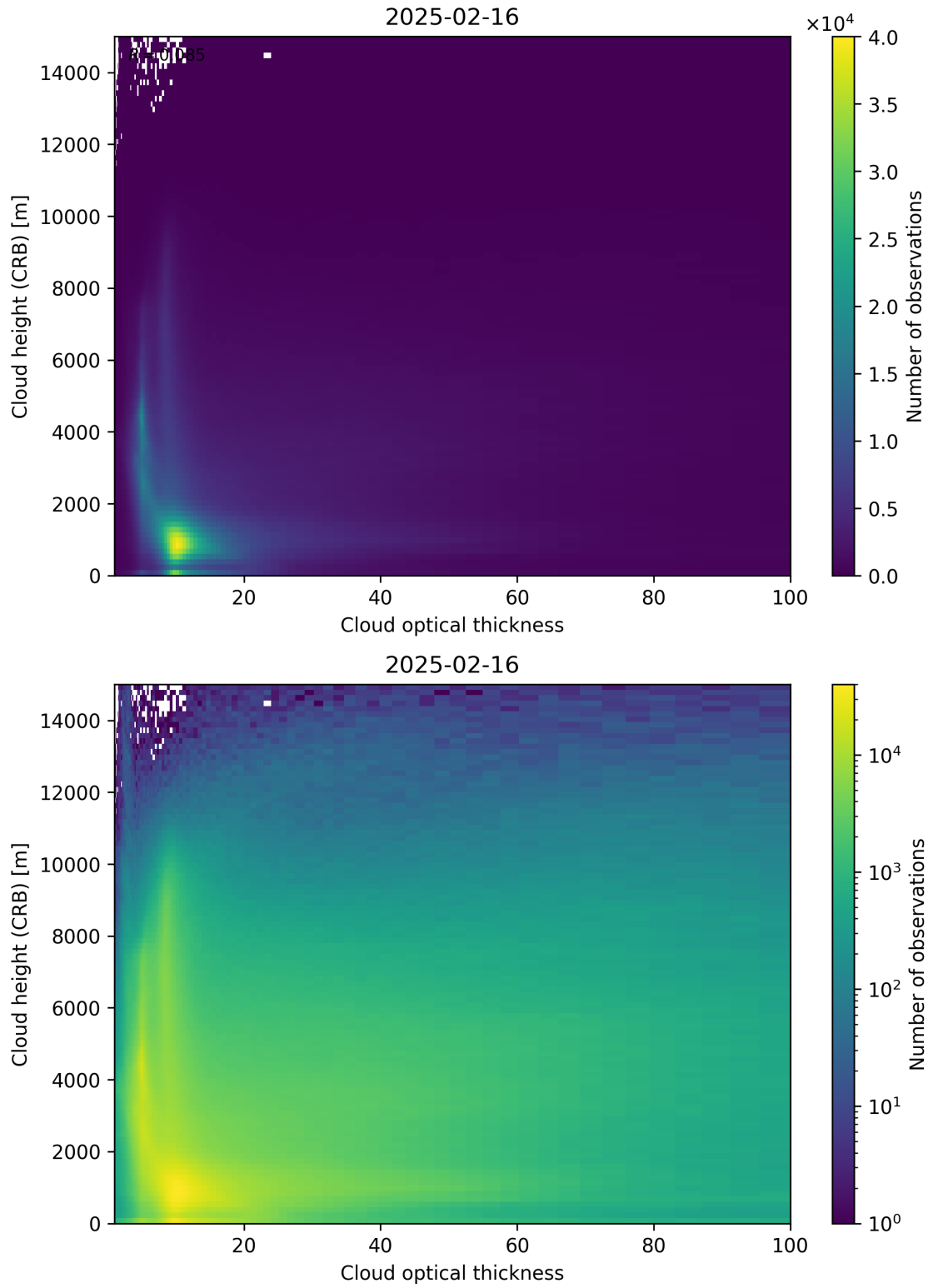
Figure 85: Scatter density plot of “Cloud optical thickness” against “Cloud height (CRB)” for 2025-02-15 to 2025-02-17.
