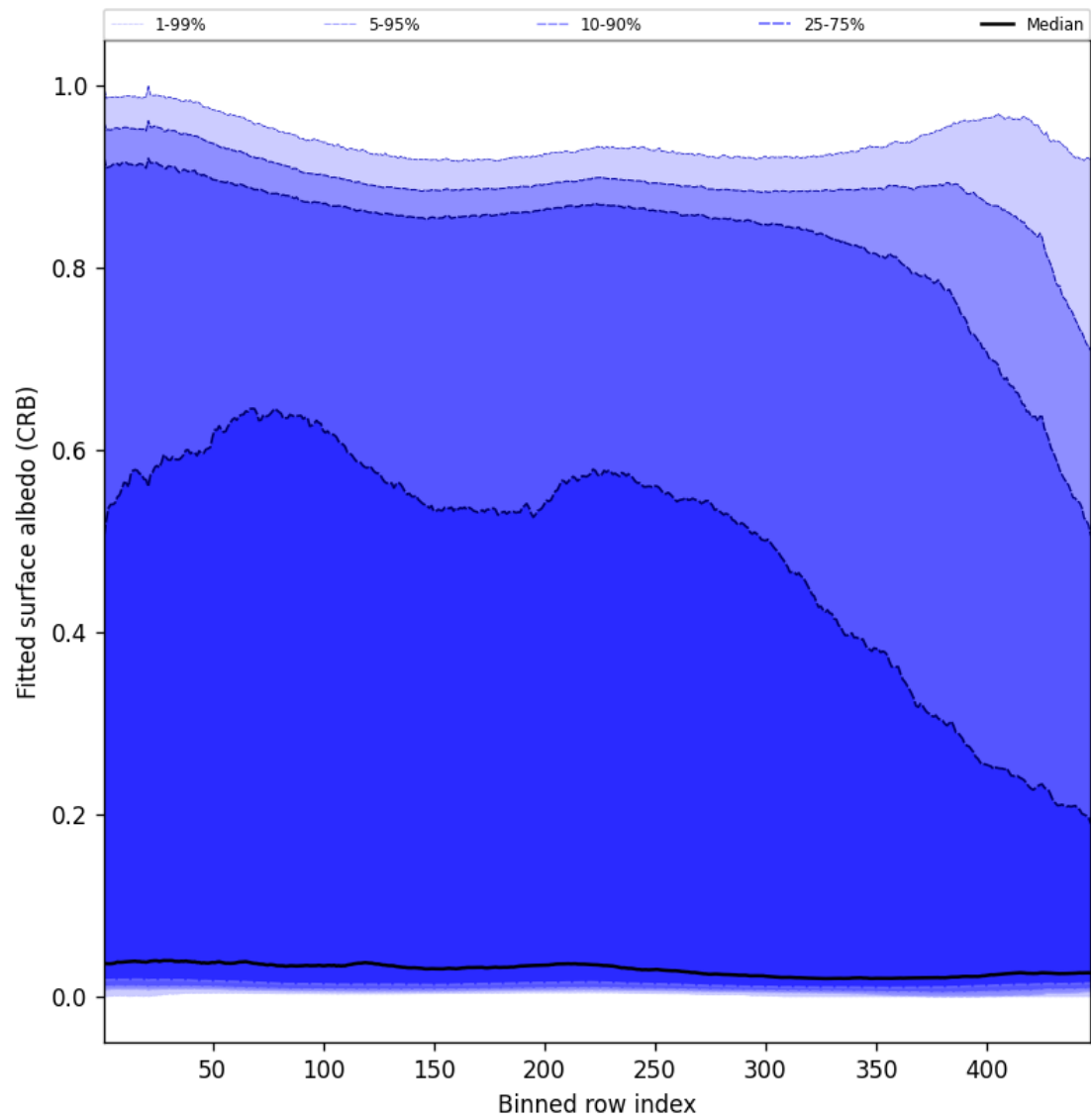
Figure 62: Along track statistics of “Fitted surface albedo (CRB)” for 2025-02-15 to 2025-02-17
