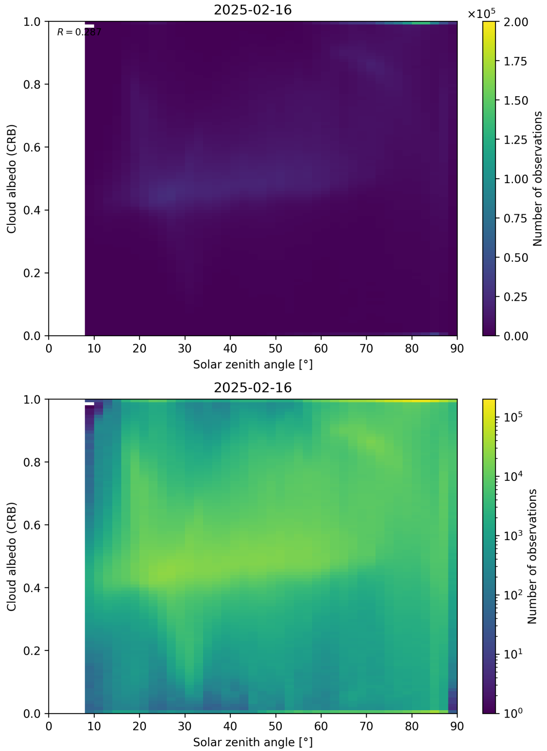
Figure 98: Scatter density plot of “Solar zenith angle” against “Cloud albedo (CRB)” for 2025-02-15 to 2025-02-17.
