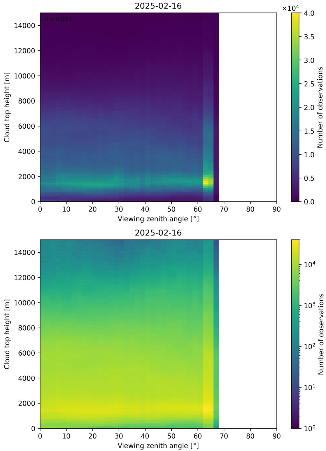
Figure 112: Scatter density plot of “Viewing zenith angle” against “Cloud top height” for 2025-02-15 to 2025-02-17.
