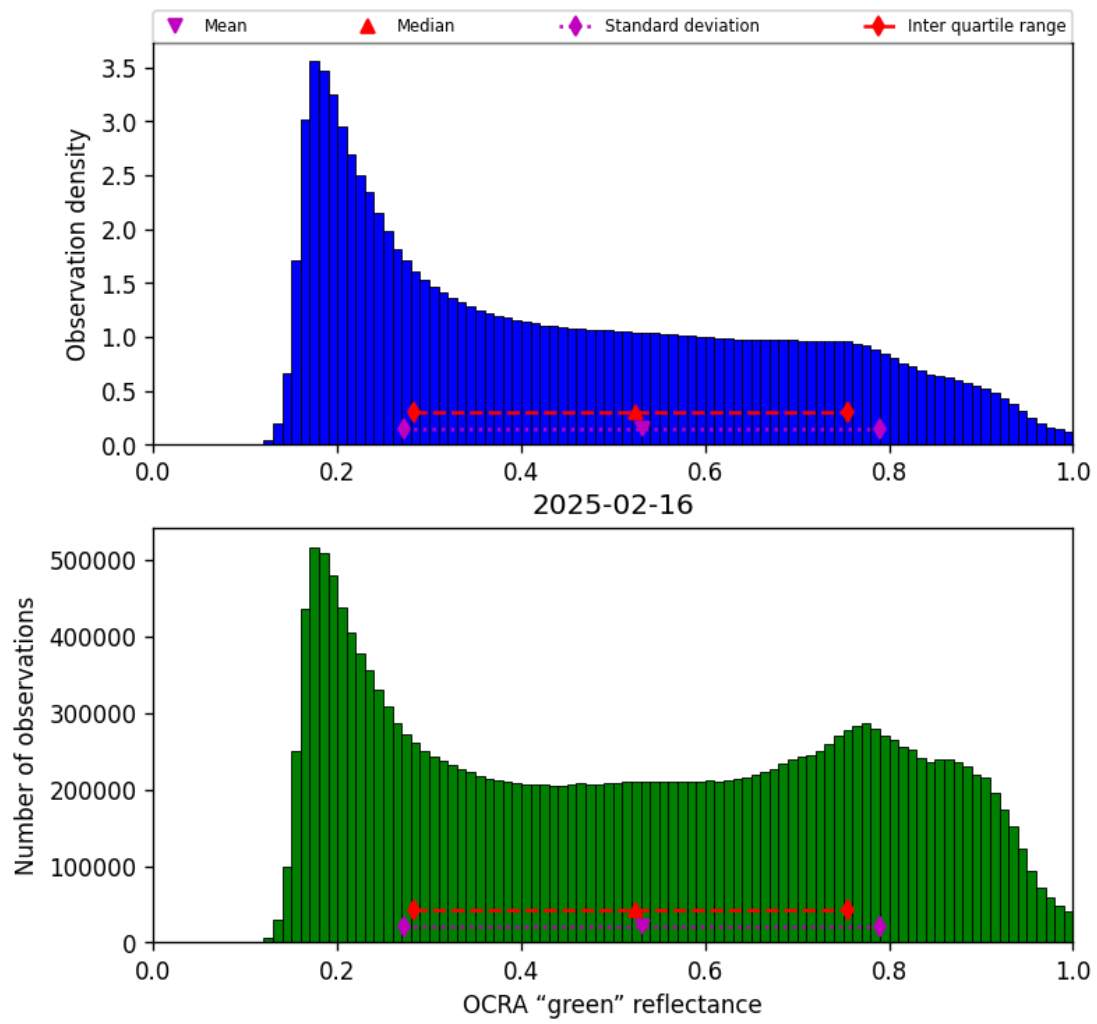
Figure 52: Histogram of “OCRA “green” reflectance” for 2025-02-15 to 2025-02-17
