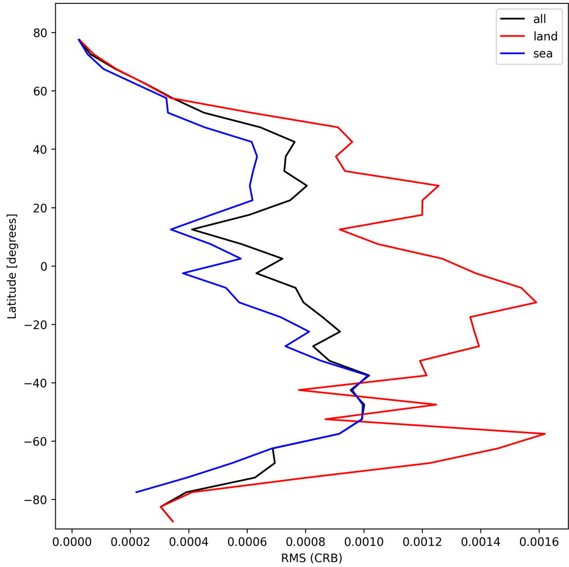
Figure 32: Zonal average of “RMS (CRB)” for 2025-02-15 to 2025-02-17.
