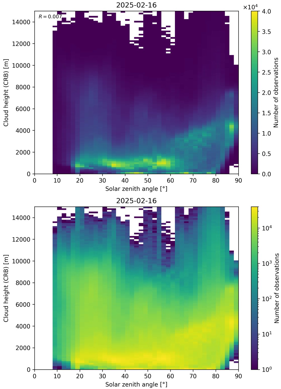
Figure 102: Scatter density plot of “Solar zenith angle” against “Cloud height (CRB)” for 2025-02-15 to 2025-02-17.
