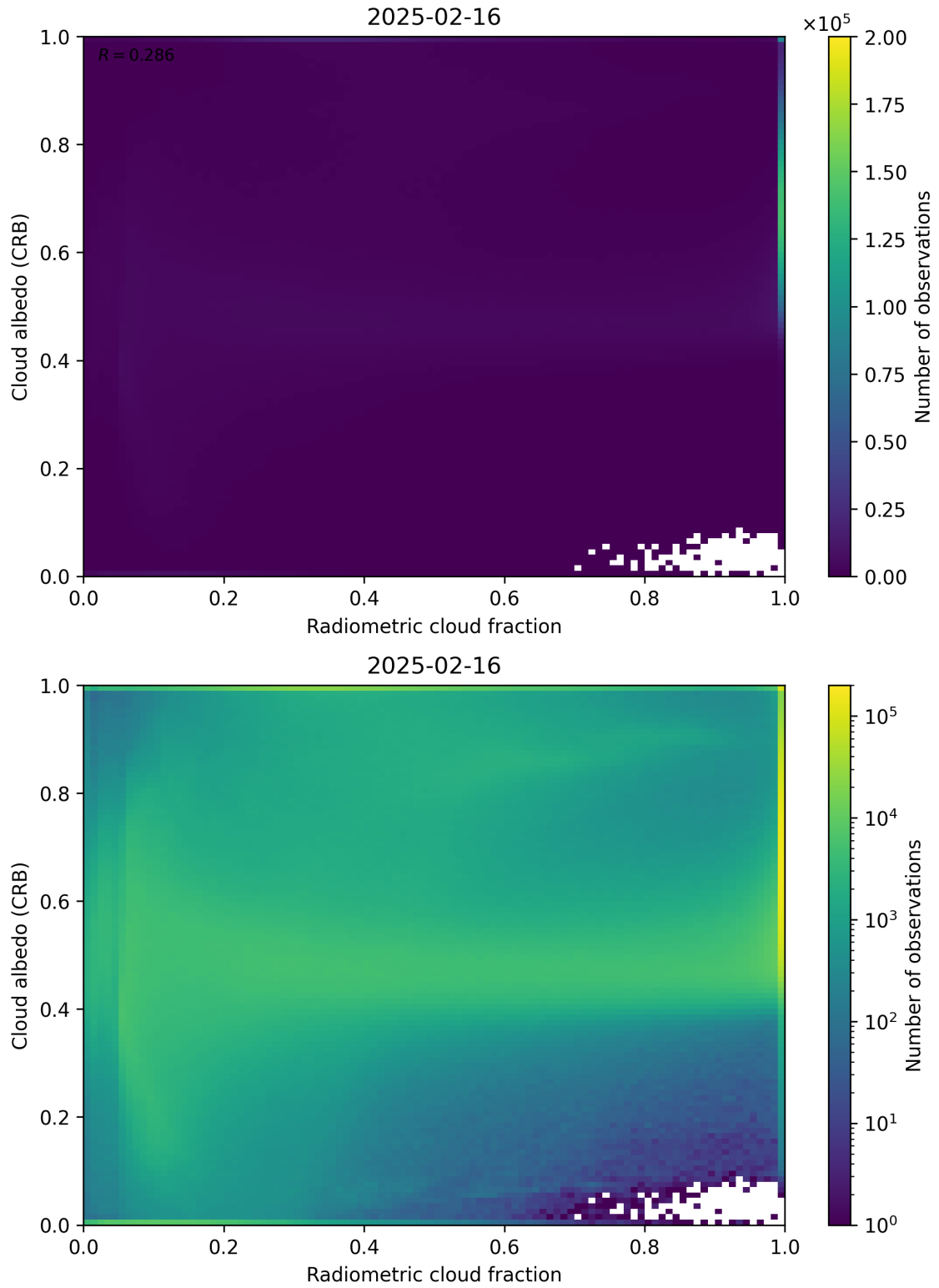
Figure 71: Scatter density plot of “Radiometric cloud fraction” against “Cloud albedo (CRB)” for 2025-02-15 to 2025-02-17.
