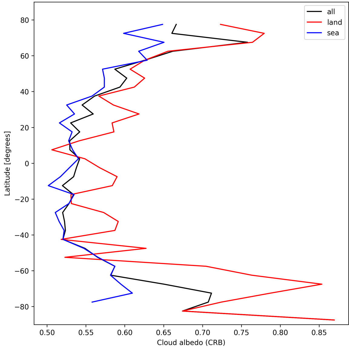
Figure 28: Zonal average of “Cloud albedo (CRB)” for 2025-02-15 to 2025-02-17.
