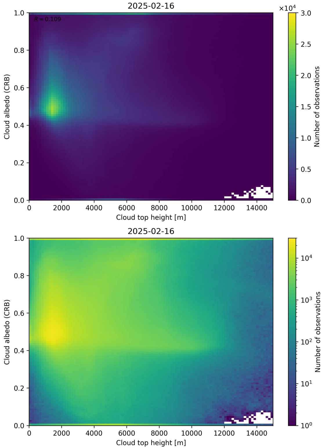
Figure 86: Scatter density plot of “Cloud top height” against “Cloud albedo (CRB)” for 2025-02-15 to 2025-02-17.
