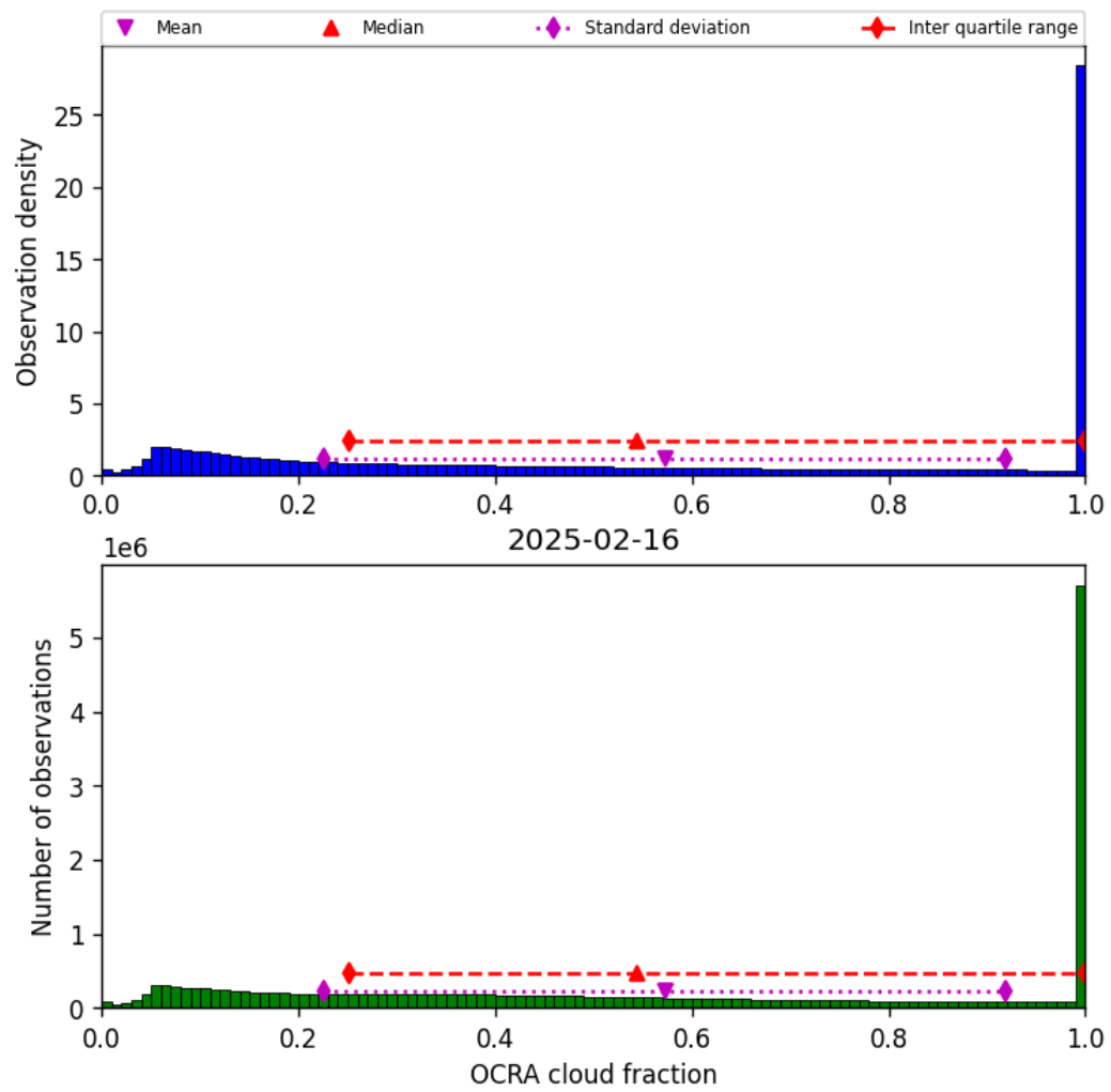
Figure 50: Histogram of “OCRA cloud fraction” for 2025-02-15 to 2025-02-17
