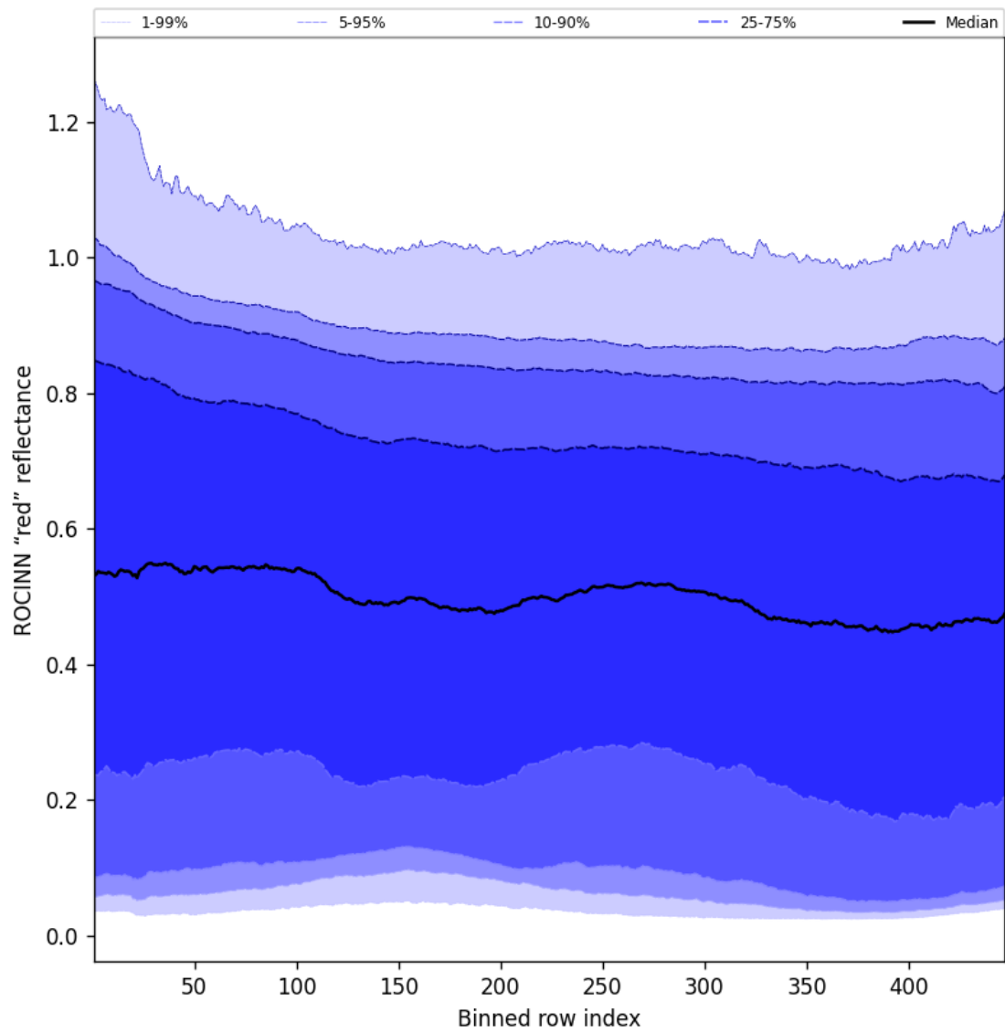
Figure 69: Along track statistics of “ROCINN “red” reflectance” for 2025-02-15 to 2025-02-17
