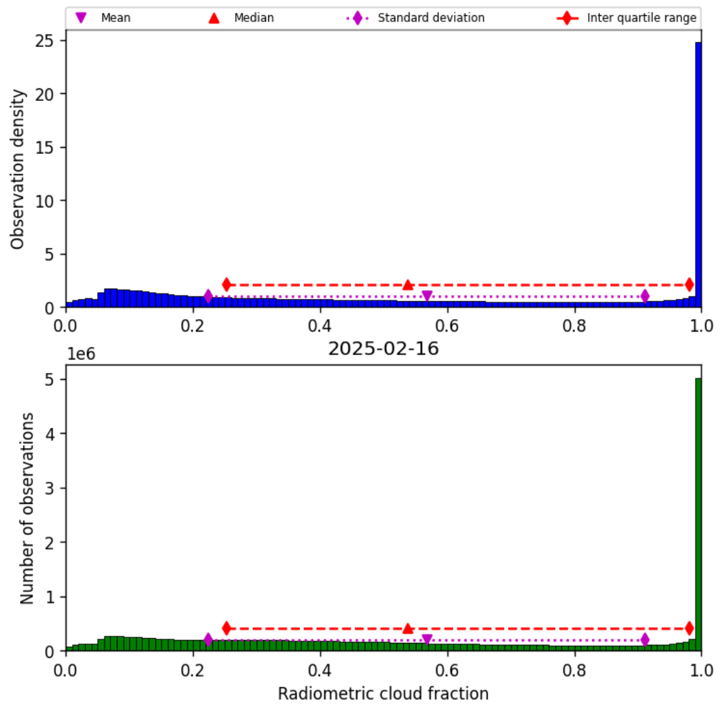
Figure 39: Histogram of “Radiometric cloud fraction” for 2025-02-15 to 2025-02-17
