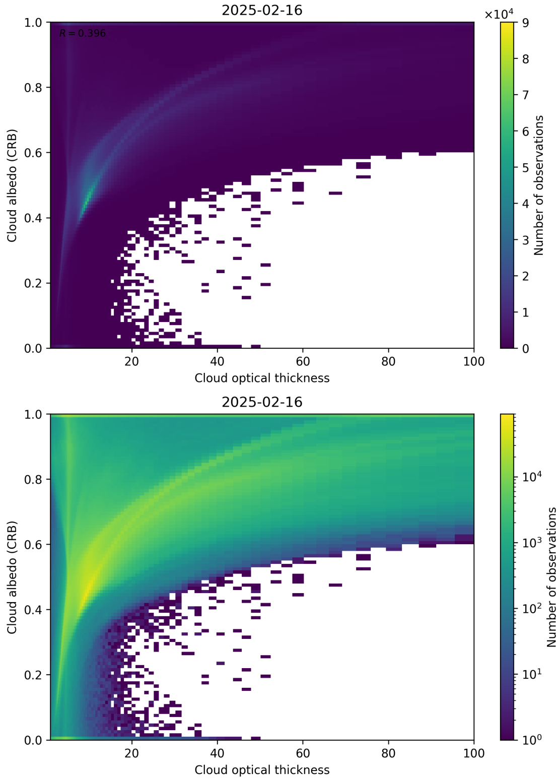
Figure 82: Scatter density plot of “Cloud optical thickness” against “Cloud albedo (CRB)” for 2025-02-15 to 2025-02-17.
