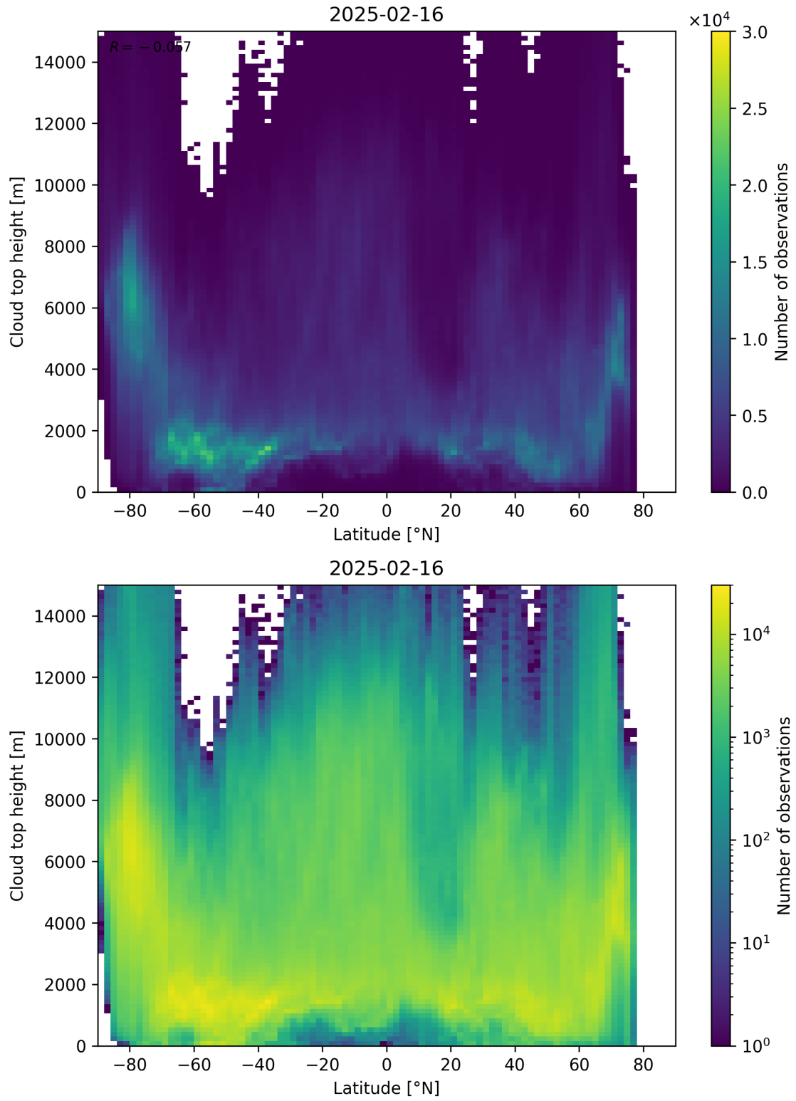
Figure 97: Scatter density plot of “Latitude” against “Cloud top height” for 2025-02-15 to 2025-02-17.
