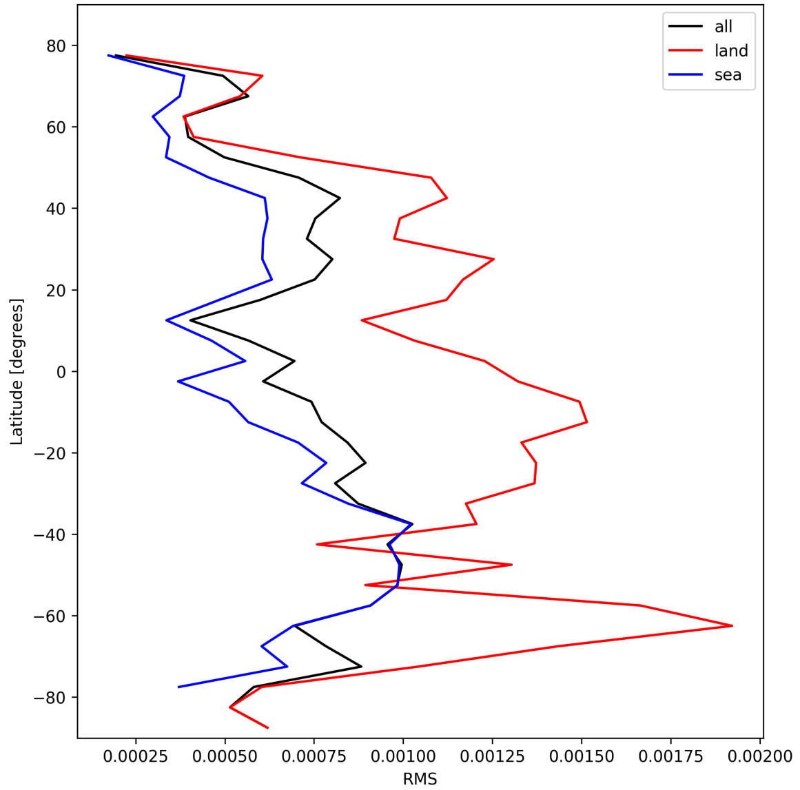
Figure 31: Zonal average of “RMS” for 2025-02-15 to 2025-02-17.
