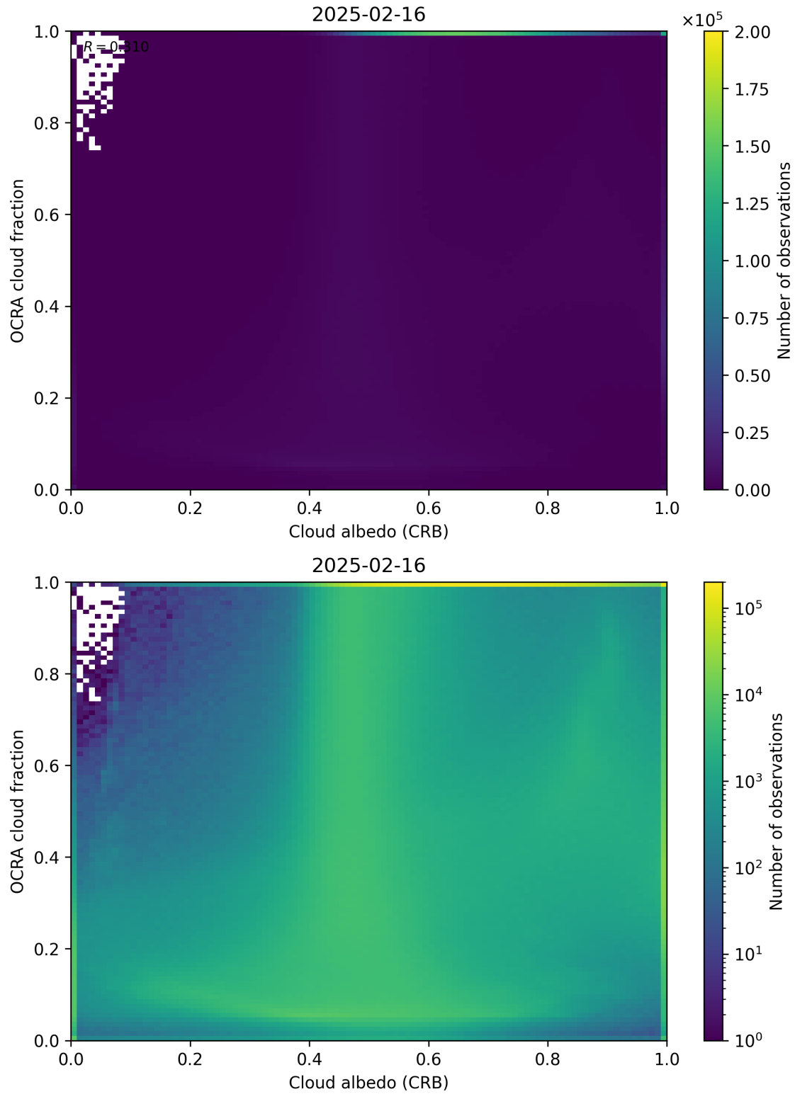
Figure 70: Scatter density plot of “Cloud albedo (CRB)” against “OCRA cloud fraction” for 2025-02-15 to 2025-02-17.
