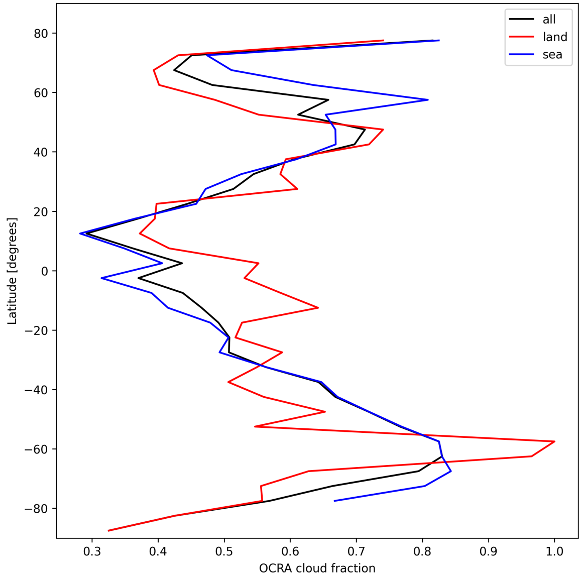
Figure 34: Zonal average of “OCRA cloud fraction” for 2025-02-15 to 2025-02-17.
