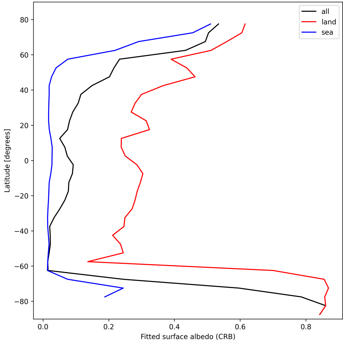
Figure 30: Zonal average of “Fitted surface albedo (CRB)” for 2025-02-15 to 2025-02-17.
