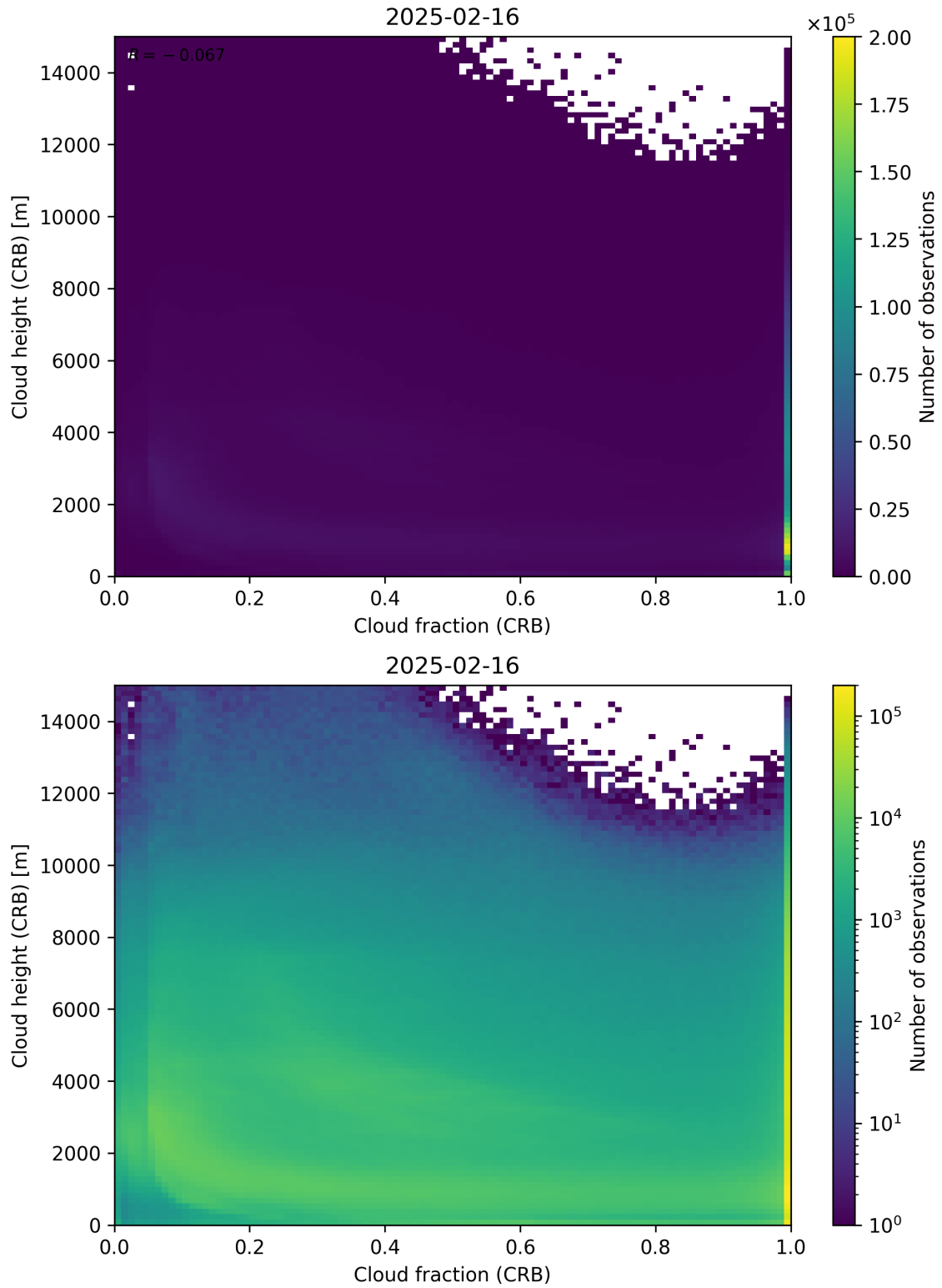
Figure 79: Scatter density plot of “Cloud fraction (CRB)” against “Cloud height (CRB)” for 2025-02-15 to 2025-02-17.
