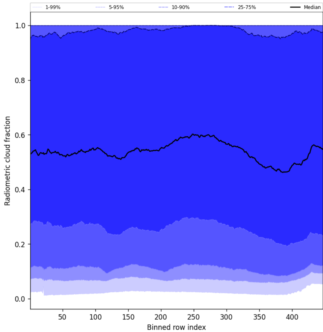
Figure 55: Along track statistics of “Radiometric cloud fraction” for 2025-02-15 to 2025-02-17
