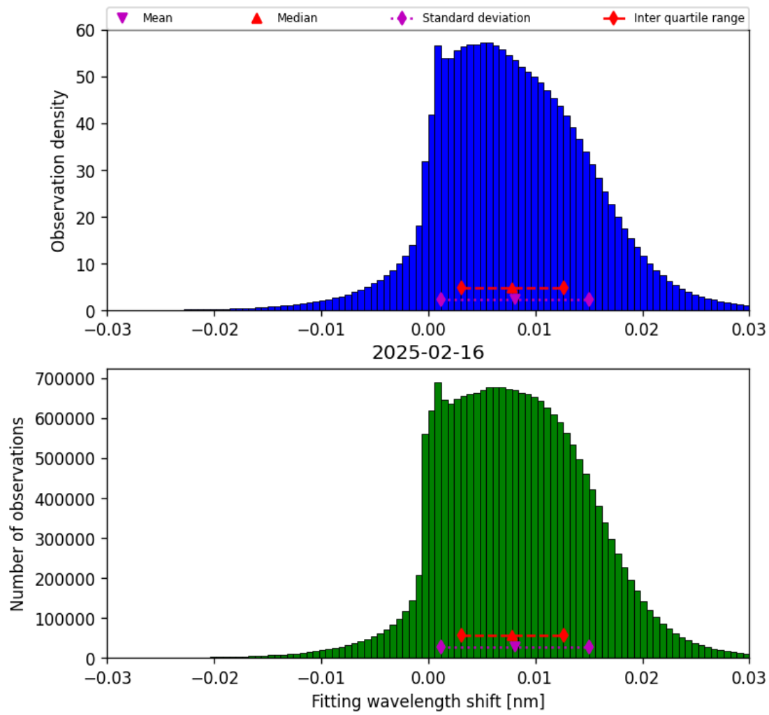
Figure 49: Histogram of “Fitting wavelength shift” for 2025-02-15 to 2025-02-17
