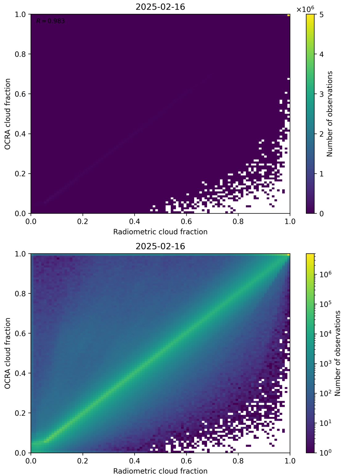
Figure 72: Scatter density plot of “Radiometric cloud fraction” against “OCRA cloud fraction” for 2025-02-15 to 2025-02-17.
