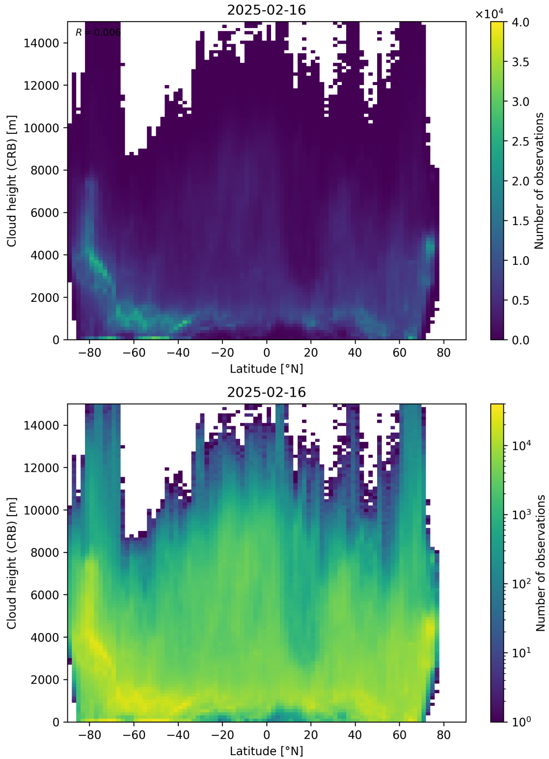
Figure 95: Scatter density plot of “Latitude” against “Cloud height (CRB)” for 2025-02-15 to 2025-02-17.
