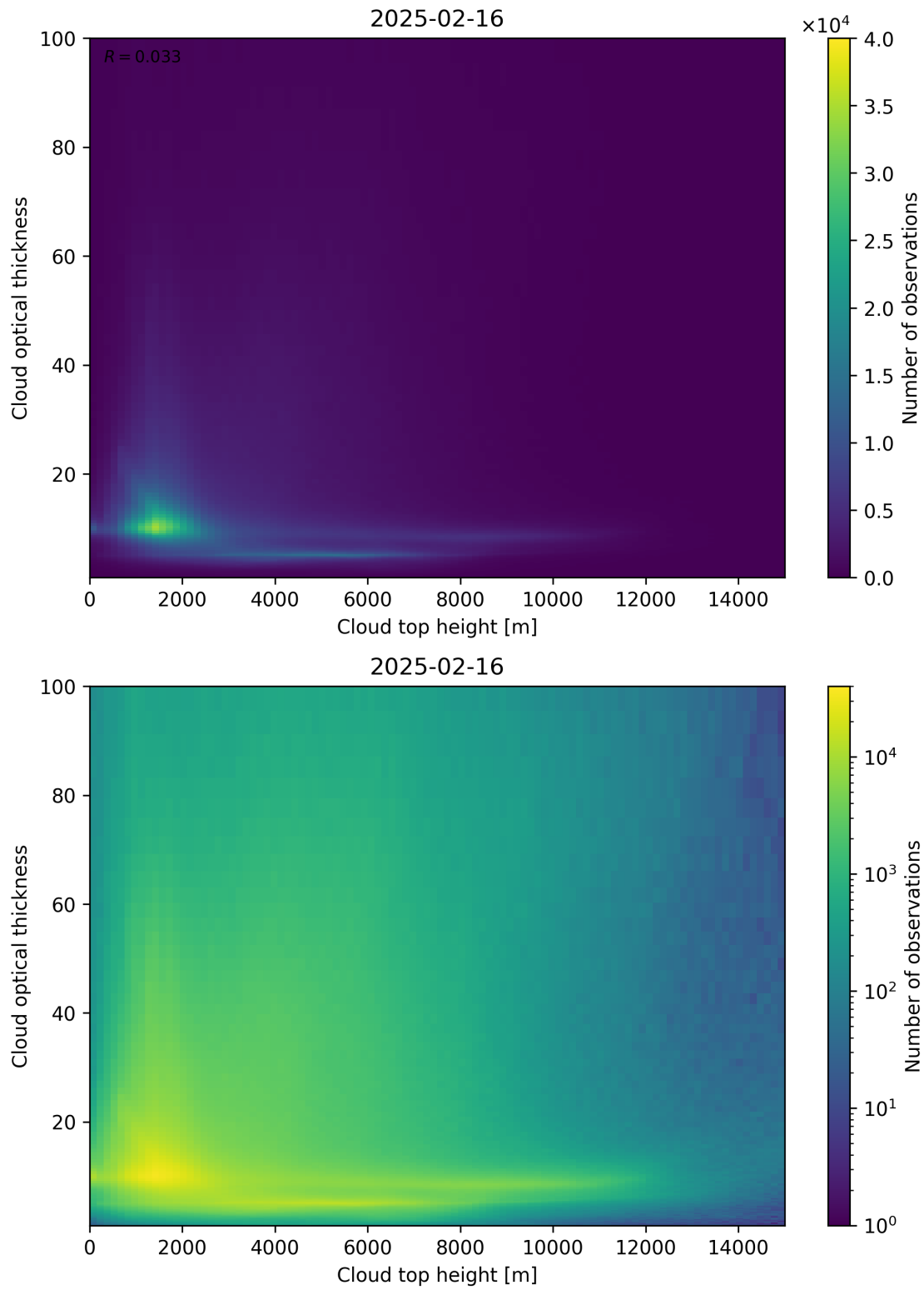
Figure 90: Scatter density plot of “Cloud top height” against “Cloud optical thickness” for 2025-02-15 to 2025-02-17.
