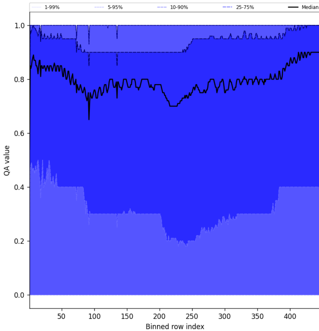
Figure 54: Along track statistics of “QA value” for 2025-02-15 to 2025-02-17
