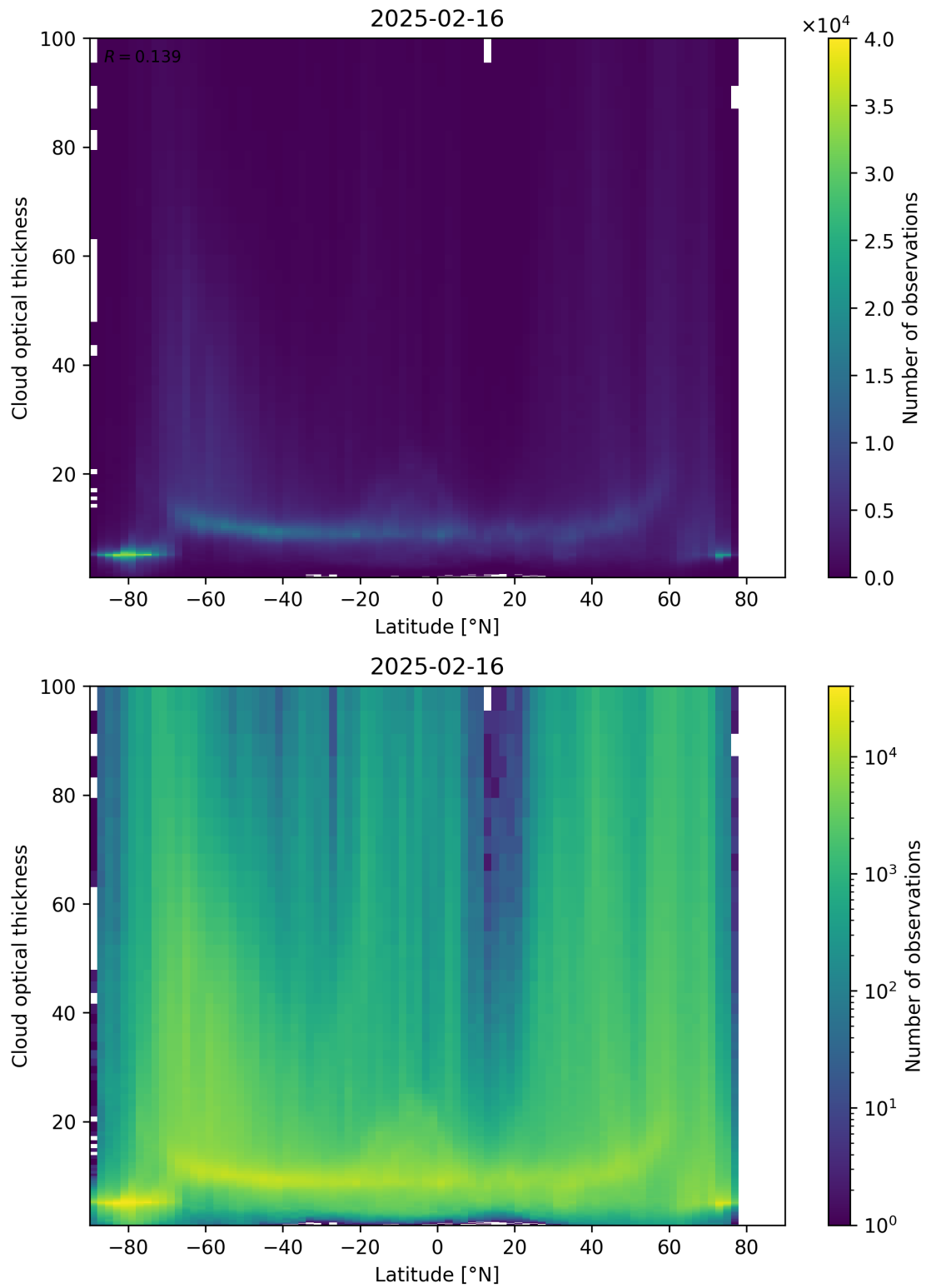
Figure 96: Scatter density plot of “Latitude” against “Cloud optical thickness” for 2025-02-15 to 2025-02-17.
