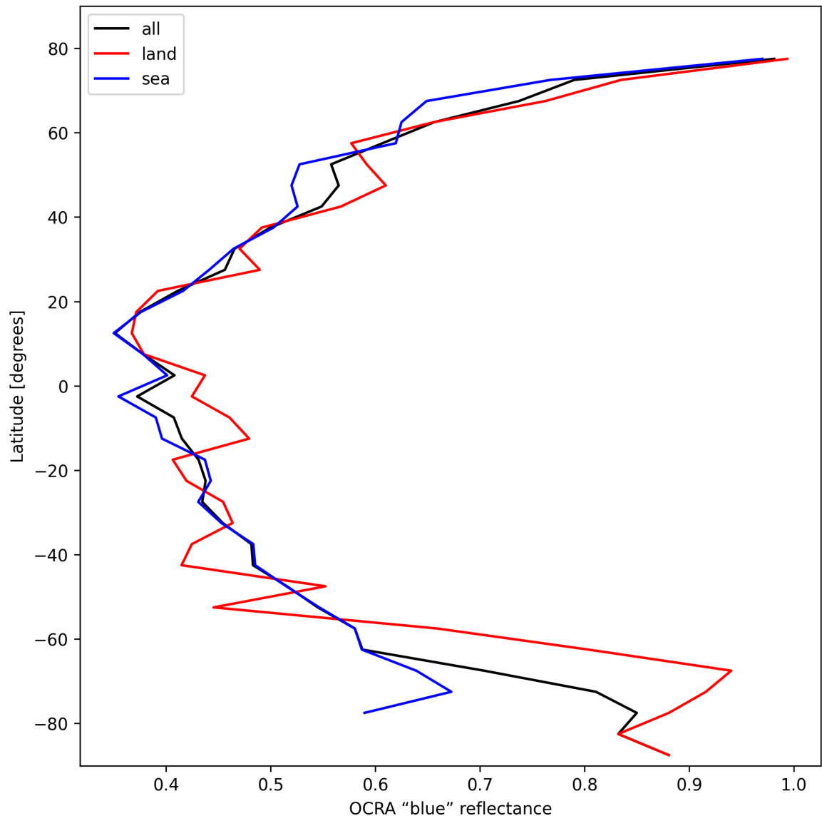
Figure 35: Zonal average of "OCRA "blue" reflectance" for 2025-02-15 to 2025-02-17.
