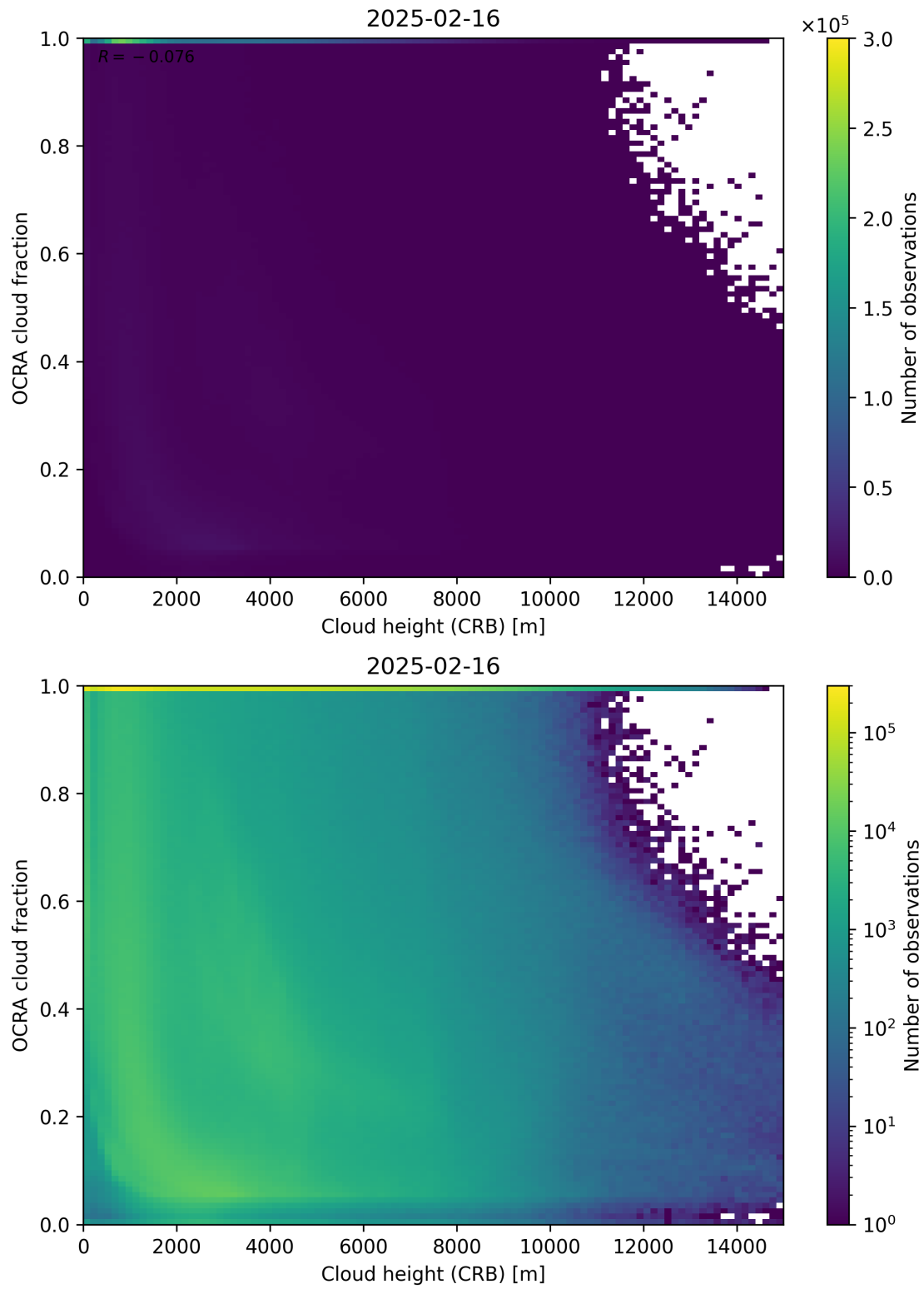
Figure 81: Scatter density plot of “Cloud height (CRB)” against “OCRA cloud fraction” for 2025-02-15 to 2025-02-17.
