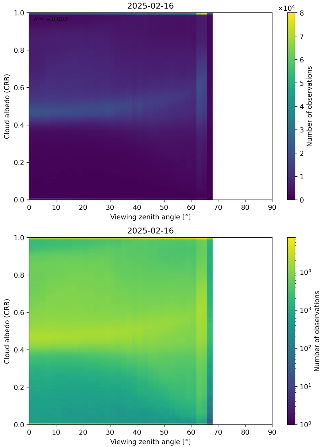
Figure 106: Scatter density plot of “Viewing zenith angle” against “Cloud albedo (CRB)” for 2025-02-15 to 2025-02-17.
