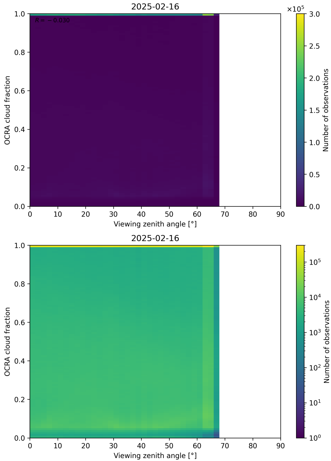
Figure 108: Scatter density plot of “Viewing zenith angle” against “OCRA cloud fraction” for 2025-02-15 to 2025-02-17.
