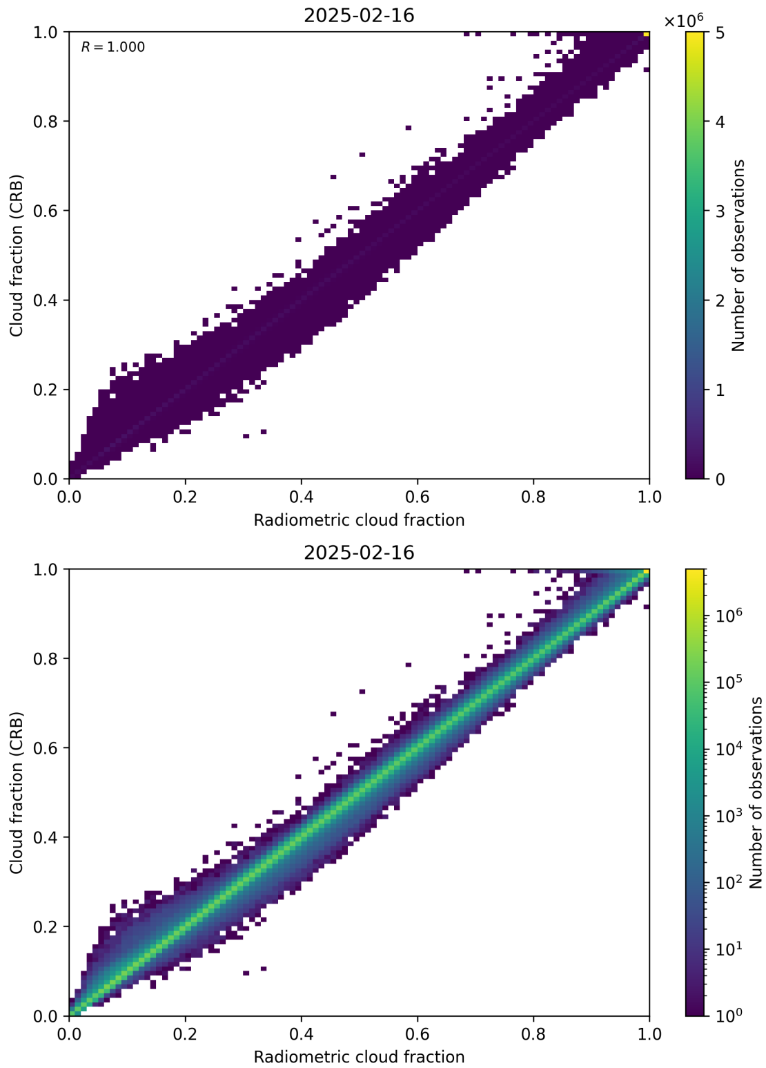
Figure 73: Scatter density plot of “Radiometric cloud fraction” against “Cloud fraction (CRB)” for 2025-02-15 to 2025-02-17.
