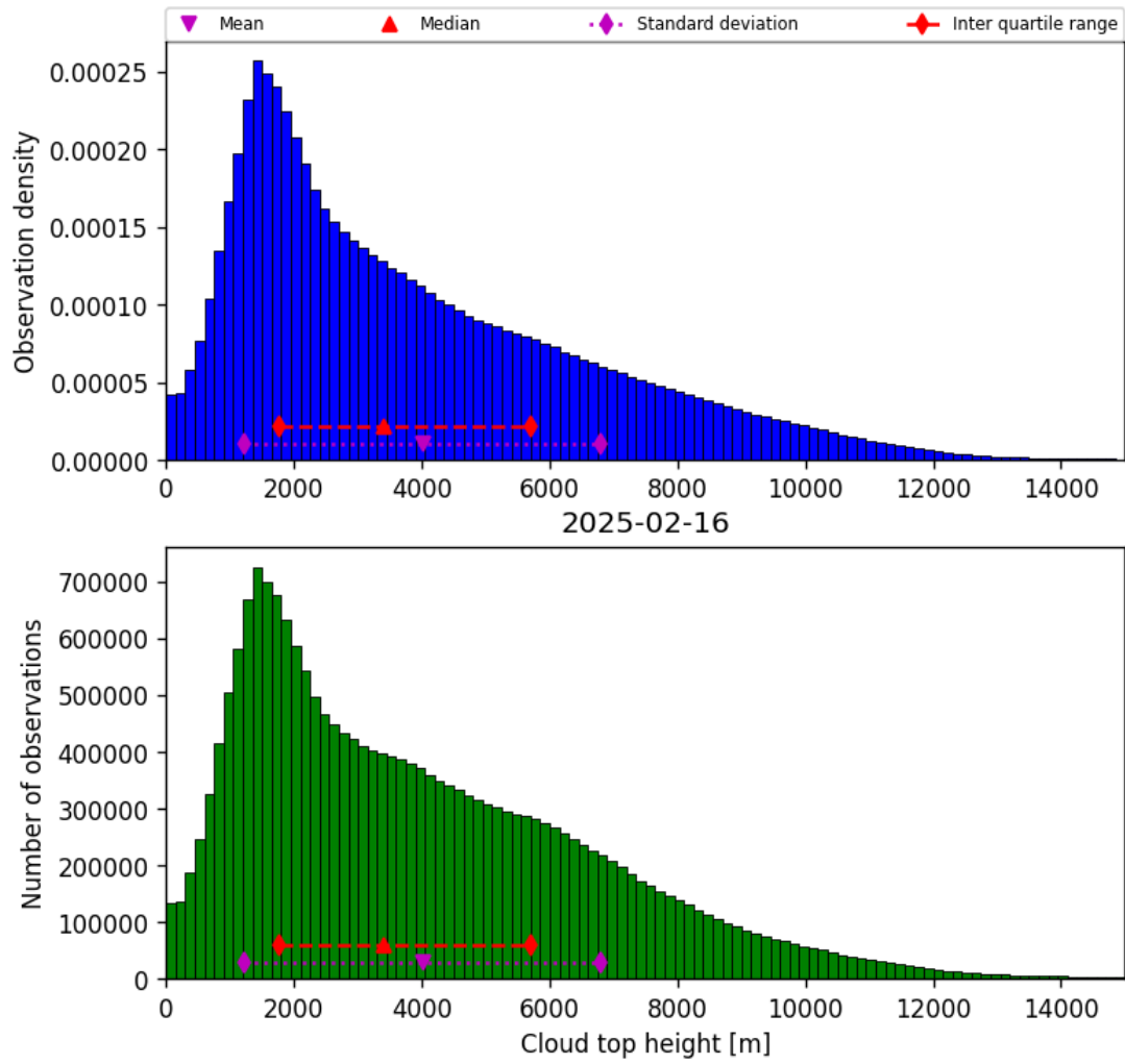
Figure 40: Histogram of “Cloud top height” for 2025-02-15 to 2025-02-17
