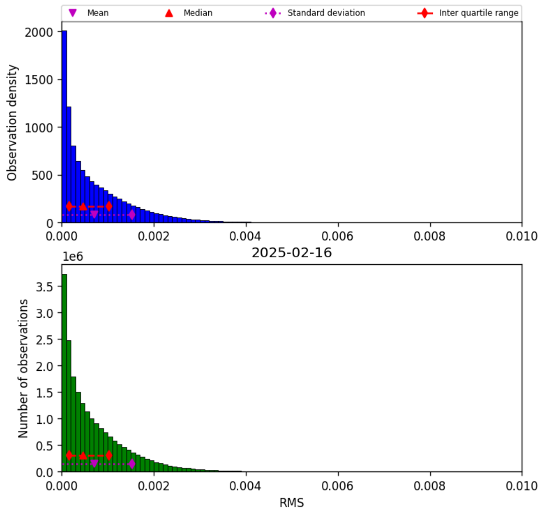
Figure 47: Histogram of “RMS” for 2025-02-15 to 2025-02-17
