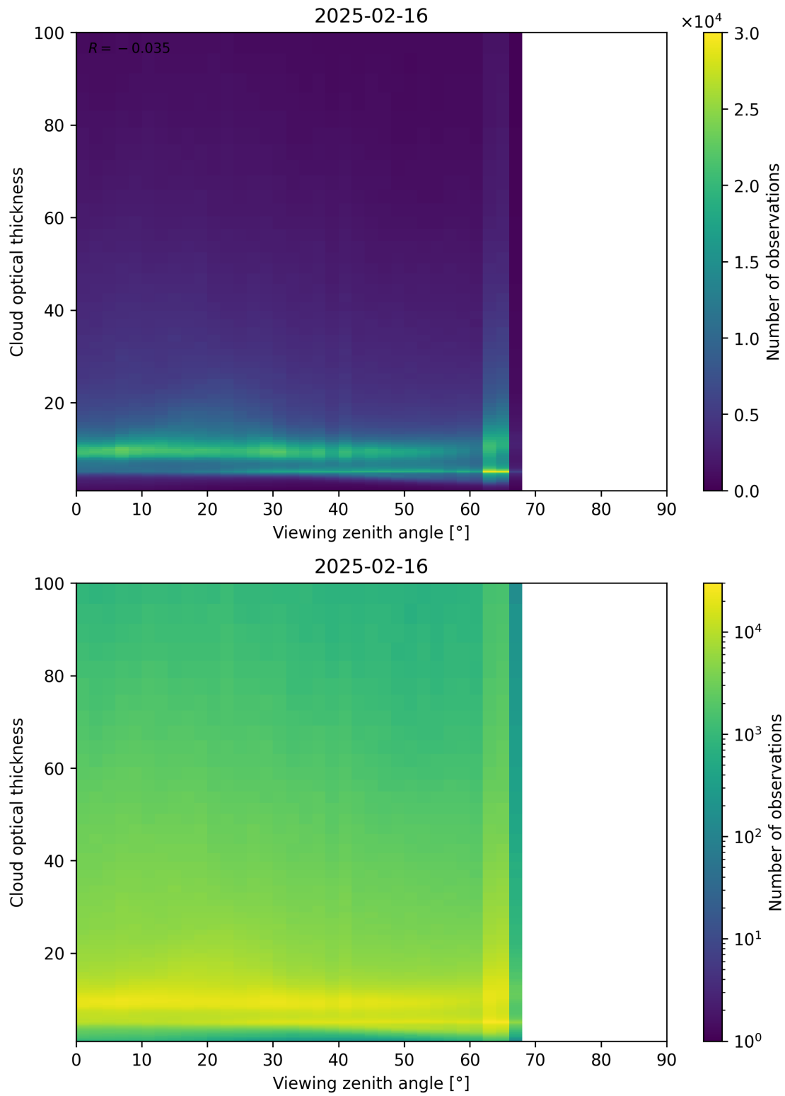
Figure 111: Scatter density plot of “Viewing zenith angle” against “Cloud optical thickness” for 2025-02-15 to 2025-02-17.
