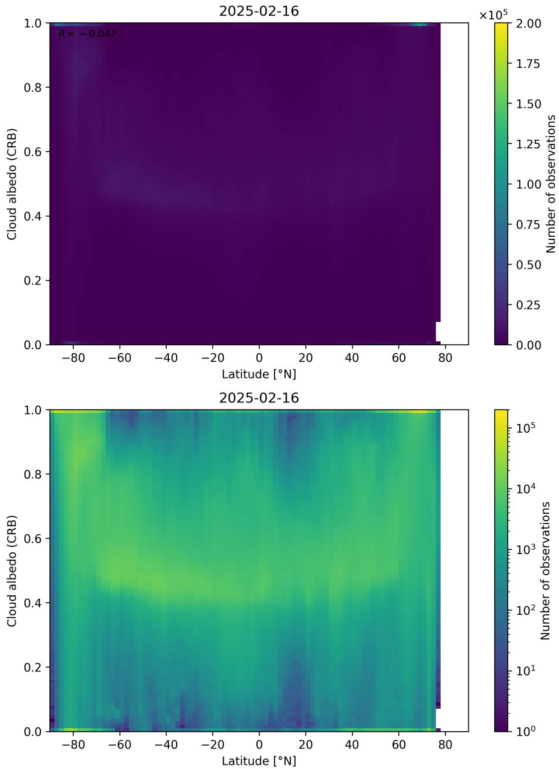
Figure 91: Scatter density plot of “Latitude” against “Cloud albedo (CRB)” for 2025-02-15 to 2025-02-17.
