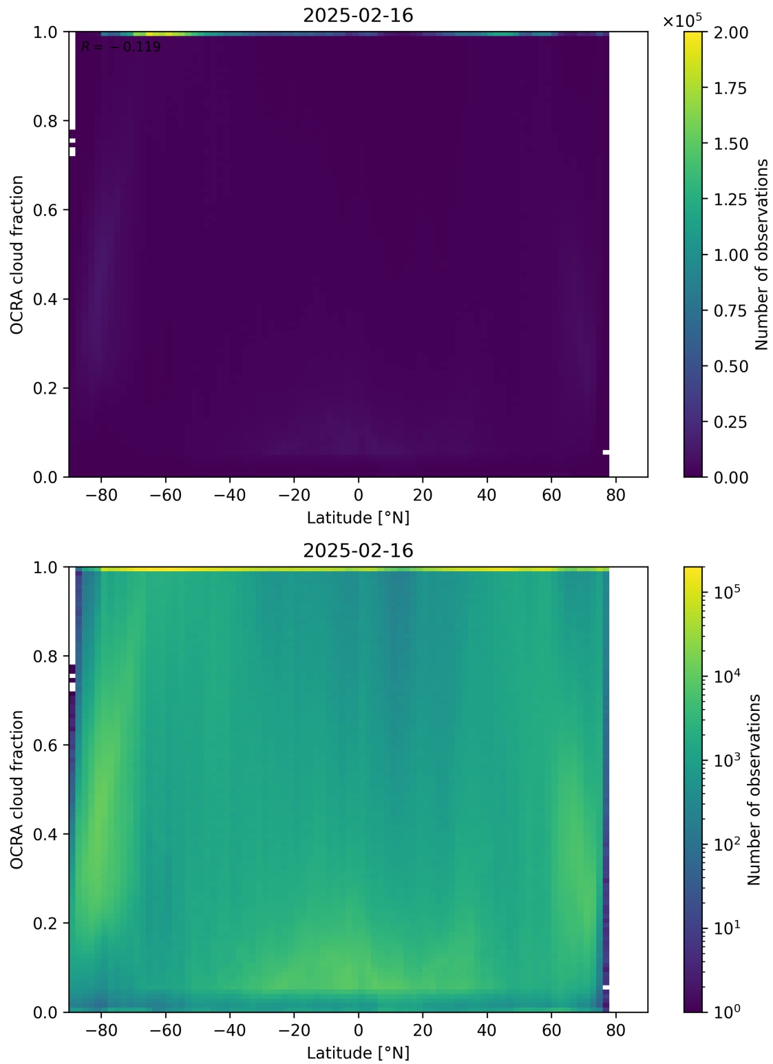
Figure 93: Scatter density plot of “Latitude” against “OCRA cloud fraction” for 2025-02-15 to 2025-02-17.
