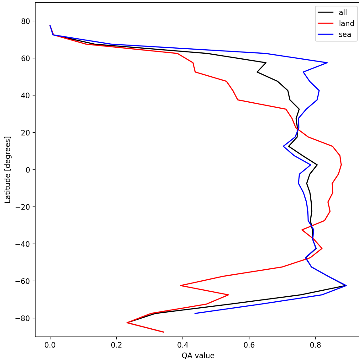
Figure 22: Zonal average of “QA value” for 2025-02-15 to 2025-02-17.
