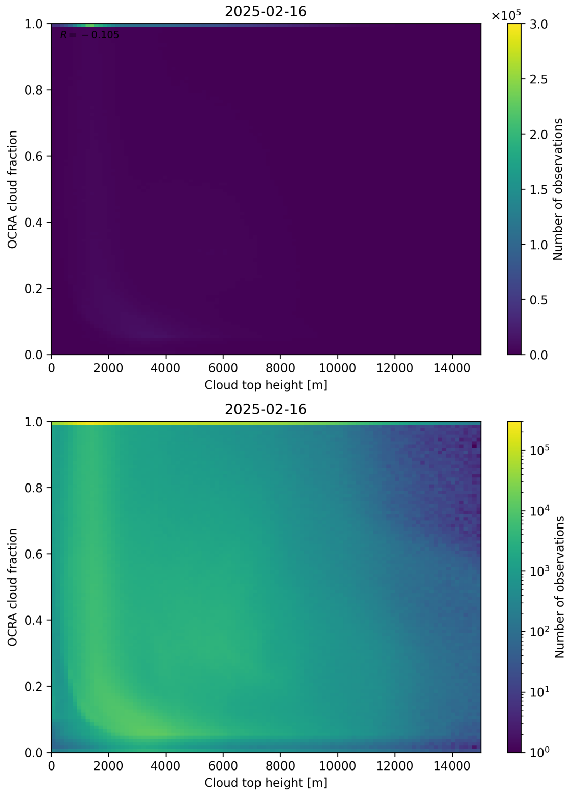
Figure 87: Scatter density plot of “Cloud top height” against “OCRA cloud fraction” for 2025-02-15 to 2025-02-17.
