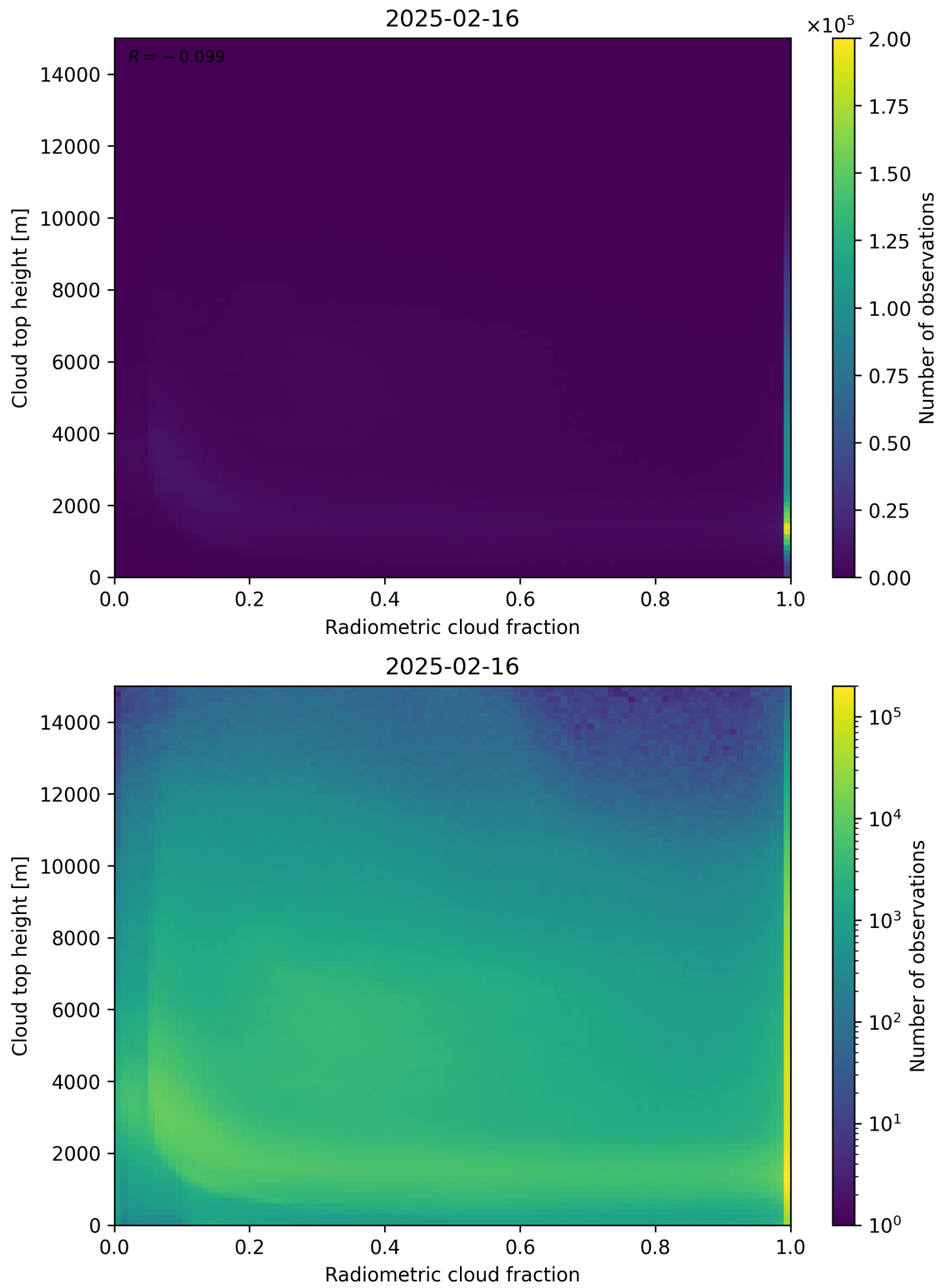
Figure 76: Scatter density plot of “Radiometric cloud fraction” against “Cloud top height” for 2025-02-15 to 2025-02-17.
