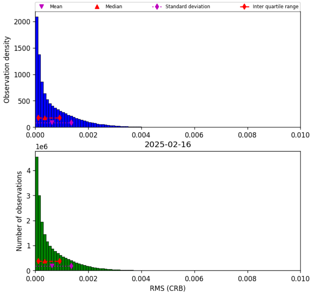
Figure 48: Histogram of “RMS (CRB)” for 2025-02-15 to 2025-02-17
