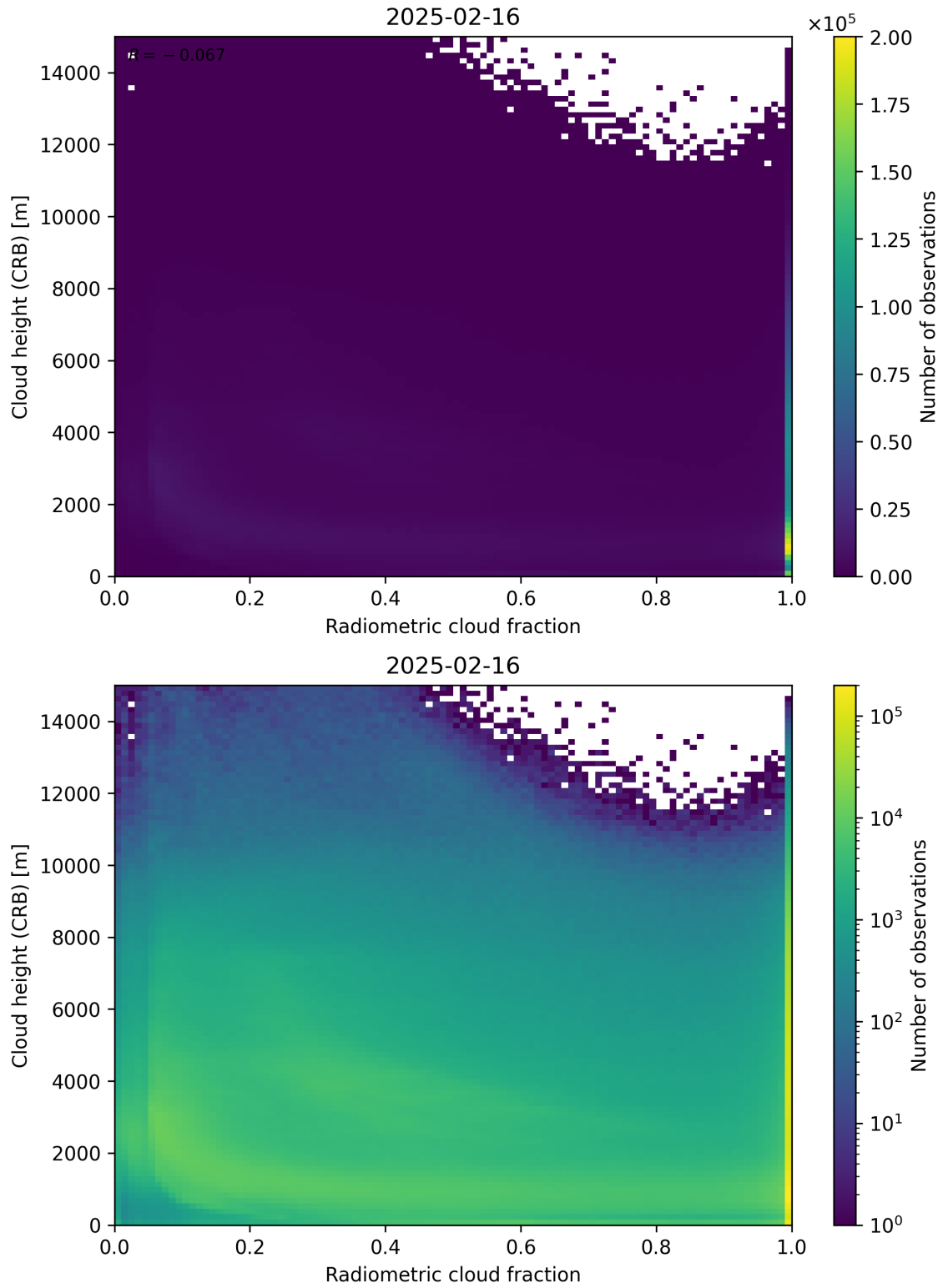
Figure 74: Scatter density plot of “Radiometric cloud fraction” against “Cloud height (CRB)” for 2025-02-15 to 2025-02-17.
