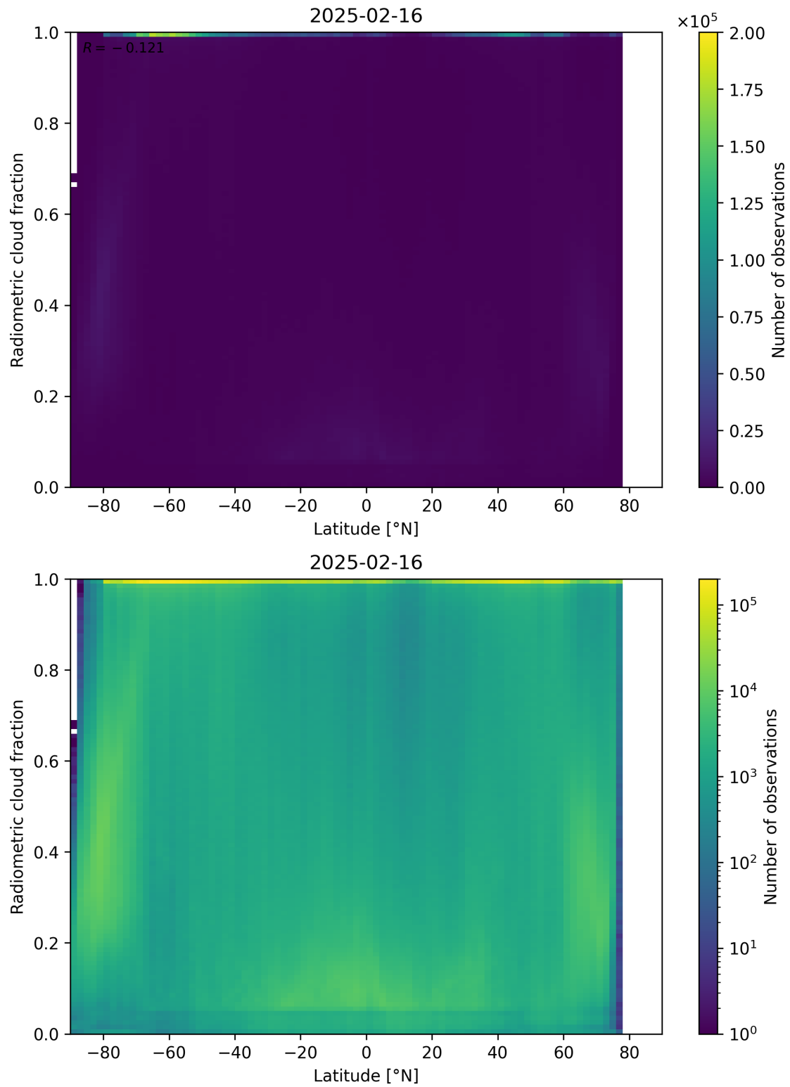
Figure 92: Scatter density plot of “Latitude” against “Radiometric cloud fraction” for 2025-02-15 to 2025-02-17.
