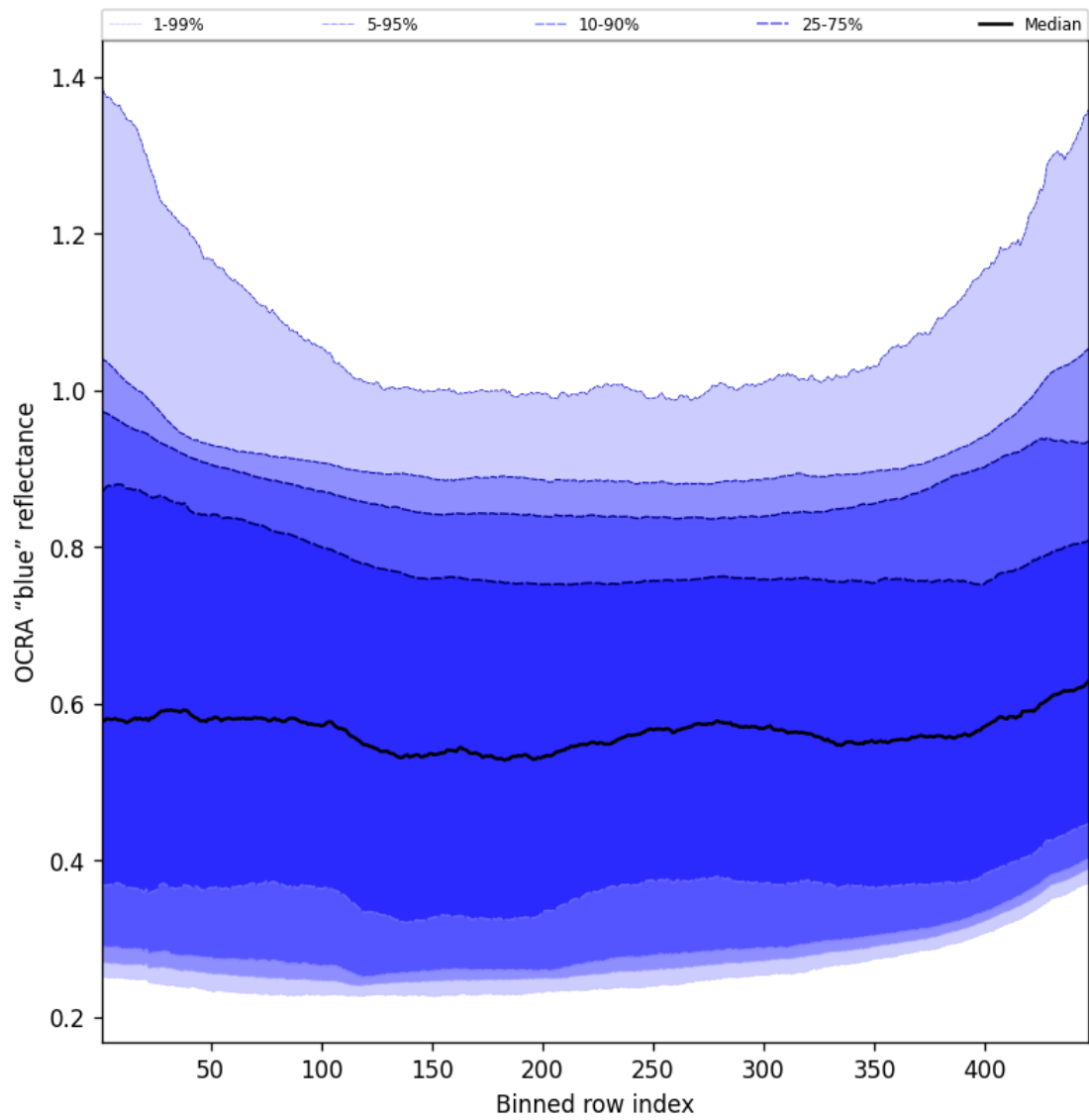
Figure 67: Along track statistics of “OCRA “blue” reflectance” for 2025-02-15 to 2025-02-17
