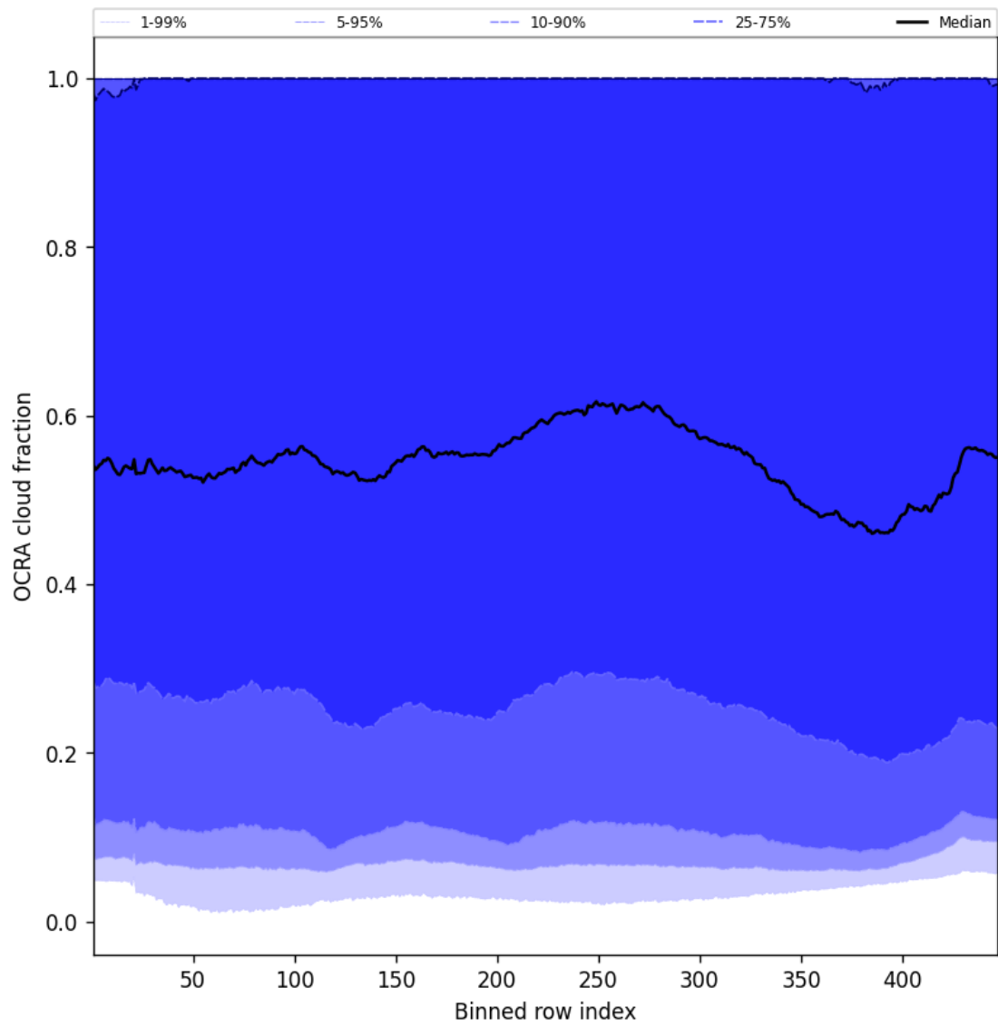
Figure 66: Along track statistics of “OCRA cloud fraction” for 2025-02-15 to 2025-02-17
