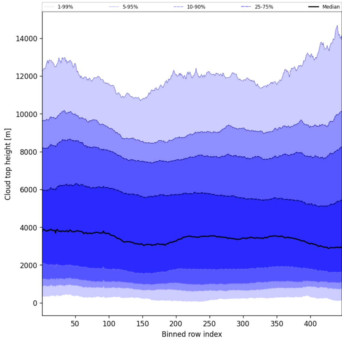
Figure 56: Along track statistics of “Cloud top height” for 2025-02-15 to 2025-02-17
