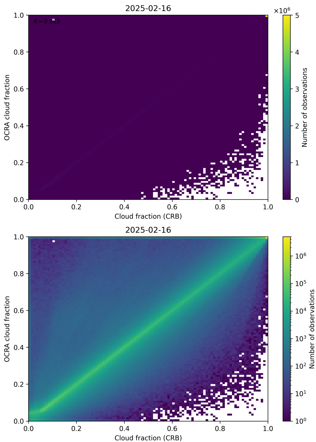
Figure 78: Scatter density plot of “Cloud fraction (CRB)” against “OCRA cloud fraction” for 2025-02-15 to 2025-02-17.
