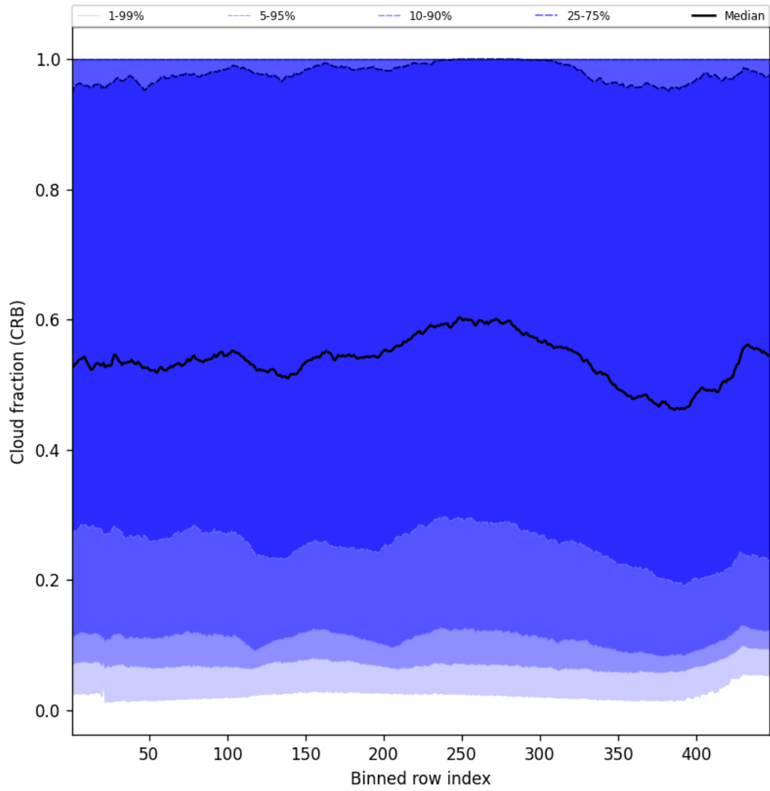
Figure 58: Along track statistics of “Cloud fraction (CRB)” for 2025-02-15 to 2025-02-17
