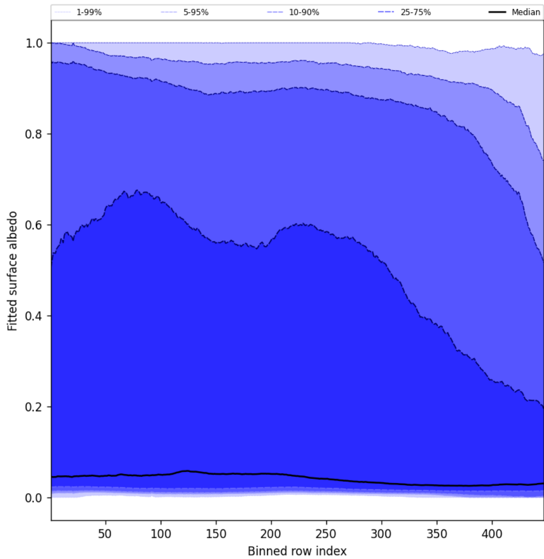
Figure 61: Along track statistics of “Fitted surface albedo” for 2025-02-15 to 2025-02-17
