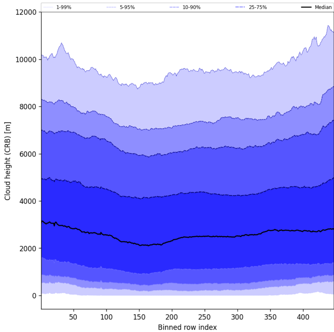
Figure 59: Along track statistics of “Cloud height (CRB)” for 2025-02-15 to 2025-02-17
