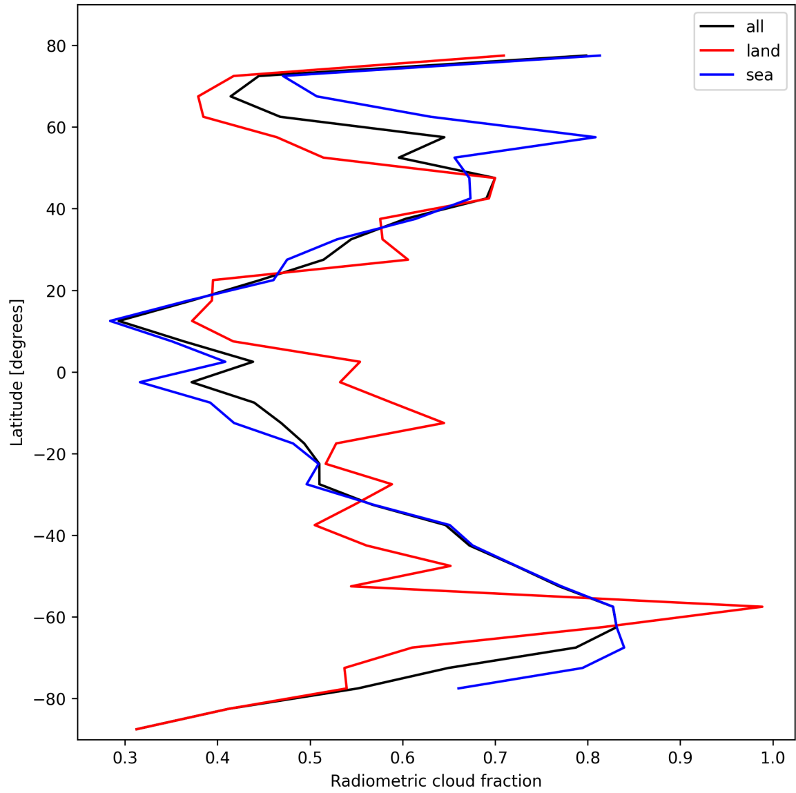
Figure 23: Zonal average of “Radiometric cloud fraction” for 2025-02-15 to 2025-02-17.
