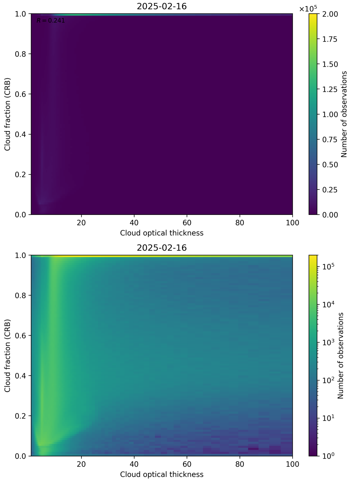
Figure 84: Scatter density plot of “Cloud optical thickness” against “Cloud fraction (CRB)” for 2025-02-15 to 2025-02-17.
