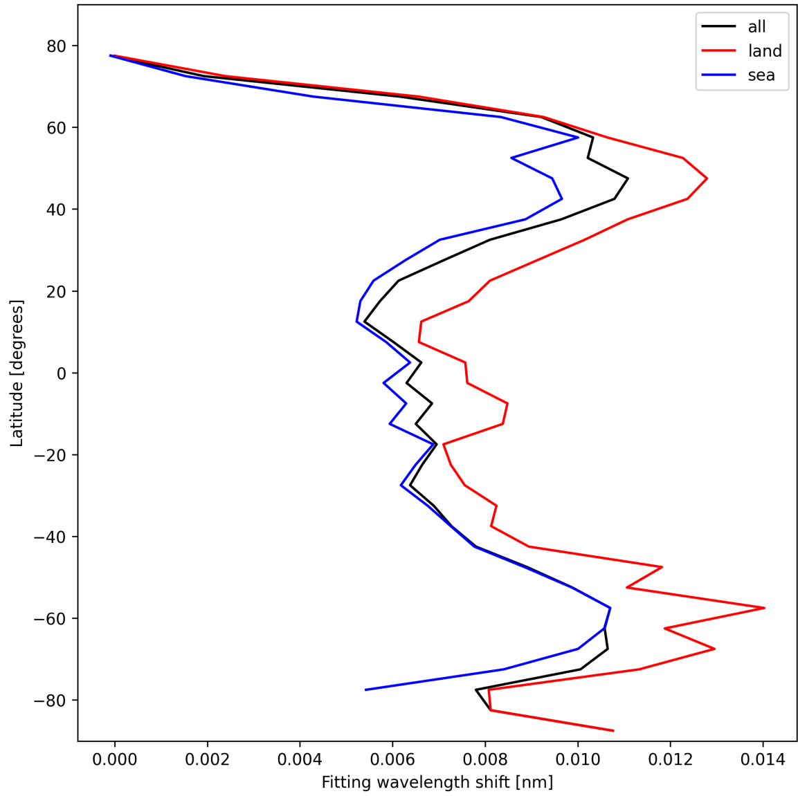
Figure 33: Zonal average of “Fitting wavelength shift” for 2025-02-15 to 2025-02-17.
