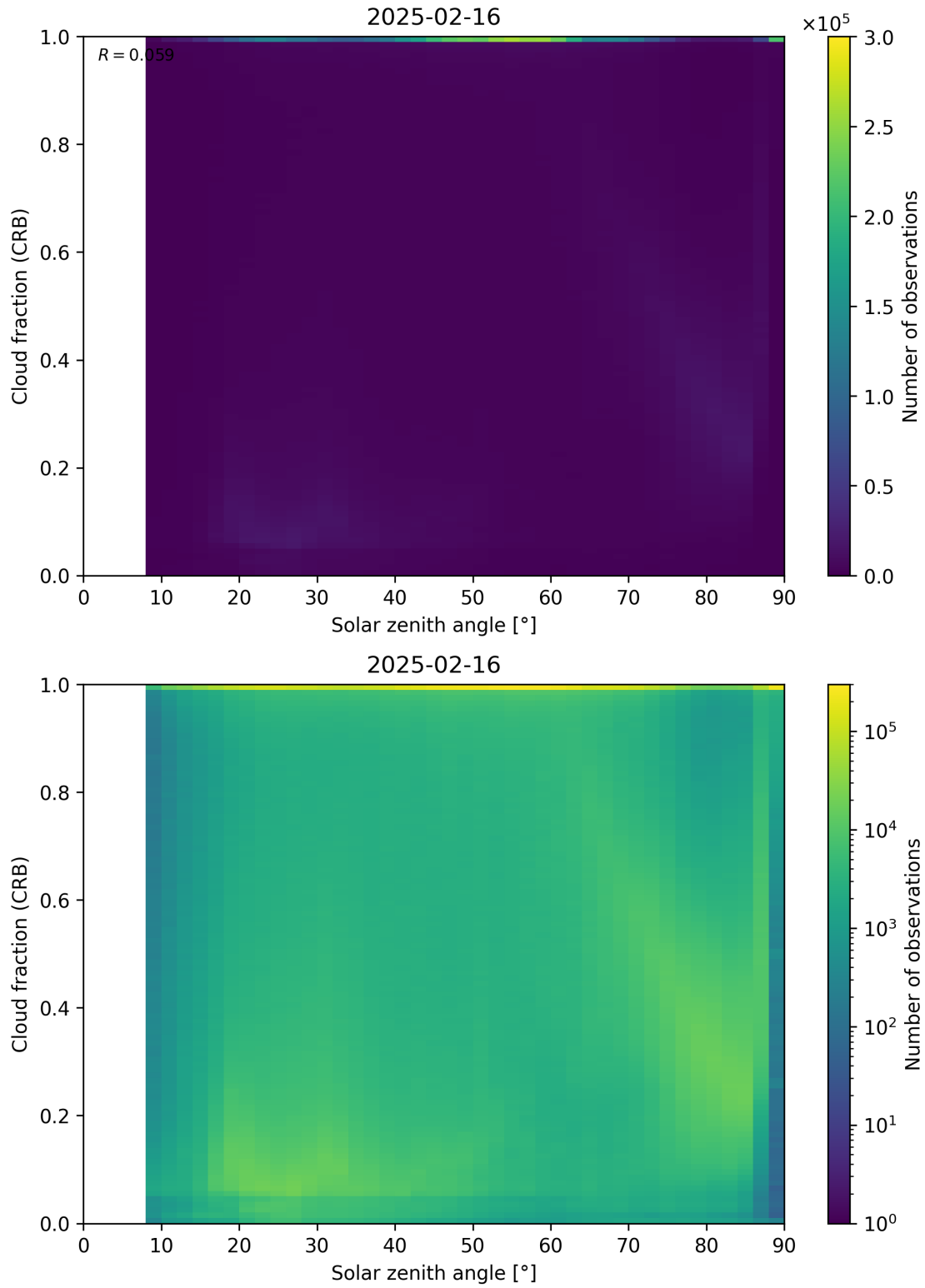
Figure 101: Scatter density plot of “Solar zenith angle” against “Cloud fraction (CRB)” for 2025-02-15 to 2025-02-17.
