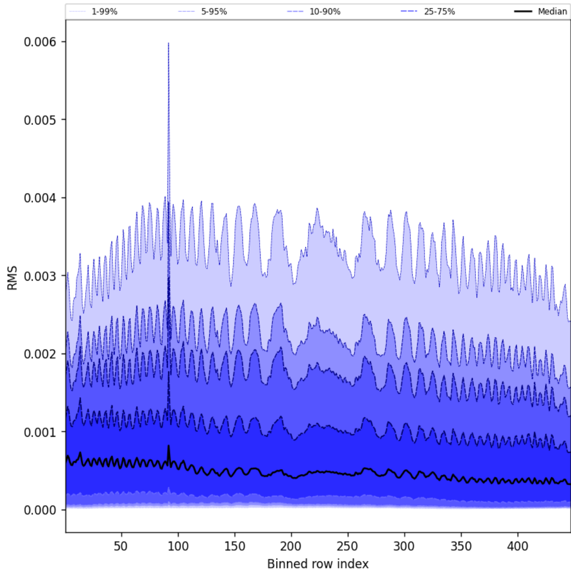
Figure 63: Along track statistics of “RMS” for 2025-02-15 to 2025-02-17
