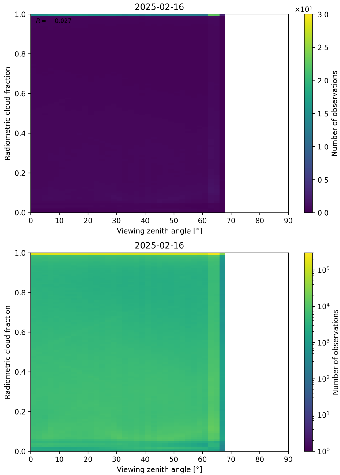
Figure 107: Scatter density plot of “Viewing zenith angle” against “Radiometric cloud fraction” for 2025-02-15 to 2025-02-17.
