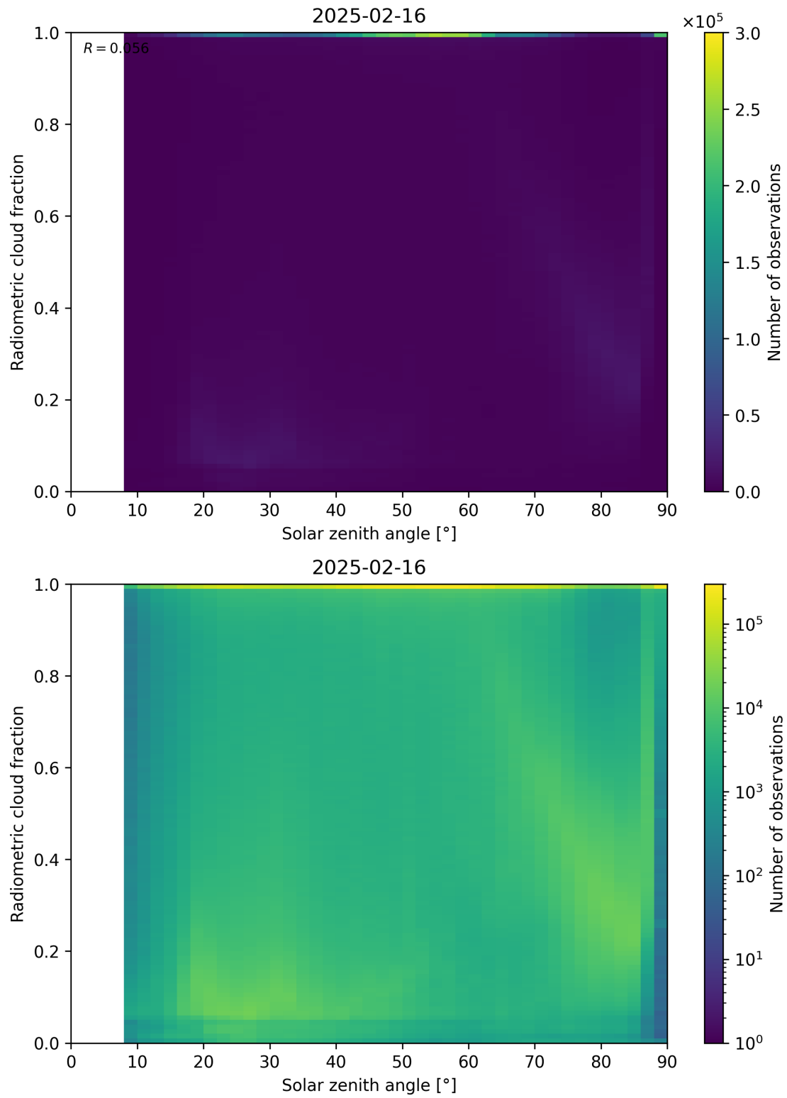
Figure 99: Scatter density plot of “Solar zenith angle” against “Radiometric cloud fraction” for 2025-02-15 to 2025-02-17.
