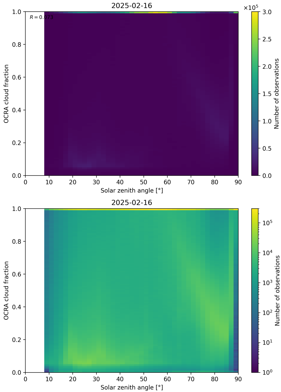
Figure 100: Scatter density plot of “Solar zenith angle” against “OCRA cloud fraction” for 2025-02-15 to 2025-02-17.
