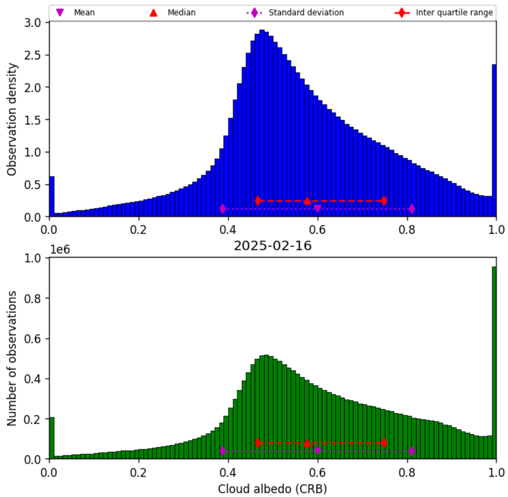
Figure 44: Histogram of “Cloud albedo (CRB)” for 2025-02-15 to 2025-02-17
