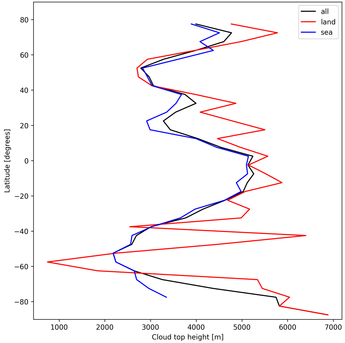
Figure 24: Zonal average of “Cloud top height” for 2025-02-15 to 2025-02-17.
