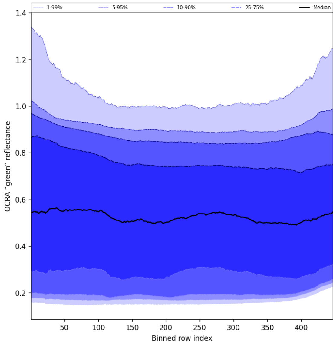
Figure 68: Along track statistics of "OCRA "green" reflectance" for 2025-02-15 to 2025-02-17
