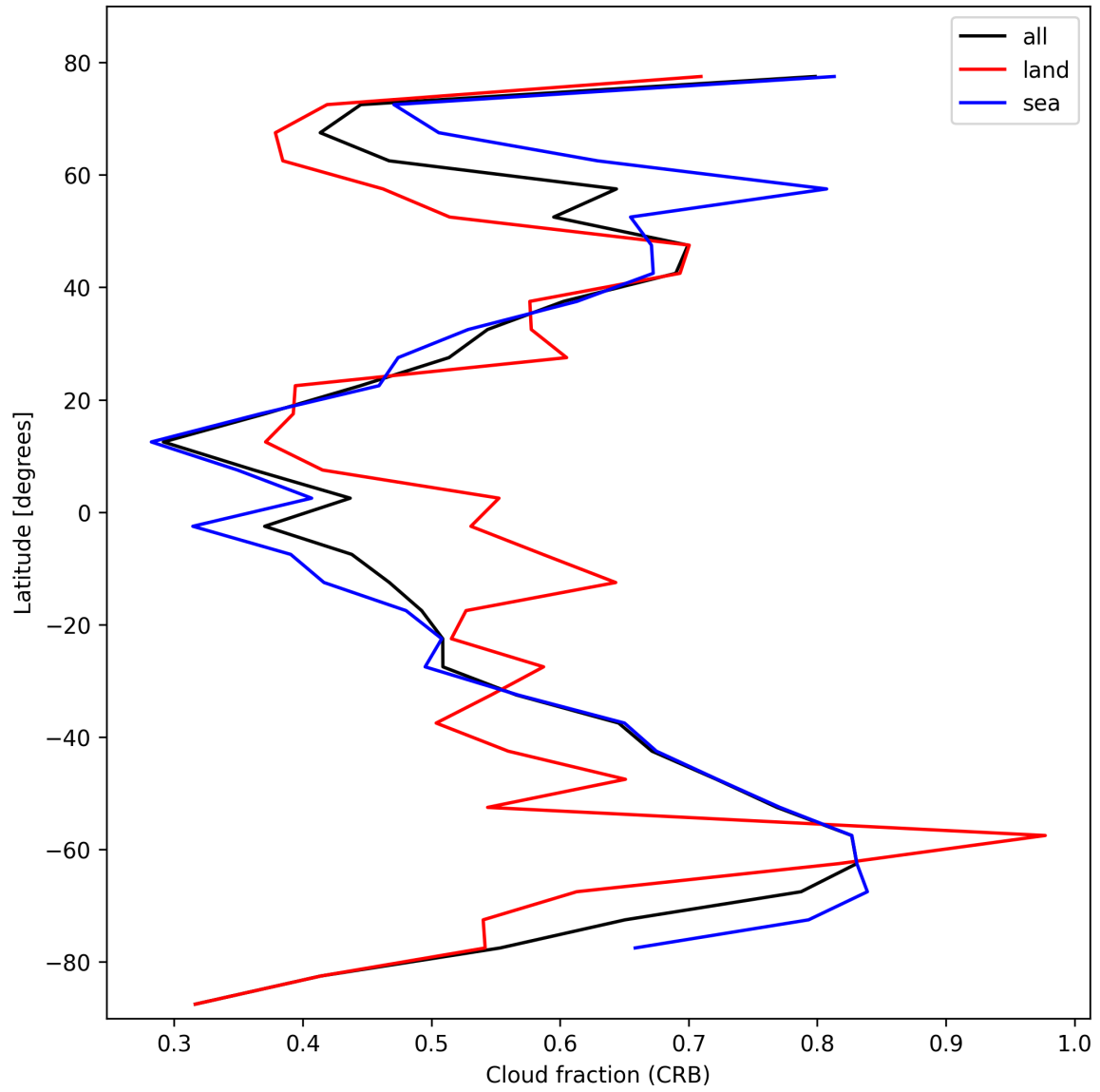
Figure 26: Zonal average of “Cloud fraction (CRB)” for 2025-02-15 to 2025-02-17.
