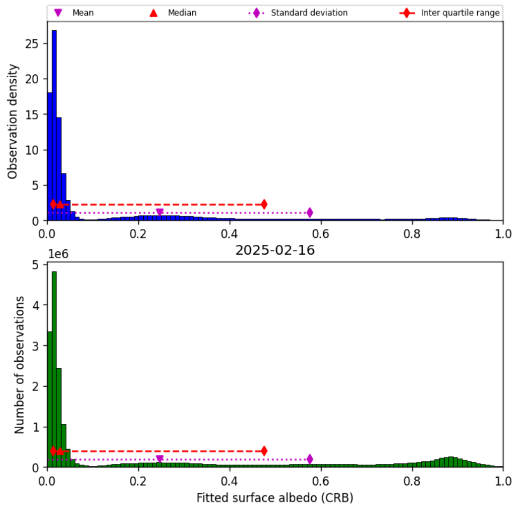
Figure 46: Histogram of “Fitted surface albedo (CRB)” for 2025-02-15 to 2025-02-17
