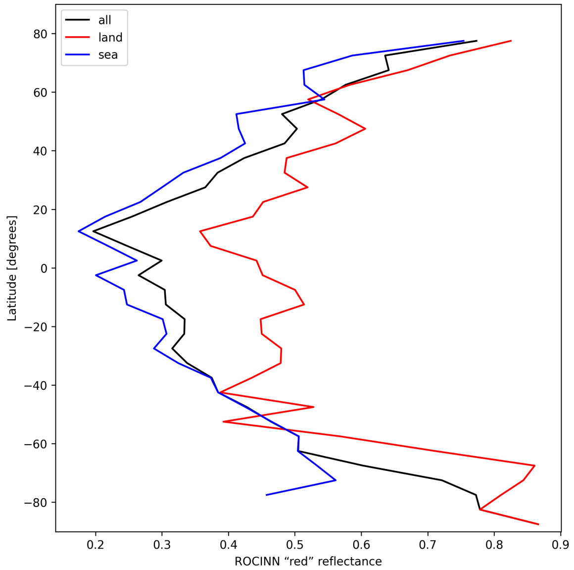
Figure 37: Zonal average of “ROCINN “red” reflectance” for 2025-02-15 to 2025-02-17.
