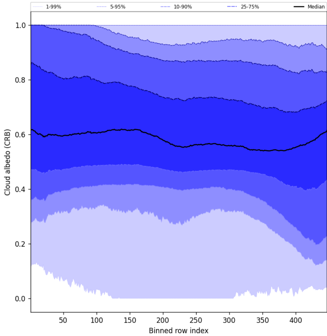
Figure 60: Along track statistics of “Cloud albedo (CRB)” for 2025-02-15 to 2025-02-17
