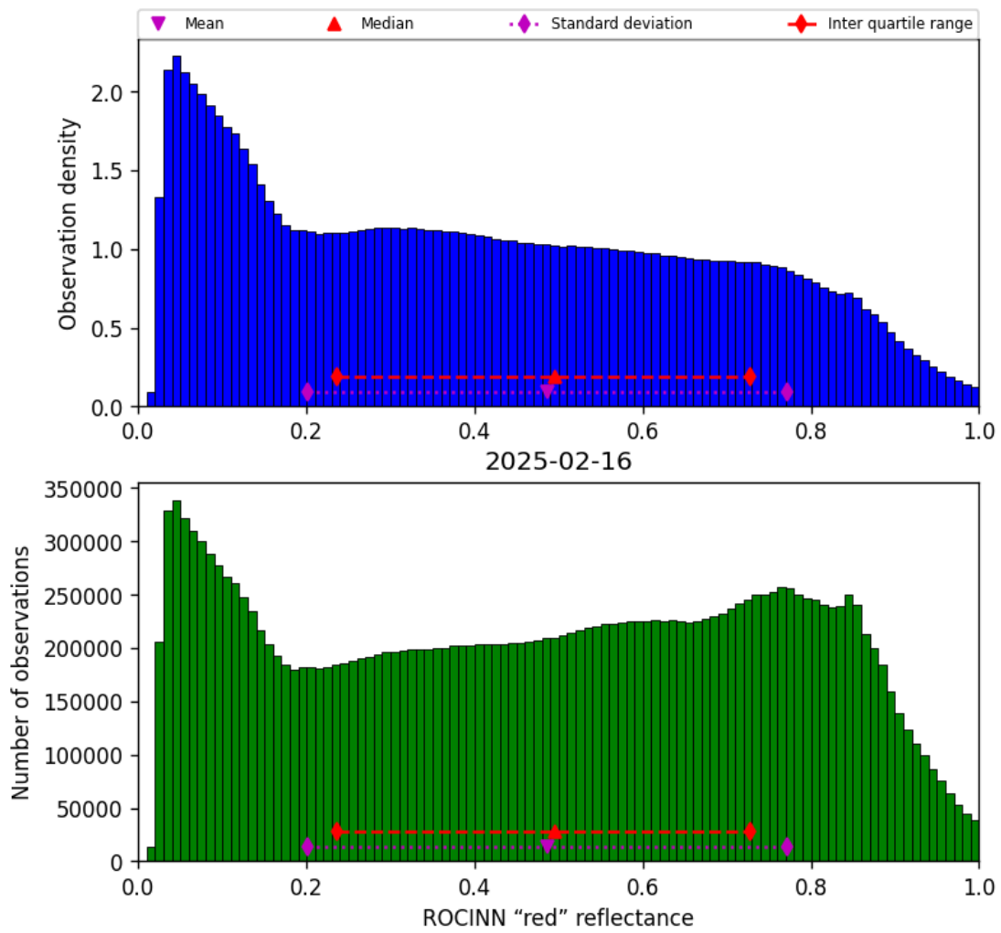
Figure 53: Histogram of “ROCINN “red” reflectance” for 2025-02-15 to 2025-02-17
