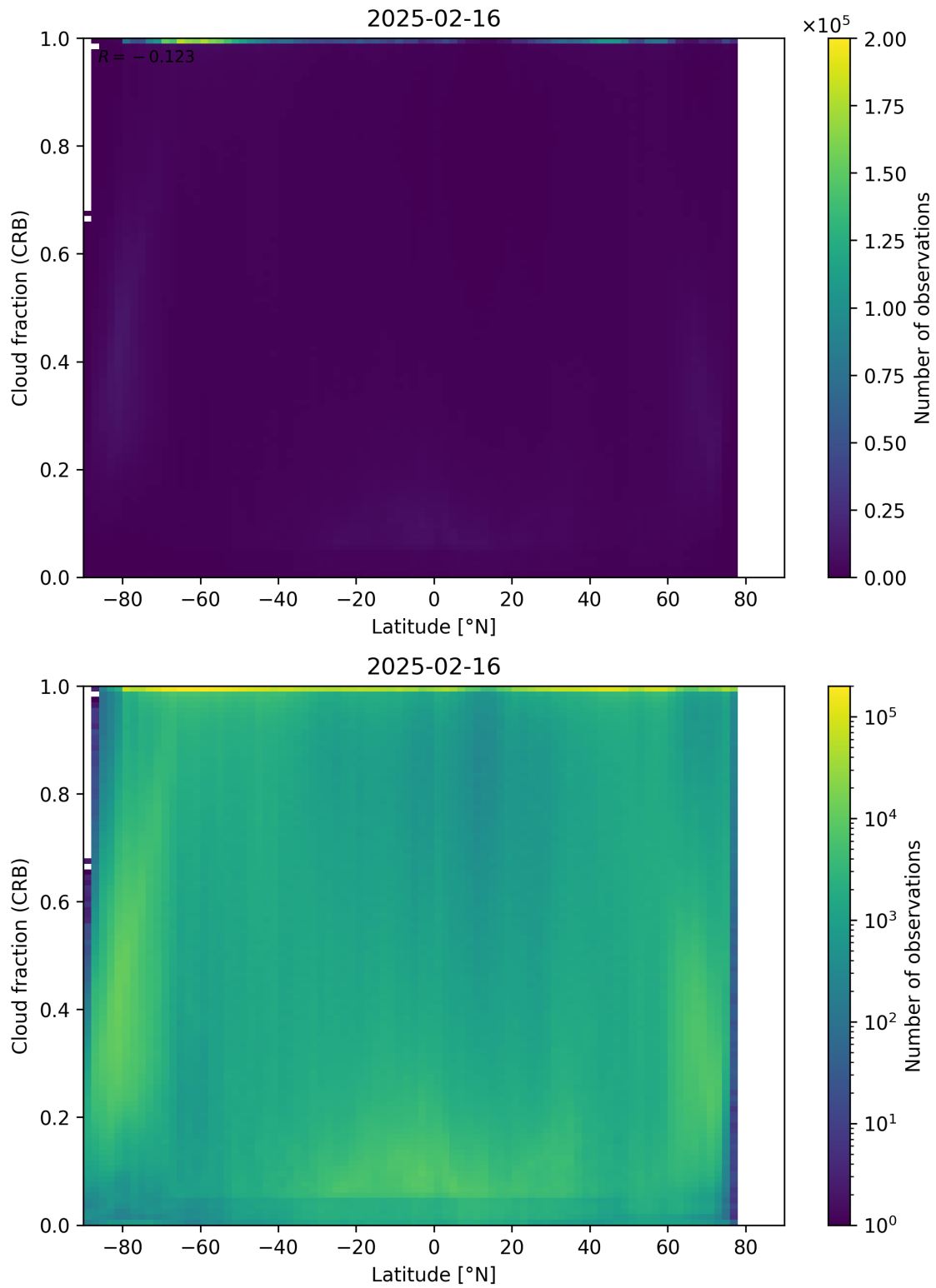
Figure 94: Scatter density plot of “Latitude” against “Cloud fraction (CRB)” for 2025-02-15 to 2025-02-17.
