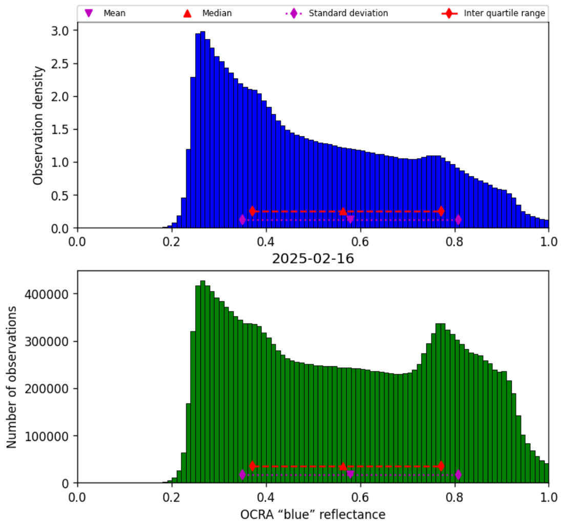
Figure 51: Histogram of “OCRA “blue” reflectance” for 2025-02-15 to 2025-02-17
