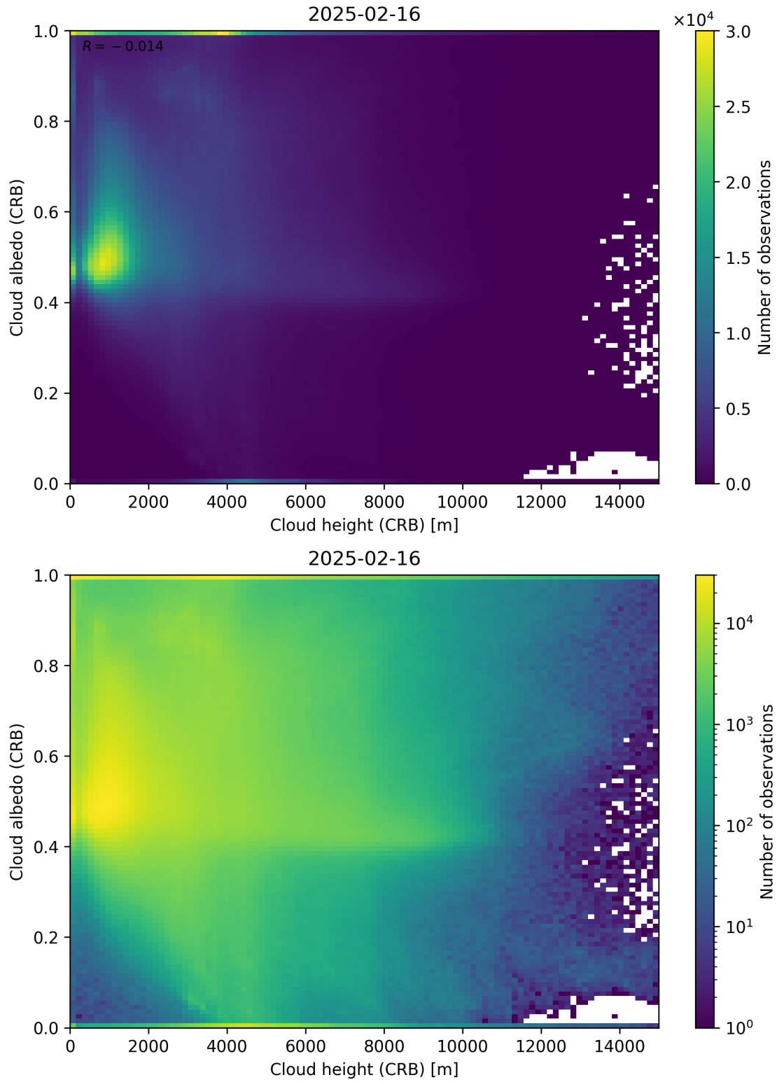
Figure 80: Scatter density plot of “Cloud height (CRB)” against “Cloud albedo (CRB)” for 2025-02-15 to 2025-02-17.
