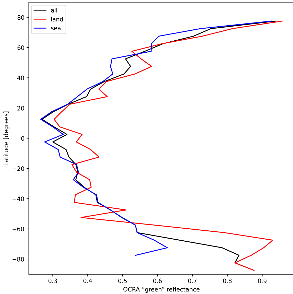
Figure 36: Zonal average of “OCRA “green” reflectance” for 2025-02-15 to 2025-02-17.
