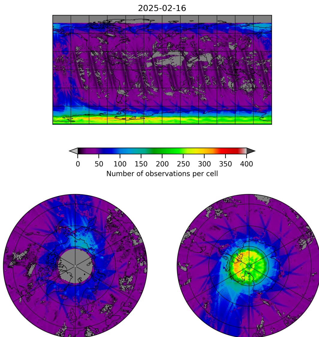
Figure 21: Map of the number of observations for 2025-02-15 to 2025-02-17
