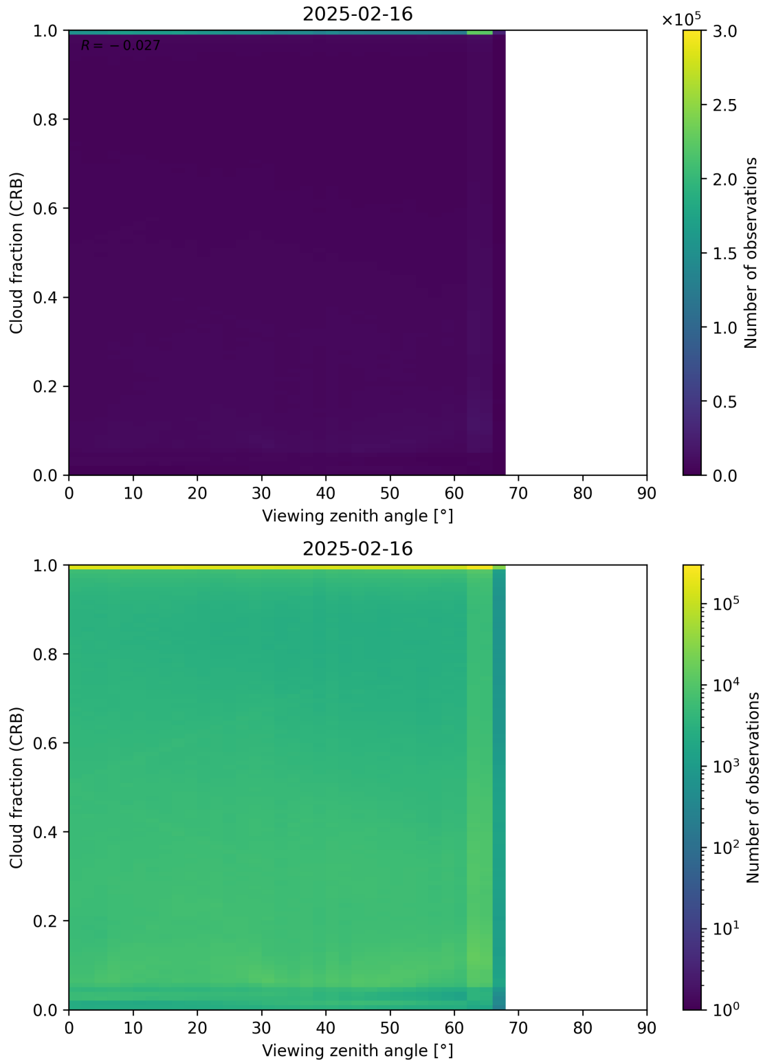
Figure 109: Scatter density plot of “Viewing zenith angle” against “Cloud fraction (CRB)” for 2025-02-15 to 2025-02-17.
