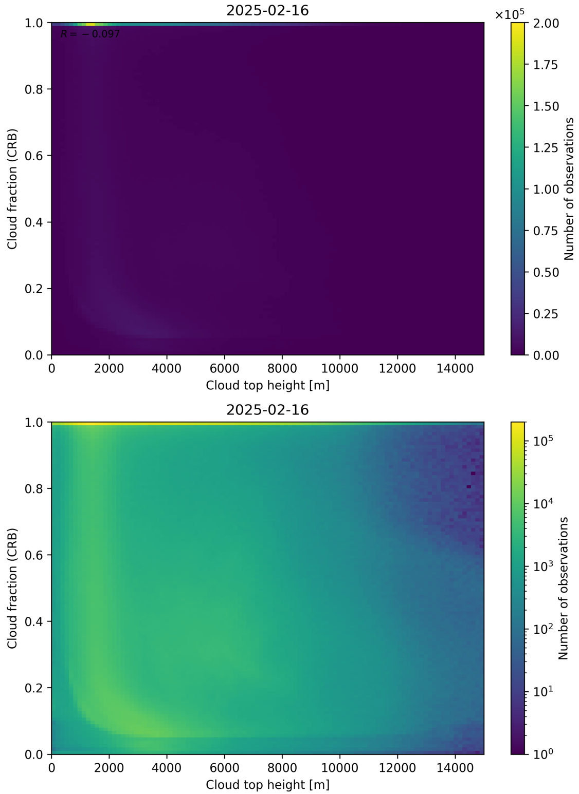
Figure 88: Scatter density plot of “Cloud top height” against “Cloud fraction (CRB)” for 2025-02-15 to 2025-02-17.
