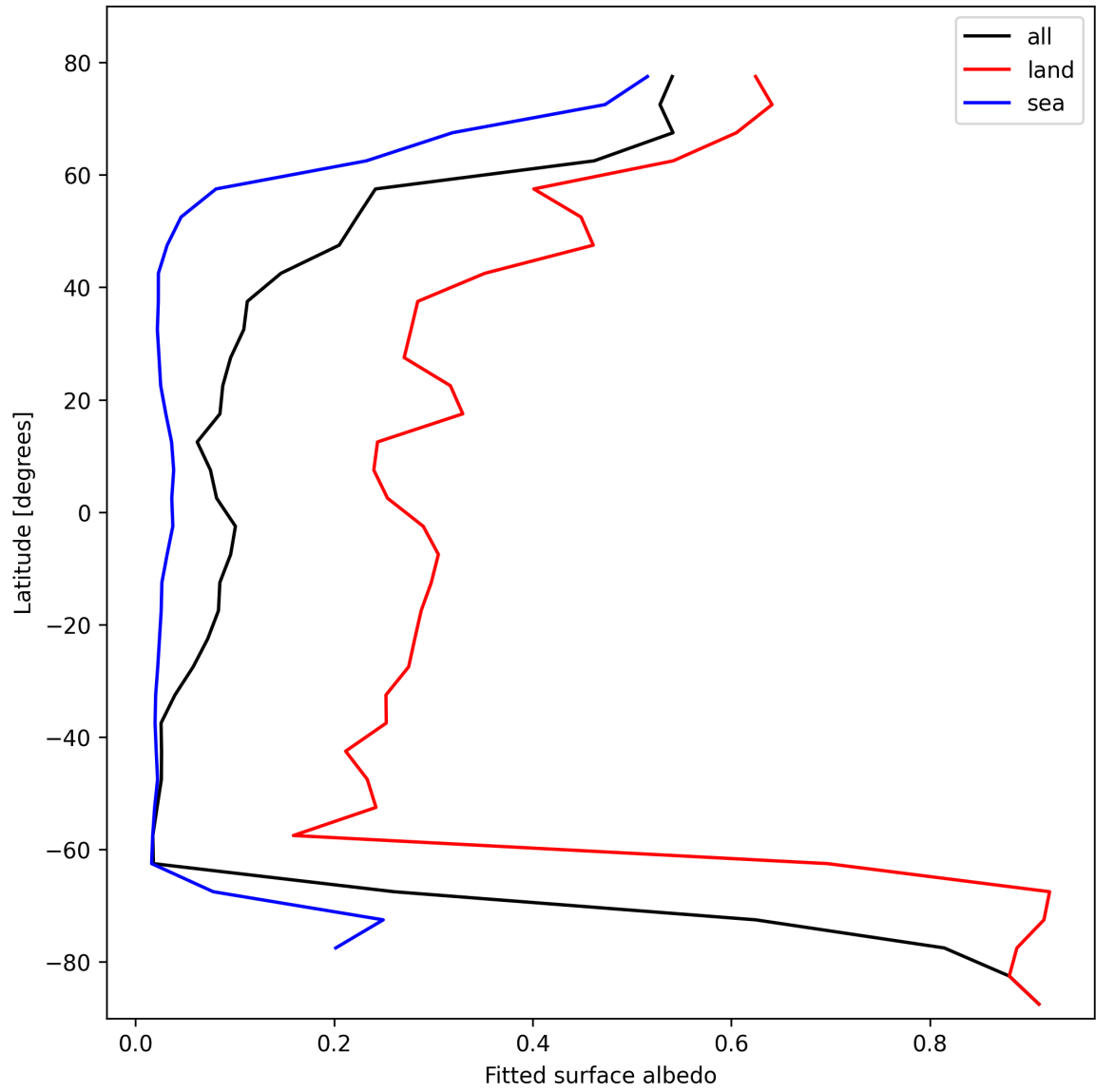
Figure 29: Zonal average of “Fitted surface albedo” for 2025-02-15 to 2025-02-17.
