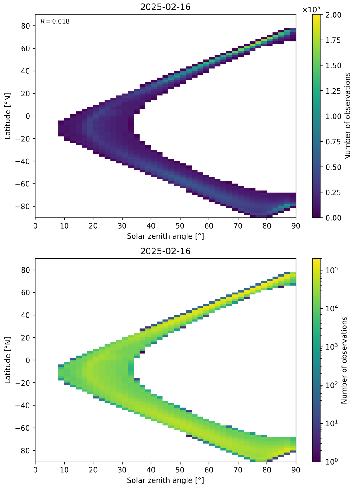
Figure 105: Scatter density plot of “Solar zenith angle” against “Latitude” for 2025-02-15 to 2025-02-17.
