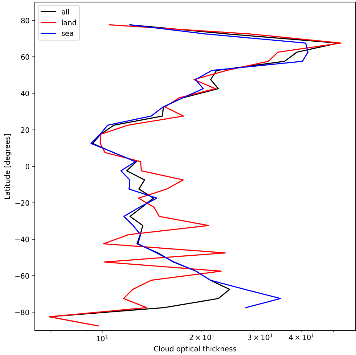
Figure 25: Zonal average of “Cloud optical thickness” for 2025-02-15 to 2025-02-17.
