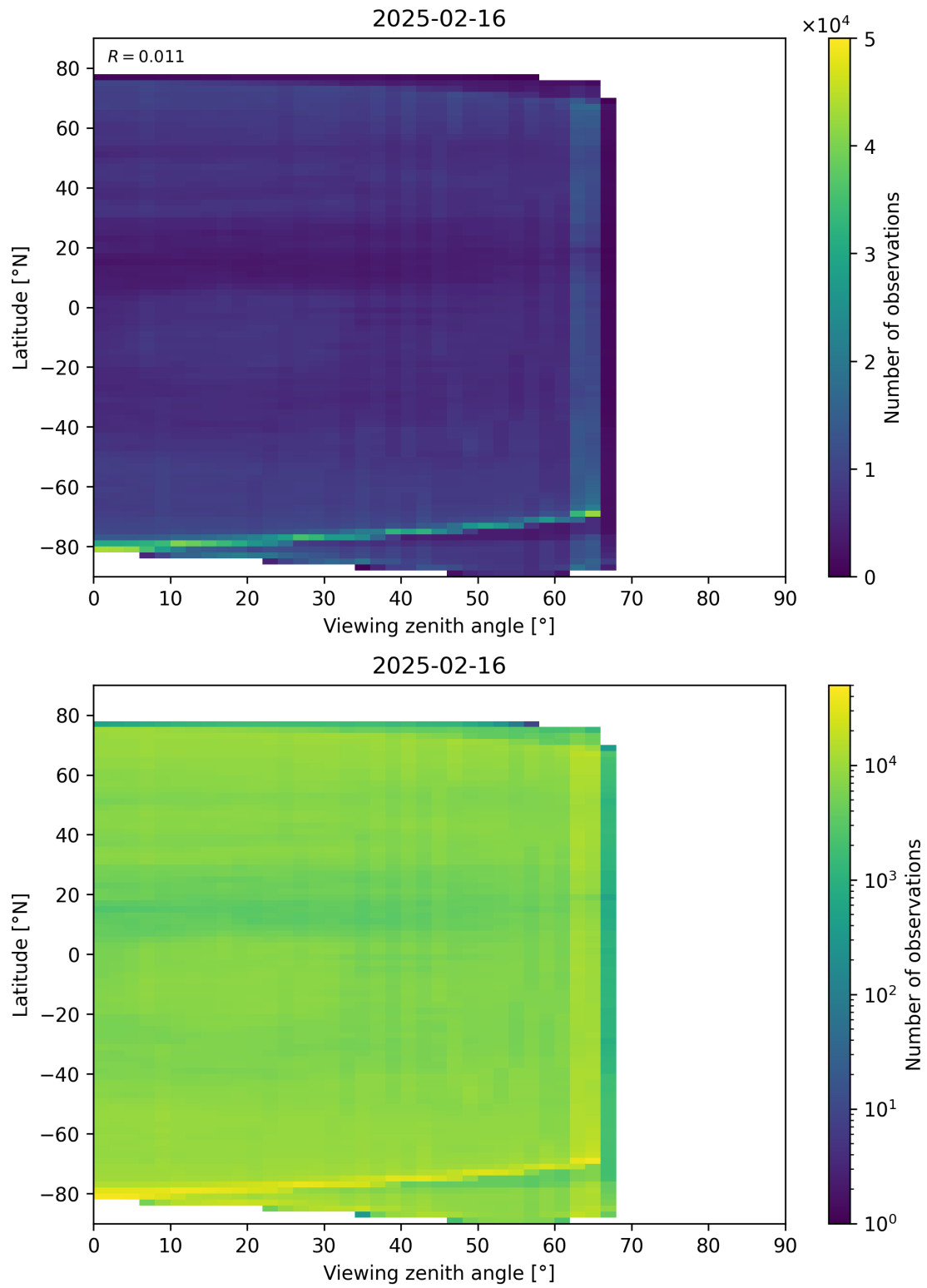
Figure 113: Scatter density plot of “Viewing zenith angle” against “Latitude” for 2025-02-15 to 2025-02-17.
