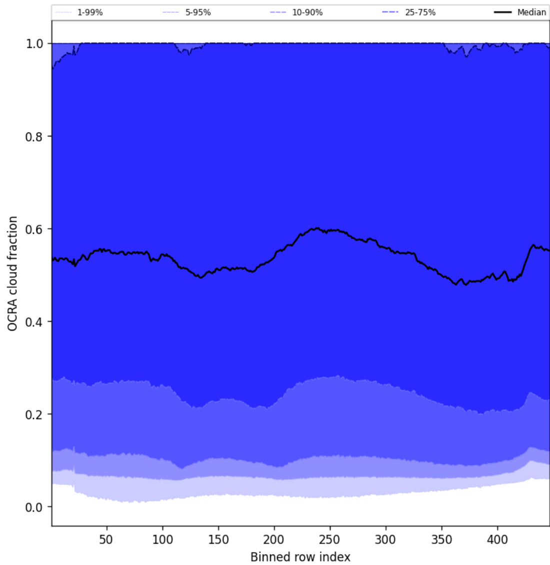
Figure 66: Along track statistics of “OCRA cloud fraction” for 2025-02-16 to 2025-02-18
