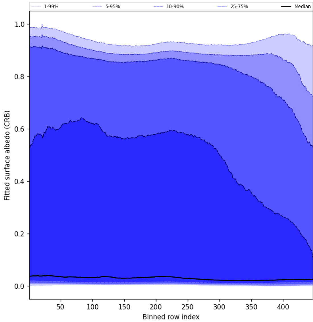
Figure 62: Along track statistics of “Fitted surface albedo (CRB)” for 2025-02-16 to 2025-02-18
