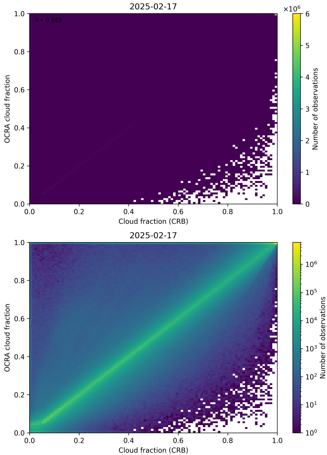
Figure 78: Scatter density plot of “Cloud fraction (CRB)” against “OCRA cloud fraction” for 2025-02-16 to 2025-02-18.
