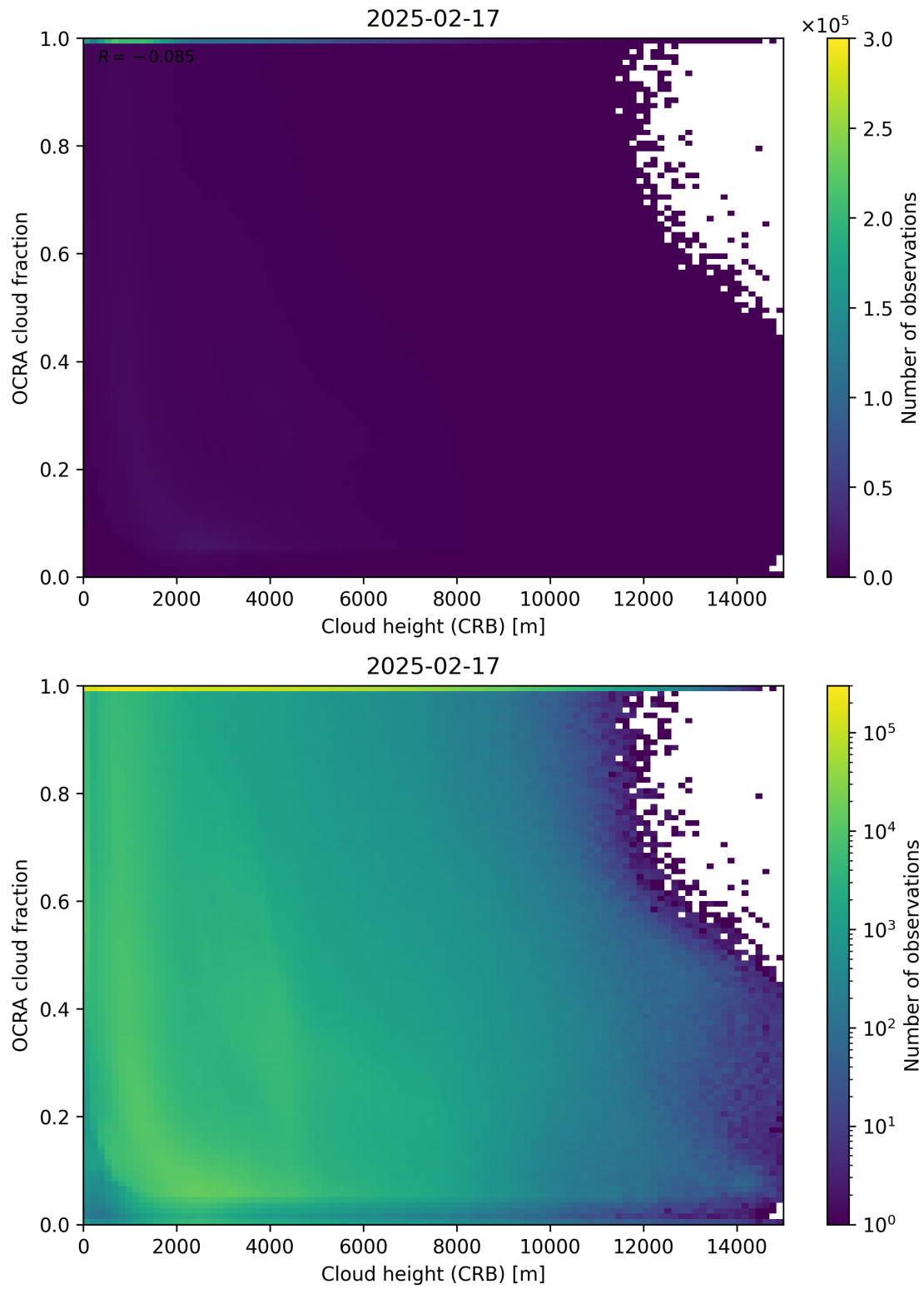
Figure 81: Scatter density plot of “Cloud height (CRB)” against “OCRA cloud fraction” for 2025-02-16 to 2025-02-18.
