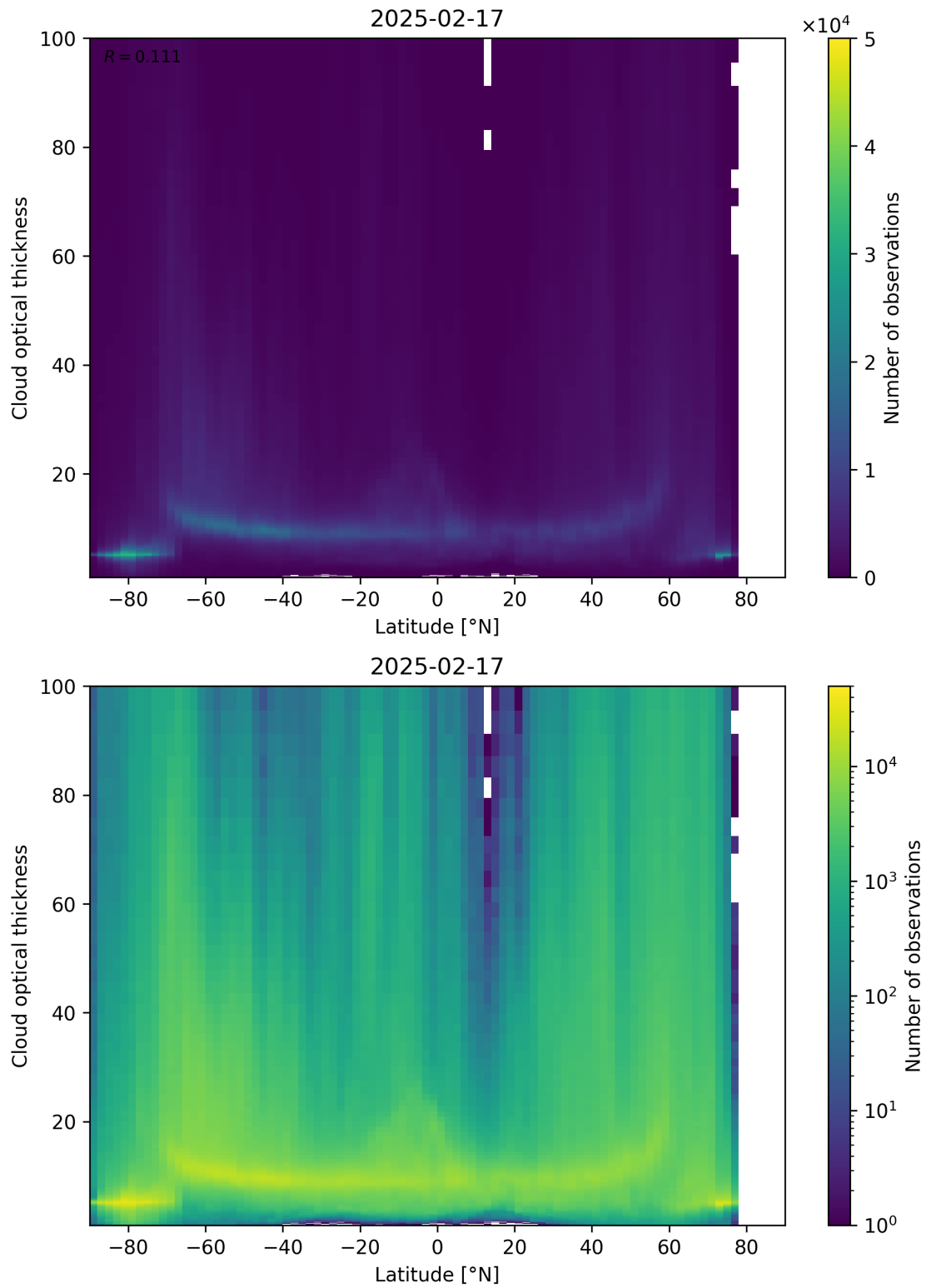
Figure 96: Scatter density plot of “Latitude” against “Cloud optical thickness” for 2025-02-16 to 2025-02-18.
