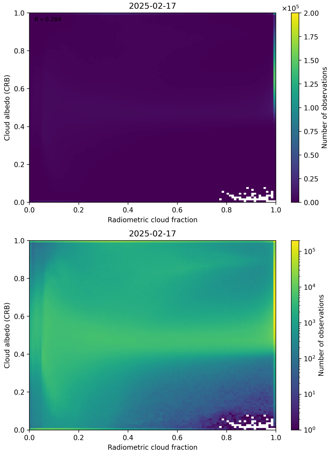
Figure 71: Scatter density plot of “Radiometric cloud fraction” against “Cloud albedo (CRB)” for 2025-02-16 to 2025-02-18.
