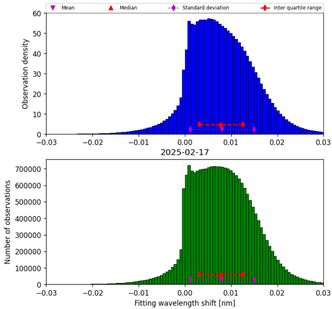
Figure 49: Histogram of “Fitting wavelength shift” for 2025-02-16 to 2025-02-18
