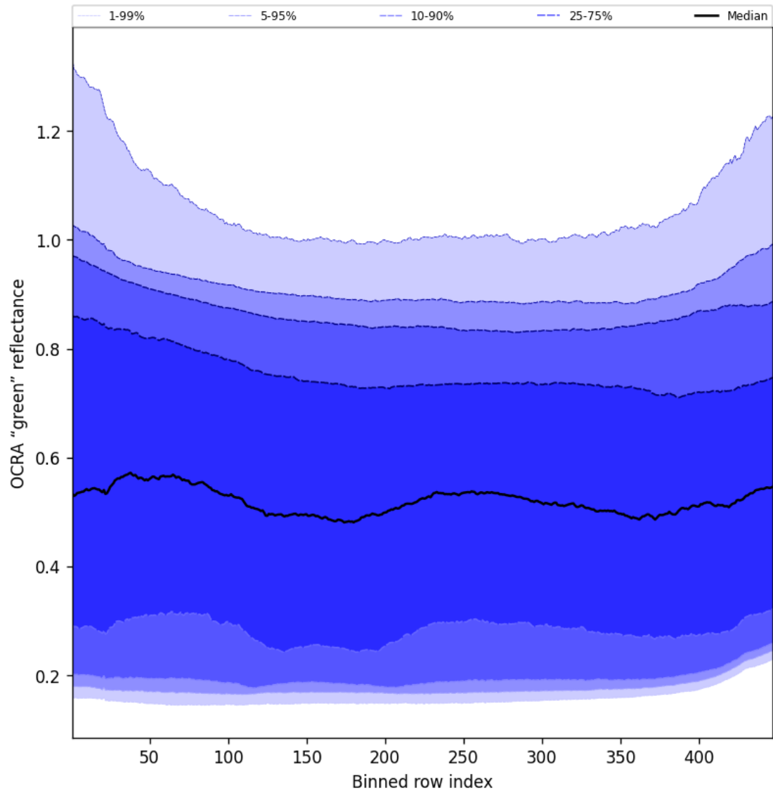
Figure 68: Along track statistics of “OCRA “green” reflectance” for 2025-02-16 to 2025-02-18
