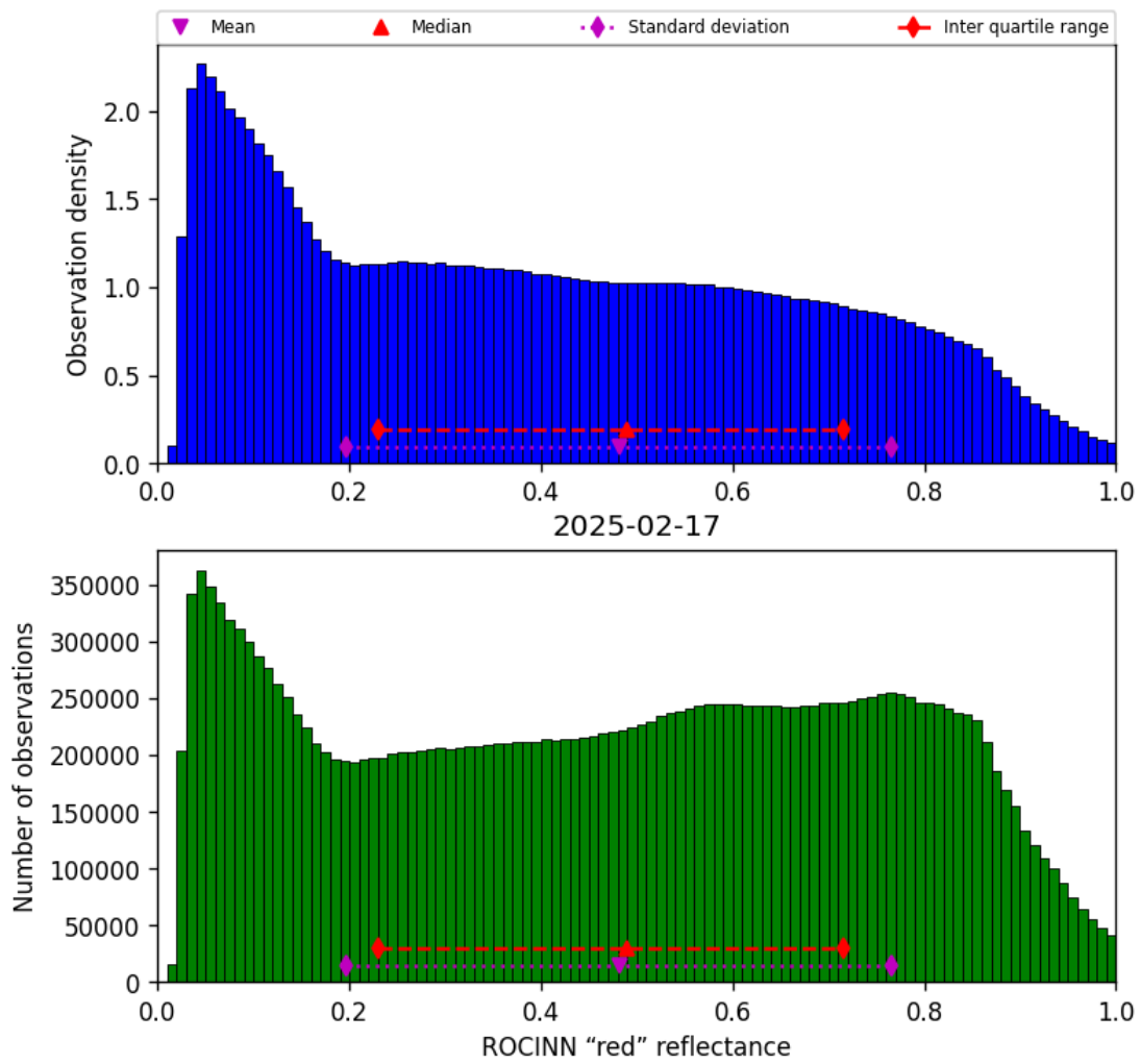
Figure 53: Histogram of “ROCINN “red” reflectance” for 2025-02-16 to 2025-02-18
