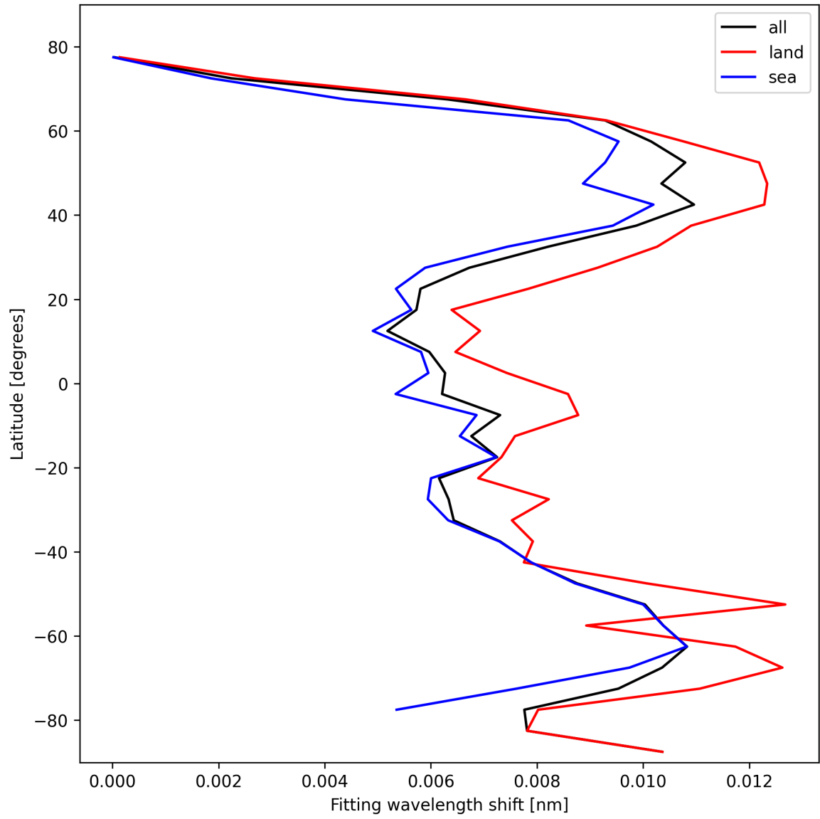
Figure 33: Zonal average of “Fitting wavelength shift” for 2025-02-16 to 2025-02-18.
