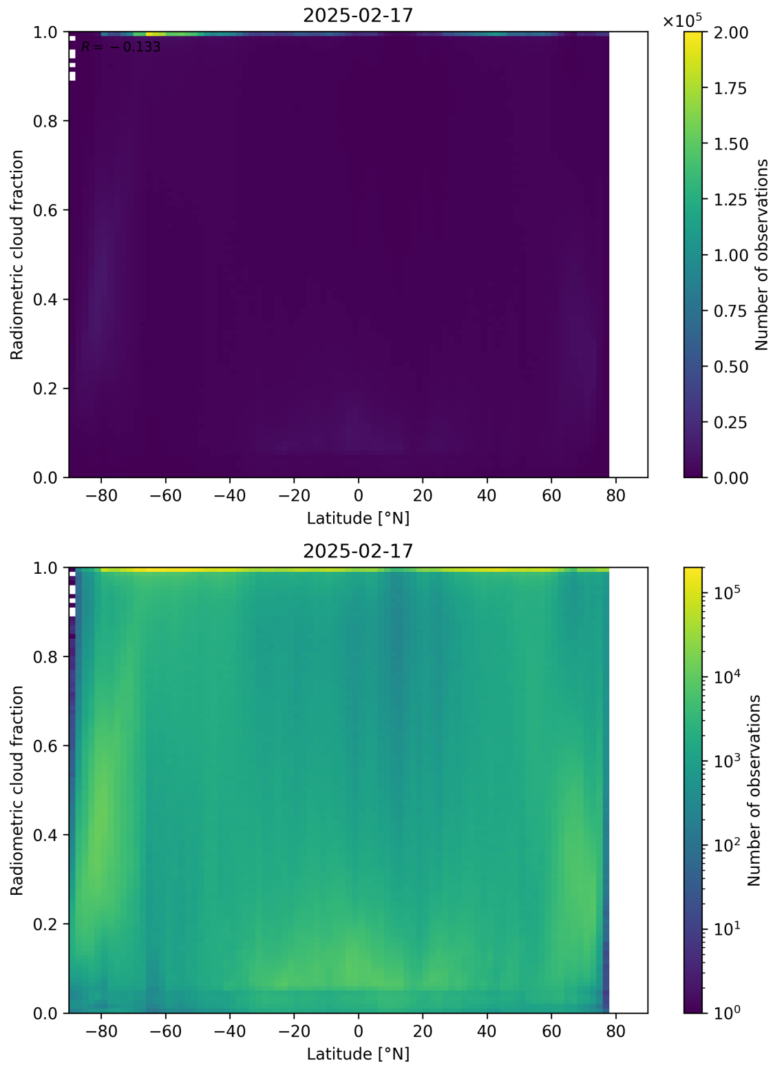
Figure 92: Scatter density plot of “Latitude” against “Radiometric cloud fraction” for 2025-02-16 to 2025-02-18.
