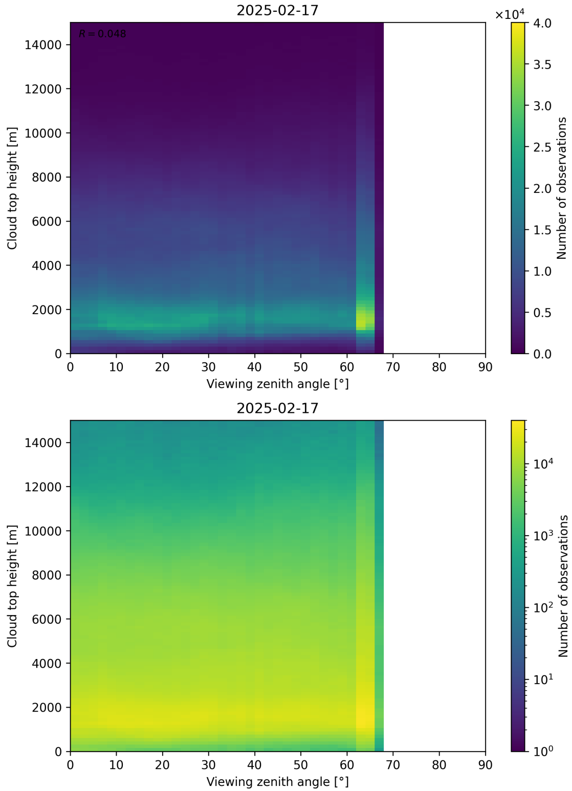
Figure 112: Scatter density plot of “Viewing zenith angle” against “Cloud top height” for 2025-02-16 to 2025-02-18.
