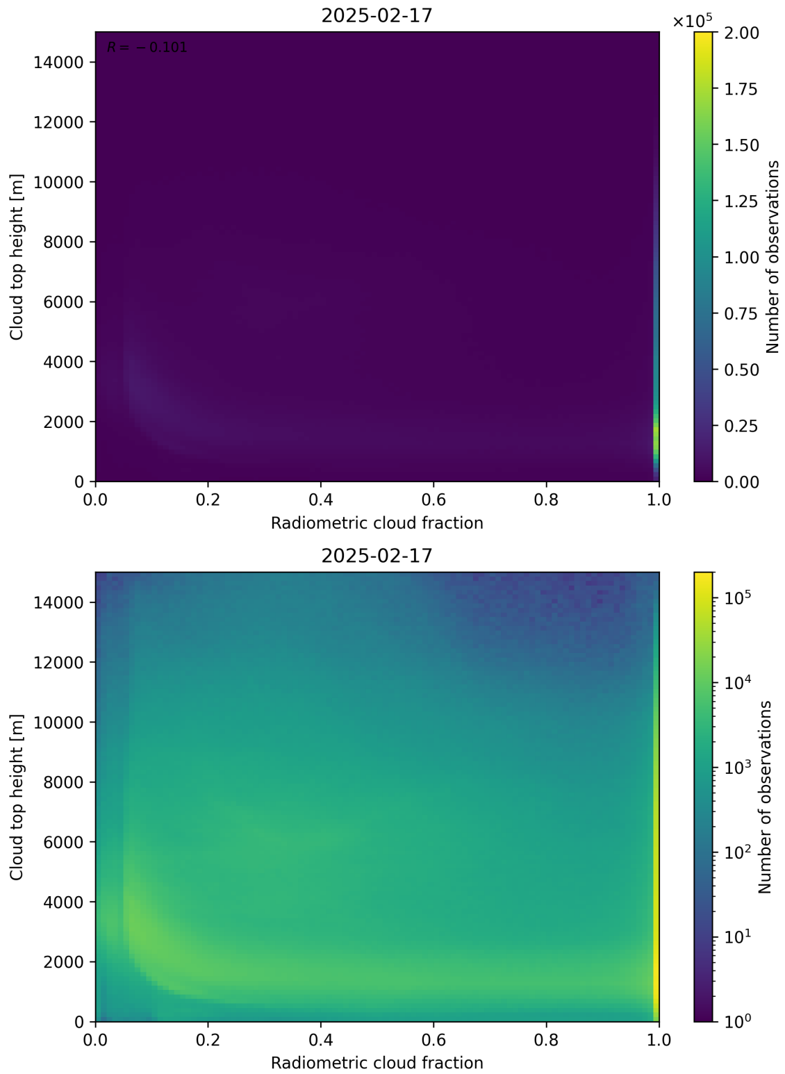
Figure 76: Scatter density plot of “Radiometric cloud fraction” against “Cloud top height” for 2025-02-16 to 2025-02-18.
