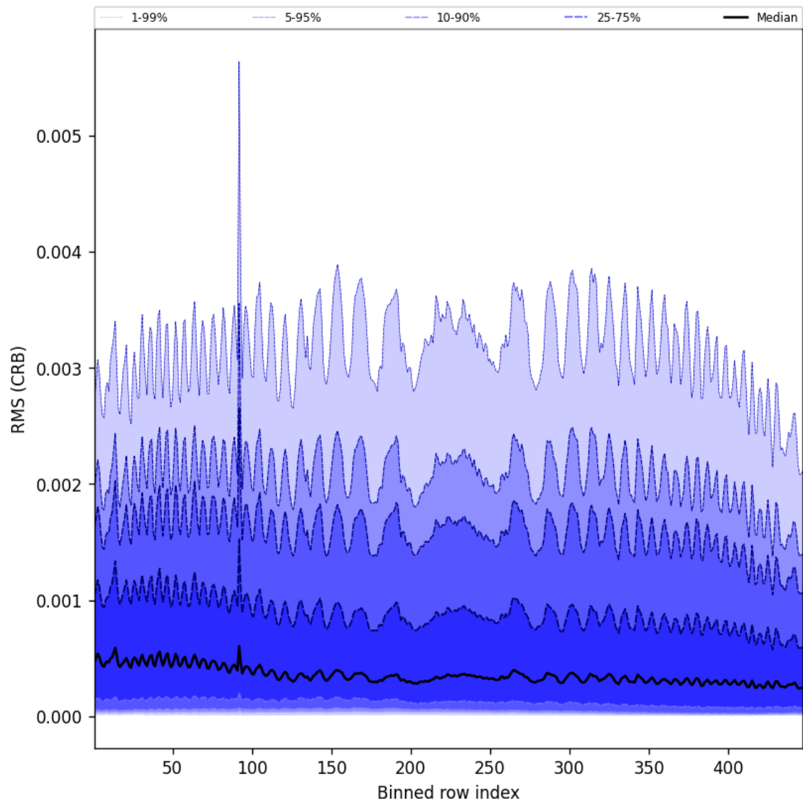
Figure 64: Along track statistics of “RMS (CRB)” for 2025-02-16 to 2025-02-18
