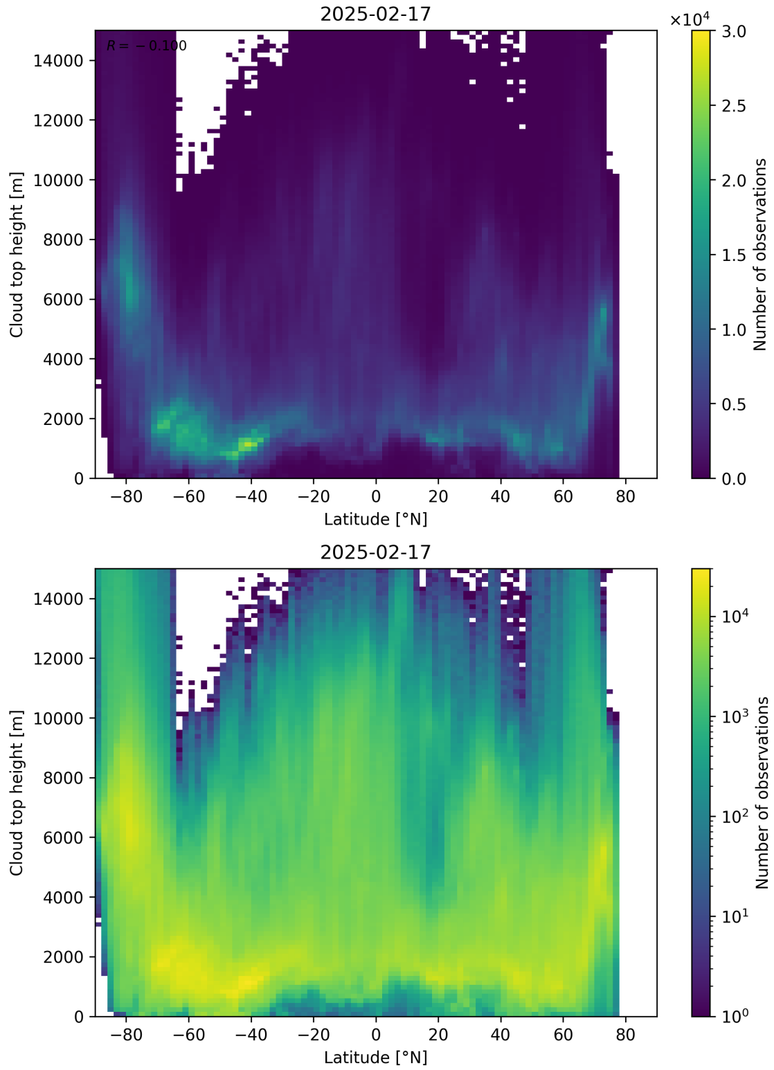
Figure 97: Scatter density plot of “Latitude” against “Cloud top height” for 2025-02-16 to 2025-02-18.
