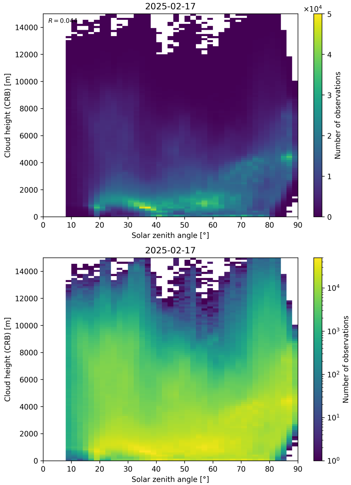
Figure 102: Scatter density plot of “Solar zenith angle” against “Cloud height (CRB)” for 2025-02-16 to 2025-02-18.
