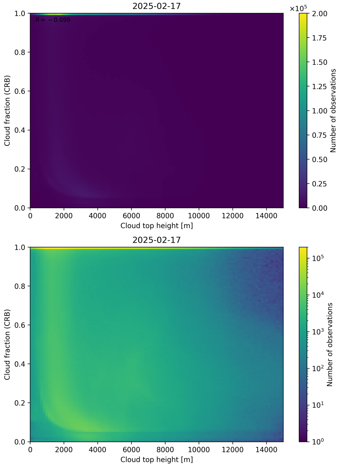
Figure 88: Scatter density plot of “Cloud top height” against “Cloud fraction (CRB)” for 2025-02-16 to 2025-02-18.
