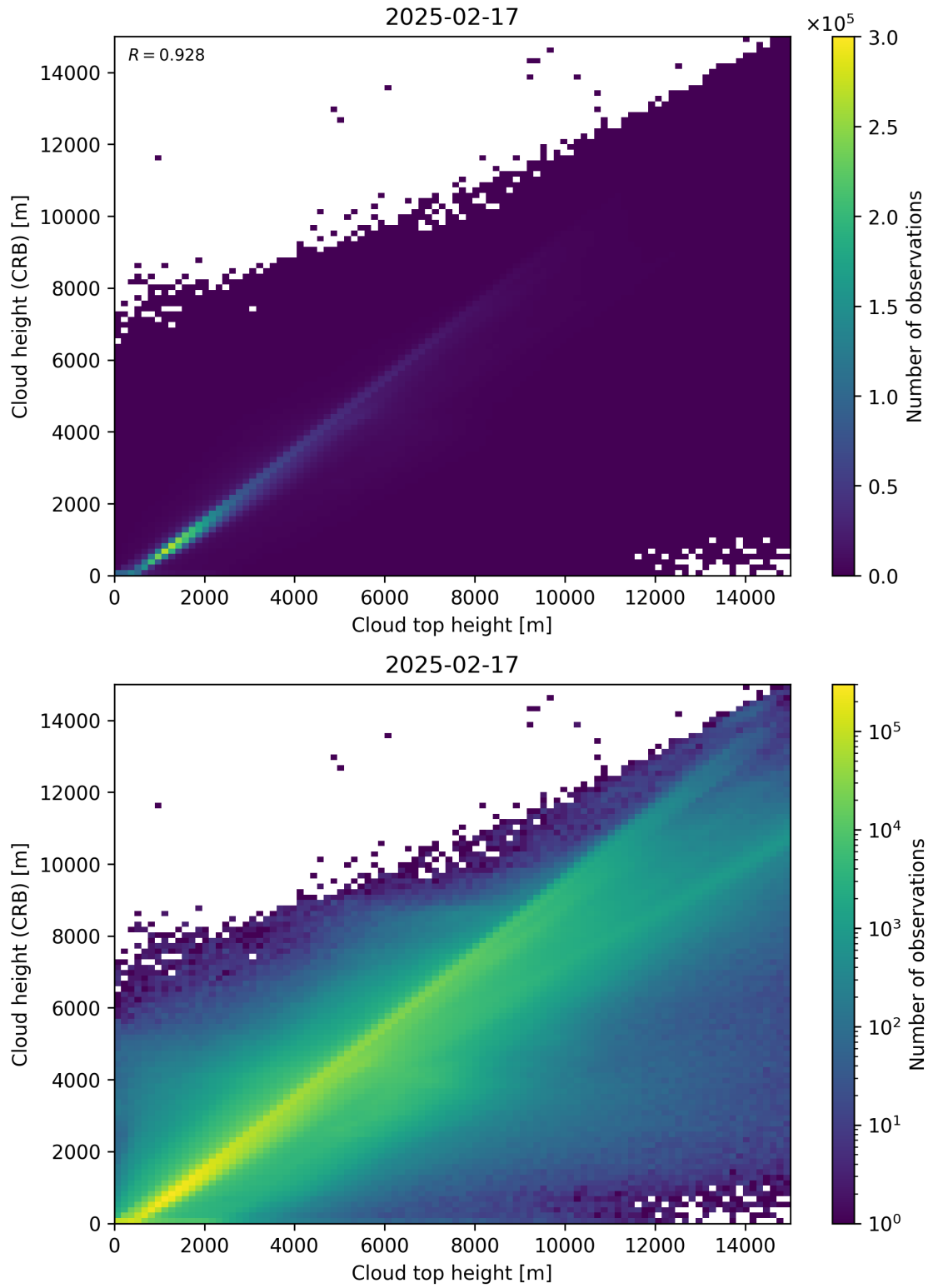
Figure 89: Scatter density plot of “Cloud top height” against “Cloud height (CRB)” for 2025-02-16 to 2025-02-18.
