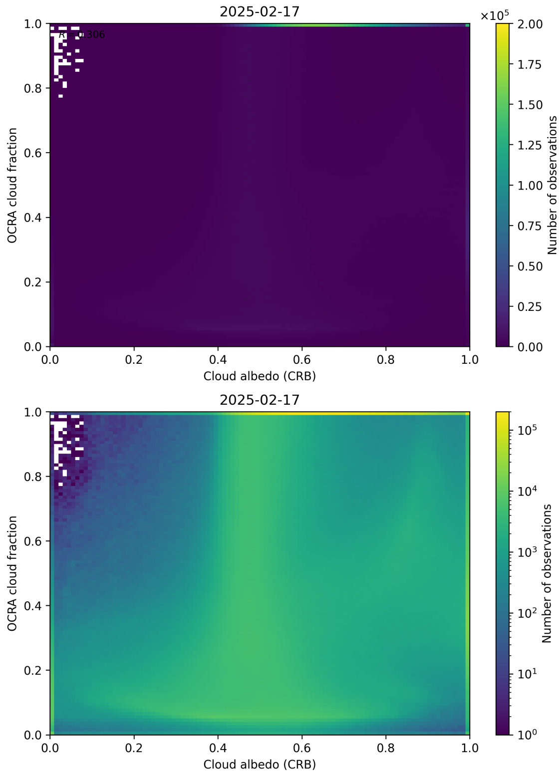
Figure 70: Scatter density plot of “Cloud albedo (CRB)” against “OCRA cloud fraction” for 2025-02-16 to 2025-02-18.
