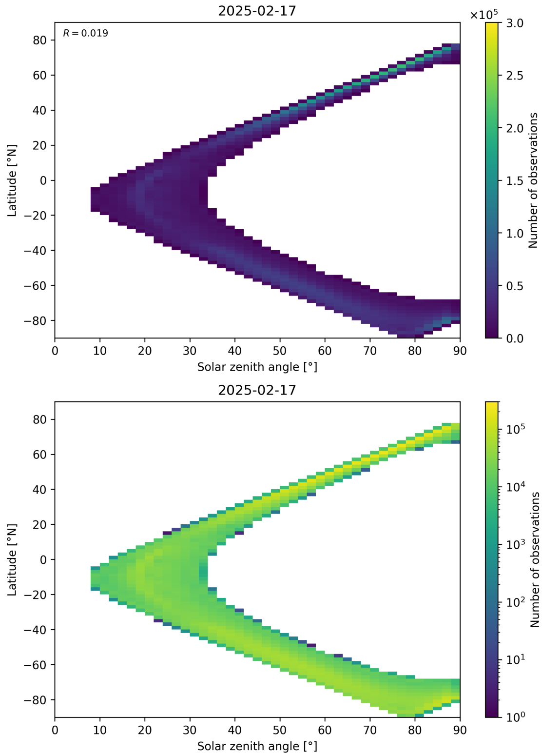
Figure 105: Scatter density plot of “Solar zenith angle” against “Latitude” for 2025-02-16 to 2025-02-18.
