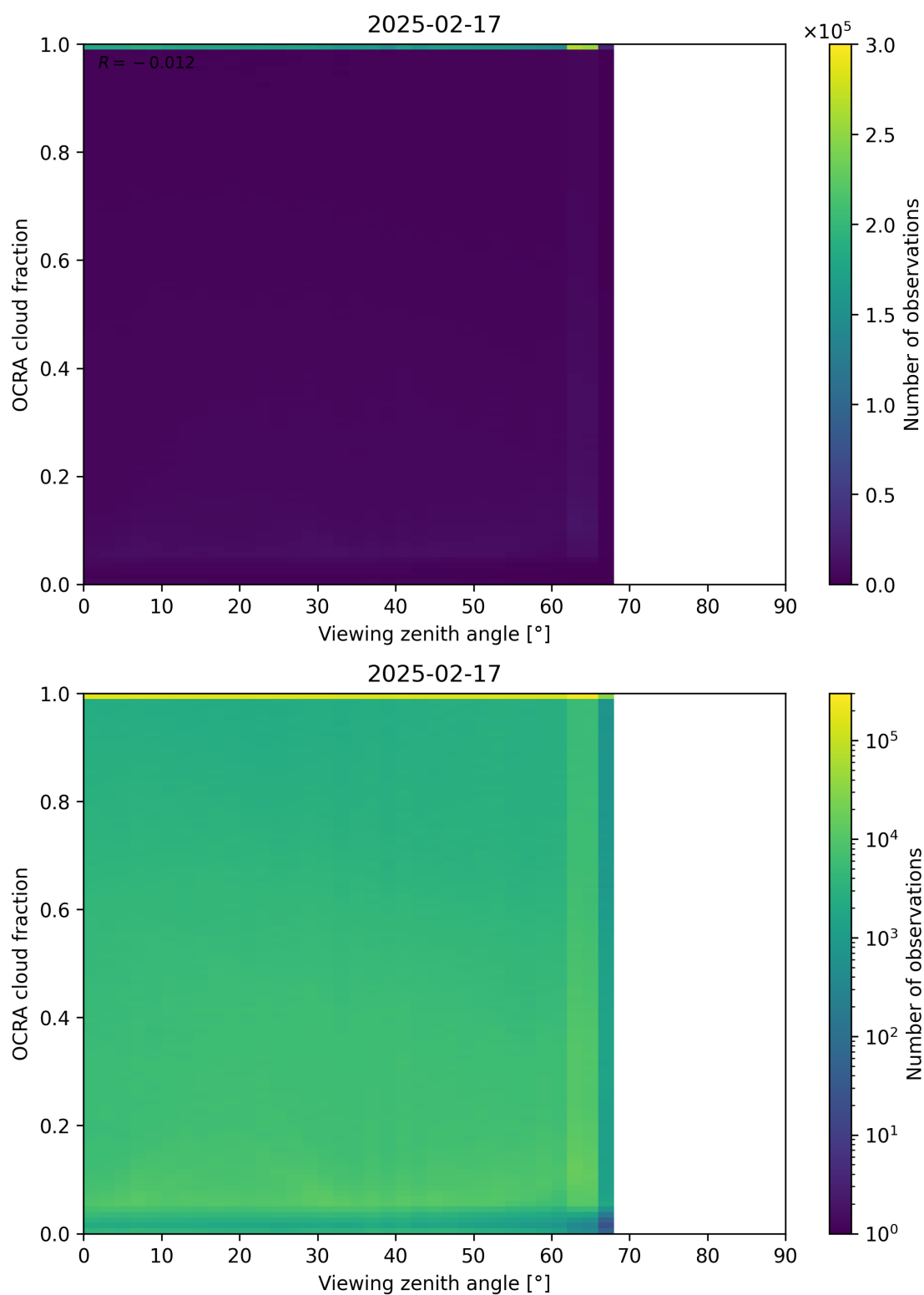
Figure 108: Scatter density plot of “Viewing zenith angle” against “OCRA cloud fraction” for 2025-02-16 to 2025-02-18.
