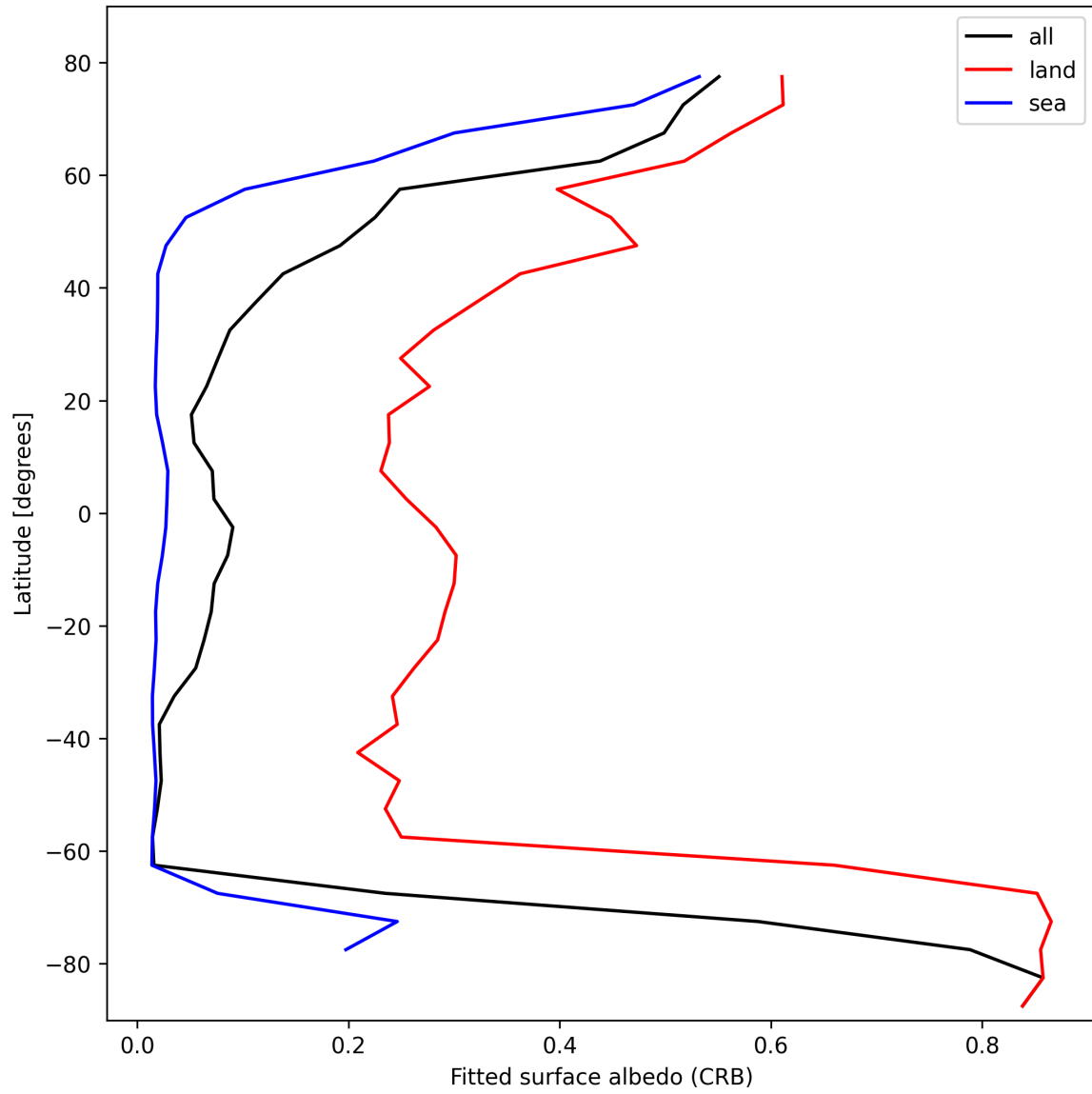
Figure 30: Zonal average of “Fitted surface albedo (CRB)” for 2025-02-16 to 2025-02-18.
