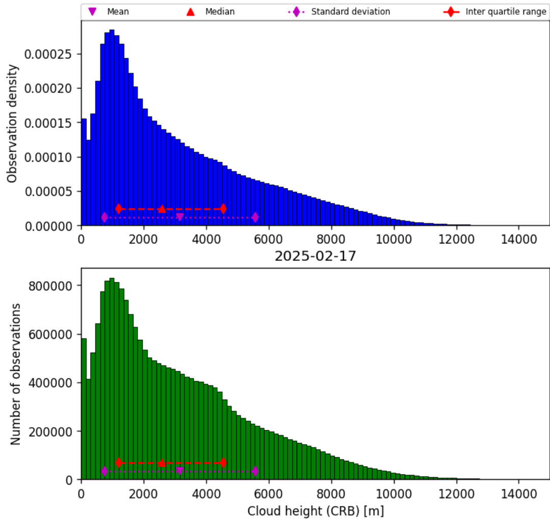
Figure 43: Histogram of “Cloud height (CRB)” for 2025-02-16 to 2025-02-18
