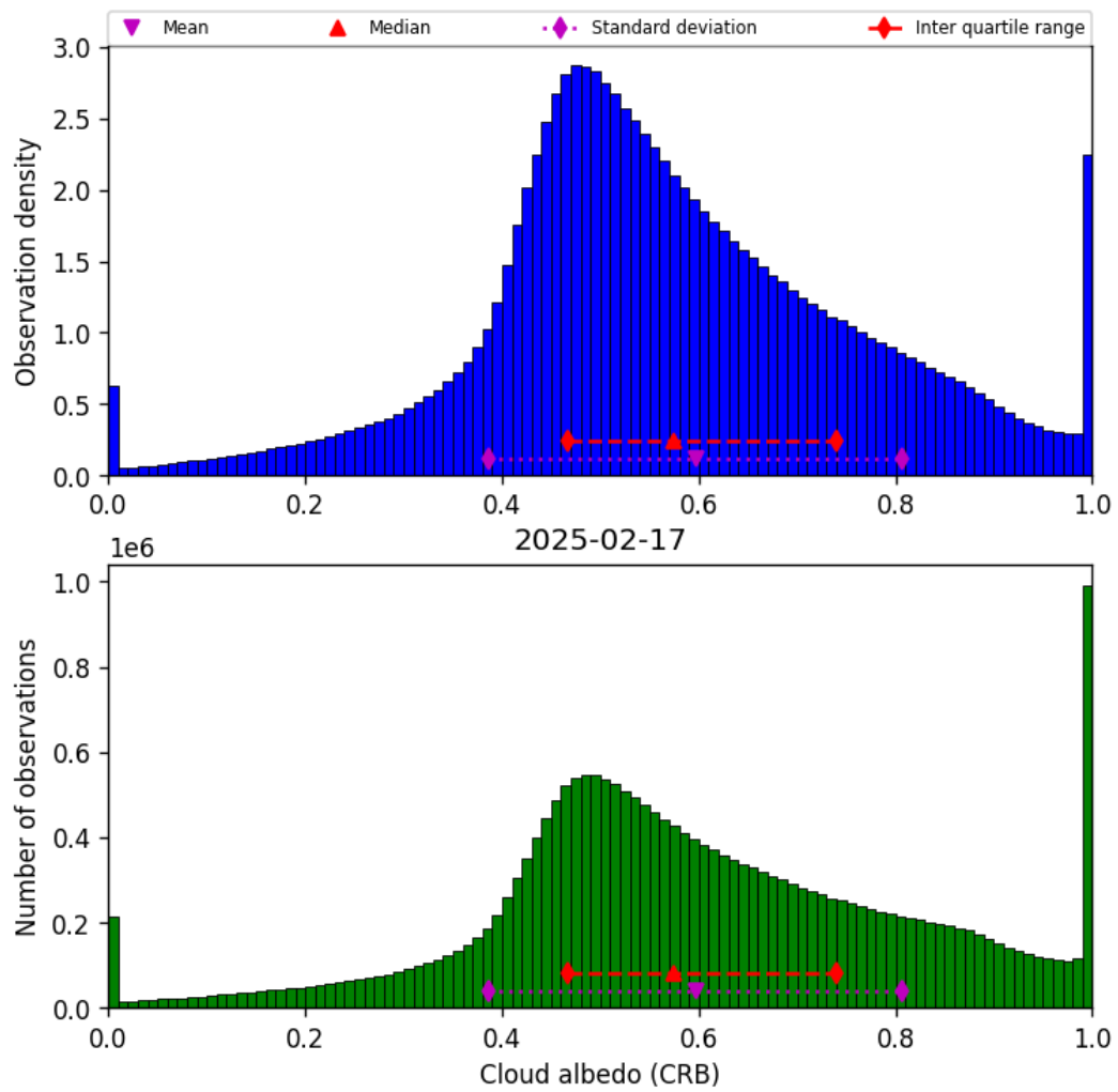
Figure 44: Histogram of “Cloud albedo (CRB)” for 2025-02-16 to 2025-02-18
