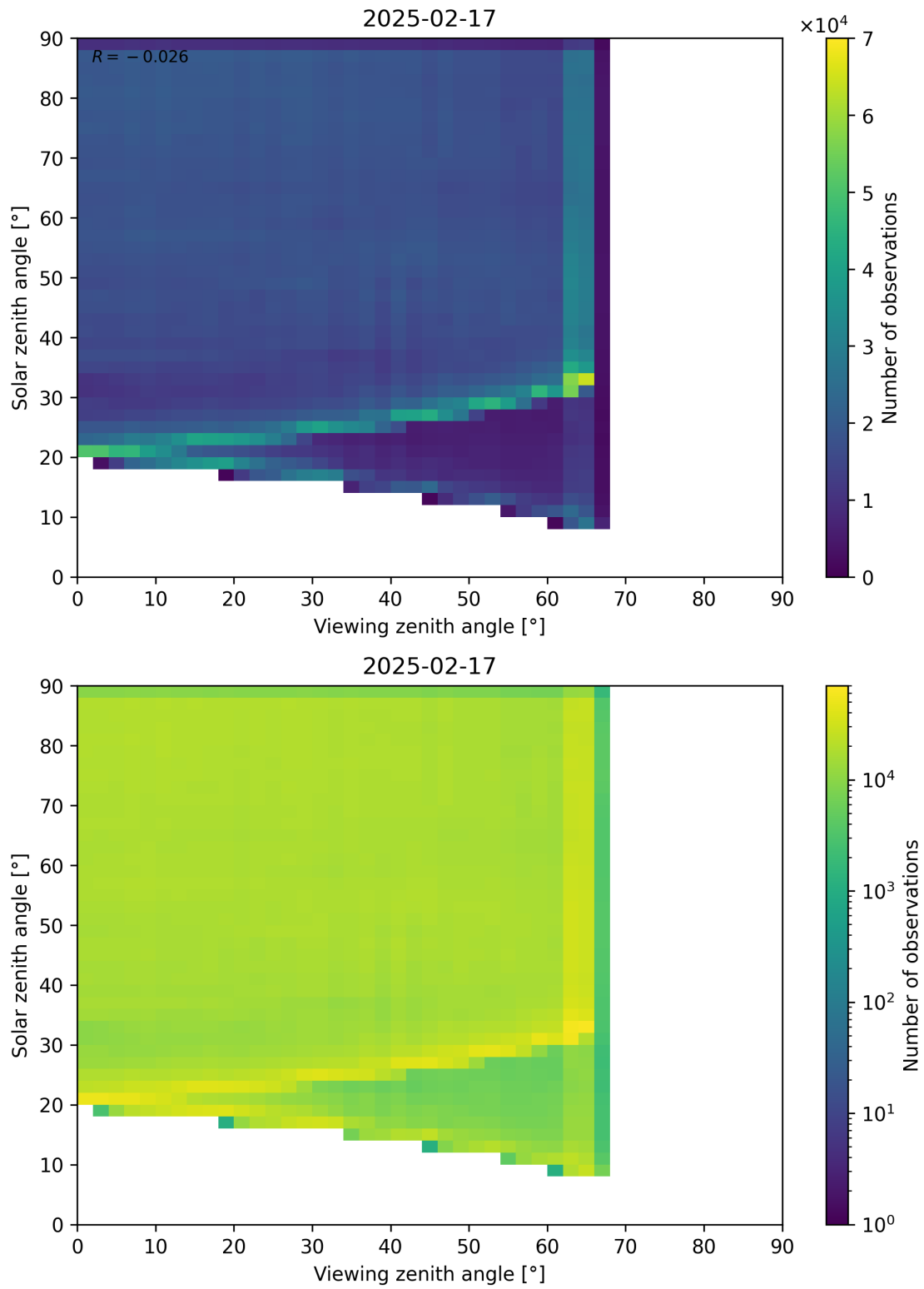
Figure 114: Scatter density plot of “Viewing zenith angle” against “Solar zenith angle” for 2025-02-16 to 2025-02-18.
