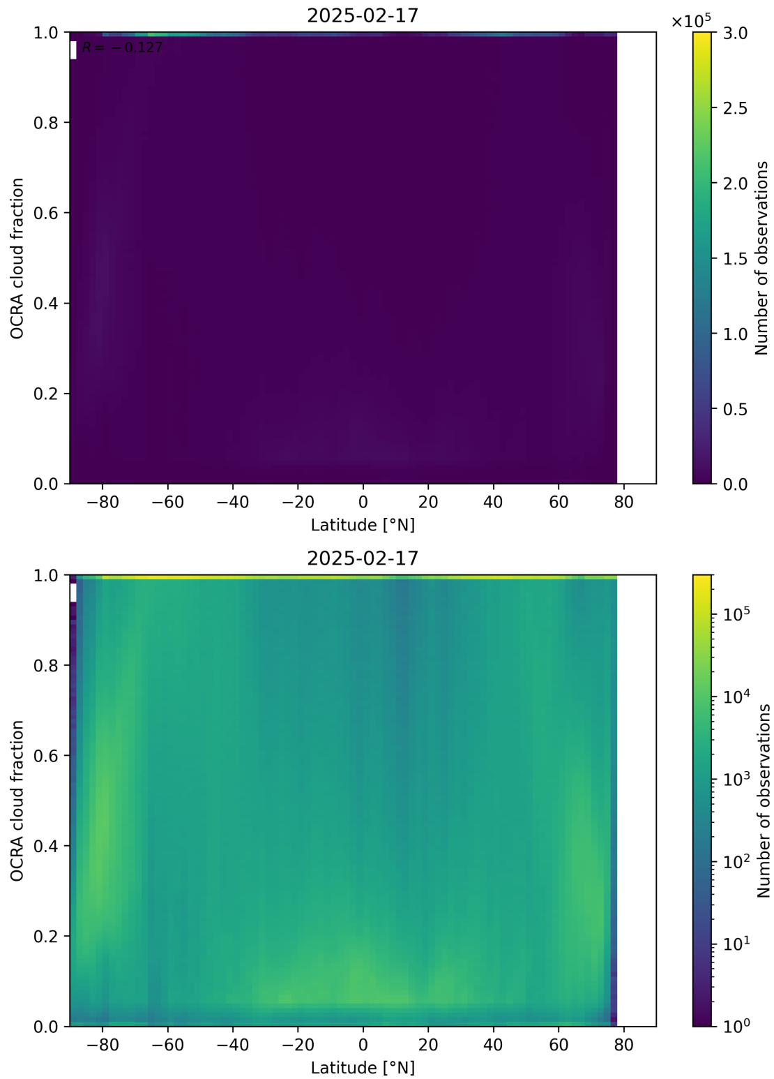
Figure 93: Scatter density plot of “Latitude” against “OCRA cloud fraction” for 2025-02-16 to 2025-02-18.
