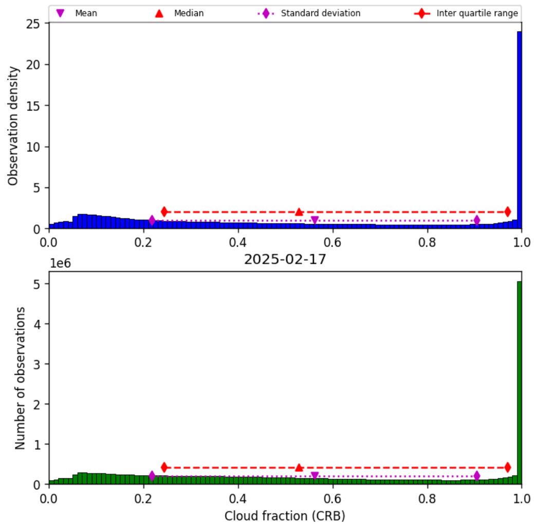
Figure 42: Histogram of “Cloud fraction (CRB)” for 2025-02-16 to 2025-02-18
