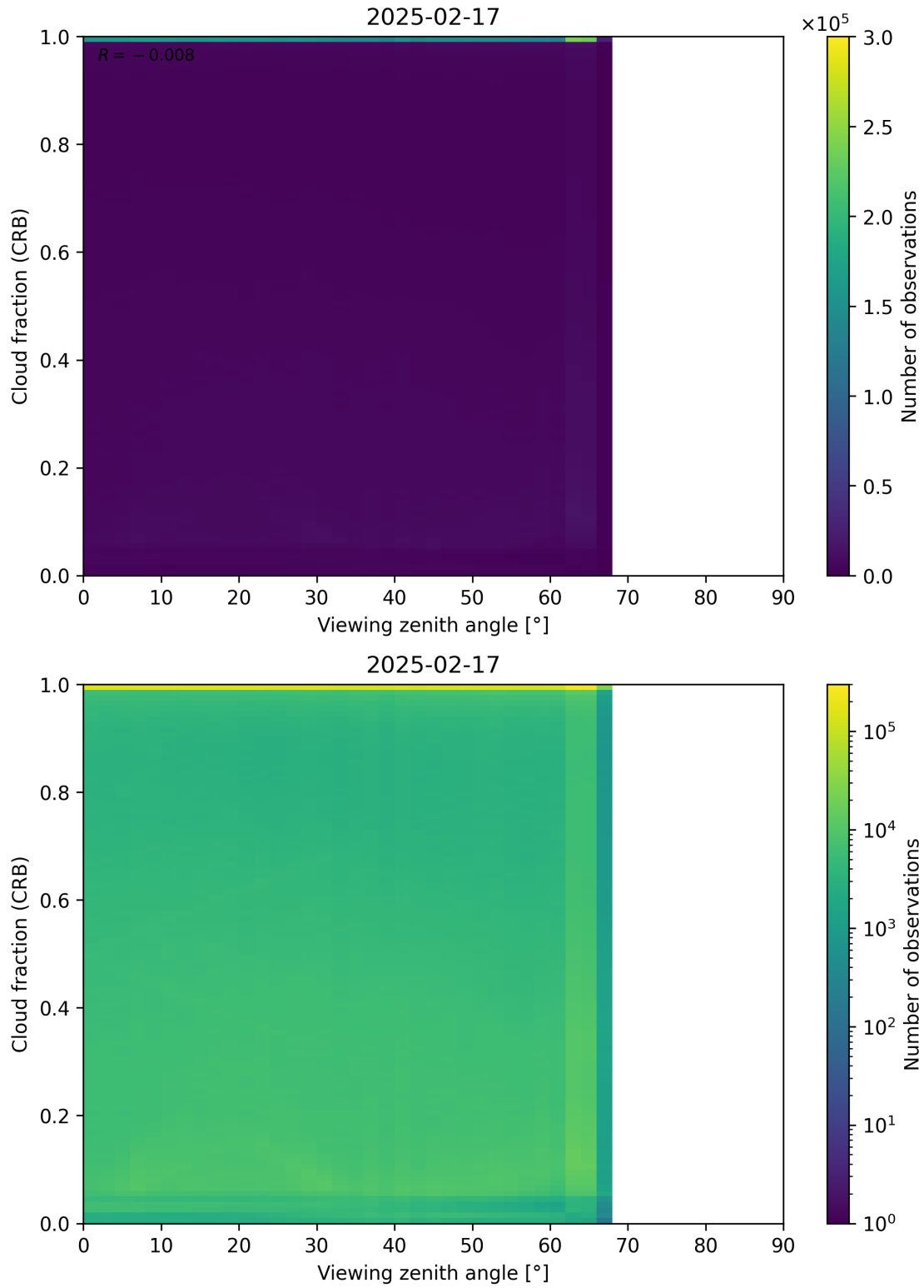
Figure 109: Scatter density plot of “Viewing zenith angle” against “Cloud fraction (CRB)” for 2025-02-16 to 2025-02-18.
