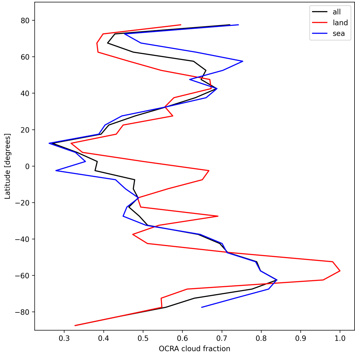
Figure 34: Zonal average of “OCRA cloud fraction” for 2025-02-16 to 2025-02-18.
