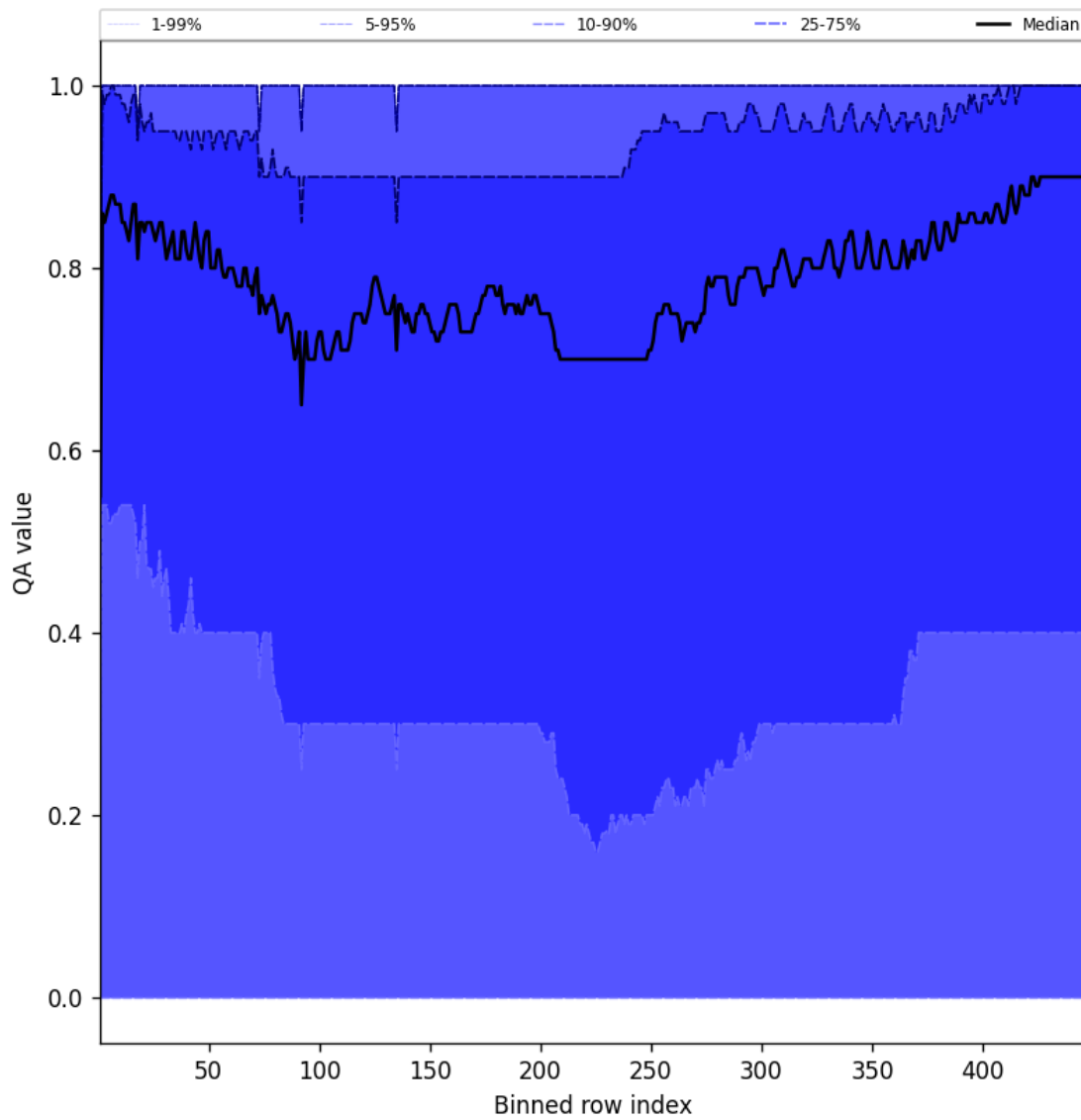
Figure 54: Along track statistics of “QA value” for 2025-02-16 to 2025-02-18
