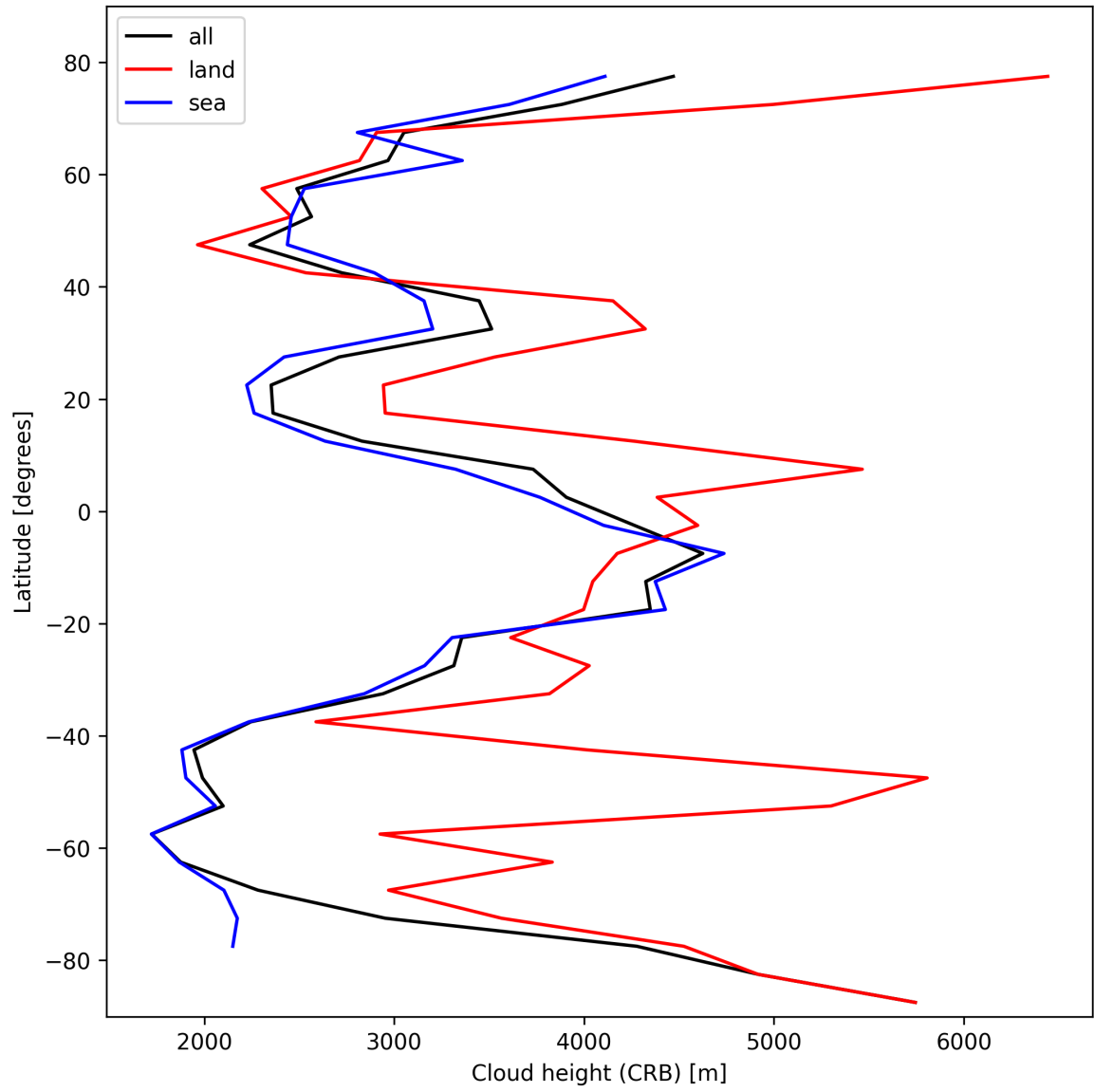
Figure 27: Zonal average of “Cloud height (CRB)” for 2025-02-16 to 2025-02-18.
