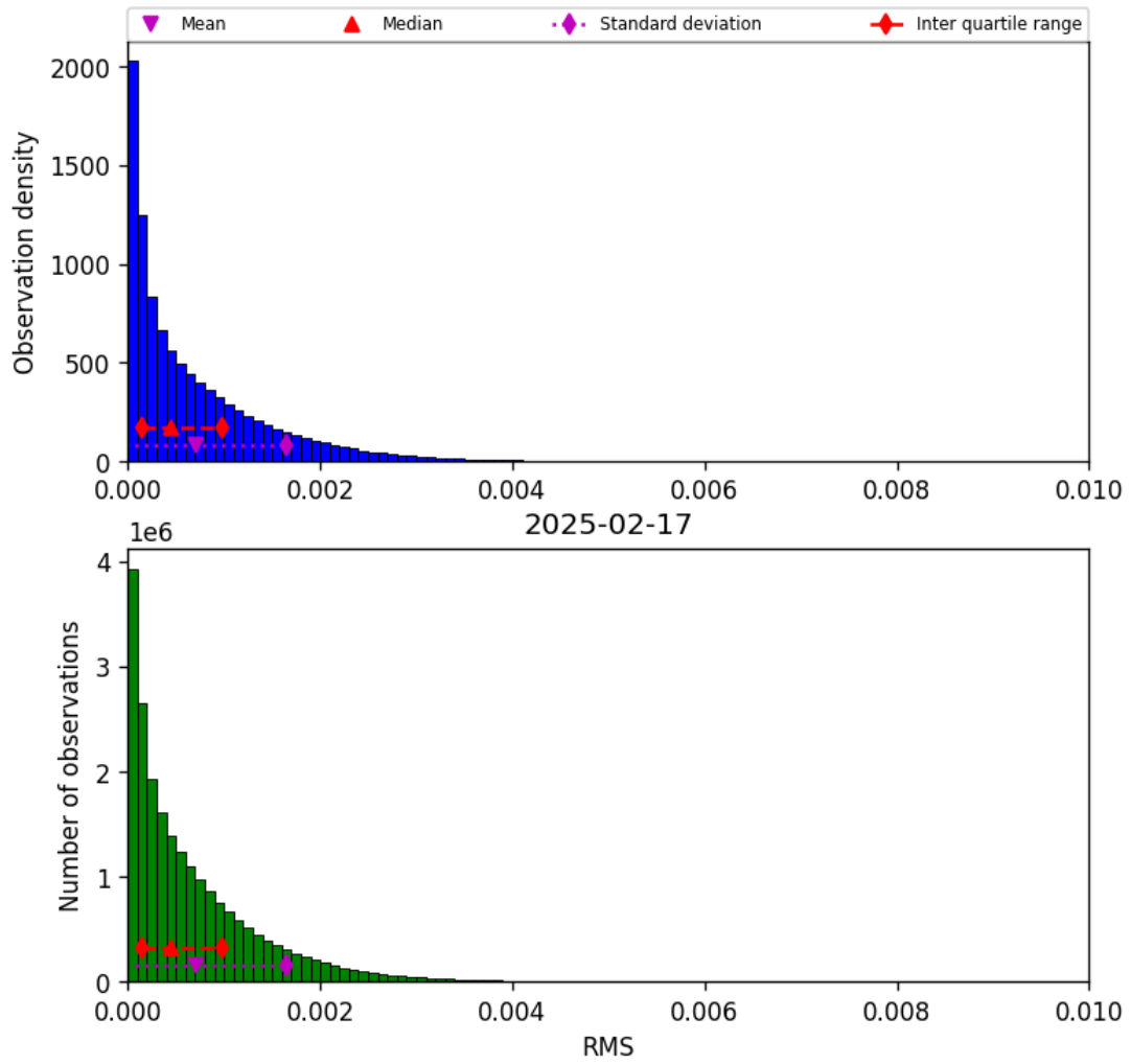
Figure 47: Histogram of “RMS” for 2025-02-16 to 2025-02-18
