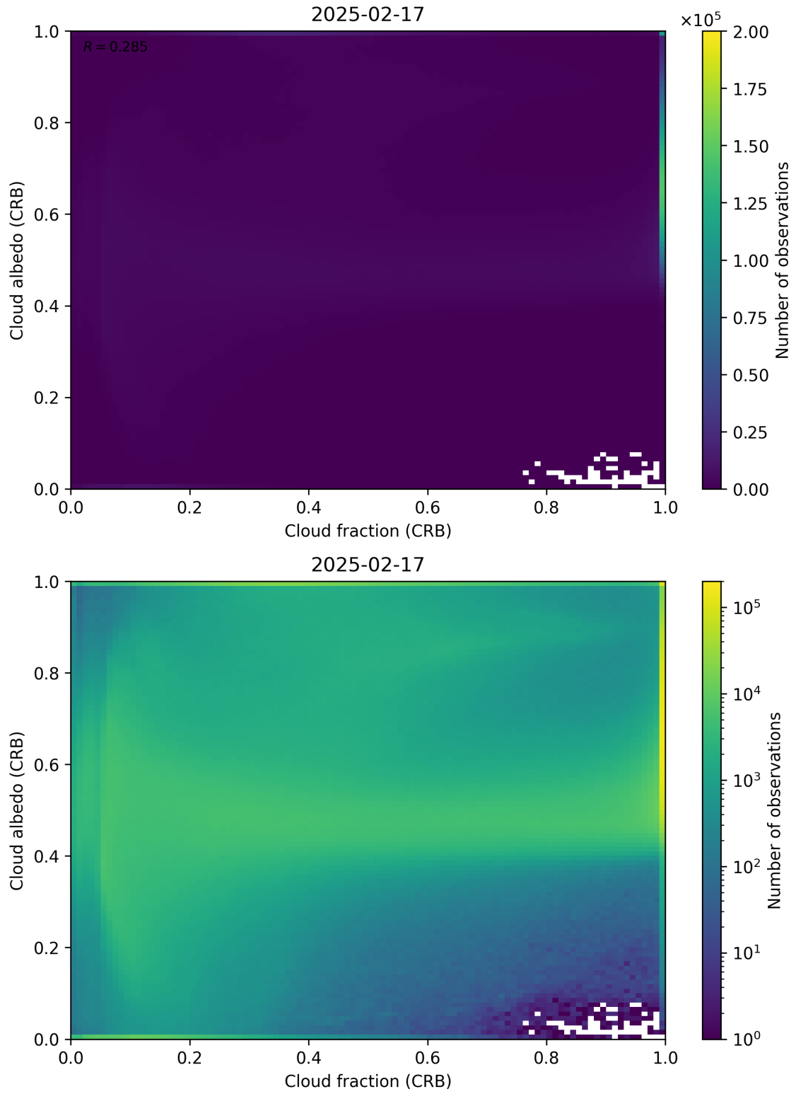
Figure 77: Scatter density plot of “Cloud fraction (CRB)” against “Cloud albedo (CRB)” for 2025-02-16 to 2025-02-18.
