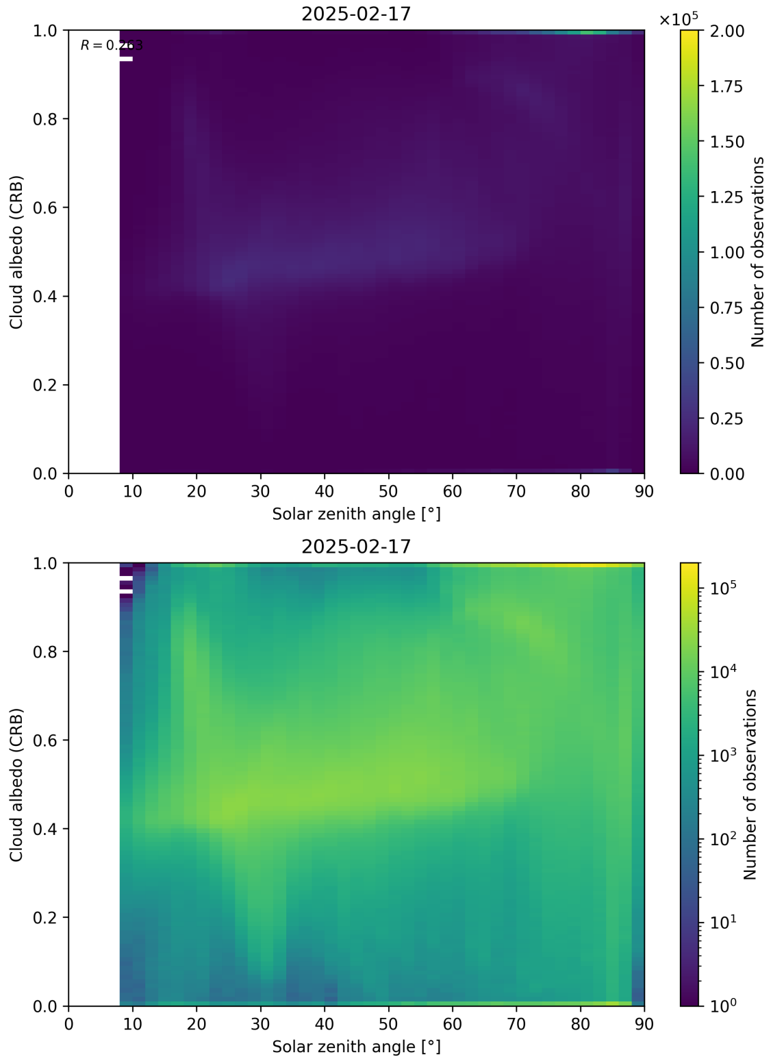
Figure 98: Scatter density plot of “Solar zenith angle” against “Cloud albedo (CRB)” for 2025-02-16 to 2025-02-18.
