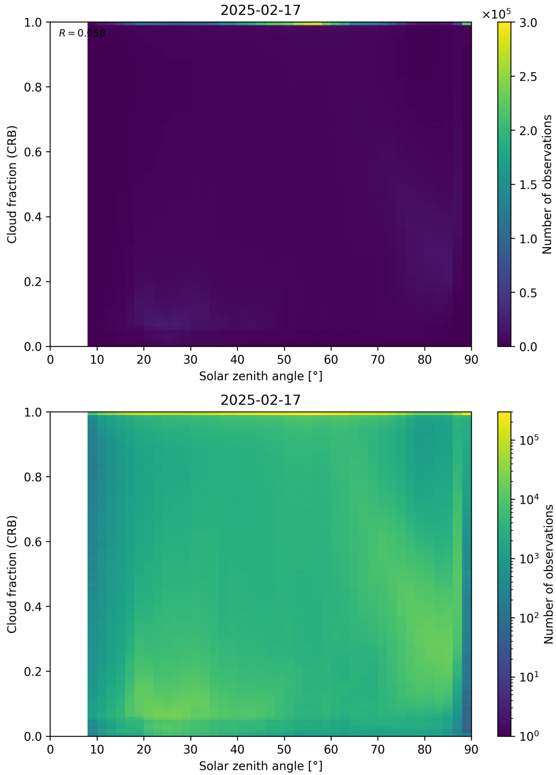
Figure 101: Scatter density plot of “Solar zenith angle” against “Cloud fraction (CRB)” for 2025-02-16 to 2025-02-18.
