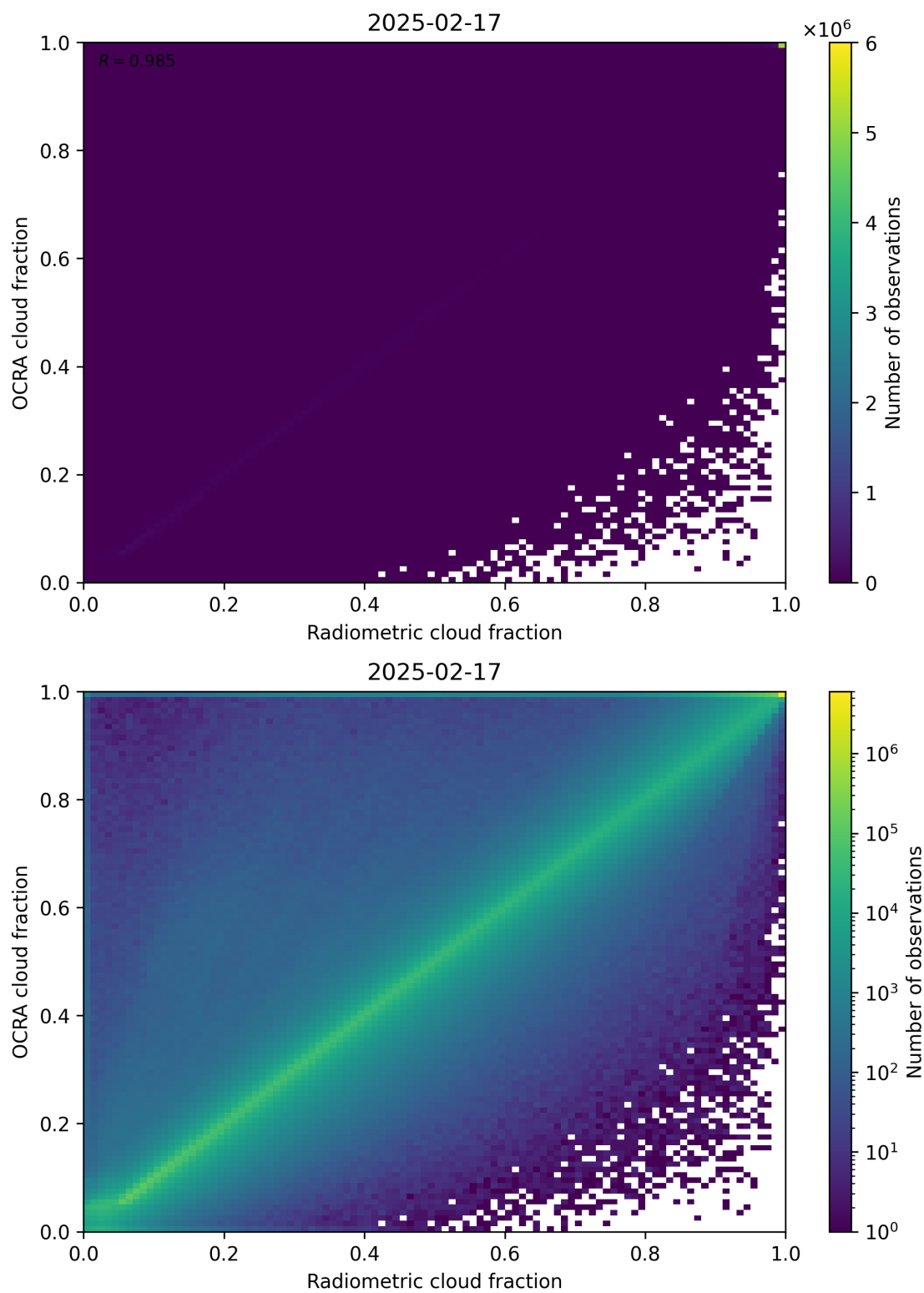
Figure 72: Scatter density plot of “Radiometric cloud fraction” against “OCRA cloud fraction” for 2025-02-16 to 2025-02-18.
