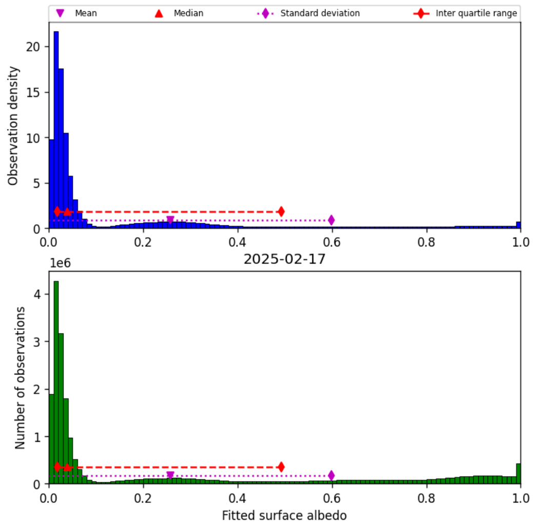
Figure 45: Histogram of “Fitted surface albedo” for 2025-02-16 to 2025-02-18
