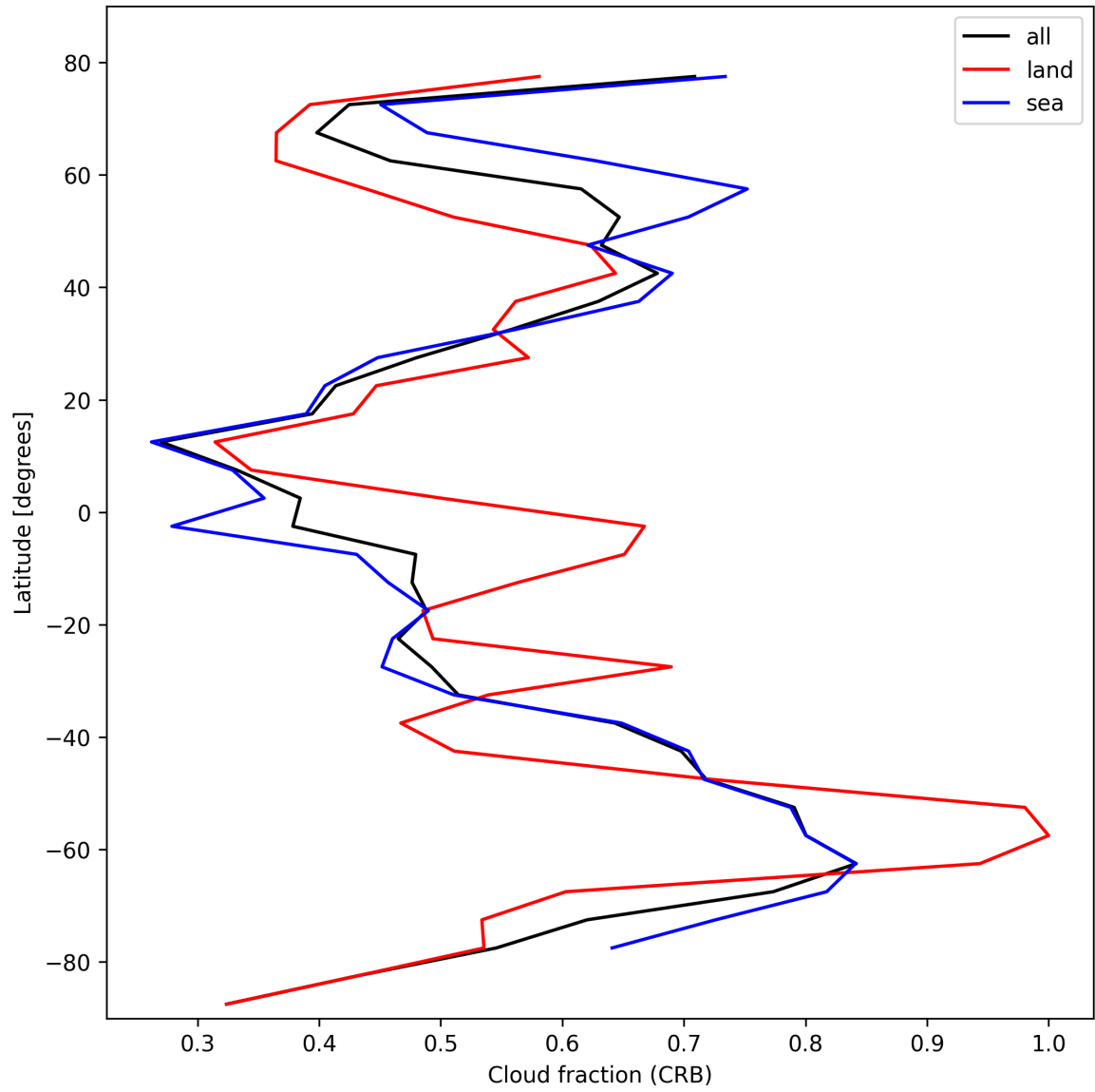
Figure 26: Zonal average of “Cloud fraction (CRB)” for 2025-02-16 to 2025-02-18.
