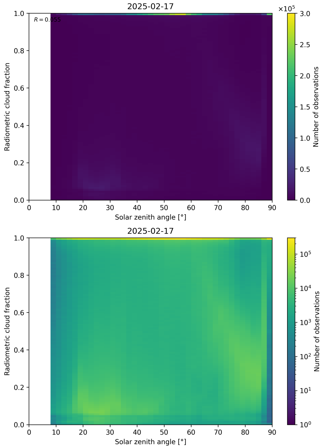
Figure 99: Scatter density plot of “Solar zenith angle” against “Radiometric cloud fraction” for 2025-02-16 to 2025-02-18.
