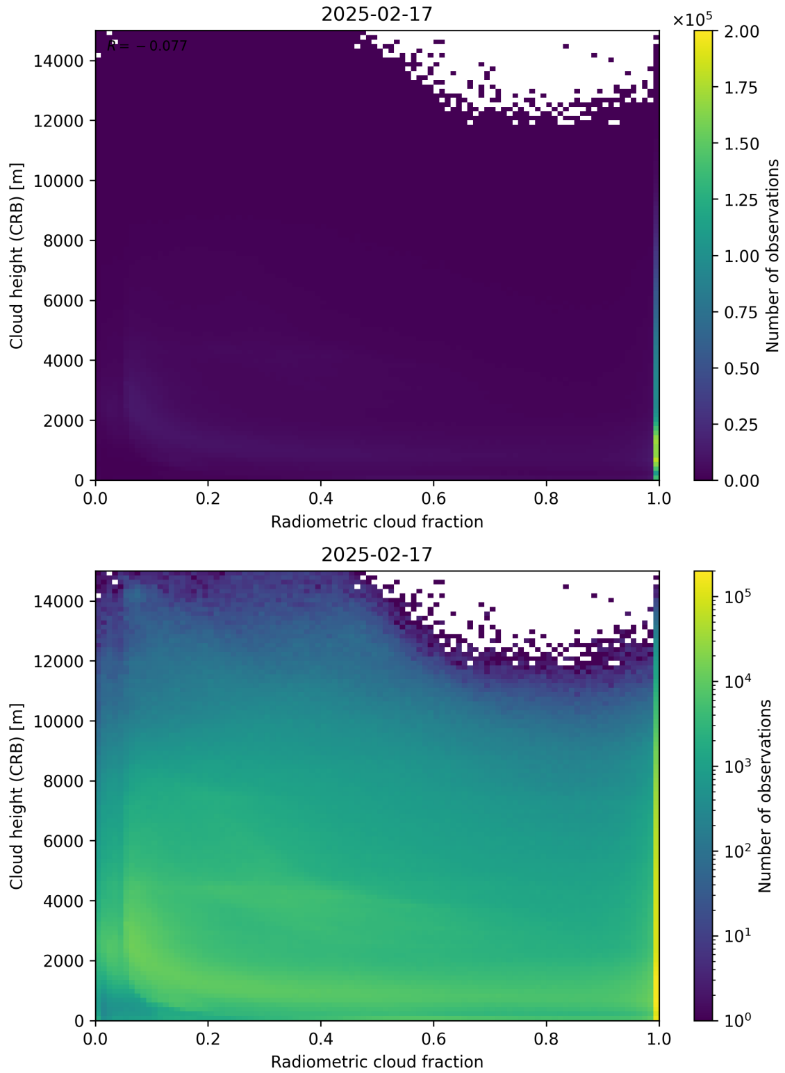
Figure 74: Scatter density plot of “Radiometric cloud fraction” against “Cloud height (CRB)” for 2025-02-16 to 2025-02-18.
