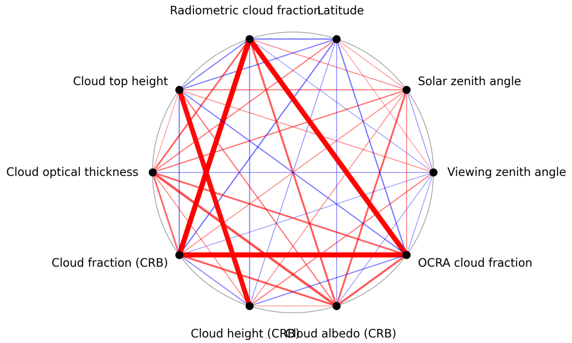
Figure 1: Map of correlation graph for 2025-02-16 to 2025-02-18.
