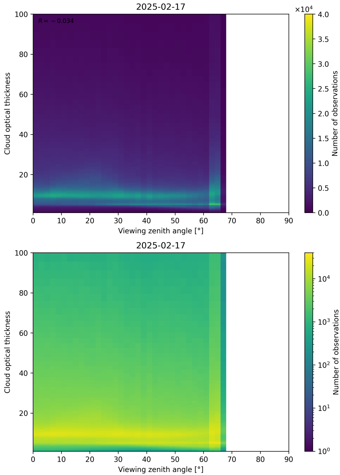
Figure 111: Scatter density plot of “Viewing zenith angle” against “Cloud optical thickness” for 2025-02-16 to 2025-02-18.
