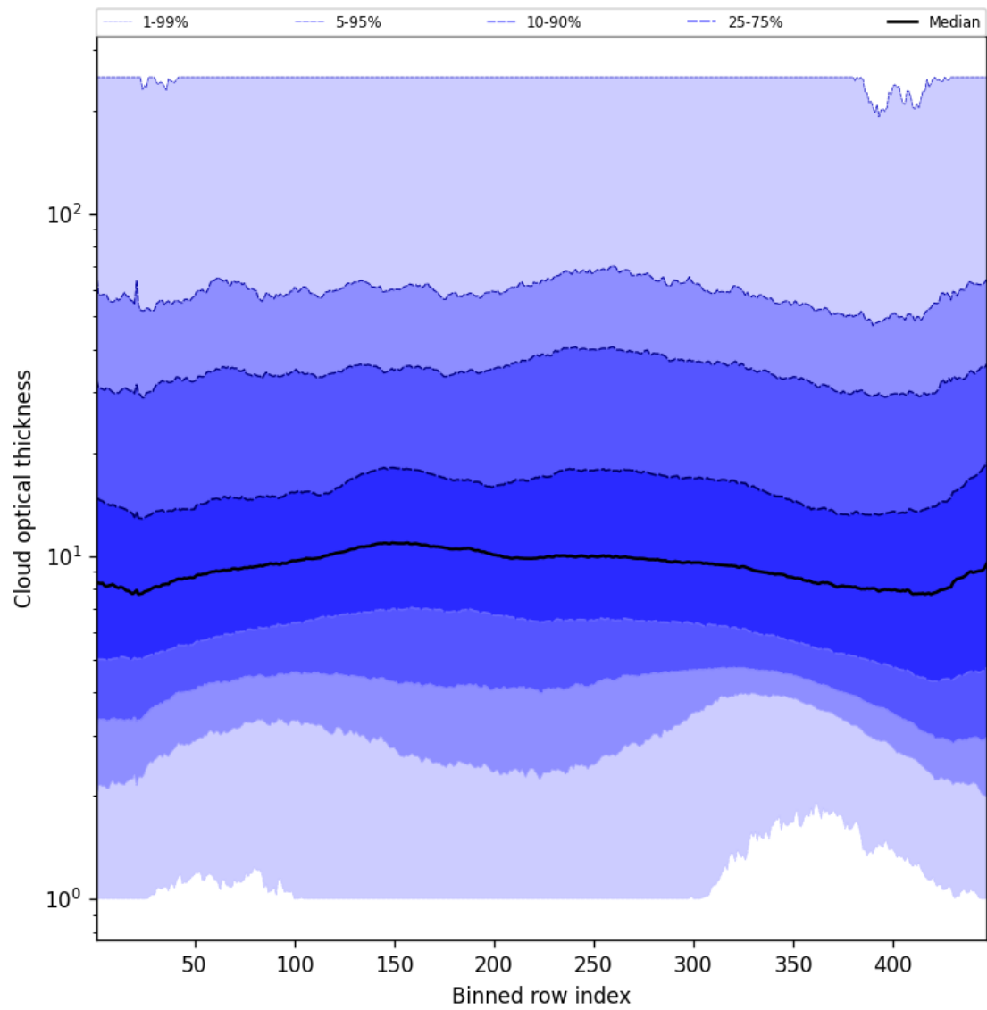
Figure 57: Along track statistics of “Cloud optical thickness” for 2025-02-16 to 2025-02-18
