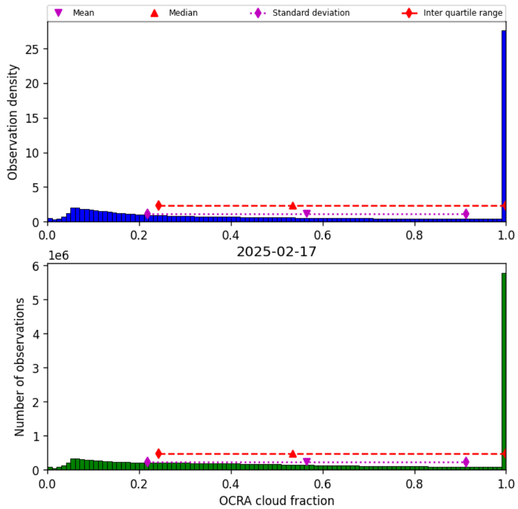
Figure 50: Histogram of “OCRA cloud fraction” for 2025-02-16 to 2025-02-18
