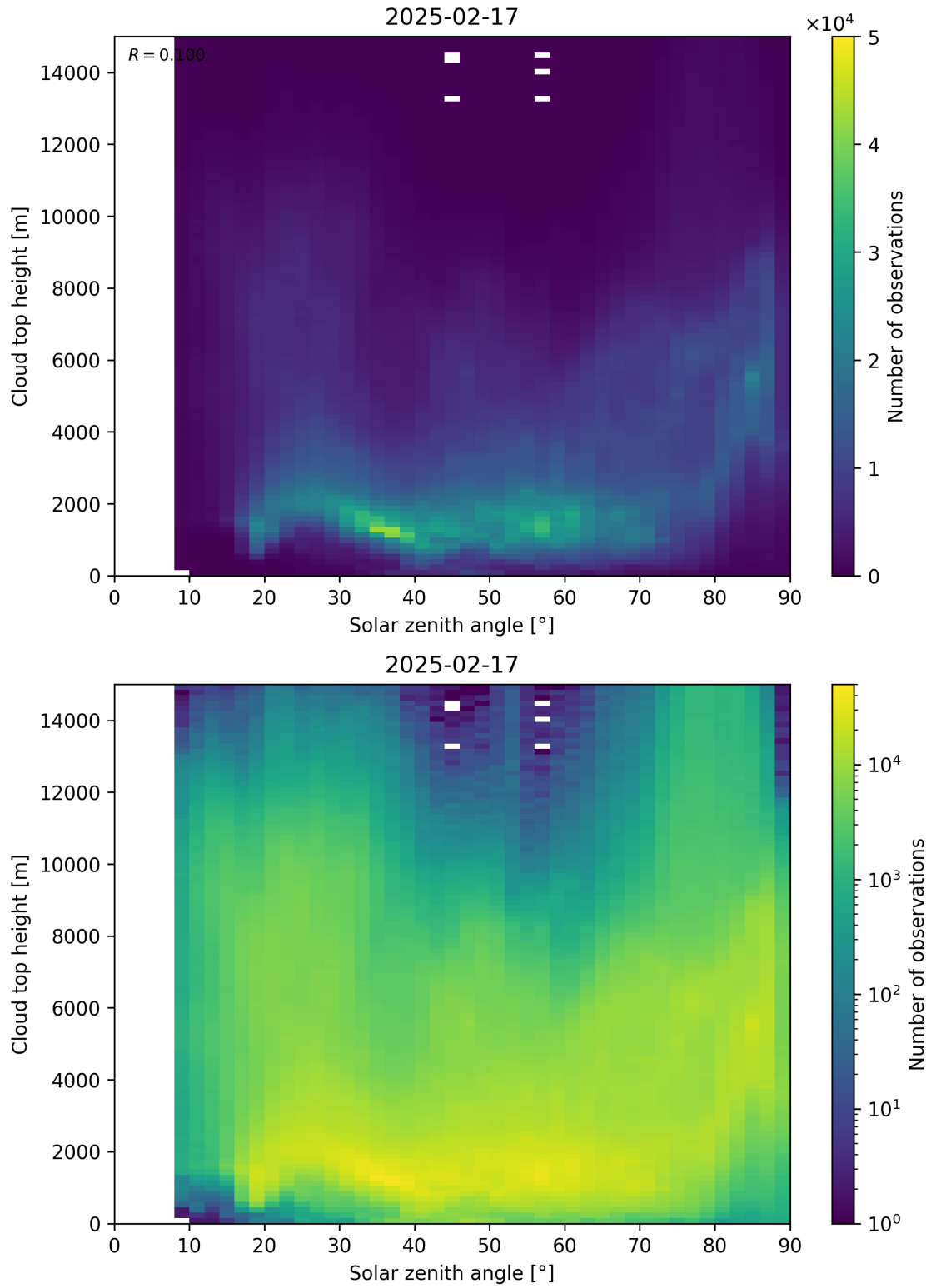
Figure 104: Scatter density plot of “Solar zenith angle” against “Cloud top height” for 2025-02-16 to 2025-02-18.
