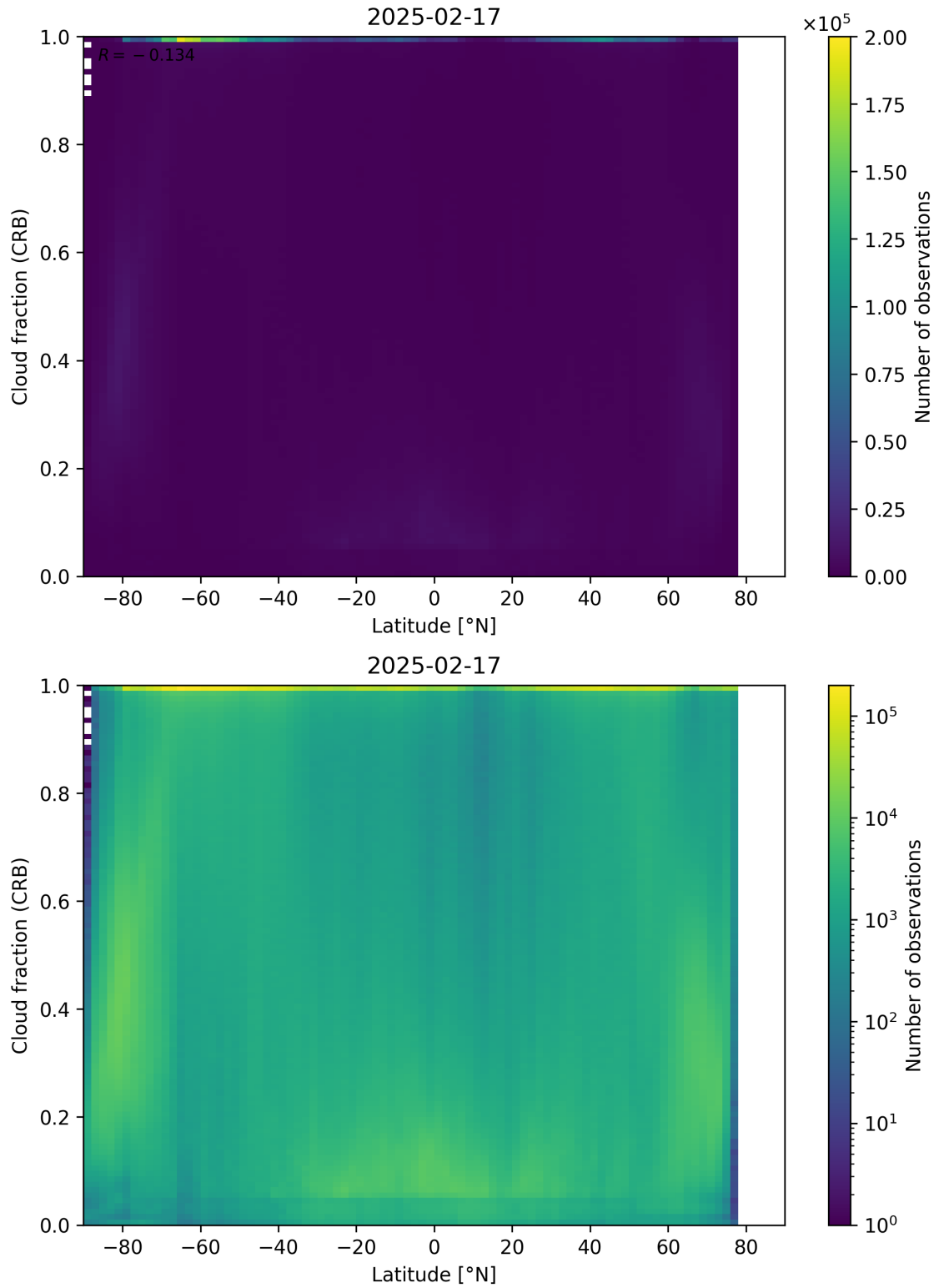
Figure 94: Scatter density plot of “Latitude” against “Cloud fraction (CRB)” for 2025-02-16 to 2025-02-18.
