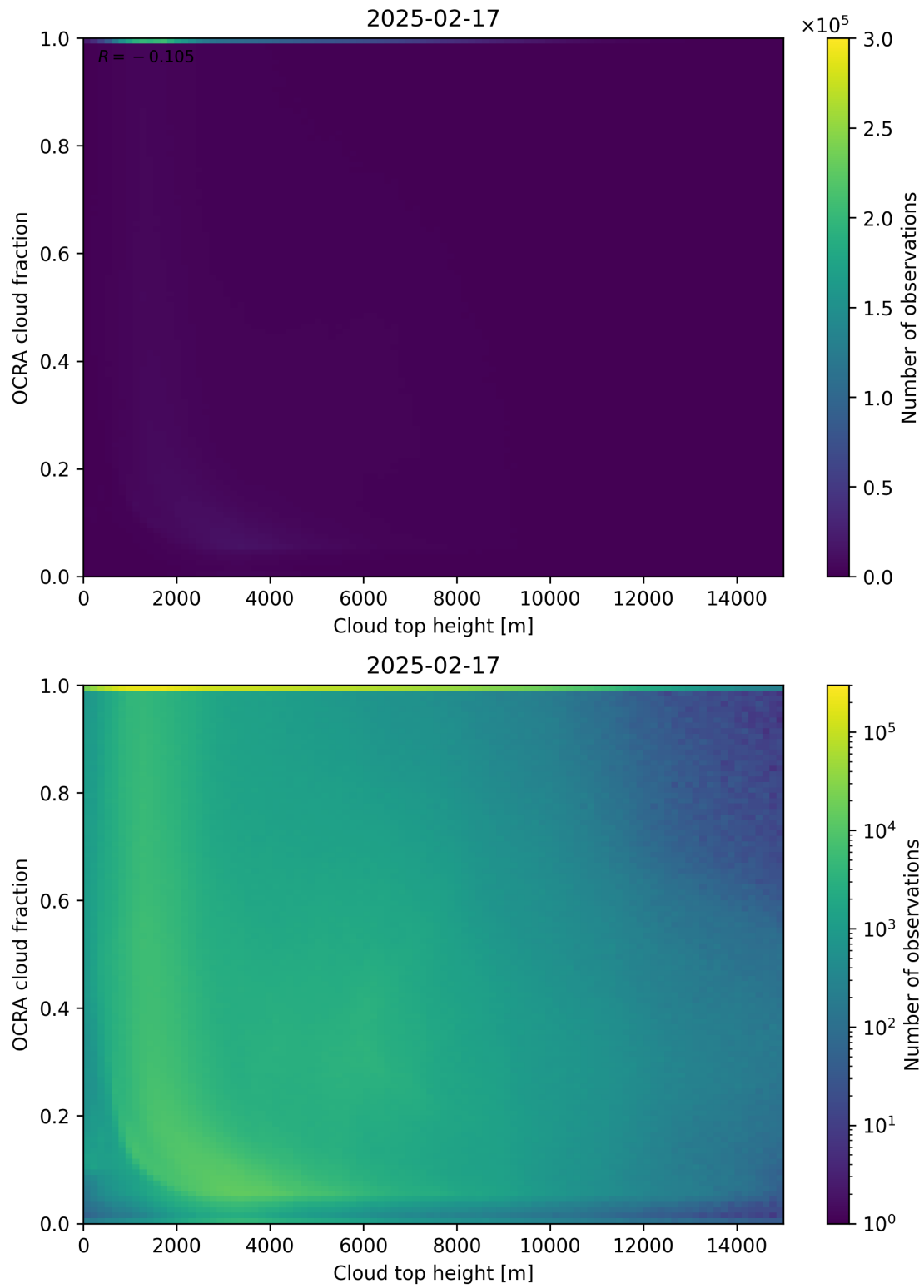
Figure 87: Scatter density plot of “Cloud top height” against “OCRA cloud fraction” for 2025-02-16 to 2025-02-18.
