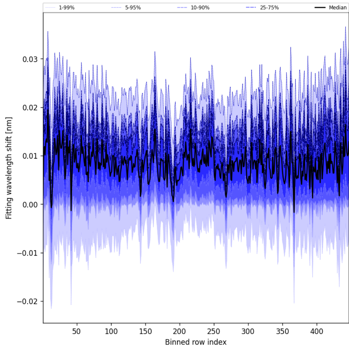
Figure 65: Along track statistics of “Fitting wavelength shift” for 2025-02-16 to 2025-02-18
