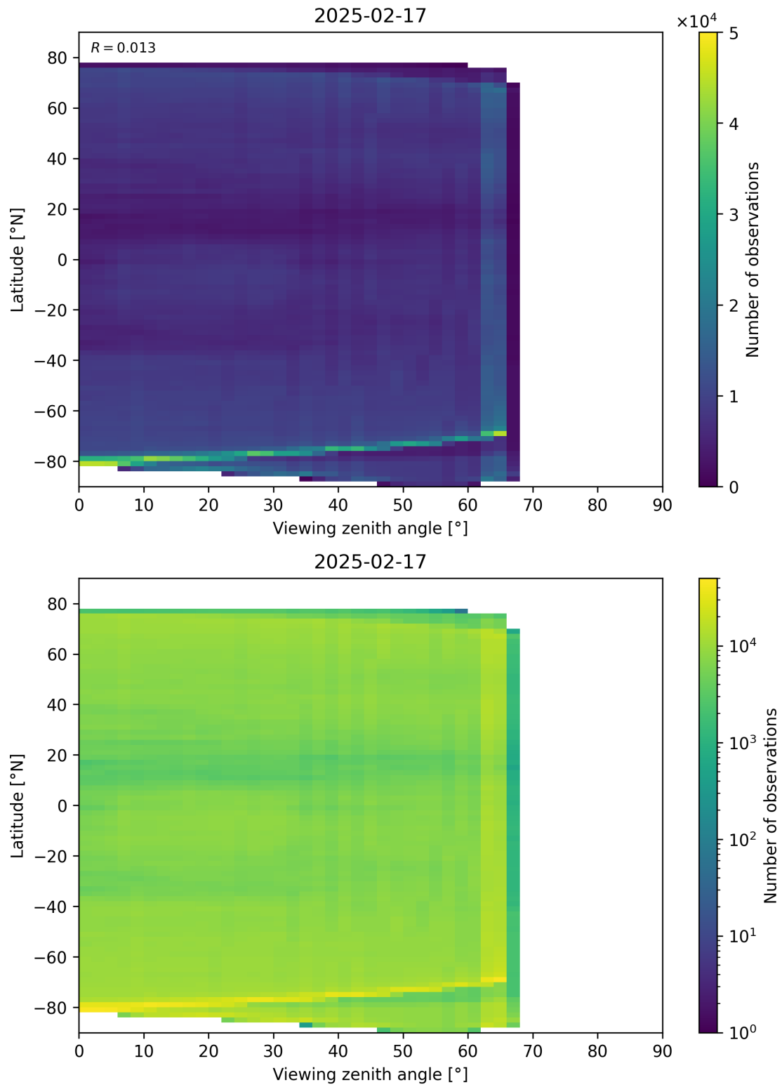
Figure 113: Scatter density plot of “Viewing zenith angle” against “Latitude” for 2025-02-16 to 2025-02-18.
