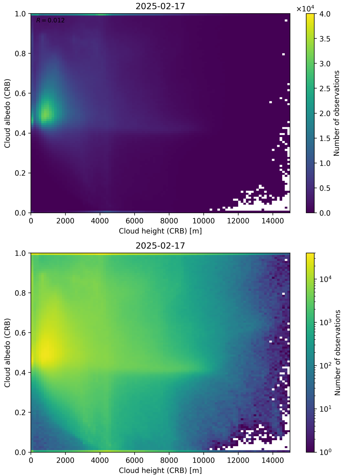
Figure 80: Scatter density plot of “Cloud height (CRB)” against “Cloud albedo (CRB)” for 2025-02-16 to 2025-02-18.
