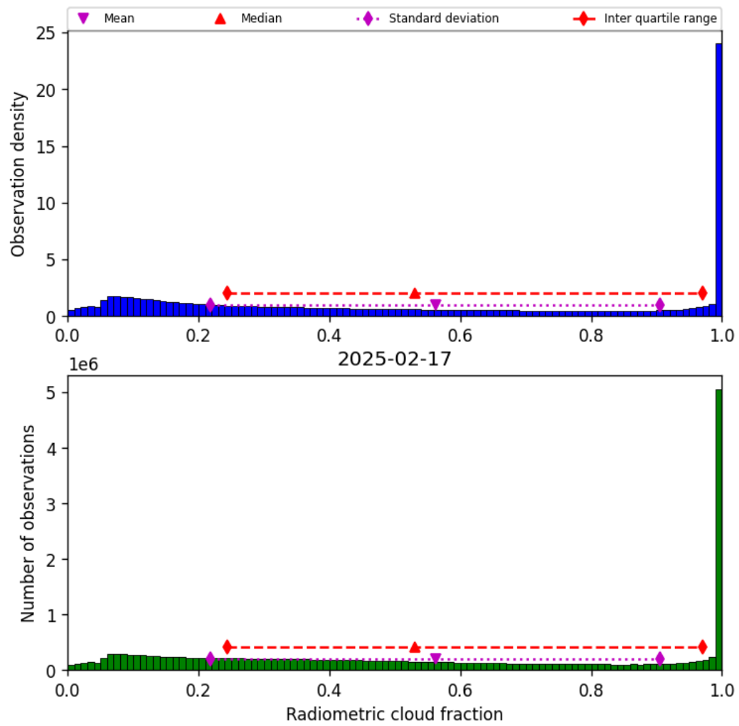
Figure 39: Histogram of “Radiometric cloud fraction” for 2025-02-16 to 2025-02-18
