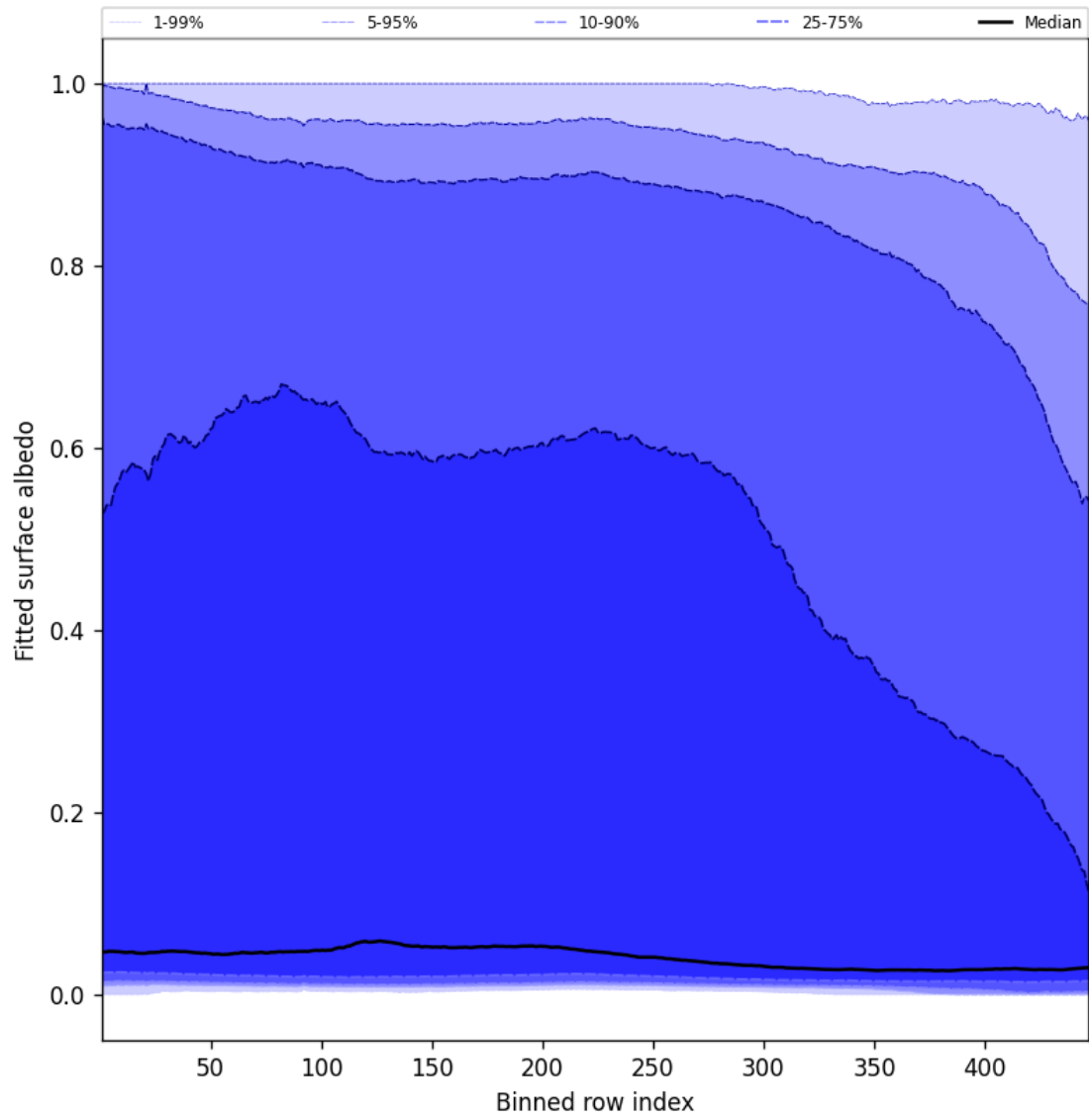
Figure 61: Along track statistics of “Fitted surface albedo” for 2025-02-16 to 2025-02-18
