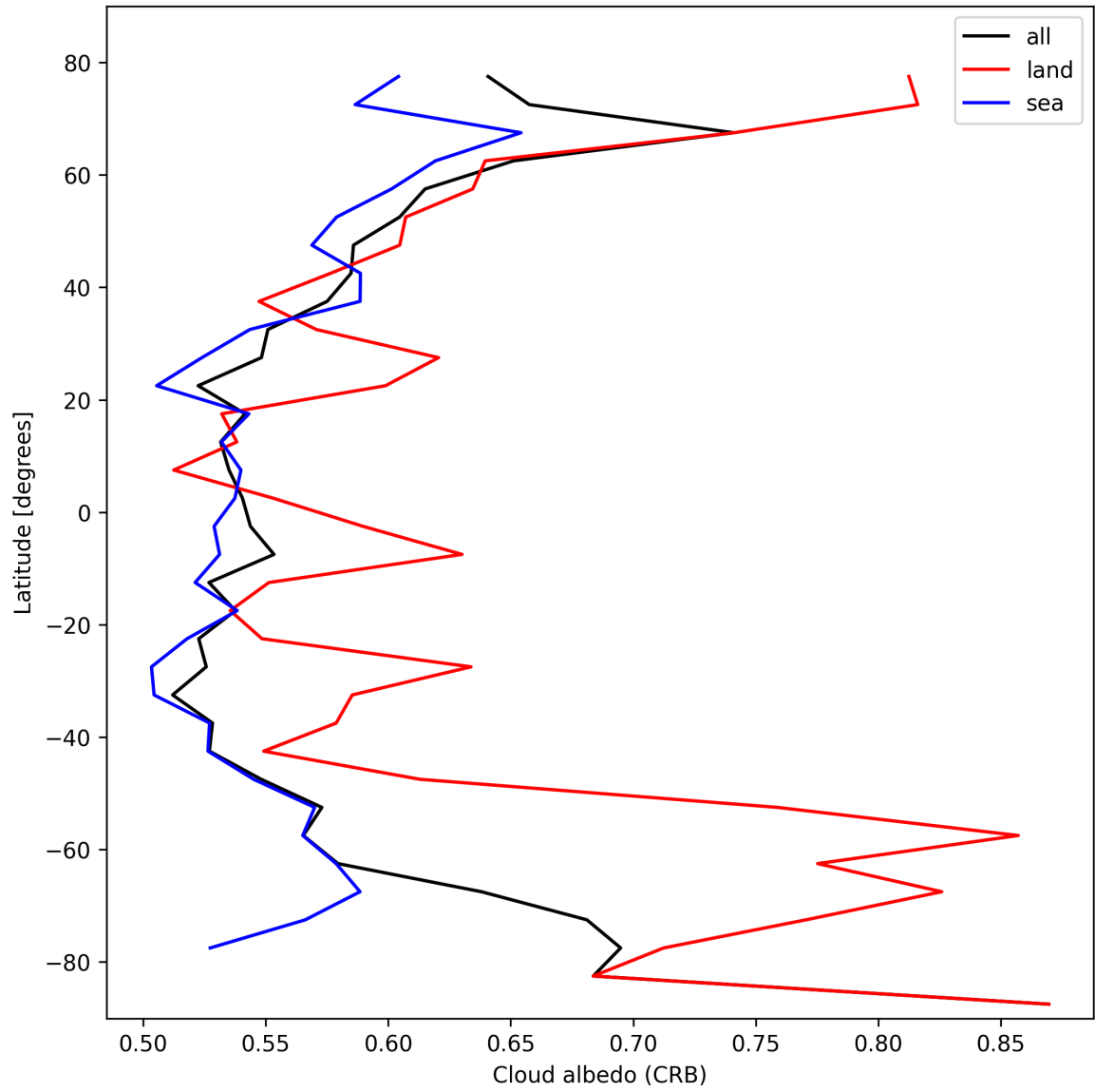
Figure 28: Zonal average of “Cloud albedo (CRB)” for 2025-02-16 to 2025-02-18.
