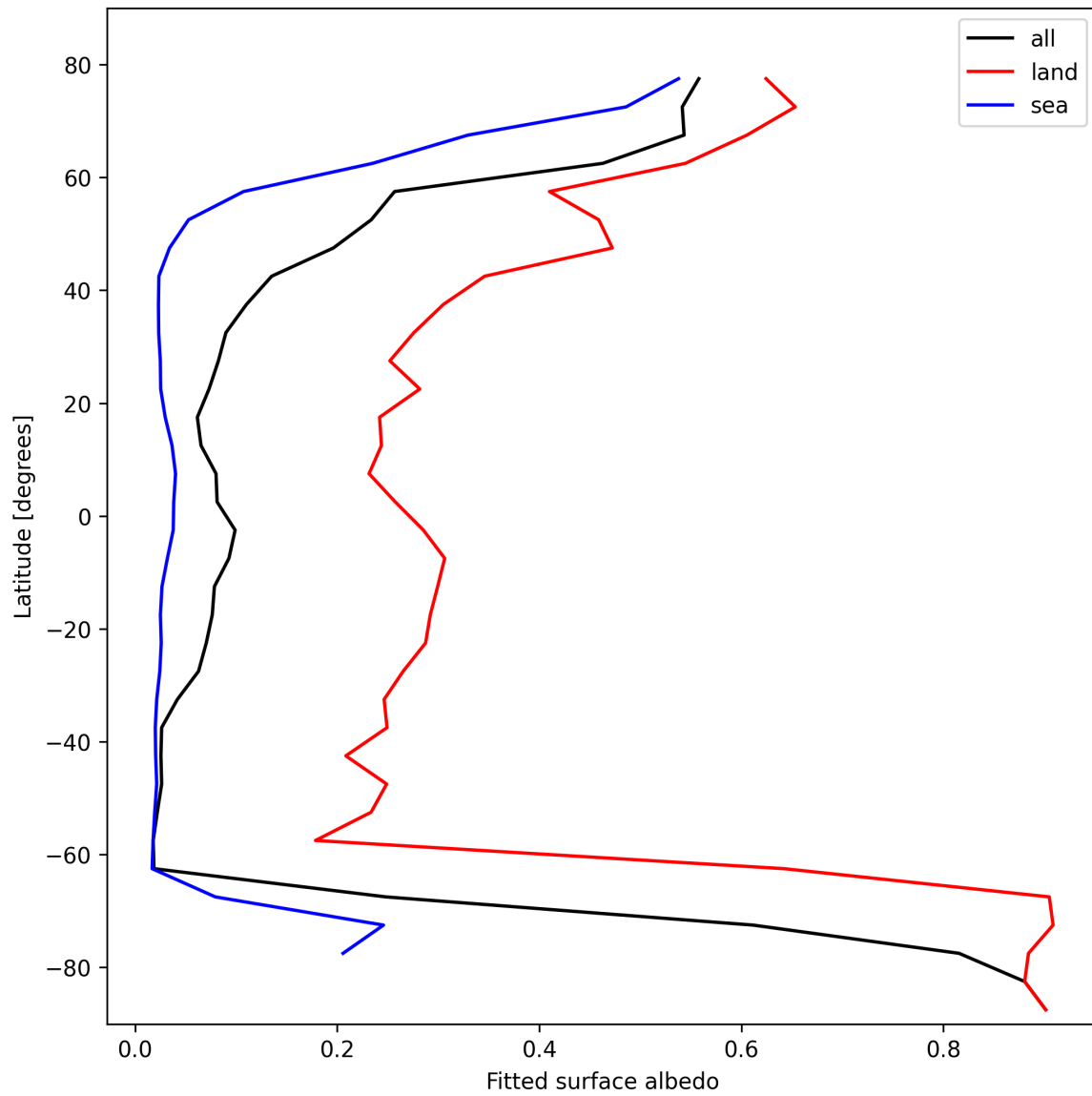
Figure 29: Zonal average of “Fitted surface albedo” for 2025-02-16 to 2025-02-18.
