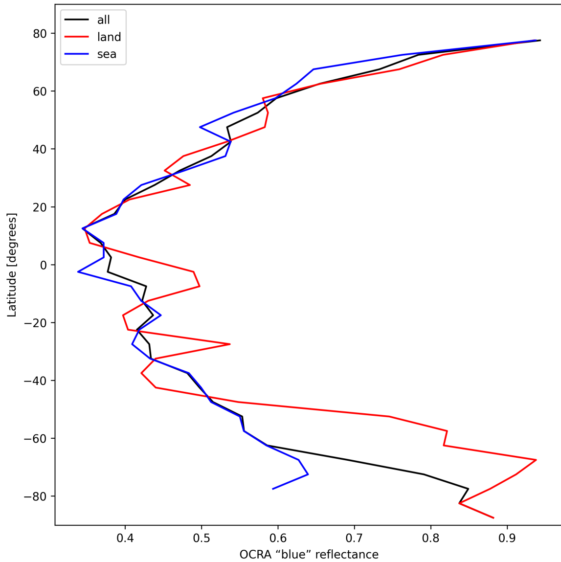
Figure 35: Zonal average of “OCRA “blue” reflectance” for 2025-02-16 to 2025-02-18.
