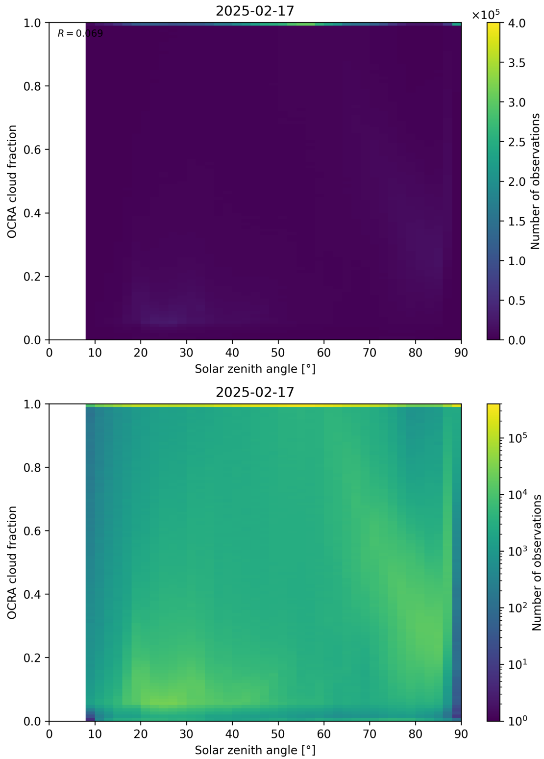
Figure 100: Scatter density plot of “Solar zenith angle” against “OCRA cloud fraction” for 2025-02-16 to 2025-02-18.
