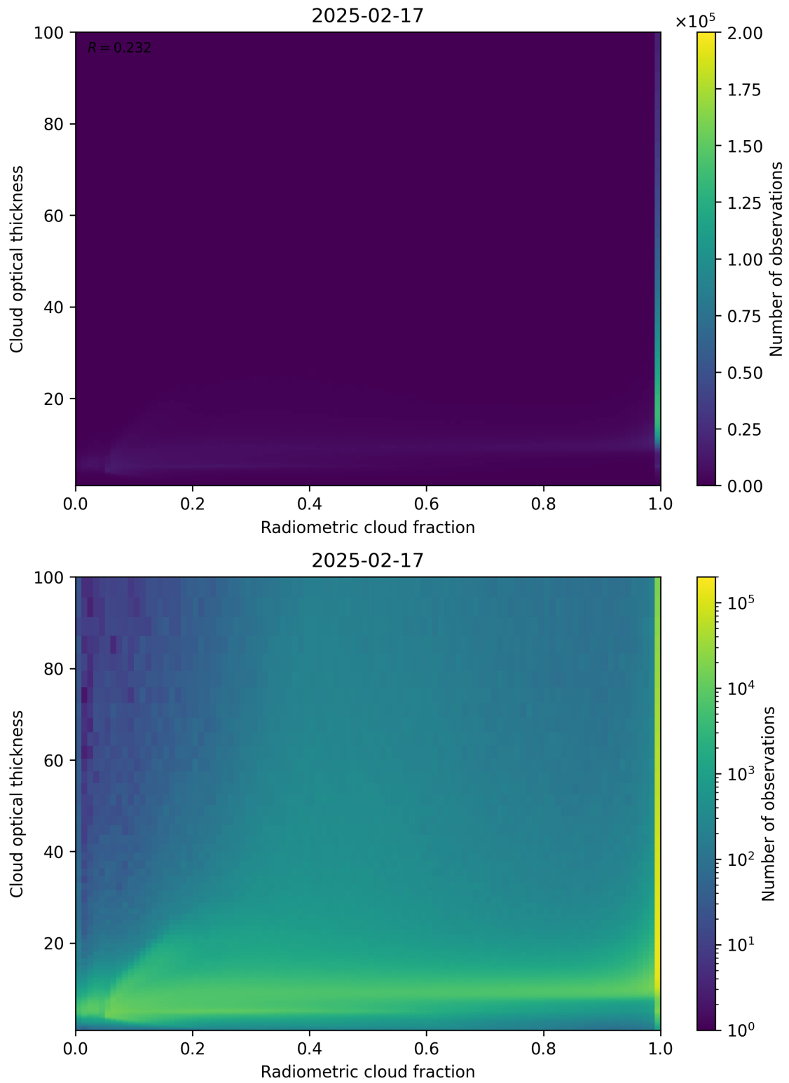
Figure 75: Scatter density plot of “Radiometric cloud fraction” against “Cloud optical thickness” for 2025-02-16 to 2025-02-18.
