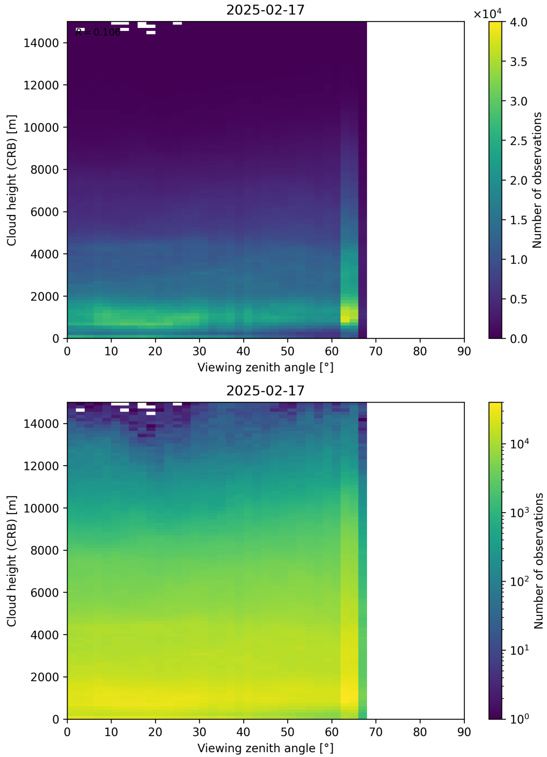
Figure 110: Scatter density plot of “Viewing zenith angle” against “Cloud height (CRB)” for 2025-02-16 to 2025-02-18.
