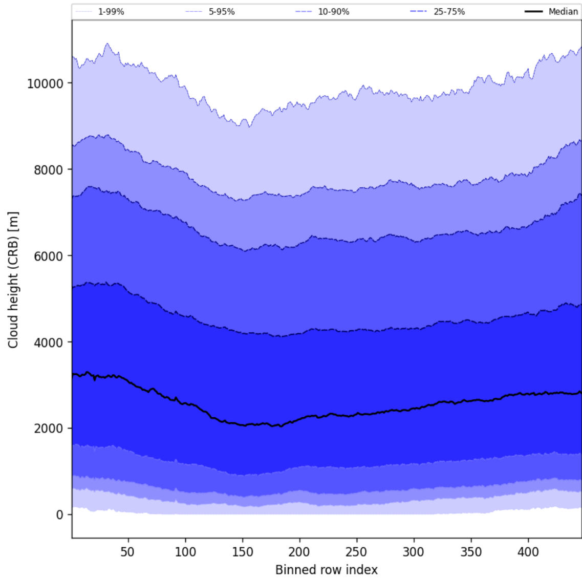
Figure 59: Along track statistics of “Cloud height (CRB)” for 2025-02-16 to 2025-02-18
