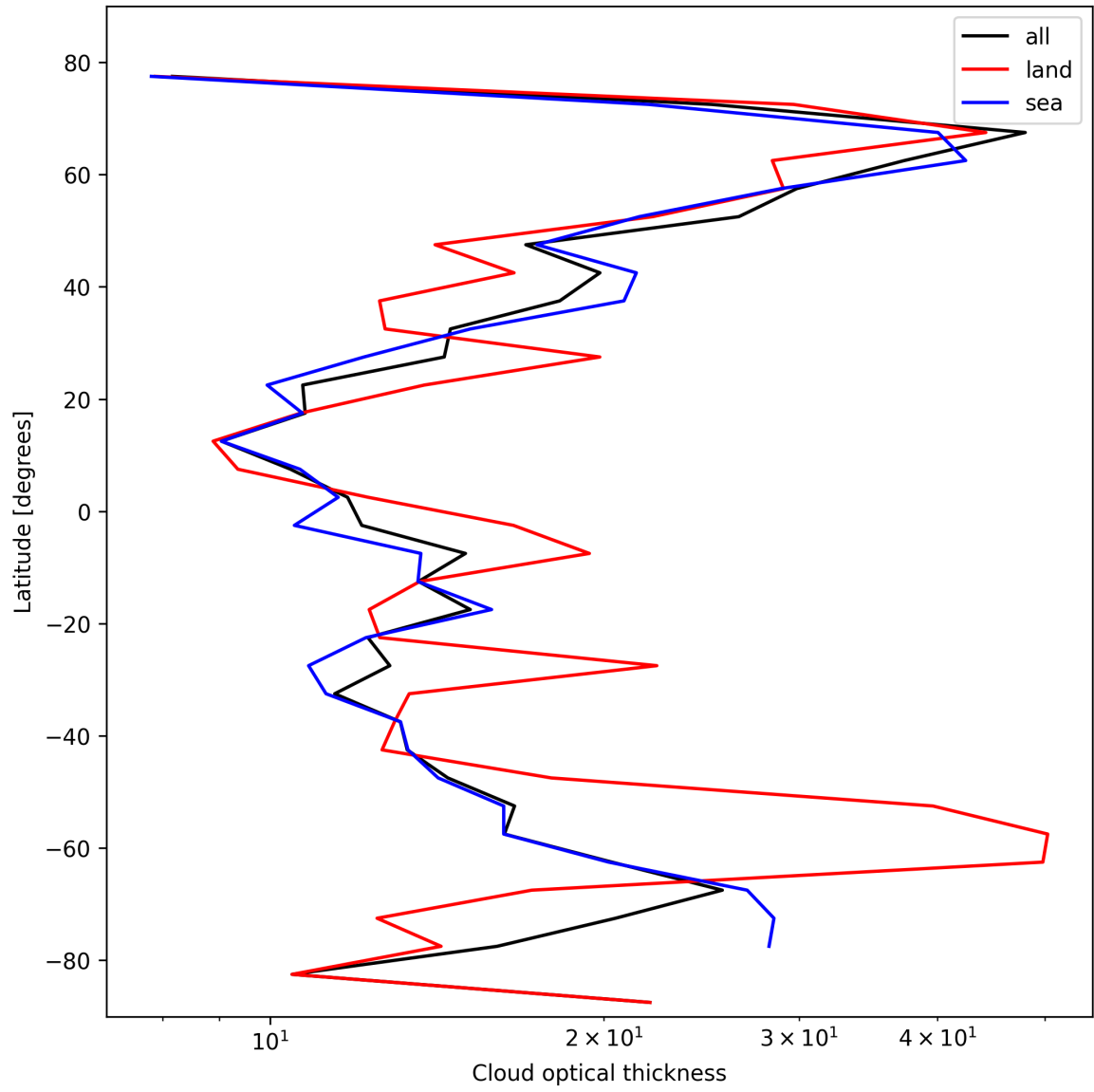
Figure 25: Zonal average of “Cloud optical thickness” for 2025-02-16 to 2025-02-18.
