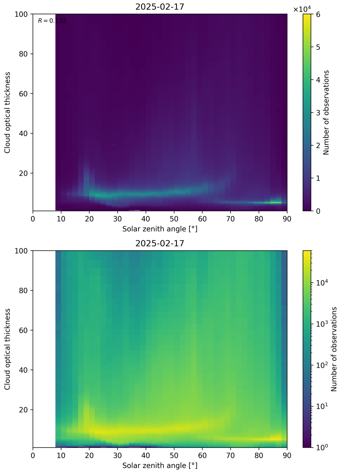
Figure 103: Scatter density plot of “Solar zenith angle” against “Cloud optical thickness” for 2025-02-16 to 2025-02-18.
