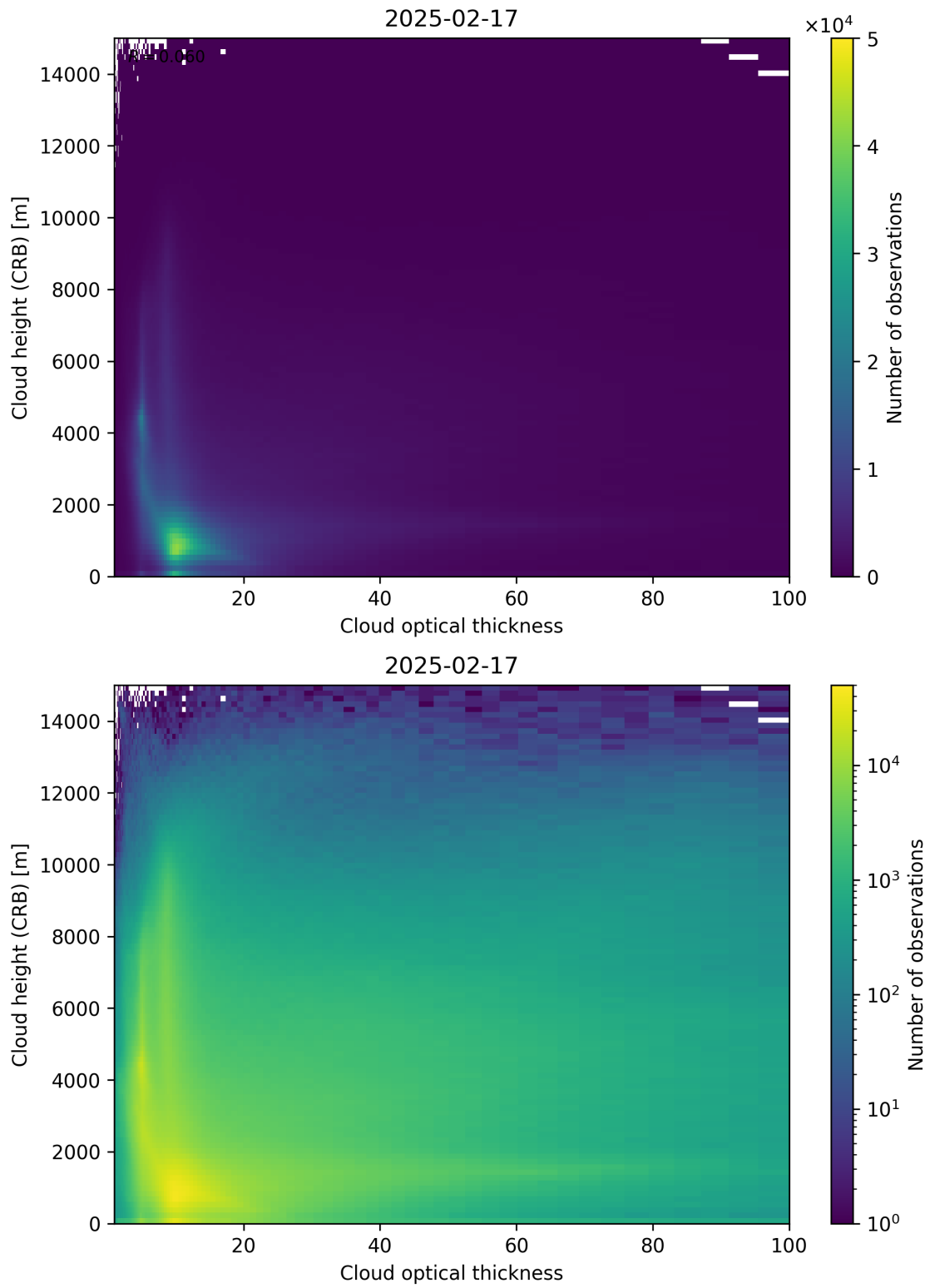
Figure 85: Scatter density plot of “Cloud optical thickness” against “Cloud height (CRB)” for 2025-02-16 to 2025-02-18.
