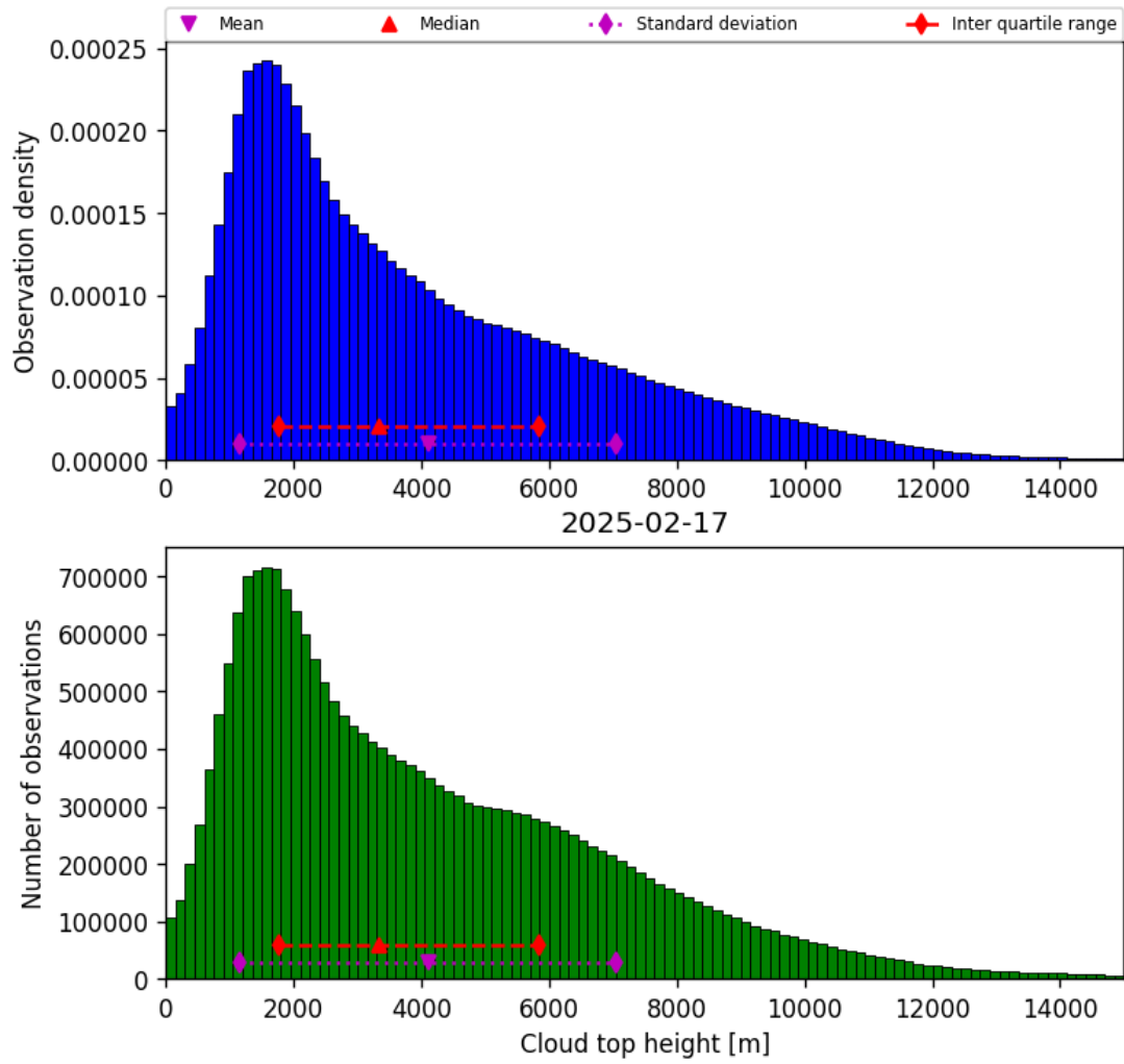
Figure 40: Histogram of “Cloud top height” for 2025-02-16 to 2025-02-18
