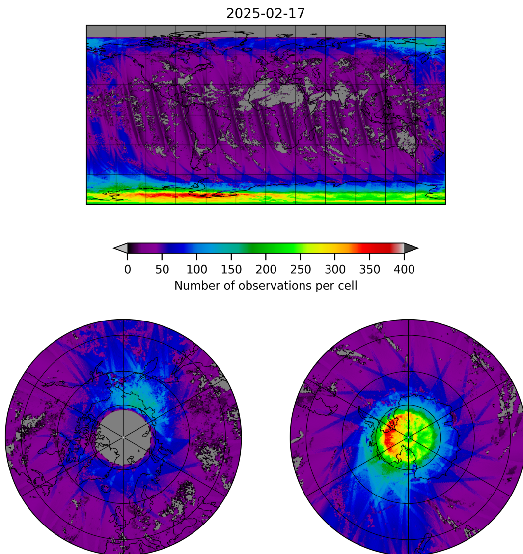
Figure 21: Map of the number of observations for 2025-02-16 to 2025-02-18
