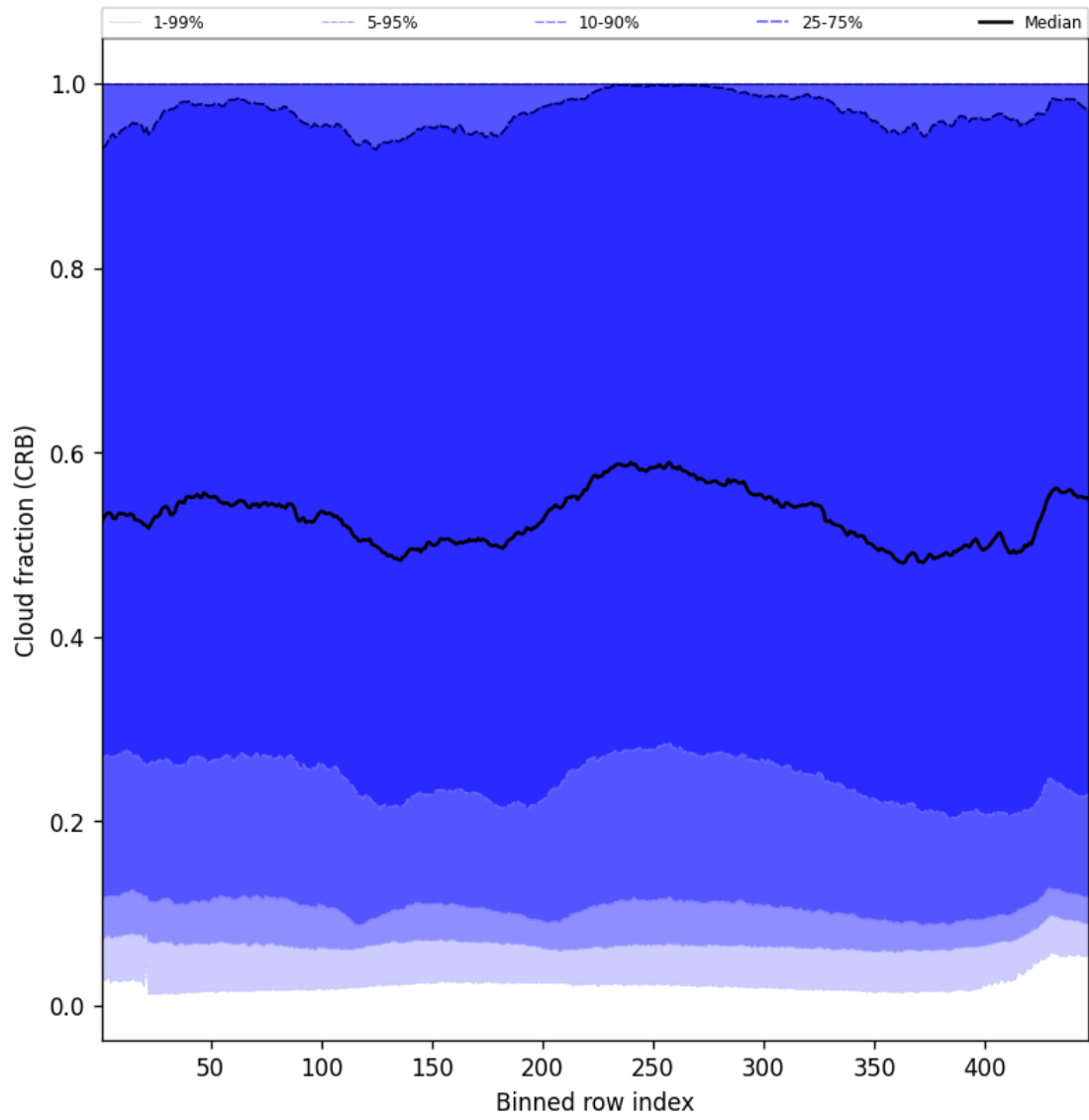
Figure 58: Along track statistics of “Cloud fraction (CRB)” for 2025-02-16 to 2025-02-18
