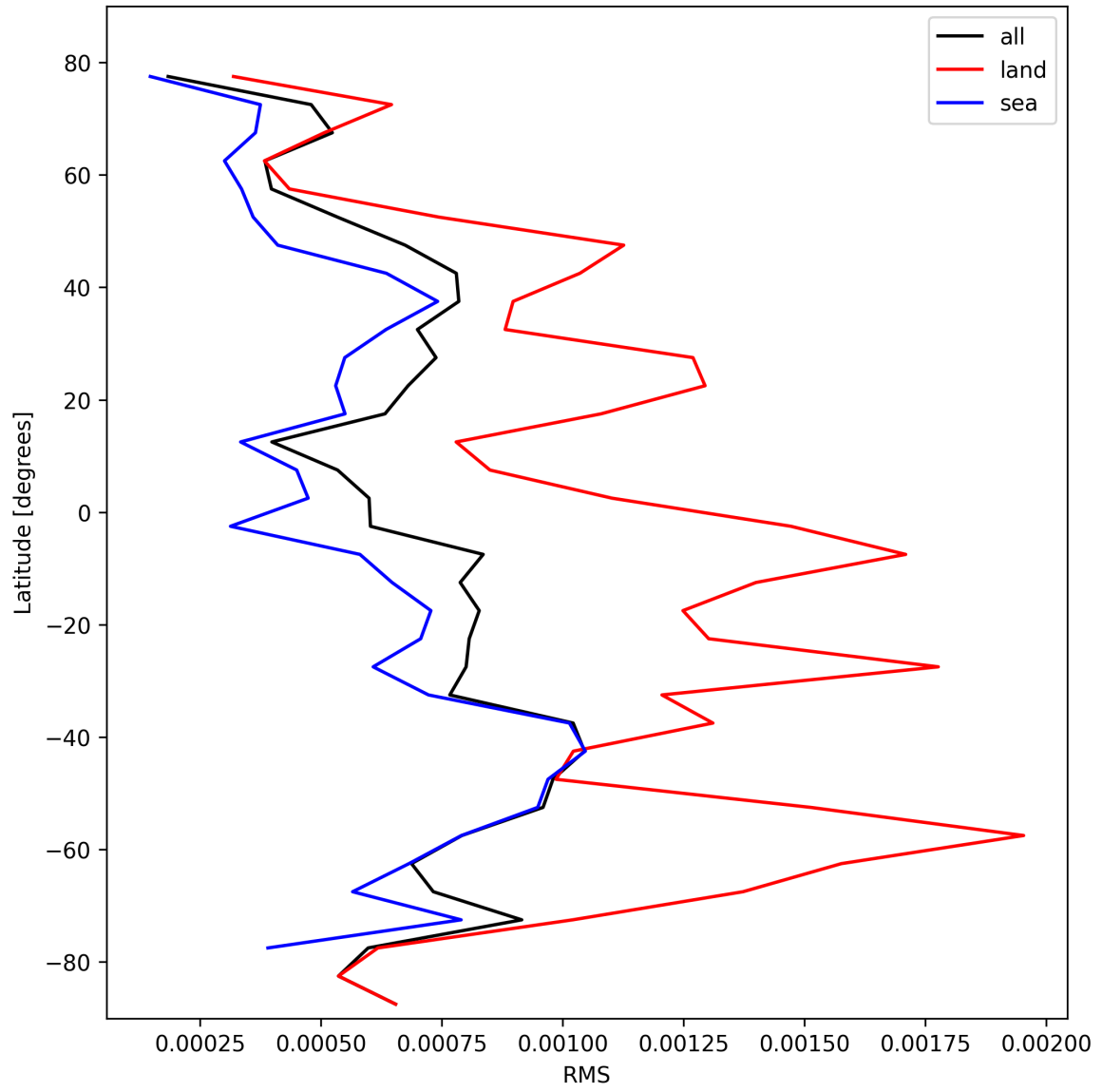
Figure 31: Zonal average of “RMS” for 2025-02-16 to 2025-02-18.
