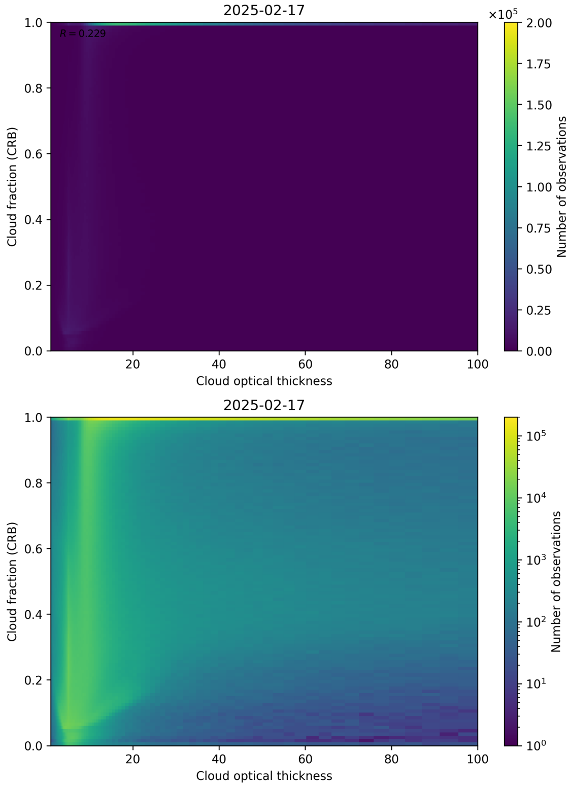
Figure 84: Scatter density plot of “Cloud optical thickness” against “Cloud fraction (CRB)” for 2025-02-16 to 2025-02-18.
