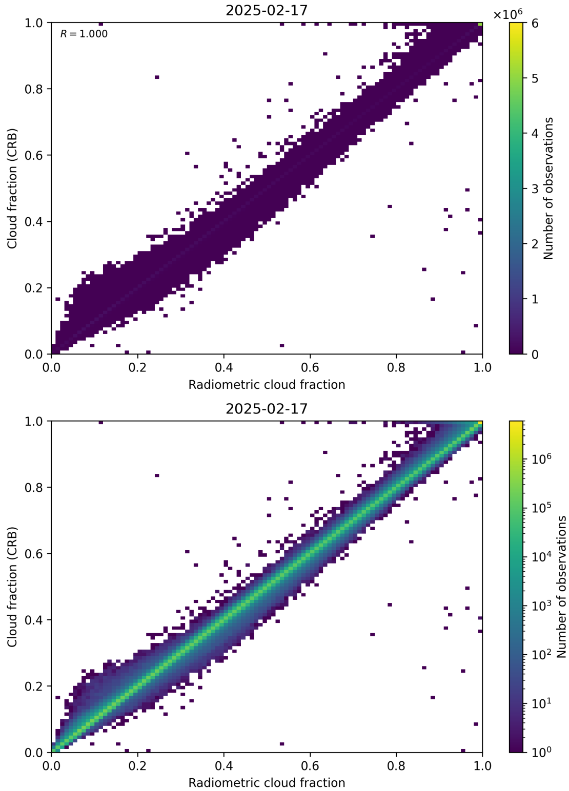
Figure 73: Scatter density plot of “Radiometric cloud fraction” against “Cloud fraction (CRB)” for 2025-02-16 to 2025-02-18.
