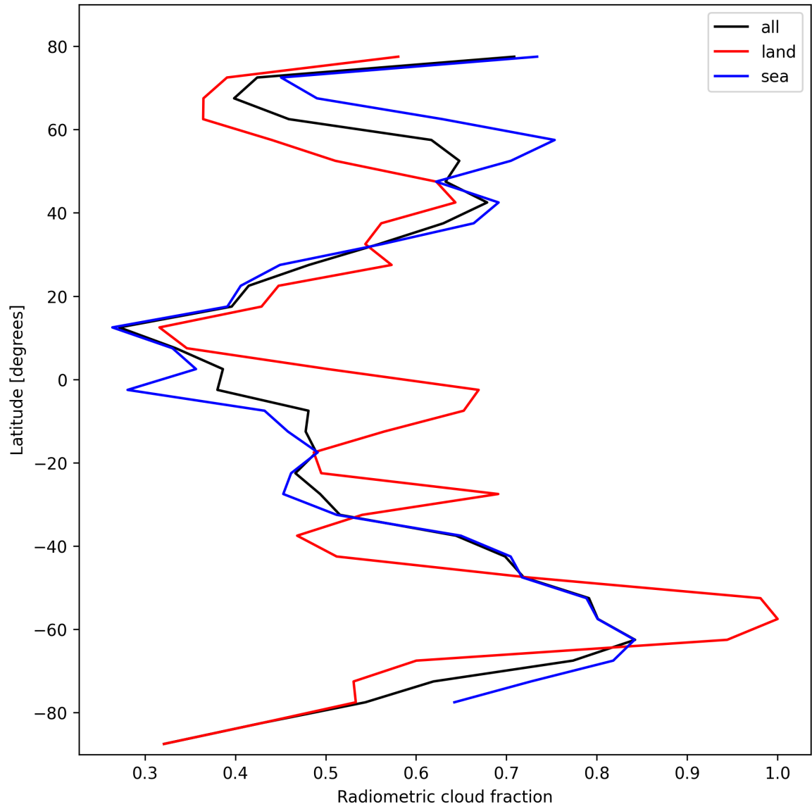
Figure 23: Zonal average of “Radiometric cloud fraction” for 2025-02-16 to 2025-02-18.
