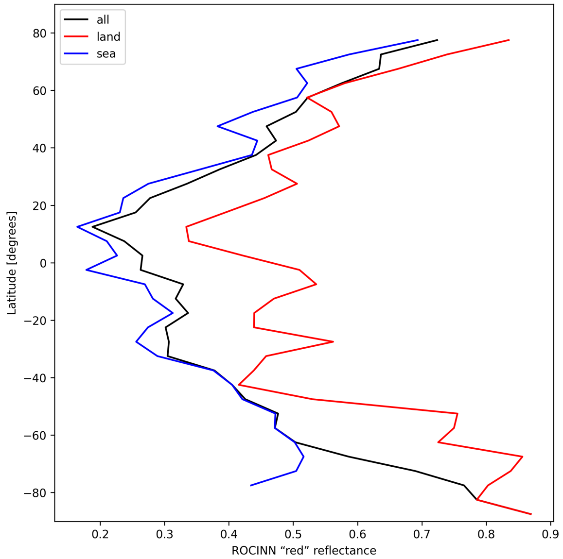
Figure 37: Zonal average of “ROCINN “red” reflectance” for 2025-02-16 to 2025-02-18.
