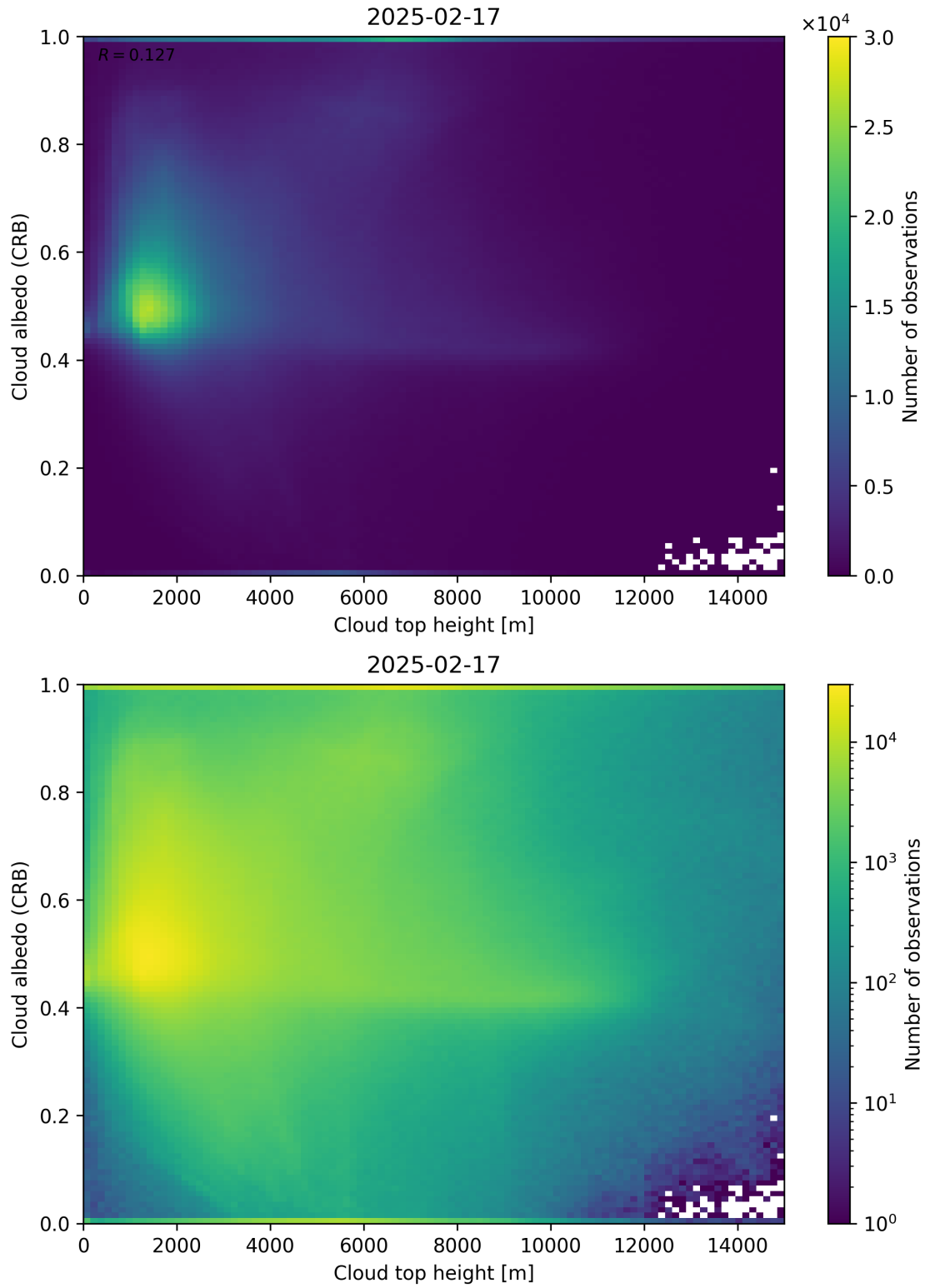
Figure 86: Scatter density plot of “Cloud top height” against “Cloud albedo (CRB)” for 2025-02-16 to 2025-02-18.
