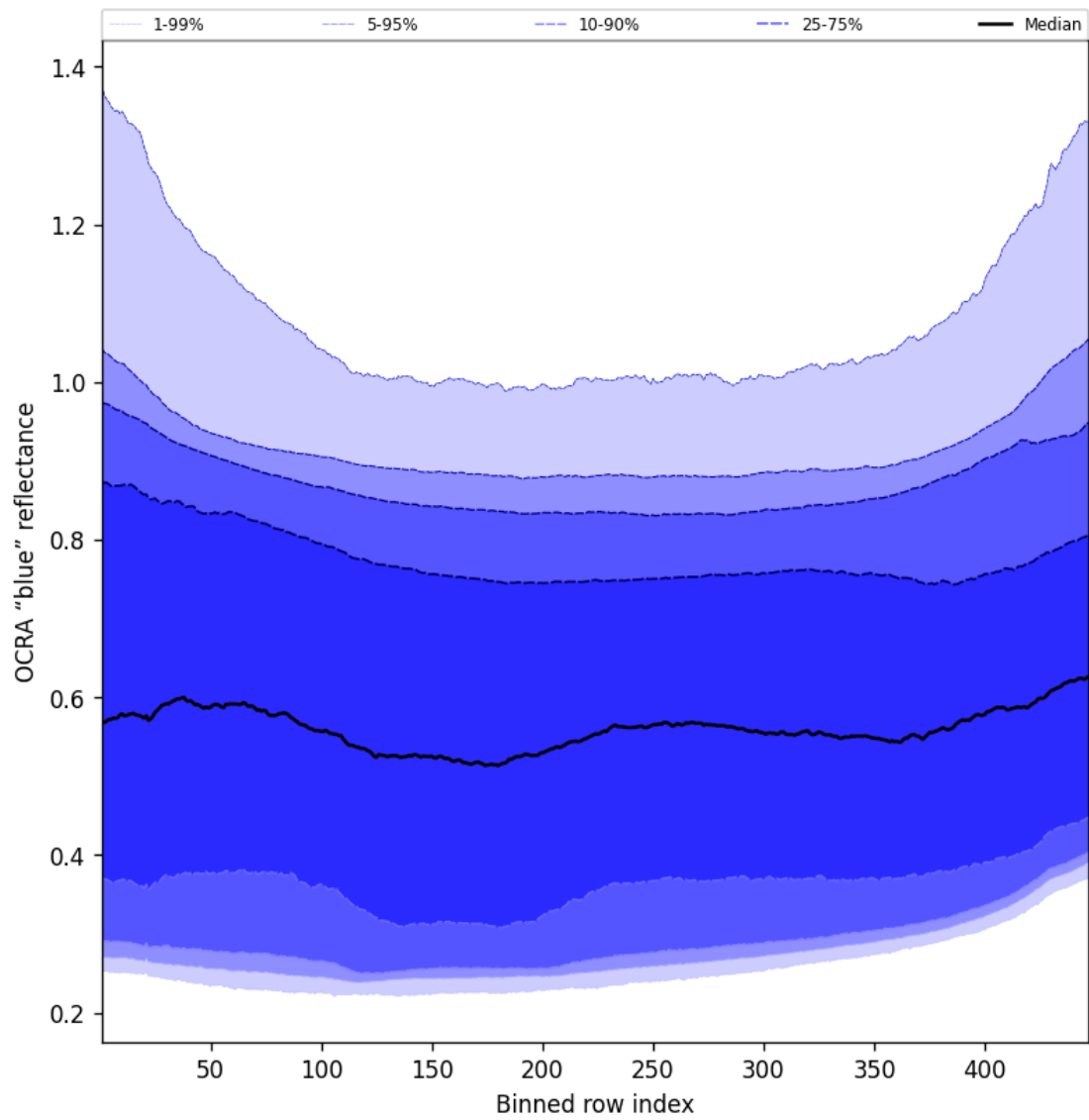
Figure 67: Along track statistics of “OCRA “blue” reflectance” for 2025-02-16 to 2025-02-18
