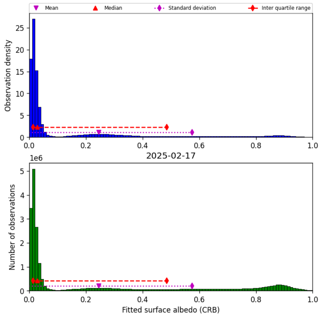
Figure 46: Histogram of “Fitted surface albedo (CRB)” for 2025-02-16 to 2025-02-18
