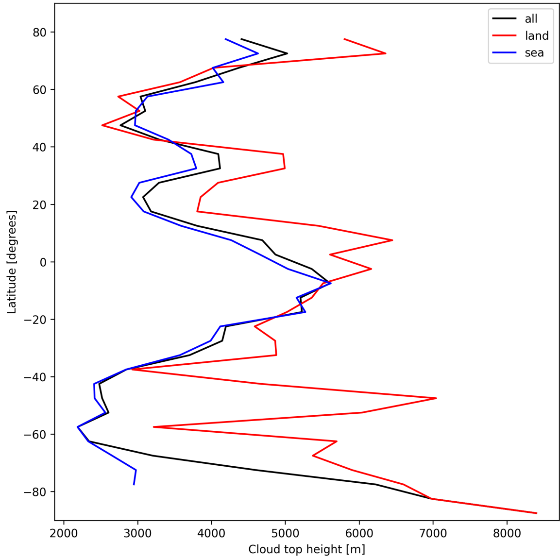
Figure 24: Zonal average of “Cloud top height” for 2025-02-16 to 2025-02-18.
