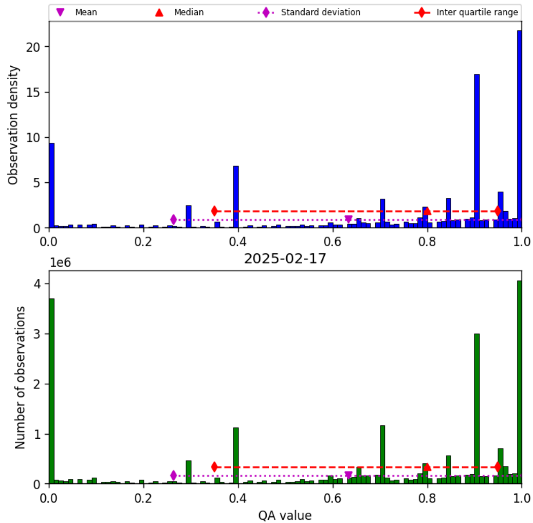
Figure 38: Histogram of “QA value” for 2025-02-16 to 2025-02-18
