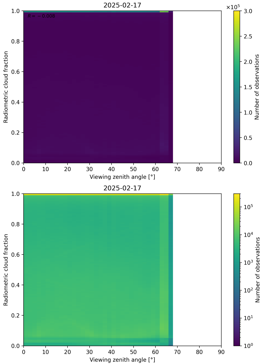
Figure 107: Scatter density plot of “Viewing zenith angle” against “Radiometric cloud fraction” for 2025-02-16 to 2025-02-18.
