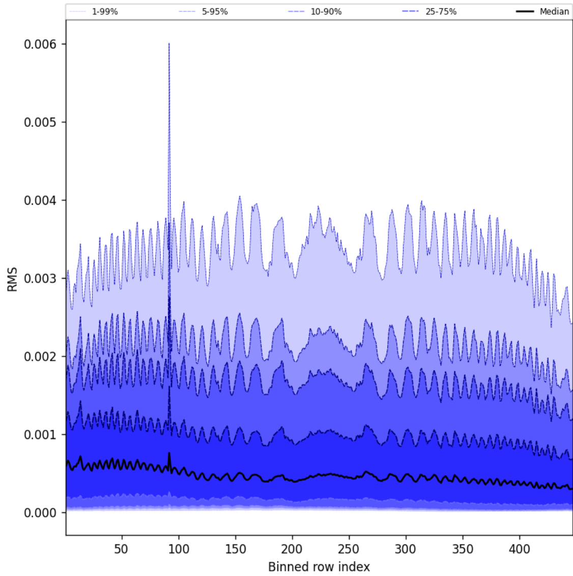
Figure 63: Along track statistics of “RMS” for 2025-02-16 to 2025-02-18
