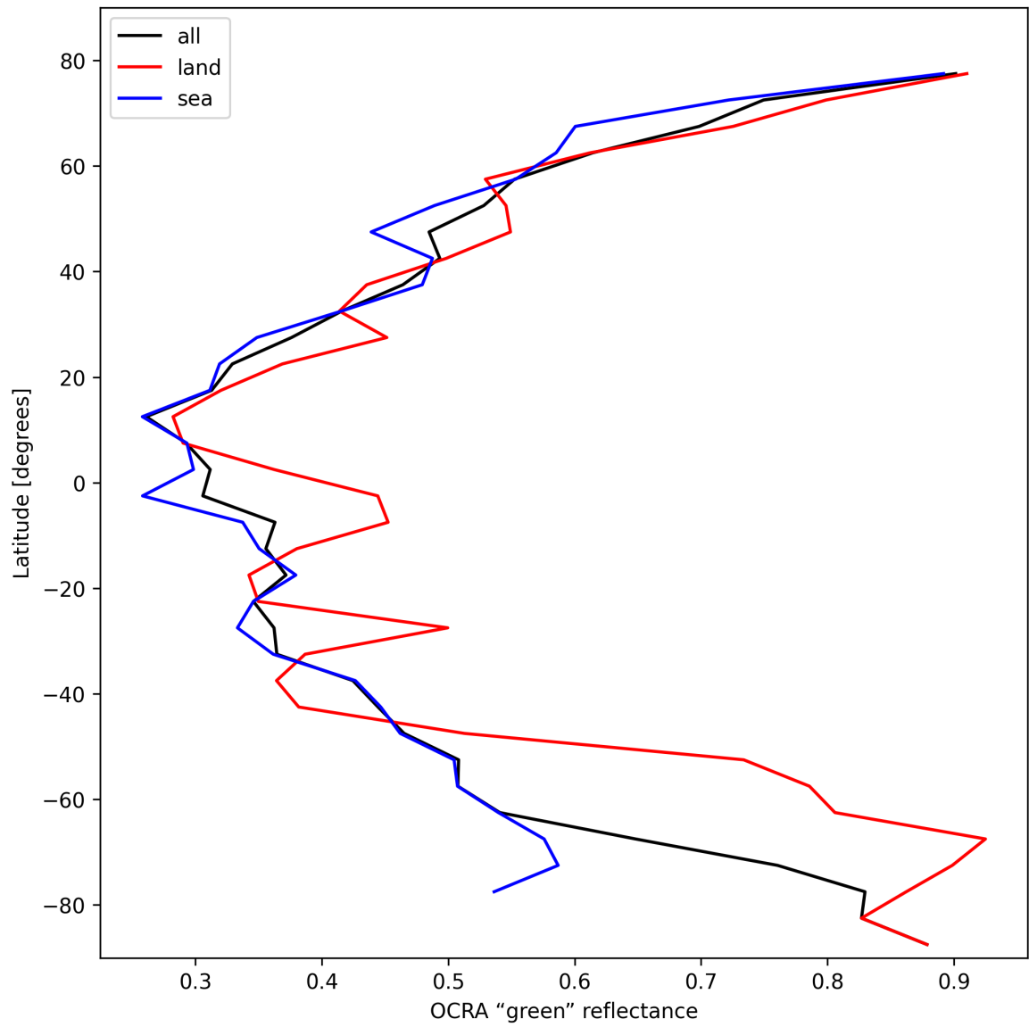
Figure 36: Zonal average of “OCRA “green” reflectance” for 2025-02-16 to 2025-02-18.
