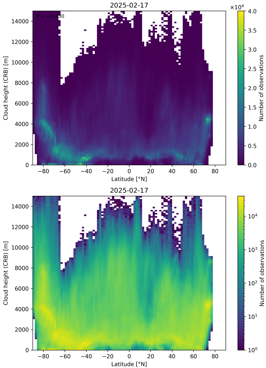
Figure 95: Scatter density plot of “Latitude” against “Cloud height (CRB)” for 2025-02-16 to 2025-02-18.
