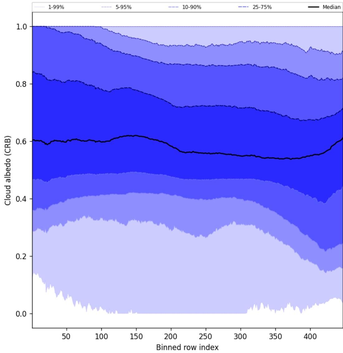
Figure 60: Along track statistics of “Cloud albedo (CRB)” for 2025-02-16 to 2025-02-18
