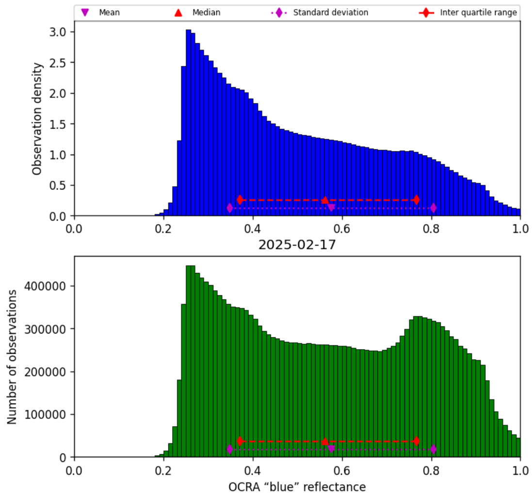
Figure 51: Histogram of “OCRA “blue” reflectance” for 2025-02-16 to 2025-02-18
