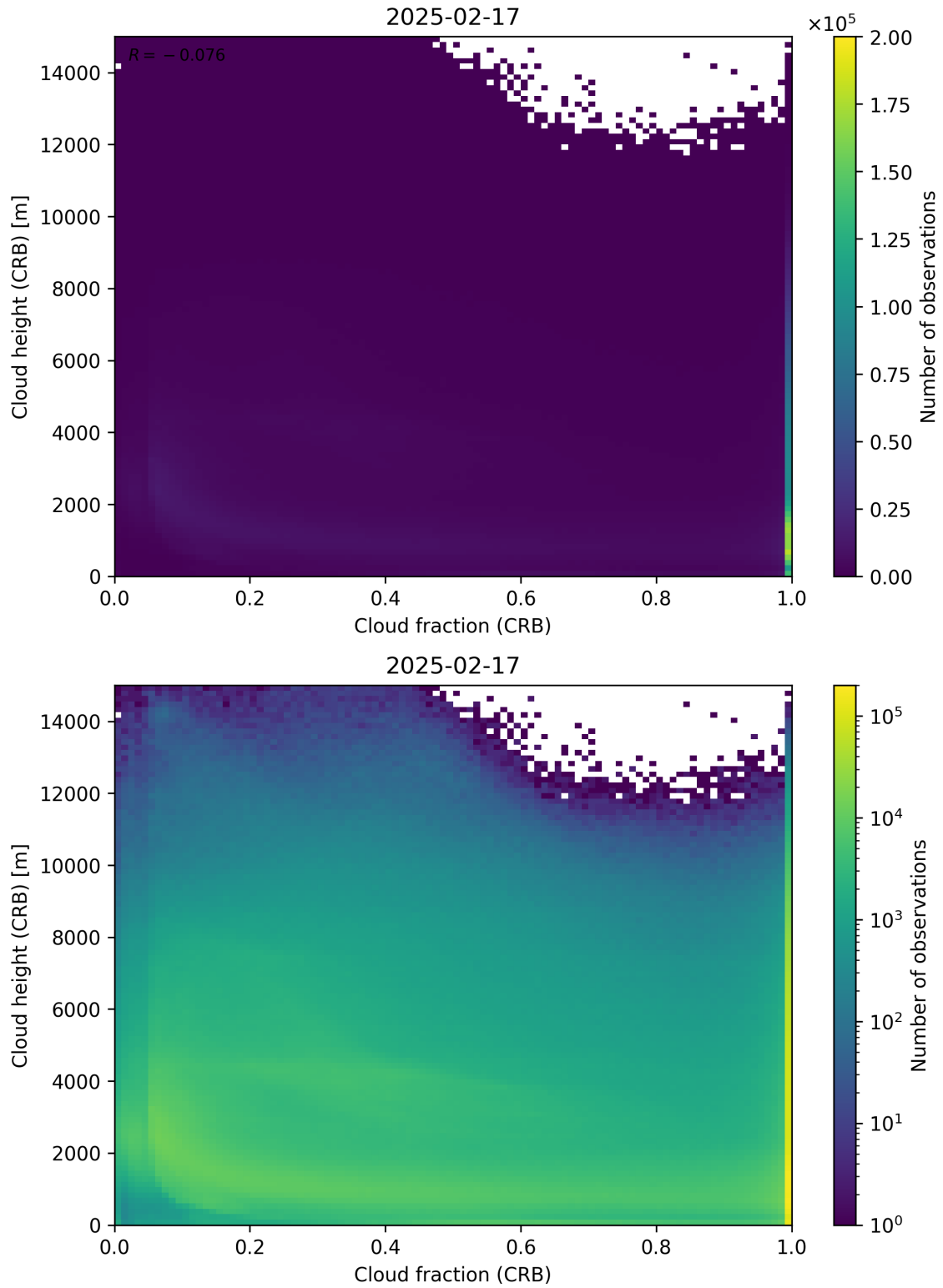
Figure 79: Scatter density plot of “Cloud fraction (CRB)” against “Cloud height (CRB)” for 2025-02-16 to 2025-02-18.
