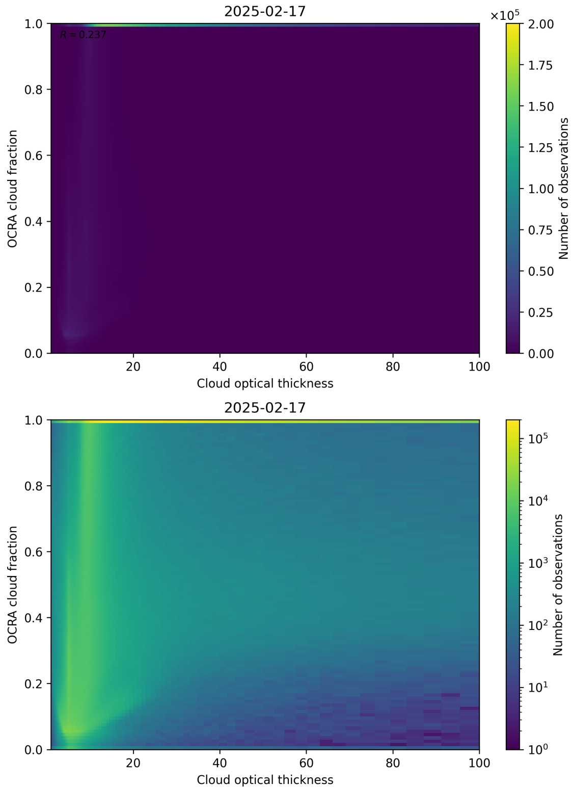
Figure 83: Scatter density plot of “Cloud optical thickness” against “OCRA cloud fraction” for 2025-02-16 to 2025-02-18.
