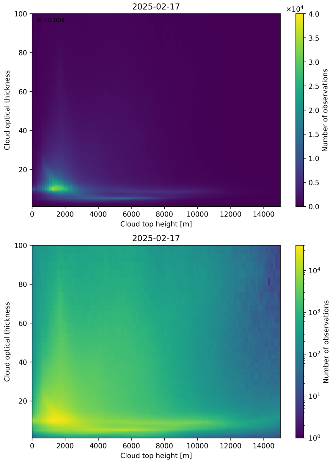
Figure 90: Scatter density plot of “Cloud top height” against “Cloud optical thickness” for 2025-02-16 to 2025-02-18.
