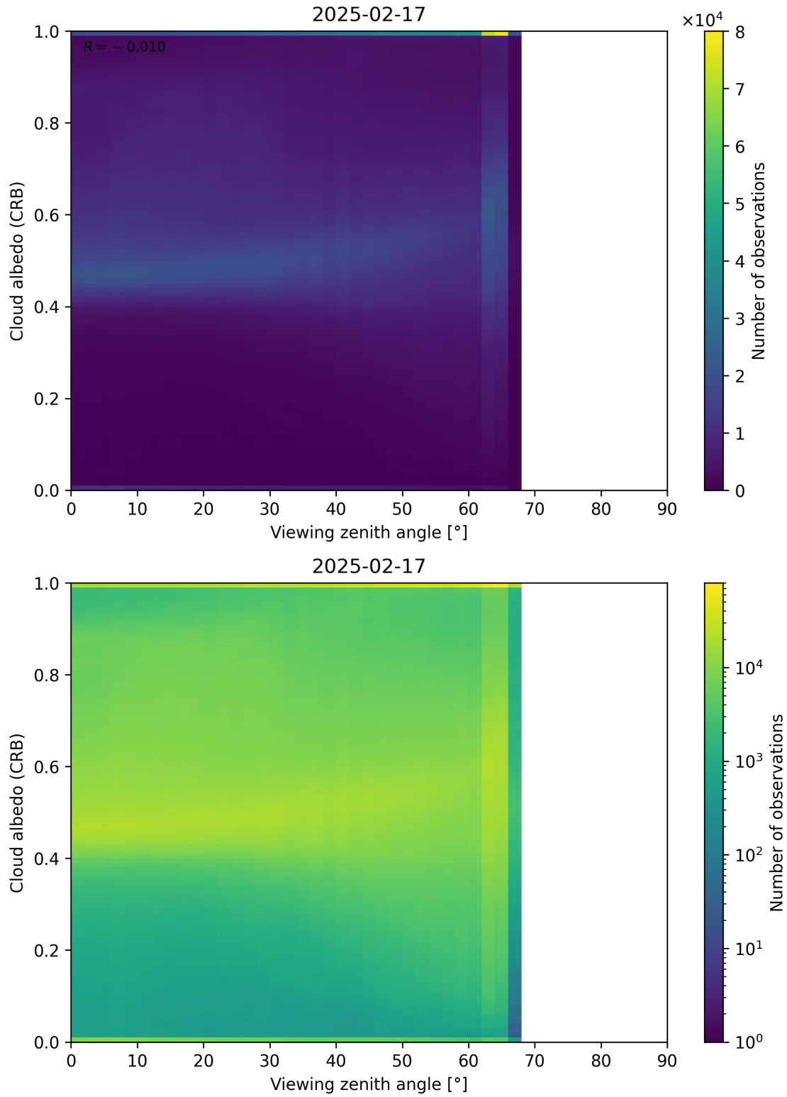
Figure 106: Scatter density plot of “Viewing zenith angle” against “Cloud albedo (CRB)” for 2025-02-16 to 2025-02-18.
