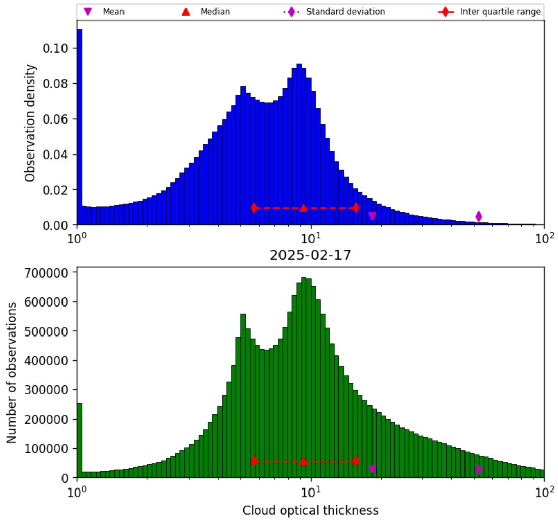
Figure 41: Histogram of “Cloud optical thickness” for 2025-02-16 to 2025-02-18
