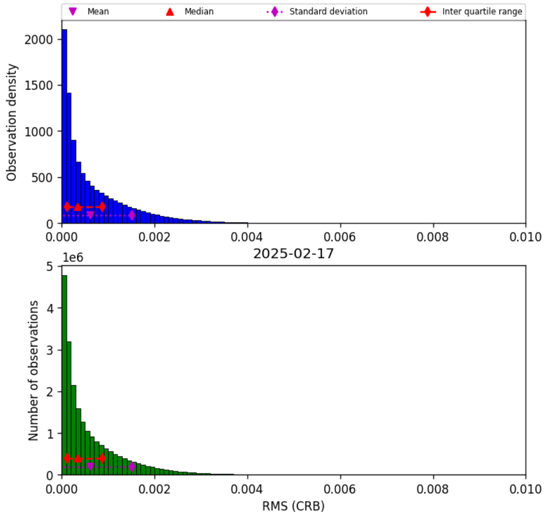
Figure 48: Histogram of “RMS (CRB)” for 2025-02-16 to 2025-02-18
