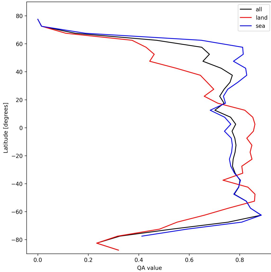
Figure 22: Zonal average of “QA value” for 2025-02-16 to 2025-02-18.
