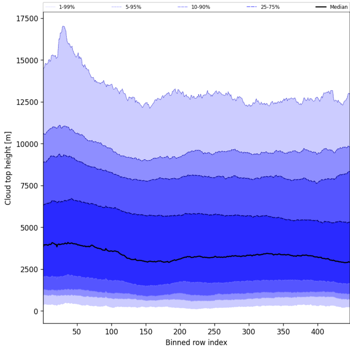
Figure 56: Along track statistics of “Cloud top height” for 2025-02-16 to 2025-02-18
