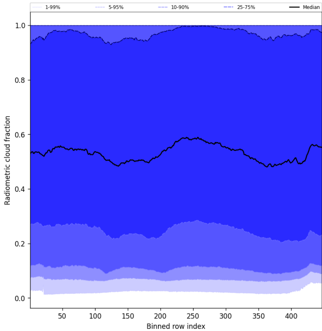
Figure 55: Along track statistics of “Radiometric cloud fraction” for 2025-02-16 to 2025-02-18
