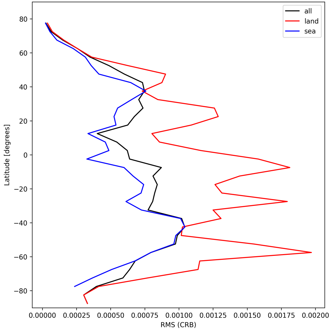
Figure 32: Zonal average of “RMS (CRB)” for 2025-02-16 to 2025-02-18.
