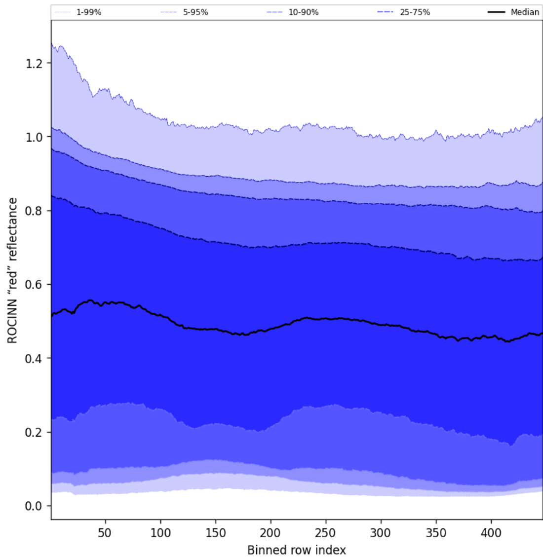
Figure 69: Along track statistics of "ROCINN "red" reflectance" for 2025-02-16 to 2025-02-18
