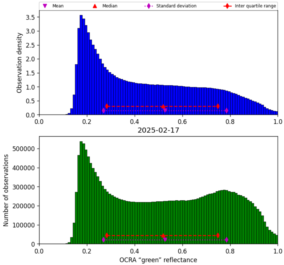
Figure 52: Histogram of “OCRA “green” reflectance” for 2025-02-16 to 2025-02-18
