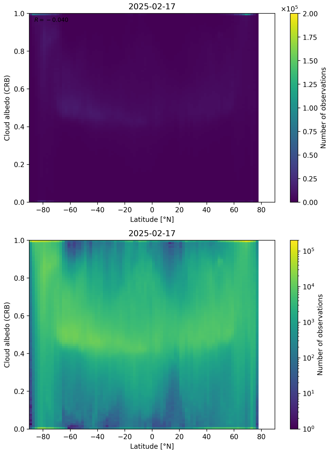
Figure 91: Scatter density plot of “Latitude” against “Cloud albedo (CRB)” for 2025-02-16 to 2025-02-18.
