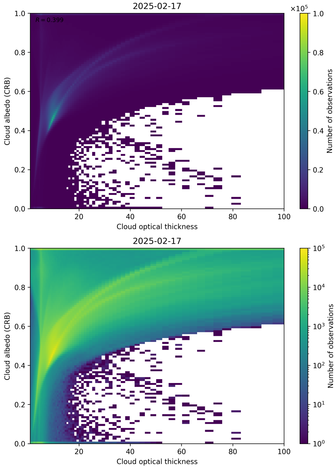
Figure 82: Scatter density plot of “Cloud optical thickness” against “Cloud albedo (CRB)” for 2025-02-16 to 2025-02-18.
