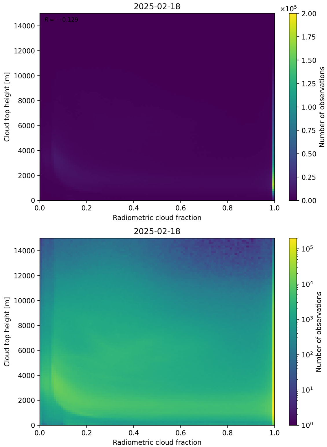
Figure 76: Scatter density plot of “Radiometric cloud fraction” against “Cloud top height” for 2025-02-18 to 2025-02-19.
