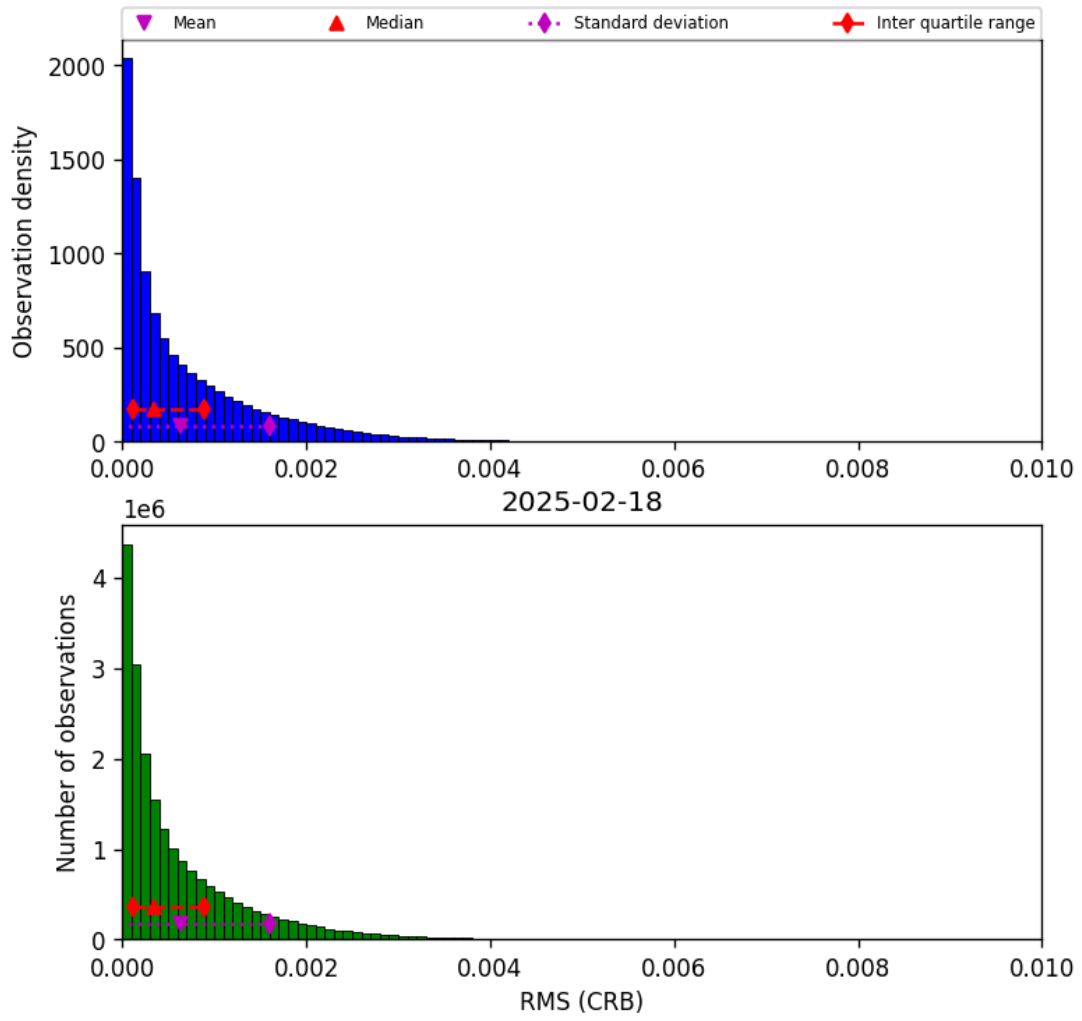
Figure 48: Histogram of “RMS (CRB)” for 2025-02-18 to 2025-02-19
