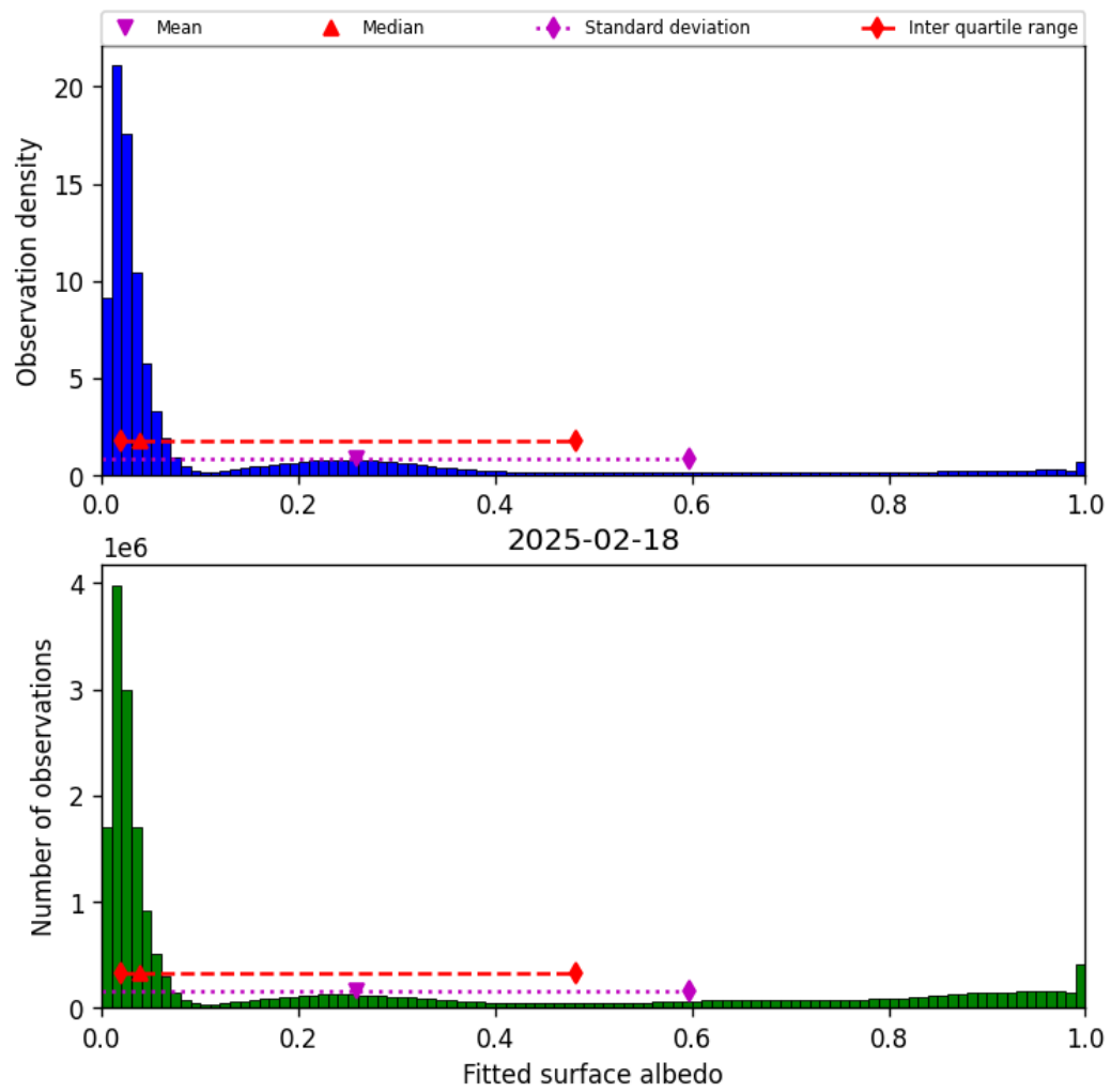
Figure 45: Histogram of “Fitted surface albedo” for 2025-02-18 to 2025-02-19
