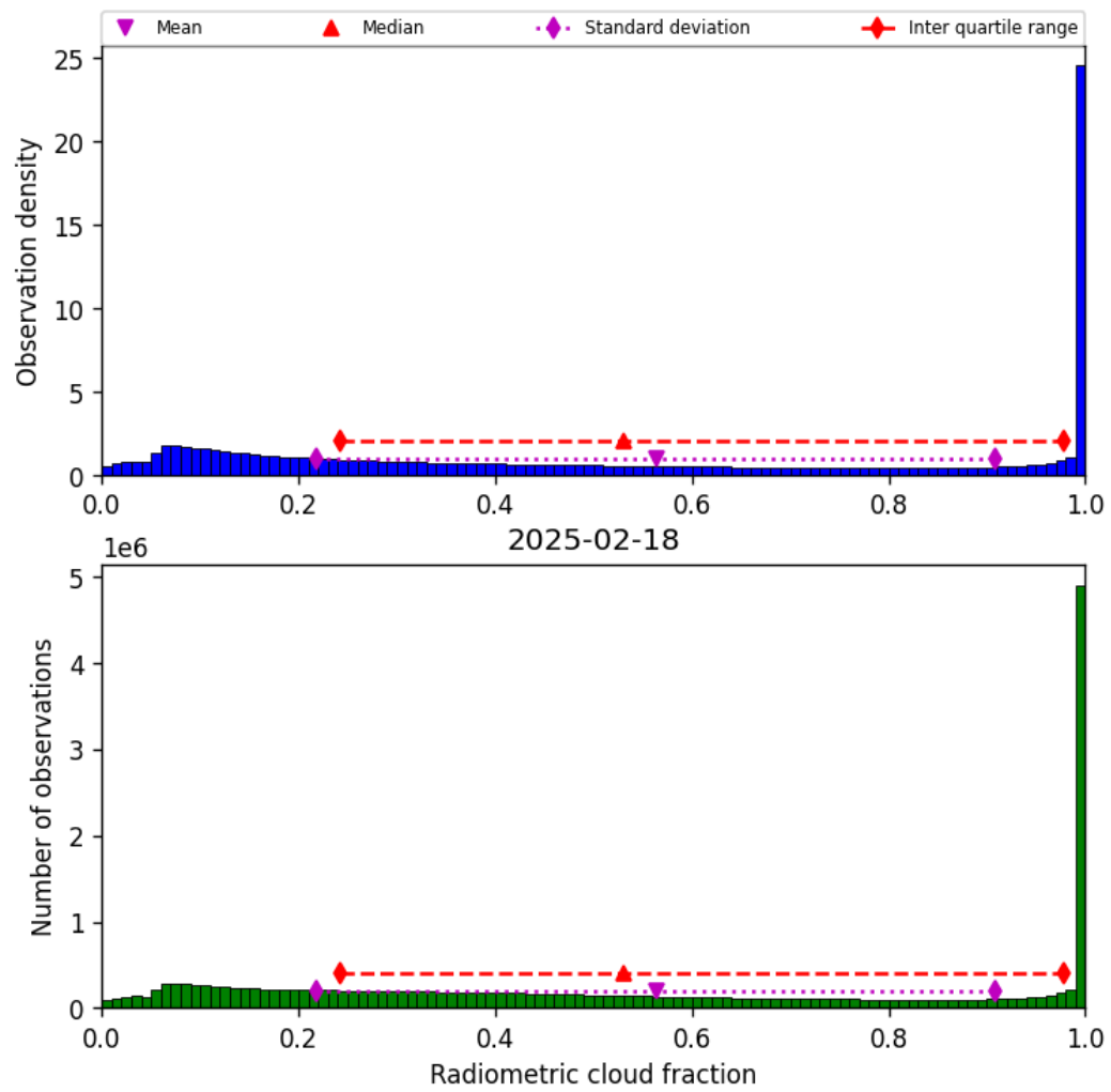
Figure 39: Histogram of “Radiometric cloud fraction” for 2025-02-18 to 2025-02-19
