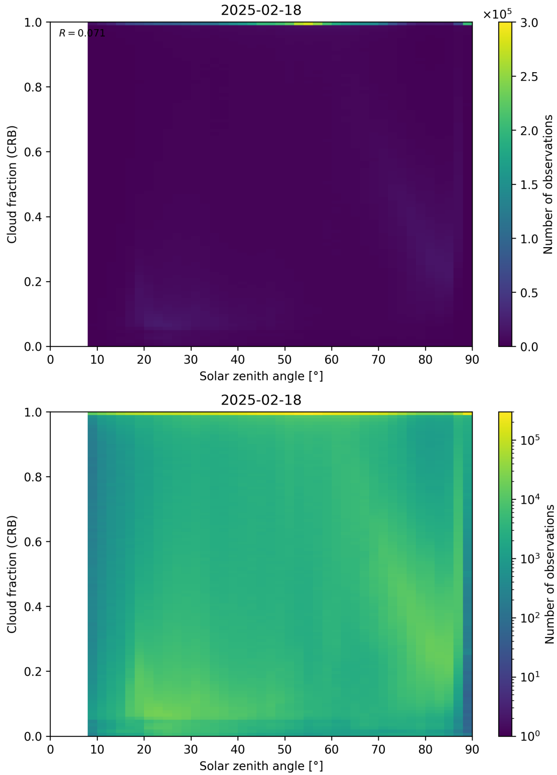
Figure 101: Scatter density plot of “Solar zenith angle” against “Cloud fraction (CRB)” for 2025-02-18 to 2025-02-19.
