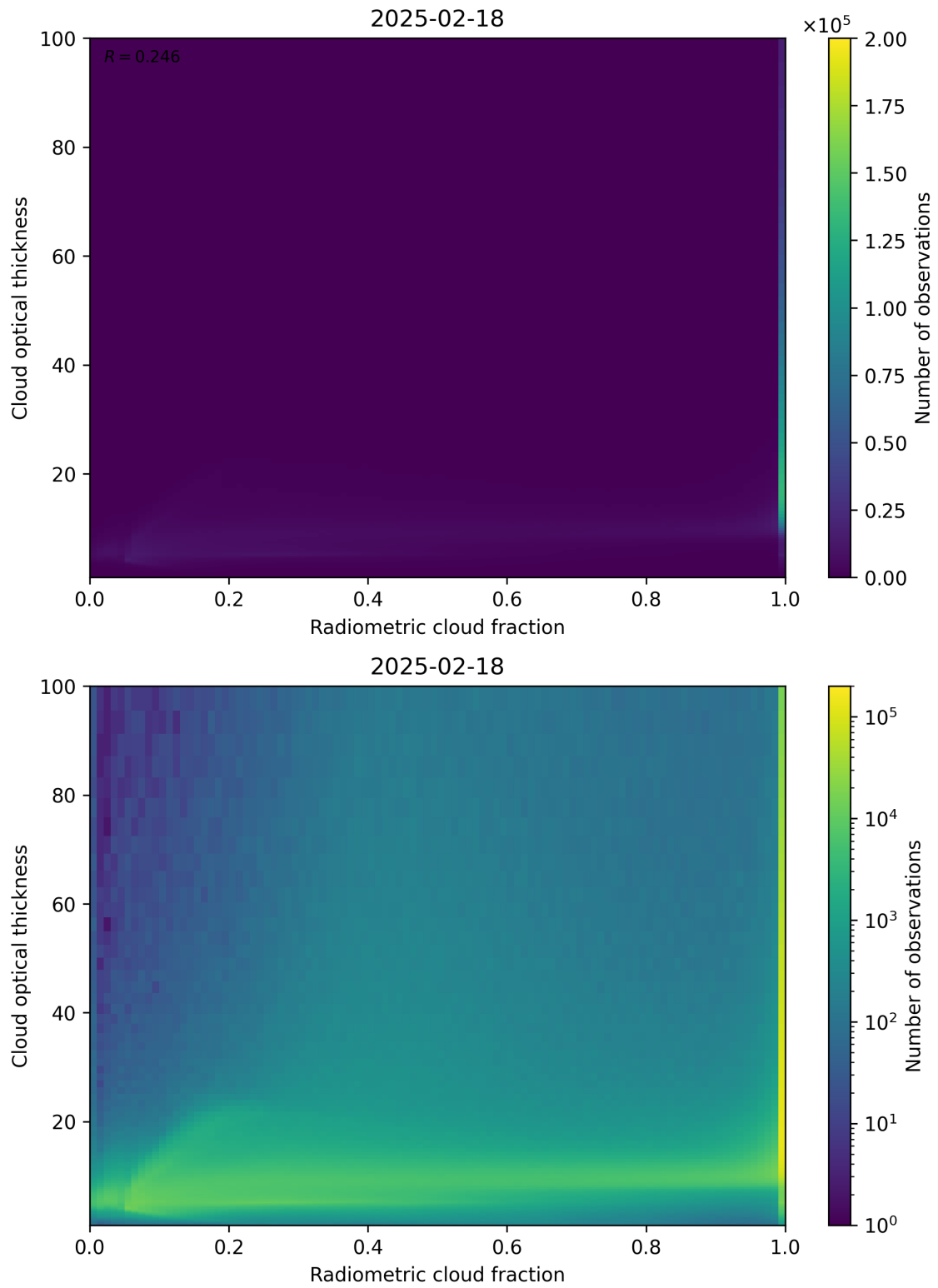
Figure 75: Scatter density plot of “Radiometric cloud fraction” against “Cloud optical thickness” for 2025-02-18 to 2025-02-19.
