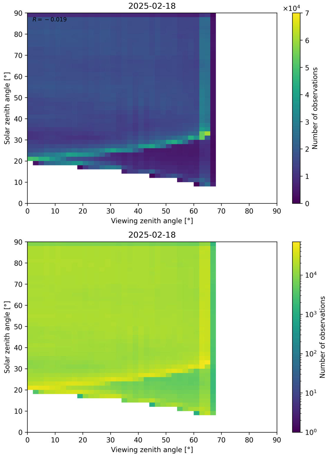
Figure 114: Scatter density plot of “Viewing zenith angle” against “Solar zenith angle” for 2025-02-18 to 2025-02-19.
