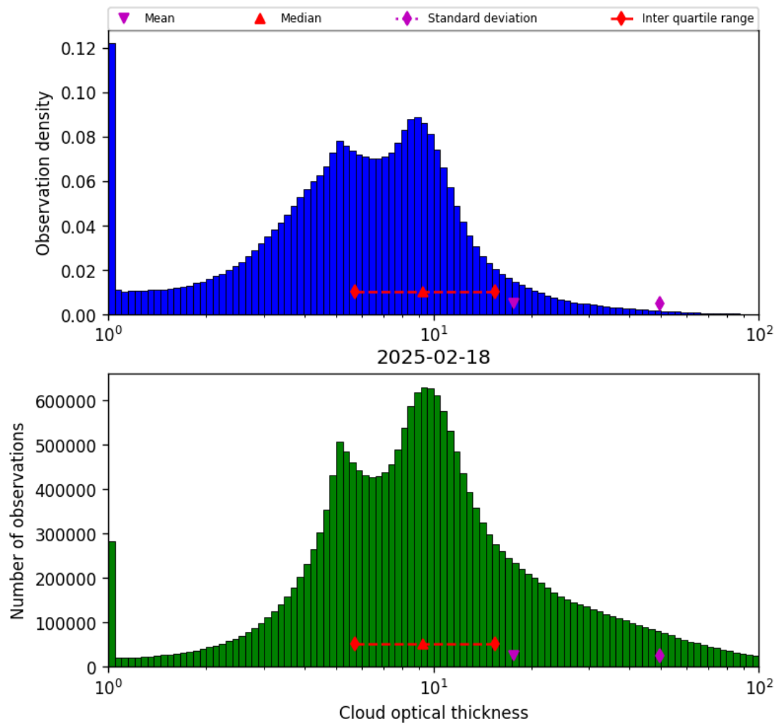
Figure 41: Histogram of “Cloud optical thickness” for 2025-02-18 to 2025-02-19
