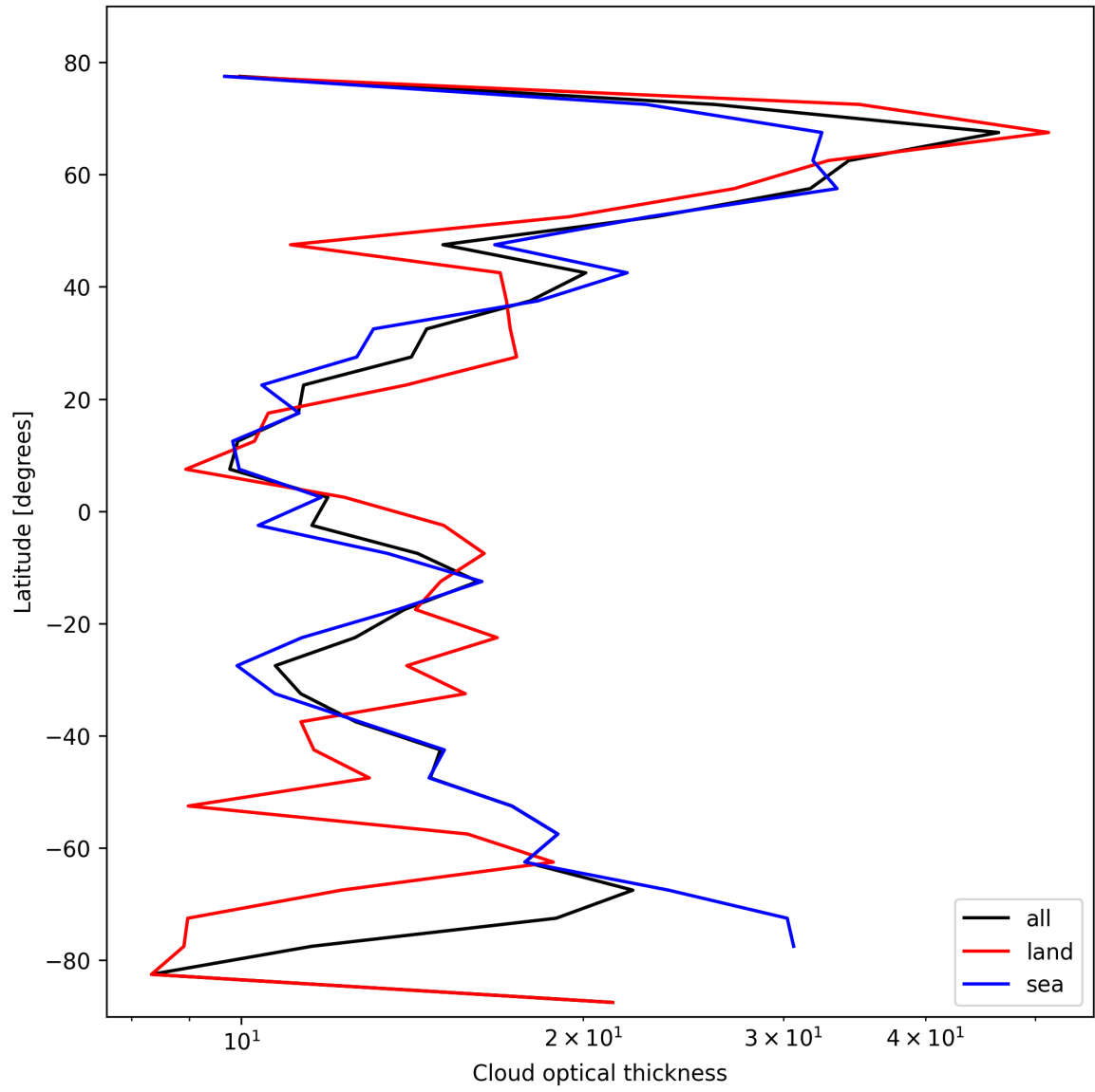
Figure 25: Zonal average of “Cloud optical thickness” for 2025-02-18 to 2025-02-19.
