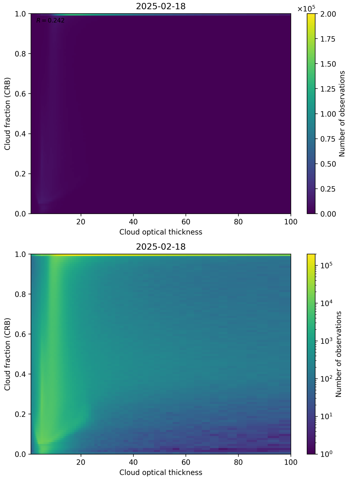
Figure 84: Scatter density plot of “Cloud optical thickness” against “Cloud fraction (CRB)” for 2025-02-18 to 2025-02-19.
