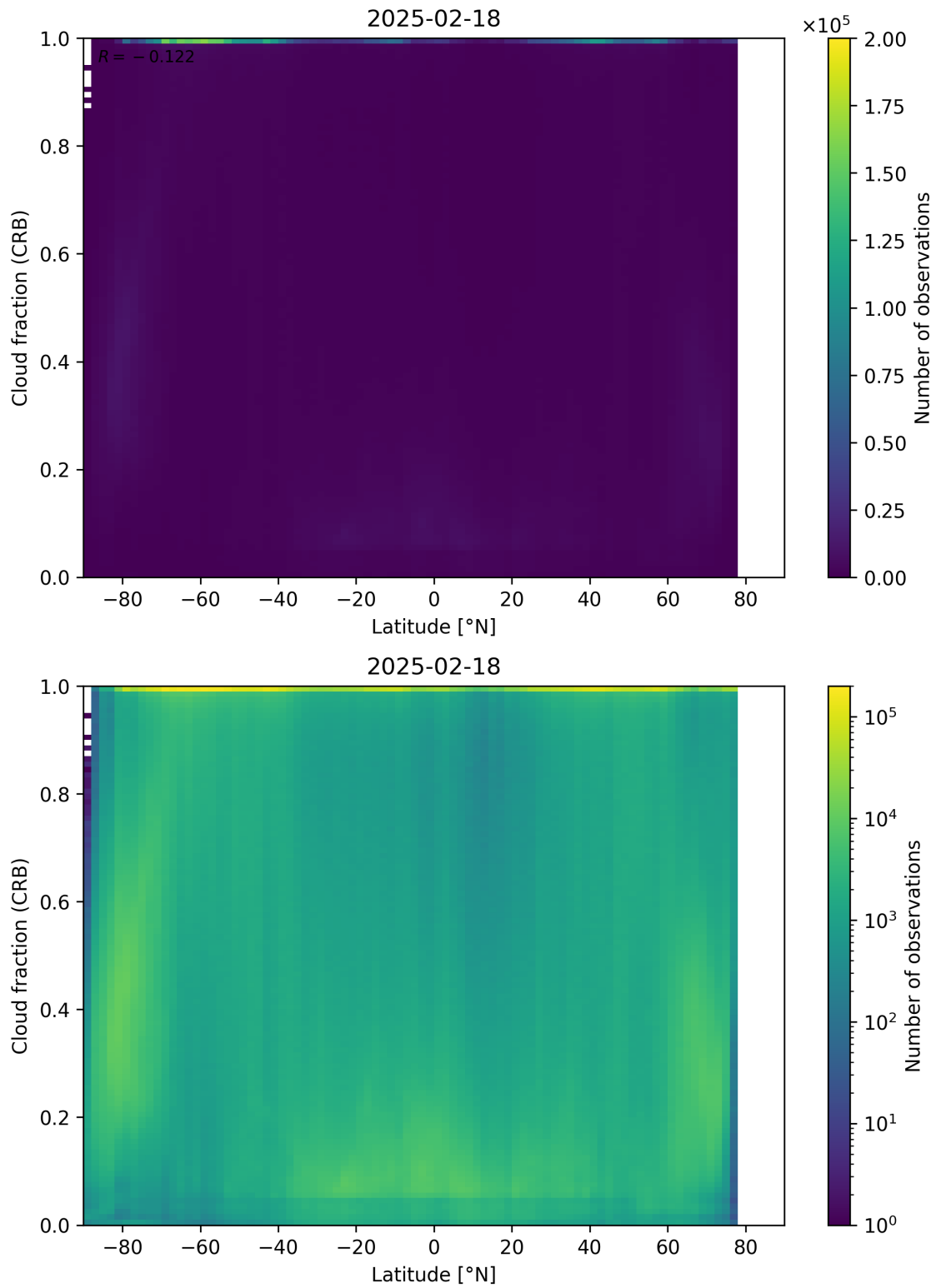
Figure 94: Scatter density plot of “Latitude” against “Cloud fraction (CRB)” for 2025-02-18 to 2025-02-19.
