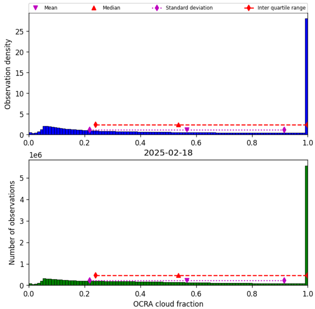
Figure 50: Histogram of “OCRA cloud fraction” for 2025-02-18 to 2025-02-19
