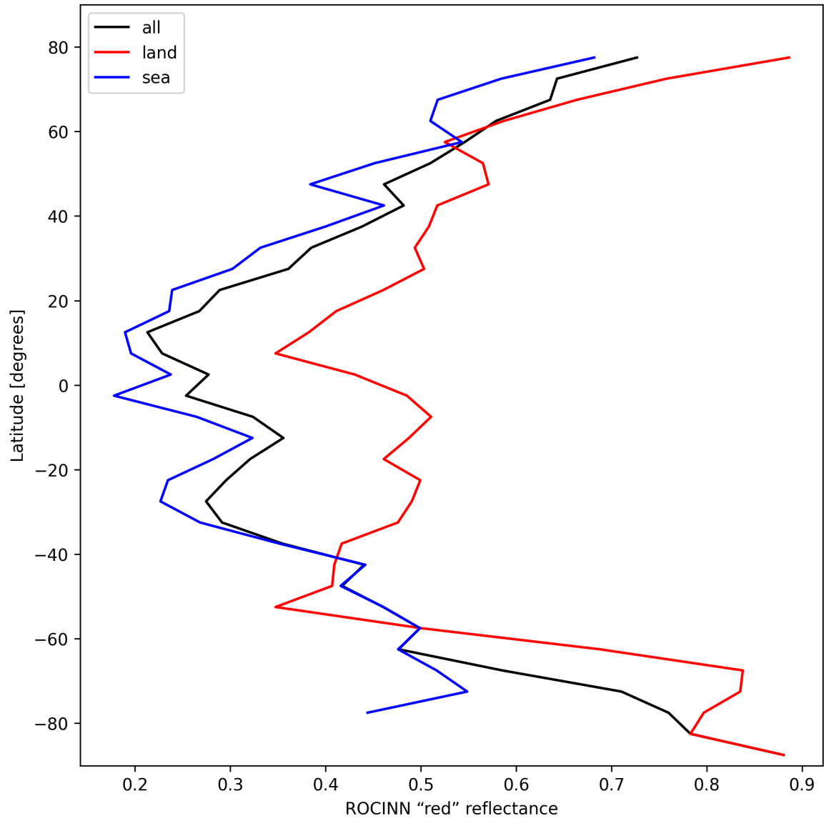
Figure 37: Zonal average of “ROCINN “red” reflectance” for 2025-02-18 to 2025-02-19.
