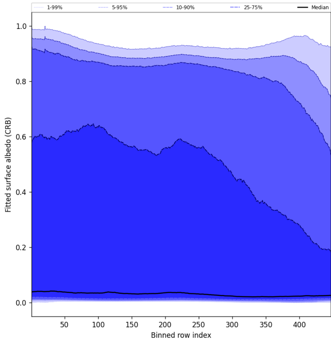
Figure 62: Along track statistics of “Fitted surface albedo (CRB)” for 2025-02-18 to 2025-02-19
