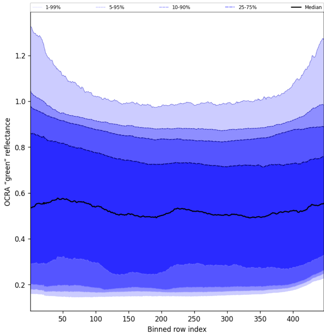
Figure 68: Along track statistics of "OCRA "green" reflectance" for 2025-02-18 to 2025-02-19
