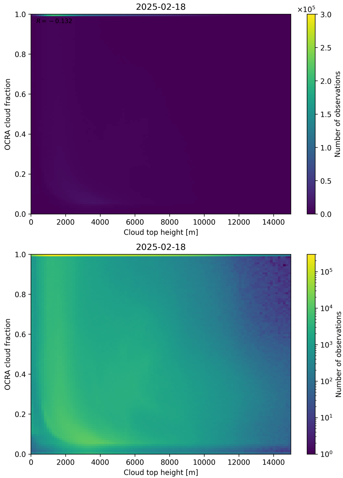
Figure 87: Scatter density plot of “Cloud top height” against “OCRA cloud fraction” for 2025-02-18 to 2025-02-19.
