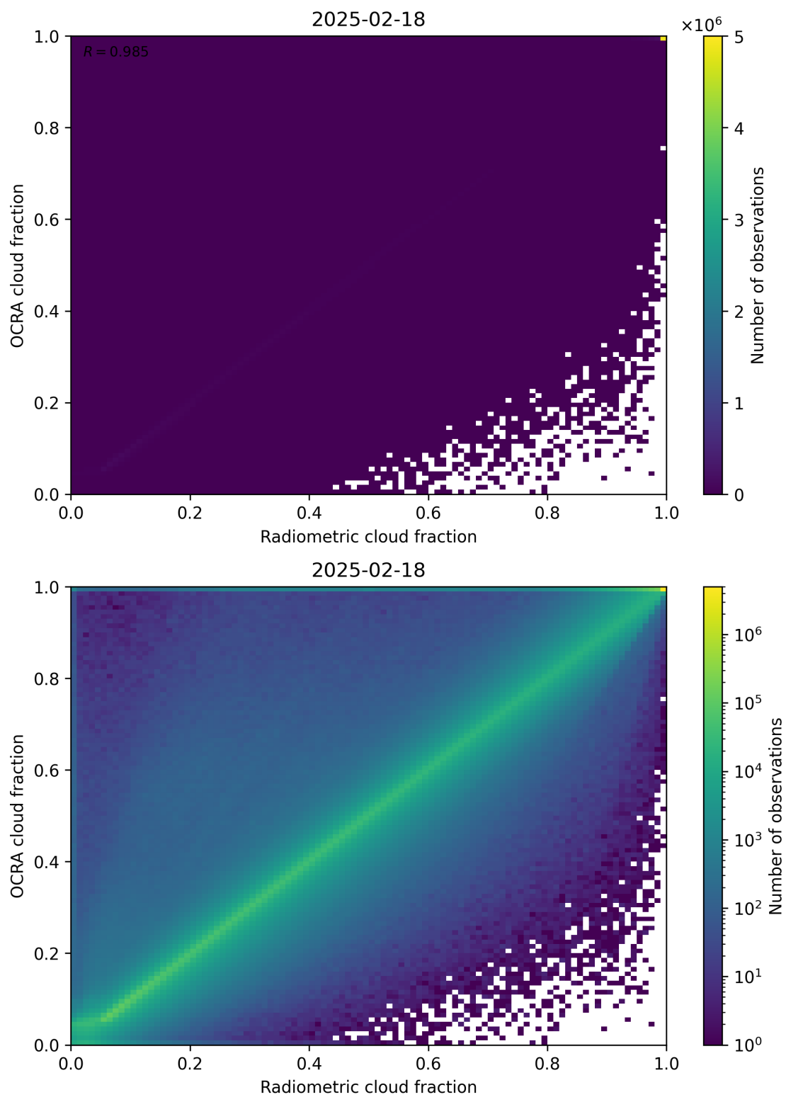
Figure 72: Scatter density plot of “Radiometric cloud fraction” against “OCRA cloud fraction” for 2025-02-18 to 2025-02-19.
