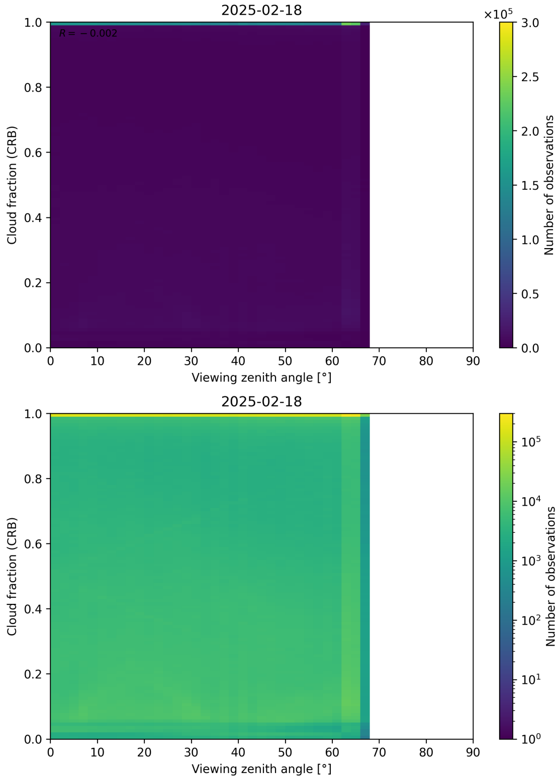
Figure 109: Scatter density plot of “Viewing zenith angle” against “Cloud fraction (CRB)” for 2025-02-18 to 2025-02-19.
