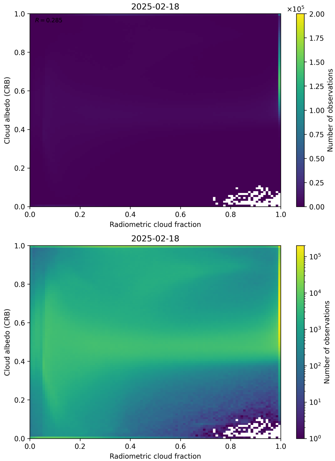
Figure 71: Scatter density plot of “Radiometric cloud fraction” against “Cloud albedo (CRB)” for 2025-02-18 to 2025-02-19.
