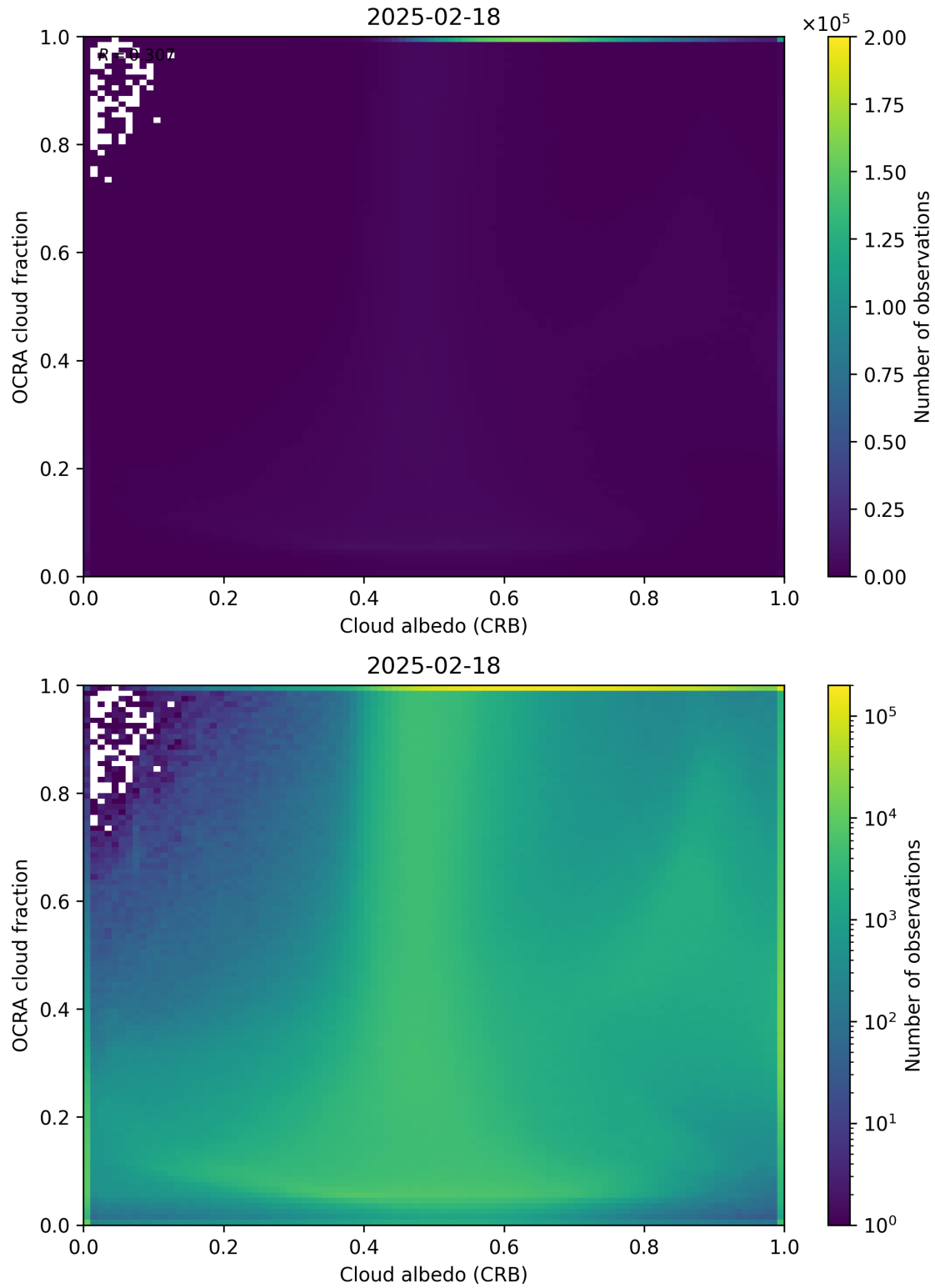
Figure 70: Scatter density plot of “Cloud albedo (CRB)” against “OCRA cloud fraction” for 2025-02-18 to 2025-02-19.
