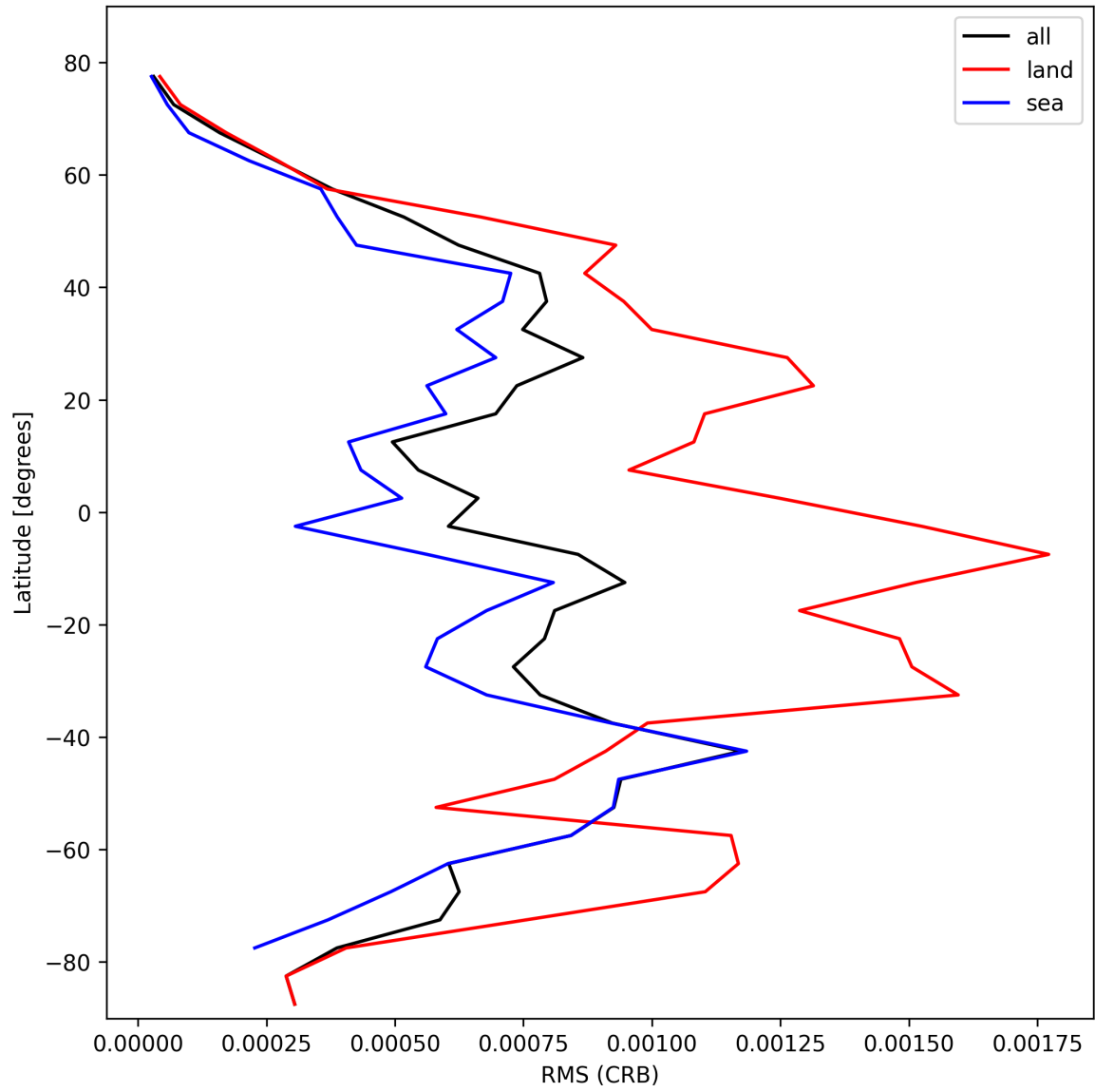
Figure 32: Zonal average of “RMS (CRB)” for 2025-02-18 to 2025-02-19.
