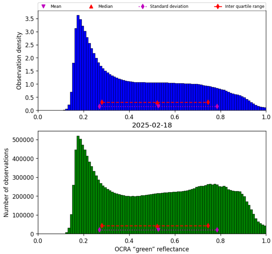
Figure 52: Histogram of “OCRA “green” reflectance” for 2025-02-18 to 2025-02-19
