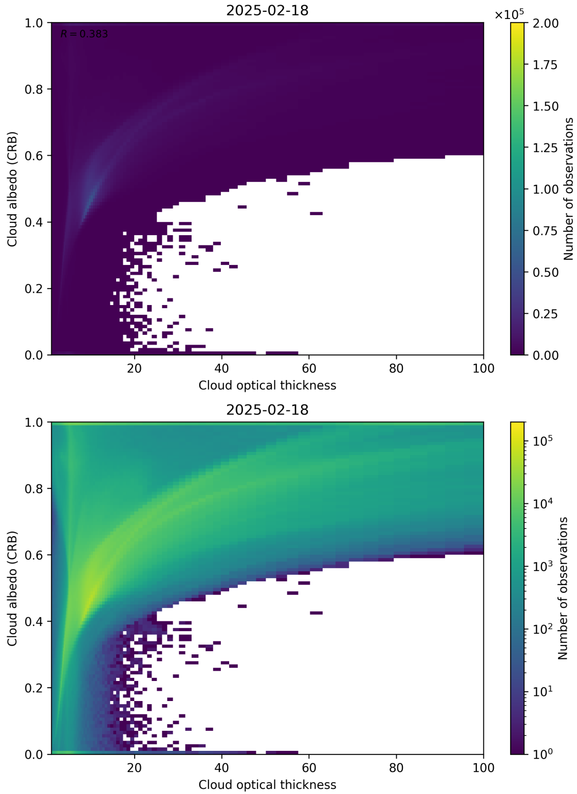
Figure 82: Scatter density plot of “Cloud optical thickness” against “Cloud albedo (CRB)” for 2025-02-18 to 2025-02-19.
