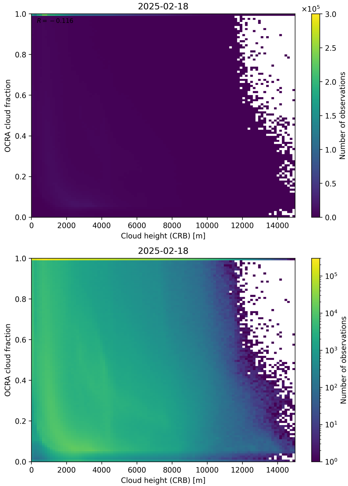
Figure 81: Scatter density plot of “Cloud height (CRB)” against “OCRA cloud fraction” for 2025-02-18 to 2025-02-19.
