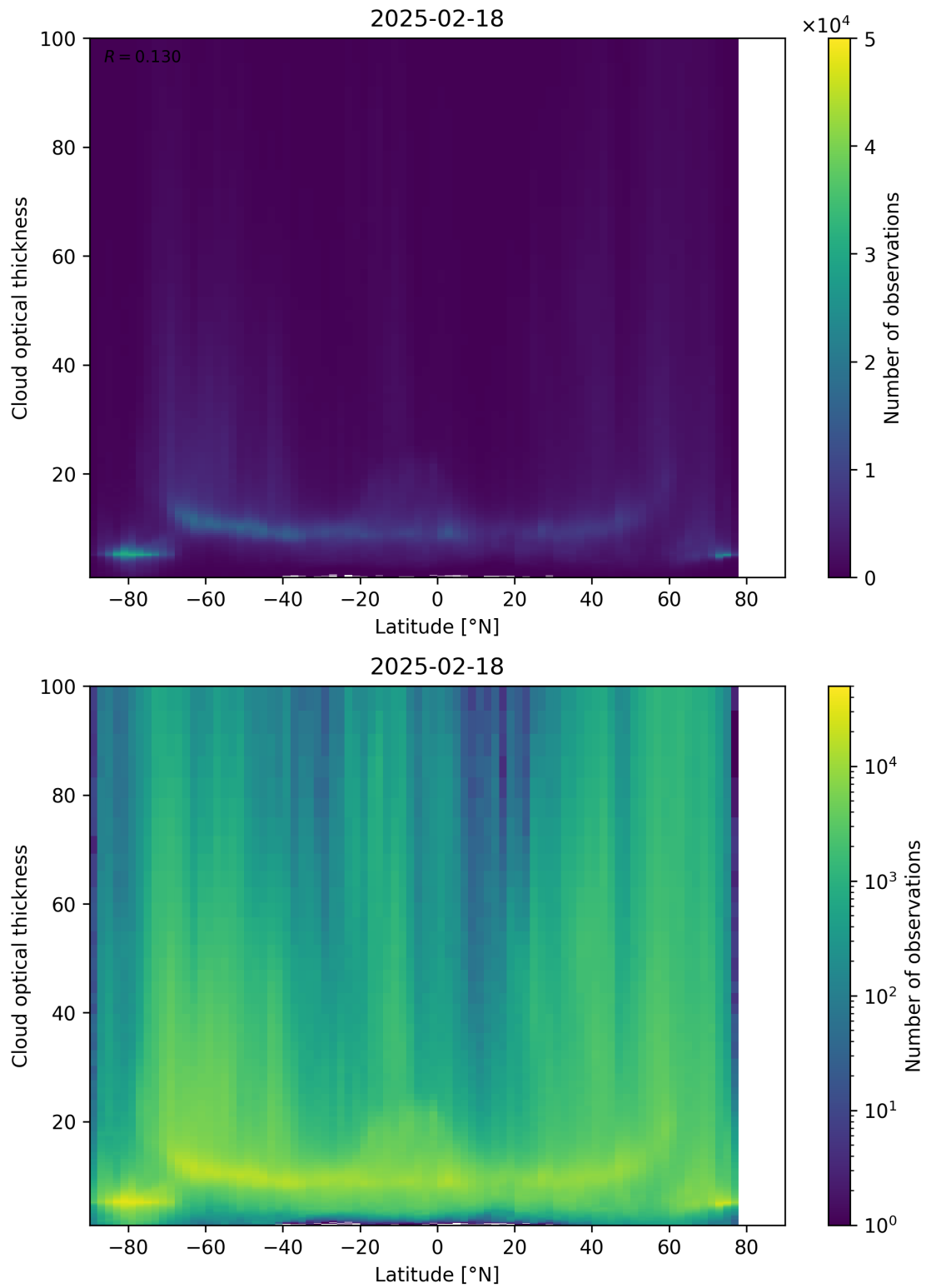
Figure 96: Scatter density plot of “Latitude” against “Cloud optical thickness” for 2025-02-18 to 2025-02-19.
