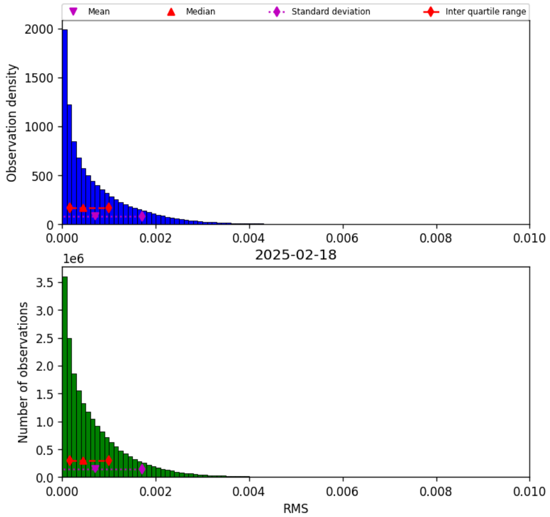
Figure 47: Histogram of “RMS” for 2025-02-18 to 2025-02-19
