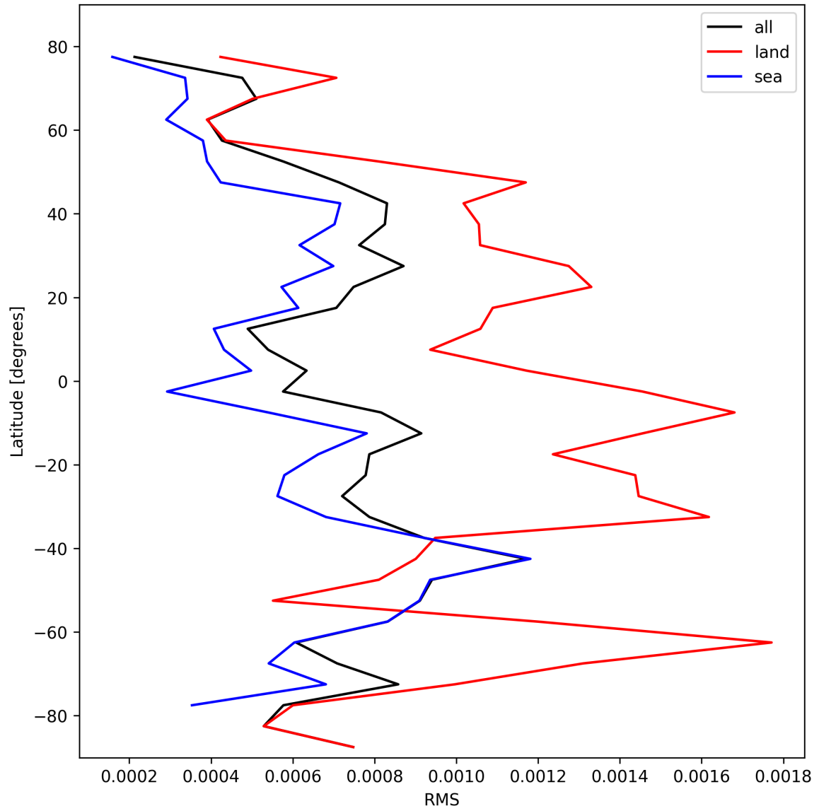
Figure 31: Zonal average of “RMS” for 2025-02-18 to 2025-02-19.
