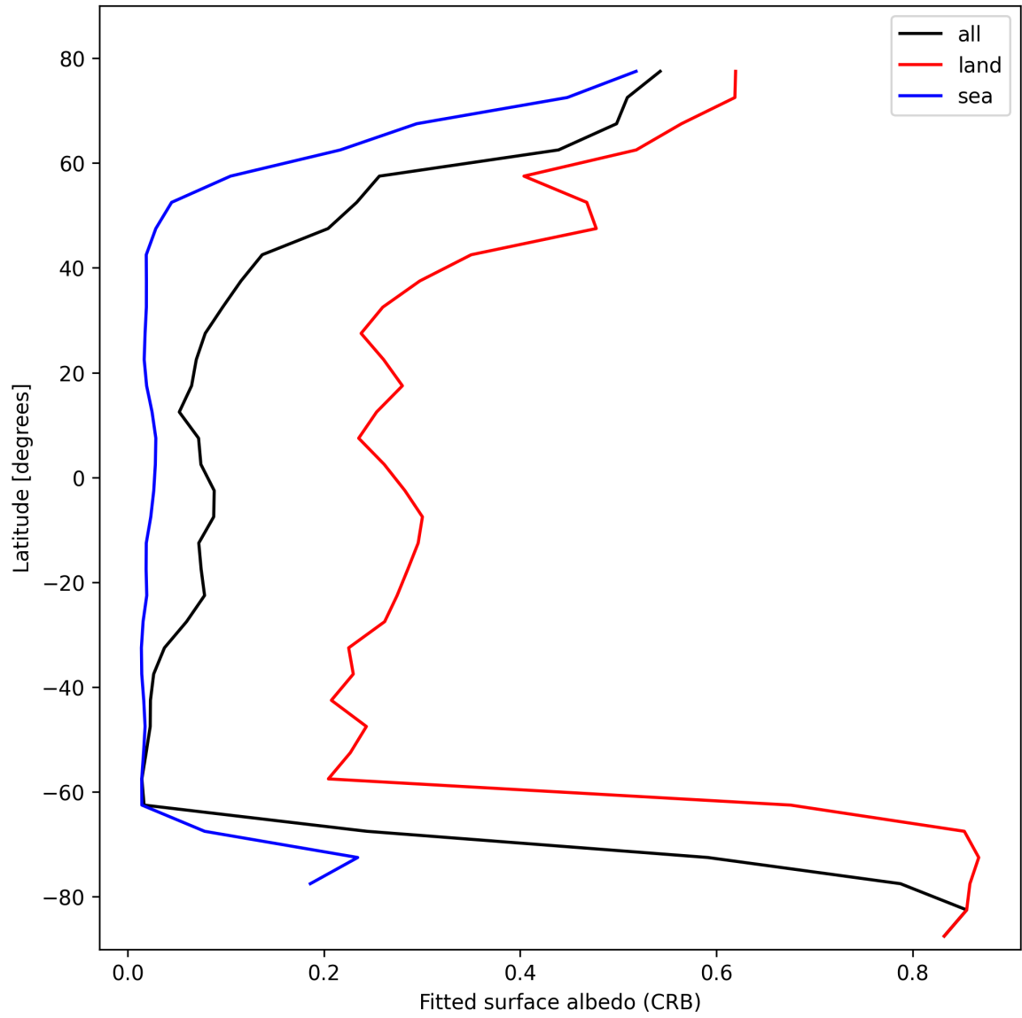
Figure 30: Zonal average of “Fitted surface albedo (CRB)” for 2025-02-18 to 2025-02-19.
