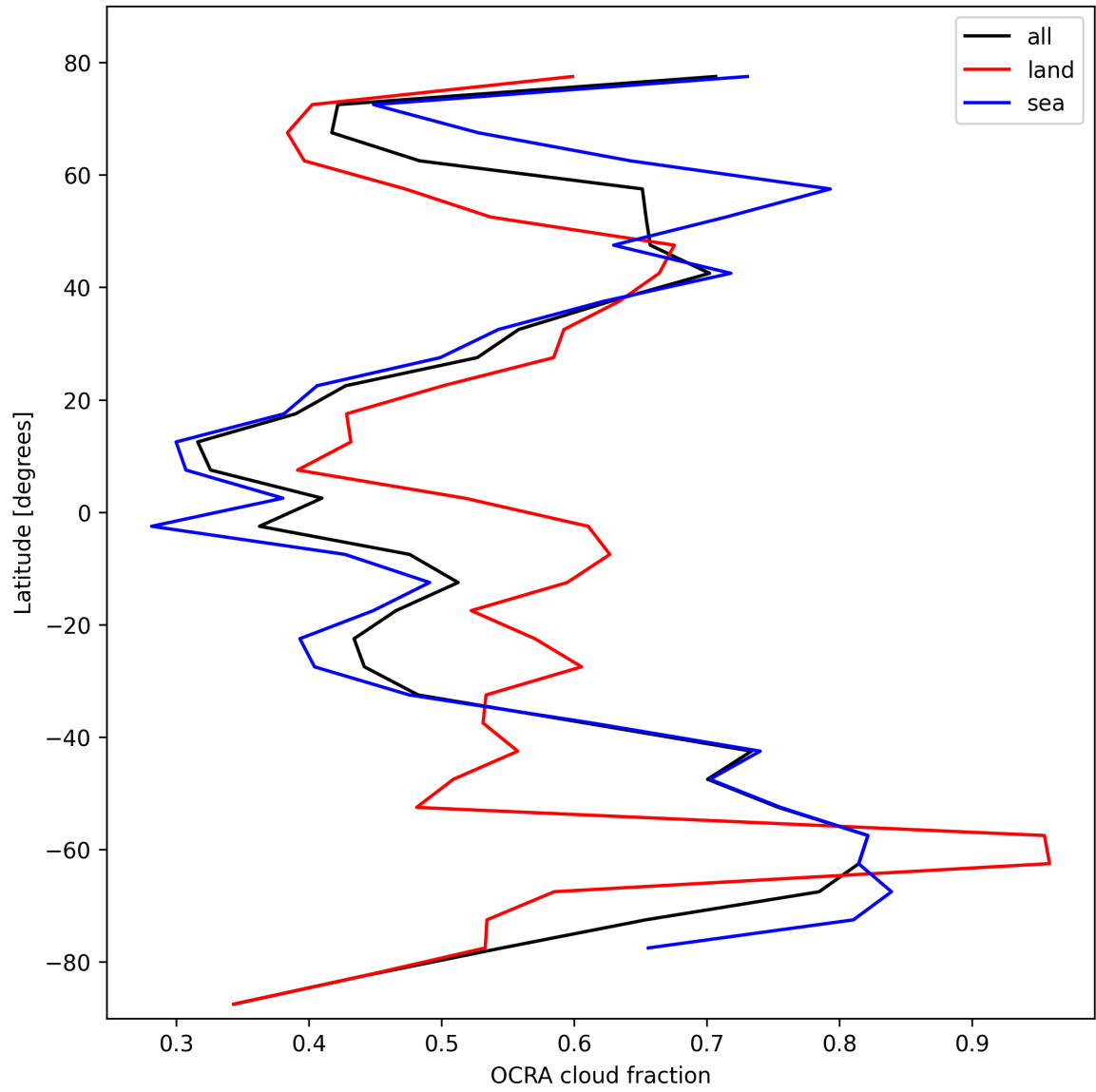
Figure 34: Zonal average of “OCRA cloud fraction” for 2025-02-18 to 2025-02-19.
