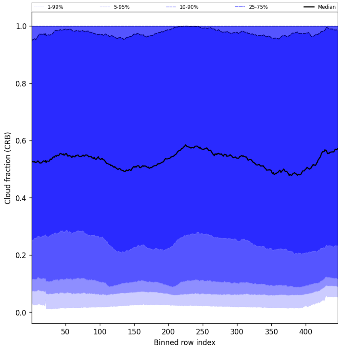
Figure 58: Along track statistics of “Cloud fraction (CRB)” for 2025-02-18 to 2025-02-19
