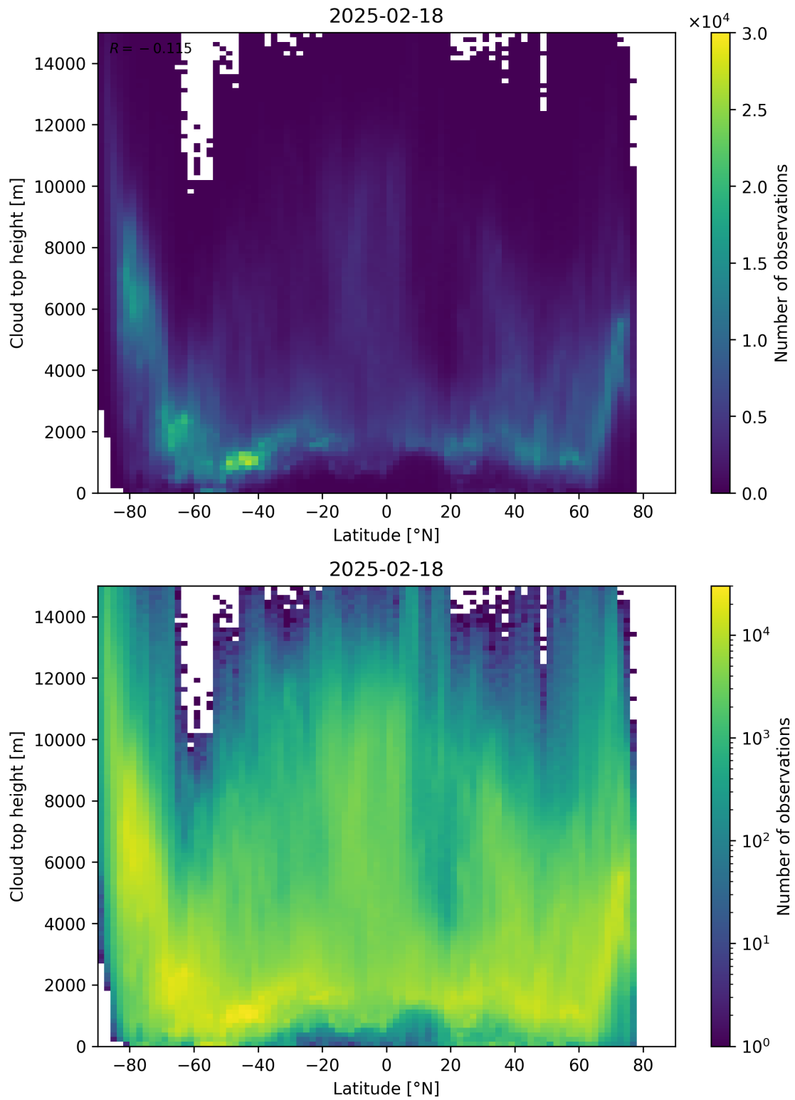
Figure 97: Scatter density plot of “Latitude” against “Cloud top height” for 2025-02-18 to 2025-02-19.
