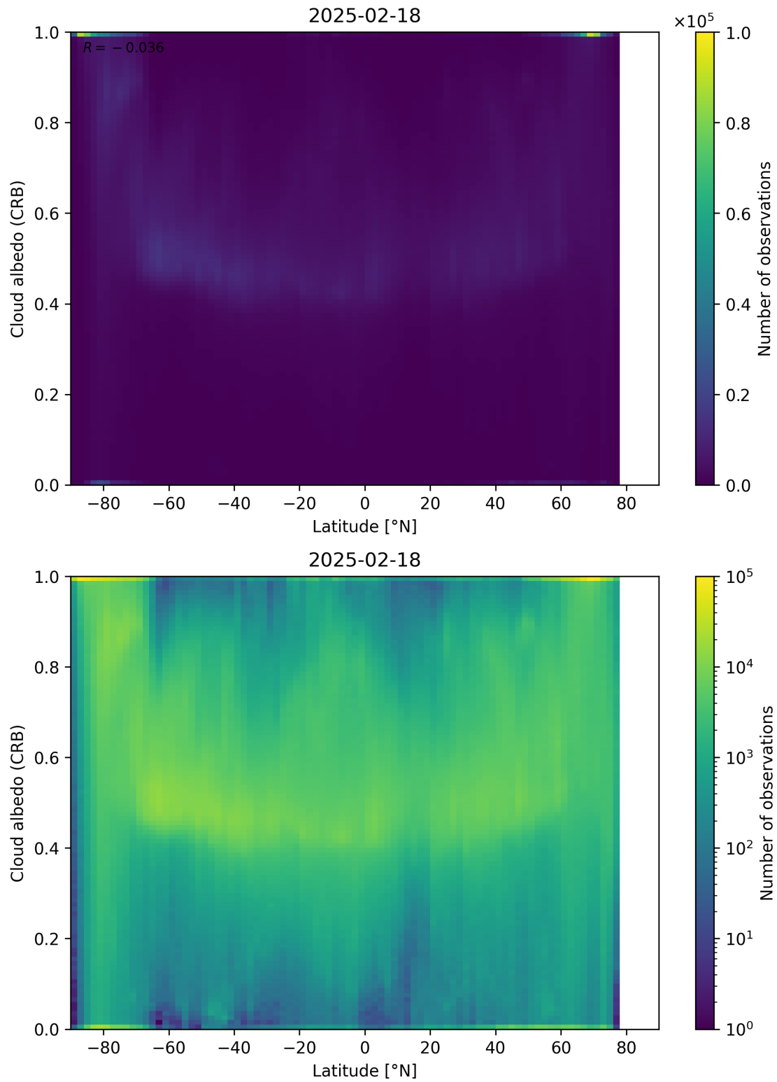
Figure 91: Scatter density plot of “Latitude” against “Cloud albedo (CRB)” for 2025-02-18 to 2025-02-19.
