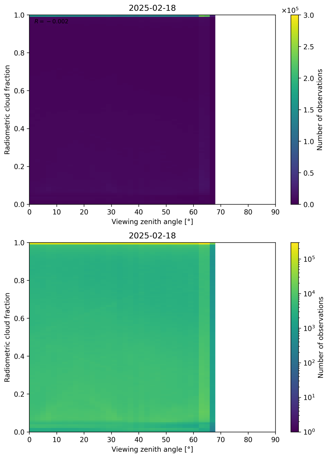
Figure 107: Scatter density plot of “Viewing zenith angle” against “Radiometric cloud fraction” for 2025-02-18 to 2025-02-19.
