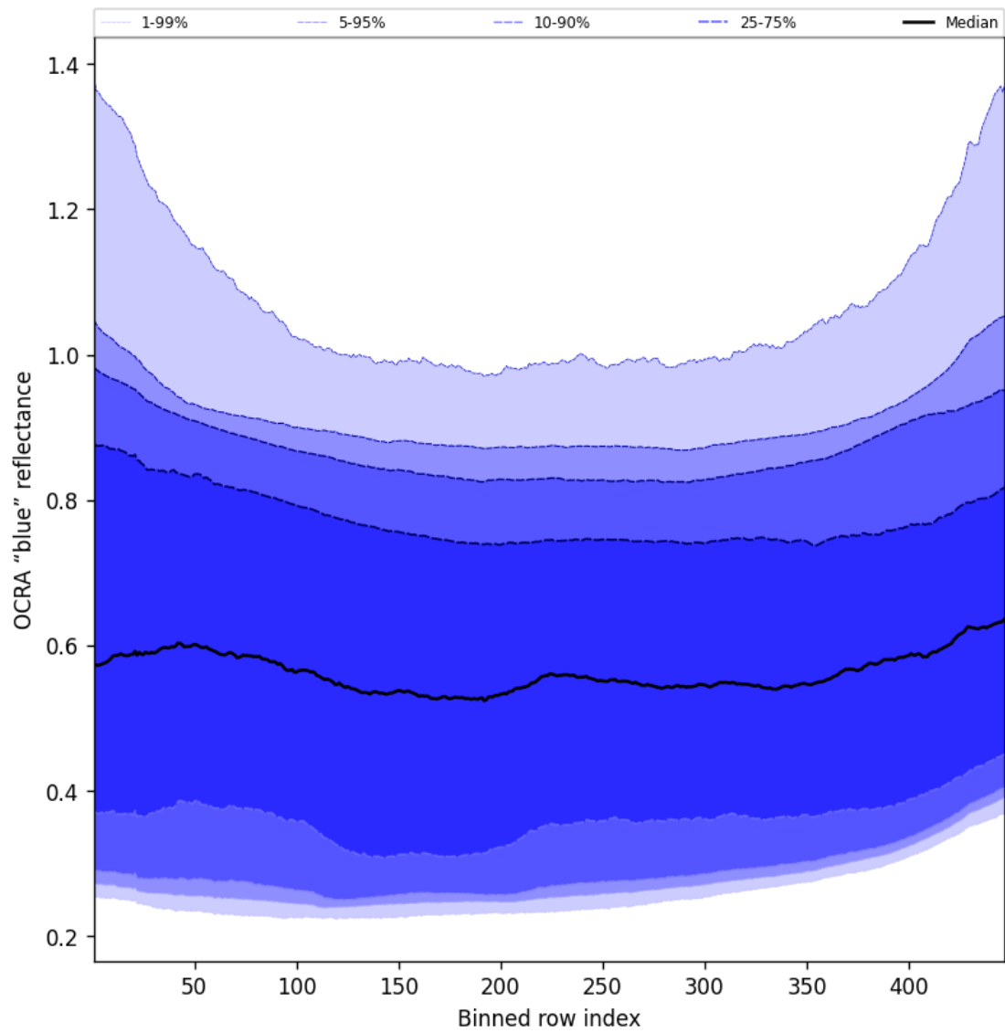
Figure 67: Along track statistics of "OCRA "blue" reflectance" for 2025-02-18 to 2025-02-19
