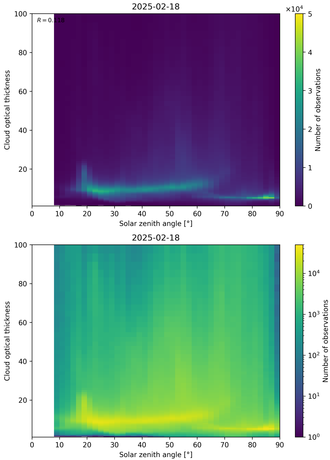
Figure 103: Scatter density plot of “Solar zenith angle” against “Cloud optical thickness” for 2025-02-18 to 2025-02-19.
