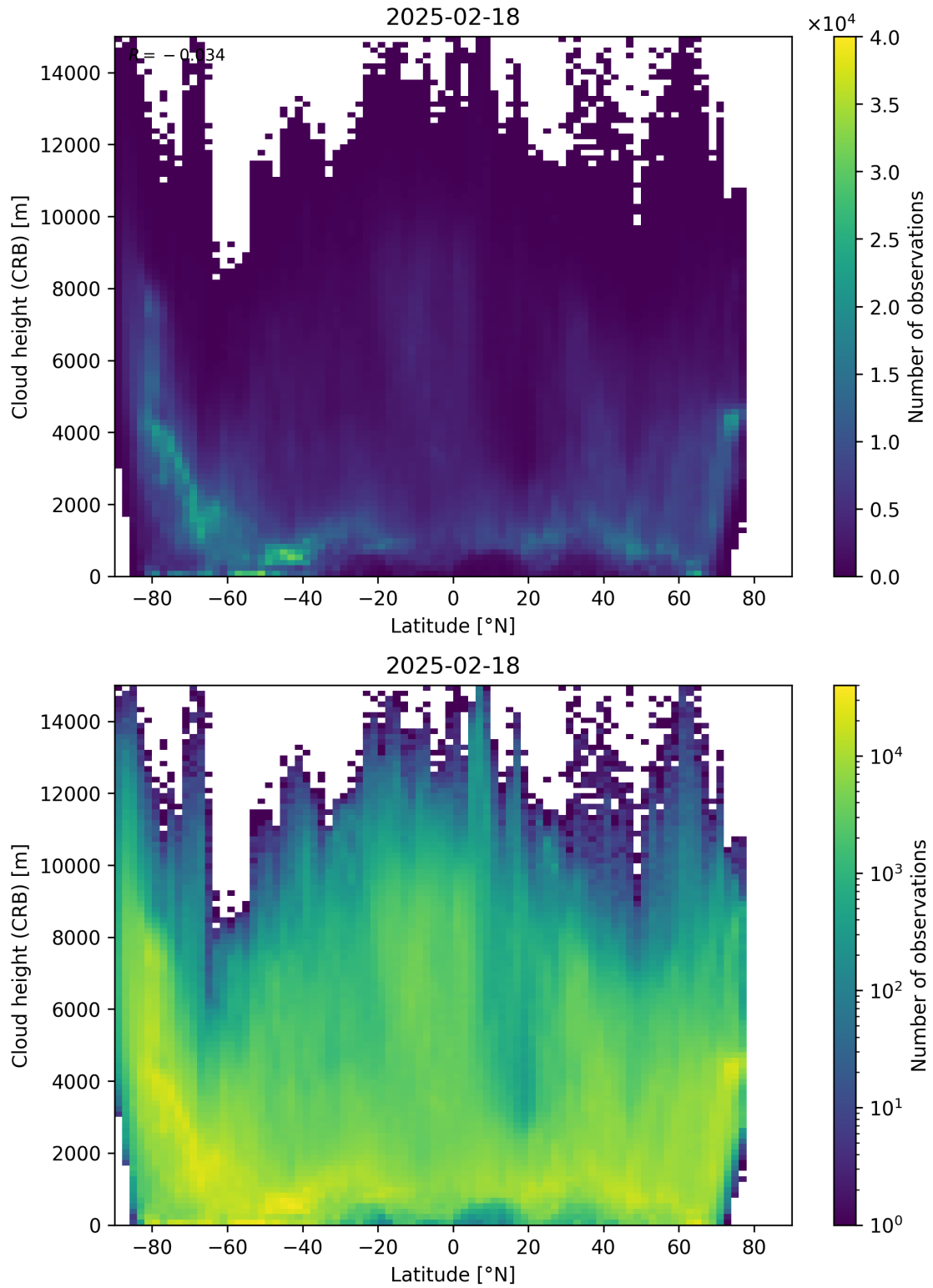
Figure 95: Scatter density plot of “Latitude” against “Cloud height (CRB)” for 2025-02-18 to 2025-02-19.
