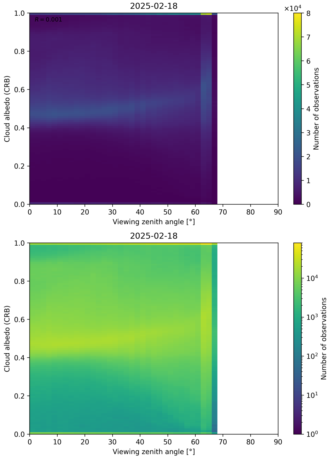
Figure 106: Scatter density plot of “Viewing zenith angle” against “Cloud albedo (CRB)” for 2025-02-18 to 2025-02-19.
