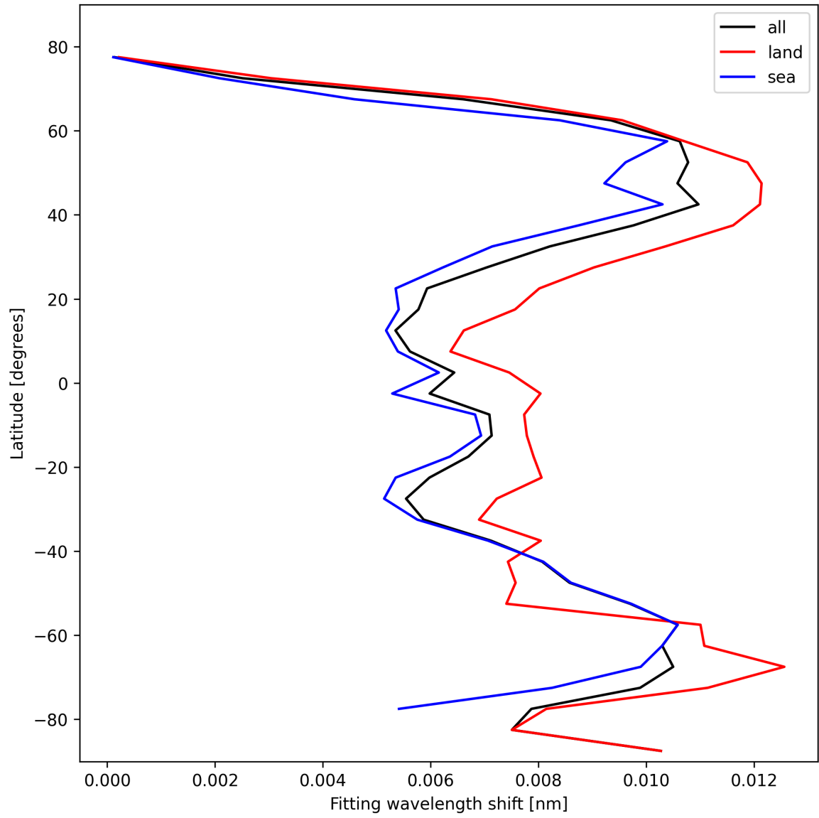
Figure 33: Zonal average of “Fitting wavelength shift” for 2025-02-18 to 2025-02-19.
