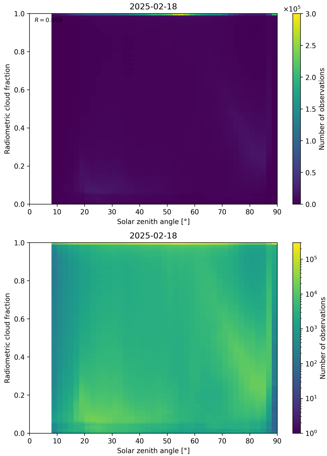
Figure 99: Scatter density plot of “Solar zenith angle” against “Radiometric cloud fraction” for 2025-02-18 to 2025-02-19.
