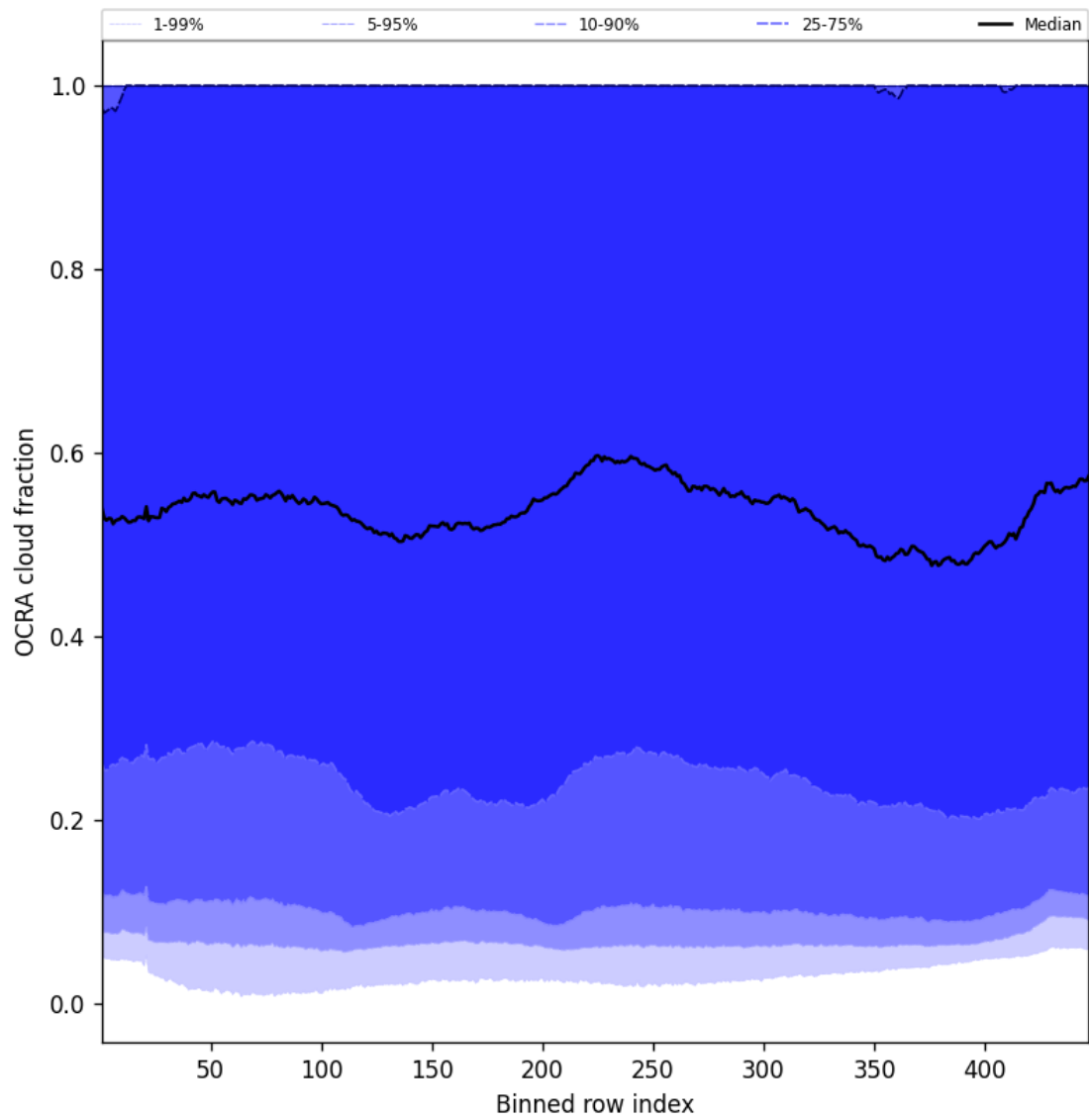
Figure 66: Along track statistics of “OCRA cloud fraction” for 2025-02-18 to 2025-02-19
