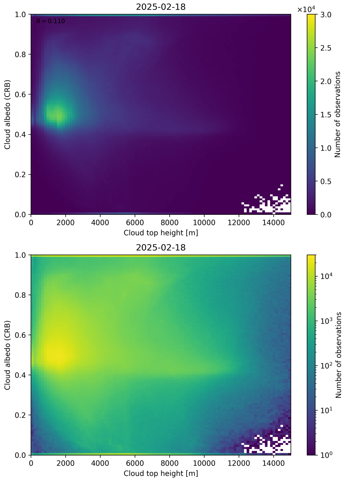
Figure 86: Scatter density plot of “Cloud top height” against “Cloud albedo (CRB)” for 2025-02-18 to 2025-02-19.
