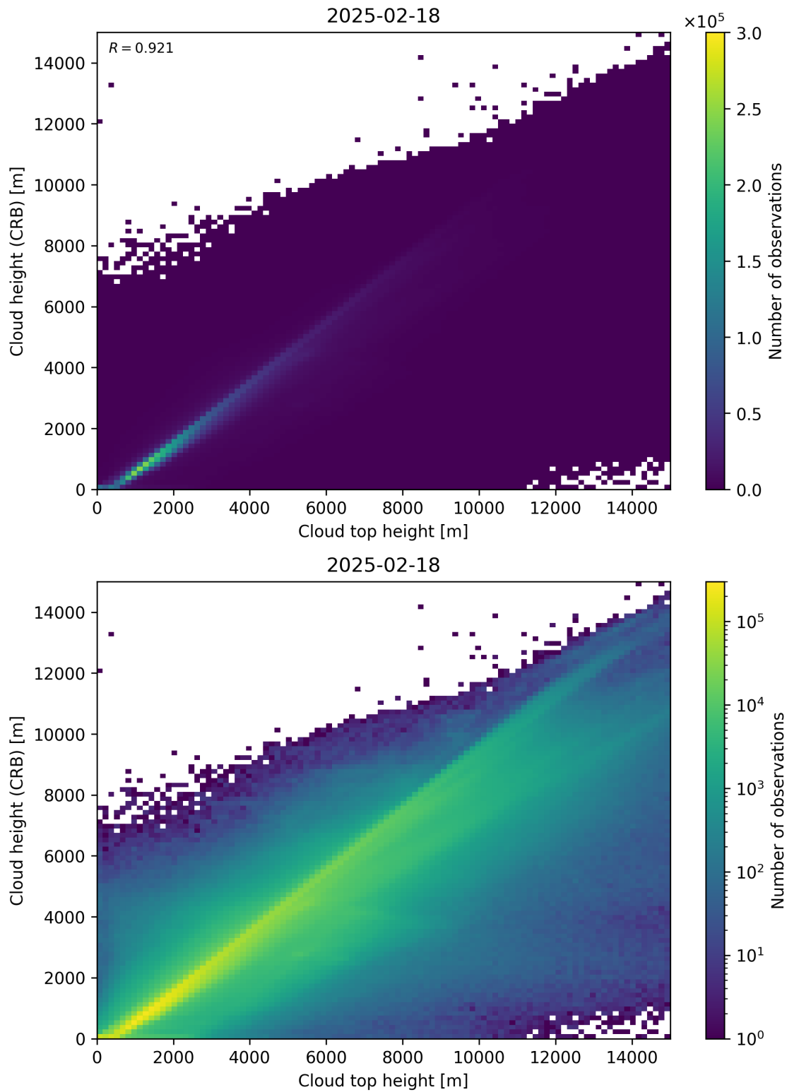
Figure 89: Scatter density plot of “Cloud top height” against “Cloud height (CRB)” for 2025-02-18 to 2025-02-19.
