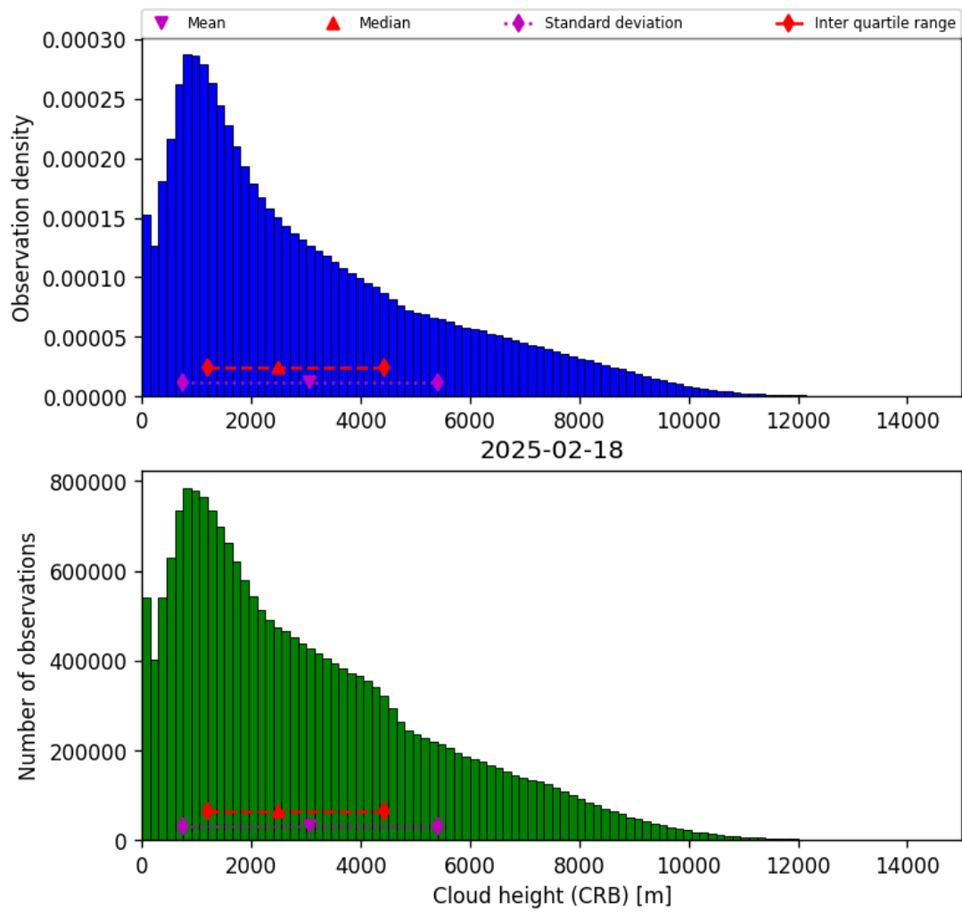
Figure 43: Histogram of “Cloud height (CRB)” for 2025-02-18 to 2025-02-19
