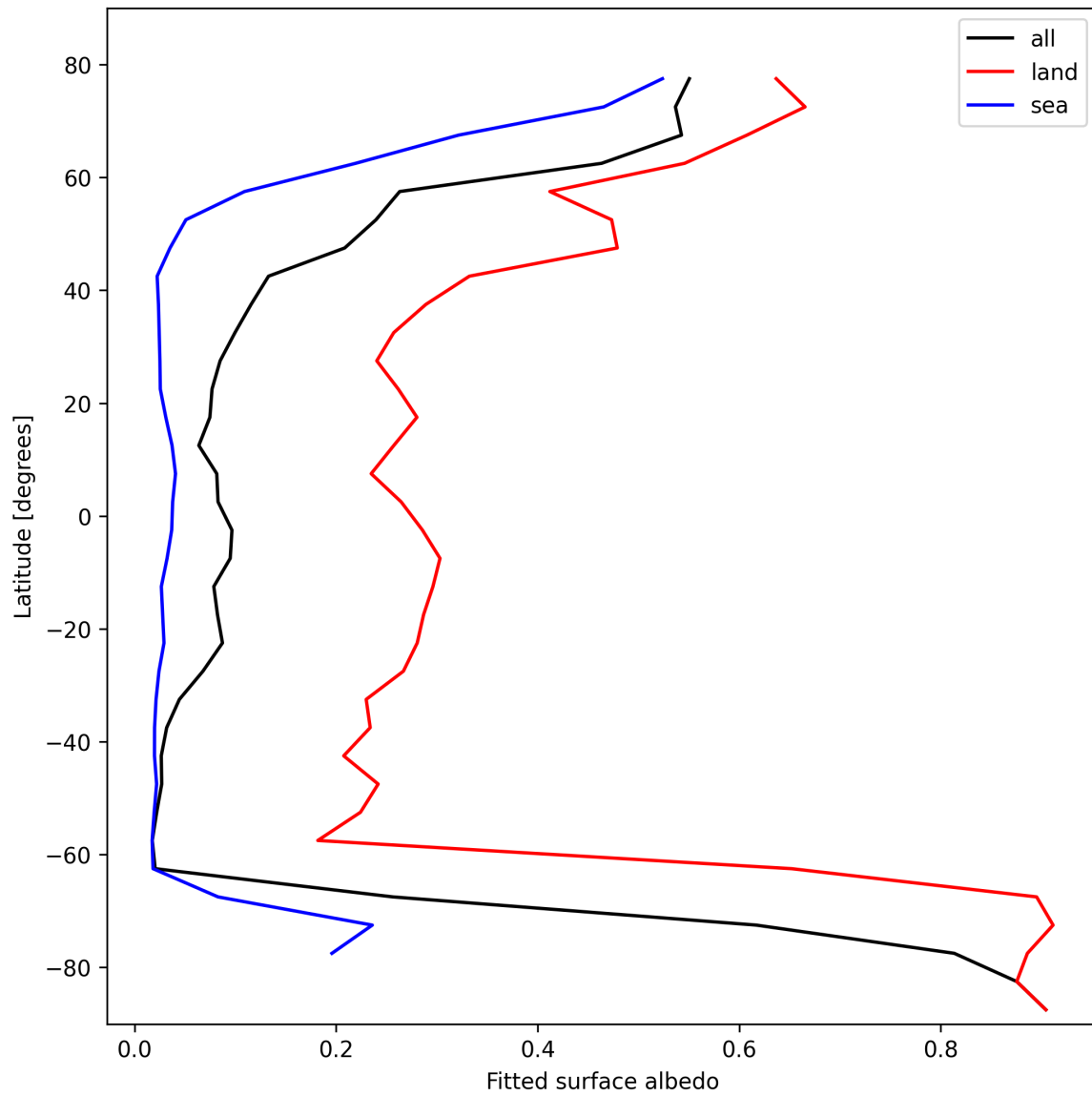
Figure 29: Zonal average of “Fitted surface albedo” for 2025-02-18 to 2025-02-19.
