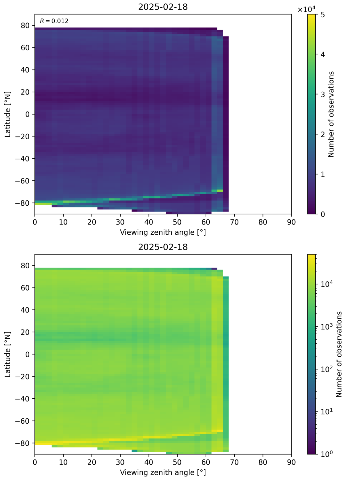
Figure 113: Scatter density plot of “Viewing zenith angle” against “Latitude” for 2025-02-18 to 2025-02-19.
