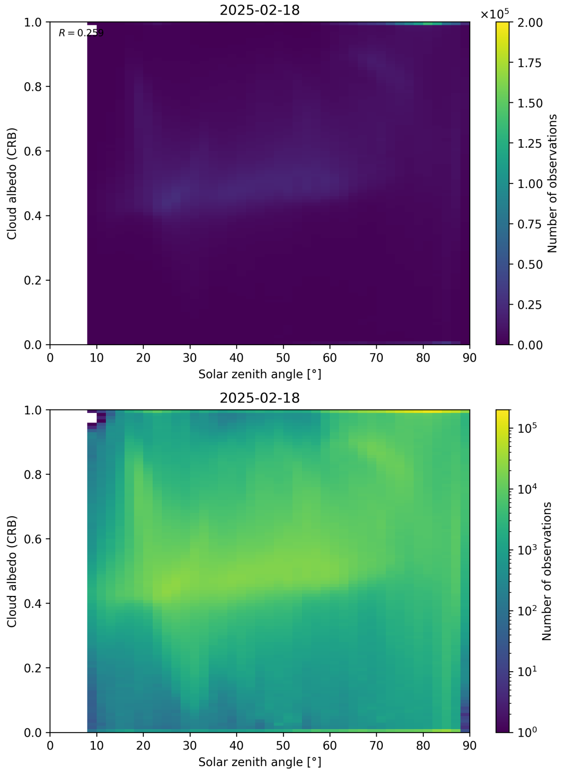
Figure 98: Scatter density plot of “Solar zenith angle” against “Cloud albedo (CRB)” for 2025-02-18 to 2025-02-19.
