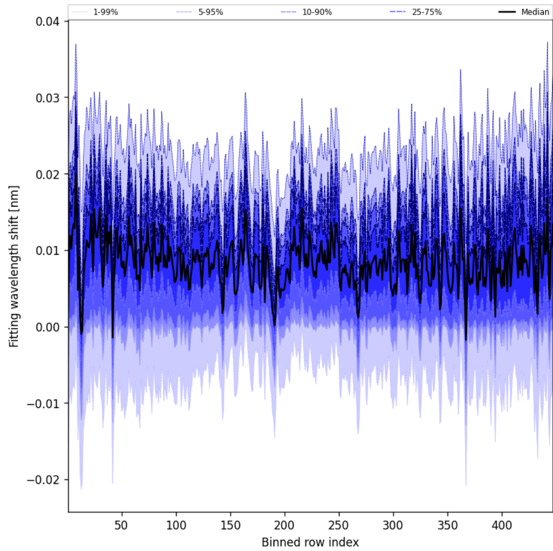
Figure 65: Along track statistics of “Fitting wavelength shift” for 2025-02-18 to 2025-02-19
