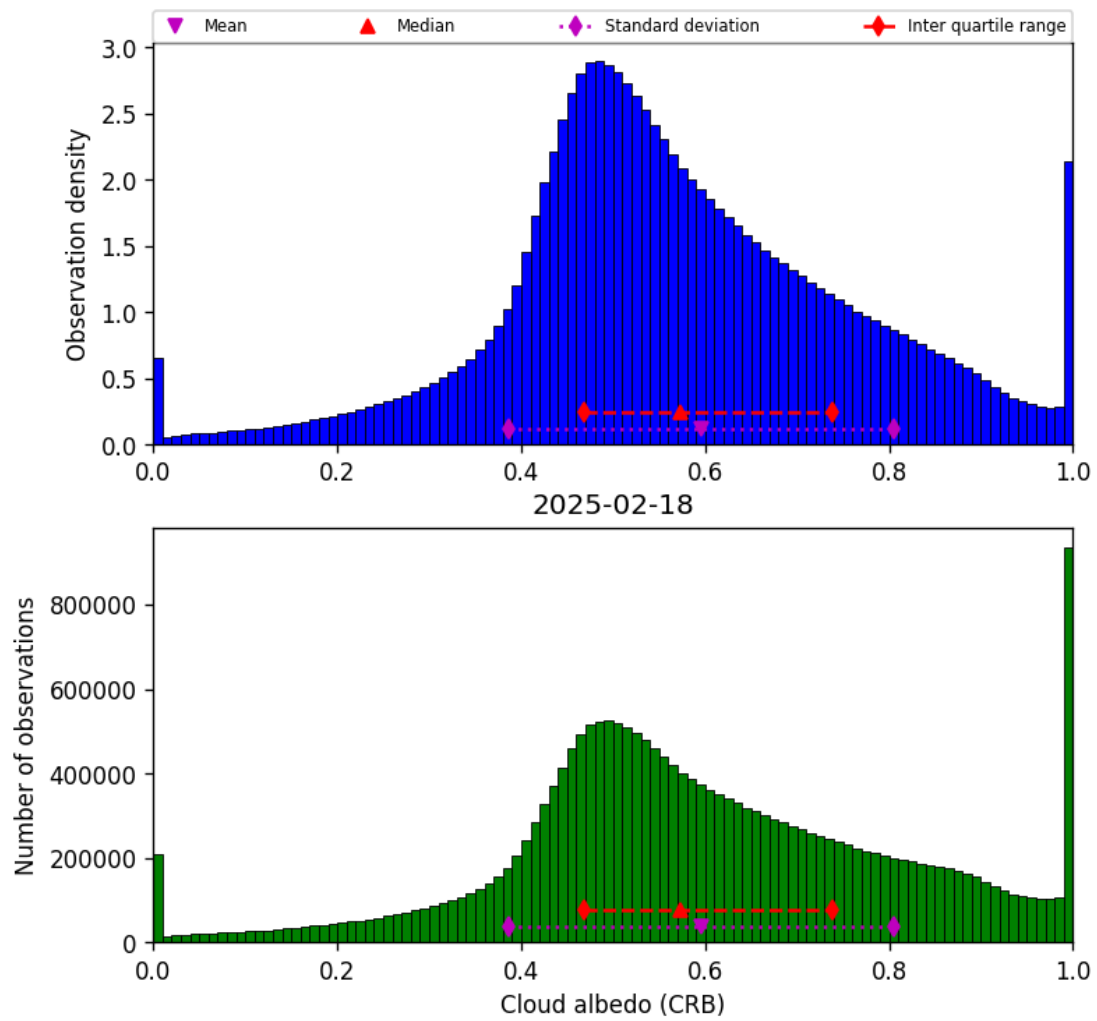
Figure 44: Histogram of “Cloud albedo (CRB)” for 2025-02-18 to 2025-02-19
