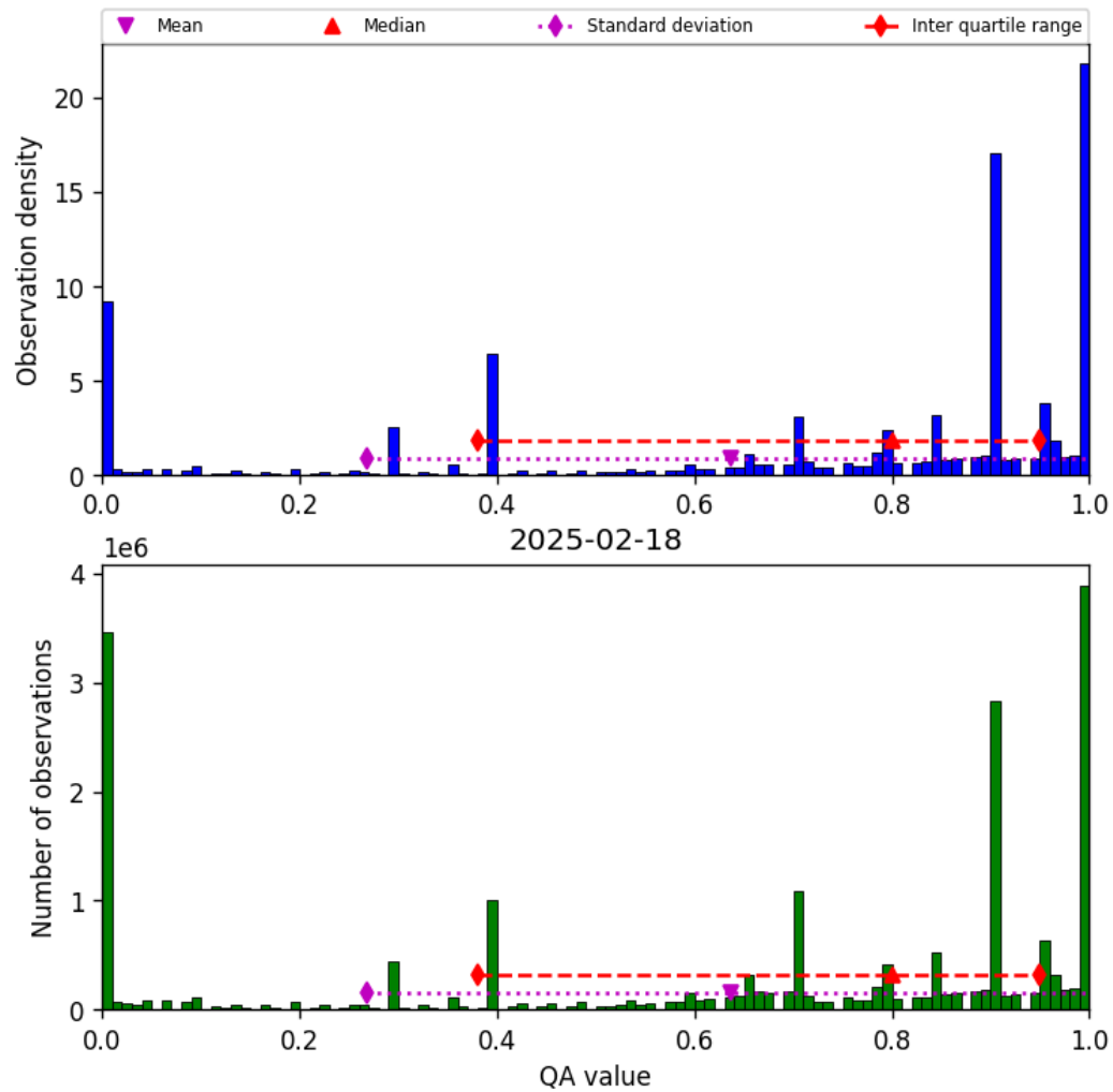
Figure 38: Histogram of “QA value” for 2025-02-18 to 2025-02-19
