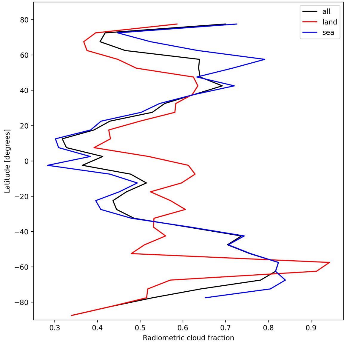
Figure 23: Zonal average of “Radiometric cloud fraction” for 2025-02-18 to 2025-02-19.
