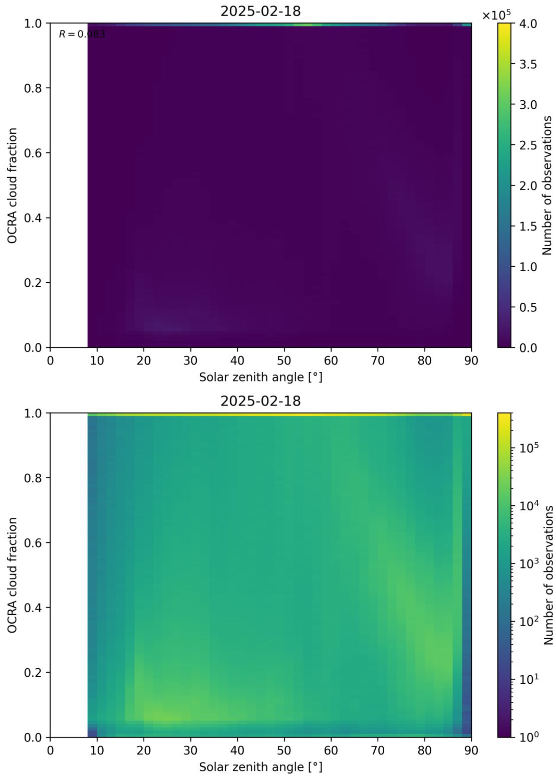
Figure 100: Scatter density plot of “Solar zenith angle” against “OCRA cloud fraction” for 2025-02-18 to 2025-02-19.
