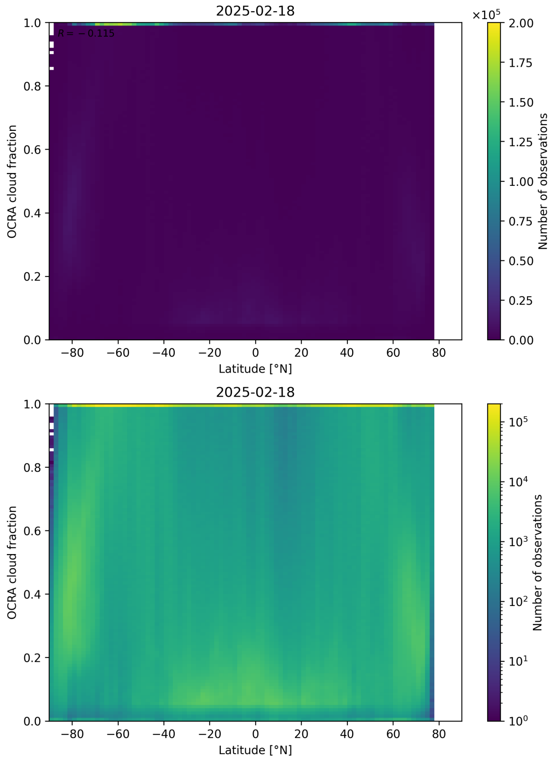
Figure 93: Scatter density plot of “Latitude” against “OCRA cloud fraction” for 2025-02-18 to 2025-02-19.
