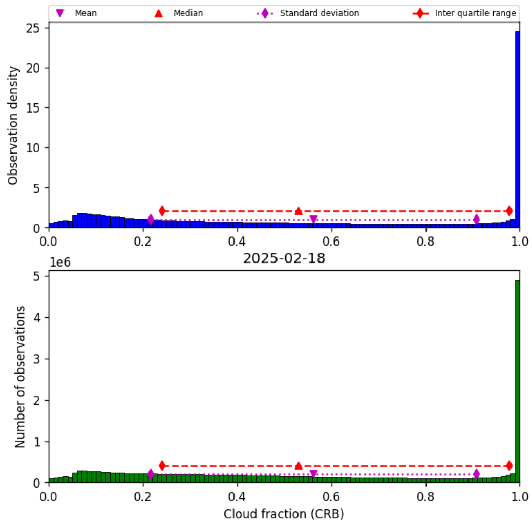
Figure 42: Histogram of “Cloud fraction (CRB)” for 2025-02-18 to 2025-02-19
