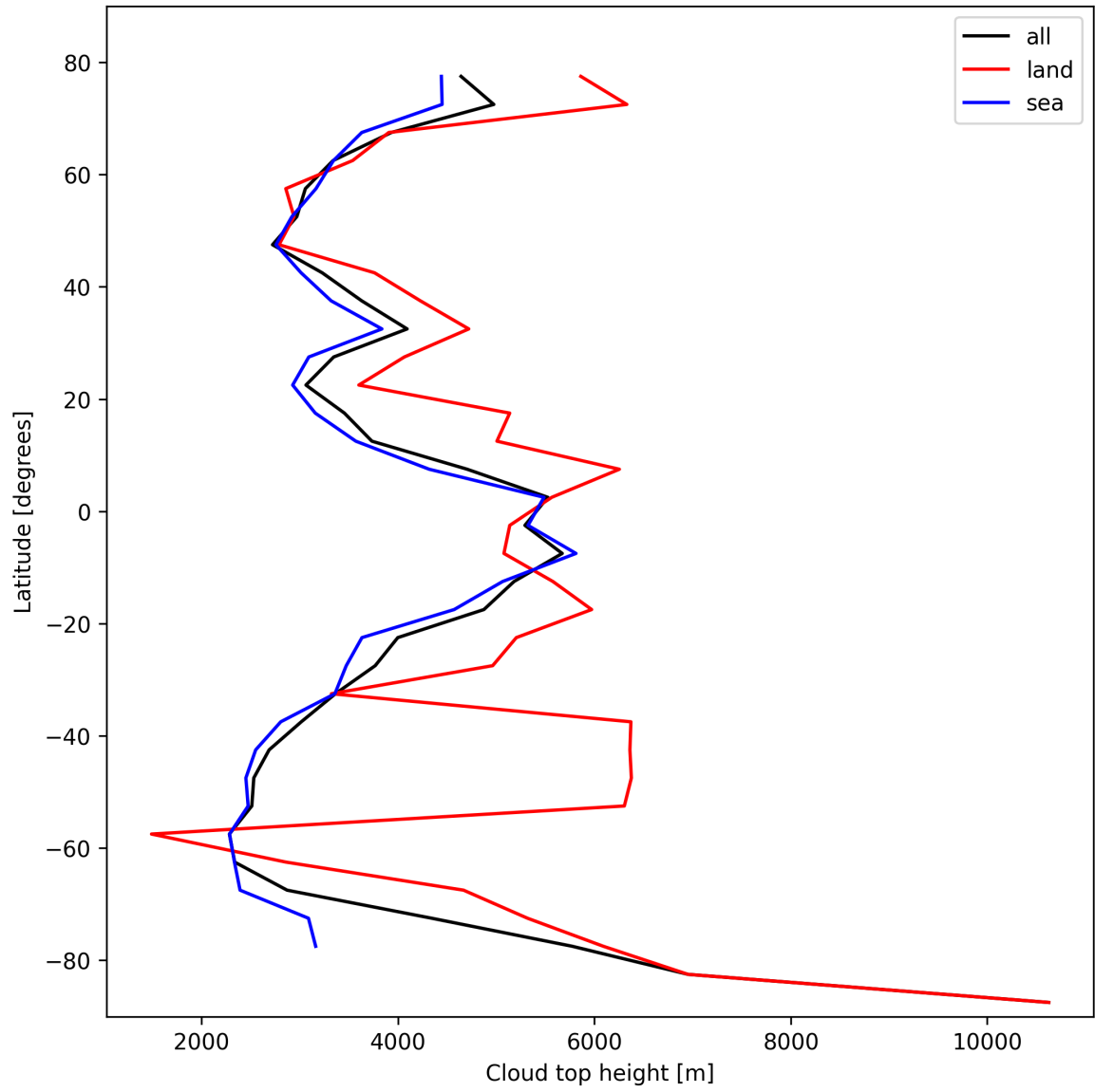
Figure 24: Zonal average of “Cloud top height” for 2025-02-18 to 2025-02-19.
