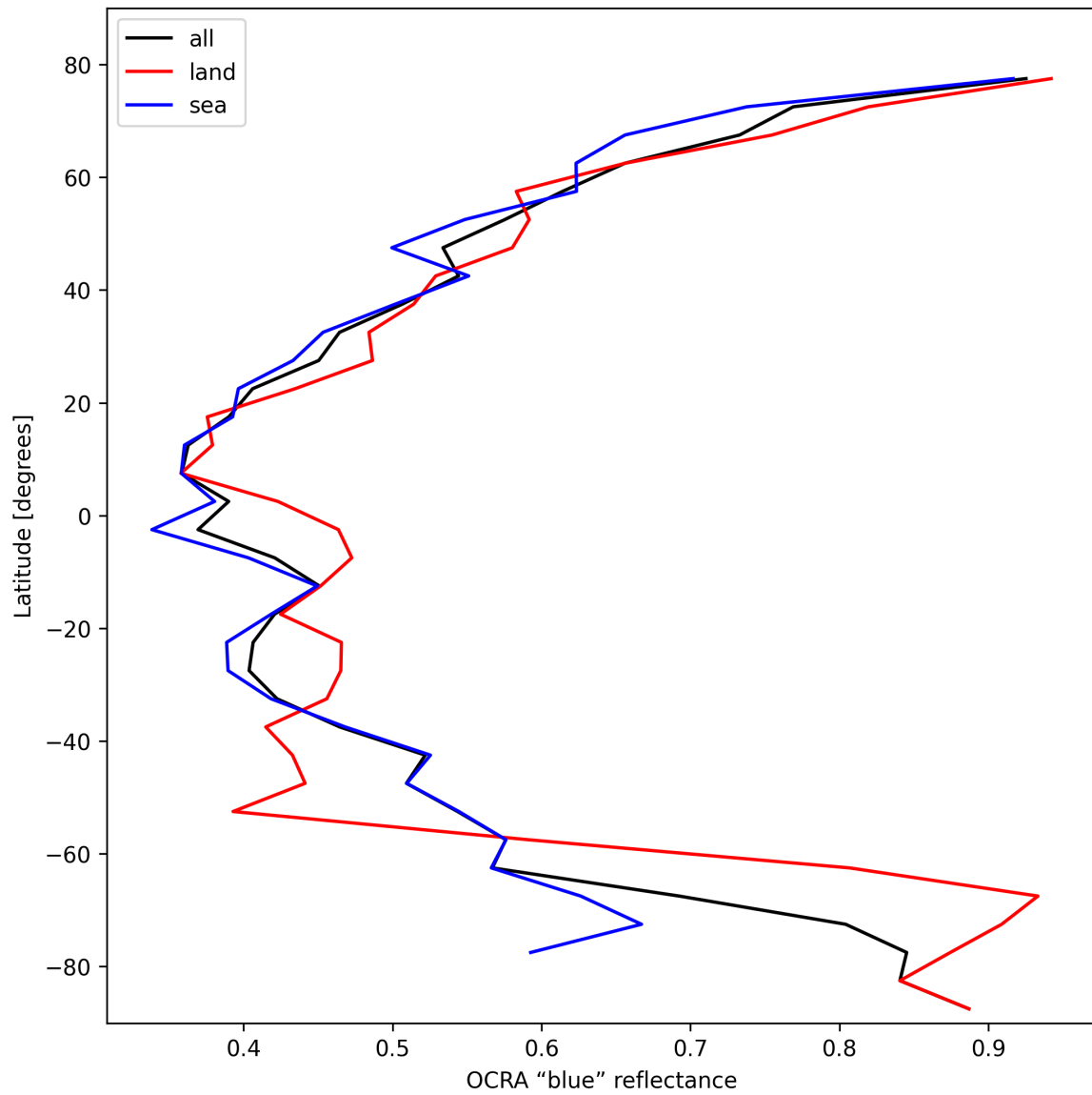
Figure 35: Zonal average of “OCRA “blue” reflectance” for 2025-02-18 to 2025-02-19.
