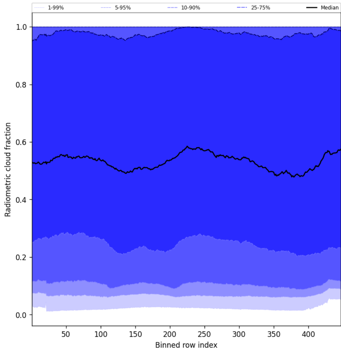
Figure 55: Along track statistics of “Radiometric cloud fraction” for 2025-02-18 to 2025-02-19
