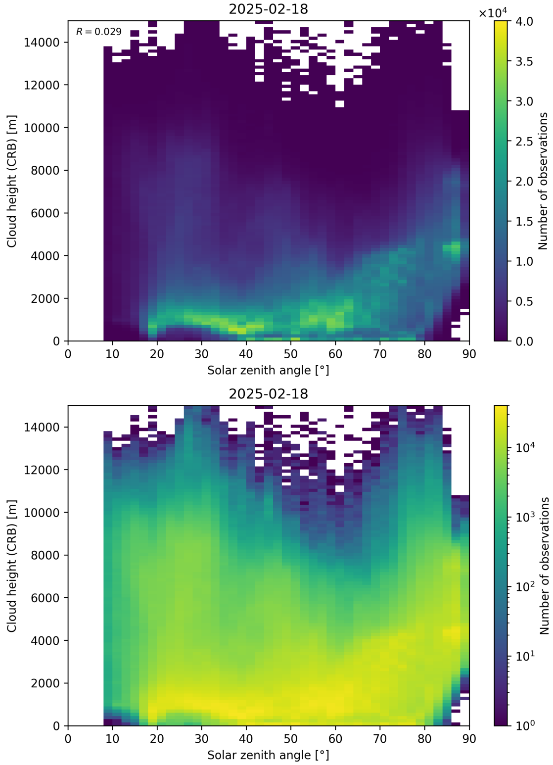
Figure 102: Scatter density plot of “Solar zenith angle” against “Cloud height (CRB)” for 2025-02-18 to 2025-02-19.
