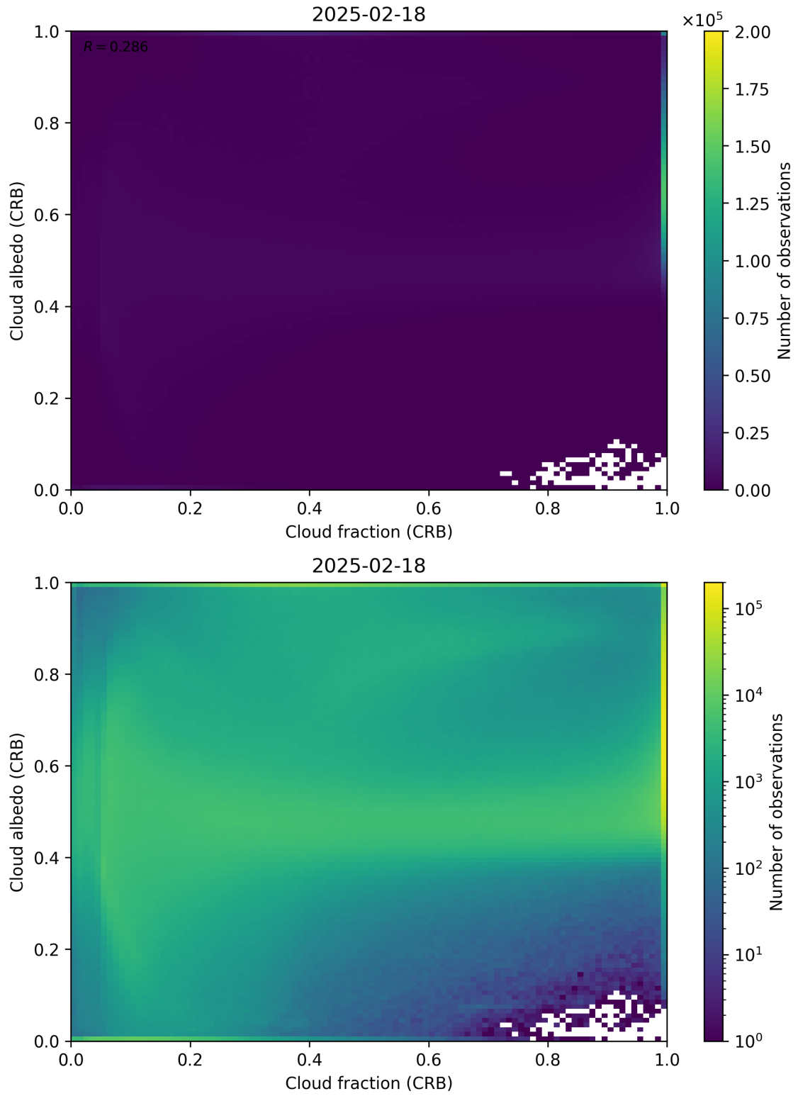
Figure 77: Scatter density plot of “Cloud fraction (CRB)” against “Cloud albedo (CRB)” for 2025-02-18 to 2025-02-19.
