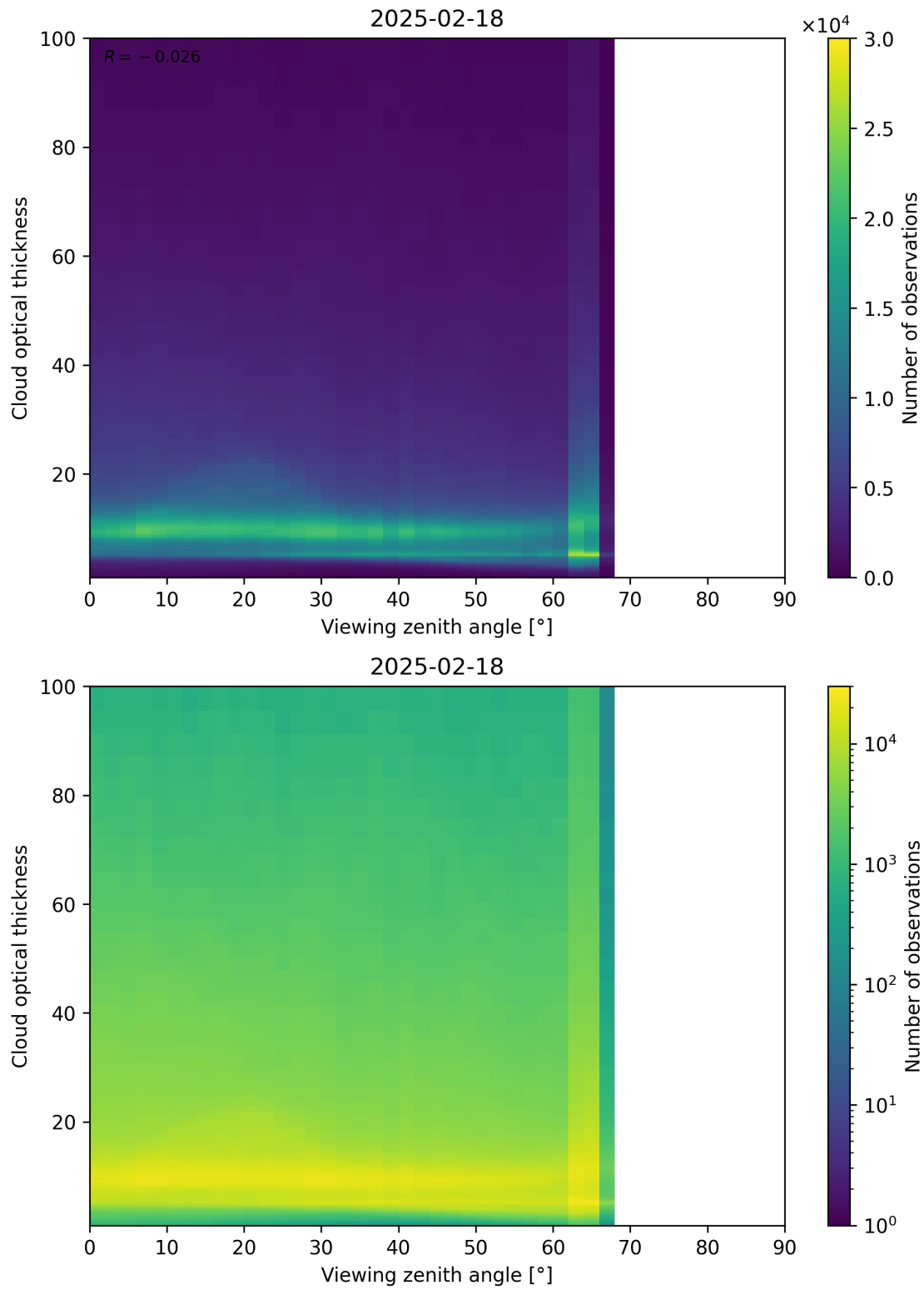
Figure 111: Scatter density plot of “Viewing zenith angle” against “Cloud optical thickness” for 2025-02-18 to 2025-02-19.
