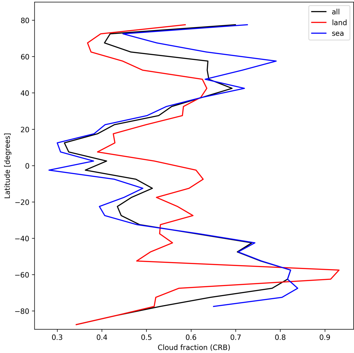
Figure 26: Zonal average of “Cloud fraction (CRB)” for 2025-02-18 to 2025-02-19.
