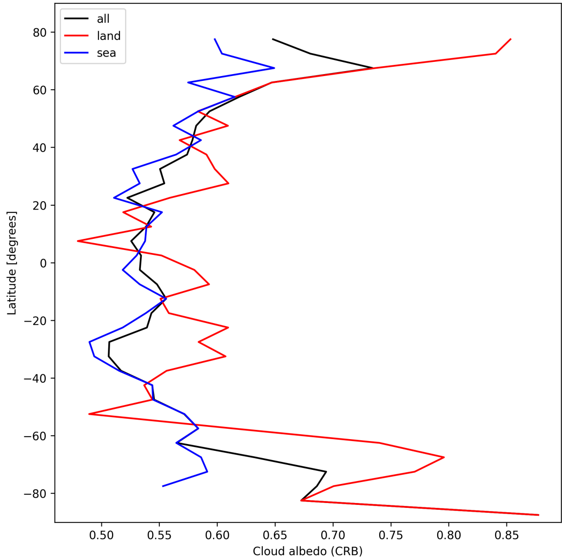
Figure 28: Zonal average of “Cloud albedo (CRB)” for 2025-02-18 to 2025-02-19.
