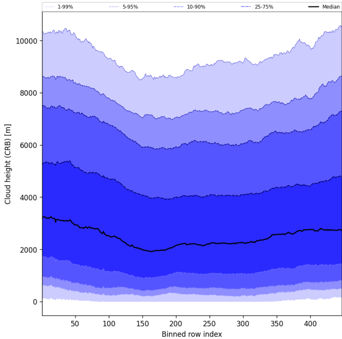
Figure 59: Along track statistics of “Cloud height (CRB)” for 2025-02-18 to 2025-02-19
