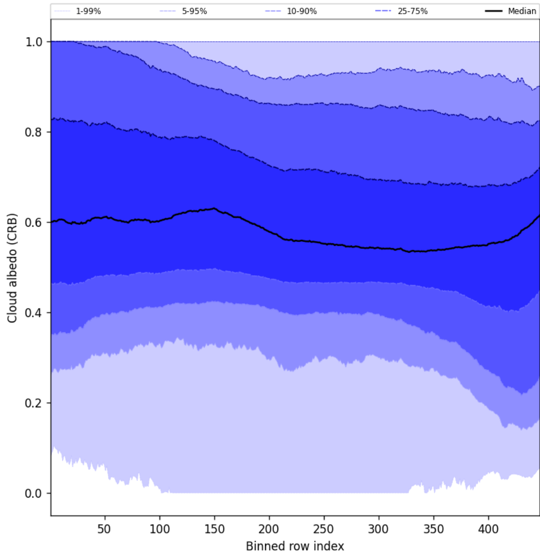
Figure 60: Along track statistics of “Cloud albedo (CRB)” for 2025-02-18 to 2025-02-19
