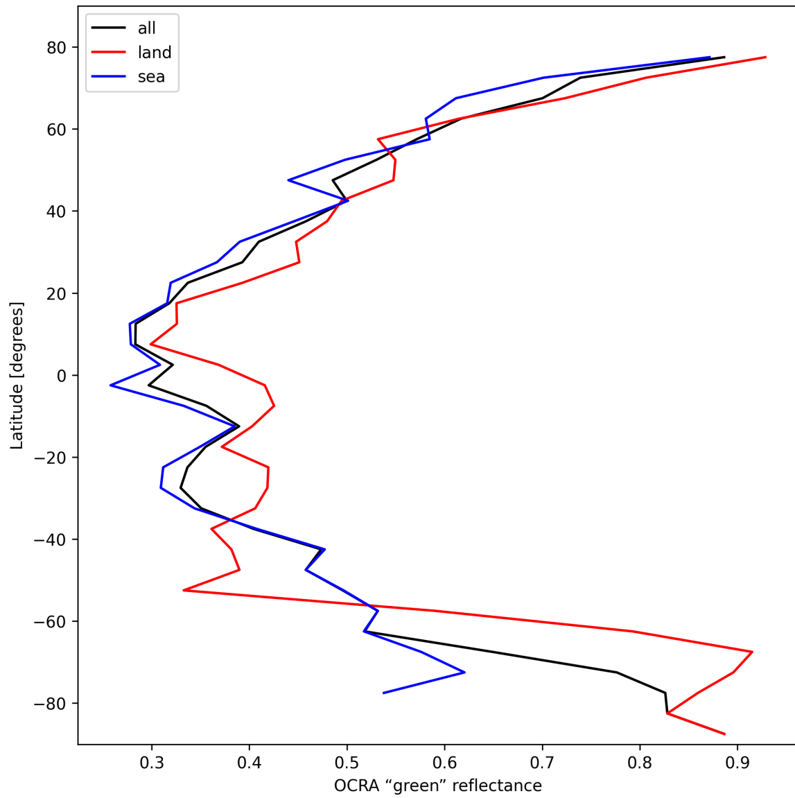
Figure 36: Zonal average of “OCRA “green” reflectance” for 2025-02-18 to 2025-02-19.
