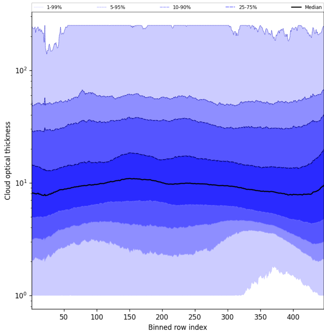
Figure 57: Along track statistics of “Cloud optical thickness” for 2025-02-18 to 2025-02-19
