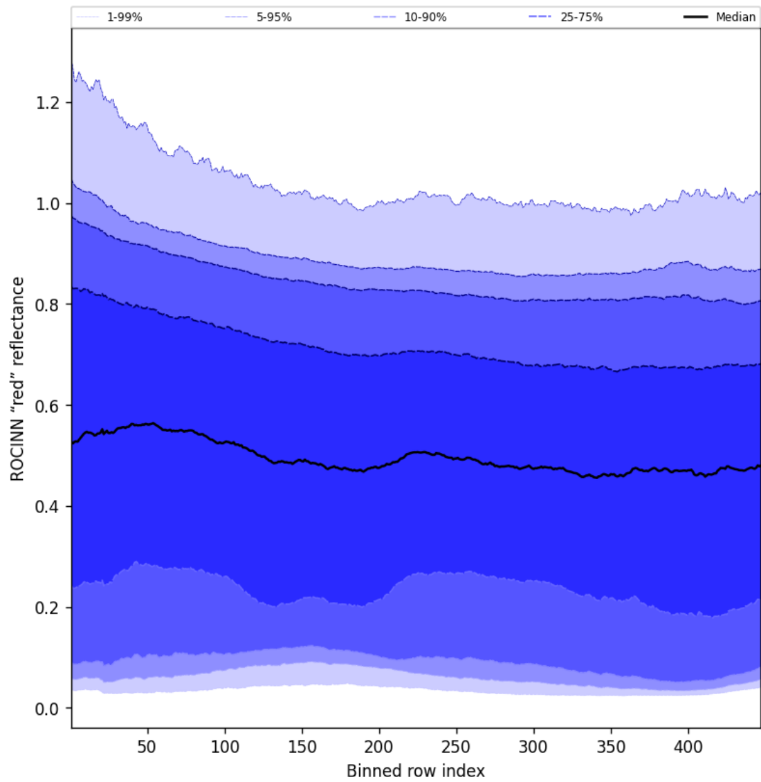
Figure 69: Along track statistics of “ROCINN “red” reflectance” for 2025-02-18 to 2025-02-19
