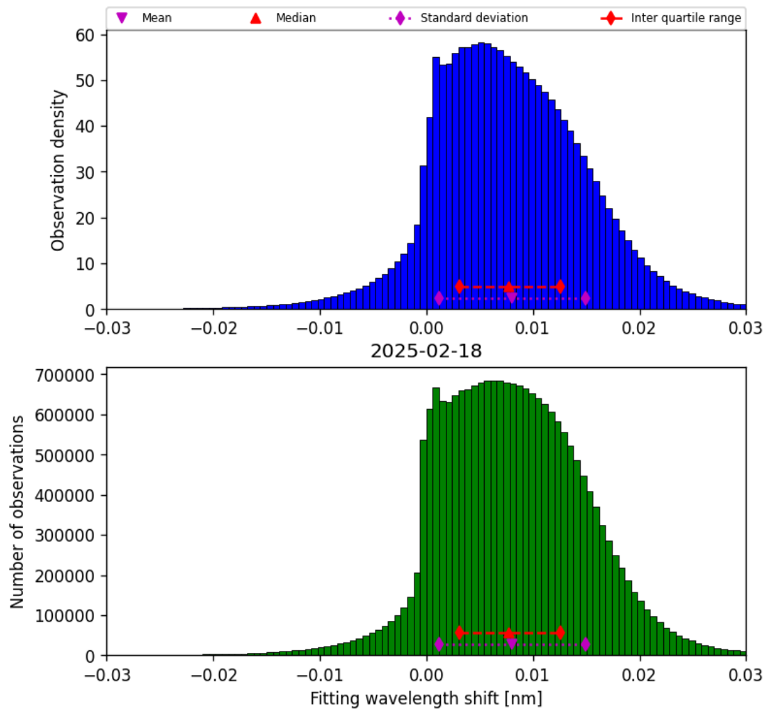
Figure 49: Histogram of “Fitting wavelength shift” for 2025-02-18 to 2025-02-19
