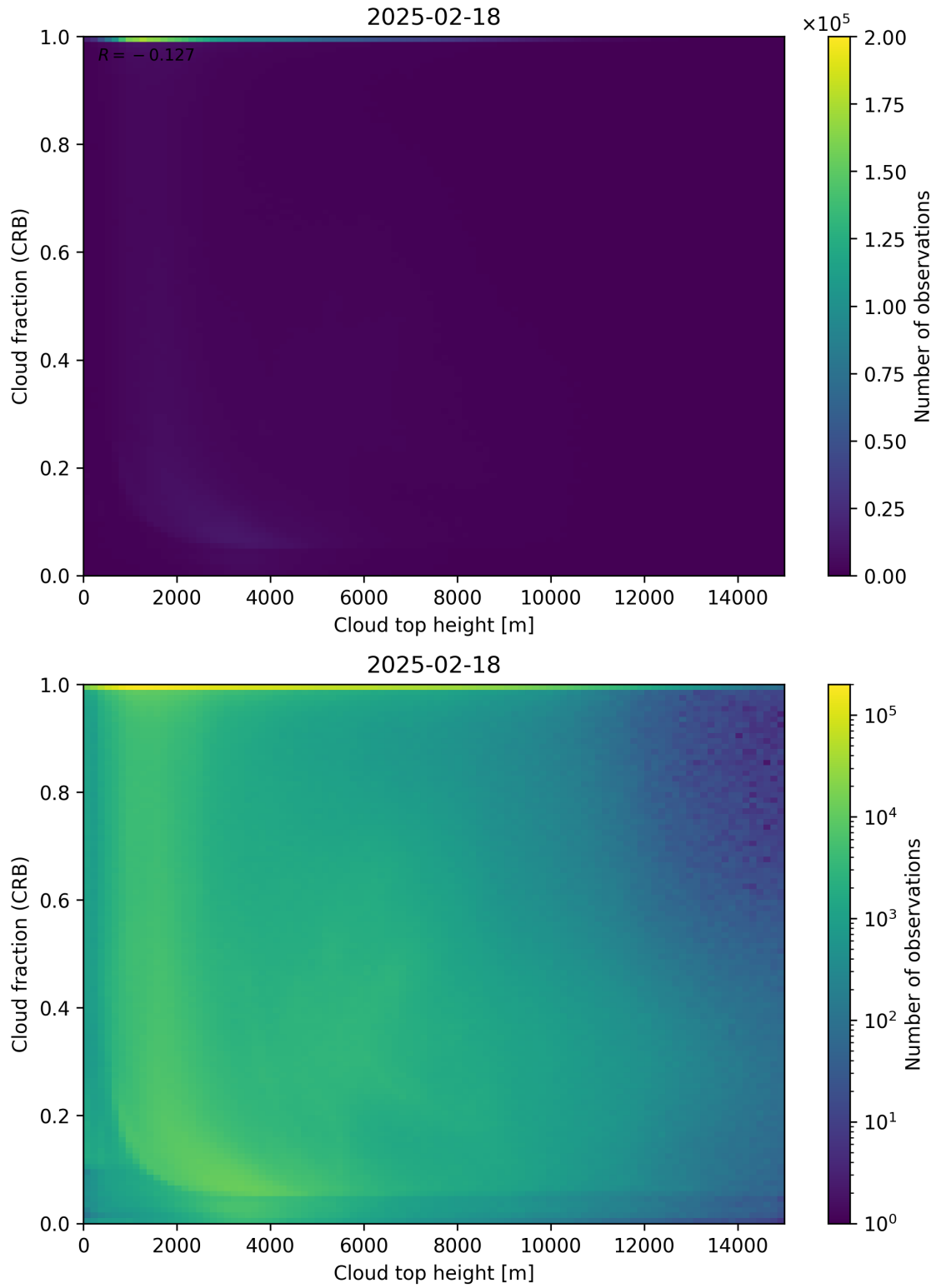
Figure 88: Scatter density plot of “Cloud top height” against “Cloud fraction (CRB)” for 2025-02-18 to 2025-02-19.
