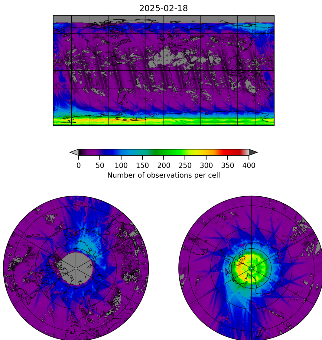
Figure 21: Map of the number of observations for 2025-02-18 to 2025-02-19
