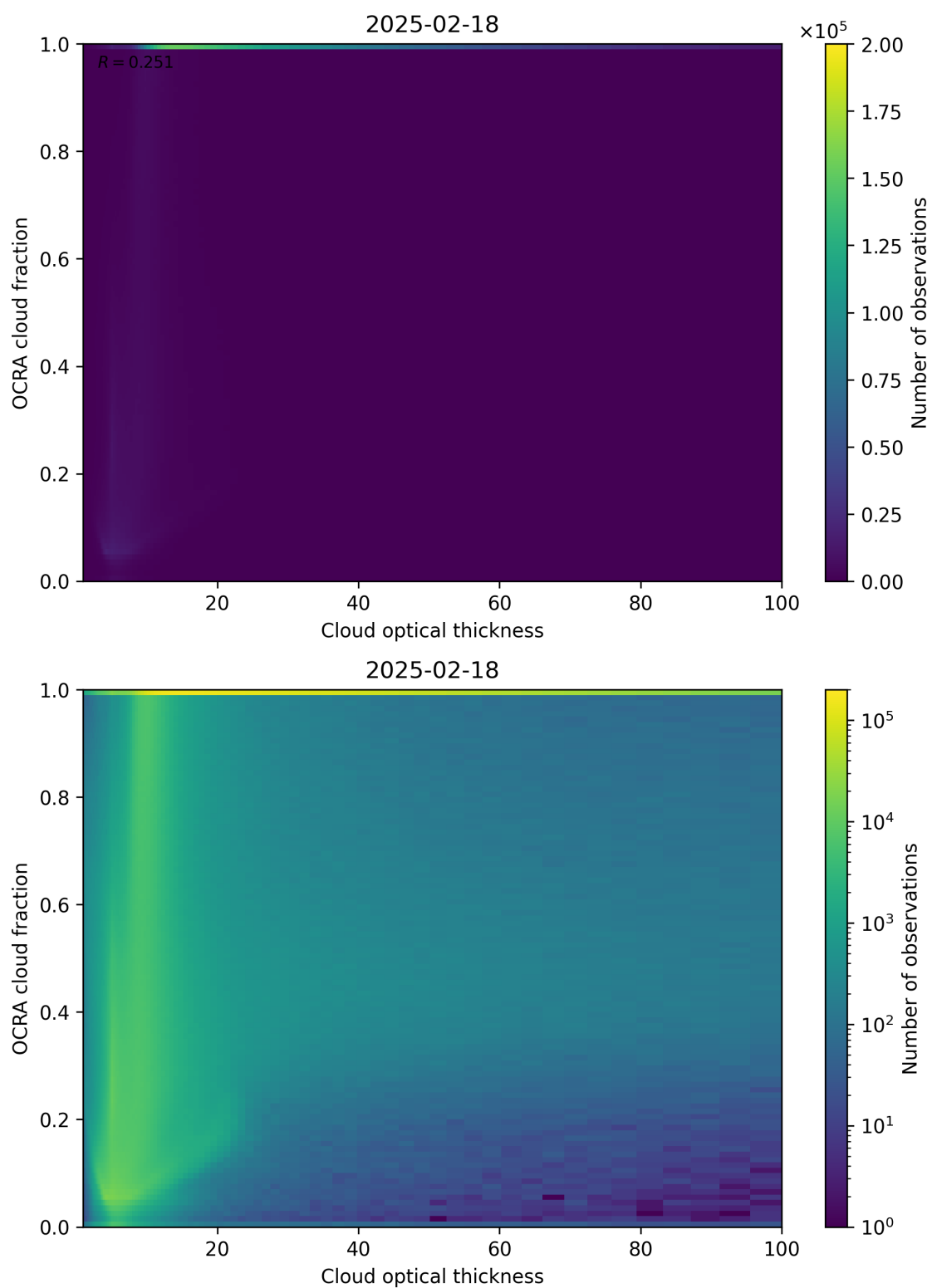
Figure 83: Scatter density plot of “Cloud optical thickness” against “OCRA cloud fraction” for 2025-02-18 to 2025-02-19.
