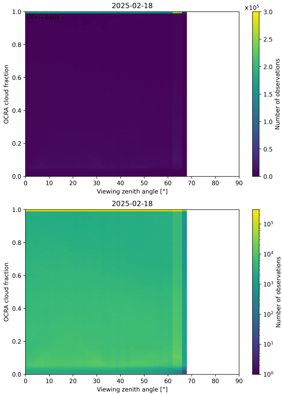
Figure 108: Scatter density plot of “Viewing zenith angle” against “OCRA cloud fraction” for 2025-02-18 to 2025-02-19.
