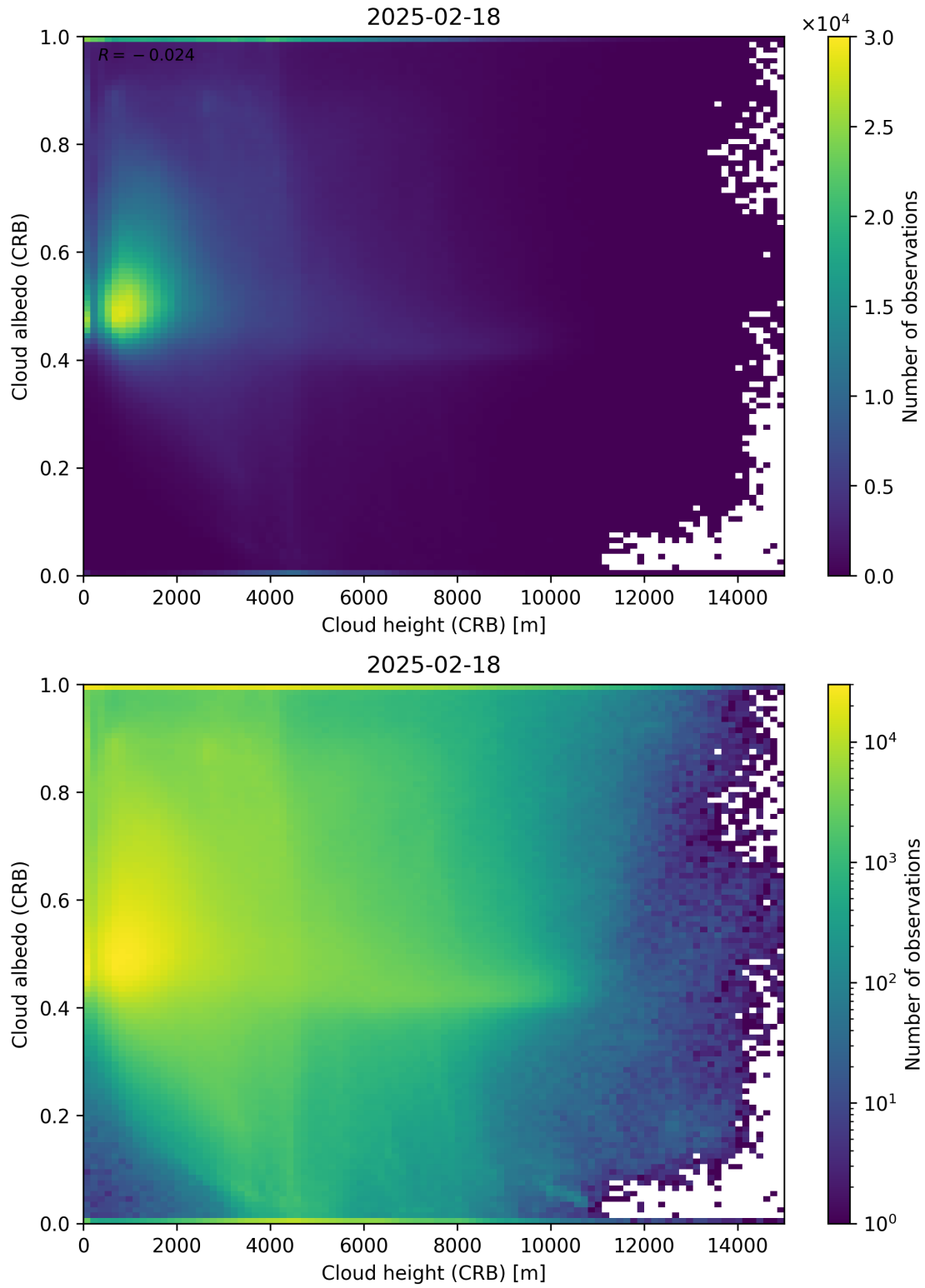
Figure 80: Scatter density plot of “Cloud height (CRB)” against “Cloud albedo (CRB)” for 2025-02-18 to 2025-02-19.
