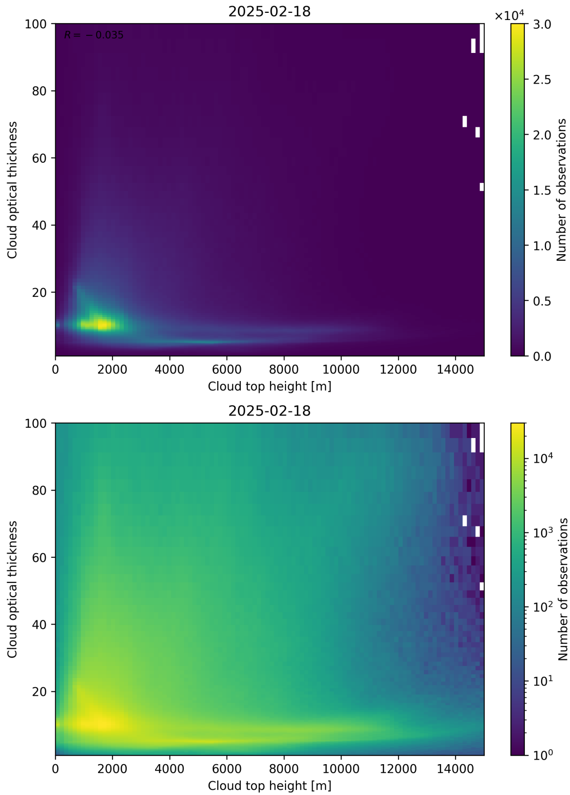
Figure 90: Scatter density plot of “Cloud top height” against “Cloud optical thickness” for 2025-02-18 to 2025-02-19.
