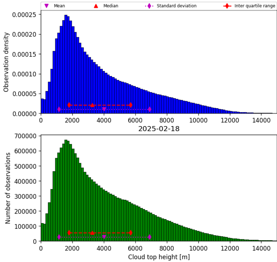
Figure 40: Histogram of “Cloud top height” for 2025-02-18 to 2025-02-19
