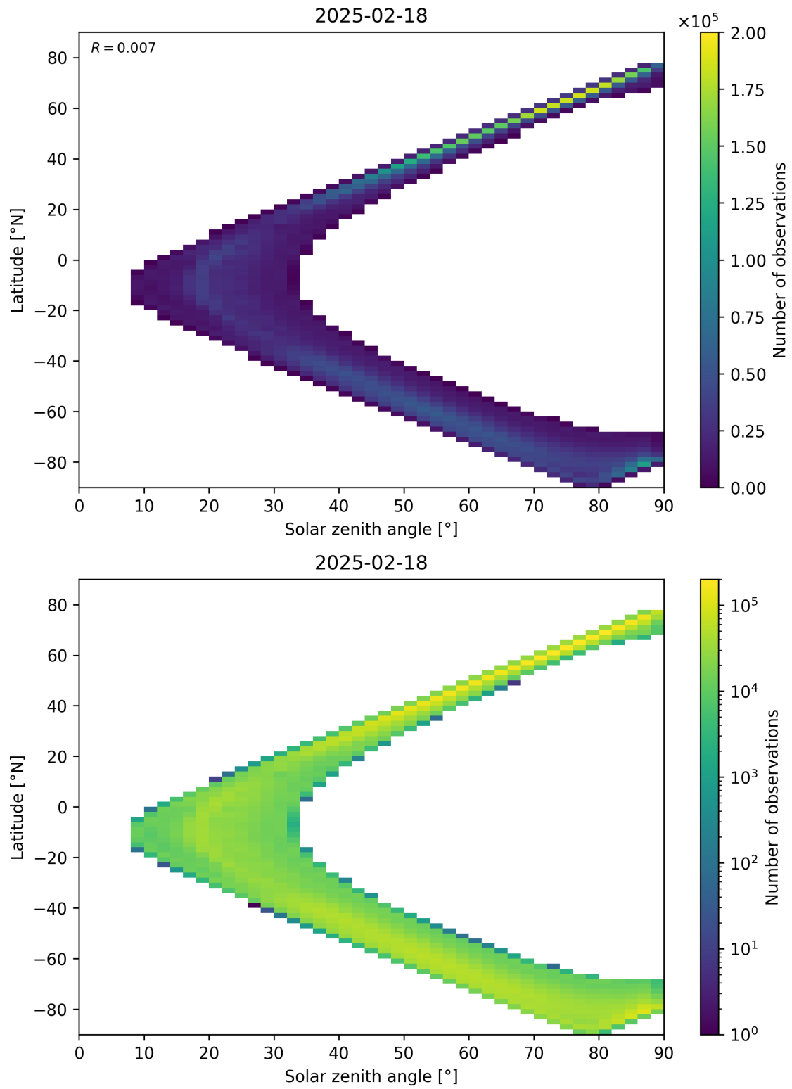
Figure 105: Scatter density plot of “Solar zenith angle” against “Latitude” for 2025-02-18 to 2025-02-19.
