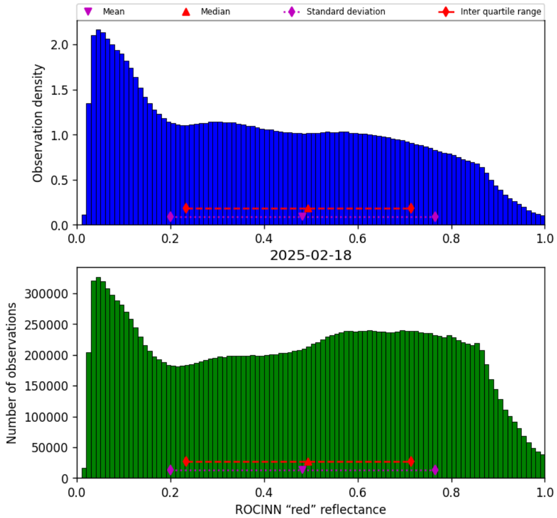
Figure 53: Histogram of “ROCINN “red” reflectance” for 2025-02-18 to 2025-02-19
