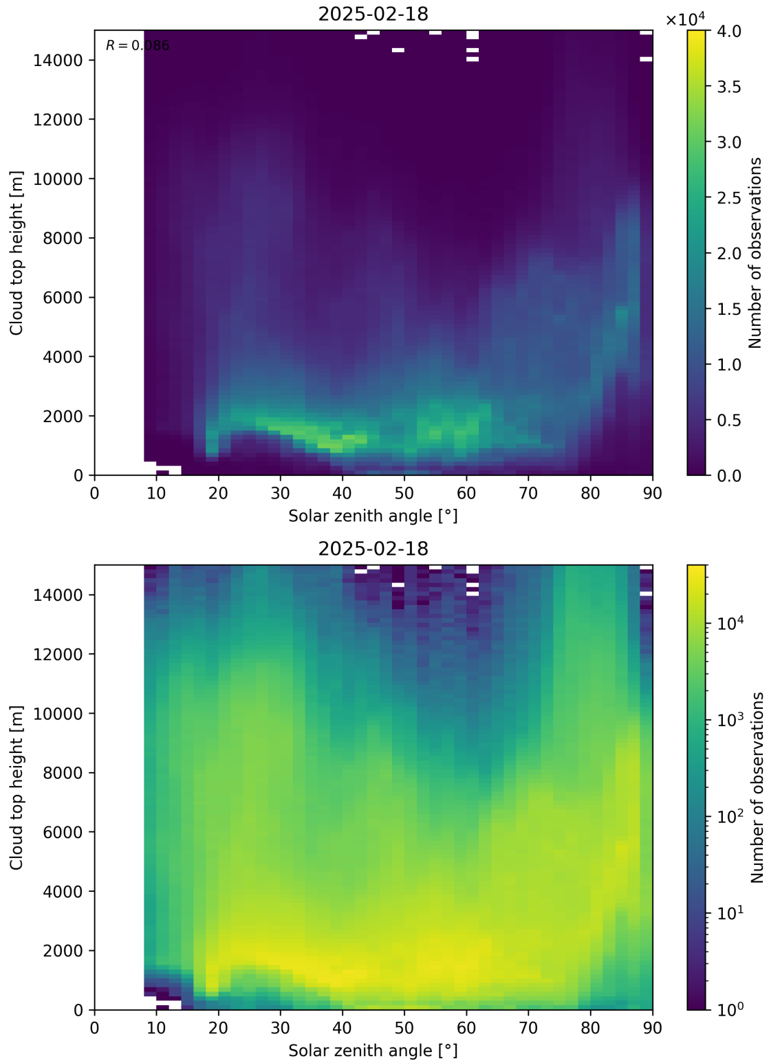
Figure 104: Scatter density plot of “Solar zenith angle” against “Cloud top height” for 2025-02-18 to 2025-02-19.
