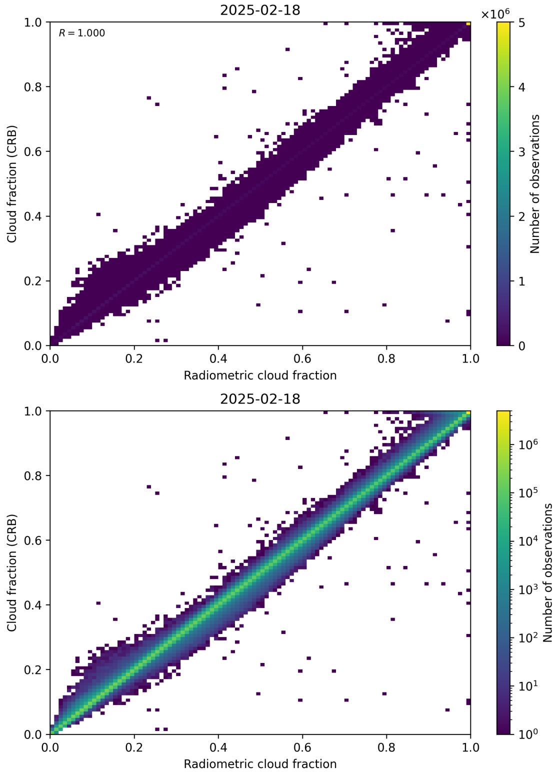
Figure 73: Scatter density plot of “Radiometric cloud fraction” against “Cloud fraction (CRB)” for 2025-02-18 to 2025-02-19.
