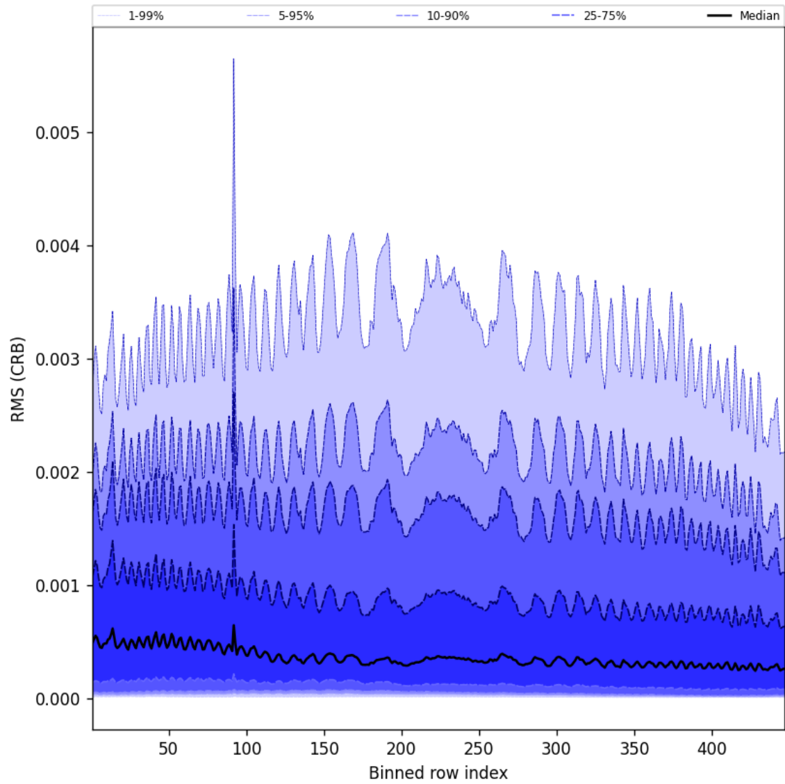
Figure 64: Along track statistics of “RMS (CRB)” for 2025-02-18 to 2025-02-19
