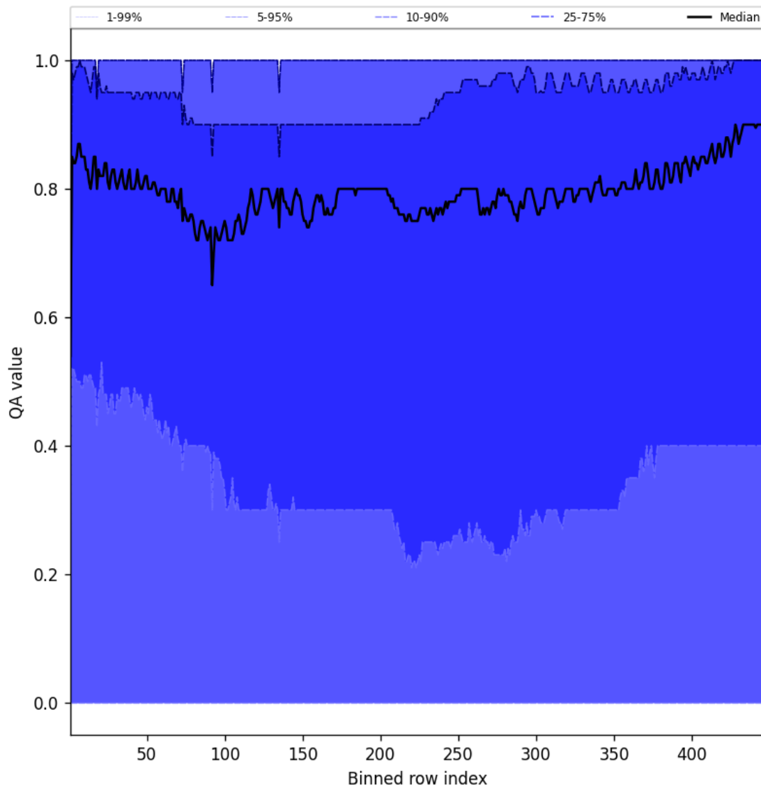
Figure 54: Along track statistics of “QA value” for 2025-02-18 to 2025-02-19
