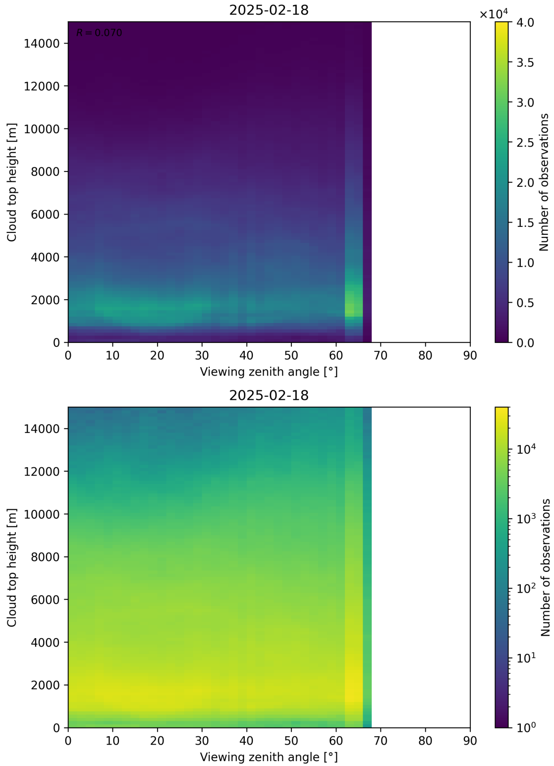
Figure 112: Scatter density plot of “Viewing zenith angle” against “Cloud top height” for 2025-02-18 to 2025-02-19.
