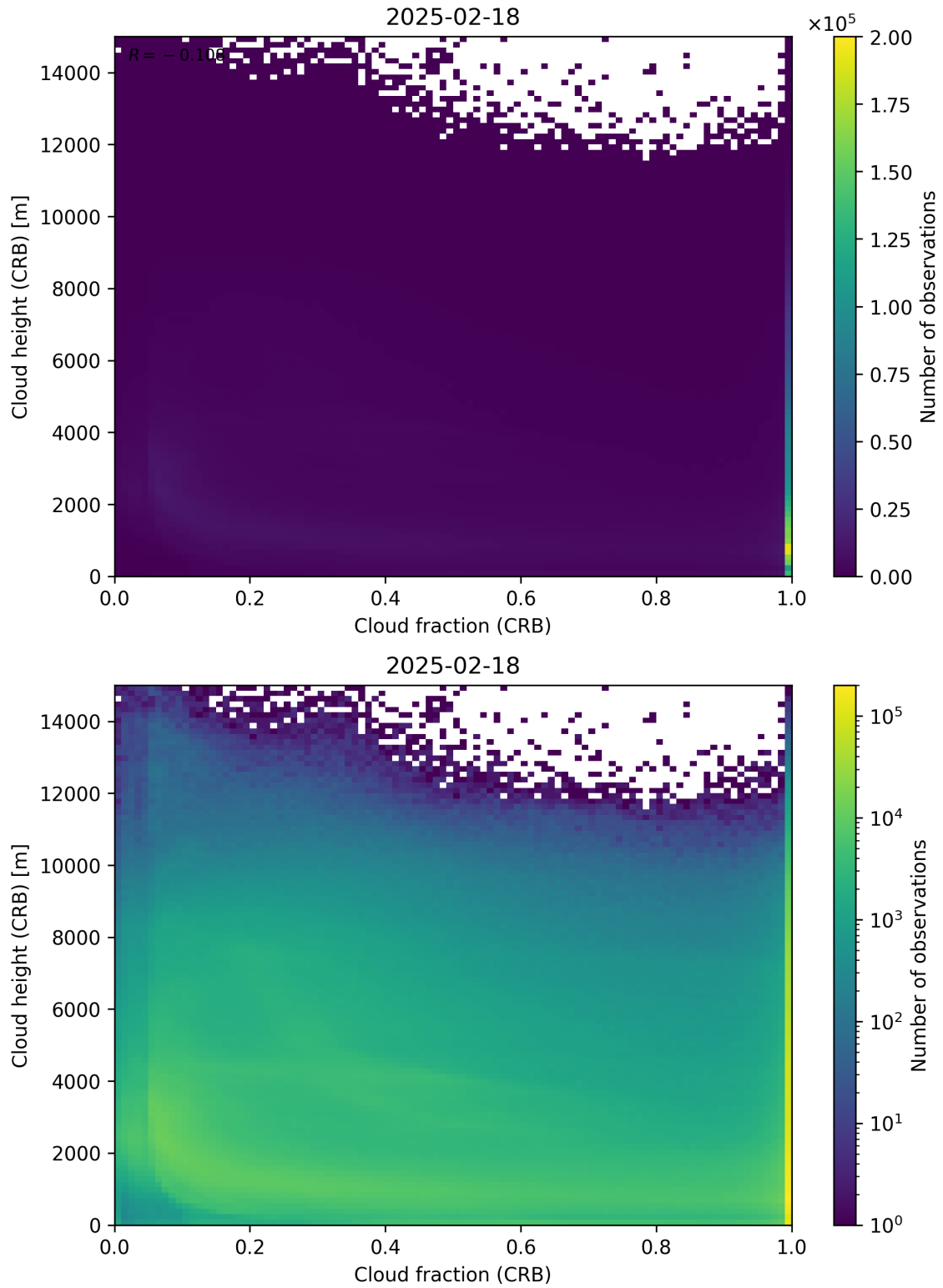
Figure 79: Scatter density plot of “Cloud fraction (CRB)” against “Cloud height (CRB)” for 2025-02-18 to 2025-02-19.
