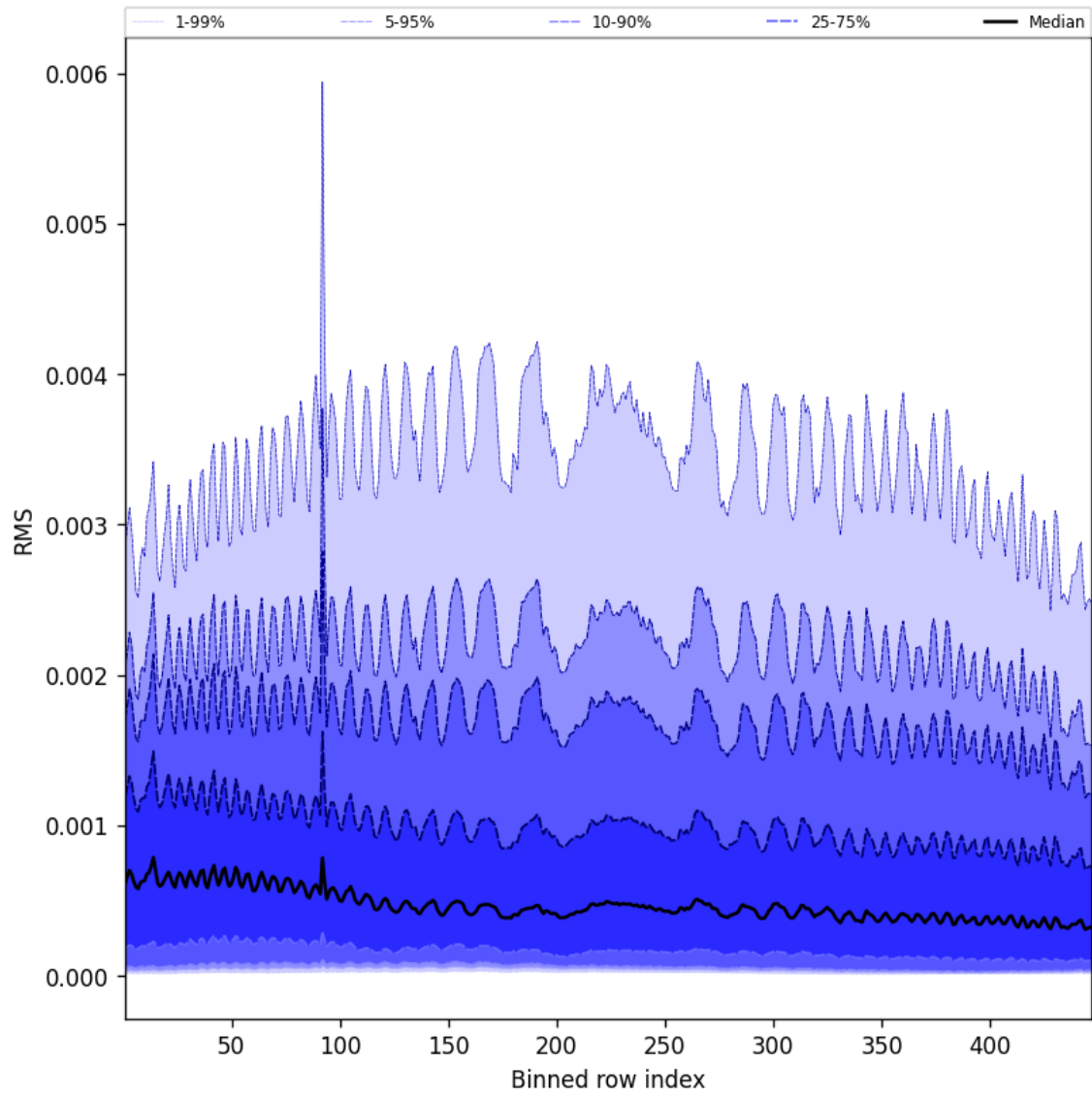
Figure 63: Along track statistics of “RMS” for 2025-02-18 to 2025-02-19
