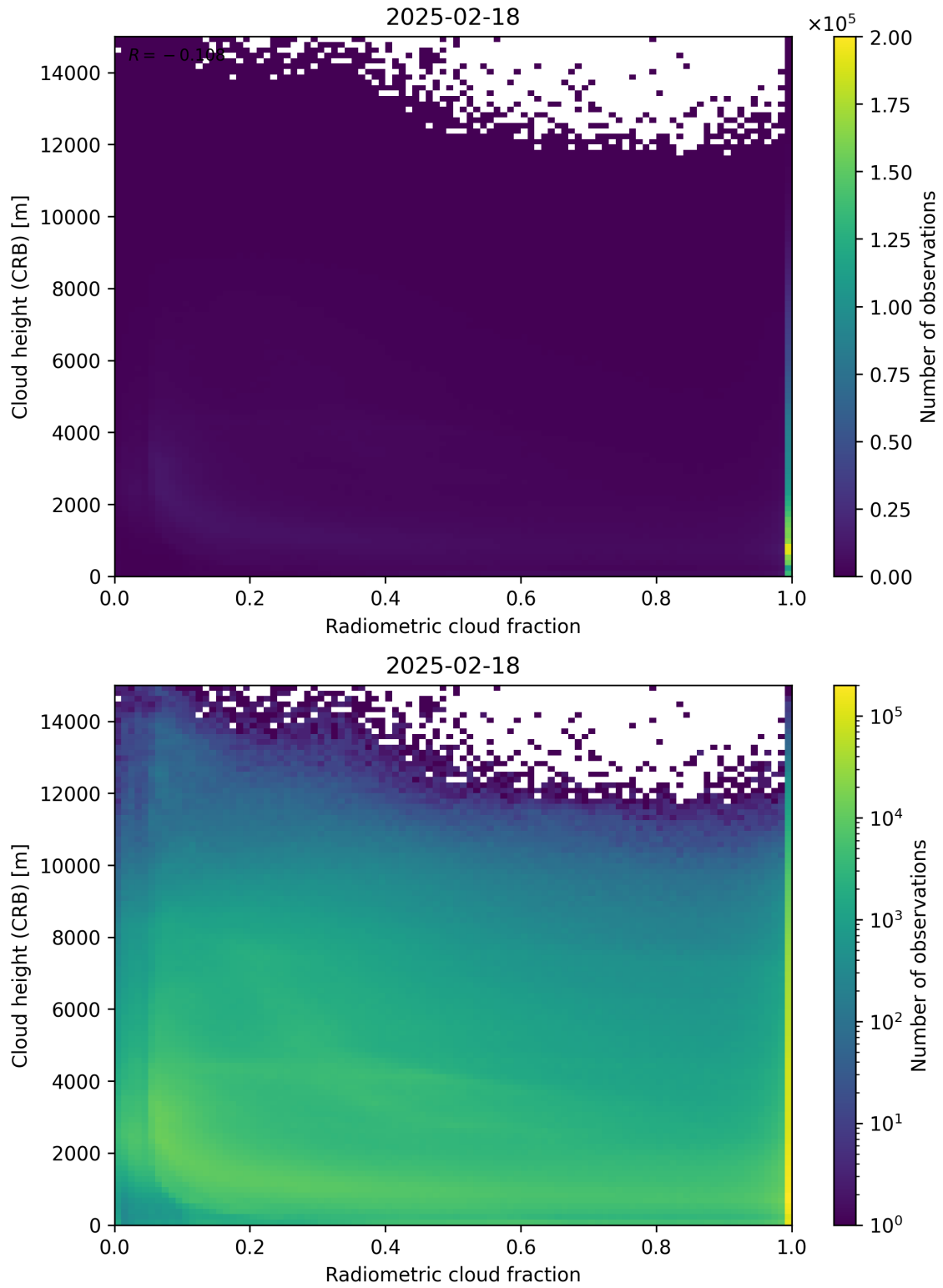
Figure 74: Scatter density plot of “Radiometric cloud fraction” against “Cloud height (CRB)” for 2025-02-18 to 2025-02-19.
