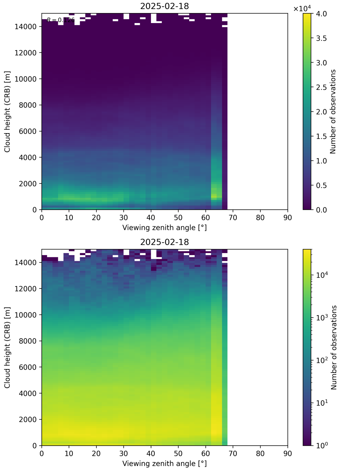
Figure 110: Scatter density plot of “Viewing zenith angle” against “Cloud height (CRB)” for 2025-02-18 to 2025-02-19.
