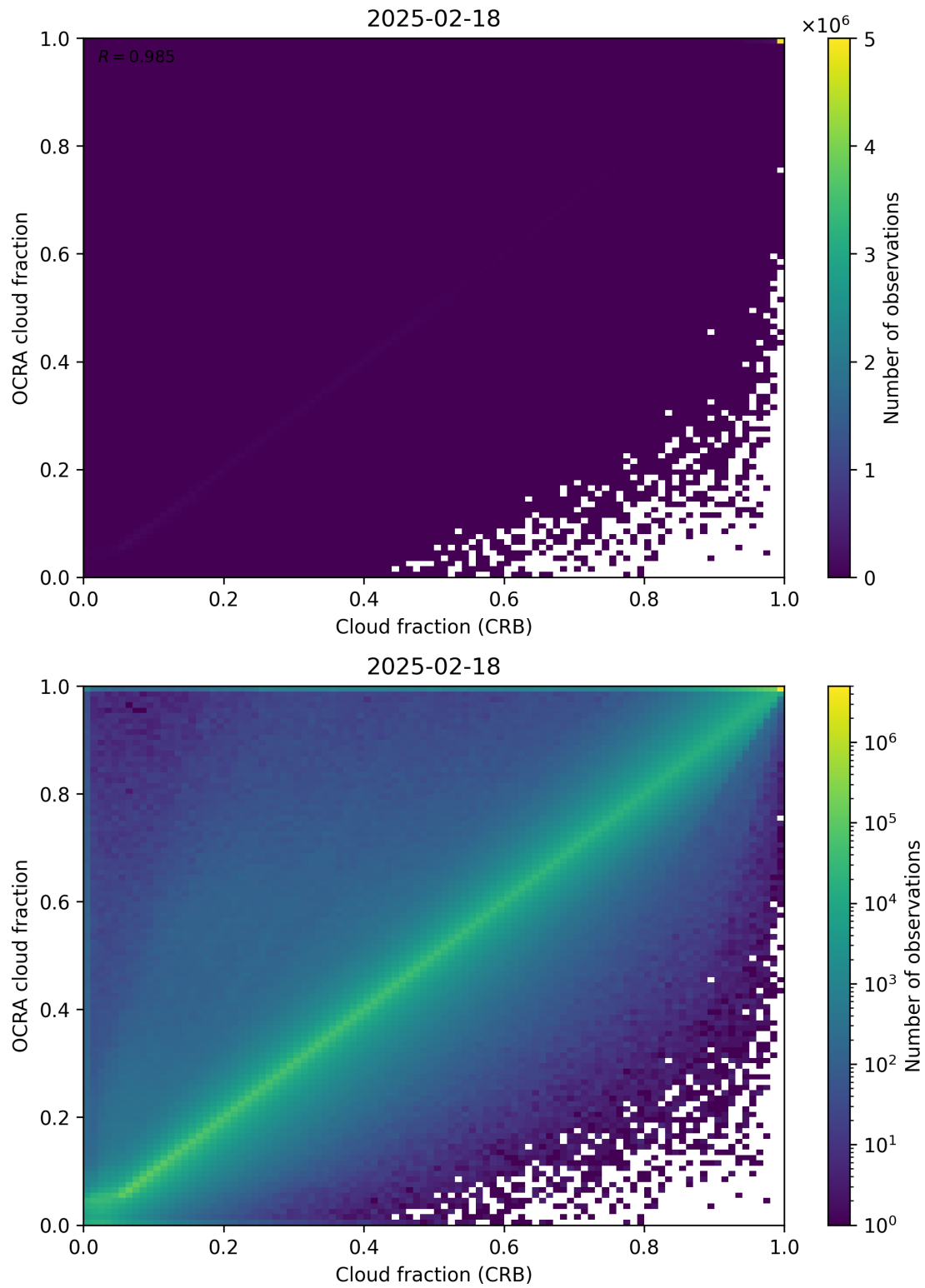
Figure 78: Scatter density plot of “Cloud fraction (CRB)” against “OCRA cloud fraction” for 2025-02-18 to 2025-02-19.
