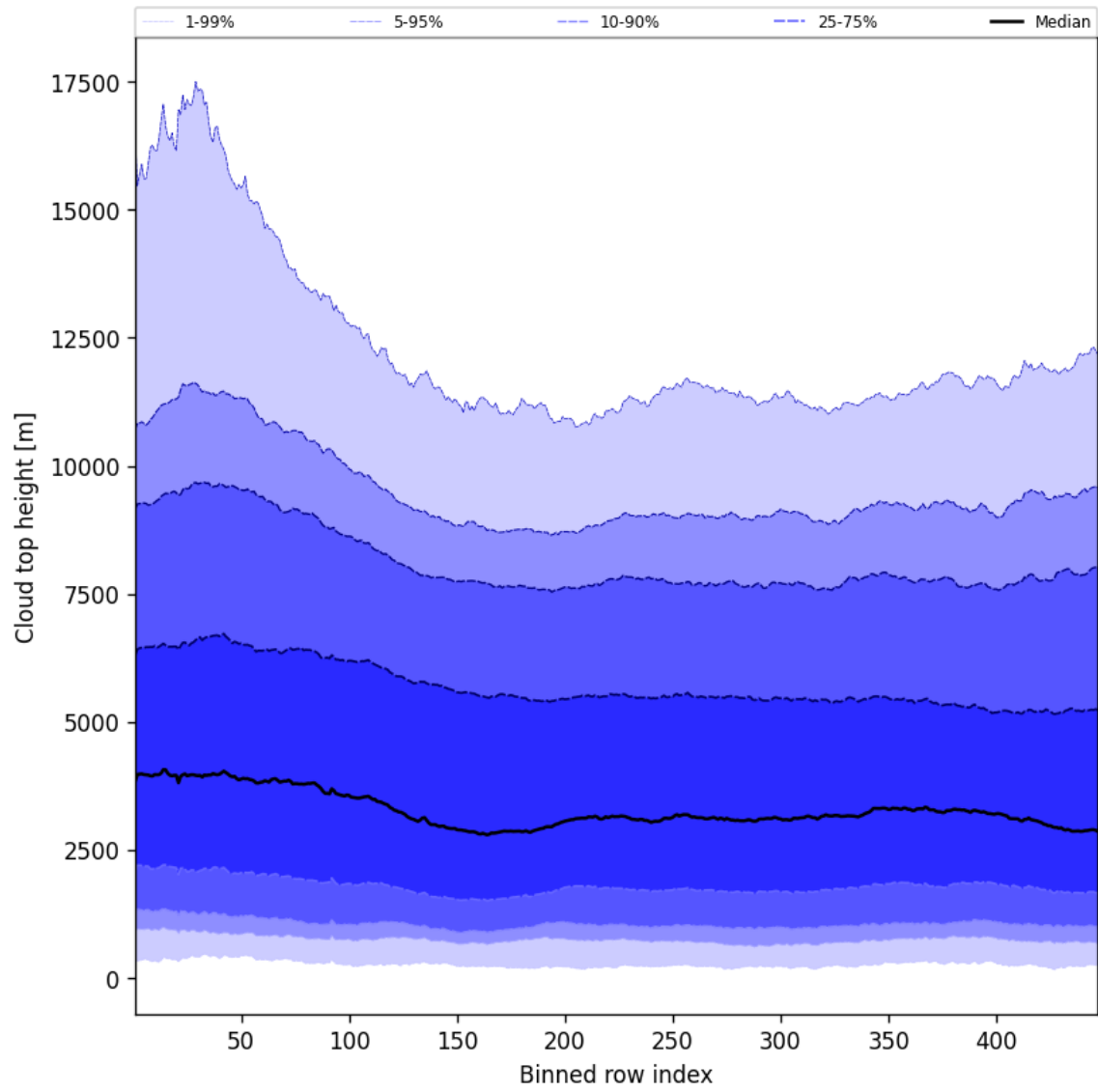
Figure 56: Along track statistics of “Cloud top height” for 2025-02-18 to 2025-02-19
