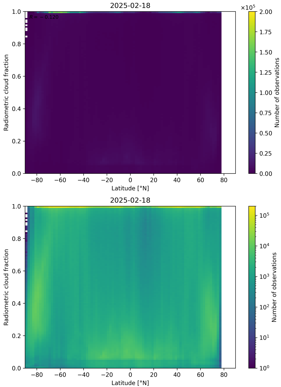
Figure 92: Scatter density plot of “Latitude” against “Radiometric cloud fraction” for 2025-02-18 to 2025-02-19.
