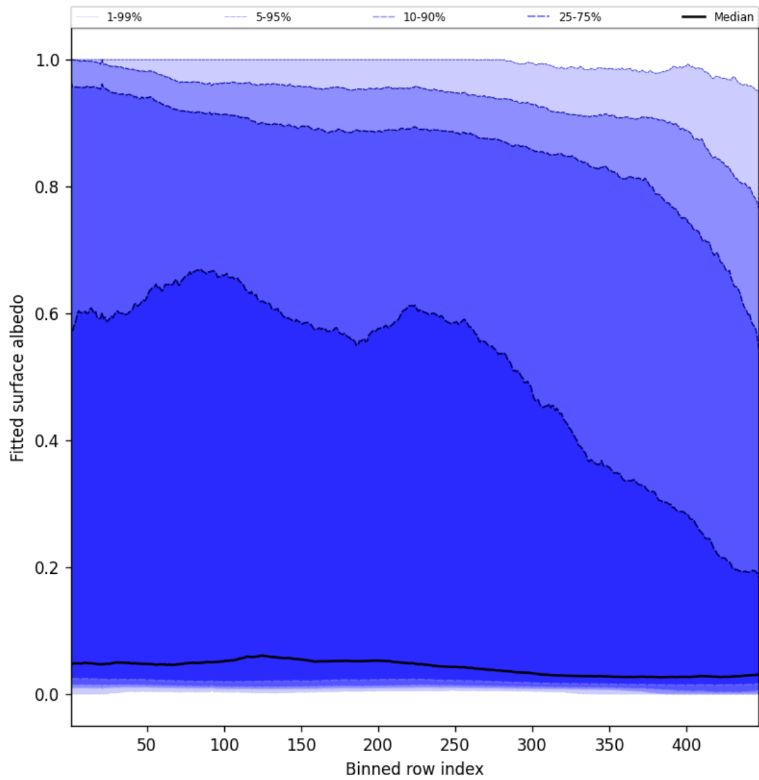
Figure 61: Along track statistics of “Fitted surface albedo” for 2025-02-18 to 2025-02-19
