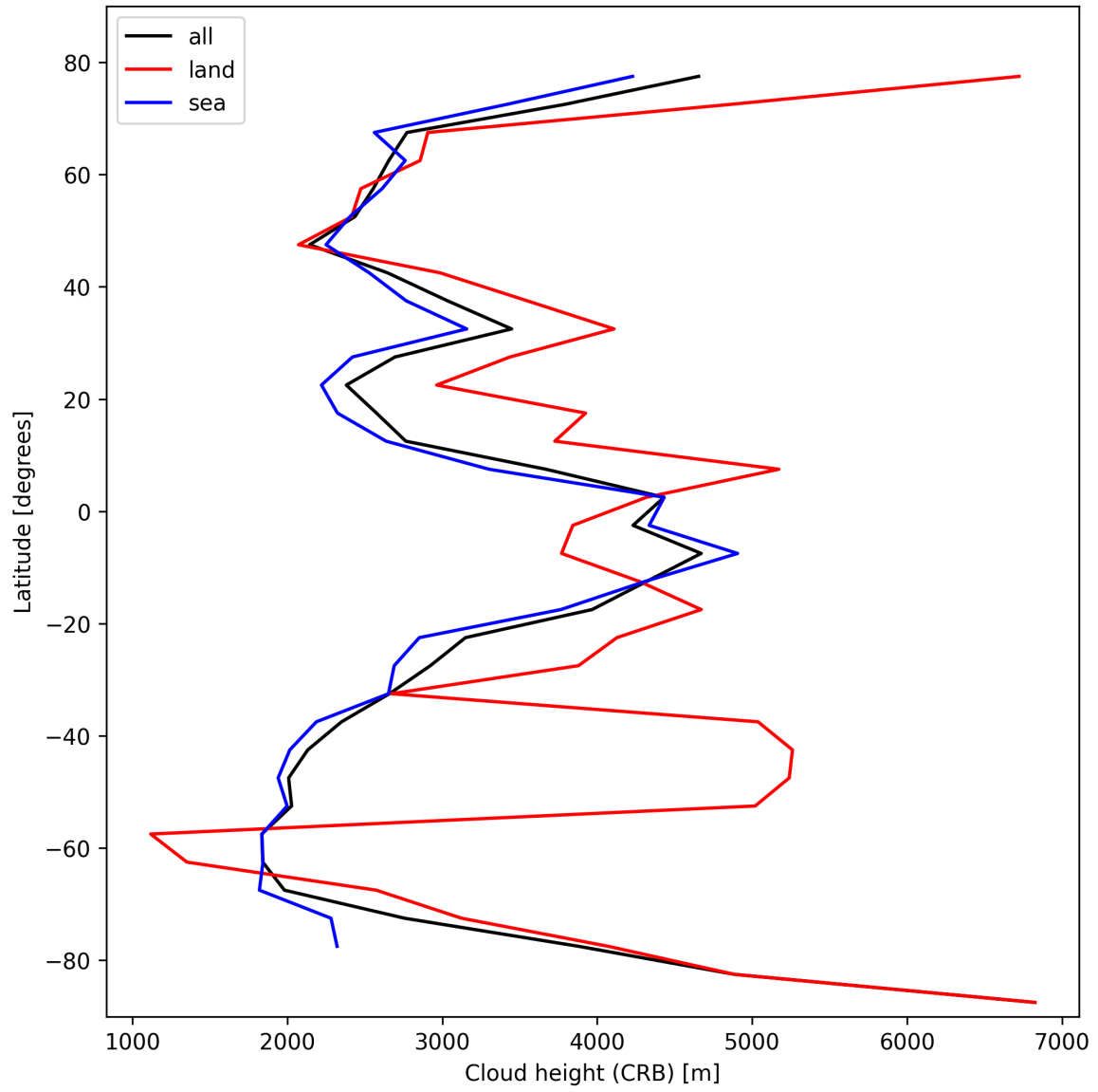
Figure 27: Zonal average of “Cloud height (CRB)” for 2025-02-18 to 2025-02-19.
