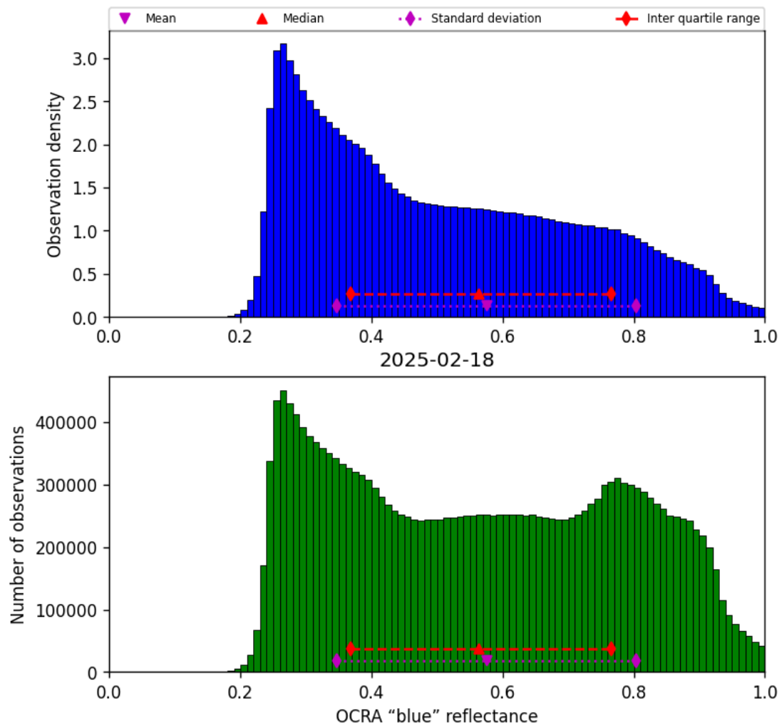
Figure 51: Histogram of “OCRA “blue” reflectance” for 2025-02-18 to 2025-02-19
