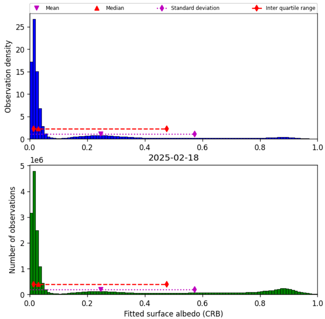
Figure 46: Histogram of “Fitted surface albedo (CRB)” for 2025-02-18 to 2025-02-19
