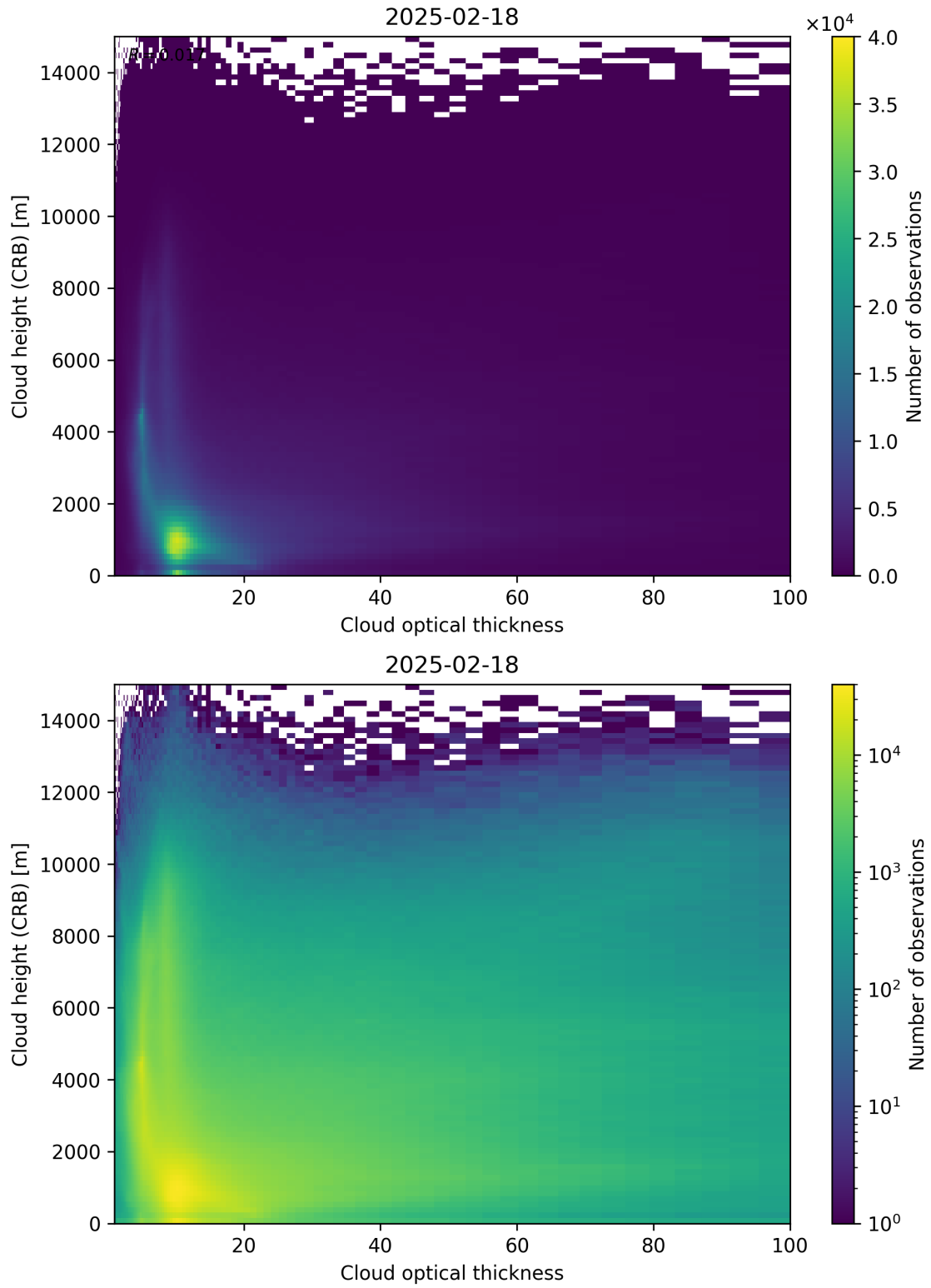
Figure 85: Scatter density plot of “Cloud optical thickness” against “Cloud height (CRB)” for 2025-02-18 to 2025-02-19.
