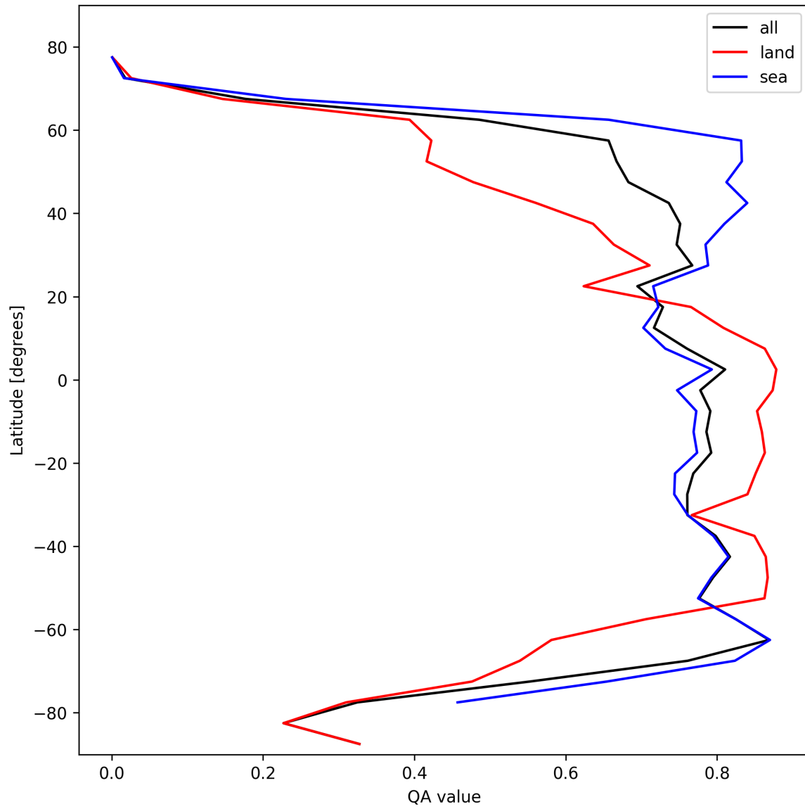
Figure 22: Zonal average of “QA value” for 2025-02-18 to 2025-02-19.
