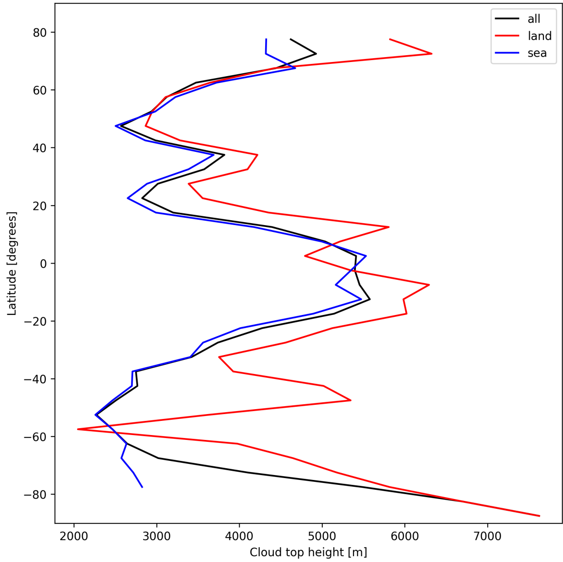
Figure 24: Zonal average of “Cloud top height” for 2025-02-19 to 2025-02-20.
