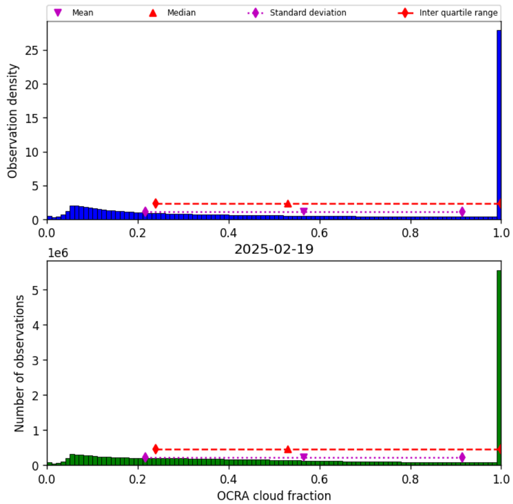
Figure 50: Histogram of “OCRA cloud fraction” for 2025-02-19 to 2025-02-20
