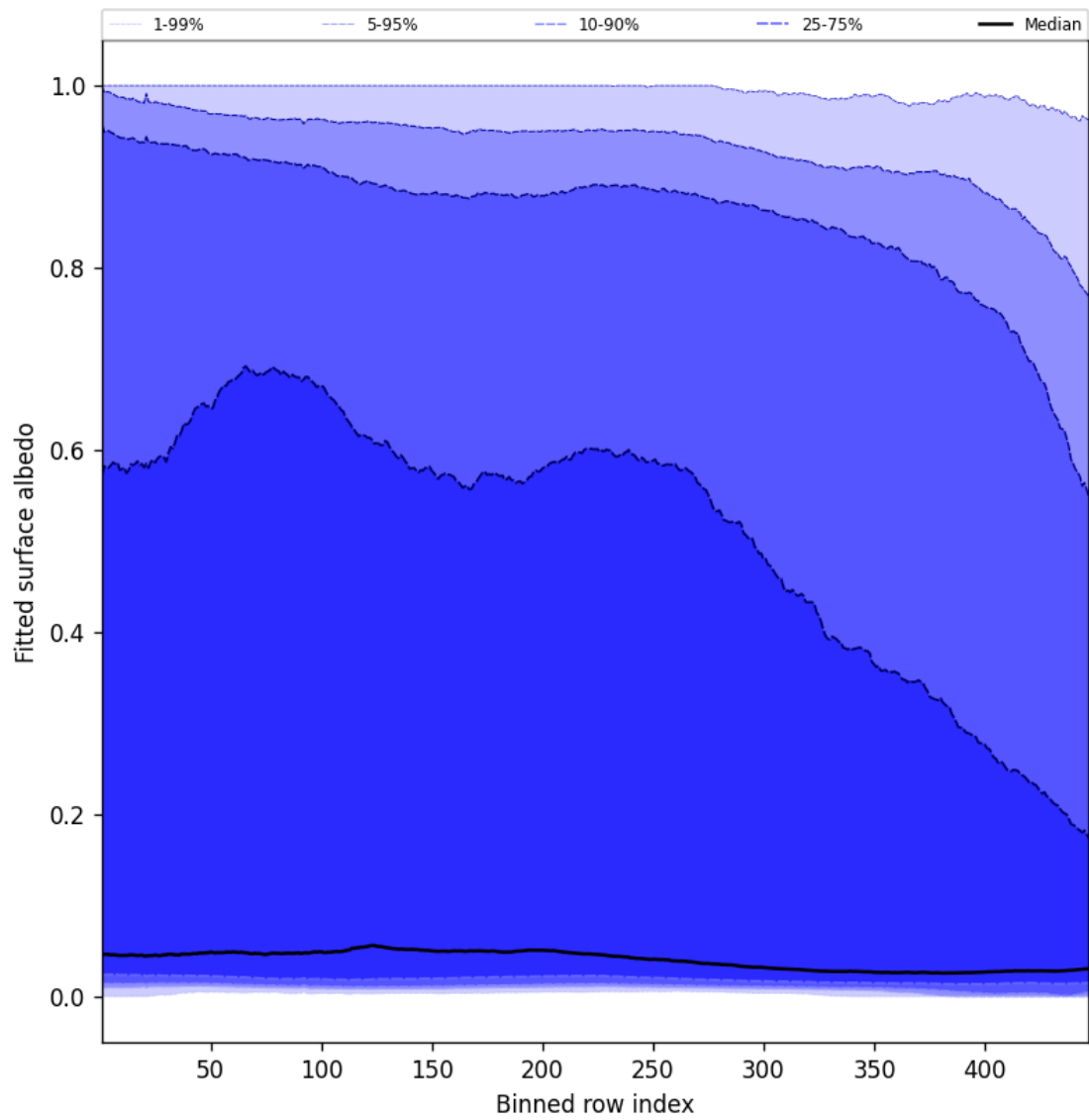
Figure 61: Along track statistics of “Fitted surface albedo” for 2025-02-19 to 2025-02-20
