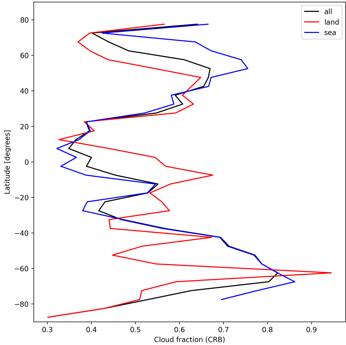
Figure 26: Zonal average of “Cloud fraction (CRB)” for 2025-02-19 to 2025-02-20.
