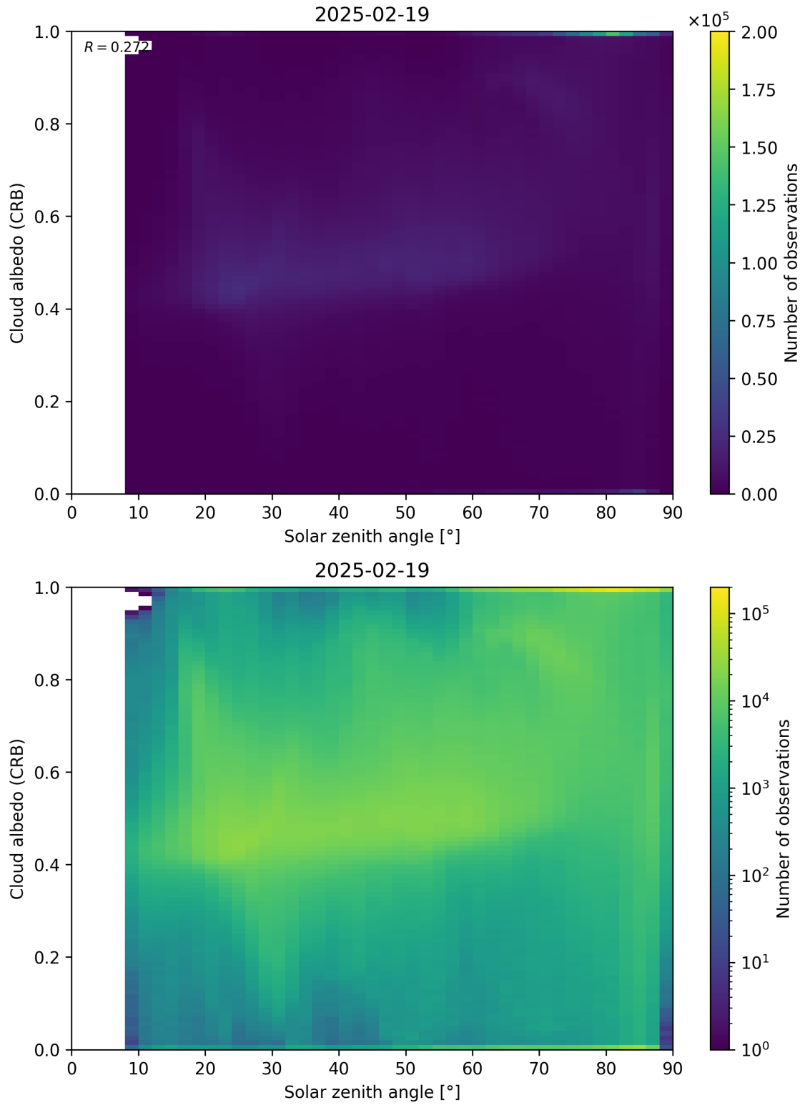
Figure 98: Scatter density plot of “Solar zenith angle” against “Cloud albedo (CRB)” for 2025-02-19 to 2025-02-20.
