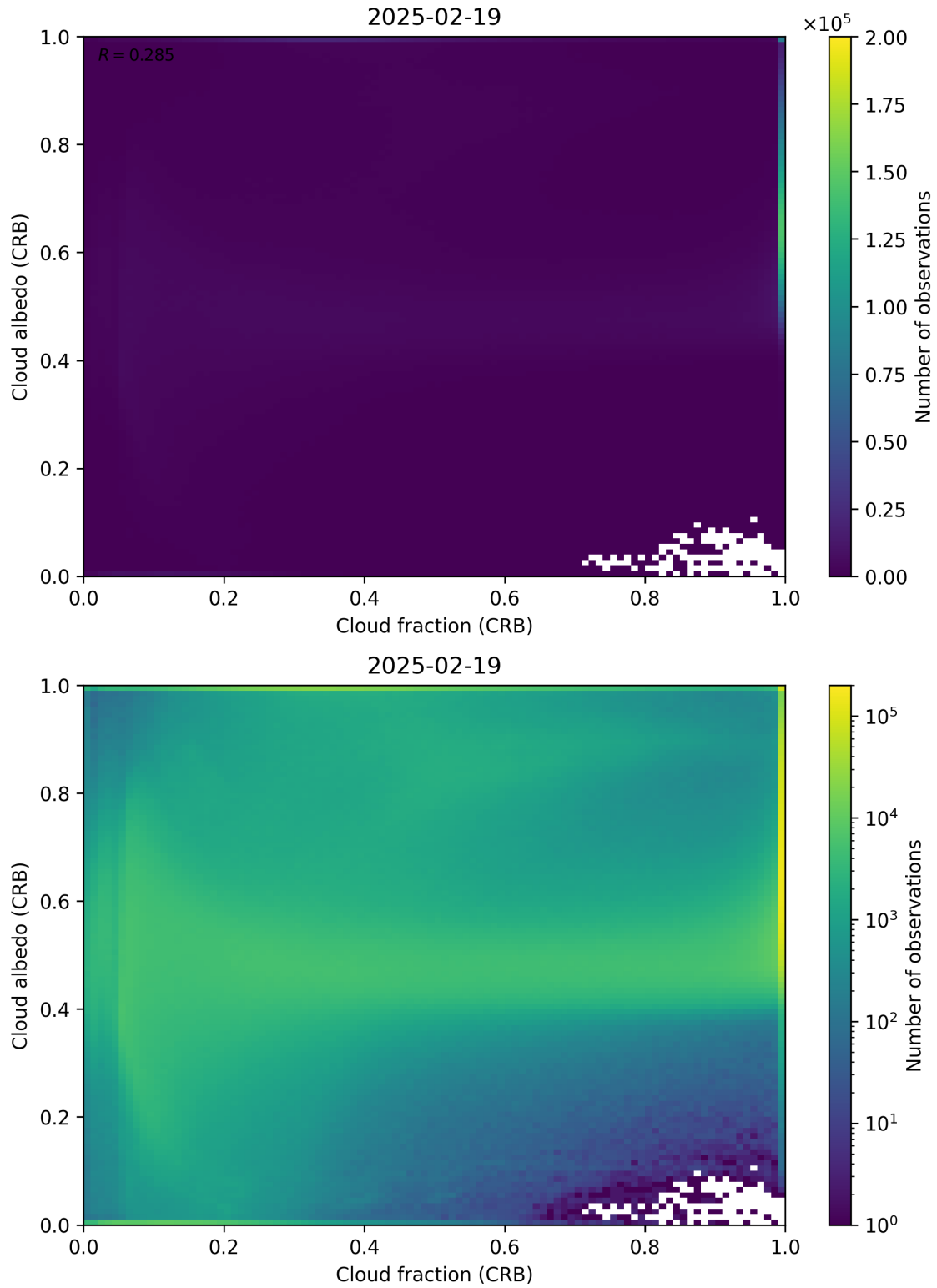
Figure 77: Scatter density plot of “Cloud fraction (CRB)” against “Cloud albedo (CRB)” for 2025-02-19 to 2025-02-20.
