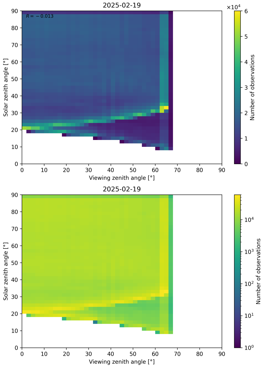
Figure 114: Scatter density plot of “Viewing zenith angle” against “Solar zenith angle” for 2025-02-19 to 2025-02-20.
