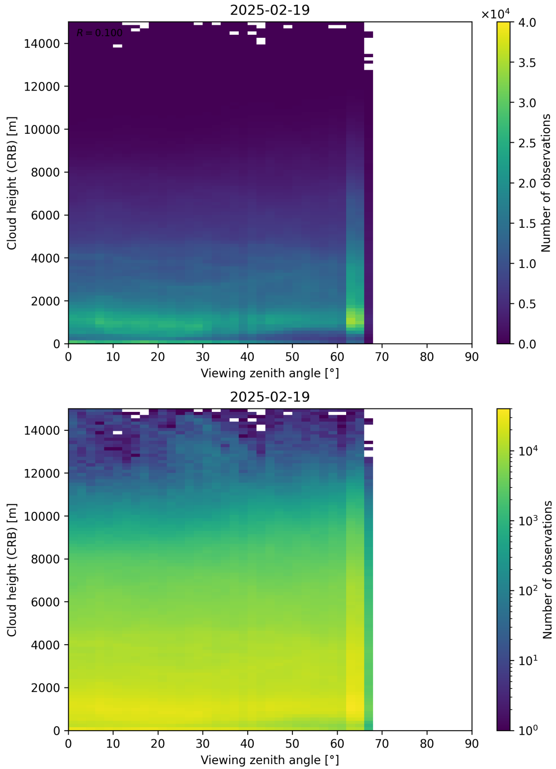
Figure 110: Scatter density plot of “Viewing zenith angle” against “Cloud height (CRB)” for 2025-02-19 to 2025-02-20.
