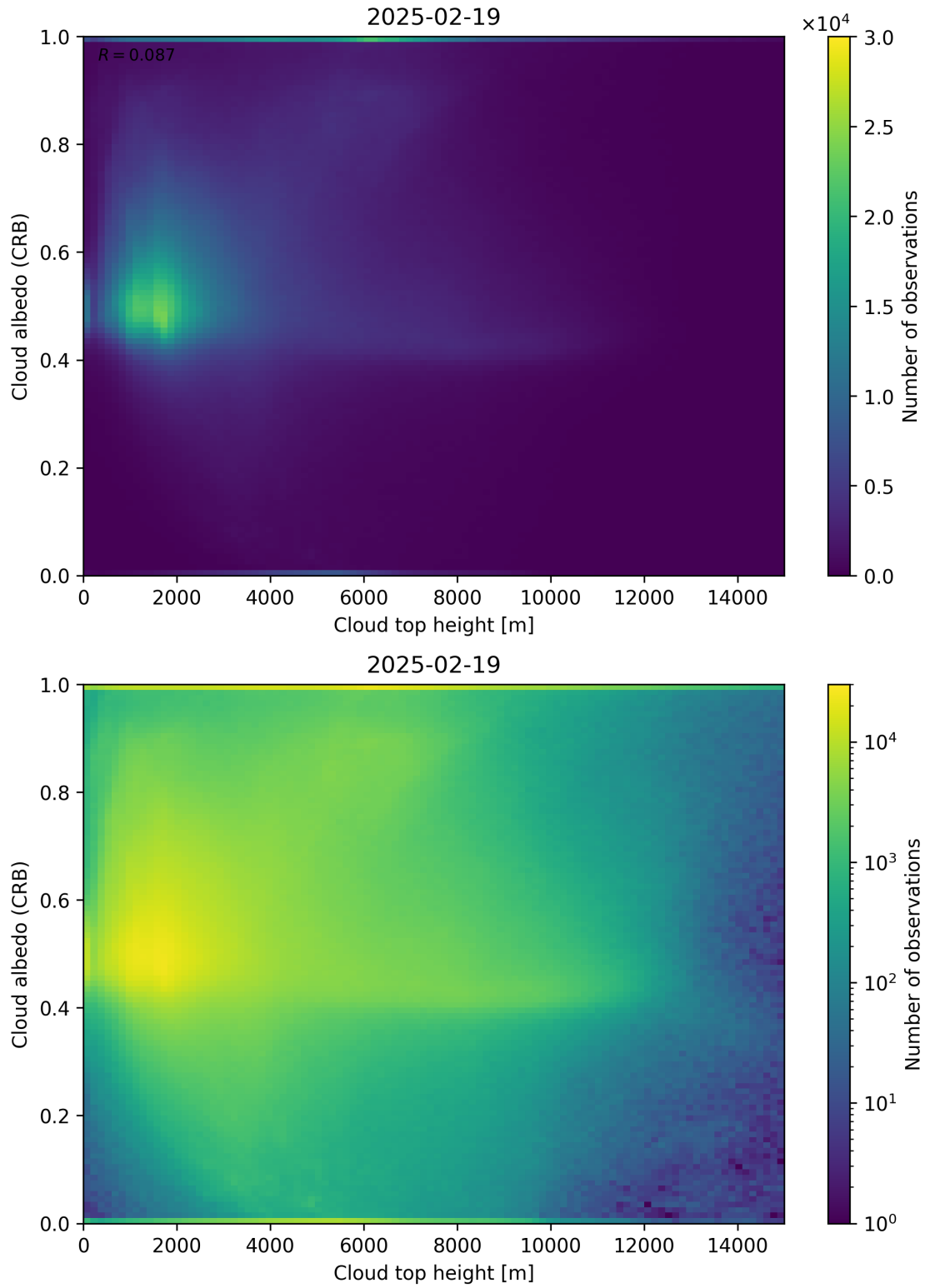
Figure 86: Scatter density plot of “Cloud top height” against “Cloud albedo (CRB)” for 2025-02-19 to 2025-02-20.
