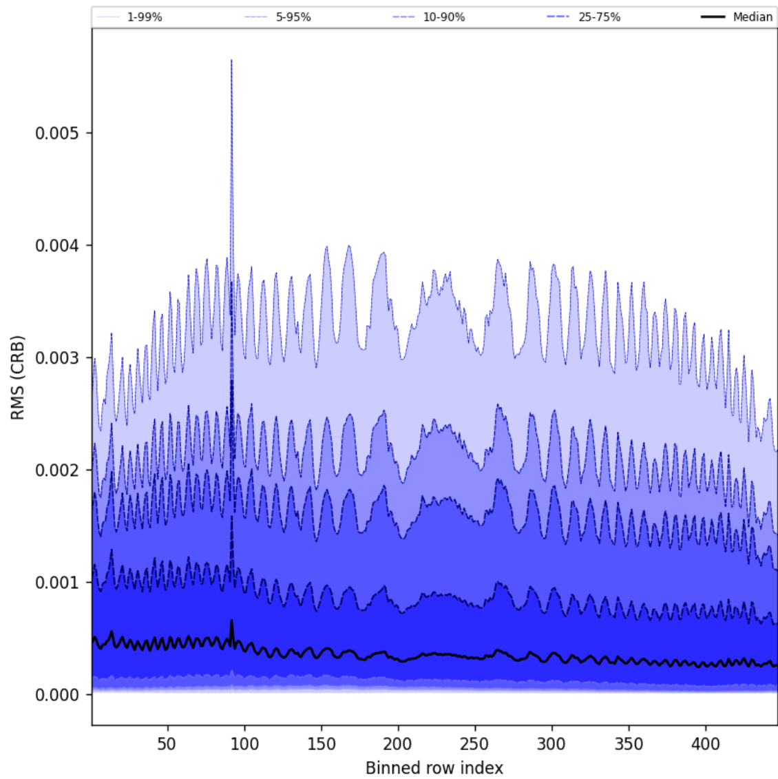
Figure 64: Along track statistics of “RMS (CRB)” for 2025-02-19 to 2025-02-20
