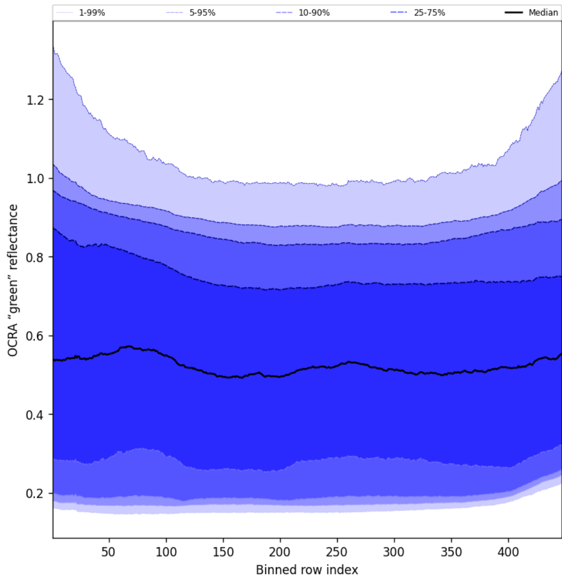
Figure 68: Along track statistics of “OCRA “green” reflectance” for 2025-02-19 to 2025-02-20
