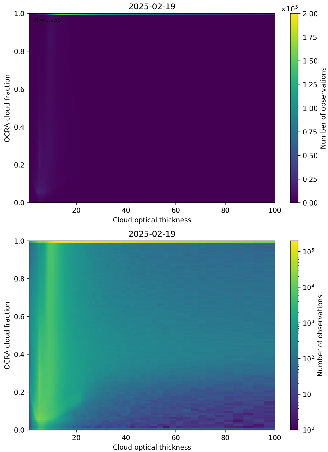
Figure 83: Scatter density plot of “Cloud optical thickness” against “OCRA cloud fraction” for 2025-02-19 to 2025-02-20.
