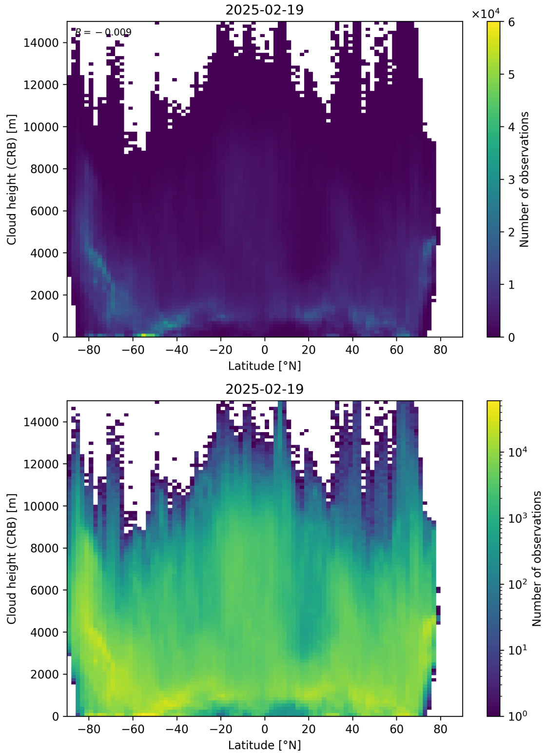
Figure 95: Scatter density plot of “Latitude” against “Cloud height (CRB)” for 2025-02-19 to 2025-02-20.
