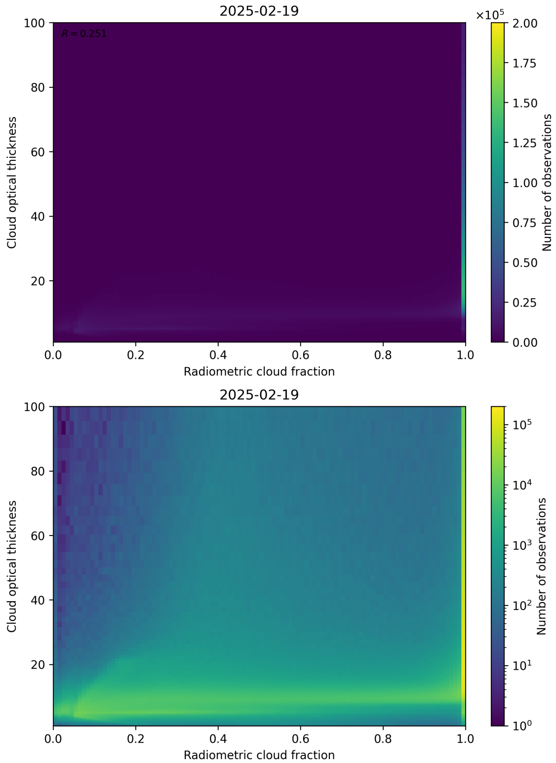
Figure 75: Scatter density plot of “Radiometric cloud fraction” against “Cloud optical thickness” for 2025-02-19 to 2025-02-20.
