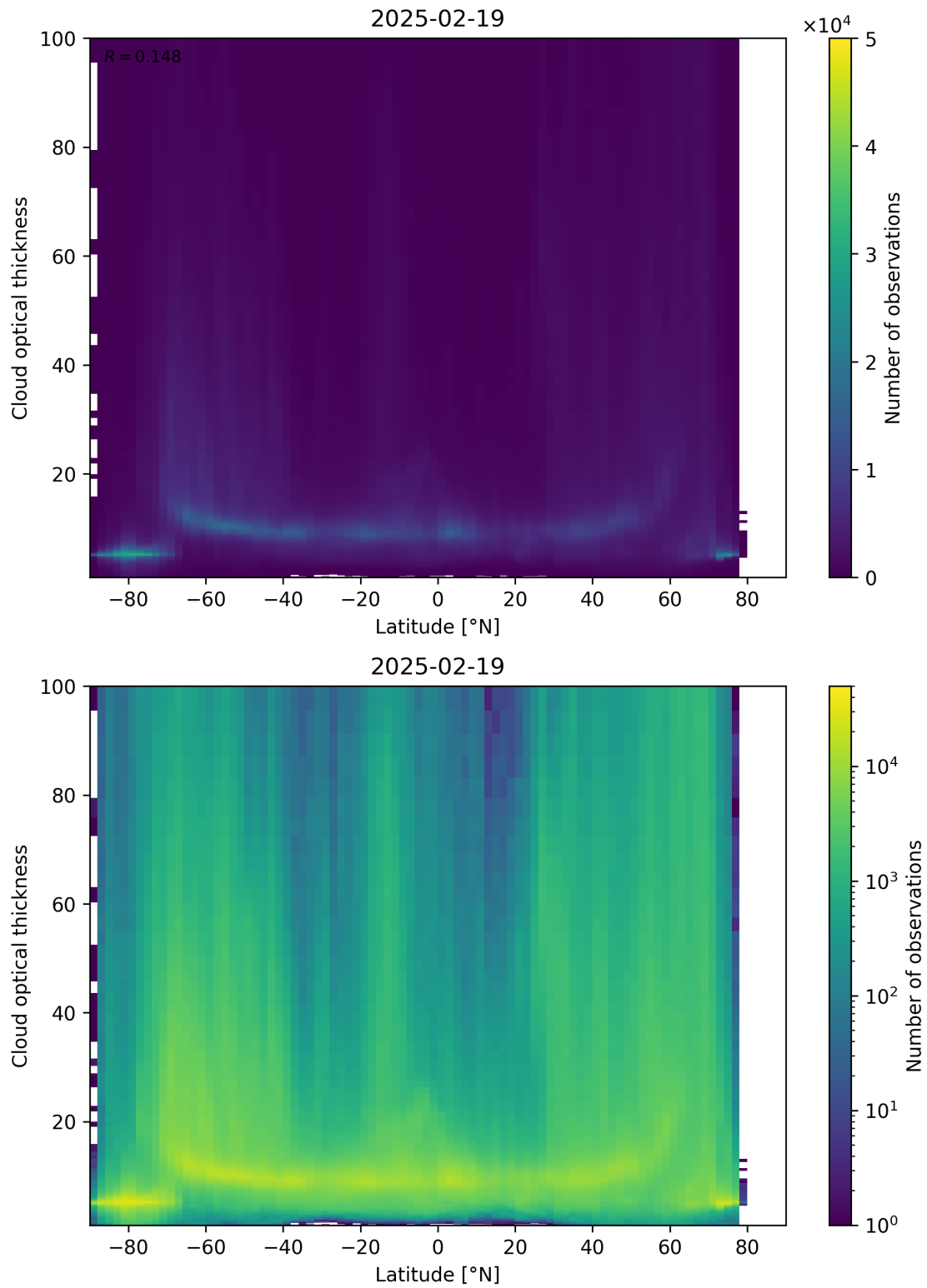
Figure 96: Scatter density plot of “Latitude” against “Cloud optical thickness” for 2025-02-19 to 2025-02-20.
