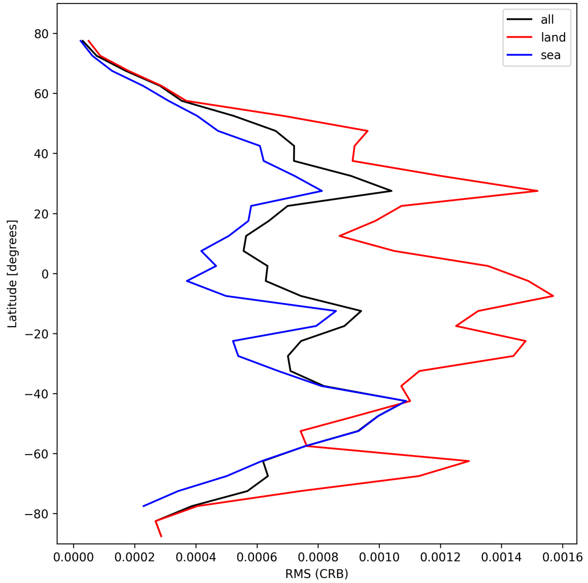
Figure 32: Zonal average of “RMS (CRB)” for 2025-02-19 to 2025-02-20.
