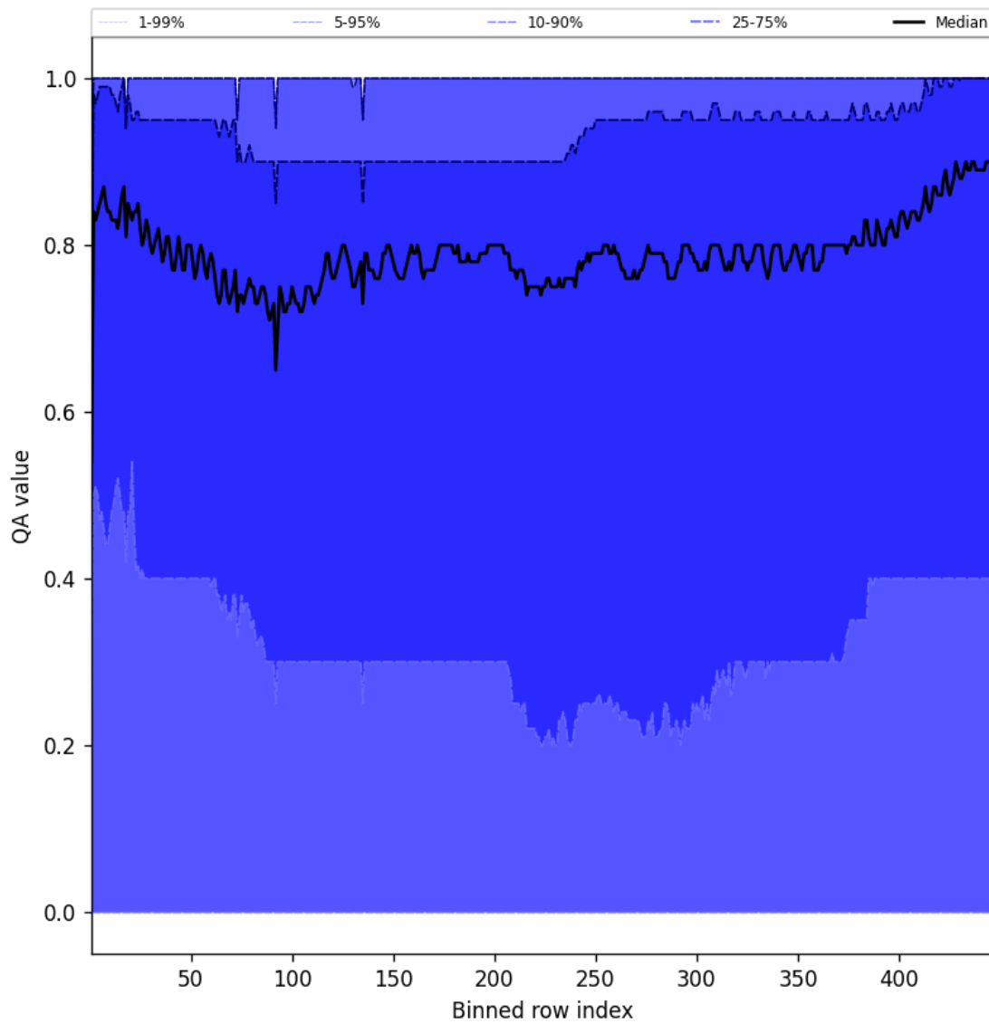
Figure 54: Along track statistics of “QA value” for 2025-02-19 to 2025-02-20
