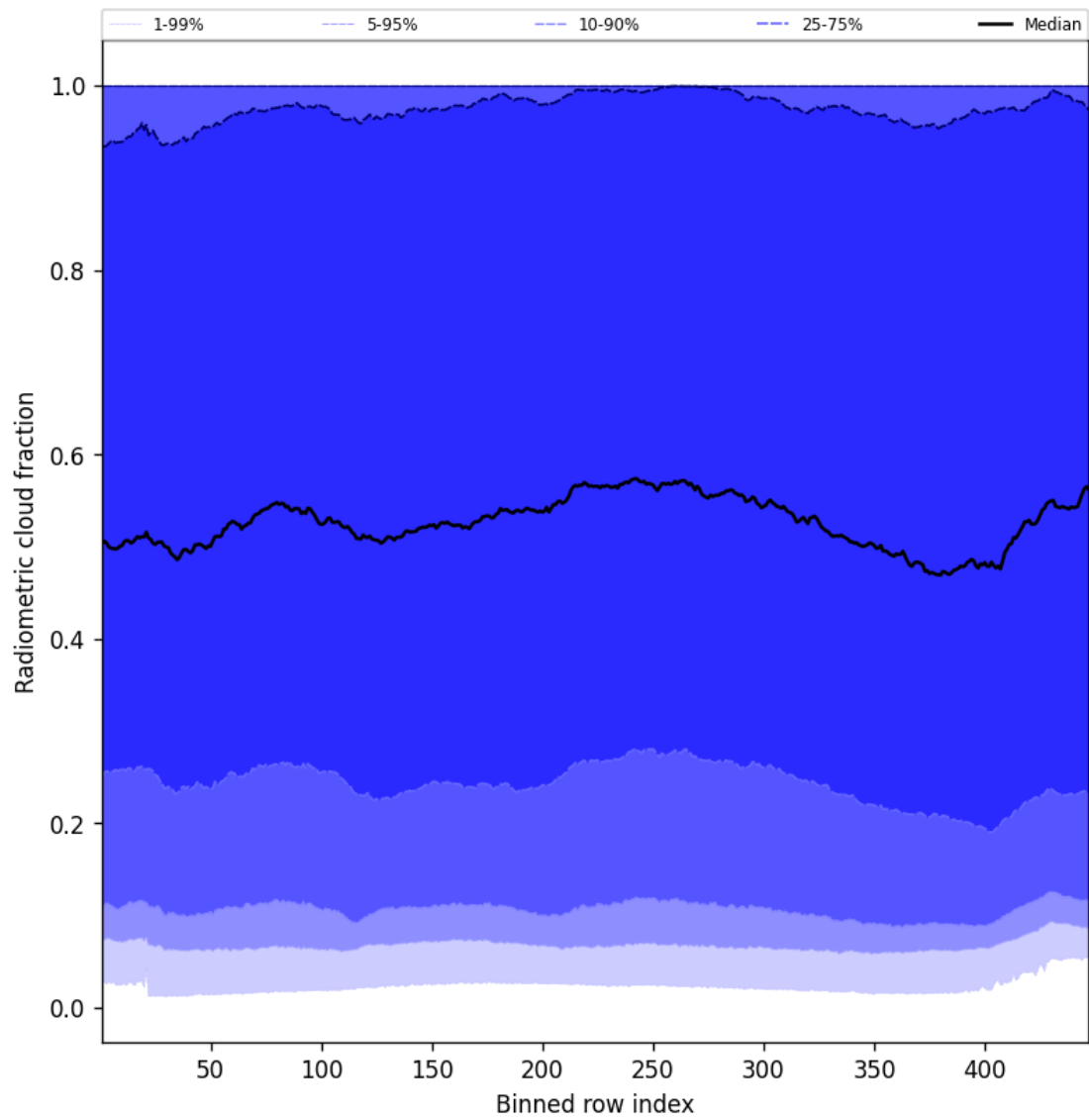
Figure 55: Along track statistics of “Radiometric cloud fraction” for 2025-02-19 to 2025-02-20
