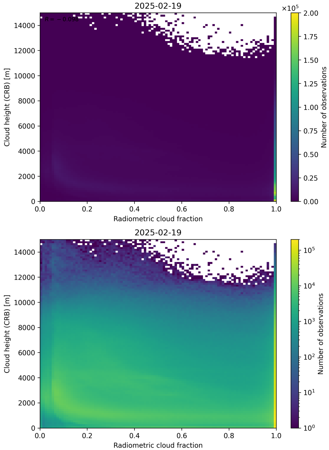
Figure 74: Scatter density plot of “Radiometric cloud fraction” against “Cloud height (CRB)” for 2025-02-19 to 2025-02-20.
