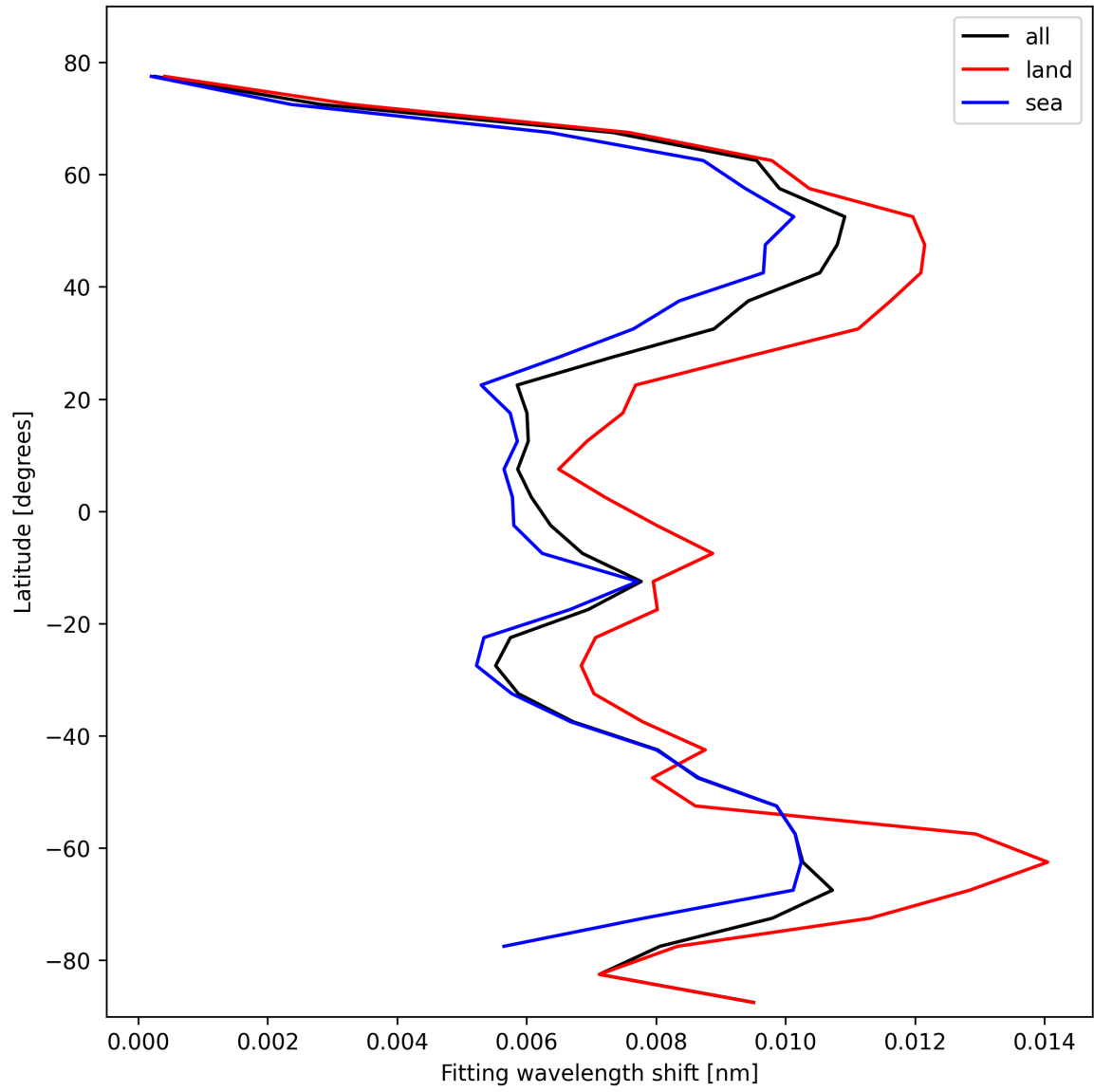
Figure 33: Zonal average of “Fitting wavelength shift” for 2025-02-19 to 2025-02-20.
