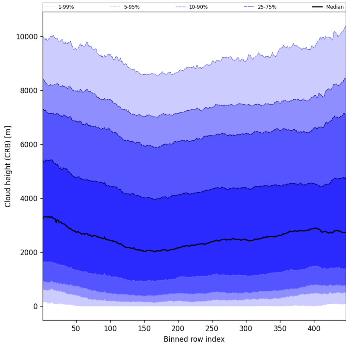
Figure 59: Along track statistics of “Cloud height (CRB)” for 2025-02-19 to 2025-02-20
