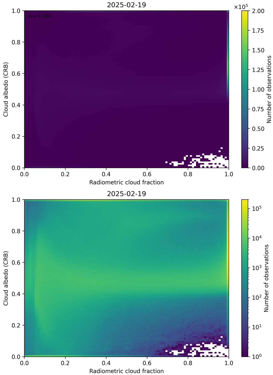
Figure 71: Scatter density plot of “Radiometric cloud fraction” against “Cloud albedo (CRB)” for 2025-02-19 to 2025-02-20.
