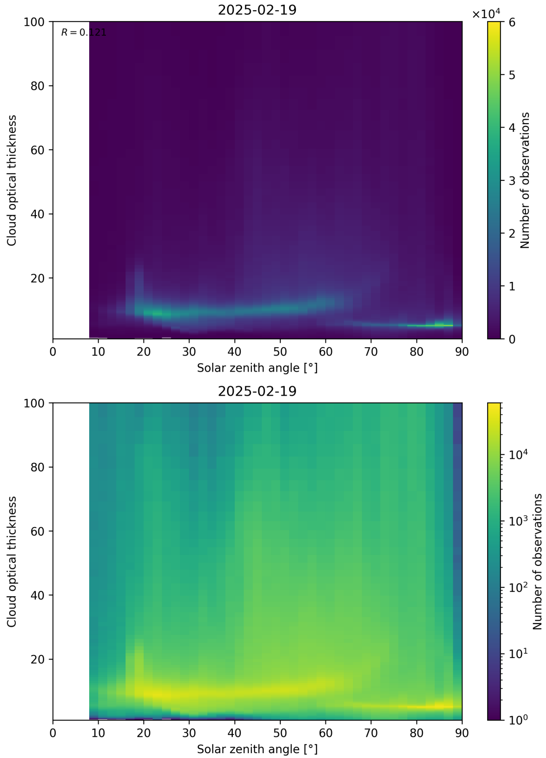
Figure 103: Scatter density plot of “Solar zenith angle” against “Cloud optical thickness” for 2025-02-19 to 2025-02-20.
