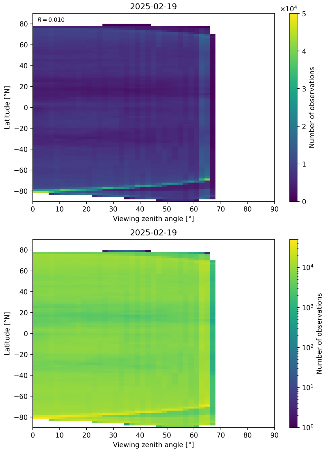
Figure 113: Scatter density plot of “Viewing zenith angle” against “Latitude” for 2025-02-19 to 2025-02-20.
