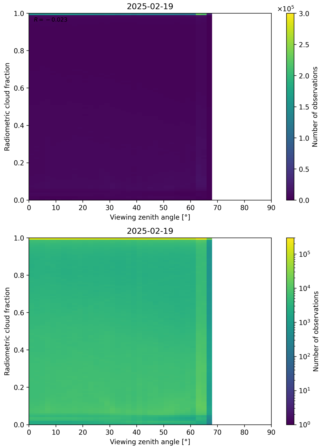
Figure 107: Scatter density plot of “Viewing zenith angle” against “Radiometric cloud fraction” for 2025-02-19 to 2025-02-20.
