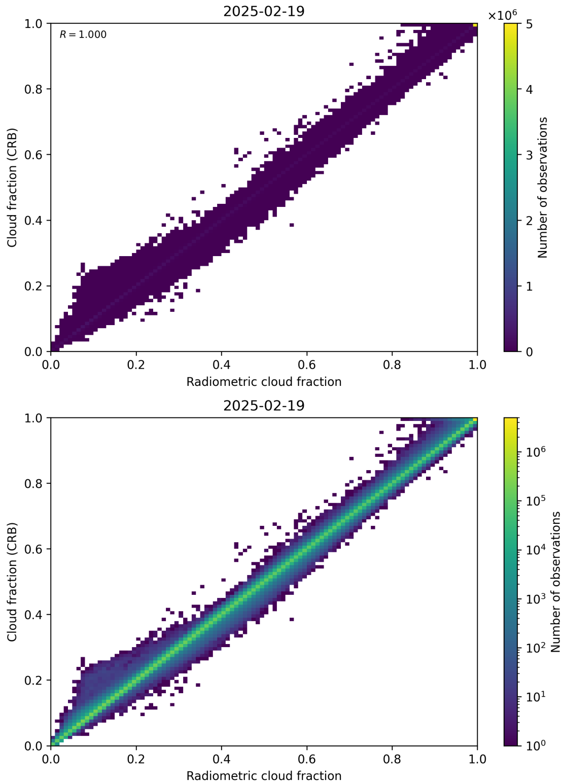
Figure 73: Scatter density plot of “Radiometric cloud fraction” against “Cloud fraction (CRB)” for 2025-02-19 to 2025-02-20.
