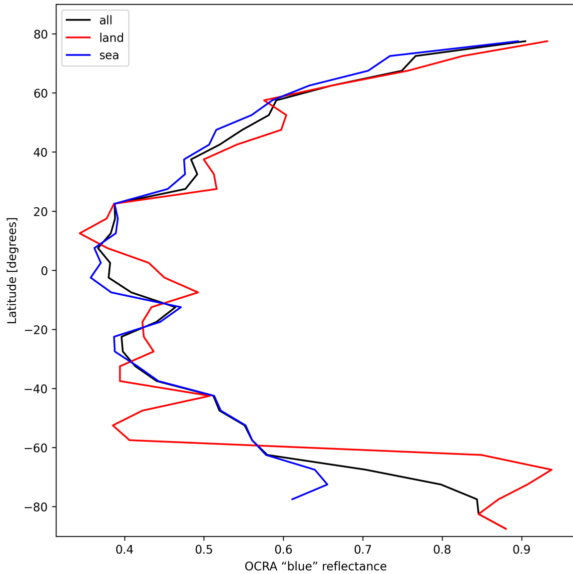
Figure 35: Zonal average of “OCRA “blue” reflectance” for 2025-02-19 to 2025-02-20.
