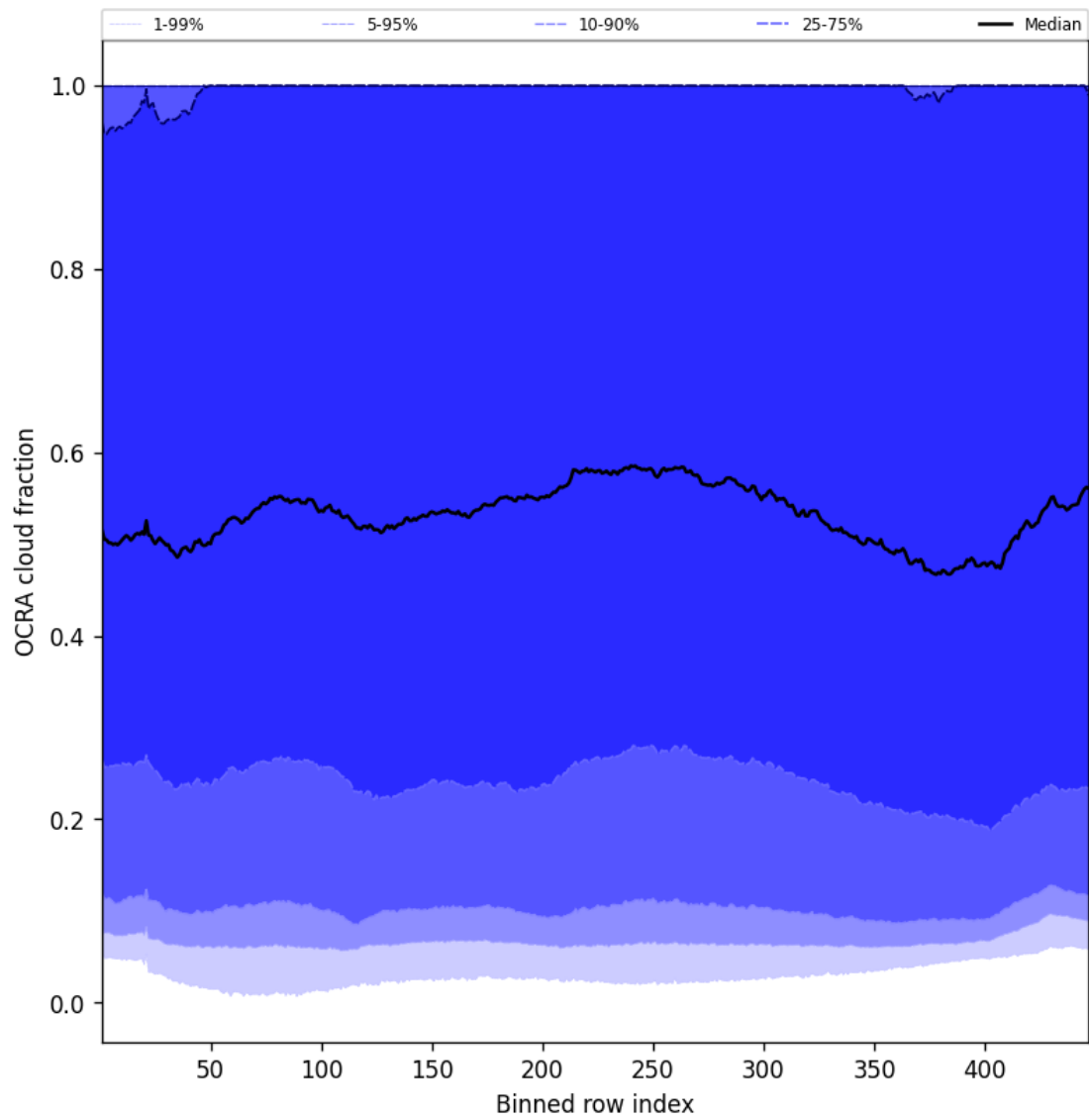
Figure 66: Along track statistics of “OCRA cloud fraction” for 2025-02-19 to 2025-02-20
