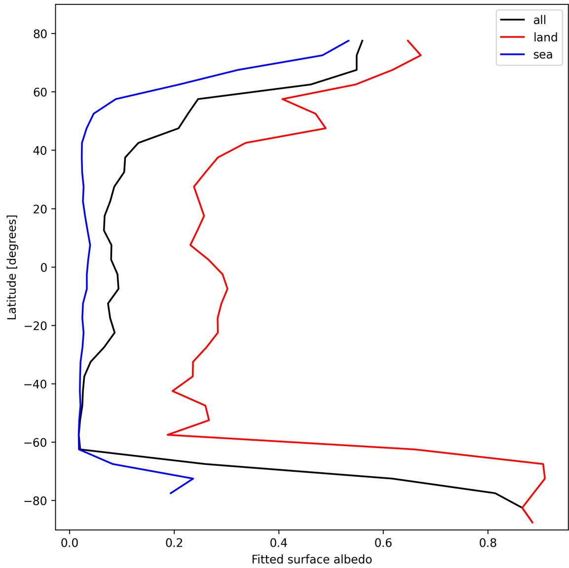
Figure 29: Zonal average of “Fitted surface albedo” for 2025-02-19 to 2025-02-20.
