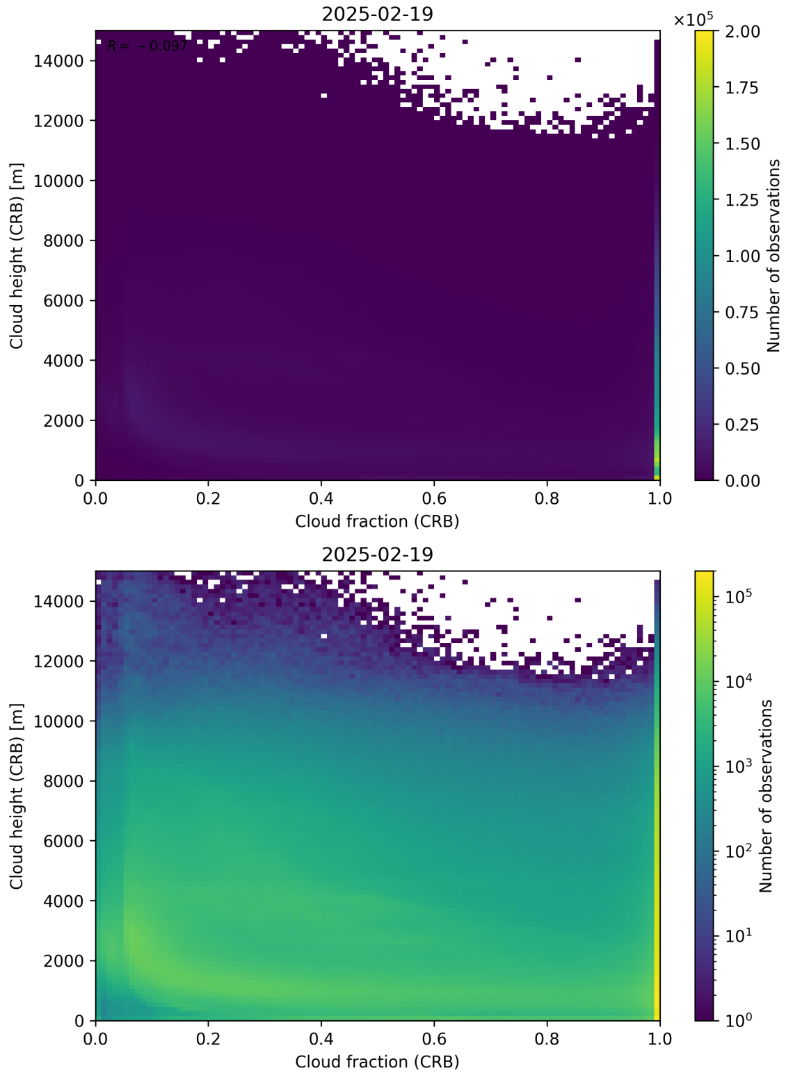
Figure 79: Scatter density plot of “Cloud fraction (CRB)” against “Cloud height (CRB)” for 2025-02-19 to 2025-02-20.
