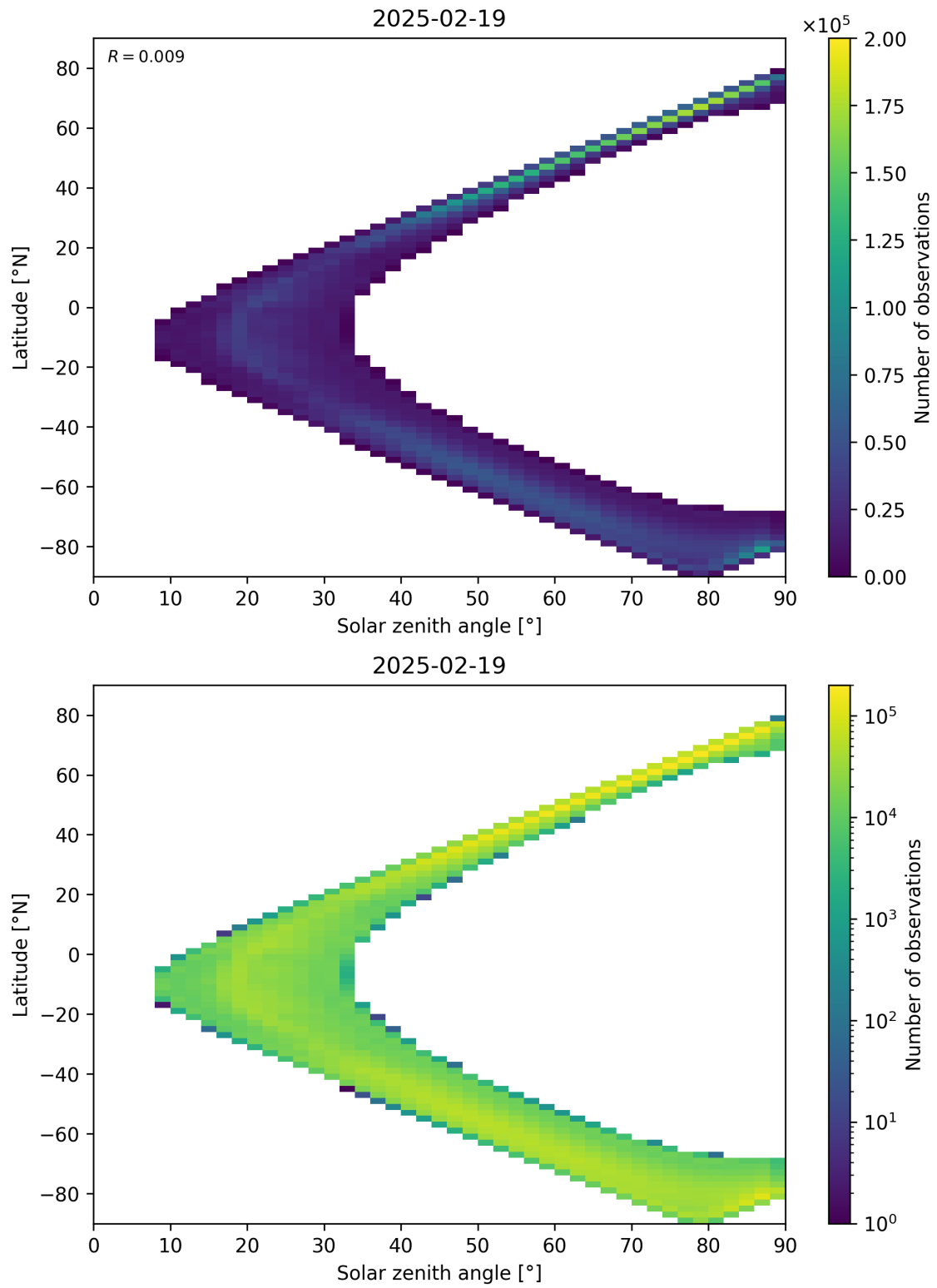
Figure 105: Scatter density plot of “Solar zenith angle” against “Latitude” for 2025-02-19 to 2025-02-20.
