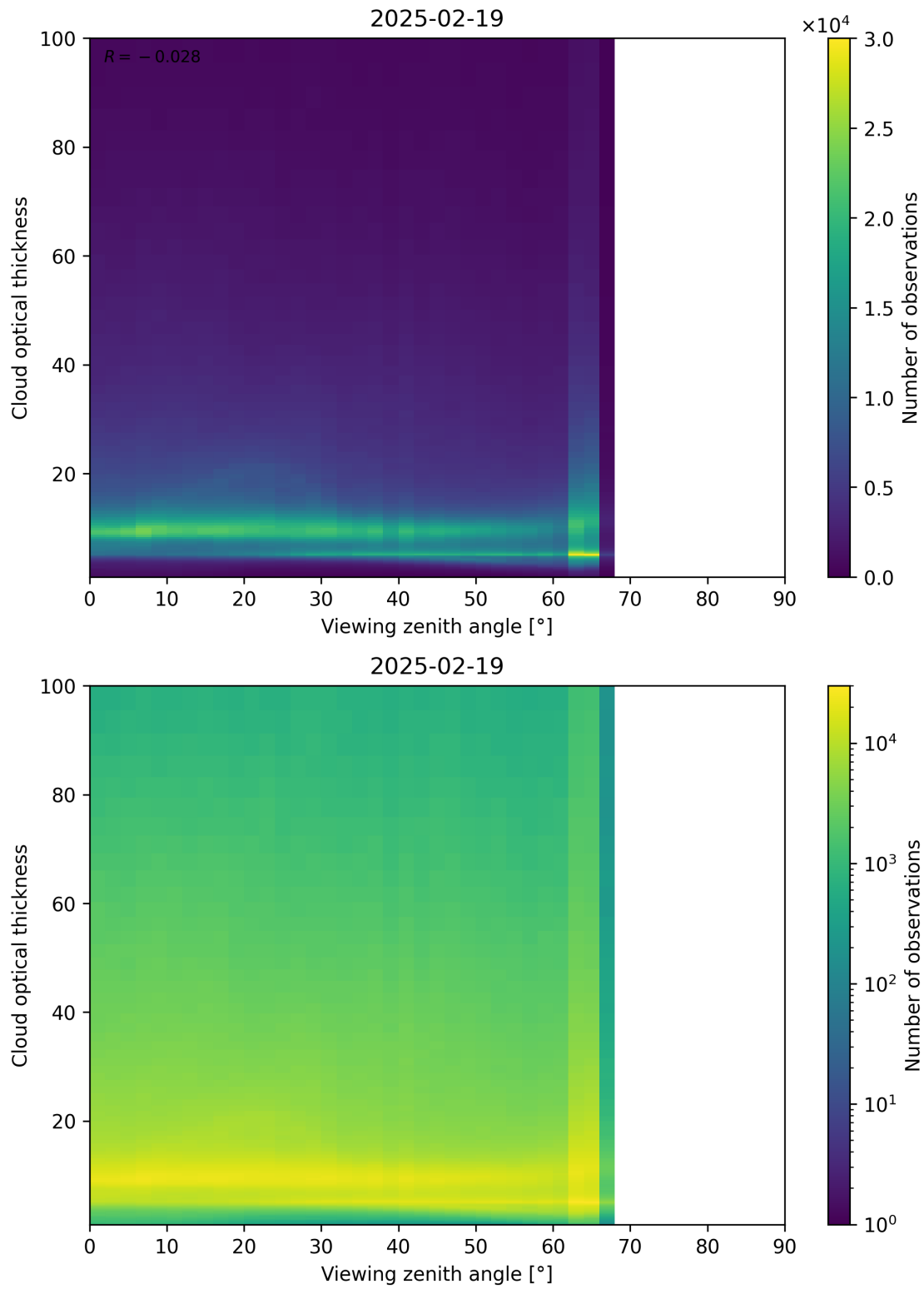
Figure 111: Scatter density plot of “Viewing zenith angle” against “Cloud optical thickness” for 2025-02-19 to 2025-02-20.
