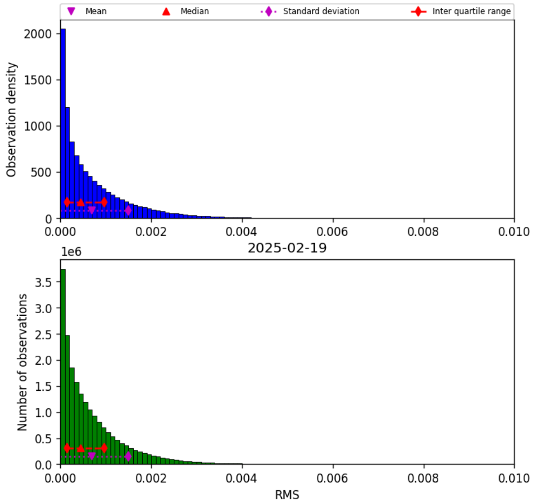
Figure 47: Histogram of “RMS” for 2025-02-19 to 2025-02-20
