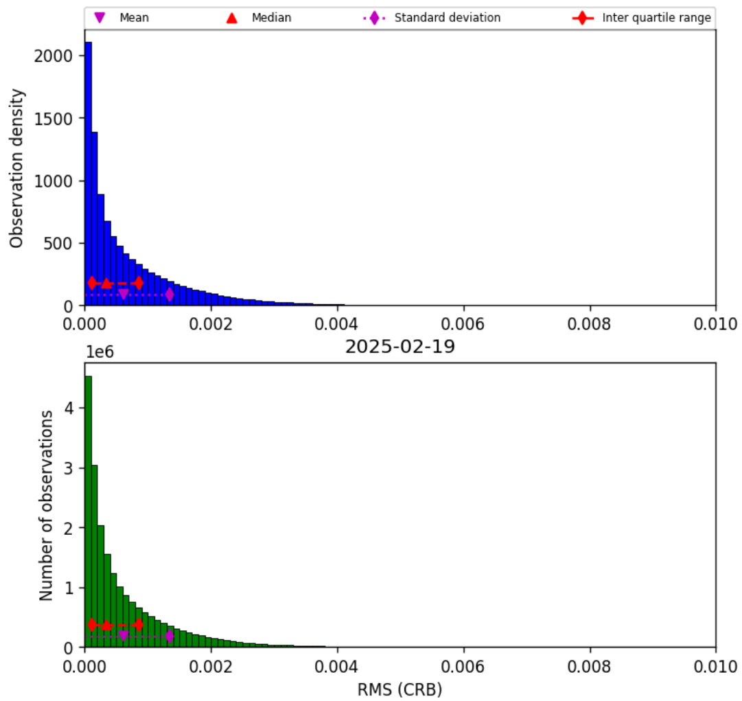
Figure 48: Histogram of “RMS (CRB)” for 2025-02-19 to 2025-02-20
