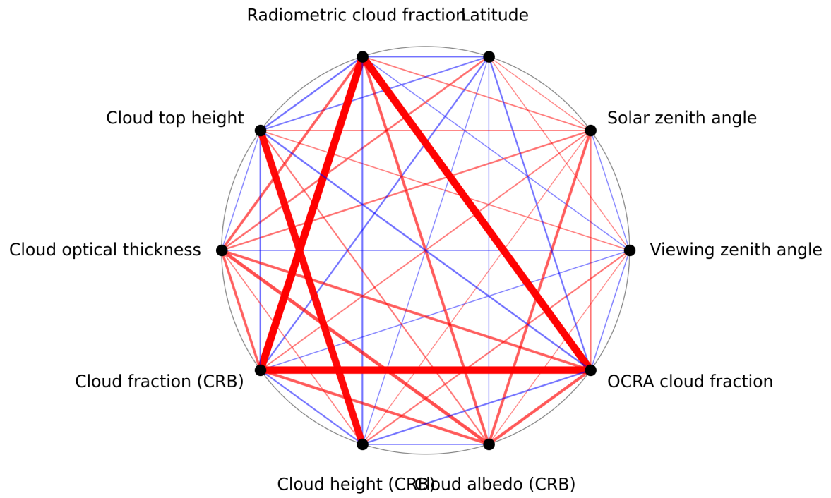
Figure 1: Map of correlation graph for 2025-02-19 to 2025-02-20.
