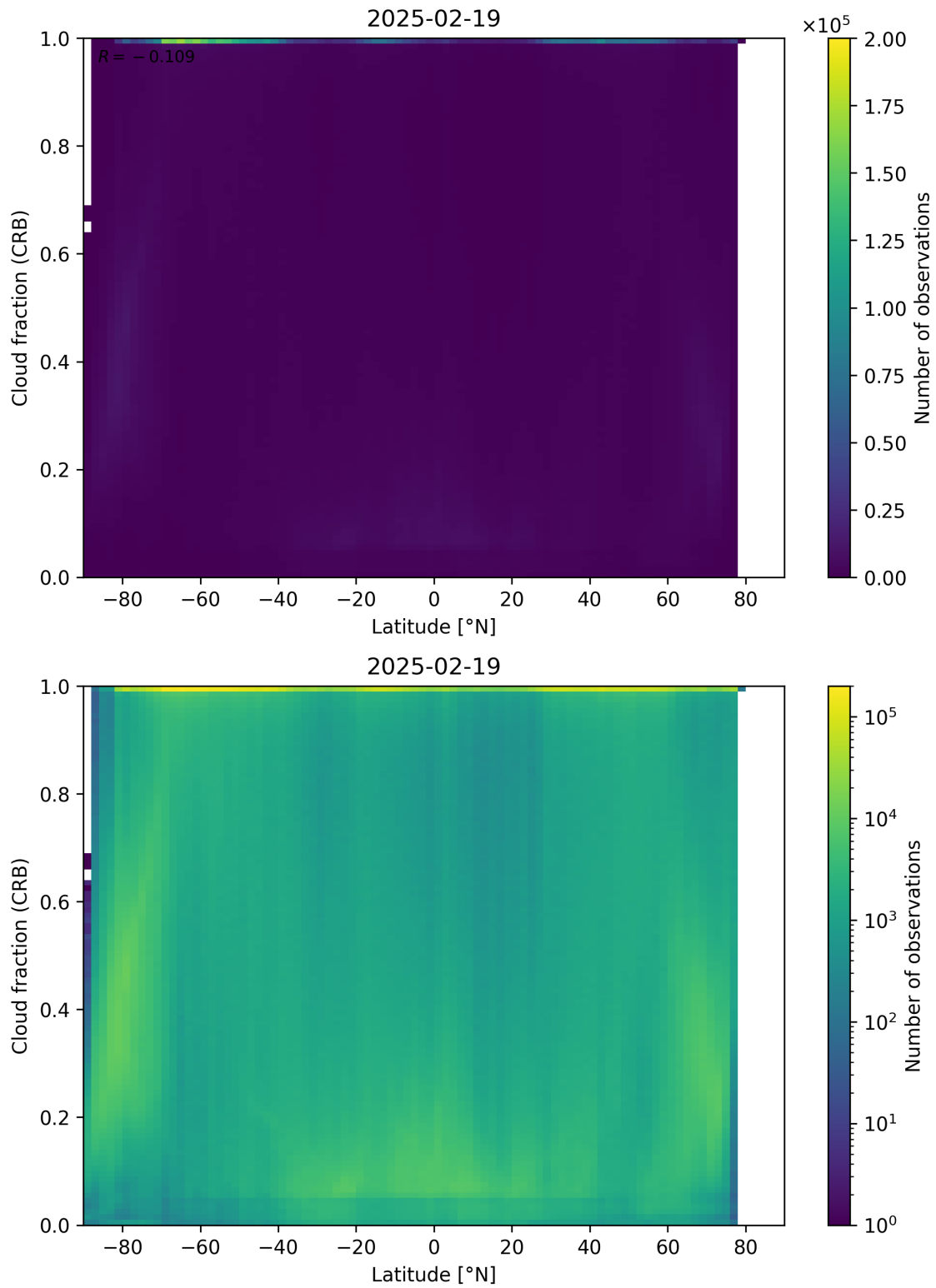
Figure 94: Scatter density plot of “Latitude” against “Cloud fraction (CRB)” for 2025-02-19 to 2025-02-20.
