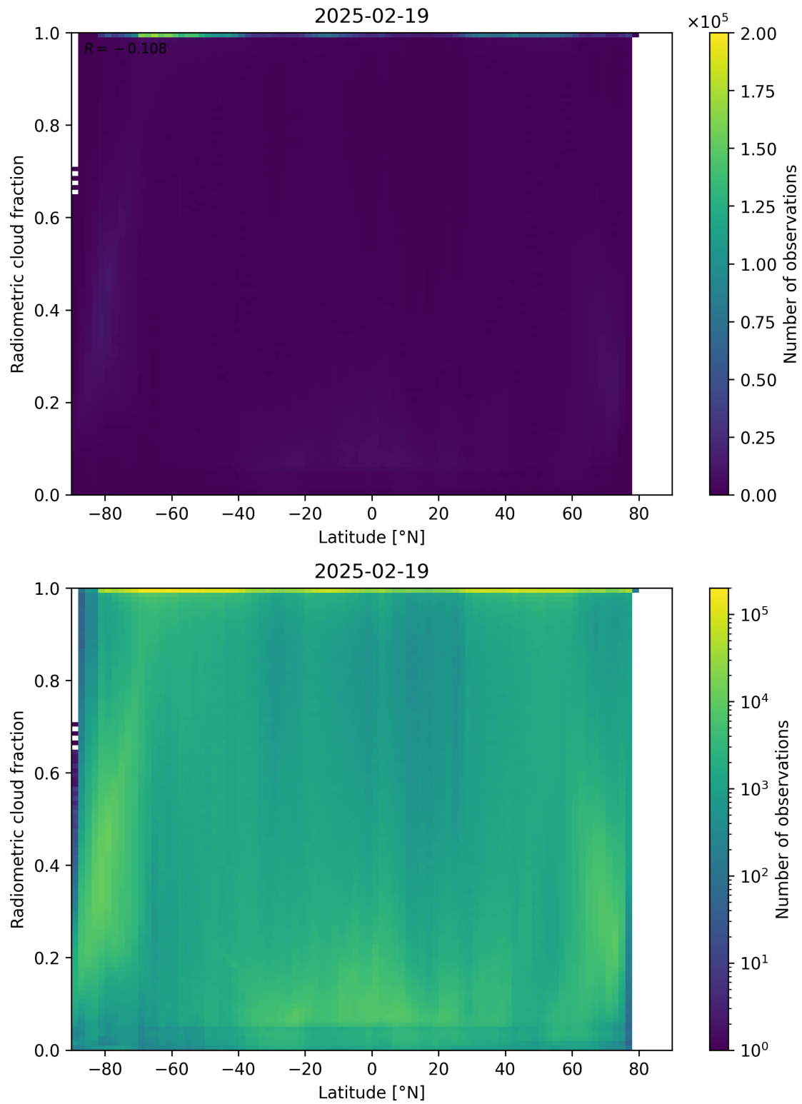
Figure 92: Scatter density plot of “Latitude” against “Radiometric cloud fraction” for 2025-02-19 to 2025-02-20.
