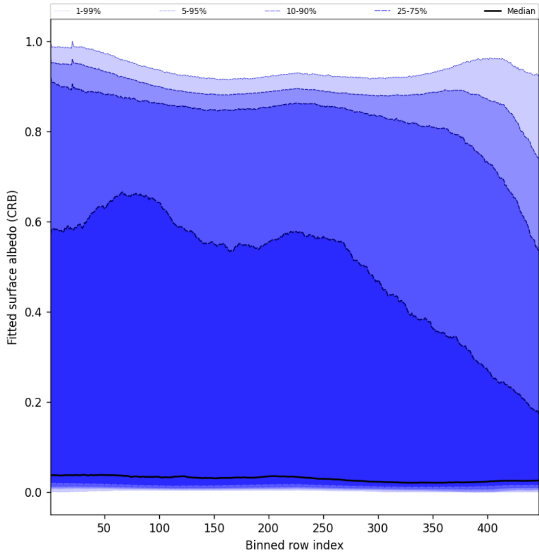
Figure 62: Along track statistics of “Fitted surface albedo (CRB)” for 2025-02-19 to 2025-02-20
