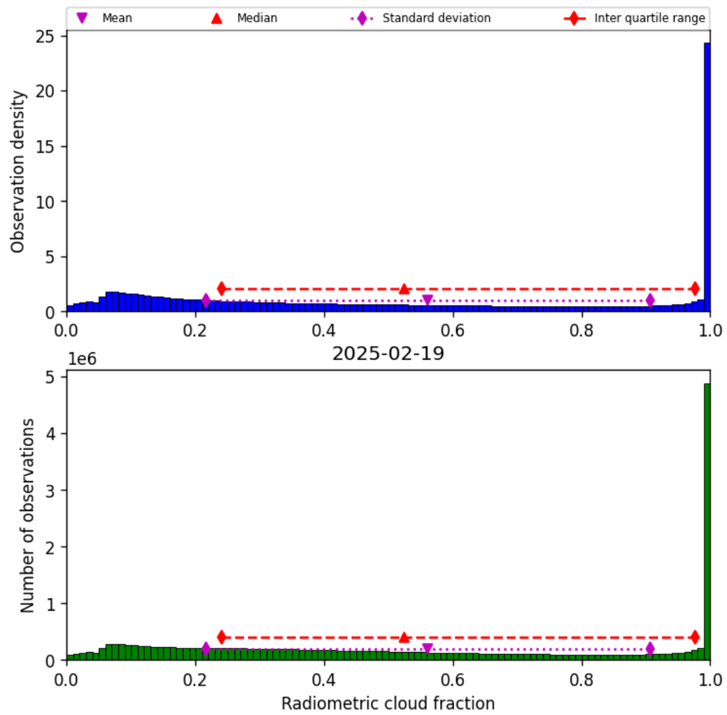
Figure 39: Histogram of “Radiometric cloud fraction” for 2025-02-19 to 2025-02-20
