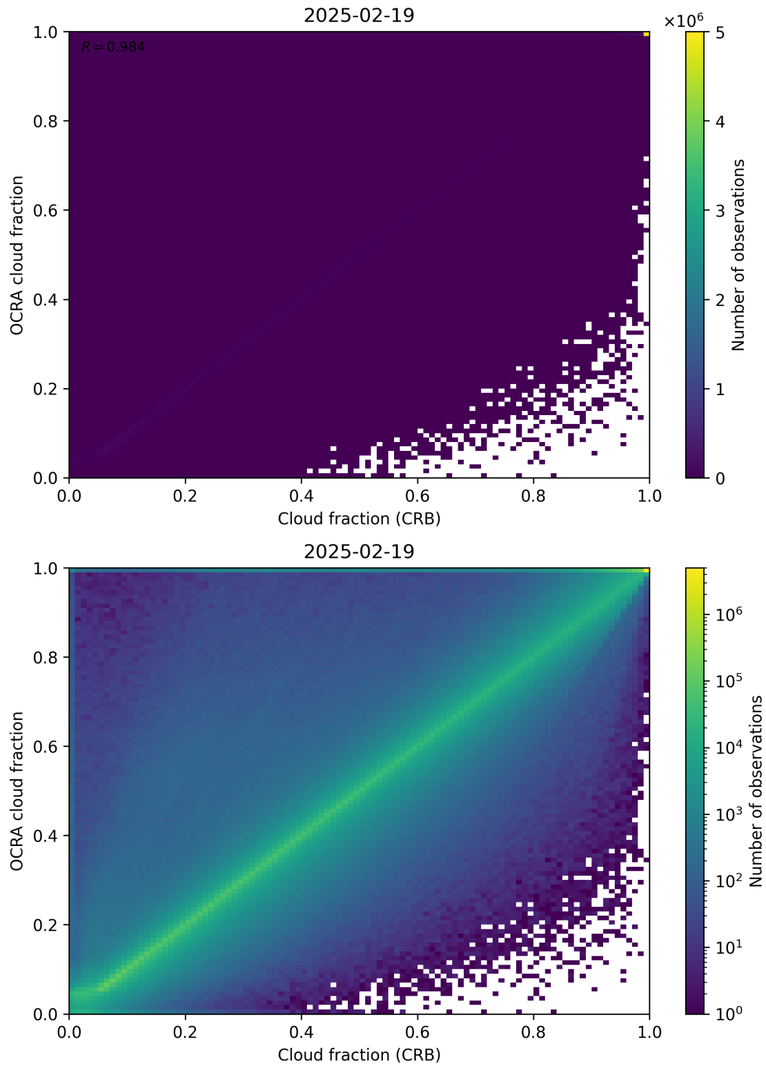
Figure 78: Scatter density plot of “Cloud fraction (CRB)” against “OCRA cloud fraction” for 2025-02-19 to 2025-02-20.
