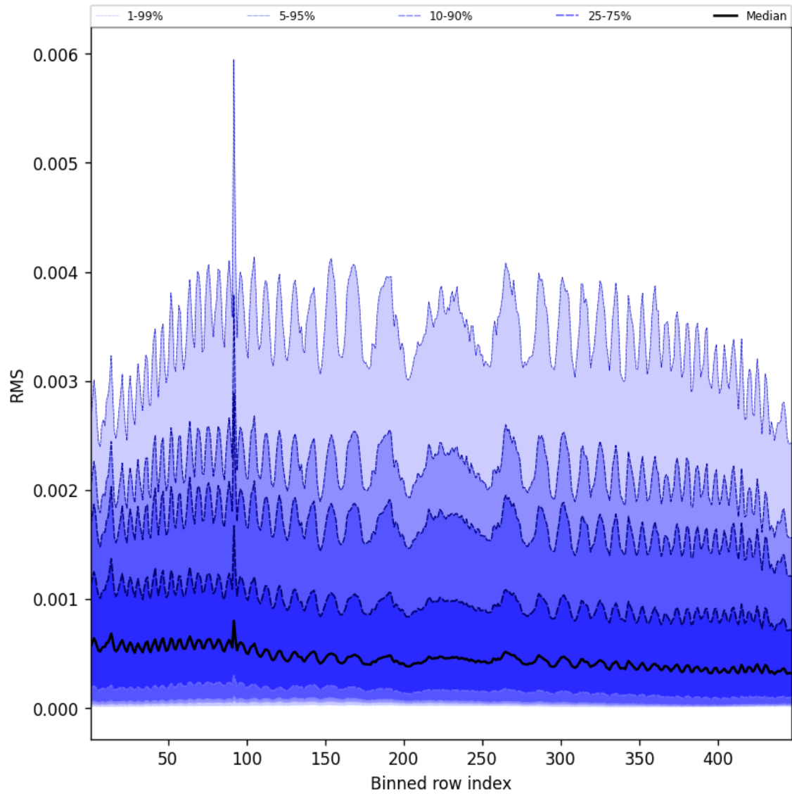
Figure 63: Along track statistics of “RMS” for 2025-02-19 to 2025-02-20
