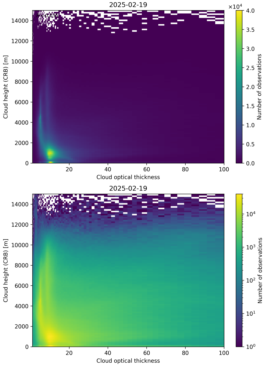
Figure 85: Scatter density plot of “Cloud optical thickness” against “Cloud height (CRB)” for 2025-02-19 to 2025-02-20.
