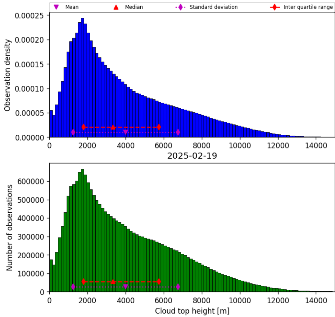
Figure 40: Histogram of “Cloud top height” for 2025-02-19 to 2025-02-20
