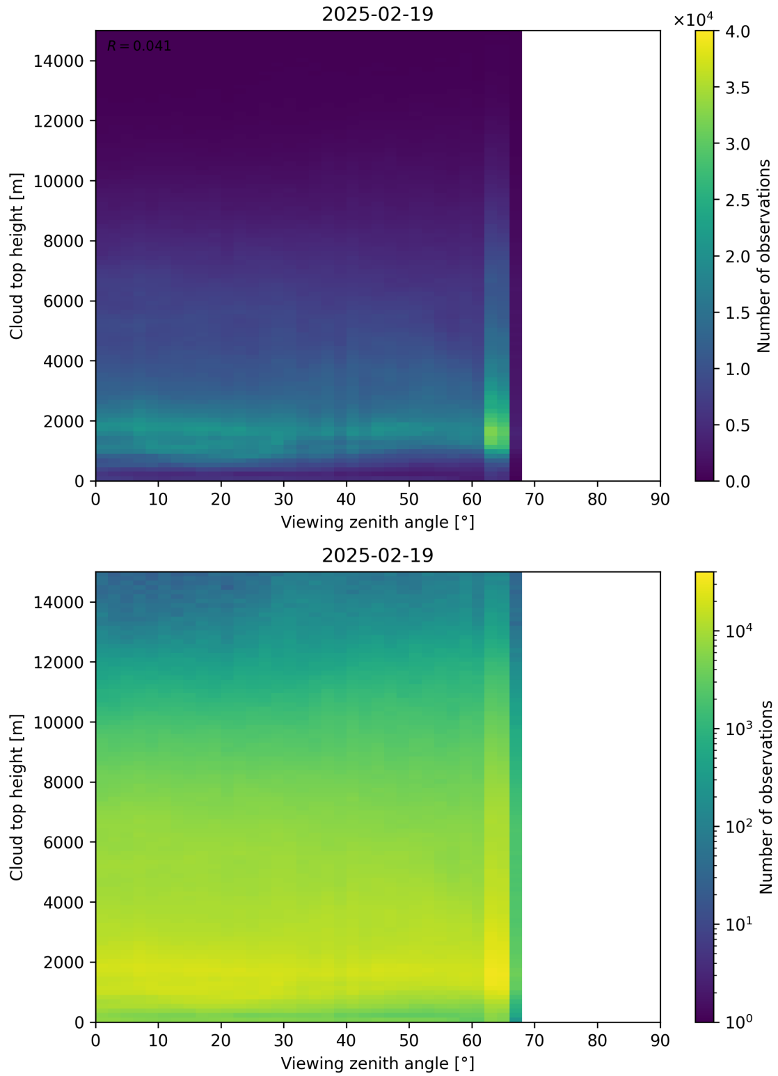
Figure 112: Scatter density plot of “Viewing zenith angle” against “Cloud top height” for 2025-02-19 to 2025-02-20.
