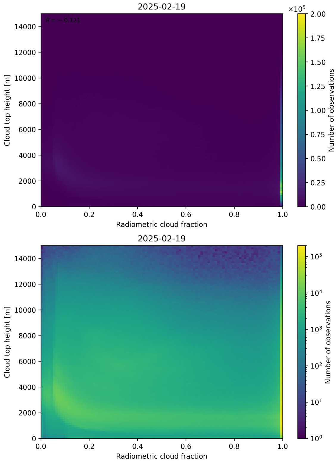
Figure 76: Scatter density plot of “Radiometric cloud fraction” against “Cloud top height” for 2025-02-19 to 2025-02-20.
