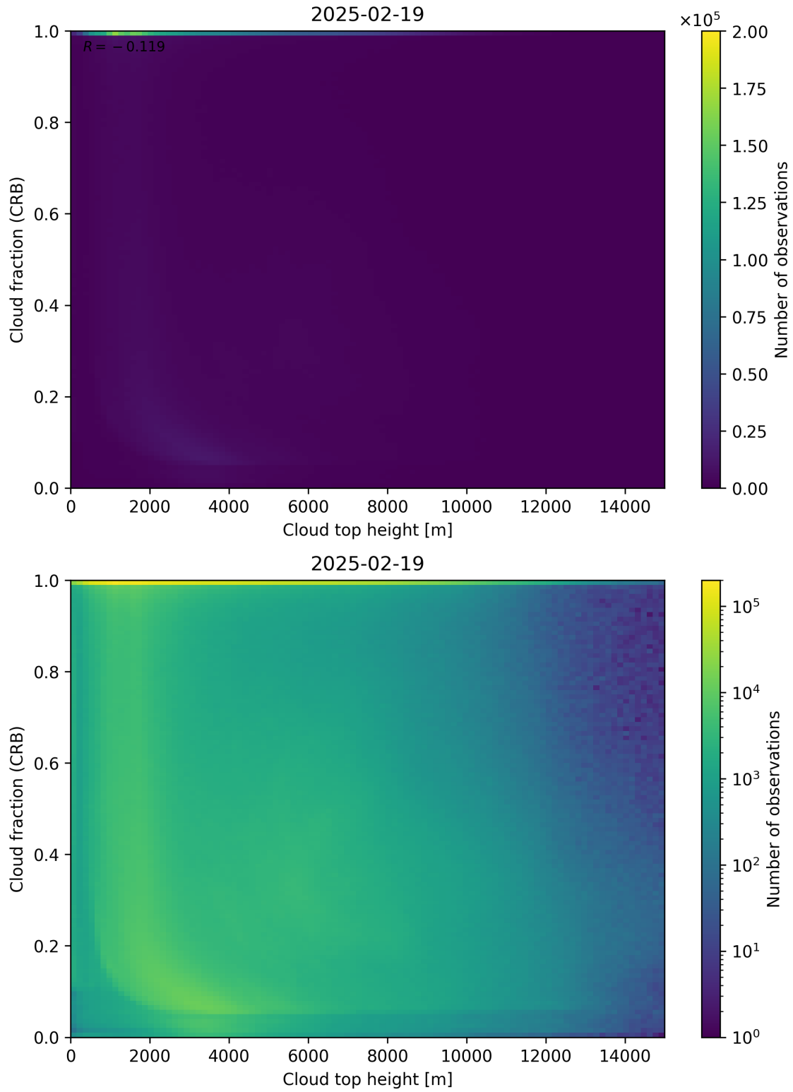
Figure 88: Scatter density plot of “Cloud top height” against “Cloud fraction (CRB)” for 2025-02-19 to 2025-02-20.
