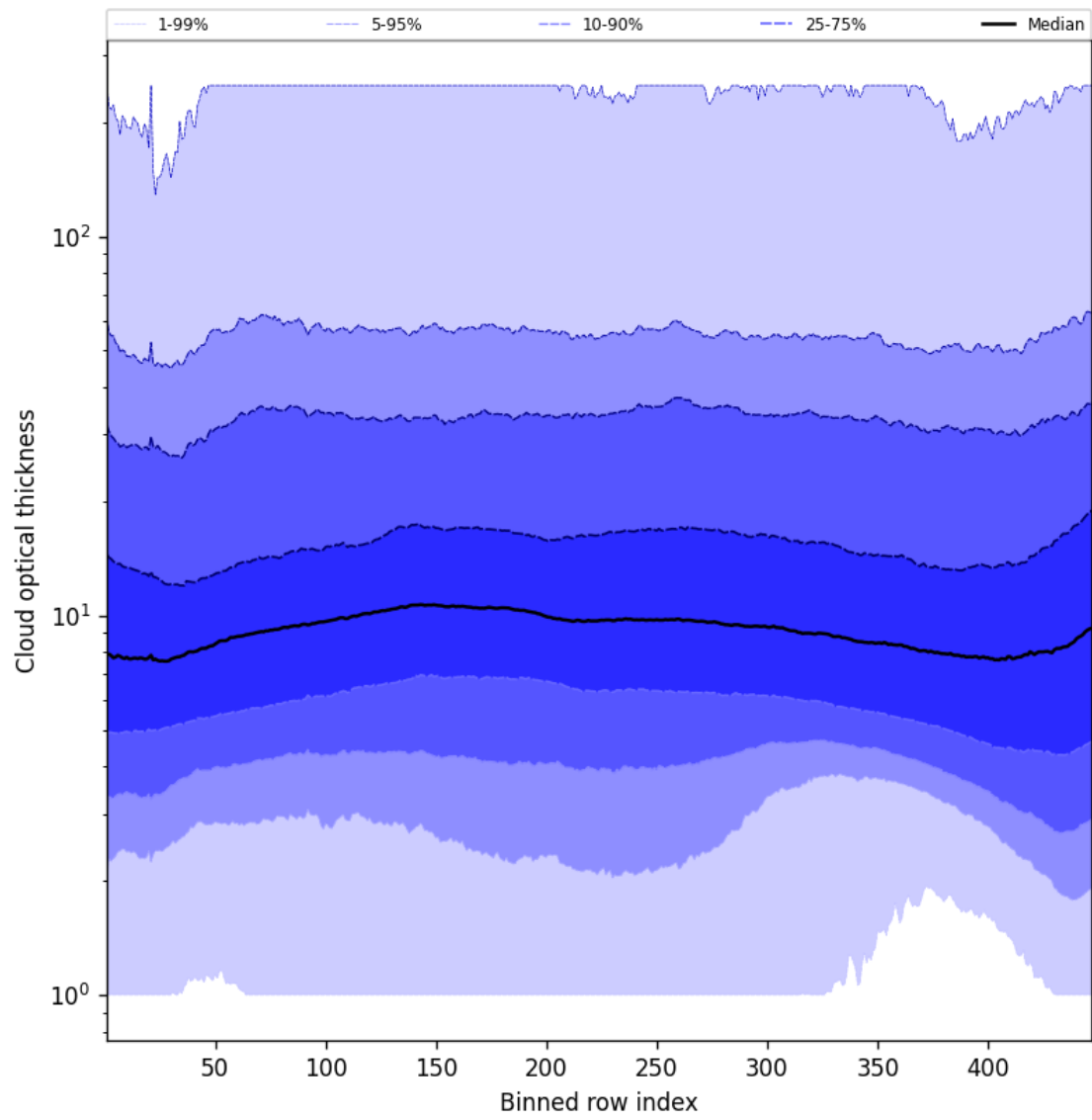
Figure 57: Along track statistics of “Cloud optical thickness” for 2025-02-19 to 2025-02-20
