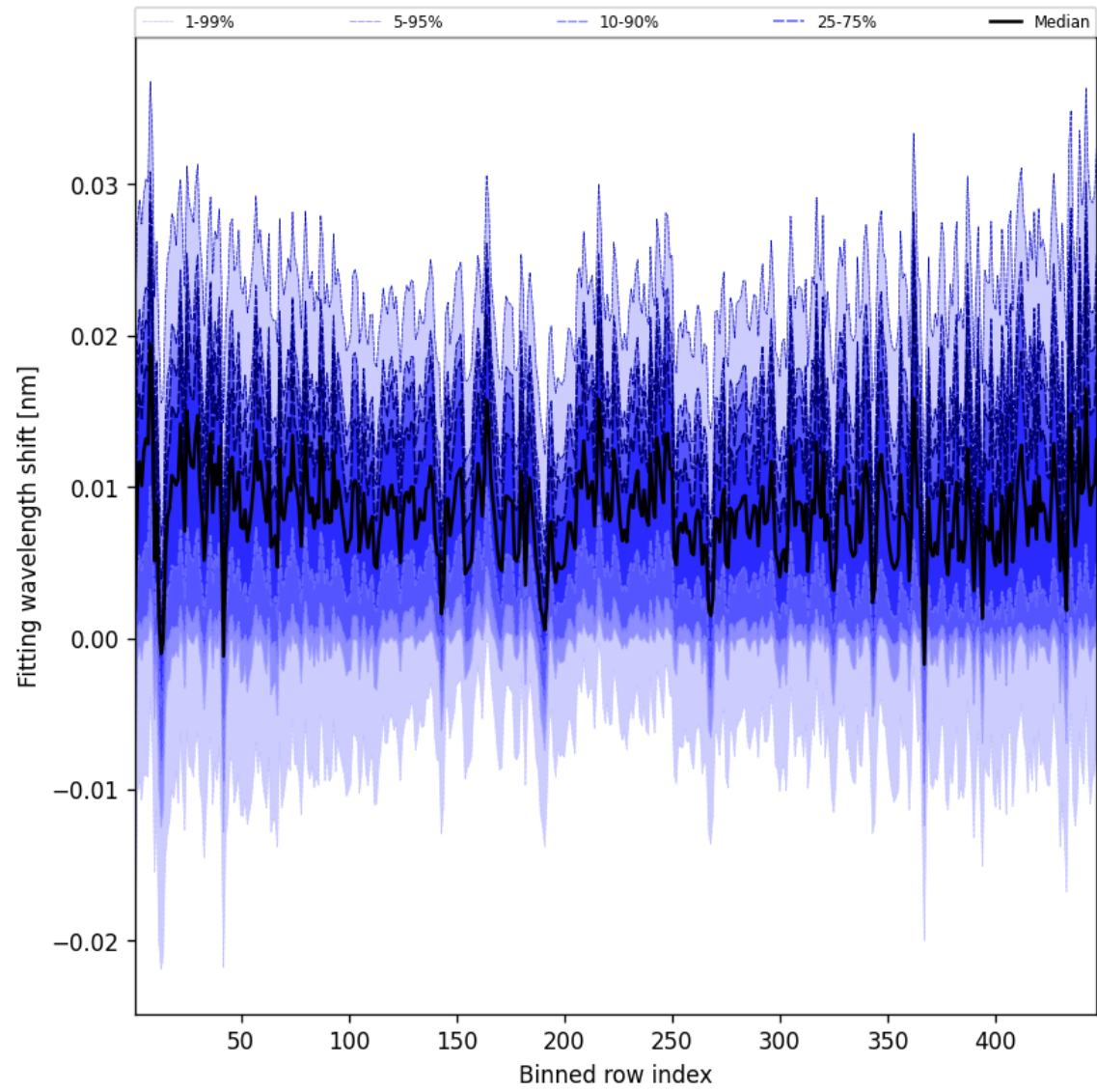
Figure 65: Along track statistics of “Fitting wavelength shift” for 2025-02-19 to 2025-02-20
