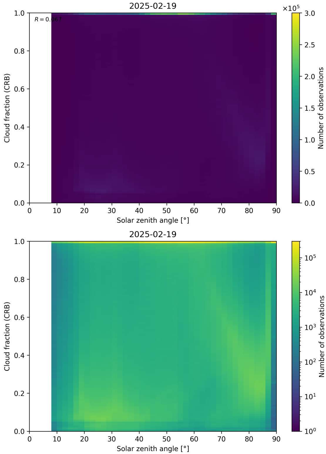
Figure 101: Scatter density plot of “Solar zenith angle” against “Cloud fraction (CRB)” for 2025-02-19 to 2025-02-20.
