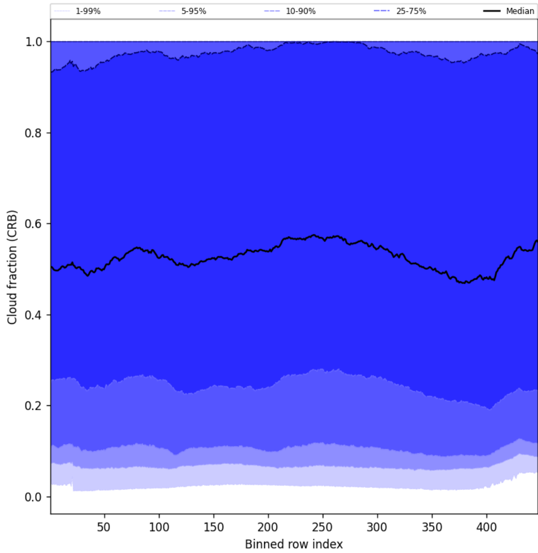
Figure 58: Along track statistics of “Cloud fraction (CRB)” for 2025-02-19 to 2025-02-20
