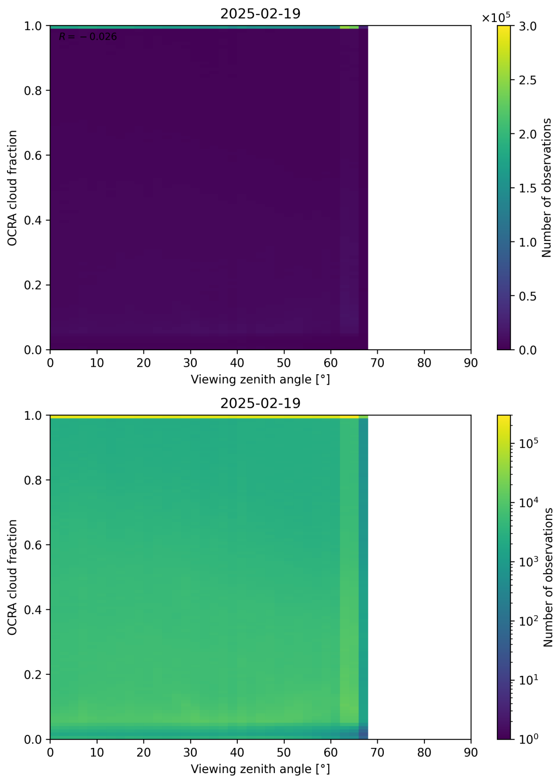
Figure 108: Scatter density plot of “Viewing zenith angle” against “OCRA cloud fraction” for 2025-02-19 to 2025-02-20.
