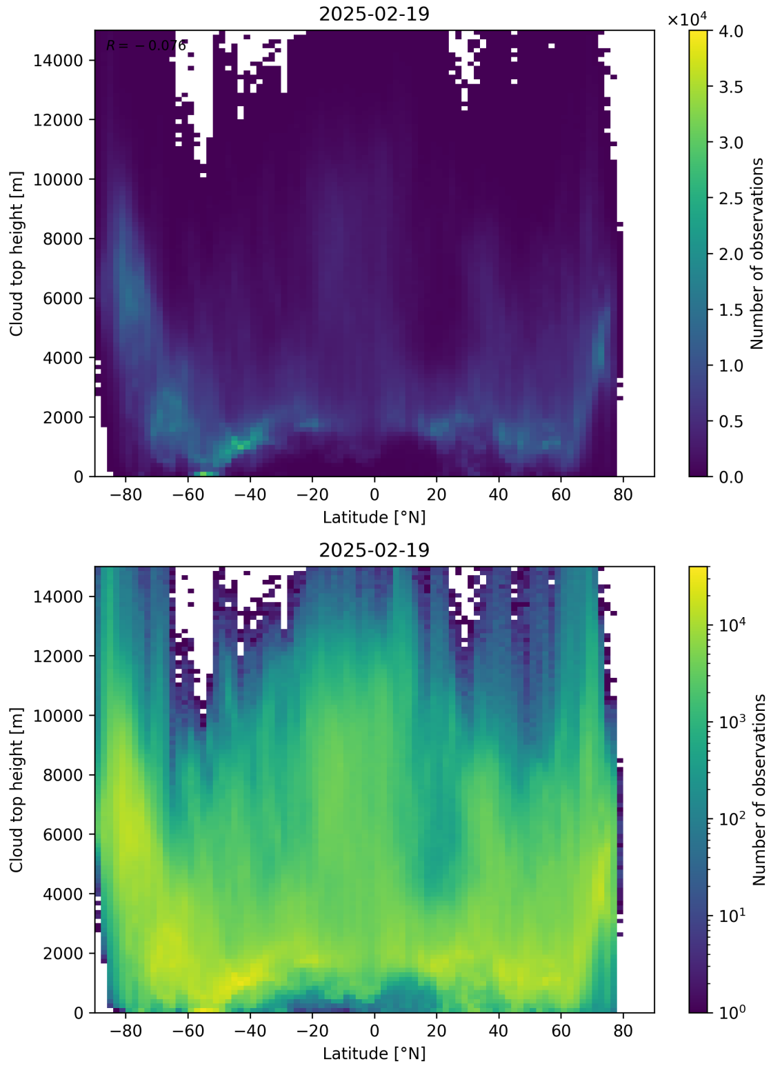
Figure 97: Scatter density plot of “Latitude” against “Cloud top height” for 2025-02-19 to 2025-02-20.
