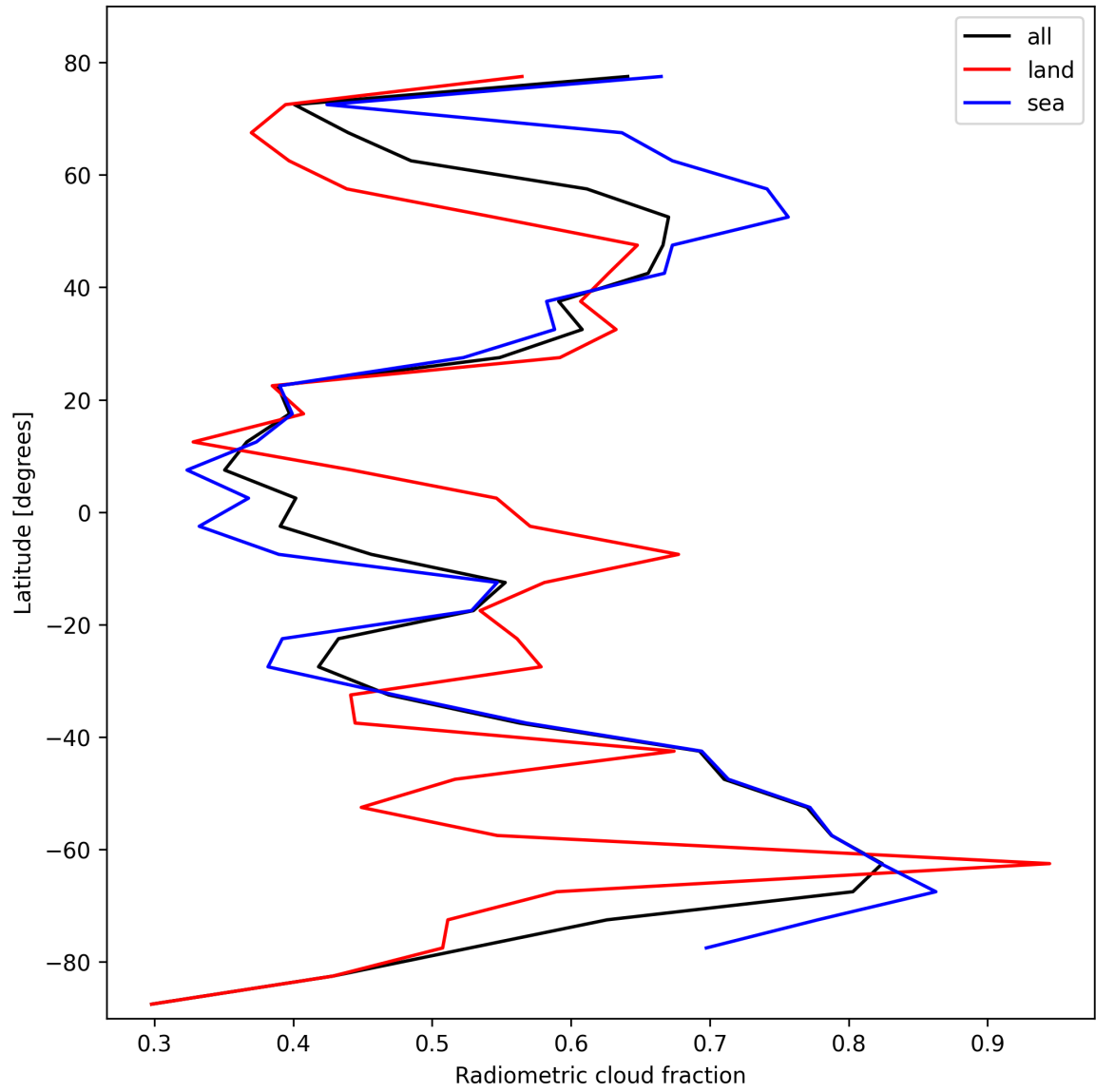
Figure 23: Zonal average of “Radiometric cloud fraction” for 2025-02-19 to 2025-02-20.
