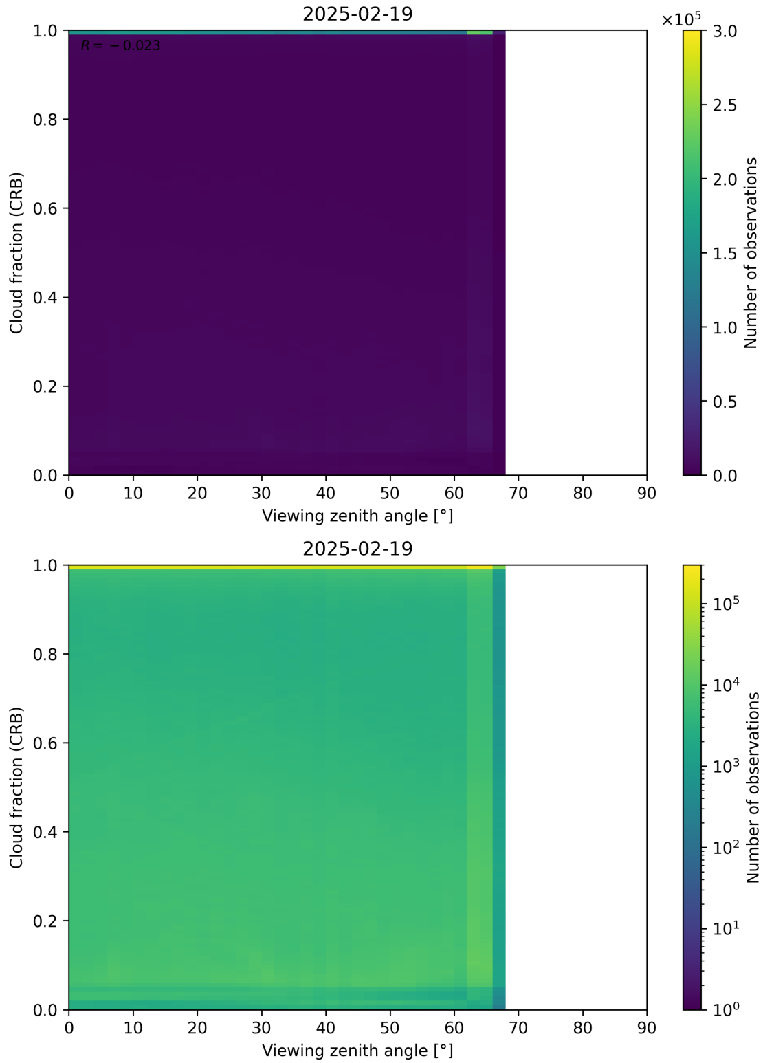
Figure 109: Scatter density plot of “Viewing zenith angle” against “Cloud fraction (CRB)” for 2025-02-19 to 2025-02-20.
