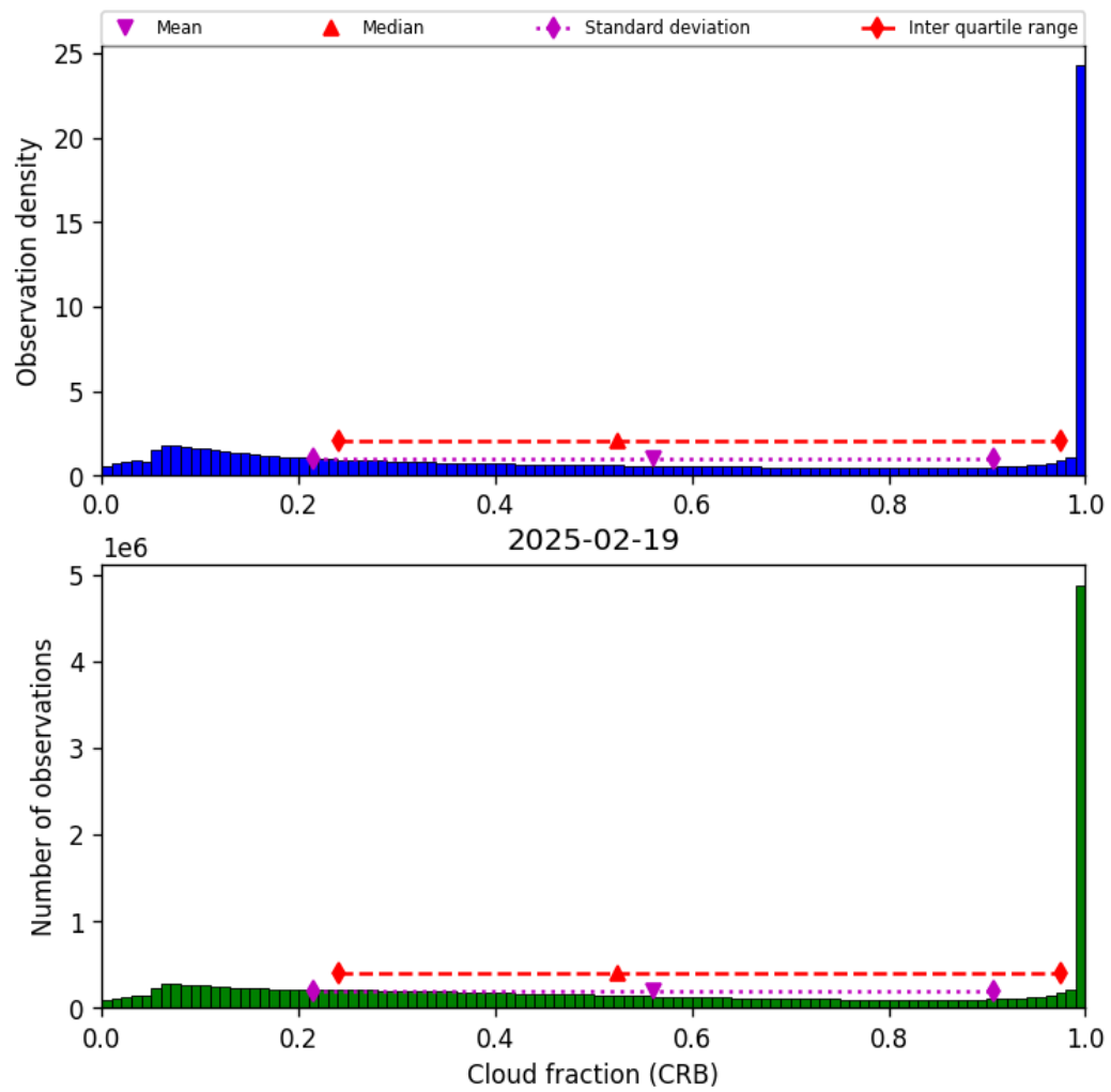
Figure 42: Histogram of “Cloud fraction (CRB)” for 2025-02-19 to 2025-02-20
