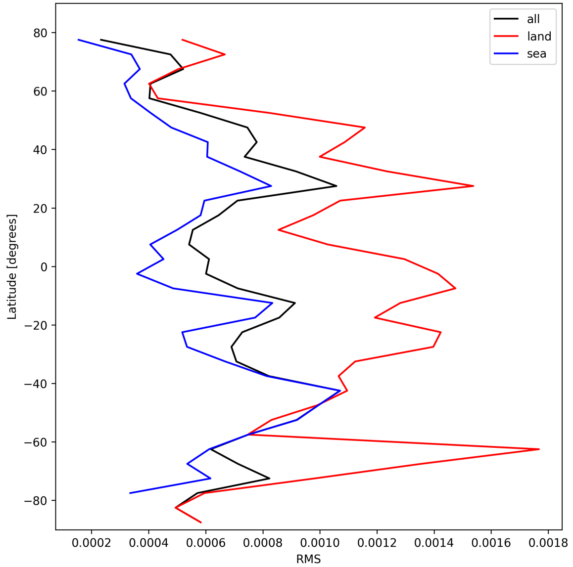
Figure 31: Zonal average of “RMS” for 2025-02-19 to 2025-02-20.
