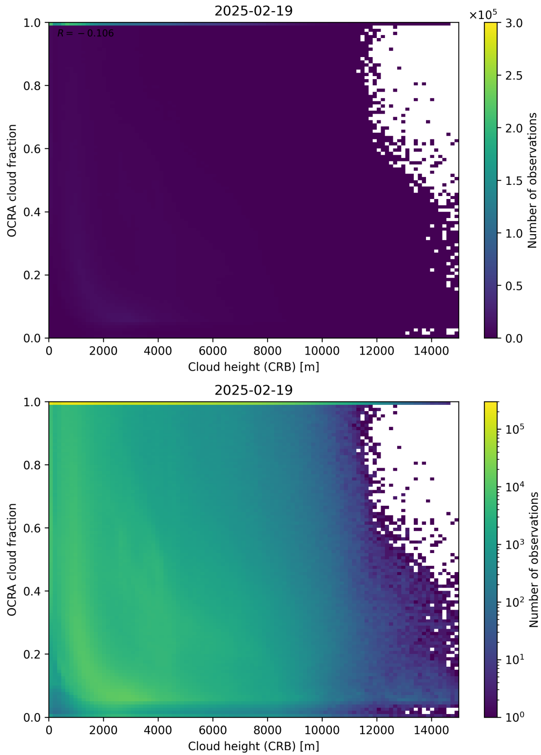
Figure 81: Scatter density plot of “Cloud height (CRB)” against “OCRA cloud fraction” for 2025-02-19 to 2025-02-20.
