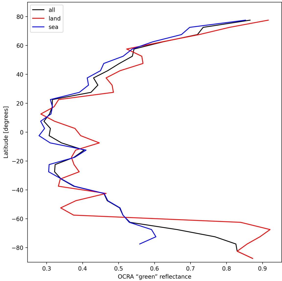
Figure 36: Zonal average of “OCRA “green” reflectance” for 2025-02-19 to 2025-02-20.
