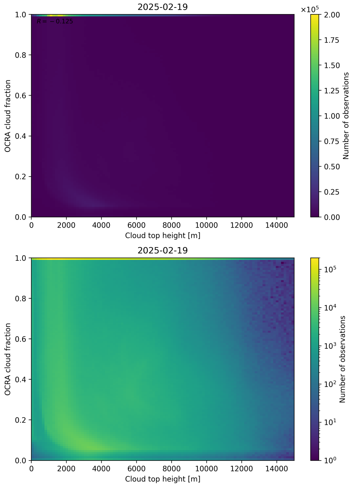
Figure 87: Scatter density plot of “Cloud top height” against “OCRA cloud fraction” for 2025-02-19 to 2025-02-20.
