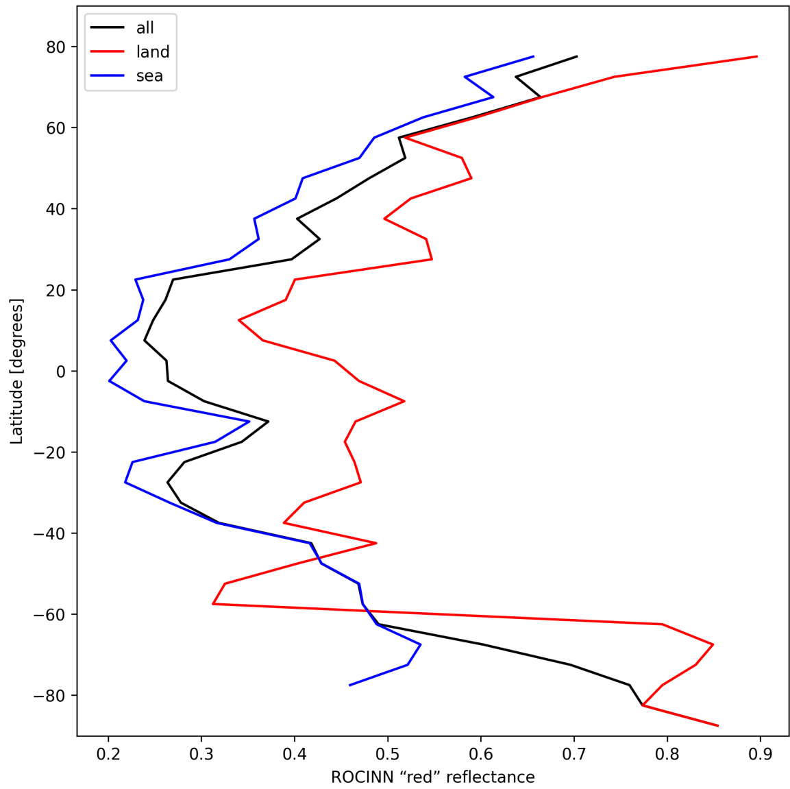
Figure 37: Zonal average of “ROCINN “red” reflectance” for 2025-02-19 to 2025-02-20.
