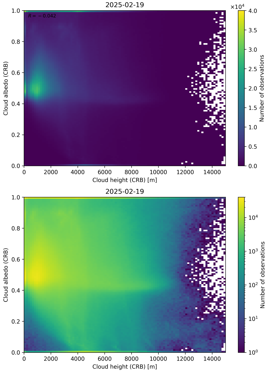
Figure 80: Scatter density plot of “Cloud height (CRB)” against “Cloud albedo (CRB)” for 2025-02-19 to 2025-02-20.
