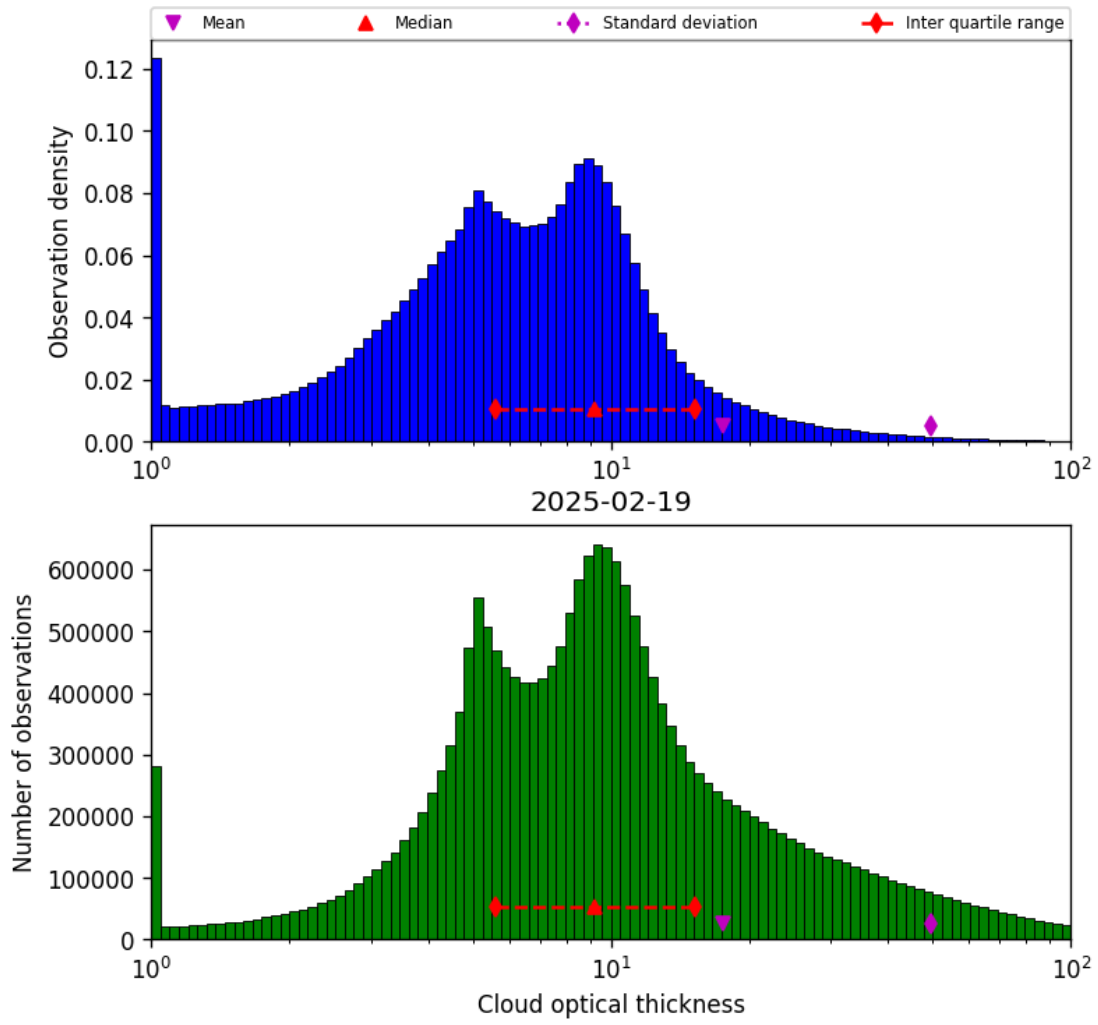
Figure 41: Histogram of “Cloud optical thickness” for 2025-02-19 to 2025-02-20
