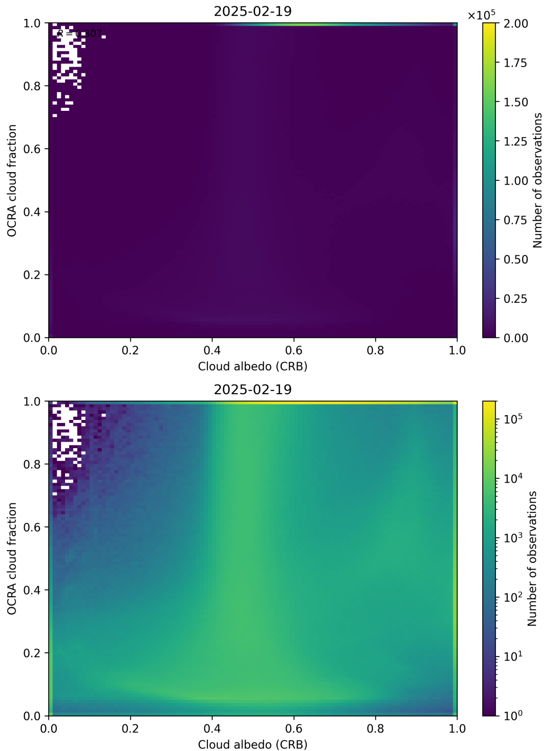
Figure 70: Scatter density plot of “Cloud albedo (CRB)” against “OCRA cloud fraction” for 2025-02-19 to 2025-02-20.
