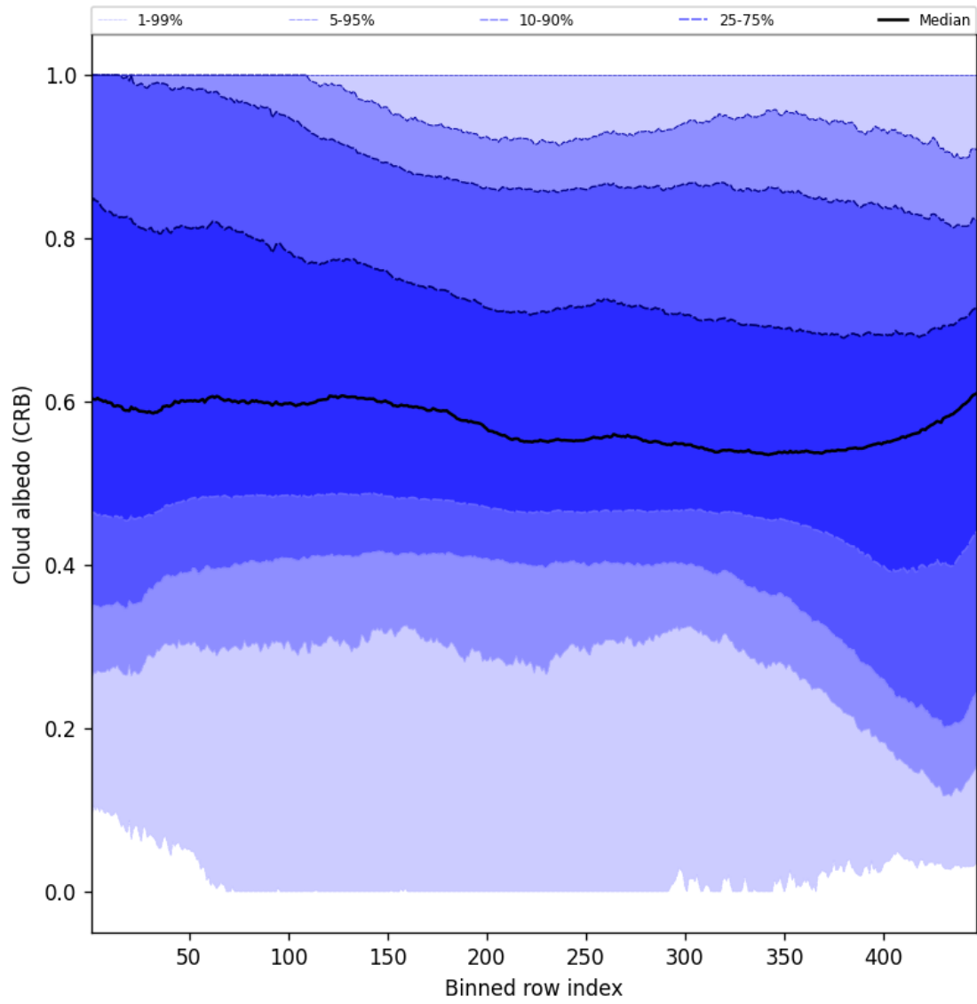
Figure 60: Along track statistics of “Cloud albedo (CRB)” for 2025-02-19 to 2025-02-20
