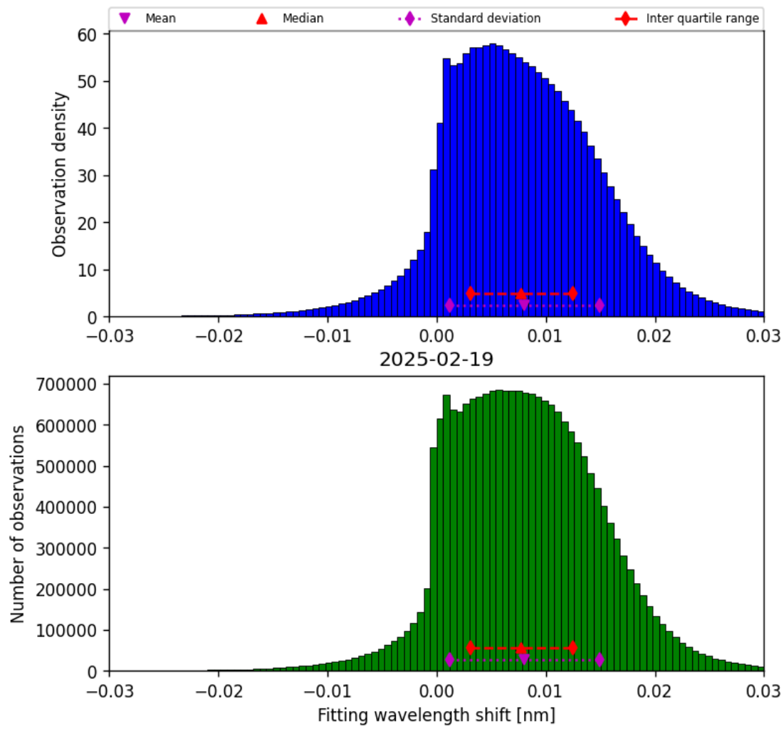
Figure 49: Histogram of “Fitting wavelength shift” for 2025-02-19 to 2025-02-20
