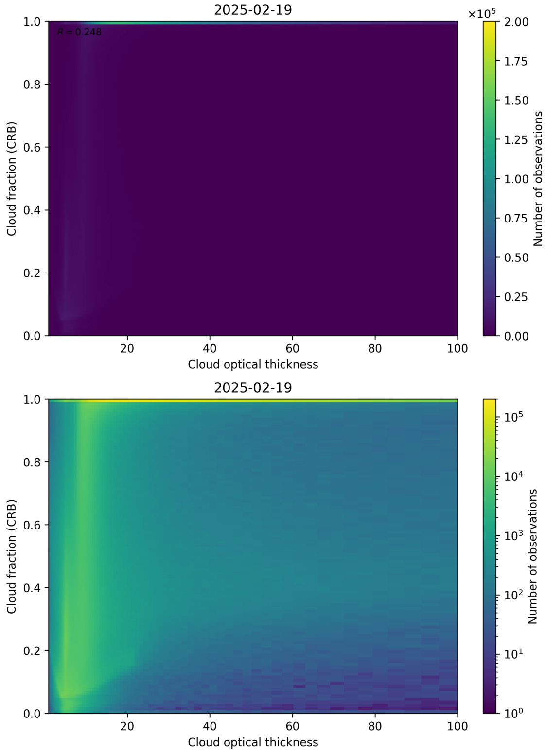
Figure 84: Scatter density plot of “Cloud optical thickness” against “Cloud fraction (CRB)” for 2025-02-19 to 2025-02-20.
