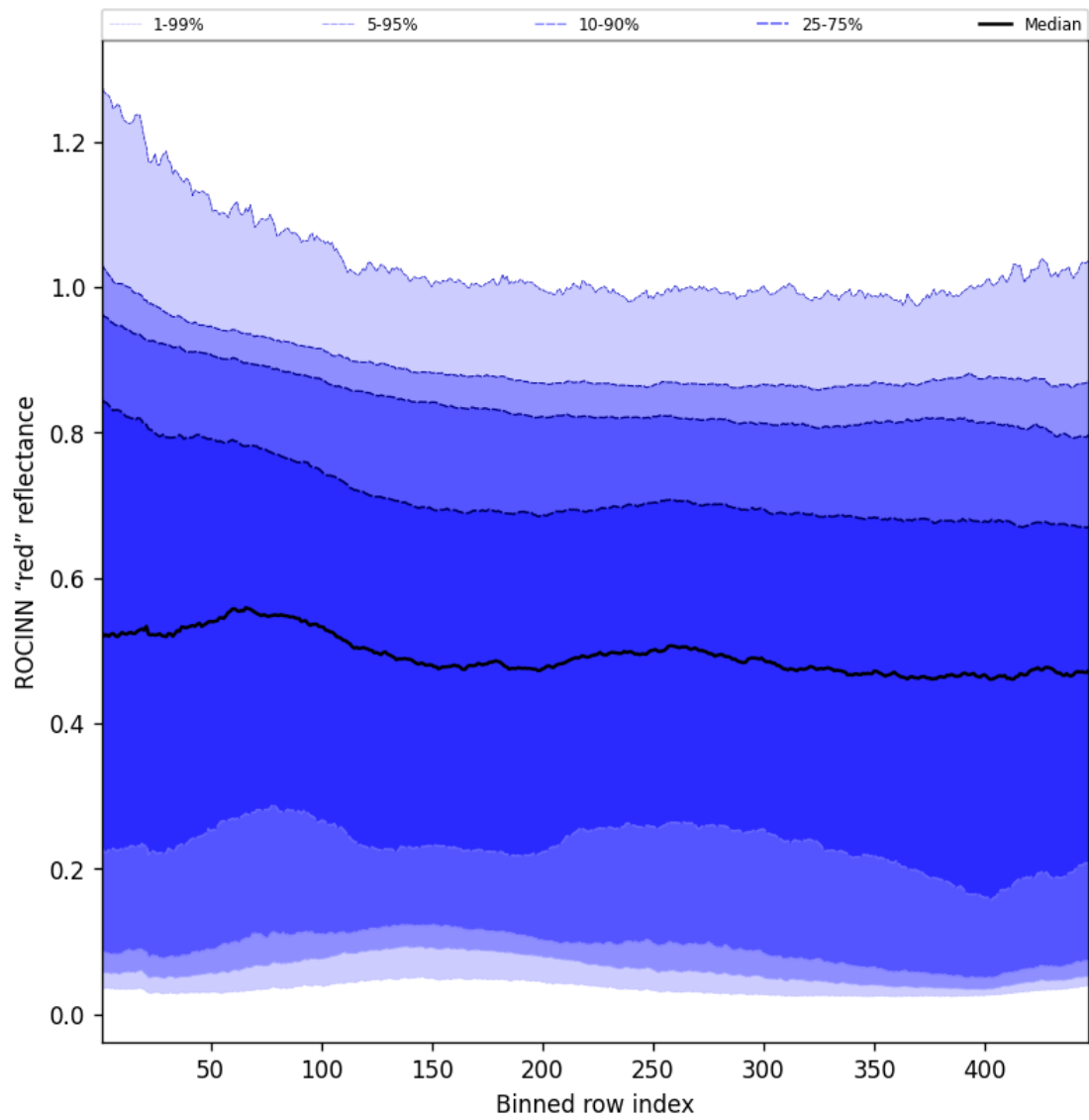
Figure 69: Along track statistics of "ROCINN "red" reflectance" for 2025-02-19 to 2025-02-20
