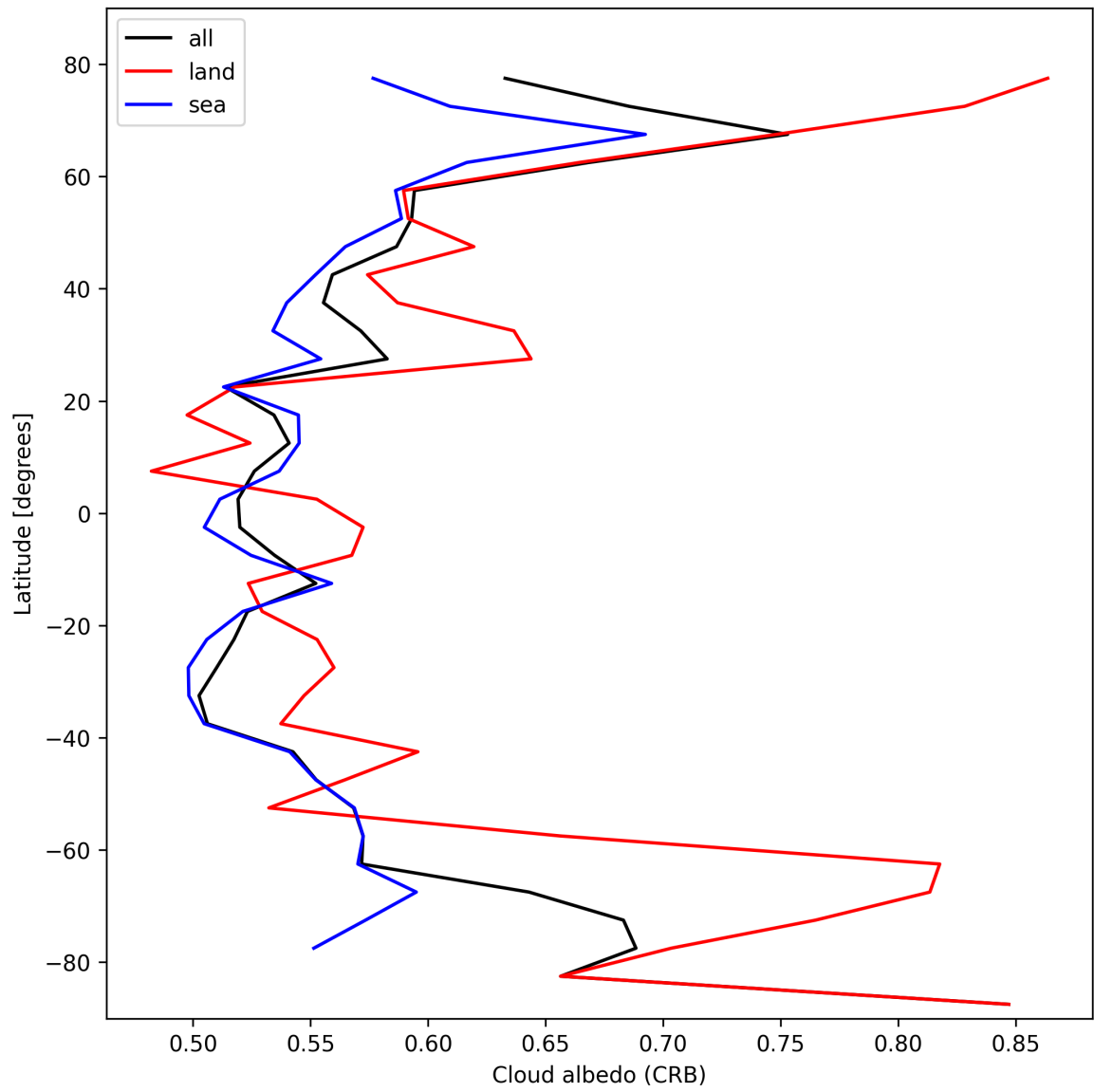
Figure 28: Zonal average of “Cloud albedo (CRB)” for 2025-02-19 to 2025-02-20.
