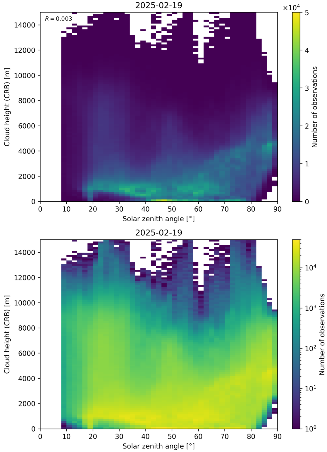
Figure 102: Scatter density plot of “Solar zenith angle” against “Cloud height (CRB)” for 2025-02-19 to 2025-02-20.
