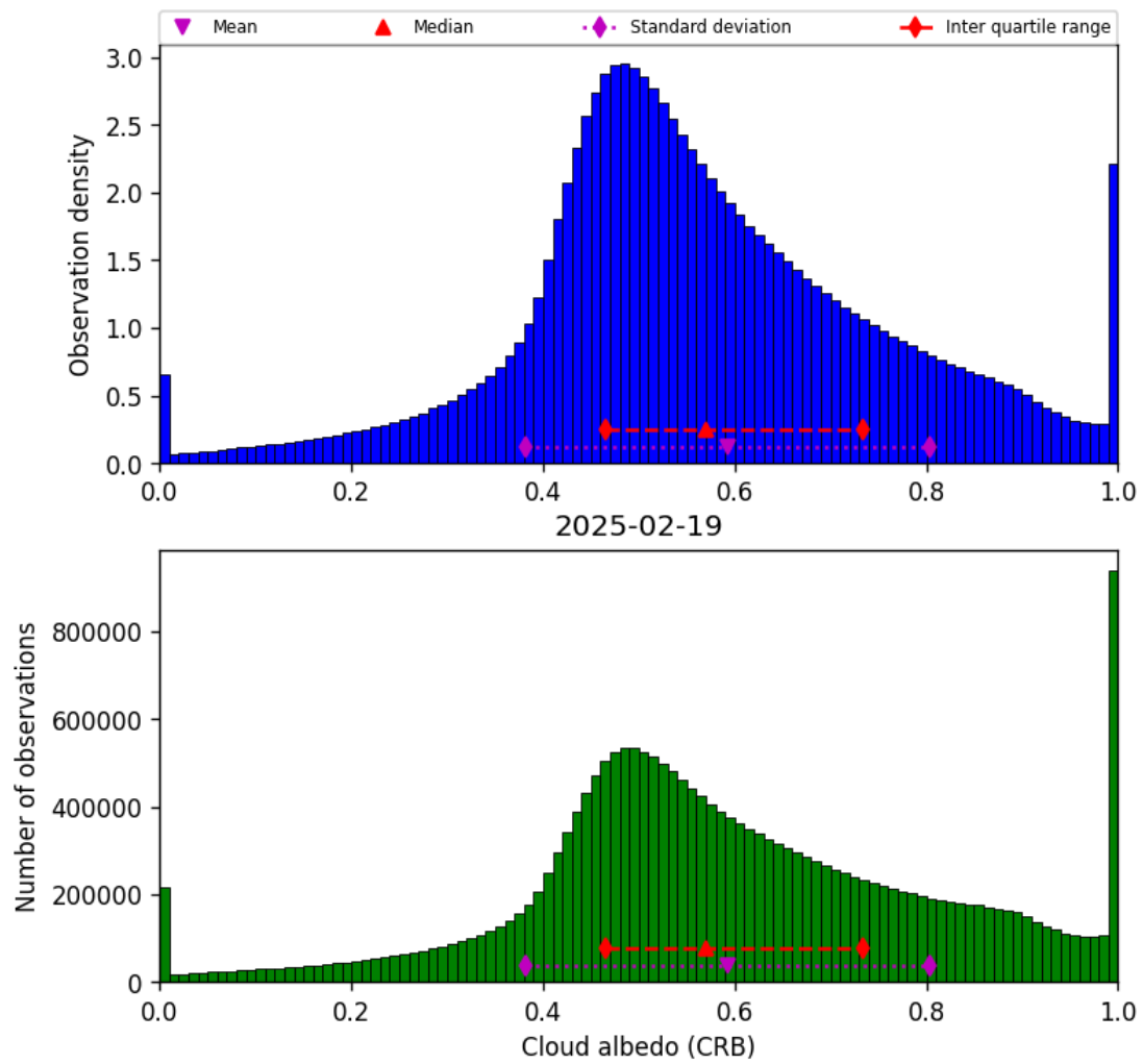
Figure 44: Histogram of “Cloud albedo (CRB)” for 2025-02-19 to 2025-02-20
