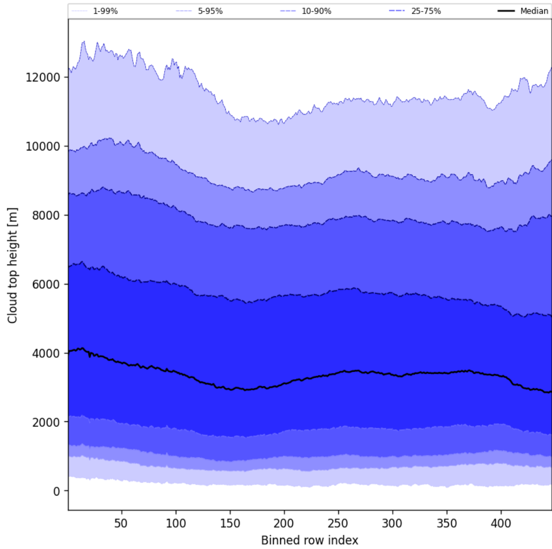
Figure 56: Along track statistics of “Cloud top height” for 2025-02-19 to 2025-02-20
