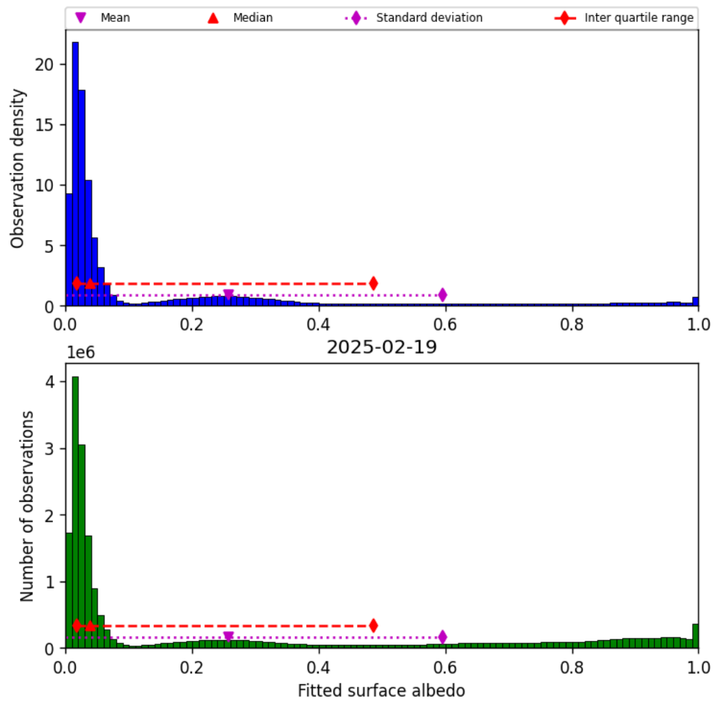
Figure 45: Histogram of “Fitted surface albedo” for 2025-02-19 to 2025-02-20
