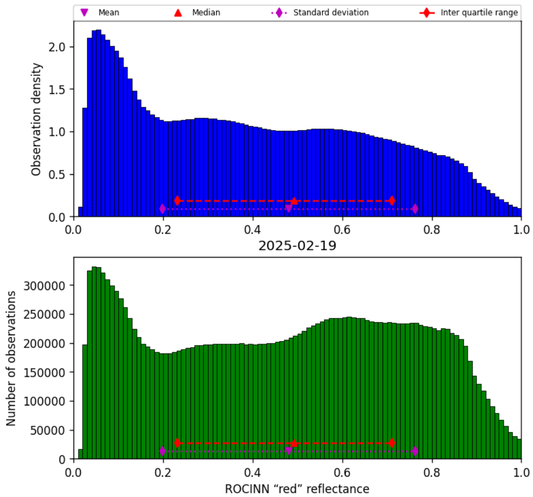
Figure 53: Histogram of “ROCINN “red” reflectance” for 2025-02-19 to 2025-02-20
