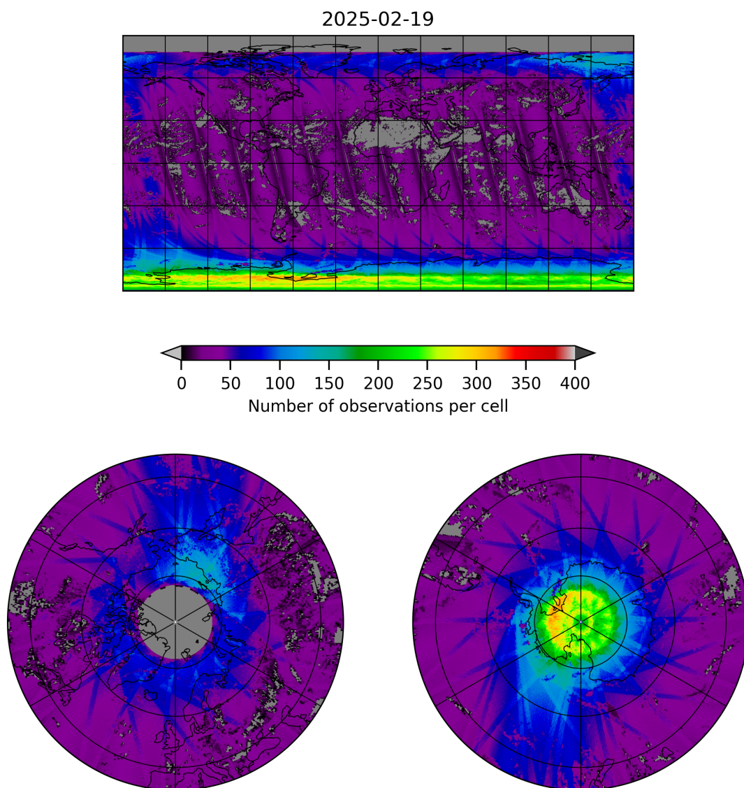
Figure 21: Map of the number of observations for 2025-02-19 to 2025-02-20
