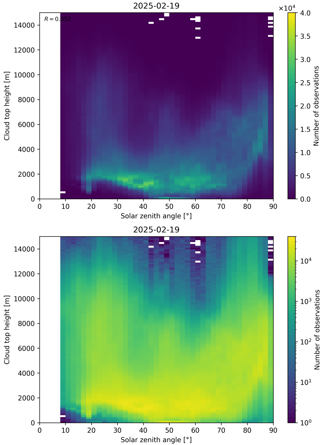
Figure 104: Scatter density plot of “Solar zenith angle” against “Cloud top height” for 2025-02-19 to 2025-02-20.
