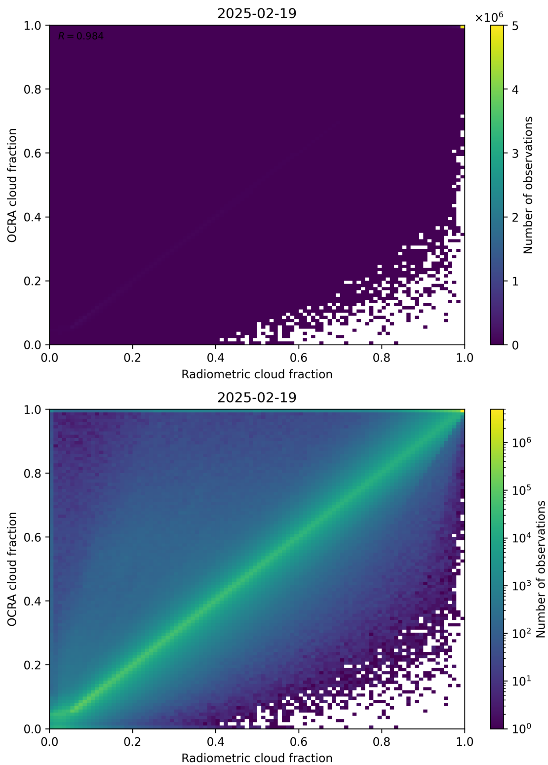
Figure 72: Scatter density plot of “Radiometric cloud fraction” against “OCRA cloud fraction” for 2025-02-19 to 2025-02-20.
