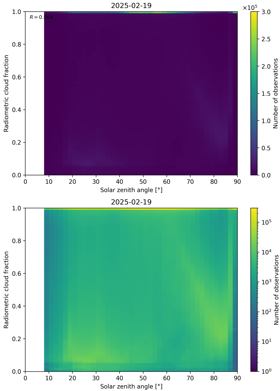
Figure 99: Scatter density plot of “Solar zenith angle” against “Radiometric cloud fraction” for 2025-02-19 to 2025-02-20.
