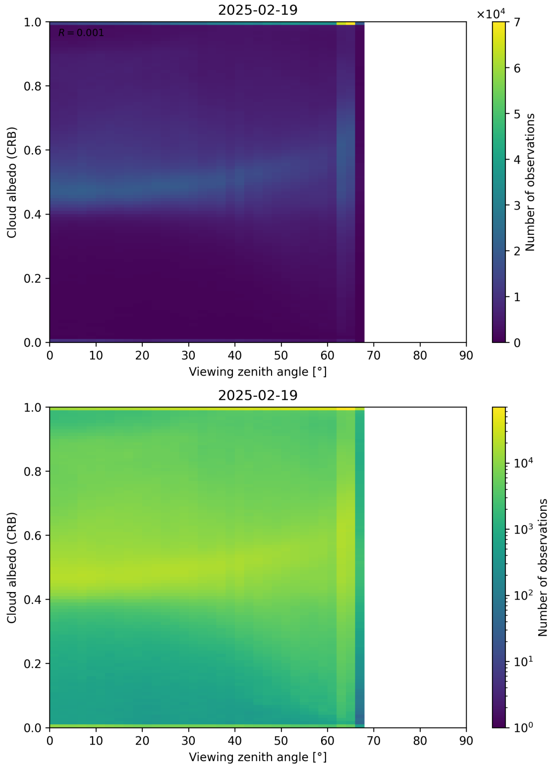
Figure 106: Scatter density plot of “Viewing zenith angle” against “Cloud albedo (CRB)” for 2025-02-19 to 2025-02-20.
