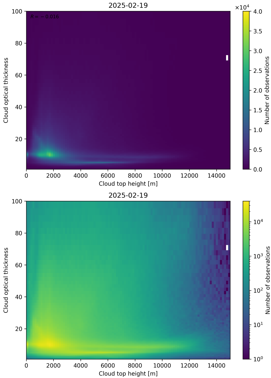
Figure 90: Scatter density plot of “Cloud top height” against “Cloud optical thickness” for 2025-02-19 to 2025-02-20.
