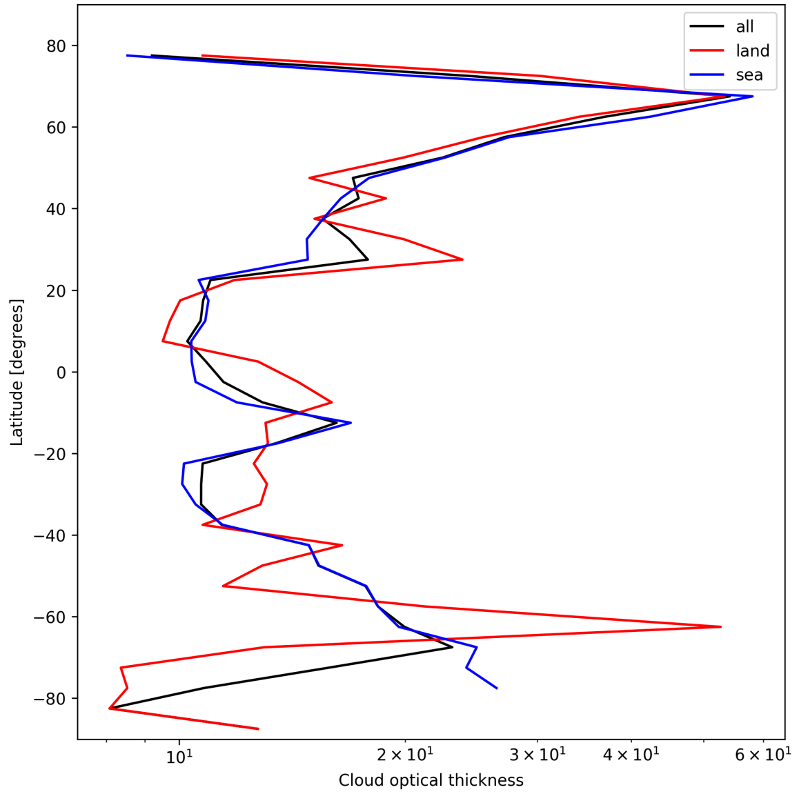
Figure 25: Zonal average of “Cloud optical thickness” for 2025-02-19 to 2025-02-20.
