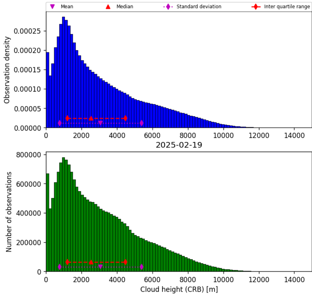
Figure 43: Histogram of “Cloud height (CRB)” for 2025-02-19 to 2025-02-20
