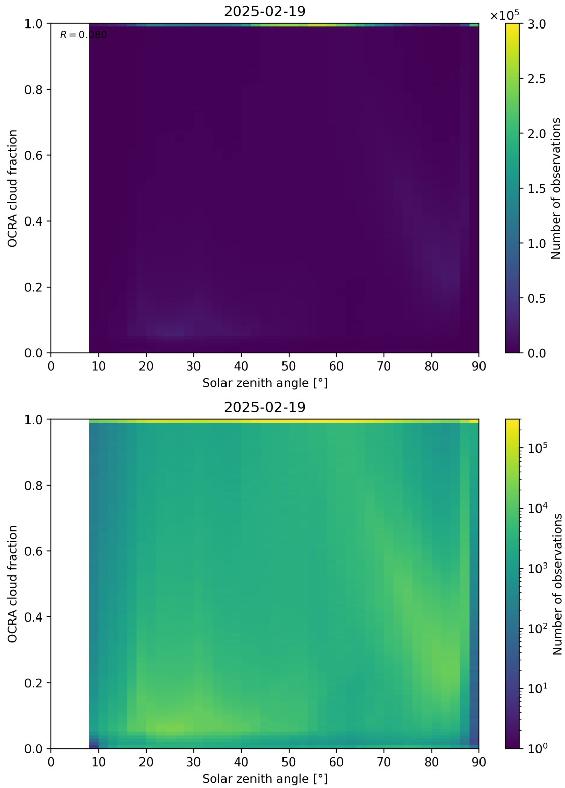
Figure 100: Scatter density plot of “Solar zenith angle” against “OCRA cloud fraction” for 2025-02-19 to 2025-02-20.
