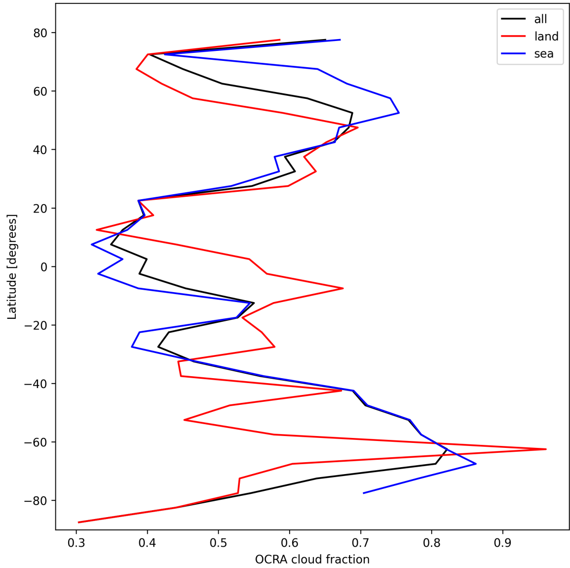
Figure 34: Zonal average of “OCRA cloud fraction” for 2025-02-19 to 2025-02-20.
