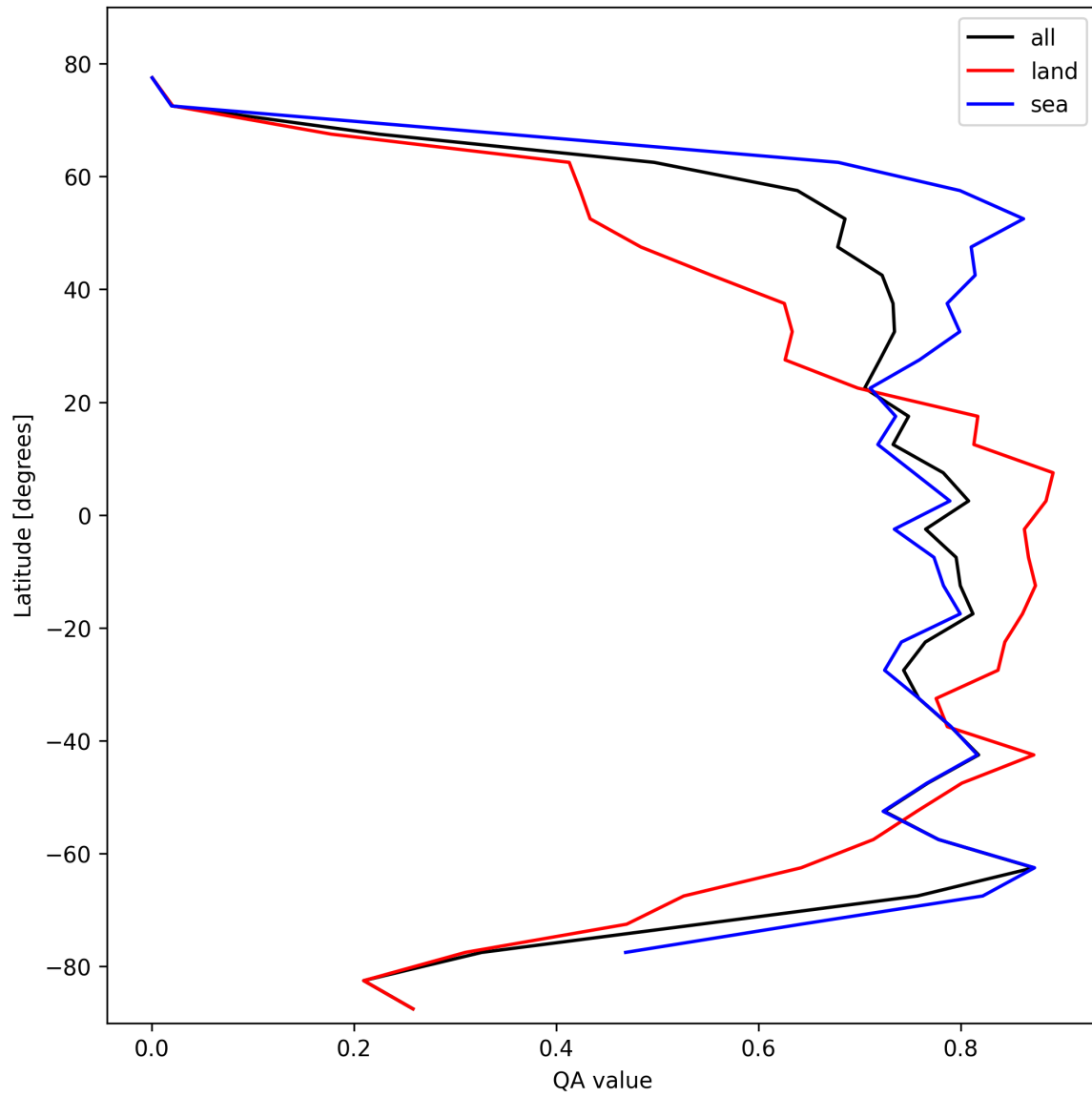
Figure 22: Zonal average of “QA value” for 2025-02-19 to 2025-02-20.
