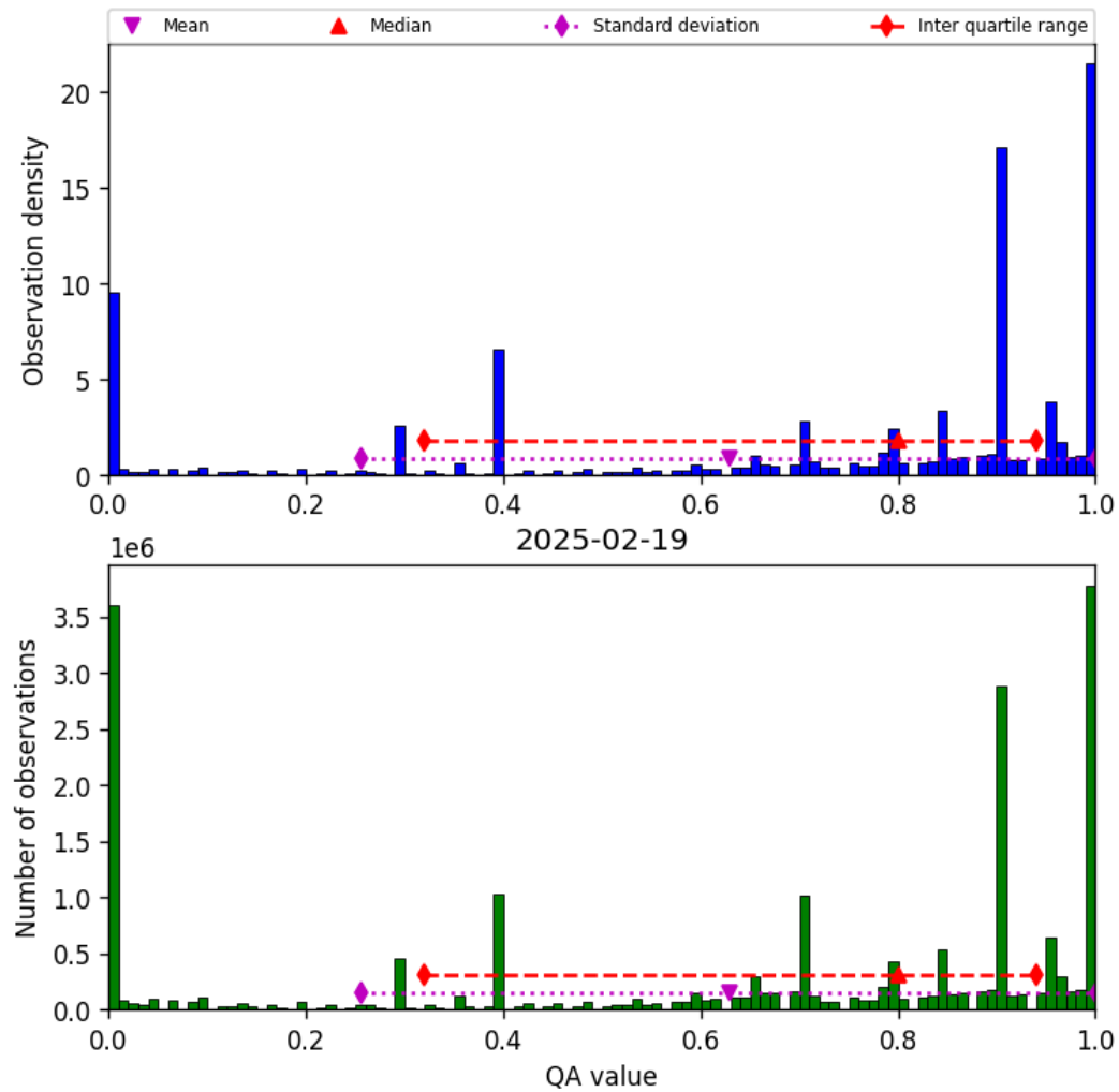
Figure 38: Histogram of “QA value” for 2025-02-19 to 2025-02-20
