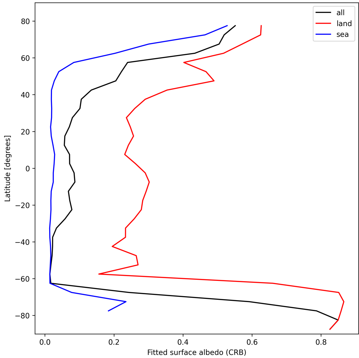
Figure 30: Zonal average of “Fitted surface albedo (CRB)” for 2025-02-19 to 2025-02-20.
