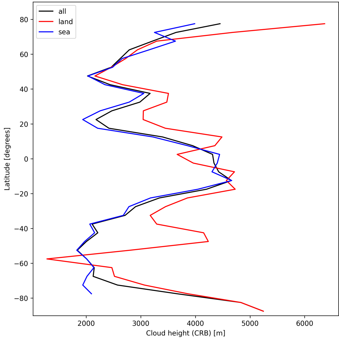
Figure 27: Zonal average of “Cloud height (CRB)” for 2025-02-19 to 2025-02-20.
