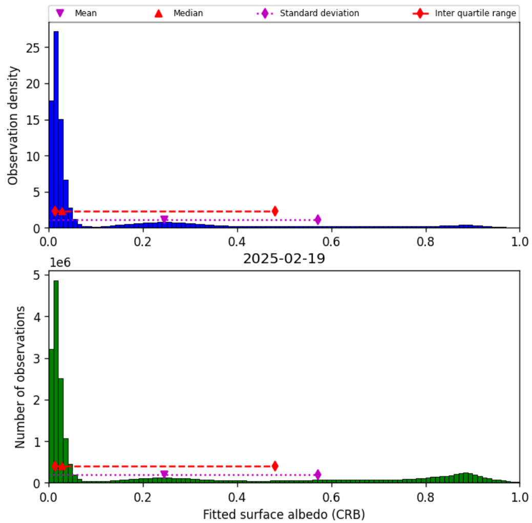
Figure 46: Histogram of “Fitted surface albedo (CRB)” for 2025-02-19 to 2025-02-20
