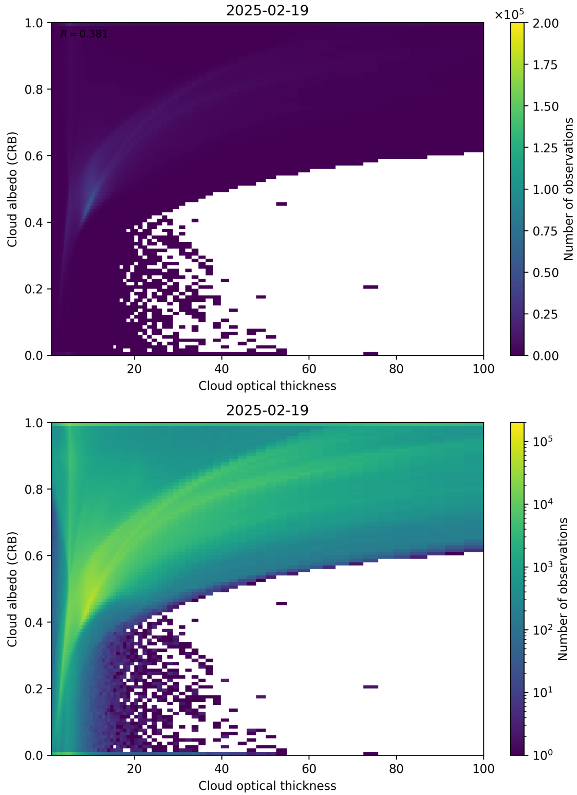
Figure 82: Scatter density plot of “Cloud optical thickness” against “Cloud albedo (CRB)” for 2025-02-19 to 2025-02-20.
