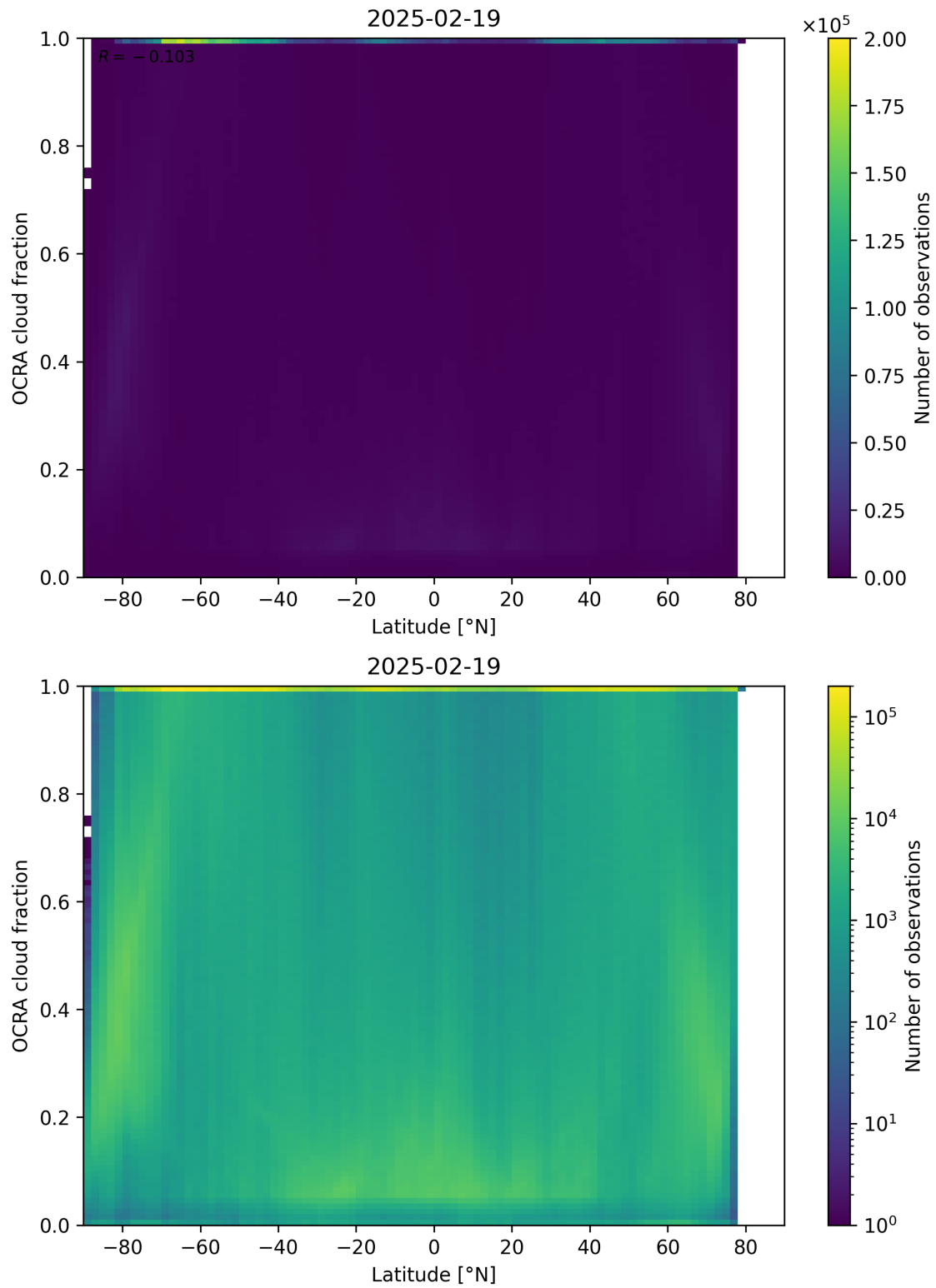
Figure 93: Scatter density plot of “Latitude” against “OCRA cloud fraction” for 2025-02-19 to 2025-02-20.
