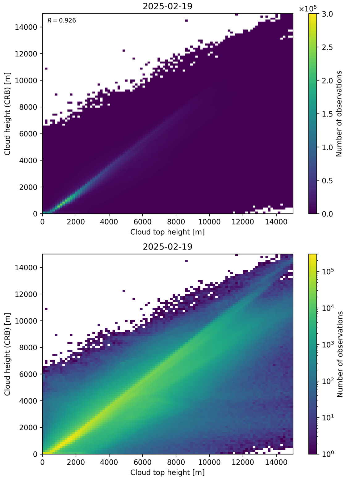
Figure 89: Scatter density plot of “Cloud top height” against “Cloud height (CRB)” for 2025-02-19 to 2025-02-20.
