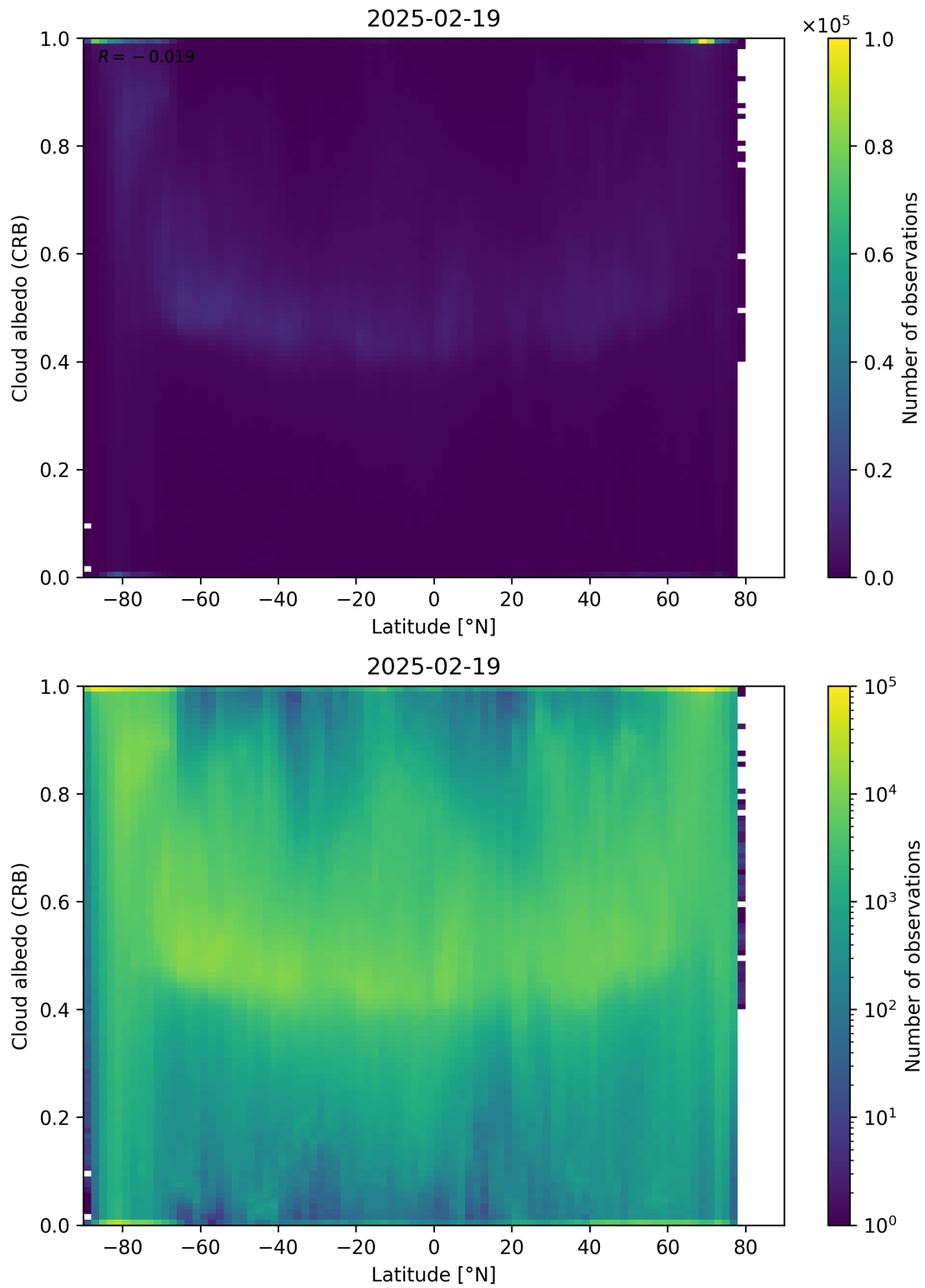
Figure 91: Scatter density plot of “Latitude” against “Cloud albedo (CRB)” for 2025-02-19 to 2025-02-20.
