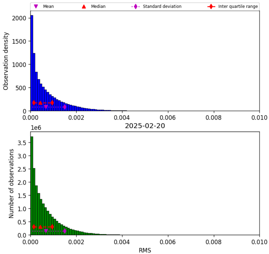
Figure 47: Histogram of “RMS” for 2025-02-19 to 2025-02-21
