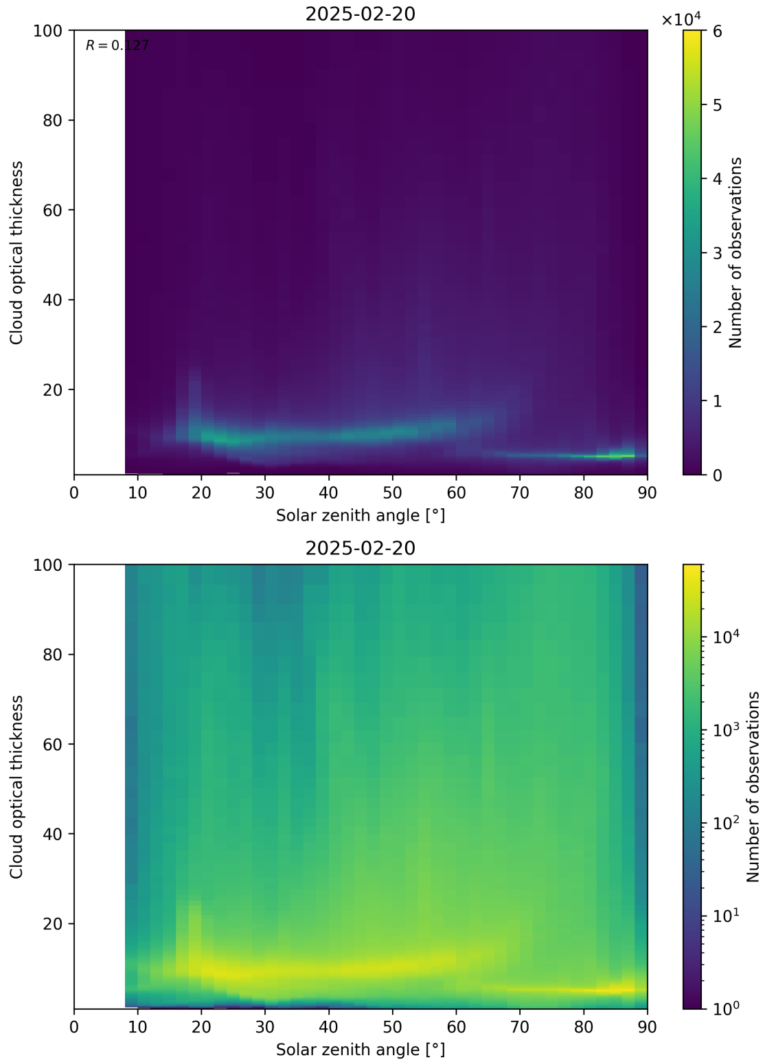
Figure 103: Scatter density plot of “Solar zenith angle” against “Cloud optical thickness” for 2025-02-19 to 2025-02-21.
