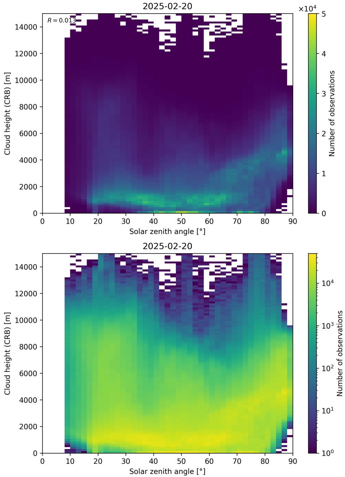
Figure 102: Scatter density plot of “Solar zenith angle” against “Cloud height (CRB)” for 2025-02-19 to 2025-02-21.
