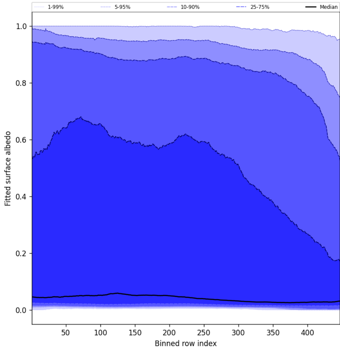
Figure 61: Along track statistics of “Fitted surface albedo” for 2025-02-19 to 2025-02-21
