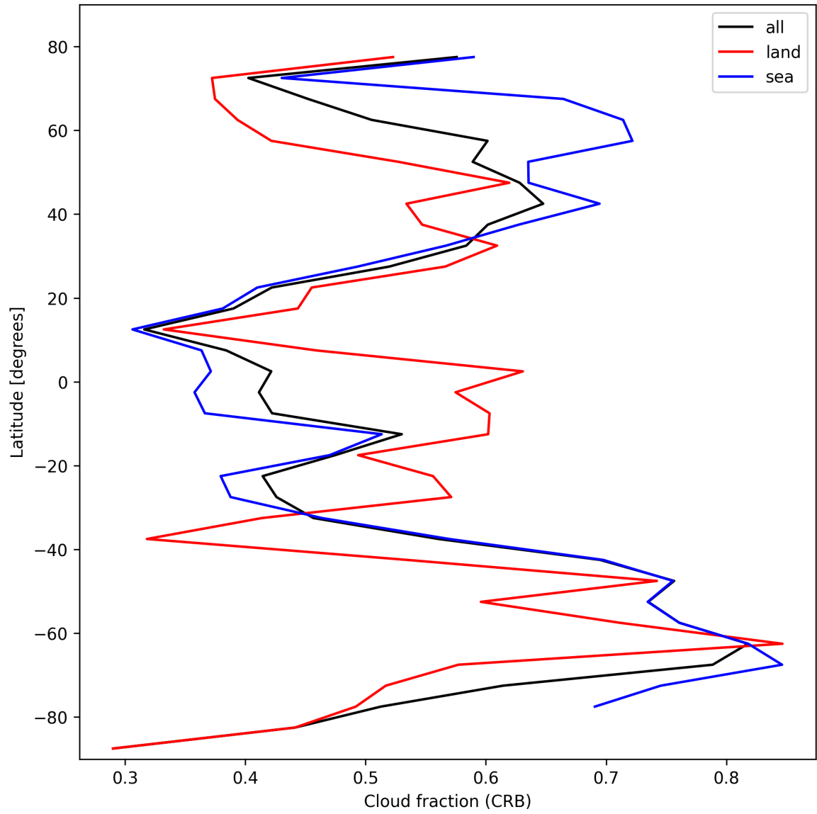
Figure 26: Zonal average of “Cloud fraction (CRB)” for 2025-02-19 to 2025-02-21.
