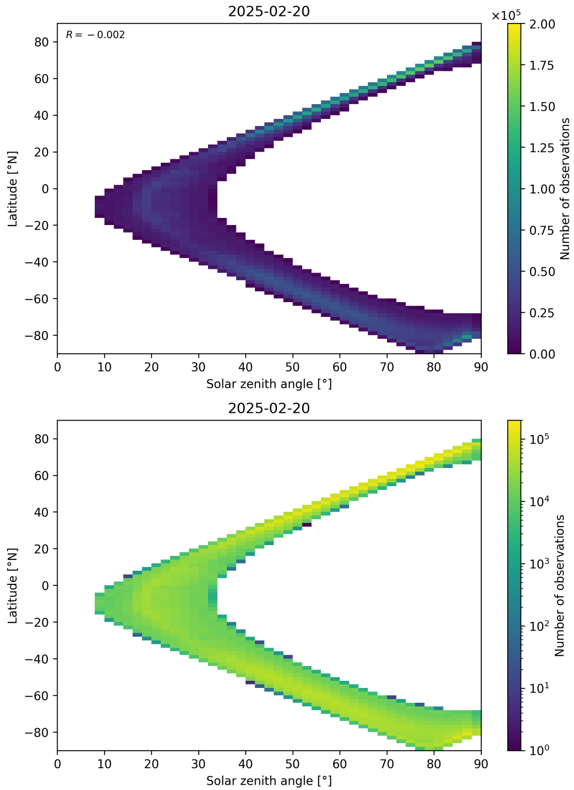
Figure 105: Scatter density plot of “Solar zenith angle” against “Latitude” for 2025-02-19 to 2025-02-21.
