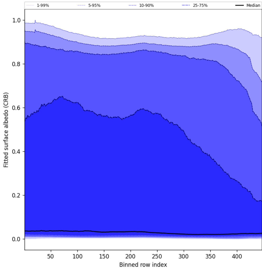
Figure 62: Along track statistics of “Fitted surface albedo (CRB)” for 2025-02-19 to 2025-02-21
