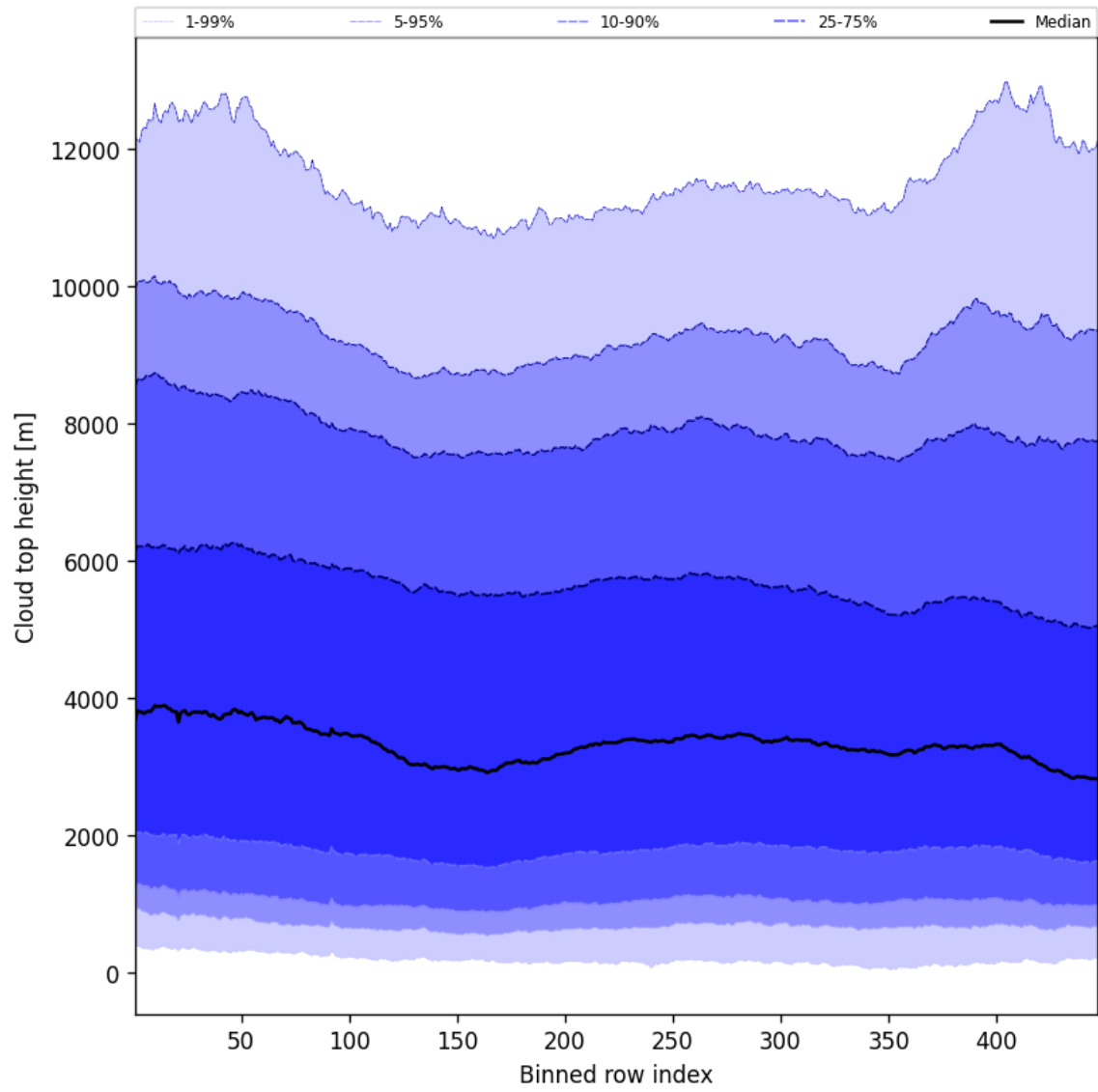
Figure 56: Along track statistics of “Cloud top height” for 2025-02-19 to 2025-02-21
