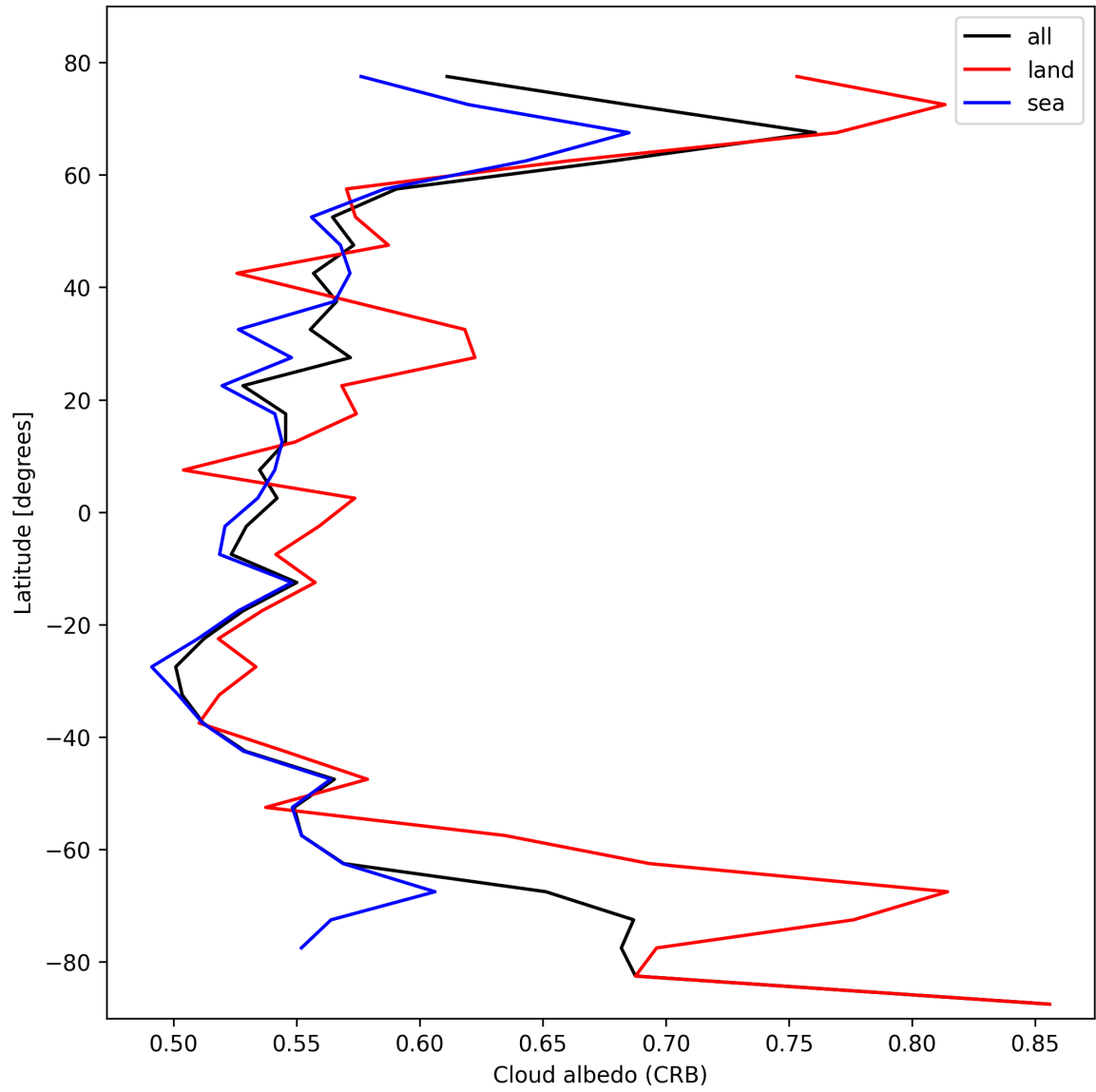
Figure 28: Zonal average of “Cloud albedo (CRB)” for 2025-02-19 to 2025-02-21.
