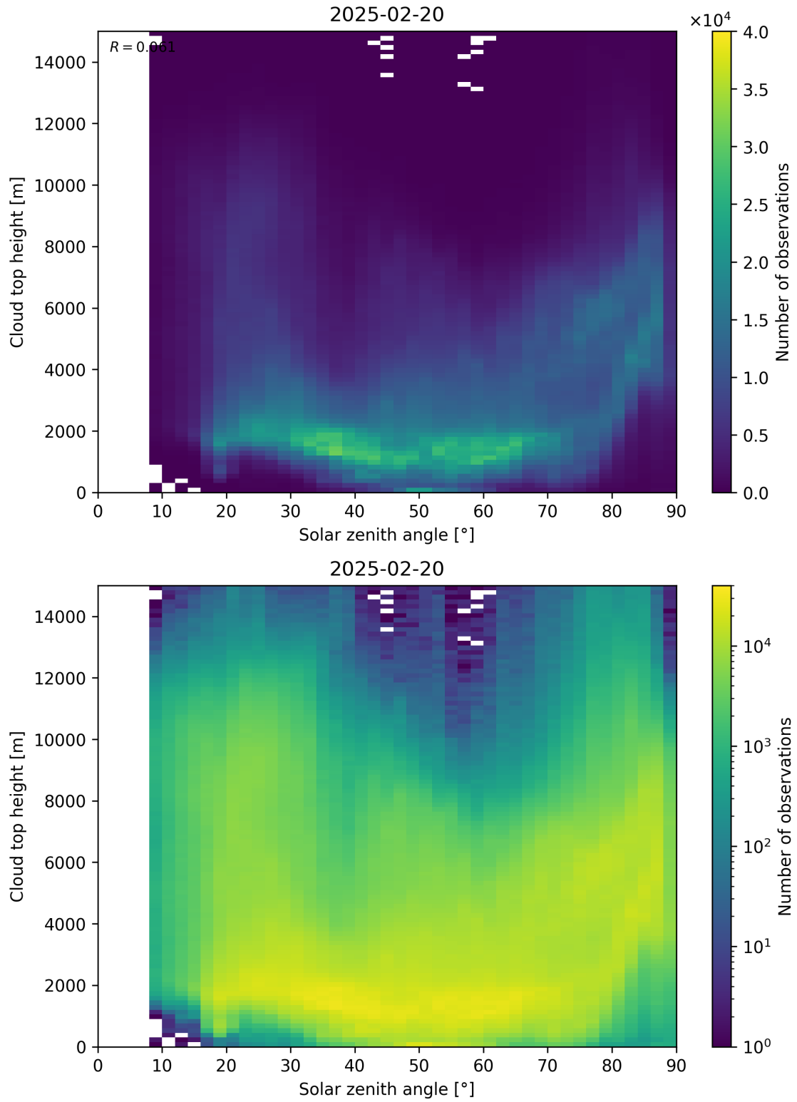
Figure 104: Scatter density plot of “Solar zenith angle” against “Cloud top height” for 2025-02-19 to 2025-02-21.
