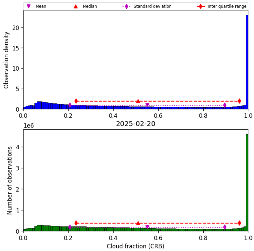
Figure 42: Histogram of “Cloud fraction (CRB)” for 2025-02-19 to 2025-02-21
