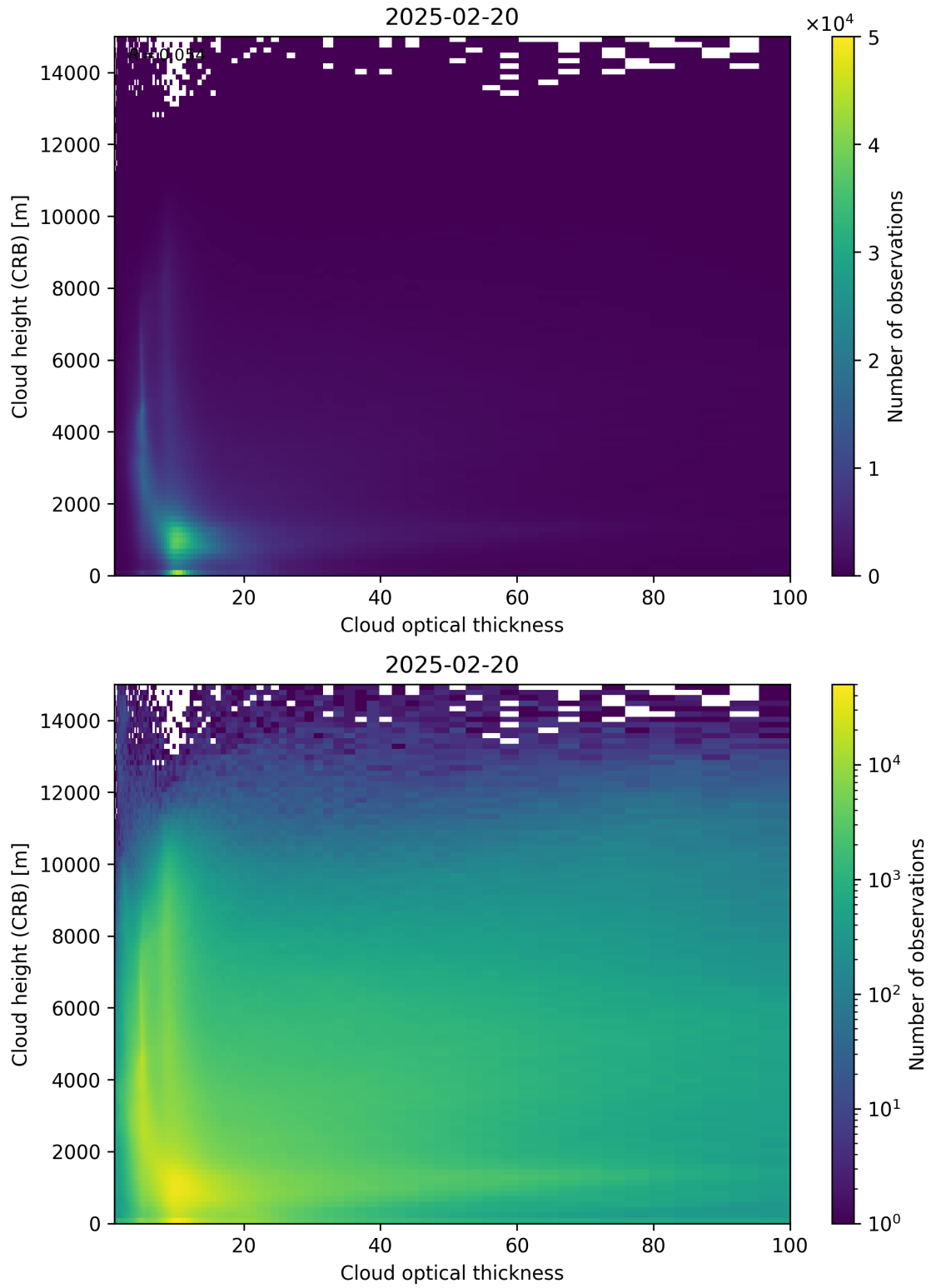
Figure 85: Scatter density plot of “Cloud optical thickness” against “Cloud height (CRB)” for 2025-02-19 to 2025-02-21.
