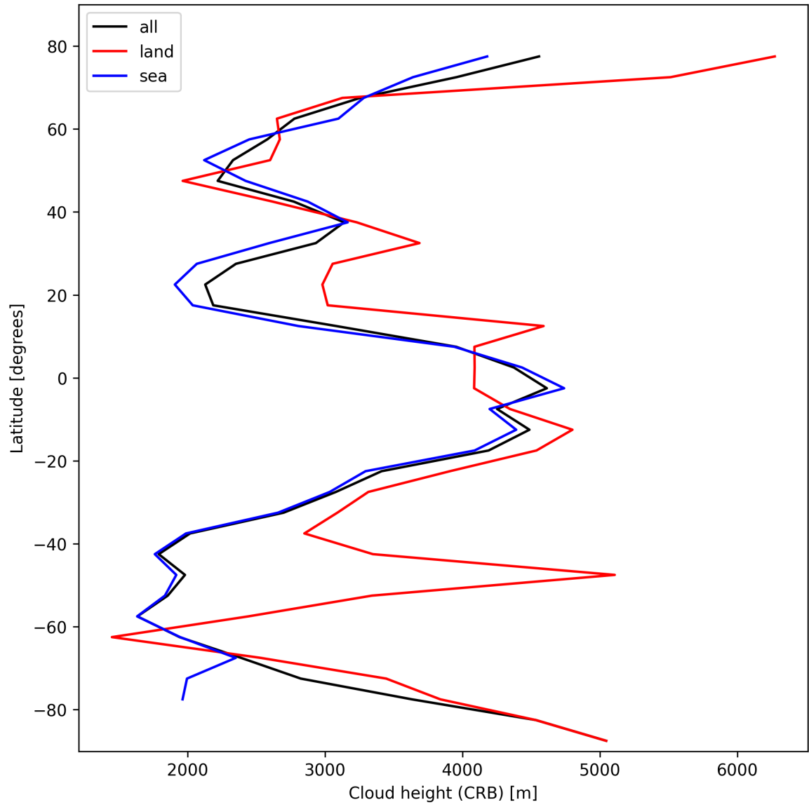
Figure 27: Zonal average of “Cloud height (CRB)” for 2025-02-19 to 2025-02-21.
