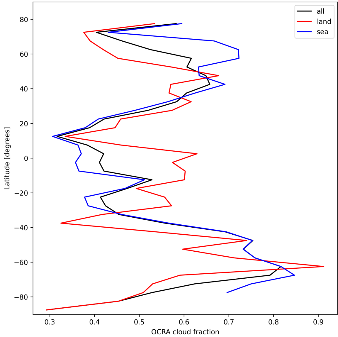
Figure 34: Zonal average of “OCRA cloud fraction” for 2025-02-19 to 2025-02-21.
