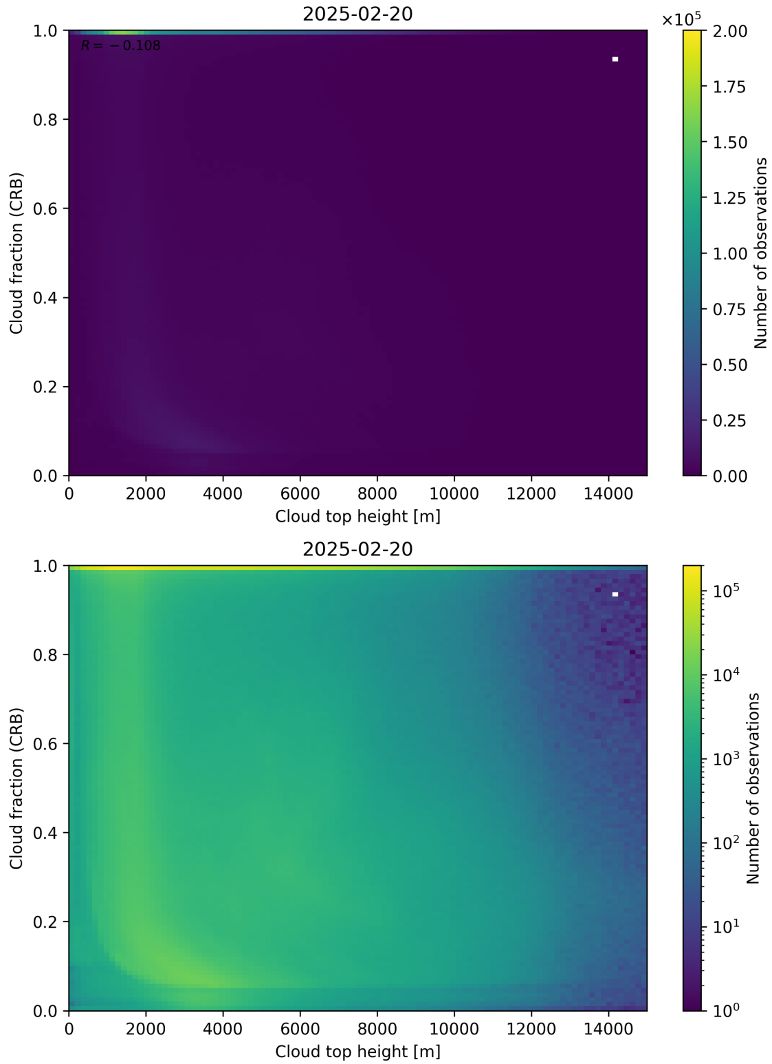
Figure 88: Scatter density plot of “Cloud top height” against “Cloud fraction (CRB)” for 2025-02-19 to 2025-02-21.
