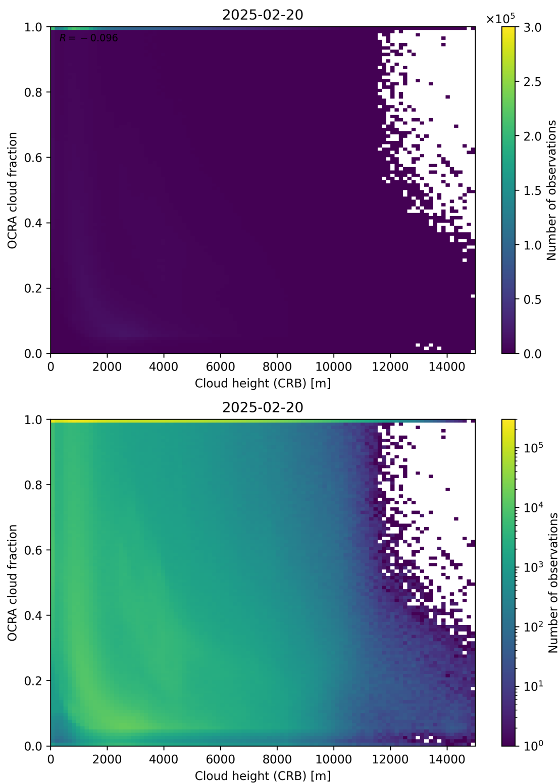
Figure 81: Scatter density plot of “Cloud height (CRB)” against “OCRA cloud fraction” for 2025-02-19 to 2025-02-21.
