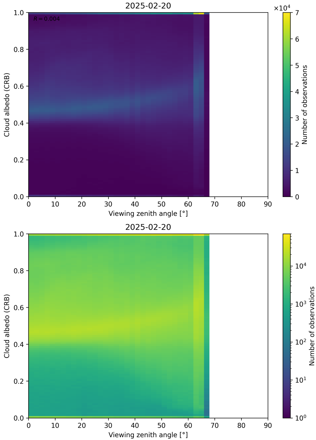
Figure 106: Scatter density plot of “Viewing zenith angle” against “Cloud albedo (CRB)” for 2025-02-19 to 2025-02-21.
