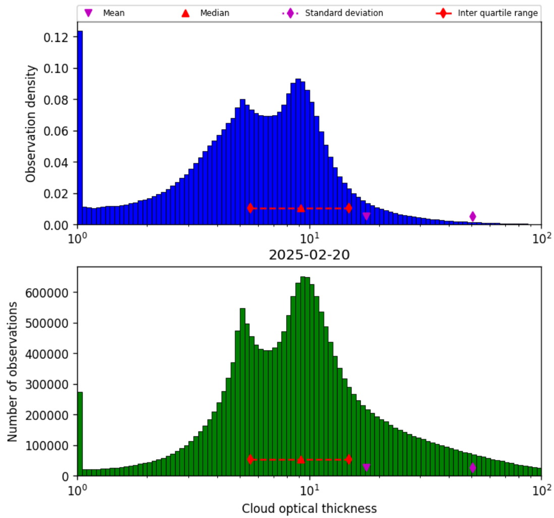
Figure 41: Histogram of “Cloud optical thickness” for 2025-02-19 to 2025-02-21
