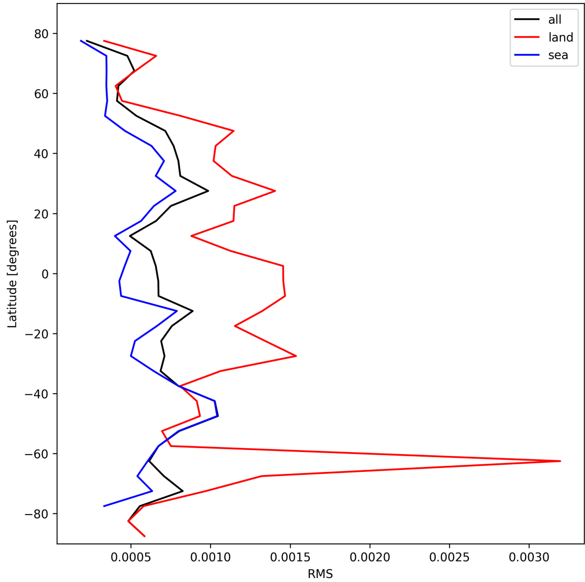
Figure 31: Zonal average of “RMS” for 2025-02-19 to 2025-02-21.
