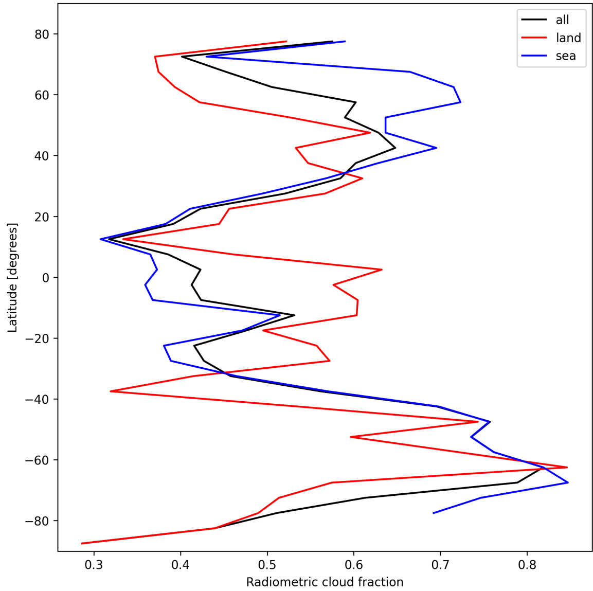
Figure 23: Zonal average of “Radiometric cloud fraction” for 2025-02-19 to 2025-02-21.
