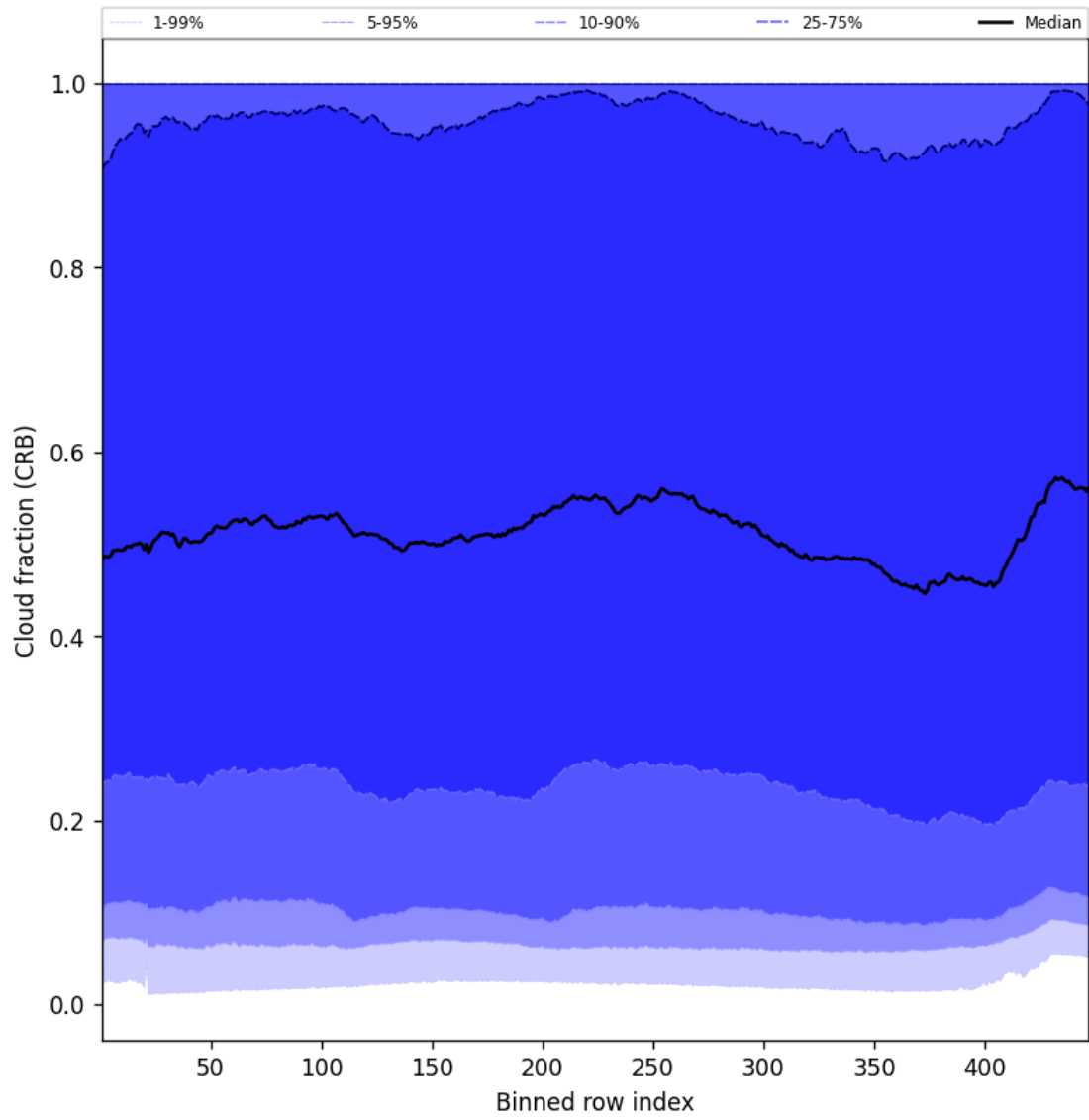
Figure 58: Along track statistics of “Cloud fraction (CRB)” for 2025-02-19 to 2025-02-21
