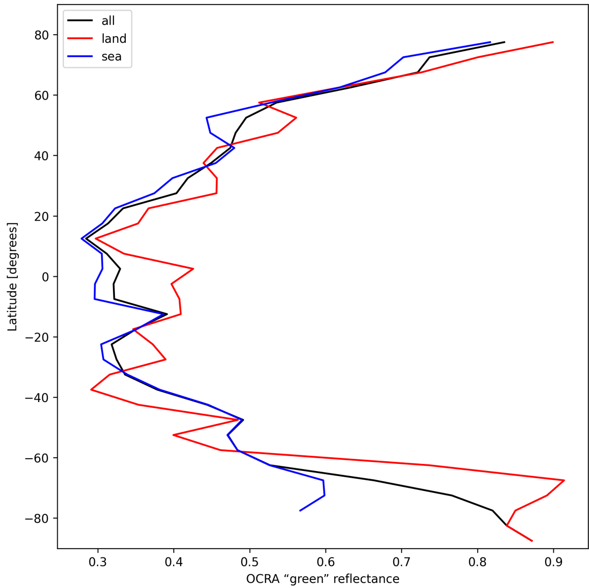
Figure 36: Zonal average of “OCRA “green” reflectance” for 2025-02-19 to 2025-02-21.
