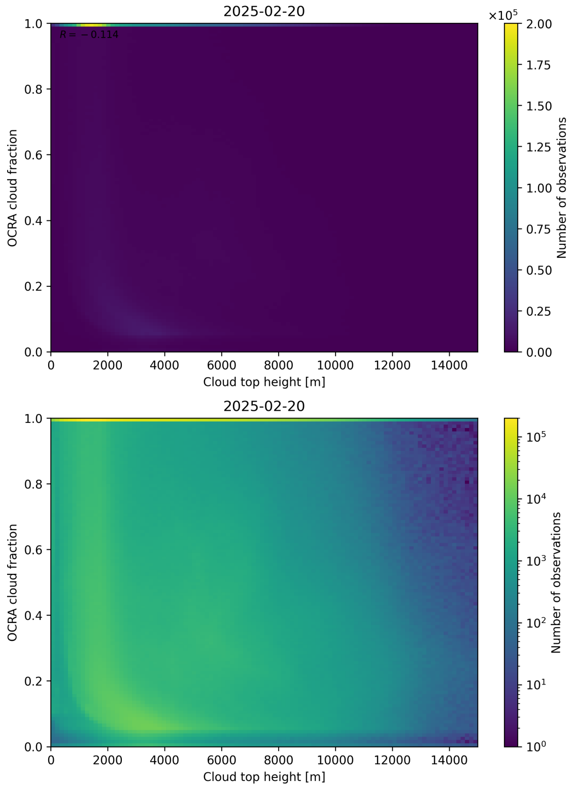
Figure 87: Scatter density plot of “Cloud top height” against “OCRA cloud fraction” for 2025-02-19 to 2025-02-21.
