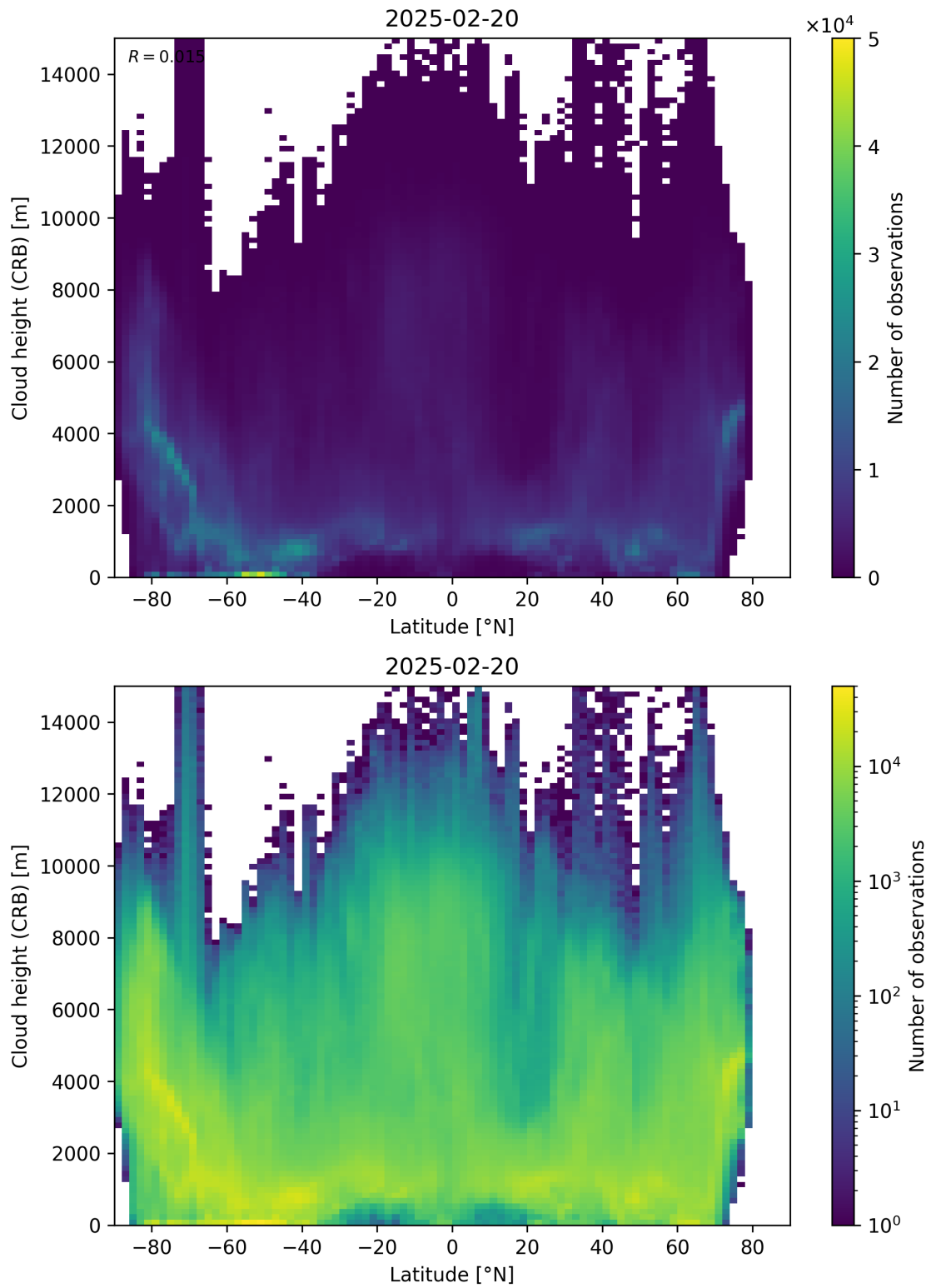
Figure 95: Scatter density plot of “Latitude” against “Cloud height (CRB)” for 2025-02-19 to 2025-02-21.
