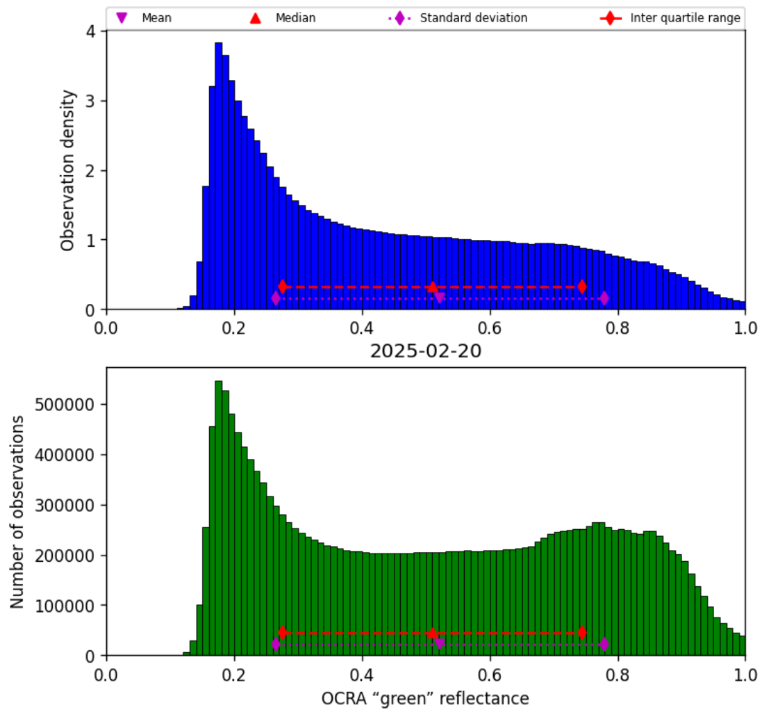
Figure 52: Histogram of “OCRA “green” reflectance” for 2025-02-19 to 2025-02-21
