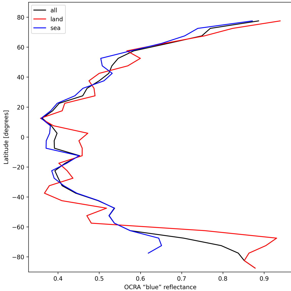
Figure 35: Zonal average of “OCRA “blue” reflectance” for 2025-02-19 to 2025-02-21.
