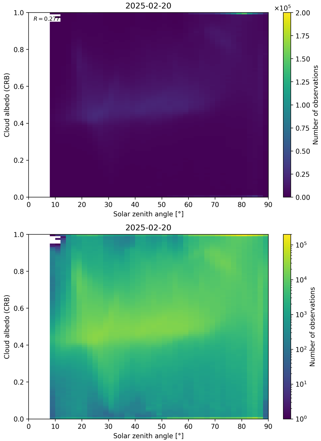
Figure 98: Scatter density plot of “Solar zenith angle” against “Cloud albedo (CRB)” for 2025-02-19 to 2025-02-21.
