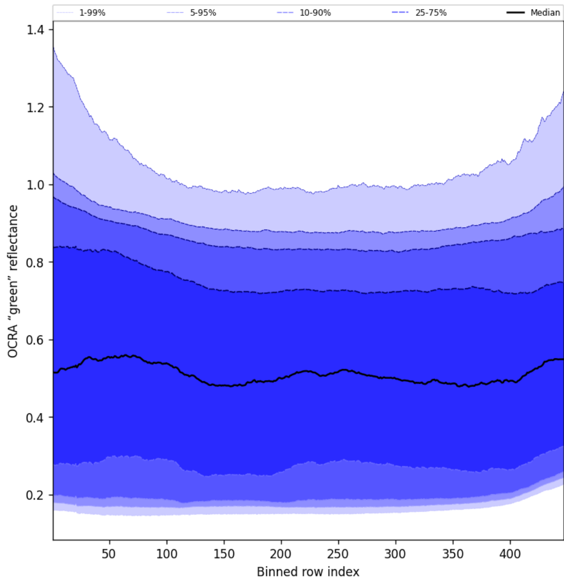
Figure 68: Along track statistics of "OCRA "green" reflectance" for 2025-02-19 to 2025-02-21
