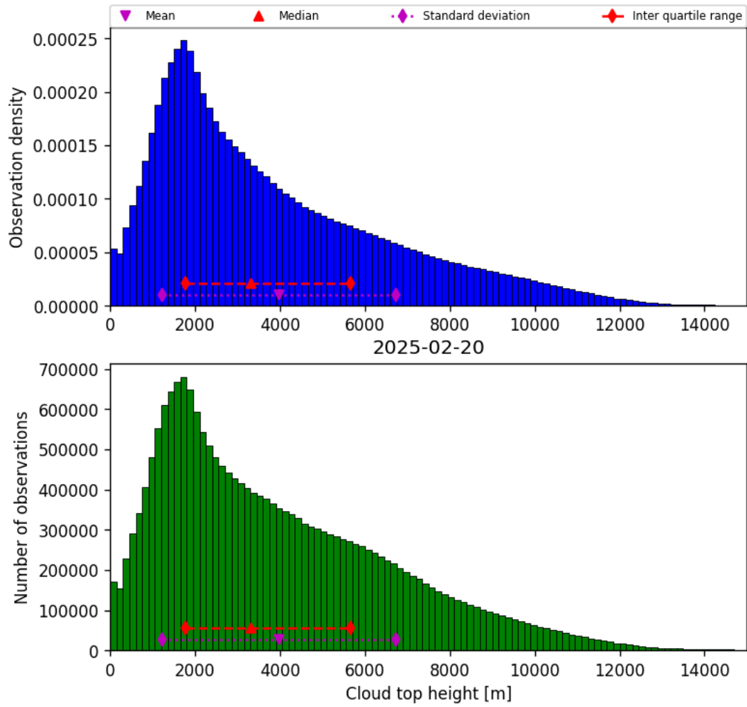
Figure 40: Histogram of “Cloud top height” for 2025-02-19 to 2025-02-21
