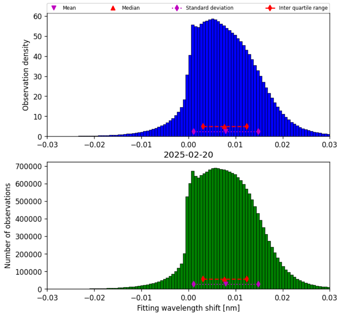
Figure 49: Histogram of “Fitting wavelength shift” for 2025-02-19 to 2025-02-21
