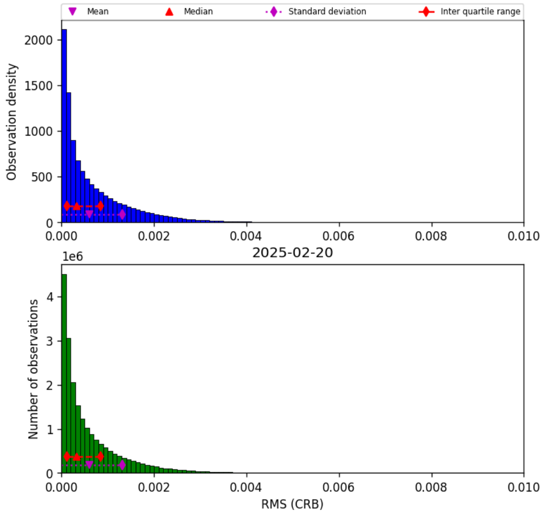
Figure 48: Histogram of “RMS (CRB)” for 2025-02-19 to 2025-02-21
