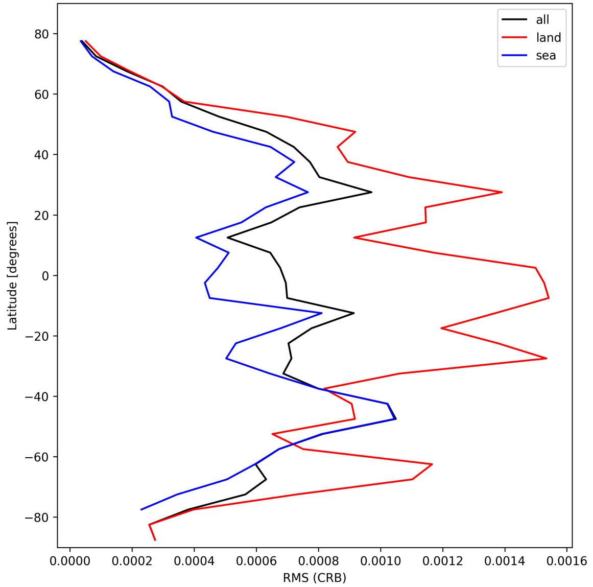
Figure 32: Zonal average of “RMS (CRB)” for 2025-02-19 to 2025-02-21.
