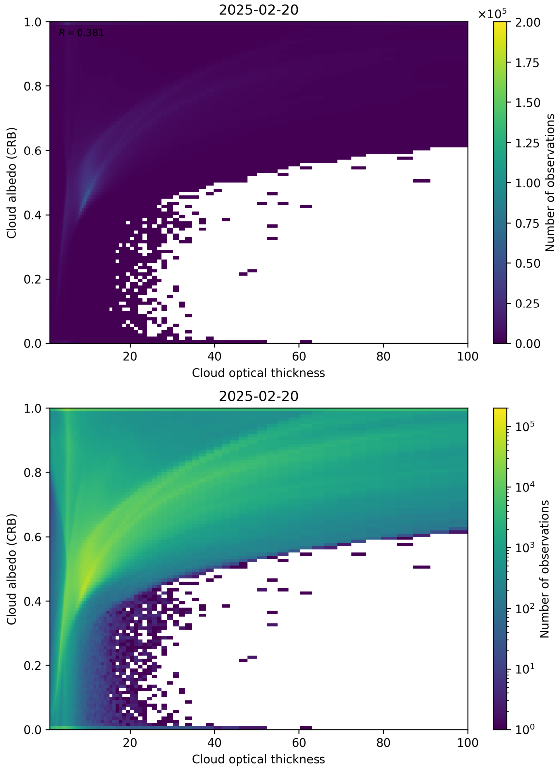
Figure 82: Scatter density plot of “Cloud optical thickness” against “Cloud albedo (CRB)” for 2025-02-19 to 2025-02-21.
