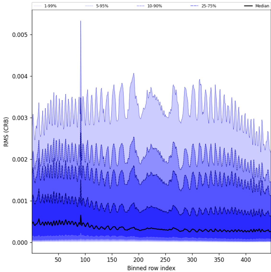
Figure 64: Along track statistics of “RMS (CRB)” for 2025-02-19 to 2025-02-21
