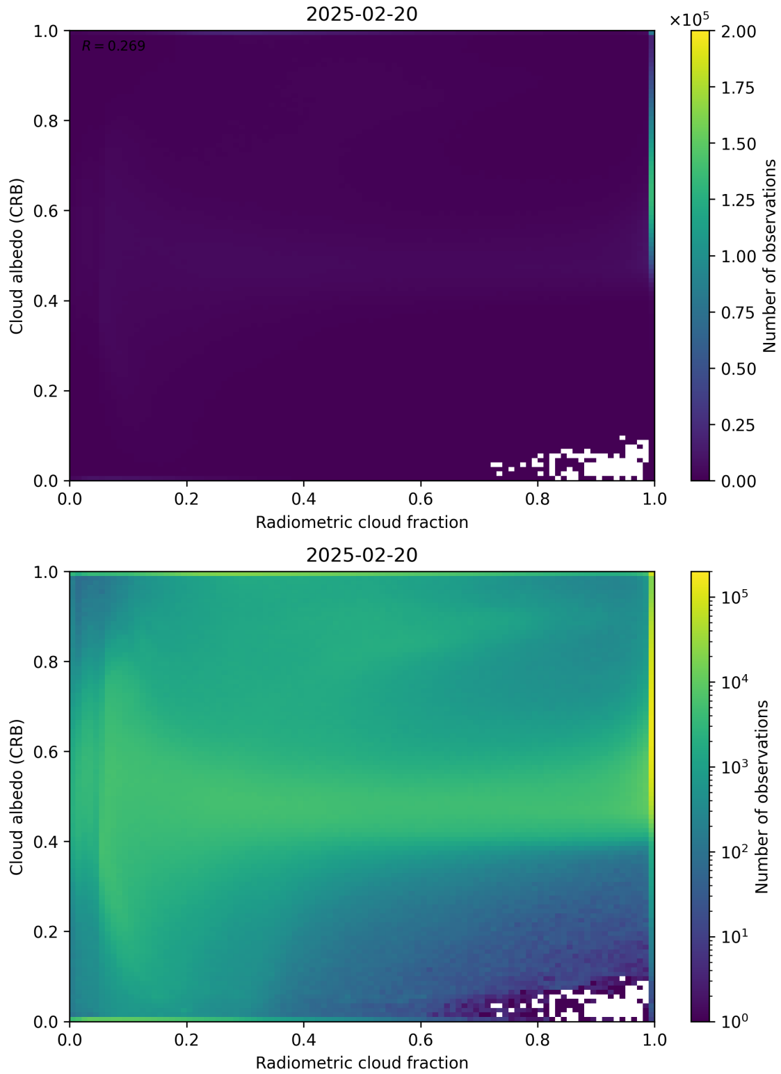
Figure 71: Scatter density plot of “Radiometric cloud fraction” against “Cloud albedo (CRB)” for 2025-02-19 to 2025-02-21.
