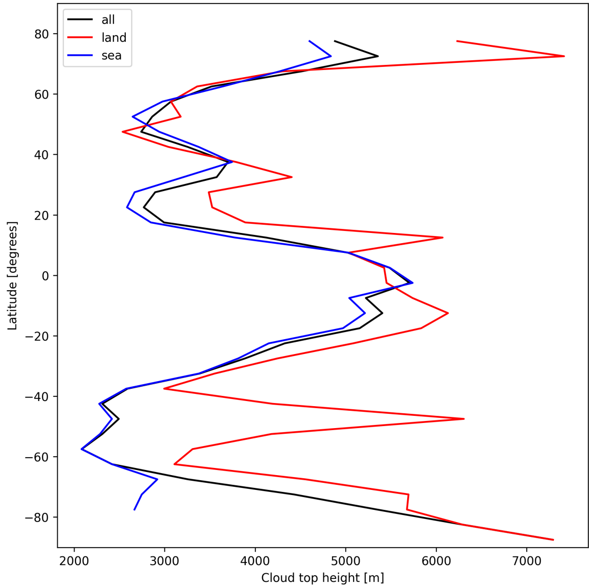
Figure 24: Zonal average of “Cloud top height” for 2025-02-19 to 2025-02-21.
