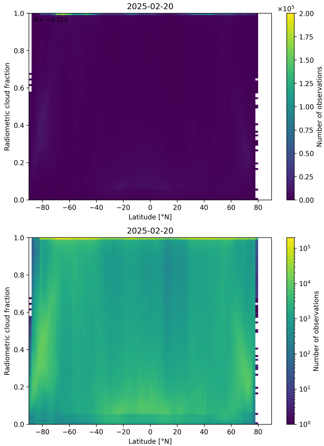
Figure 92: Scatter density plot of “Latitude” against “Radiometric cloud fraction” for 2025-02-19 to 2025-02-21.
