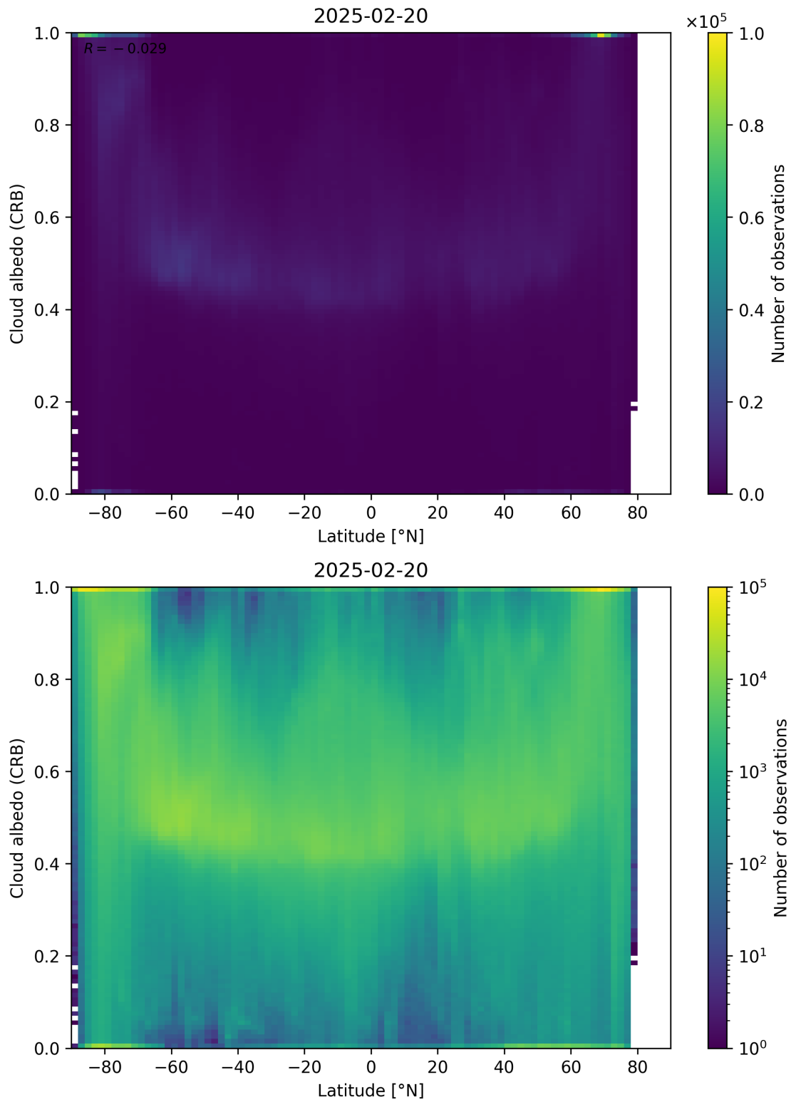
Figure 91: Scatter density plot of “Latitude” against “Cloud albedo (CRB)” for 2025-02-19 to 2025-02-21.
