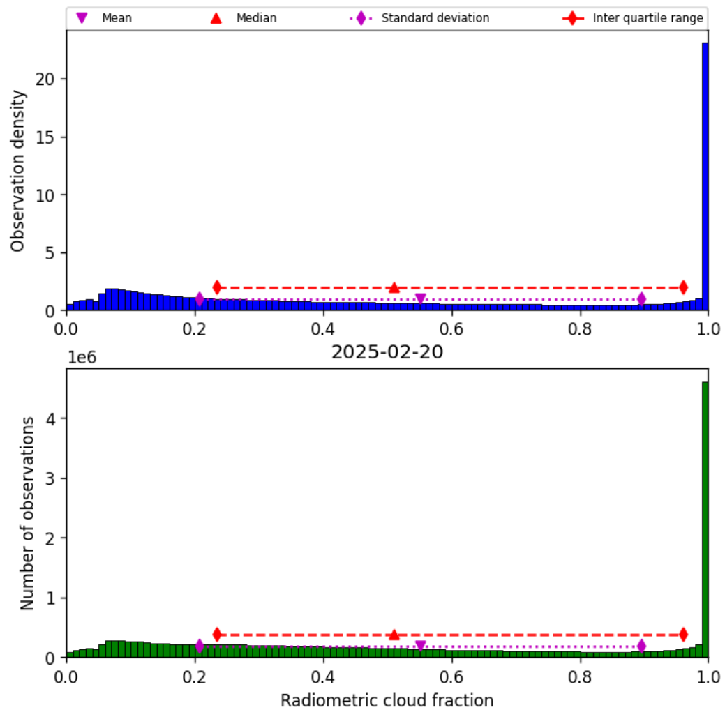
Figure 39: Histogram of “Radiometric cloud fraction” for 2025-02-19 to 2025-02-21
