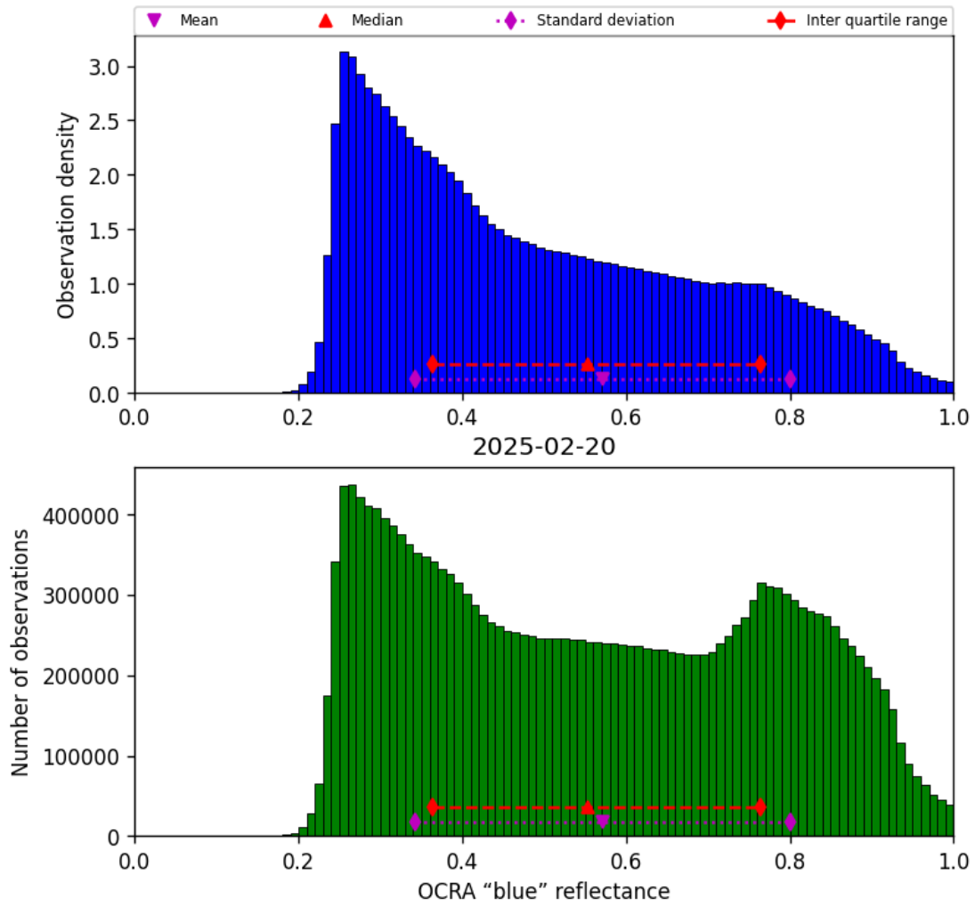
Figure 51: Histogram of “OCRA “blue” reflectance” for 2025-02-19 to 2025-02-21
