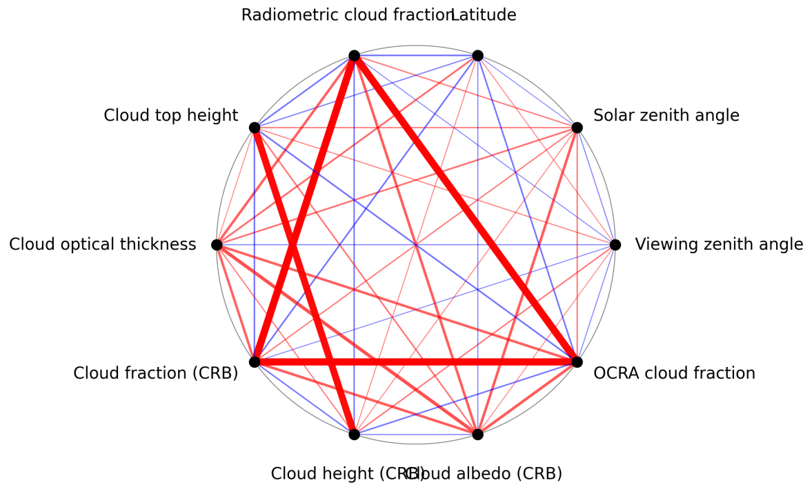
Figure 1: Map of correlation graph for 2025-02-19 to 2025-02-21.
