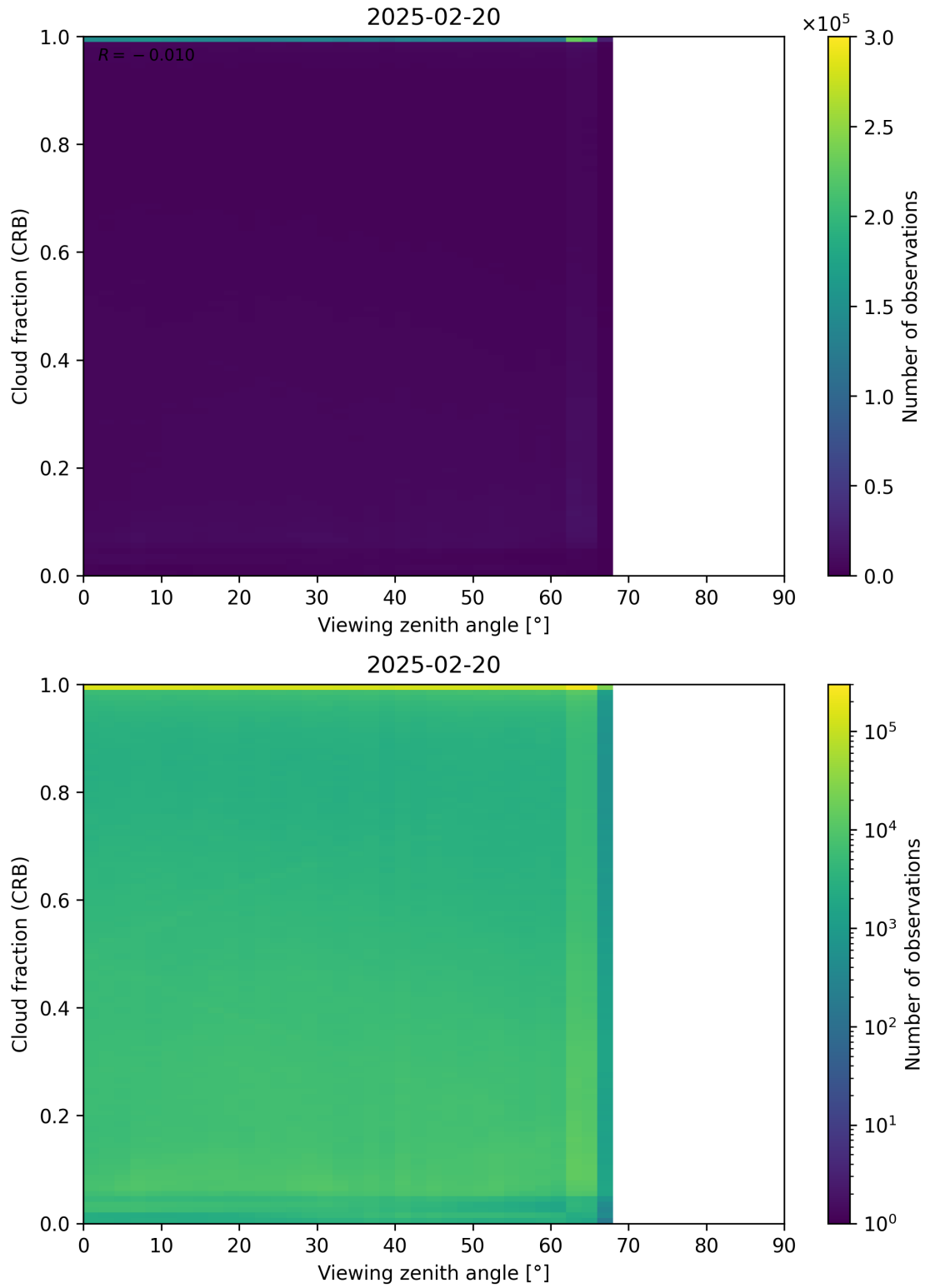
Figure 109: Scatter density plot of “Viewing zenith angle” against “Cloud fraction (CRB)” for 2025-02-19 to 2025-02-21.
