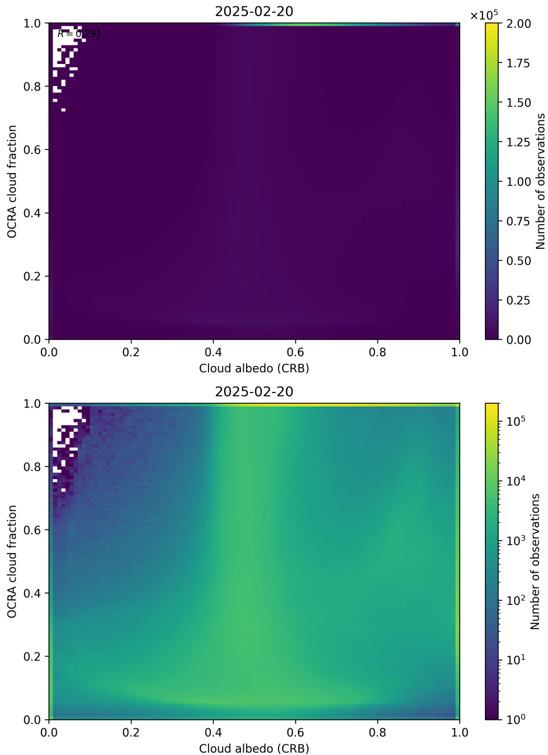
Figure 70: Scatter density plot of “Cloud albedo (CRB)” against “OCRA cloud fraction” for 2025-02-19 to 2025-02-21.
