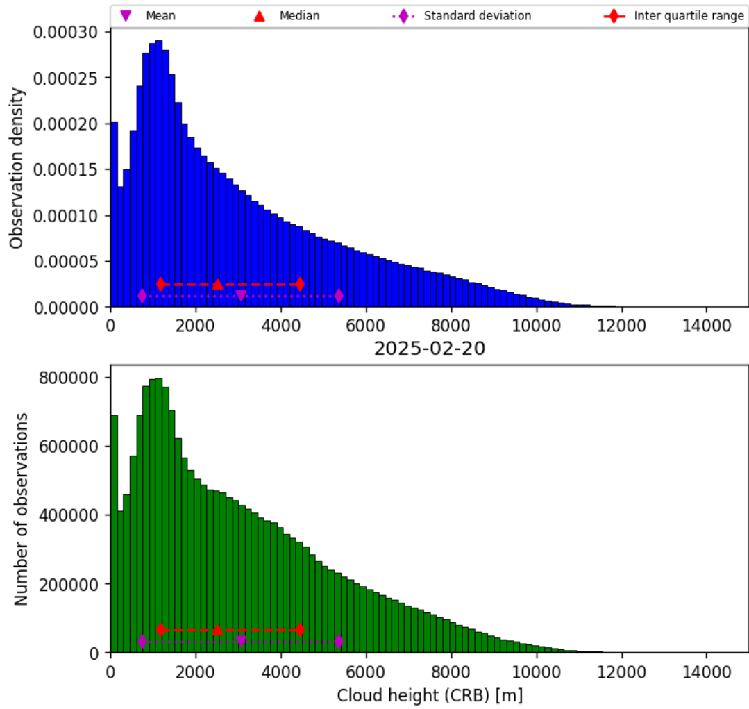
Figure 43: Histogram of “Cloud height (CRB)” for 2025-02-19 to 2025-02-21
