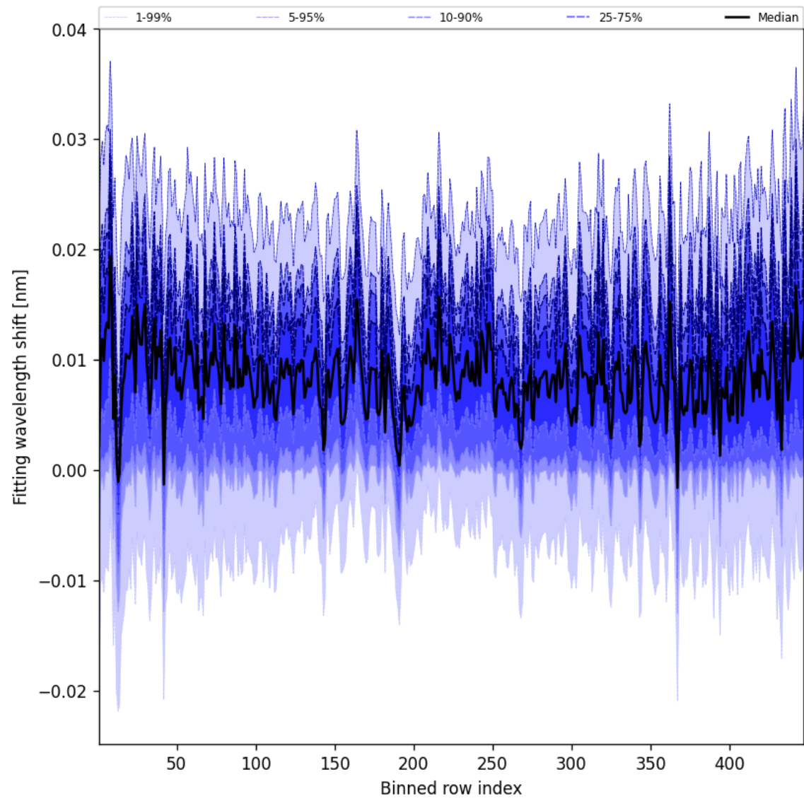
Figure 65: Along track statistics of “Fitting wavelength shift” for 2025-02-19 to 2025-02-21
