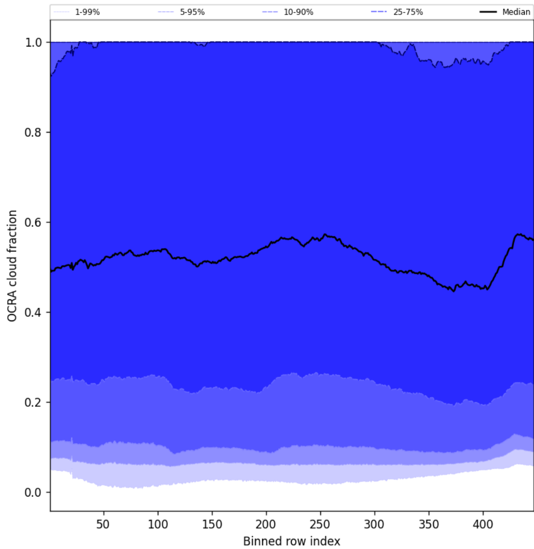
Figure 66: Along track statistics of “OCRA cloud fraction” for 2025-02-19 to 2025-02-21
