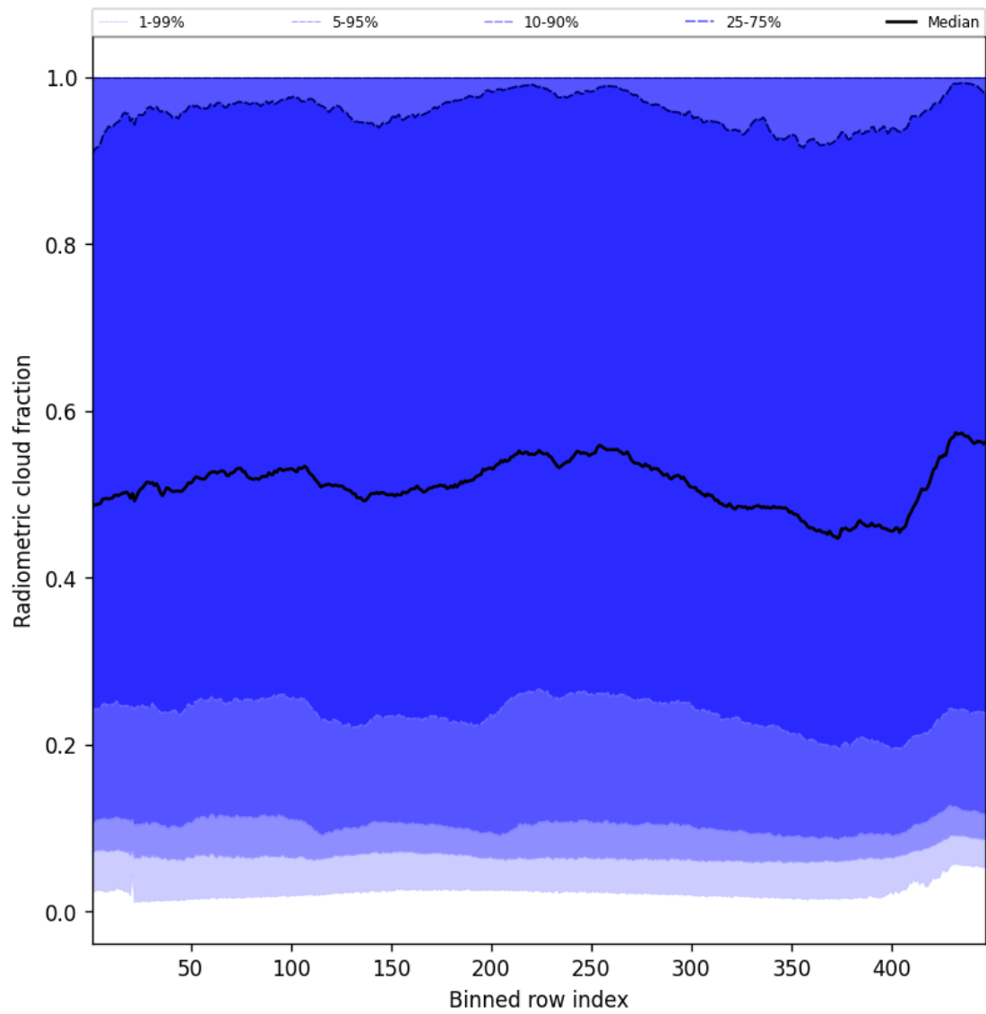
Figure 55: Along track statistics of “Radiometric cloud fraction” for 2025-02-19 to 2025-02-21
