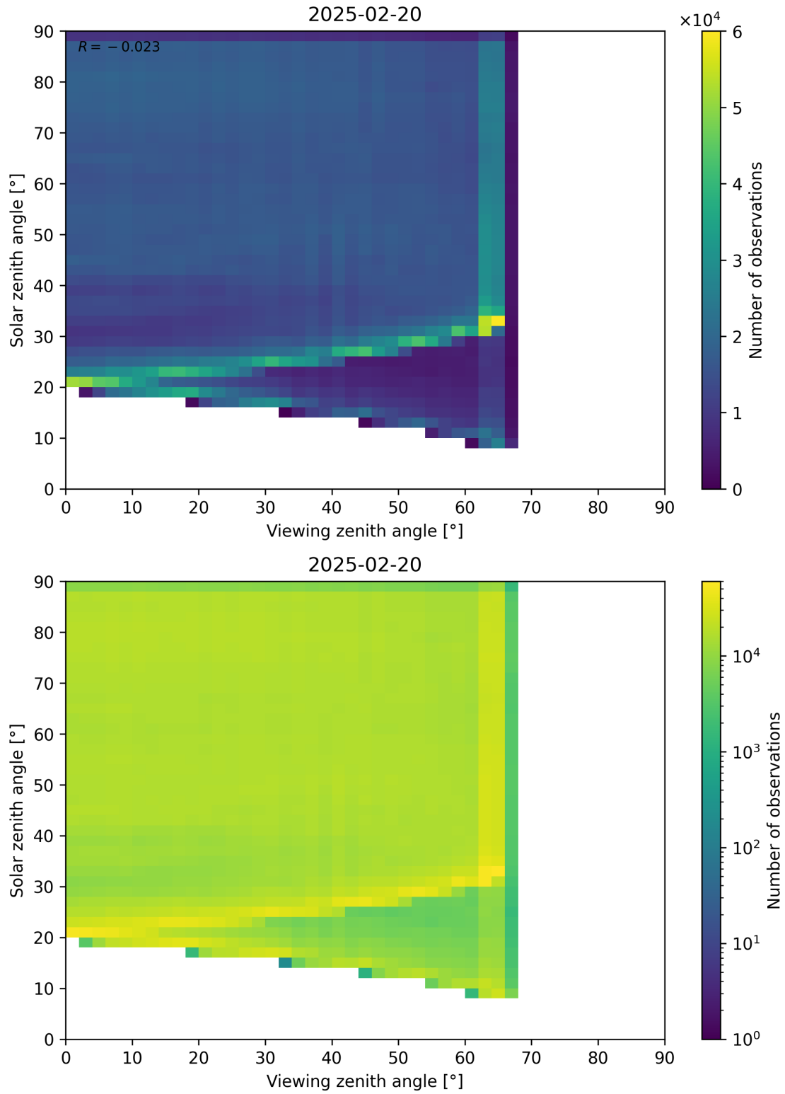
Figure 114: Scatter density plot of “Viewing zenith angle” against “Solar zenith angle” for 2025-02-19 to 2025-02-21.
