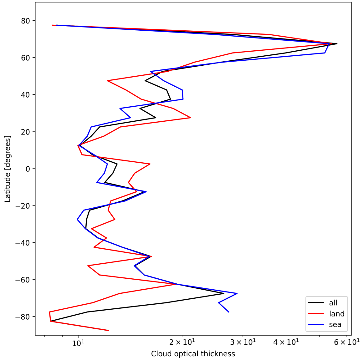
Figure 25: Zonal average of “Cloud optical thickness” for 2025-02-19 to 2025-02-21.
