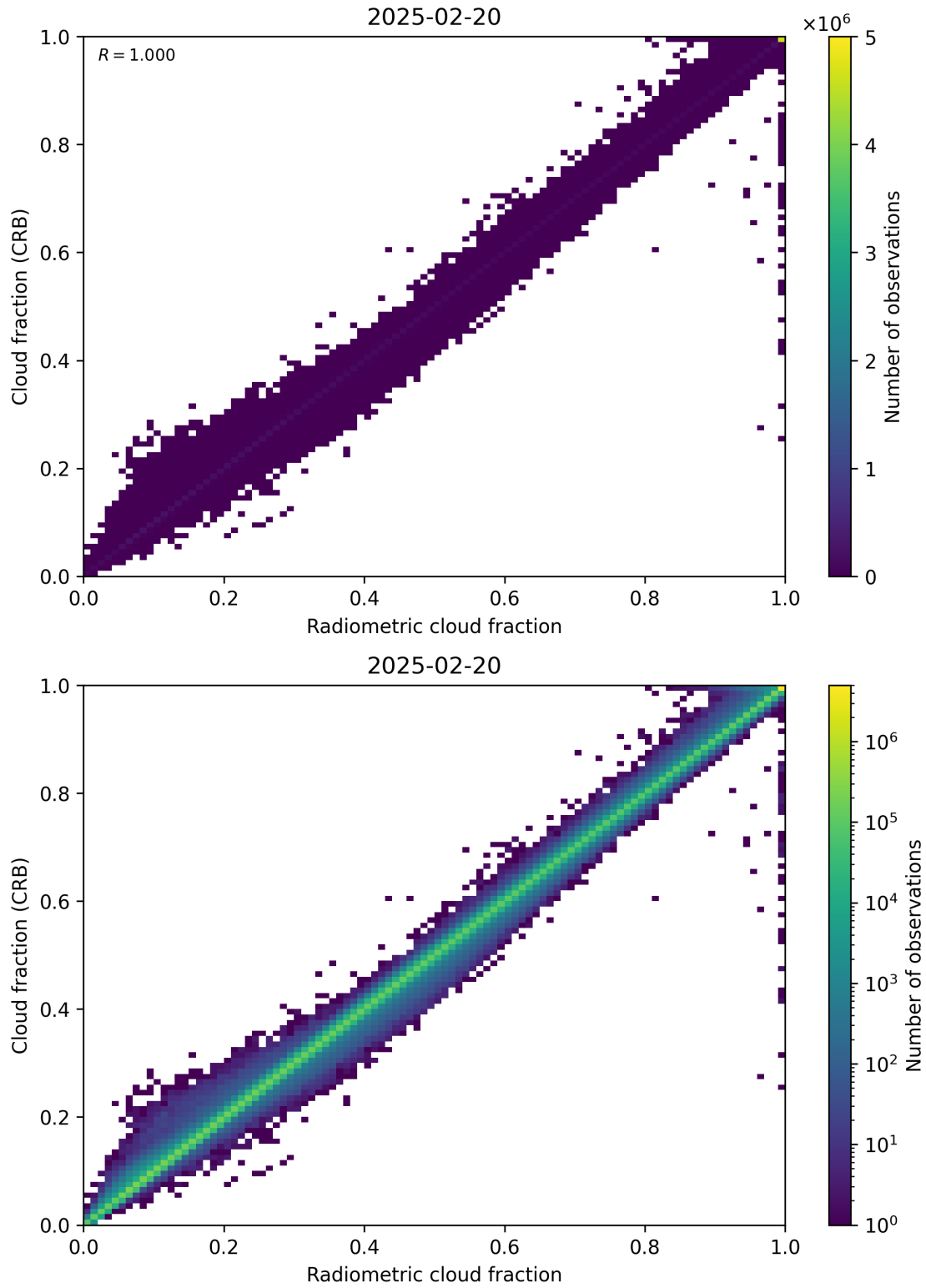
Figure 73: Scatter density plot of “Radiometric cloud fraction” against “Cloud fraction (CRB)” for 2025-02-19 to 2025-02-21.
