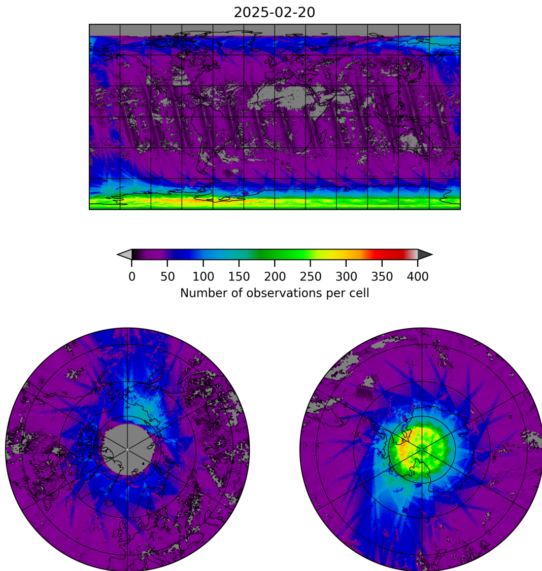
Figure 21: Map of the number of observations for 2025-02-19 to 2025-02-21
