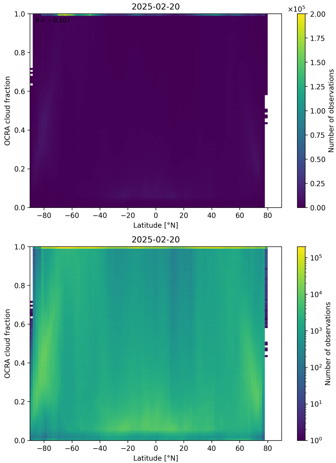
Figure 93: Scatter density plot of “Latitude” against “OCRA cloud fraction” for 2025-02-19 to 2025-02-21.
