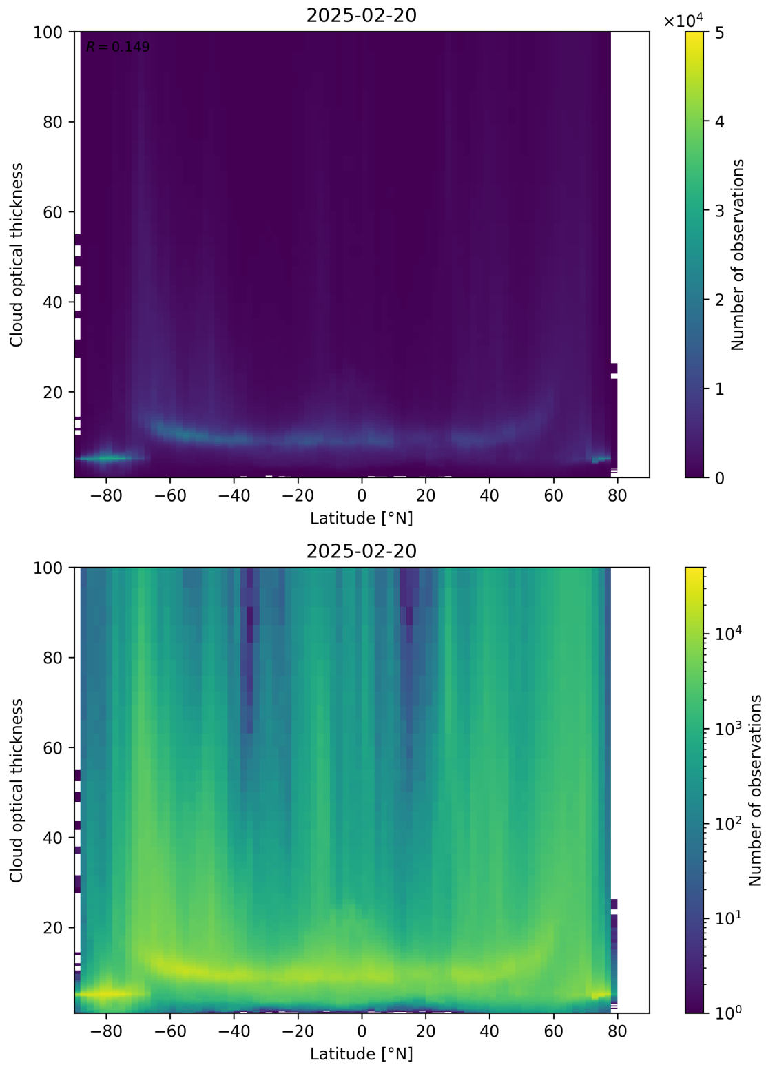
Figure 96: Scatter density plot of “Latitude” against “Cloud optical thickness” for 2025-02-19 to 2025-02-21.
