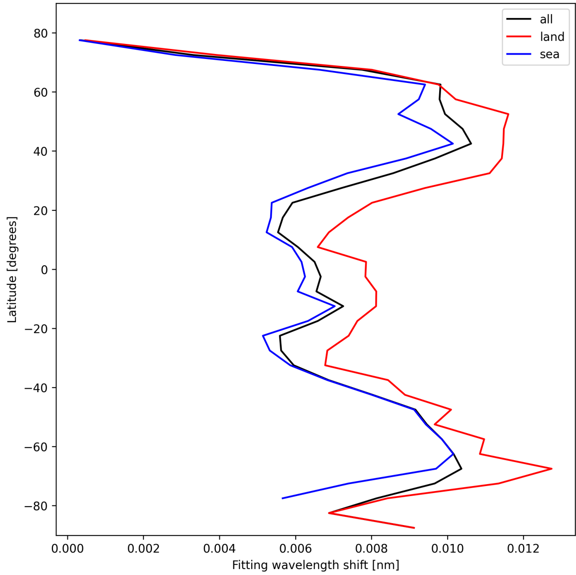
Figure 33: Zonal average of “Fitting wavelength shift” for 2025-02-19 to 2025-02-21.
