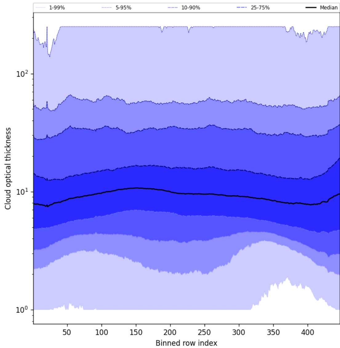
Figure 57: Along track statistics of “Cloud optical thickness” for 2025-02-19 to 2025-02-21
