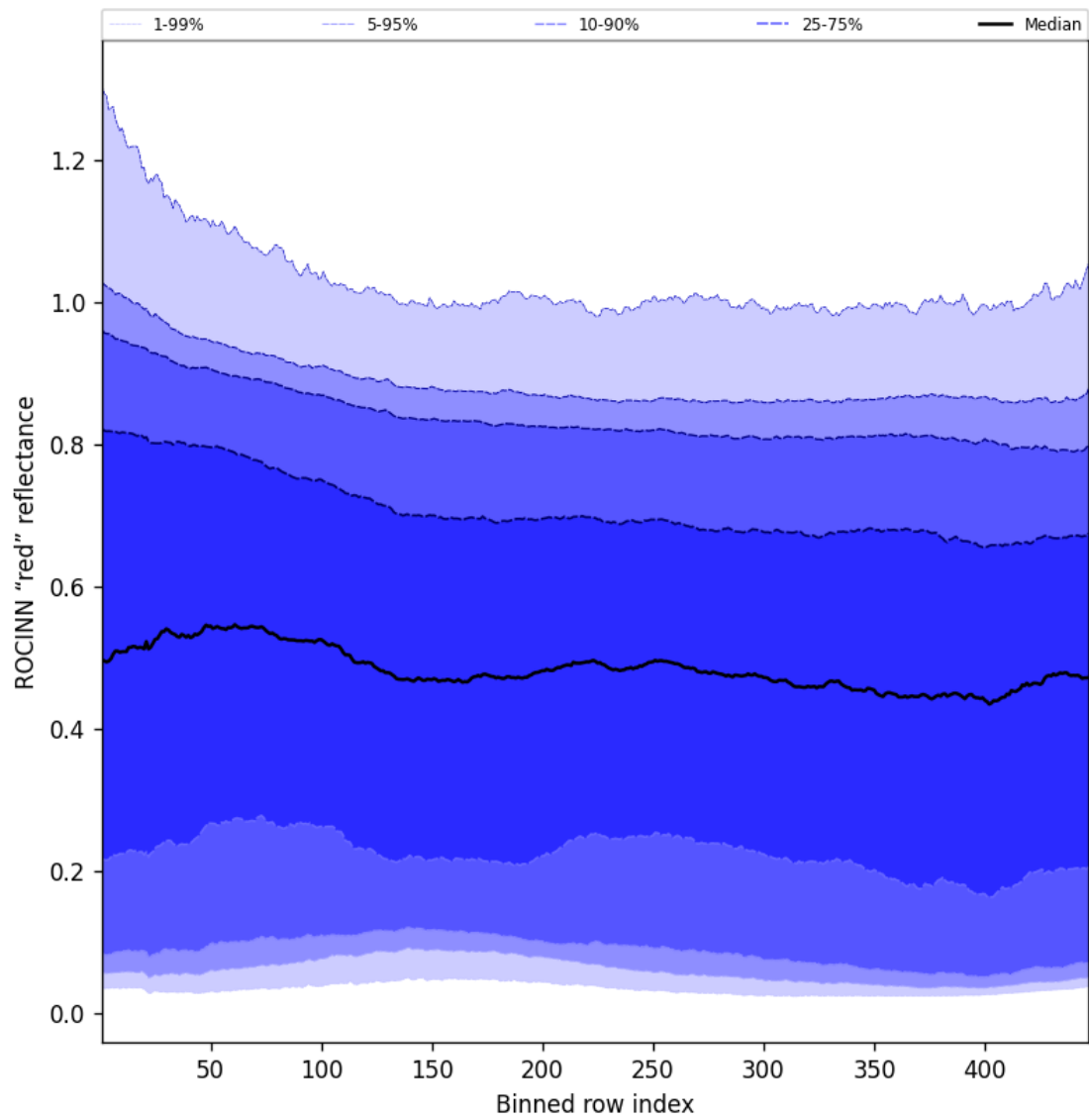
Figure 69: Along track statistics of “ROCINN “red” reflectance” for 2025-02-19 to 2025-02-21
