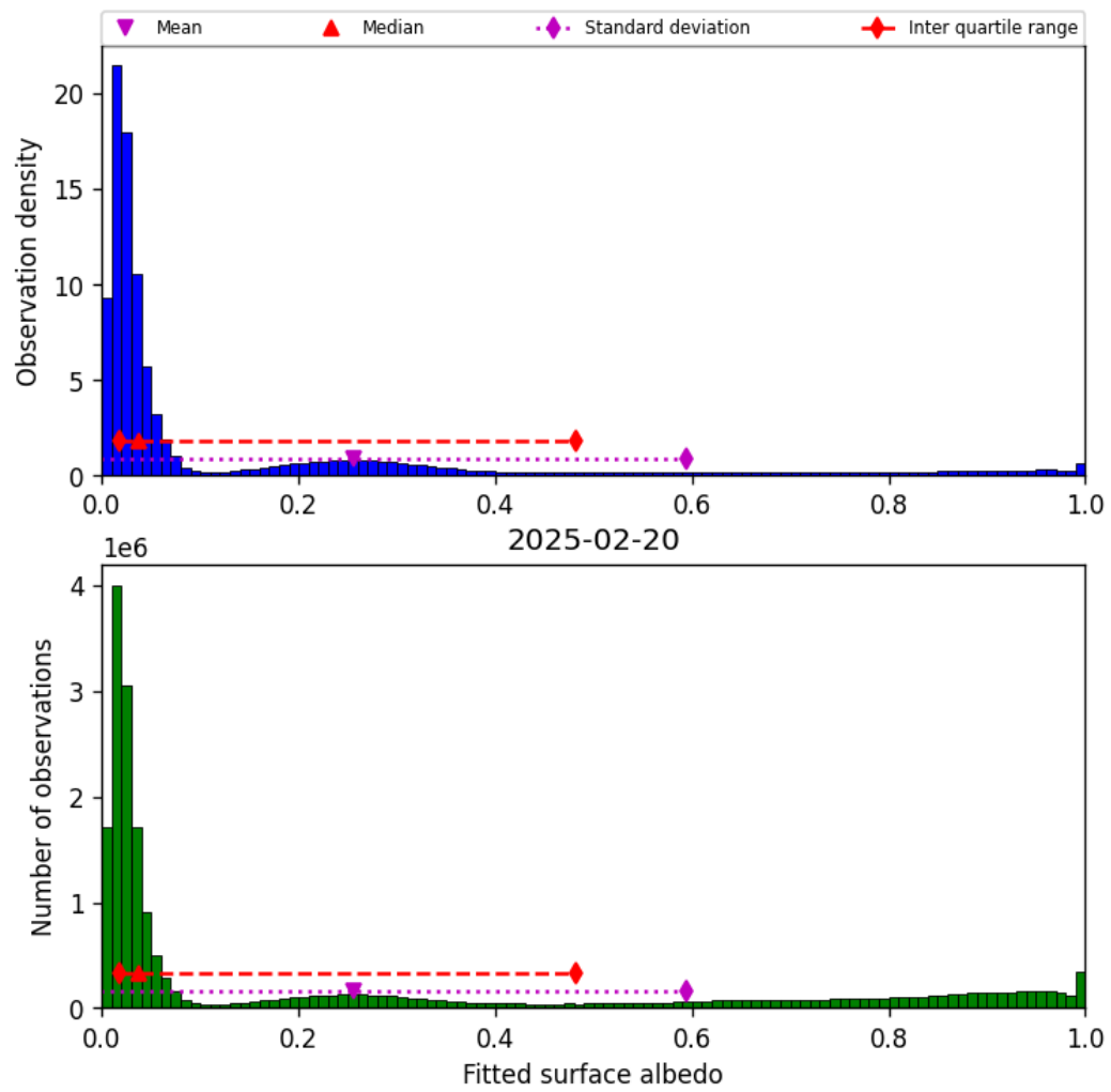
Figure 45: Histogram of “Fitted surface albedo” for 2025-02-19 to 2025-02-21
