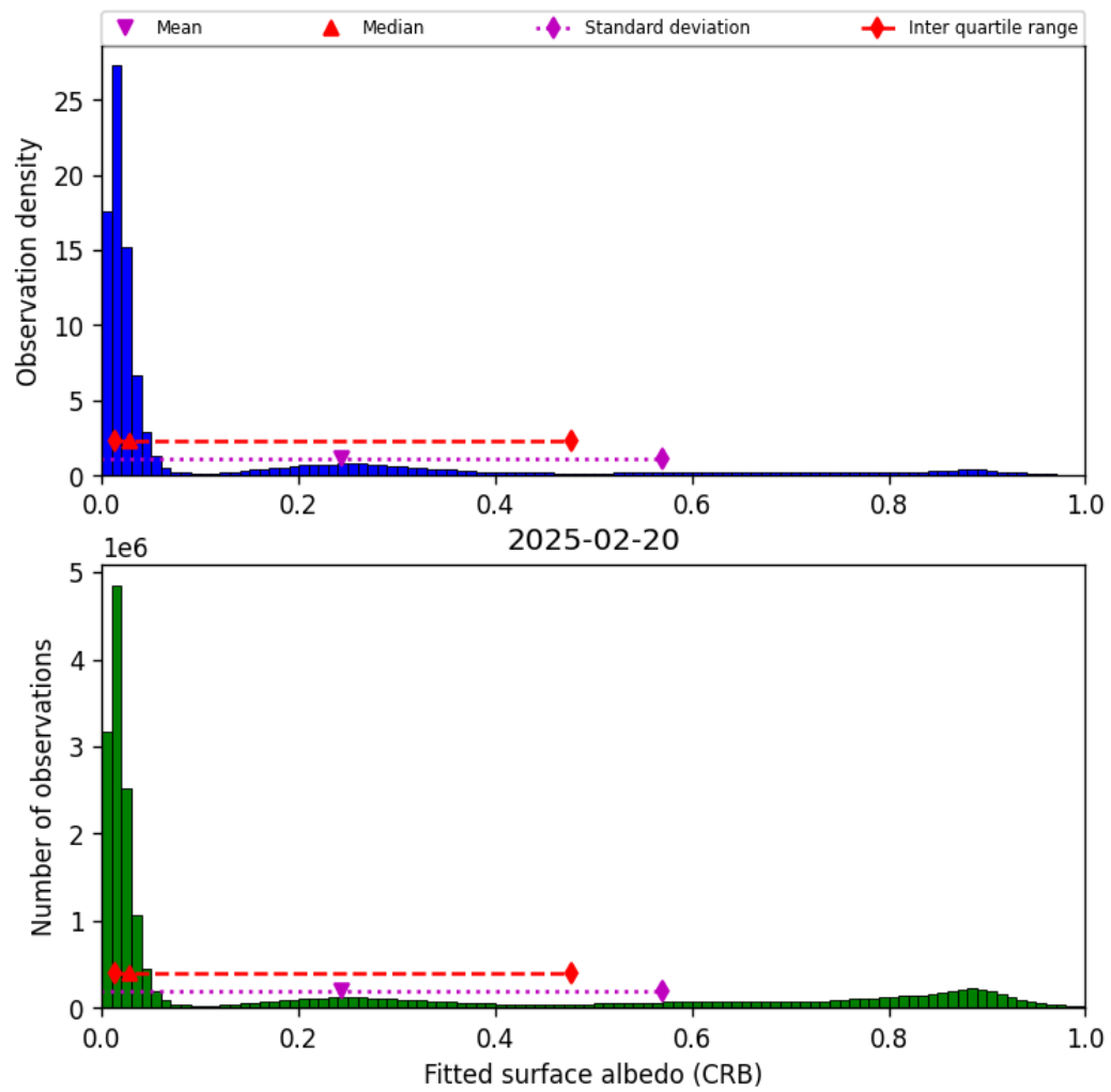
Figure 46: Histogram of “Fitted surface albedo (CRB)” for 2025-02-19 to 2025-02-21
