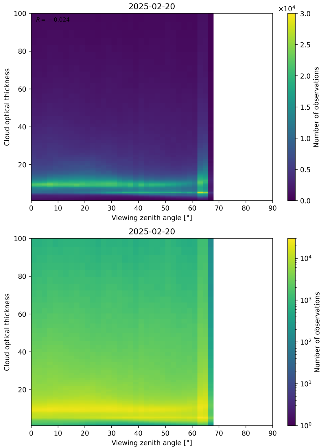
Figure 111: Scatter density plot of “Viewing zenith angle” against “Cloud optical thickness” for 2025-02-19 to 2025-02-21.
