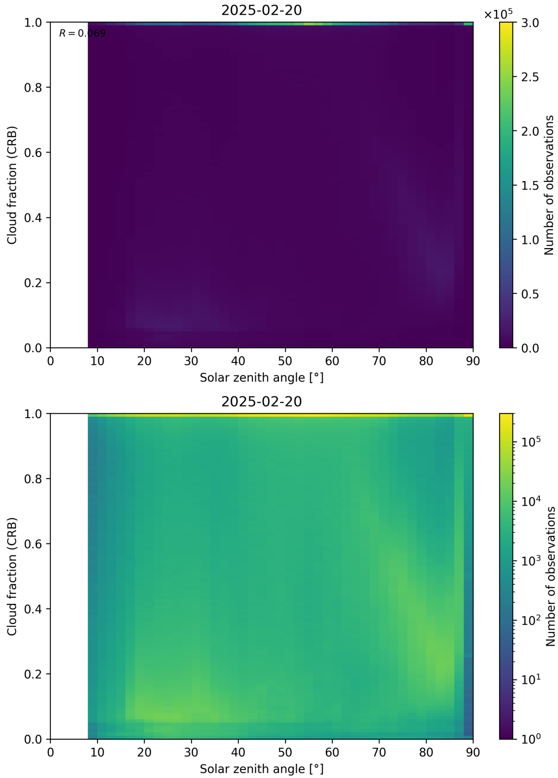
Figure 101: Scatter density plot of “Solar zenith angle” against “Cloud fraction (CRB)” for 2025-02-19 to 2025-02-21.
