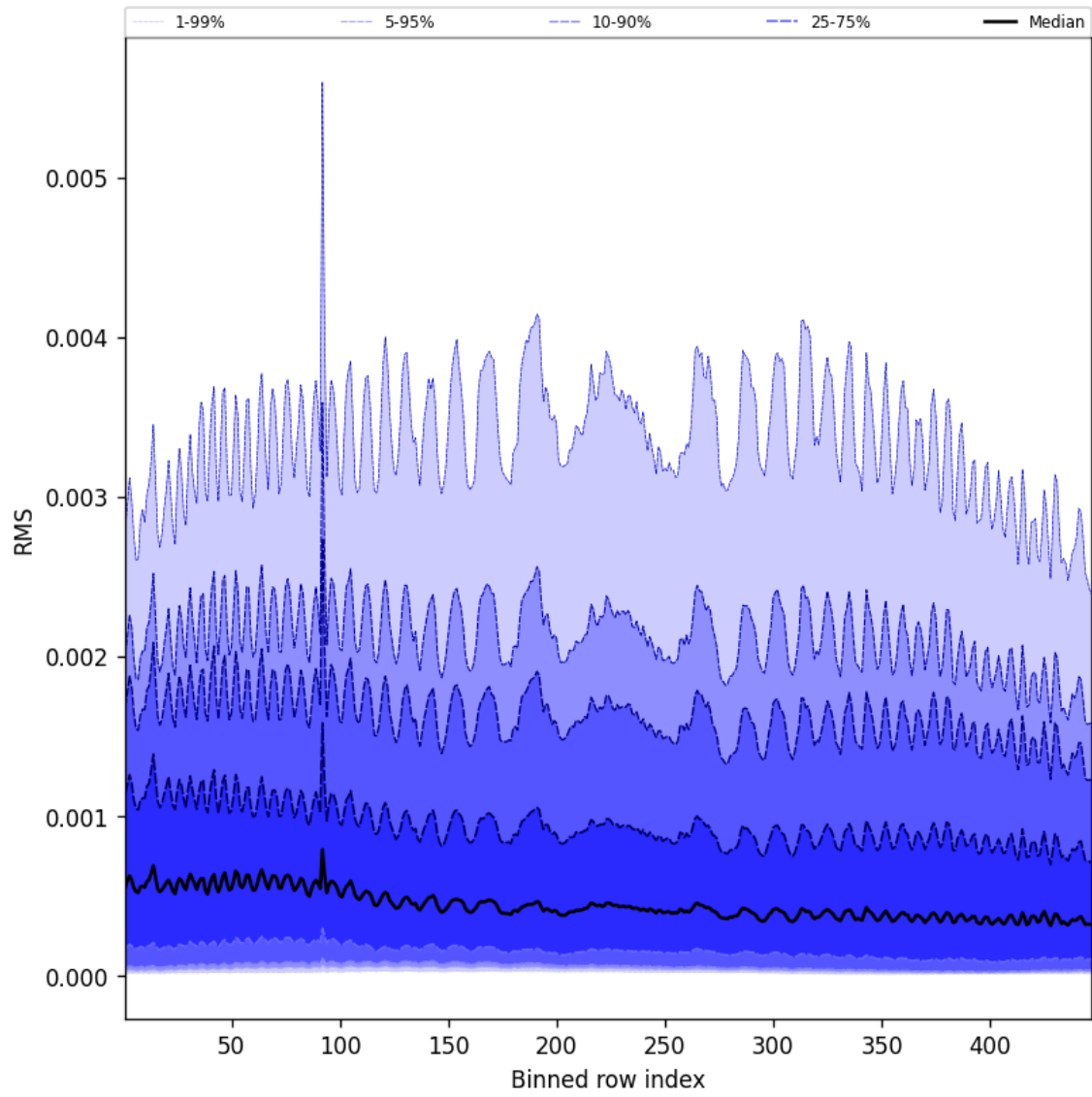
Figure 63: Along track statistics of “RMS” for 2025-02-19 to 2025-02-21
