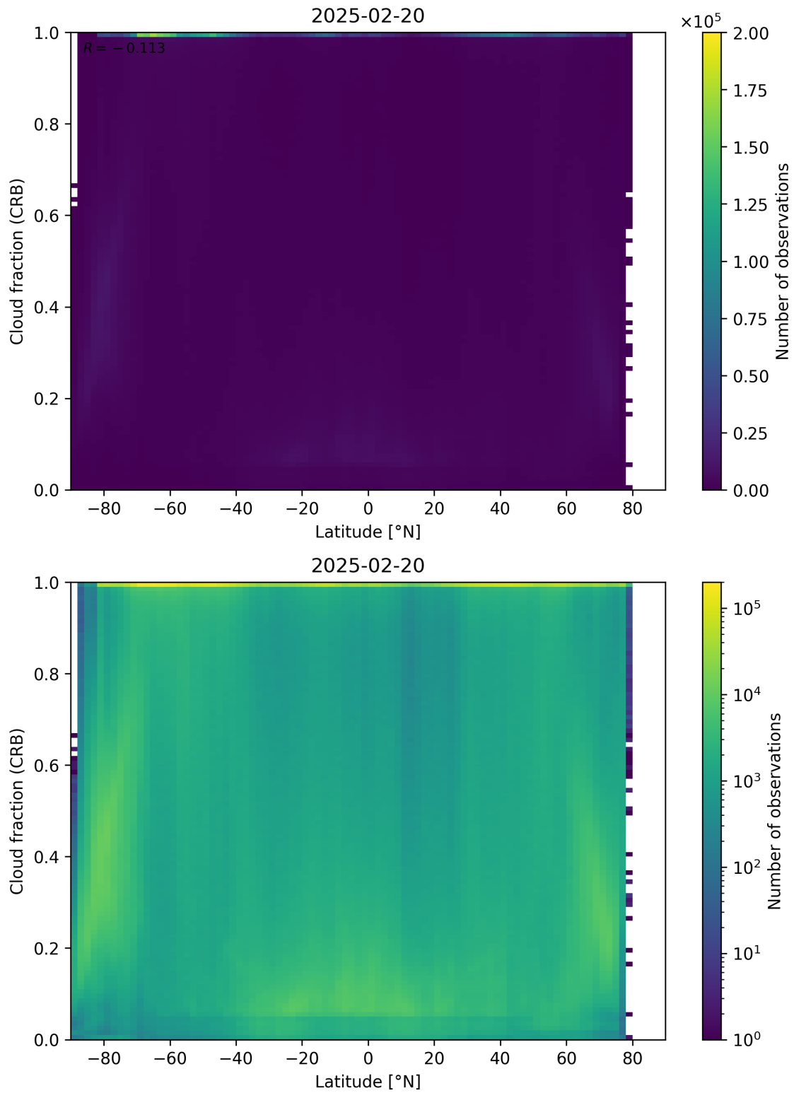
Figure 94: Scatter density plot of “Latitude” against “Cloud fraction (CRB)” for 2025-02-19 to 2025-02-21.
