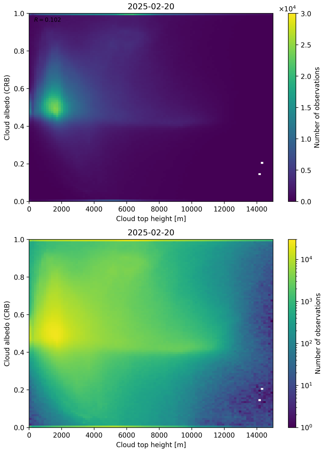
Figure 86: Scatter density plot of “Cloud top height” against “Cloud albedo (CRB)” for 2025-02-19 to 2025-02-21.
