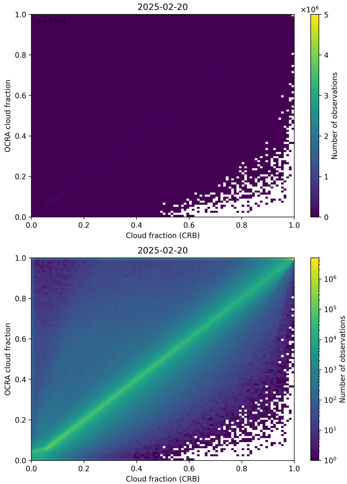
Figure 78: Scatter density plot of “Cloud fraction (CRB)” against “OCRA cloud fraction” for 2025-02-19 to 2025-02-21.
