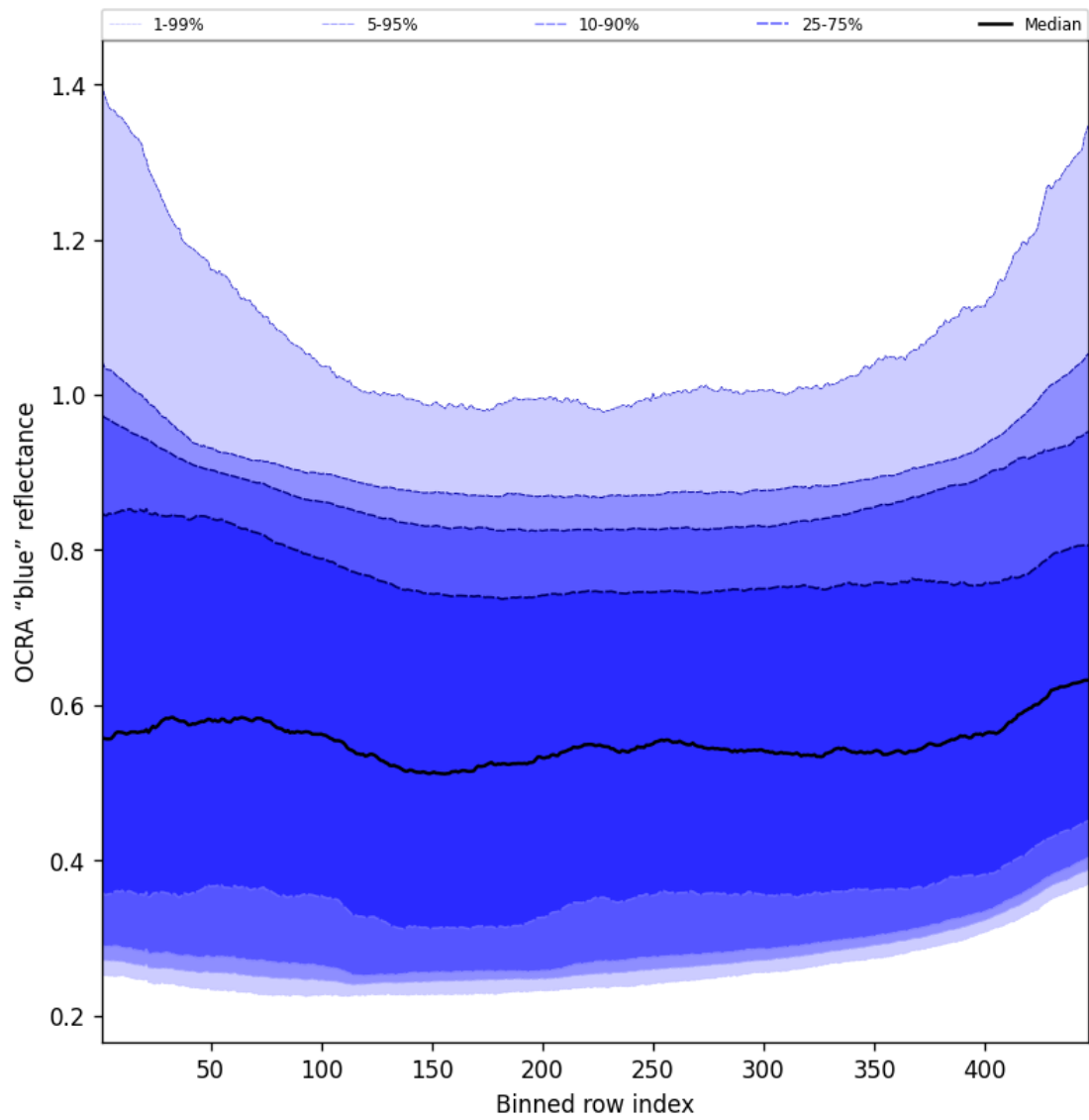
Figure 67: Along track statistics of “OCRA “blue” reflectance” for 2025-02-19 to 2025-02-21
