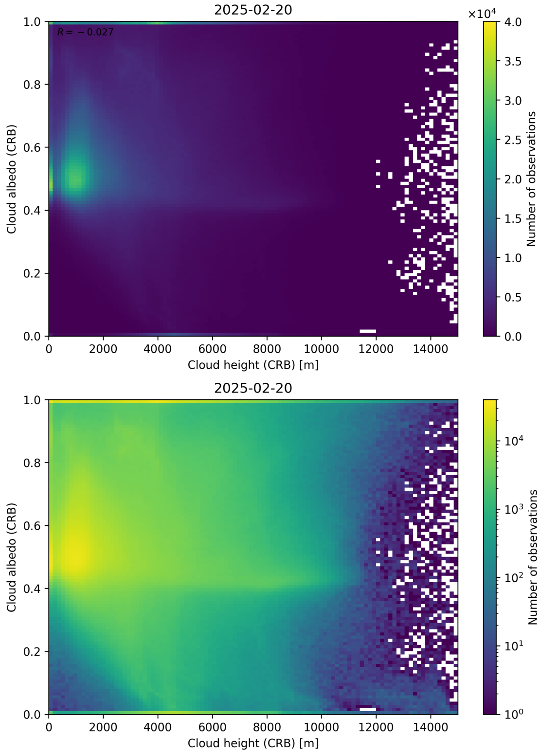
Figure 80: Scatter density plot of “Cloud height (CRB)” against “Cloud albedo (CRB)” for 2025-02-19 to 2025-02-21.
