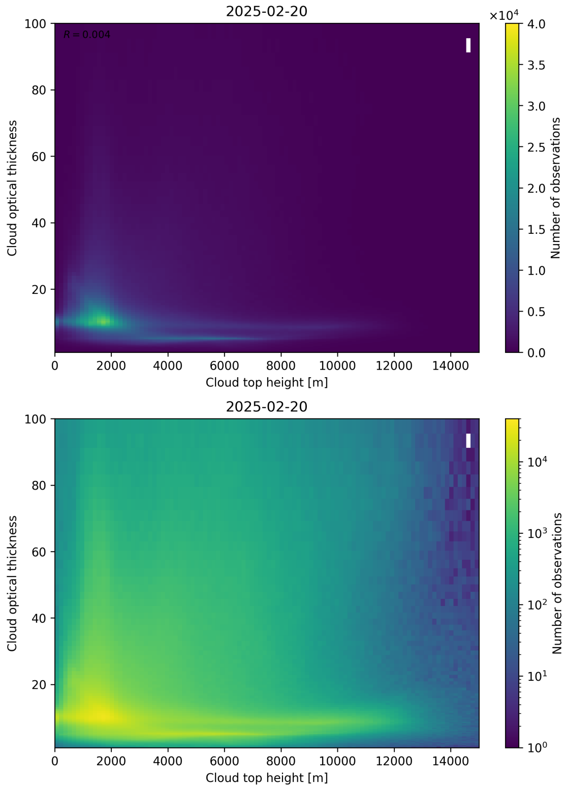
Figure 90: Scatter density plot of “Cloud top height” against “Cloud optical thickness” for 2025-02-19 to 2025-02-21.
