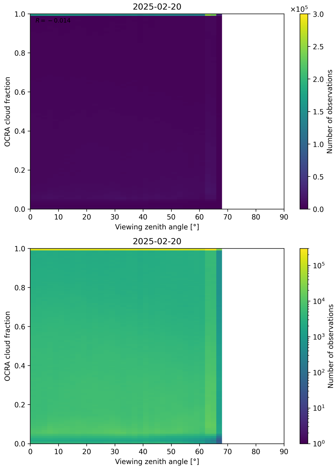
Figure 108: Scatter density plot of “Viewing zenith angle” against “OCRA cloud fraction” for 2025-02-19 to 2025-02-21.
