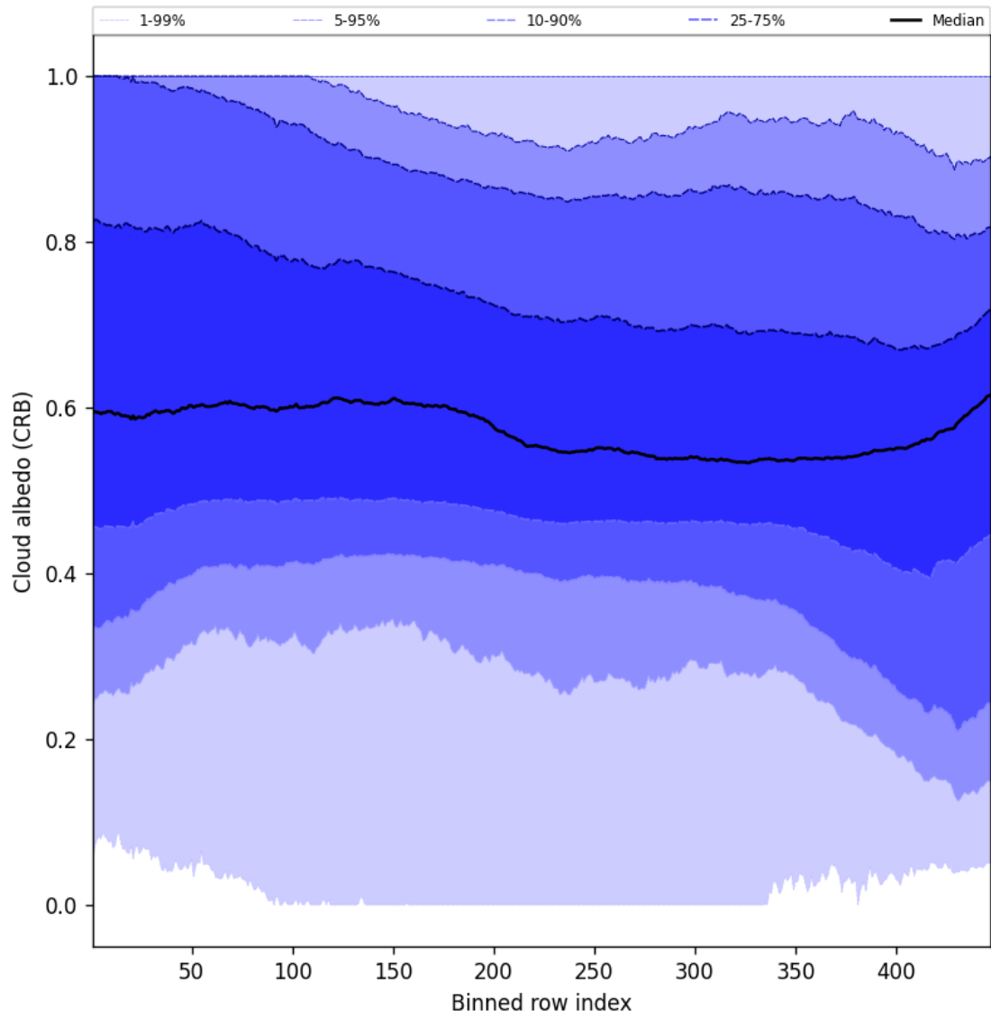
Figure 60: Along track statistics of “Cloud albedo (CRB)” for 2025-02-19 to 2025-02-21
