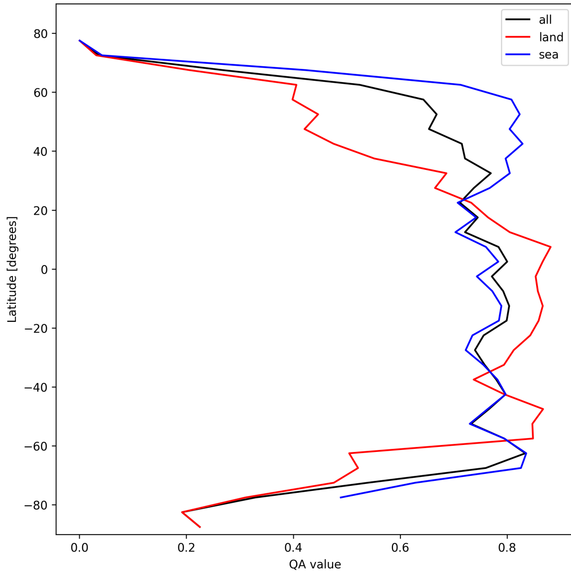
Figure 22: Zonal average of “QA value” for 2025-02-19 to 2025-02-21.
