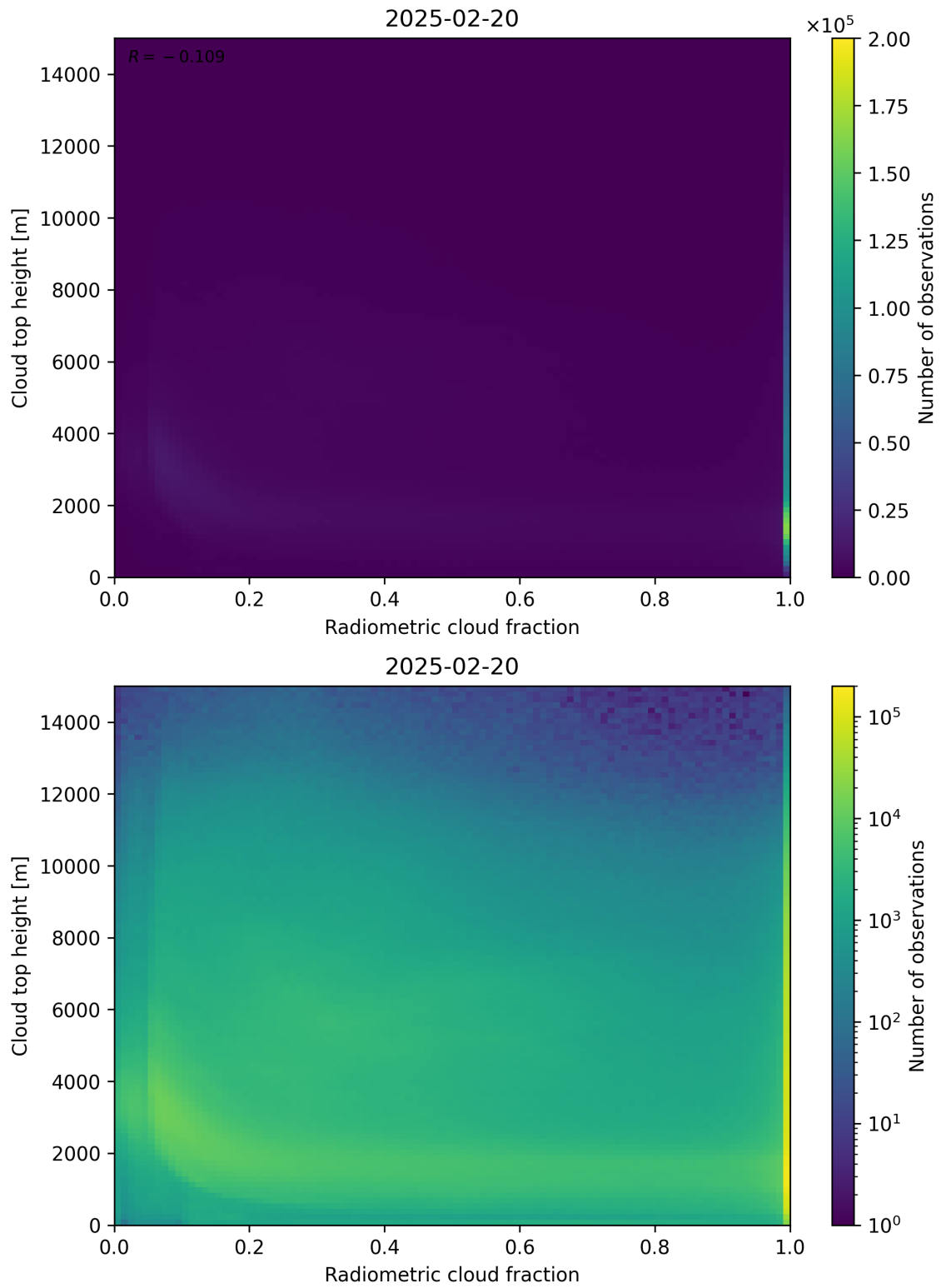
Figure 76: Scatter density plot of “Radiometric cloud fraction” against “Cloud top height” for 2025-02-19 to 2025-02-21.
