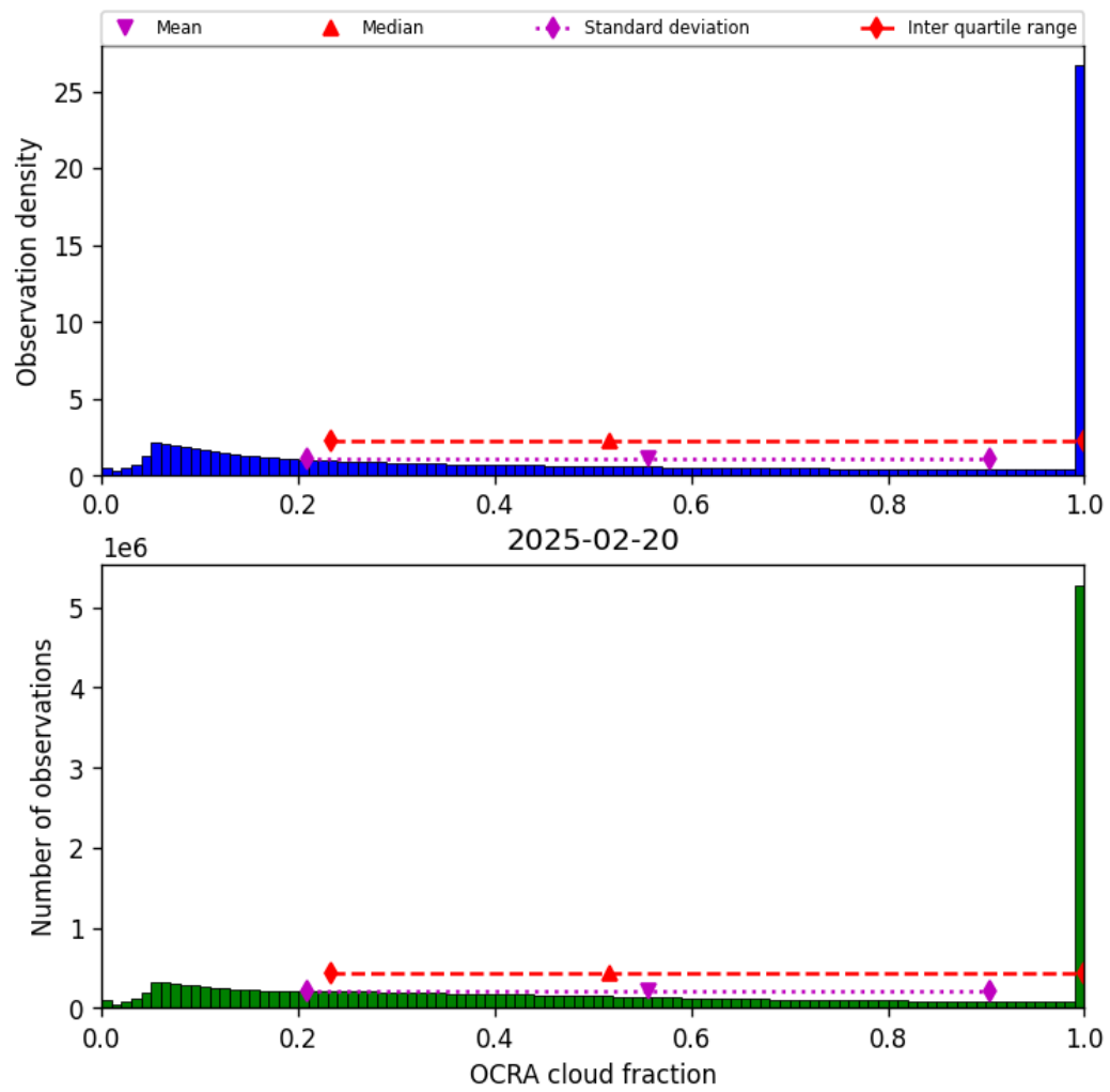
Figure 50: Histogram of “OCRA cloud fraction” for 2025-02-19 to 2025-02-21
