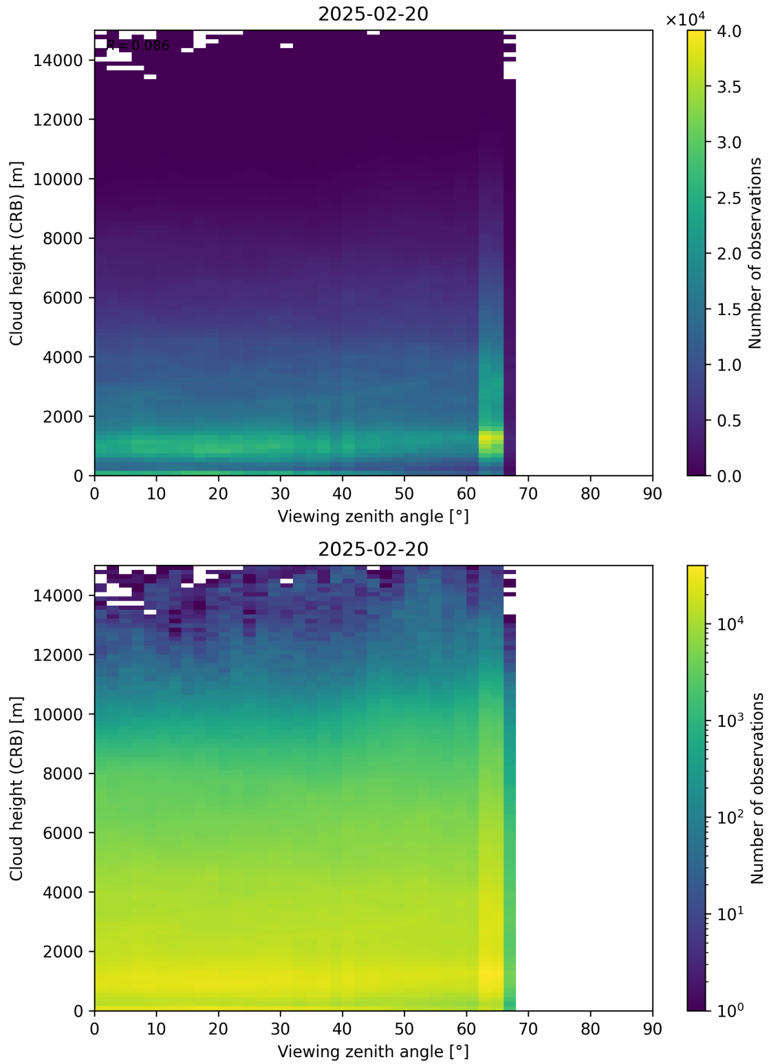
Figure 110: Scatter density plot of “Viewing zenith angle” against “Cloud height (CRB)” for 2025-02-19 to 2025-02-21.
