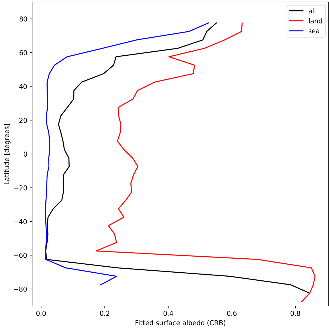
Figure 30: Zonal average of “Fitted surface albedo (CRB)” for 2025-02-19 to 2025-02-21.
