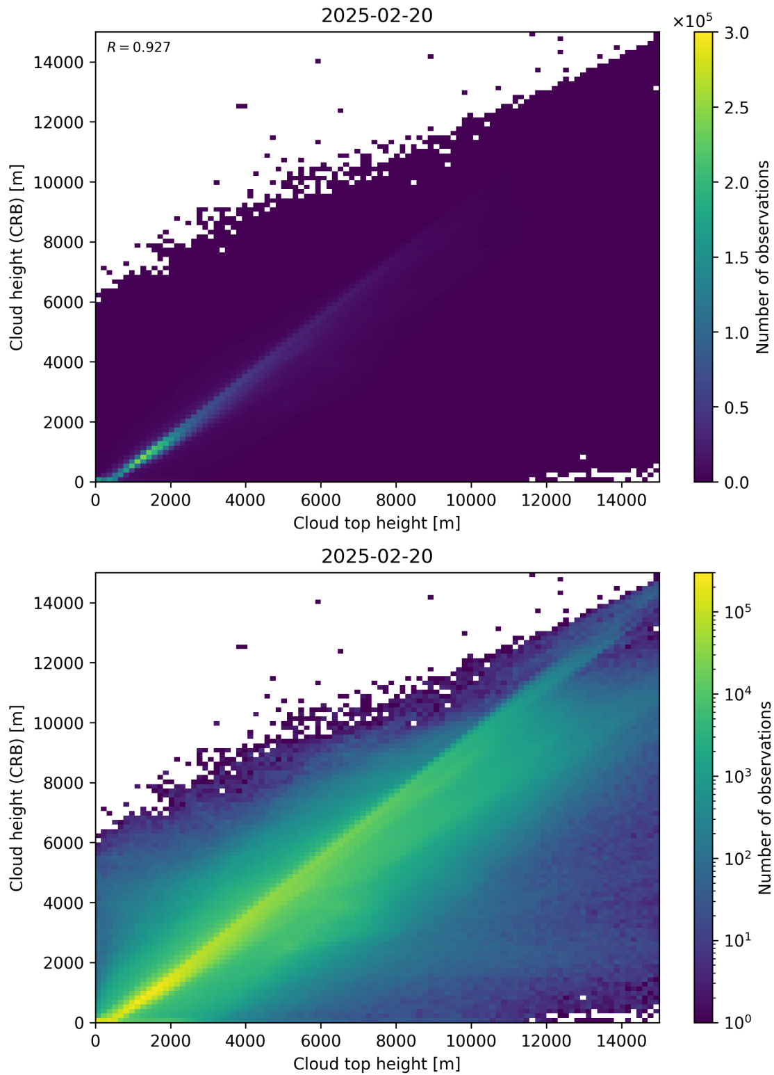
Figure 89: Scatter density plot of “Cloud top height” against “Cloud height (CRB)” for 2025-02-19 to 2025-02-21.
