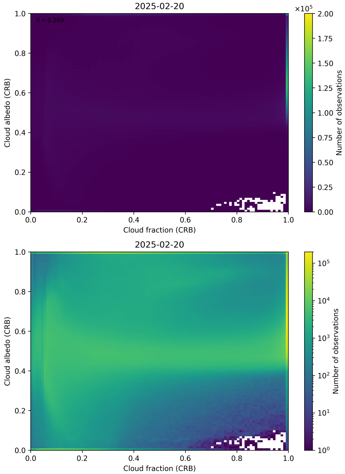
Figure 77: Scatter density plot of “Cloud fraction (CRB)” against “Cloud albedo (CRB)” for 2025-02-19 to 2025-02-21.
