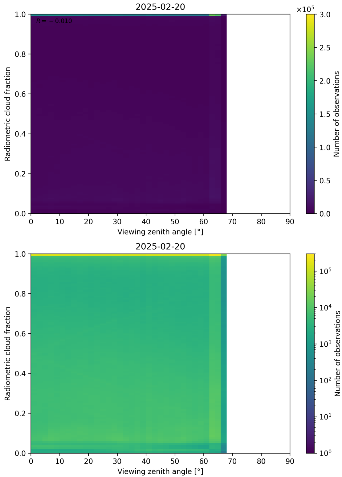
Figure 107: Scatter density plot of “Viewing zenith angle” against “Radiometric cloud fraction” for 2025-02-19 to 2025-02-21.
