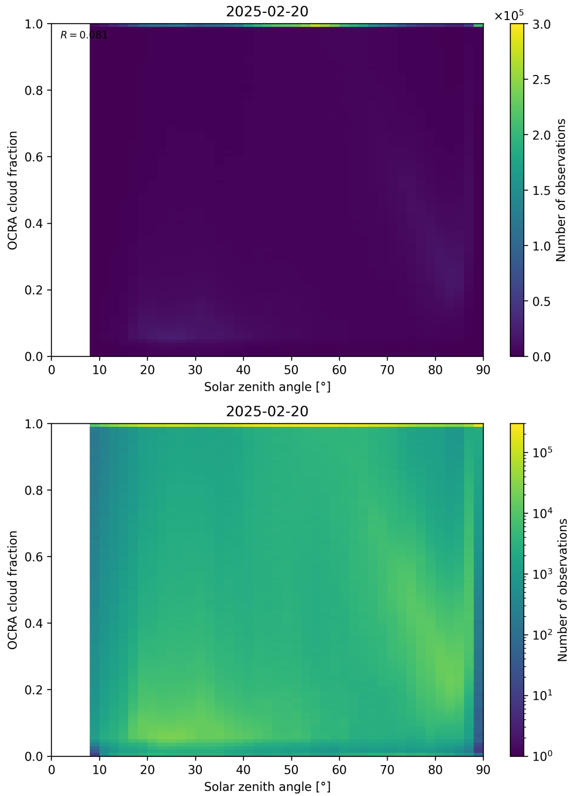
Figure 100: Scatter density plot of “Solar zenith angle” against “OCRA cloud fraction” for 2025-02-19 to 2025-02-21.
