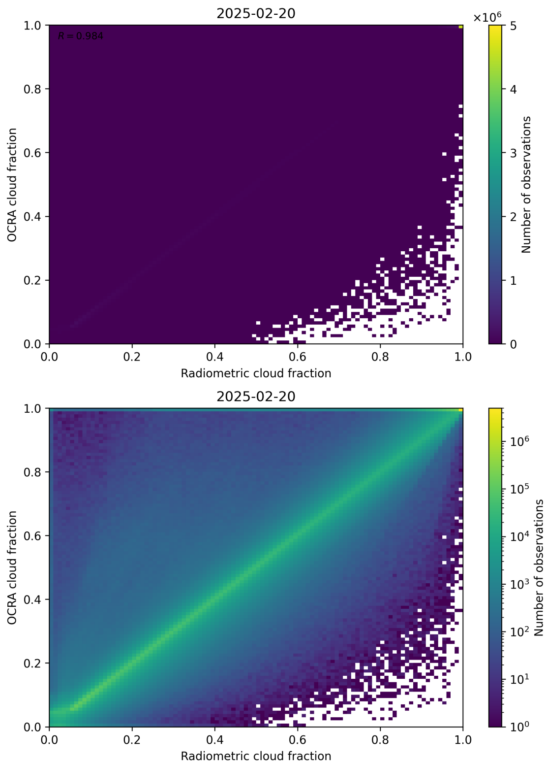
Figure 72: Scatter density plot of “Radiometric cloud fraction” against “OCRA cloud fraction” for 2025-02-19 to 2025-02-21.
