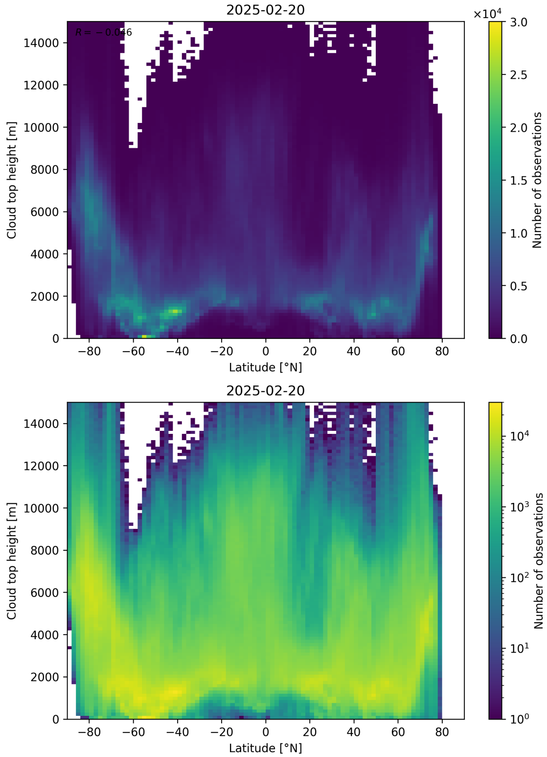
Figure 97: Scatter density plot of “Latitude” against “Cloud top height” for 2025-02-19 to 2025-02-21.
