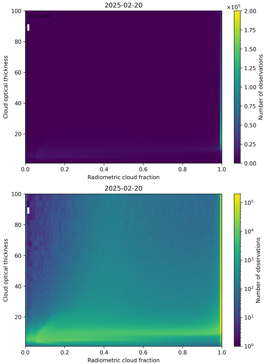
Figure 75: Scatter density plot of “Radiometric cloud fraction” against “Cloud optical thickness” for 2025-02-19 to 2025-02-21.
