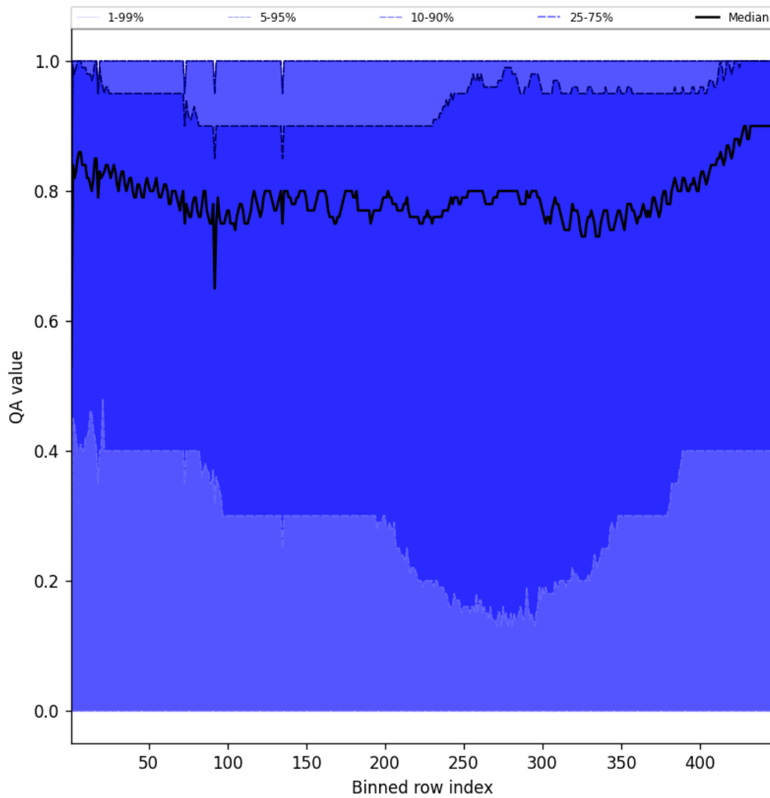
Figure 54: Along track statistics of “QA value” for 2025-02-19 to 2025-02-21
