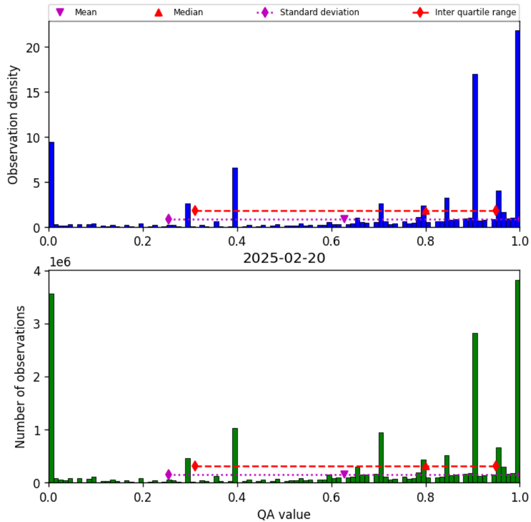
Figure 38: Histogram of “QA value” for 2025-02-19 to 2025-02-21
