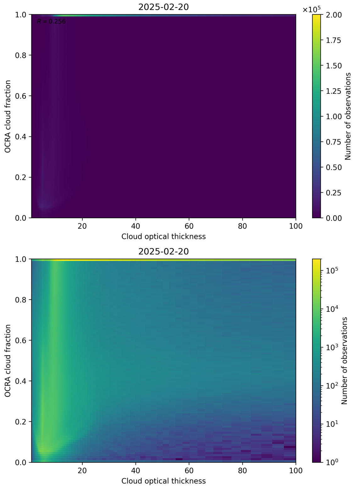
Figure 83: Scatter density plot of “Cloud optical thickness” against “OCRA cloud fraction” for 2025-02-19 to 2025-02-21.
