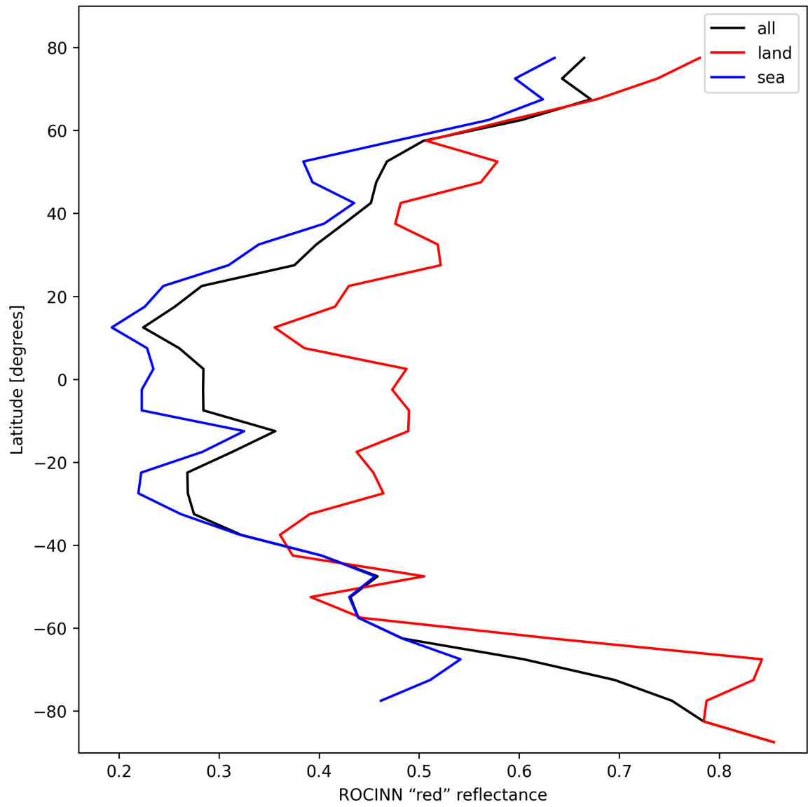
Figure 37: Zonal average of “ROCINN “red” reflectance” for 2025-02-19 to 2025-02-21.
