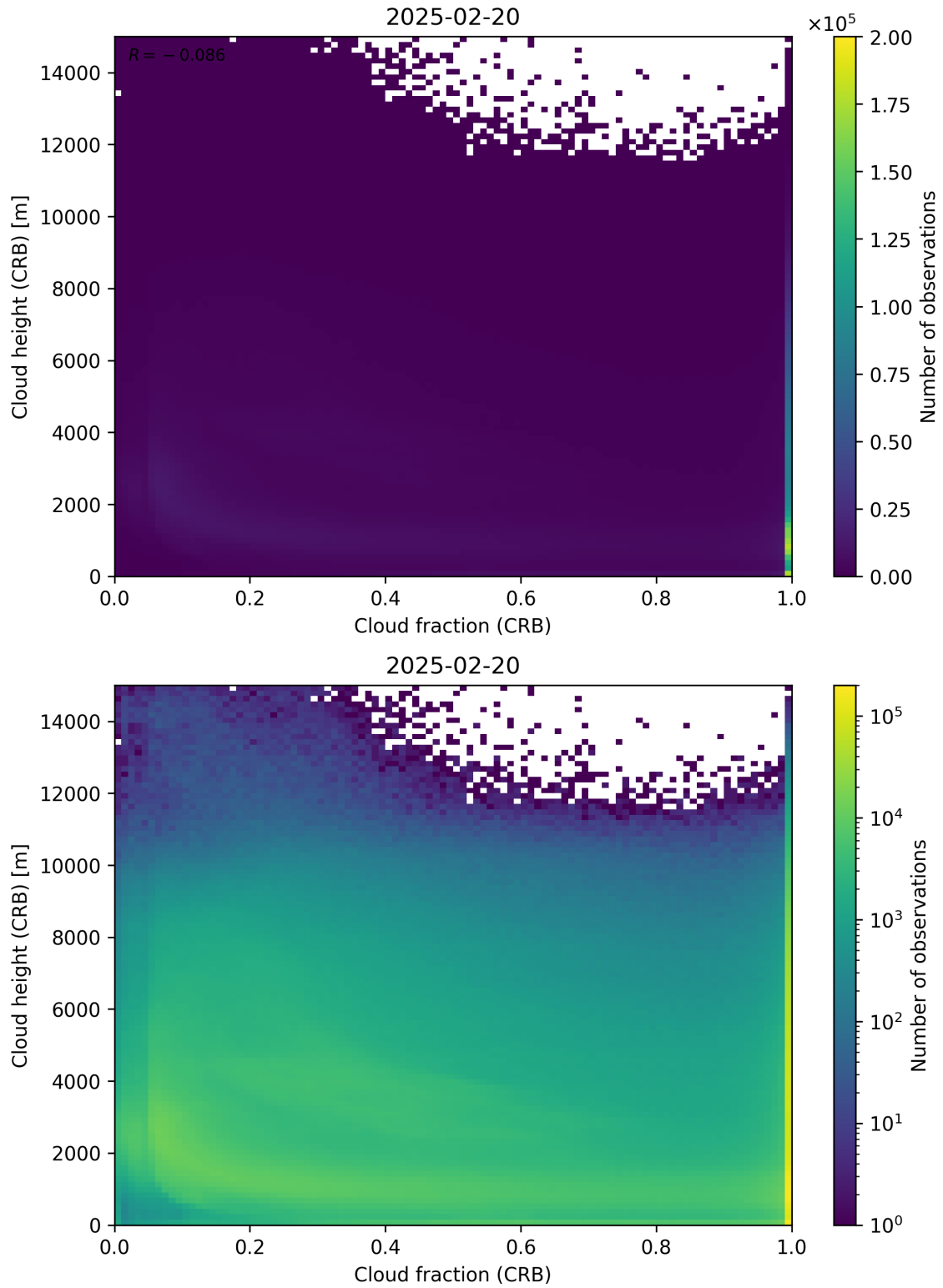
Figure 79: Scatter density plot of “Cloud fraction (CRB)” against “Cloud height (CRB)” for 2025-02-19 to 2025-02-21.
