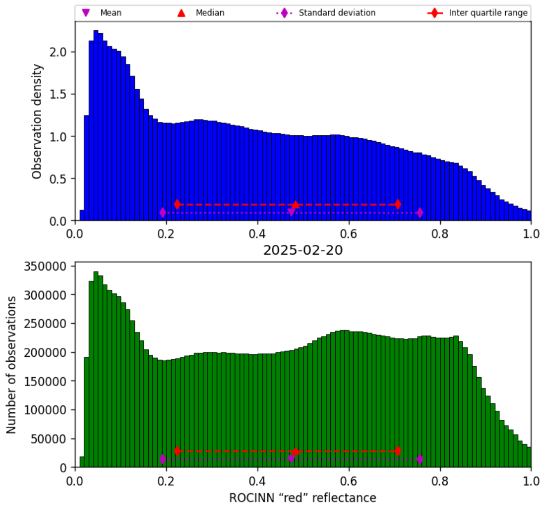
Figure 53: Histogram of “ROCINN “red” reflectance” for 2025-02-19 to 2025-02-21
