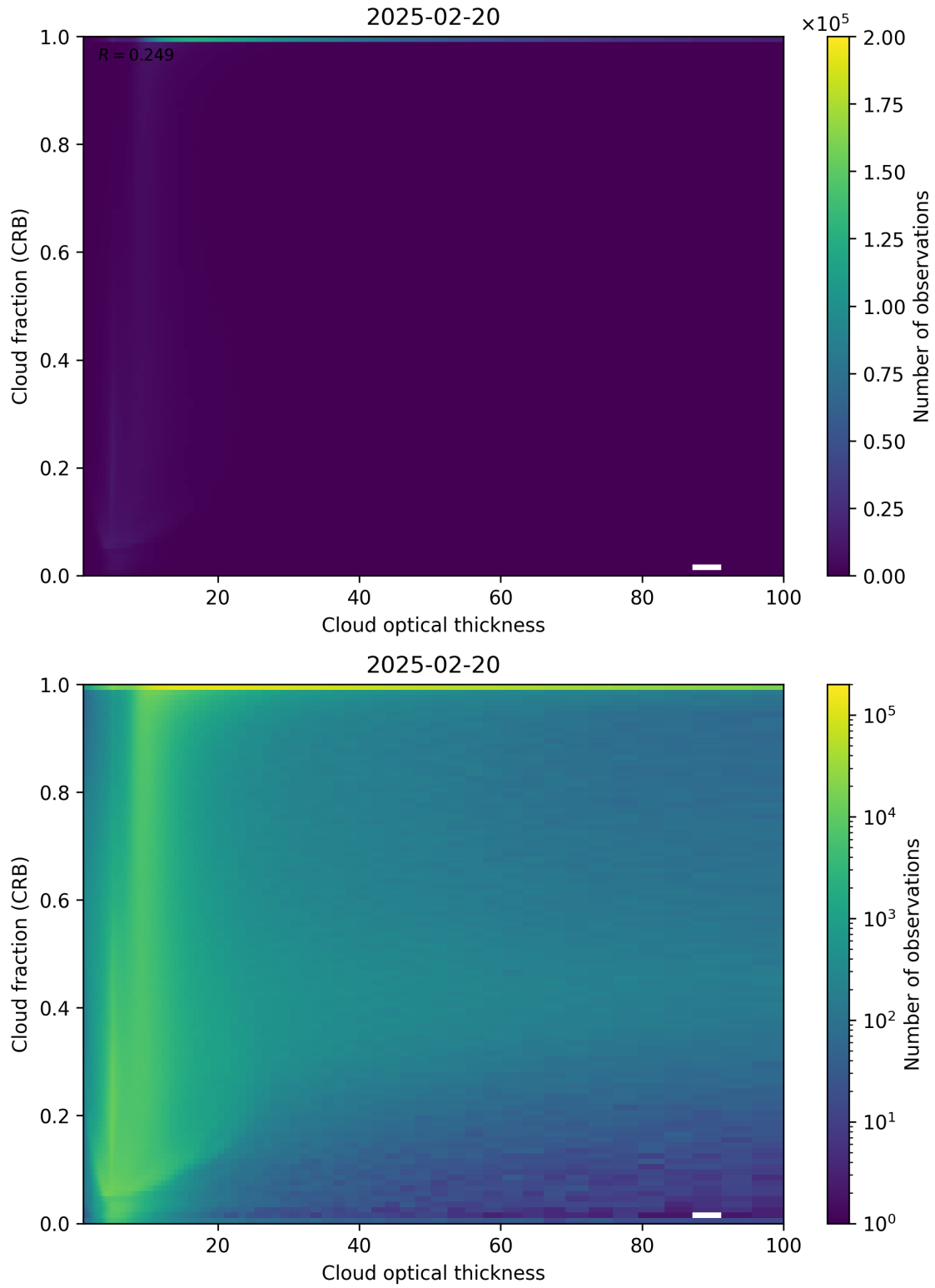
Figure 84: Scatter density plot of “Cloud optical thickness” against “Cloud fraction (CRB)” for 2025-02-19 to 2025-02-21.
