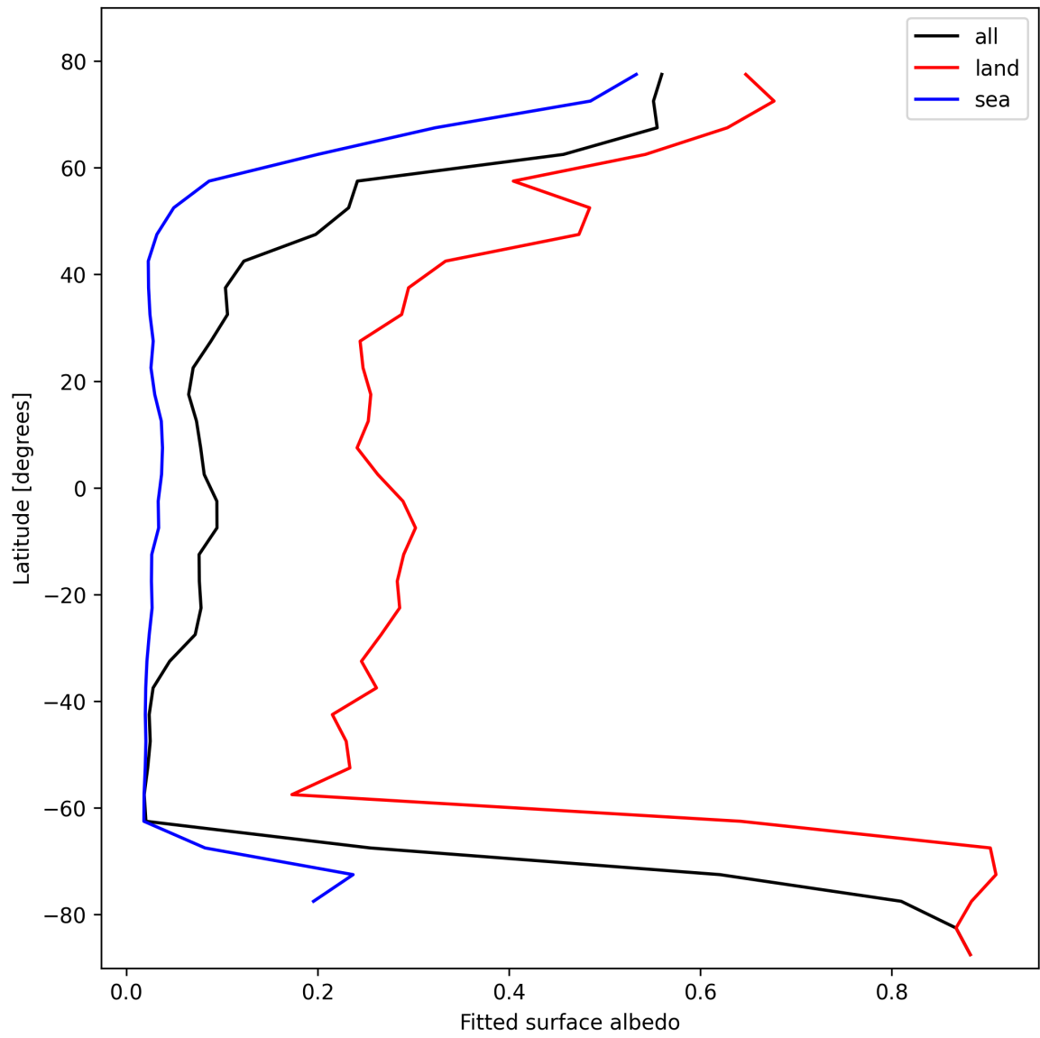
Figure 29: Zonal average of “Fitted surface albedo” for 2025-02-19 to 2025-02-21.
