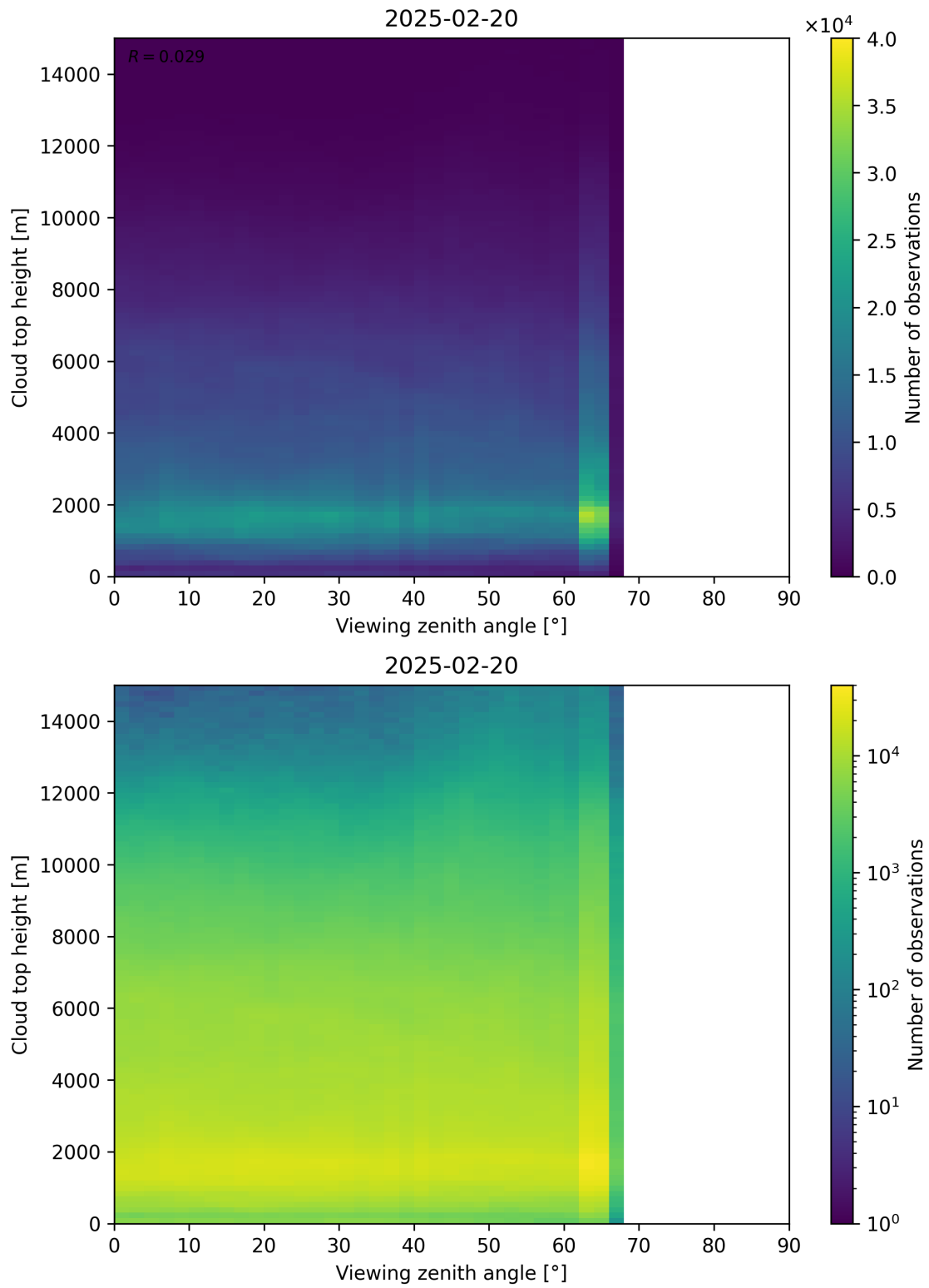
Figure 112: Scatter density plot of “Viewing zenith angle” against “Cloud top height” for 2025-02-19 to 2025-02-21.
