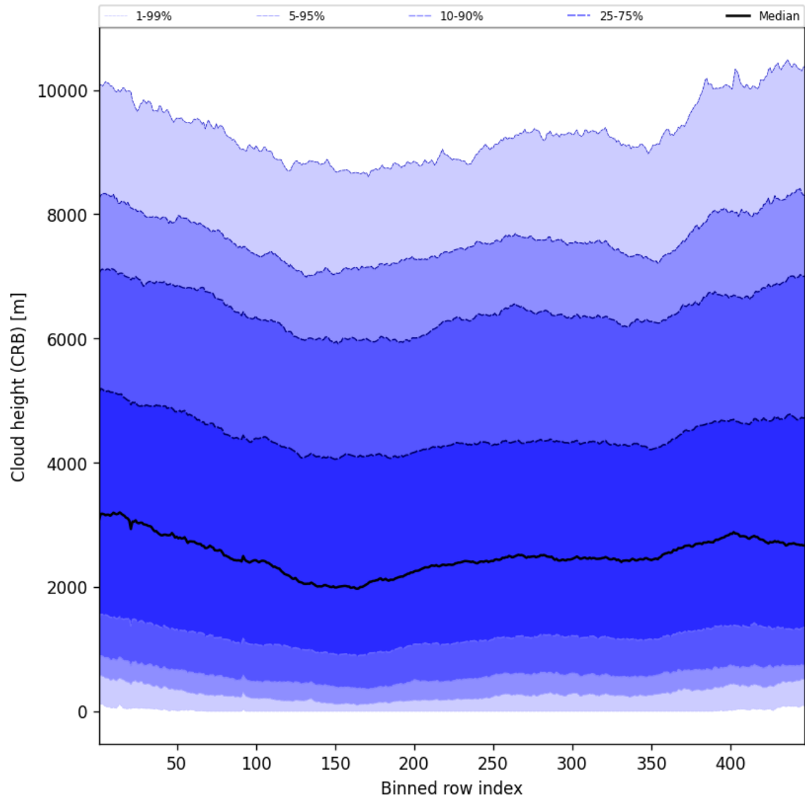
Figure 59: Along track statistics of “Cloud height (CRB)” for 2025-02-19 to 2025-02-21
