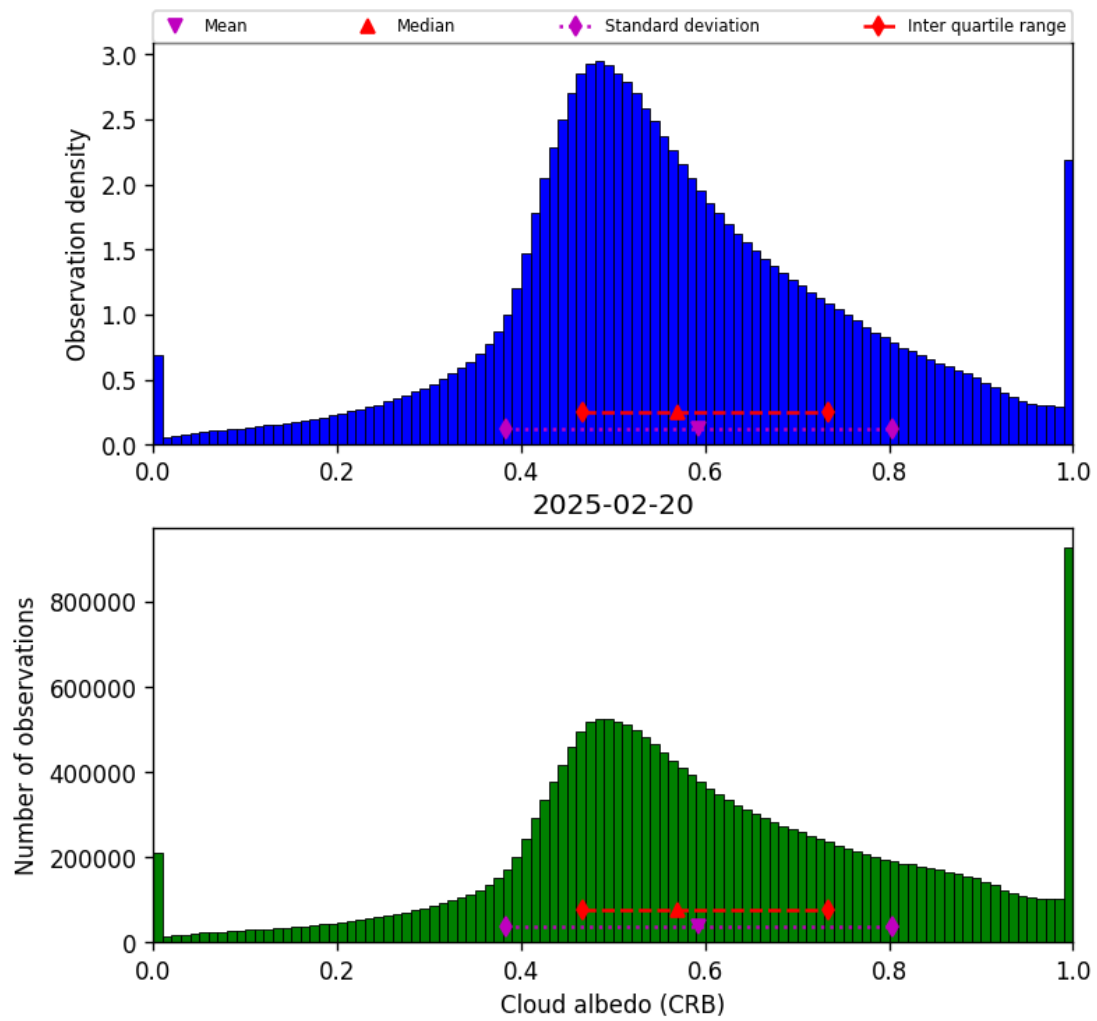
Figure 44: Histogram of “Cloud albedo (CRB)” for 2025-02-19 to 2025-02-21
