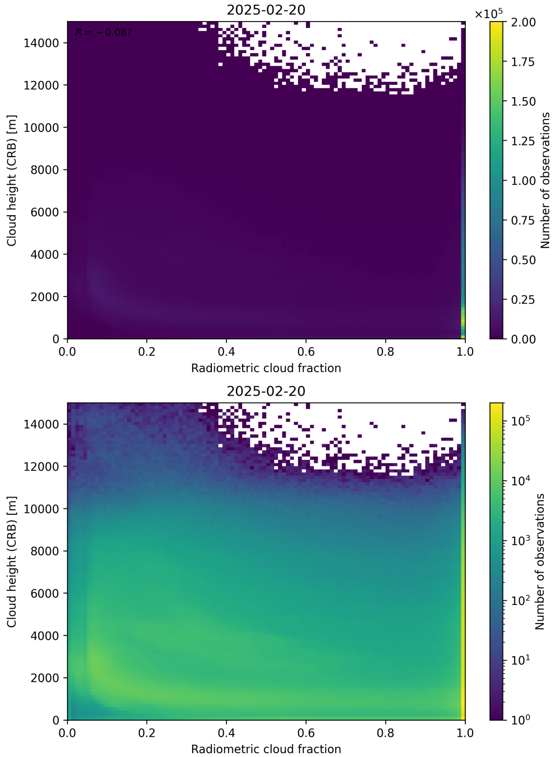
Figure 74: Scatter density plot of “Radiometric cloud fraction” against “Cloud height (CRB)” for 2025-02-19 to 2025-02-21.
