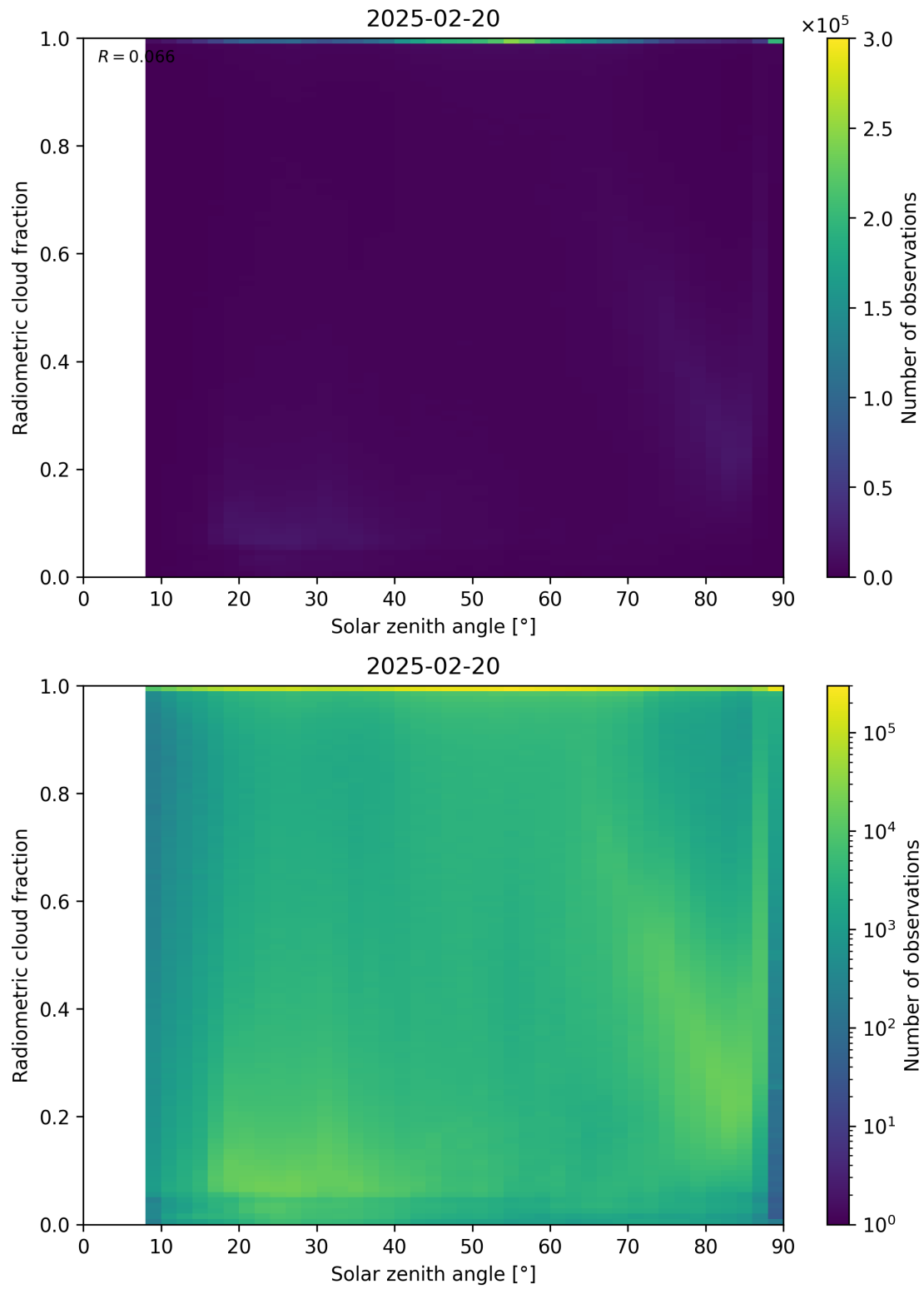
Figure 99: Scatter density plot of “Solar zenith angle” against “Radiometric cloud fraction” for 2025-02-19 to 2025-02-21.
