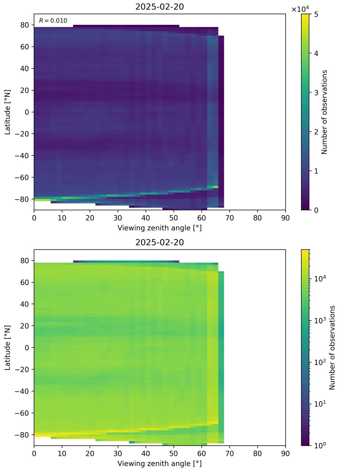
Figure 113: Scatter density plot of “Viewing zenith angle” against “Latitude” for 2025-02-19 to 2025-02-21.
