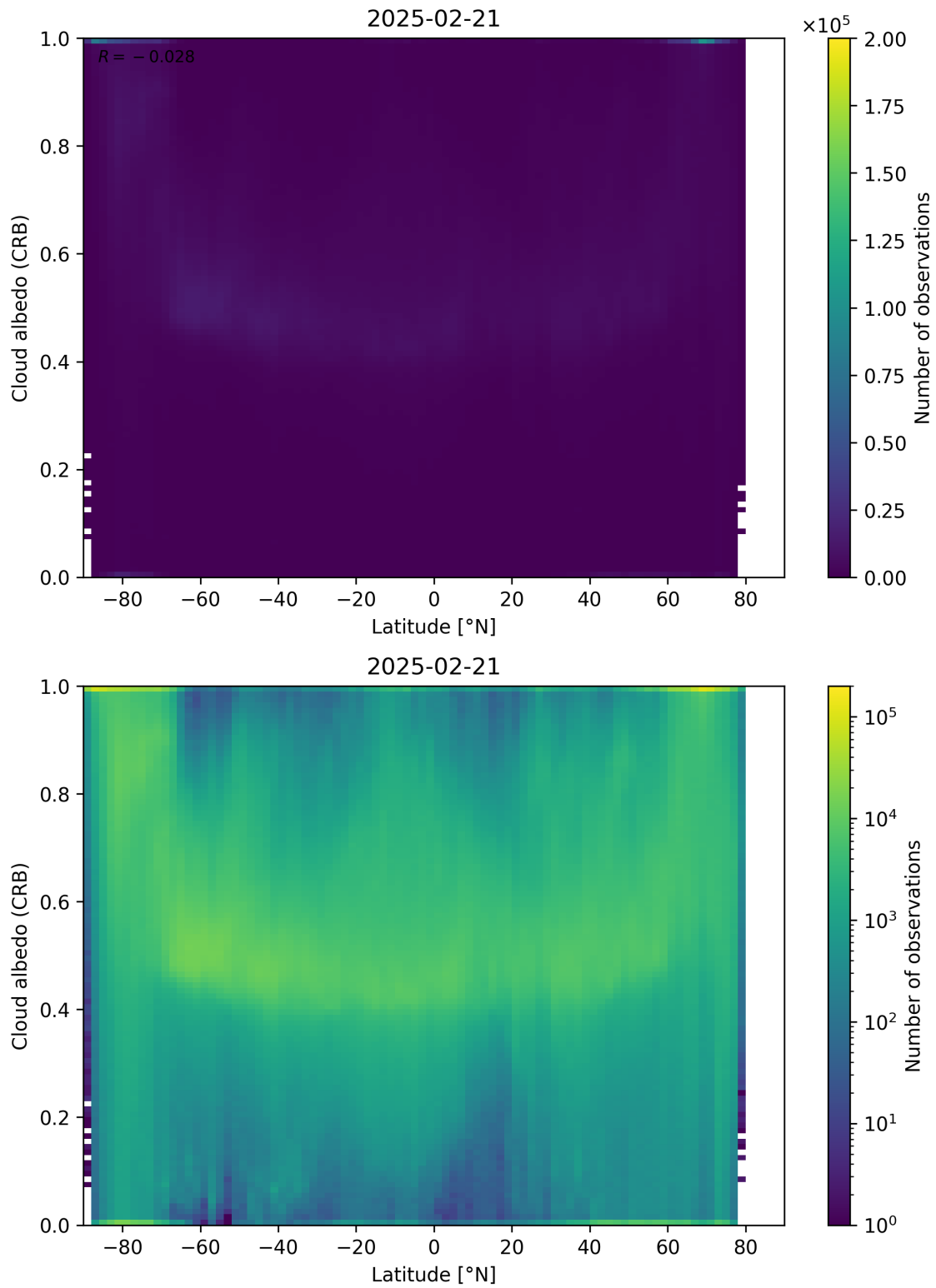
Figure 91: Scatter density plot of “Latitude” against “Cloud albedo (CRB)” for 2025-02-20 to 2025-02-22.
