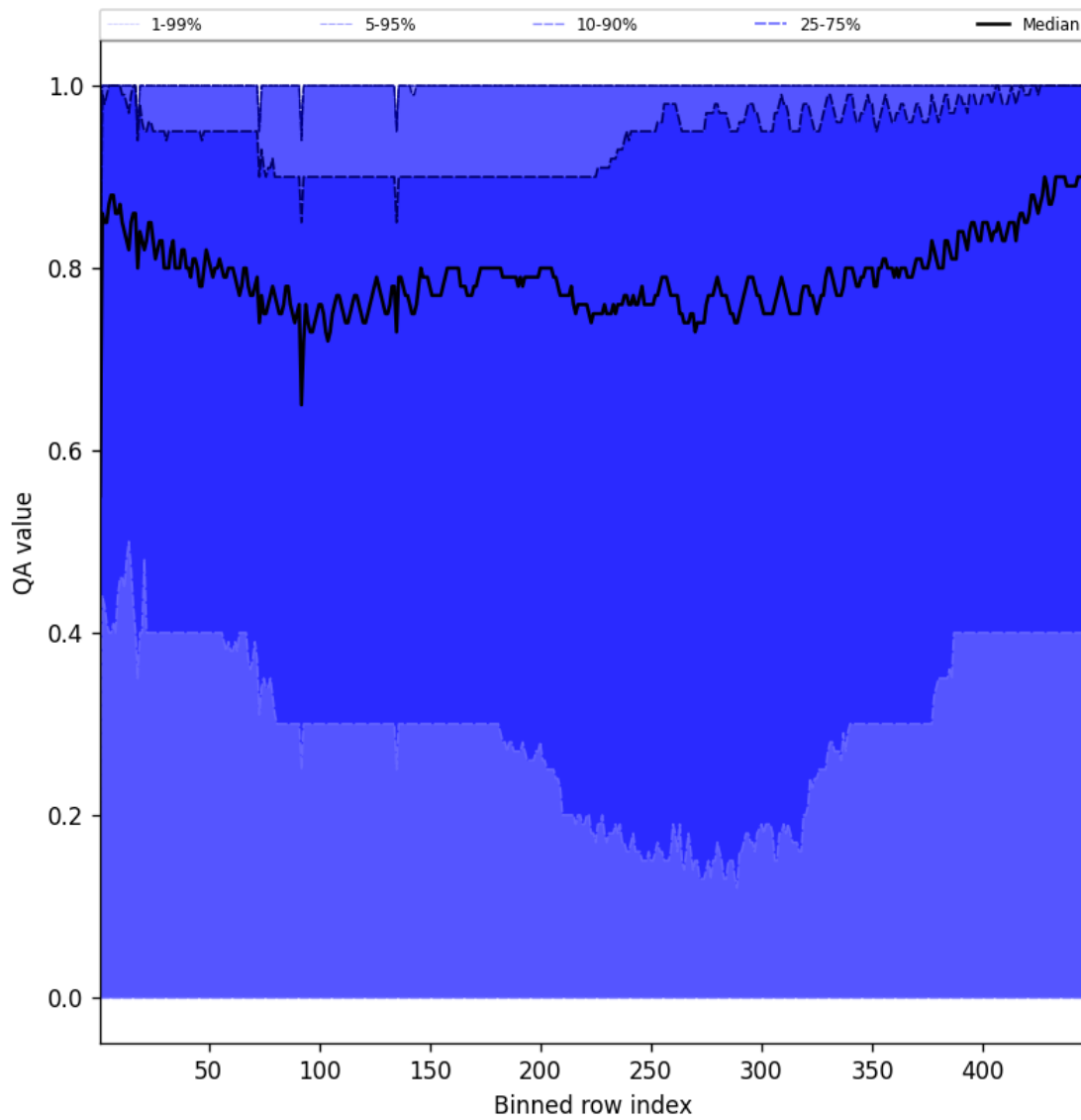
Figure 54: Along track statistics of “QA value” for 2025-02-20 to 2025-02-22
