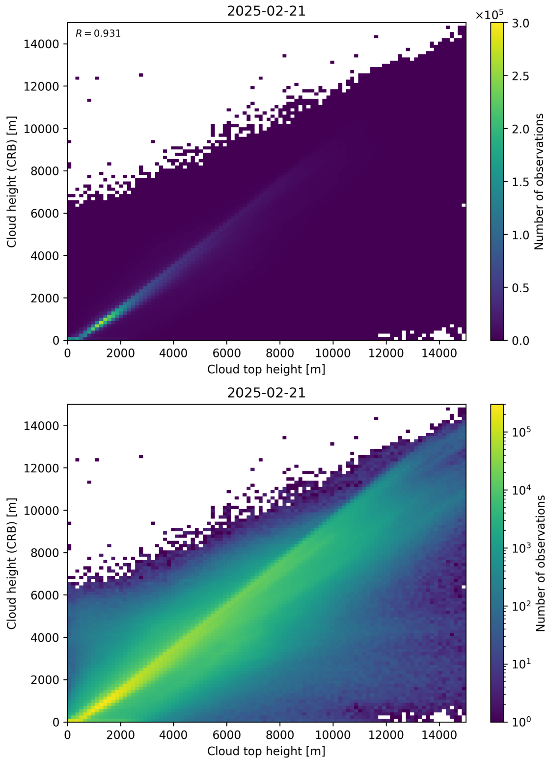
Figure 89: Scatter density plot of “Cloud top height” against “Cloud height (CRB)” for 2025-02-20 to 2025-02-22.
