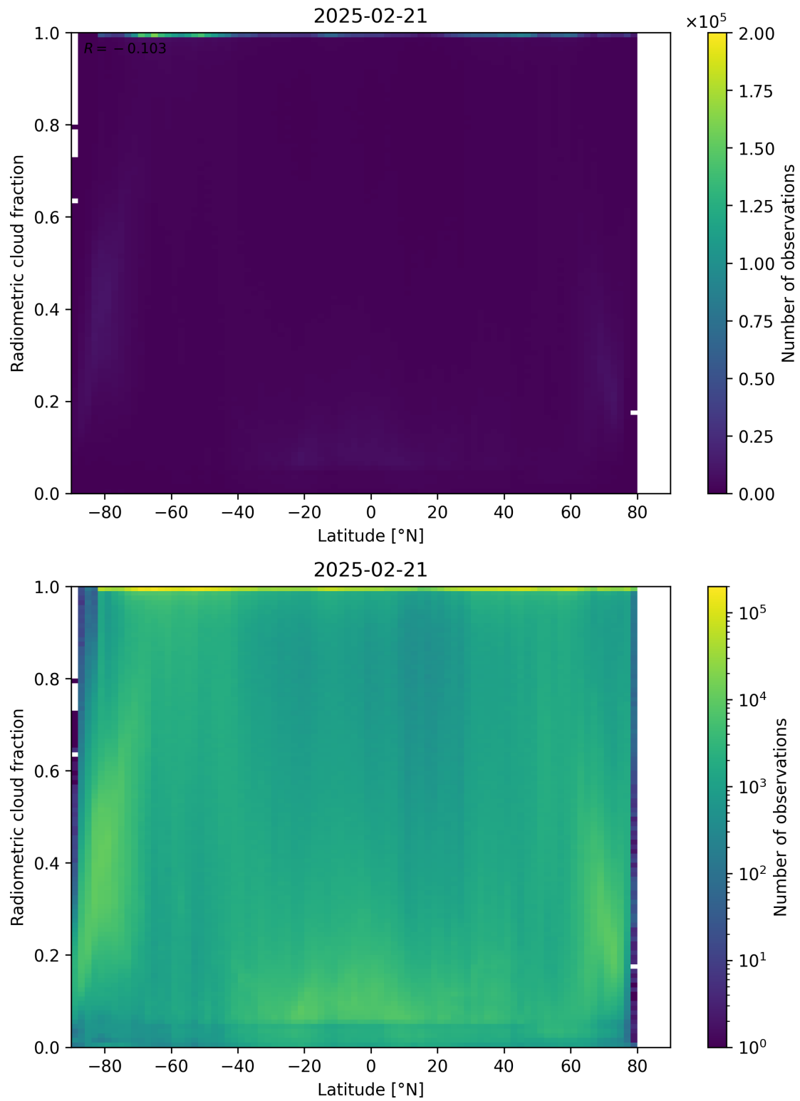
Figure 92: Scatter density plot of “Latitude” against “Radiometric cloud fraction” for 2025-02-20 to 2025-02-22.
