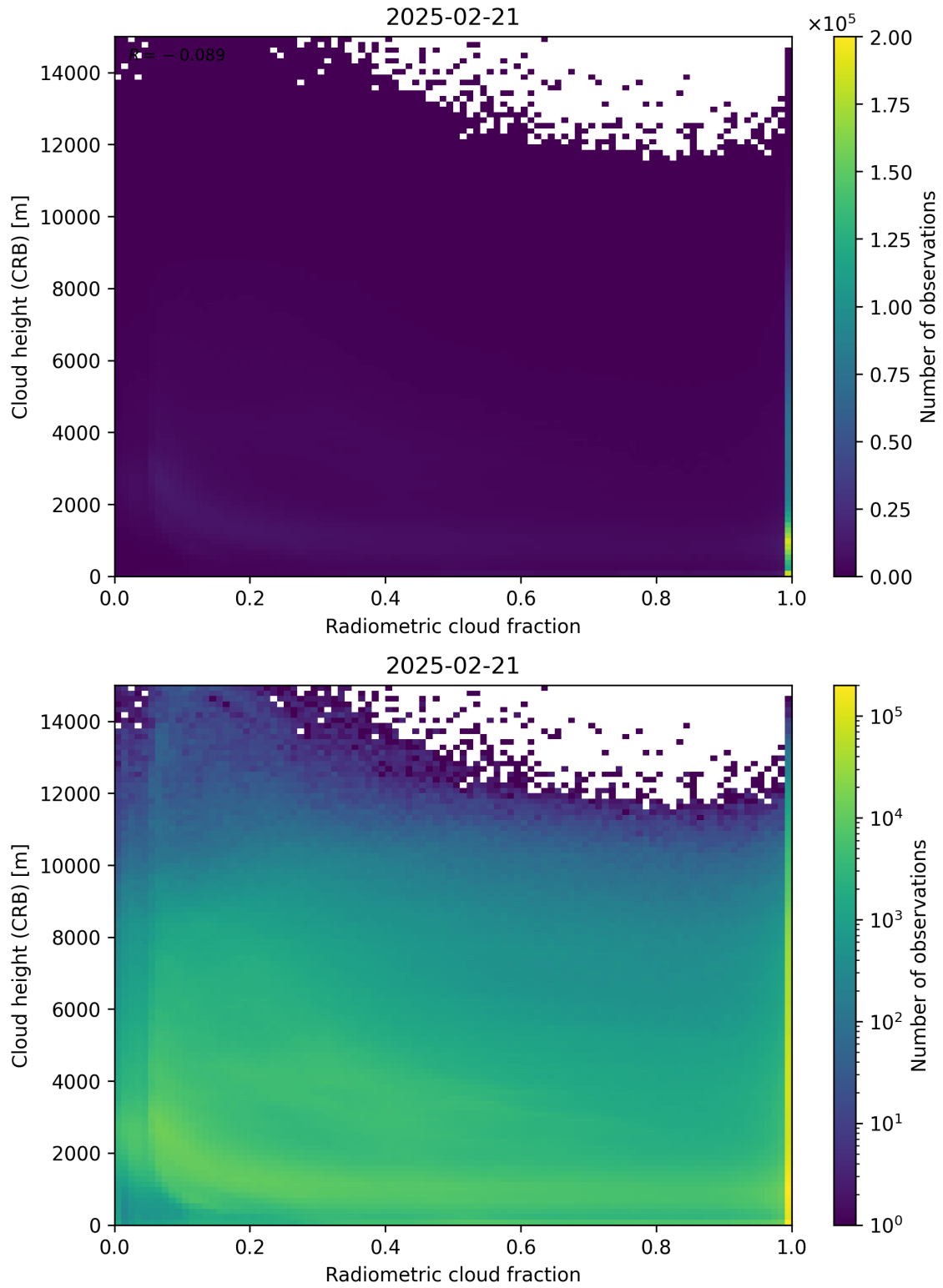
Figure 74: Scatter density plot of “Radiometric cloud fraction” against “Cloud height (CRB)” for 2025-02-20 to 2025-02-22.
