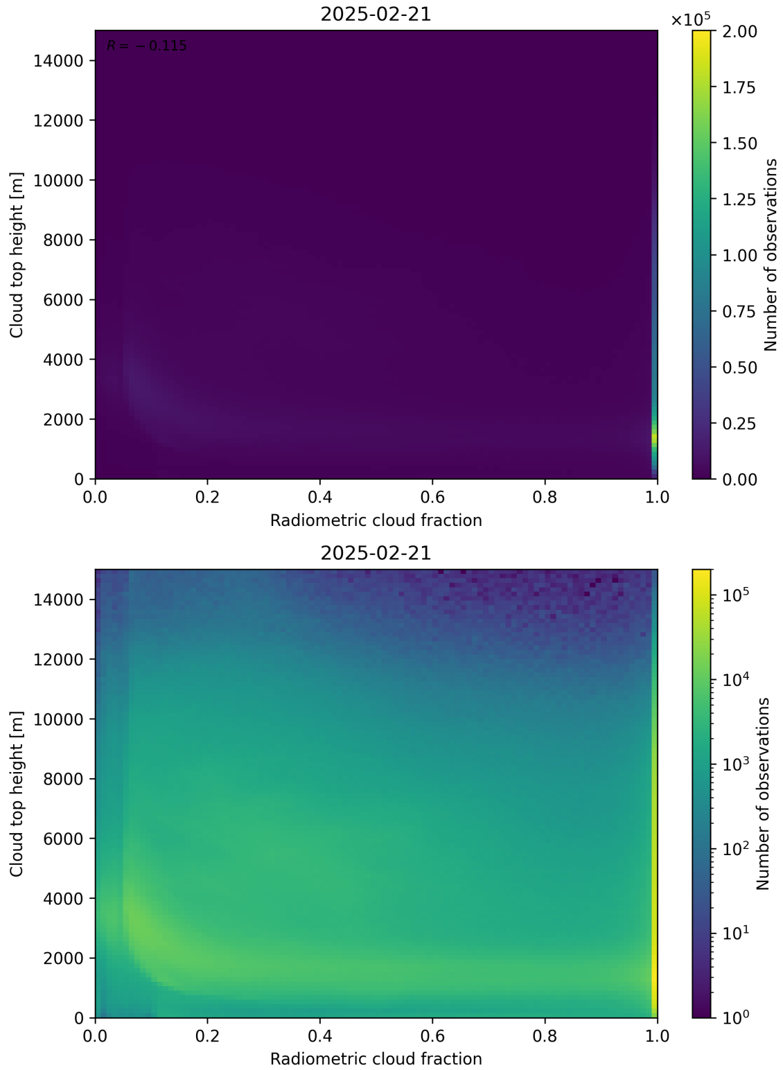
Figure 76: Scatter density plot of “Radiometric cloud fraction” against “Cloud top height” for 2025-02-20 to 2025-02-22.
