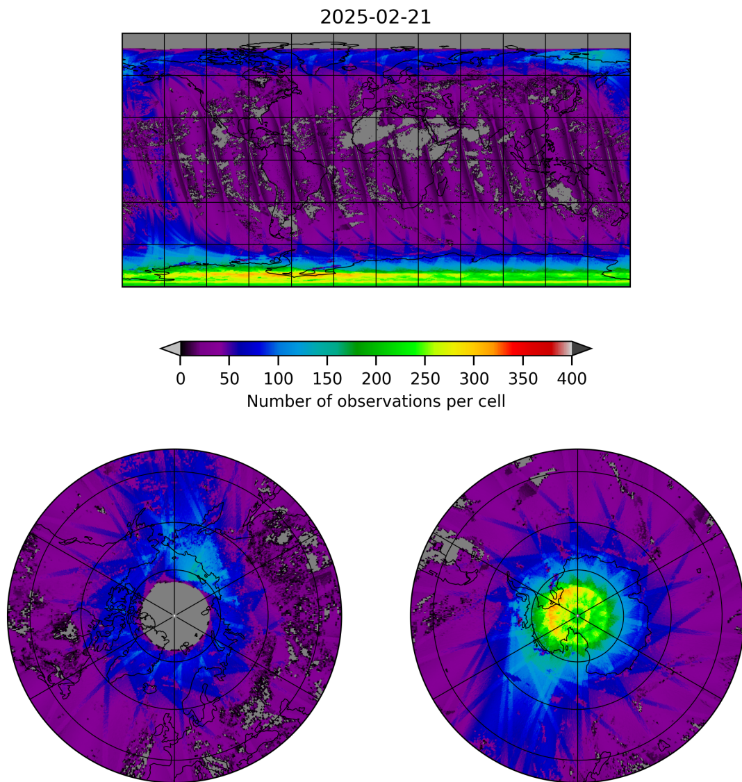
Figure 21: Map of the number of observations for 2025-02-20 to 2025-02-22
