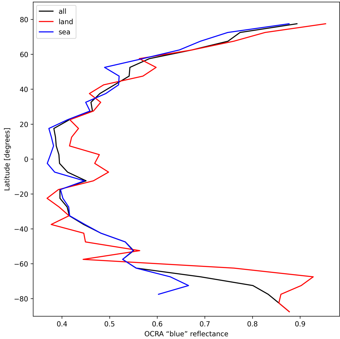
Figure 35: Zonal average of “OCRA “blue” reflectance” for 2025-02-20 to 2025-02-22.
