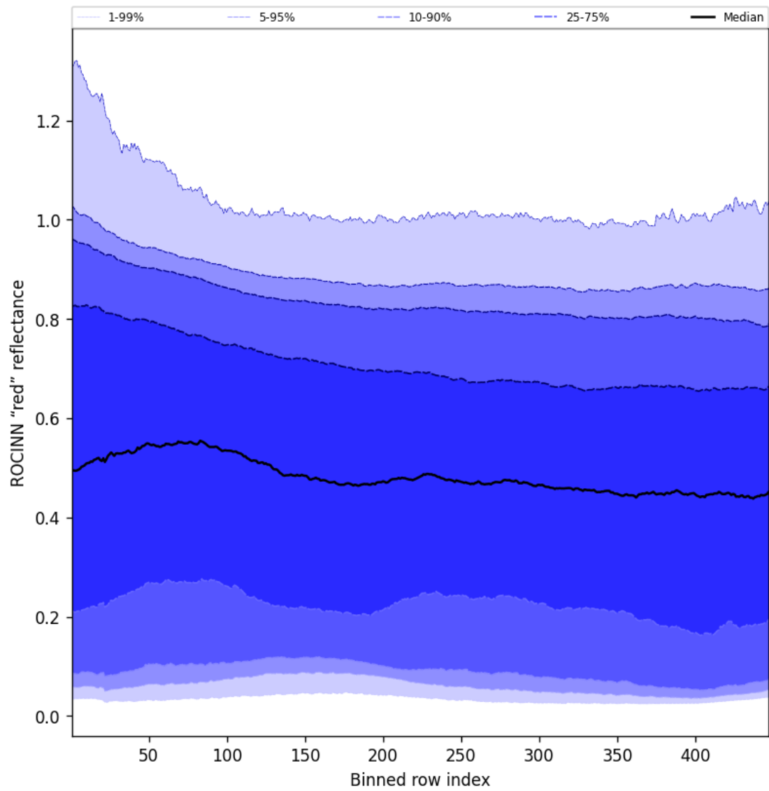
Figure 69: Along track statistics of "ROCINN "red" reflectance" for 2025-02-20 to 2025-02-22
