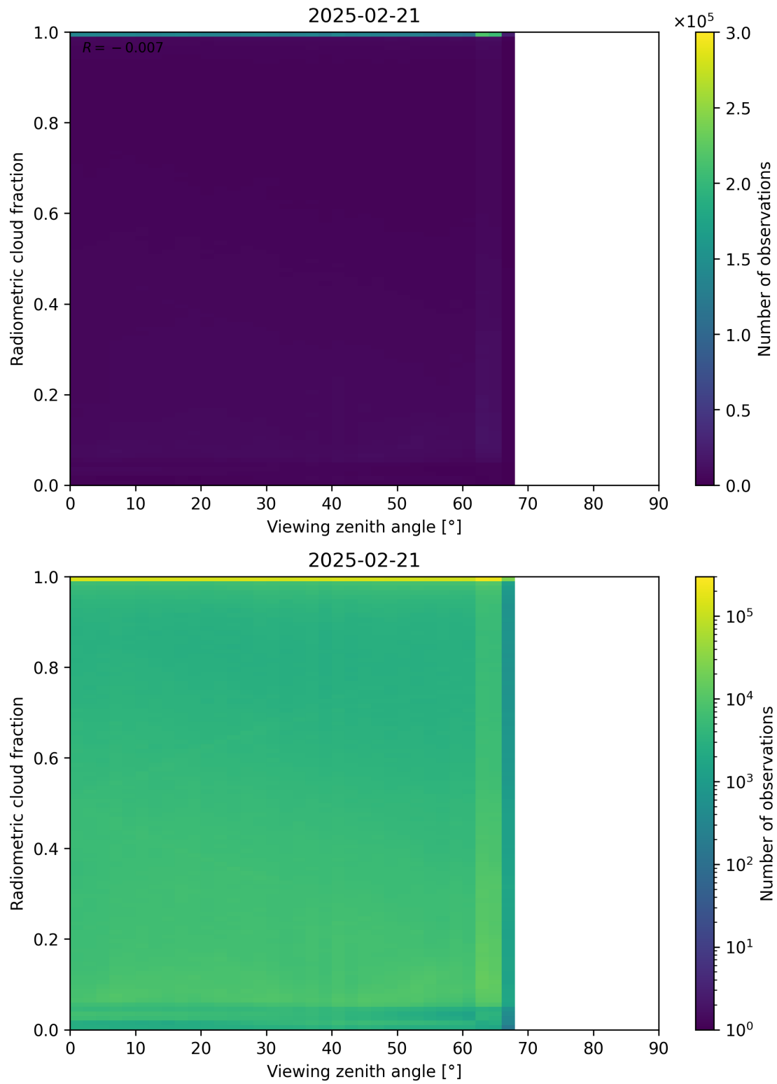
Figure 107: Scatter density plot of “Viewing zenith angle” against “Radiometric cloud fraction” for 2025-02-20 to 2025-02-22.
