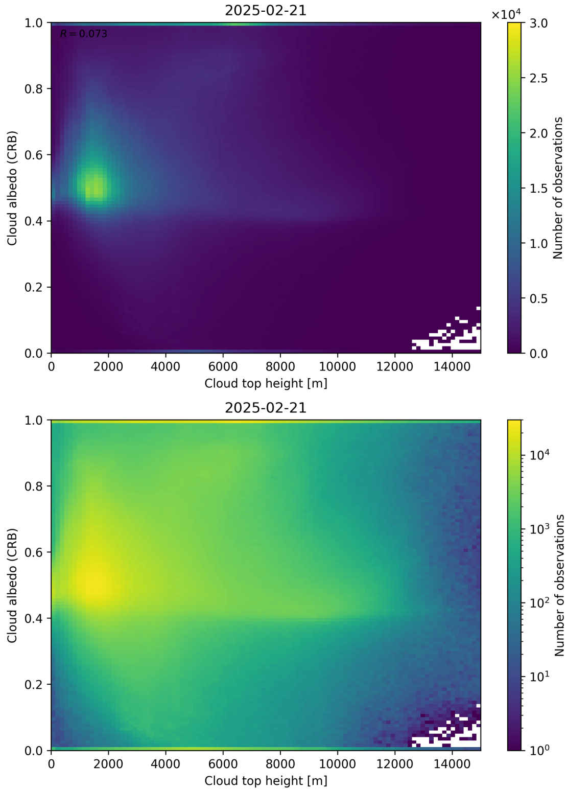
Figure 86: Scatter density plot of “Cloud top height” against “Cloud albedo (CRB)” for 2025-02-20 to 2025-02-22.
