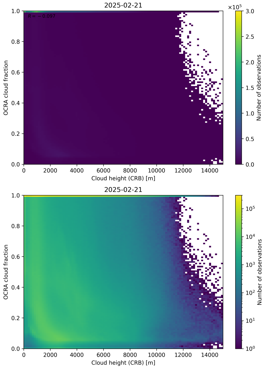
Figure 81: Scatter density plot of “Cloud height (CRB)” against “OCRA cloud fraction” for 2025-02-20 to 2025-02-22.
