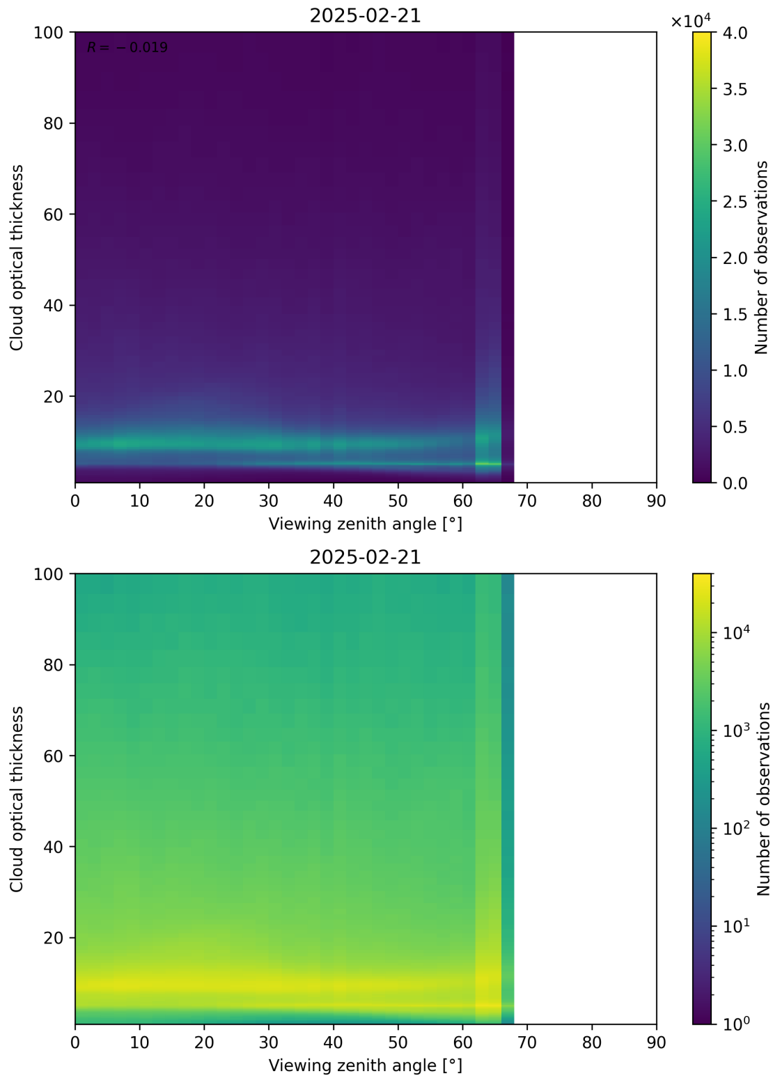
Figure 111: Scatter density plot of “Viewing zenith angle” against “Cloud optical thickness” for 2025-02-20 to 2025-02-22.
