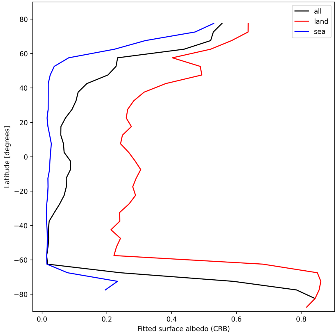
Figure 30: Zonal average of “Fitted surface albedo (CRB)” for 2025-02-20 to 2025-02-22.
