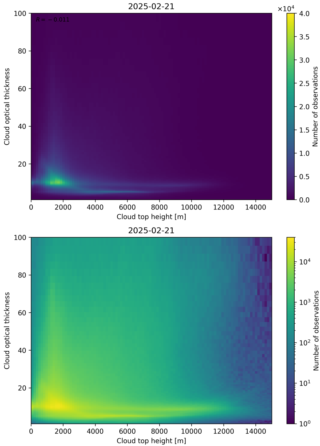
Figure 90: Scatter density plot of “Cloud top height” against “Cloud optical thickness” for 2025-02-20 to 2025-02-22.
