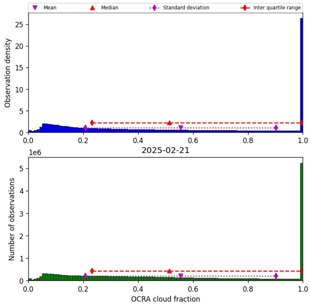
Figure 50: Histogram of “OCRA cloud fraction” for 2025-02-20 to 2025-02-22
