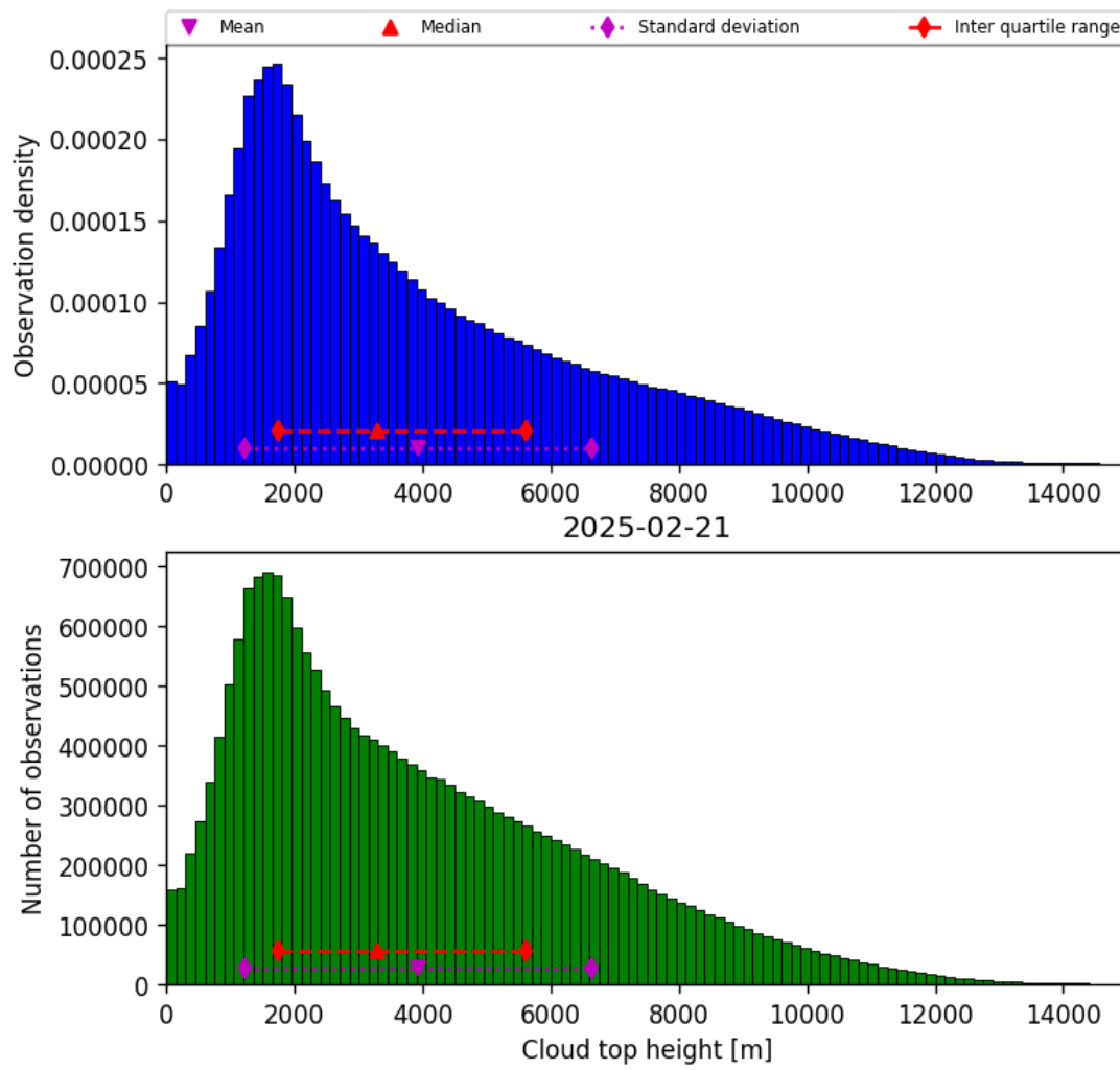
Figure 40: Histogram of “Cloud top height” for 2025-02-20 to 2025-02-22
