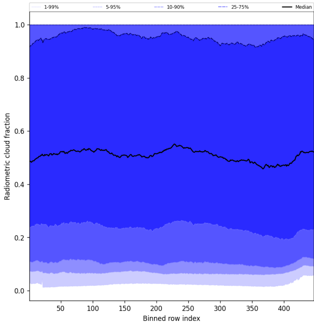
Figure 55: Along track statistics of “Radiometric cloud fraction” for 2025-02-20 to 2025-02-22
