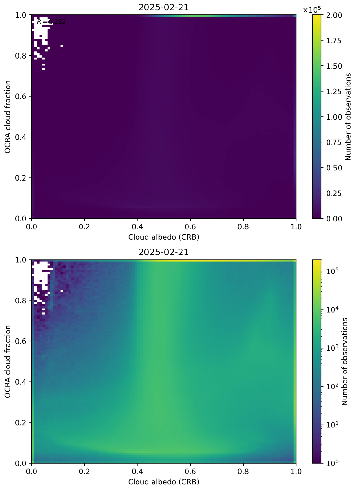
Figure 70: Scatter density plot of “Cloud albedo (CRB)” against “OCRA cloud fraction” for 2025-02-20 to 2025-02-22.
