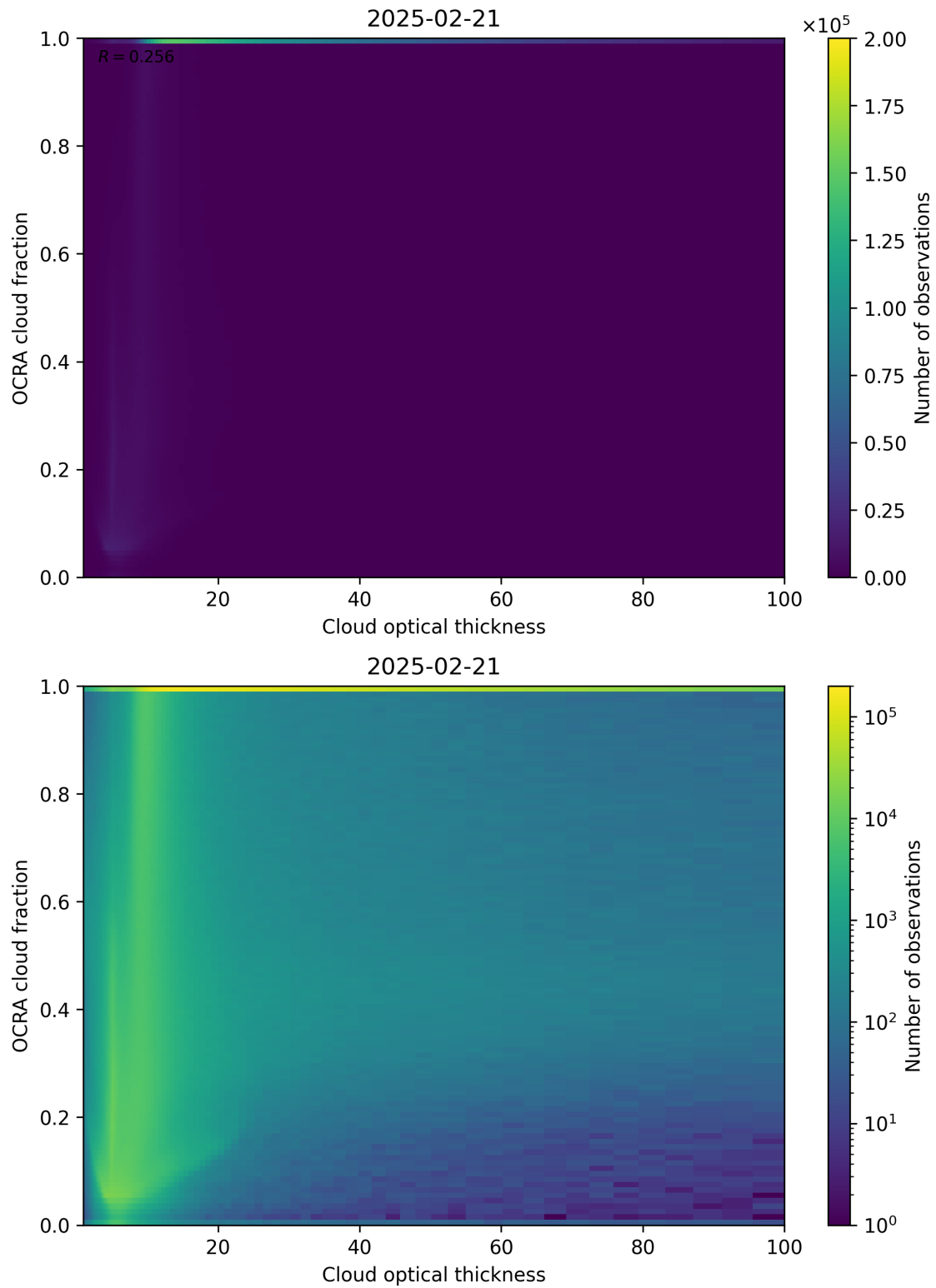
Figure 83: Scatter density plot of “Cloud optical thickness” against “OCRA cloud fraction” for 2025-02-20 to 2025-02-22.
