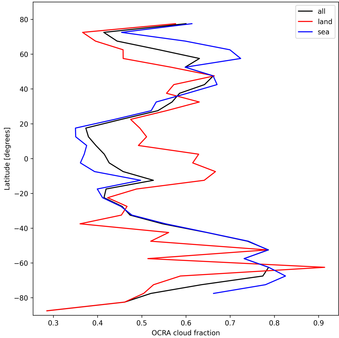
Figure 34: Zonal average of “OCRA cloud fraction” for 2025-02-20 to 2025-02-22.
