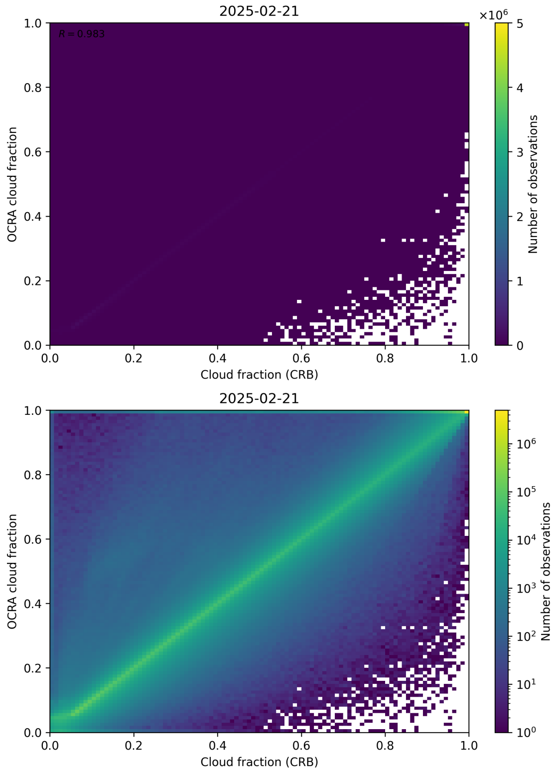
Figure 78: Scatter density plot of “Cloud fraction (CRB)” against “OCRA cloud fraction” for 2025-02-20 to 2025-02-22.
