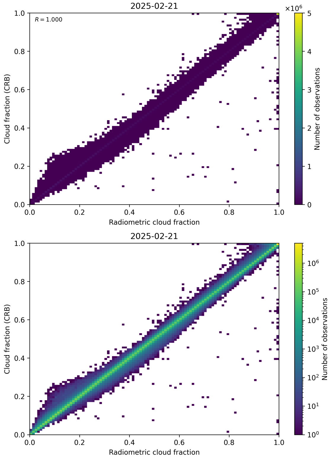
Figure 73: Scatter density plot of “Radiometric cloud fraction” against “Cloud fraction (CRB)” for 2025-02-20 to 2025-02-22.
