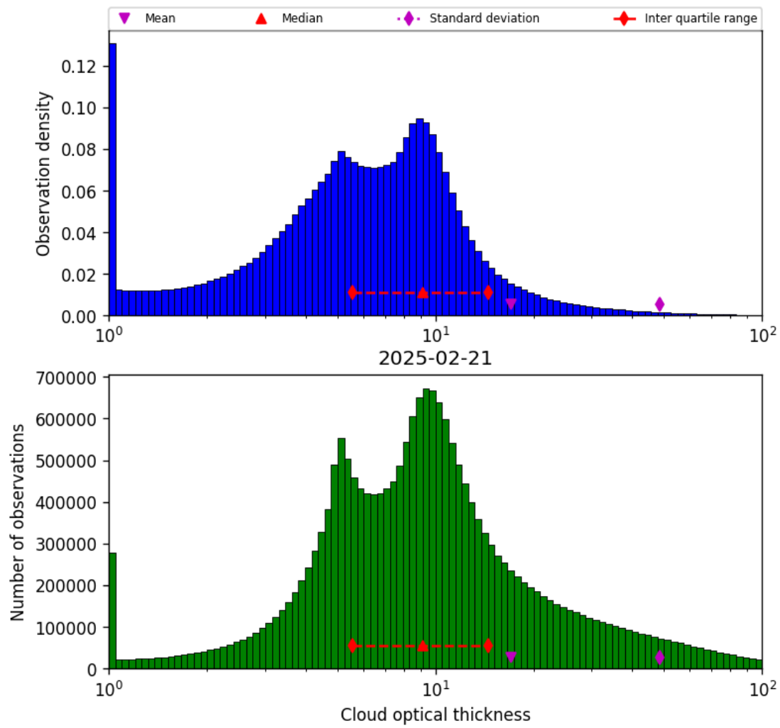
Figure 41: Histogram of “Cloud optical thickness” for 2025-02-20 to 2025-02-22
