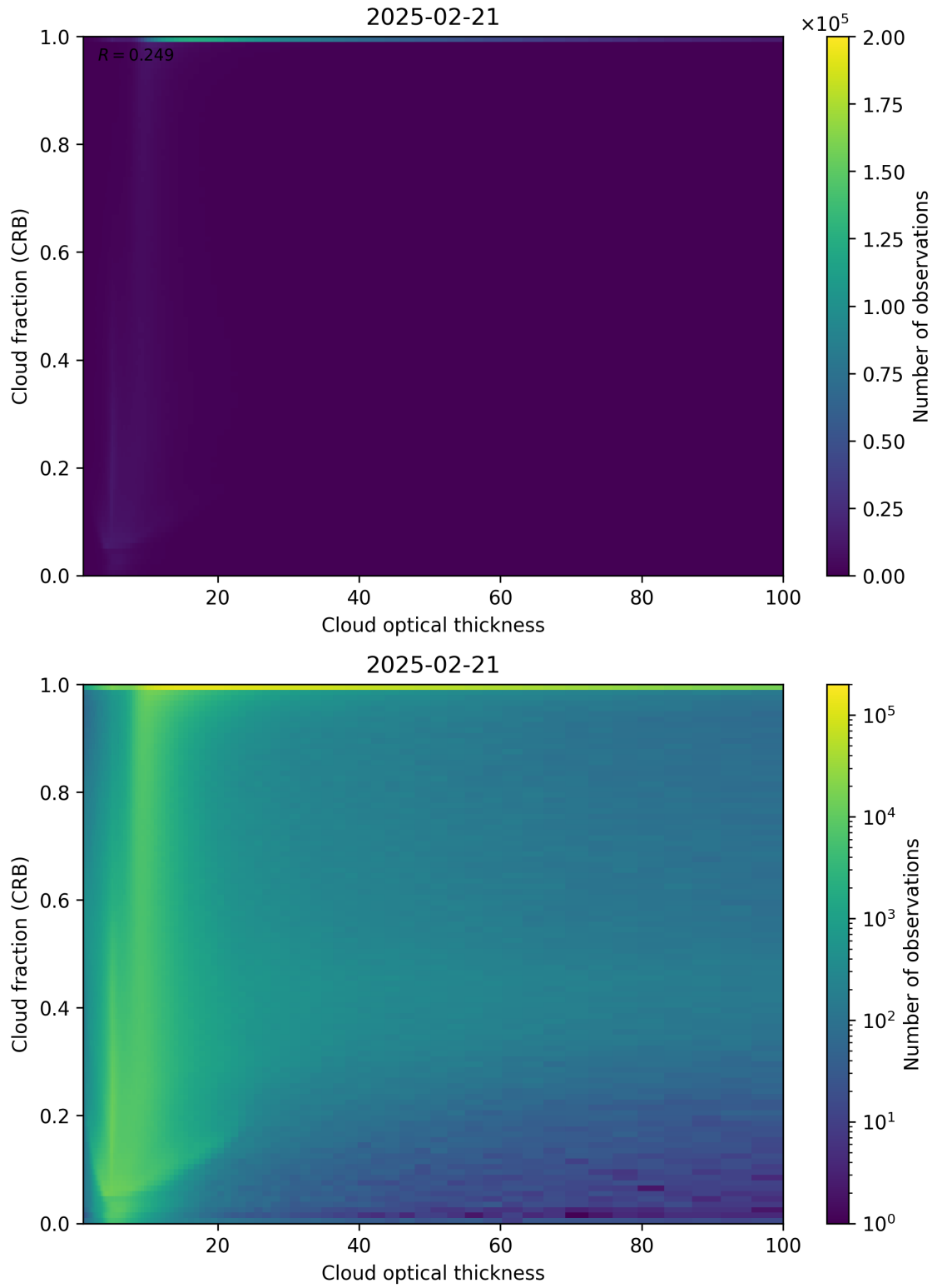
Figure 84: Scatter density plot of “Cloud optical thickness” against “Cloud fraction (CRB)” for 2025-02-20 to 2025-02-22.
