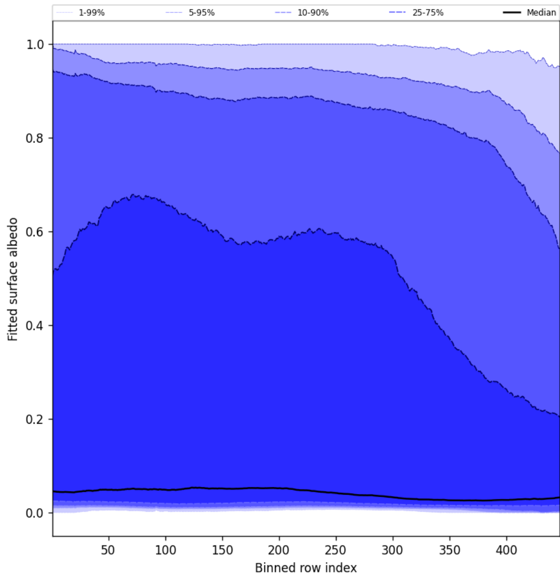
Figure 61: Along track statistics of “Fitted surface albedo” for 2025-02-20 to 2025-02-22
