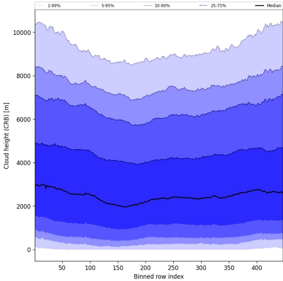
Figure 59: Along track statistics of “Cloud height (CRB)” for 2025-02-20 to 2025-02-22
