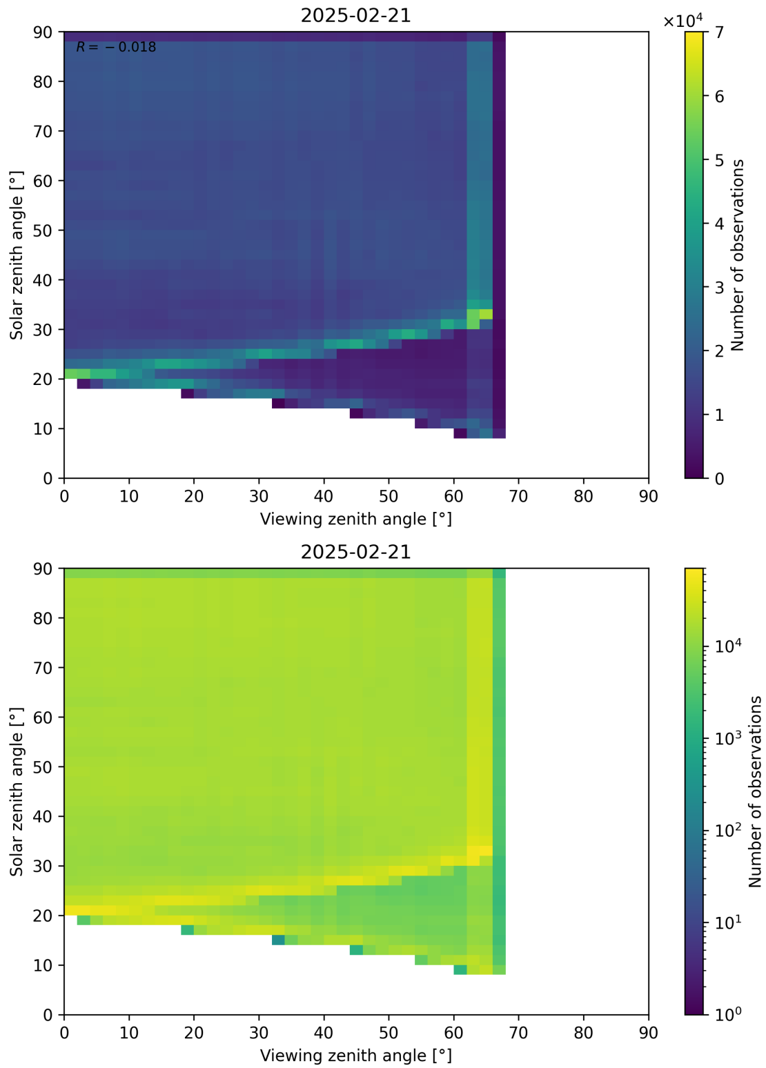
Figure 114: Scatter density plot of “Viewing zenith angle” against “Solar zenith angle” for 2025-02-20 to 2025-02-22.
