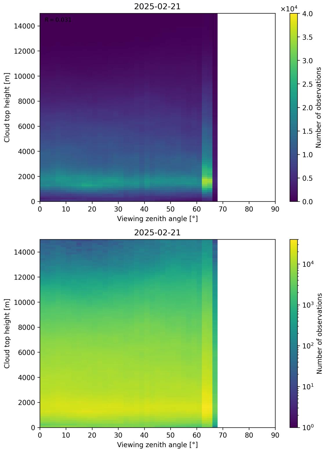
Figure 112: Scatter density plot of “Viewing zenith angle” against “Cloud top height” for 2025-02-20 to 2025-02-22.
