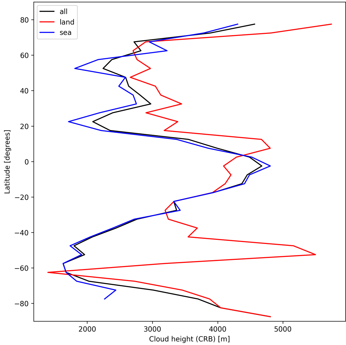
Figure 27: Zonal average of “Cloud height (CRB)” for 2025-02-20 to 2025-02-22.
