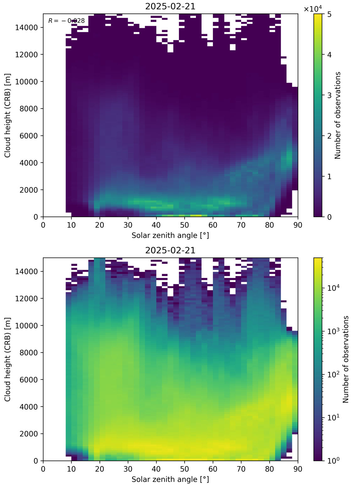
Figure 102: Scatter density plot of “Solar zenith angle” against “Cloud height (CRB)” for 2025-02-20 to 2025-02-22.
