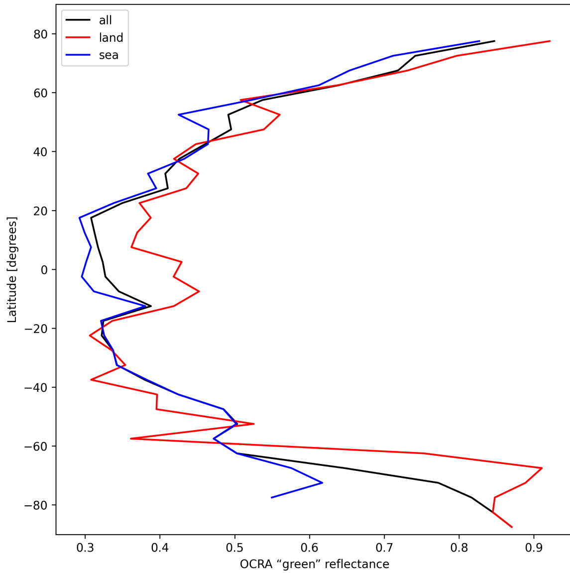
Figure 36: Zonal average of “OCRA “green” reflectance” for 2025-02-20 to 2025-02-22.
