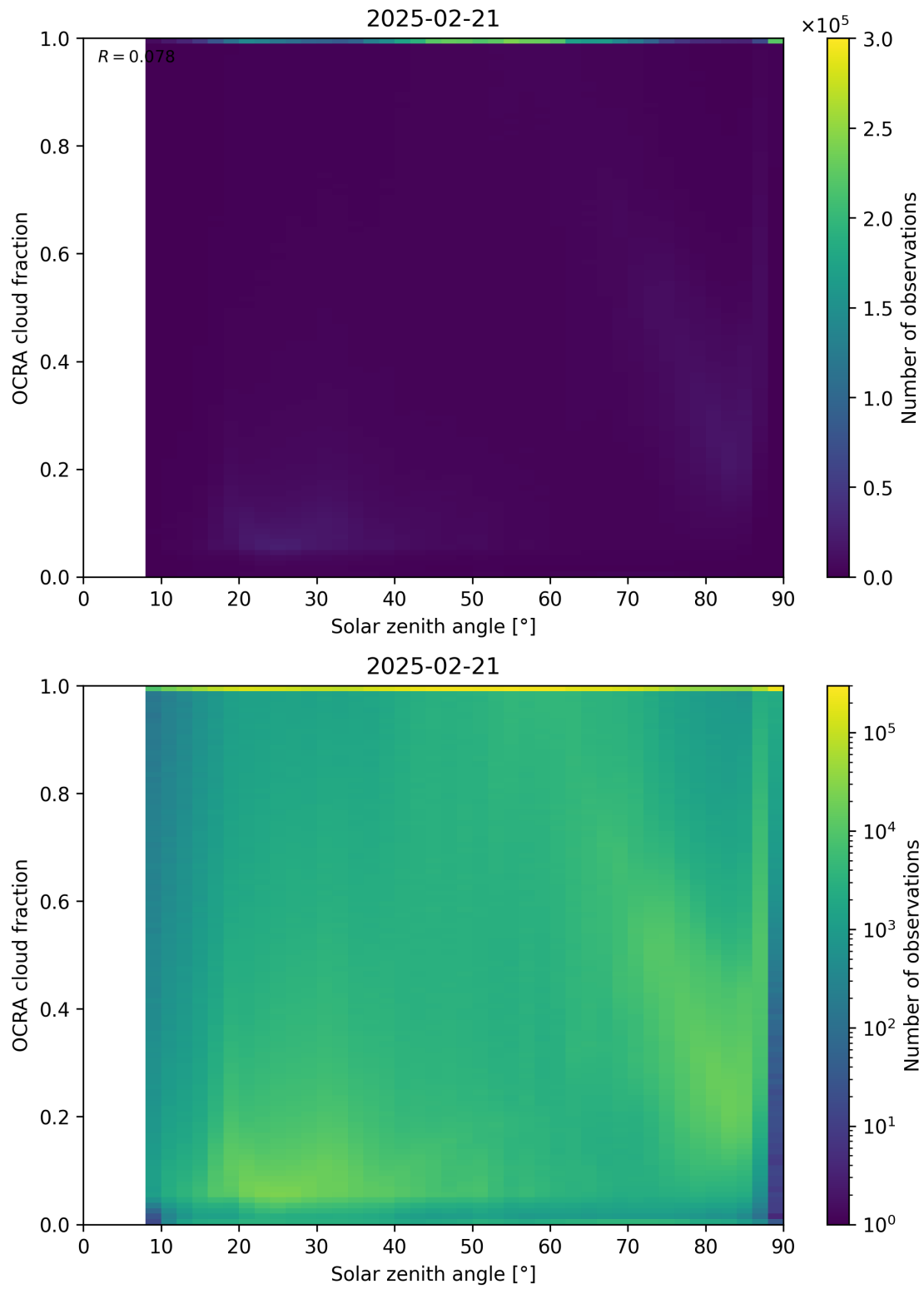
Figure 100: Scatter density plot of “Solar zenith angle” against “OCRA cloud fraction” for 2025-02-20 to 2025-02-22.
