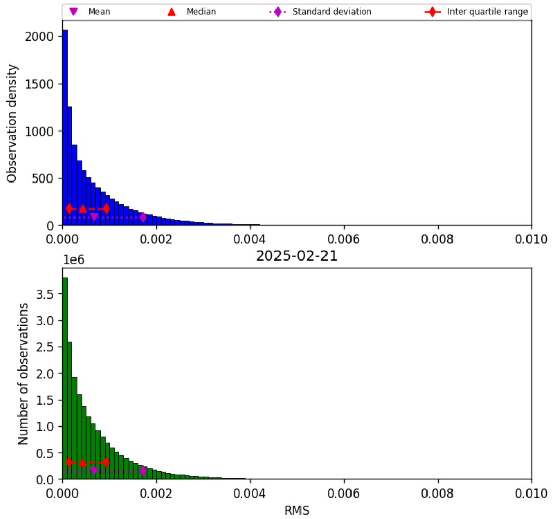
Figure 47: Histogram of “RMS” for 2025-02-20 to 2025-02-22
