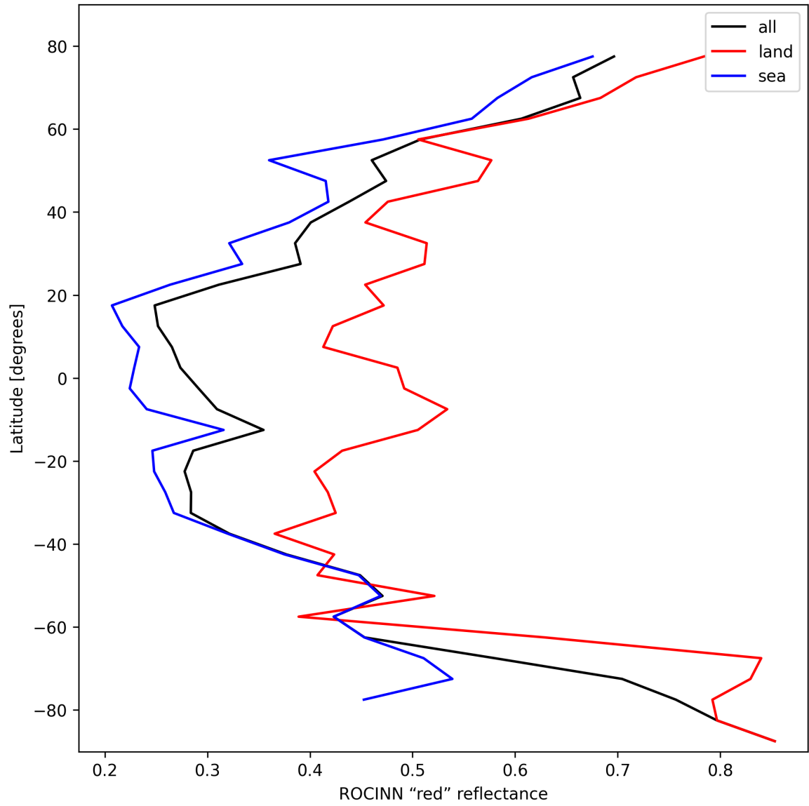
Figure 37: Zonal average of "ROCINN "red" reflectance" for 2025-02-20 to 2025-02-22.
