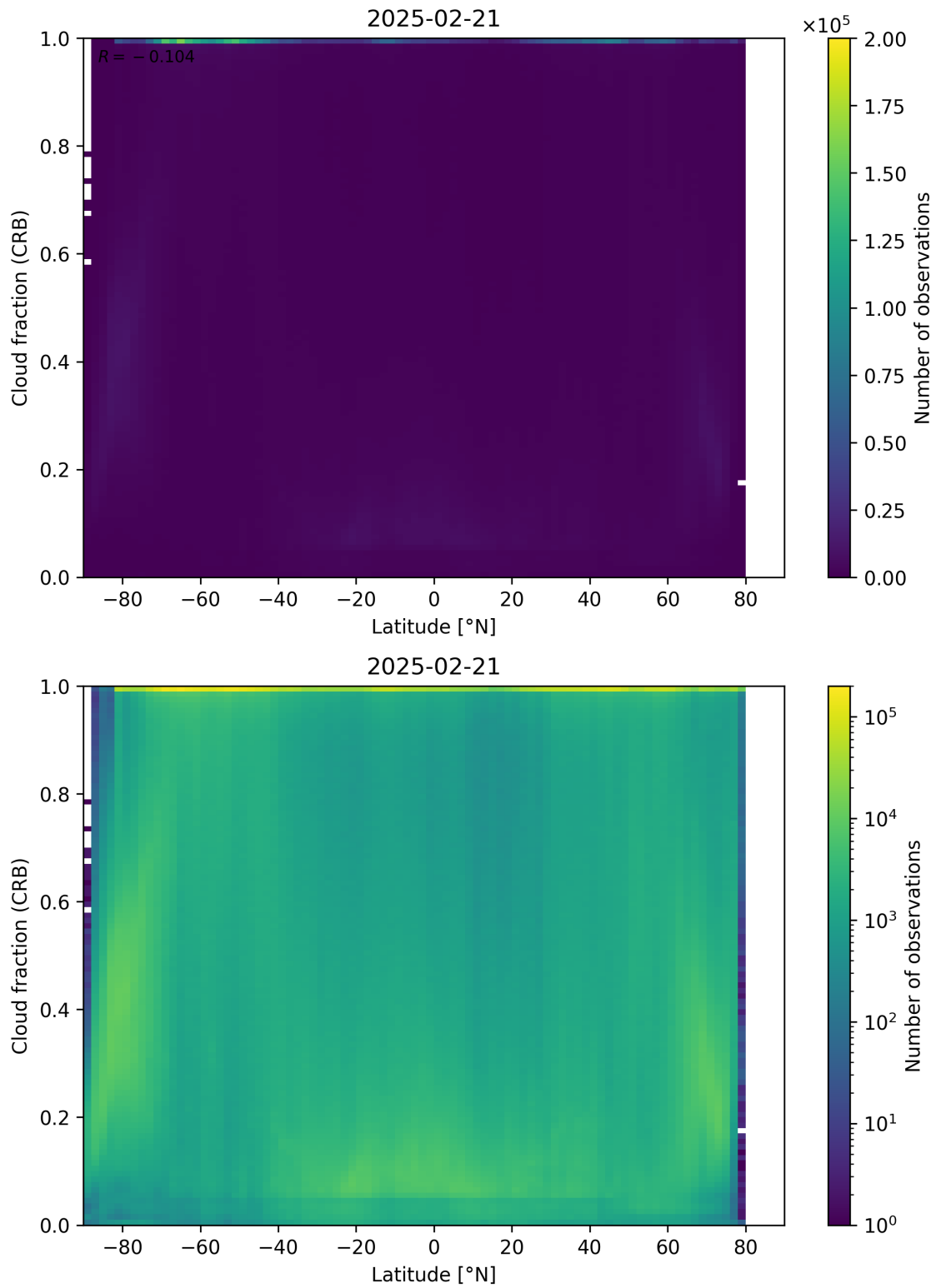
Figure 94: Scatter density plot of “Latitude” against “Cloud fraction (CRB)” for 2025-02-20 to 2025-02-22.
