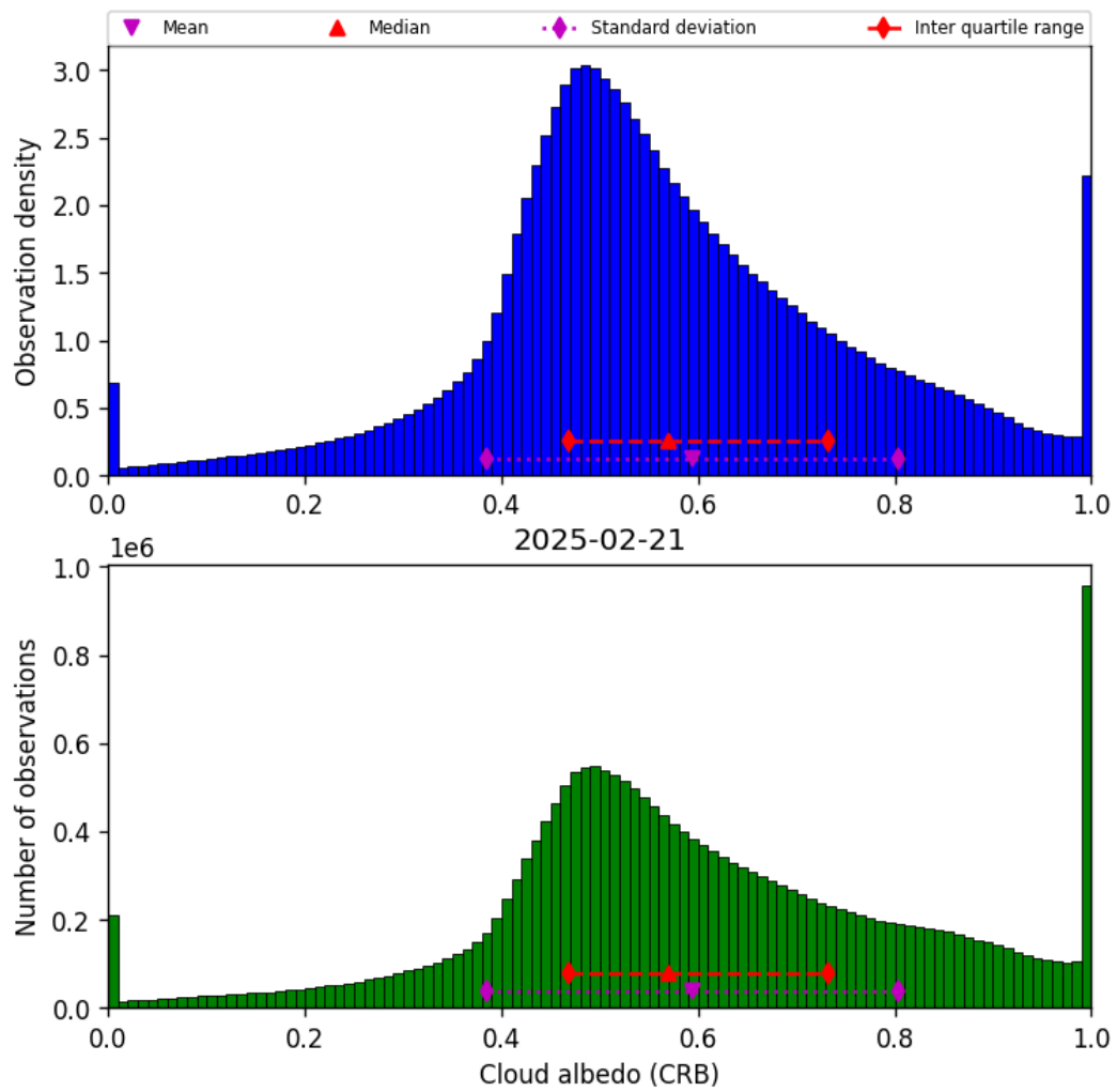
Figure 44: Histogram of “Cloud albedo (CRB)” for 2025-02-20 to 2025-02-22
