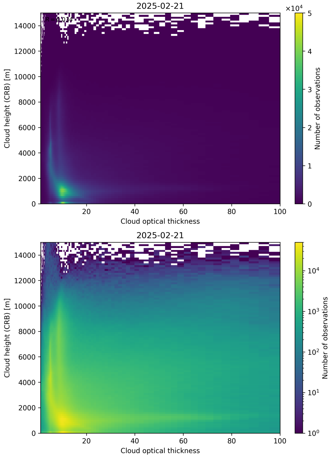
Figure 85: Scatter density plot of “Cloud optical thickness” against “Cloud height (CRB)” for 2025-02-20 to 2025-02-22.
