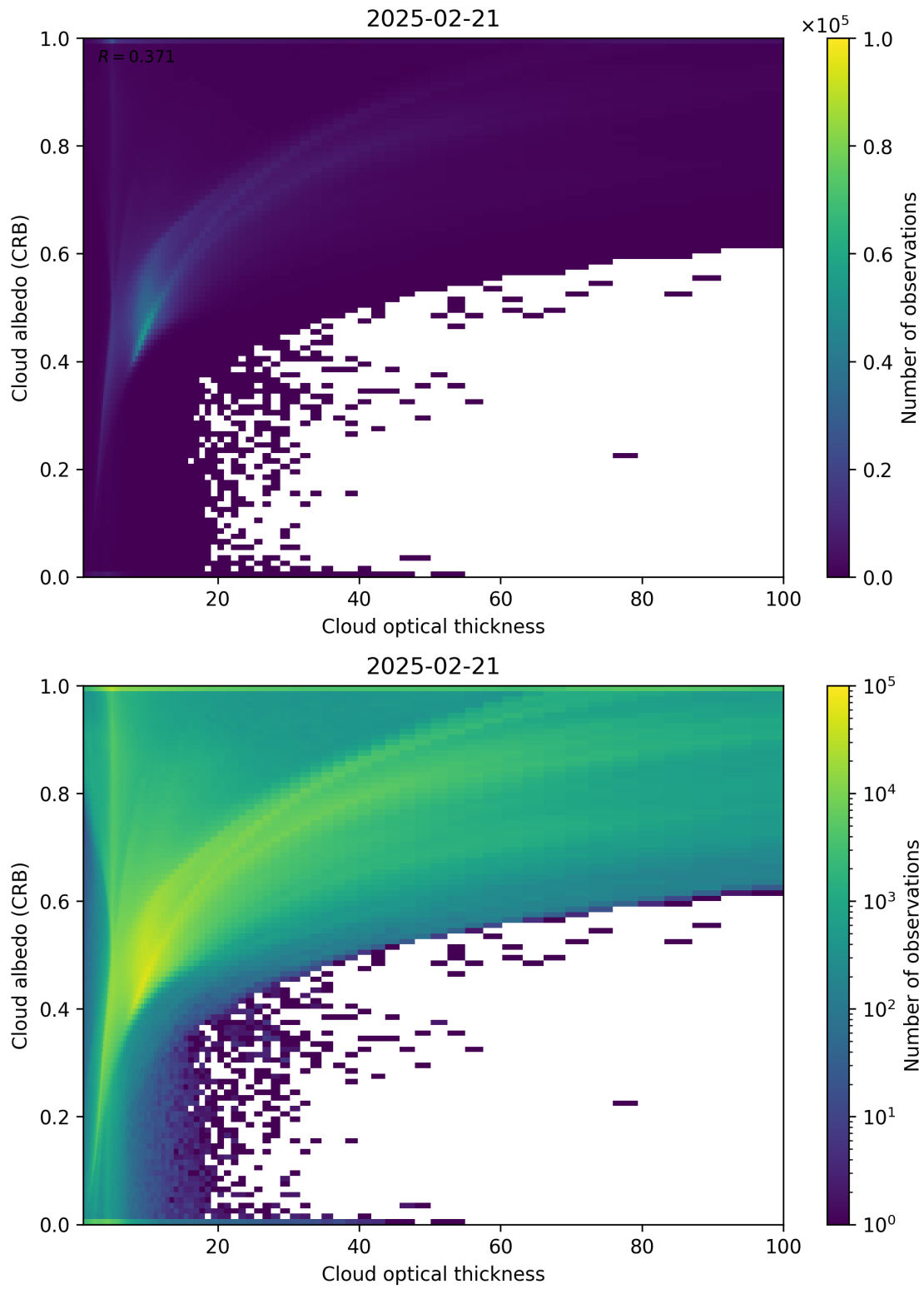
Figure 82: Scatter density plot of “Cloud optical thickness” against “Cloud albedo (CRB)” for 2025-02-20 to 2025-02-22.
