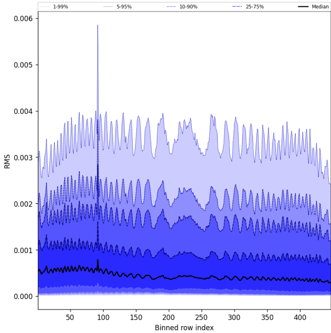
Figure 63: Along track statistics of “RMS” for 2025-02-20 to 2025-02-22
