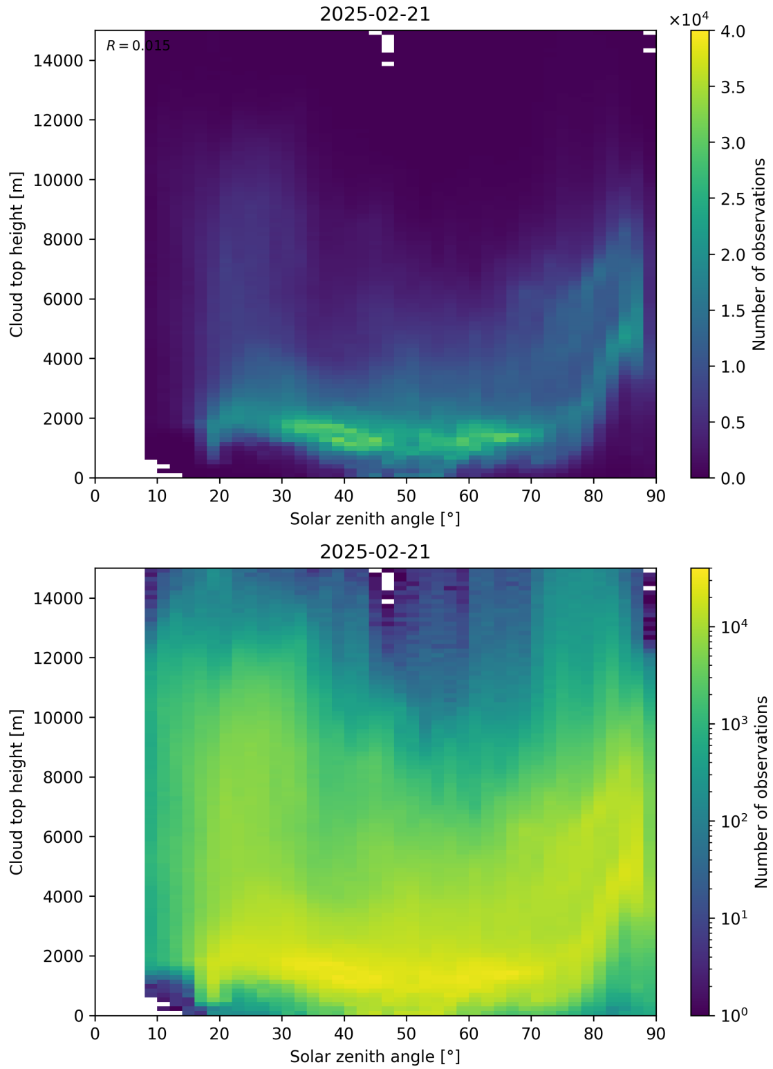
Figure 104: Scatter density plot of “Solar zenith angle” against “Cloud top height” for 2025-02-20 to 2025-02-22.
