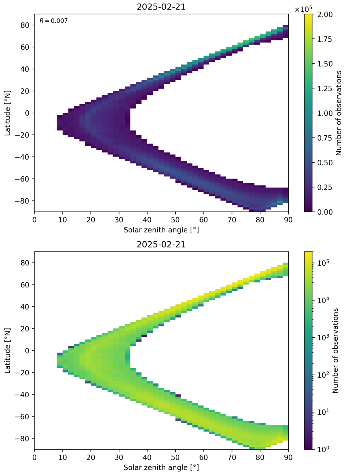
Figure 105: Scatter density plot of “Solar zenith angle” against “Latitude” for 2025-02-20 to 2025-02-22.
