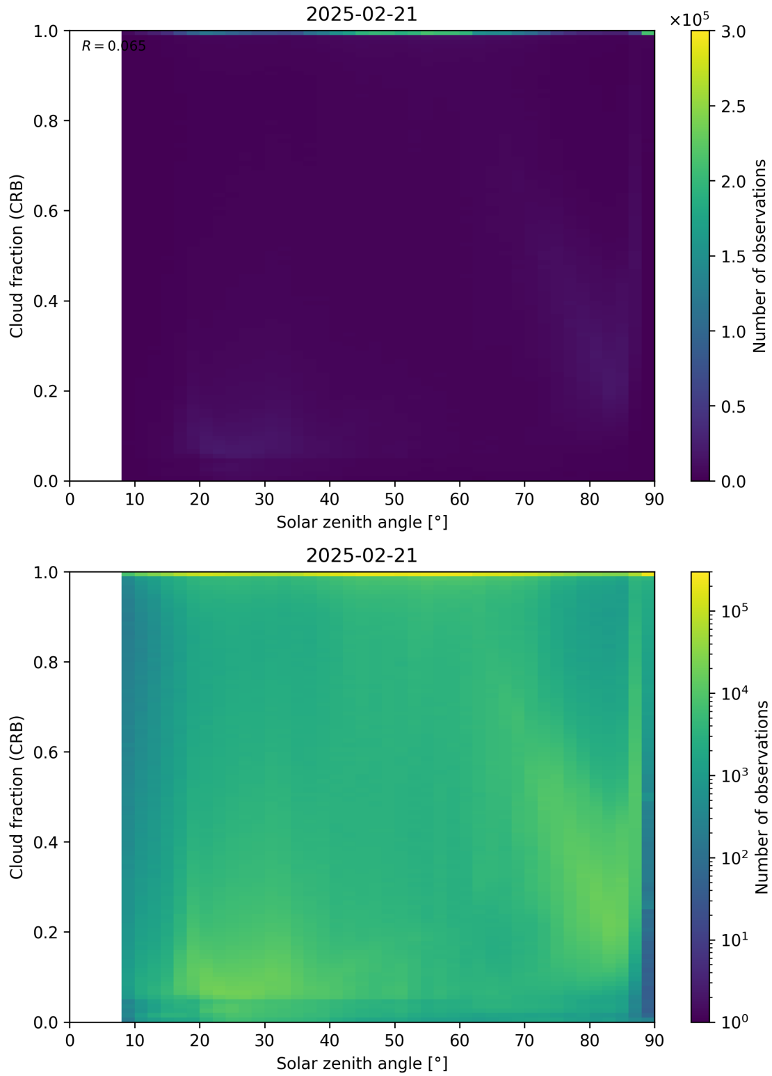
Figure 101: Scatter density plot of “Solar zenith angle” against “Cloud fraction (CRB)” for 2025-02-20 to 2025-02-22.
