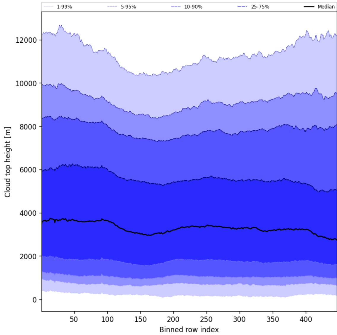
Figure 56: Along track statistics of “Cloud top height” for 2025-02-20 to 2025-02-22
