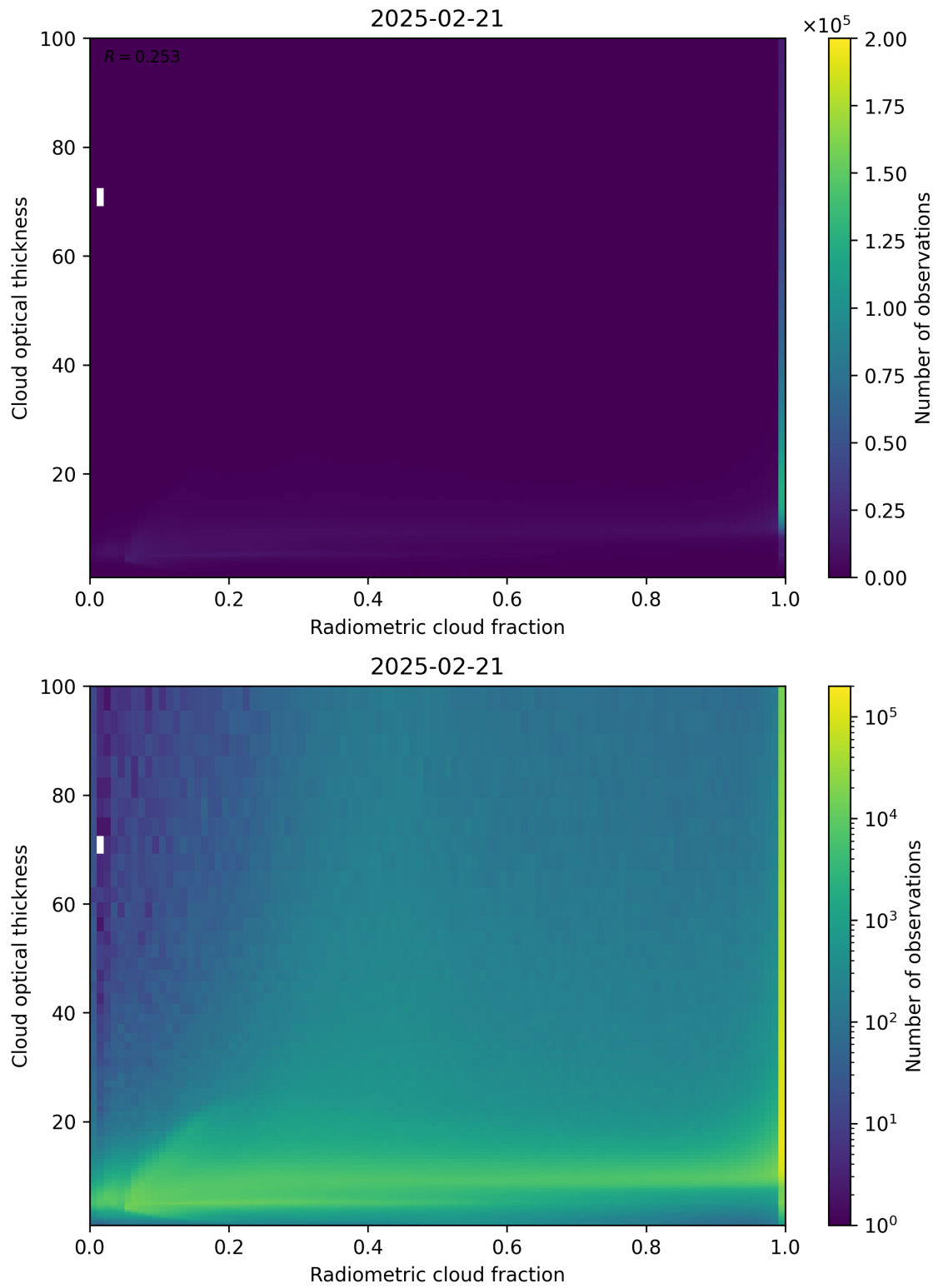
Figure 75: Scatter density plot of “Radiometric cloud fraction” against “Cloud optical thickness” for 2025-02-20 to 2025-02-22.
