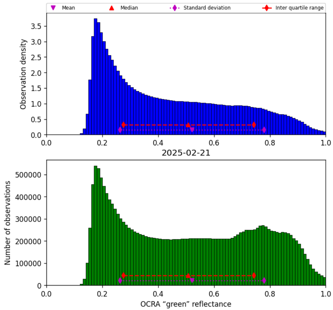
Figure 52: Histogram of “OCRA “green” reflectance” for 2025-02-20 to 2025-02-22
