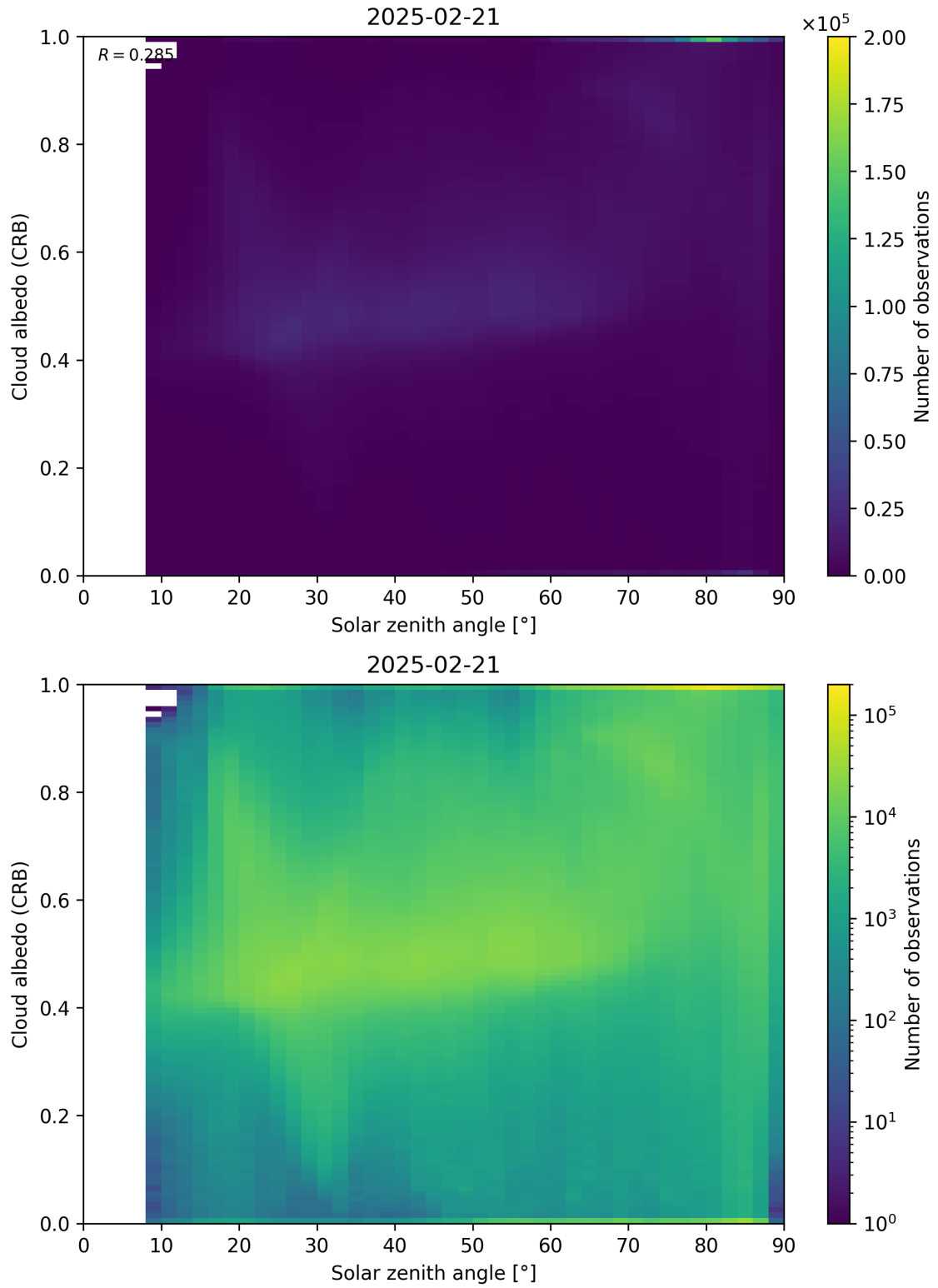
Figure 98: Scatter density plot of “Solar zenith angle” against “Cloud albedo (CRB)” for 2025-02-20 to 2025-02-22.
