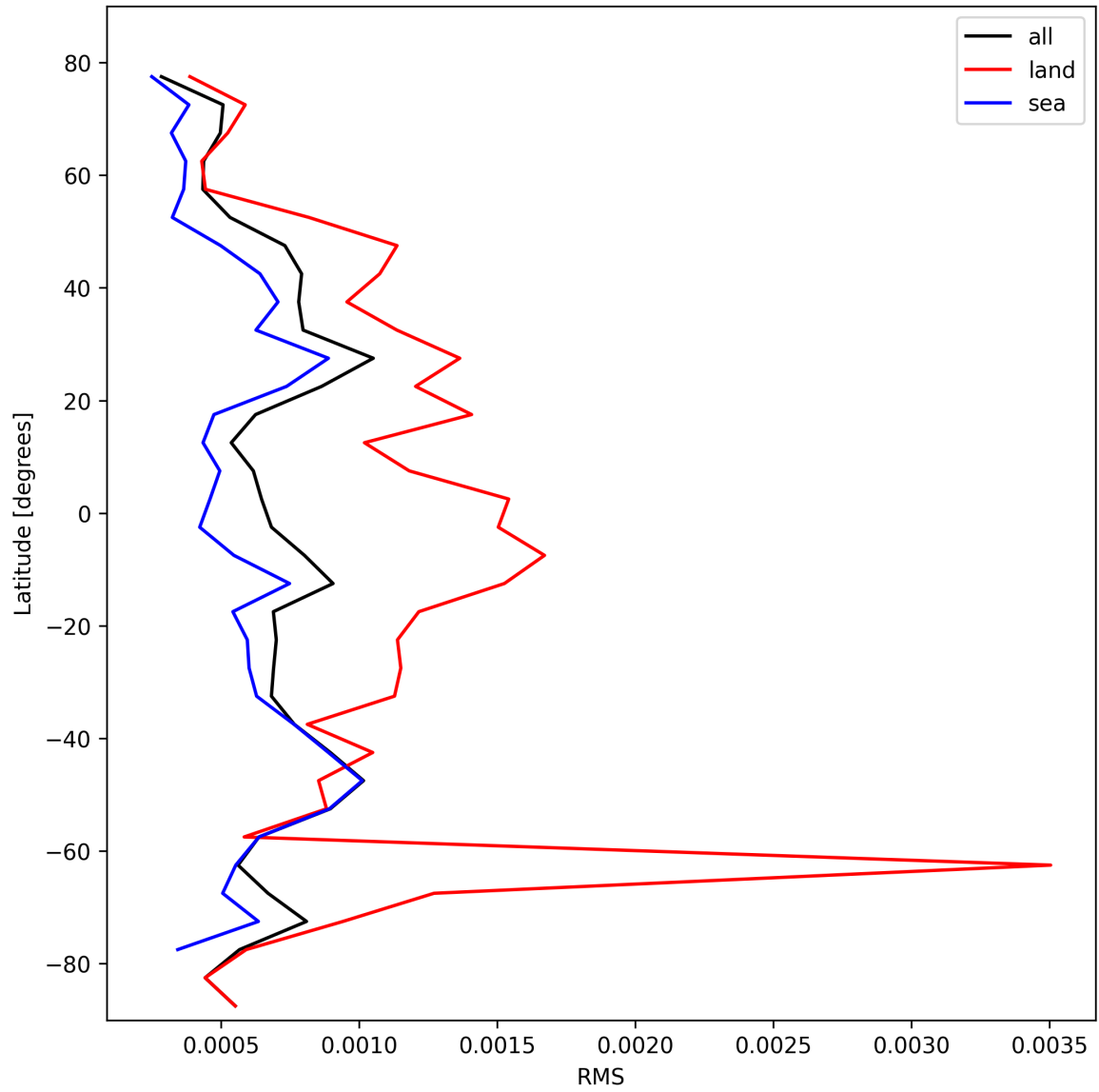
Figure 31: Zonal average of “RMS” for 2025-02-20 to 2025-02-22.
