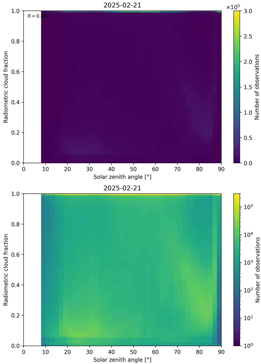
Figure 99: Scatter density plot of “Solar zenith angle” against “Radiometric cloud fraction” for 2025-02-20 to 2025-02-22.
