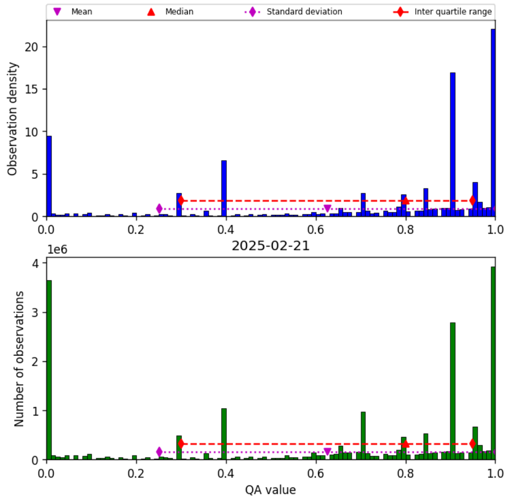
Figure 38: Histogram of “QA value” for 2025-02-20 to 2025-02-22
