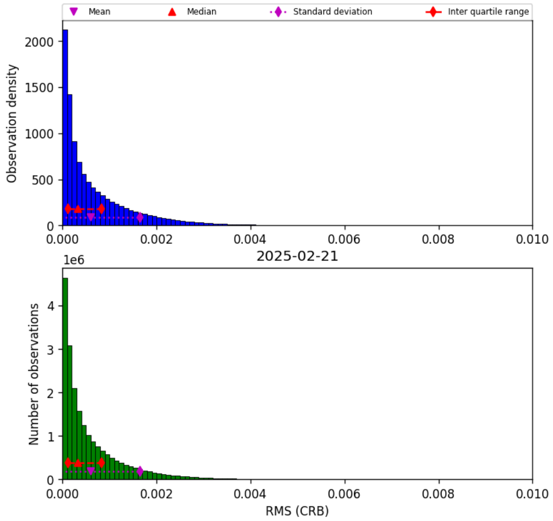
Figure 48: Histogram of “RMS (CRB)” for 2025-02-20 to 2025-02-22
