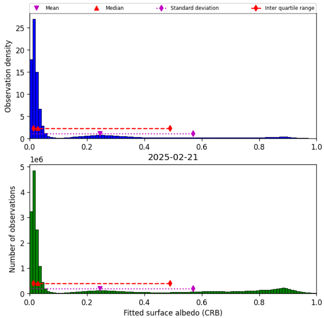
Figure 46: Histogram of “Fitted surface albedo (CRB)” for 2025-02-20 to 2025-02-22
