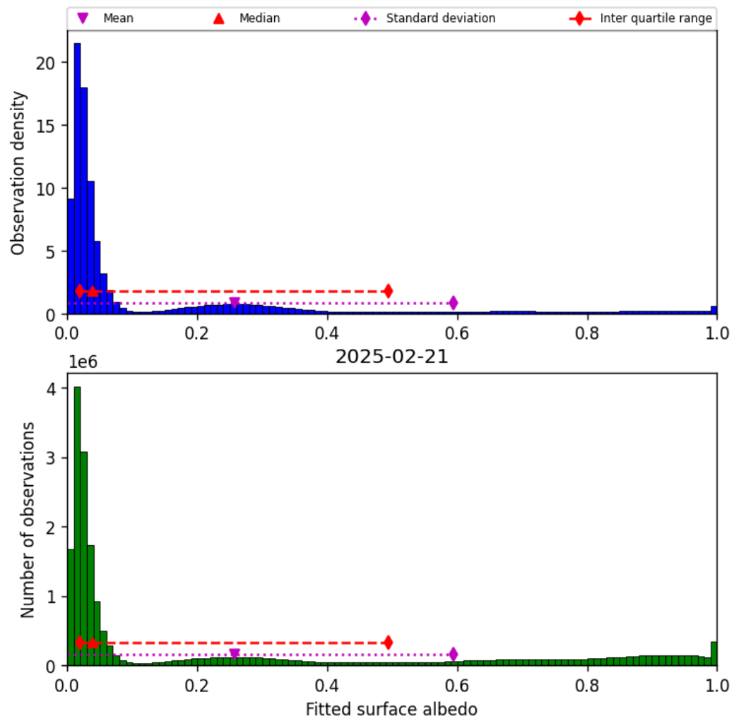
Figure 45: Histogram of “Fitted surface albedo” for 2025-02-20 to 2025-02-22
