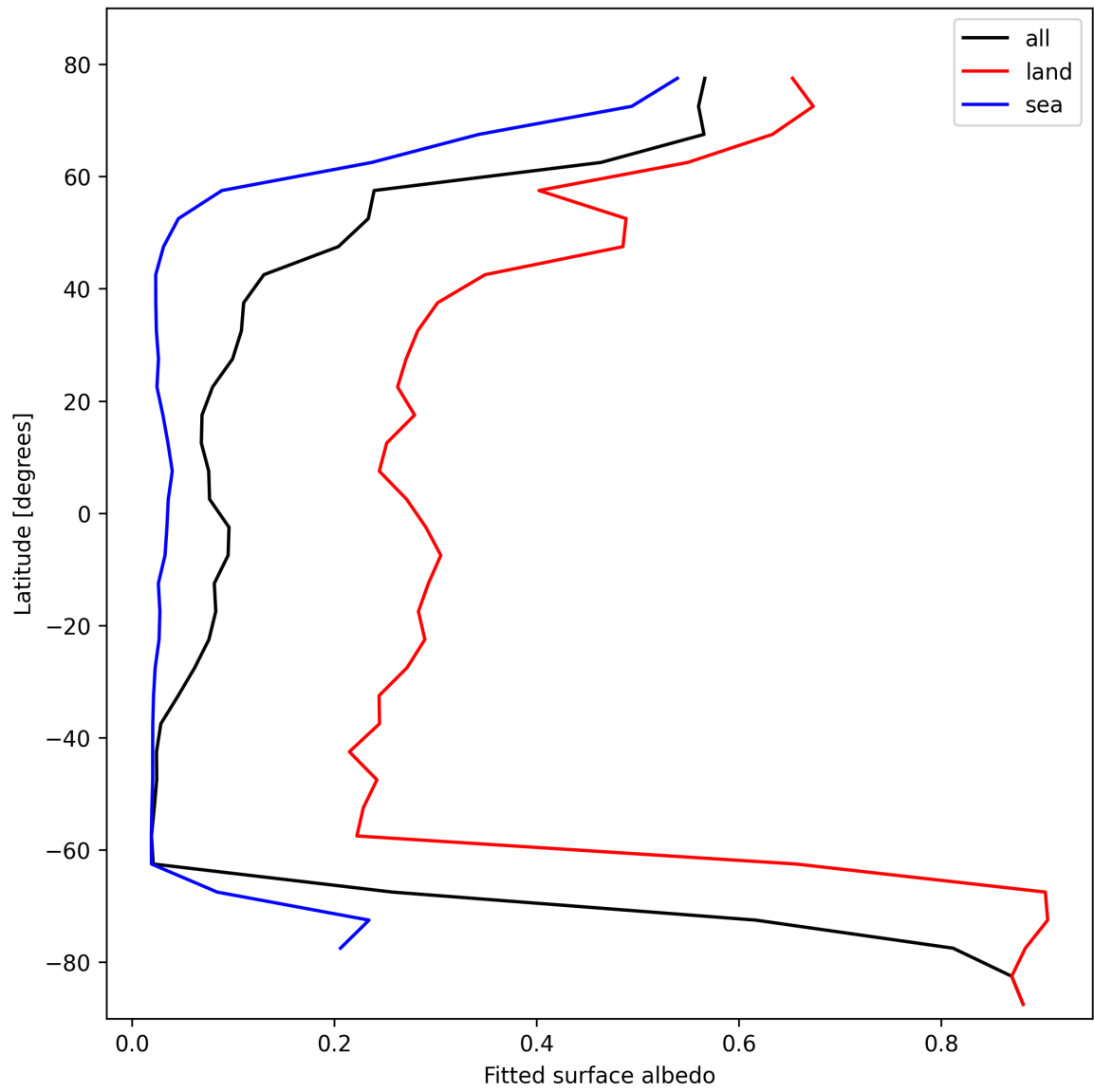
Figure 29: Zonal average of “Fitted surface albedo” for 2025-02-20 to 2025-02-22.
