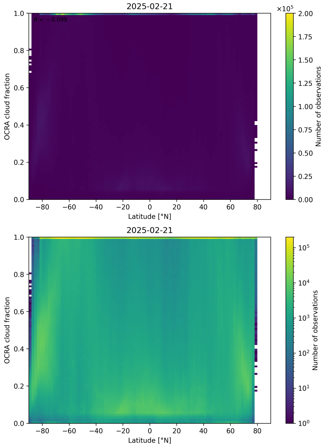
Figure 93: Scatter density plot of “Latitude” against “OCRA cloud fraction” for 2025-02-20 to 2025-02-22.
