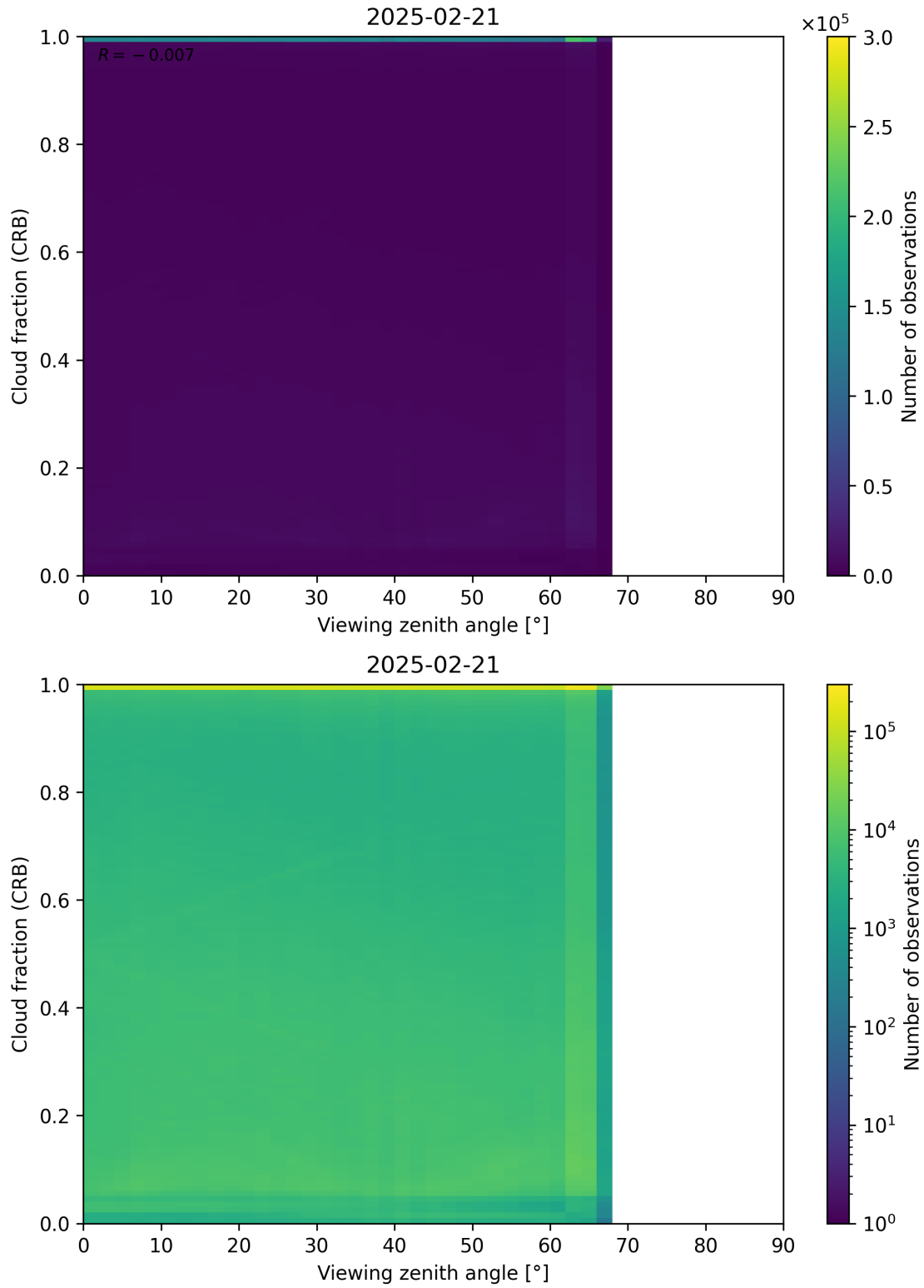
Figure 109: Scatter density plot of “Viewing zenith angle” against “Cloud fraction (CRB)” for 2025-02-20 to 2025-02-22.
