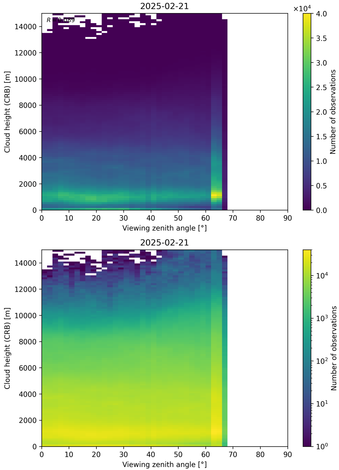
Figure 110: Scatter density plot of “Viewing zenith angle” against “Cloud height (CRB)” for 2025-02-20 to 2025-02-22.
