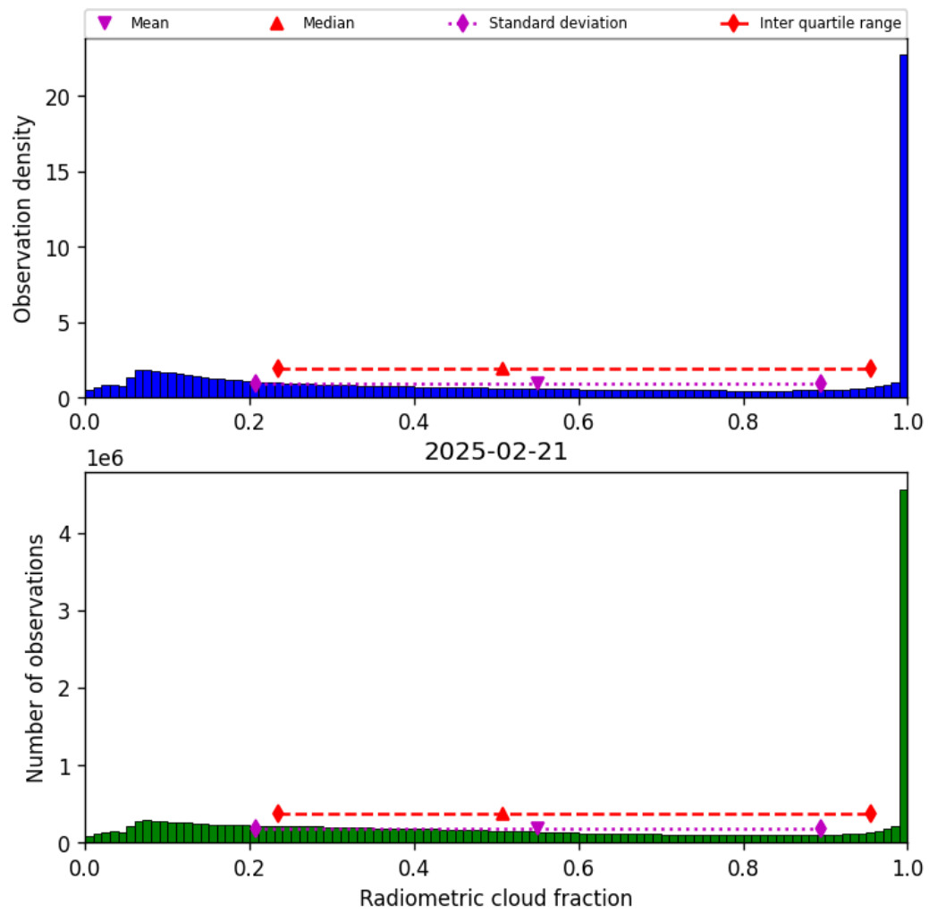
Figure 39: Histogram of “Radiometric cloud fraction” for 2025-02-20 to 2025-02-22
