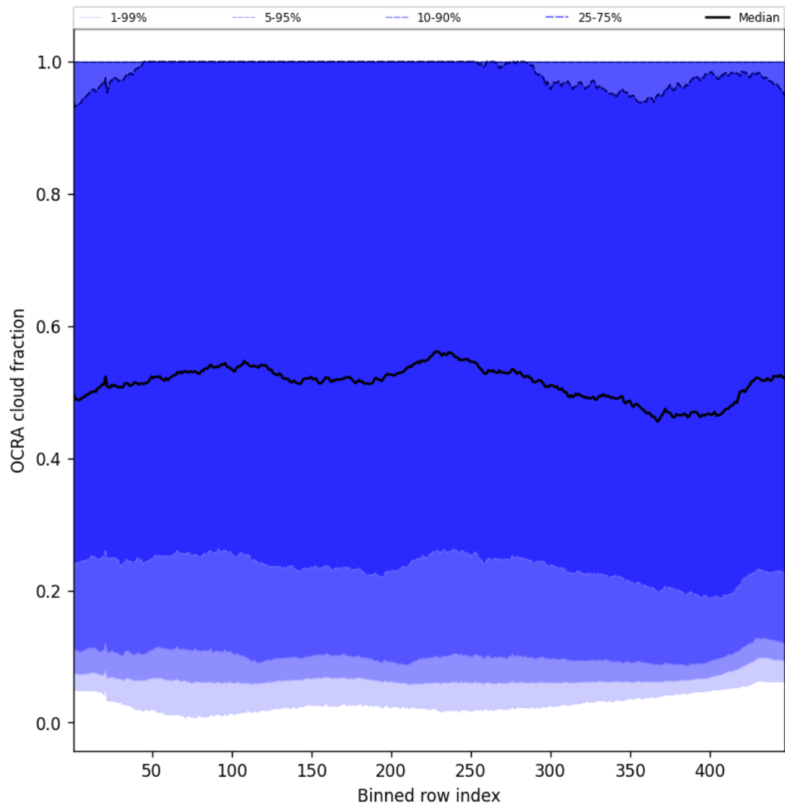
Figure 66: Along track statistics of “OCRA cloud fraction” for 2025-02-20 to 2025-02-22
