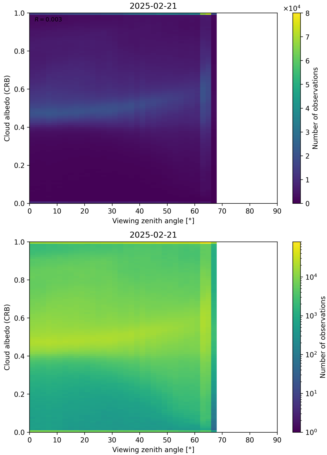
Figure 106: Scatter density plot of “Viewing zenith angle” against “Cloud albedo (CRB)” for 2025-02-20 to 2025-02-22.
