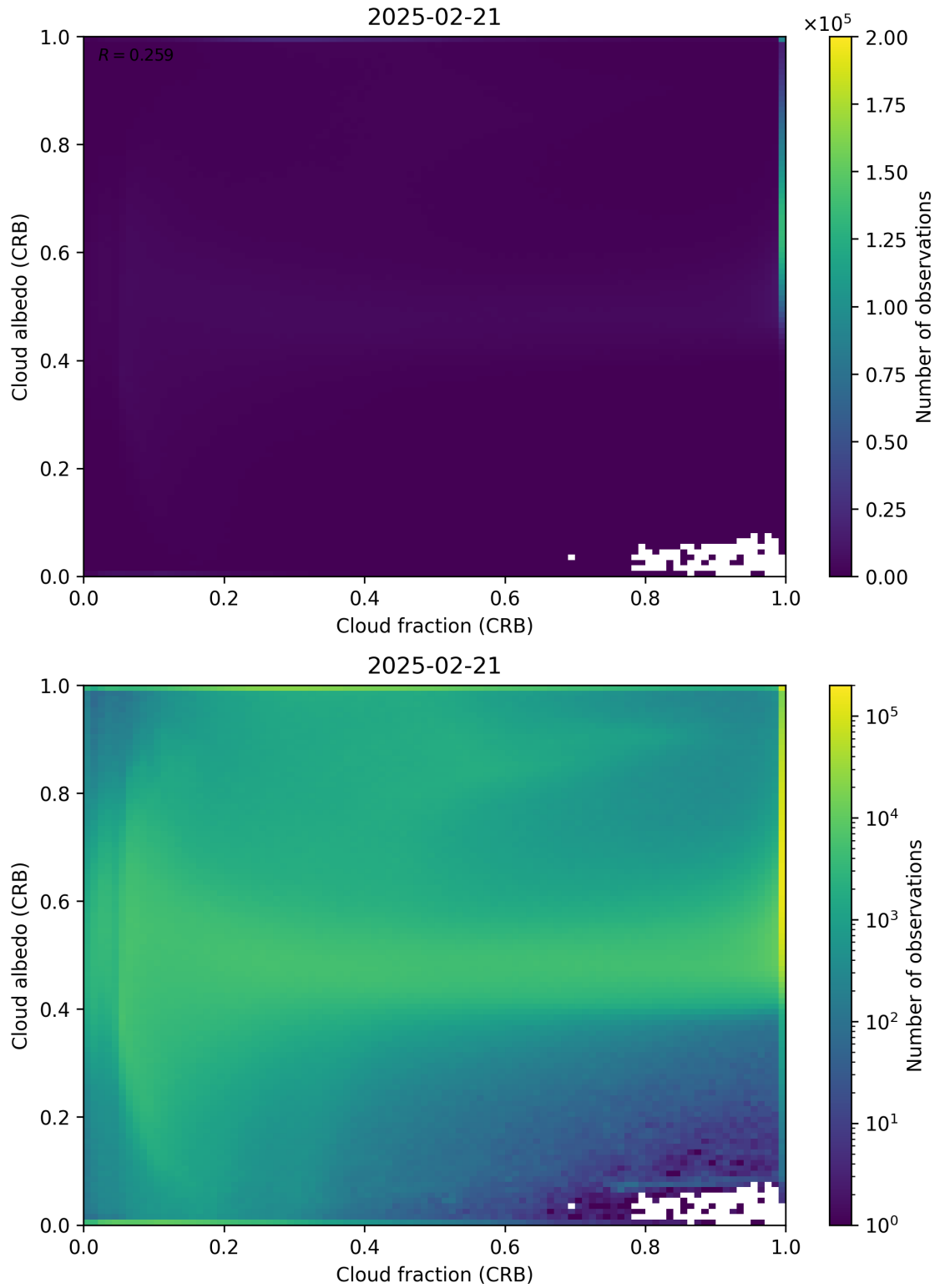
Figure 77: Scatter density plot of “Cloud fraction (CRB)” against “Cloud albedo (CRB)” for 2025-02-20 to 2025-02-22.
