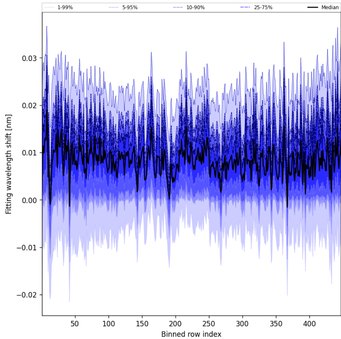
Figure 65: Along track statistics of “Fitting wavelength shift” for 2025-02-20 to 2025-02-22
