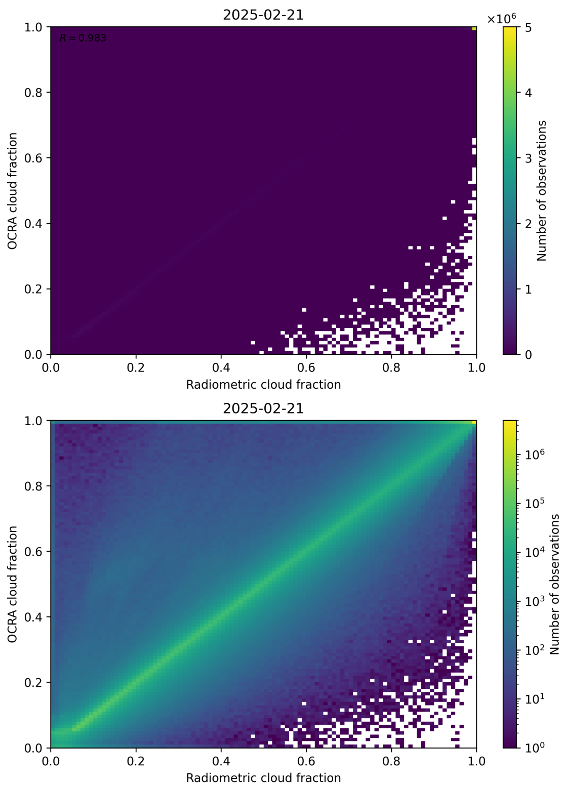
Figure 72: Scatter density plot of “Radiometric cloud fraction” against “OCRA cloud fraction” for 2025-02-20 to 2025-02-22.
