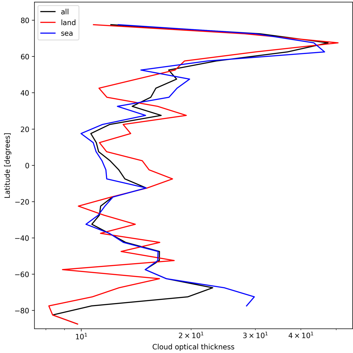
Figure 25: Zonal average of “Cloud optical thickness” for 2025-02-20 to 2025-02-22.
