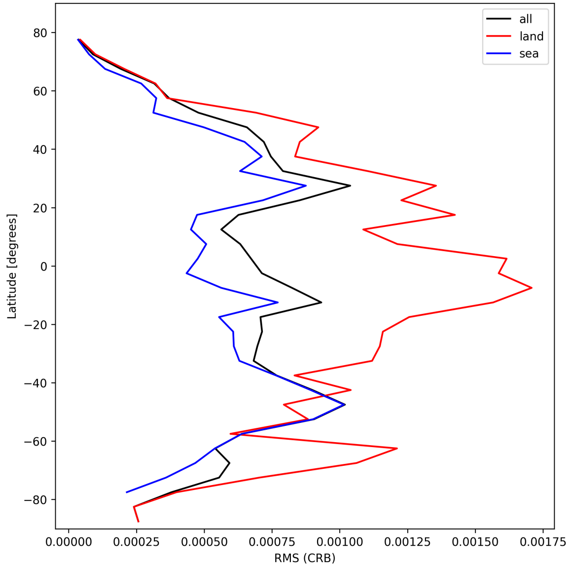
Figure 32: Zonal average of “RMS (CRB)” for 2025-02-20 to 2025-02-22.
