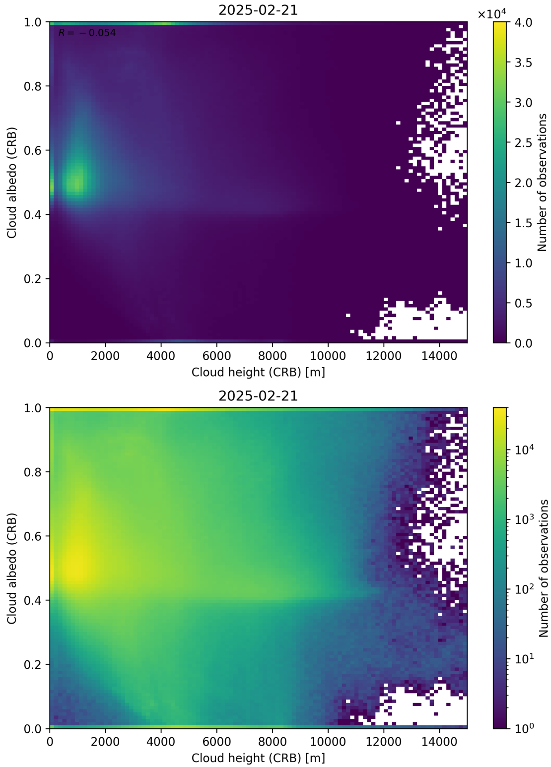
Figure 80: Scatter density plot of “Cloud height (CRB)” against “Cloud albedo (CRB)” for 2025-02-20 to 2025-02-22.
