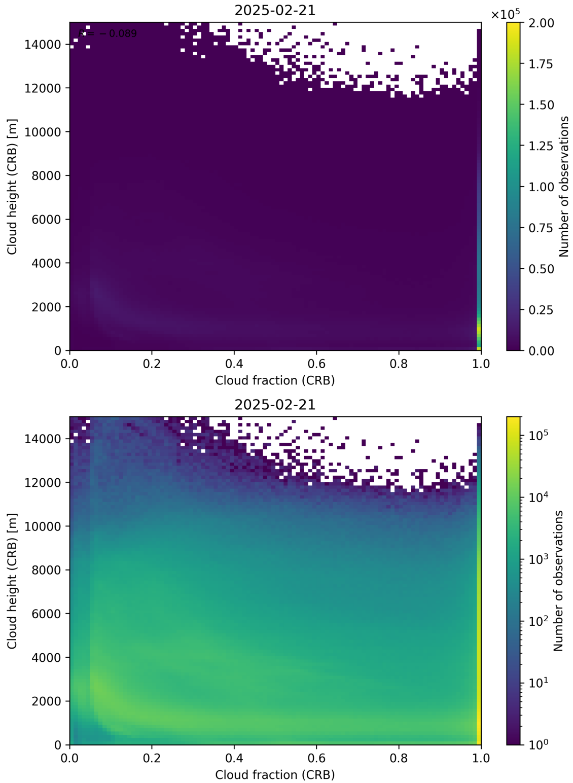
Figure 79: Scatter density plot of “Cloud fraction (CRB)” against “Cloud height (CRB)” for 2025-02-20 to 2025-02-22.
