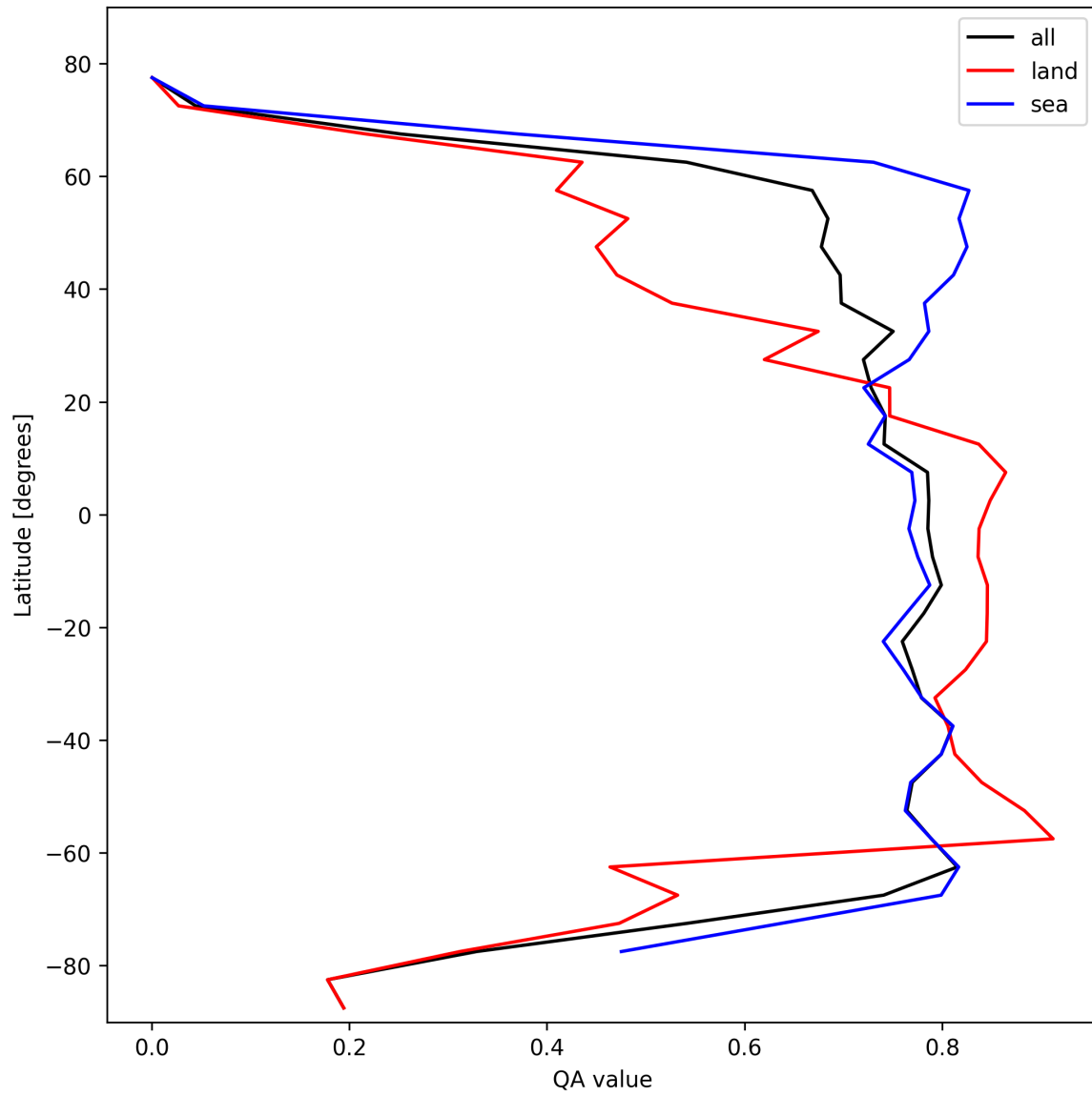
Figure 22: Zonal average of “QA value” for 2025-02-20 to 2025-02-22.
