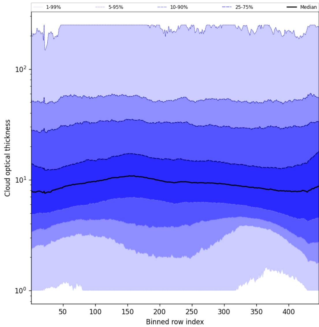
Figure 57: Along track statistics of “Cloud optical thickness” for 2025-02-20 to 2025-02-22
