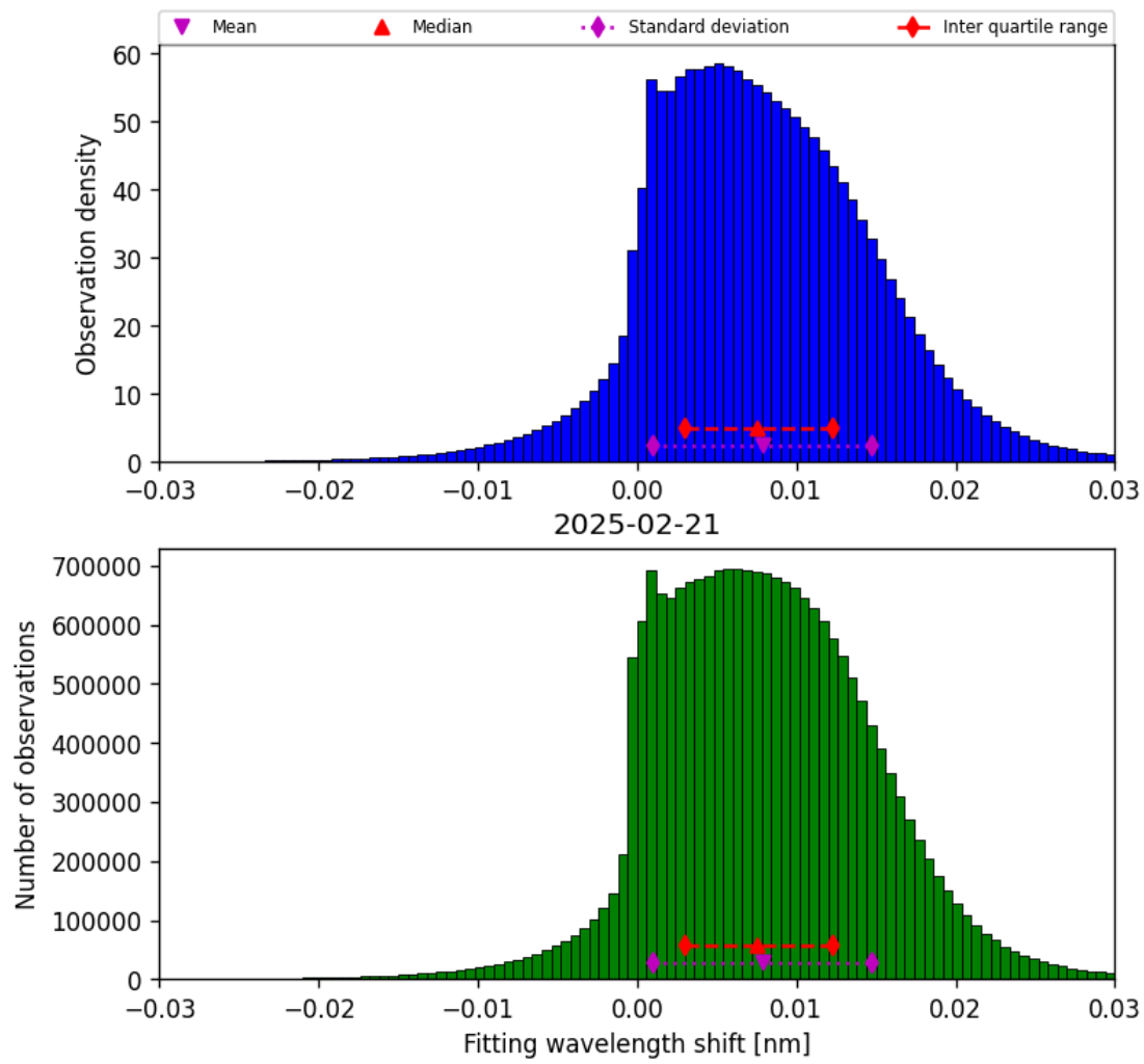
Figure 49: Histogram of “Fitting wavelength shift” for 2025-02-20 to 2025-02-22
