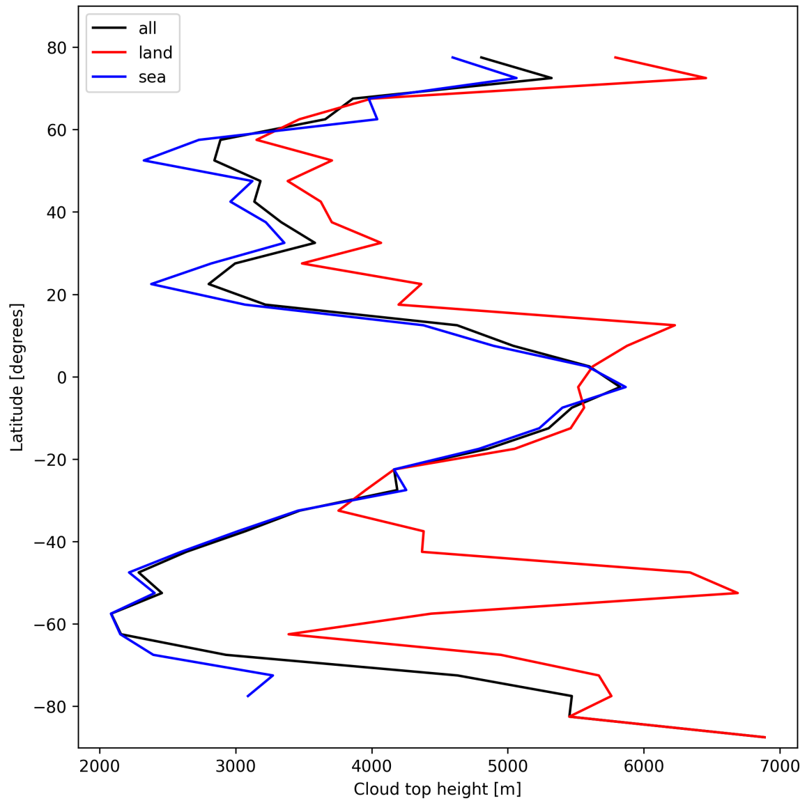
Figure 24: Zonal average of “Cloud top height” for 2025-02-20 to 2025-02-22.
