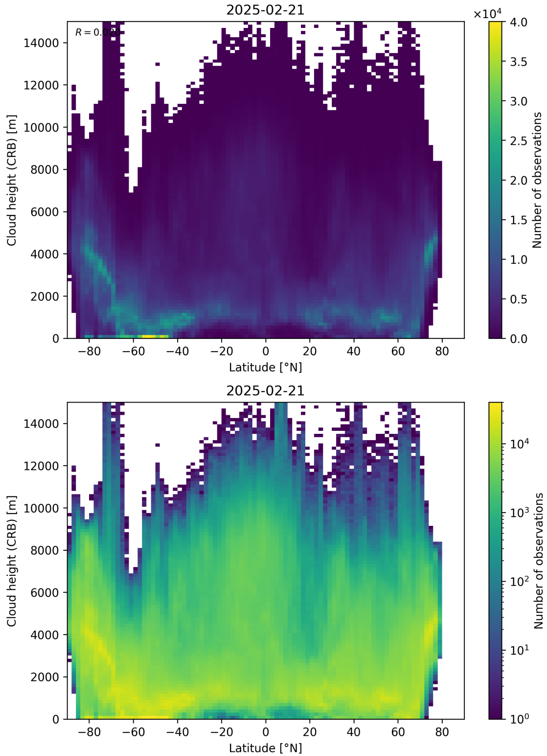
Figure 95: Scatter density plot of “Latitude” against “Cloud height (CRB)” for 2025-02-20 to 2025-02-22.
