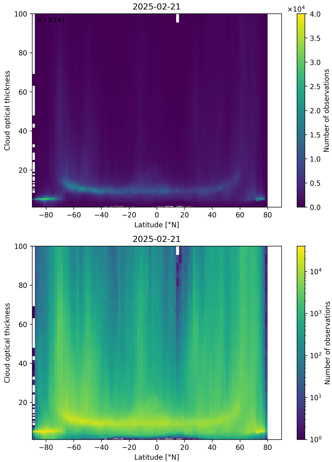
Figure 96: Scatter density plot of “Latitude” against “Cloud optical thickness” for 2025-02-20 to 2025-02-22.
