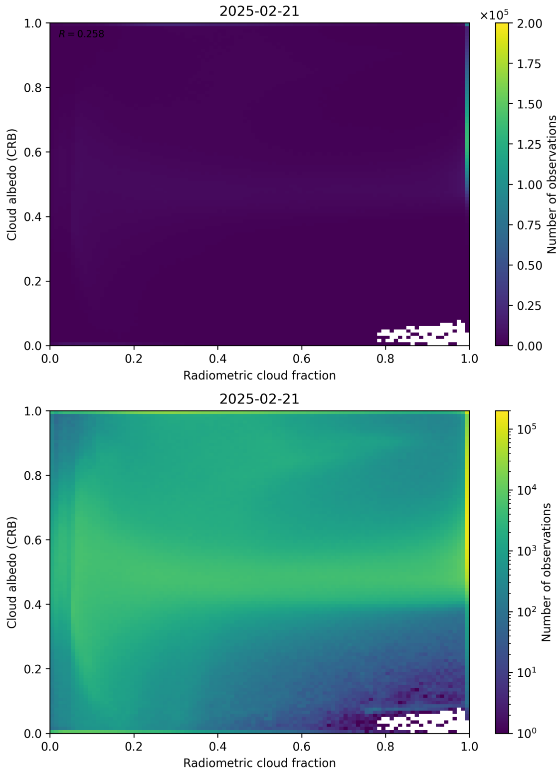
Figure 71: Scatter density plot of “Radiometric cloud fraction” against “Cloud albedo (CRB)” for 2025-02-20 to 2025-02-22.
