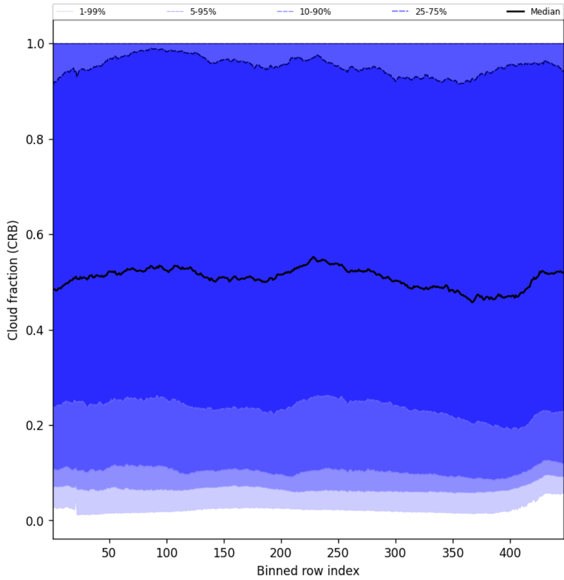
Figure 58: Along track statistics of “Cloud fraction (CRB)” for 2025-02-20 to 2025-02-22
