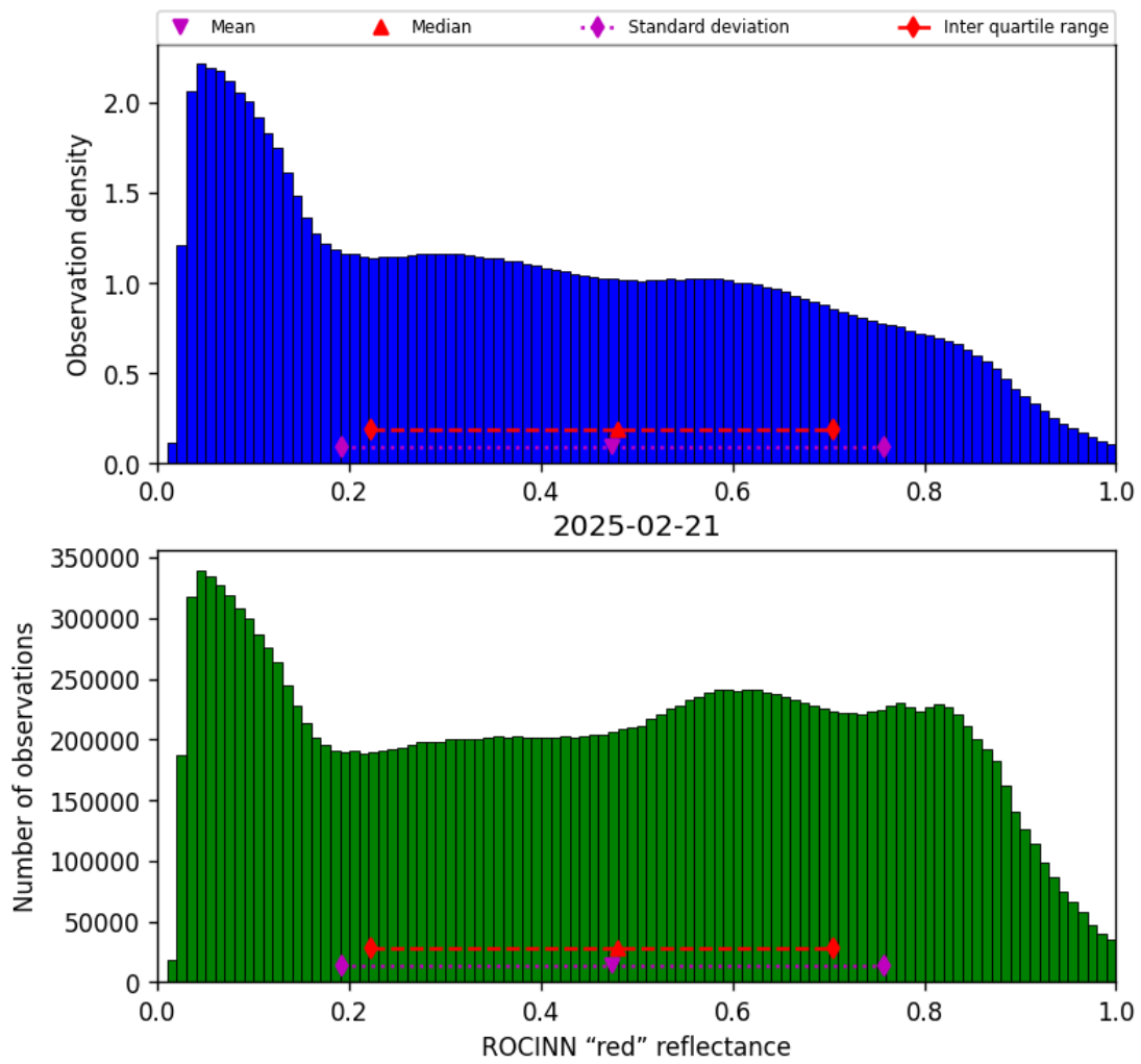
Figure 53: Histogram of “ROCINN “red” reflectance” for 2025-02-20 to 2025-02-22
