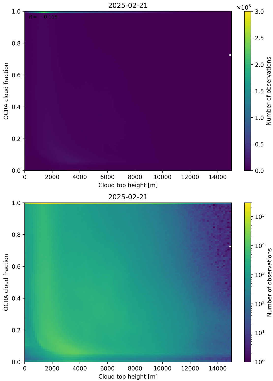
Figure 87: Scatter density plot of “Cloud top height” against “OCRA cloud fraction” for 2025-02-20 to 2025-02-22.
