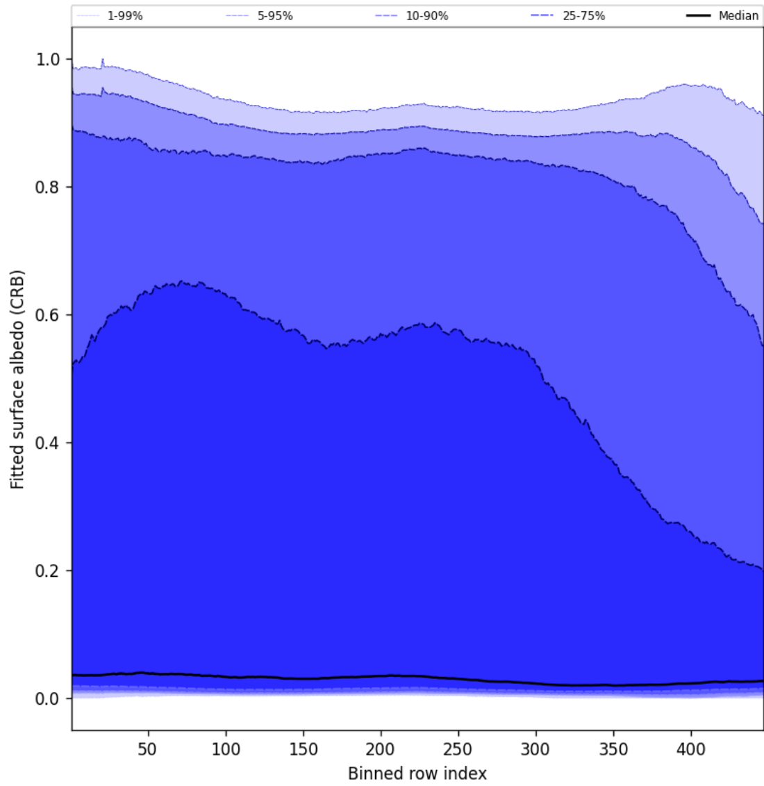
Figure 62: Along track statistics of “Fitted surface albedo (CRB)” for 2025-02-20 to 2025-02-22
