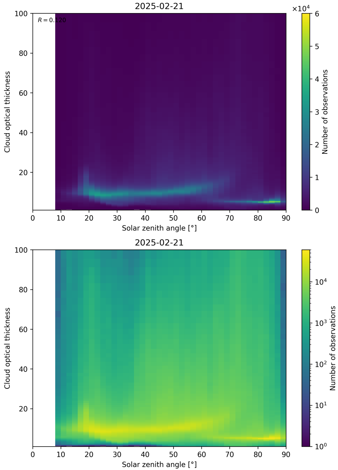
Figure 103: Scatter density plot of “Solar zenith angle” against “Cloud optical thickness” for 2025-02-20 to 2025-02-22.
