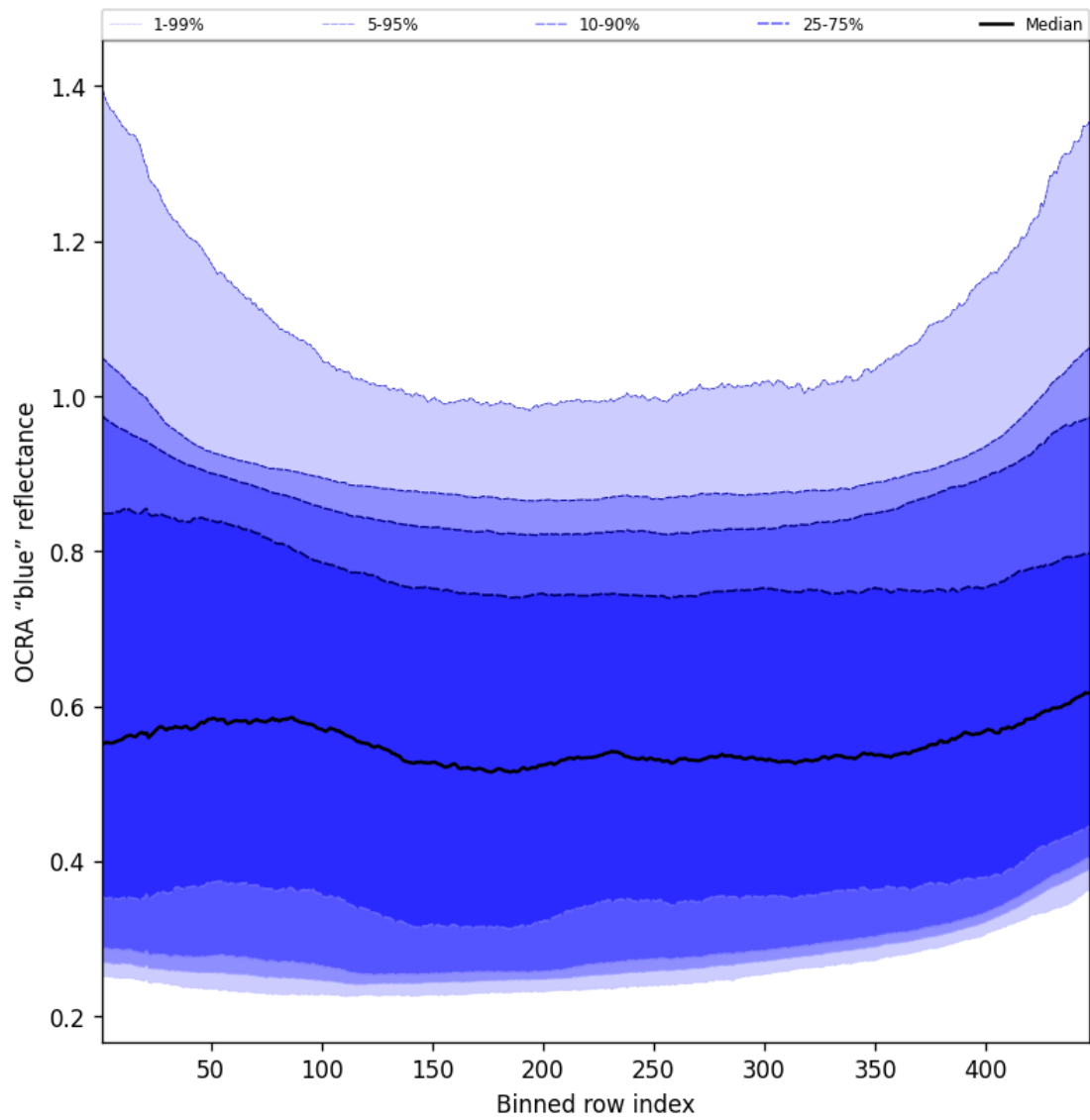
Figure 67: Along track statistics of "OCRA "blue" reflectance" for 2025-02-20 to 2025-02-22
