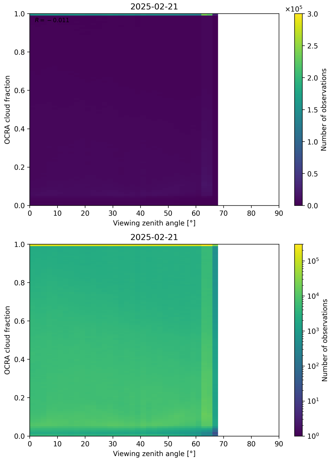
Figure 108: Scatter density plot of “Viewing zenith angle” against “OCRA cloud fraction” for 2025-02-20 to 2025-02-22.
