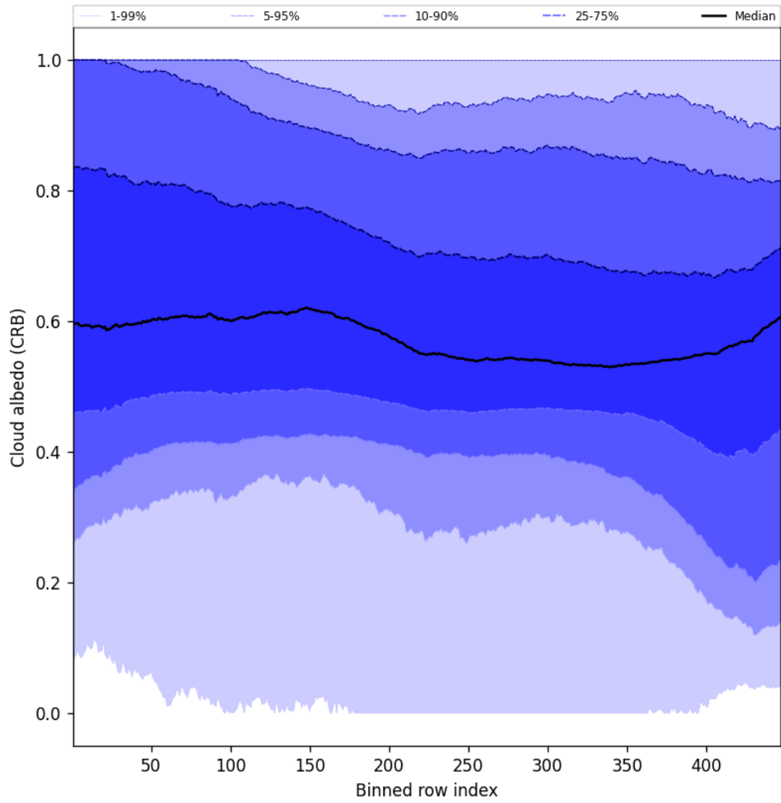
Figure 60: Along track statistics of “Cloud albedo (CRB)” for 2025-02-20 to 2025-02-22
