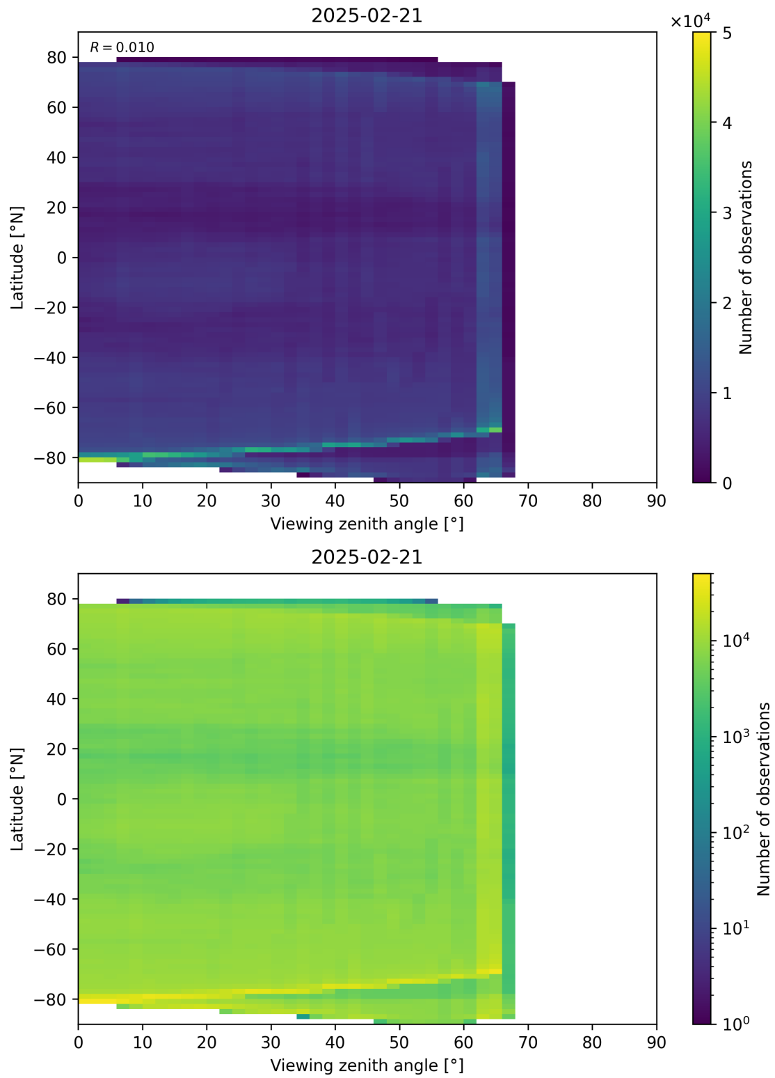
Figure 113: Scatter density plot of “Viewing zenith angle” against “Latitude” for 2025-02-20 to 2025-02-22.
