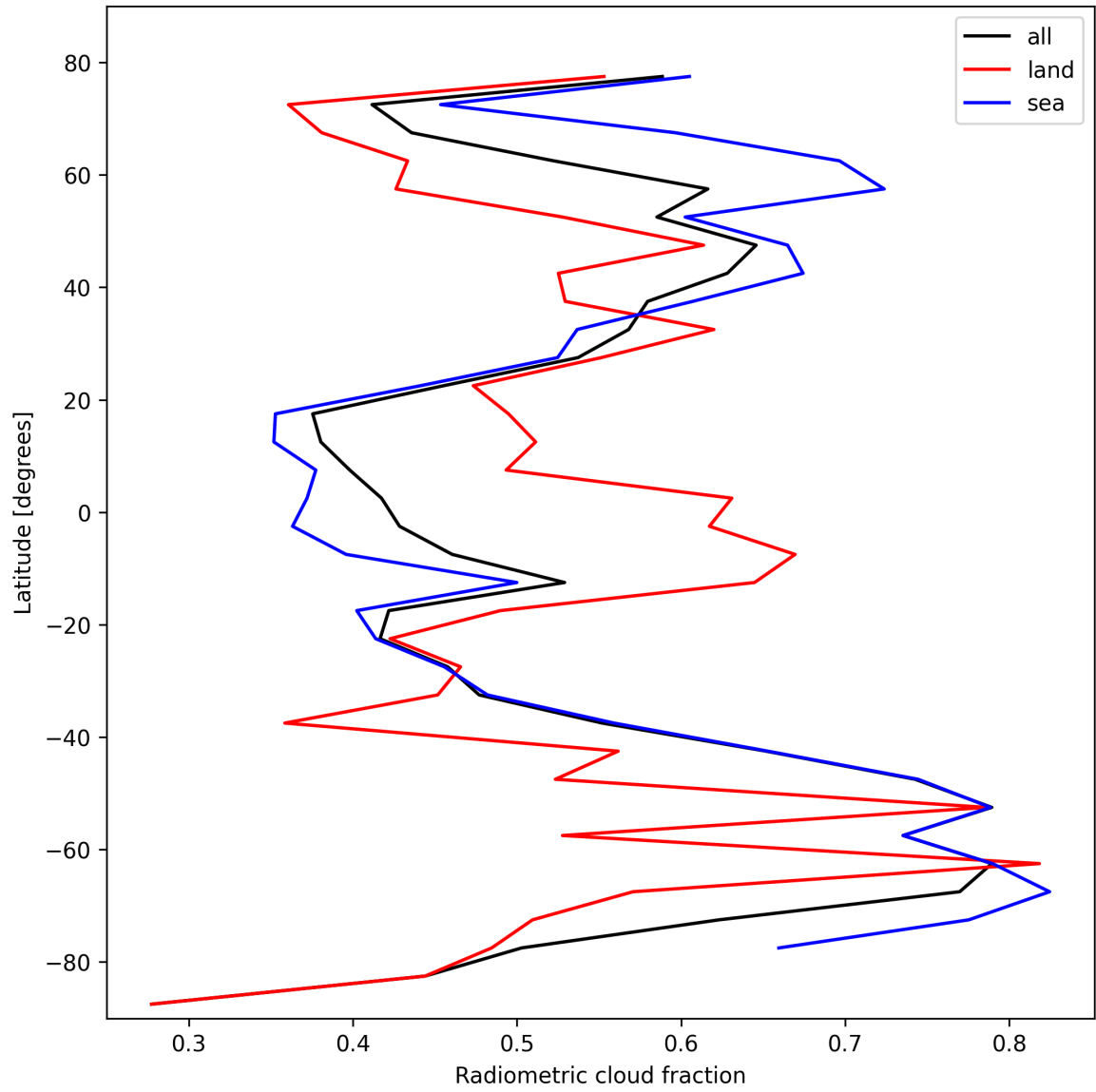
Figure 23: Zonal average of “Radiometric cloud fraction” for 2025-02-20 to 2025-02-22.
