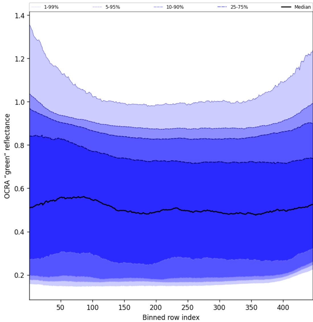
Figure 68: Along track statistics of "OCRA "green" reflectance" for 2025-02-20 to 2025-02-22
