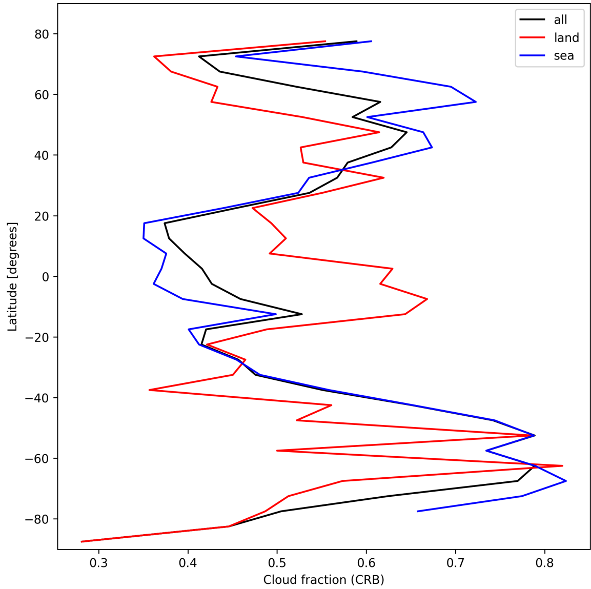
Figure 26: Zonal average of “Cloud fraction (CRB)” for 2025-02-20 to 2025-02-22.
