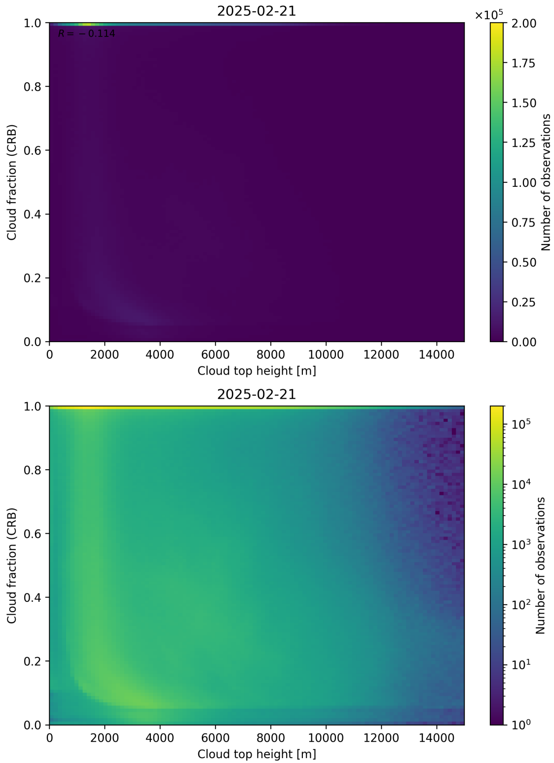
Figure 88: Scatter density plot of “Cloud top height” against “Cloud fraction (CRB)” for 2025-02-20 to 2025-02-22.
