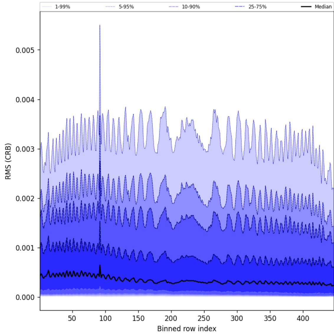
Figure 64: Along track statistics of “RMS (CRB)” for 2025-02-20 to 2025-02-22
