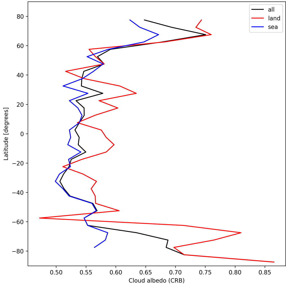
Figure 28: Zonal average of “Cloud albedo (CRB)” for 2025-02-20 to 2025-02-22.
