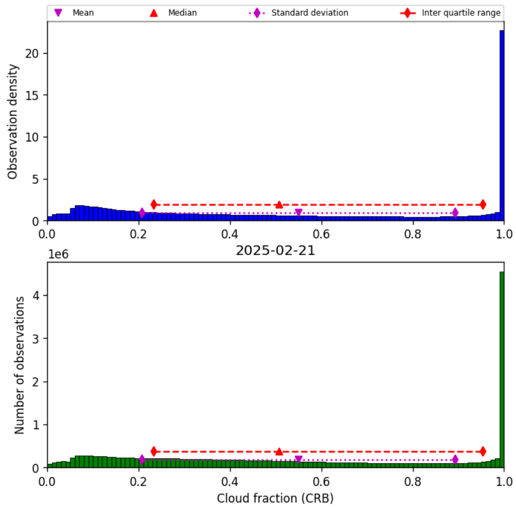
Figure 42: Histogram of “Cloud fraction (CRB)” for 2025-02-20 to 2025-02-22
