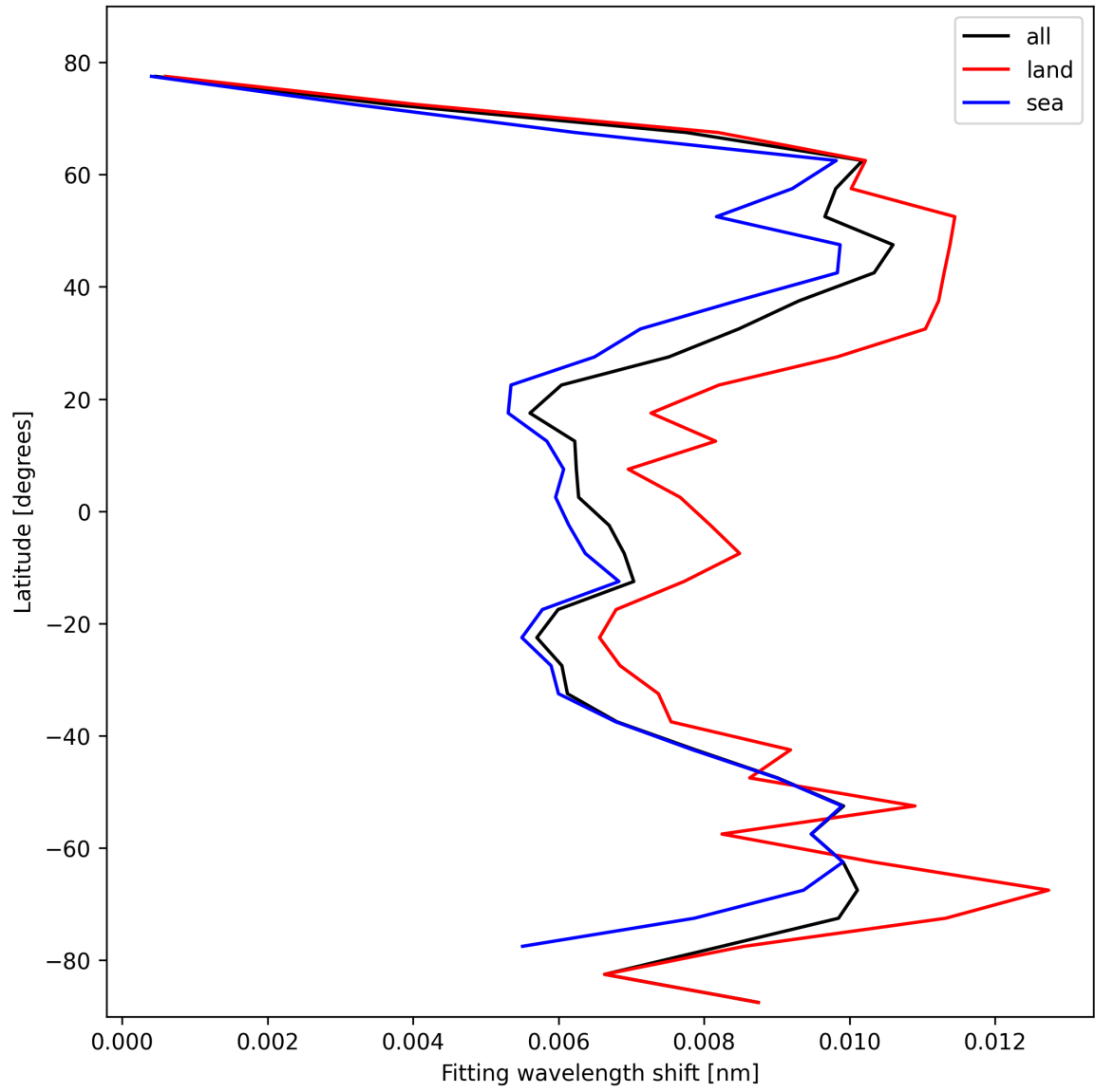
Figure 33: Zonal average of “Fitting wavelength shift” for 2025-02-20 to 2025-02-22.
