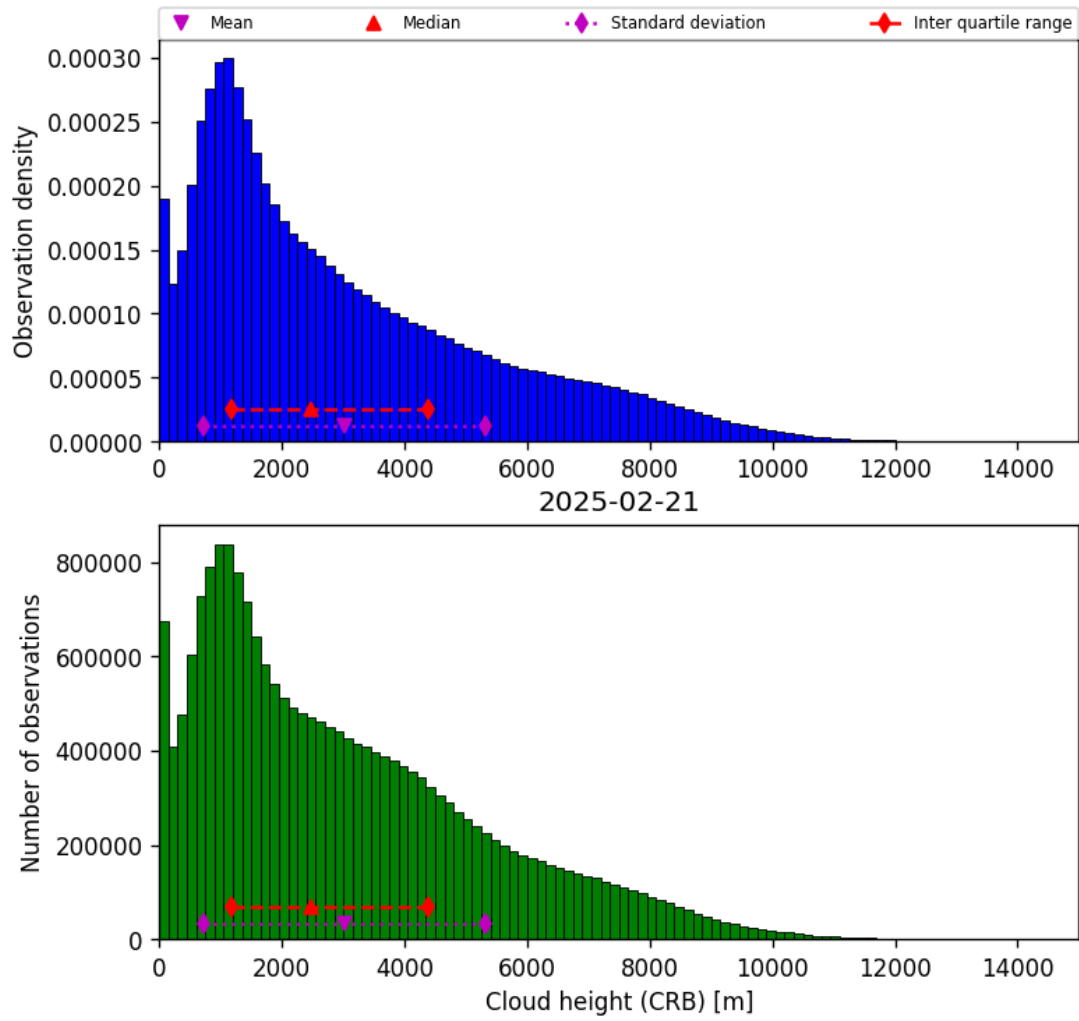
Figure 43: Histogram of “Cloud height (CRB)” for 2025-02-20 to 2025-02-22
