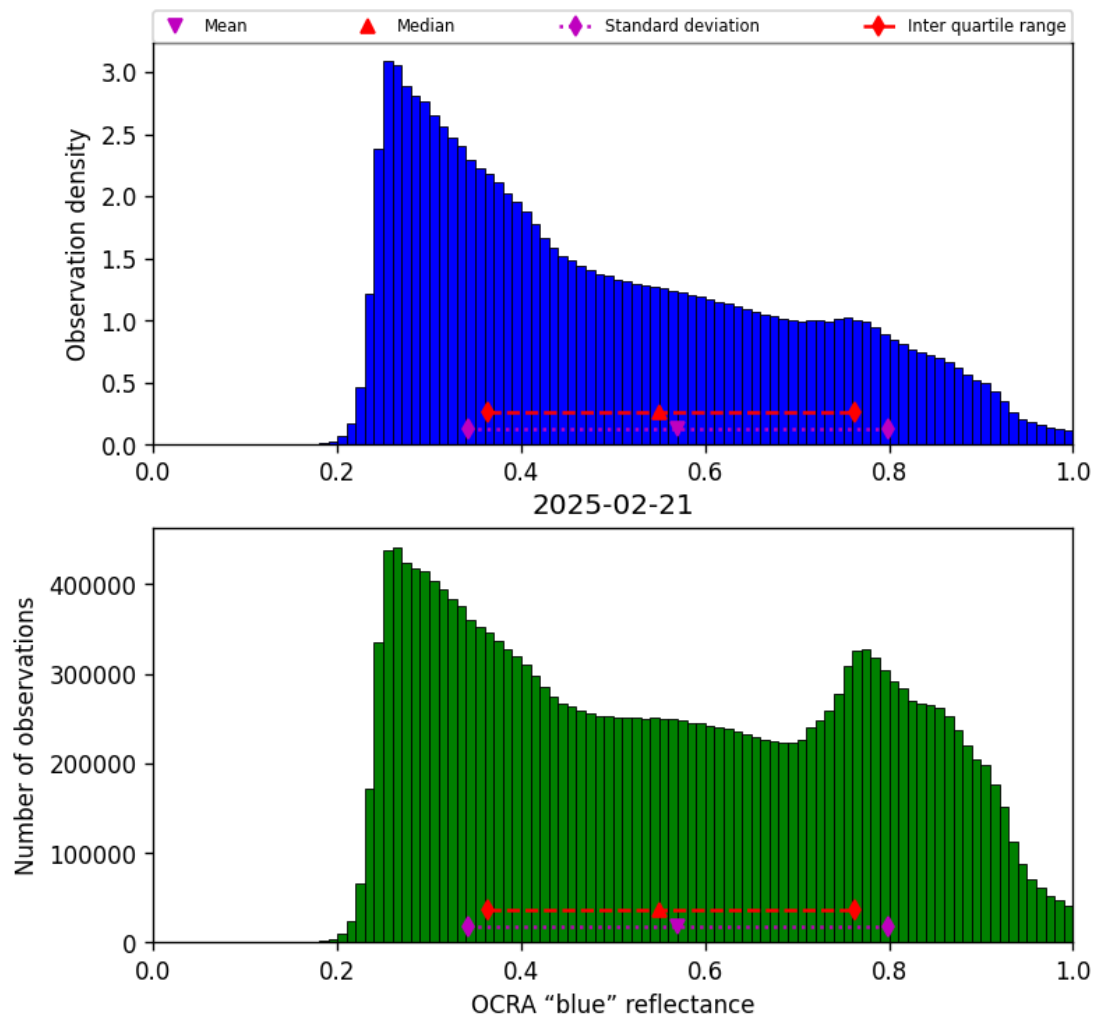
Figure 51: Histogram of “OCRA “blue” reflectance” for 2025-02-20 to 2025-02-22
