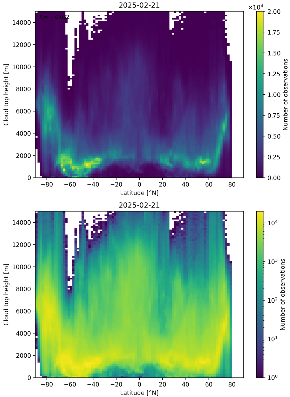
Figure 97: Scatter density plot of “Latitude” against “Cloud top height” for 2025-02-20 to 2025-02-22.
