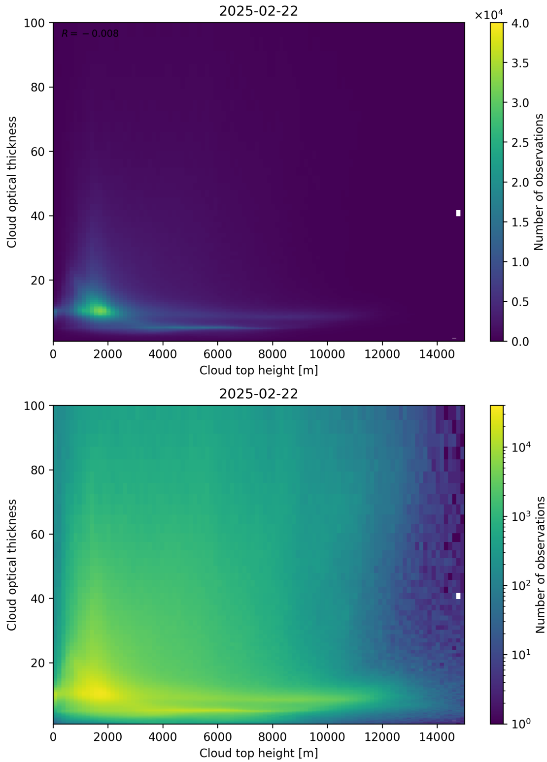
Figure 90: Scatter density plot of “Cloud top height” against “Cloud optical thickness” for 2025-02-21 to 2025-02-23.
