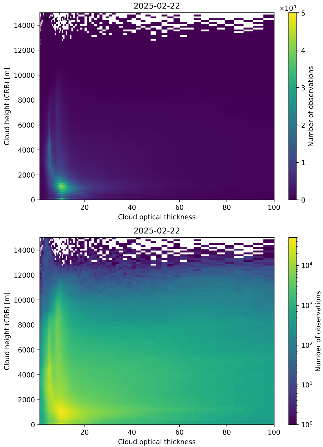
Figure 85: Scatter density plot of “Cloud optical thickness” against “Cloud height (CRB)” for 2025-02-21 to 2025-02-23.
