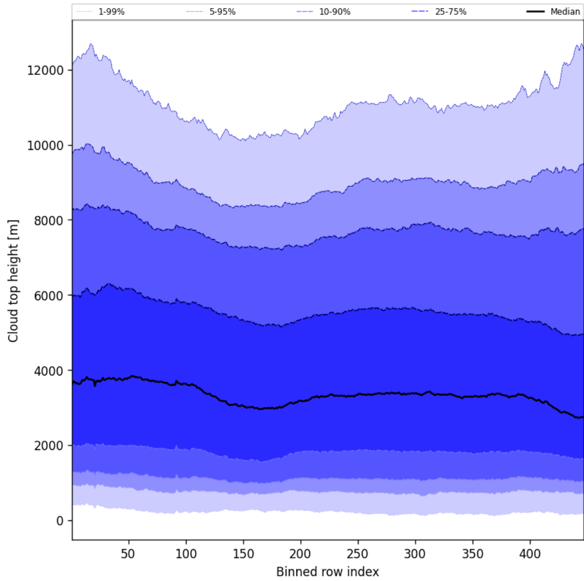
Figure 56: Along track statistics of “Cloud top height” for 2025-02-21 to 2025-02-23
