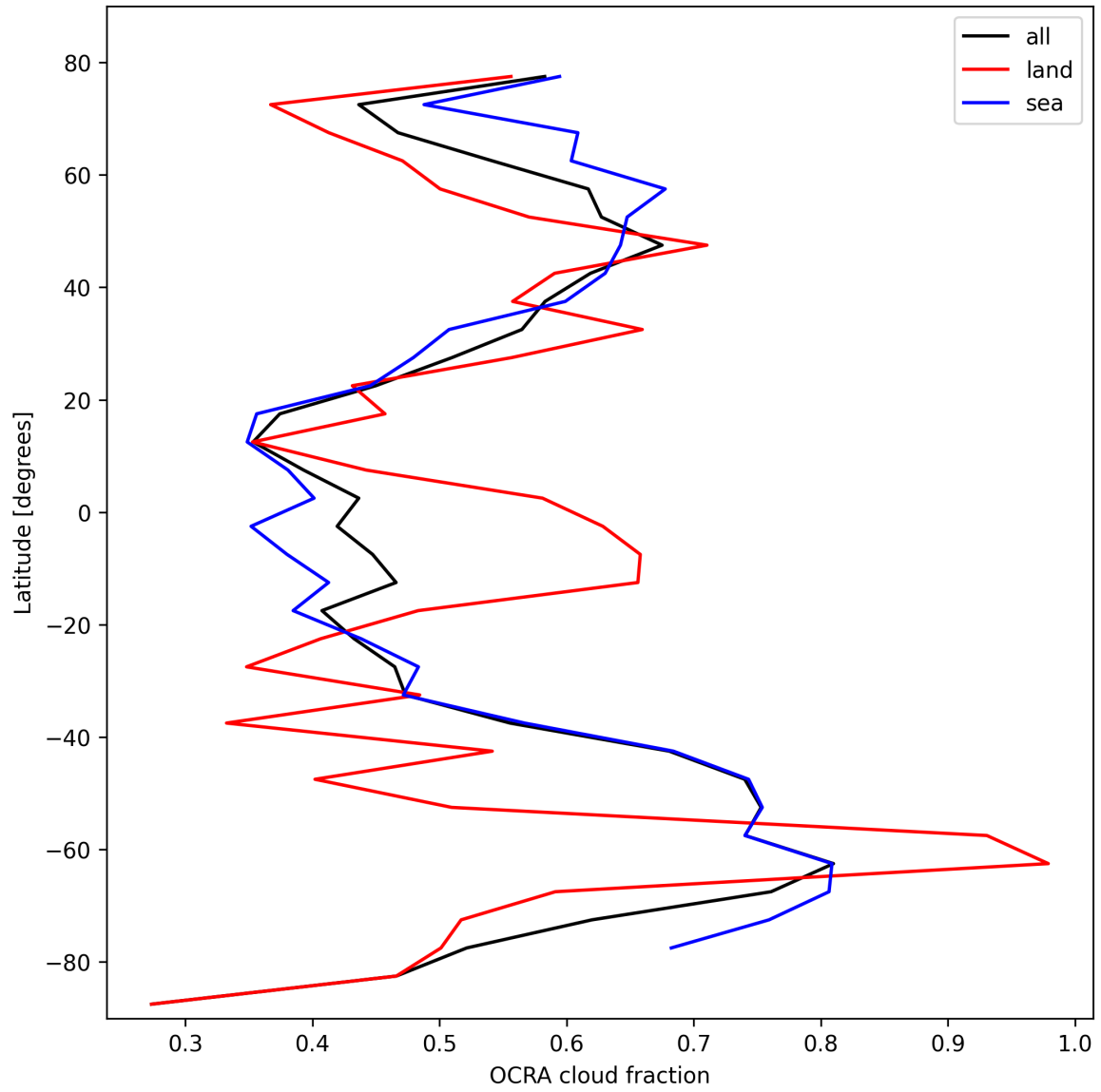
Figure 34: Zonal average of “OCRA cloud fraction” for 2025-02-21 to 2025-02-23.
