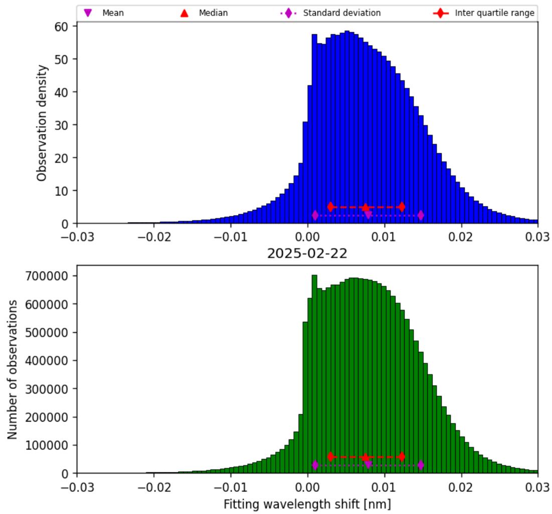
Figure 49: Histogram of “Fitting wavelength shift” for 2025-02-21 to 2025-02-23
