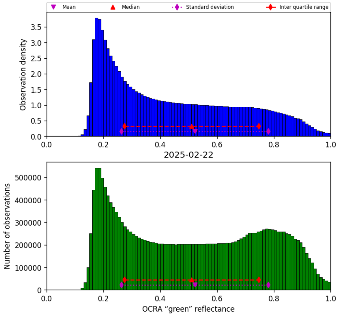
Figure 52: Histogram of “OCRA “green” reflectance” for 2025-02-21 to 2025-02-23
