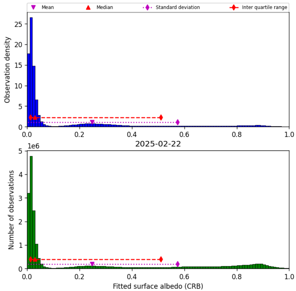
Figure 46: Histogram of “Fitted surface albedo (CRB)” for 2025-02-21 to 2025-02-23
