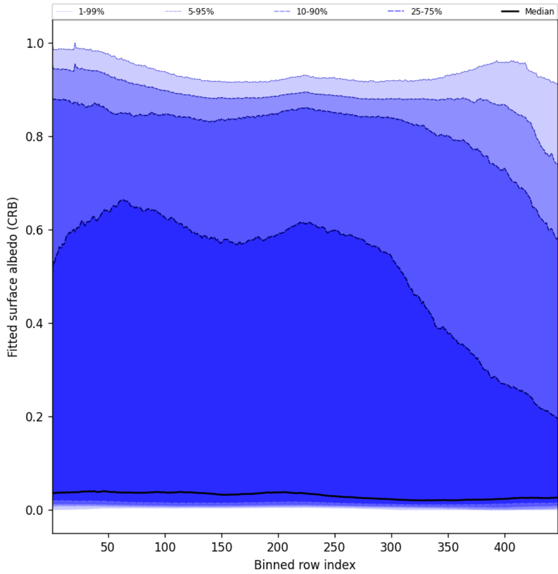
Figure 62: Along track statistics of “Fitted surface albedo (CRB)” for 2025-02-21 to 2025-02-23
