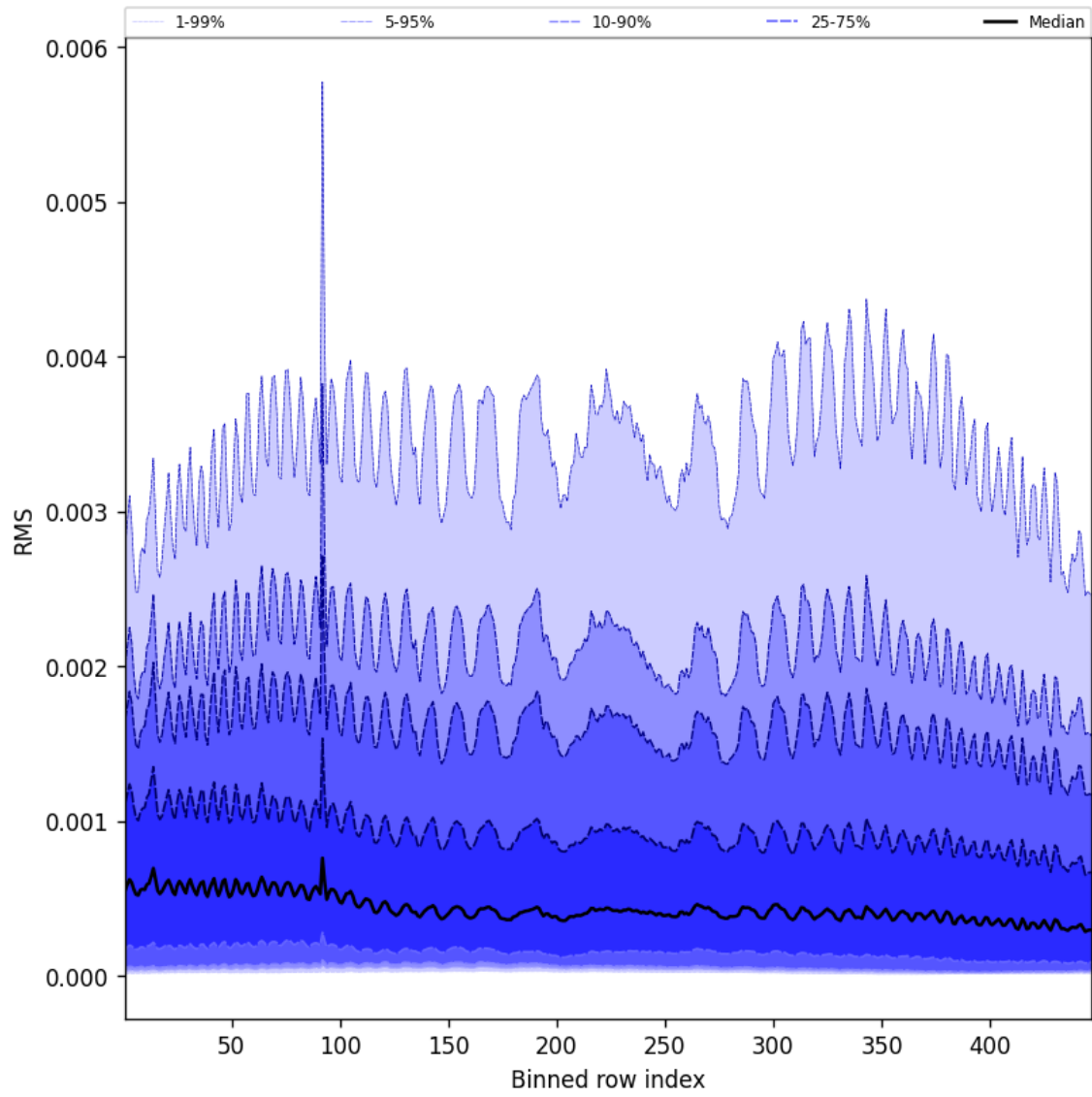
Figure 63: Along track statistics of “RMS” for 2025-02-21 to 2025-02-23
