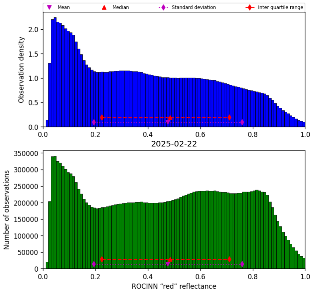
Figure 53: Histogram of “ROCINN “red” reflectance” for 2025-02-21 to 2025-02-23
