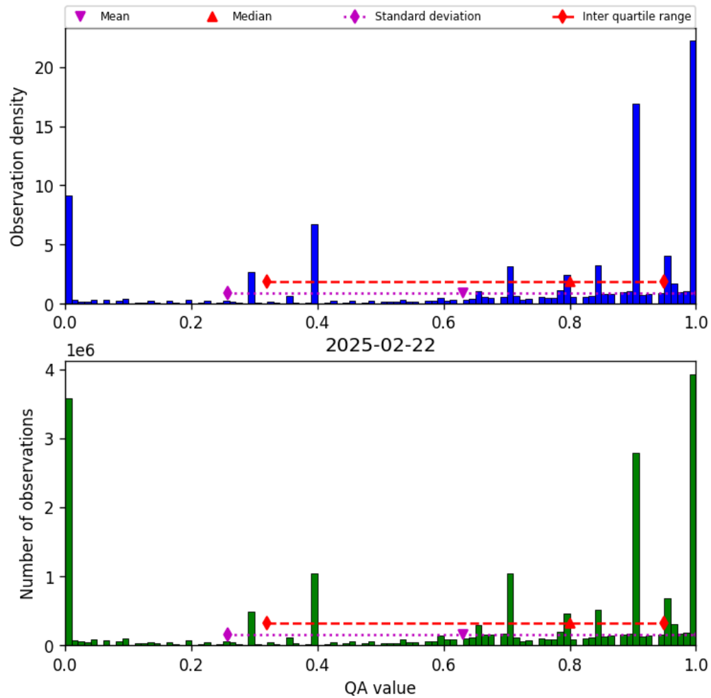
Figure 38: Histogram of “QA value” for 2025-02-21 to 2025-02-23
