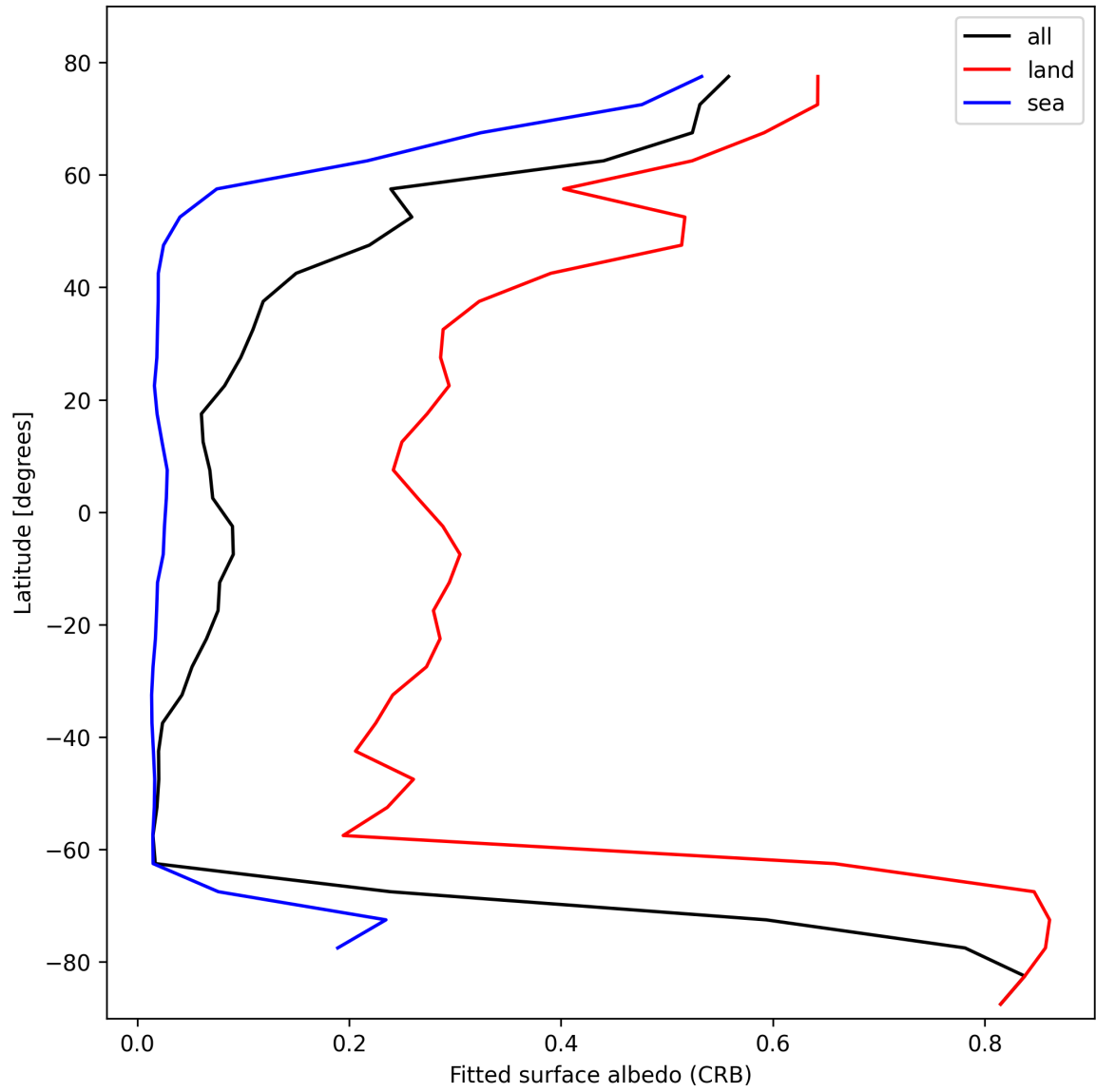
Figure 30: Zonal average of “Fitted surface albedo (CRB)” for 2025-02-21 to 2025-02-23.
