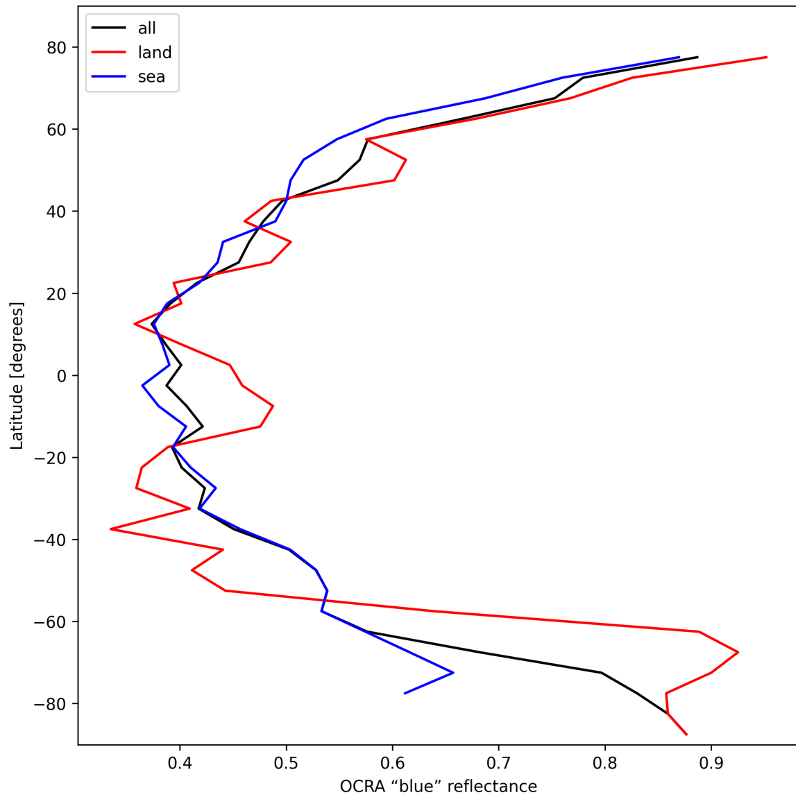
Figure 35: Zonal average of “OCRA “blue” reflectance” for 2025-02-21 to 2025-02-23.
