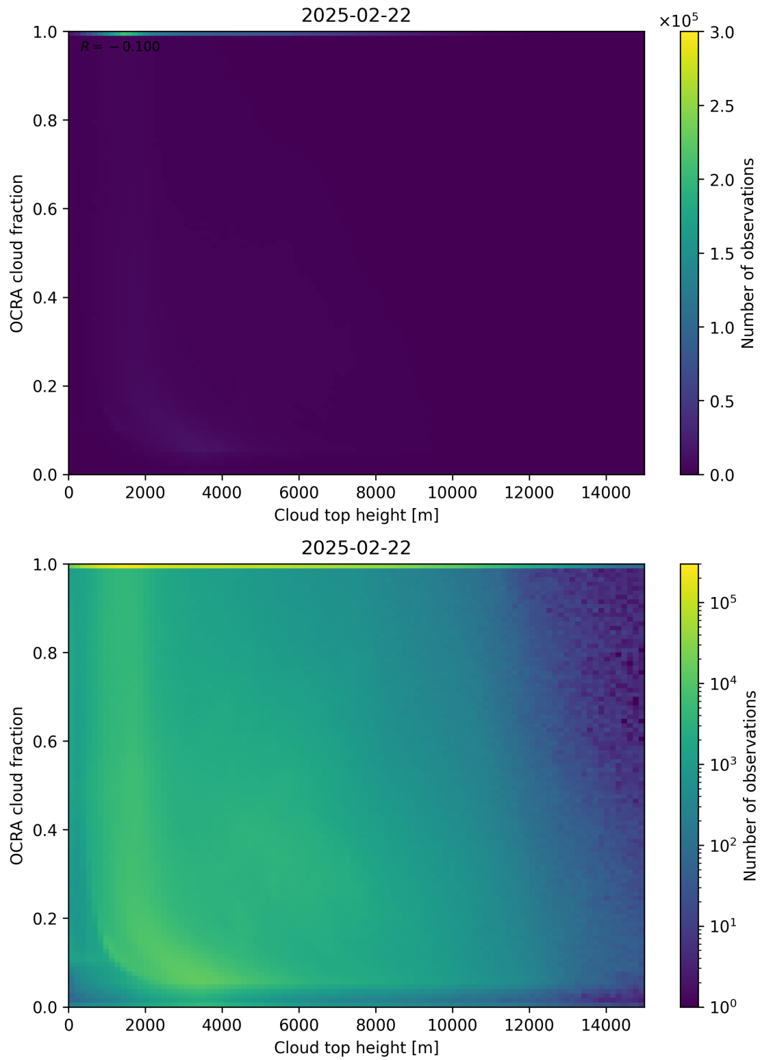
Figure 87: Scatter density plot of “Cloud top height” against “OCRA cloud fraction” for 2025-02-21 to 2025-02-23.
