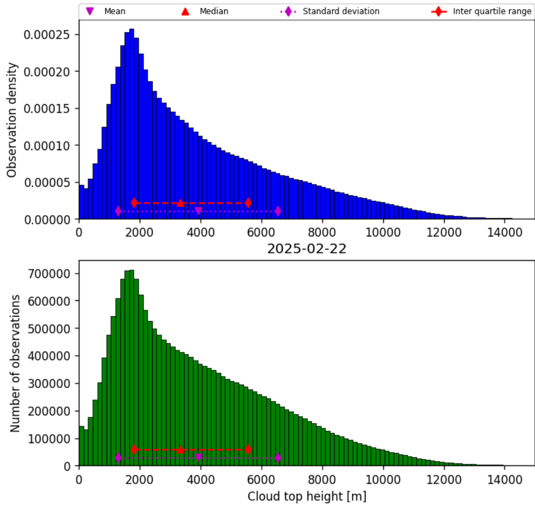
Figure 40: Histogram of “Cloud top height” for 2025-02-21 to 2025-02-23
