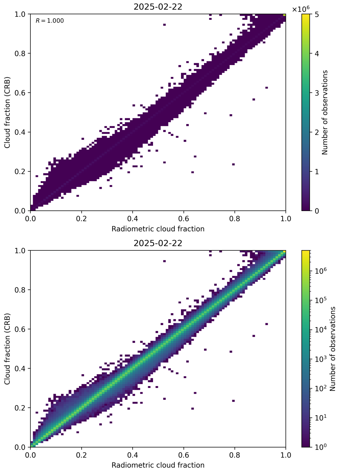
Figure 73: Scatter density plot of “Radiometric cloud fraction” against “Cloud fraction (CRB)” for 2025-02-21 to 2025-02-23.
