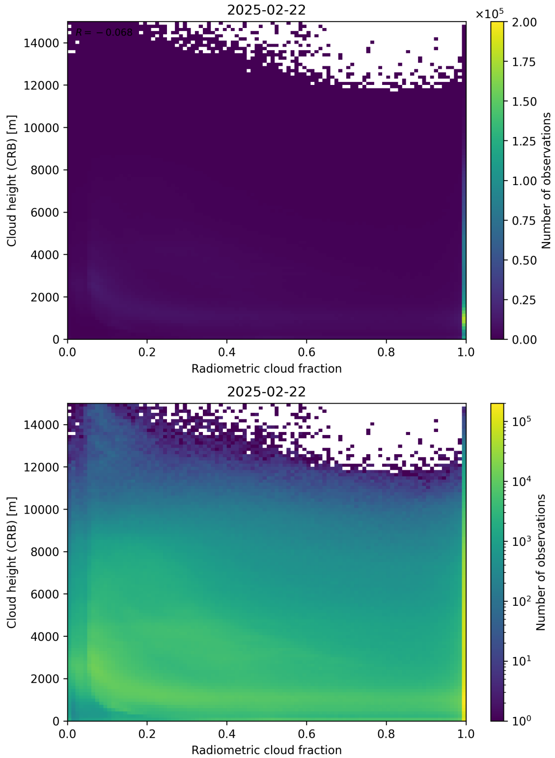
Figure 74: Scatter density plot of “Radiometric cloud fraction” against “Cloud height (CRB)” for 2025-02-21 to 2025-02-23.
