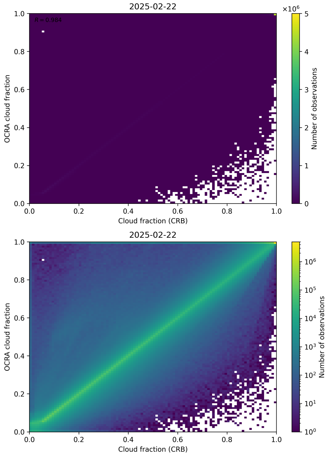
Figure 78: Scatter density plot of “Cloud fraction (CRB)” against “OCRA cloud fraction” for 2025-02-21 to 2025-02-23.
