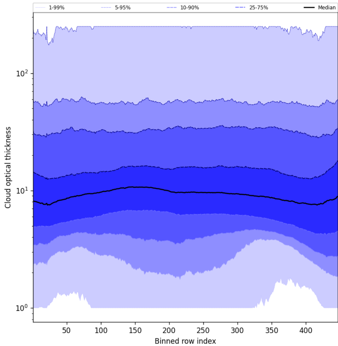
Figure 57: Along track statistics of “Cloud optical thickness” for 2025-02-21 to 2025-02-23
