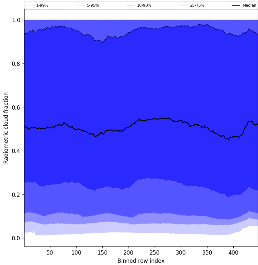
Figure 55: Along track statistics of “Radiometric cloud fraction” for 2025-02-21 to 2025-02-23
