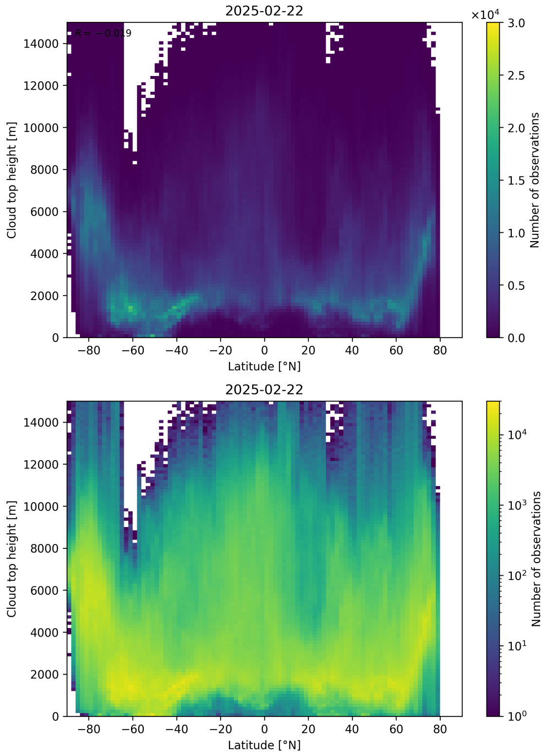
Figure 97: Scatter density plot of “Latitude” against “Cloud top height” for 2025-02-21 to 2025-02-23.
