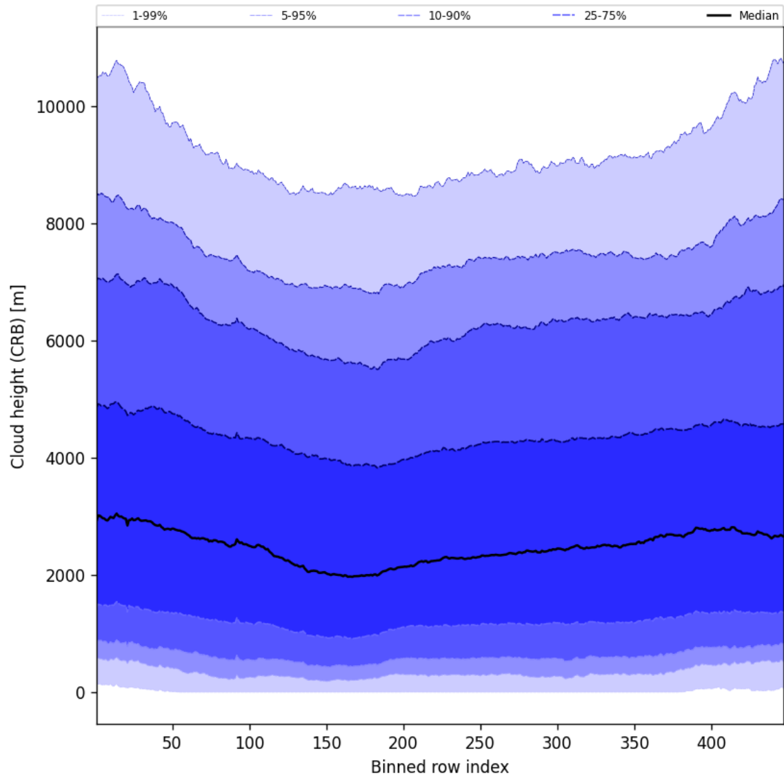
Figure 59: Along track statistics of “Cloud height (CRB)” for 2025-02-21 to 2025-02-23
