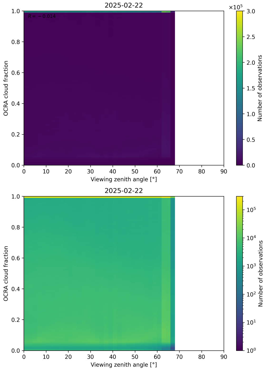
Figure 108: Scatter density plot of “Viewing zenith angle” against “OCRA cloud fraction” for 2025-02-21 to 2025-02-23.
