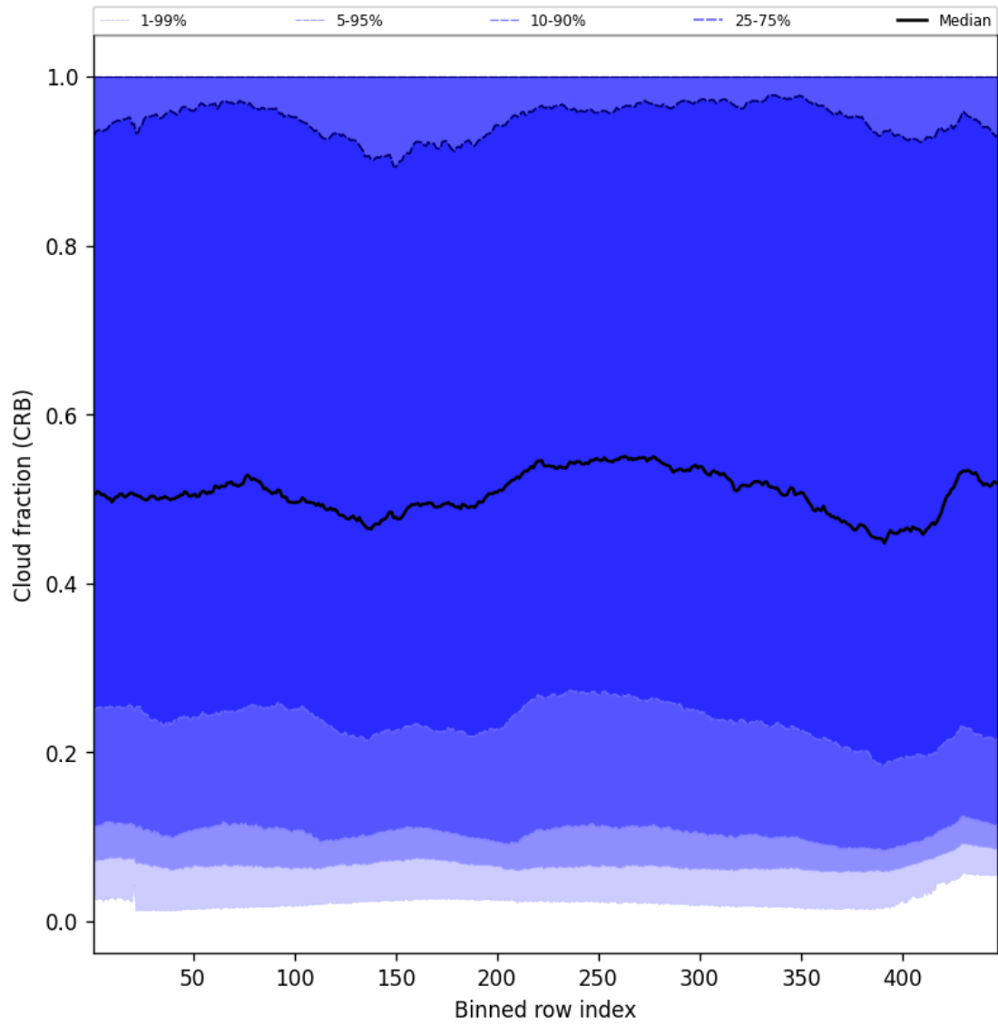
Figure 58: Along track statistics of “Cloud fraction (CRB)” for 2025-02-21 to 2025-02-23
