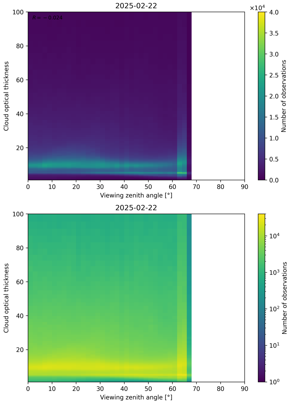
Figure 111: Scatter density plot of “Viewing zenith angle” against “Cloud optical thickness” for 2025-02-21 to 2025-02-23.
