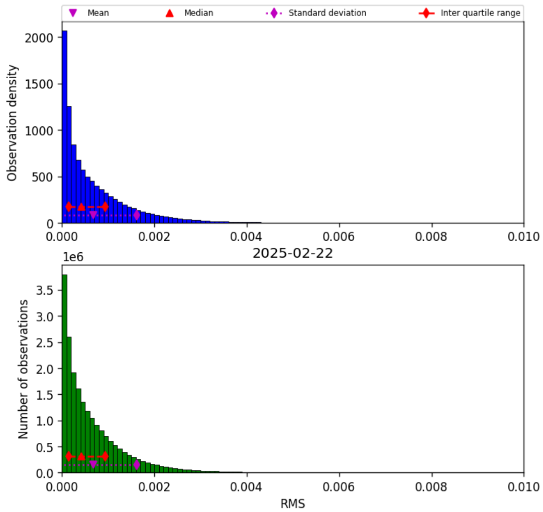
Figure 47: Histogram of “RMS” for 2025-02-21 to 2025-02-23
