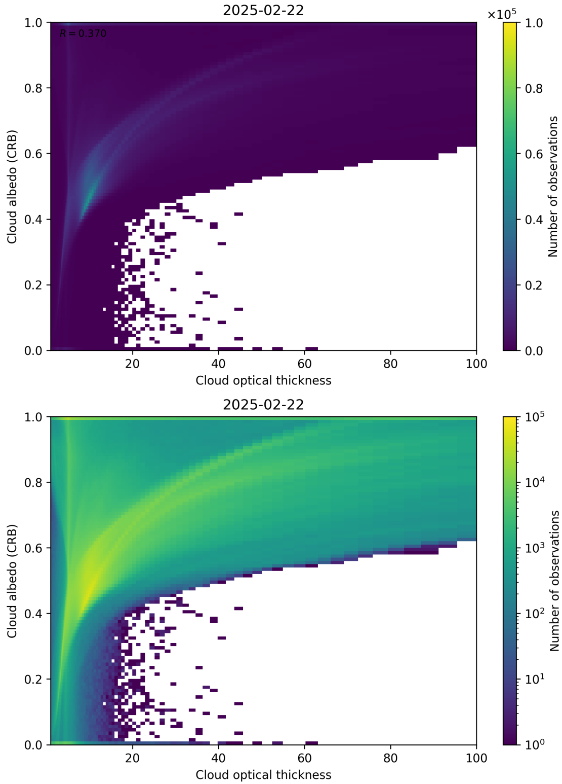
Figure 82: Scatter density plot of “Cloud optical thickness” against “Cloud albedo (CRB)” for 2025-02-21 to 2025-02-23.
