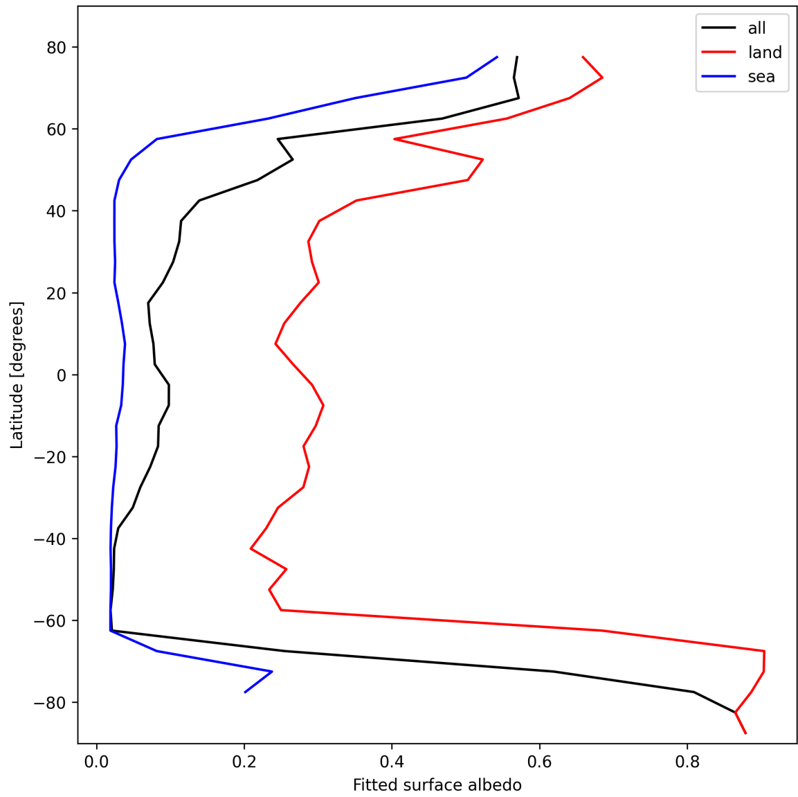
Figure 29: Zonal average of “Fitted surface albedo” for 2025-02-21 to 2025-02-23.
