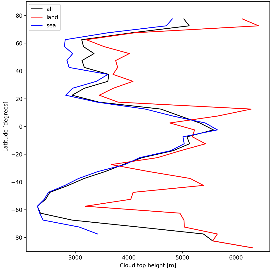
Figure 24: Zonal average of “Cloud top height” for 2025-02-21 to 2025-02-23.
