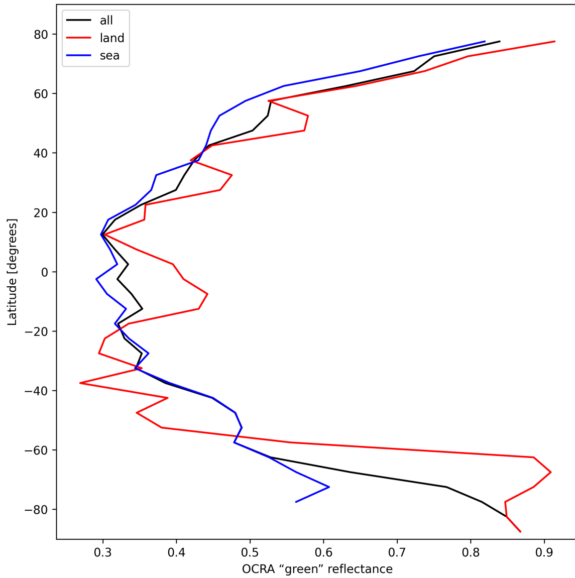
Figure 36: Zonal average of “OCRA “green” reflectance” for 2025-02-21 to 2025-02-23.
