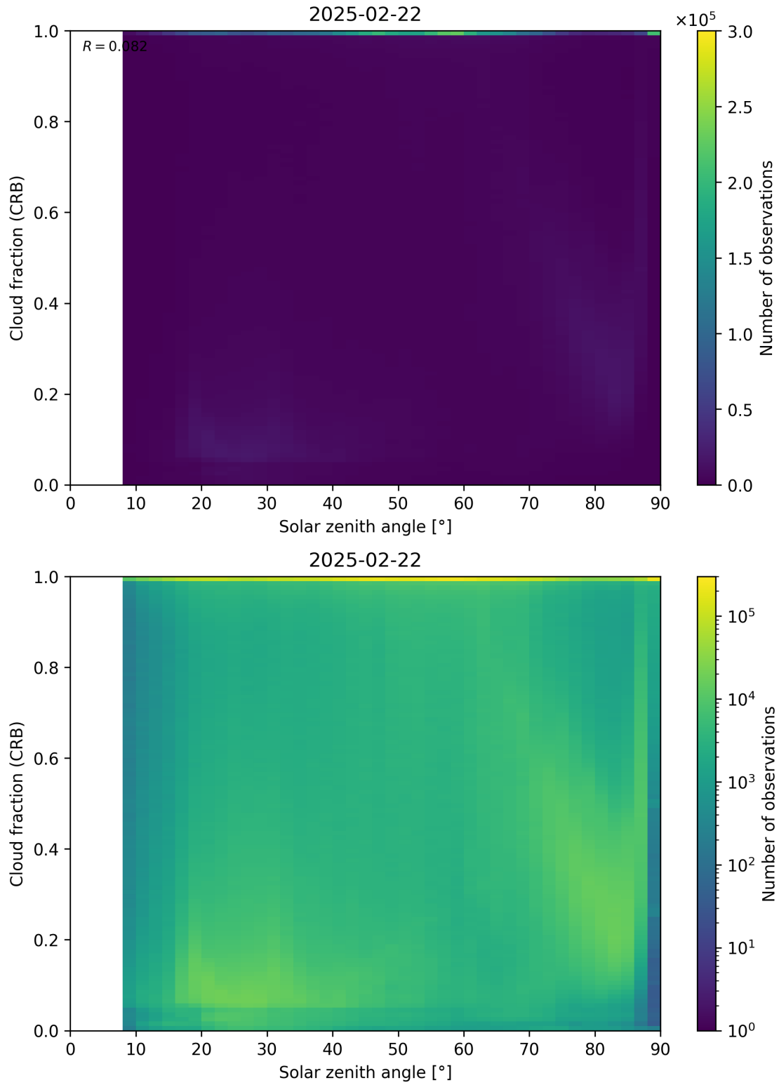
Figure 101: Scatter density plot of “Solar zenith angle” against “Cloud fraction (CRB)” for 2025-02-21 to 2025-02-23.
