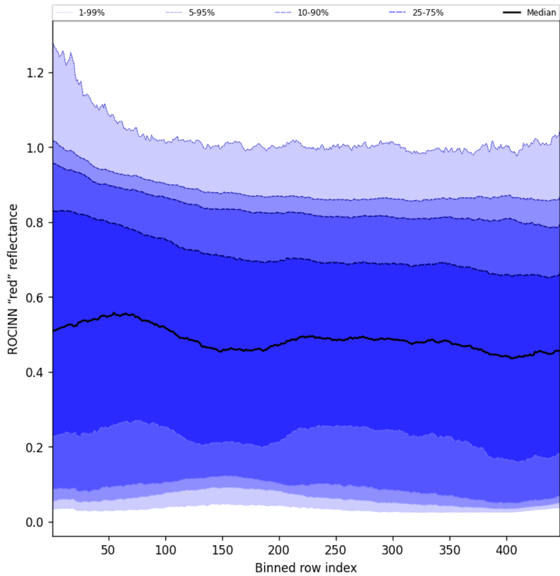
Figure 69: Along track statistics of "ROCINN "red" reflectance" for 2025-02-21 to 2025-02-23
