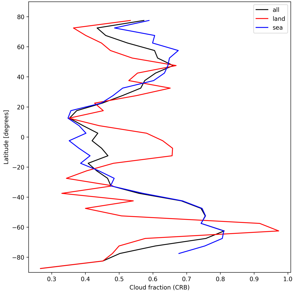
Figure 26: Zonal average of “Cloud fraction (CRB)” for 2025-02-21 to 2025-02-23.
