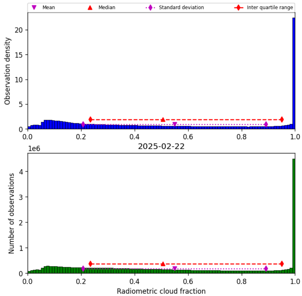
Figure 39: Histogram of “Radiometric cloud fraction” for 2025-02-21 to 2025-02-23
