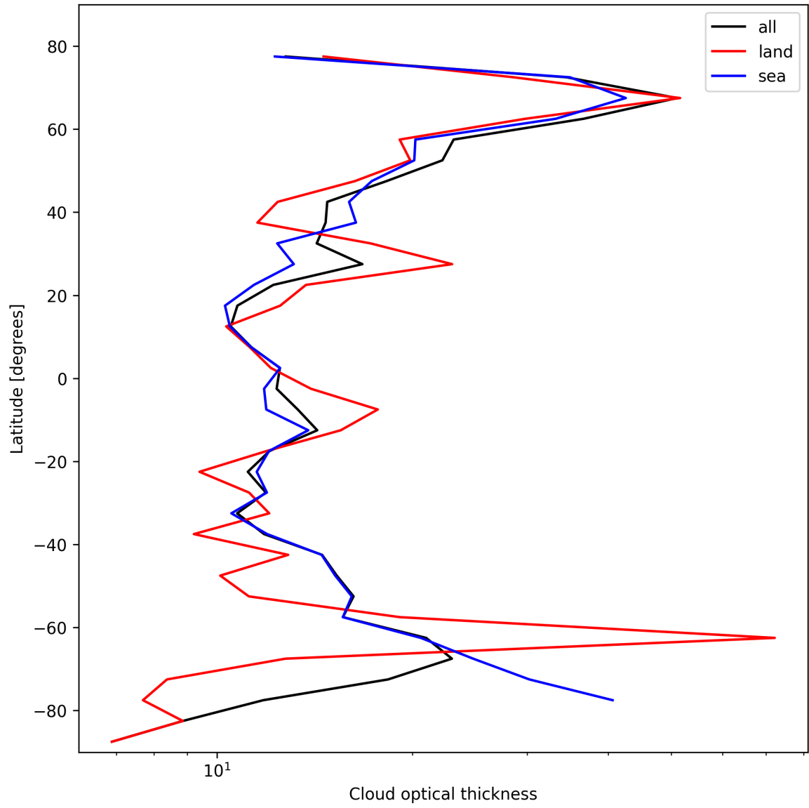
Figure 25: Zonal average of “Cloud optical thickness” for 2025-02-21 to 2025-02-23.
