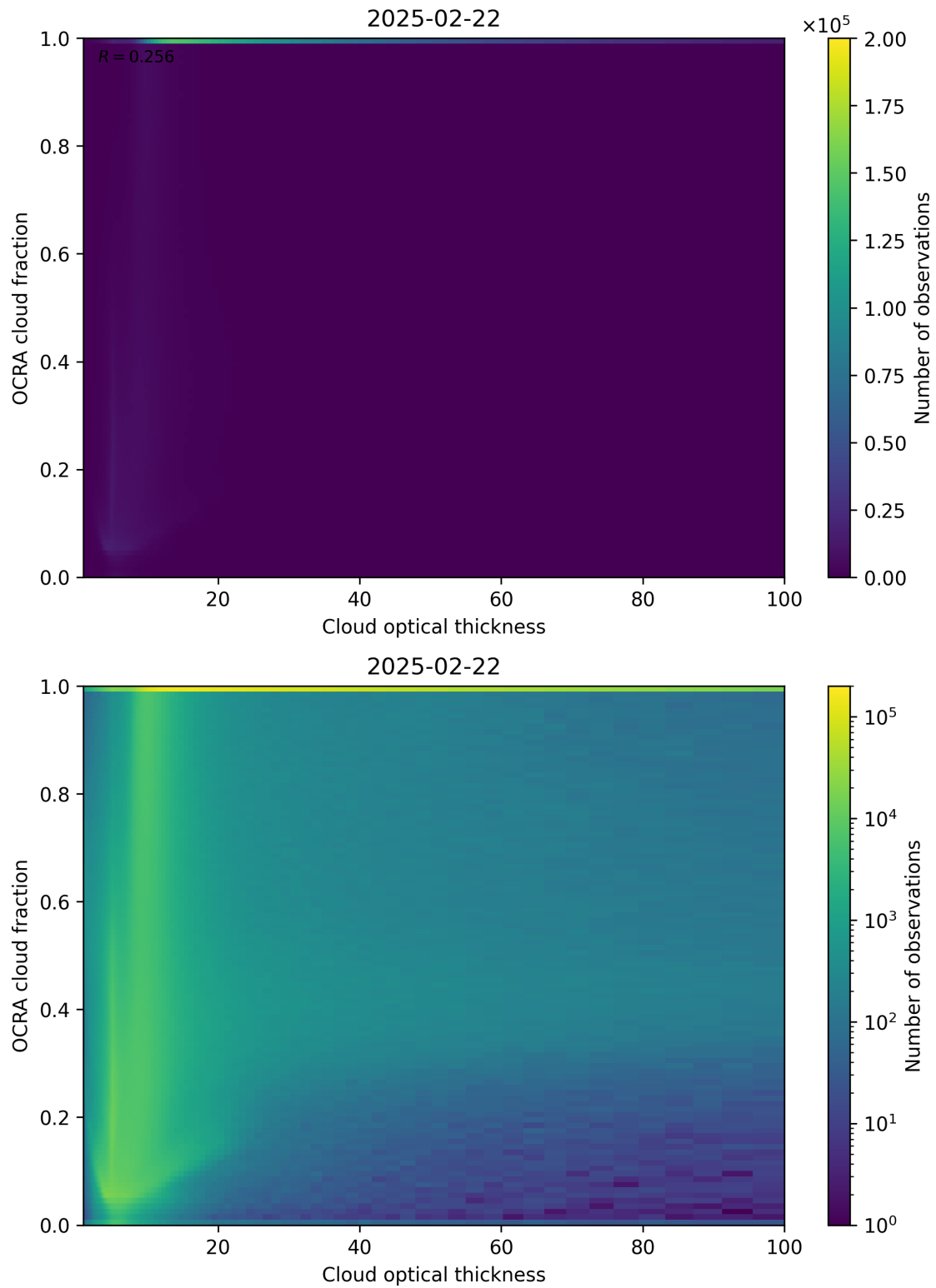
Figure 83: Scatter density plot of “Cloud optical thickness” against “OCRA cloud fraction” for 2025-02-21 to 2025-02-23.
