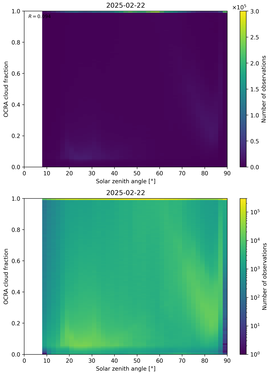
Figure 100: Scatter density plot of “Solar zenith angle” against “OCRA cloud fraction” for 2025-02-21 to 2025-02-23.
