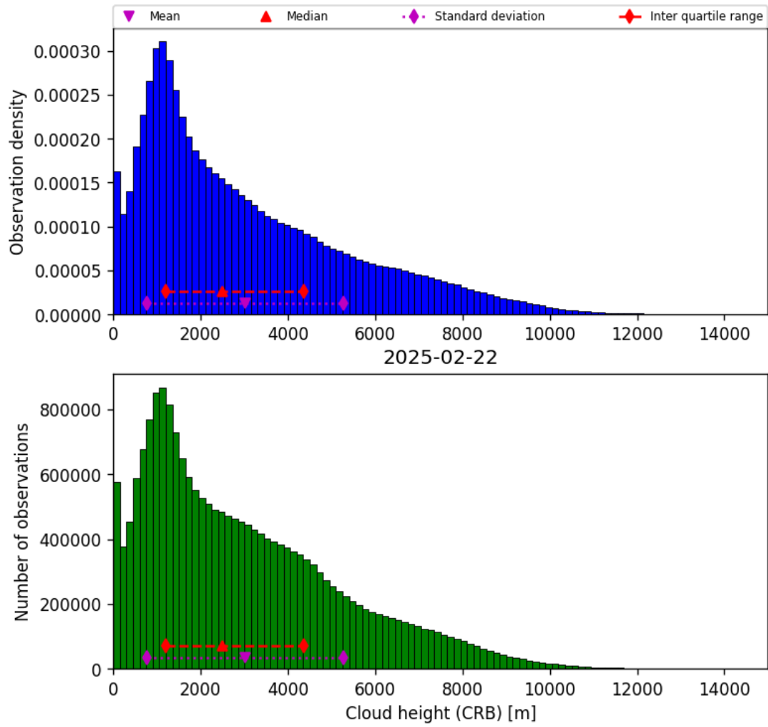
Figure 43: Histogram of “Cloud height (CRB)” for 2025-02-21 to 2025-02-23
