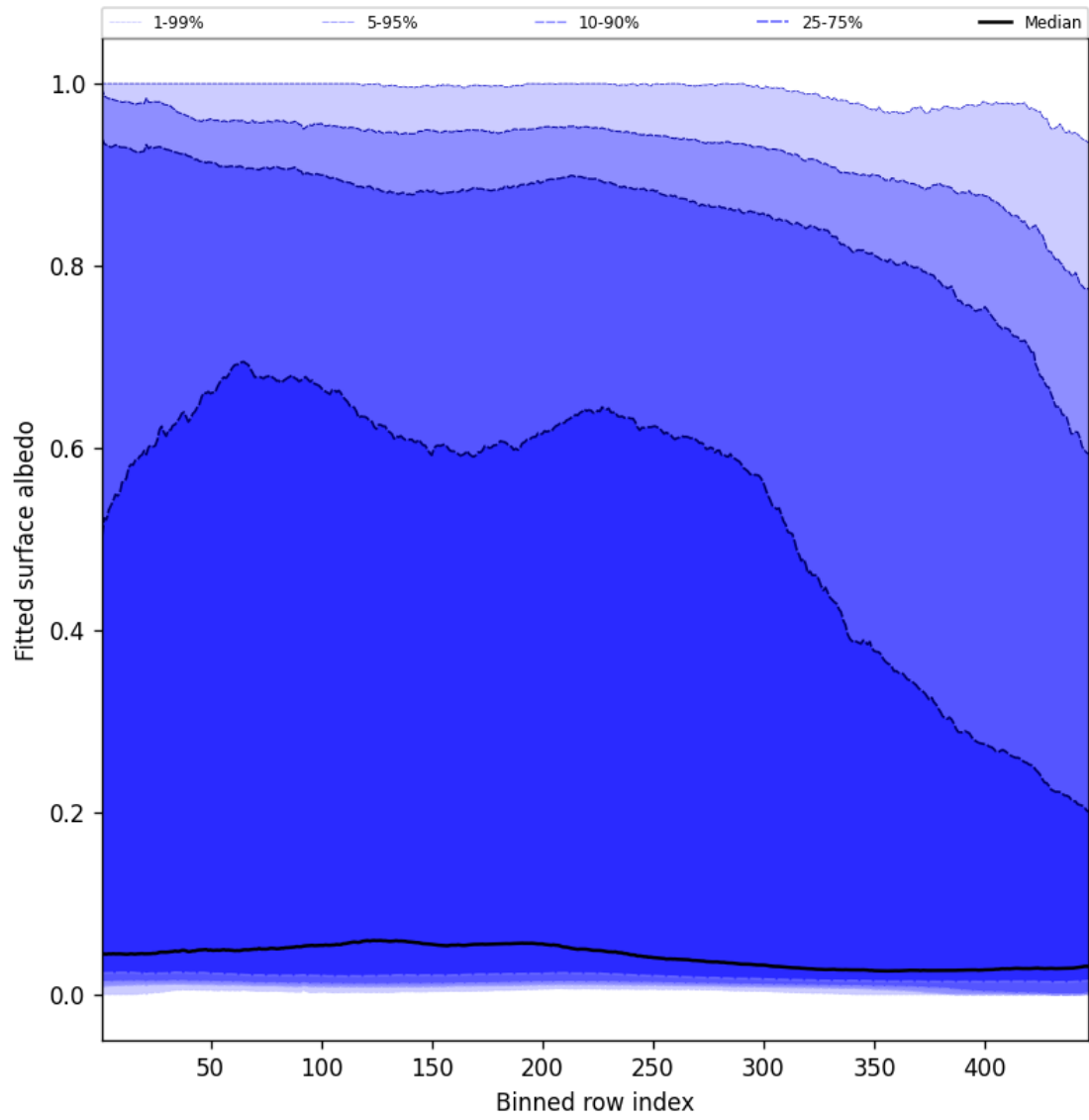
Figure 61: Along track statistics of “Fitted surface albedo” for 2025-02-21 to 2025-02-23
