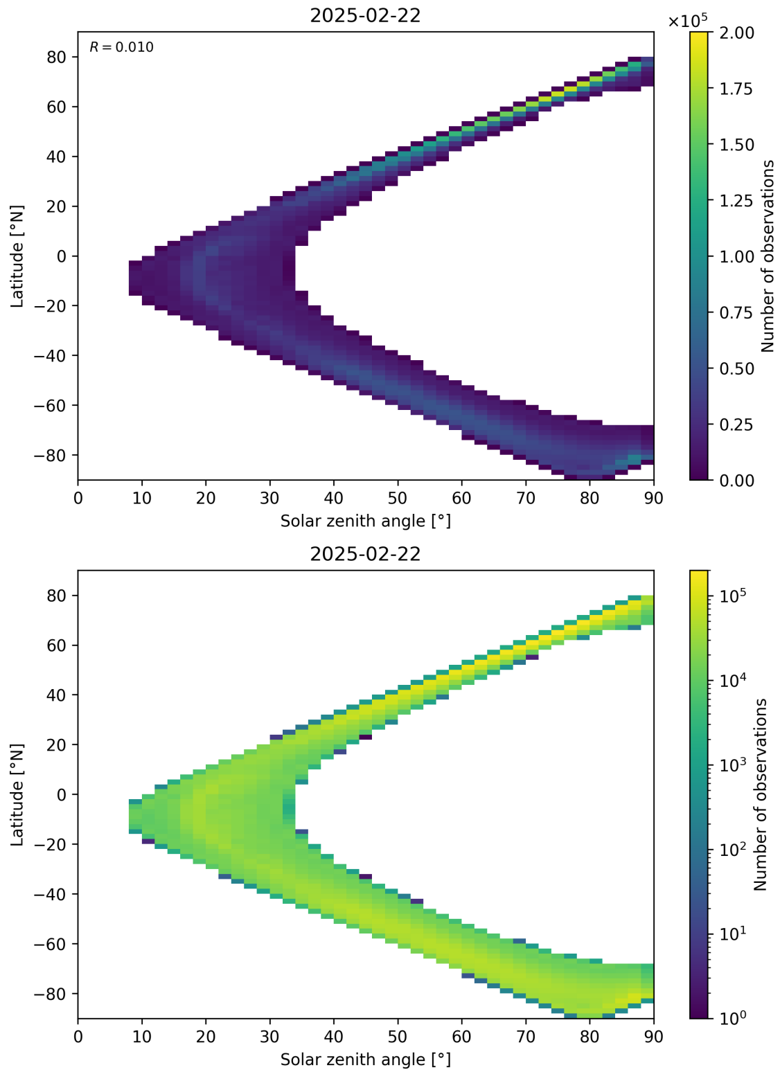
Figure 105: Scatter density plot of “Solar zenith angle” against “Latitude” for 2025-02-21 to 2025-02-23.
