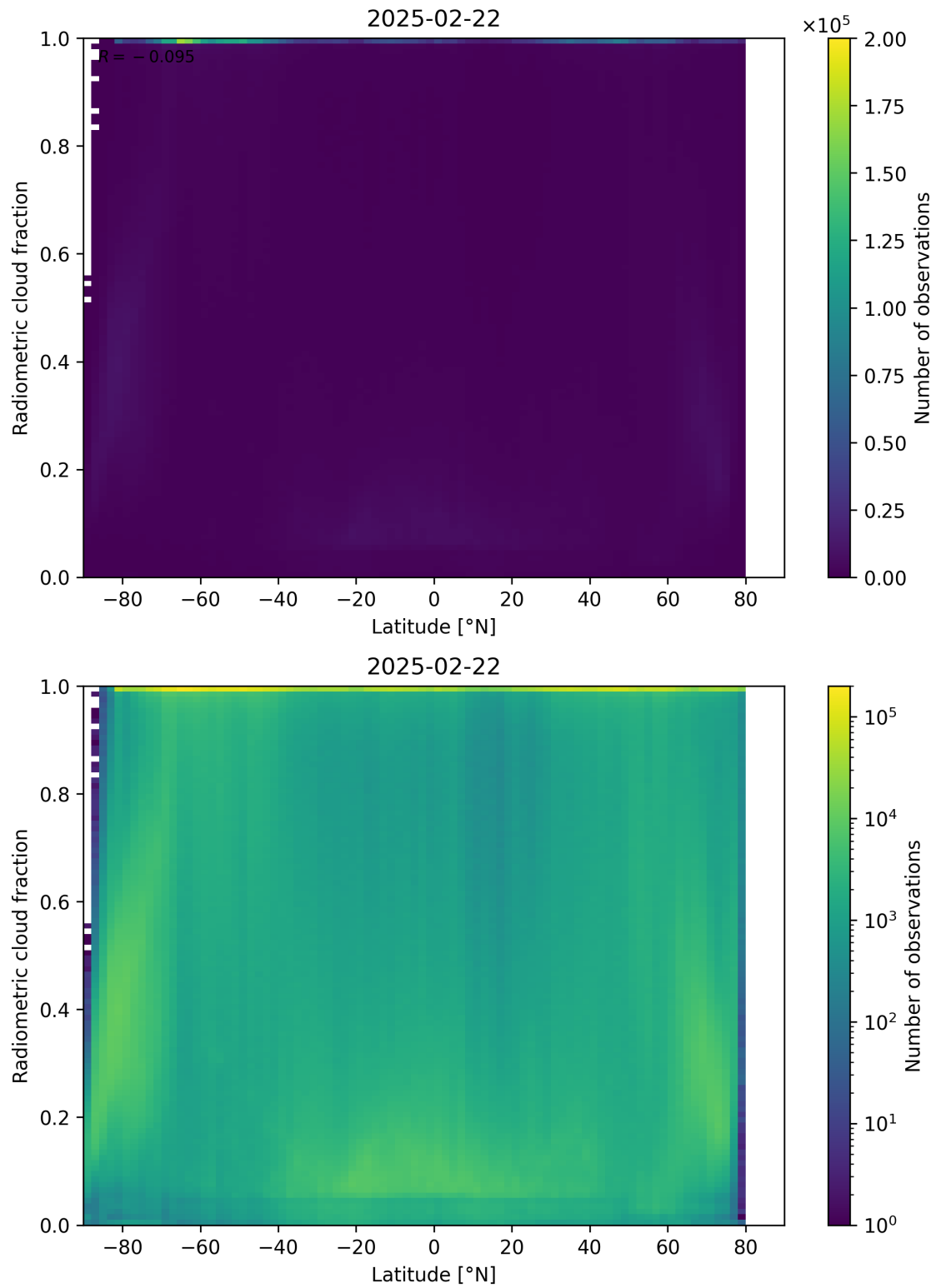
Figure 92: Scatter density plot of “Latitude” against “Radiometric cloud fraction” for 2025-02-21 to 2025-02-23.
