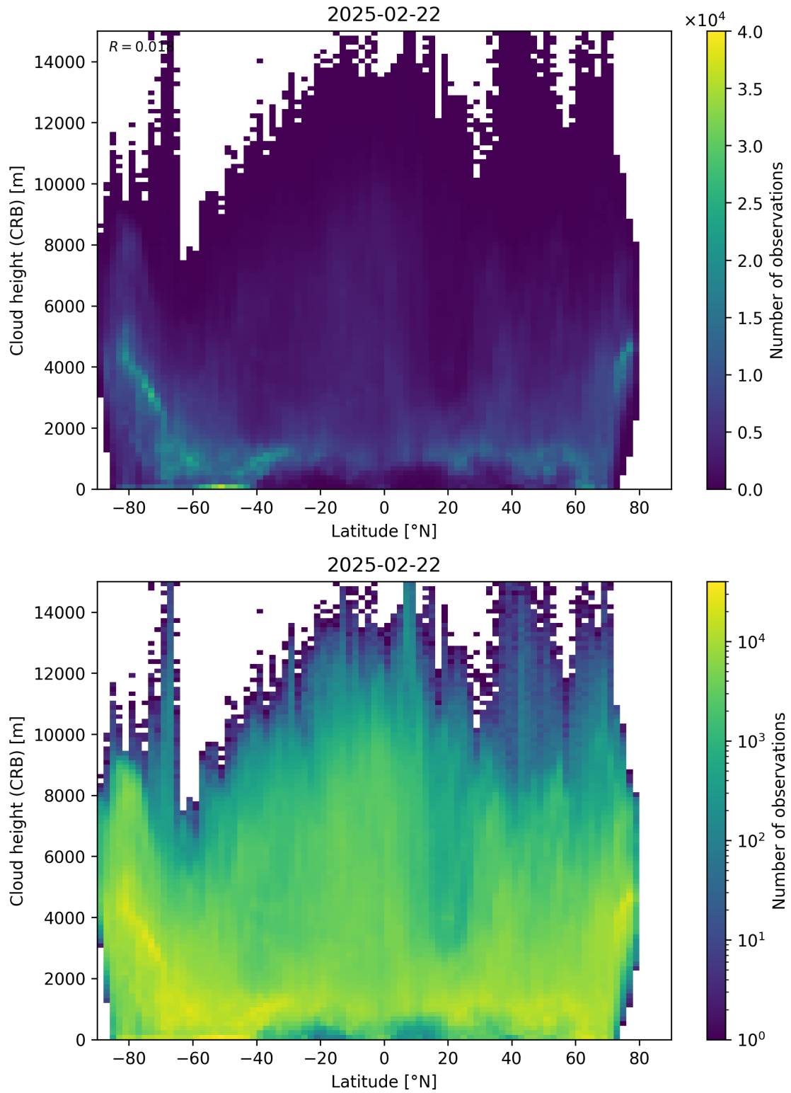
Figure 95: Scatter density plot of “Latitude” against “Cloud height (CRB)” for 2025-02-21 to 2025-02-23.
