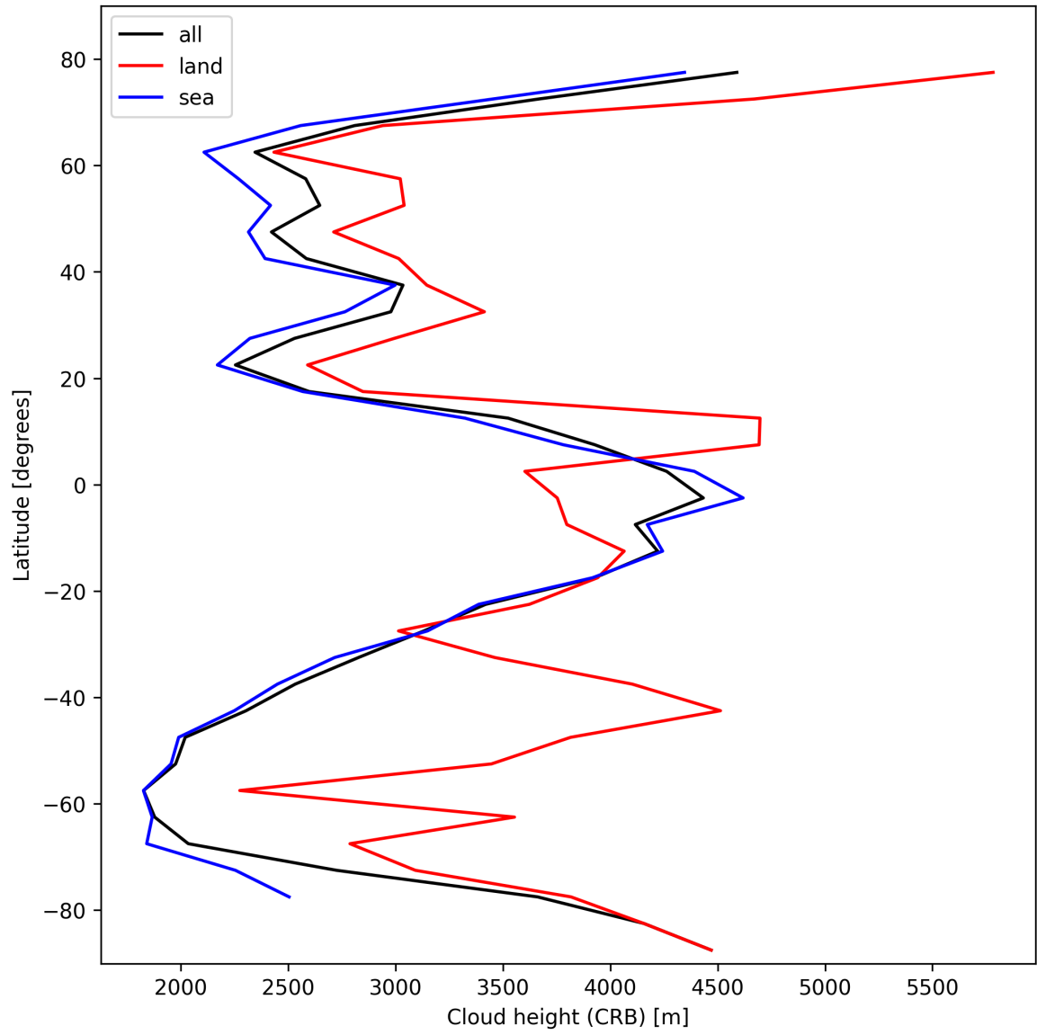
Figure 27: Zonal average of “Cloud height (CRB)” for 2025-02-21 to 2025-02-23.
