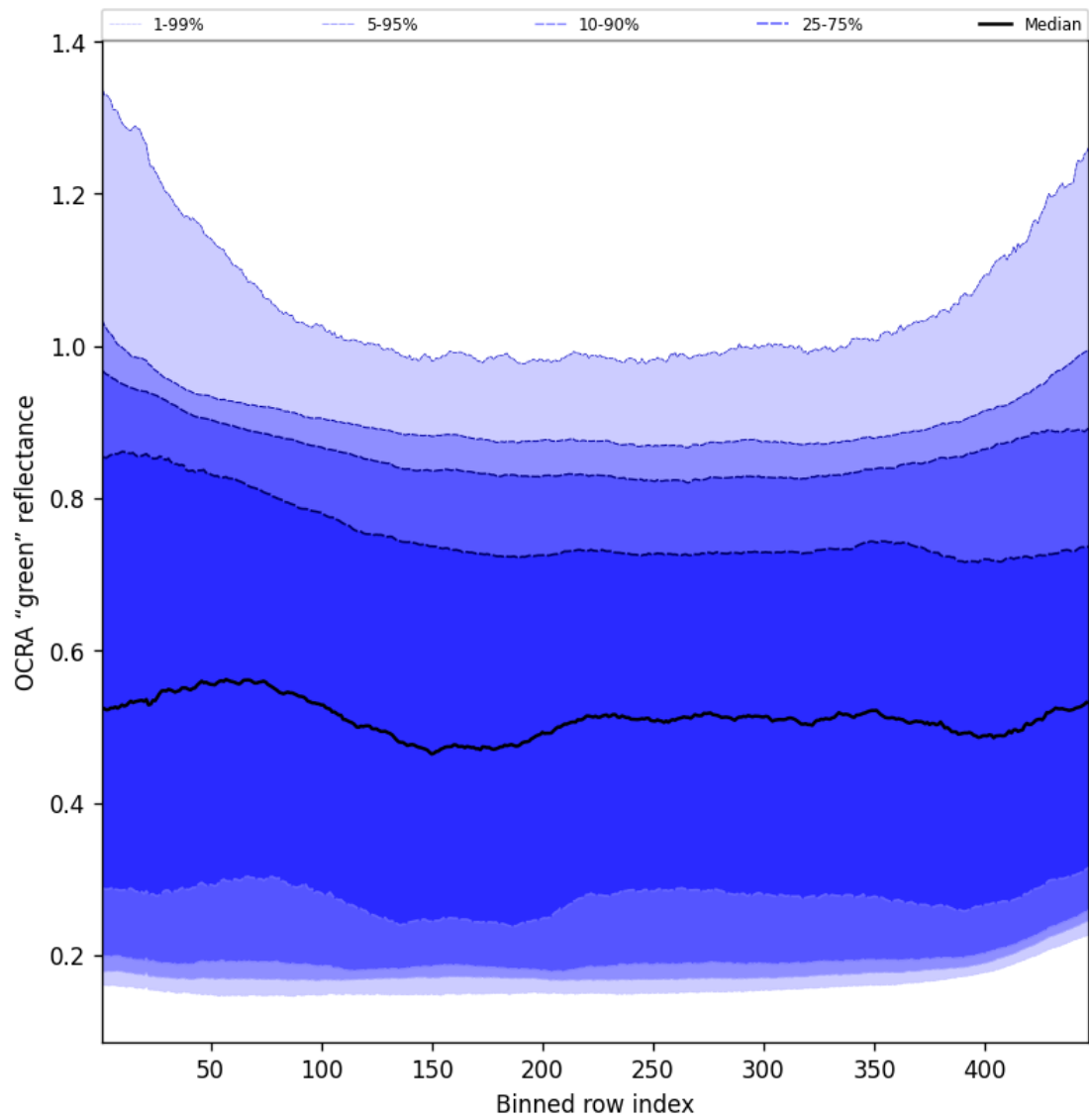
Figure 68: Along track statistics of “OCRA “green” reflectance” for 2025-02-21 to 2025-02-23
