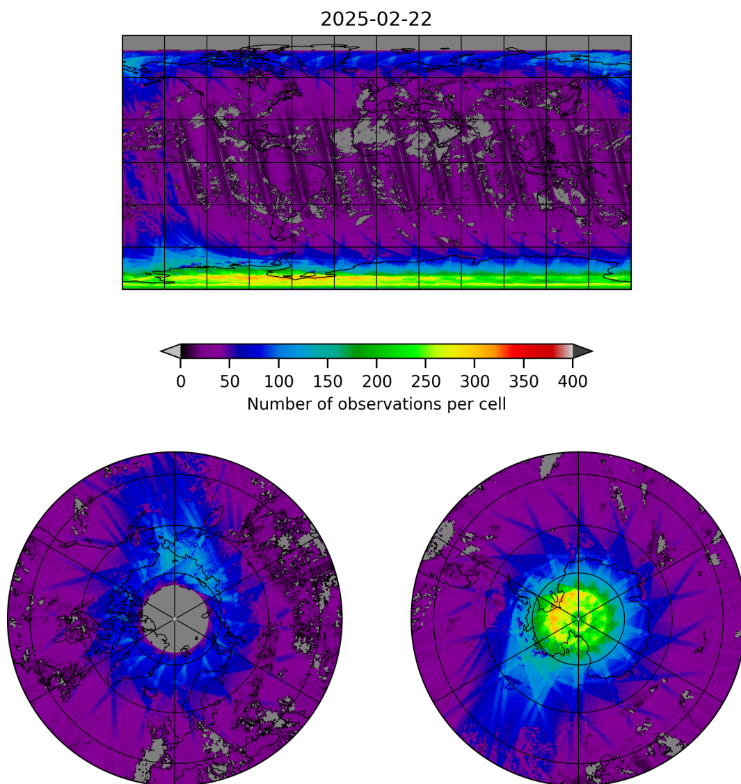
Figure 21: Map of the number of observations for 2025-02-21 to 2025-02-23
