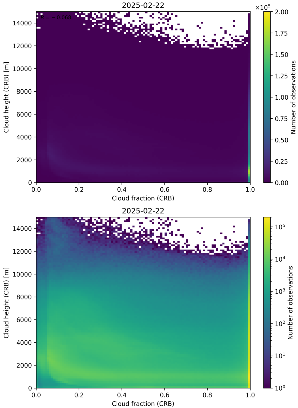
Figure 79: Scatter density plot of “Cloud fraction (CRB)” against “Cloud height (CRB)” for 2025-02-21 to 2025-02-23.
