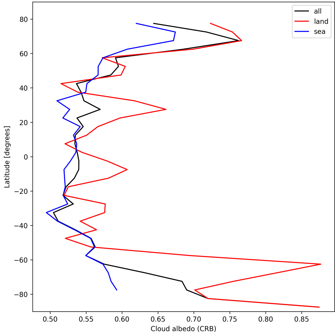
Figure 28: Zonal average of “Cloud albedo (CRB)” for 2025-02-21 to 2025-02-23.
