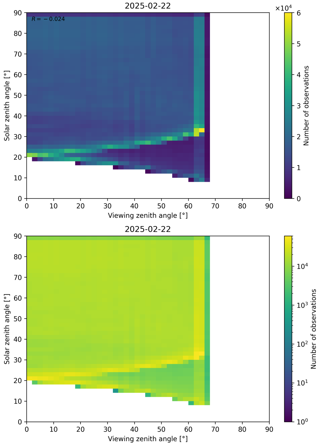
Figure 114: Scatter density plot of “Viewing zenith angle” against “Solar zenith angle” for 2025-02-21 to 2025-02-23.
