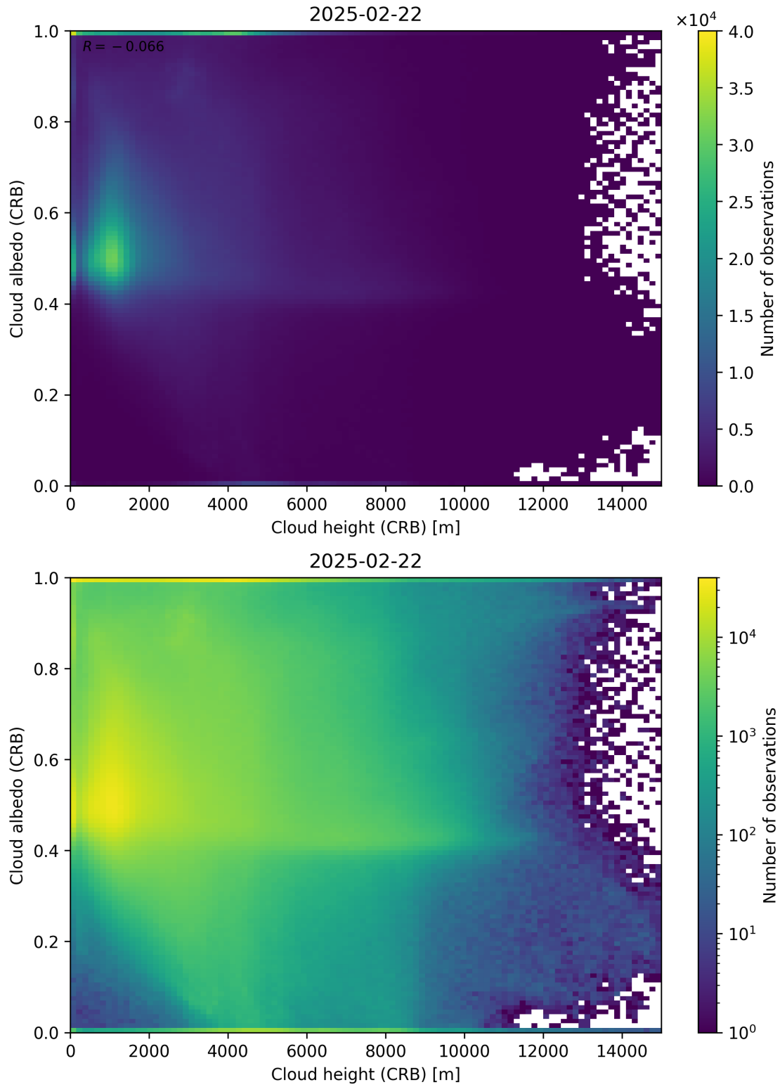
Figure 80: Scatter density plot of “Cloud height (CRB)” against “Cloud albedo (CRB)” for 2025-02-21 to 2025-02-23.
