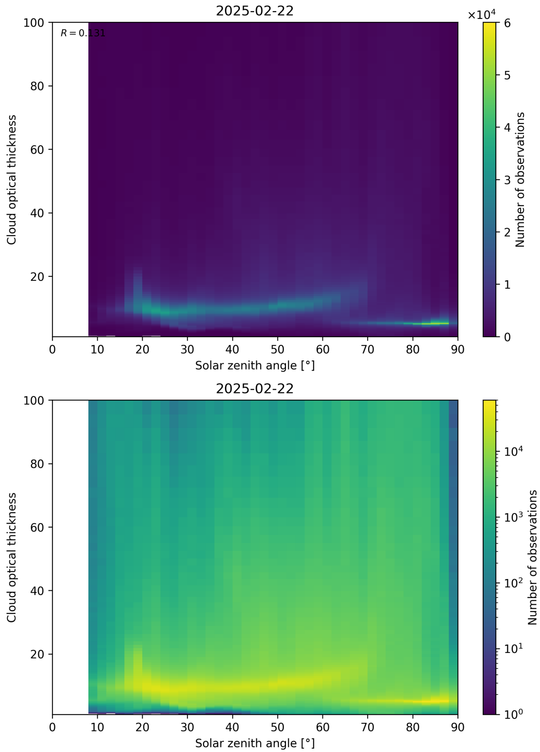
Figure 103: Scatter density plot of “Solar zenith angle” against “Cloud optical thickness” for 2025-02-21 to 2025-02-23.
