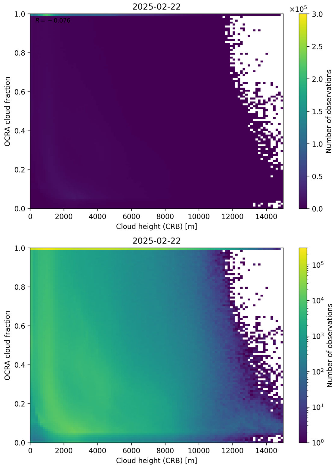
Figure 81: Scatter density plot of “Cloud height (CRB)” against “OCRA cloud fraction” for 2025-02-21 to 2025-02-23.
