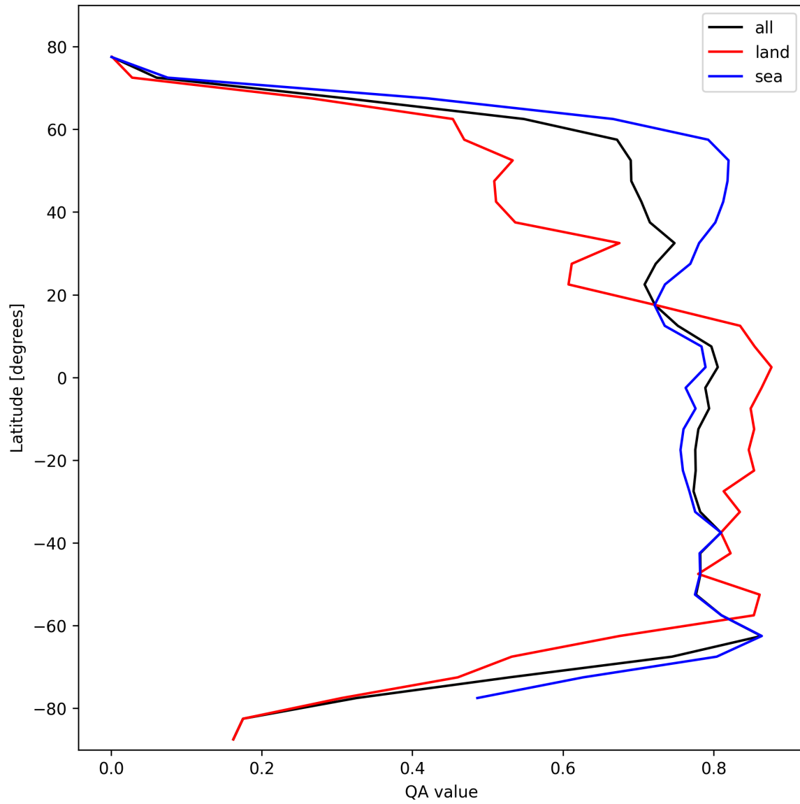
Figure 22: Zonal average of “QA value” for 2025-02-21 to 2025-02-23.
