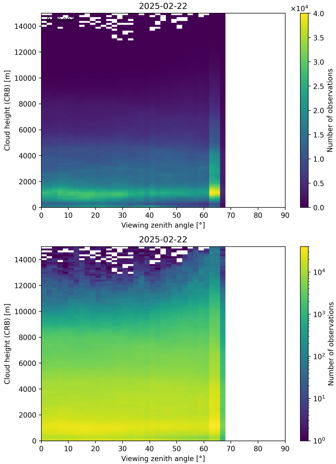
Figure 110: Scatter density plot of “Viewing zenith angle” against “Cloud height (CRB)” for 2025-02-21 to 2025-02-23.
