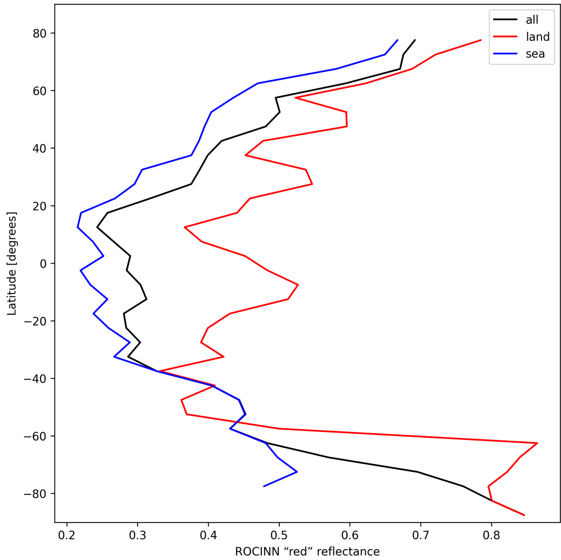
Figure 37: Zonal average of “ROCINN “red” reflectance” for 2025-02-21 to 2025-02-23.
