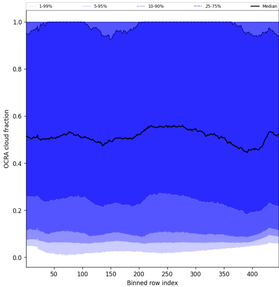
Figure 66: Along track statistics of “OCRA cloud fraction” for 2025-02-21 to 2025-02-23
