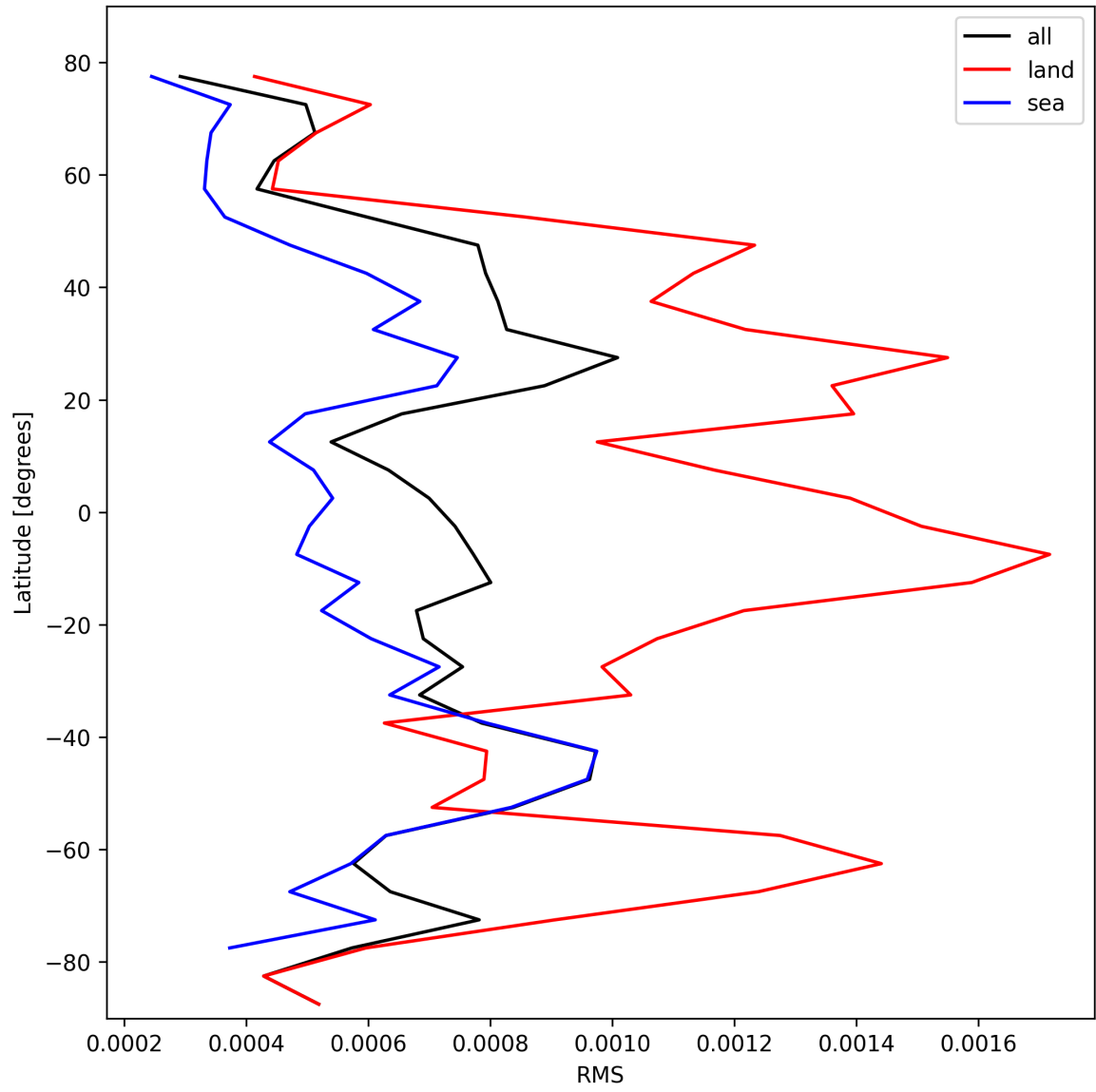
Figure 31: Zonal average of “RMS” for 2025-02-21 to 2025-02-23.
