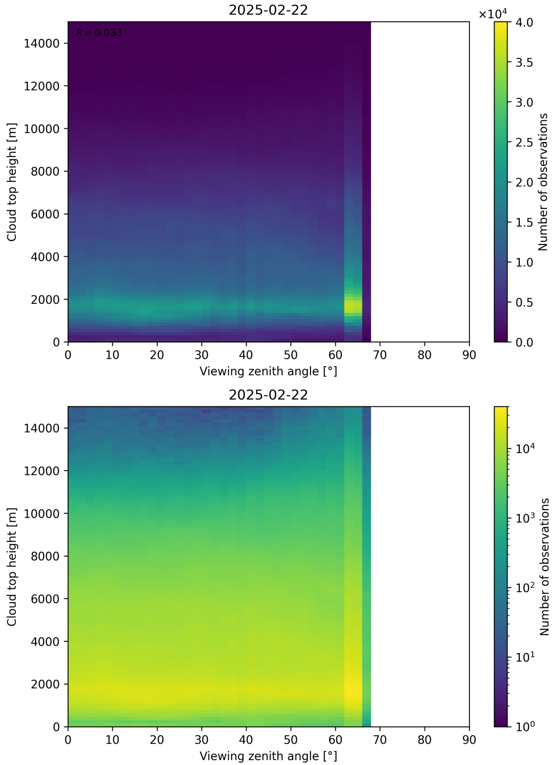
Figure 112: Scatter density plot of “Viewing zenith angle” against “Cloud top height” for 2025-02-21 to 2025-02-23.
