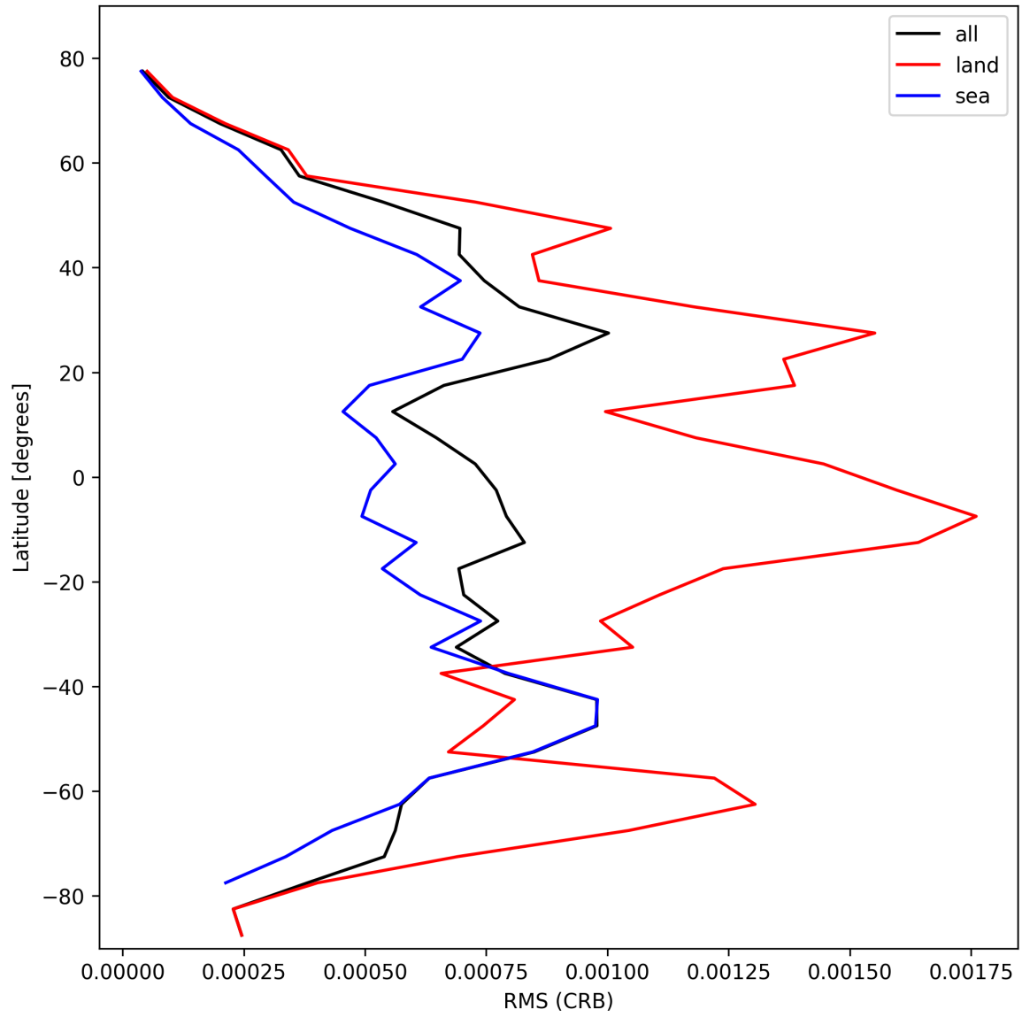
Figure 32: Zonal average of “RMS (CRB)” for 2025-02-21 to 2025-02-23.
