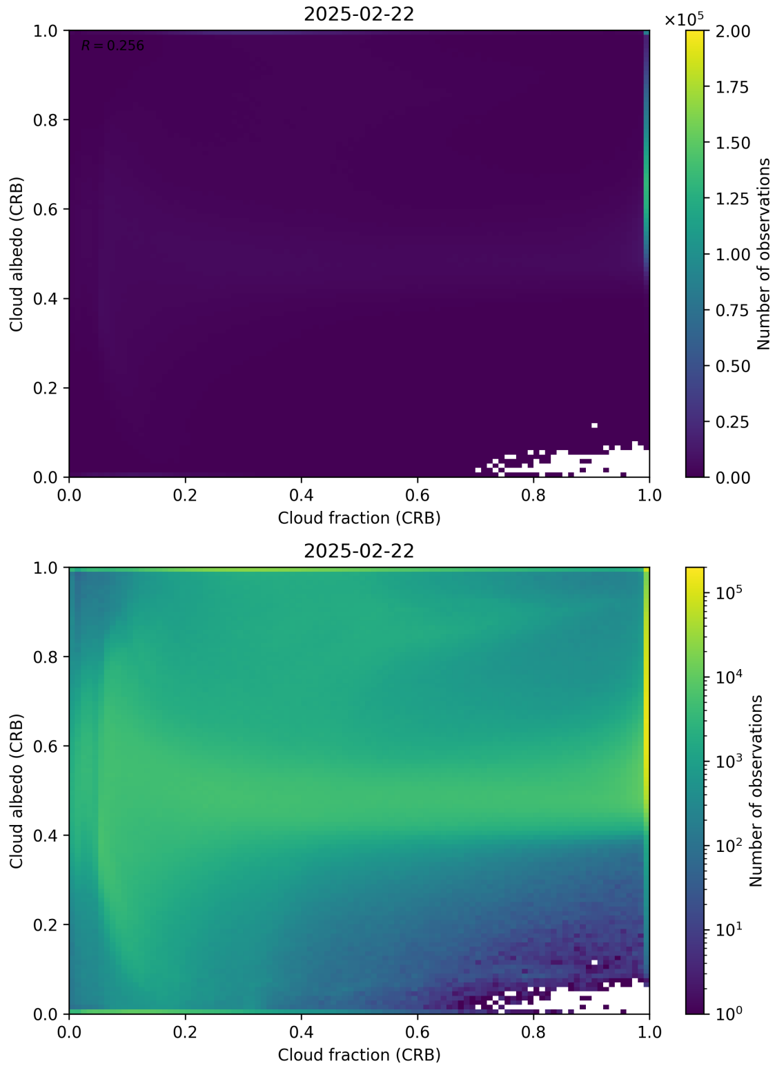
Figure 77: Scatter density plot of “Cloud fraction (CRB)” against “Cloud albedo (CRB)” for 2025-02-21 to 2025-02-23.
