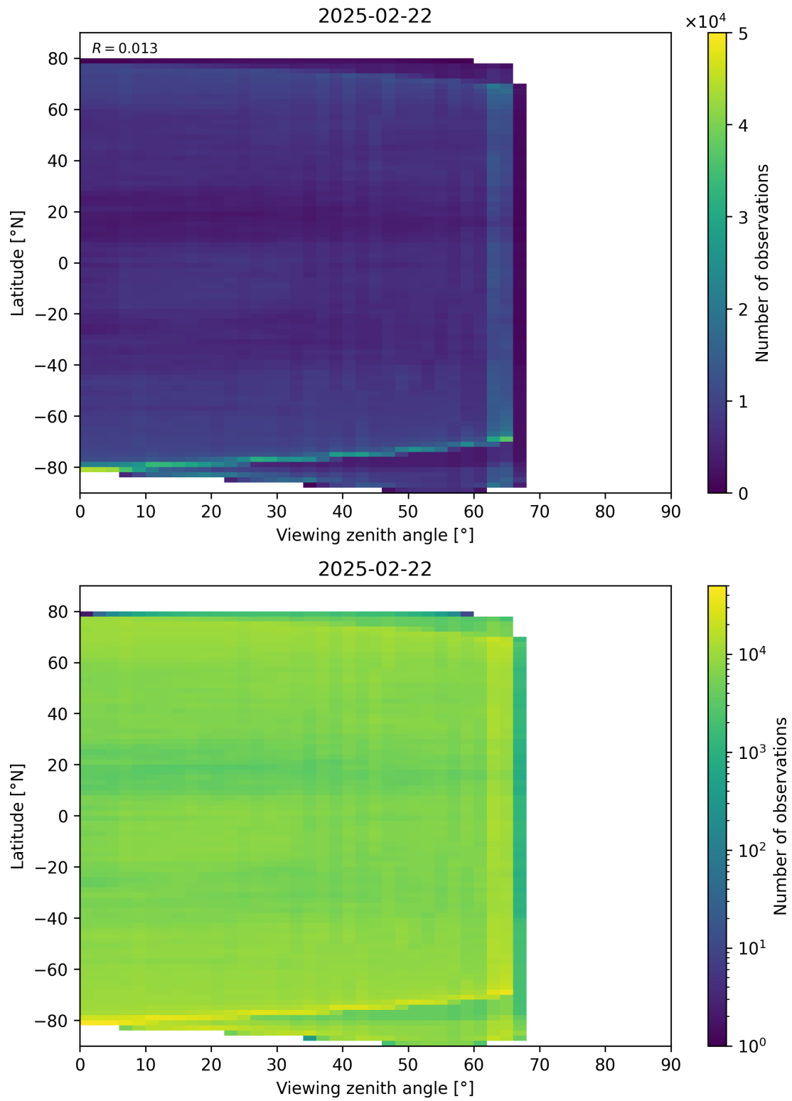
Figure 113: Scatter density plot of “Viewing zenith angle” against “Latitude” for 2025-02-21 to 2025-02-23.
