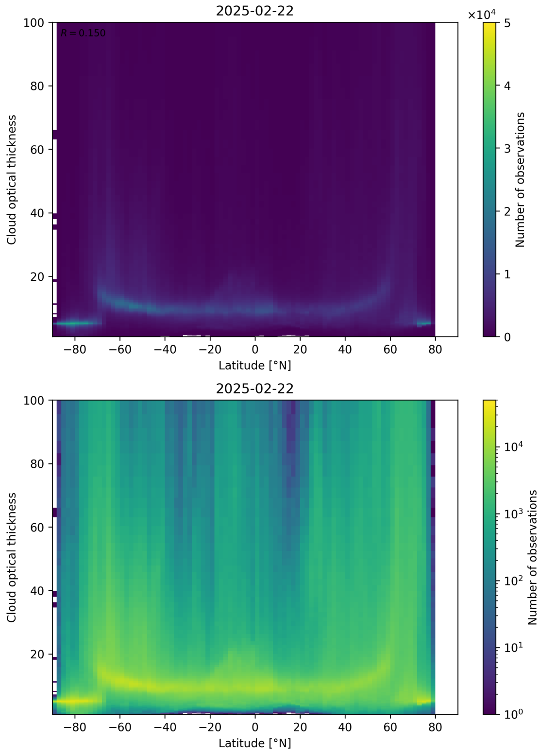
Figure 96: Scatter density plot of “Latitude” against “Cloud optical thickness” for 2025-02-21 to 2025-02-23.
