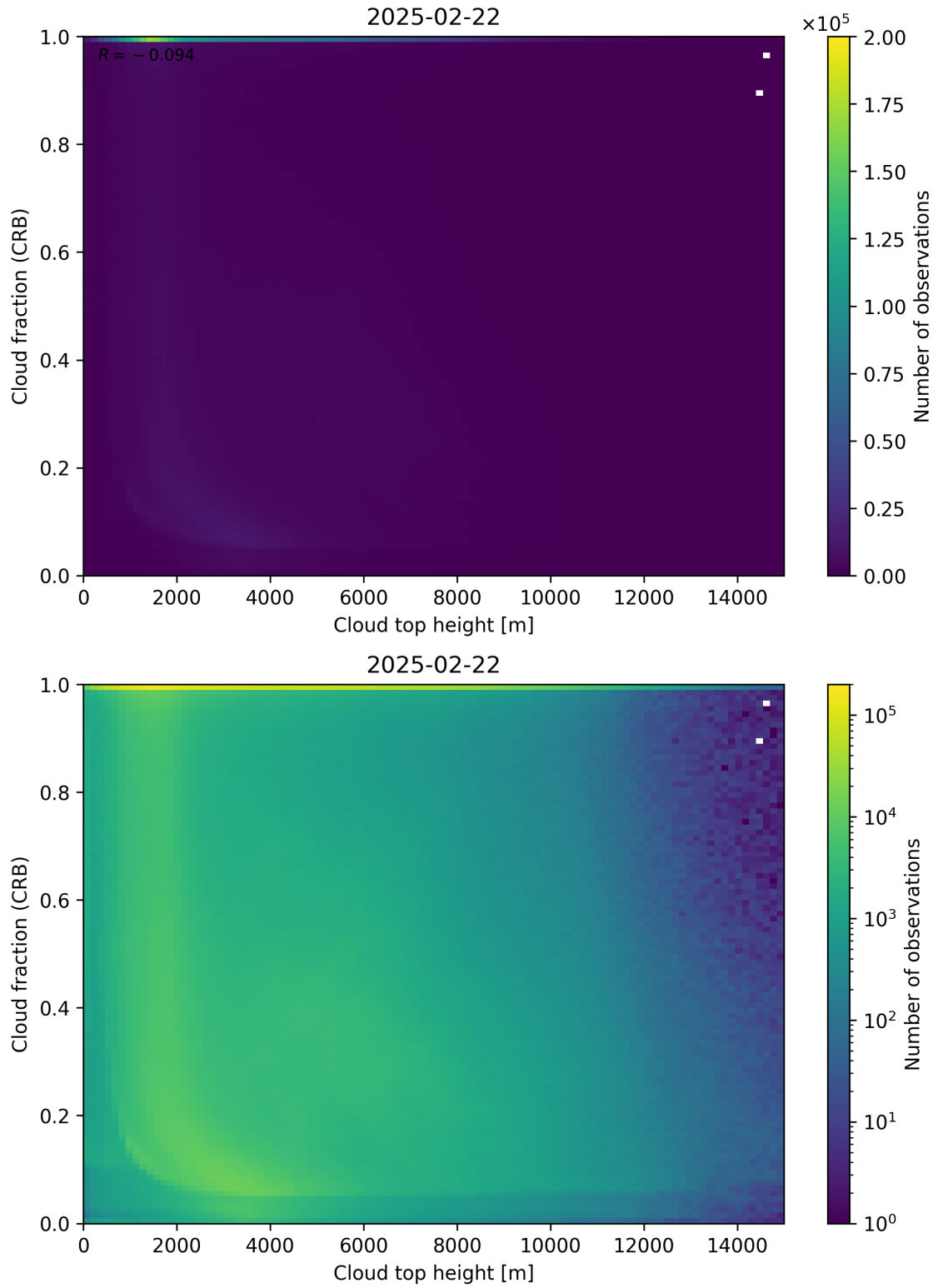
Figure 88: Scatter density plot of “Cloud top height” against “Cloud fraction (CRB)” for 2025-02-21 to 2025-02-23.
