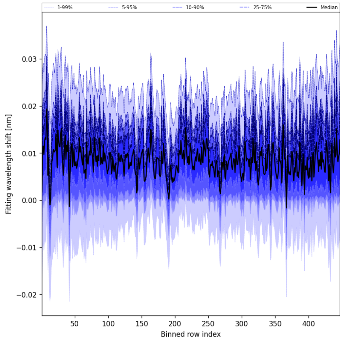
Figure 65: Along track statistics of “Fitting wavelength shift” for 2025-02-21 to 2025-02-23
