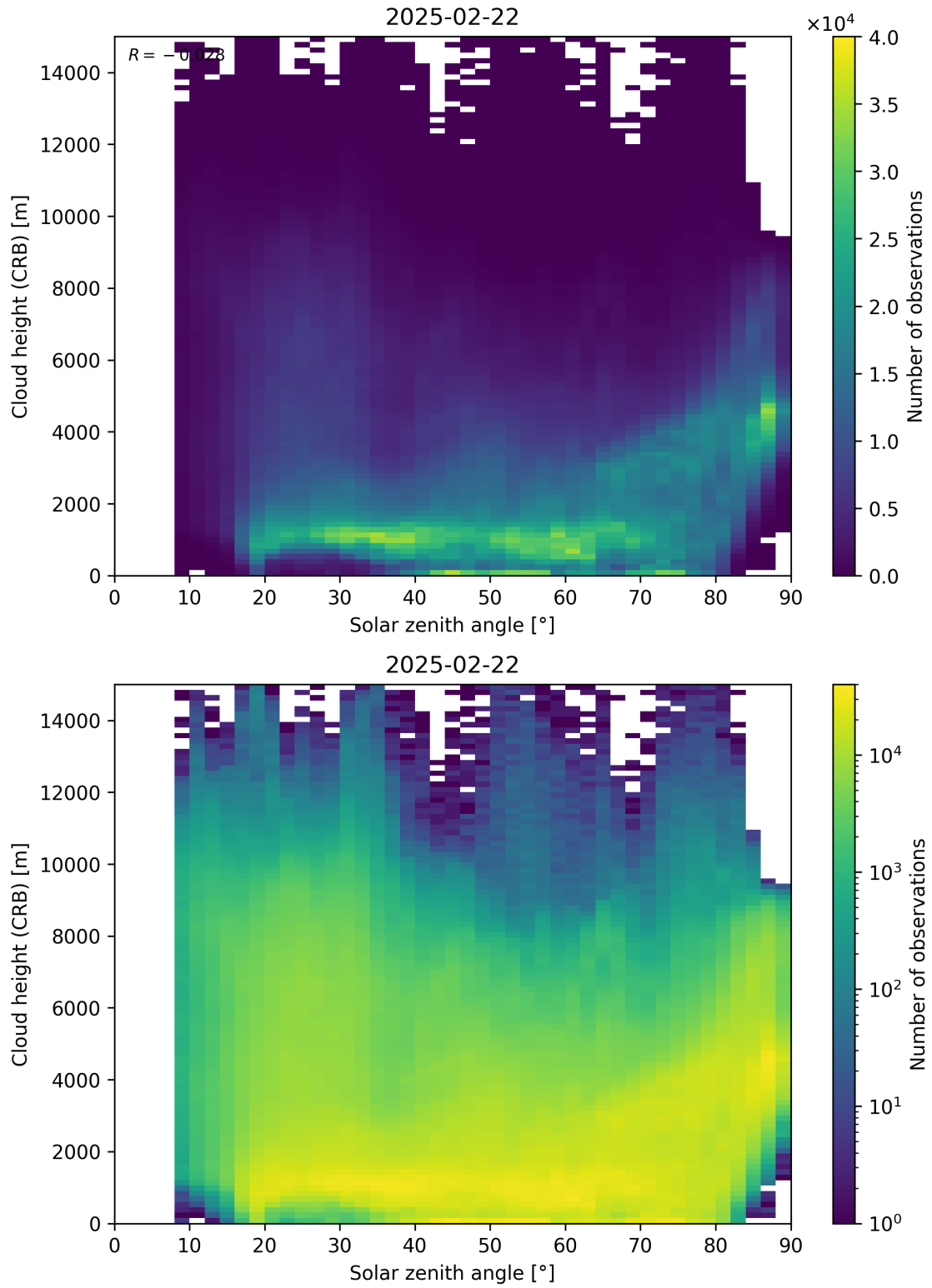
Figure 102: Scatter density plot of “Solar zenith angle” against “Cloud height (CRB)” for 2025-02-21 to 2025-02-23.
