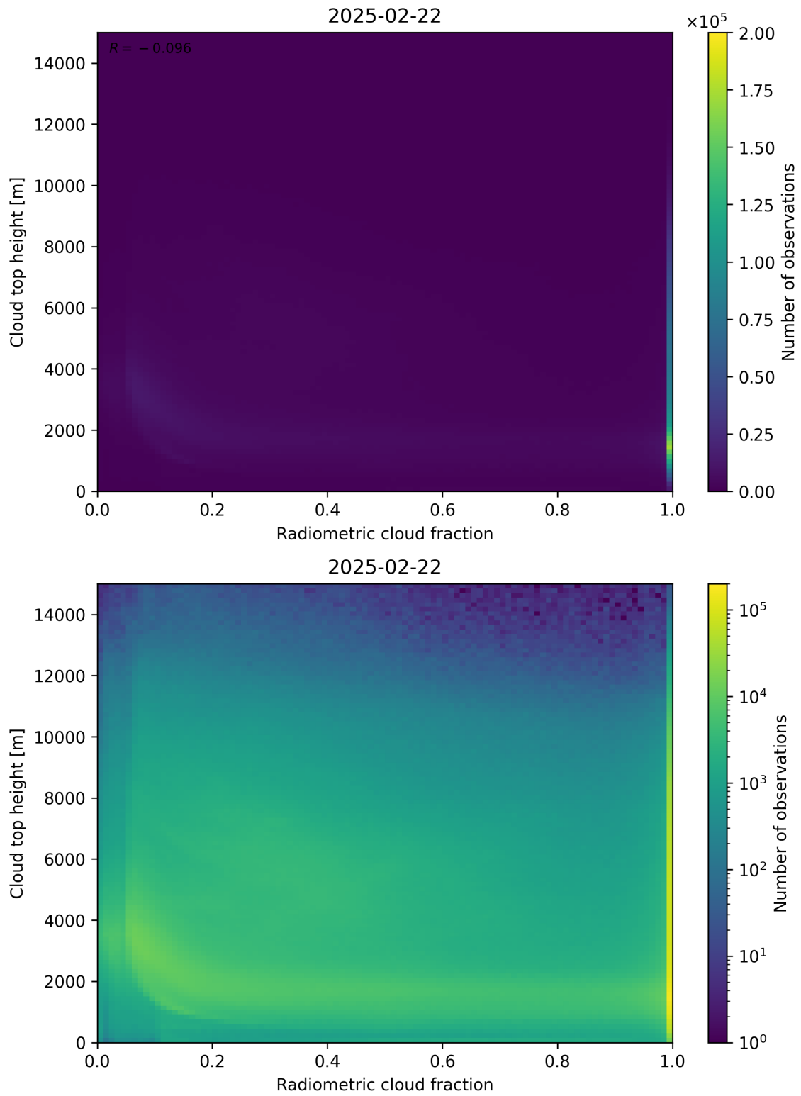
Figure 76: Scatter density plot of “Radiometric cloud fraction” against “Cloud top height” for 2025-02-21 to 2025-02-23.
