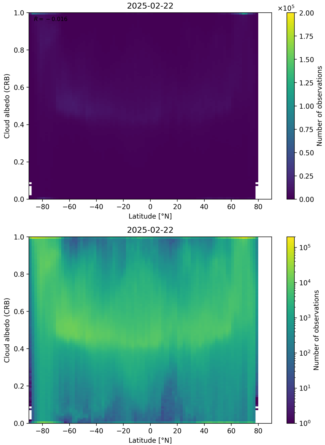
Figure 91: Scatter density plot of “Latitude” against “Cloud albedo (CRB)” for 2025-02-21 to 2025-02-23.
