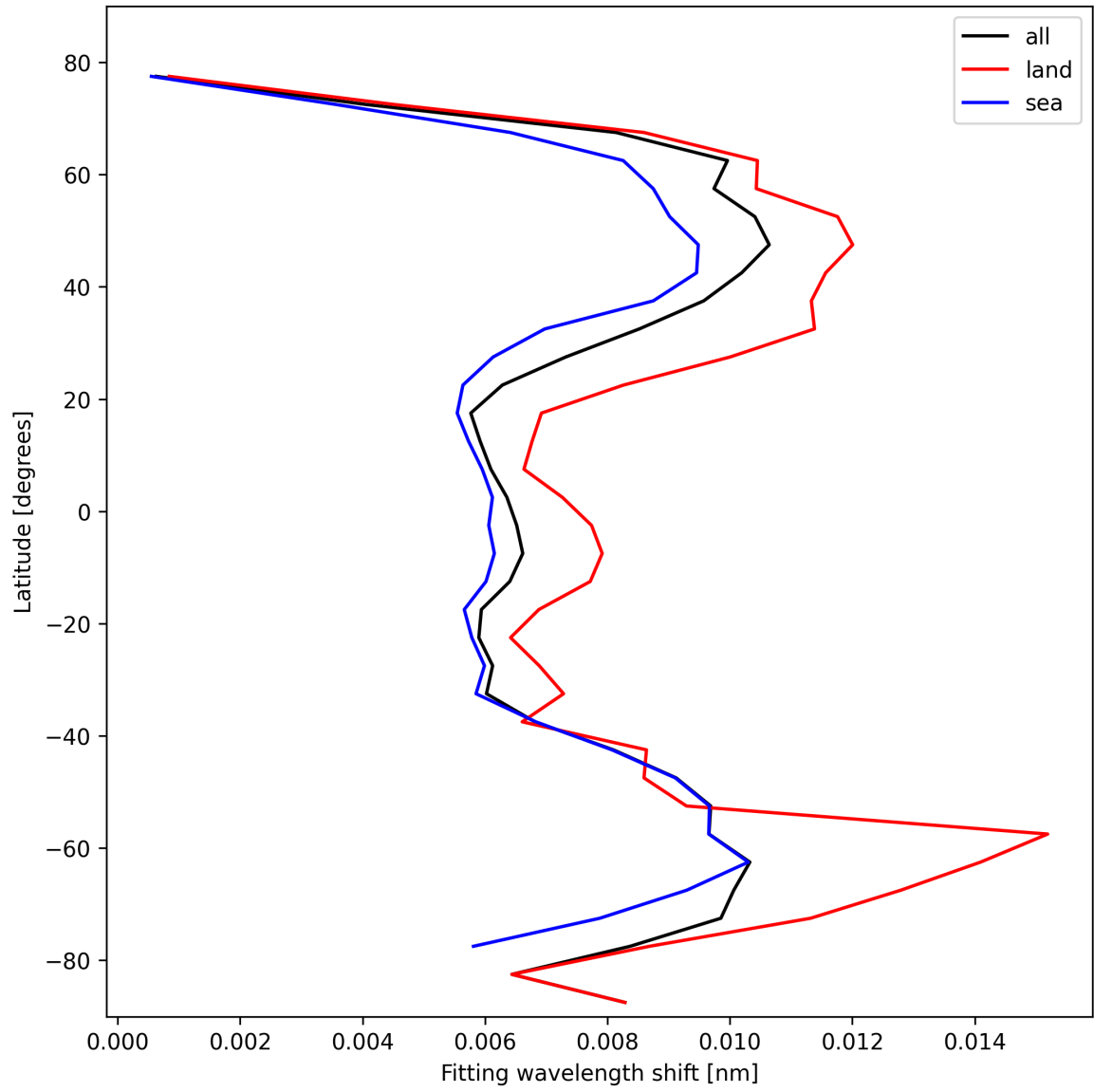
Figure 33: Zonal average of “Fitting wavelength shift” for 2025-02-21 to 2025-02-23.
