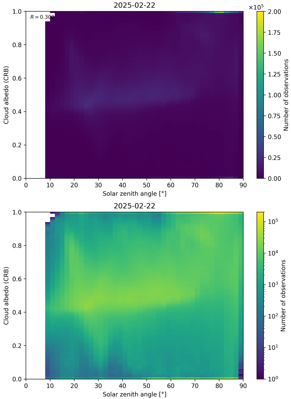
Figure 98: Scatter density plot of “Solar zenith angle” against “Cloud albedo (CRB)” for 2025-02-21 to 2025-02-23.
