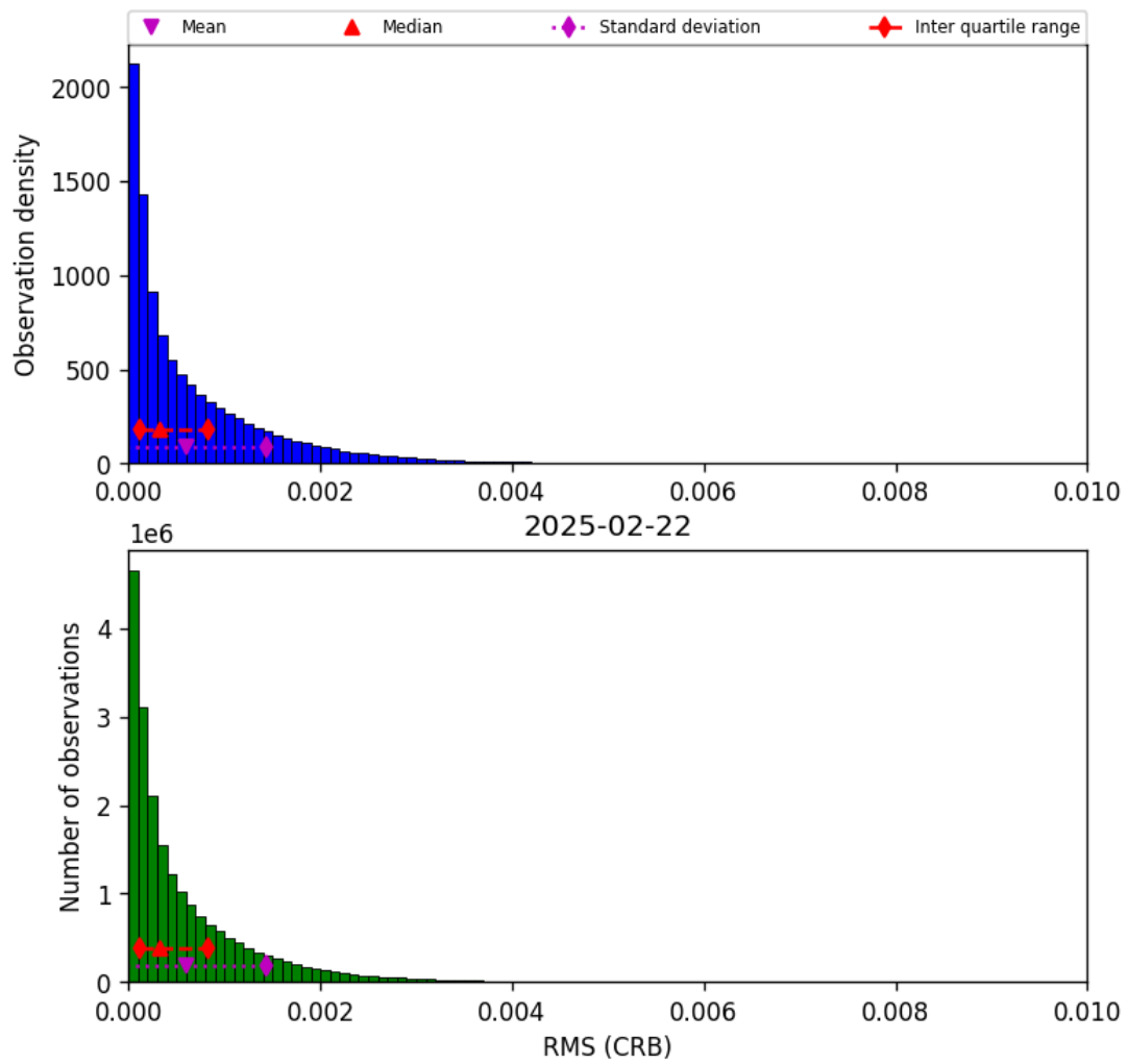
Figure 48: Histogram of “RMS (CRB)” for 2025-02-21 to 2025-02-23
