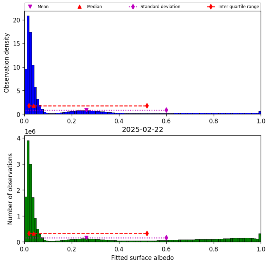
Figure 45: Histogram of “Fitted surface albedo” for 2025-02-21 to 2025-02-23
