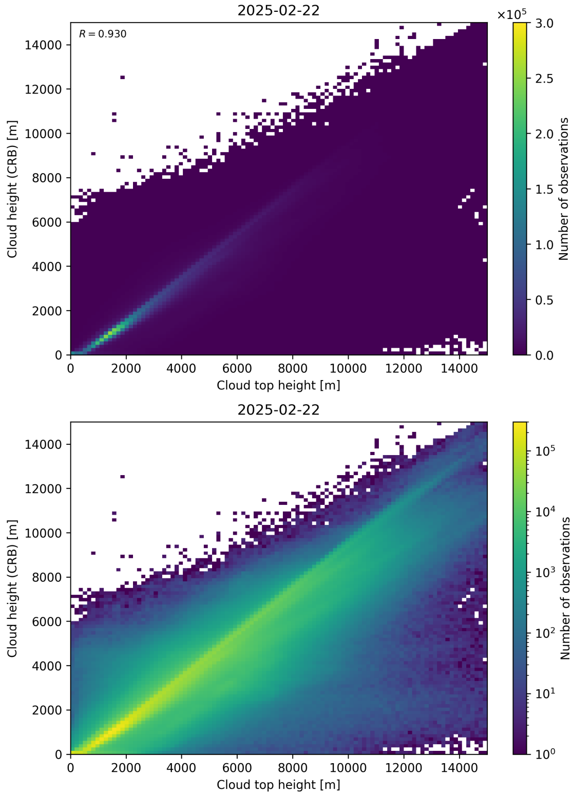
Figure 89: Scatter density plot of “Cloud top height” against “Cloud height (CRB)” for 2025-02-21 to 2025-02-23.
