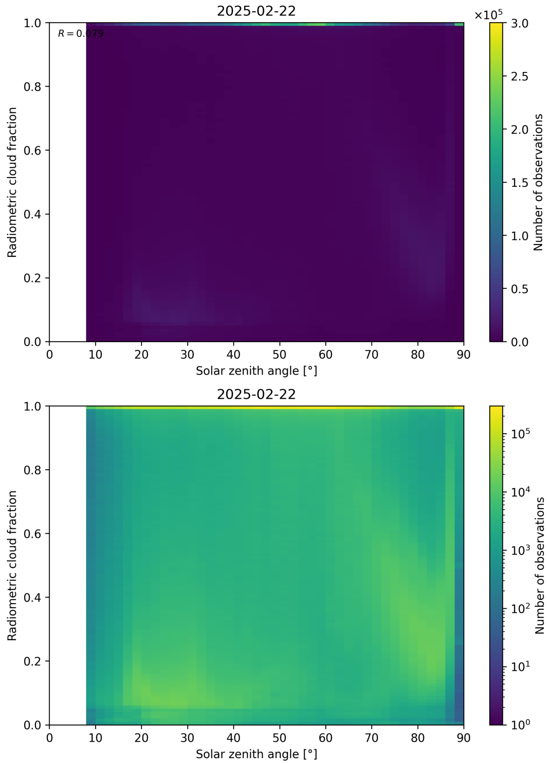
Figure 99: Scatter density plot of “Solar zenith angle” against “Radiometric cloud fraction” for 2025-02-21 to 2025-02-23.
