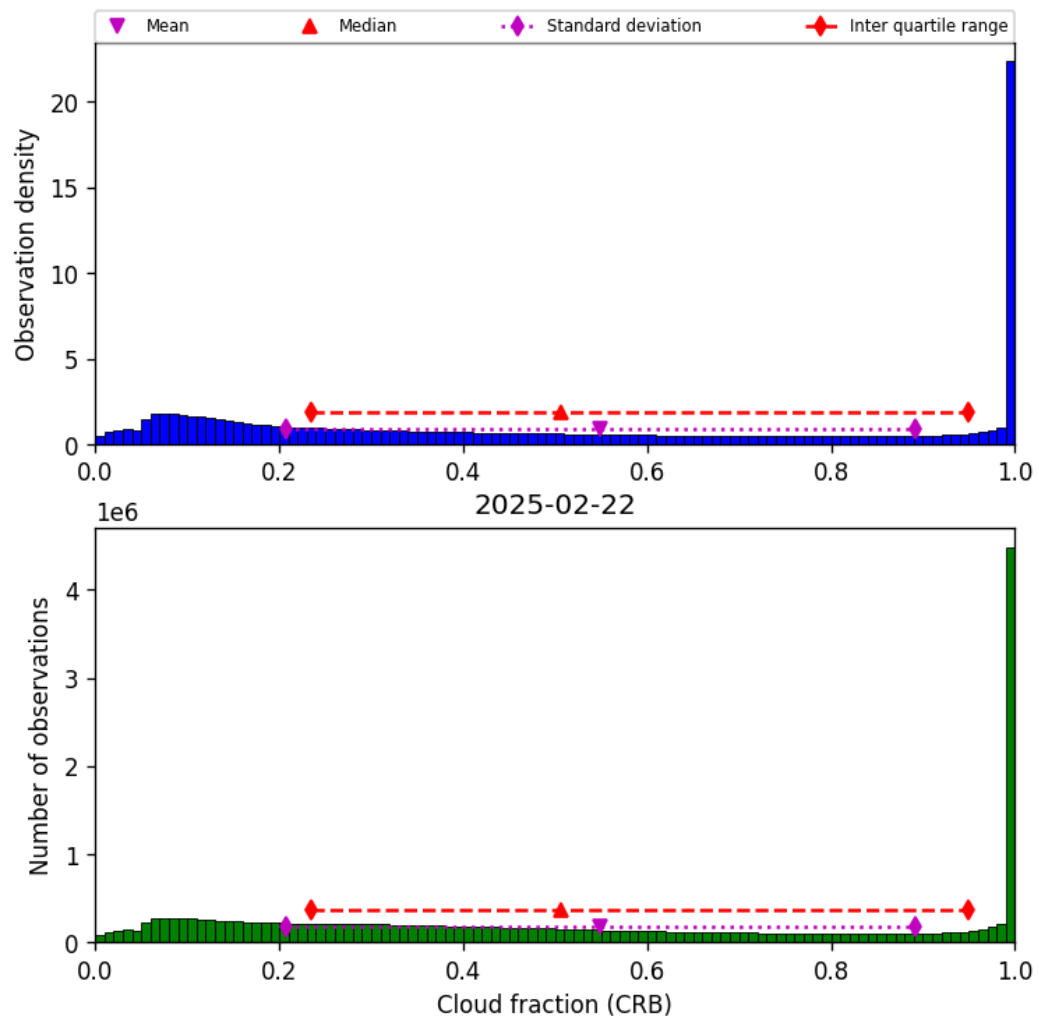
Figure 42: Histogram of “Cloud fraction (CRB)” for 2025-02-21 to 2025-02-23
