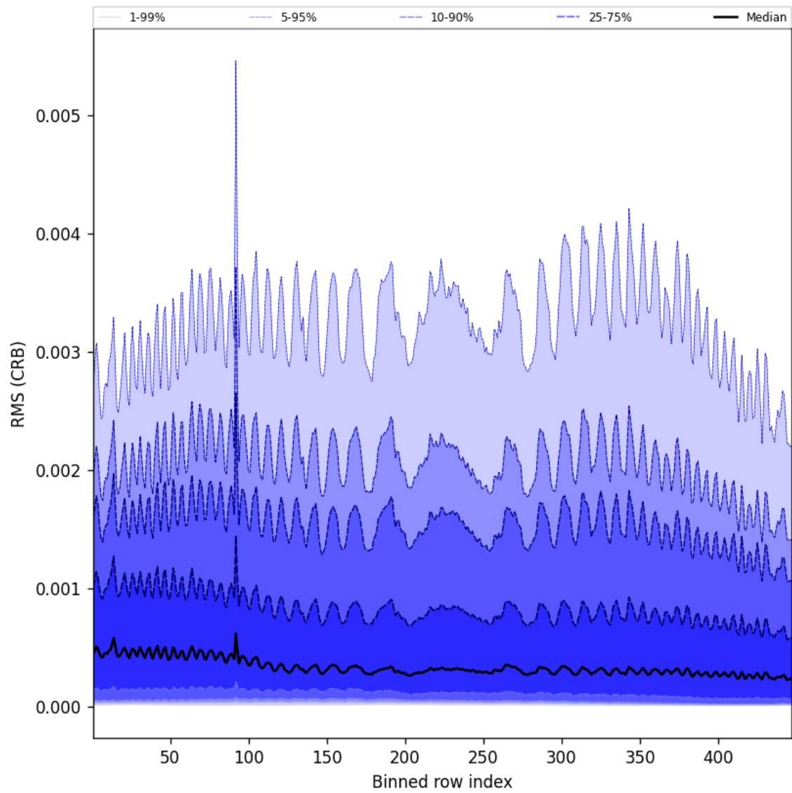
Figure 64: Along track statistics of “RMS (CRB)” for 2025-02-21 to 2025-02-23
