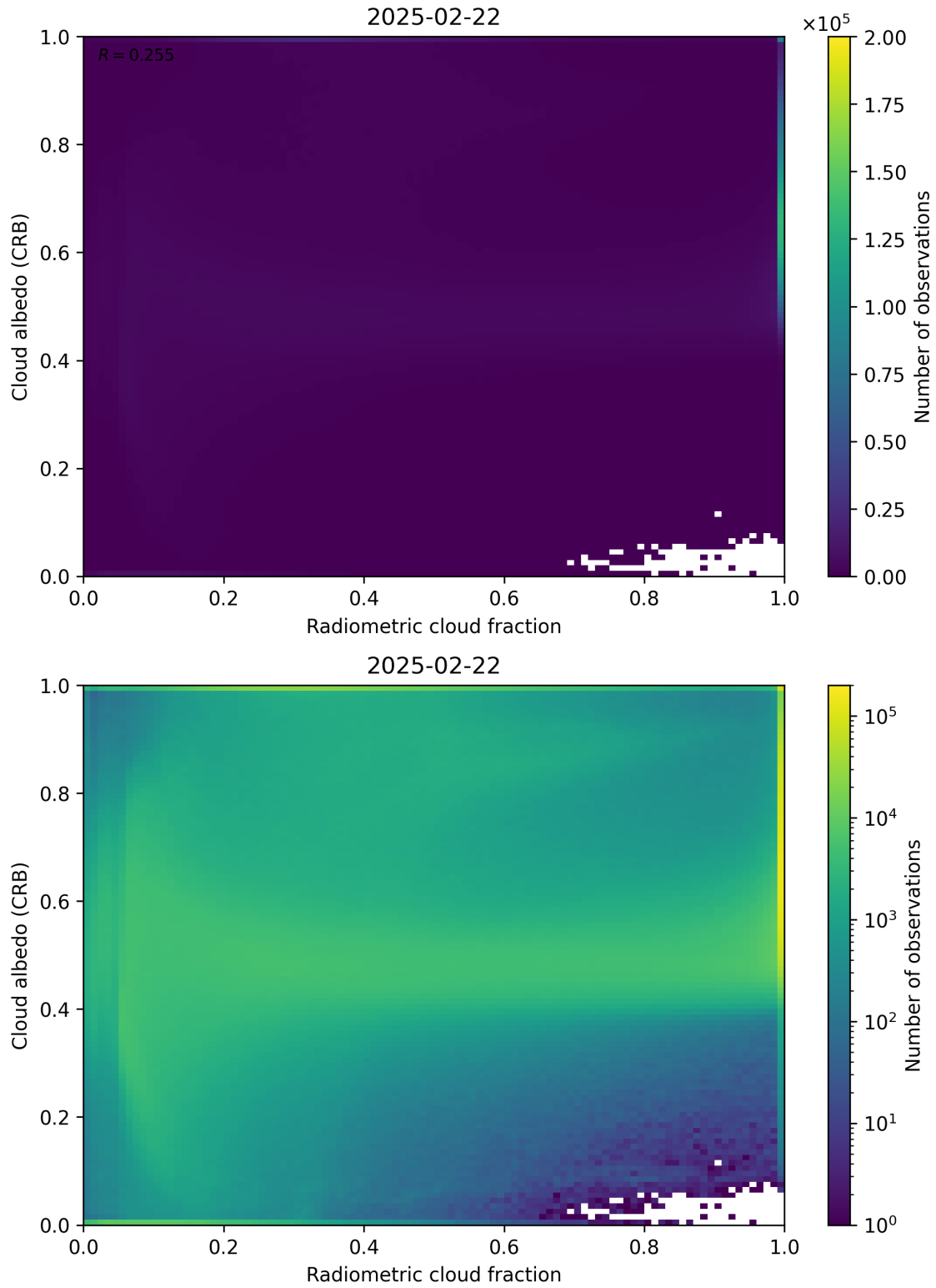
Figure 71: Scatter density plot of “Radiometric cloud fraction” against “Cloud albedo (CRB)” for 2025-02-21 to 2025-02-23.
