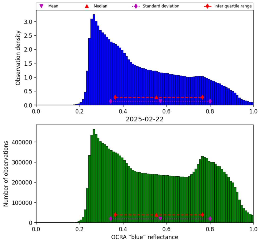
Figure 51: Histogram of “OCRA “blue” reflectance” for 2025-02-21 to 2025-02-23
