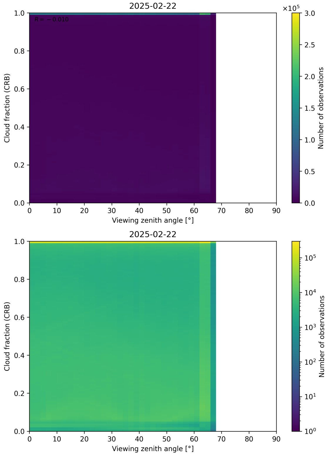
Figure 109: Scatter density plot of “Viewing zenith angle” against “Cloud fraction (CRB)” for 2025-02-21 to 2025-02-23.
