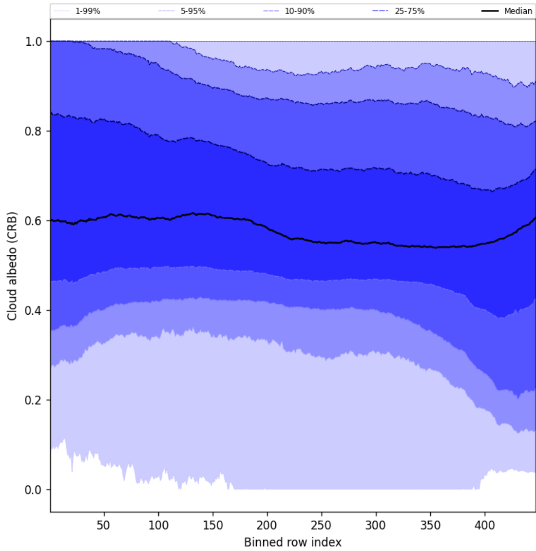
Figure 60: Along track statistics of “Cloud albedo (CRB)” for 2025-02-21 to 2025-02-23
