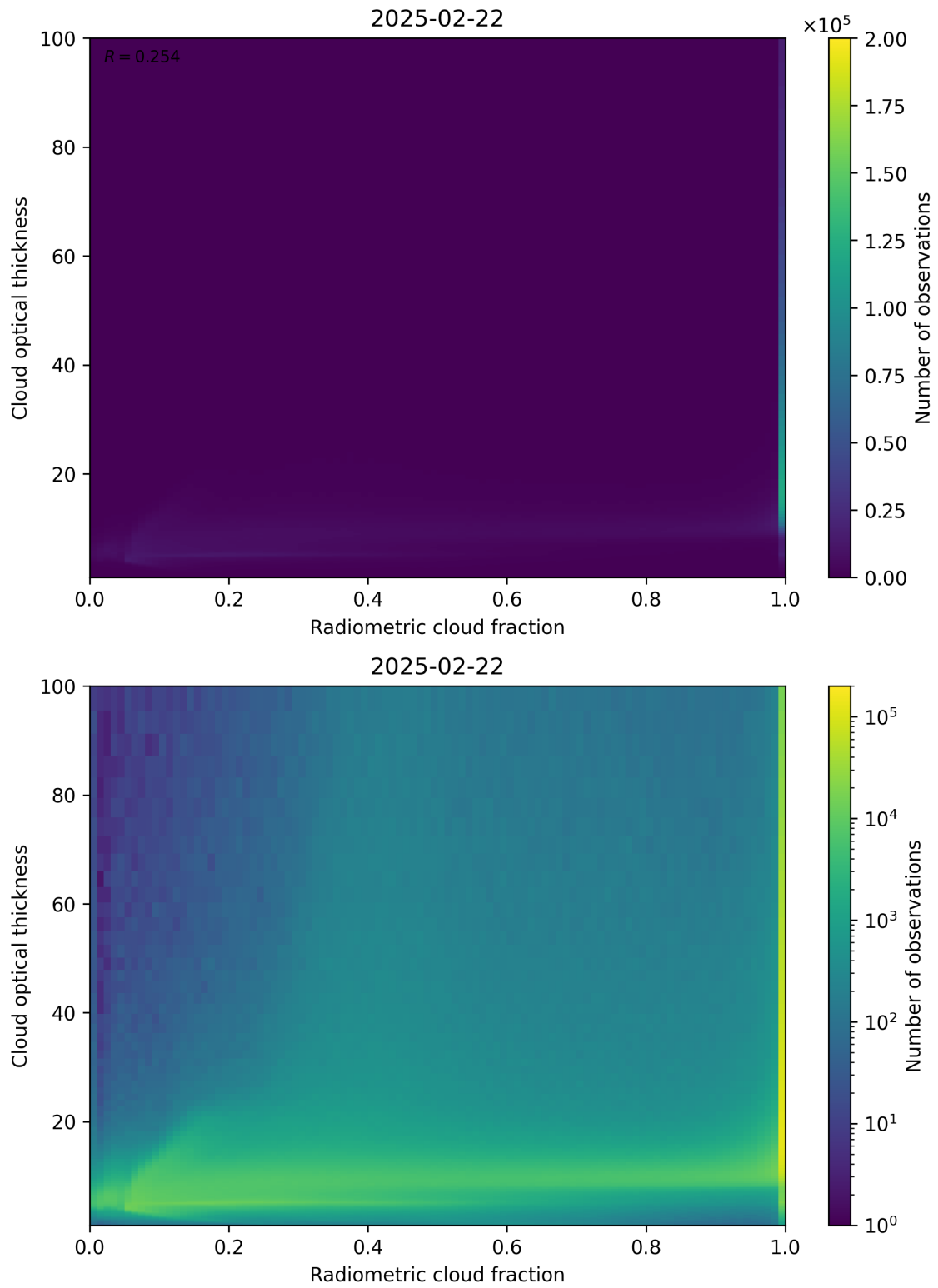
Figure 75: Scatter density plot of “Radiometric cloud fraction” against “Cloud optical thickness” for 2025-02-21 to 2025-02-23.
