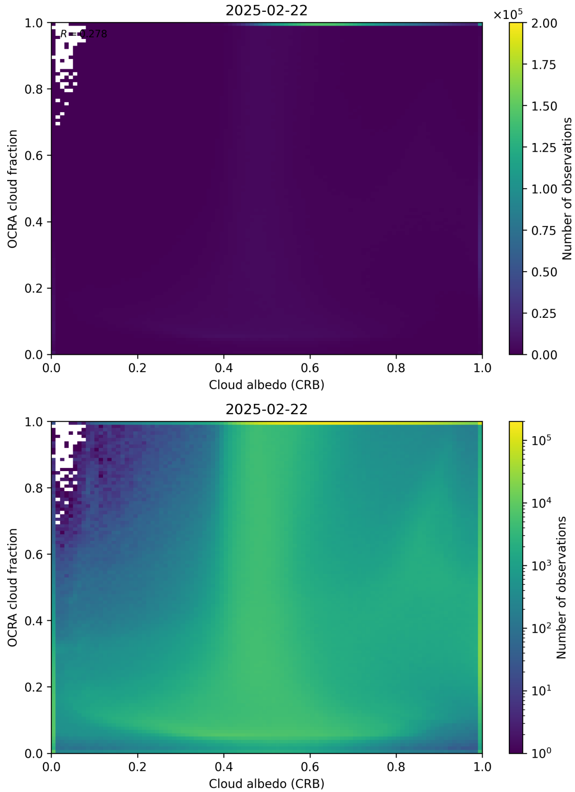
Figure 70: Scatter density plot of “Cloud albedo (CRB)” against “OCRA cloud fraction” for 2025-02-21 to 2025-02-23.
