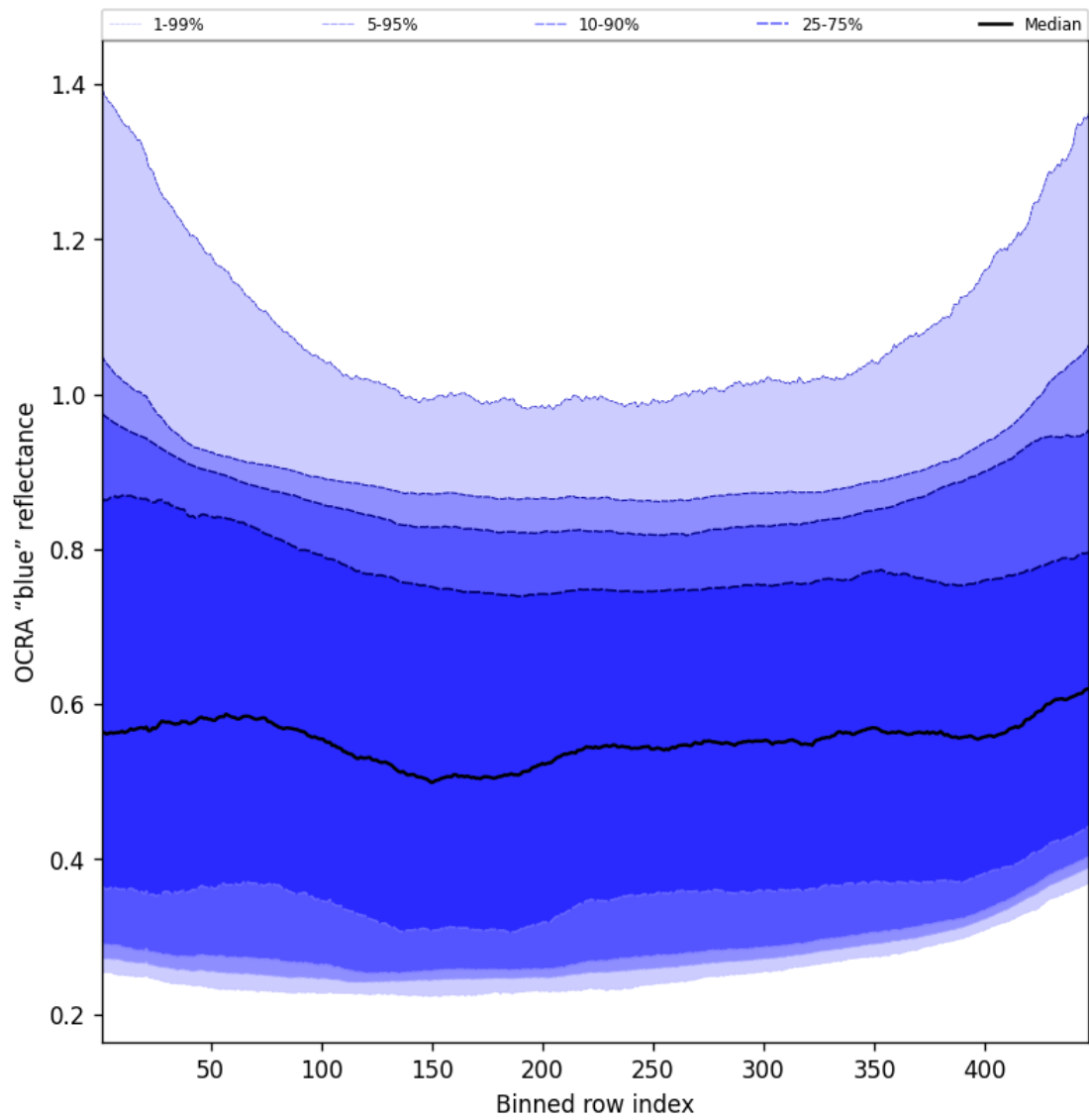
Figure 67: Along track statistics of "OCRA "blue" reflectance" for 2025-02-21 to 2025-02-23
