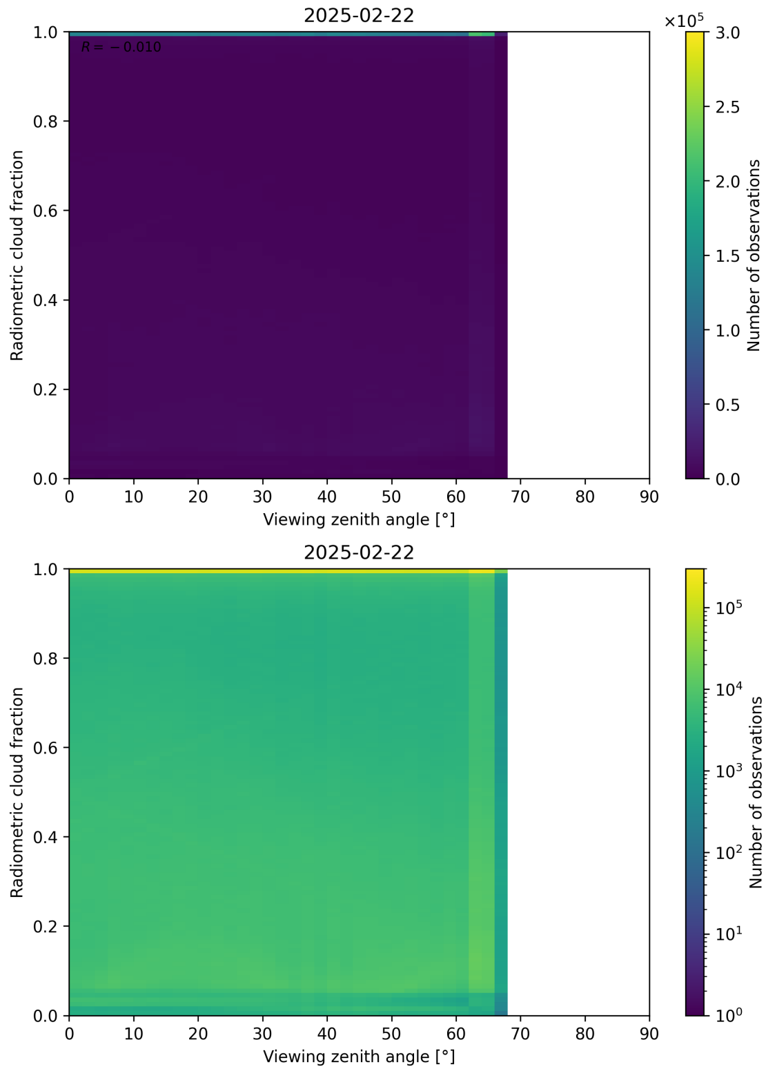
Figure 107: Scatter density plot of “Viewing zenith angle” against “Radiometric cloud fraction” for 2025-02-21 to 2025-02-23.
