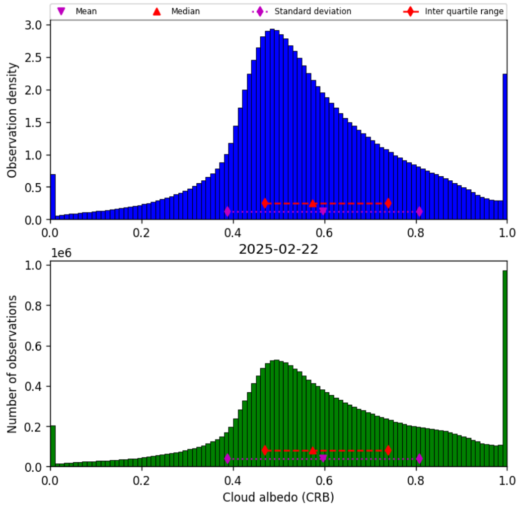
Figure 44: Histogram of “Cloud albedo (CRB)” for 2025-02-21 to 2025-02-23
