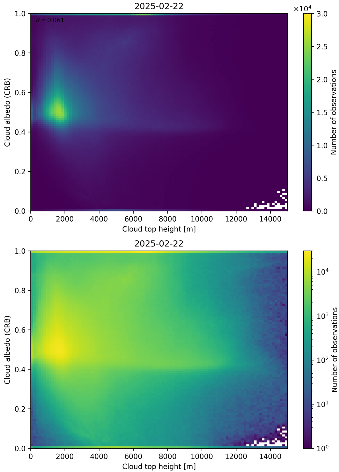
Figure 86: Scatter density plot of “Cloud top height” against “Cloud albedo (CRB)” for 2025-02-21 to 2025-02-23.
