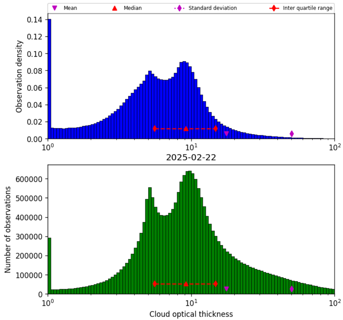
Figure 41: Histogram of “Cloud optical thickness” for 2025-02-21 to 2025-02-23
