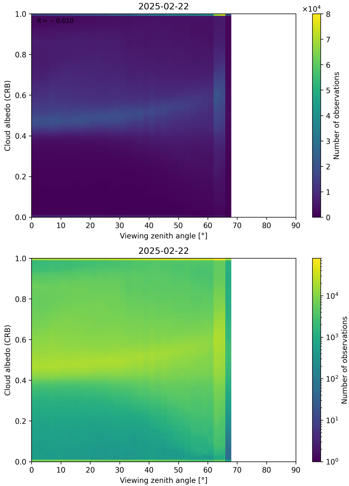
Figure 106: Scatter density plot of “Viewing zenith angle” against “Cloud albedo (CRB)” for 2025-02-21 to 2025-02-23.
