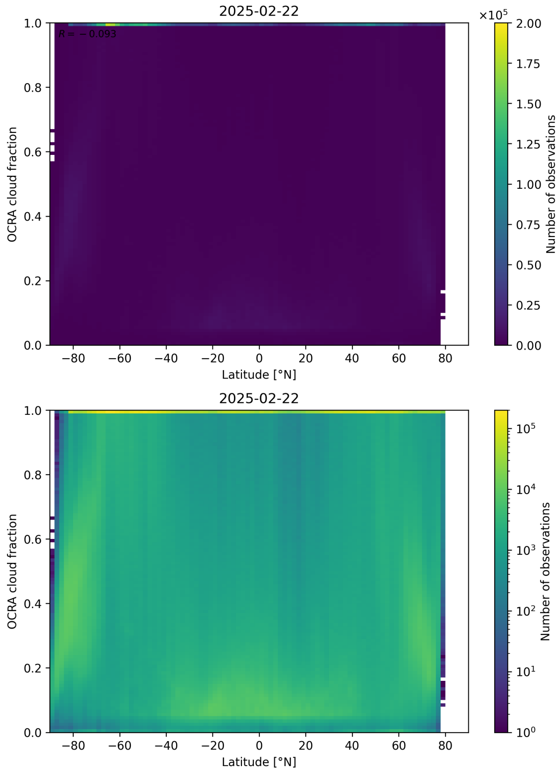
Figure 93: Scatter density plot of “Latitude” against “OCRA cloud fraction” for 2025-02-21 to 2025-02-23.
