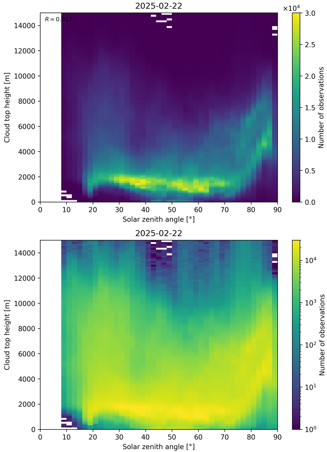
Figure 104: Scatter density plot of “Solar zenith angle” against “Cloud top height” for 2025-02-21 to 2025-02-23.
