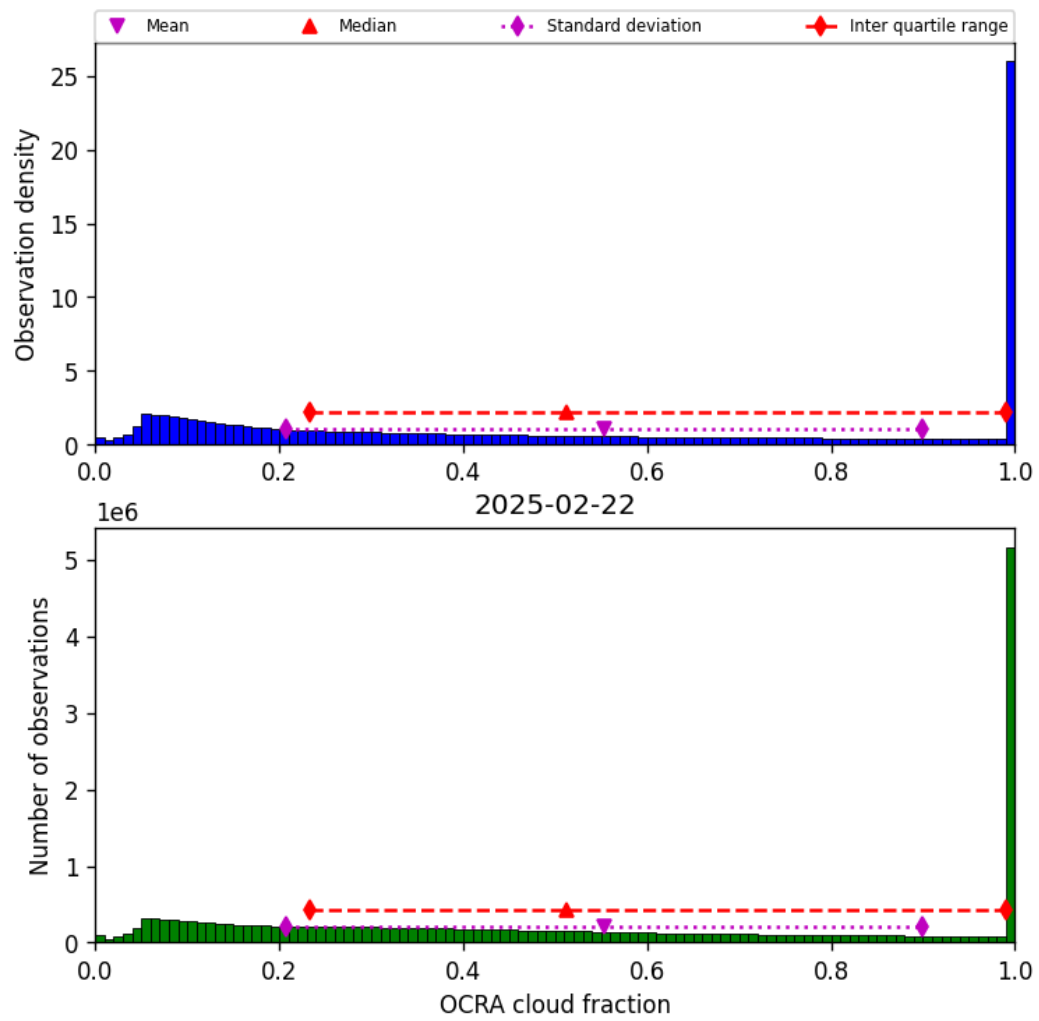
Figure 50: Histogram of “OCRA cloud fraction” for 2025-02-21 to 2025-02-23
