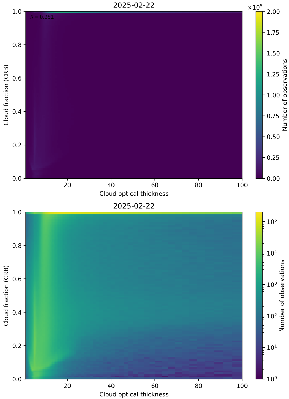
Figure 84: Scatter density plot of “Cloud optical thickness” against “Cloud fraction (CRB)” for 2025-02-21 to 2025-02-23.
