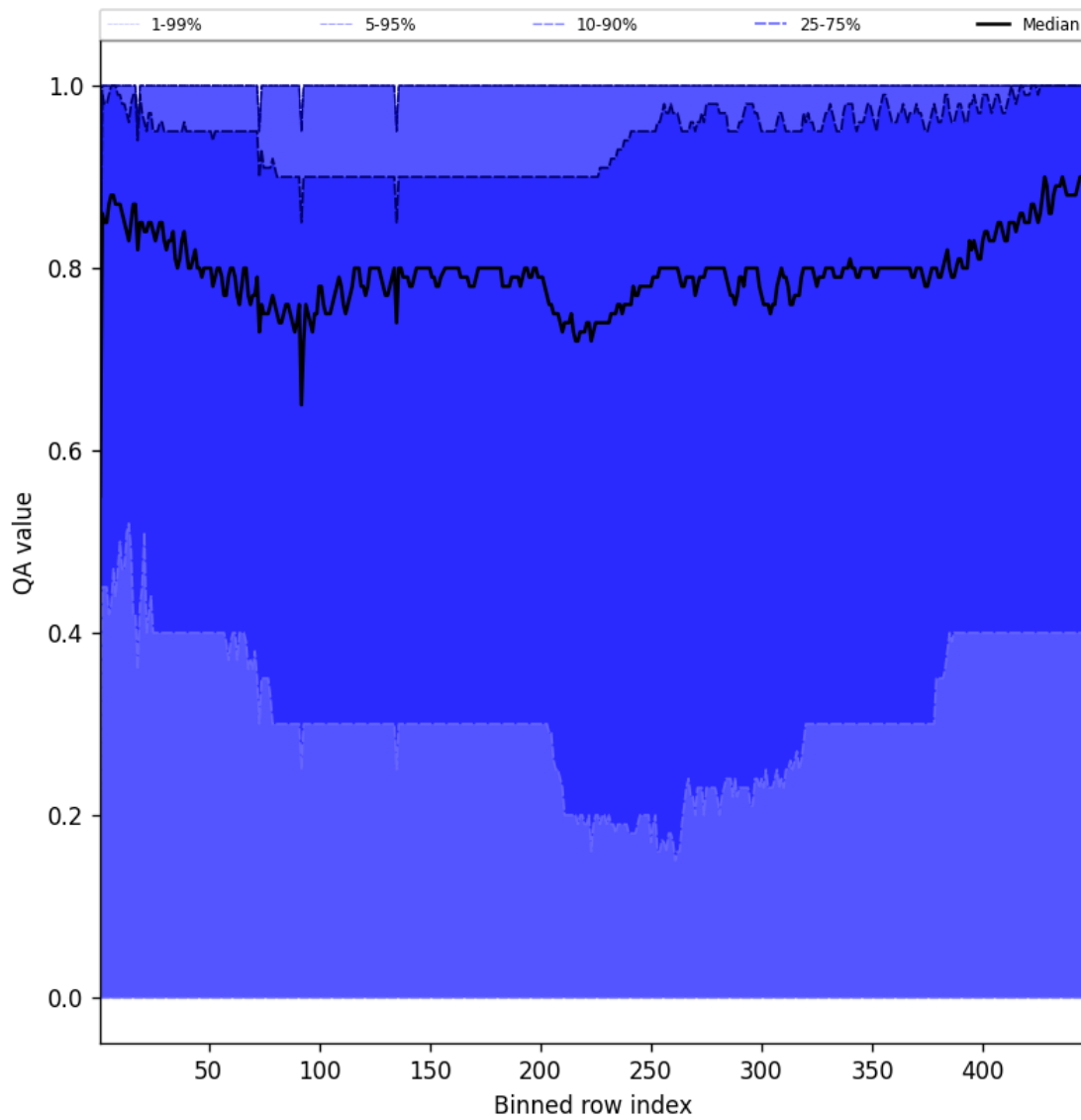
Figure 54: Along track statistics of “QA value” for 2025-02-21 to 2025-02-23
