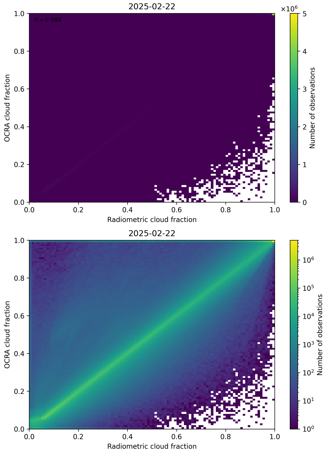
Figure 72: Scatter density plot of “Radiometric cloud fraction” against “OCRA cloud fraction” for 2025-02-21 to 2025-02-23.
