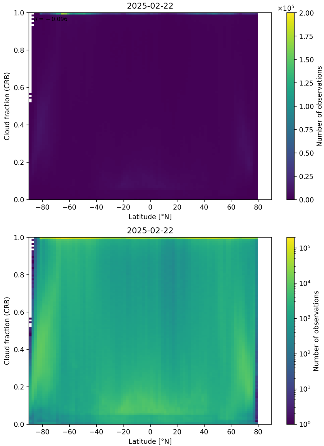
Figure 94: Scatter density plot of “Latitude” against “Cloud fraction (CRB)” for 2025-02-21 to 2025-02-23.
