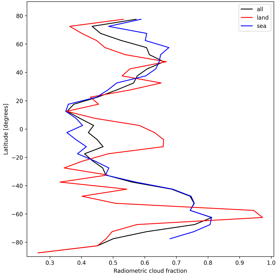
Figure 23: Zonal average of “Radiometric cloud fraction” for 2025-02-21 to 2025-02-23.
