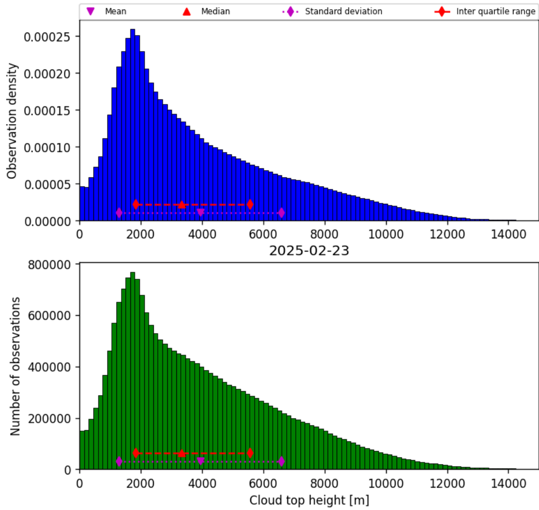
Figure 40: Histogram of “Cloud top height” for 2025-02-22 to 2025-02-24
