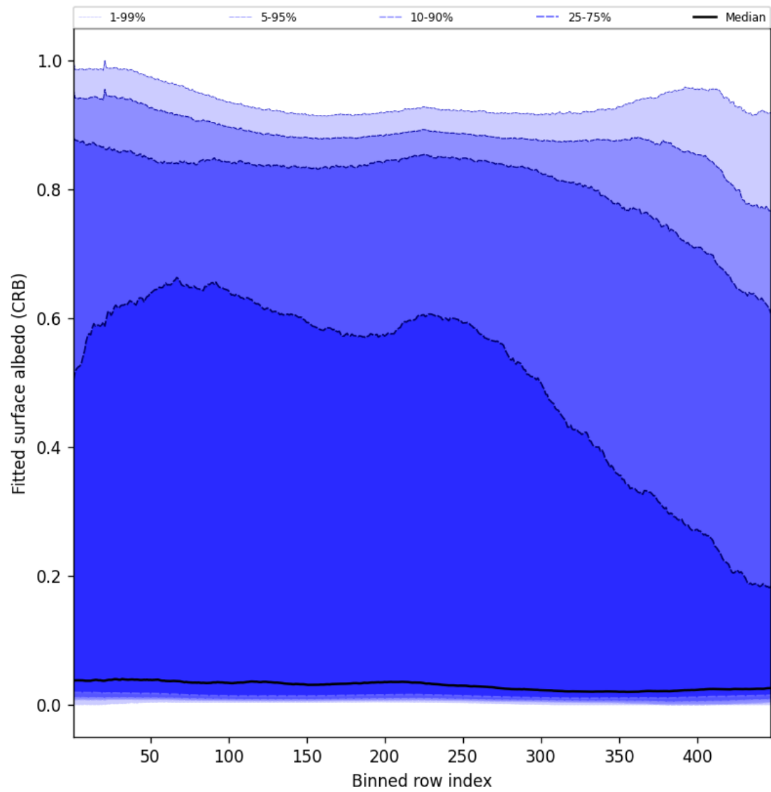
Figure 62: Along track statistics of “Fitted surface albedo (CRB)” for 2025-02-22 to 2025-02-24
