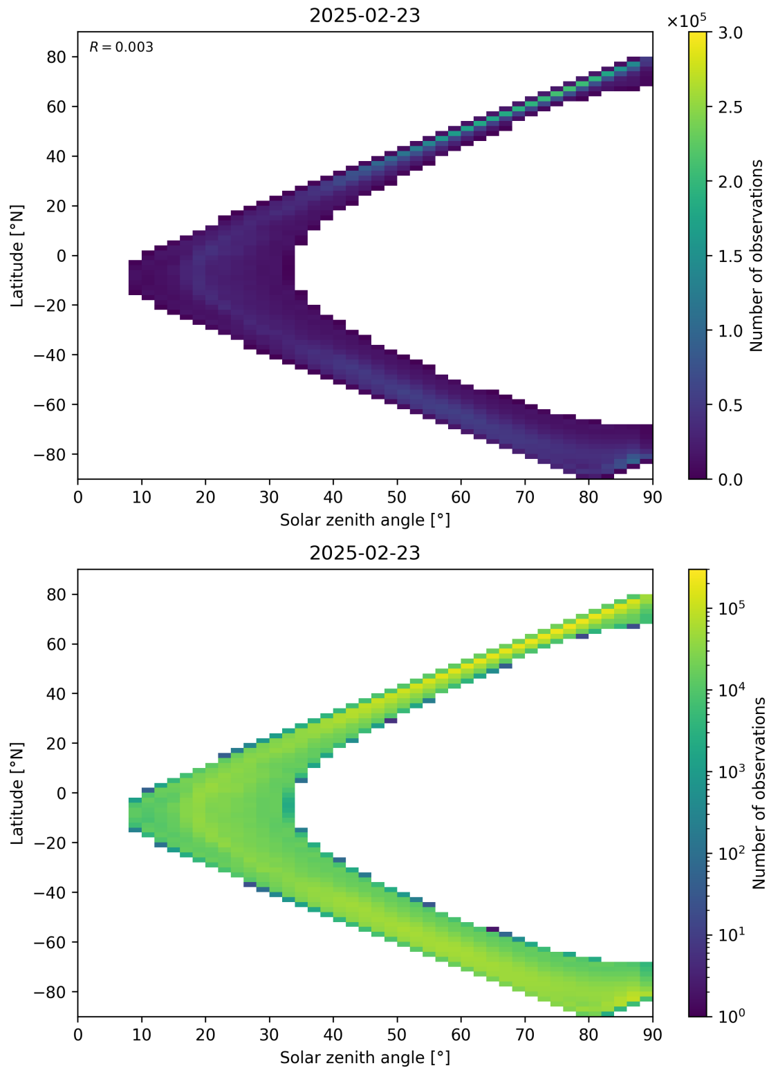
Figure 105: Scatter density plot of “Solar zenith angle” against “Latitude” for 2025-02-22 to 2025-02-24.
