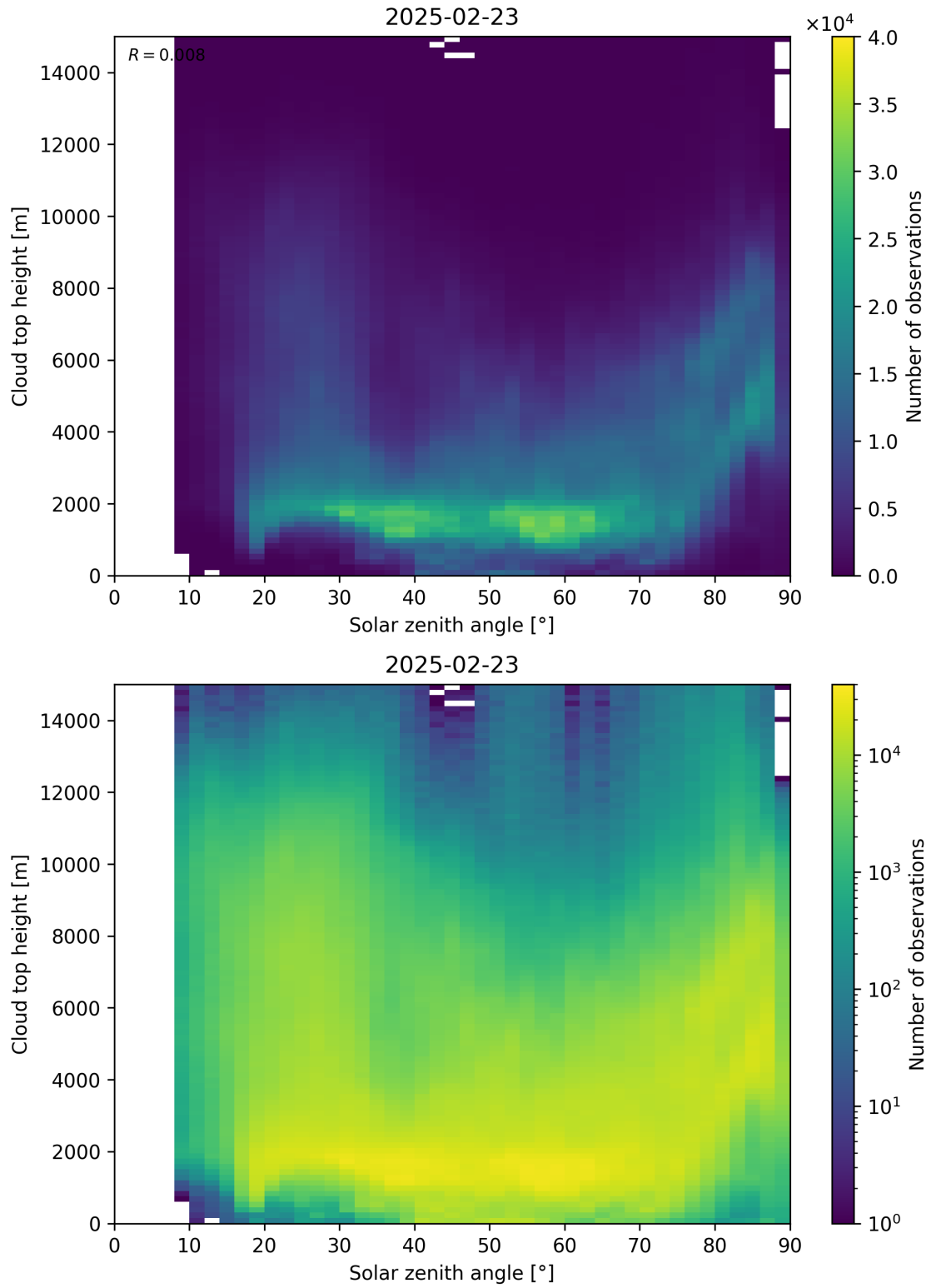
Figure 104: Scatter density plot of “Solar zenith angle” against “Cloud top height” for 2025-02-22 to 2025-02-24.
