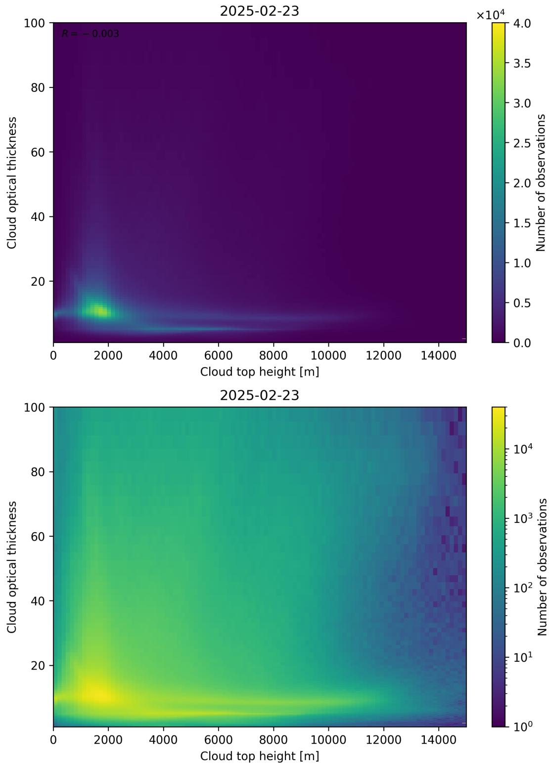
Figure 90: Scatter density plot of “Cloud top height” against “Cloud optical thickness” for 2025-02-22 to 2025-02-24.
