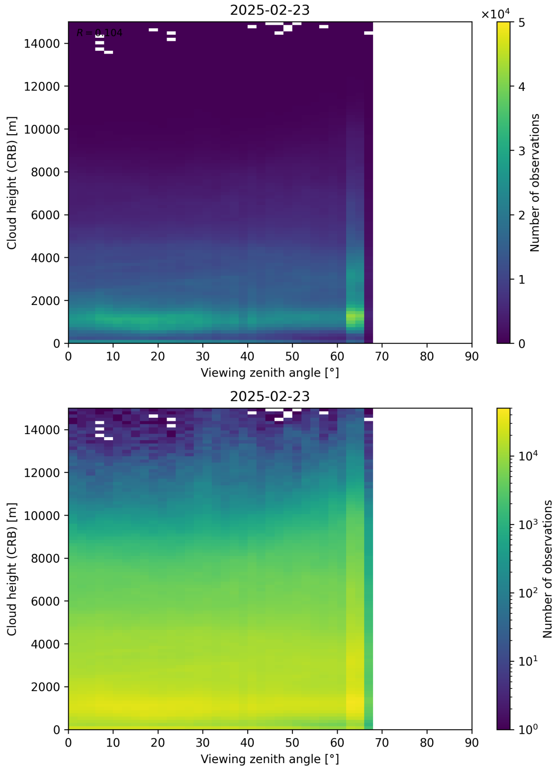
Figure 110: Scatter density plot of “Viewing zenith angle” against “Cloud height (CRB)” for 2025-02-22 to 2025-02-24.
