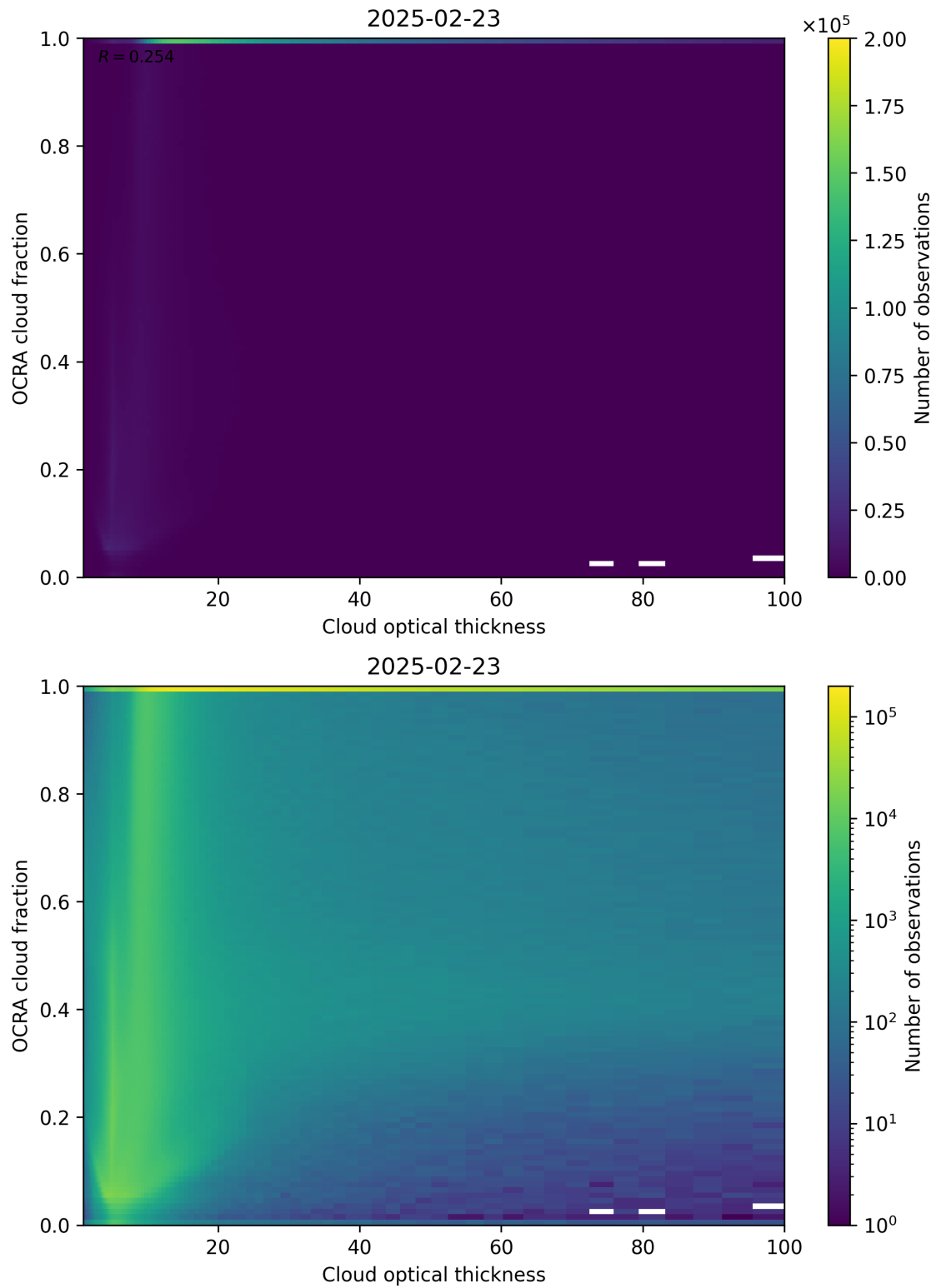
Figure 83: Scatter density plot of “Cloud optical thickness” against “OCRA cloud fraction” for 2025-02-22 to 2025-02-24.
