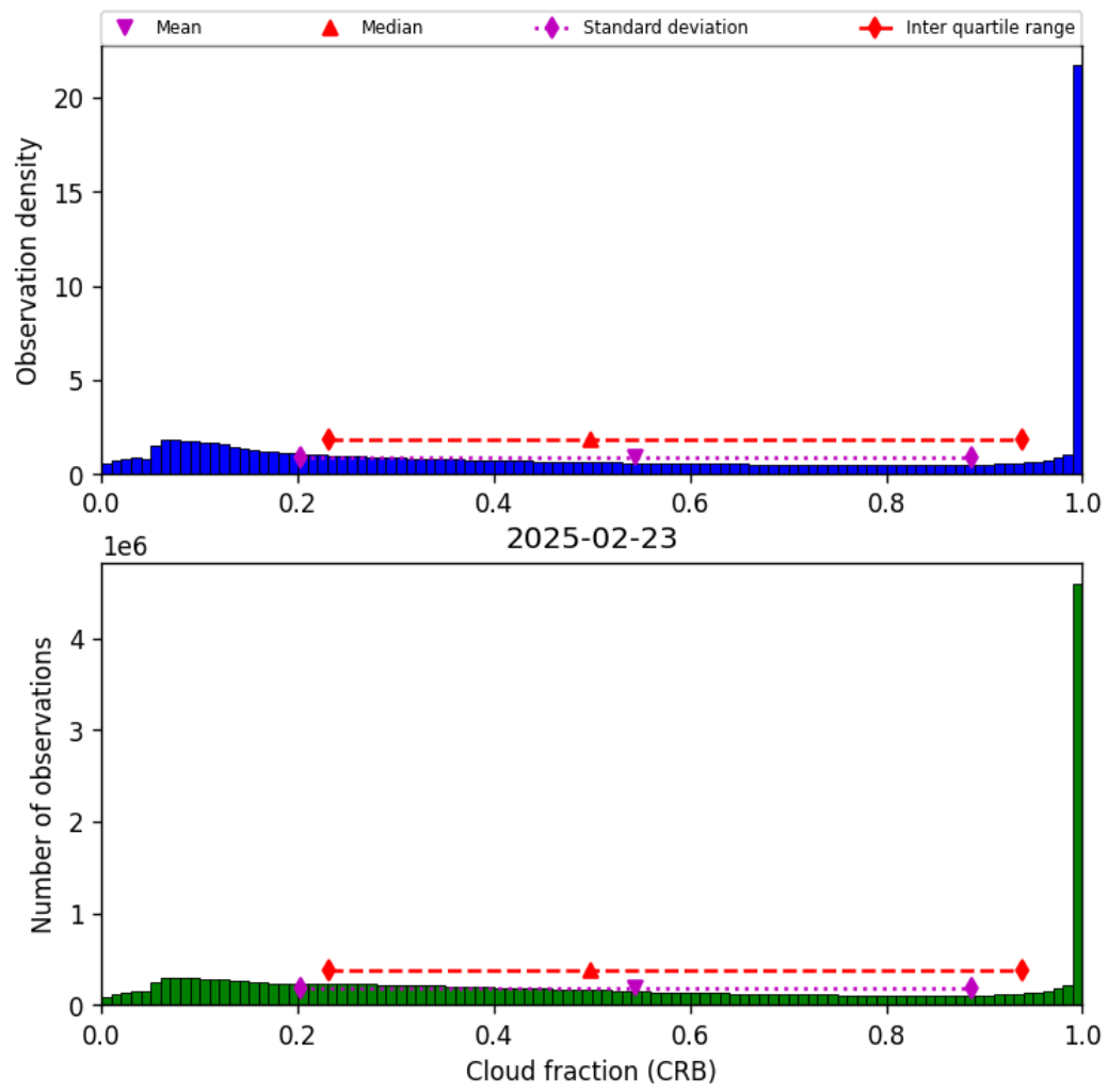
Figure 42: Histogram of “Cloud fraction (CRB)” for 2025-02-22 to 2025-02-24
