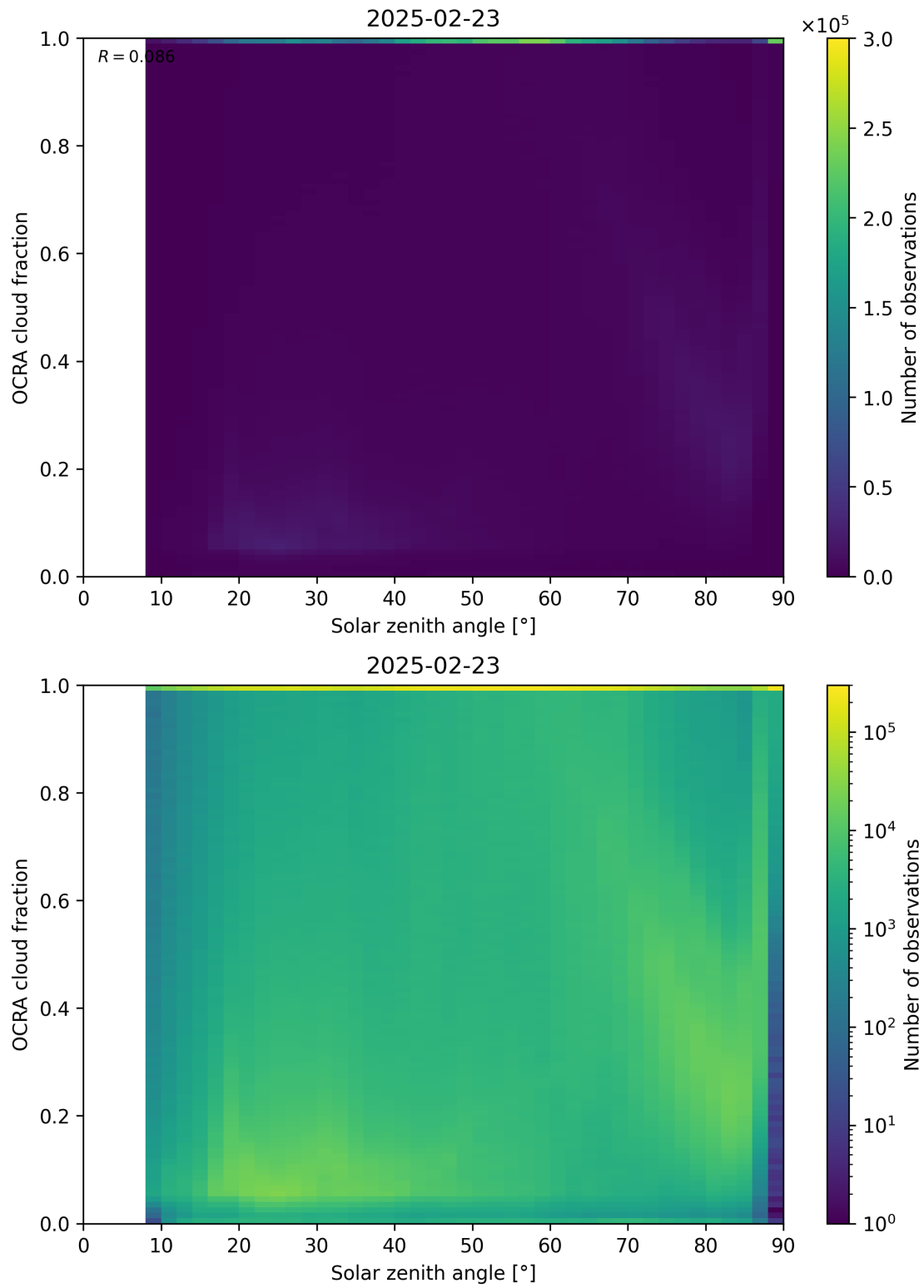
Figure 100: Scatter density plot of “Solar zenith angle” against “OCRA cloud fraction” for 2025-02-22 to 2025-02-24.
