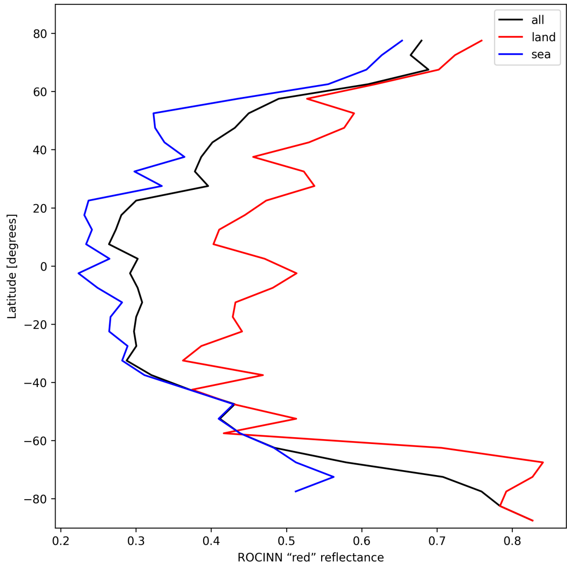
Figure 37: Zonal average of “ROCINN “red” reflectance” for 2025-02-22 to 2025-02-24.
