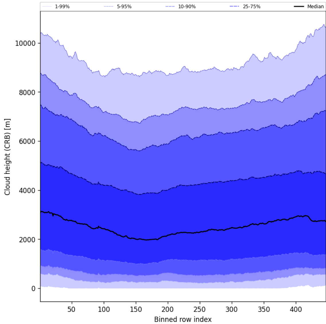
Figure 59: Along track statistics of “Cloud height (CRB)” for 2025-02-22 to 2025-02-24
