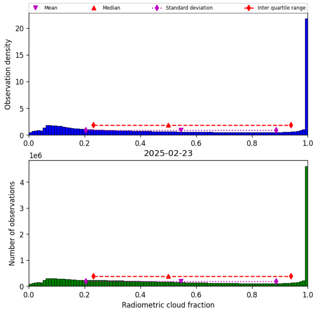
Figure 39: Histogram of “Radiometric cloud fraction” for 2025-02-22 to 2025-02-24
