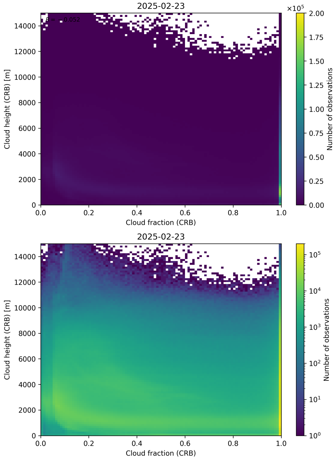
Figure 79: Scatter density plot of “Cloud fraction (CRB)” against “Cloud height (CRB)” for 2025-02-22 to 2025-02-24.
