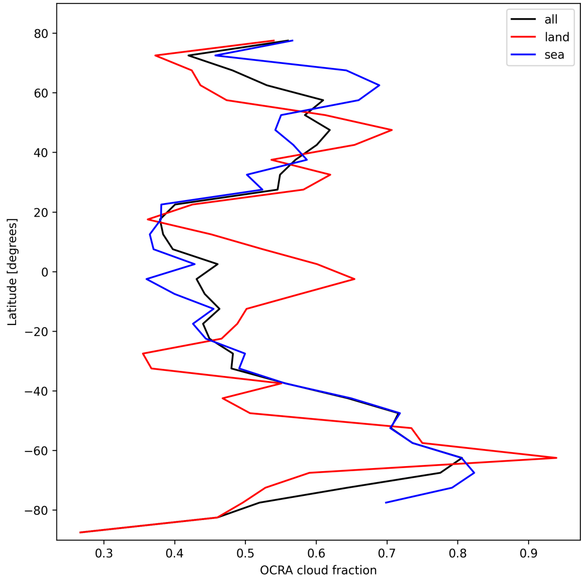
Figure 34: Zonal average of “OCRA cloud fraction” for 2025-02-22 to 2025-02-24.
