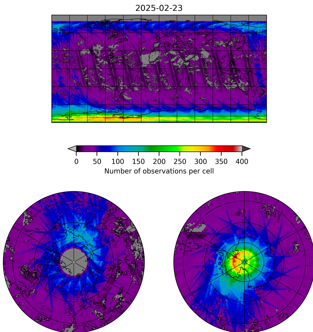
Figure 21: Map of the number of observations for 2025-02-22 to 2025-02-24
