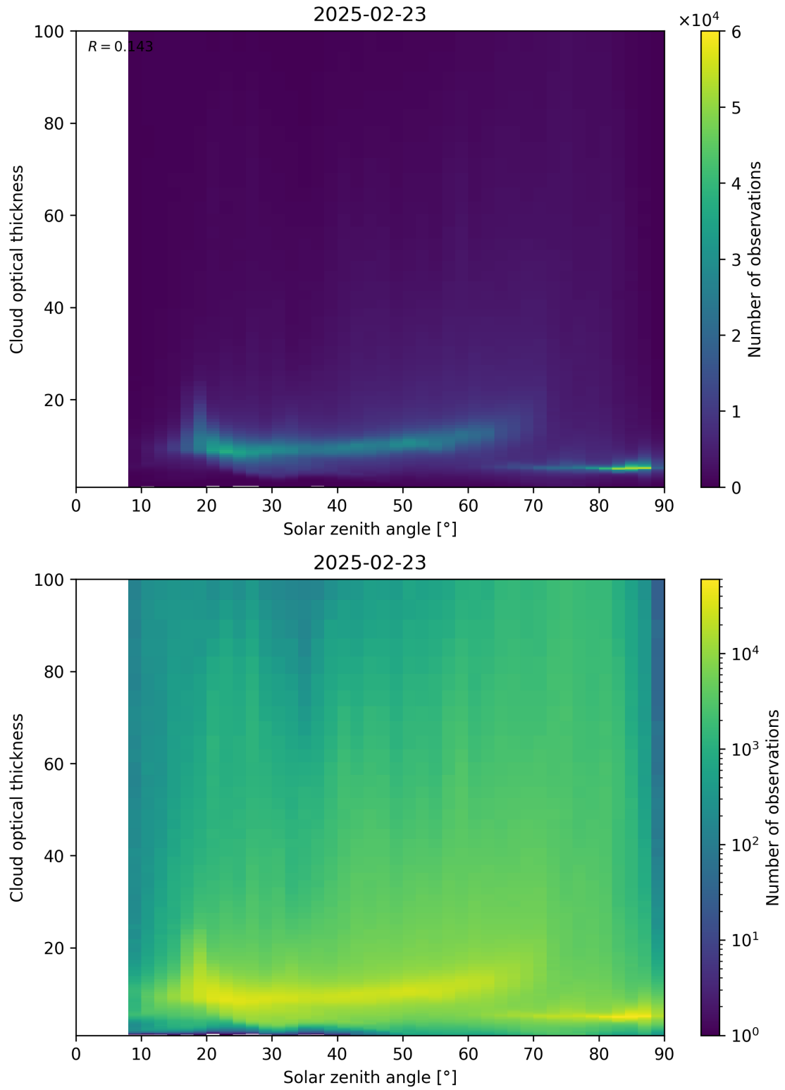
Figure 103: Scatter density plot of “Solar zenith angle” against “Cloud optical thickness” for 2025-02-22 to 2025-02-24.
