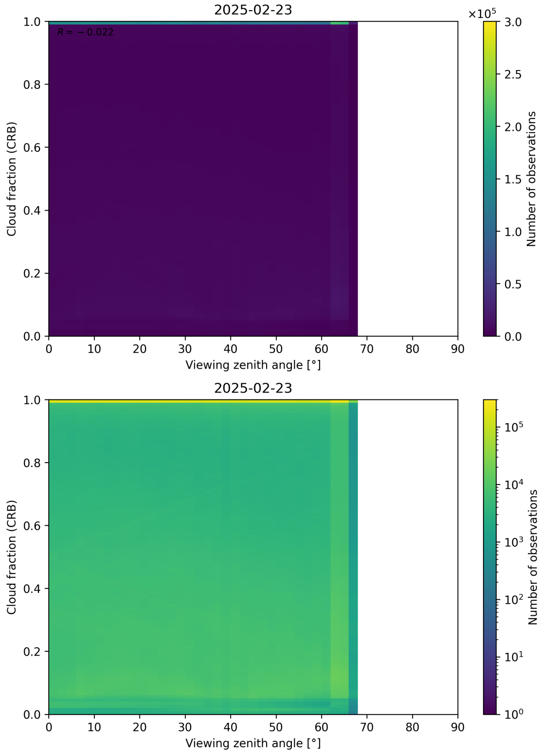
Figure 109: Scatter density plot of “Viewing zenith angle” against “Cloud fraction (CRB)” for 2025-02-22 to 2025-02-24.
