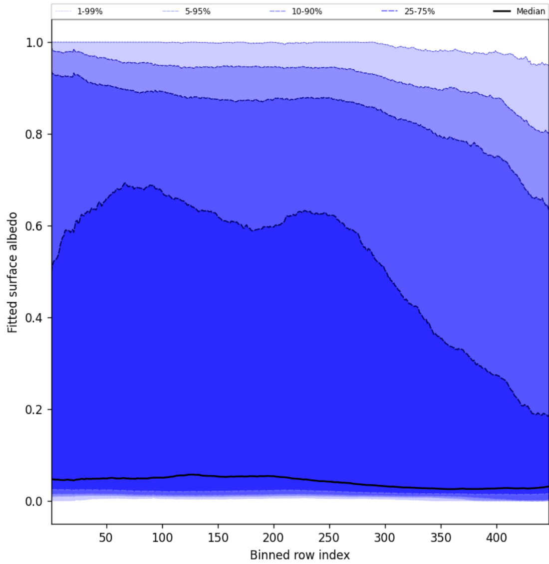
Figure 61: Along track statistics of “Fitted surface albedo” for 2025-02-22 to 2025-02-24
