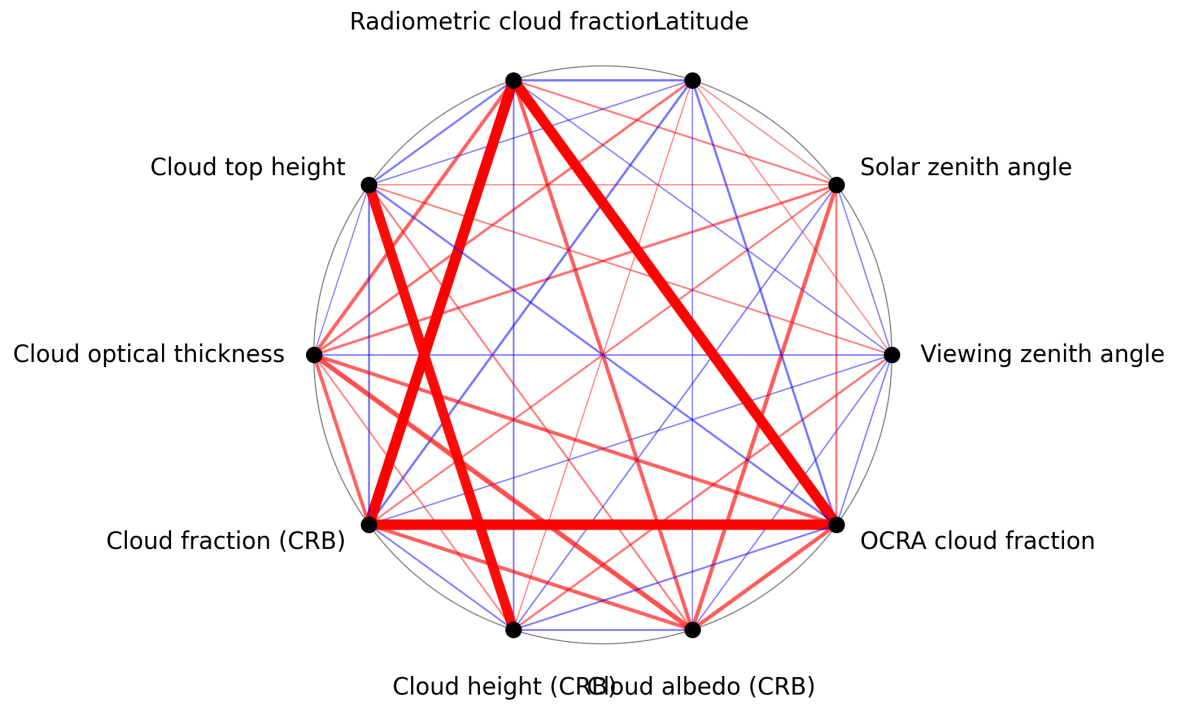
Figure 1: Map of correlation graph for 2025-02-22 to 2025-02-24.
