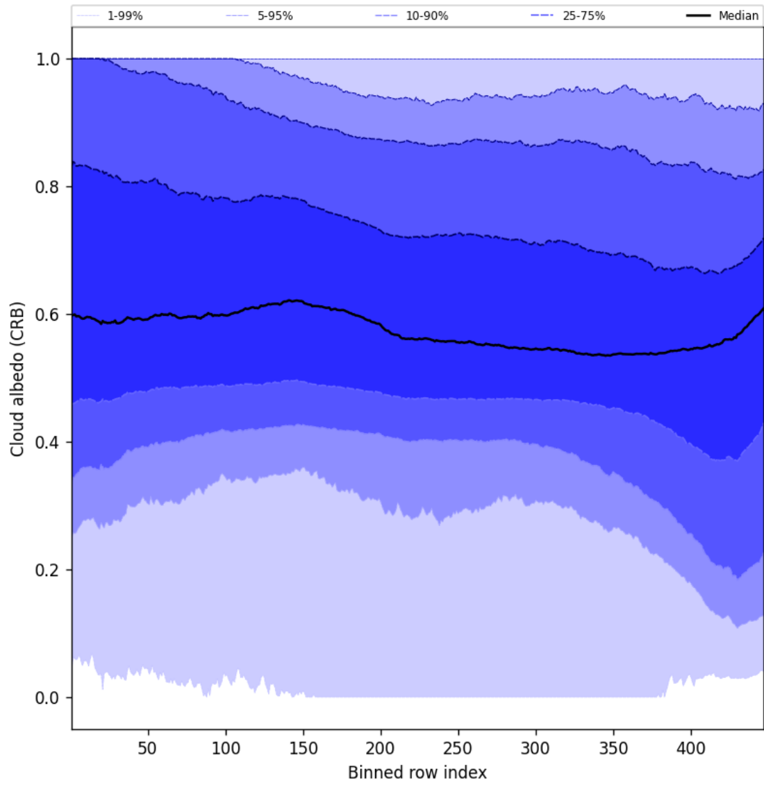
Figure 60: Along track statistics of “Cloud albedo (CRB)” for 2025-02-22 to 2025-02-24
