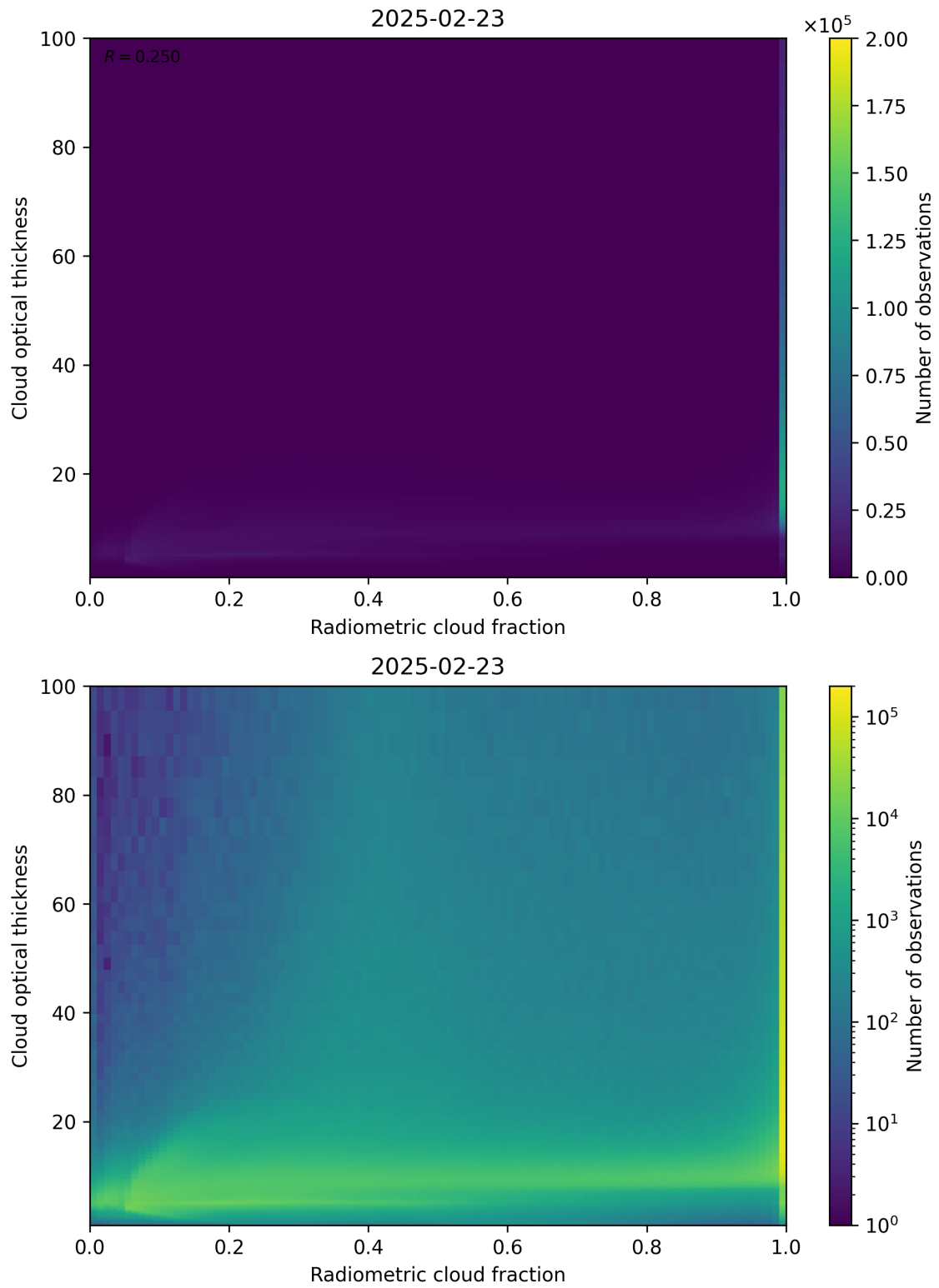
Figure 75: Scatter density plot of “Radiometric cloud fraction” against “Cloud optical thickness” for 2025-02-22 to 2025-02-24.
