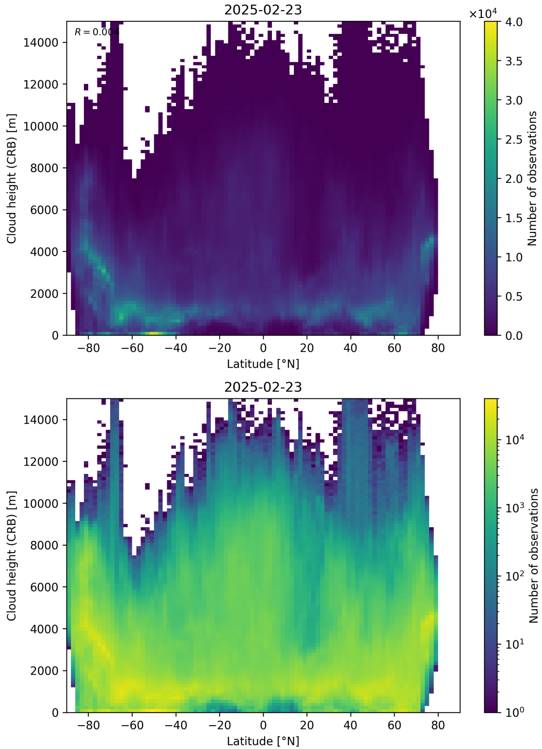
Figure 95: Scatter density plot of “Latitude” against “Cloud height (CRB)” for 2025-02-22 to 2025-02-24.
