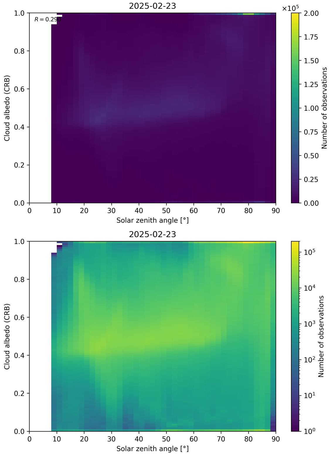
Figure 98: Scatter density plot of “Solar zenith angle” against “Cloud albedo (CRB)” for 2025-02-22 to 2025-02-24.
