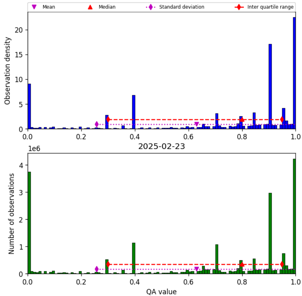
Figure 38: Histogram of “QA value” for 2025-02-22 to 2025-02-24
