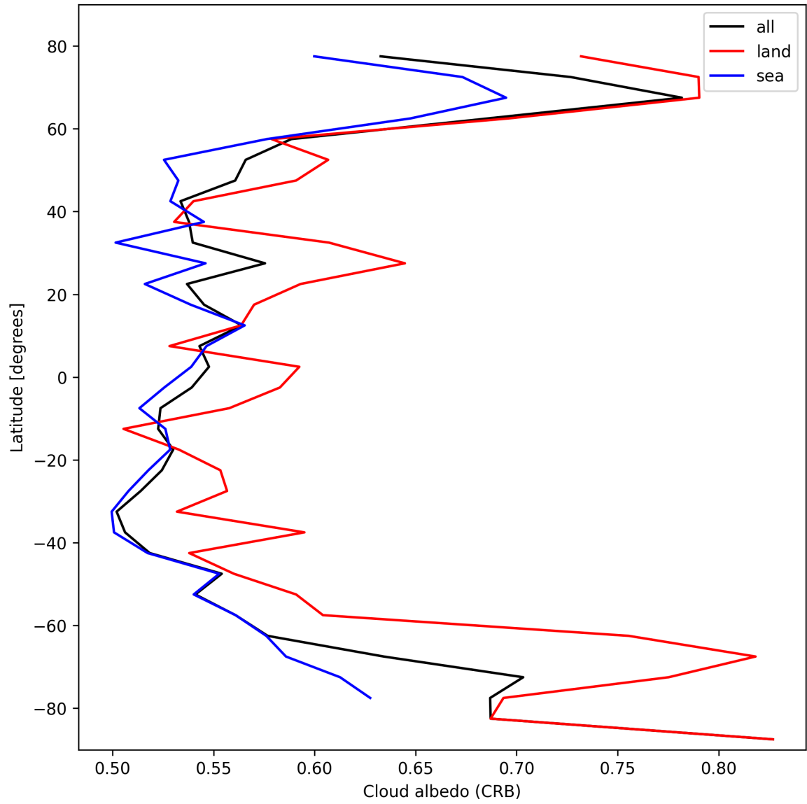
Figure 28: Zonal average of “Cloud albedo (CRB)” for 2025-02-22 to 2025-02-24.
