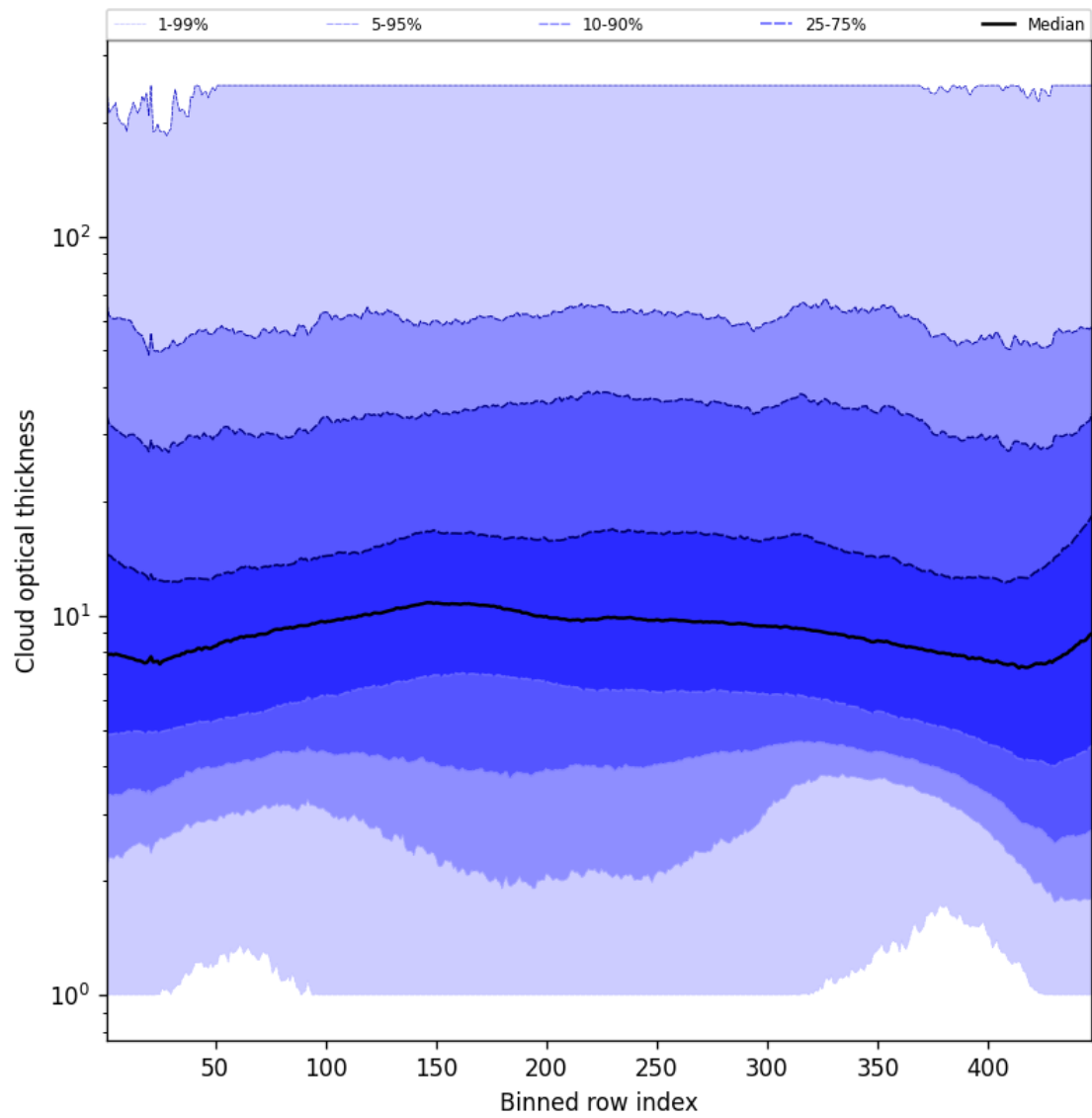
Figure 57: Along track statistics of “Cloud optical thickness” for 2025-02-22 to 2025-02-24
