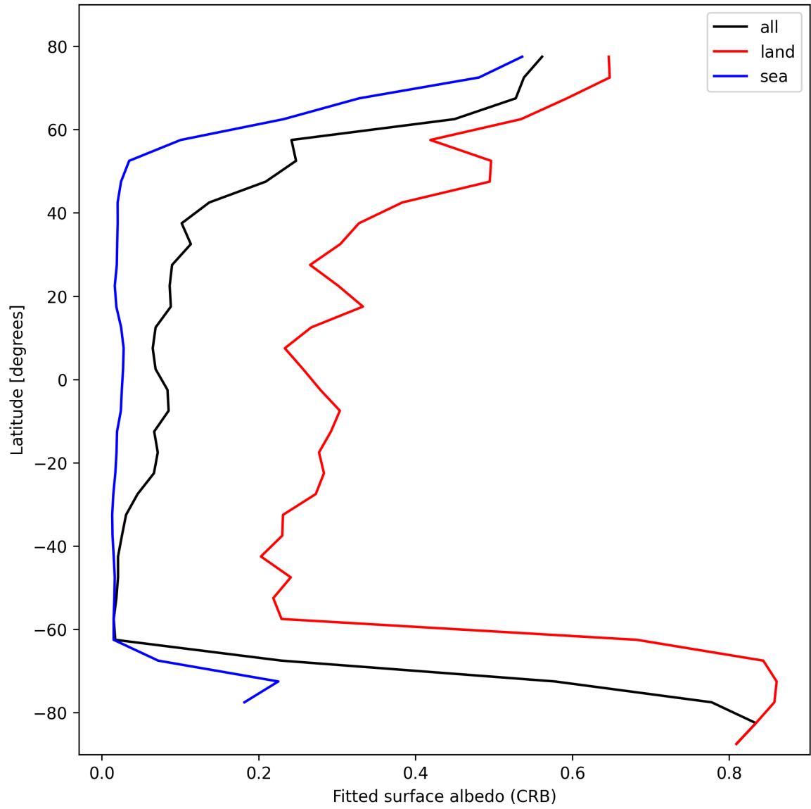
Figure 30: Zonal average of “Fitted surface albedo (CRB)” for 2025-02-22 to 2025-02-24.
