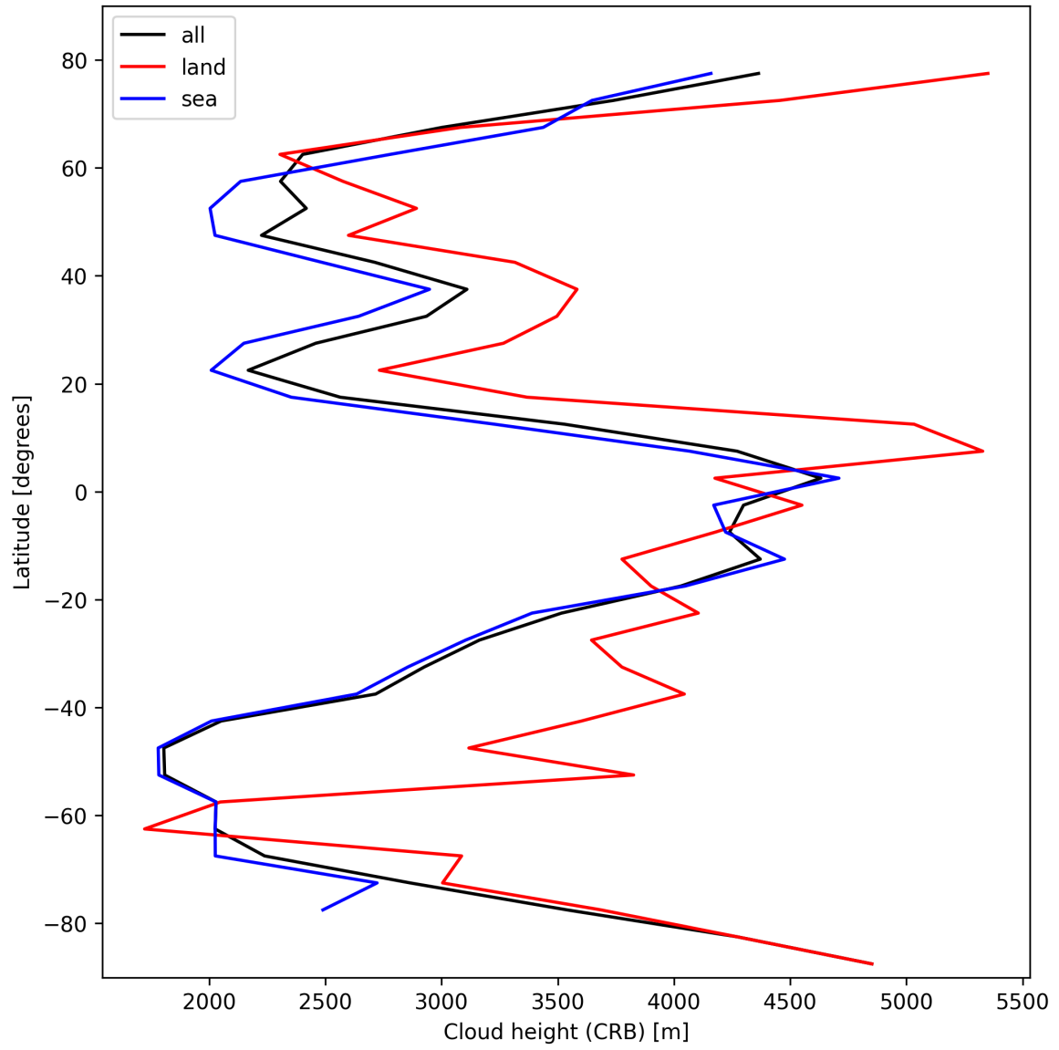
Figure 27: Zonal average of “Cloud height (CRB)” for 2025-02-22 to 2025-02-24.
