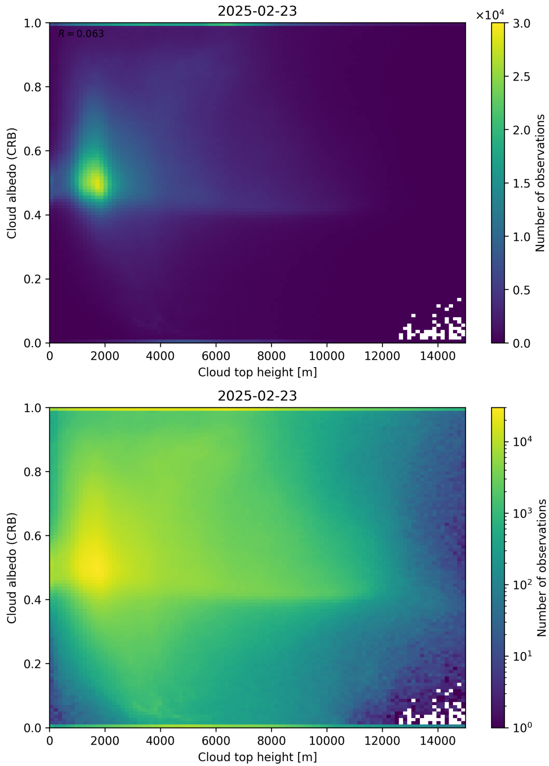
Figure 86: Scatter density plot of “Cloud top height” against “Cloud albedo (CRB)” for 2025-02-22 to 2025-02-24.
