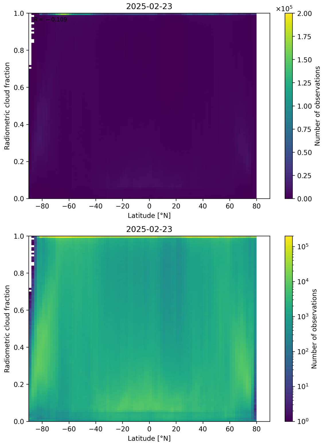
Figure 92: Scatter density plot of “Latitude” against “Radiometric cloud fraction” for 2025-02-22 to 2025-02-24.
