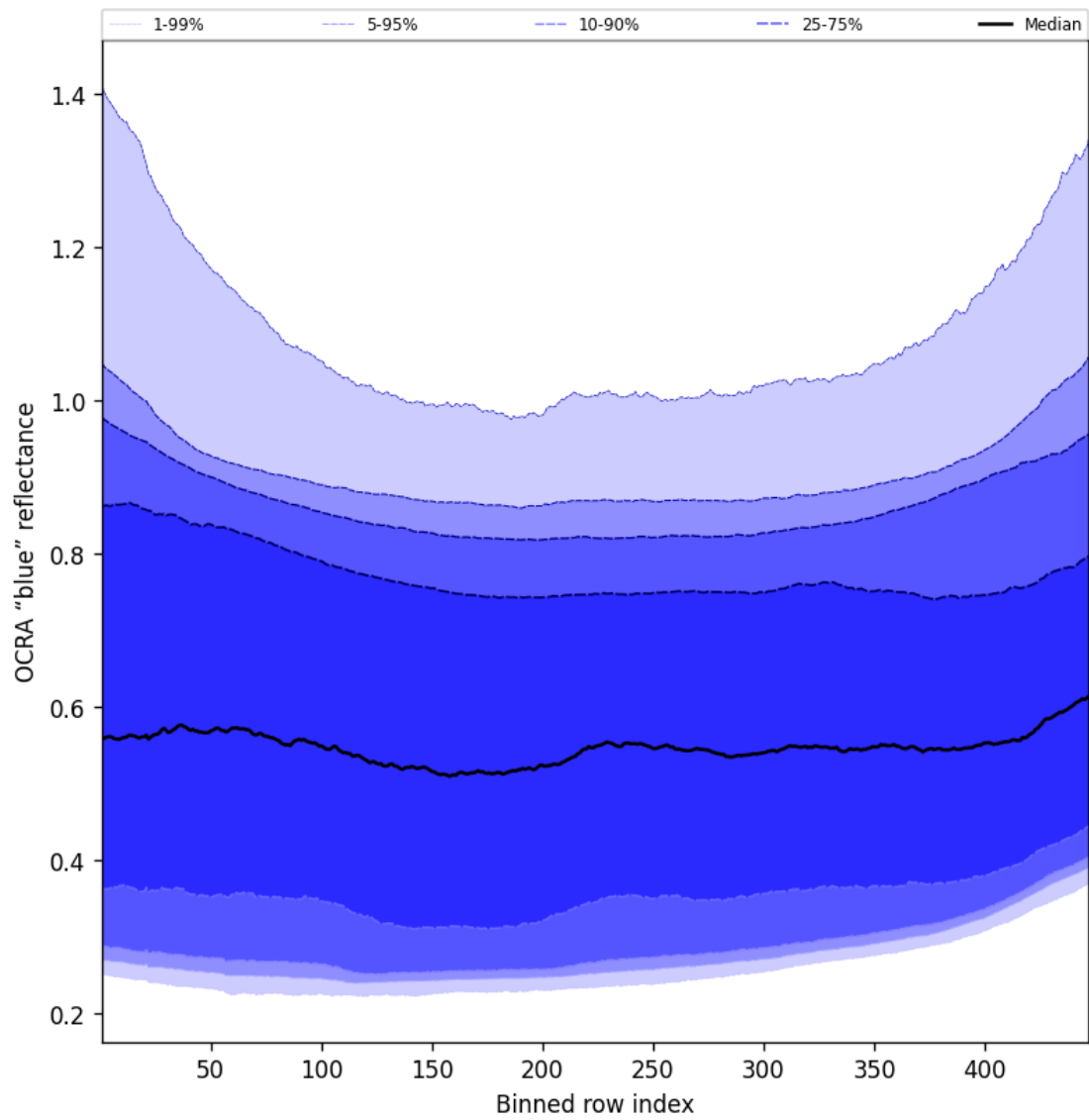
Figure 67: Along track statistics of “OCRA “blue” reflectance” for 2025-02-22 to 2025-02-24
