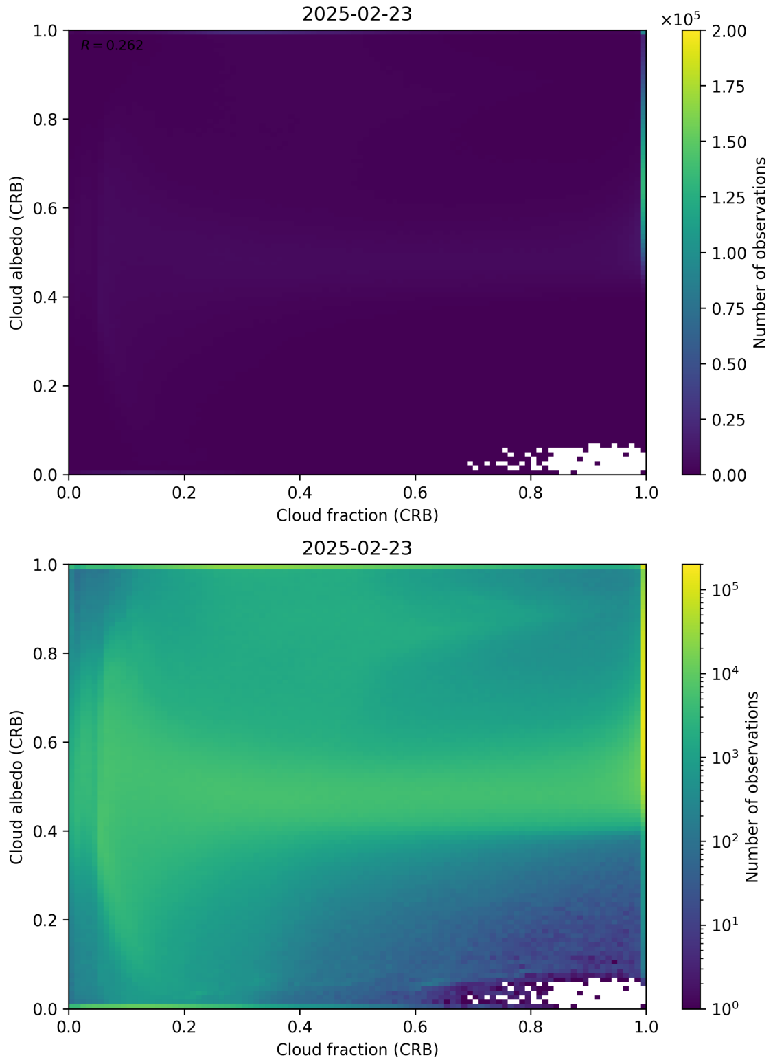
Figure 77: Scatter density plot of “Cloud fraction (CRB)” against “Cloud albedo (CRB)” for 2025-02-22 to 2025-02-24.
