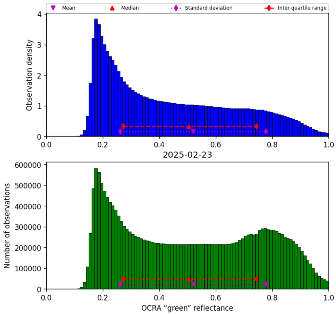
Figure 52: Histogram of “OCRA “green” reflectance” for 2025-02-22 to 2025-02-24
