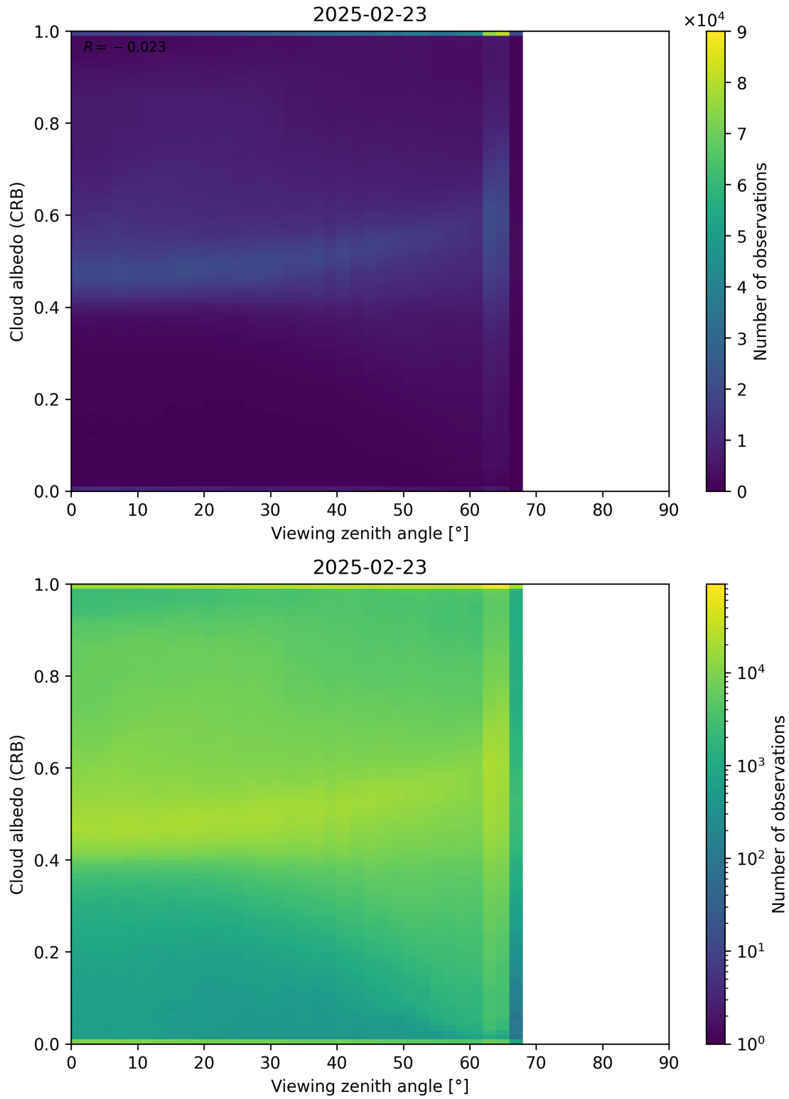
Figure 106: Scatter density plot of “Viewing zenith angle” against “Cloud albedo (CRB)” for 2025-02-22 to 2025-02-24.
