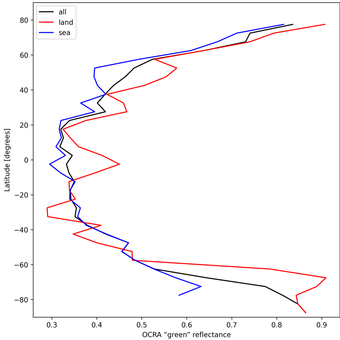
Figure 36: Zonal average of “OCRA “green” reflectance” for 2025-02-22 to 2025-02-24.
