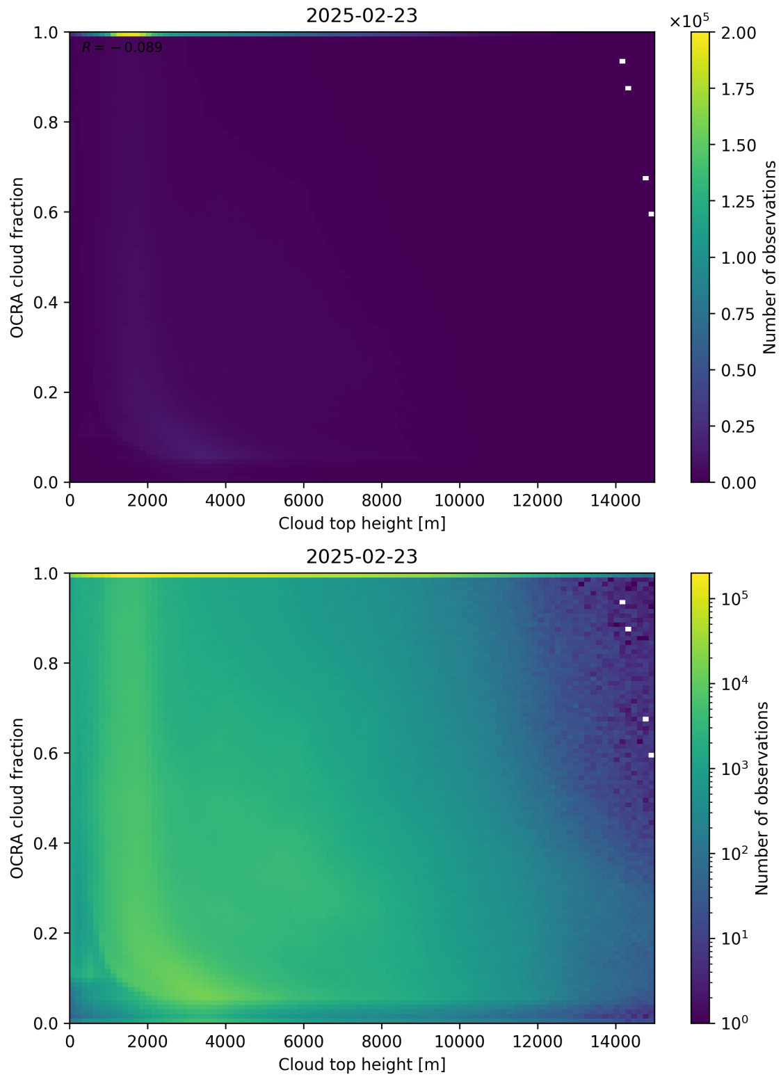
Figure 87: Scatter density plot of “Cloud top height” against “OCRA cloud fraction” for 2025-02-22 to 2025-02-24.
