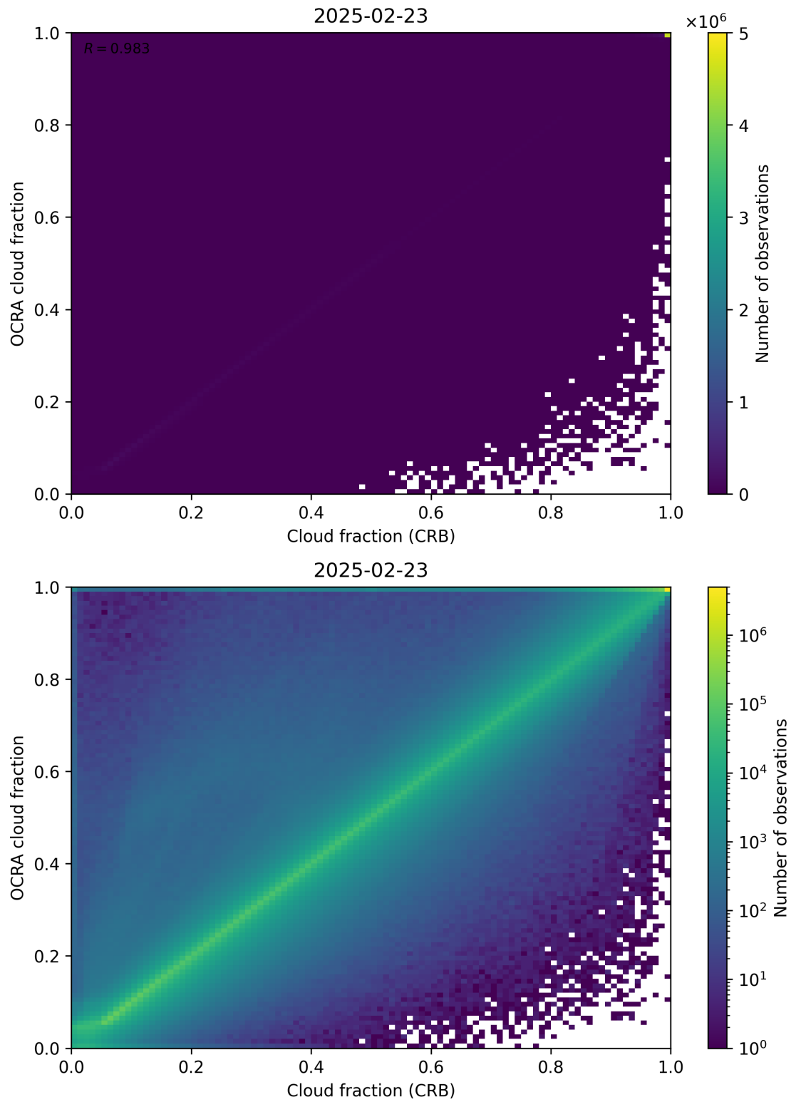
Figure 78: Scatter density plot of “Cloud fraction (CRB)” against “OCRA cloud fraction” for 2025-02-22 to 2025-02-24.
