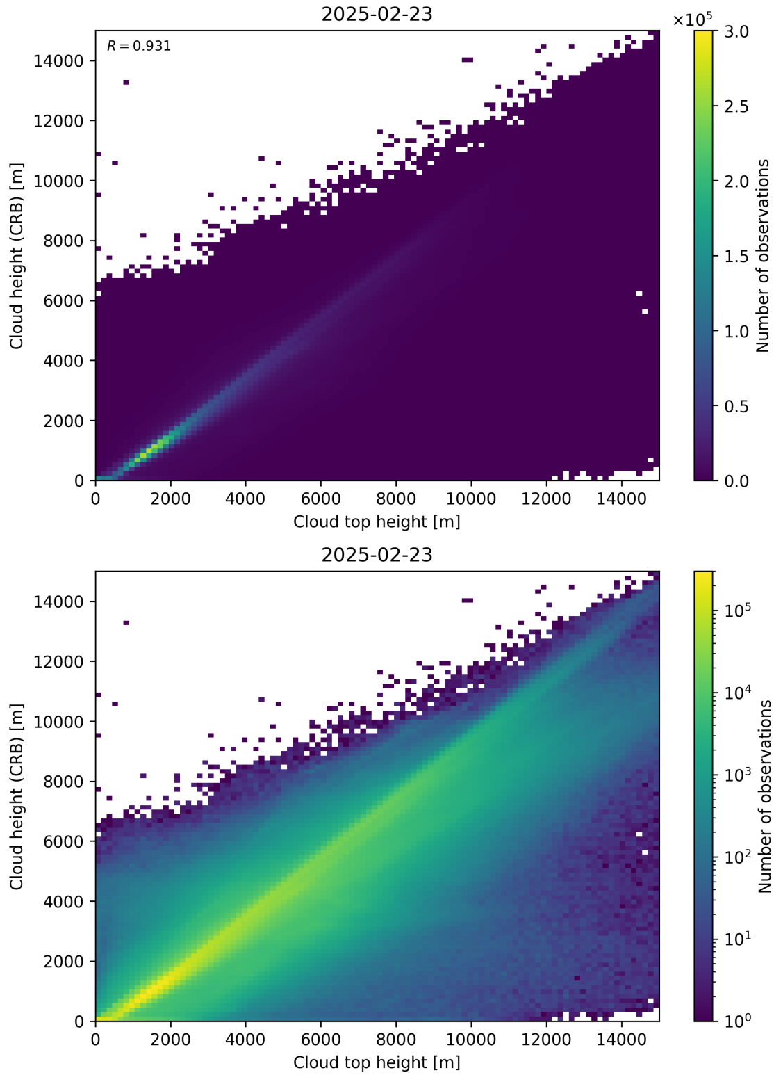
Figure 89: Scatter density plot of “Cloud top height” against “Cloud height (CRB)” for 2025-02-22 to 2025-02-24.
