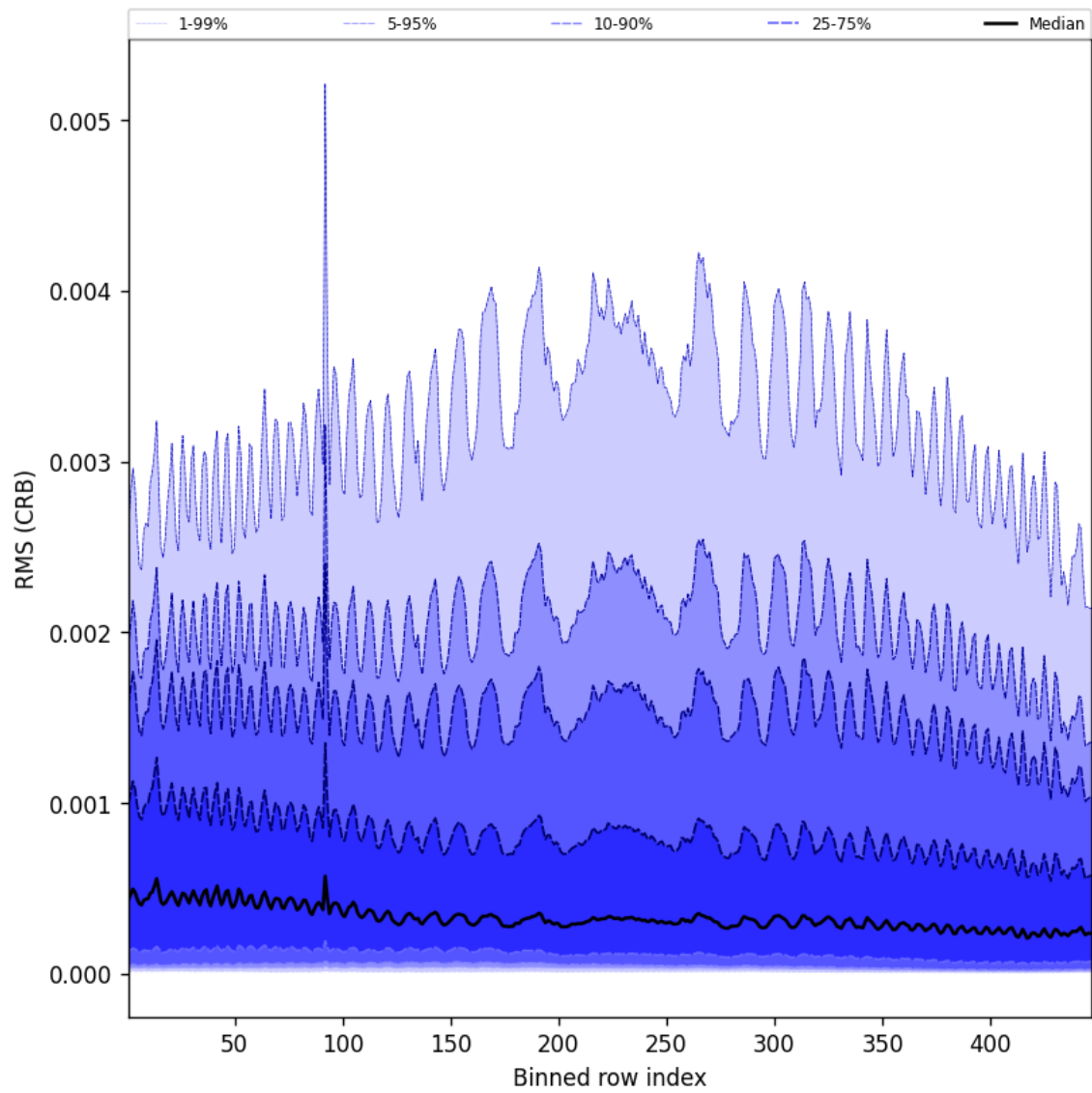
Figure 64: Along track statistics of “RMS (CRB)” for 2025-02-22 to 2025-02-24
