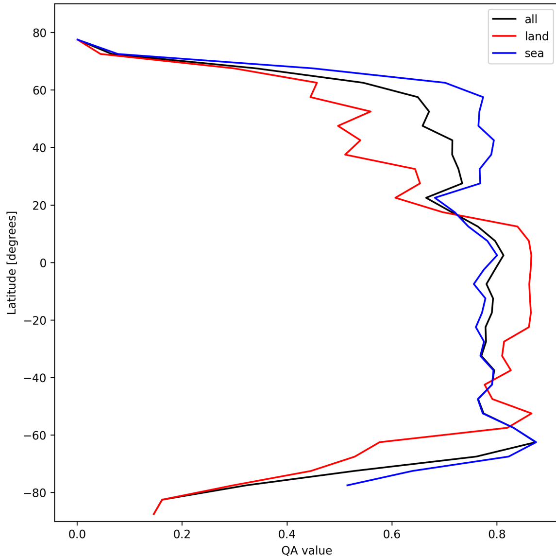
Figure 22: Zonal average of “QA value” for 2025-02-22 to 2025-02-24.
