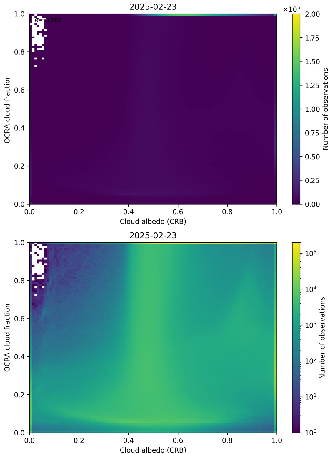
Figure 70: Scatter density plot of “Cloud albedo (CRB)” against “OCRA cloud fraction” for 2025-02-22 to 2025-02-24.
