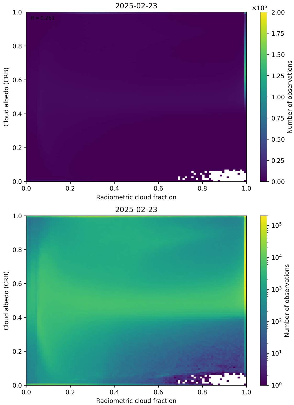
Figure 71: Scatter density plot of “Radiometric cloud fraction” against “Cloud albedo (CRB)” for 2025-02-22 to 2025-02-24.
