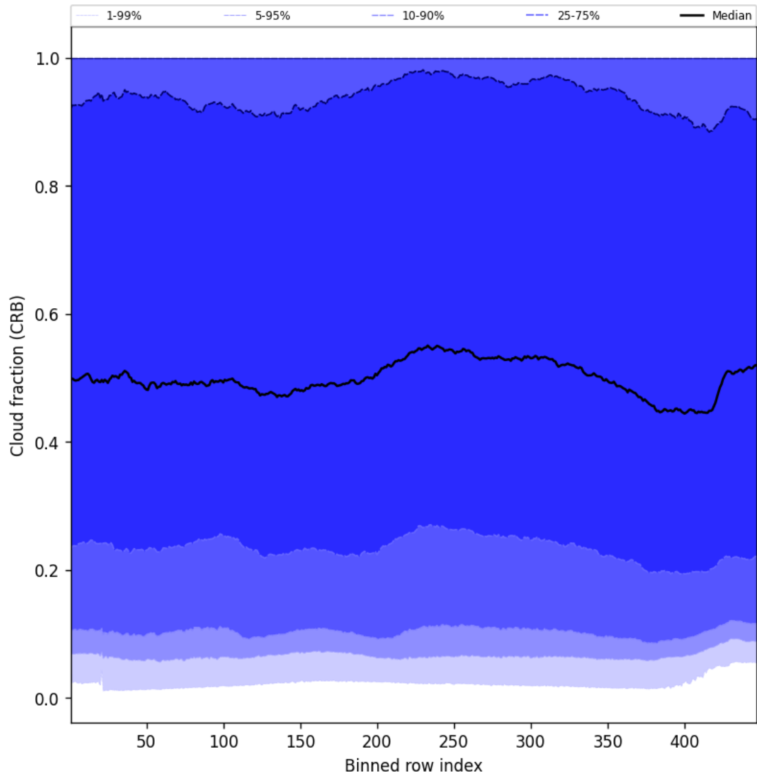
Figure 58: Along track statistics of “Cloud fraction (CRB)” for 2025-02-22 to 2025-02-24
