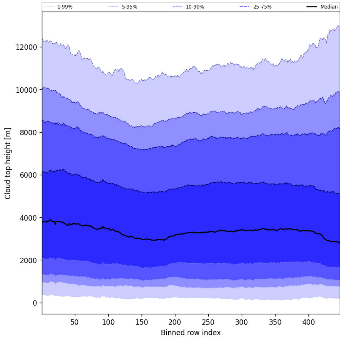
Figure 56: Along track statistics of “Cloud top height” for 2025-02-22 to 2025-02-24
