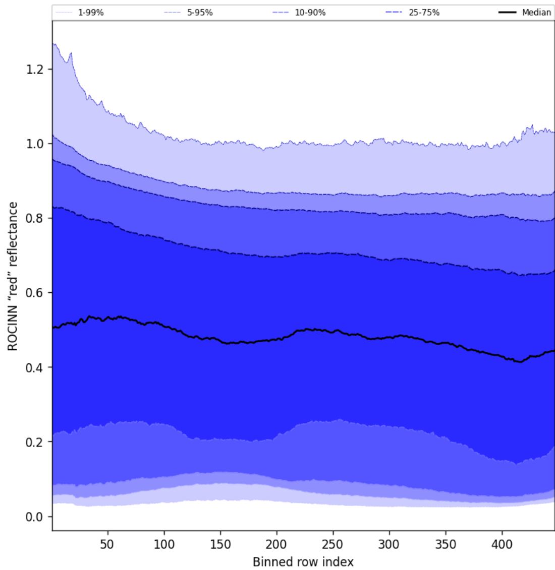
Figure 69: Along track statistics of “ROCINN “red” reflectance” for 2025-02-22 to 2025-02-24
