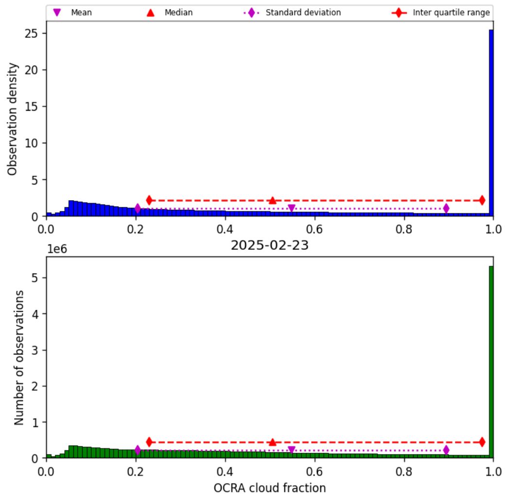
Figure 50: Histogram of “OCRA cloud fraction” for 2025-02-22 to 2025-02-24
