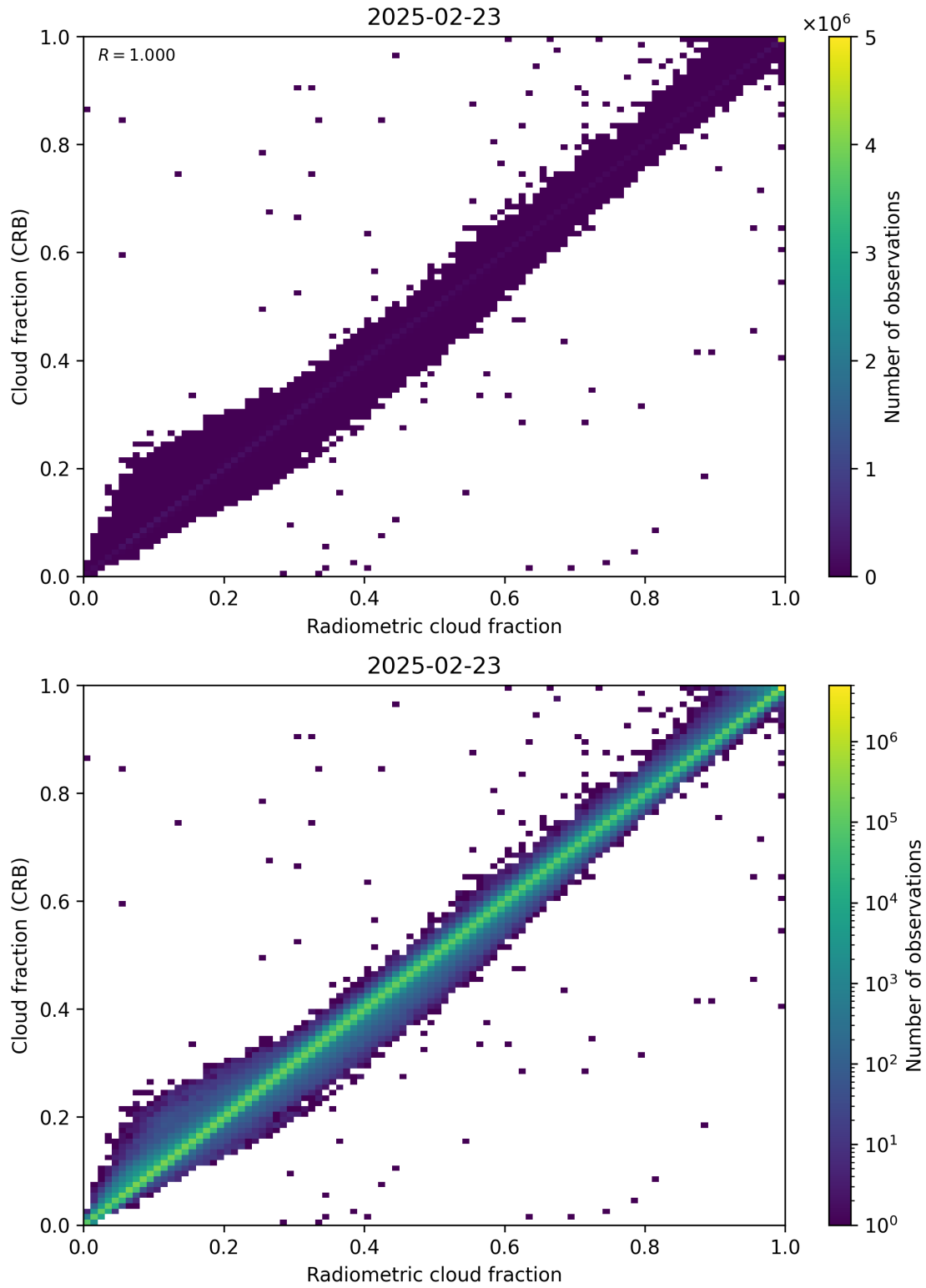
Figure 73: Scatter density plot of “Radiometric cloud fraction” against “Cloud fraction (CRB)” for 2025-02-22 to 2025-02-24.
