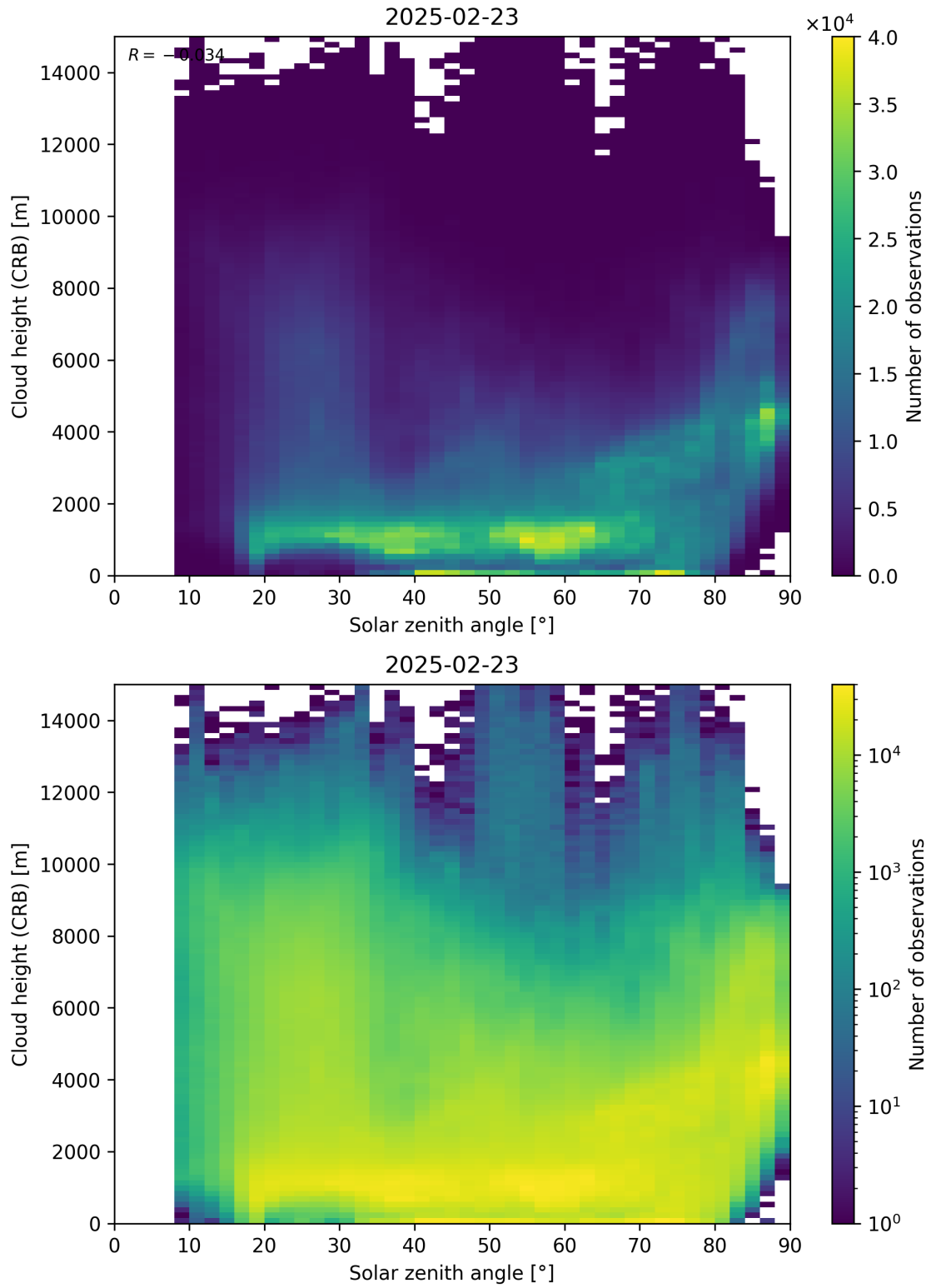
Figure 102: Scatter density plot of “Solar zenith angle” against “Cloud height (CRB)” for 2025-02-22 to 2025-02-24.
