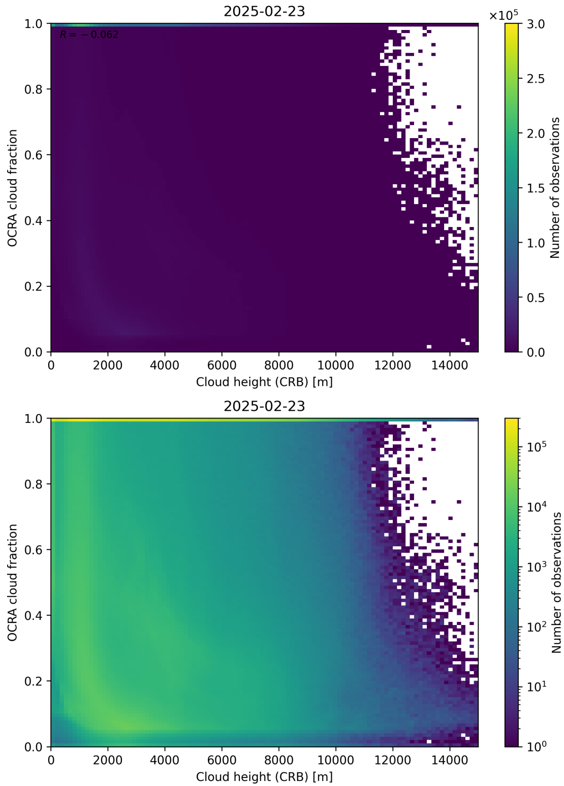
Figure 81: Scatter density plot of “Cloud height (CRB)” against “OCRA cloud fraction” for 2025-02-22 to 2025-02-24.
