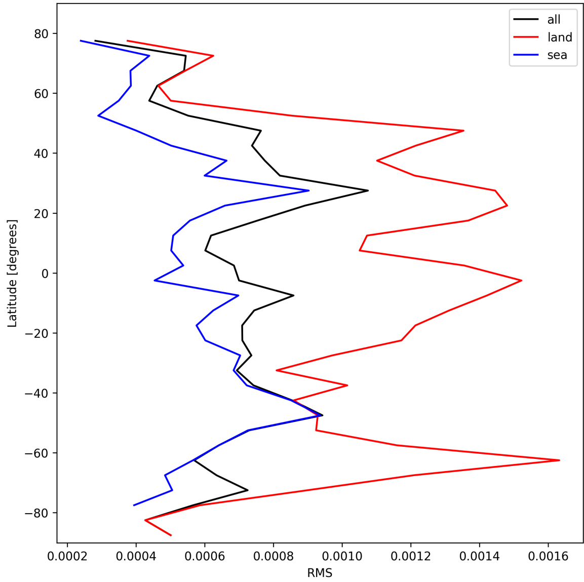
Figure 31: Zonal average of “RMS” for 2025-02-22 to 2025-02-24.
