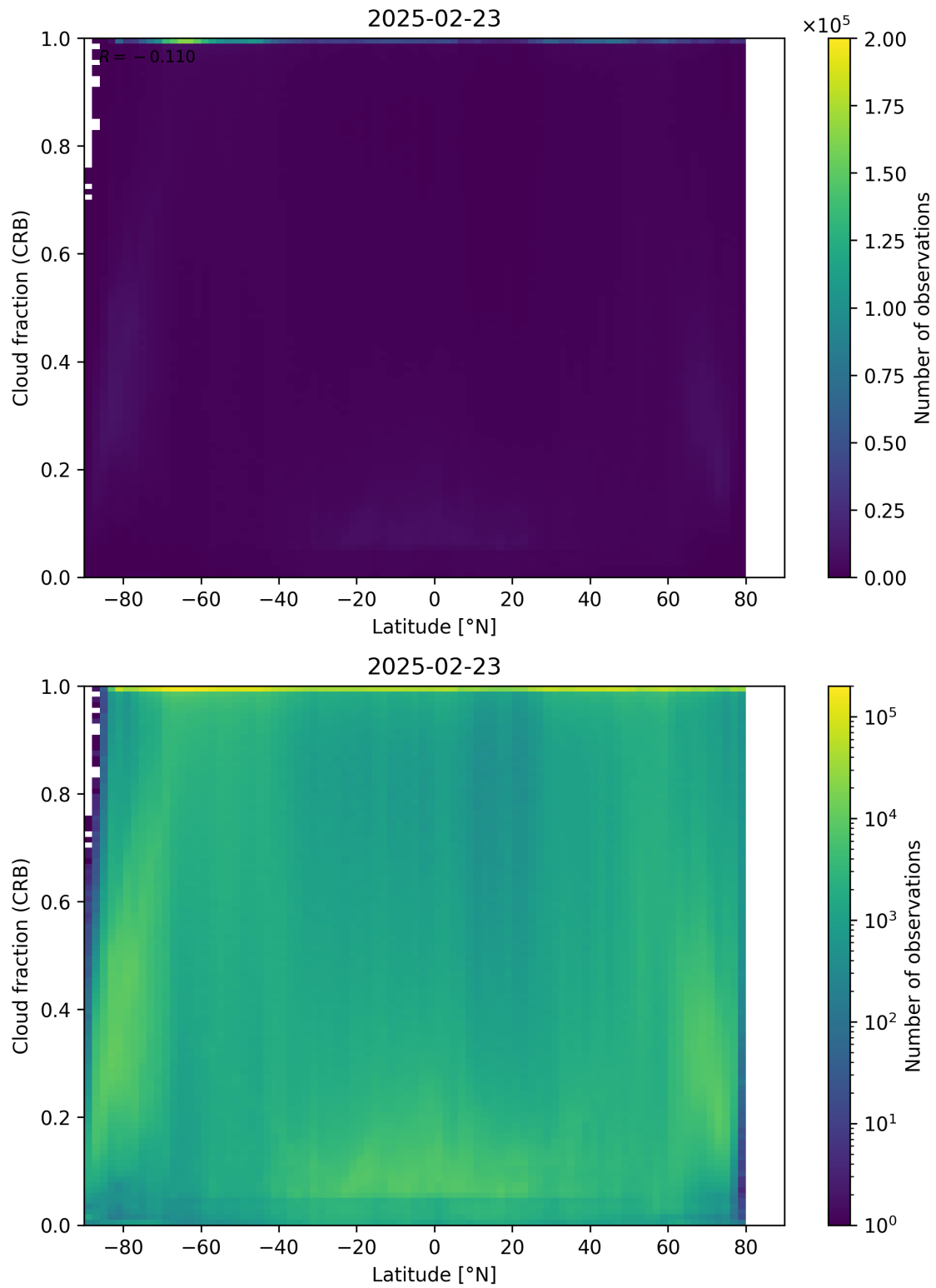
Figure 94: Scatter density plot of “Latitude” against “Cloud fraction (CRB)” for 2025-02-22 to 2025-02-24.
