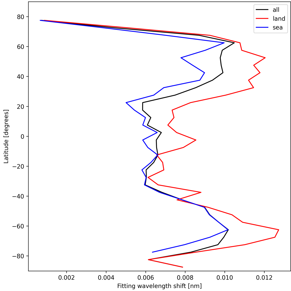
Figure 33: Zonal average of “Fitting wavelength shift” for 2025-02-22 to 2025-02-24.
