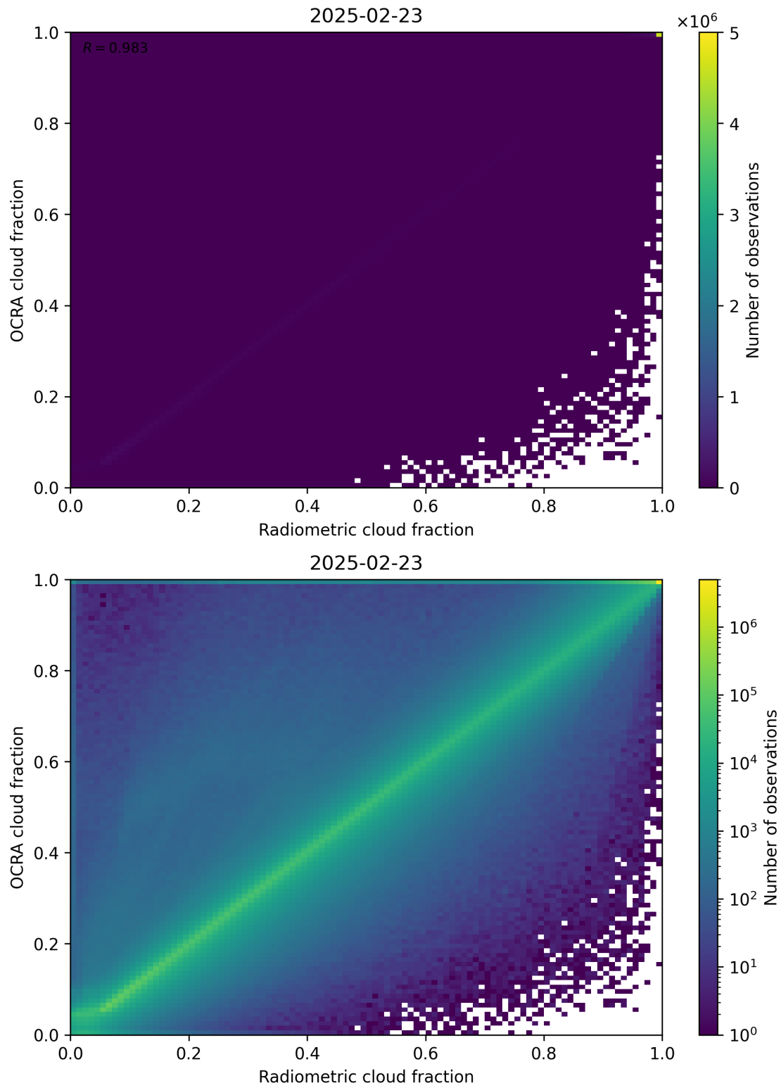
Figure 72: Scatter density plot of “Radiometric cloud fraction” against “OCRA cloud fraction” for 2025-02-22 to 2025-02-24.
