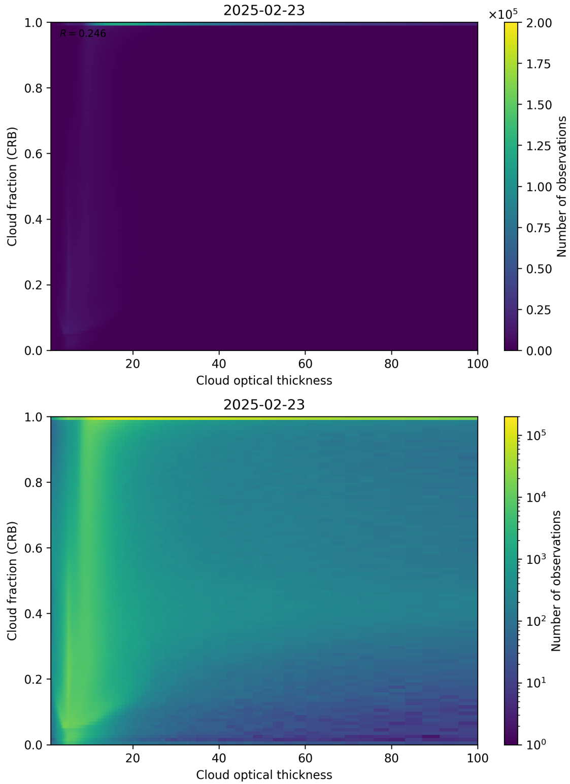
Figure 84: Scatter density plot of “Cloud optical thickness” against “Cloud fraction (CRB)” for 2025-02-22 to 2025-02-24.
