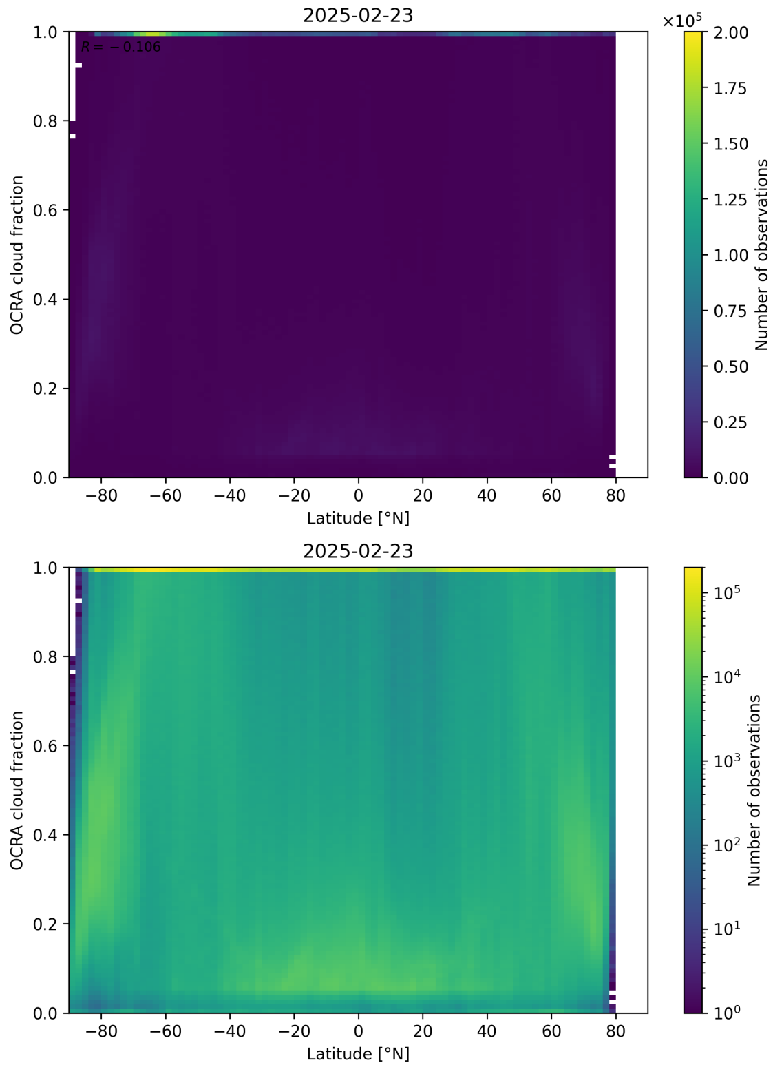
Figure 93: Scatter density plot of “Latitude” against “OCRA cloud fraction” for 2025-02-22 to 2025-02-24.
