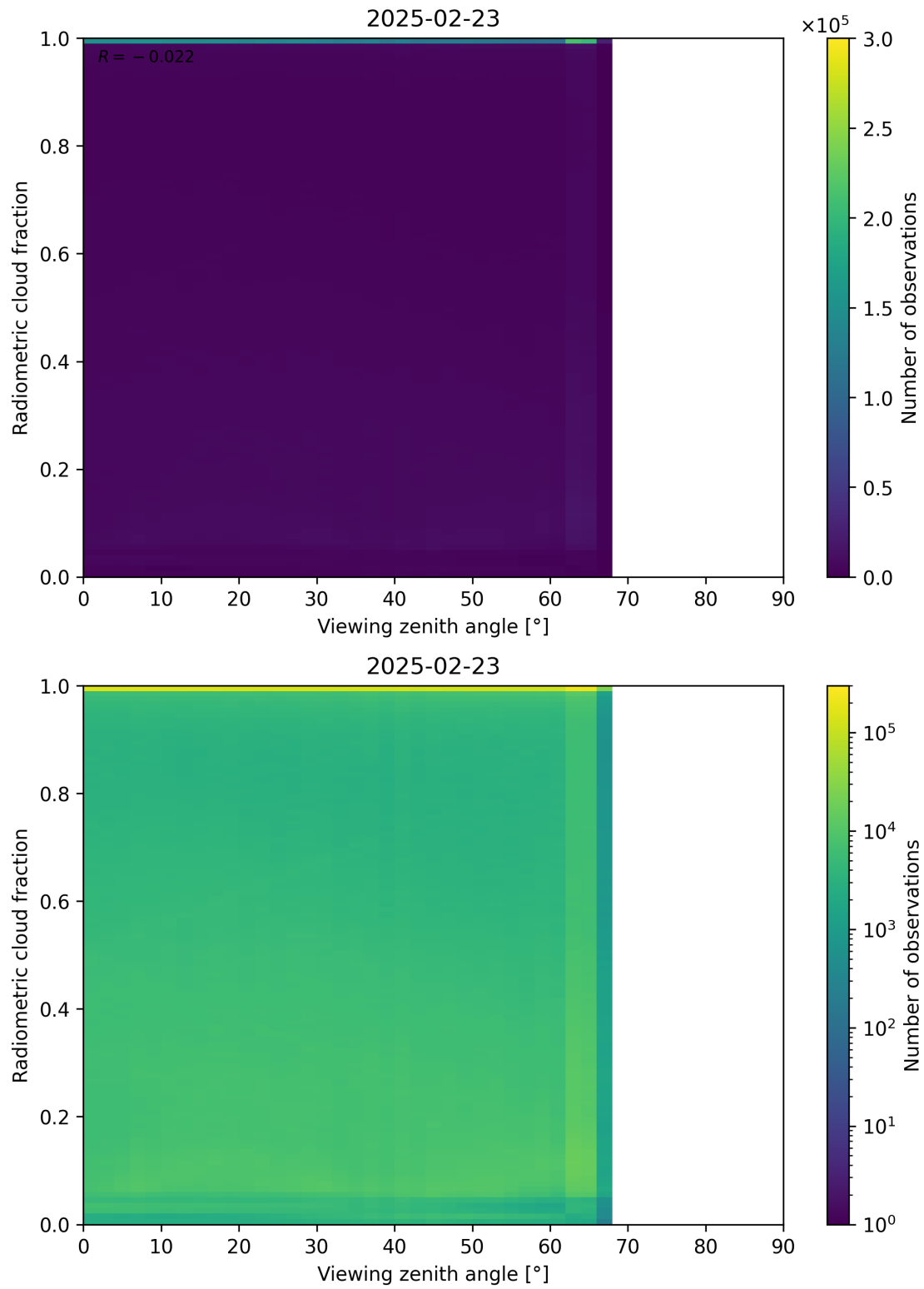
Figure 107: Scatter density plot of “Viewing zenith angle” against “Radiometric cloud fraction” for 2025-02-22 to 2025-02-24.
