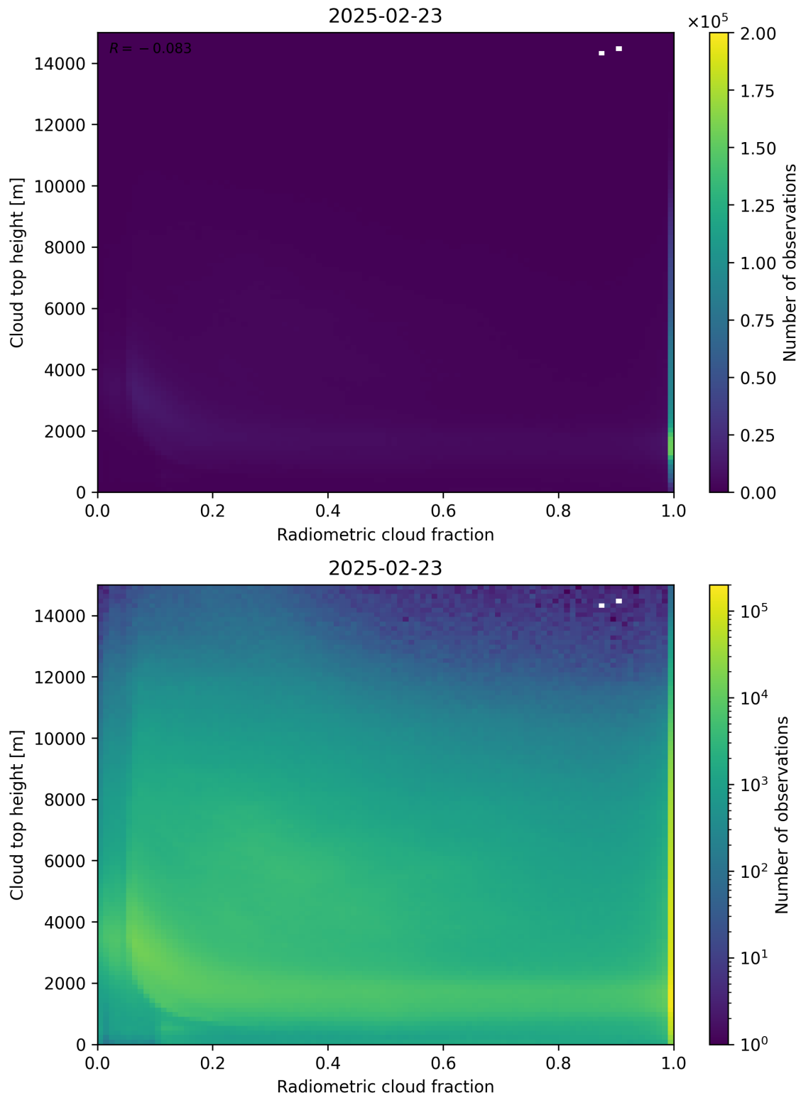
Figure 76: Scatter density plot of “Radiometric cloud fraction” against “Cloud top height” for 2025-02-22 to 2025-02-24.
