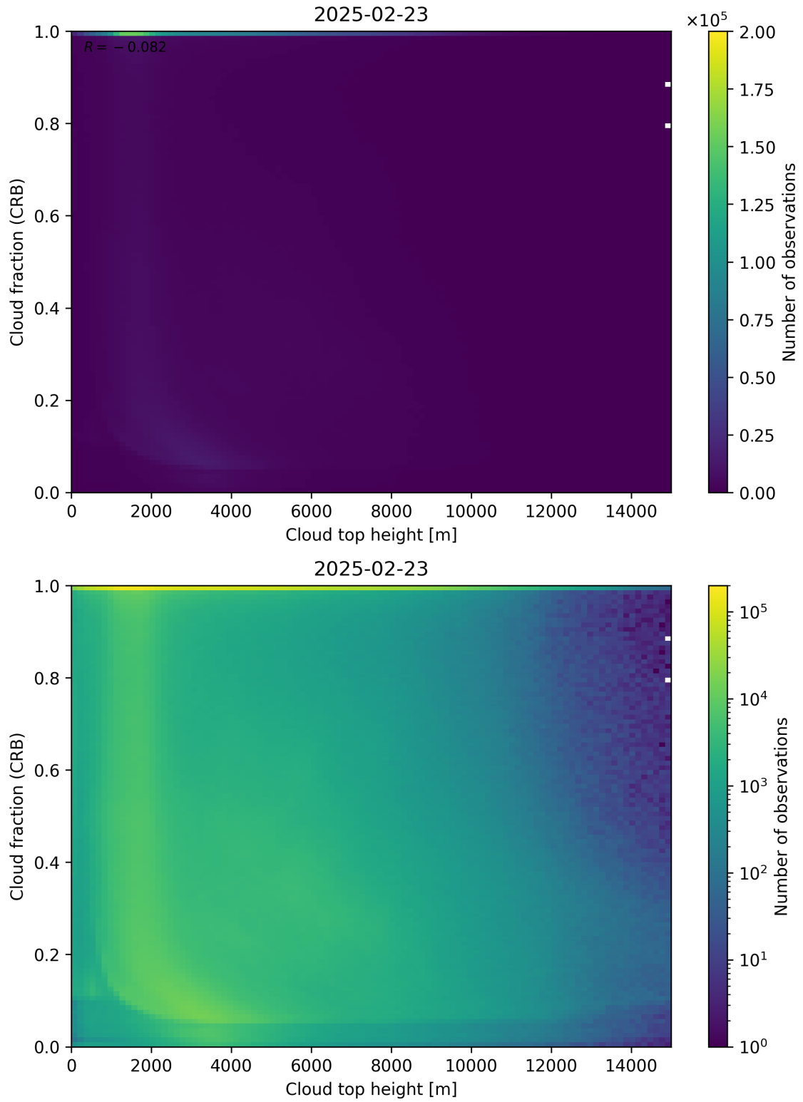
Figure 88: Scatter density plot of “Cloud top height” against “Cloud fraction (CRB)” for 2025-02-22 to 2025-02-24.
