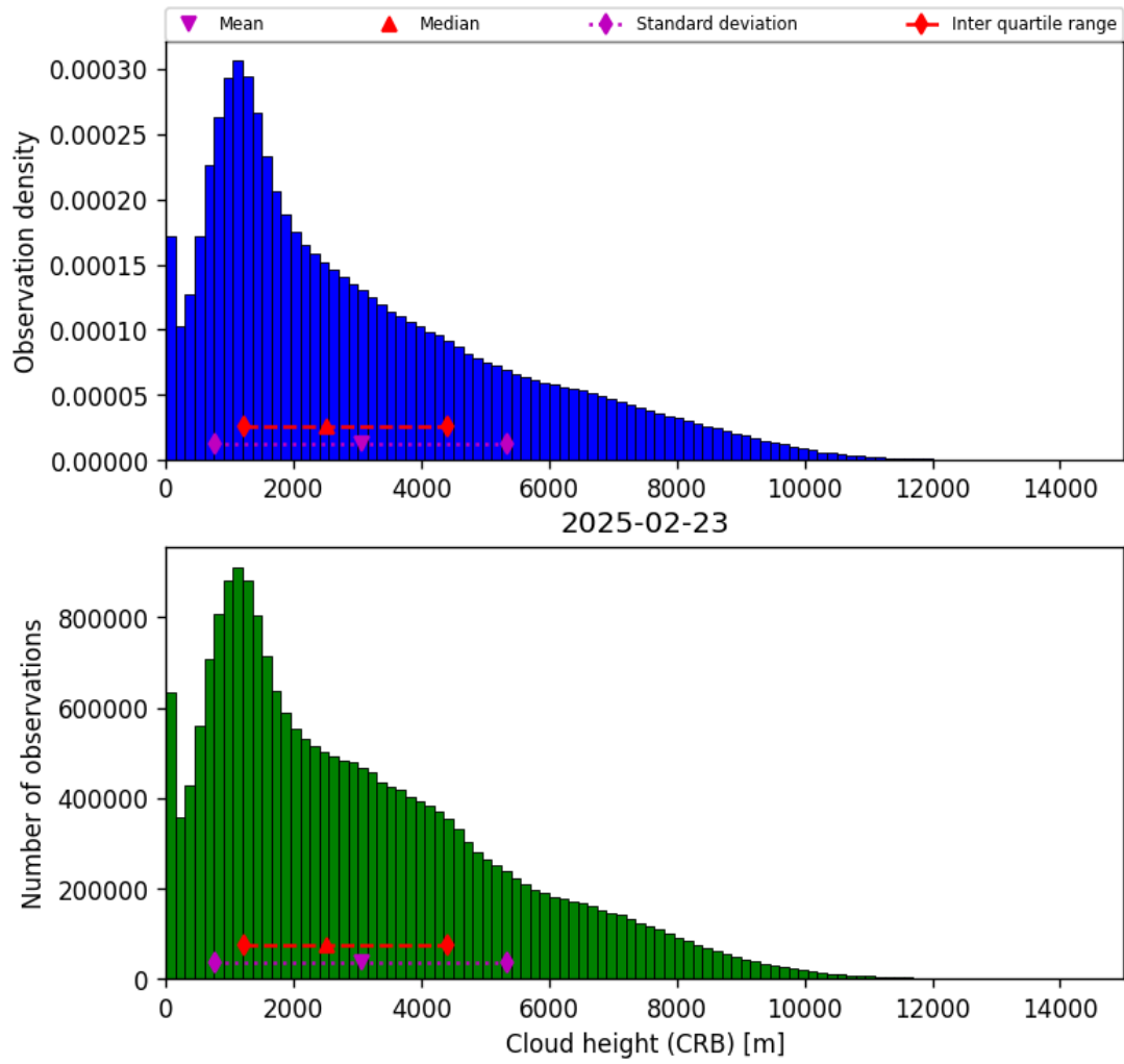
Figure 43: Histogram of “Cloud height (CRB)” for 2025-02-22 to 2025-02-24
