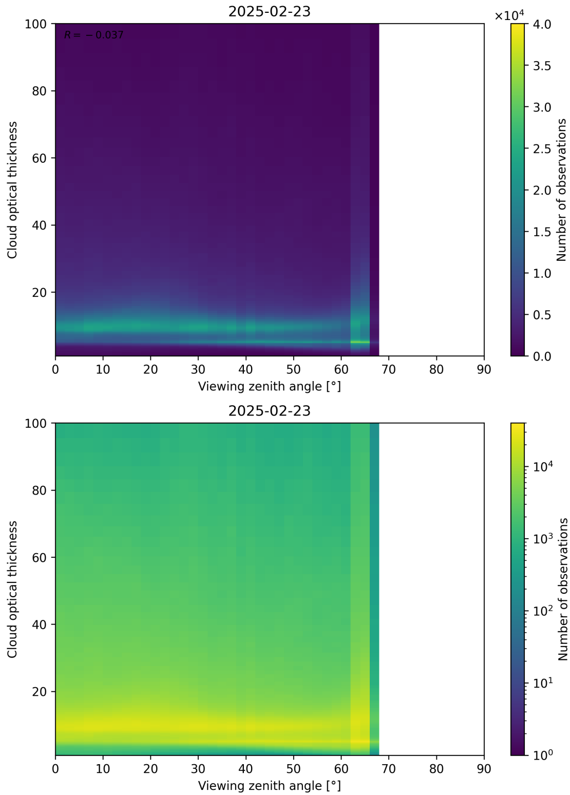
Figure 111: Scatter density plot of “Viewing zenith angle” against “Cloud optical thickness” for 2025-02-22 to 2025-02-24.
