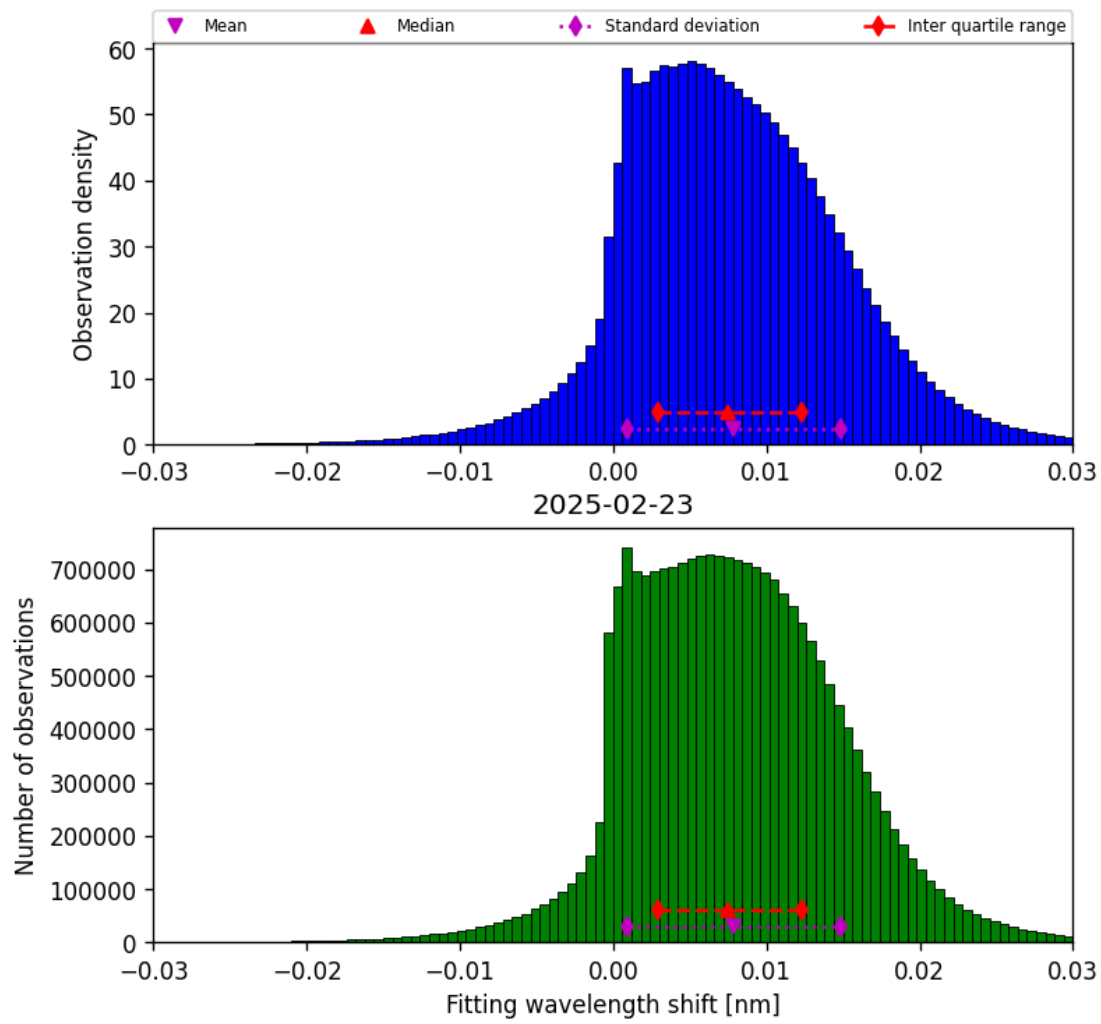
Figure 49: Histogram of “Fitting wavelength shift” for 2025-02-22 to 2025-02-24
