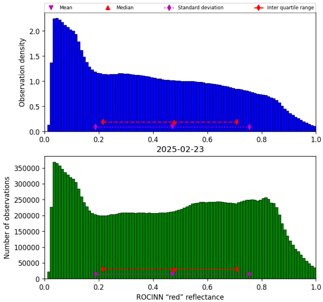
Figure 53: Histogram of “ROCINN “red” reflectance” for 2025-02-22 to 2025-02-24
