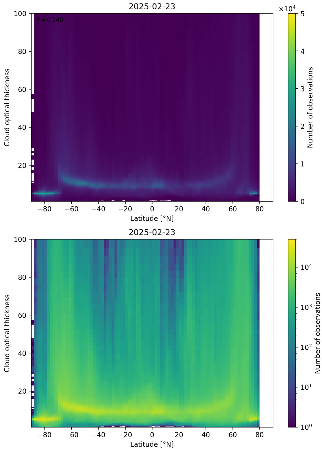
Figure 96: Scatter density plot of “Latitude” against “Cloud optical thickness” for 2025-02-22 to 2025-02-24.
