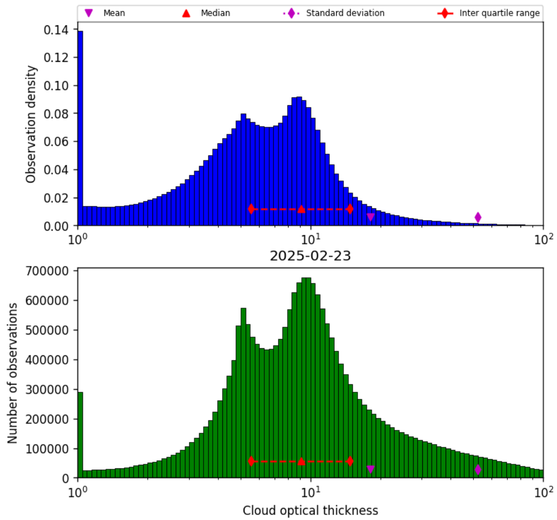
Figure 41: Histogram of “Cloud optical thickness” for 2025-02-22 to 2025-02-24
