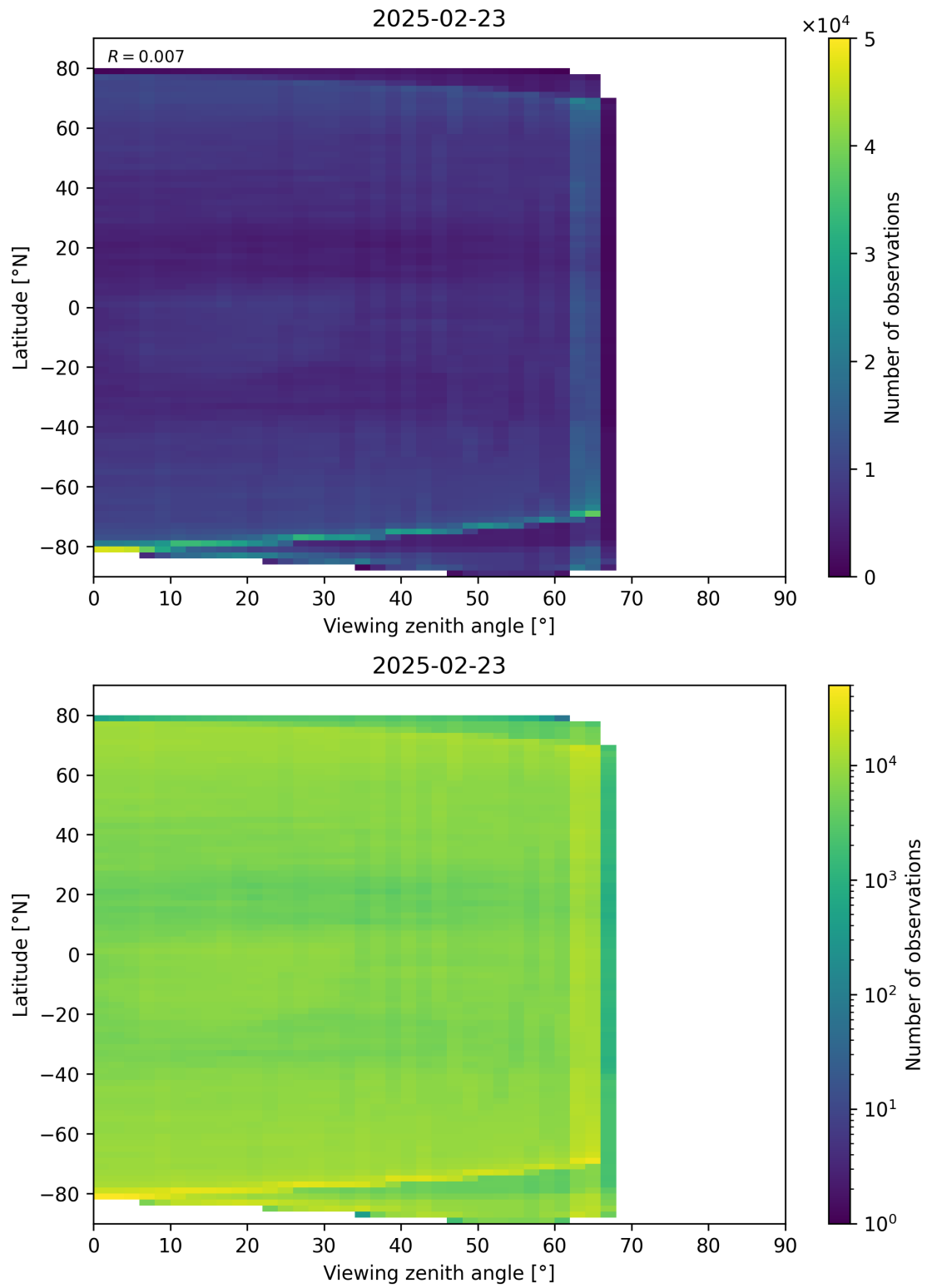
Figure 113: Scatter density plot of “Viewing zenith angle” against “Latitude” for 2025-02-22 to 2025-02-24.
