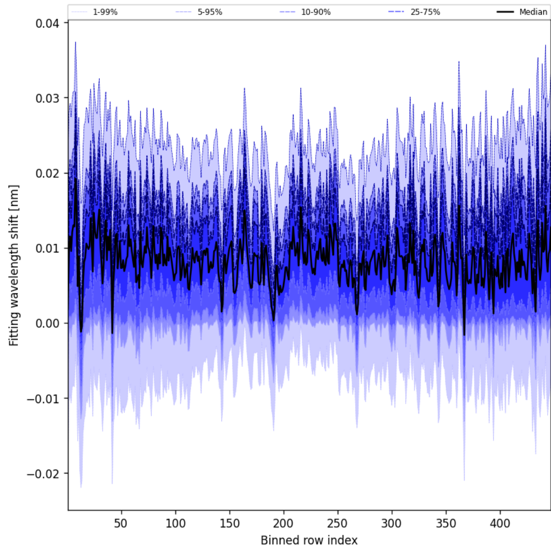
Figure 65: Along track statistics of “Fitting wavelength shift” for 2025-02-22 to 2025-02-24
