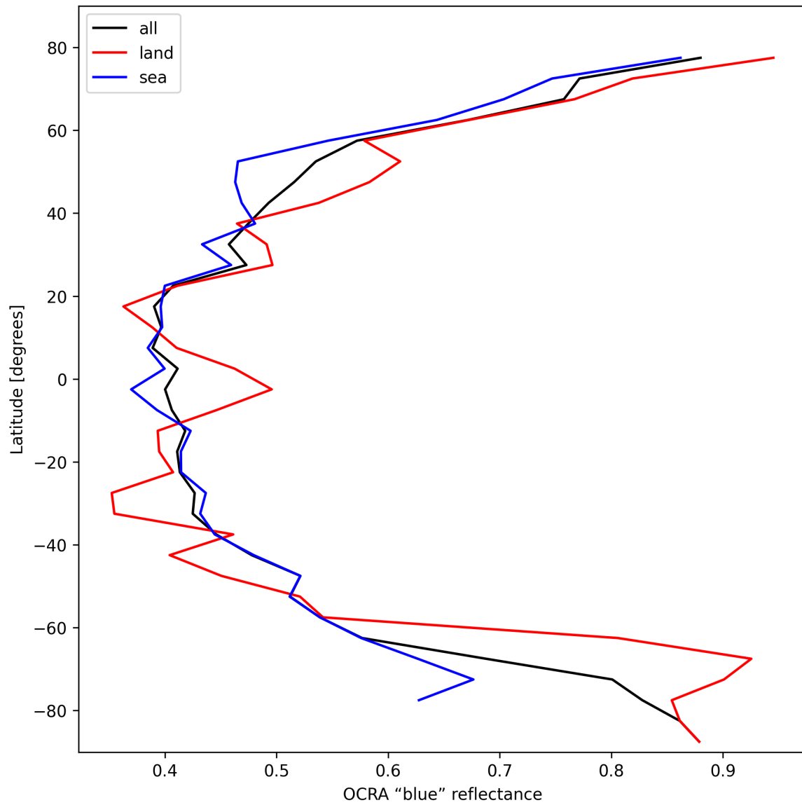
Figure 35: Zonal average of “OCRA “blue” reflectance” for 2025-02-22 to 2025-02-24.
