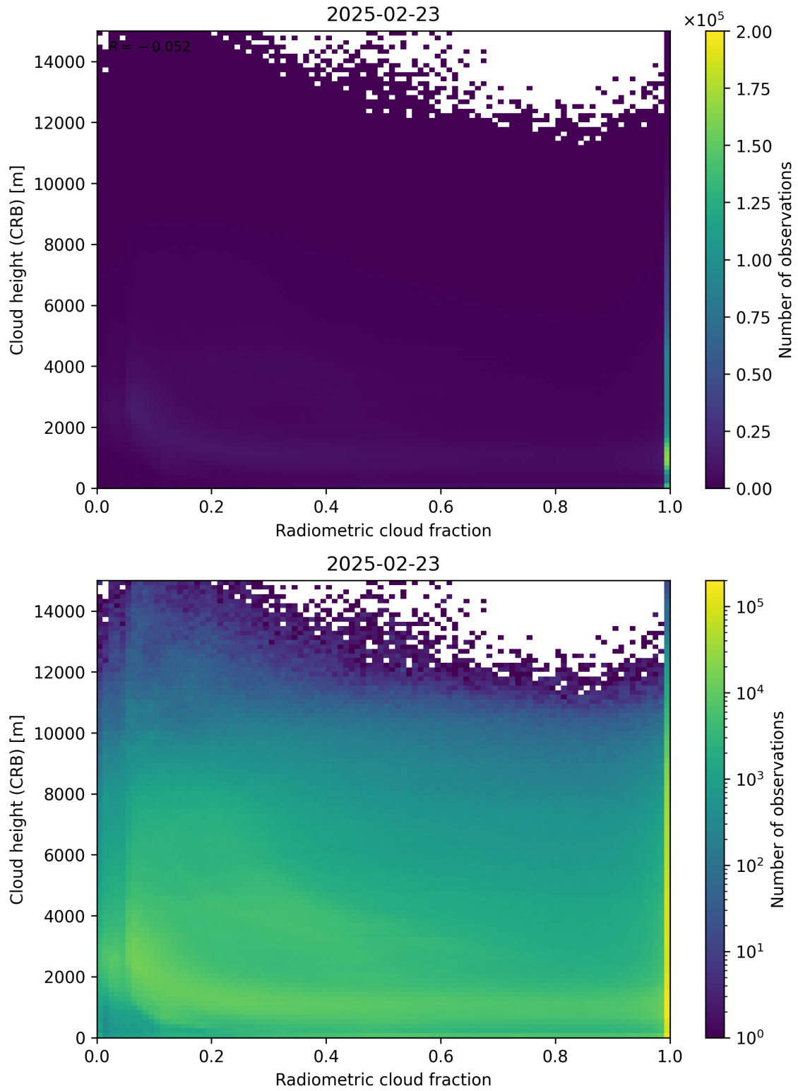
Figure 74: Scatter density plot of “Radiometric cloud fraction” against “Cloud height (CRB)” for 2025-02-22 to 2025-02-24.
