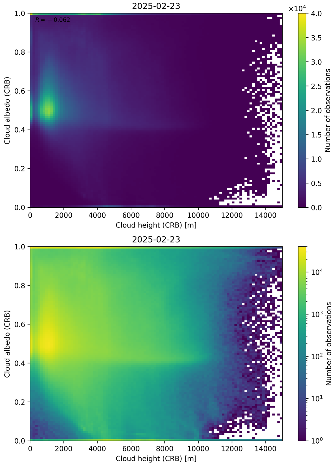
Figure 80: Scatter density plot of “Cloud height (CRB)” against “Cloud albedo (CRB)” for 2025-02-22 to 2025-02-24.
