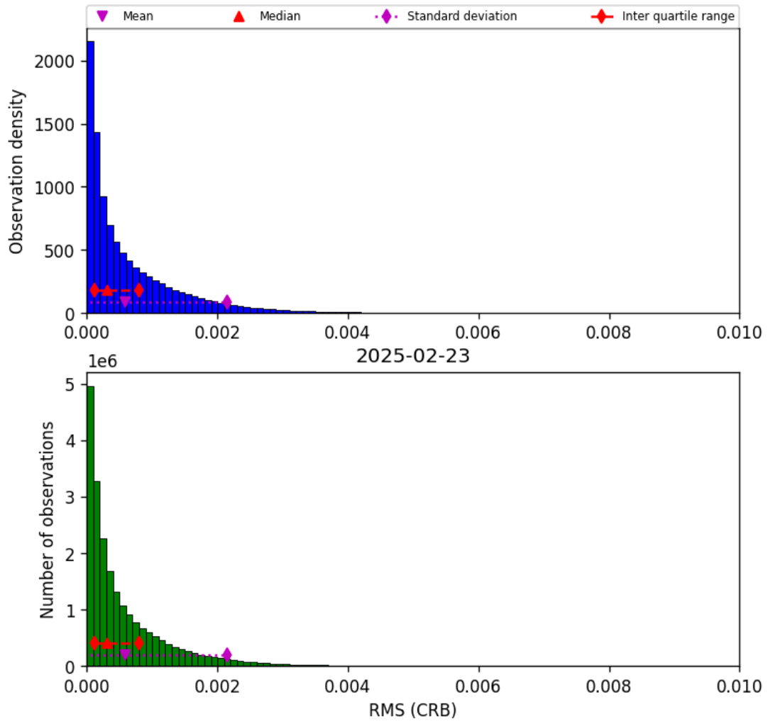
Figure 48: Histogram of “RMS (CRB)” for 2025-02-22 to 2025-02-24
