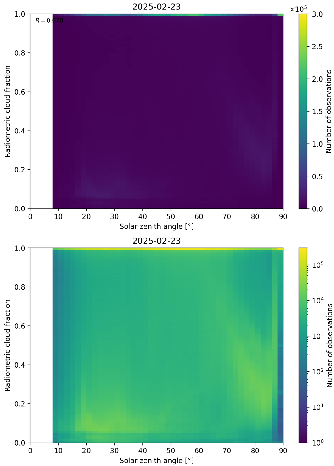
Figure 99: Scatter density plot of “Solar zenith angle” against “Radiometric cloud fraction” for 2025-02-22 to 2025-02-24.
