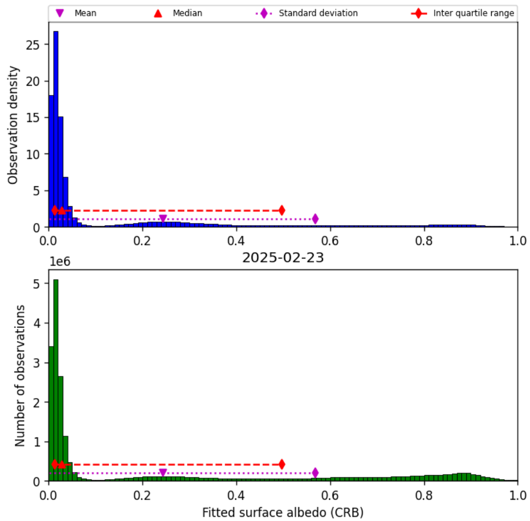
Figure 46: Histogram of “Fitted surface albedo (CRB)” for 2025-02-22 to 2025-02-24
