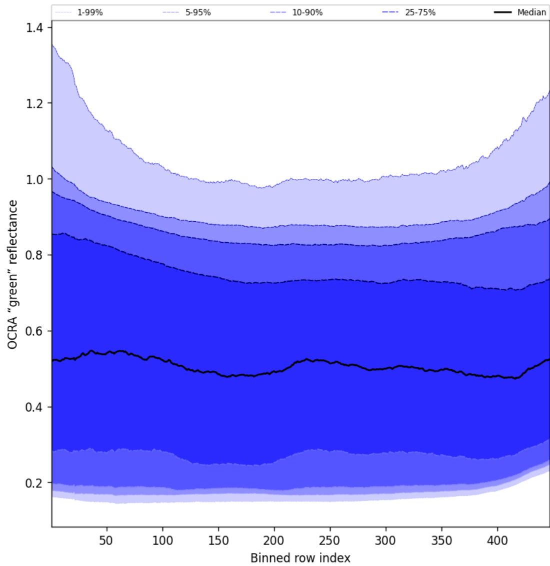
Figure 68: Along track statistics of “OCRA “green” reflectance” for 2025-02-22 to 2025-02-24
