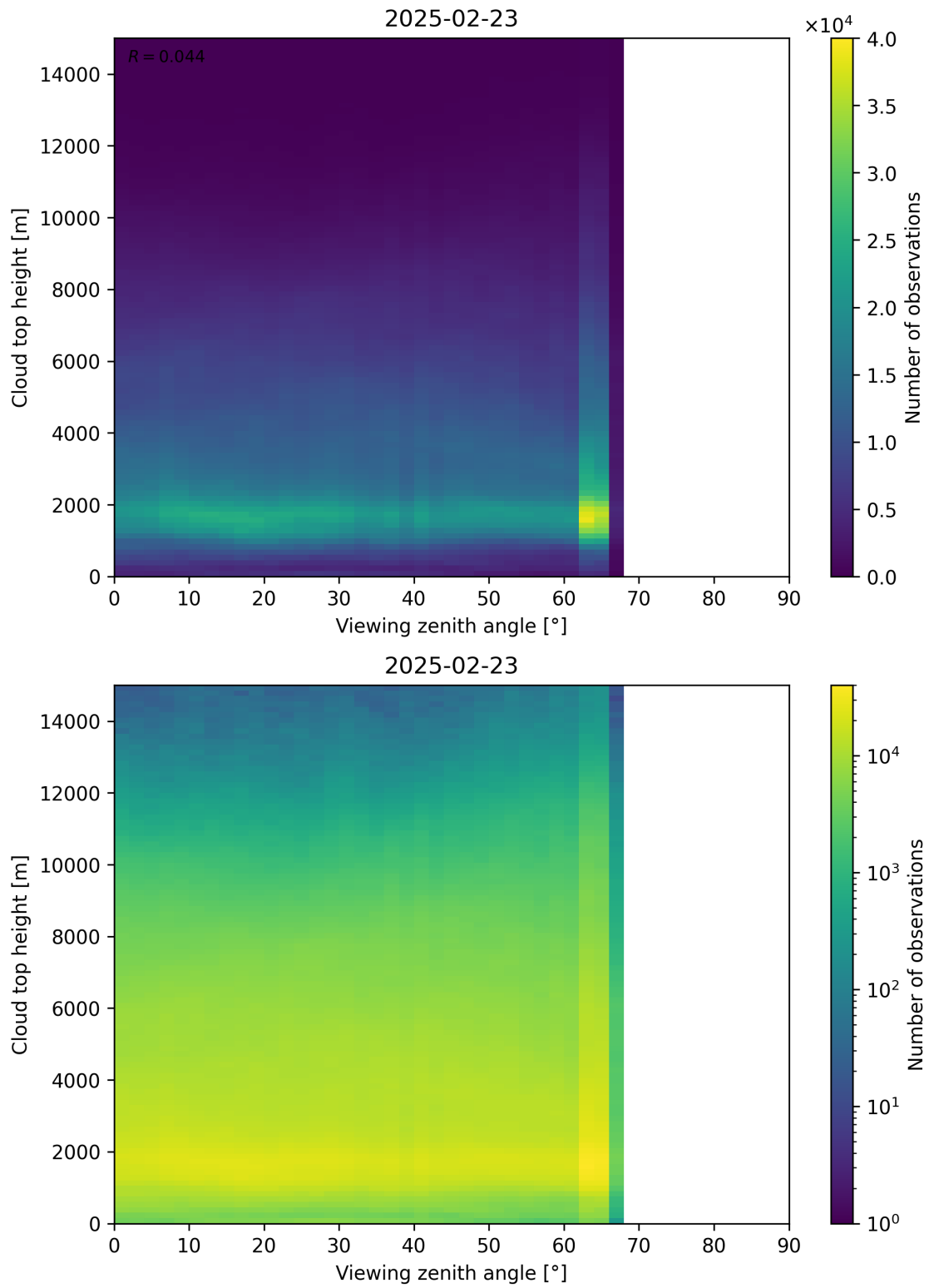
Figure 112: Scatter density plot of “Viewing zenith angle” against “Cloud top height” for 2025-02-22 to 2025-02-24.
