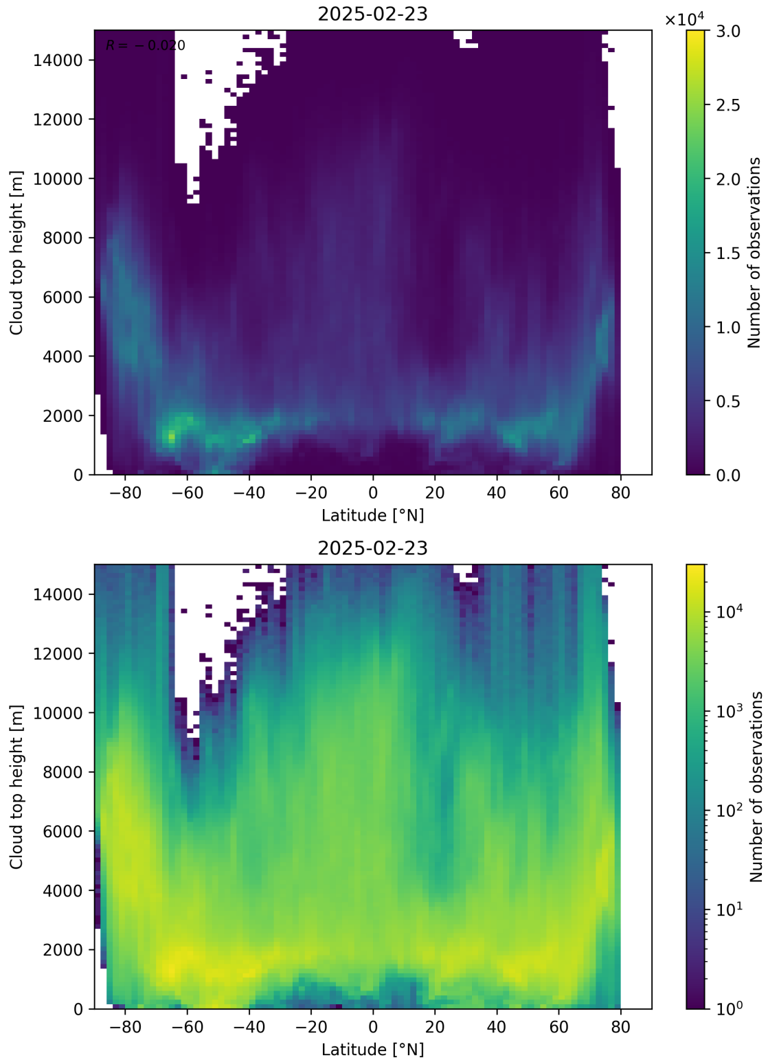
Figure 97: Scatter density plot of “Latitude” against “Cloud top height” for 2025-02-22 to 2025-02-24.
