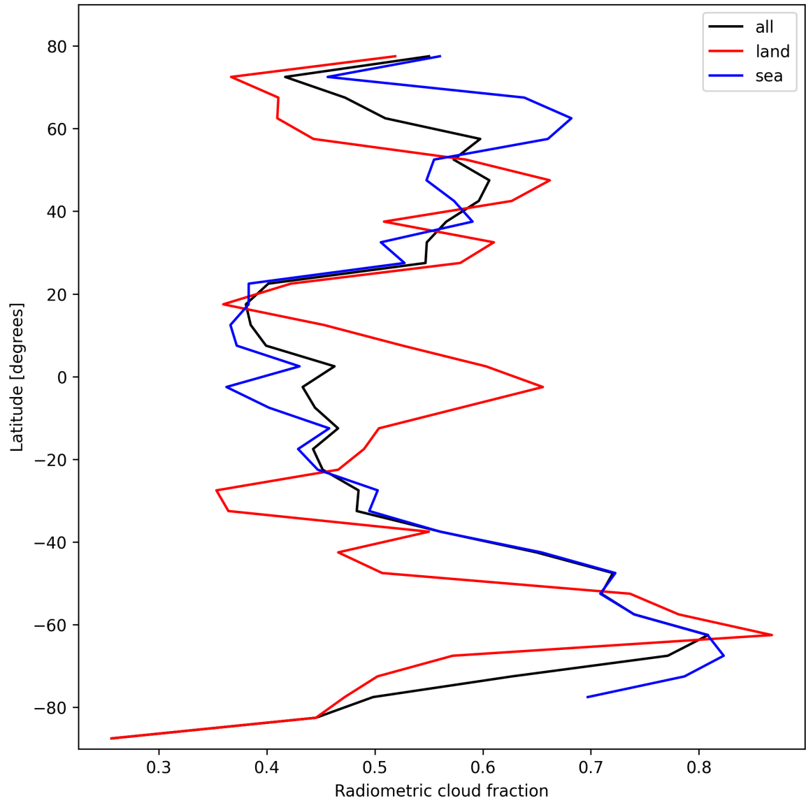
Figure 23: Zonal average of “Radiometric cloud fraction” for 2025-02-22 to 2025-02-24.
