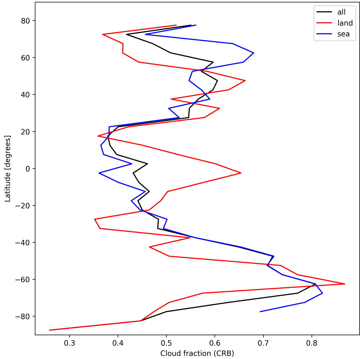
Figure 26: Zonal average of “Cloud fraction (CRB)” for 2025-02-22 to 2025-02-24.
