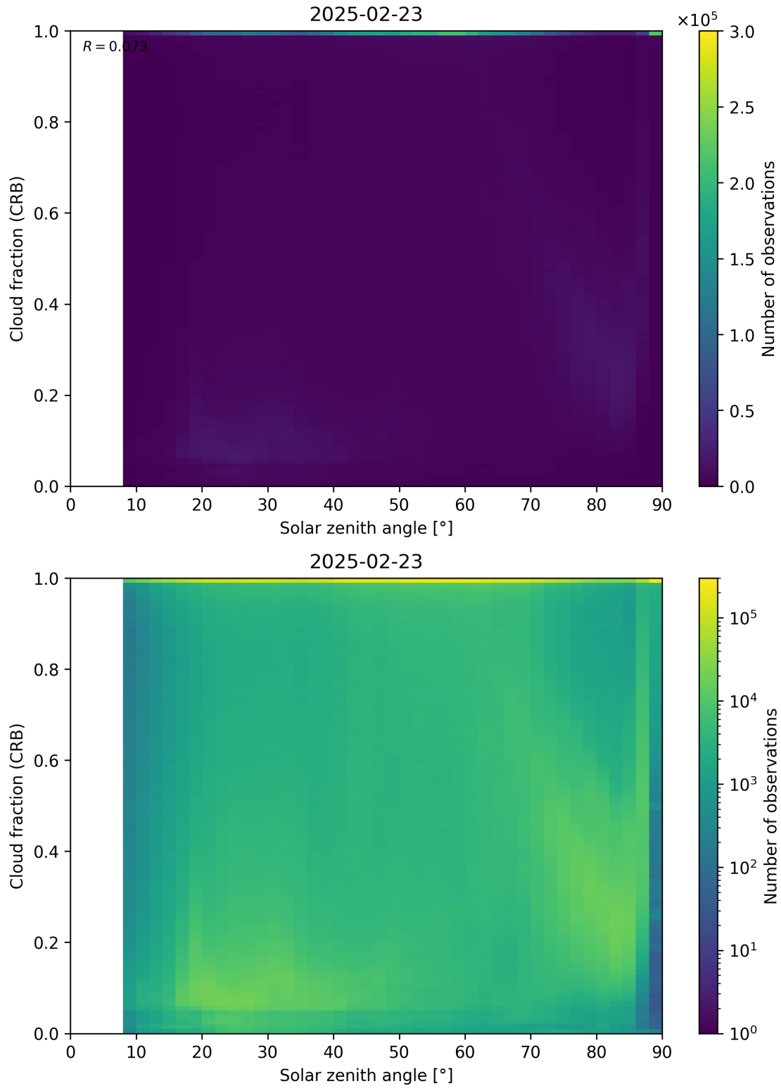
Figure 101: Scatter density plot of “Solar zenith angle” against “Cloud fraction (CRB)” for 2025-02-22 to 2025-02-24.
