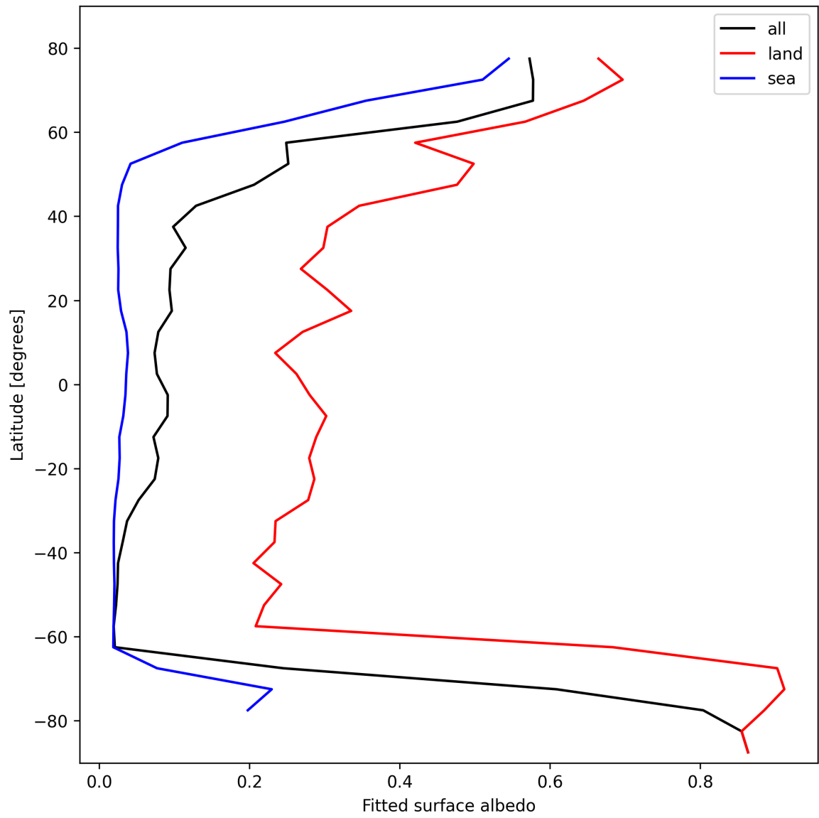
Figure 29: Zonal average of “Fitted surface albedo” for 2025-02-22 to 2025-02-24.
