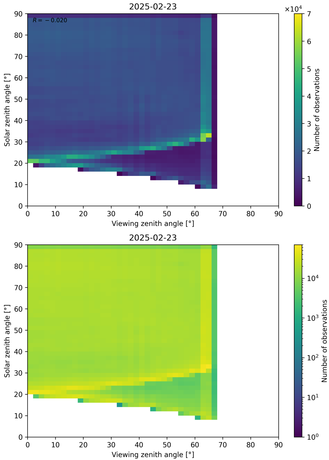
Figure 114: Scatter density plot of “Viewing zenith angle” against “Solar zenith angle” for 2025-02-22 to 2025-02-24.
