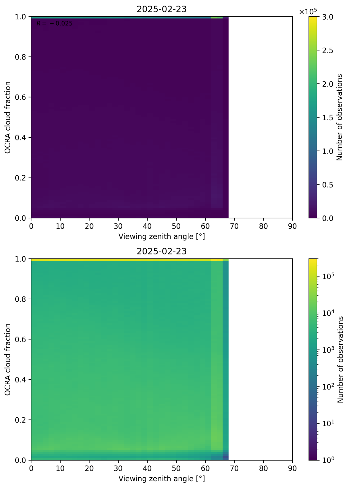
Figure 108: Scatter density plot of “Viewing zenith angle” against “OCRA cloud fraction” for 2025-02-22 to 2025-02-24.
