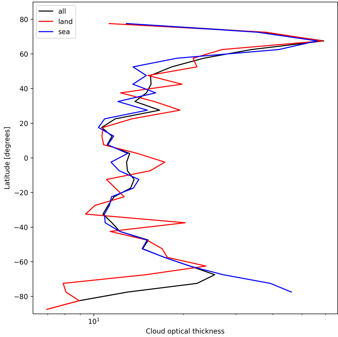
Figure 25: Zonal average of “Cloud optical thickness” for 2025-02-22 to 2025-02-24.
