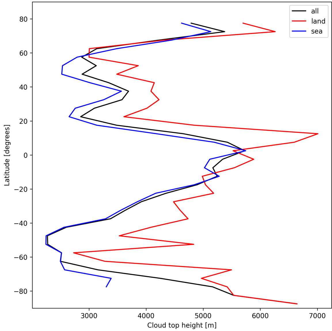
Figure 24: Zonal average of “Cloud top height” for 2025-02-22 to 2025-02-24.
