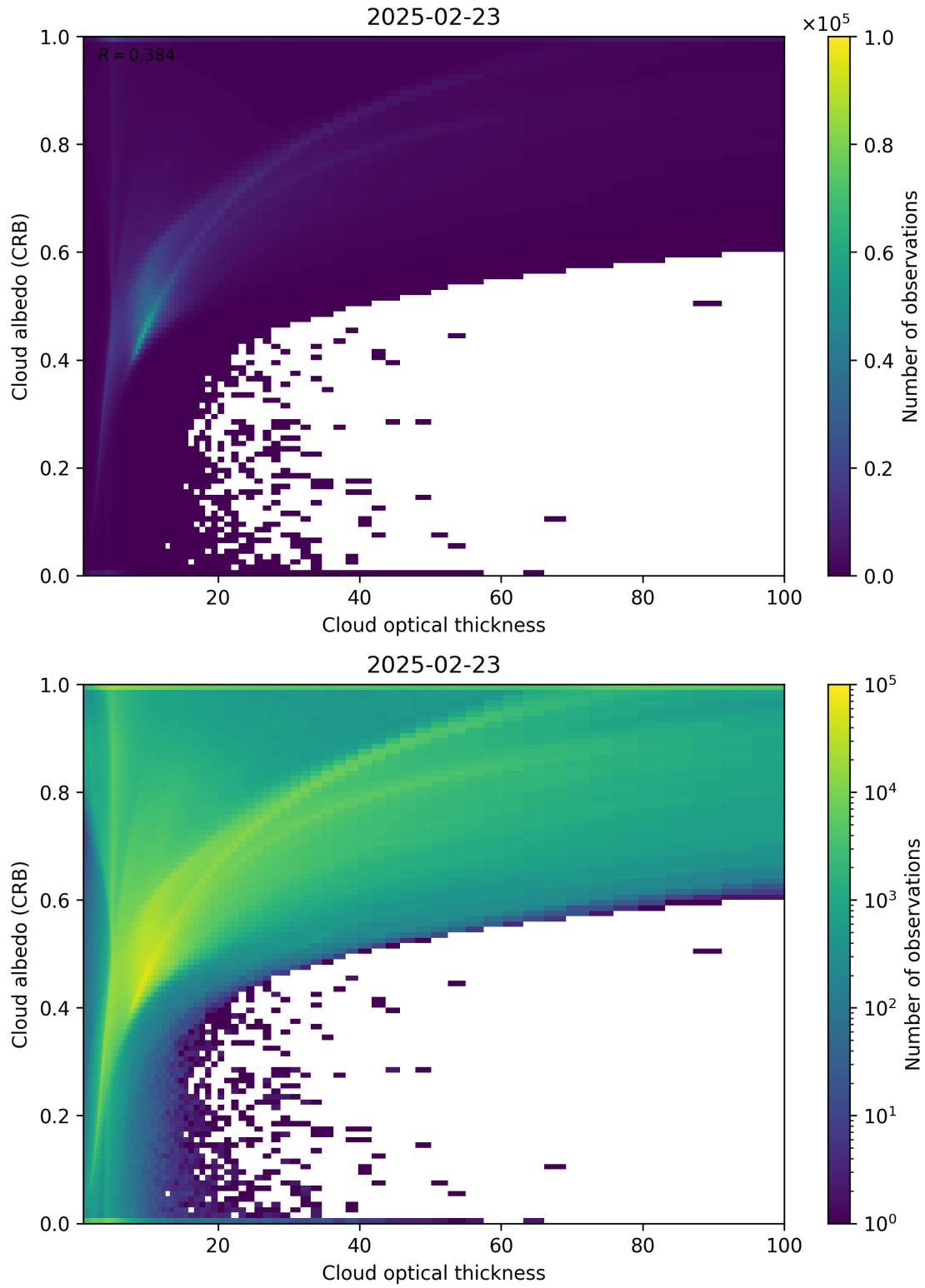
Figure 82: Scatter density plot of “Cloud optical thickness” against “Cloud albedo (CRB)” for 2025-02-22 to 2025-02-24.
