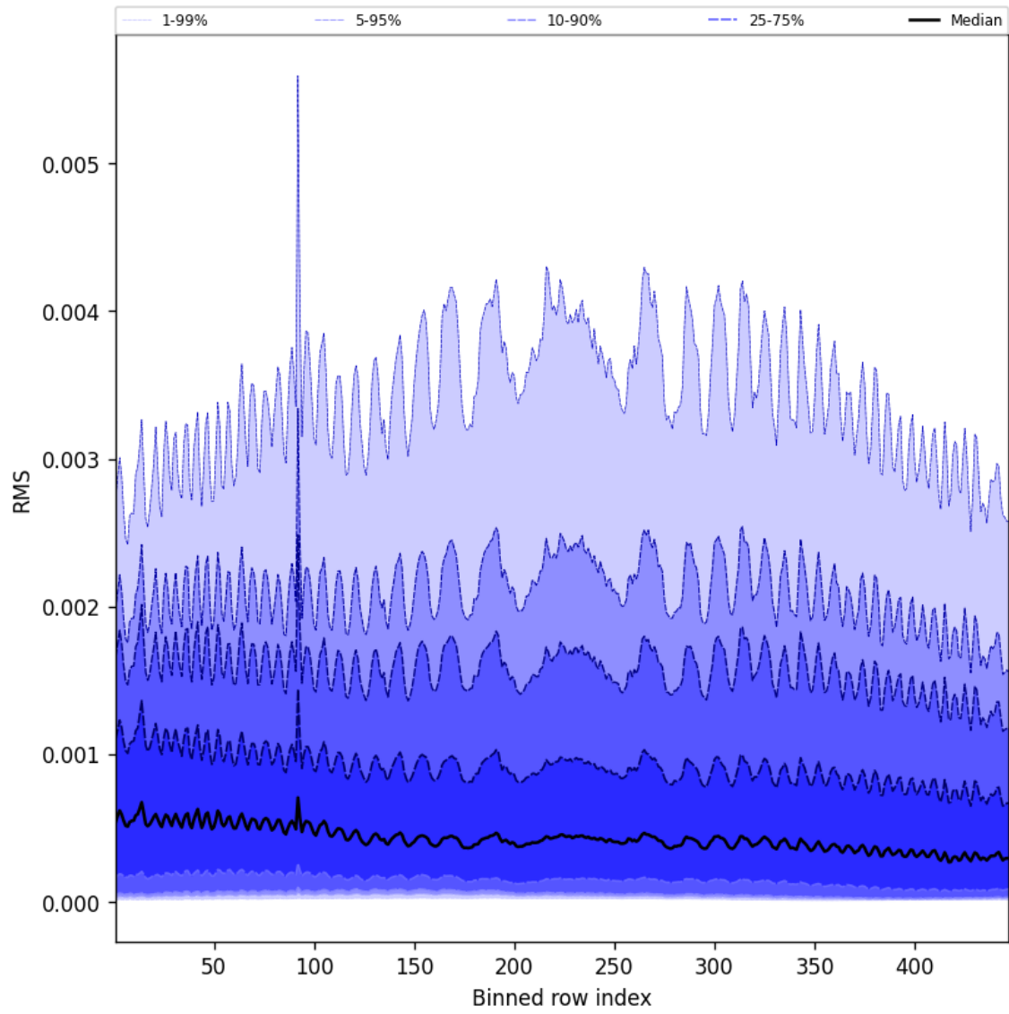
Figure 63: Along track statistics of “RMS” for 2025-02-22 to 2025-02-24
