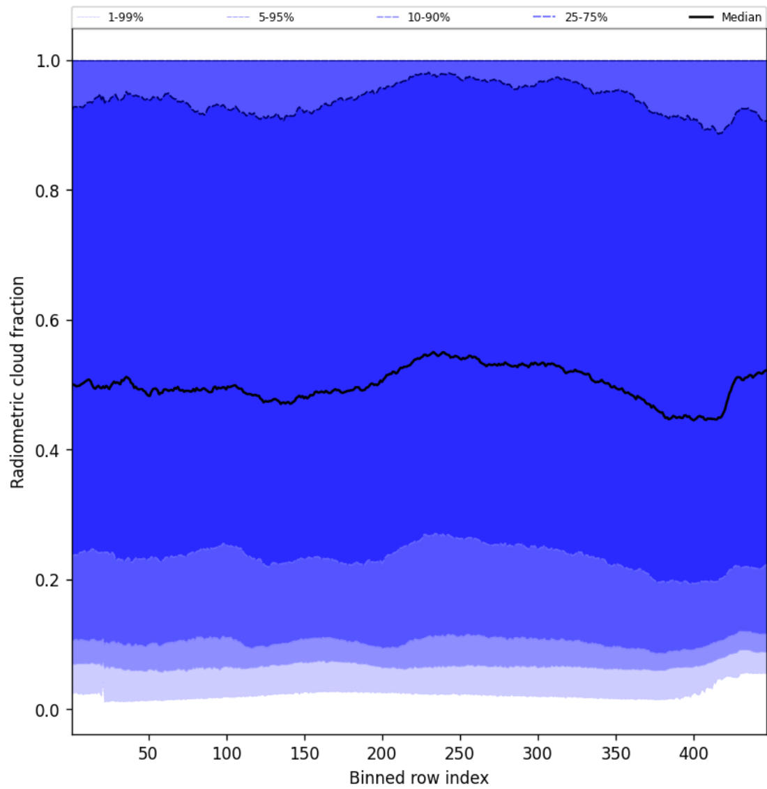
Figure 55: Along track statistics of “Radiometric cloud fraction” for 2025-02-22 to 2025-02-24
