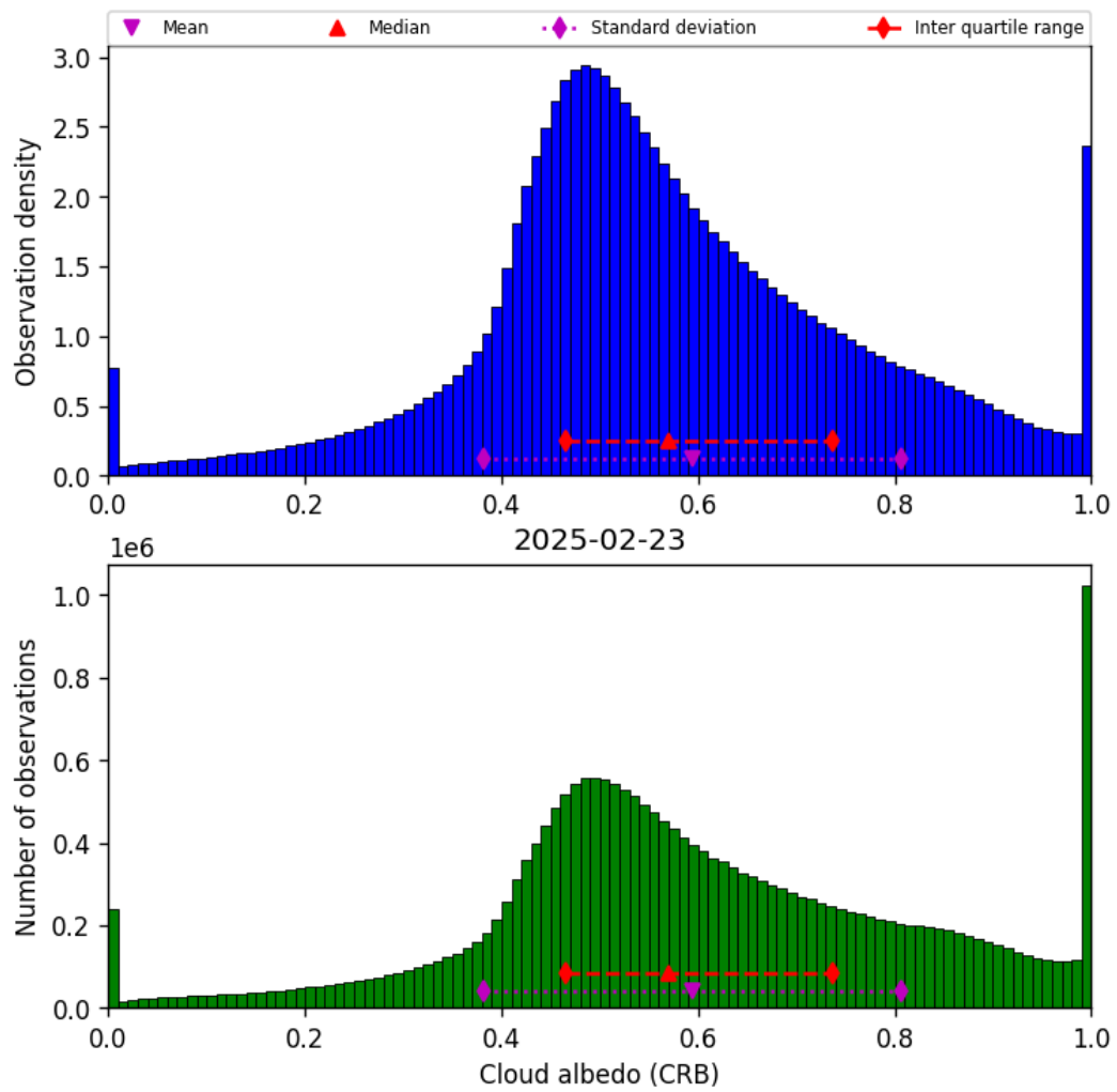
Figure 44: Histogram of “Cloud albedo (CRB)” for 2025-02-22 to 2025-02-24
