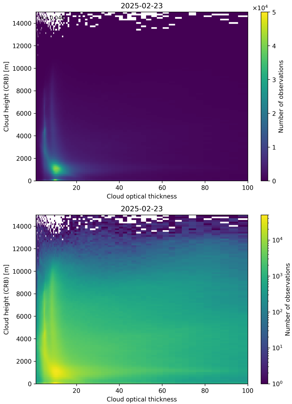
Figure 85: Scatter density plot of “Cloud optical thickness” against “Cloud height (CRB)” for 2025-02-22 to 2025-02-24.
