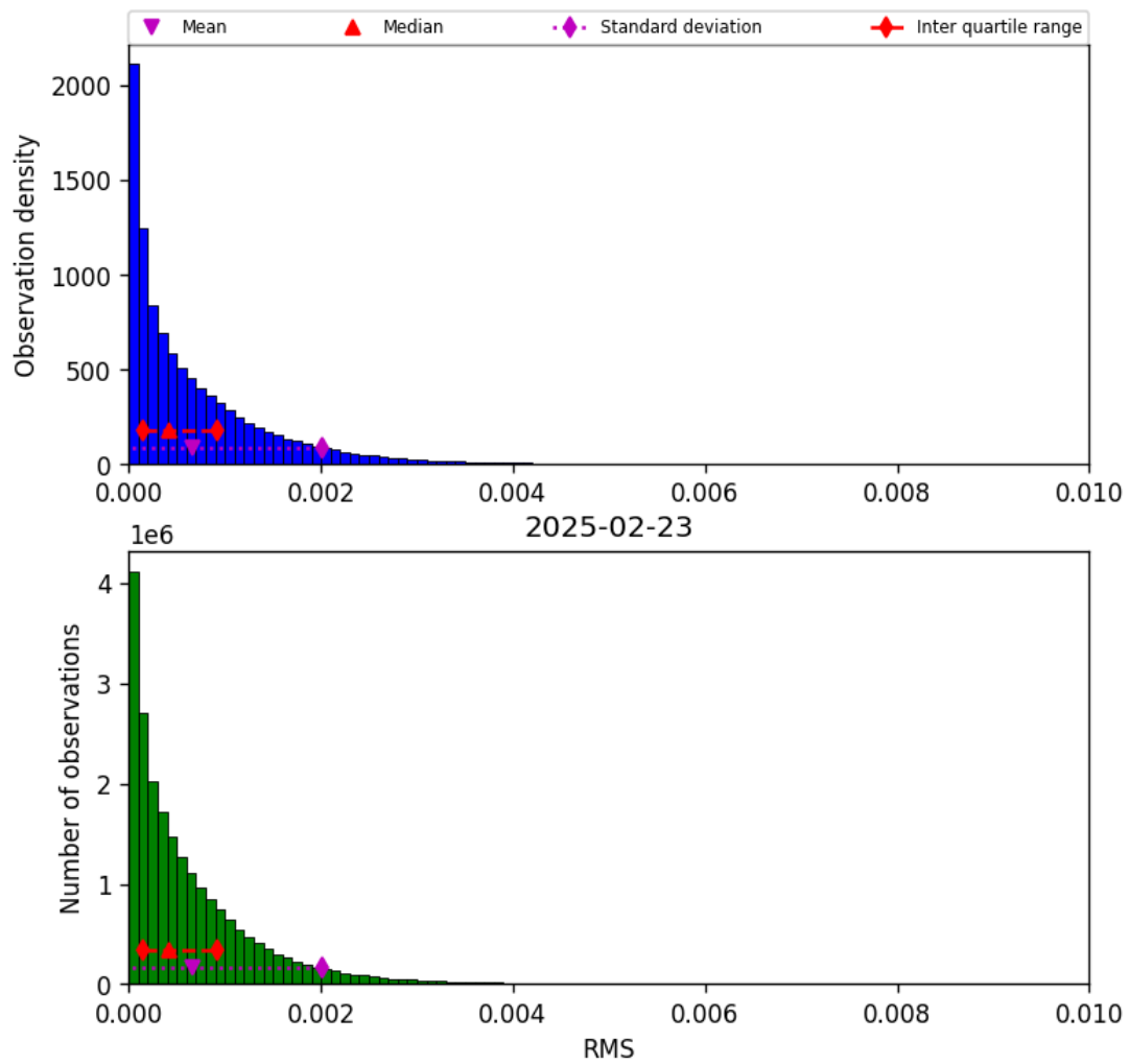
Figure 47: Histogram of “RMS” for 2025-02-22 to 2025-02-24
