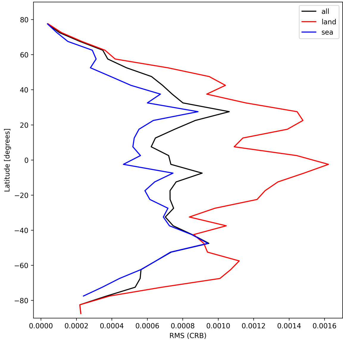
Figure 32: Zonal average of “RMS (CRB)” for 2025-02-22 to 2025-02-24.
