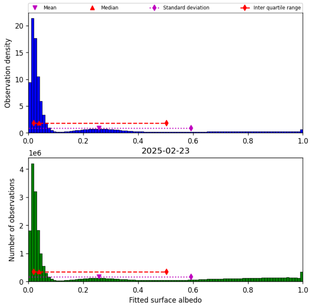
Figure 45: Histogram of “Fitted surface albedo” for 2025-02-22 to 2025-02-24
