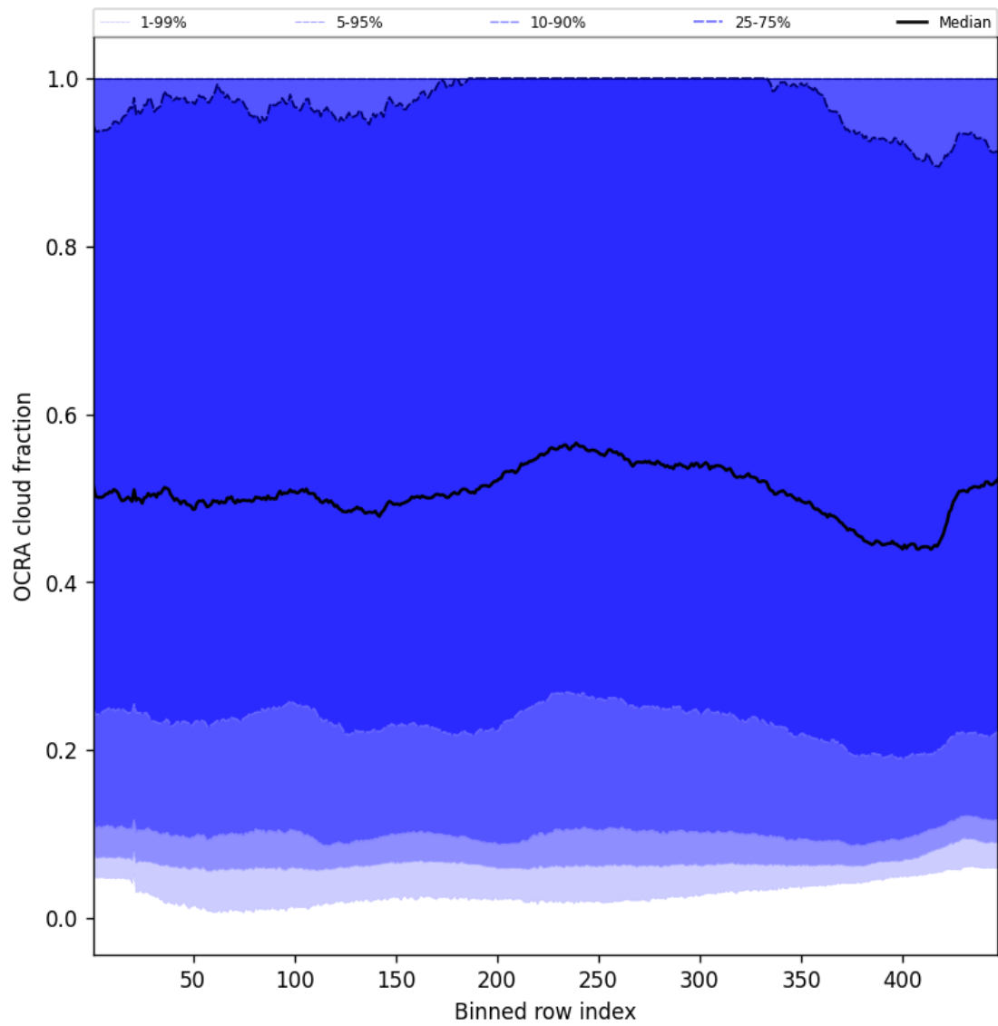
Figure 66: Along track statistics of “OCRA cloud fraction” for 2025-02-22 to 2025-02-24
