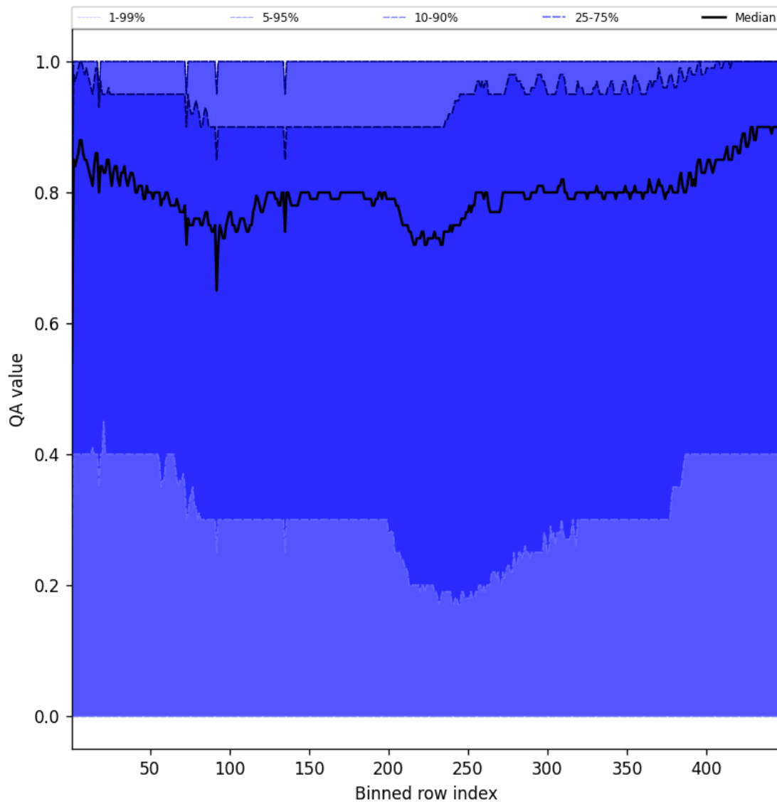
Figure 54: Along track statistics of “QA value” for 2025-02-22 to 2025-02-24
