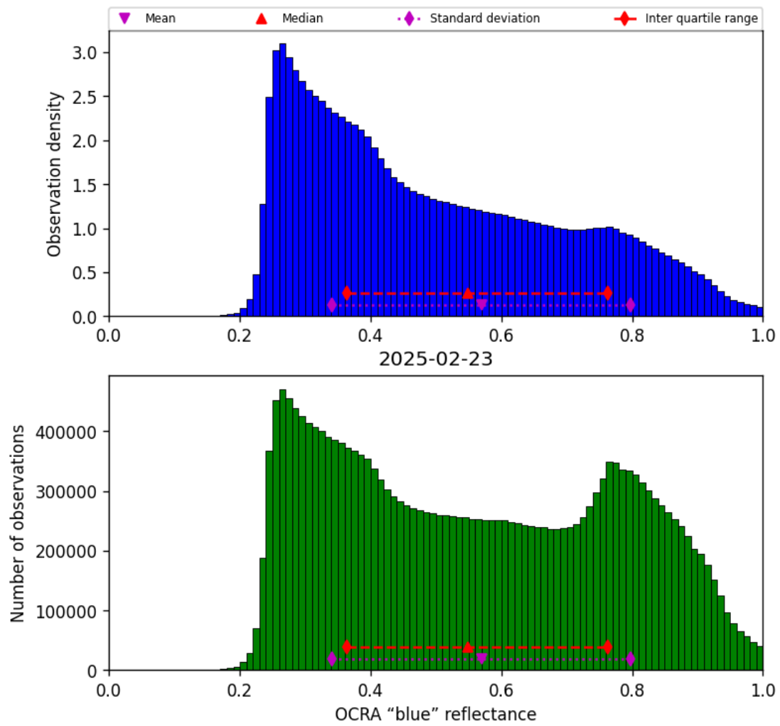
Figure 51: Histogram of “OCRA “blue” reflectance” for 2025-02-22 to 2025-02-24
