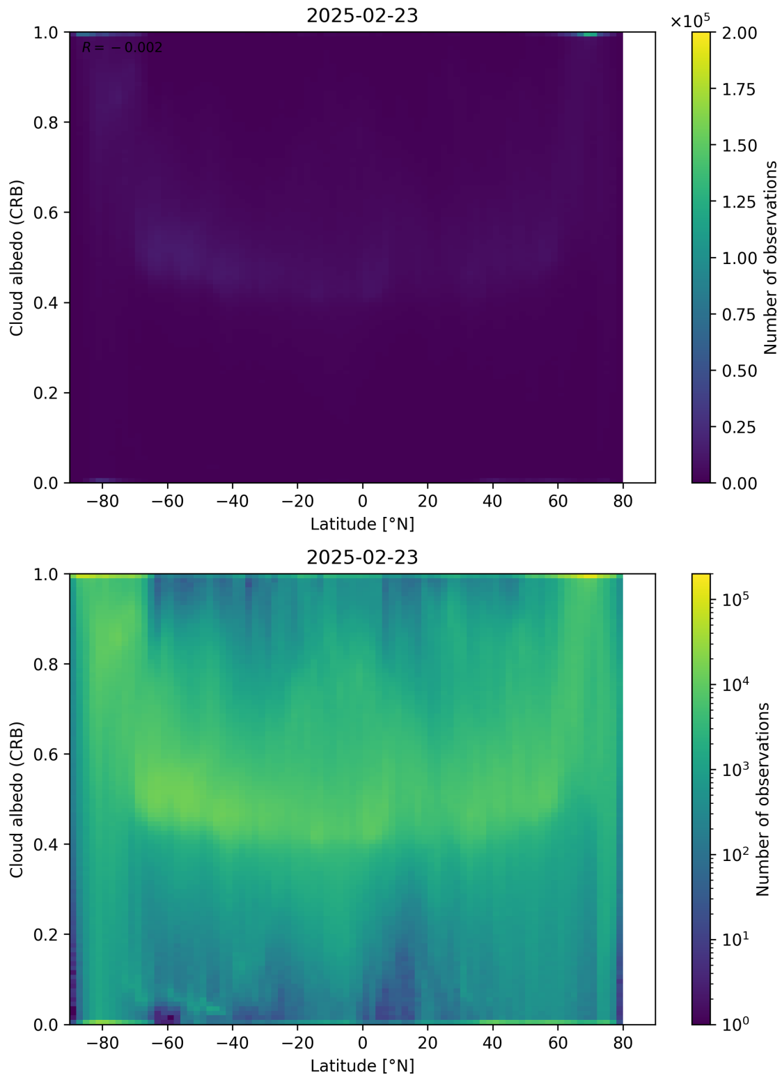
Figure 91: Scatter density plot of “Latitude” against “Cloud albedo (CRB)” for 2025-02-22 to 2025-02-24.
