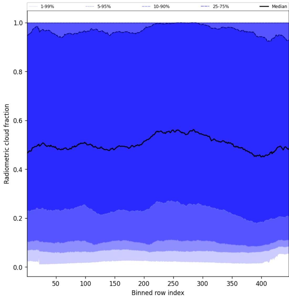
Figure 55: Along track statistics of “Radiometric cloud fraction” for 2025-02-24 to 2025-02-26
