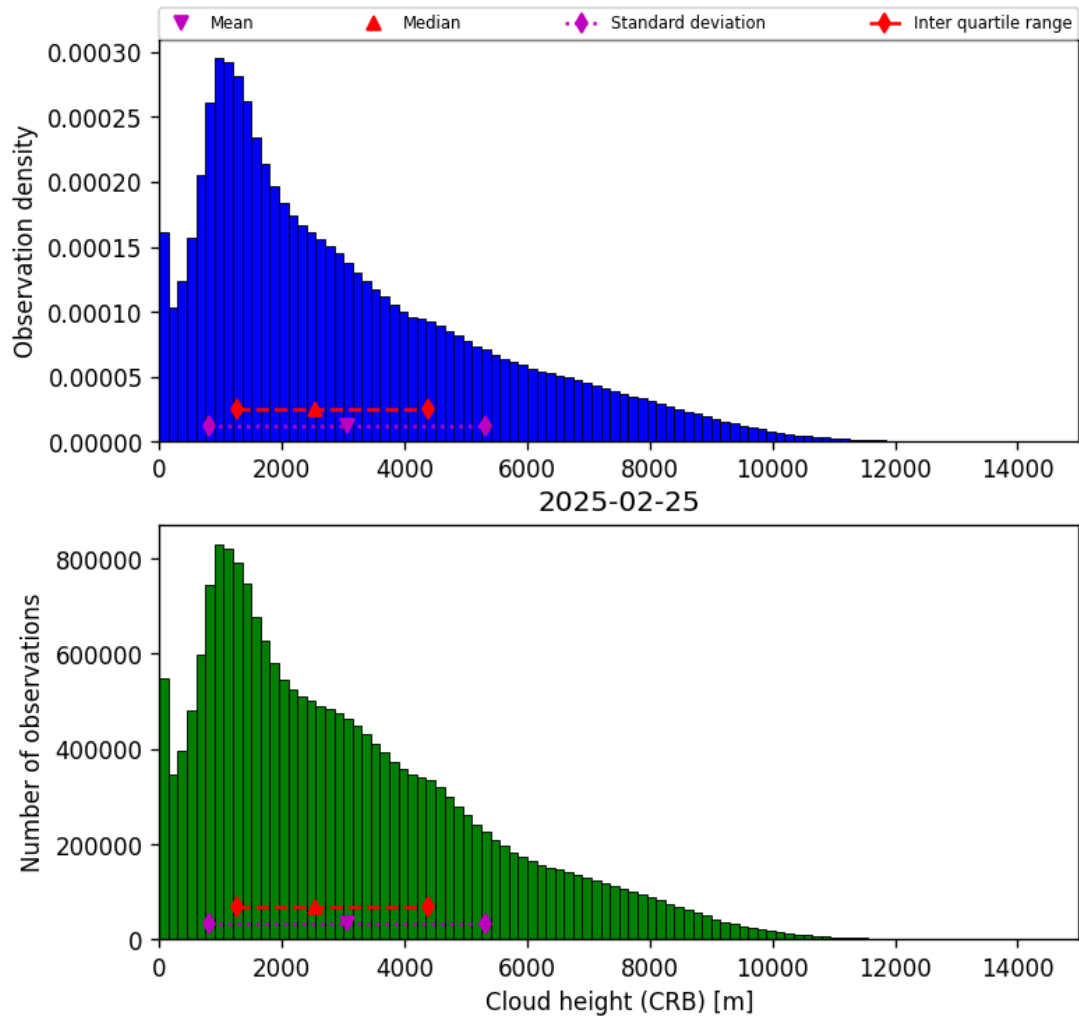
Figure 43: Histogram of “Cloud height (CRB)” for 2025-02-24 to 2025-02-26
