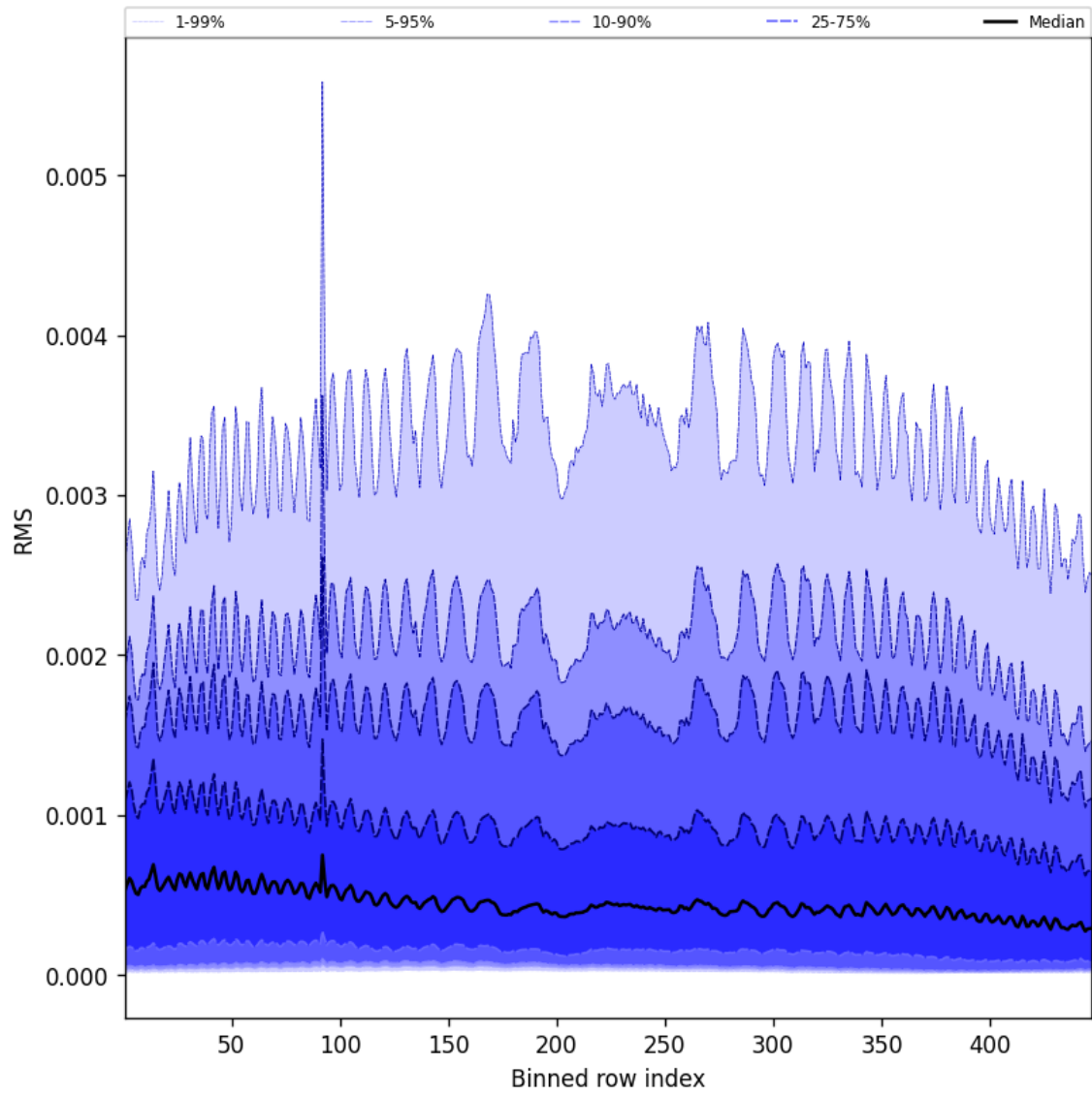
Figure 63: Along track statistics of “RMS” for 2025-02-24 to 2025-02-26
