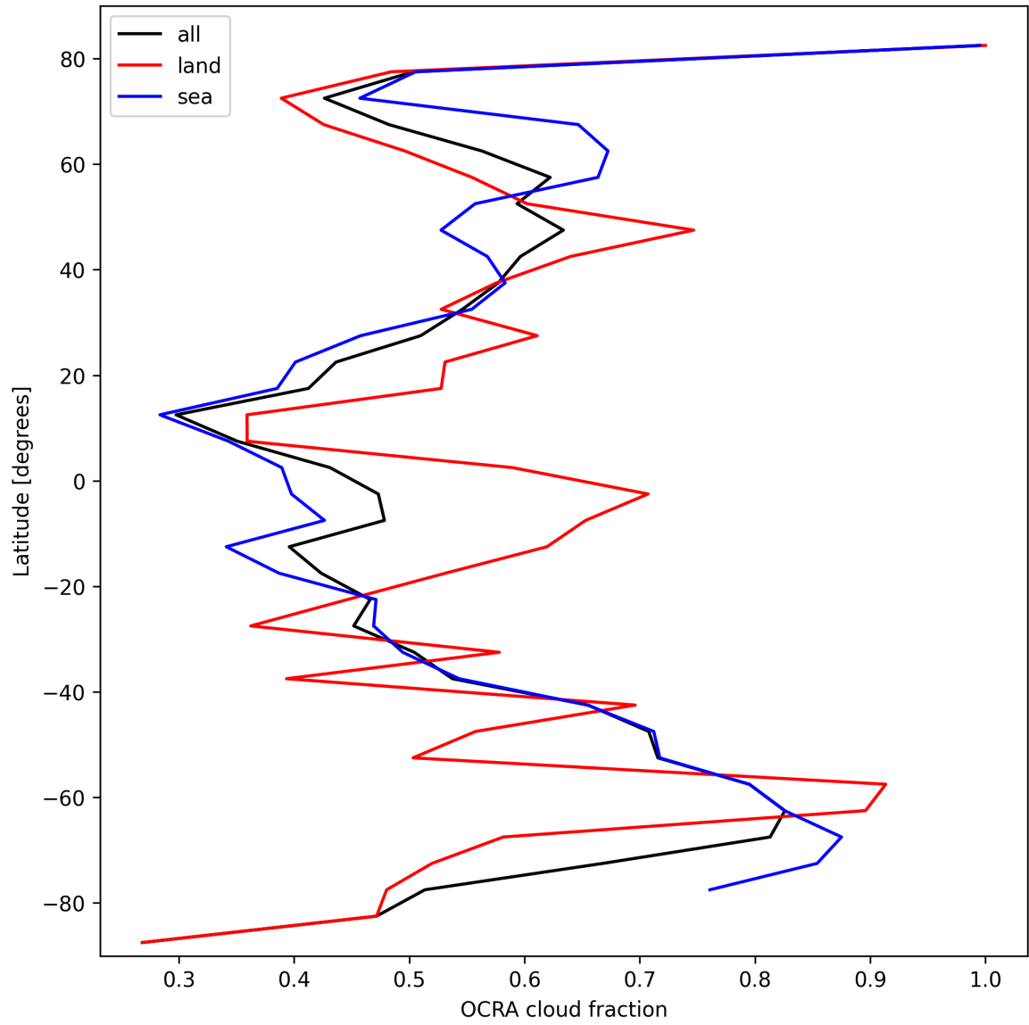
Figure 34: Zonal average of “OCRA cloud fraction” for 2025-02-24 to 2025-02-26.
