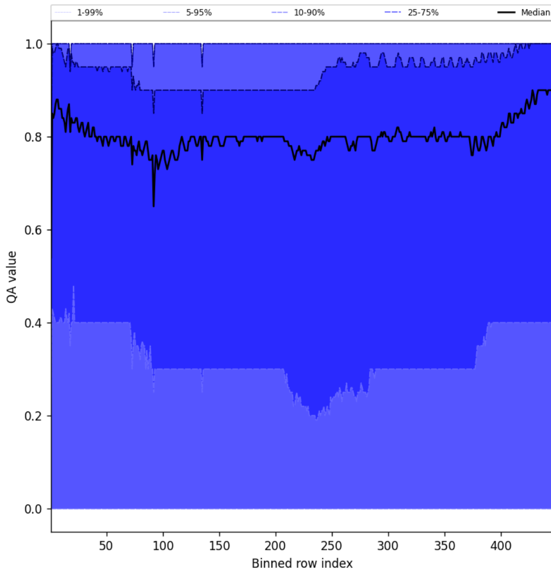
Figure 54: Along track statistics of “QA value” for 2025-02-24 to 2025-02-26
