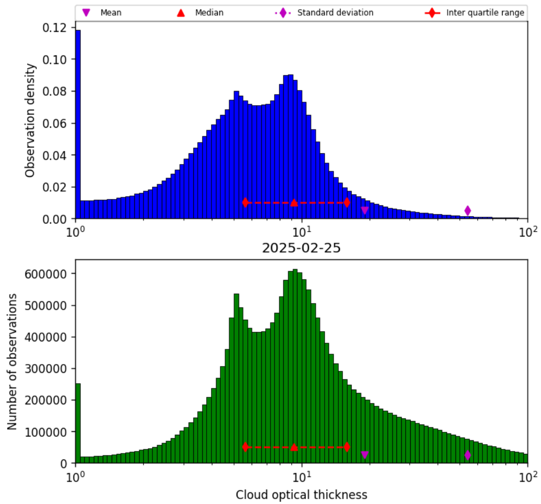
Figure 41: Histogram of “Cloud optical thickness” for 2025-02-24 to 2025-02-26
