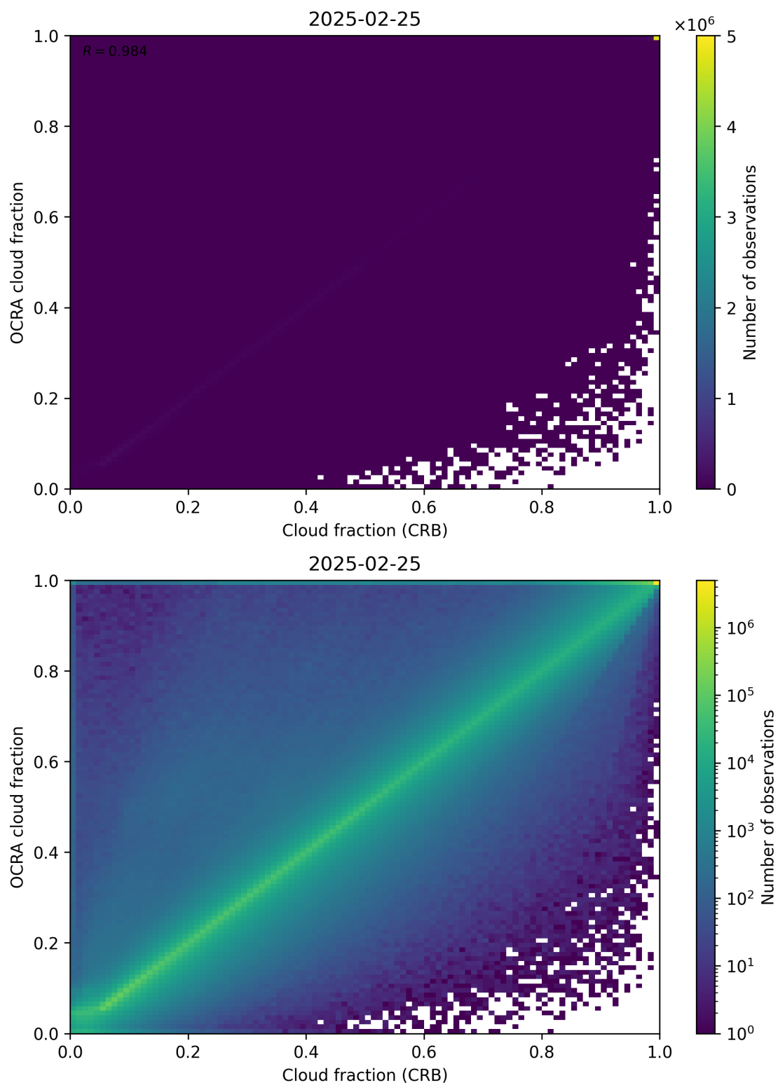
Figure 78: Scatter density plot of “Cloud fraction (CRB)” against “OCRA cloud fraction” for 2025-02-24 to 2025-02-26.
