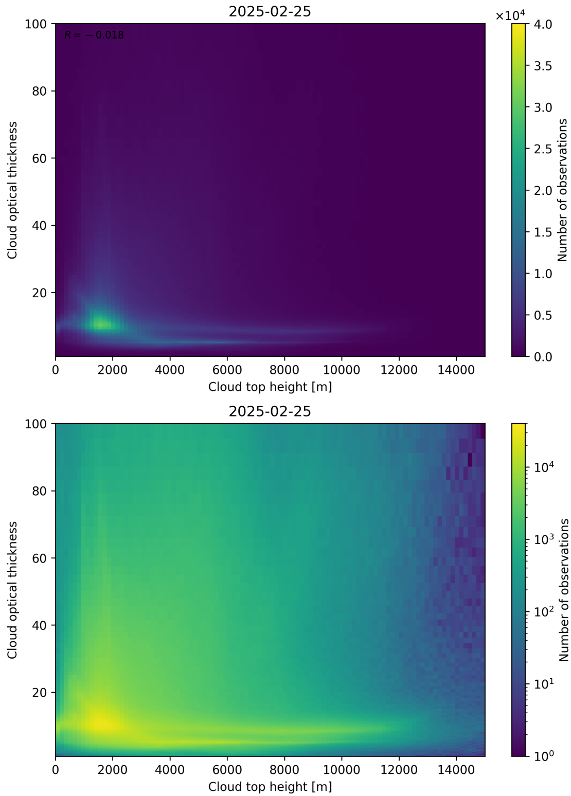
Figure 90: Scatter density plot of “Cloud top height” against “Cloud optical thickness” for 2025-02-24 to 2025-02-26.
