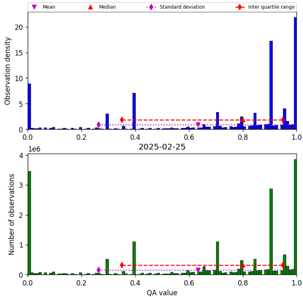
Figure 38: Histogram of “QA value” for 2025-02-24 to 2025-02-26
