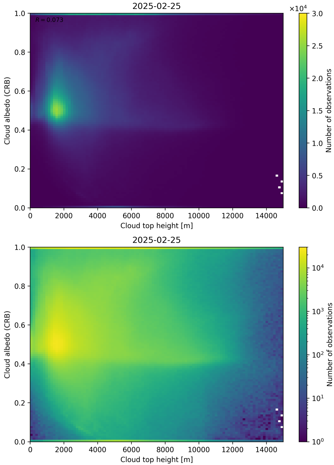
Figure 86: Scatter density plot of “Cloud top height” against “Cloud albedo (CRB)” for 2025-02-24 to 2025-02-26.
