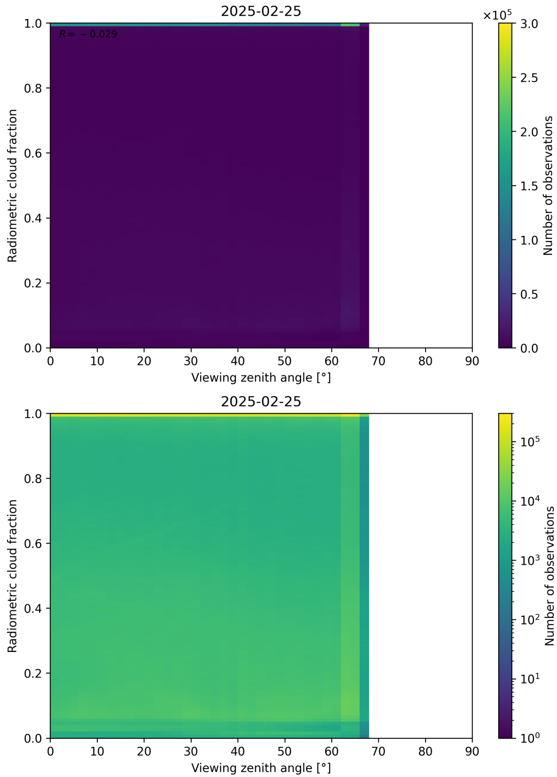
Figure 107: Scatter density plot of “Viewing zenith angle” against “Radiometric cloud fraction” for 2025-02-24 to 2025-02-26.
