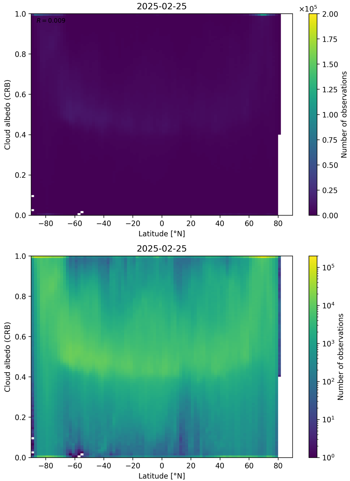
Figure 91: Scatter density plot of “Latitude” against “Cloud albedo (CRB)” for 2025-02-24 to 2025-02-26.
