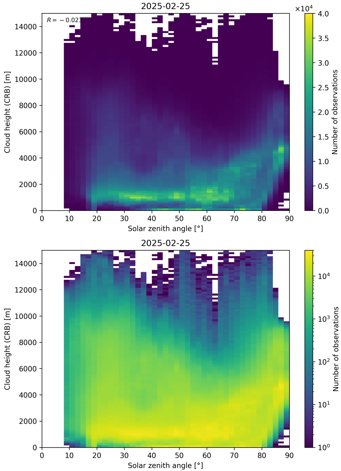
Figure 102: Scatter density plot of “Solar zenith angle” against “Cloud height (CRB)” for 2025-02-24 to 2025-02-26.
