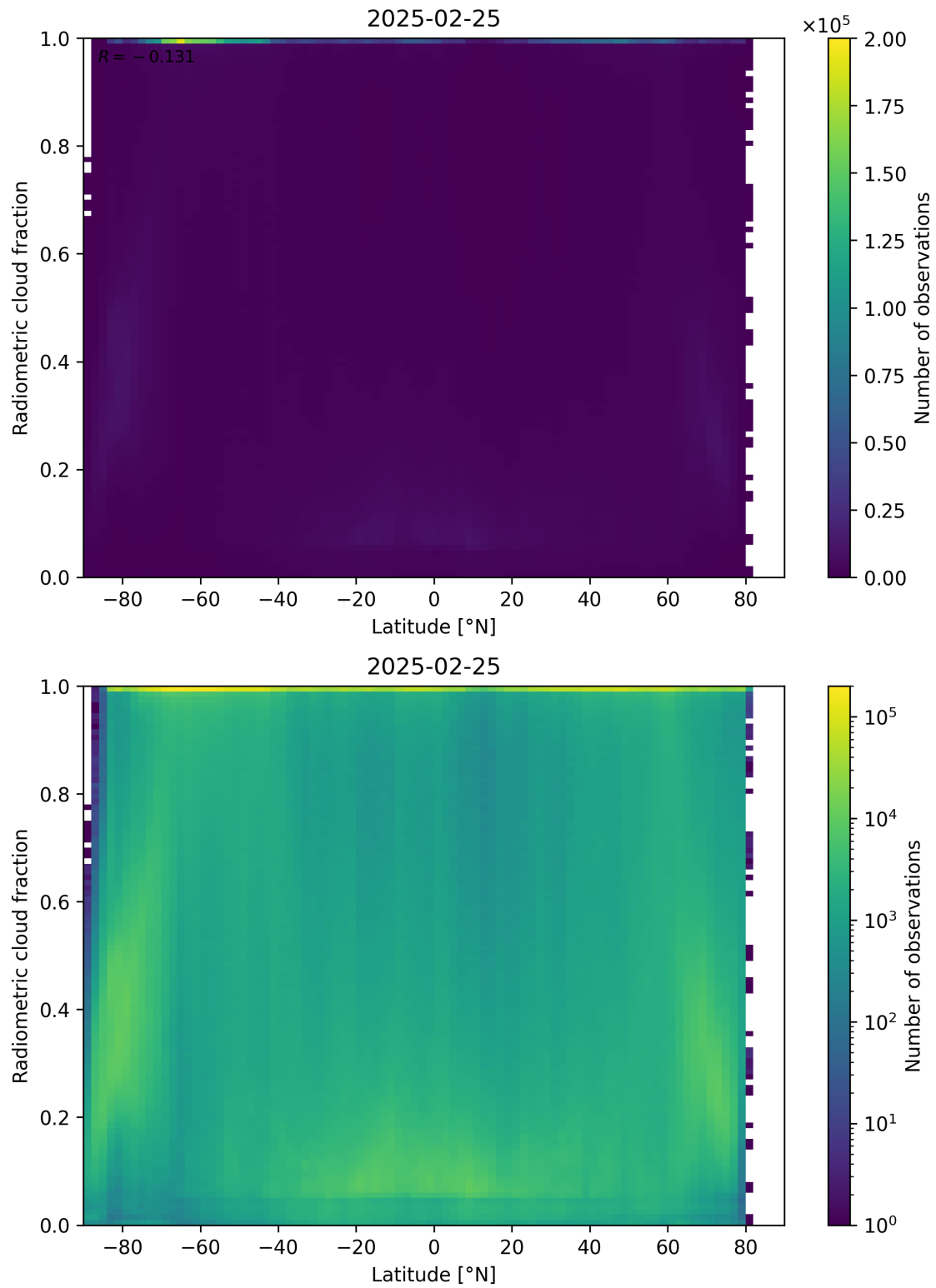
Figure 92: Scatter density plot of “Latitude” against “Radiometric cloud fraction” for 2025-02-24 to 2025-02-26.
