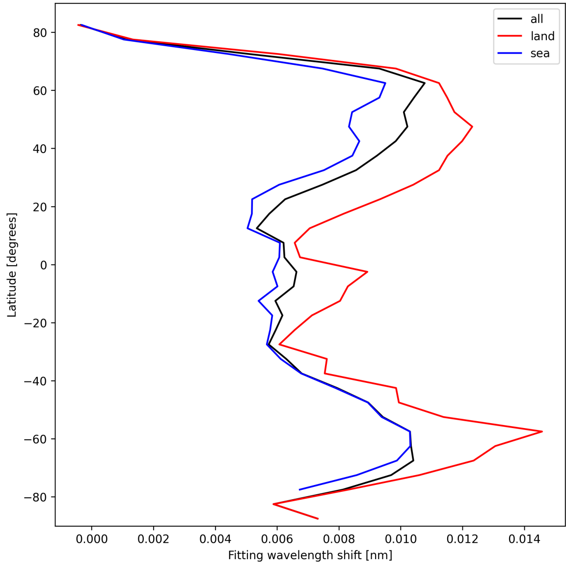
Figure 33: Zonal average of “Fitting wavelength shift” for 2025-02-24 to 2025-02-26.
