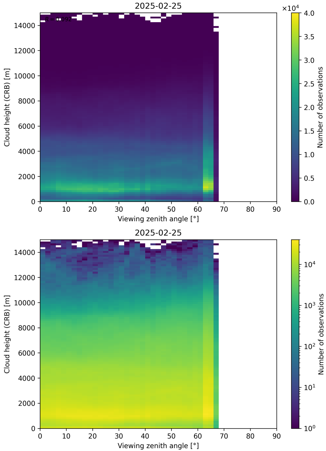
Figure 110: Scatter density plot of “Viewing zenith angle” against “Cloud height (CRB)” for 2025-02-24 to 2025-02-26.
