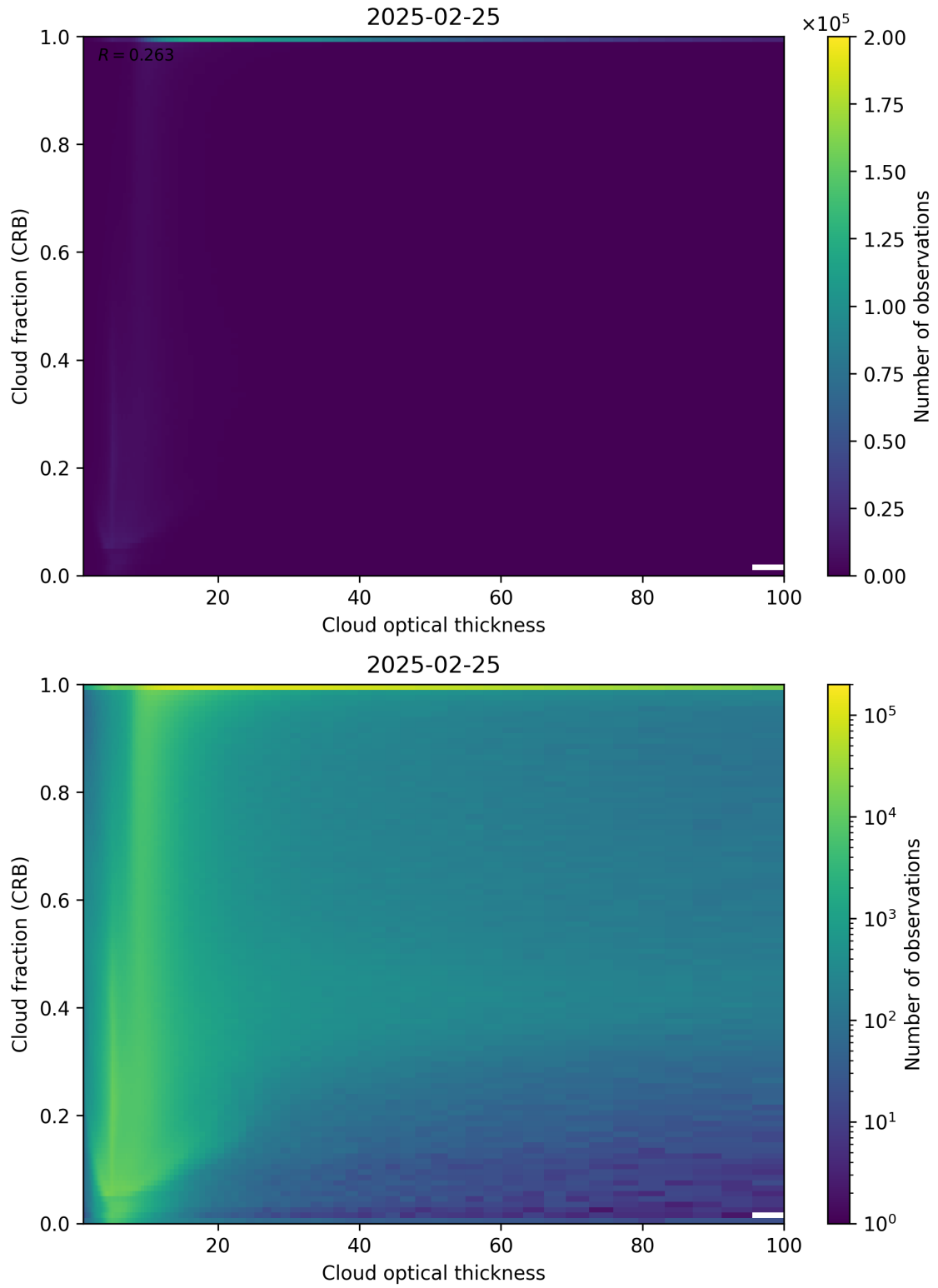
Figure 84: Scatter density plot of “Cloud optical thickness” against “Cloud fraction (CRB)” for 2025-02-24 to 2025-02-26.
