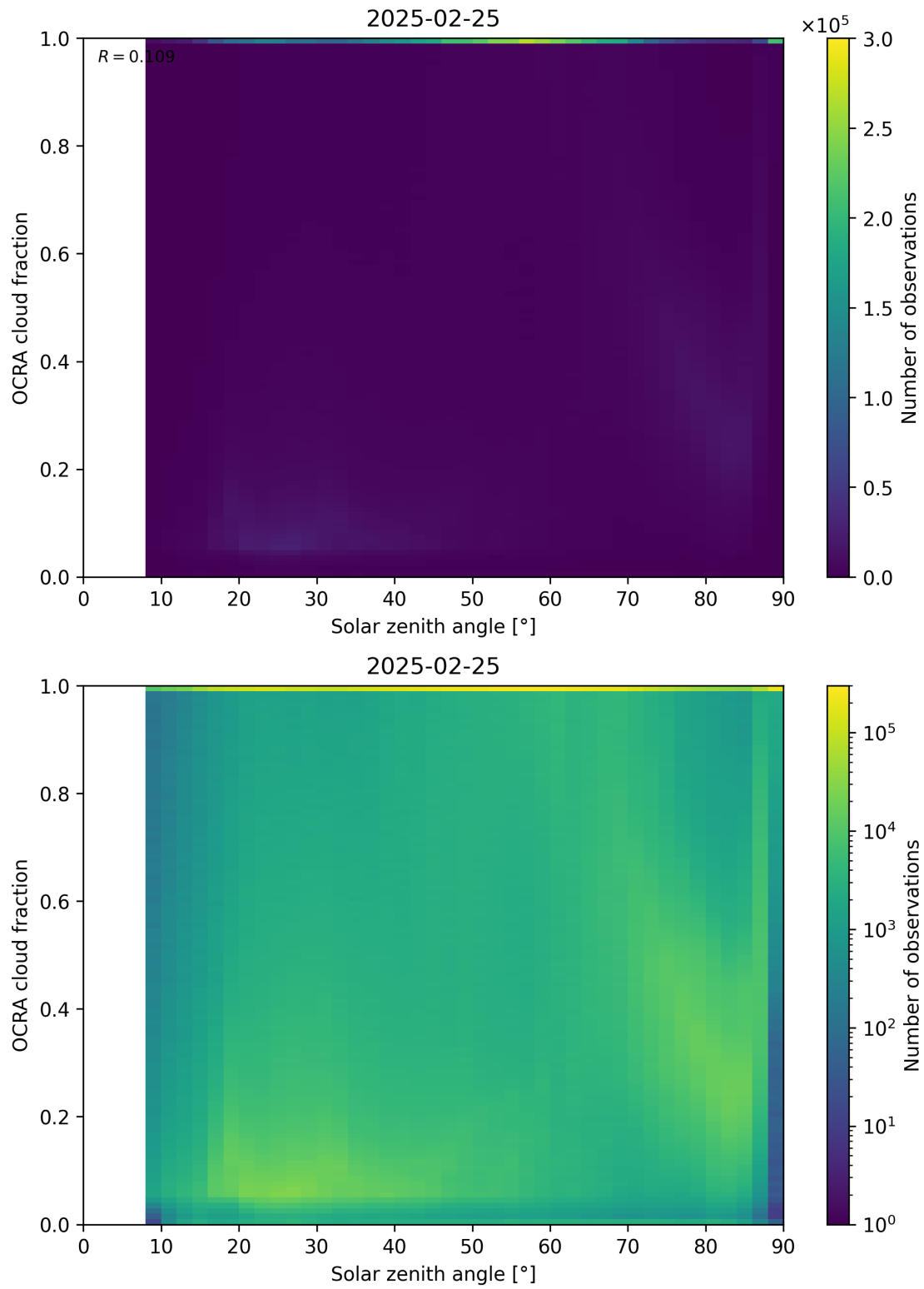
Figure 100: Scatter density plot of “Solar zenith angle” against “OCRA cloud fraction” for 2025-02-24 to 2025-02-26.
