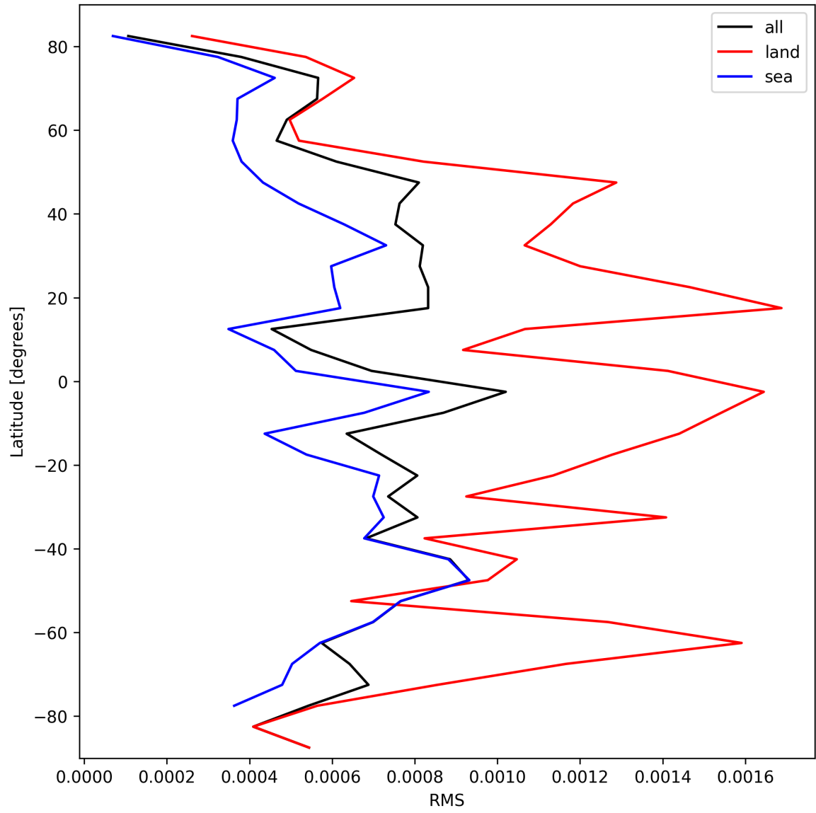
Figure 31: Zonal average of “RMS” for 2025-02-24 to 2025-02-26.
