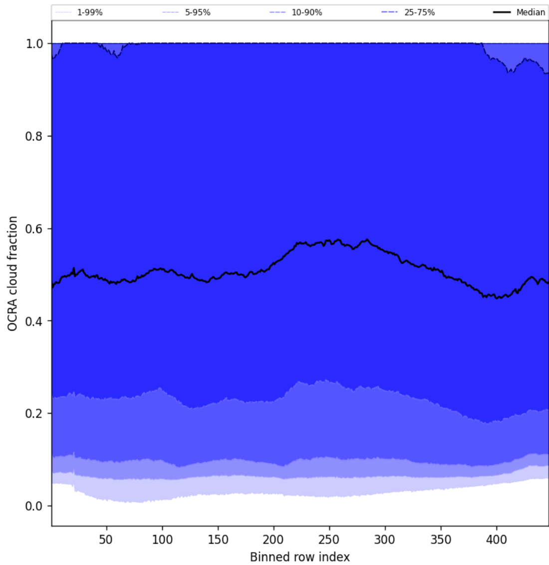
Figure 66: Along track statistics of “OCRA cloud fraction” for 2025-02-24 to 2025-02-26
