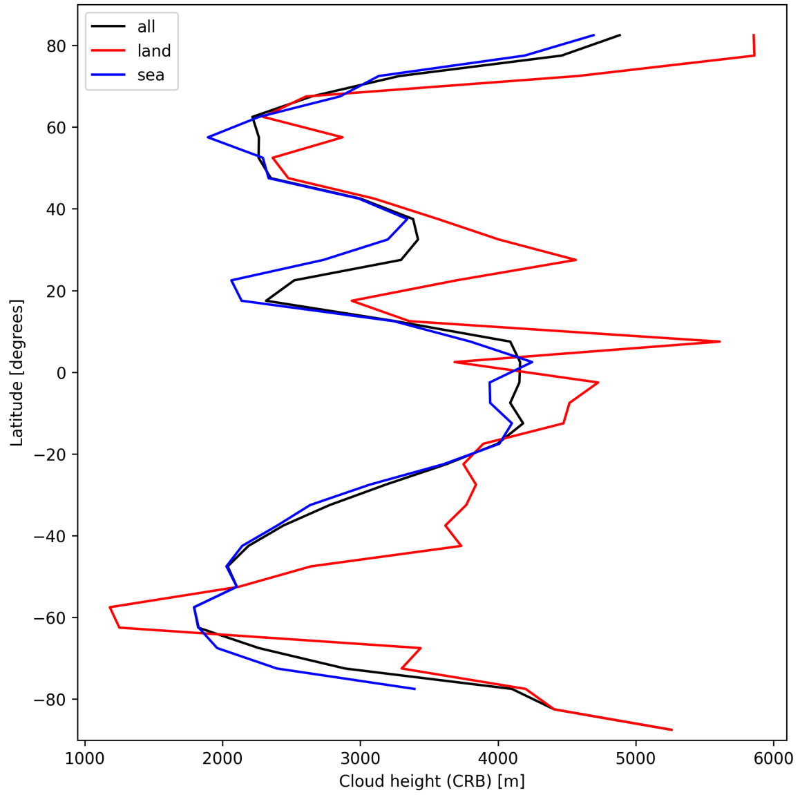
Figure 27: Zonal average of “Cloud height (CRB)” for 2025-02-24 to 2025-02-26.
