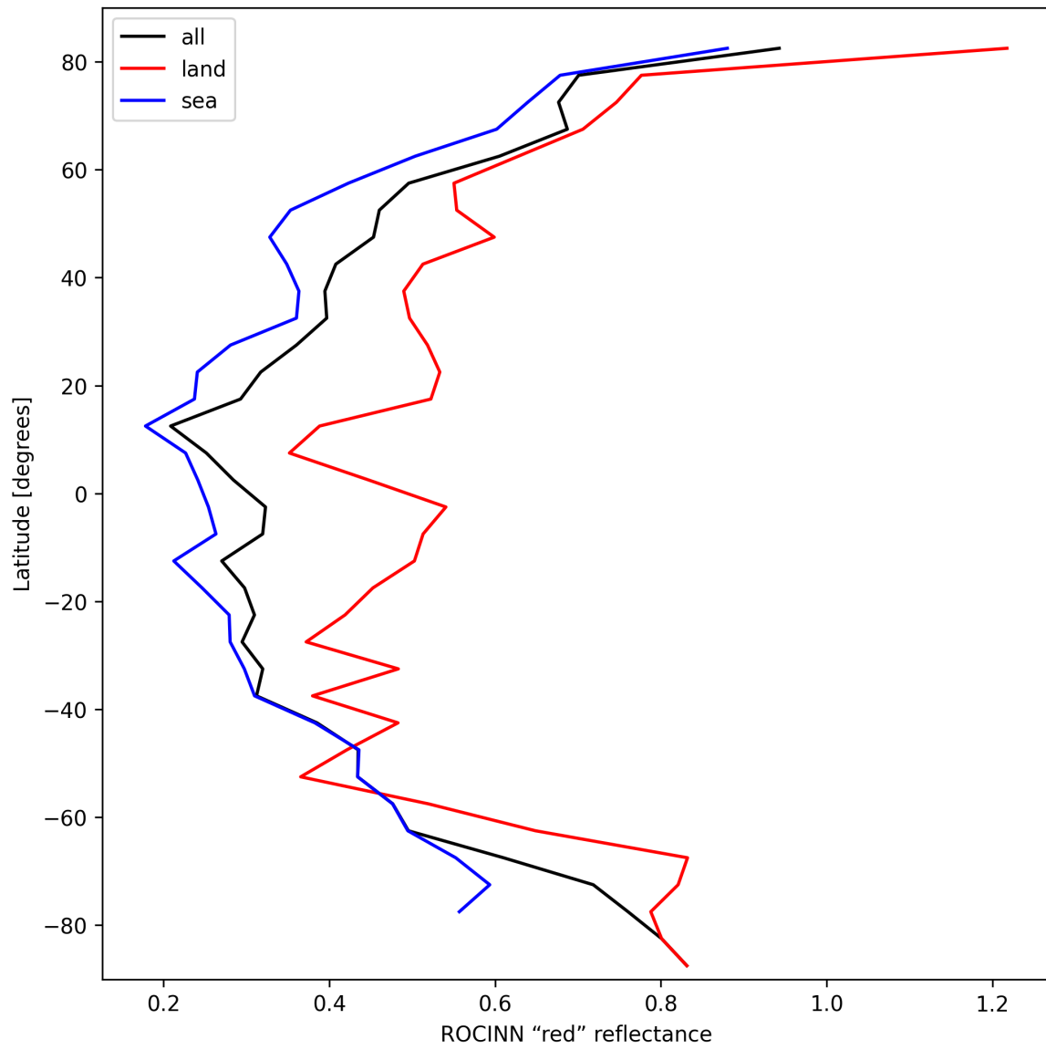
Figure 37: Zonal average of “ROCINN “red” reflectance” for 2025-02-24 to 2025-02-26.
