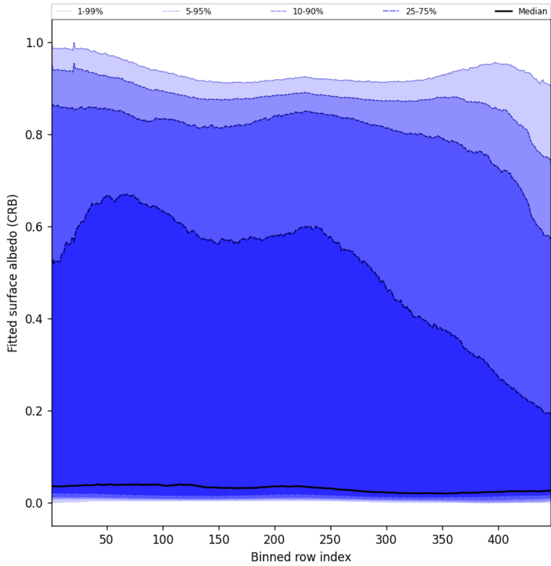
Figure 62: Along track statistics of “Fitted surface albedo (CRB)” for 2025-02-24 to 2025-02-26
