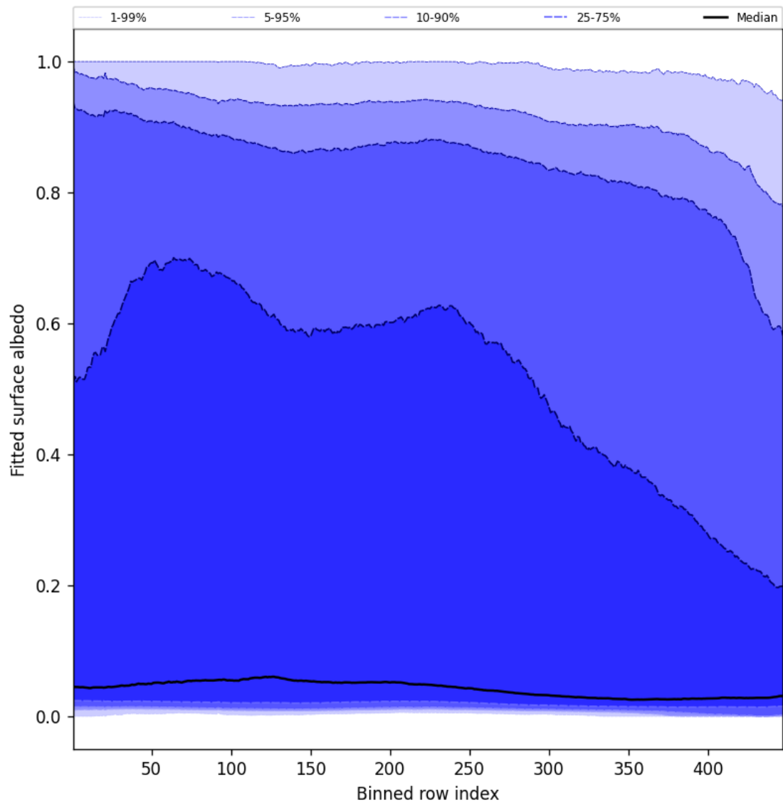
Figure 61: Along track statistics of “Fitted surface albedo” for 2025-02-24 to 2025-02-26
