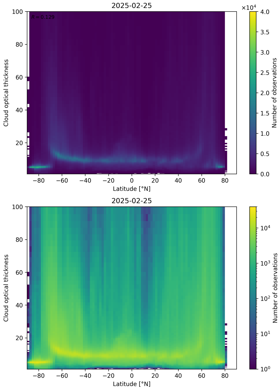
Figure 96: Scatter density plot of “Latitude” against “Cloud optical thickness” for 2025-02-24 to 2025-02-26.
