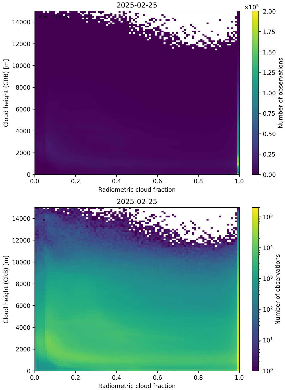
Figure 74: Scatter density plot of “Radiometric cloud fraction” against “Cloud height (CRB)” for 2025-02-24 to 2025-02-26.
