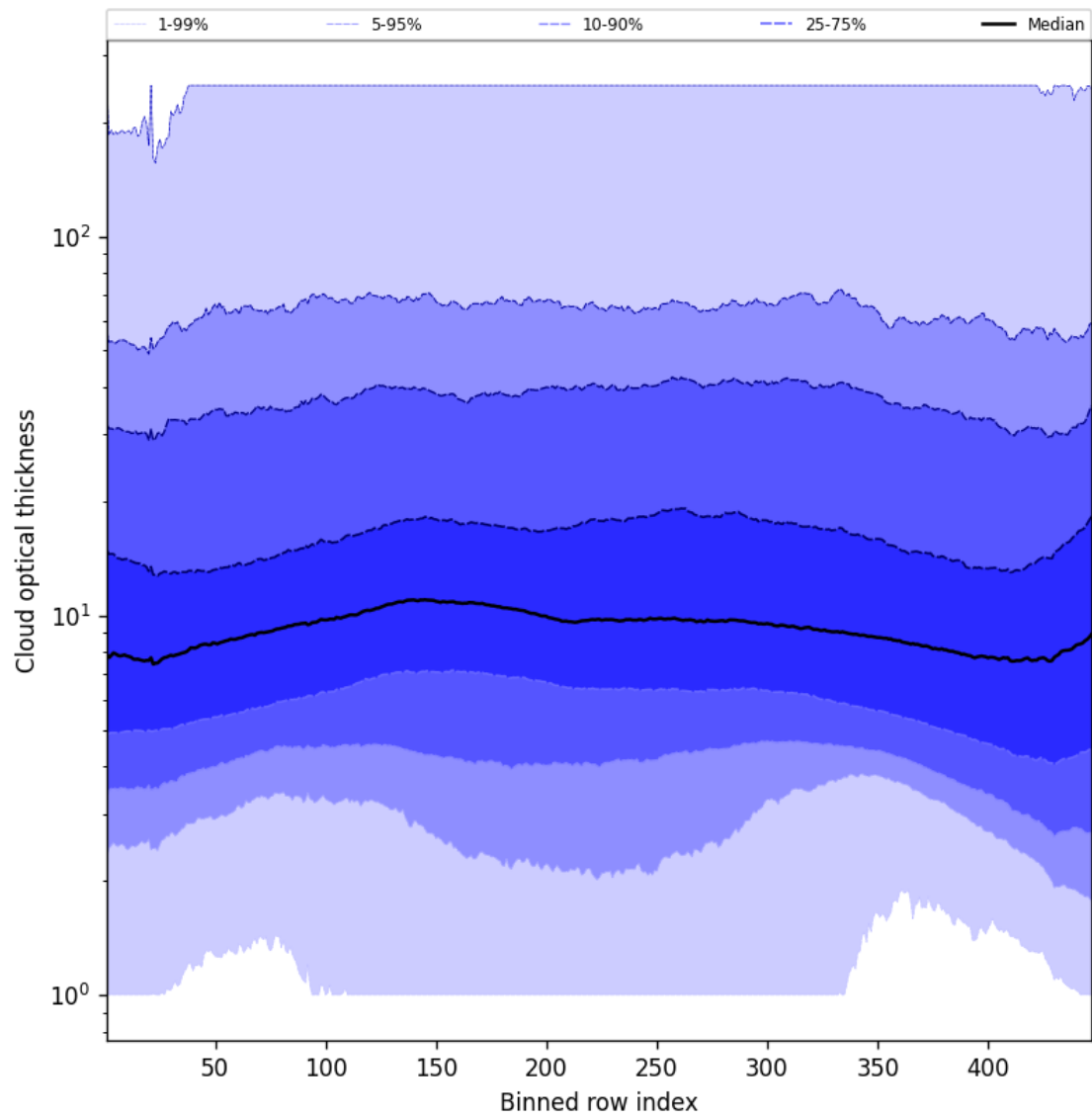
Figure 57: Along track statistics of “Cloud optical thickness” for 2025-02-24 to 2025-02-26
