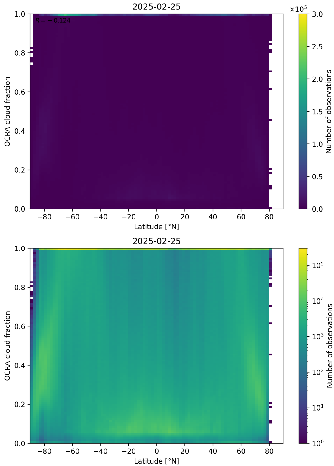
Figure 93: Scatter density plot of “Latitude” against “OCRA cloud fraction” for 2025-02-24 to 2025-02-26.
