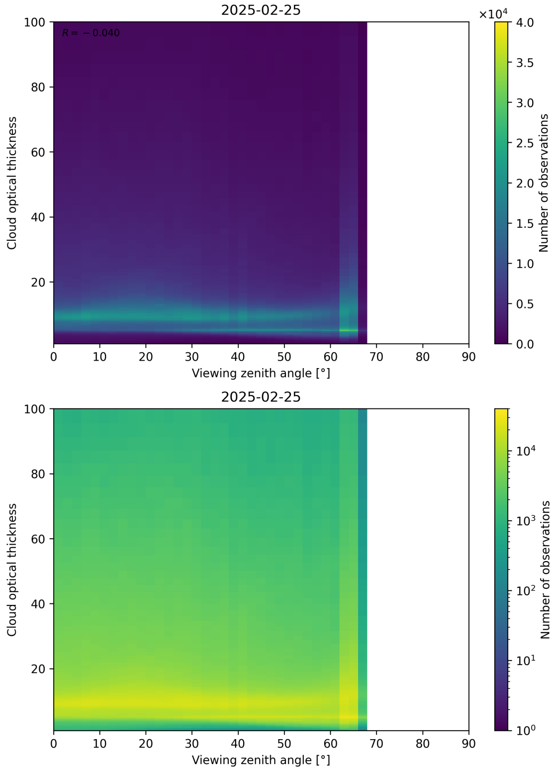
Figure 111: Scatter density plot of “Viewing zenith angle” against “Cloud optical thickness” for 2025-02-24 to 2025-02-26.
