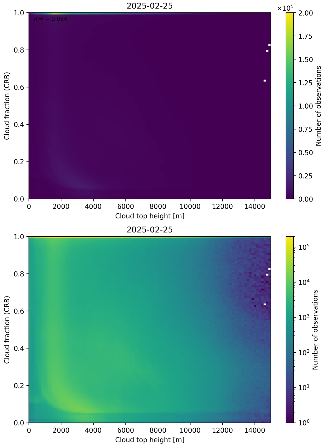
Figure 88: Scatter density plot of “Cloud top height” against “Cloud fraction (CRB)” for 2025-02-24 to 2025-02-26.
