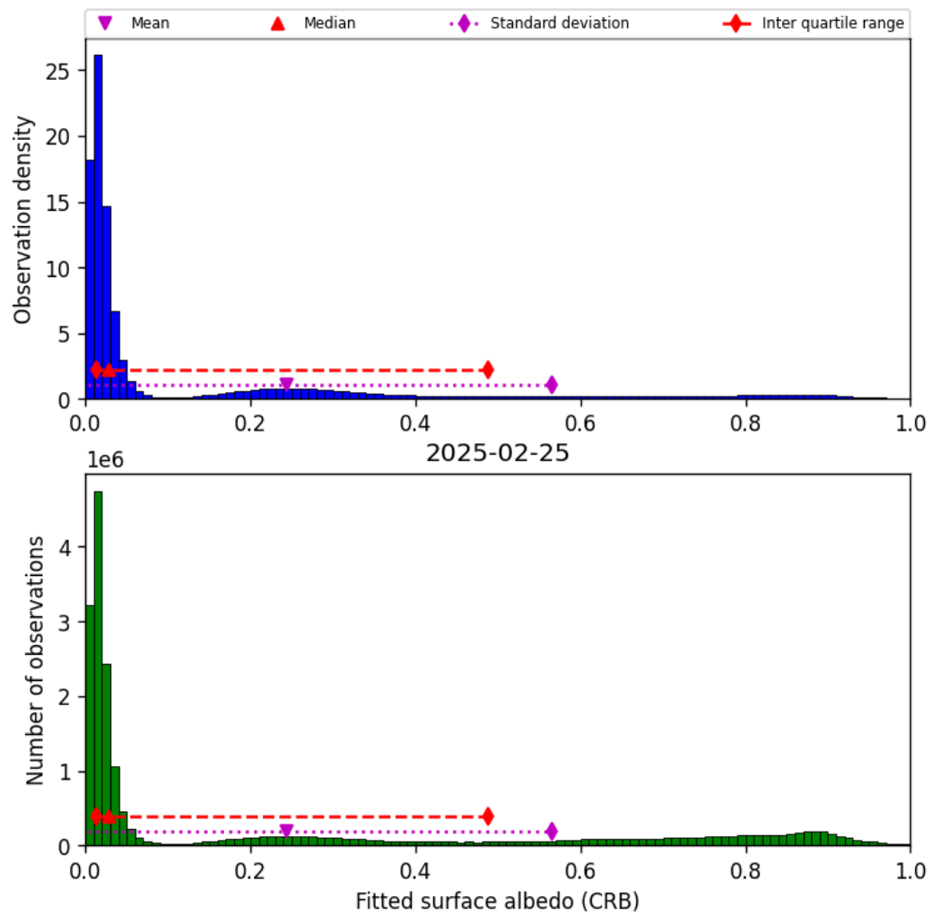
Figure 46: Histogram of “Fitted surface albedo (CRB)” for 2025-02-24 to 2025-02-26
