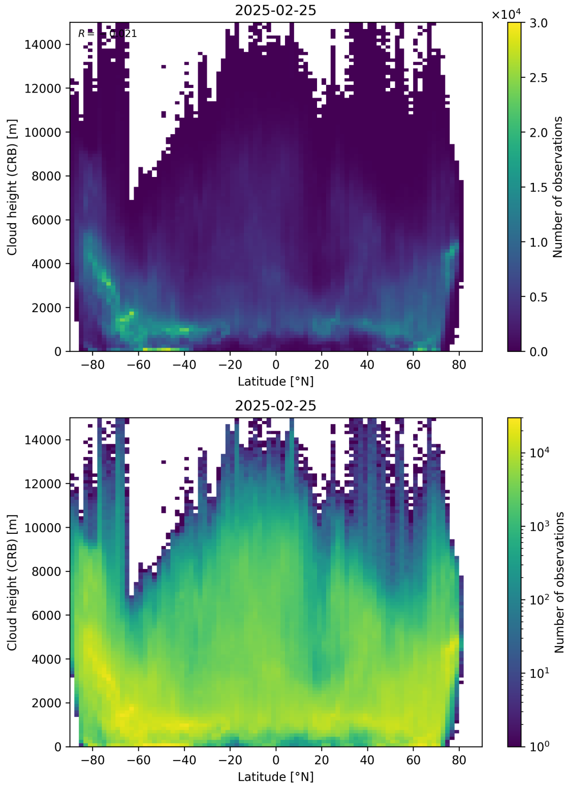
Figure 95: Scatter density plot of “Latitude” against “Cloud height (CRB)” for 2025-02-24 to 2025-02-26.
