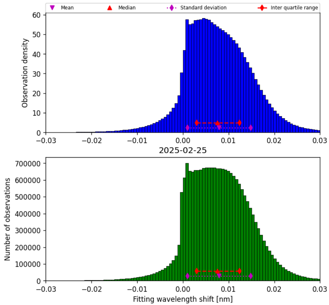
Figure 49: Histogram of “Fitting wavelength shift” for 2025-02-24 to 2025-02-26
