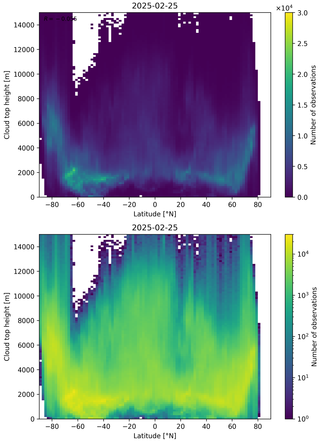
Figure 97: Scatter density plot of “Latitude” against “Cloud top height” for 2025-02-24 to 2025-02-26.
