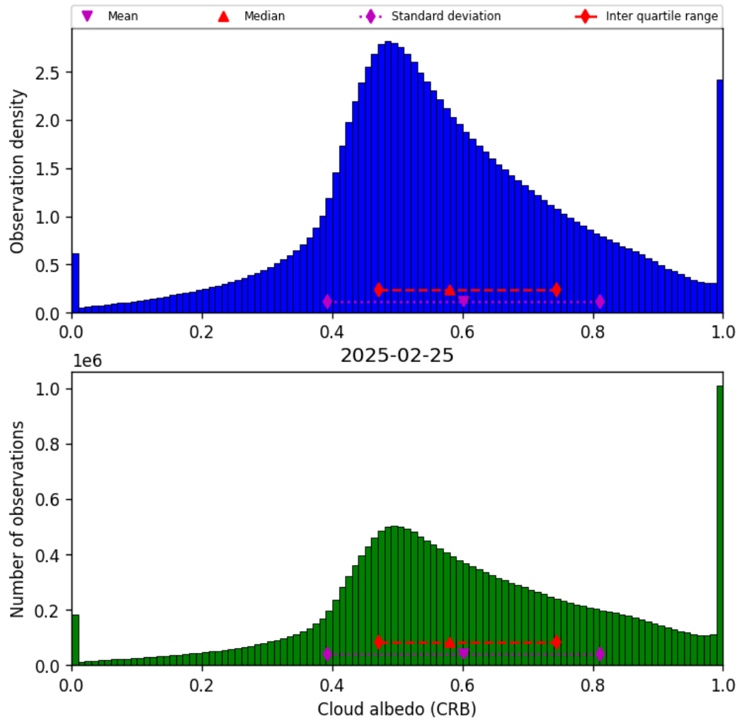
Figure 44: Histogram of “Cloud albedo (CRB)” for 2025-02-24 to 2025-02-26
