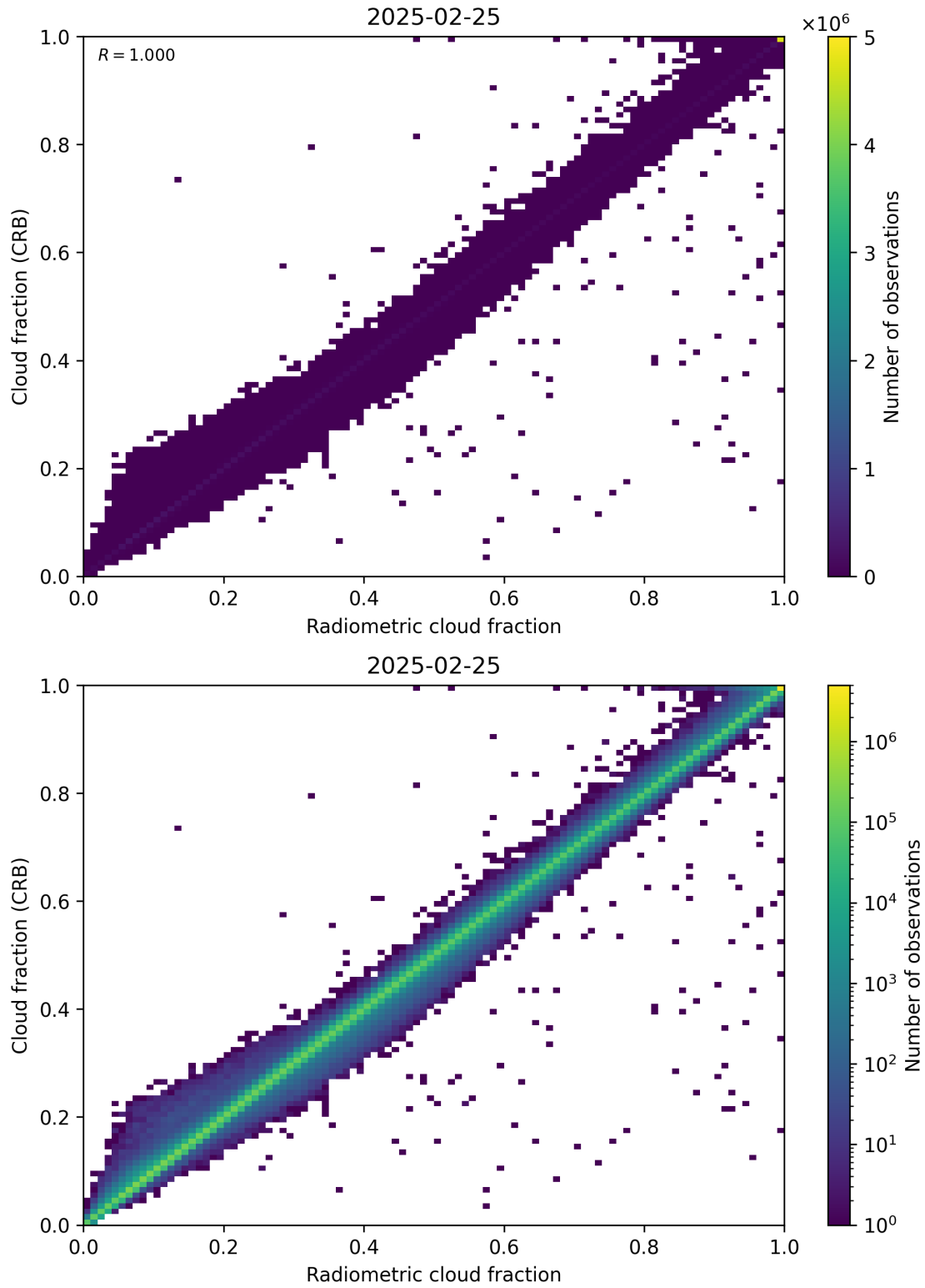
Figure 73: Scatter density plot of “Radiometric cloud fraction” against “Cloud fraction (CRB)” for 2025-02-24 to 2025-02-26.
