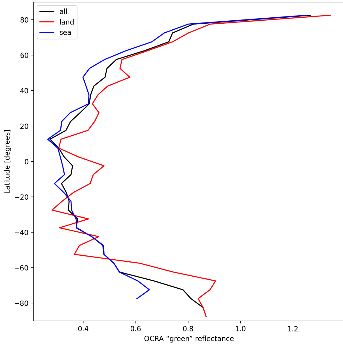
Figure 36: Zonal average of “OCRA “green” reflectance” for 2025-02-24 to 2025-02-26.
