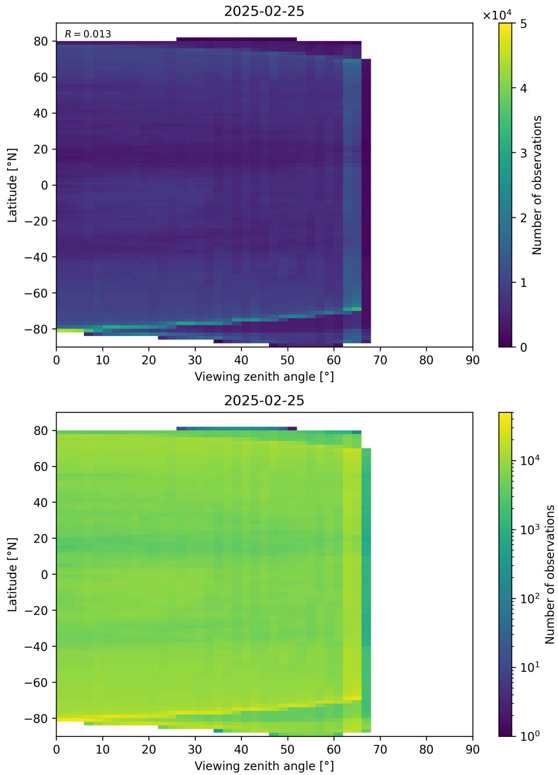
Figure 113: Scatter density plot of “Viewing zenith angle” against “Latitude” for 2025-02-24 to 2025-02-26.
