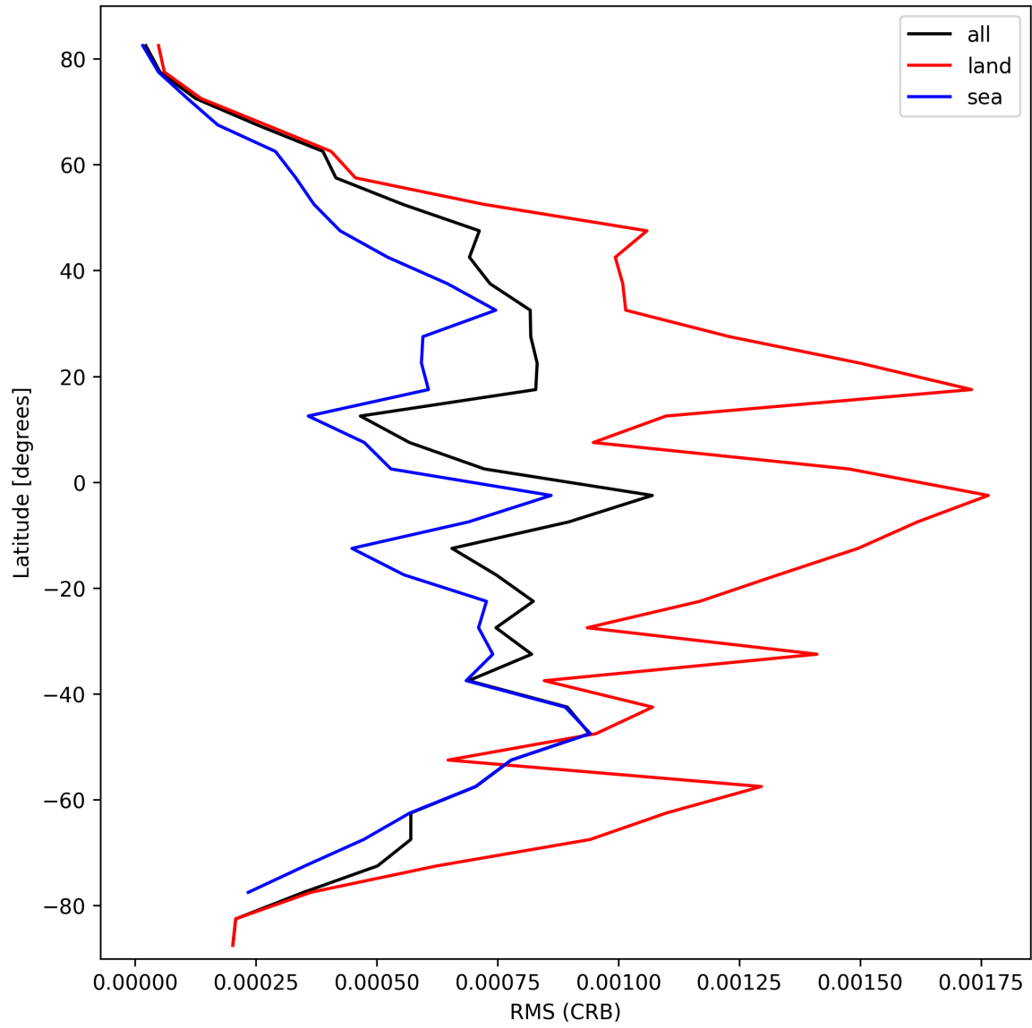
Figure 32: Zonal average of “RMS (CRB)” for 2025-02-24 to 2025-02-26.
