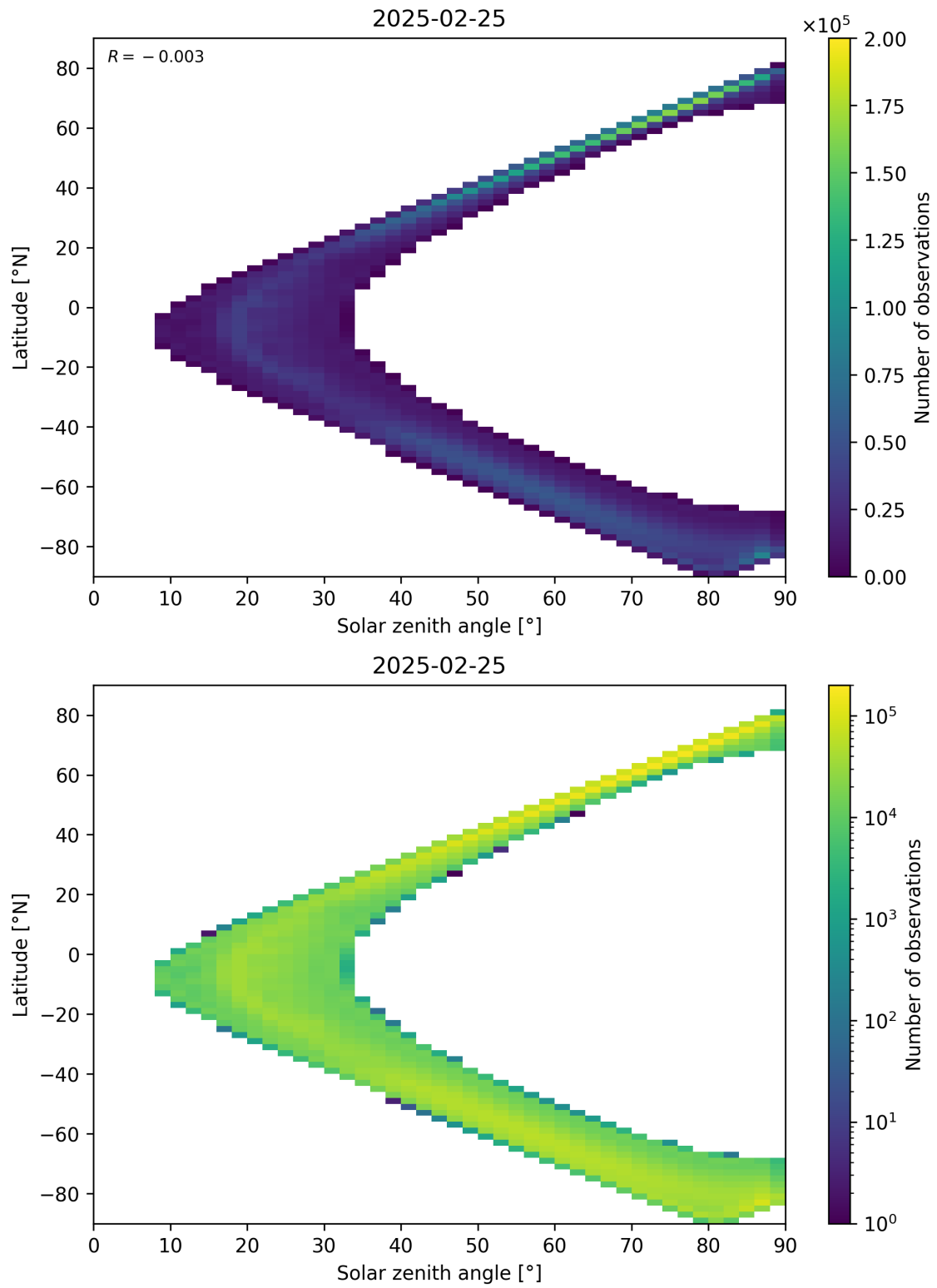
Figure 105: Scatter density plot of “Solar zenith angle” against “Latitude” for 2025-02-24 to 2025-02-26.
