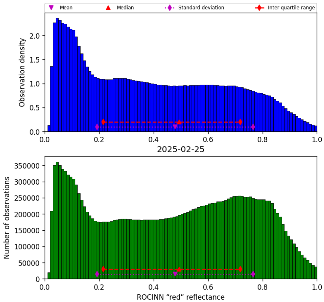
Figure 53: Histogram of “ROCINN “red” reflectance” for 2025-02-24 to 2025-02-26
