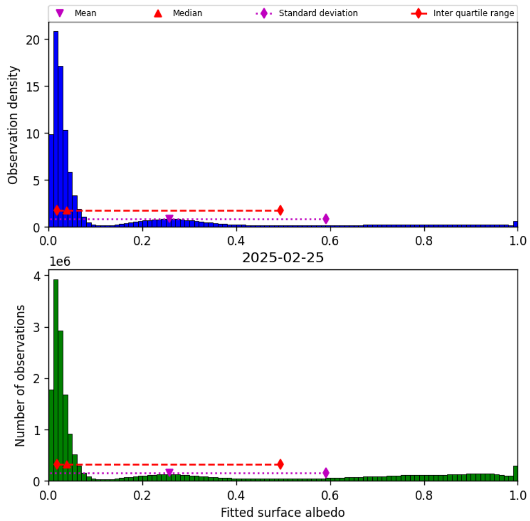
Figure 45: Histogram of “Fitted surface albedo” for 2025-02-24 to 2025-02-26
