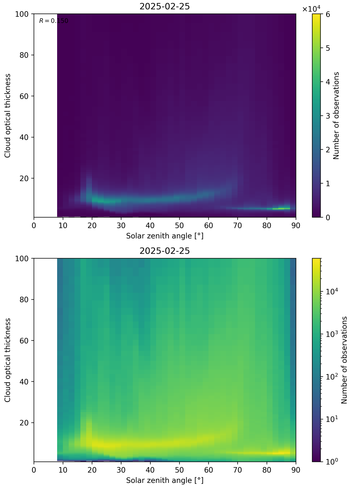
Figure 103: Scatter density plot of “Solar zenith angle” against “Cloud optical thickness” for 2025-02-24 to 2025-02-26.
