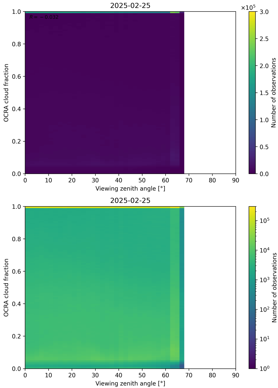
Figure 108: Scatter density plot of “Viewing zenith angle” against “OCRA cloud fraction” for 2025-02-24 to 2025-02-26.
