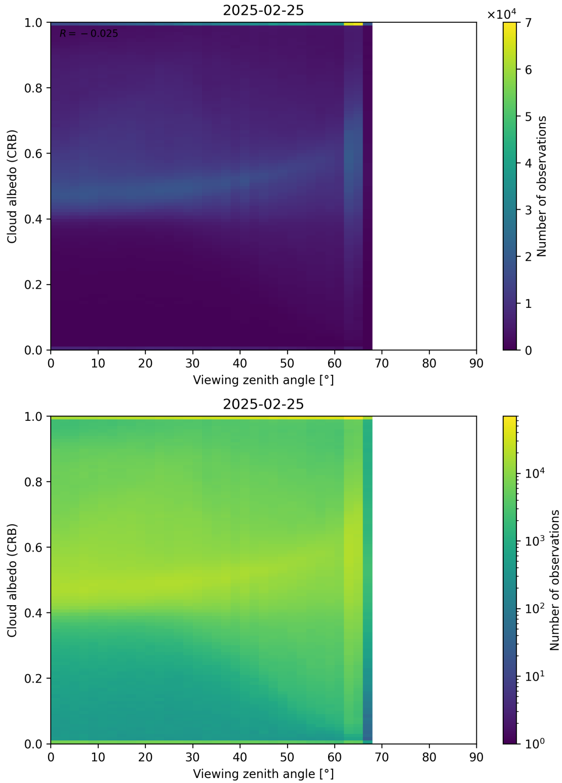
Figure 106: Scatter density plot of “Viewing zenith angle” against “Cloud albedo (CRB)” for 2025-02-24 to 2025-02-26.
