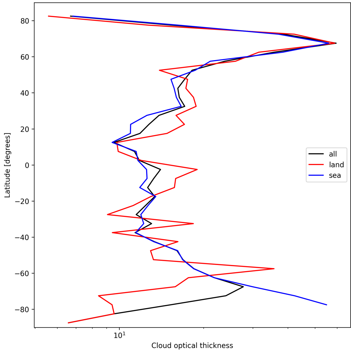
Figure 25: Zonal average of “Cloud optical thickness” for 2025-02-24 to 2025-02-26.
