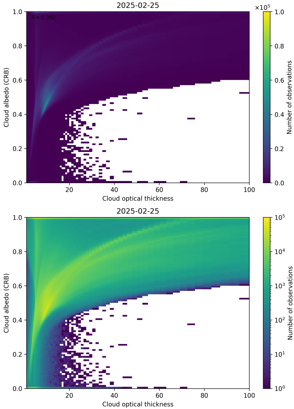
Figure 82: Scatter density plot of “Cloud optical thickness” against “Cloud albedo (CRB)” for 2025-02-24 to 2025-02-26.
