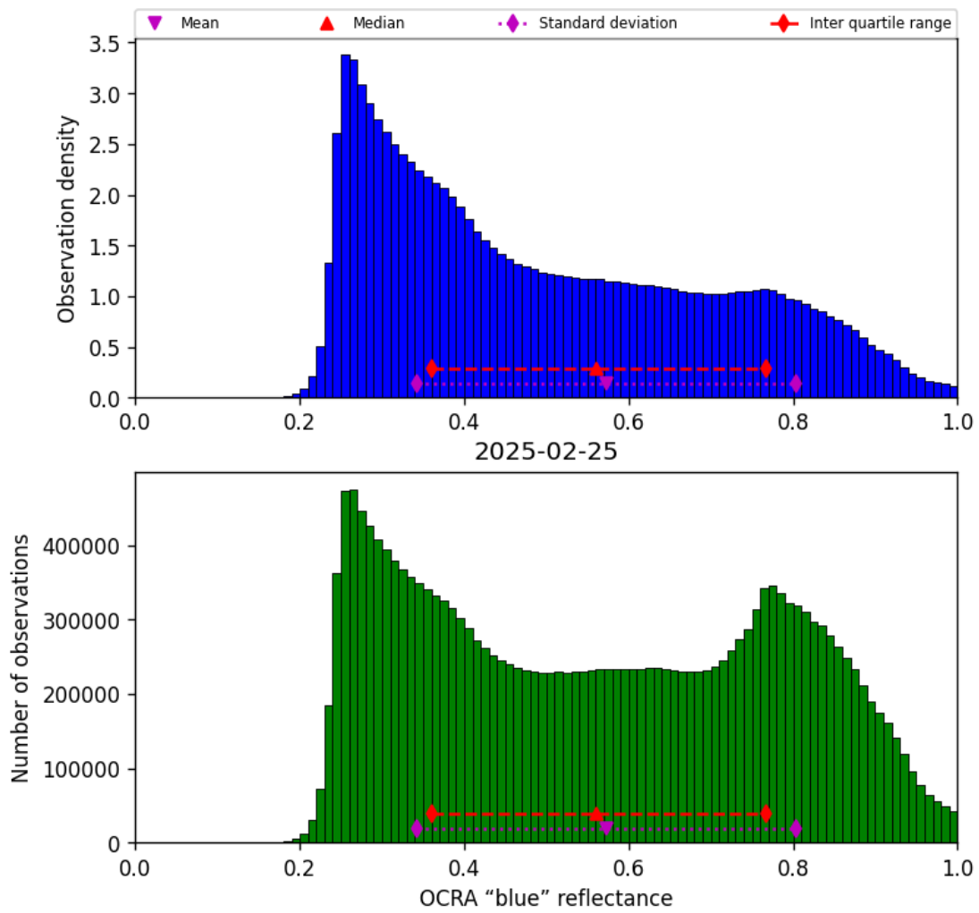
Figure 51: Histogram of “OCRA “blue” reflectance” for 2025-02-24 to 2025-02-26
