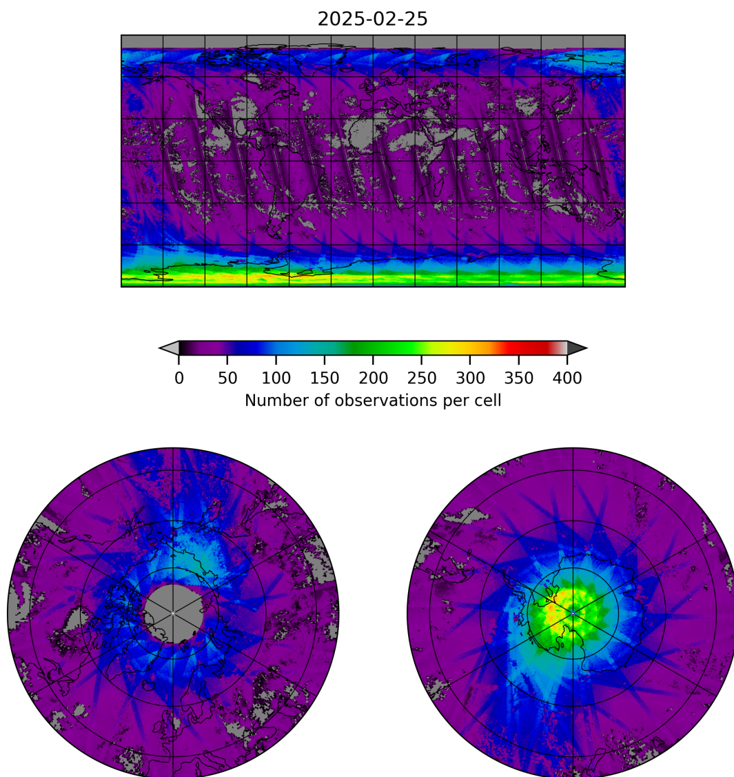
Figure 21: Map of the number of observations for 2025-02-24 to 2025-02-26
