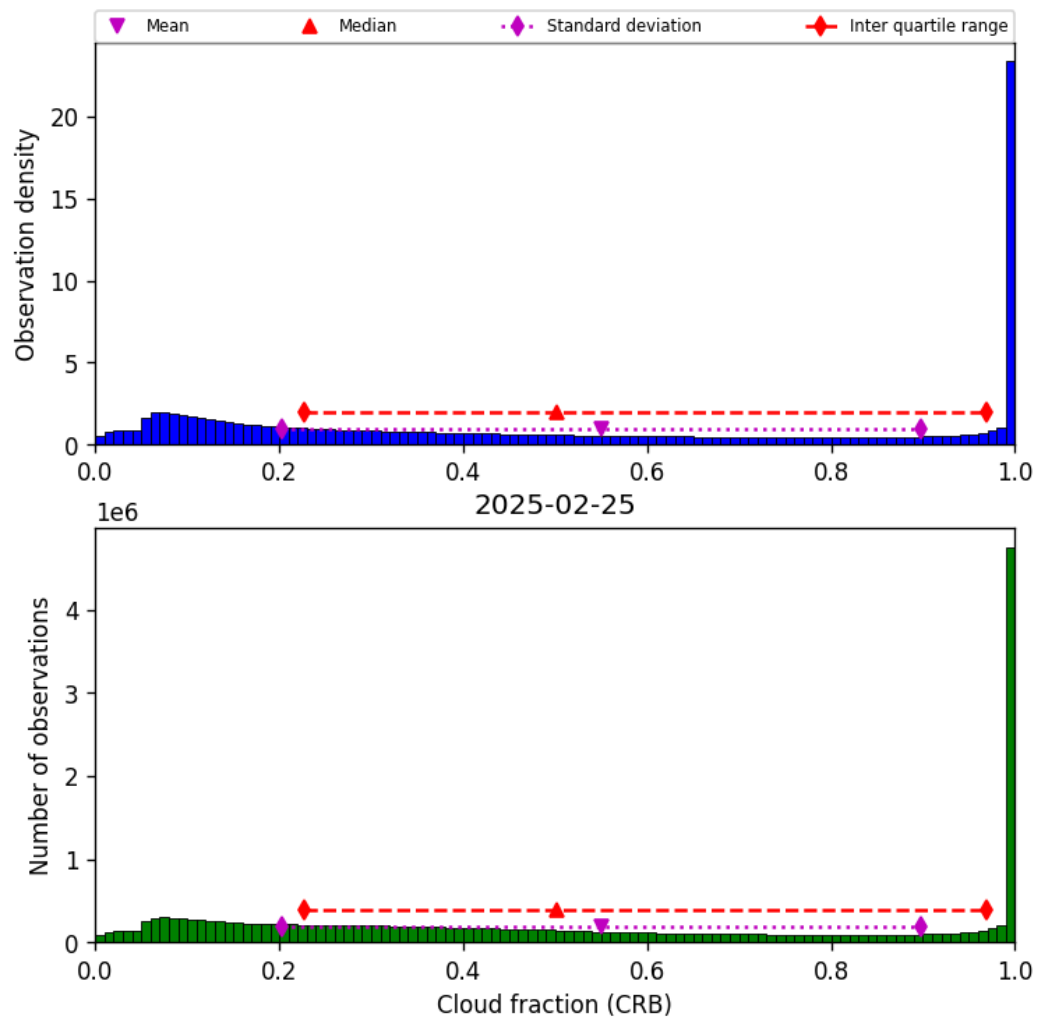
Figure 42: Histogram of “Cloud fraction (CRB)” for 2025-02-24 to 2025-02-26
