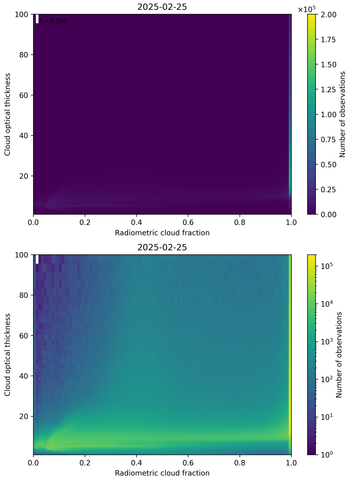
Figure 75: Scatter density plot of “Radiometric cloud fraction” against “Cloud optical thickness” for 2025-02-24 to 2025-02-26.
