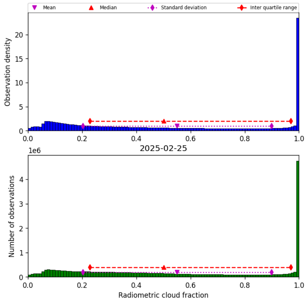
Figure 39: Histogram of "Radiometric cloud fraction" for 2025-02-24 to 2025-02-26
