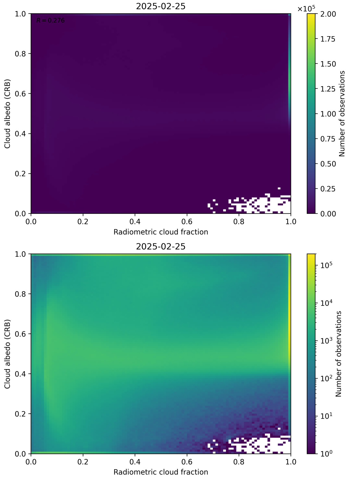
Figure 71: Scatter density plot of “Radiometric cloud fraction” against “Cloud albedo (CRB)” for 2025-02-24 to 2025-02-26.
