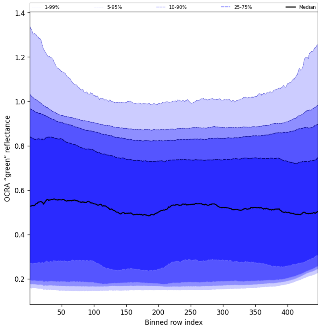
Figure 68: Along track statistics of "OCRA "green" reflectance" for 2025-02-24 to 2025-02-26
