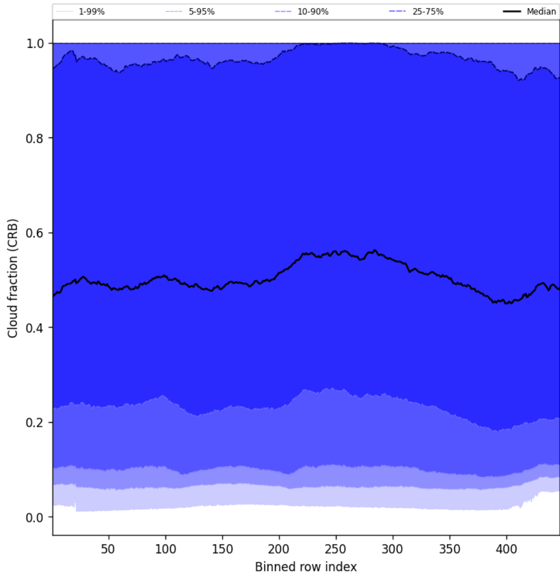
Figure 58: Along track statistics of “Cloud fraction (CRB)” for 2025-02-24 to 2025-02-26
