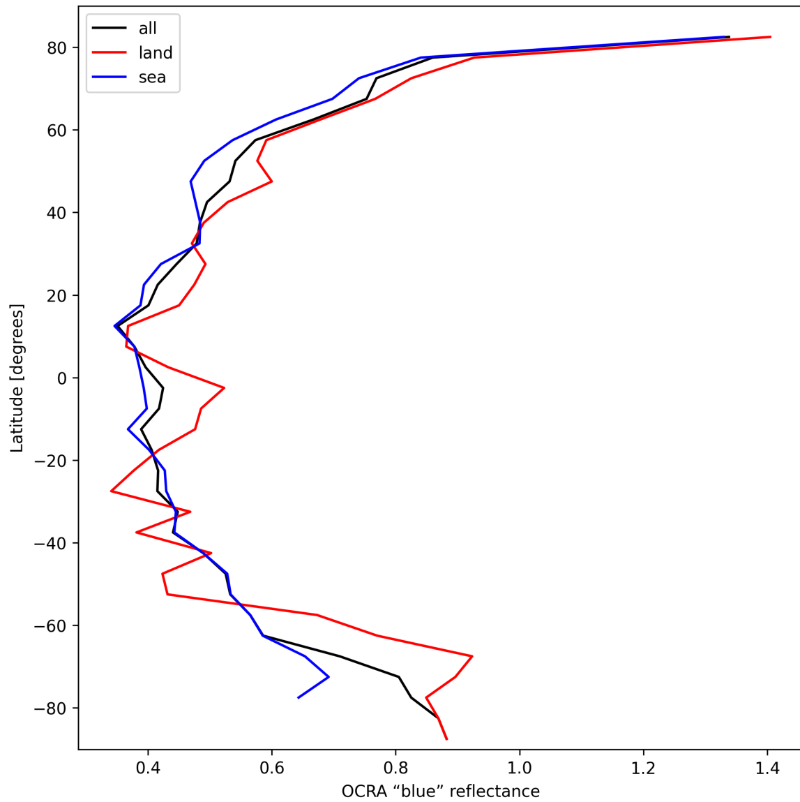
Figure 35: Zonal average of “OCRA “blue” reflectance” for 2025-02-24 to 2025-02-26.
