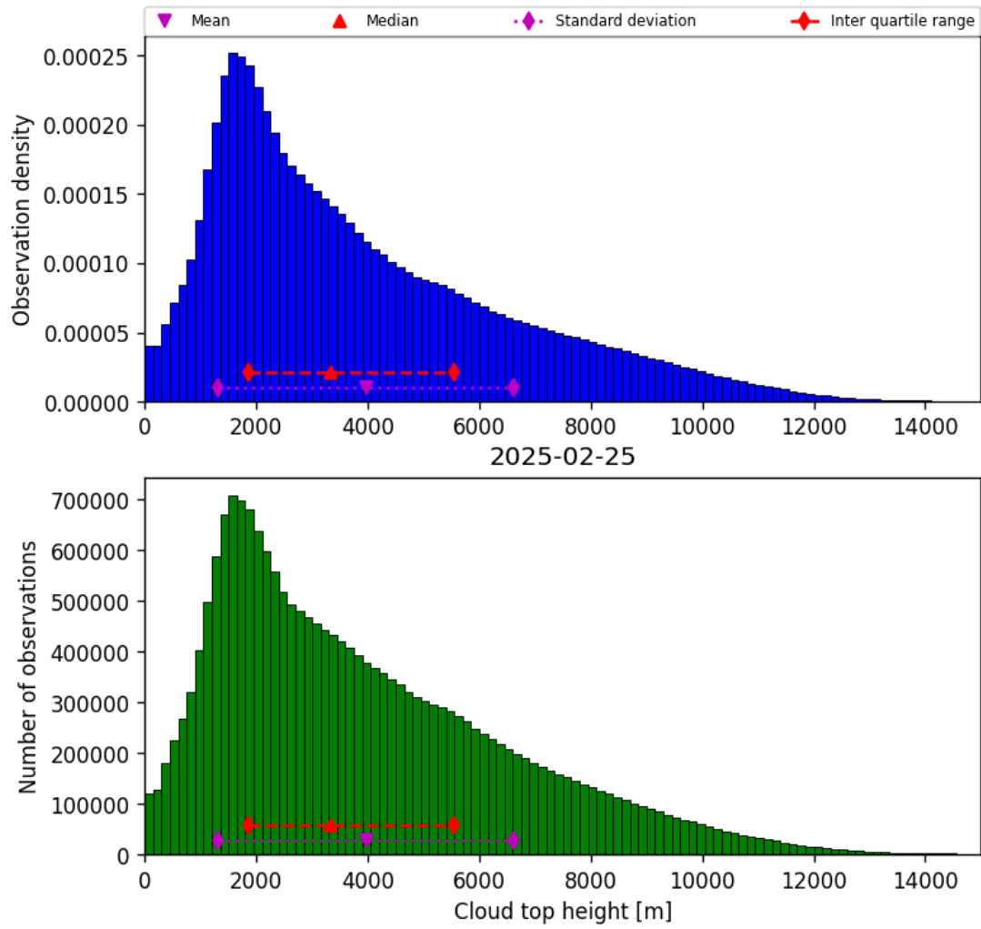
Figure 40: Histogram of “Cloud top height” for 2025-02-24 to 2025-02-26
