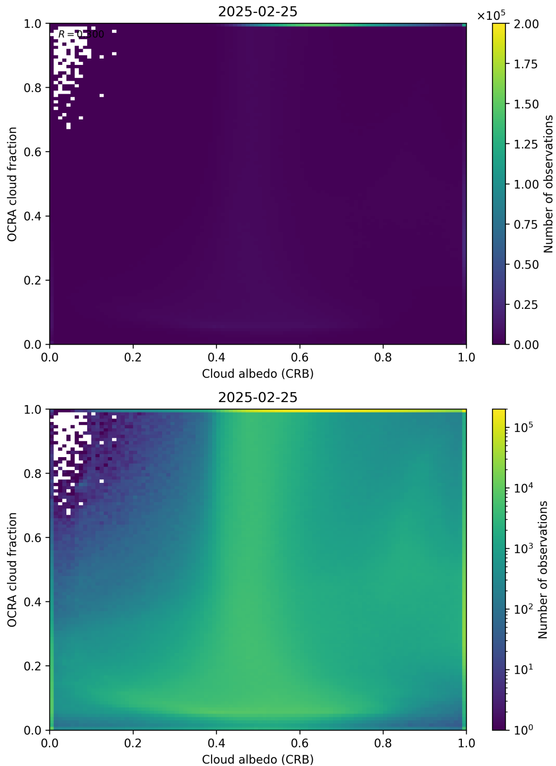
Figure 70: Scatter density plot of “Cloud albedo (CRB)” against “OCRA cloud fraction” for 2025-02-24 to 2025-02-26.
