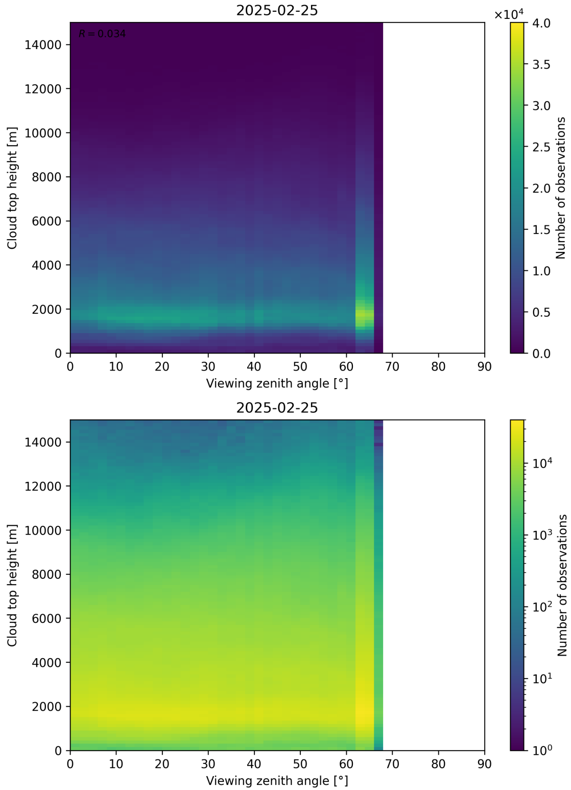
Figure 112: Scatter density plot of “Viewing zenith angle” against “Cloud top height” for 2025-02-24 to 2025-02-26.
