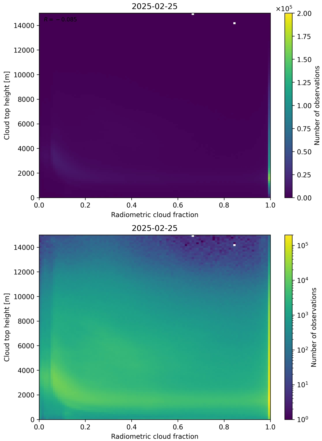
Figure 76: Scatter density plot of “Radiometric cloud fraction” against “Cloud top height” for 2025-02-24 to 2025-02-26.
