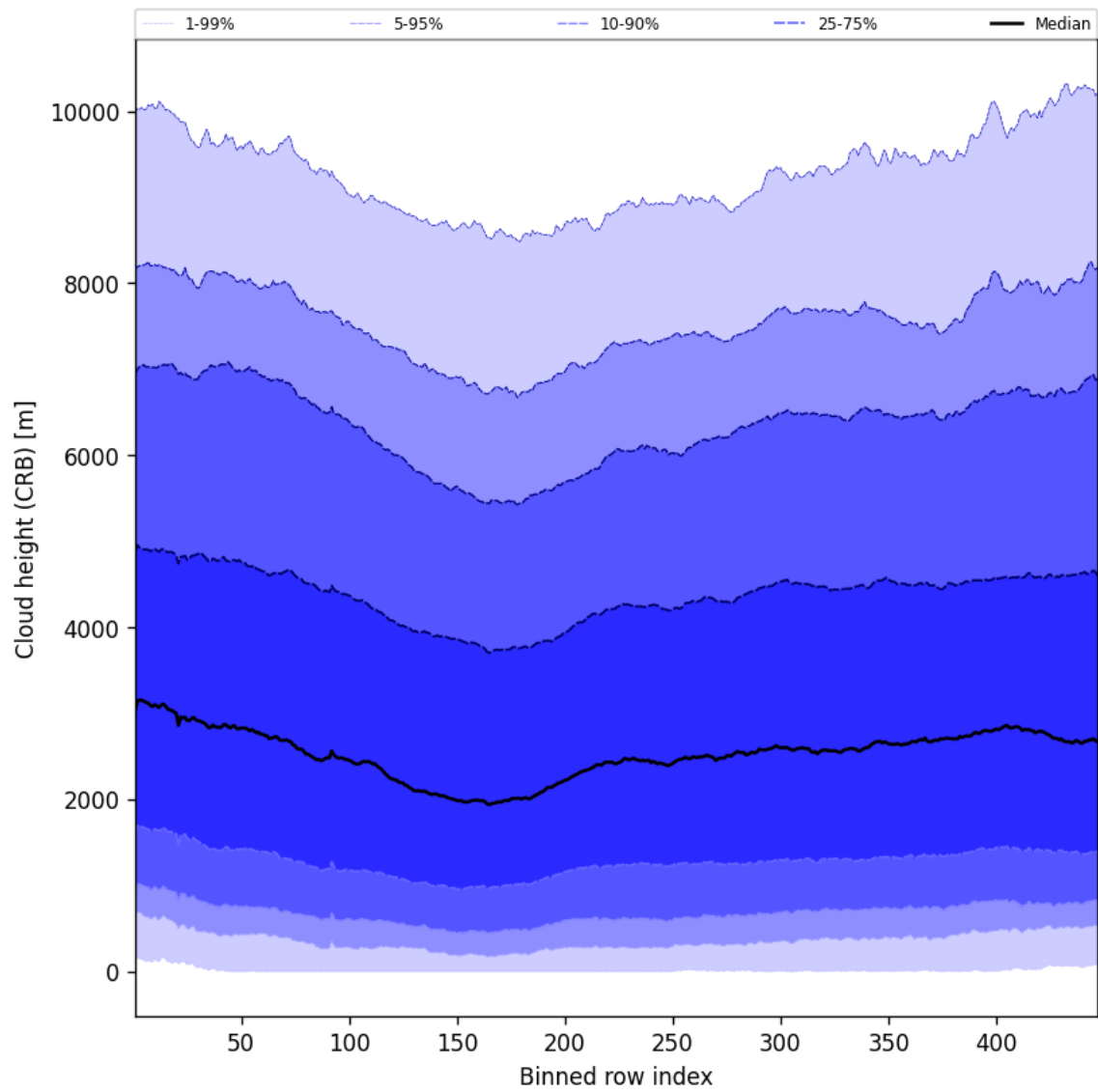
Figure 59: Along track statistics of “Cloud height (CRB)” for 2025-02-24 to 2025-02-26
