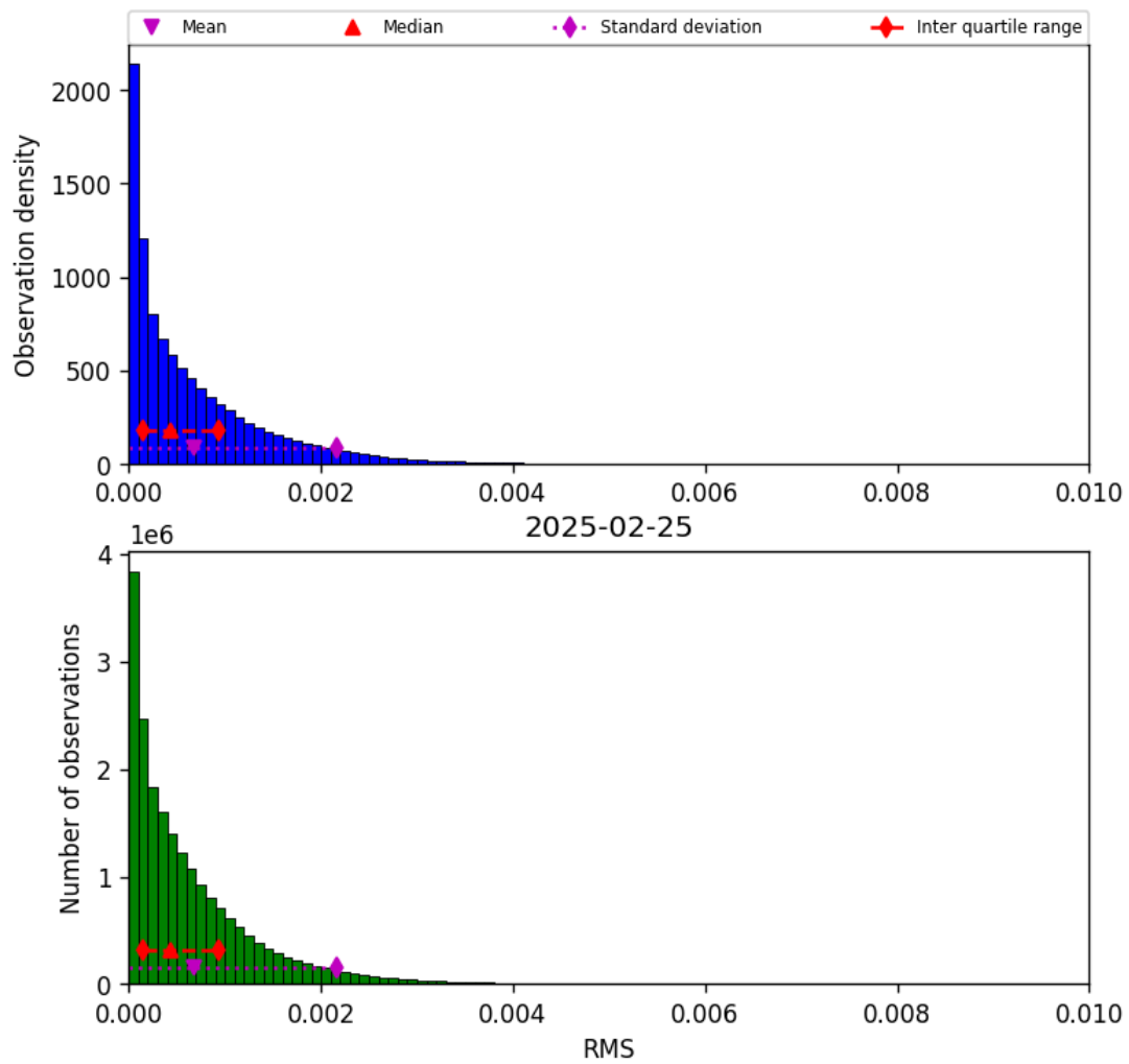
Figure 47: Histogram of “RMS” for 2025-02-24 to 2025-02-26
