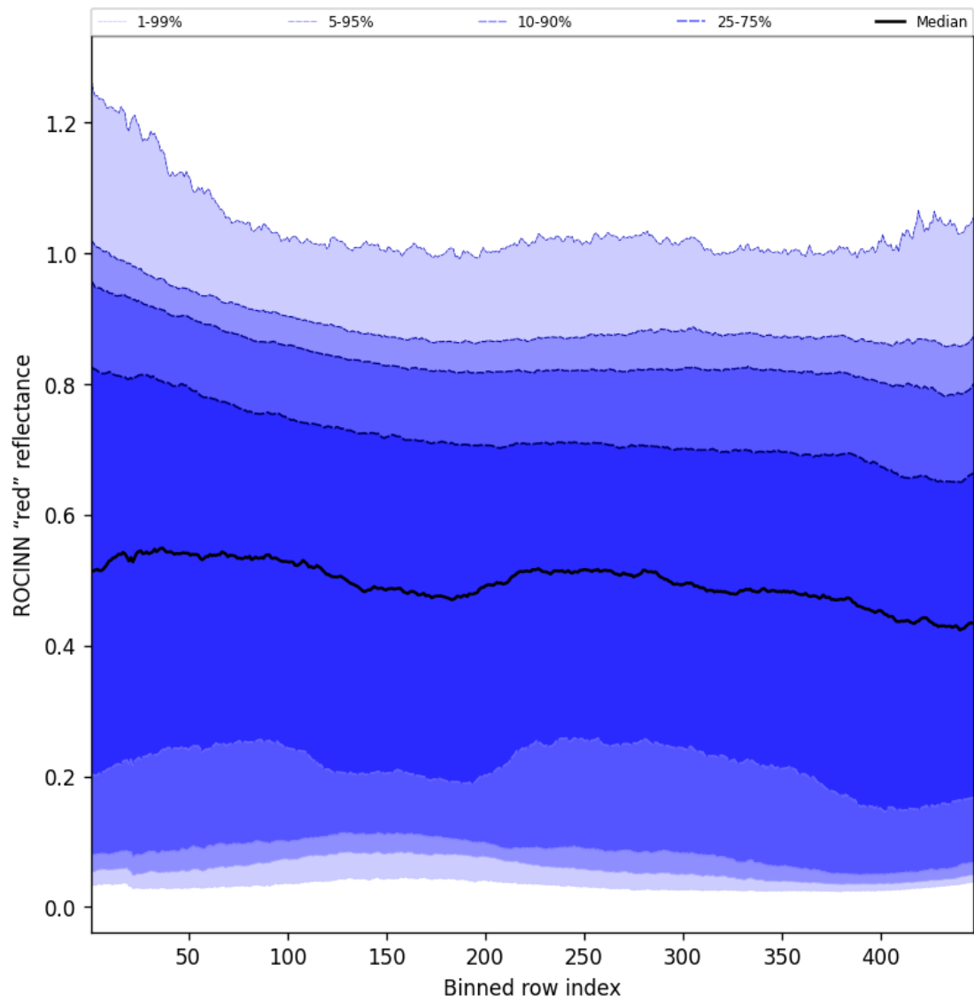
Figure 69: Along track statistics of “ROCINN “red” reflectance” for 2025-02-24 to 2025-02-26
