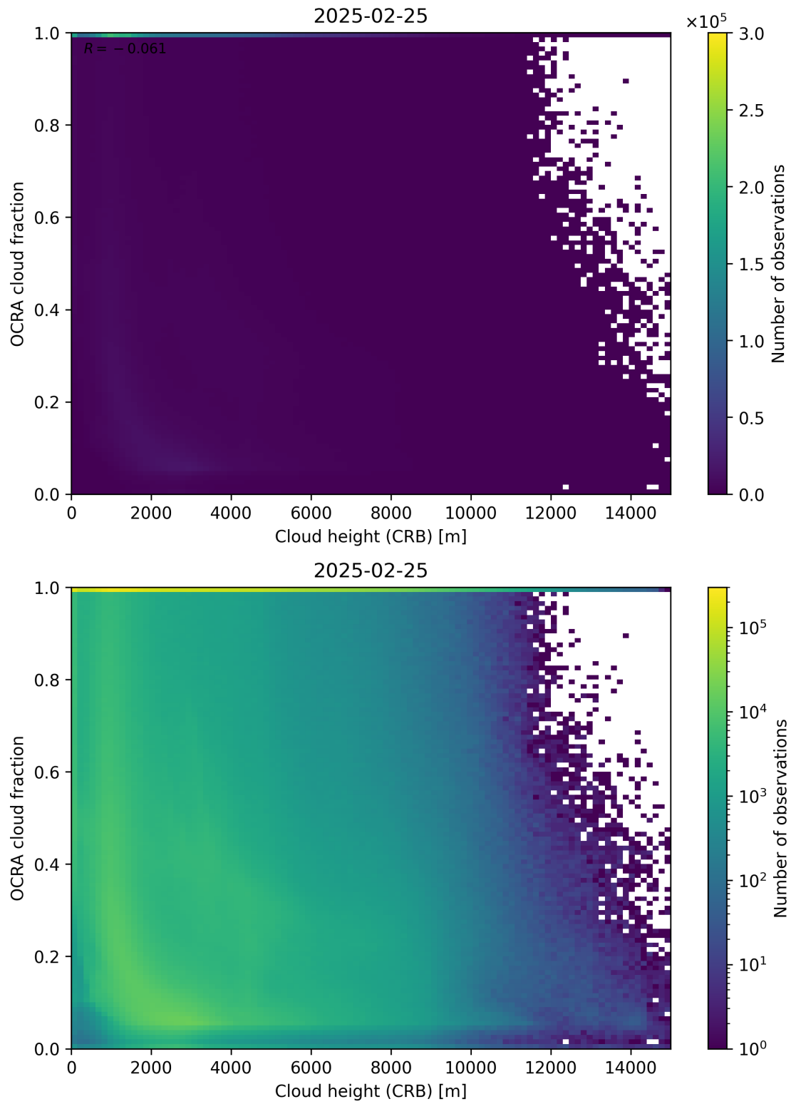
Figure 81: Scatter density plot of “Cloud height (CRB)” against “OCRA cloud fraction” for 2025-02-24 to 2025-02-26.
