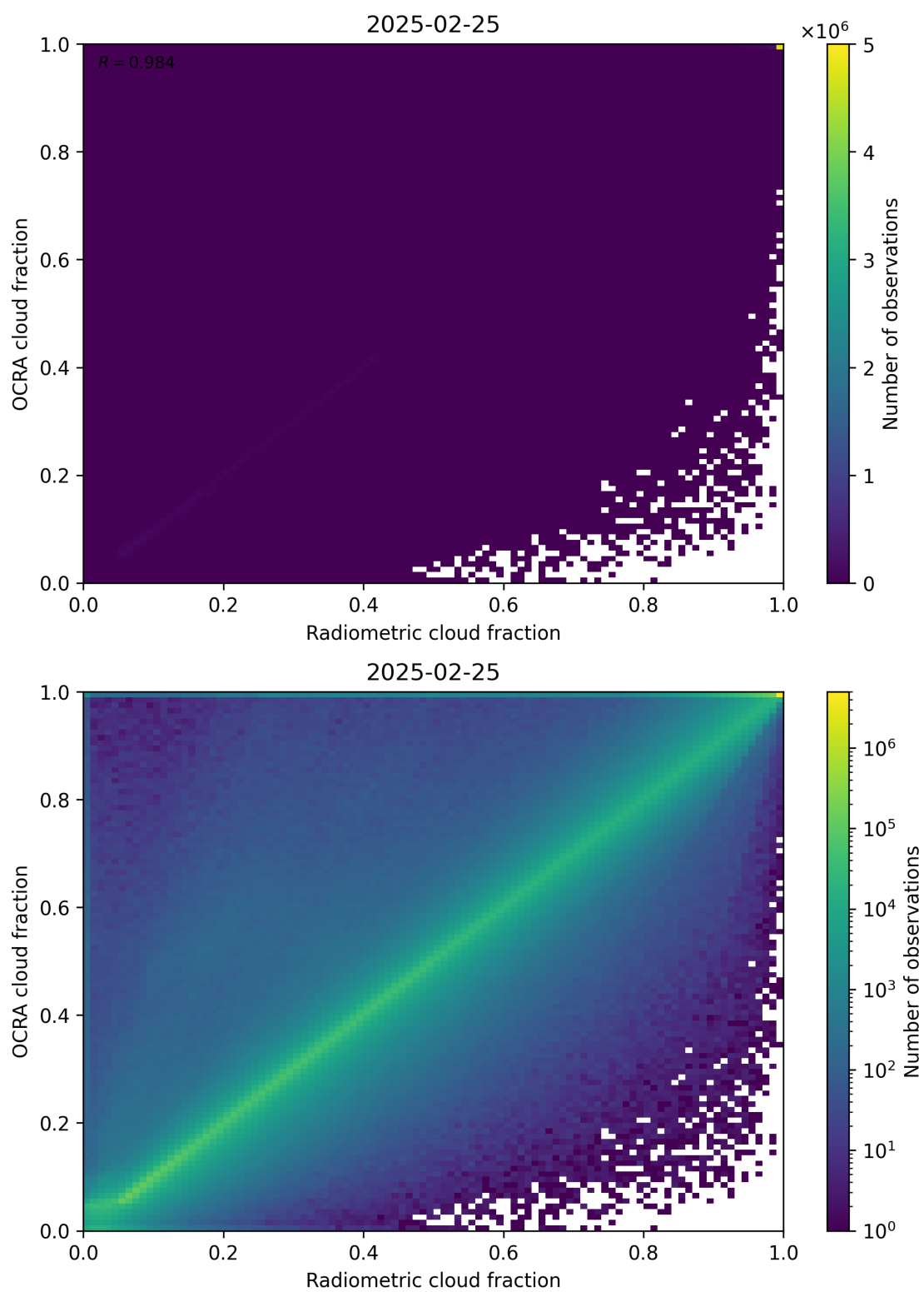
Figure 72: Scatter density plot of “Radiometric cloud fraction” against “OCRA cloud fraction” for 2025-02-24 to 2025-02-26.
