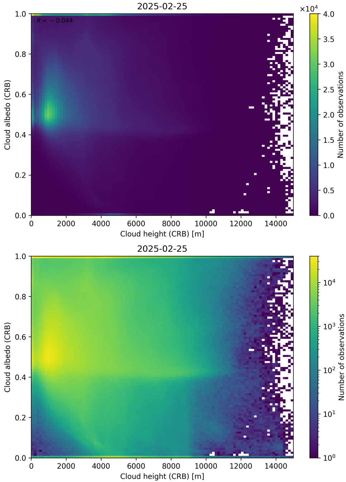
Figure 80: Scatter density plot of “Cloud height (CRB)” against “Cloud albedo (CRB)” for 2025-02-24 to 2025-02-26.
