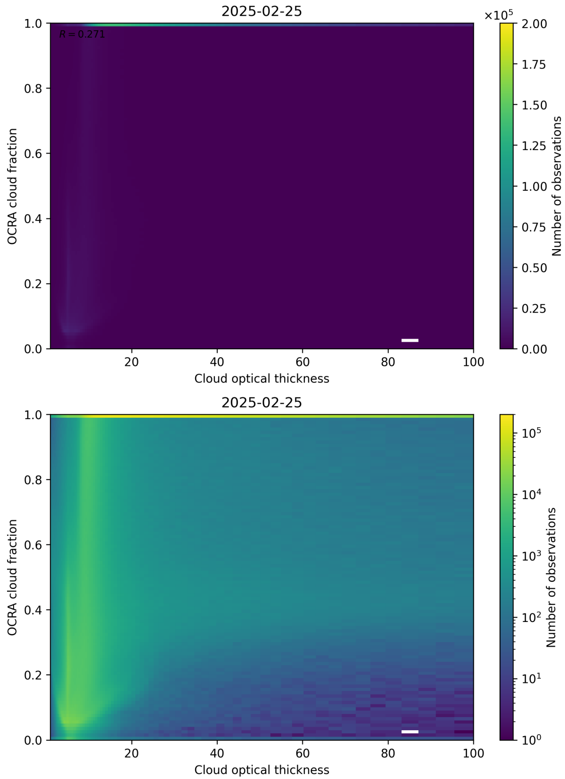
Figure 83: Scatter density plot of “Cloud optical thickness” against “OCRA cloud fraction” for 2025-02-24 to 2025-02-26.
