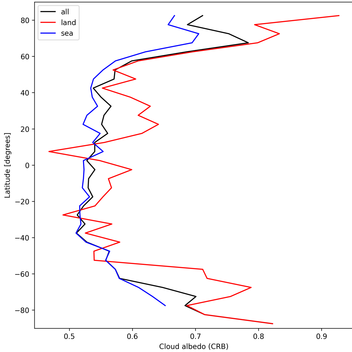
Figure 28: Zonal average of “Cloud albedo (CRB)” for 2025-02-24 to 2025-02-26.
