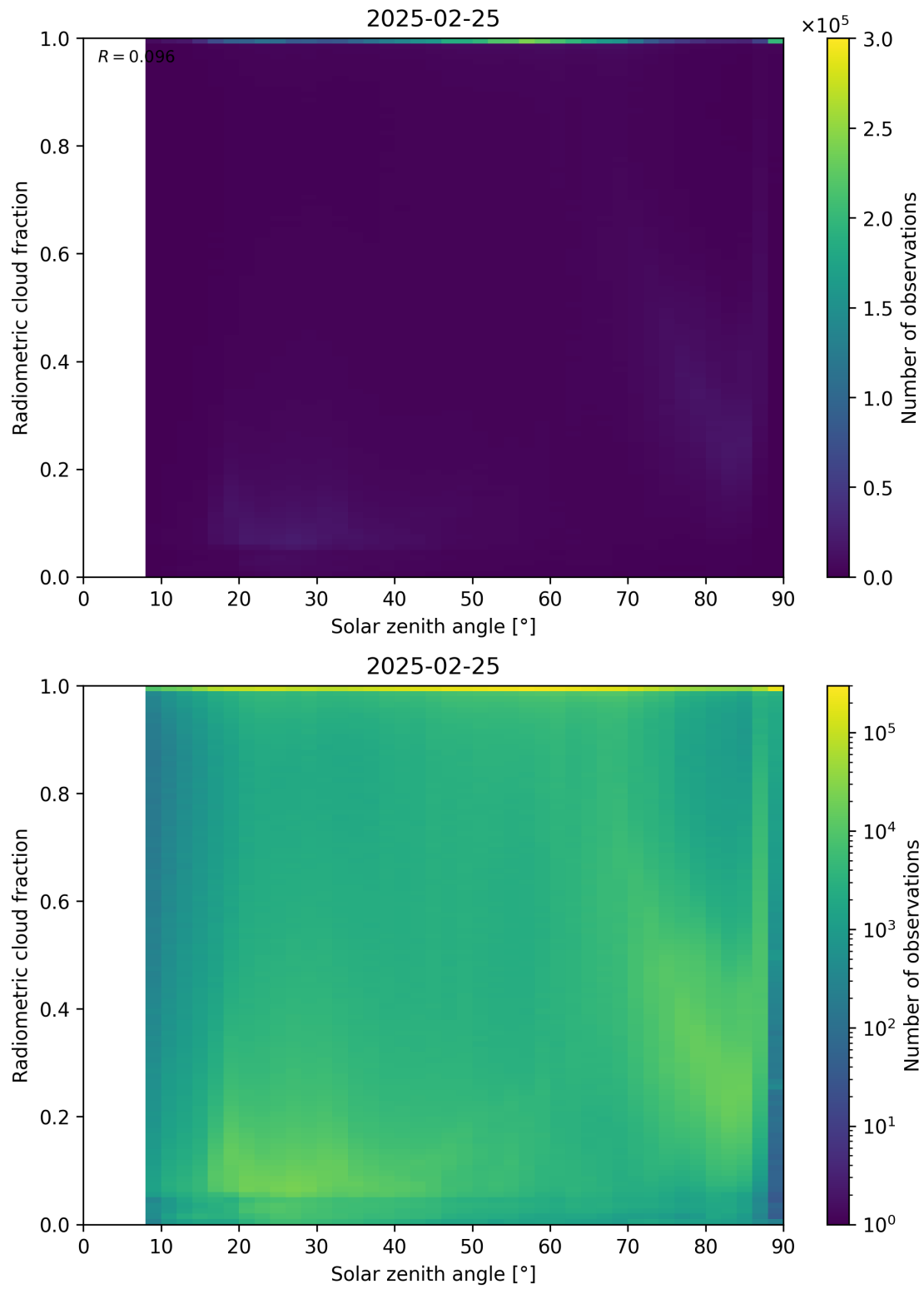
Figure 99: Scatter density plot of “Solar zenith angle” against “Radiometric cloud fraction” for 2025-02-24 to 2025-02-26.
