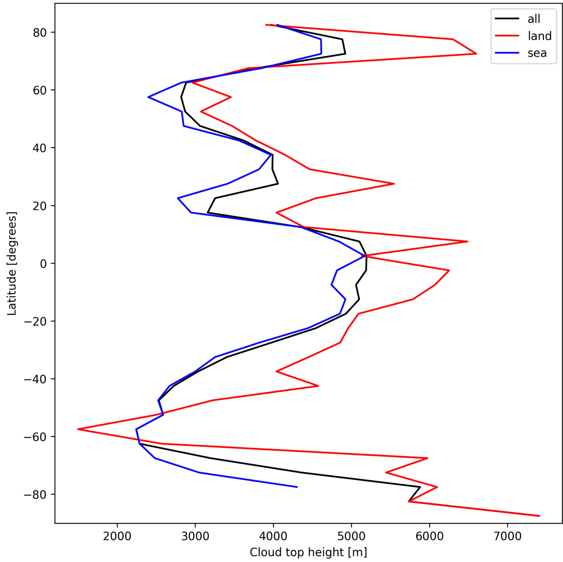
Figure 24: Zonal average of “Cloud top height” for 2025-02-24 to 2025-02-26.
