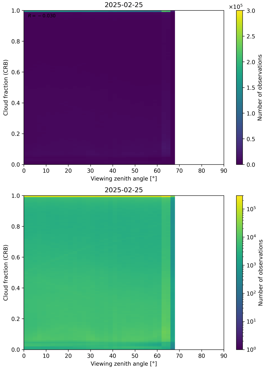
Figure 109: Scatter density plot of “Viewing zenith angle” against “Cloud fraction (CRB)” for 2025-02-24 to 2025-02-26.
