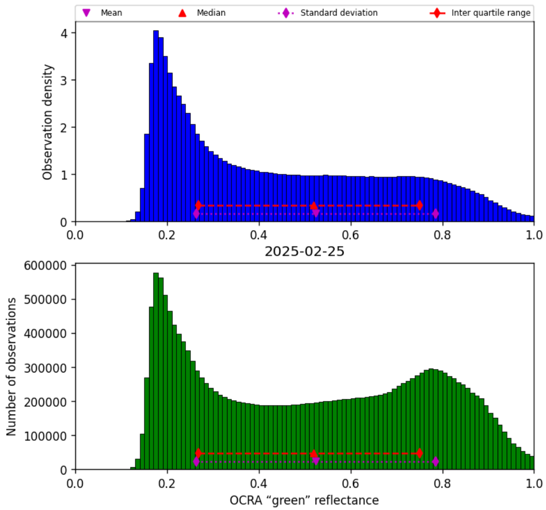
Figure 52: Histogram of “OCRA “green” reflectance” for 2025-02-24 to 2025-02-26
