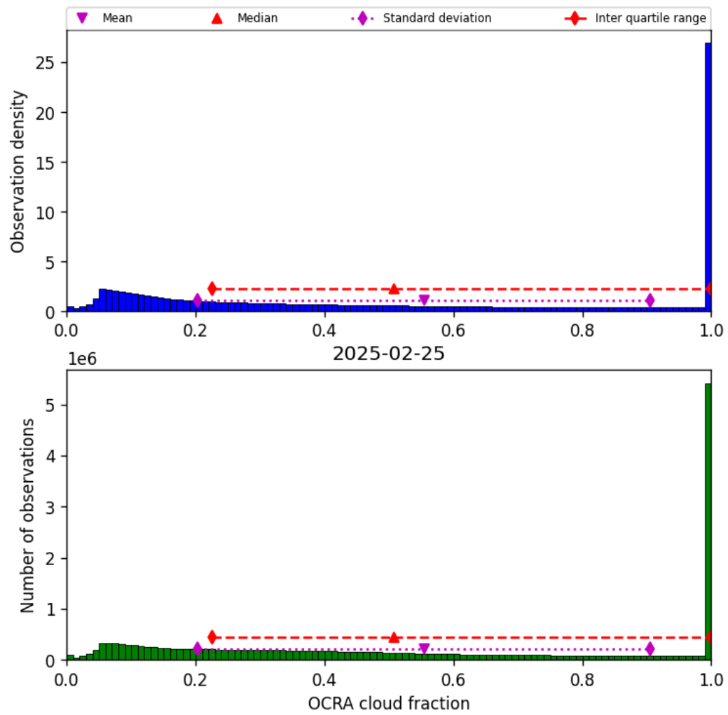
Figure 50: Histogram of “OCRA cloud fraction” for 2025-02-24 to 2025-02-26
