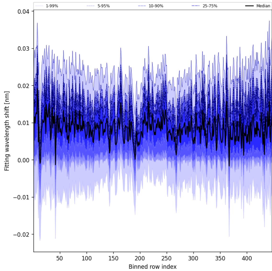
Figure 65: Along track statistics of “Fitting wavelength shift” for 2025-02-24 to 2025-02-26
