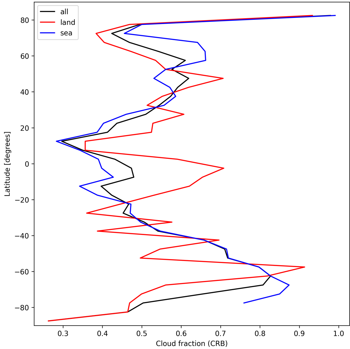
Figure 26: Zonal average of “Cloud fraction (CRB)” for 2025-02-24 to 2025-02-26.
