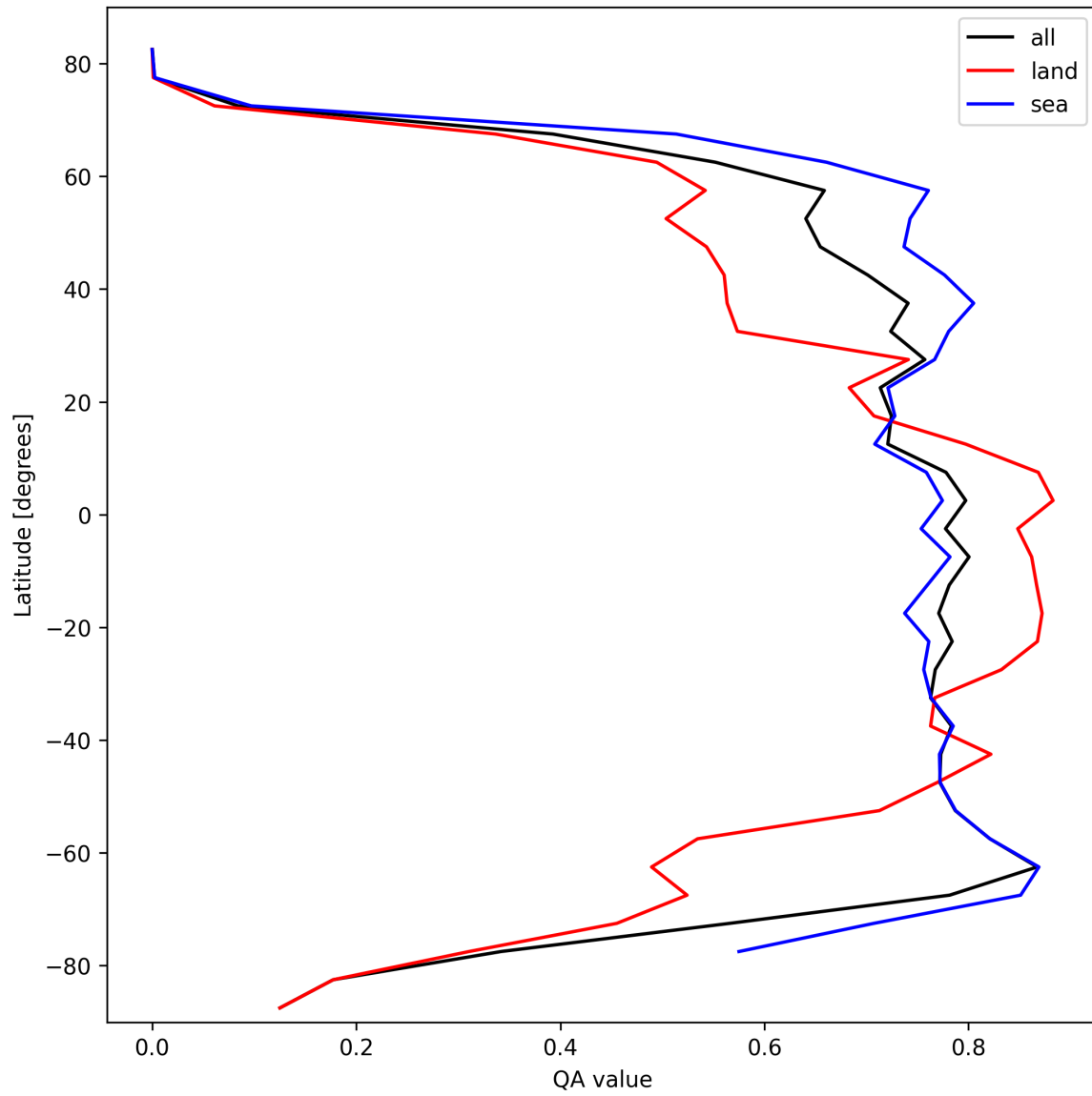
Figure 22: Zonal average of “QA value” for 2025-02-24 to 2025-02-26.
