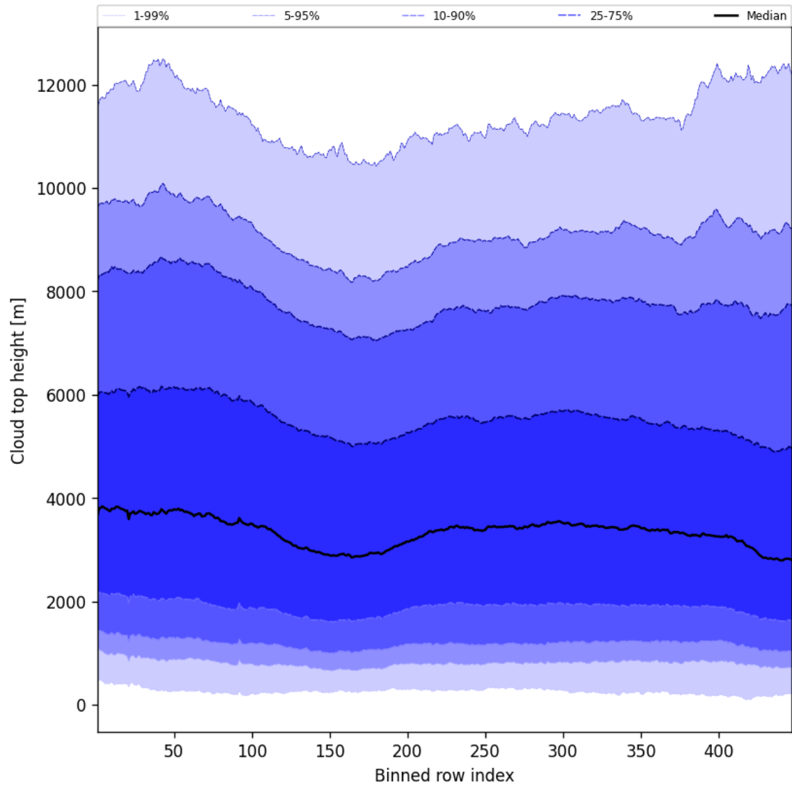
Figure 56: Along track statistics of “Cloud top height” for 2025-02-24 to 2025-02-26
