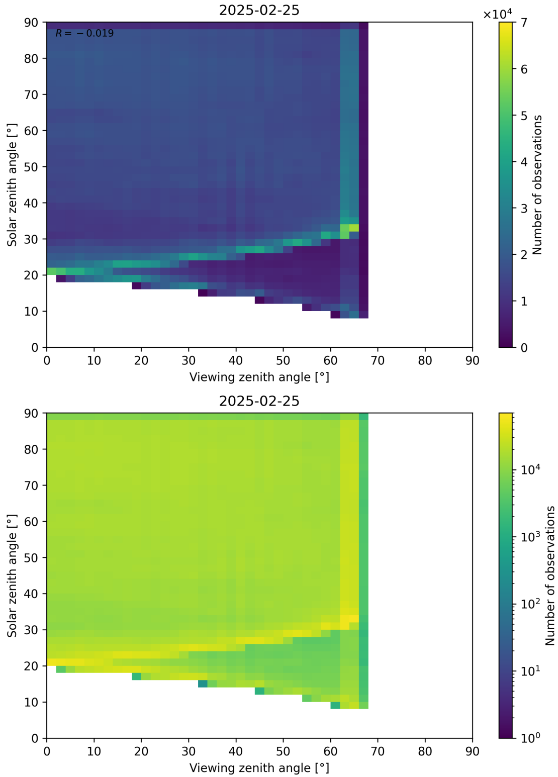
Figure 114: Scatter density plot of “Viewing zenith angle” against “Solar zenith angle” for 2025-02-24 to 2025-02-26.
