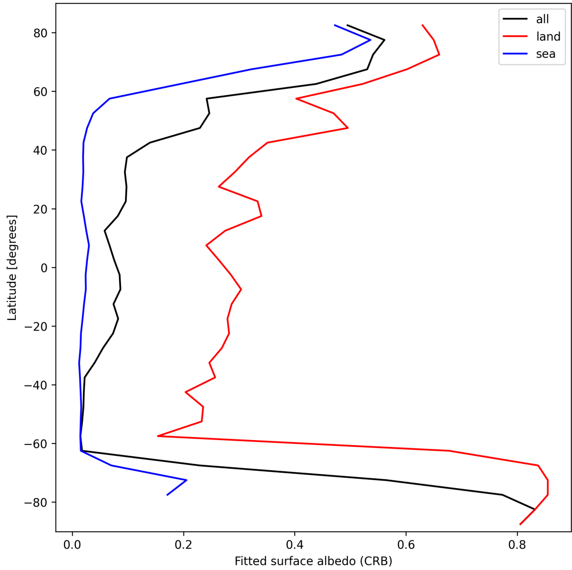
Figure 30: Zonal average of “Fitted surface albedo (CRB)” for 2025-02-24 to 2025-02-26.
