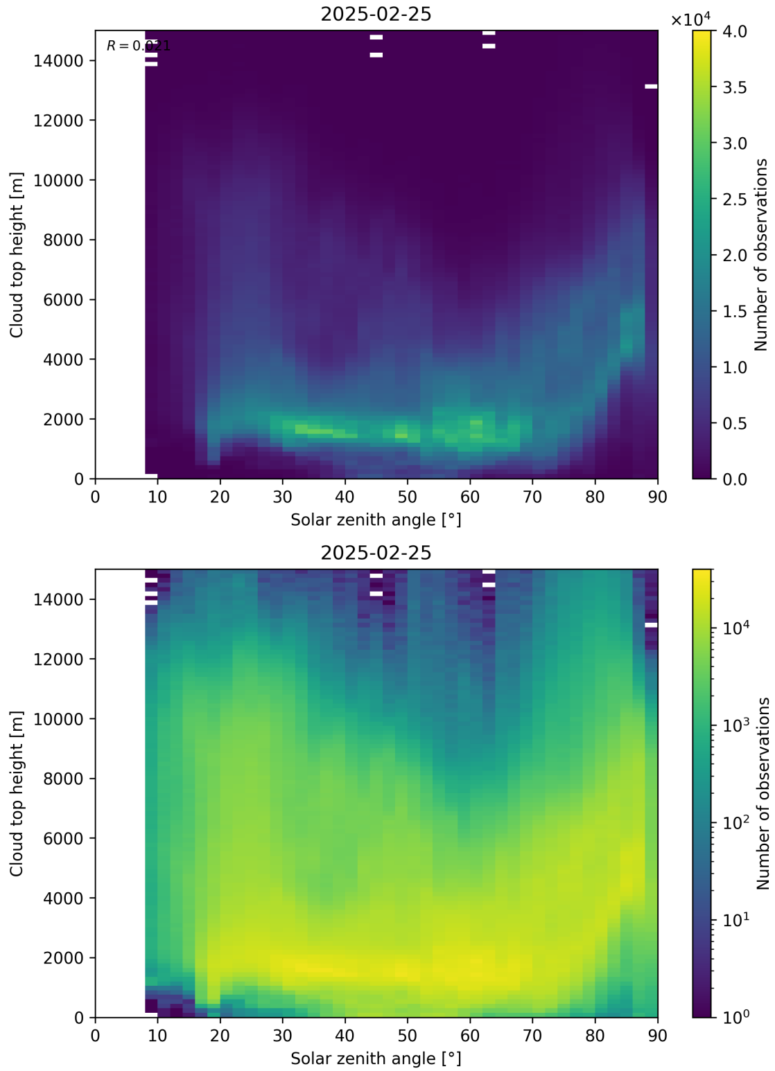
Figure 104: Scatter density plot of “Solar zenith angle” against “Cloud top height” for 2025-02-24 to 2025-02-26.
