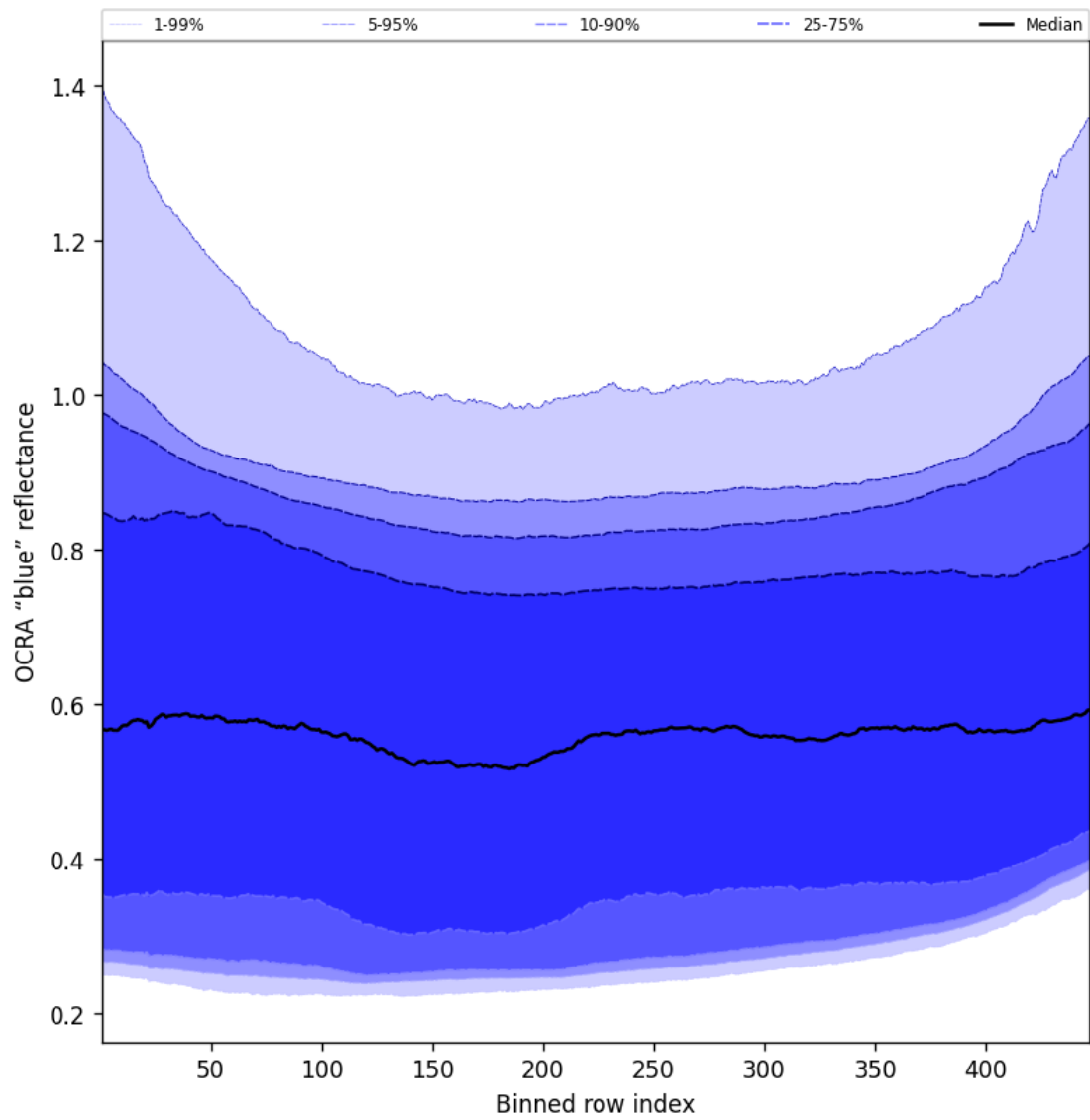
Figure 67: Along track statistics of “OCRA “blue” reflectance” for 2025-02-24 to 2025-02-26
