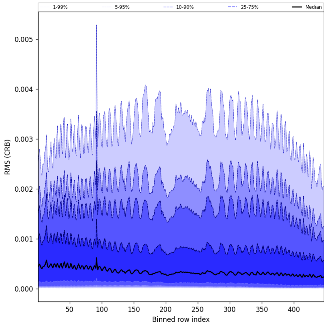
Figure 64: Along track statistics of “RMS (CRB)” for 2025-02-24 to 2025-02-26
