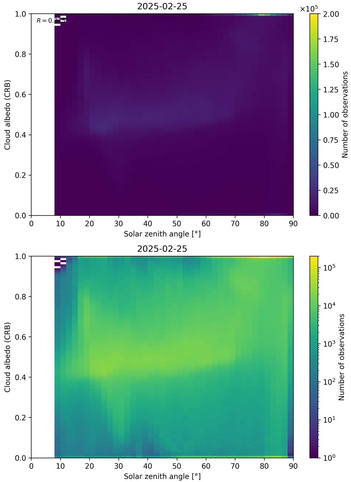
Figure 98: Scatter density plot of “Solar zenith angle” against “Cloud albedo (CRB)” for 2025-02-24 to 2025-02-26.
