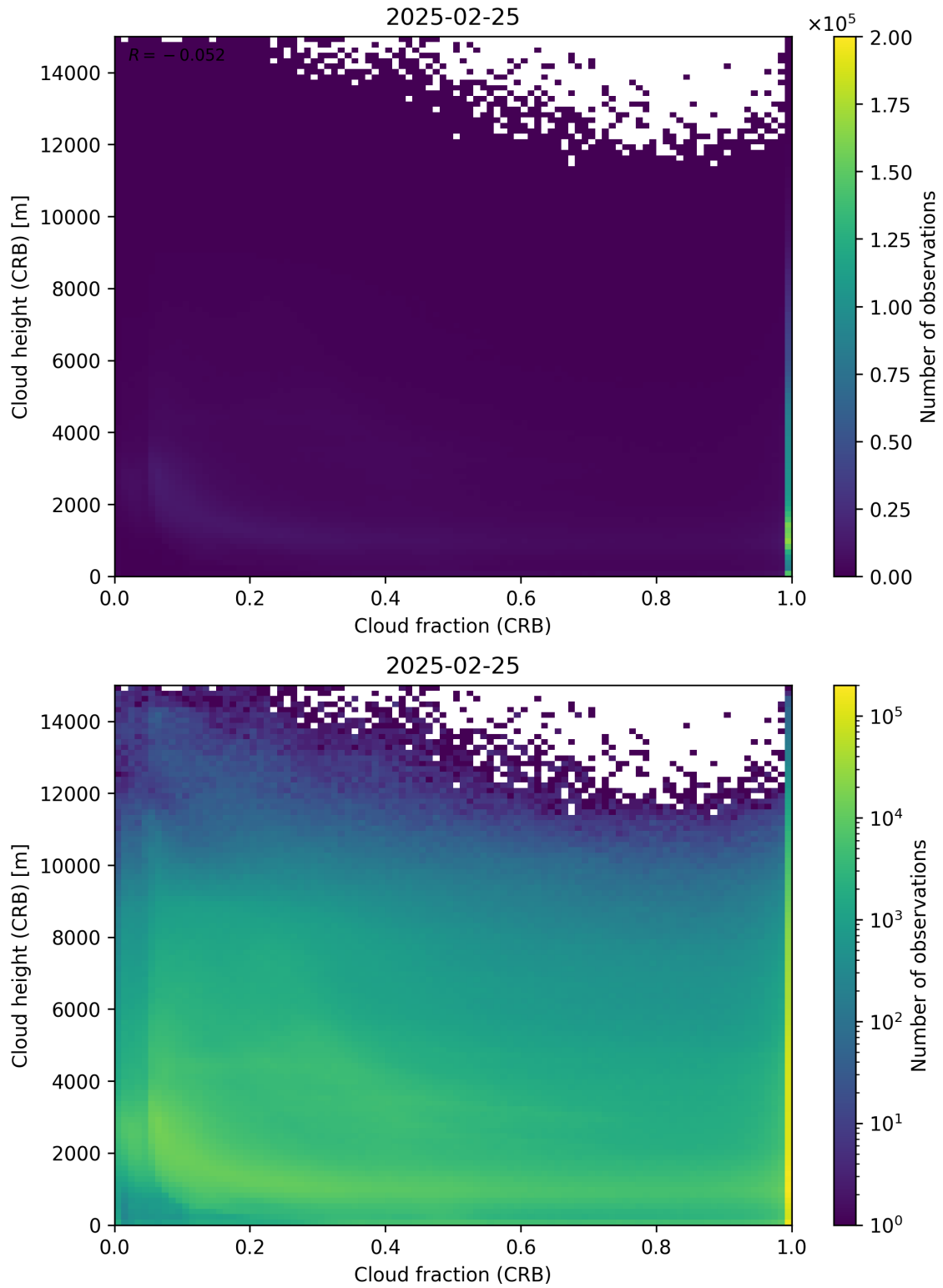
Figure 79: Scatter density plot of “Cloud fraction (CRB)” against “Cloud height (CRB)” for 2025-02-24 to 2025-02-26.
