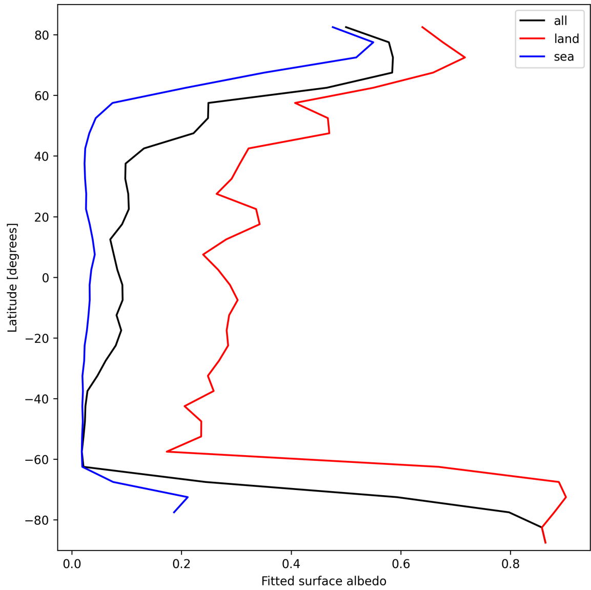
Figure 29: Zonal average of “Fitted surface albedo” for 2025-02-24 to 2025-02-26.
