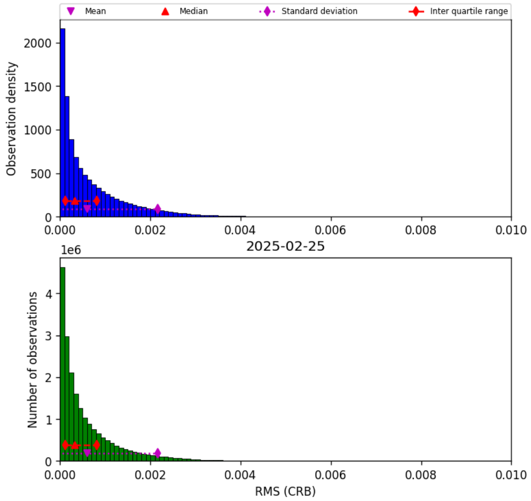
Figure 48: Histogram of “RMS (CRB)” for 2025-02-24 to 2025-02-26
