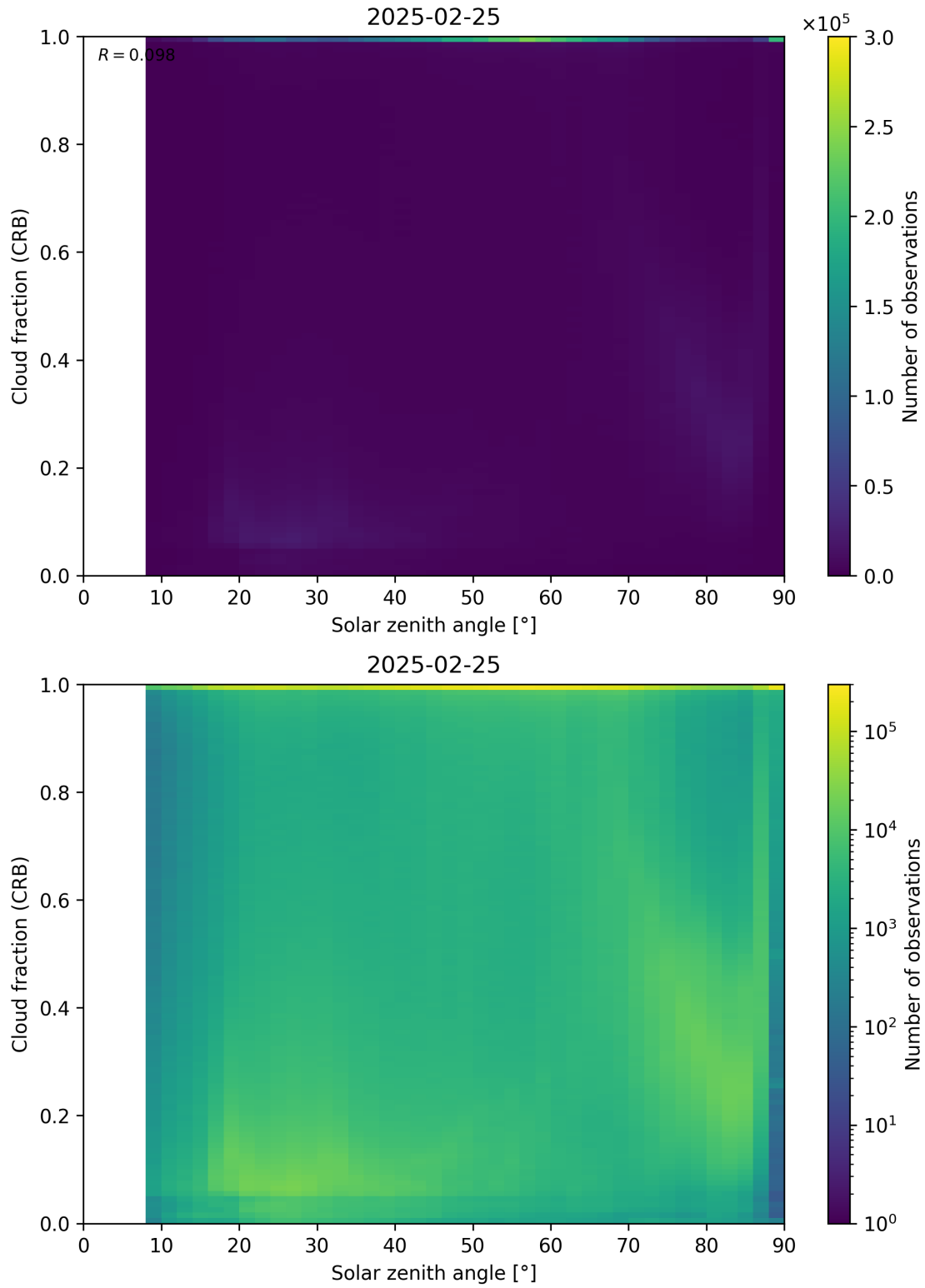
Figure 101: Scatter density plot of “Solar zenith angle” against “Cloud fraction (CRB)” for 2025-02-24 to 2025-02-26.
