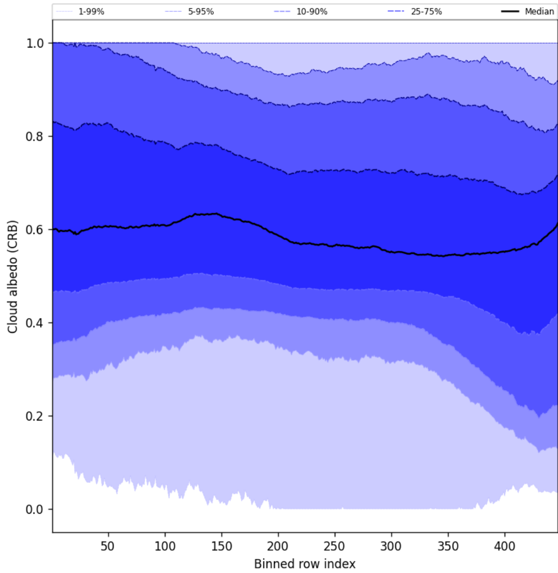
Figure 60: Along track statistics of “Cloud albedo (CRB)” for 2025-02-24 to 2025-02-26
