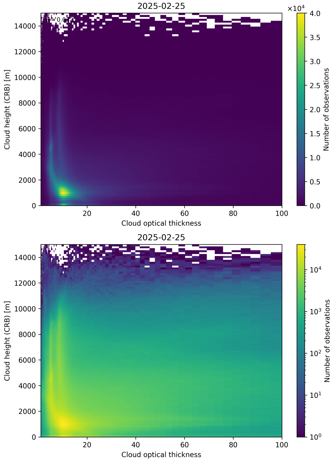
Figure 85: Scatter density plot of “Cloud optical thickness” against “Cloud height (CRB)” for 2025-02-24 to 2025-02-26.
