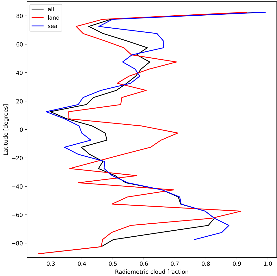
Figure 23: Zonal average of “Radiometric cloud fraction” for 2025-02-24 to 2025-02-26.
