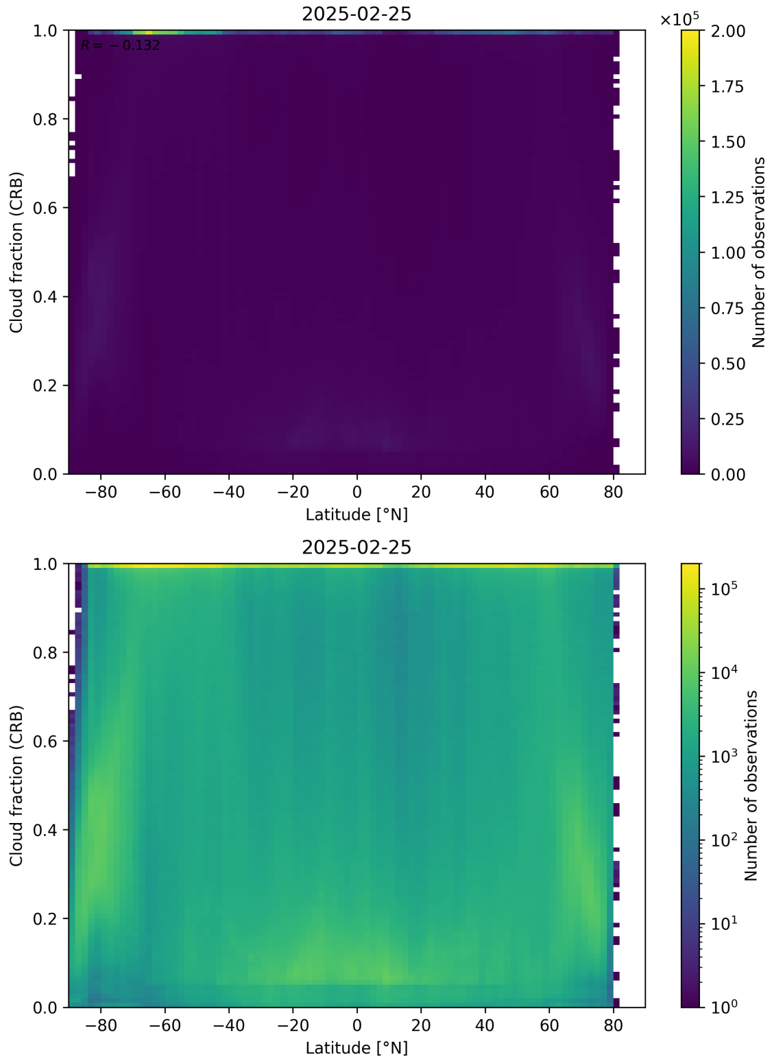
Figure 94: Scatter density plot of “Latitude” against “Cloud fraction (CRB)” for 2025-02-24 to 2025-02-26.
