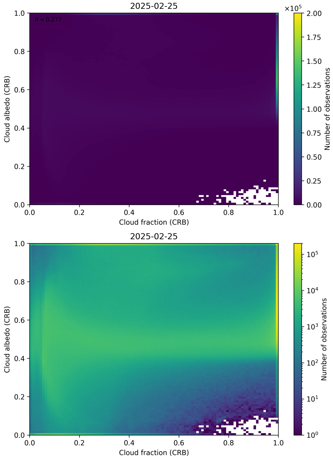
Figure 77: Scatter density plot of “Cloud fraction (CRB)” against “Cloud albedo (CRB)” for 2025-02-24 to 2025-02-26.
