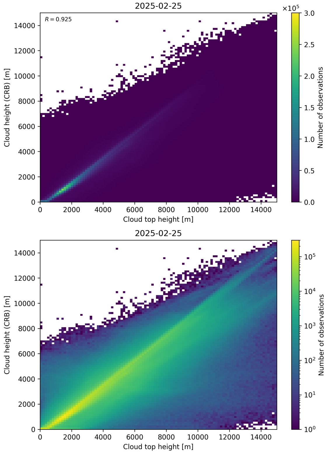
Figure 89: Scatter density plot of “Cloud top height” against “Cloud height (CRB)” for 2025-02-24 to 2025-02-26.
