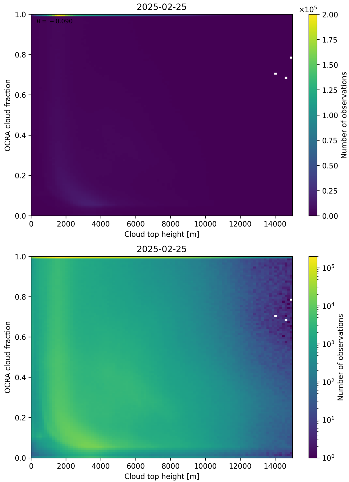
Figure 87: Scatter density plot of “Cloud top height” against “OCRA cloud fraction” for 2025-02-24 to 2025-02-26.
