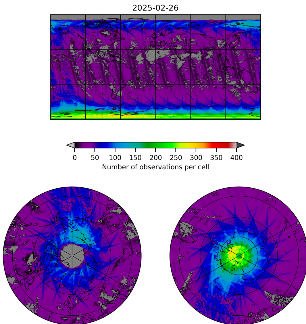
Figure 21: Map of the number of observations for 2025-02-25 to 2025-02-27
