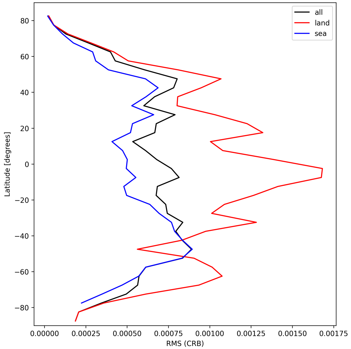
Figure 32: Zonal average of “RMS (CRB)” for 2025-02-25 to 2025-02-27.
