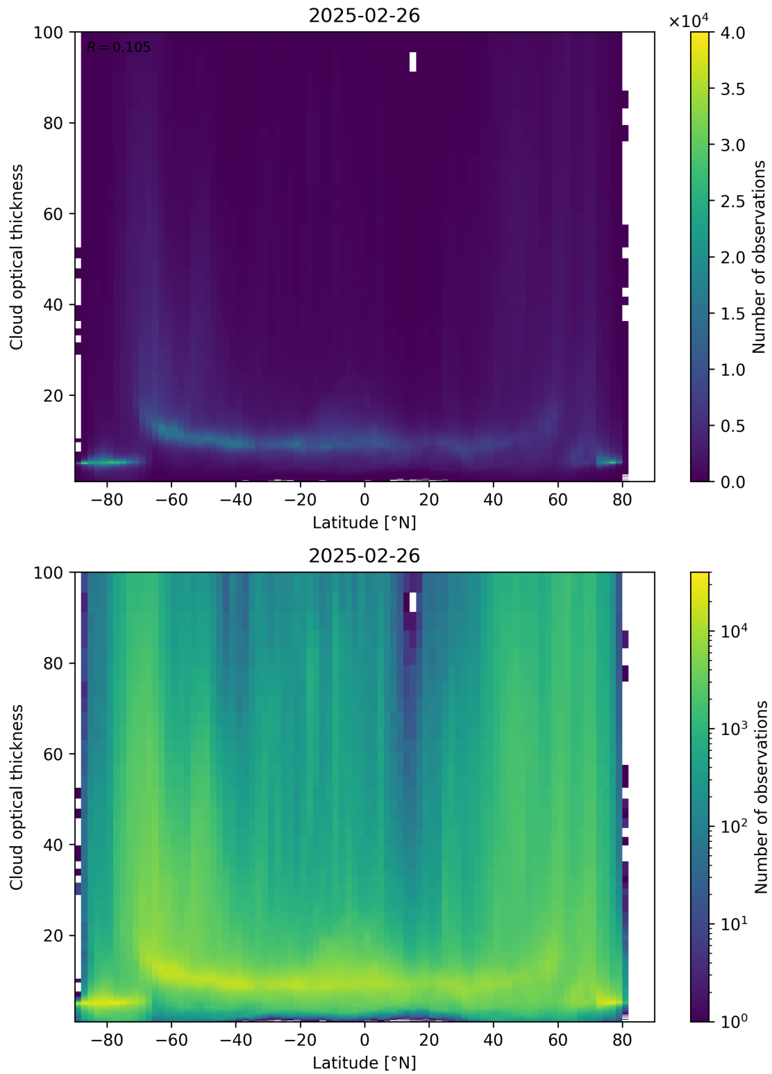
Figure 96: Scatter density plot of “Latitude” against “Cloud optical thickness” for 2025-02-25 to 2025-02-27.
