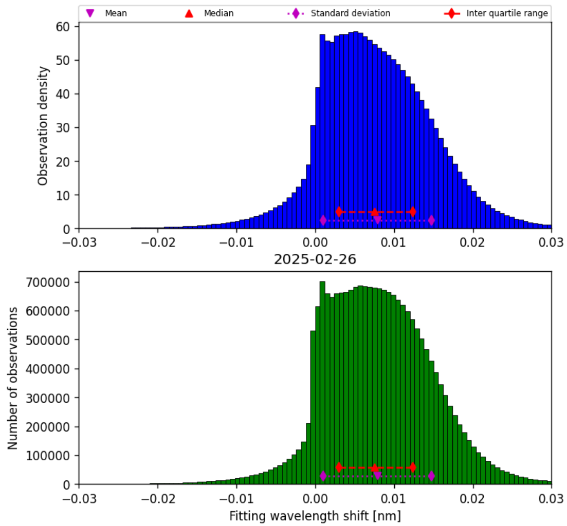
Figure 49: Histogram of “Fitting wavelength shift” for 2025-02-25 to 2025-02-27
