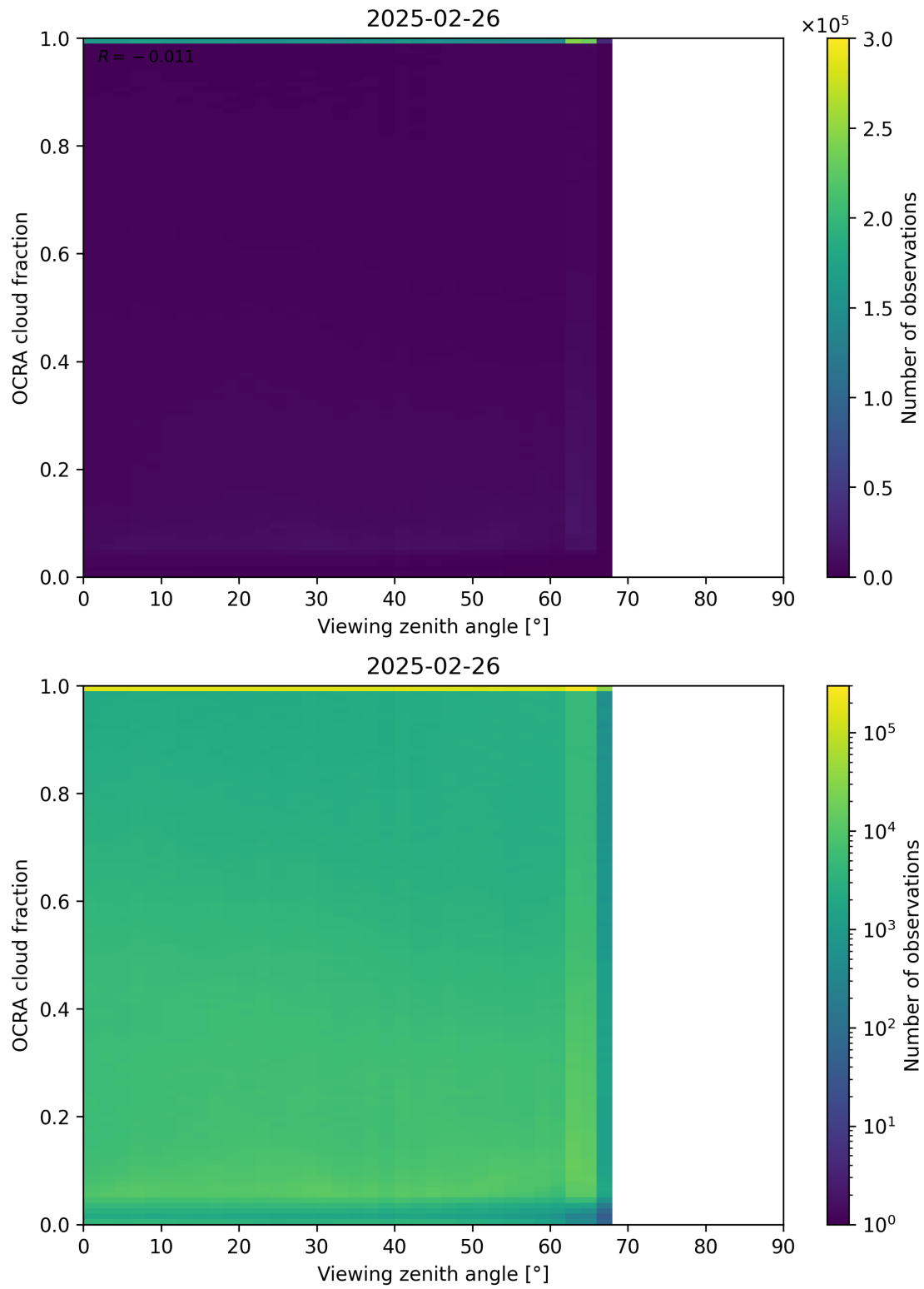
Figure 108: Scatter density plot of “Viewing zenith angle” against “OCRA cloud fraction” for 2025-02-25 to 2025-02-27.
