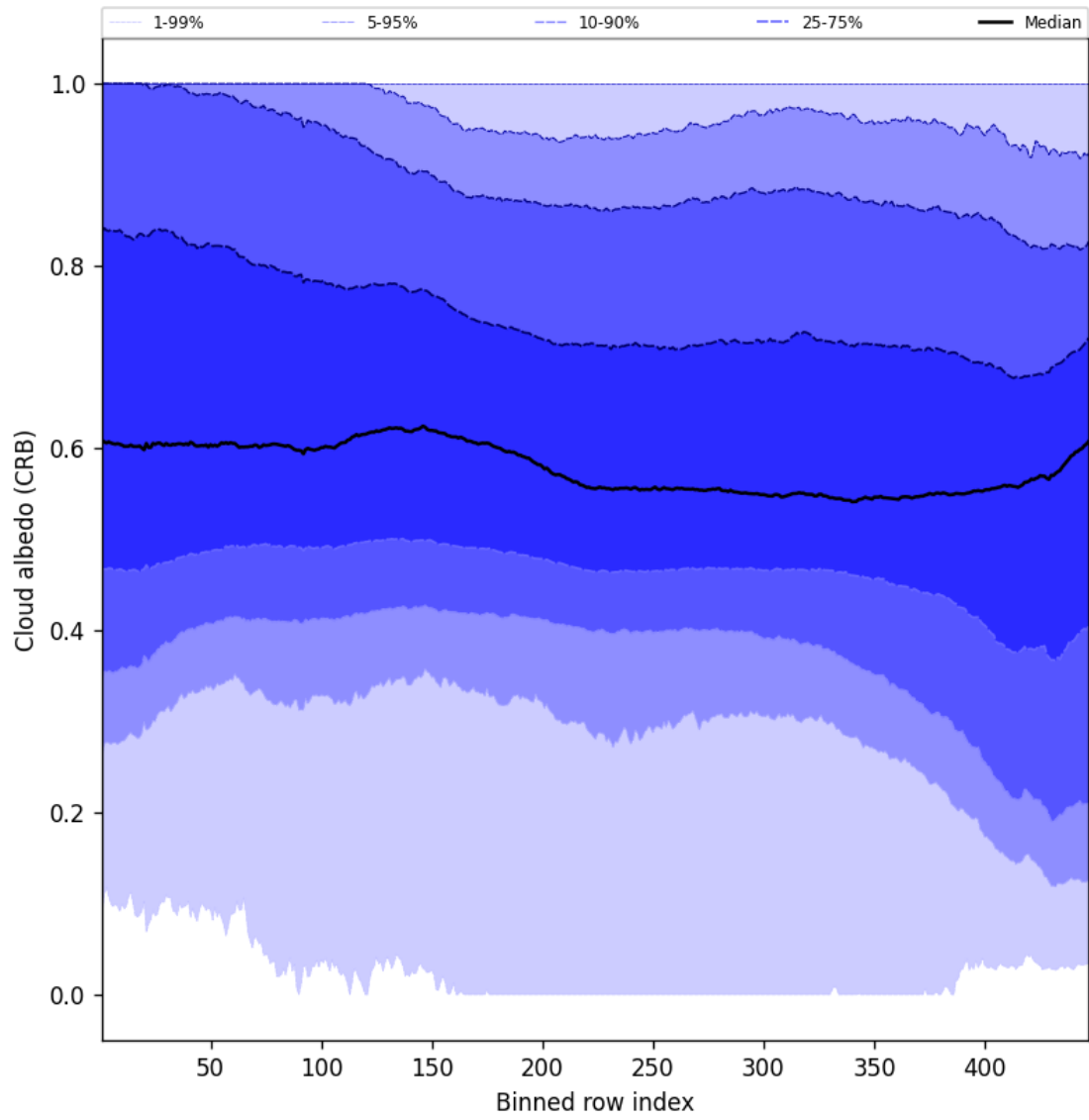
Figure 60: Along track statistics of “Cloud albedo (CRB)” for 2025-02-25 to 2025-02-27
