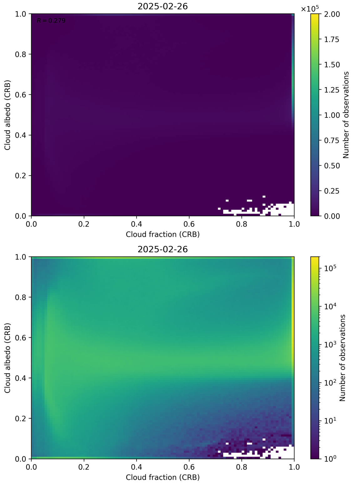
Figure 77: Scatter density plot of “Cloud fraction (CRB)” against “Cloud albedo (CRB)” for 2025-02-25 to 2025-02-27.
