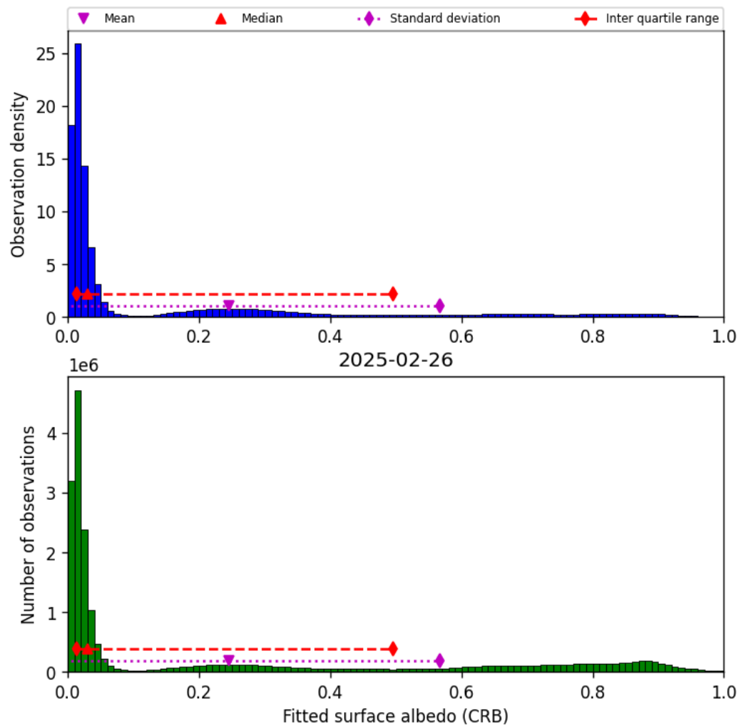
Figure 46: Histogram of “Fitted surface albedo (CRB)” for 2025-02-25 to 2025-02-27
