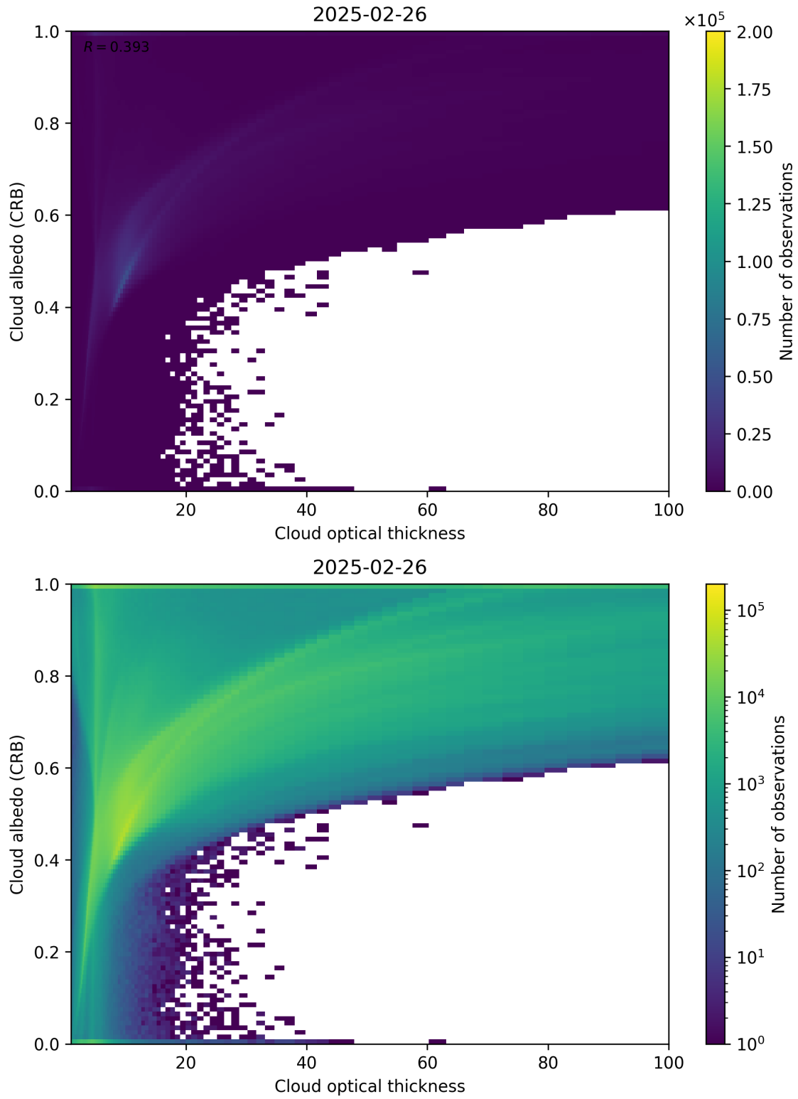
Figure 82: Scatter density plot of “Cloud optical thickness” against “Cloud albedo (CRB)” for 2025-02-25 to 2025-02-27.
