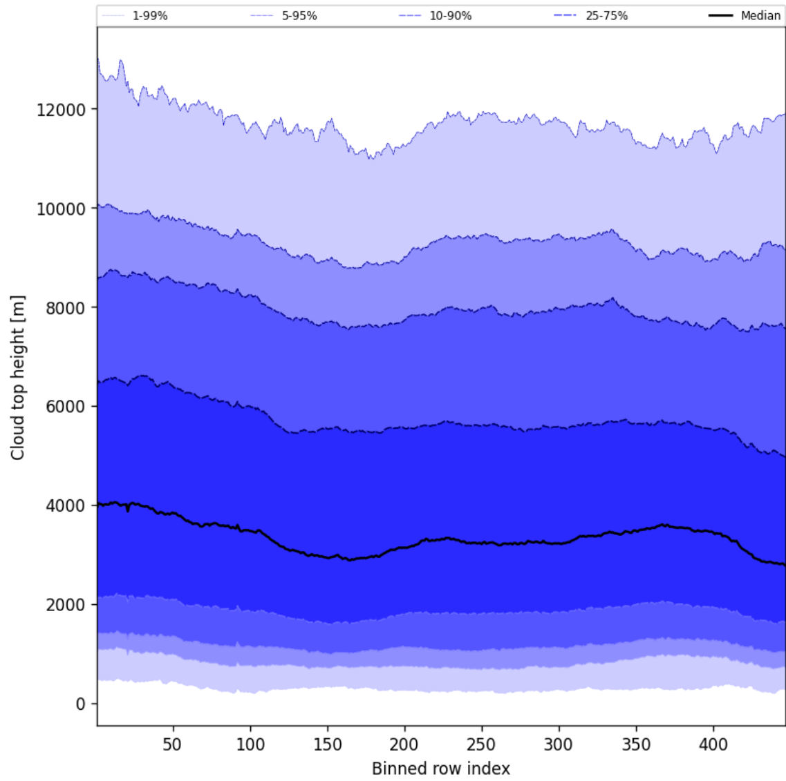
Figure 56: Along track statistics of “Cloud top height” for 2025-02-25 to 2025-02-27
