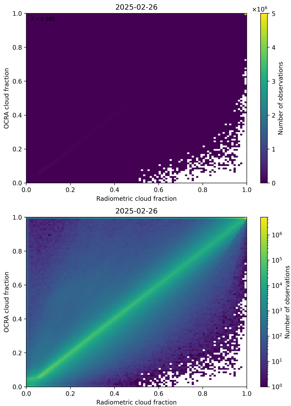
Figure 72: Scatter density plot of “Radiometric cloud fraction” against “OCRA cloud fraction” for 2025-02-25 to 2025-02-27.
