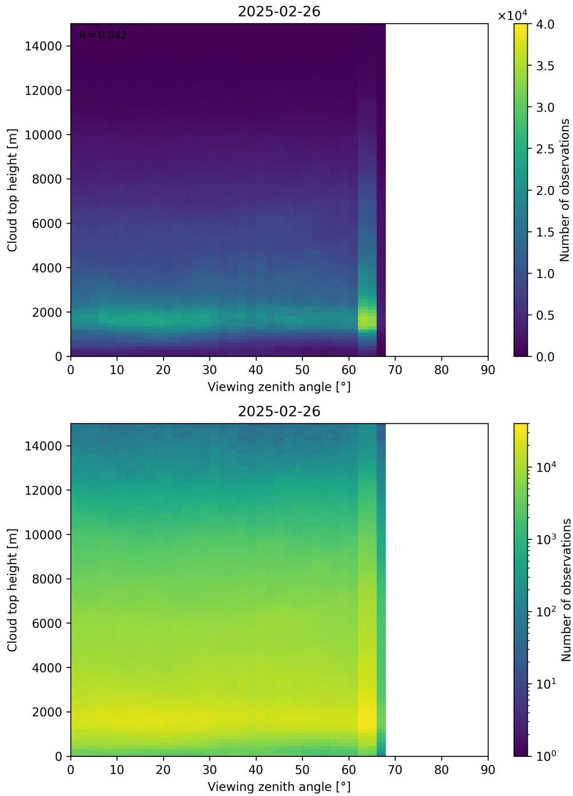
Figure 112: Scatter density plot of “Viewing zenith angle” against “Cloud top height” for 2025-02-25 to 2025-02-27.
