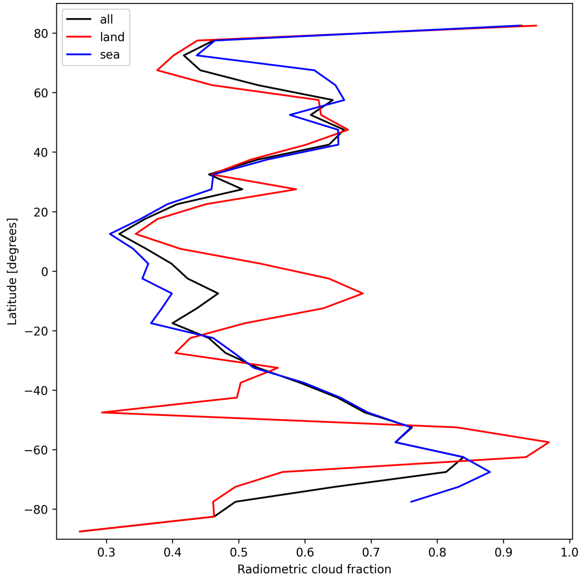
Figure 23: Zonal average of “Radiometric cloud fraction” for 2025-02-25 to 2025-02-27.
