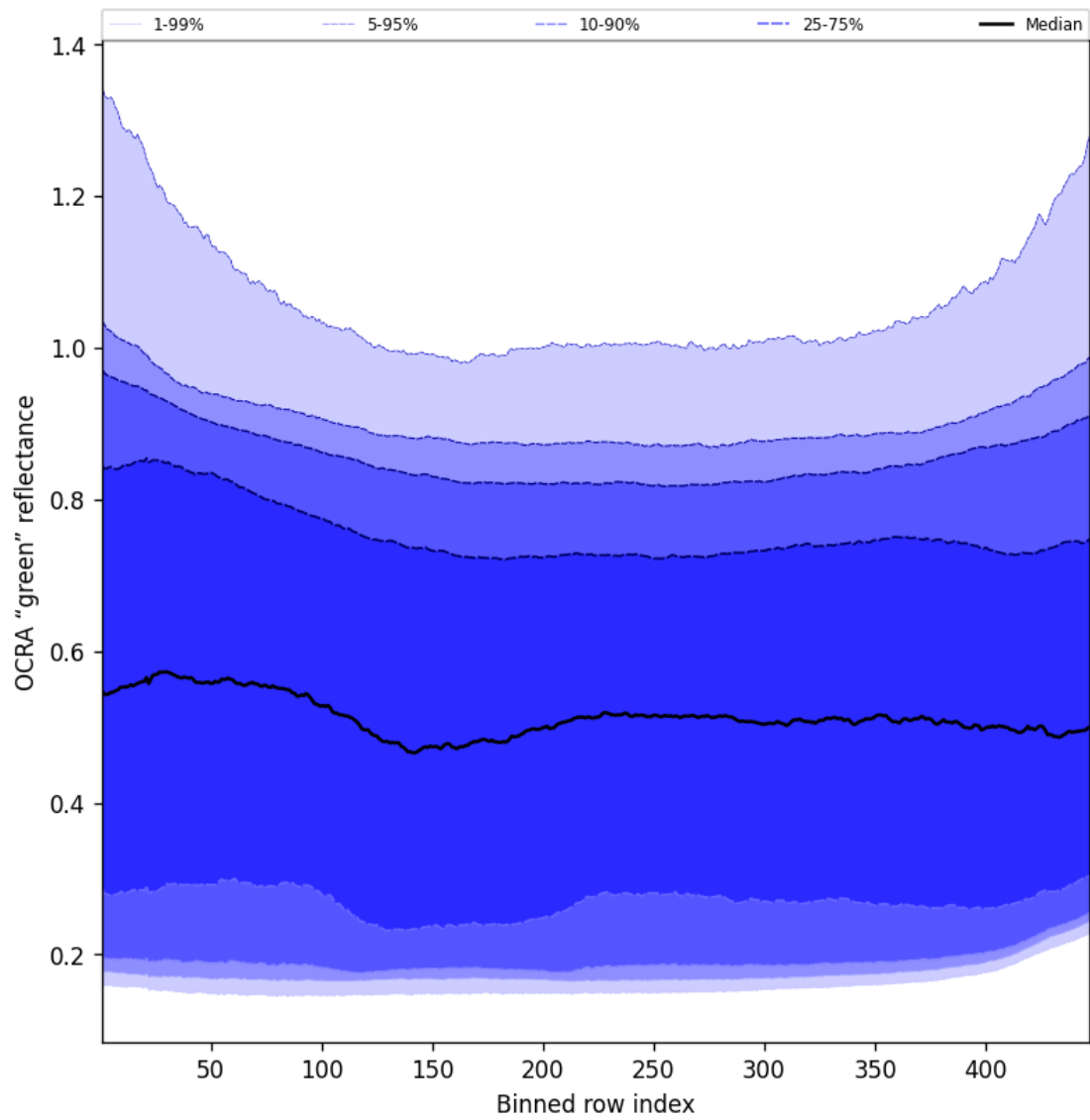
Figure 68: Along track statistics of “OCRA “green” reflectance” for 2025-02-25 to 2025-02-27
