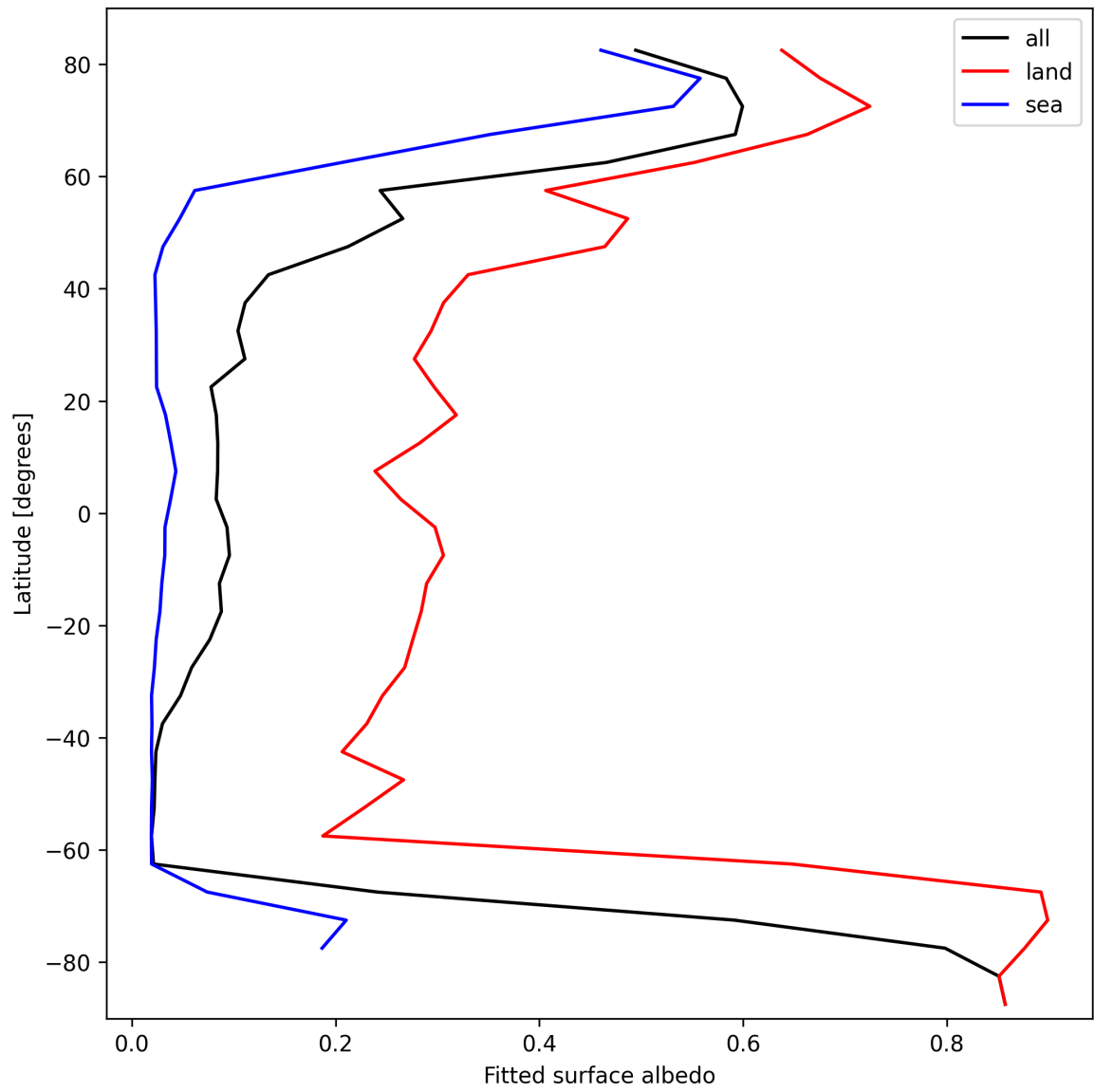
Figure 29: Zonal average of “Fitted surface albedo” for 2025-02-25 to 2025-02-27.
