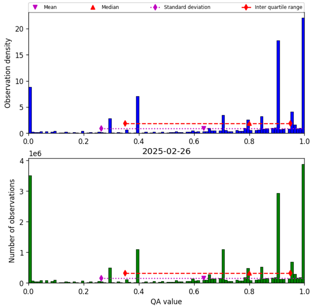
Figure 38: Histogram of “QA value” for 2025-02-25 to 2025-02-27
