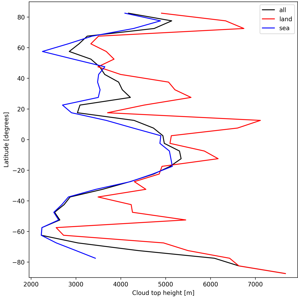
Figure 24: Zonal average of “Cloud top height” for 2025-02-25 to 2025-02-27.
