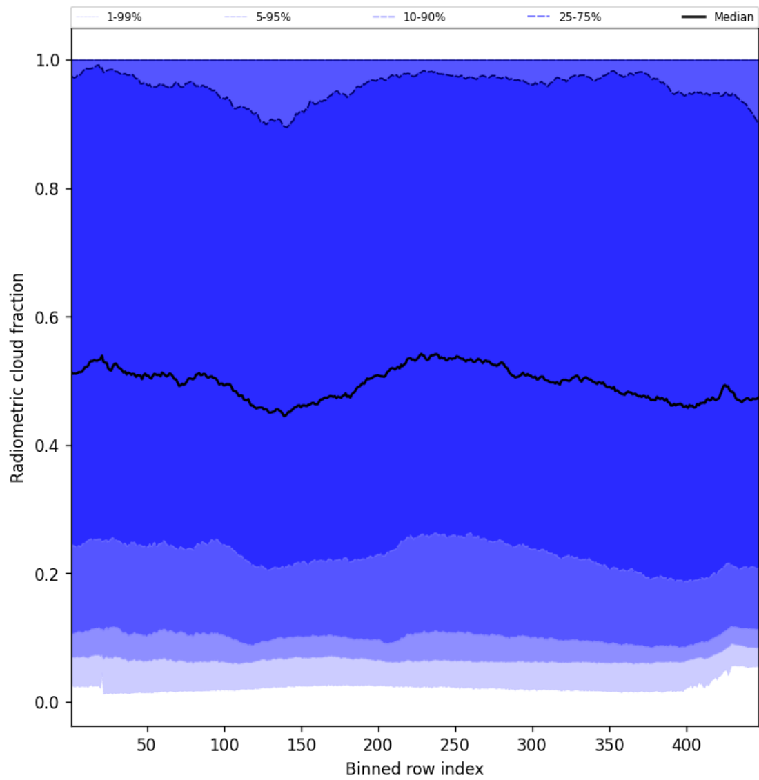
Figure 55: Along track statistics of “Radiometric cloud fraction” for 2025-02-25 to 2025-02-27
