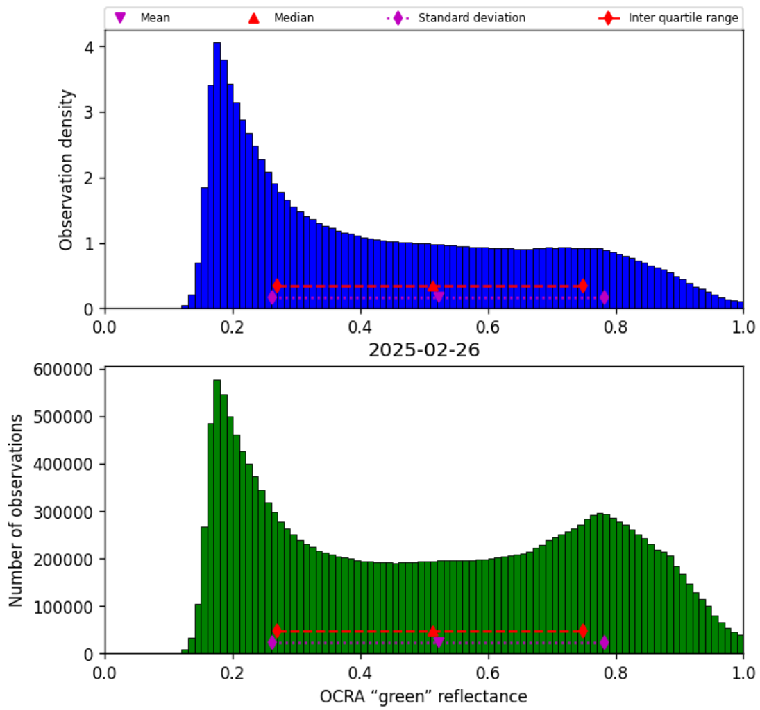
Figure 52: Histogram of “OCRA “green” reflectance” for 2025-02-25 to 2025-02-27
