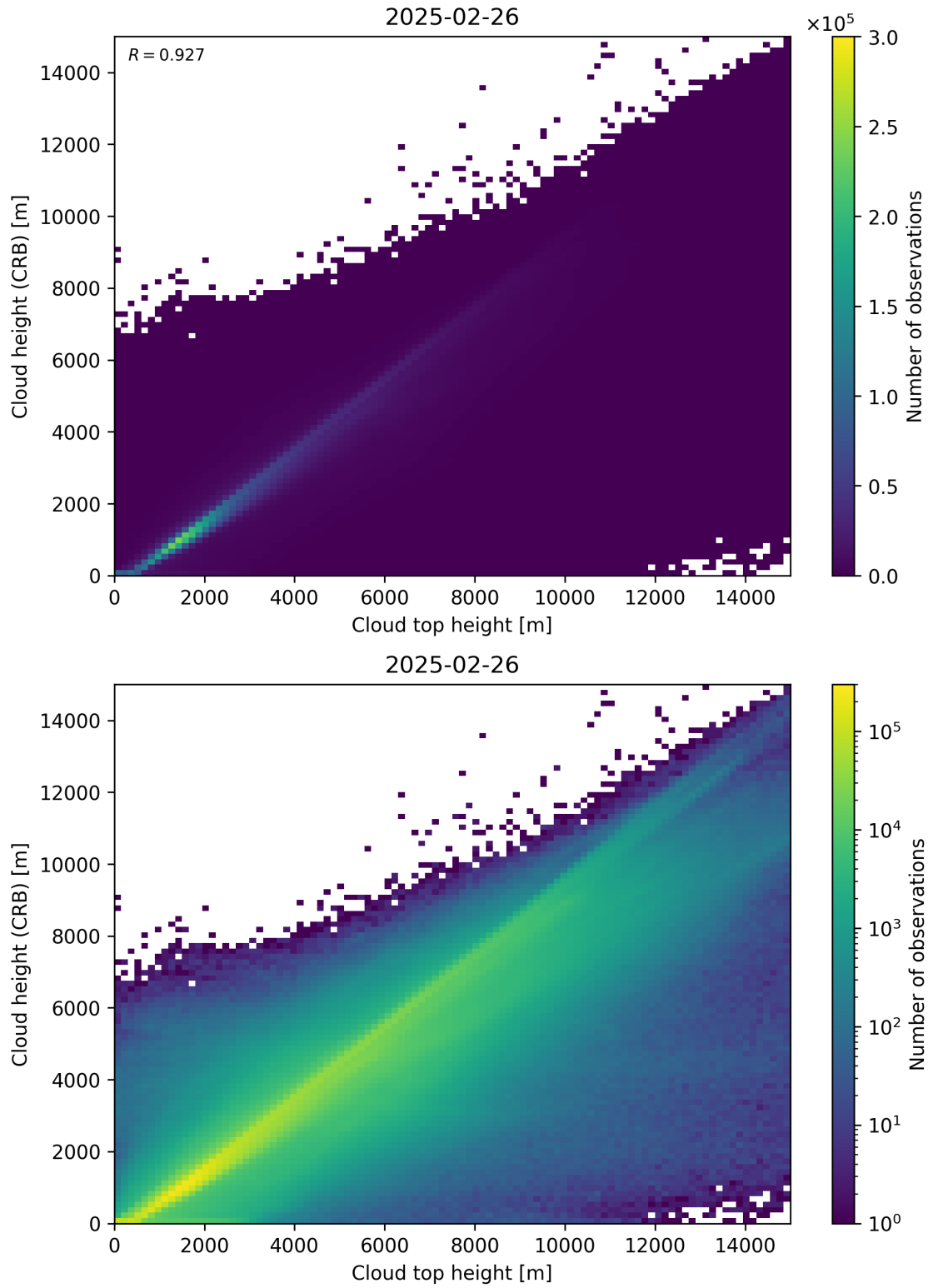
Figure 89: Scatter density plot of “Cloud top height” against “Cloud height (CRB)” for 2025-02-25 to 2025-02-27.
