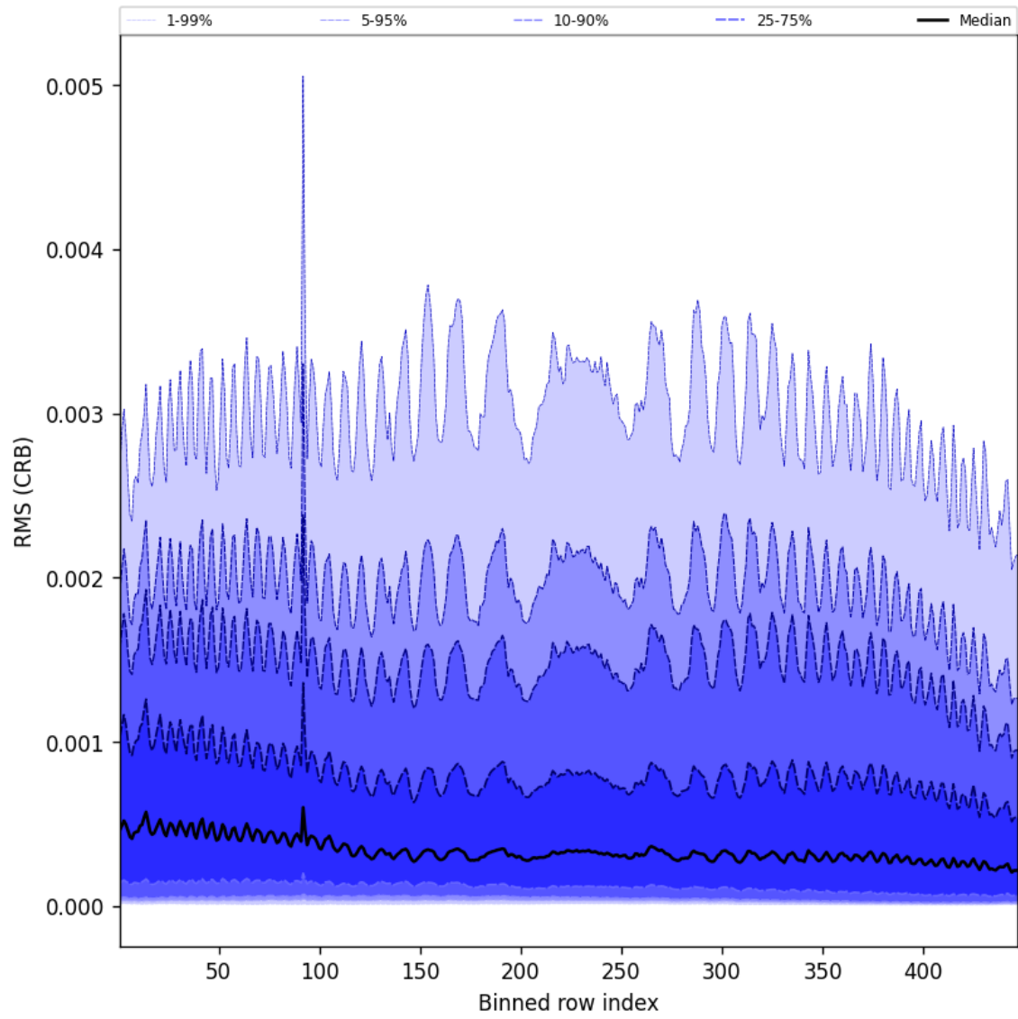
Figure 64: Along track statistics of “RMS (CRB)” for 2025-02-25 to 2025-02-27
