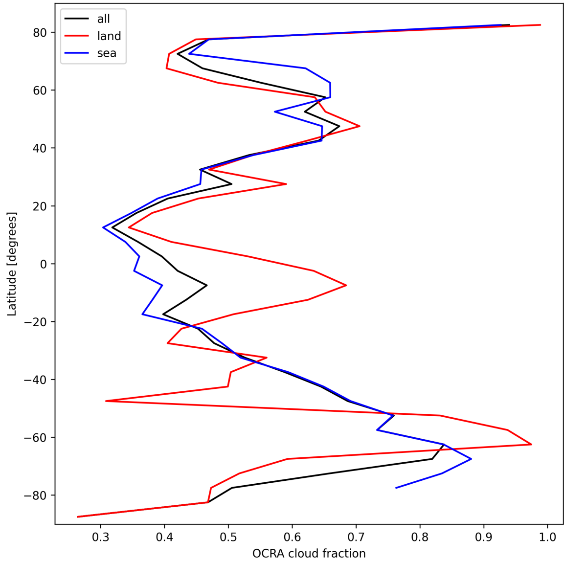
Figure 34: Zonal average of “OCRA cloud fraction” for 2025-02-25 to 2025-02-27.
