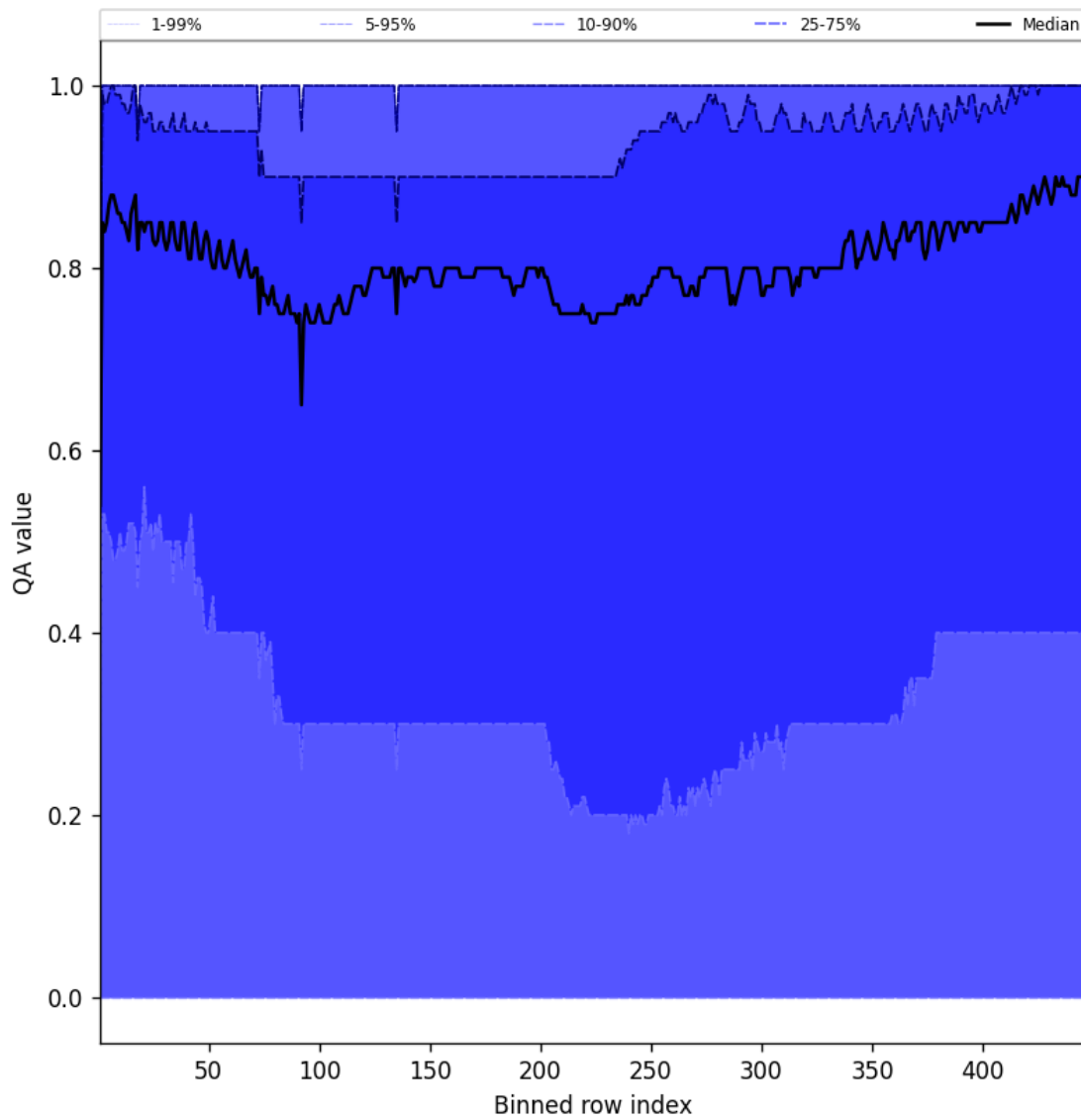
Figure 54: Along track statistics of “QA value” for 2025-02-25 to 2025-02-27
