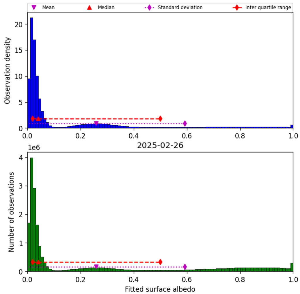
Figure 45: Histogram of “Fitted surface albedo” for 2025-02-25 to 2025-02-27
