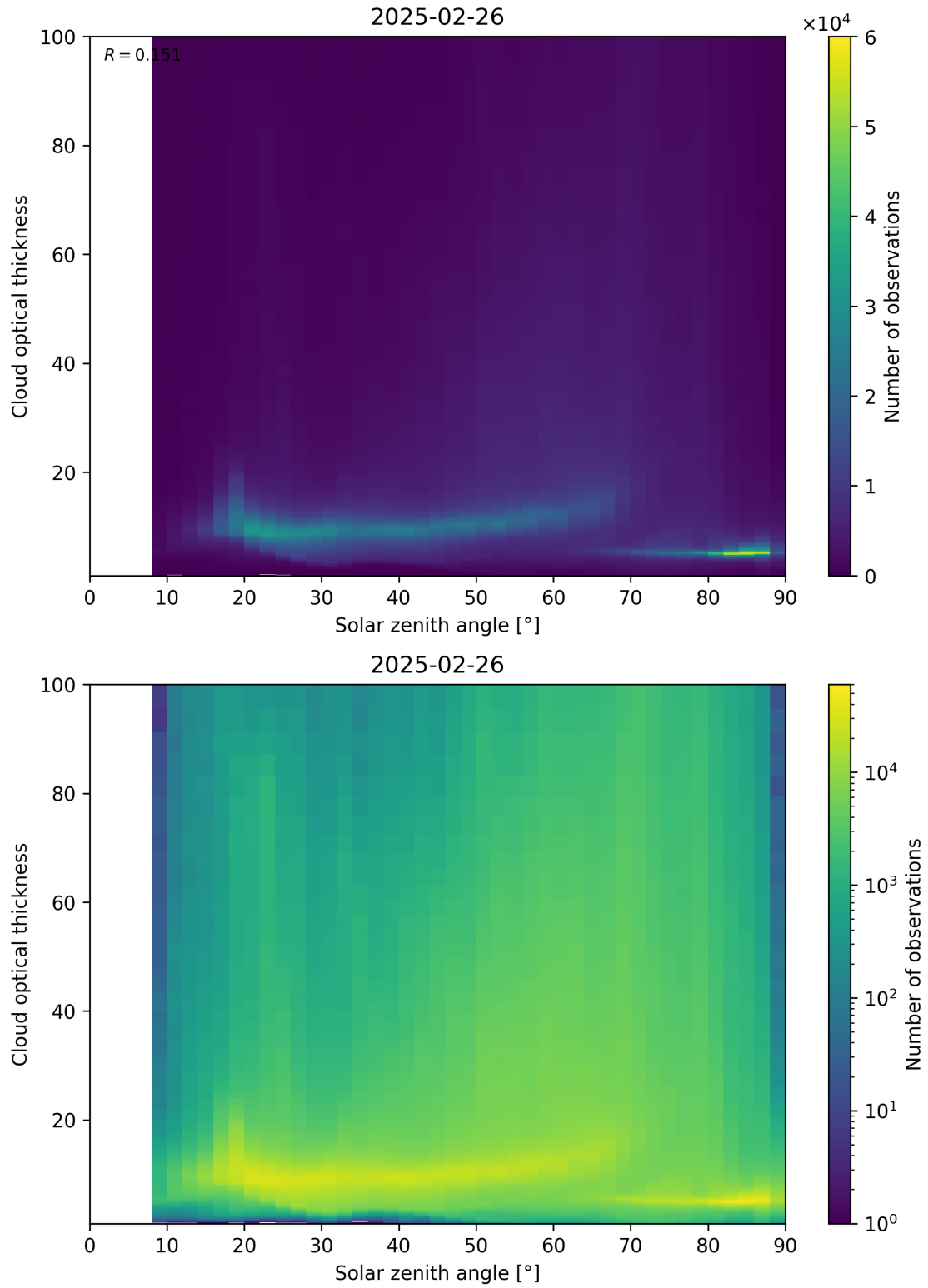
Figure 103: Scatter density plot of “Solar zenith angle” against “Cloud optical thickness” for 2025-02-25 to 2025-02-27.
