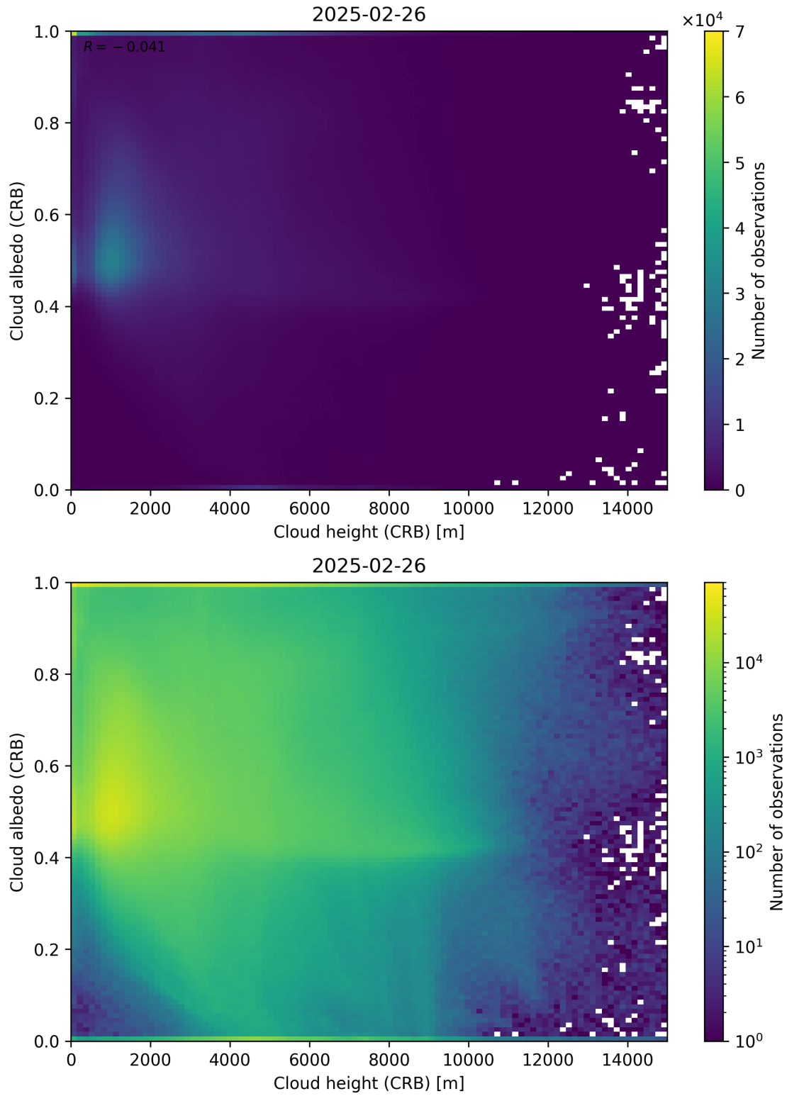
Figure 80: Scatter density plot of “Cloud height (CRB)” against “Cloud albedo (CRB)” for 2025-02-25 to 2025-02-27.
