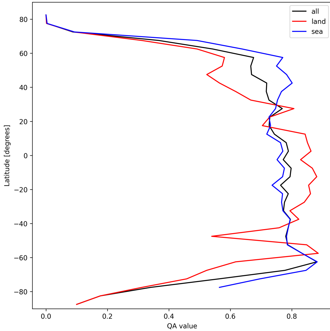
Figure 22: Zonal average of “QA value” for 2025-02-25 to 2025-02-27.
