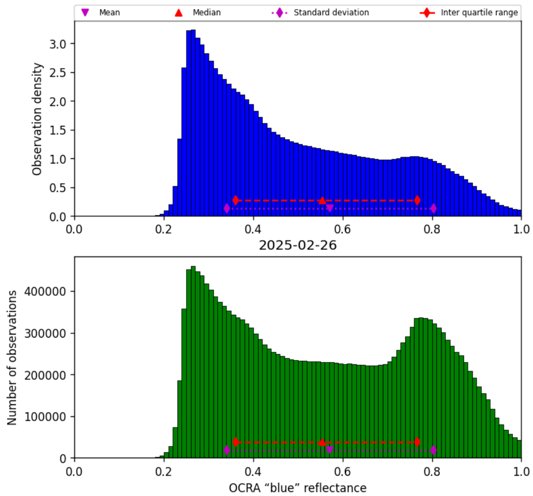
Figure 51: Histogram of “OCRA “blue” reflectance” for 2025-02-25 to 2025-02-27
