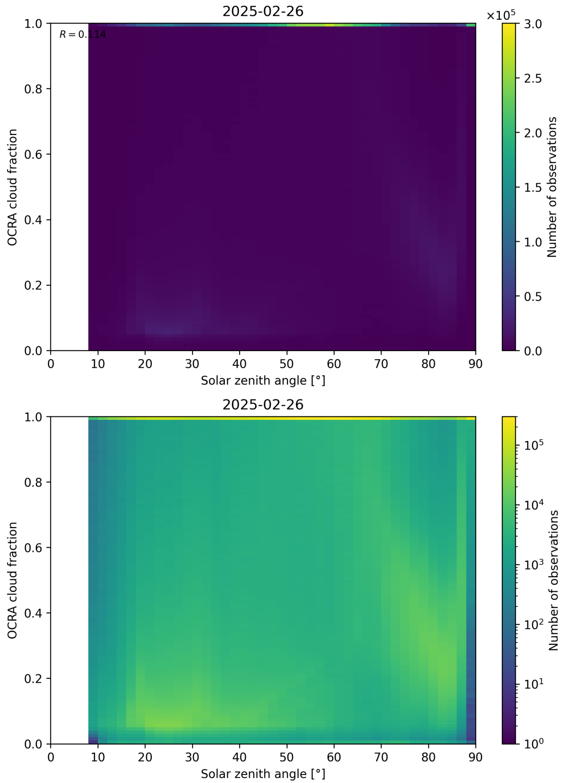
Figure 100: Scatter density plot of “Solar zenith angle” against “OCRA cloud fraction” for 2025-02-25 to 2025-02-27.
