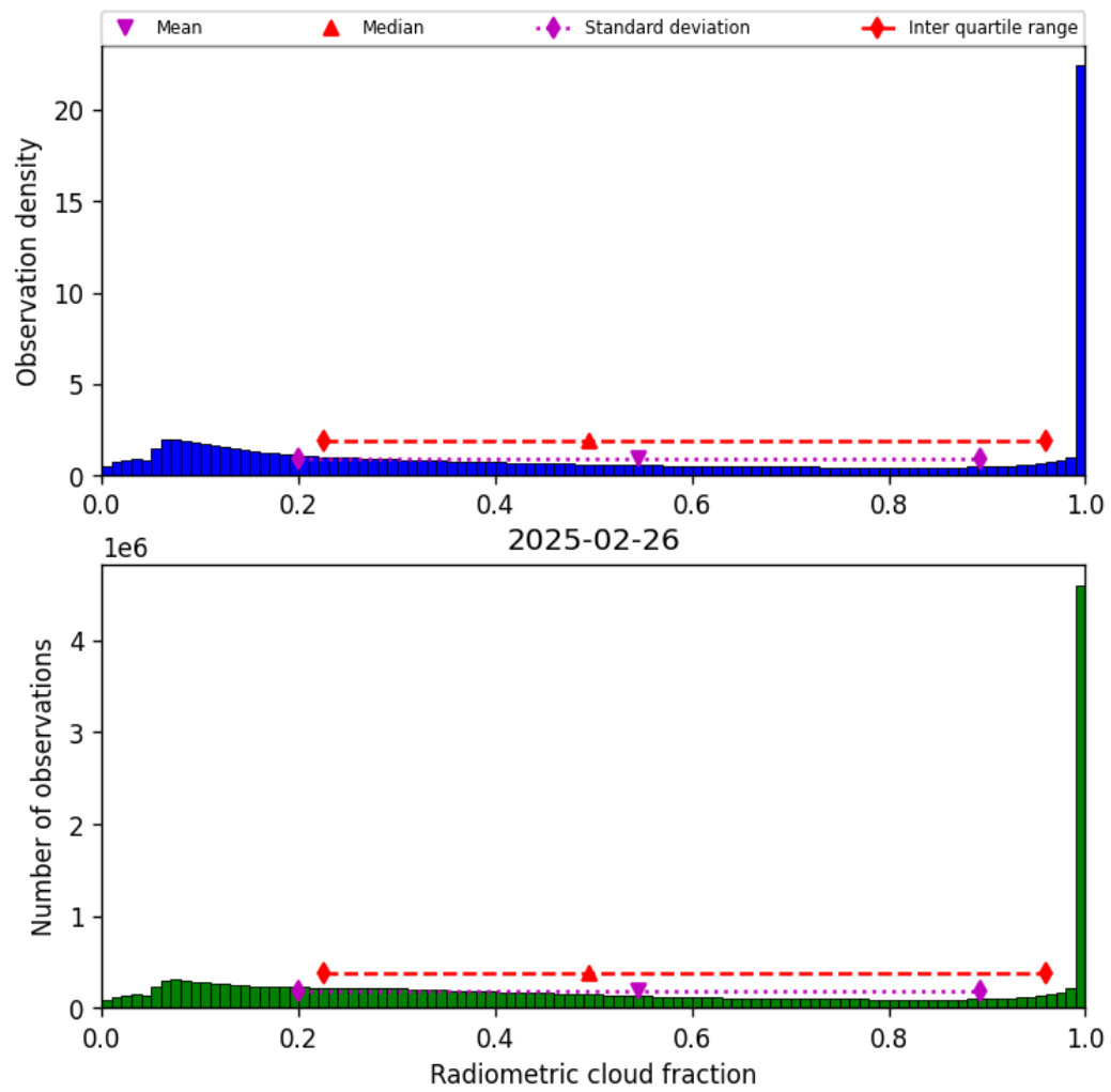
Figure 39: Histogram of “Radiometric cloud fraction” for 2025-02-25 to 2025-02-27
