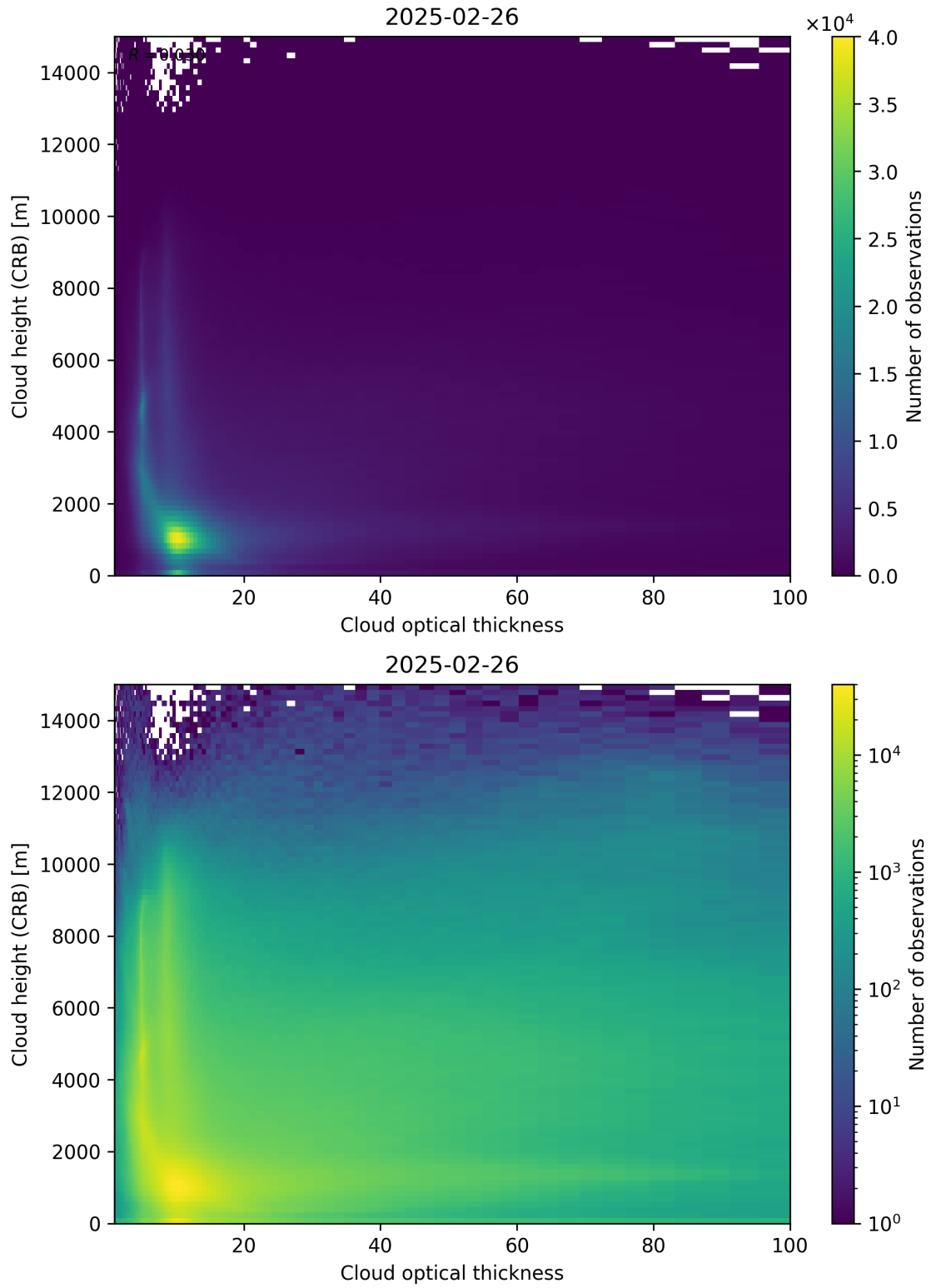
Figure 85: Scatter density plot of “Cloud optical thickness” against “Cloud height (CRB)” for 2025-02-25 to 2025-02-27.
