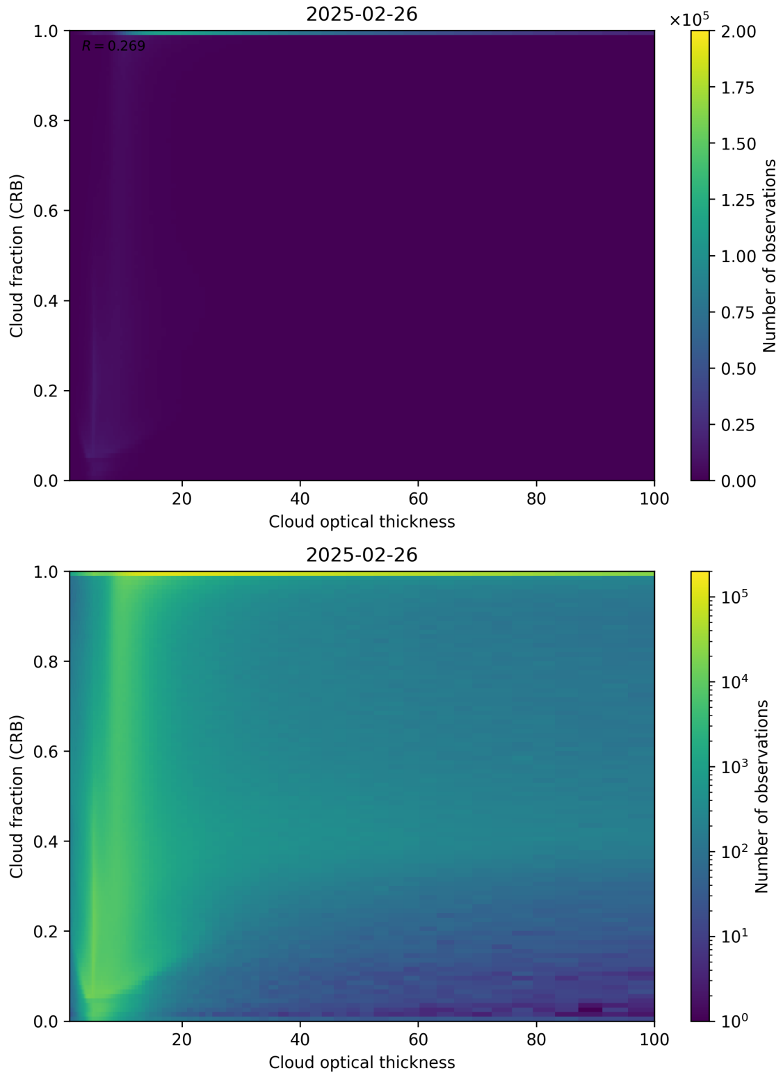
Figure 84: Scatter density plot of “Cloud optical thickness” against “Cloud fraction (CRB)” for 2025-02-25 to 2025-02-27.
