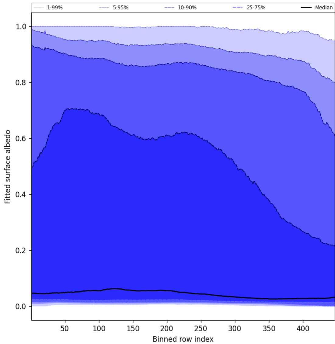
Figure 61: Along track statistics of “Fitted surface albedo” for 2025-02-25 to 2025-02-27
