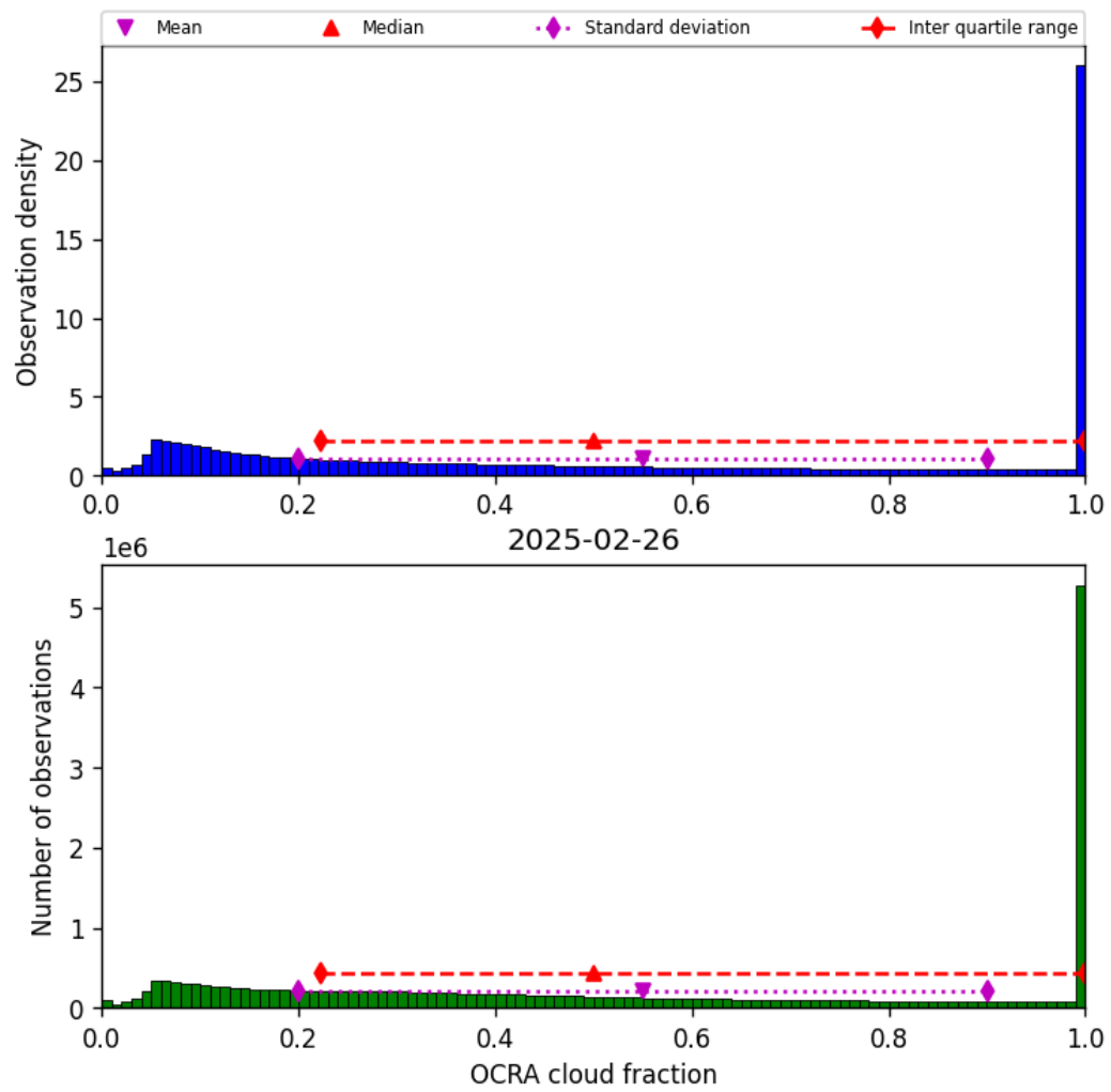
Figure 50: Histogram of “OCRA cloud fraction” for 2025-02-25 to 2025-02-27
