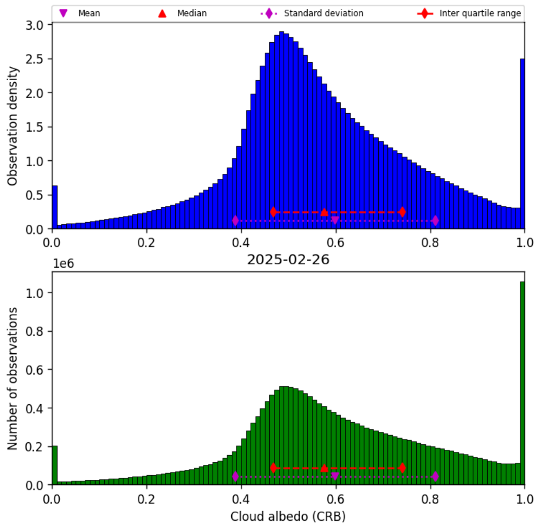
Figure 44: Histogram of “Cloud albedo (CRB)” for 2025-02-25 to 2025-02-27
