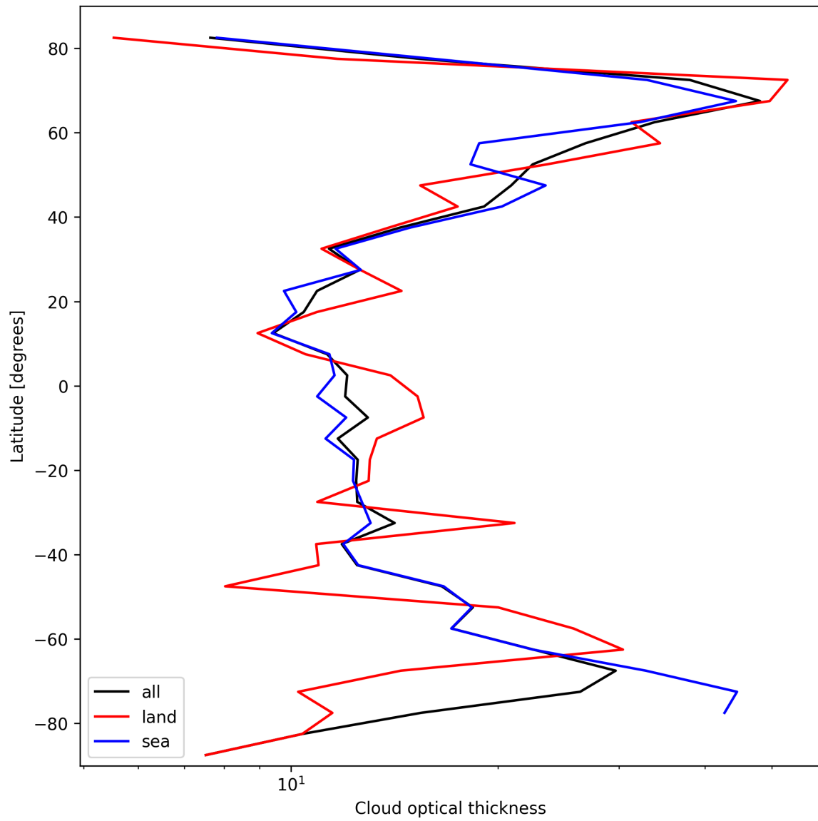
Figure 25: Zonal average of “Cloud optical thickness” for 2025-02-25 to 2025-02-27.
