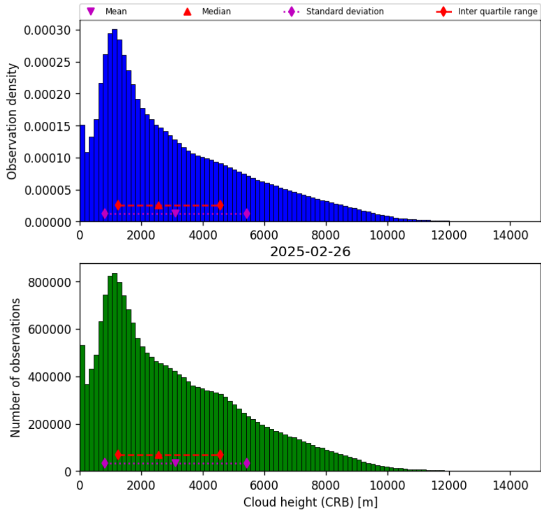
Figure 43: Histogram of “Cloud height (CRB)” for 2025-02-25 to 2025-02-27
