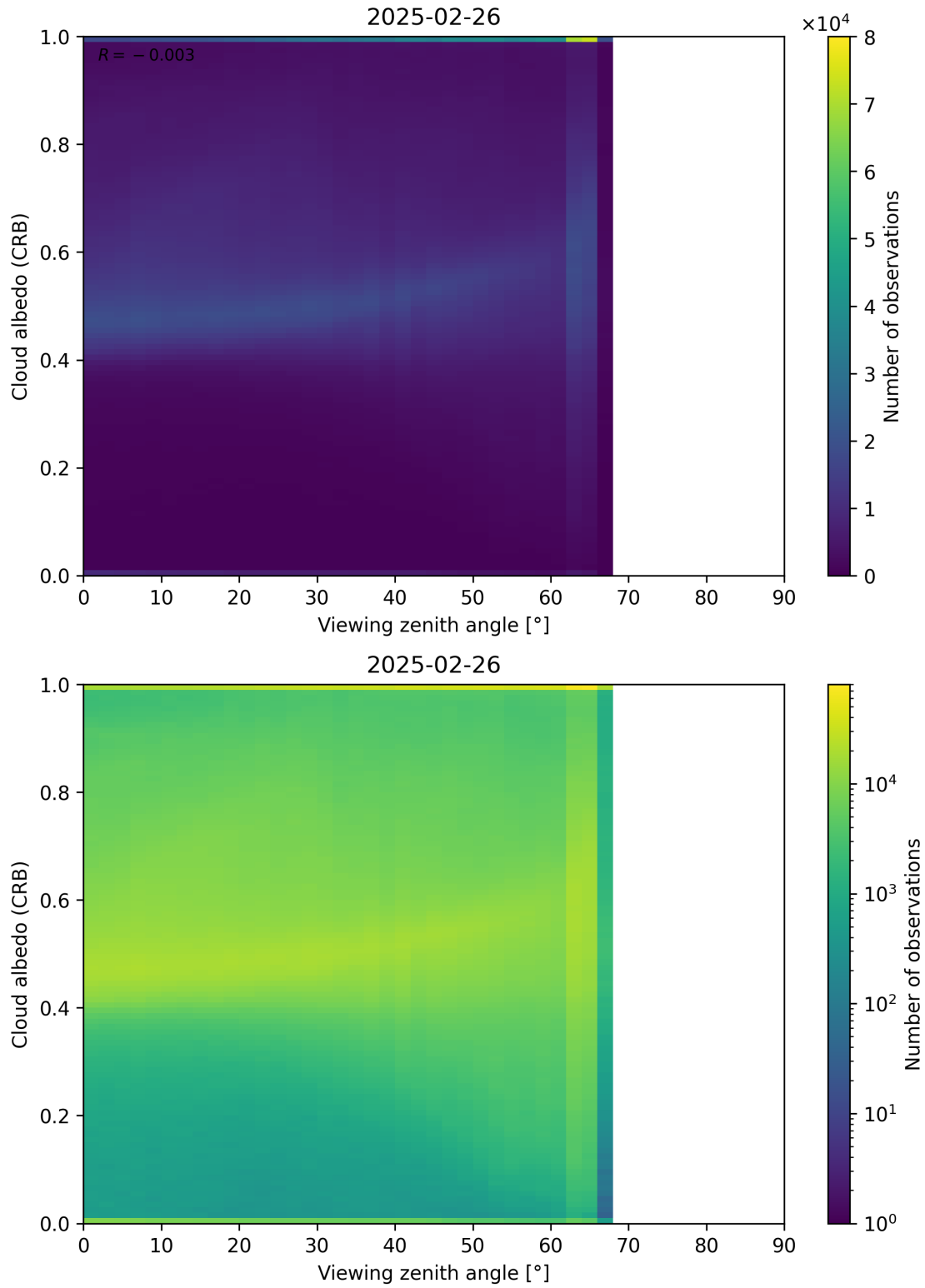
Figure 106: Scatter density plot of “Viewing zenith angle” against “Cloud albedo (CRB)” for 2025-02-25 to 2025-02-27.
