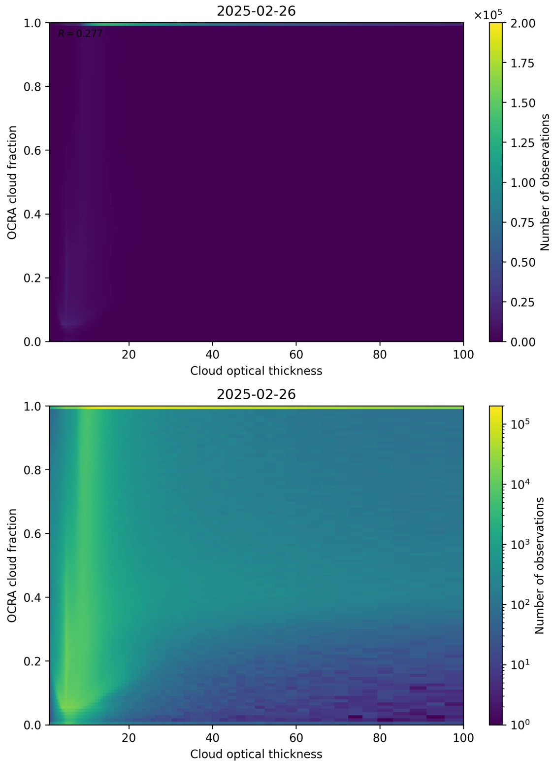
Figure 83: Scatter density plot of “Cloud optical thickness” against “OCRA cloud fraction” for 2025-02-25 to 2025-02-27.
