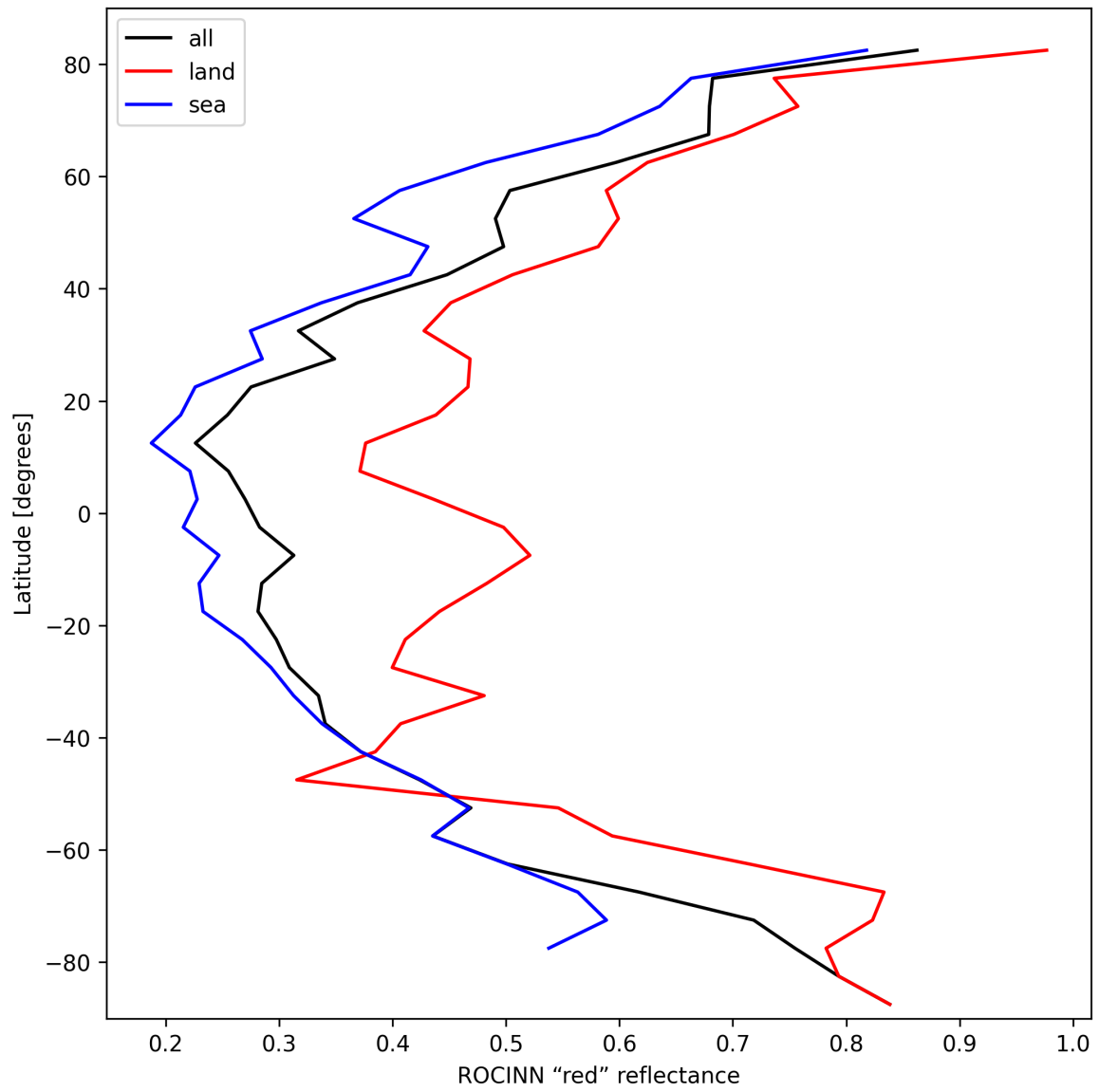
Figure 37: Zonal average of “ROCINN “red” reflectance” for 2025-02-25 to 2025-02-27.
