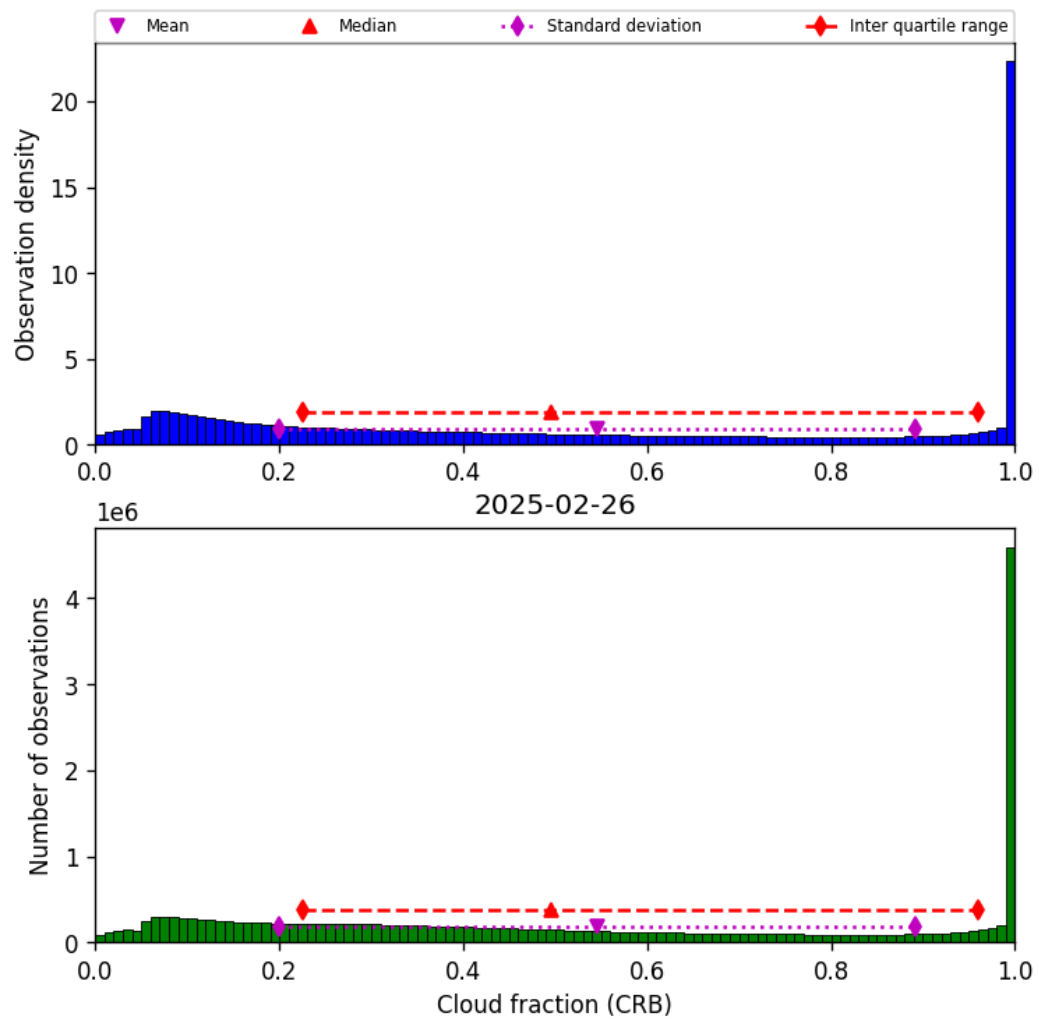
Figure 42: Histogram of “Cloud fraction (CRB)” for 2025-02-25 to 2025-02-27
