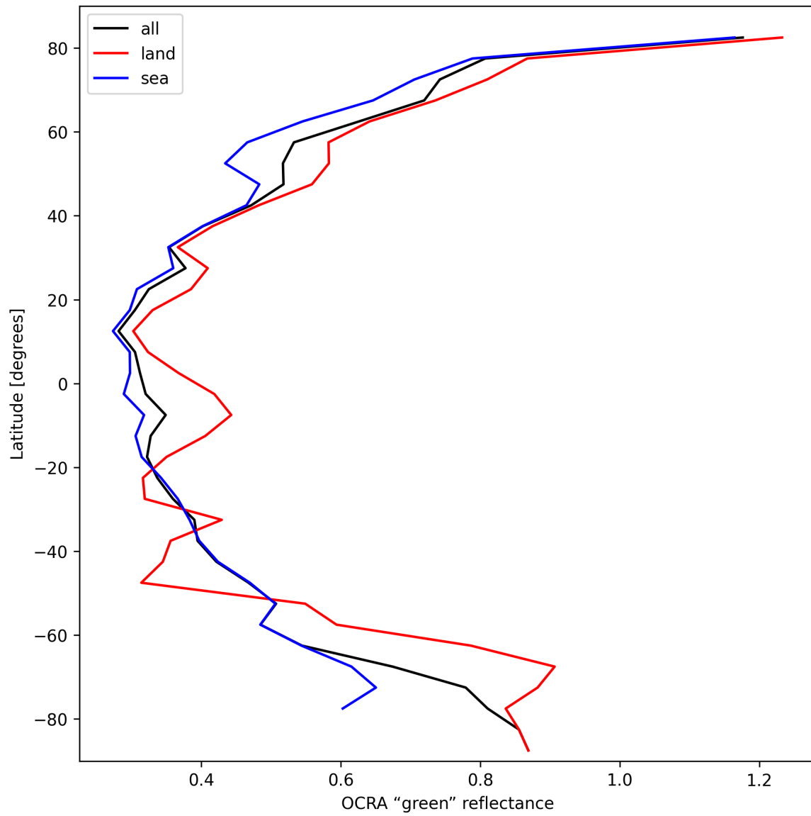
Figure 36: Zonal average of “OCRA “green” reflectance” for 2025-02-25 to 2025-02-27.
