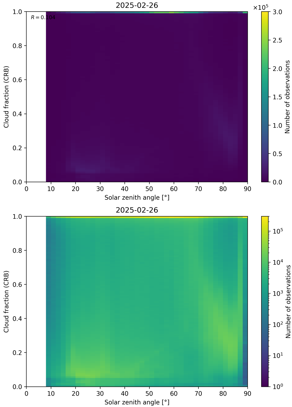
Figure 101: Scatter density plot of “Solar zenith angle” against “Cloud fraction (CRB)” for 2025-02-25 to 2025-02-27.
