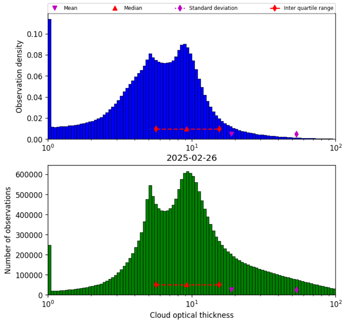
Figure 41: Histogram of “Cloud optical thickness” for 2025-02-25 to 2025-02-27
