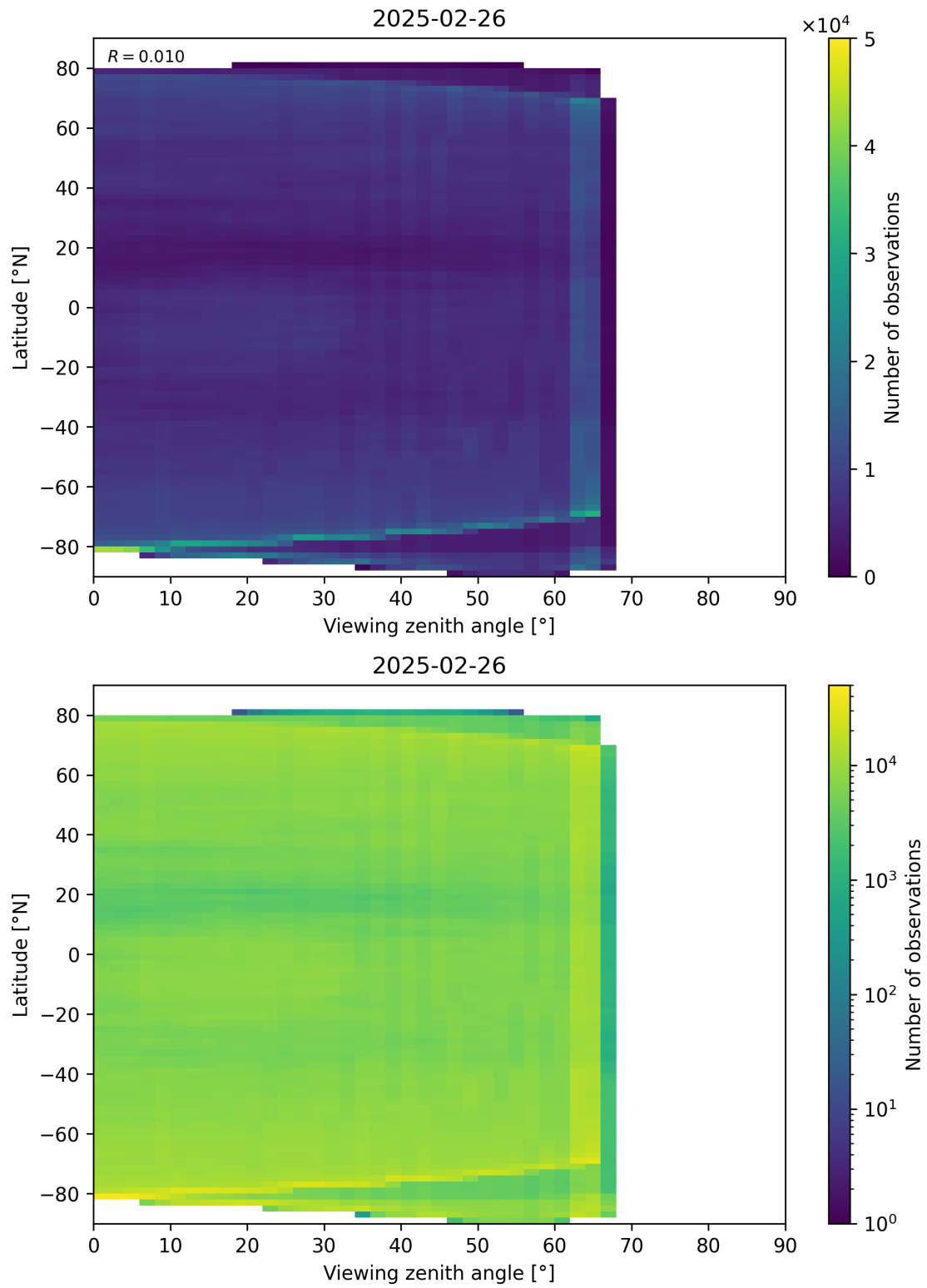
Figure 113: Scatter density plot of “Viewing zenith angle” against “Latitude” for 2025-02-25 to 2025-02-27.
