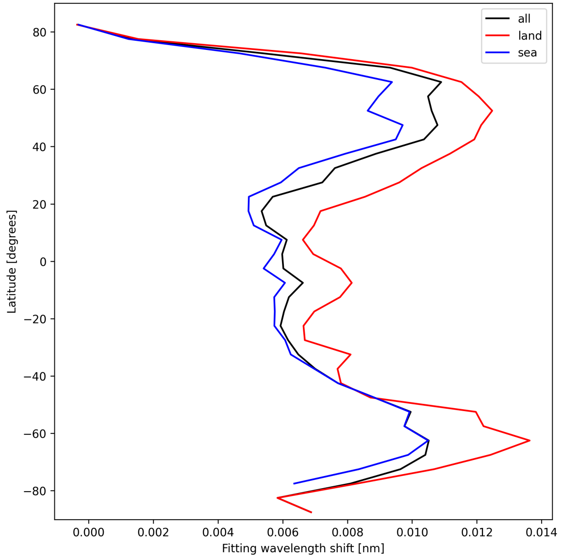
Figure 33: Zonal average of “Fitting wavelength shift” for 2025-02-25 to 2025-02-27.
