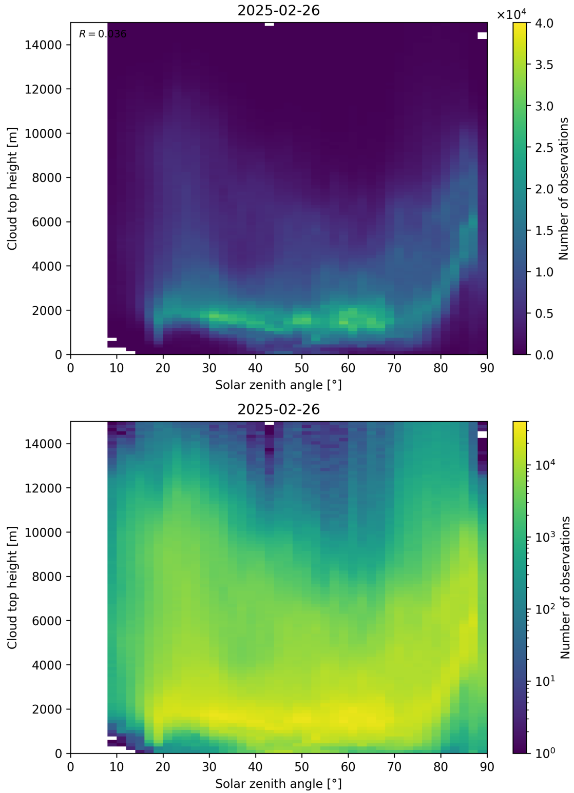
Figure 104: Scatter density plot of “Solar zenith angle” against “Cloud top height” for 2025-02-25 to 2025-02-27.
