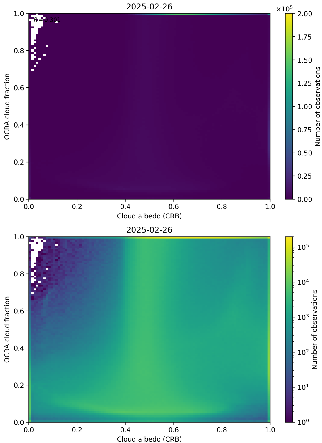
Figure 70: Scatter density plot of “Cloud albedo (CRB)” against “OCRA cloud fraction” for 2025-02-25 to 2025-02-27.
