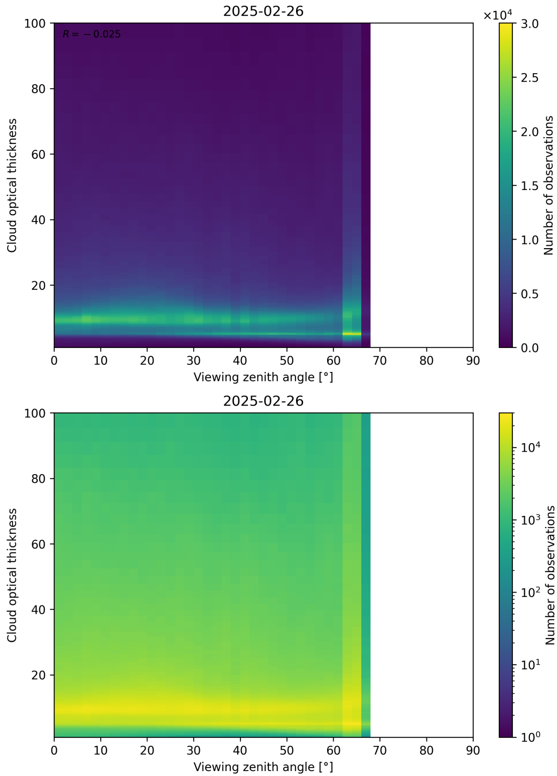
Figure 111: Scatter density plot of “Viewing zenith angle” against “Cloud optical thickness” for 2025-02-25 to 2025-02-27.
