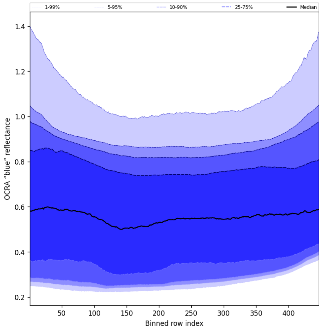
Figure 67: Along track statistics of “OCRA “blue” reflectance” for 2025-02-25 to 2025-02-27
