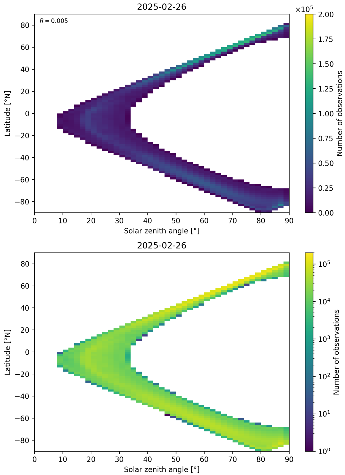
Figure 105: Scatter density plot of “Solar zenith angle” against “Latitude” for 2025-02-25 to 2025-02-27.
