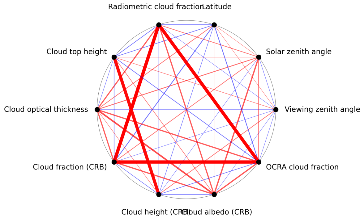
Figure 1: Map of correlation graph for 2025-02-25 to 2025-02-27.
