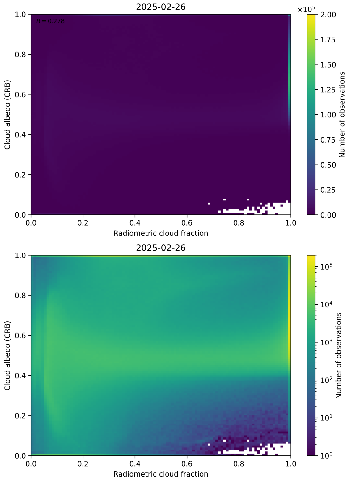
Figure 71: Scatter density plot of “Radiometric cloud fraction” against “Cloud albedo (CRB)” for 2025-02-25 to 2025-02-27.
