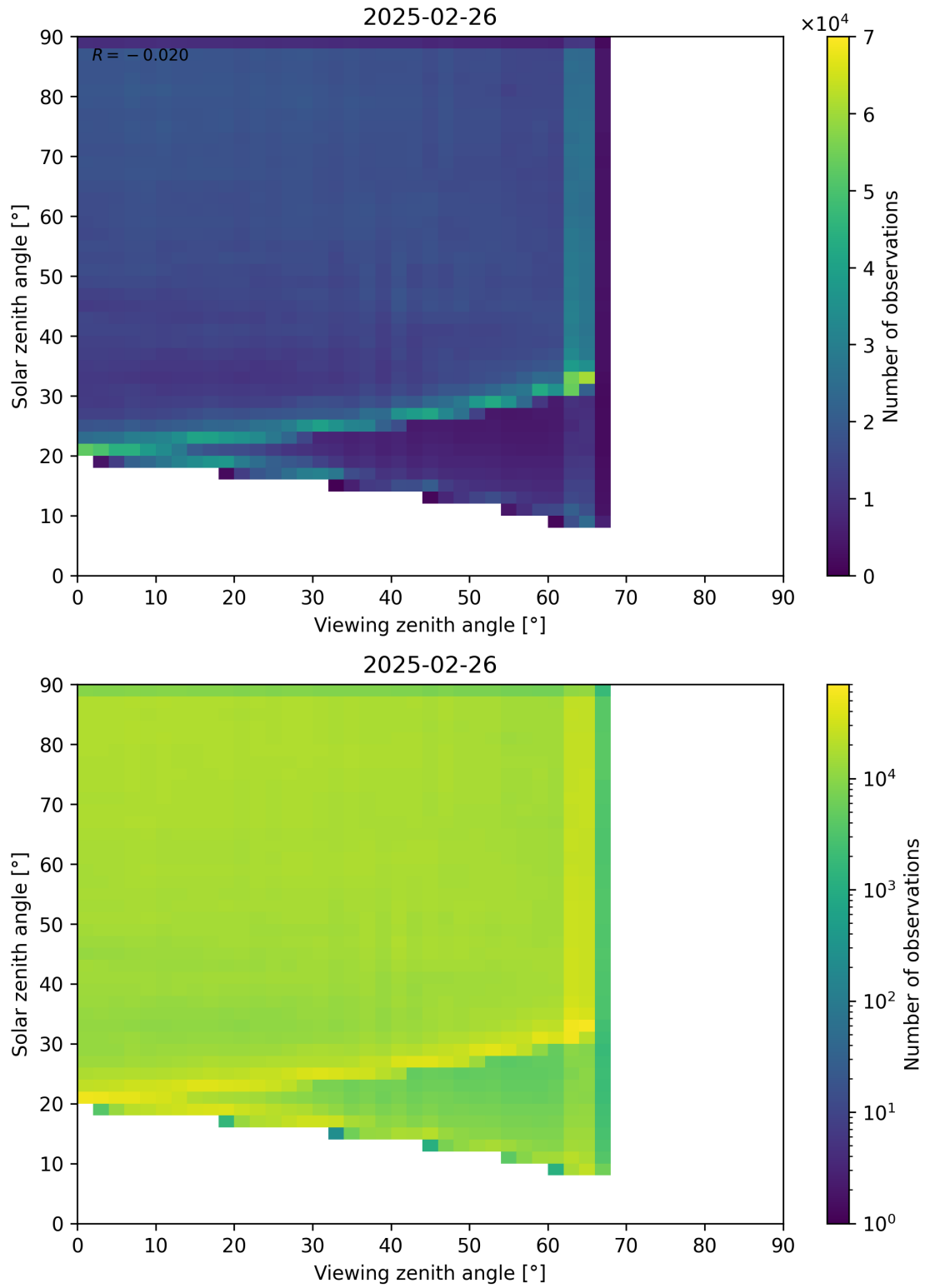
Figure 114: Scatter density plot of “Viewing zenith angle” against “Solar zenith angle” for 2025-02-25 to 2025-02-27.
