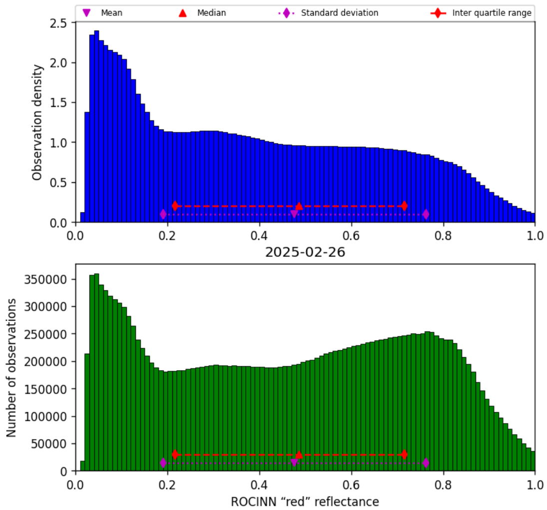
Figure 53: Histogram of “ROCINN “red” reflectance” for 2025-02-25 to 2025-02-27
