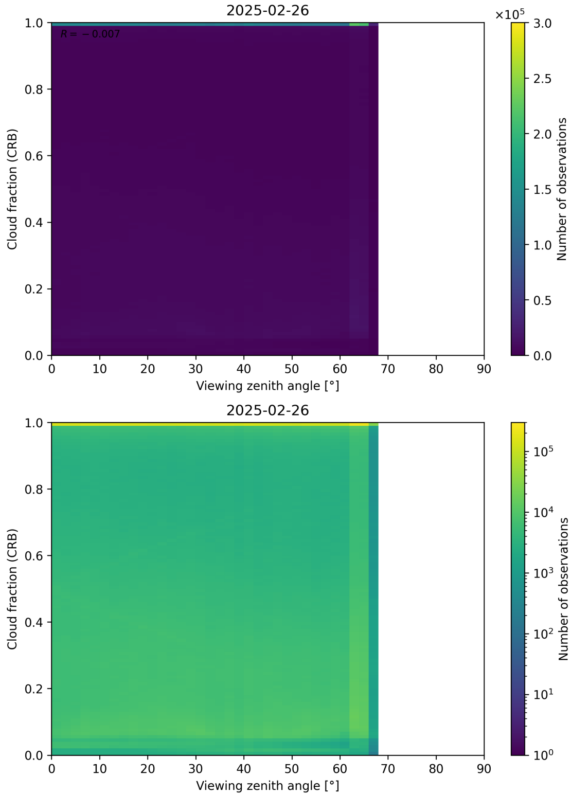
Figure 109: Scatter density plot of “Viewing zenith angle” against “Cloud fraction (CRB)” for 2025-02-25 to 2025-02-27.
