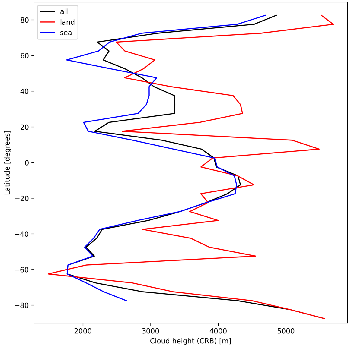
Figure 27: Zonal average of “Cloud height (CRB)” for 2025-02-25 to 2025-02-27.
