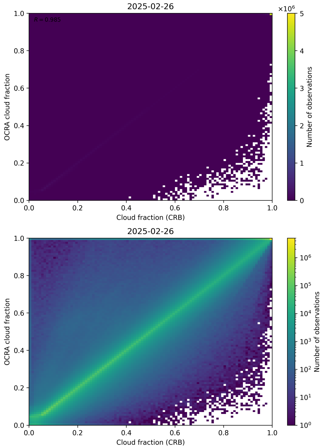
Figure 78: Scatter density plot of “Cloud fraction (CRB)” against “OCRA cloud fraction” for 2025-02-25 to 2025-02-27.
