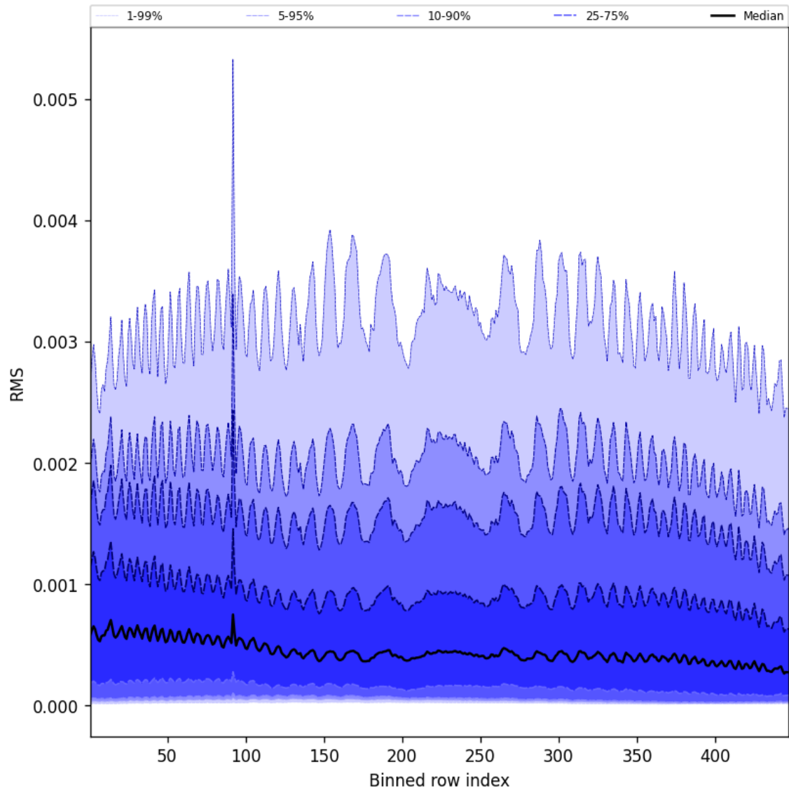
Figure 63: Along track statistics of “RMS” for 2025-02-25 to 2025-02-27
