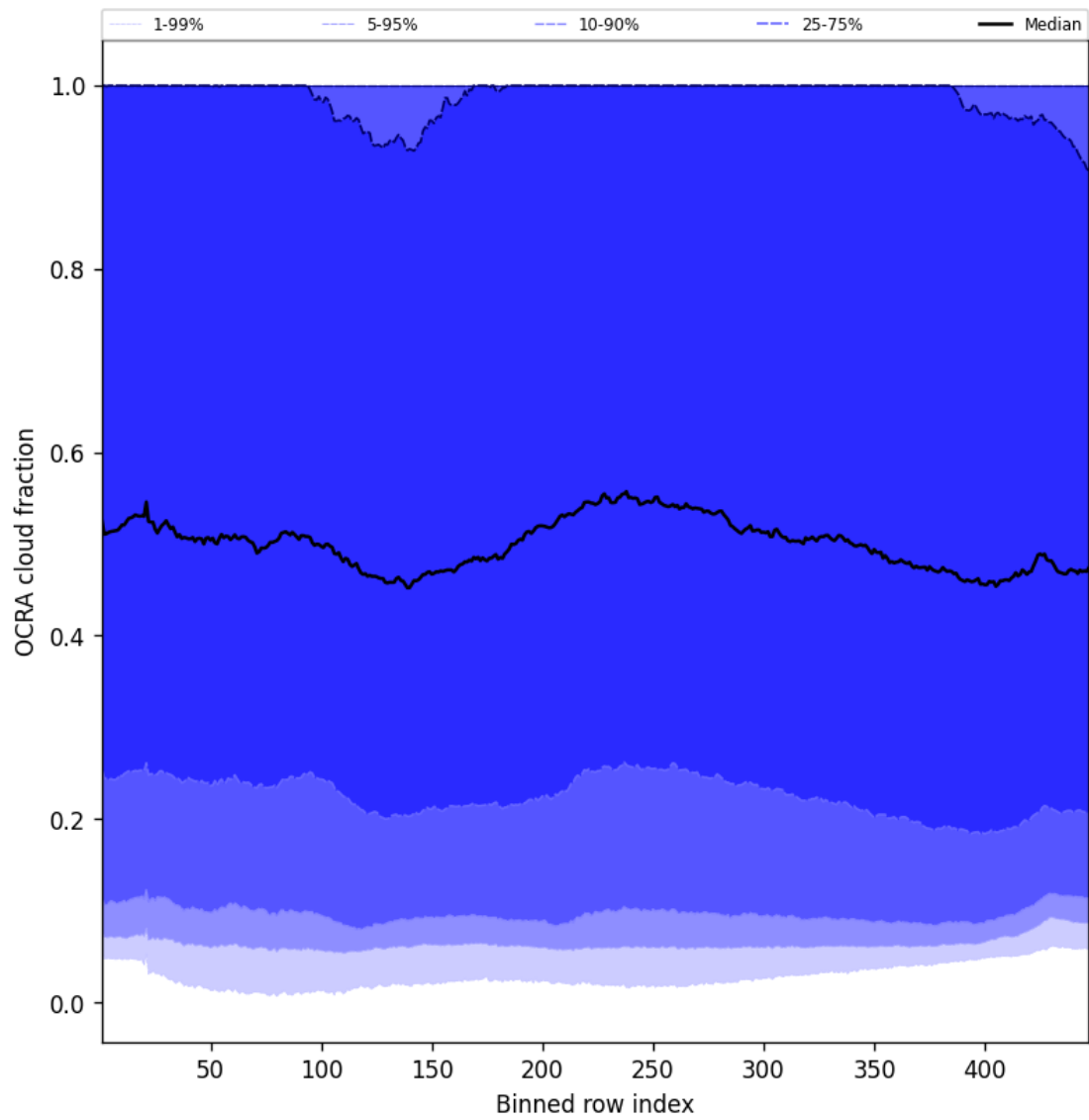
Figure 66: Along track statistics of “OCRA cloud fraction” for 2025-02-25 to 2025-02-27
