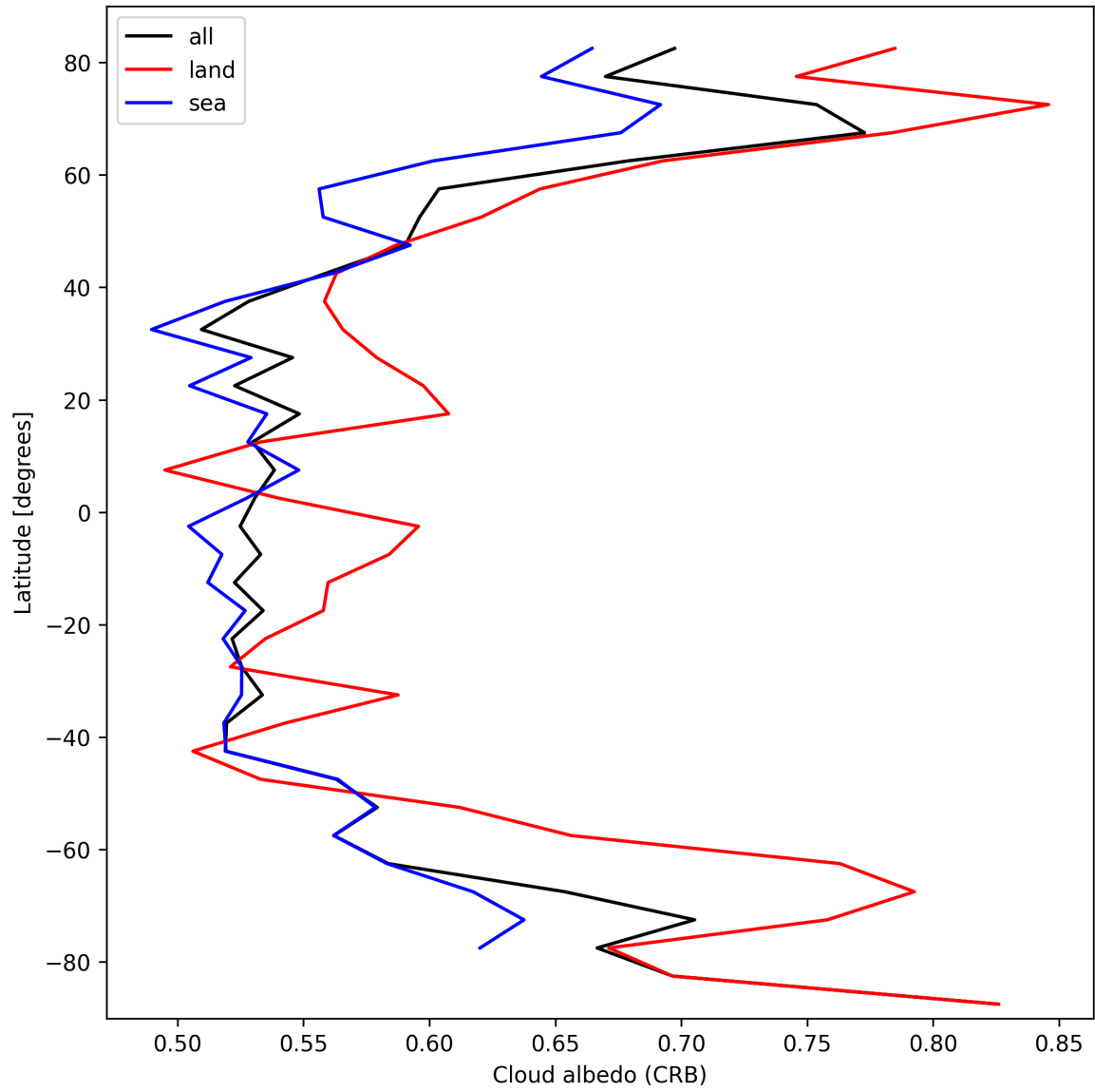
Figure 28: Zonal average of “Cloud albedo (CRB)” for 2025-02-25 to 2025-02-27.
