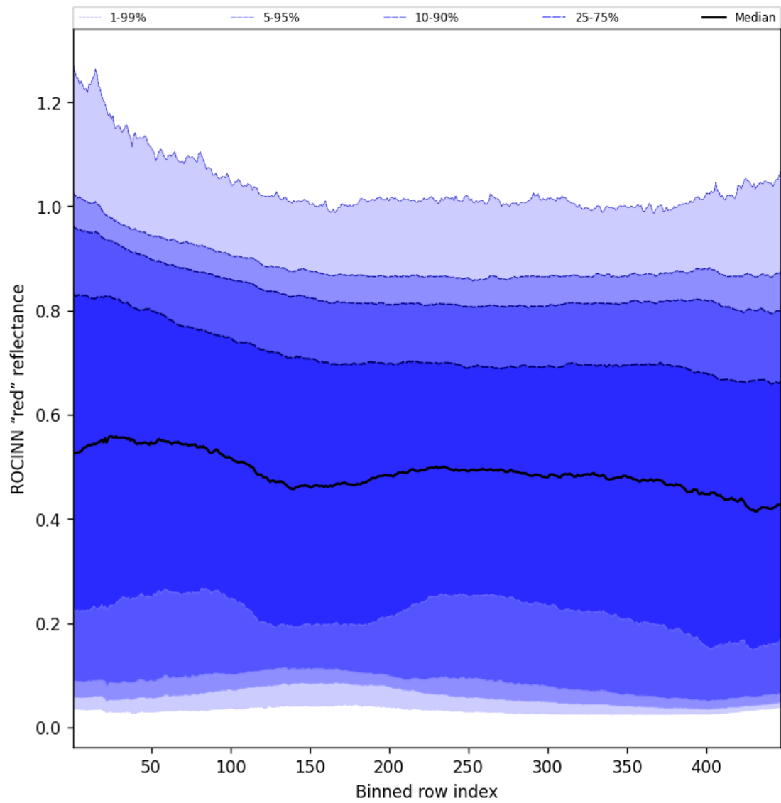
Figure 69: Along track statistics of "ROCINN "red" reflectance" for 2025-02-25 to 2025-02-27
