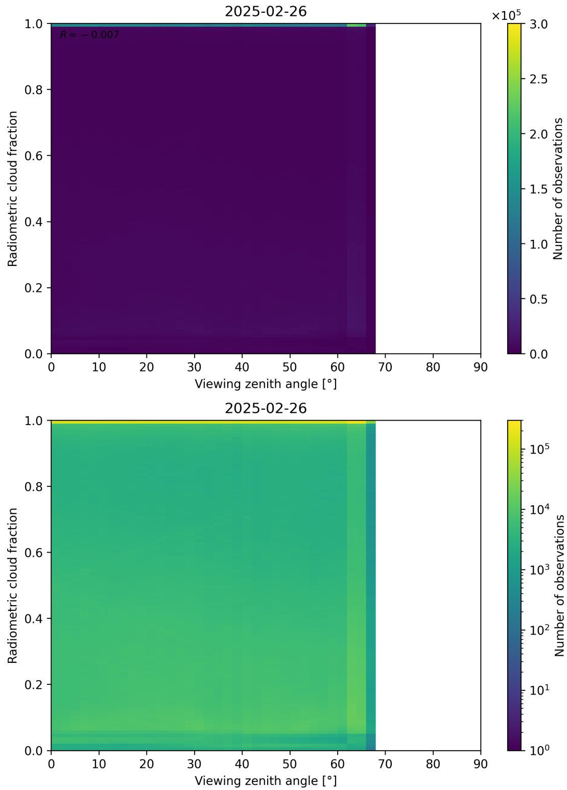
Figure 107: Scatter density plot of “Viewing zenith angle” against “Radiometric cloud fraction” for 2025-02-25 to 2025-02-27.
