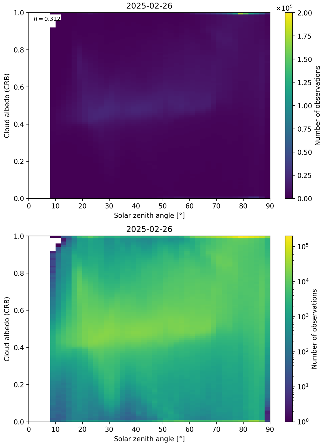
Figure 98: Scatter density plot of “Solar zenith angle” against “Cloud albedo (CRB)” for 2025-02-25 to 2025-02-27.
