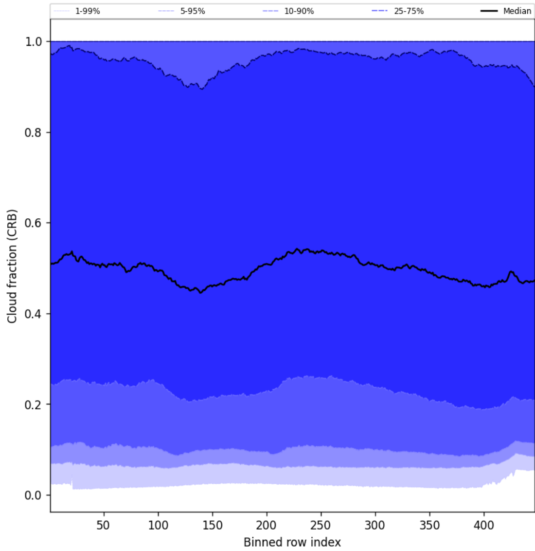
Figure 58: Along track statistics of “Cloud fraction (CRB)” for 2025-02-25 to 2025-02-27
