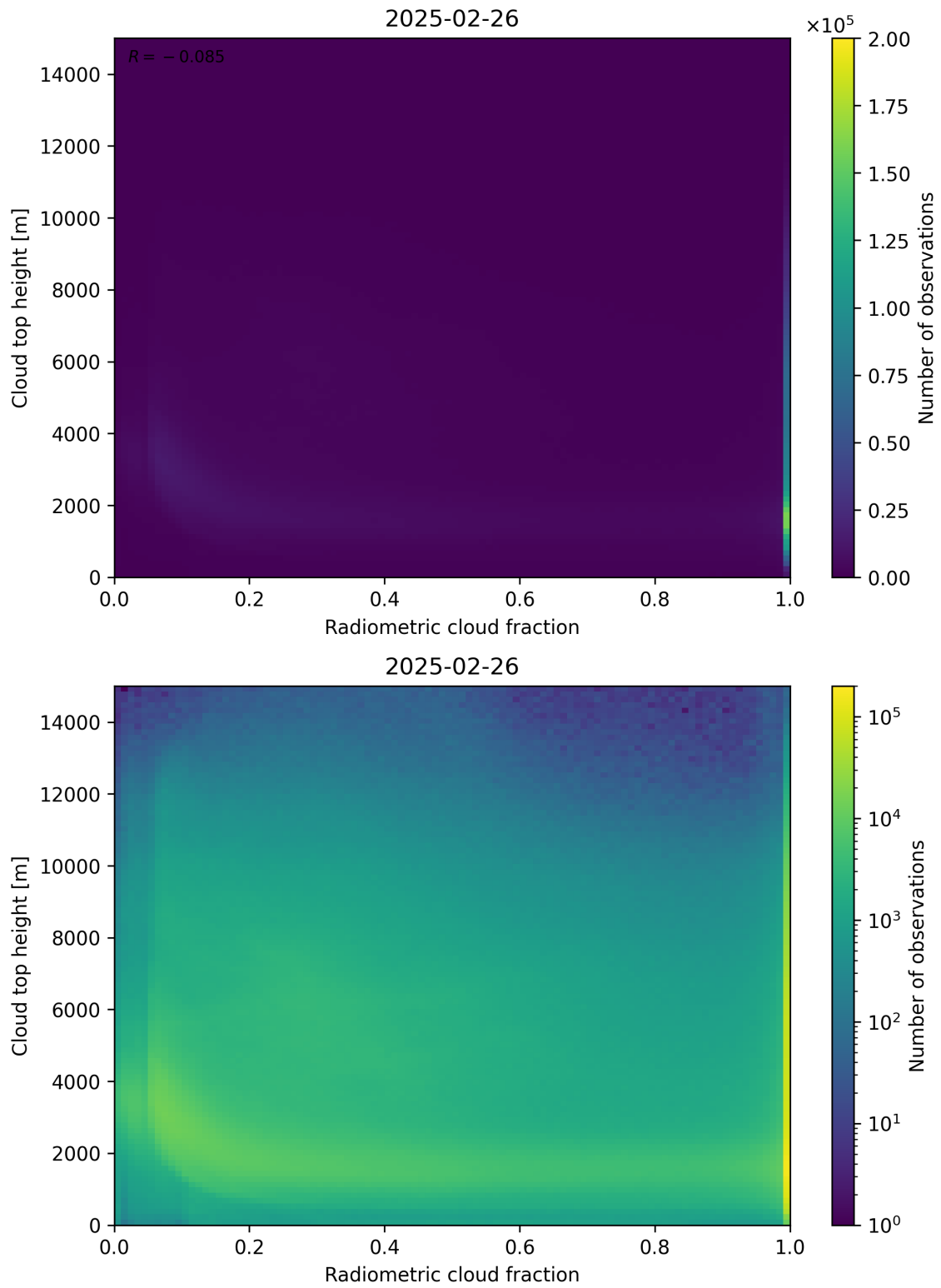
Figure 76: Scatter density plot of “Radiometric cloud fraction” against “Cloud top height” for 2025-02-25 to 2025-02-27.
