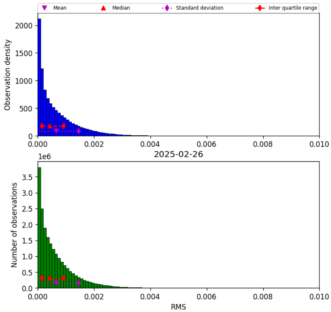
Figure 47: Histogram of “RMS” for 2025-02-25 to 2025-02-27
