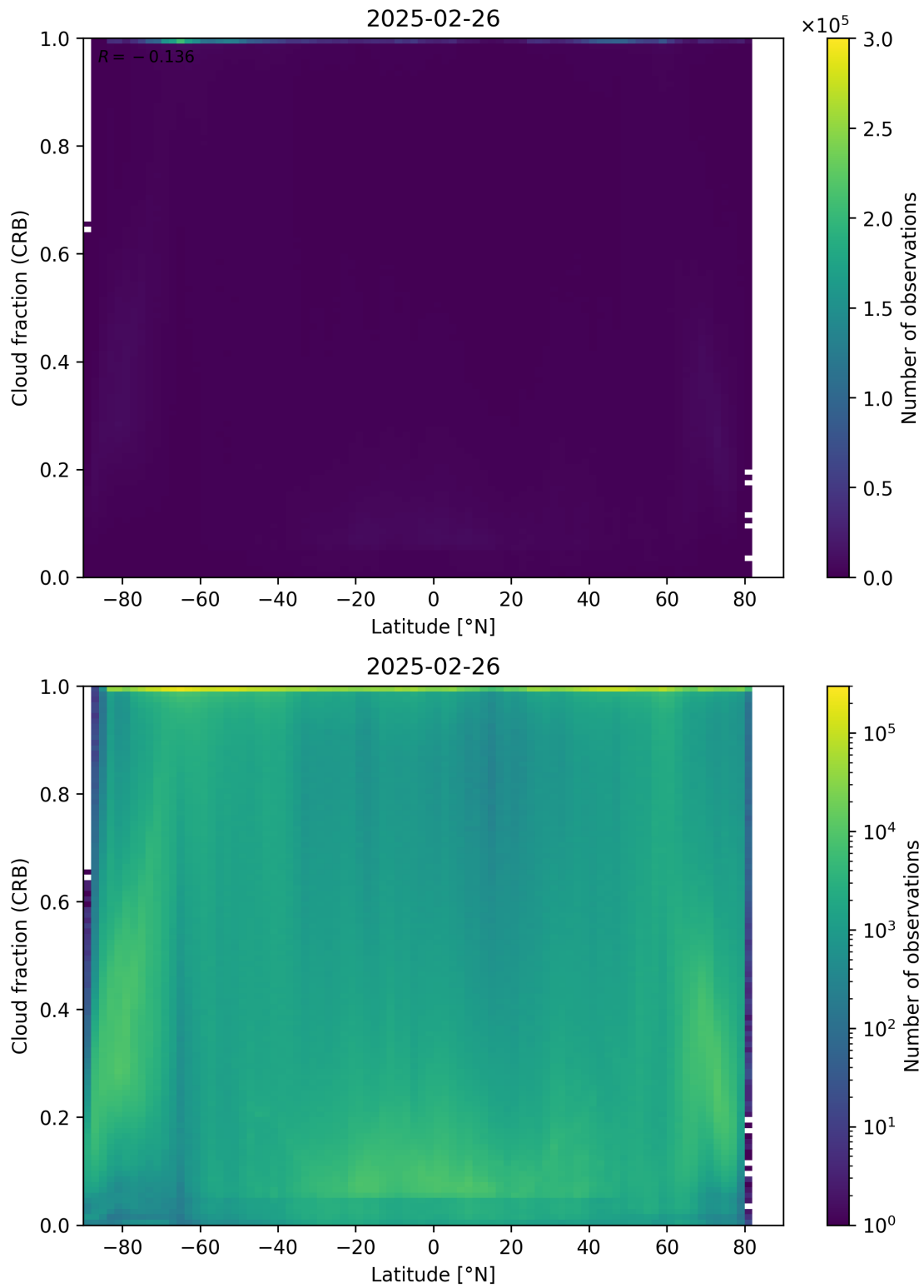
Figure 94: Scatter density plot of “Latitude” against “Cloud fraction (CRB)” for 2025-02-25 to 2025-02-27.
