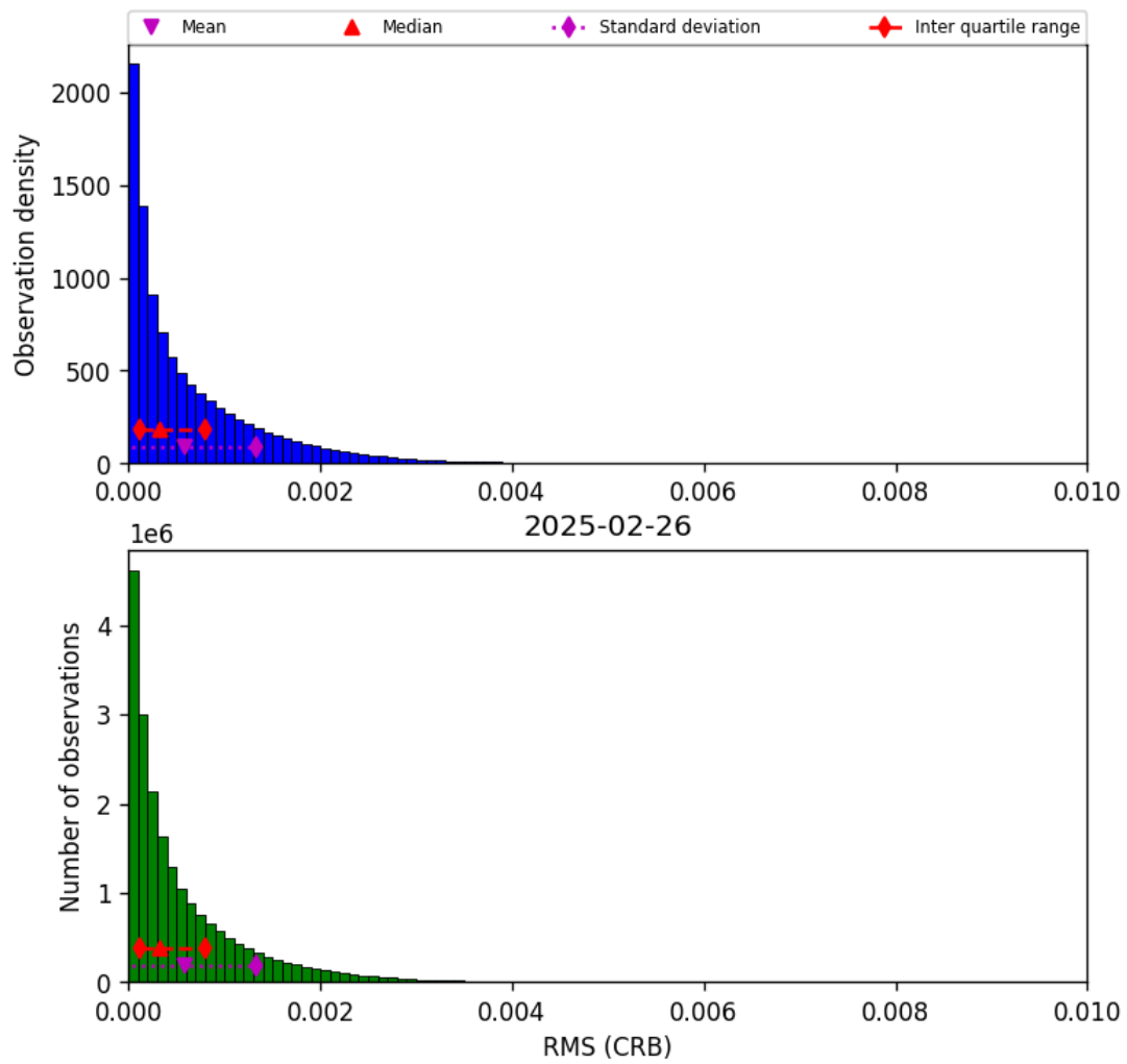
Figure 48: Histogram of “RMS (CRB)” for 2025-02-25 to 2025-02-27
