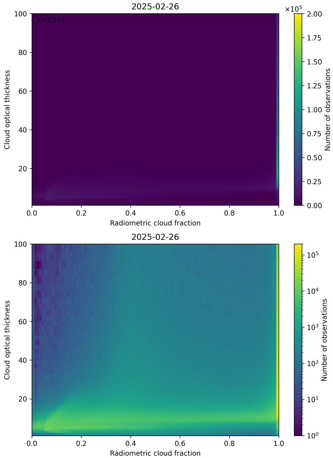
Figure 75: Scatter density plot of “Radiometric cloud fraction” against “Cloud optical thickness” for 2025-02-25 to 2025-02-27.
