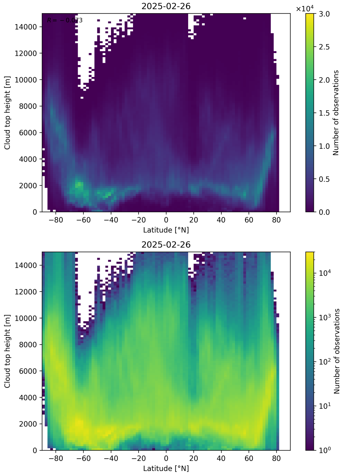
Figure 97: Scatter density plot of “Latitude” against “Cloud top height” for 2025-02-25 to 2025-02-27.
