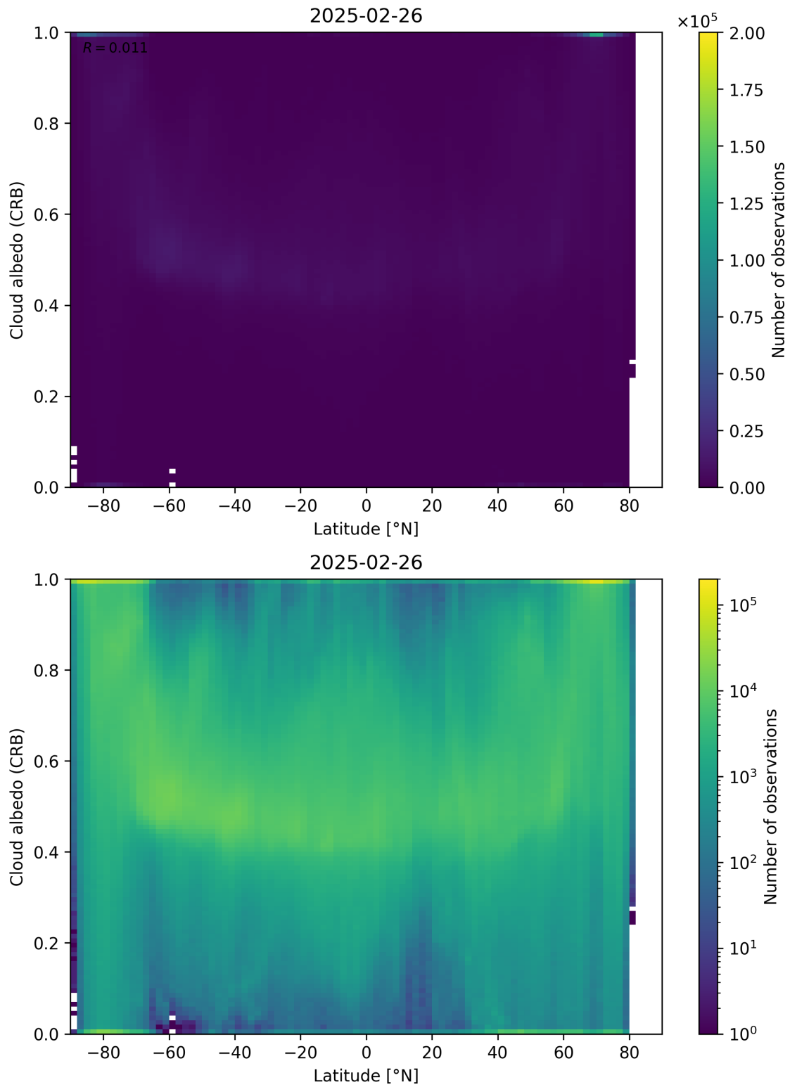
Figure 91: Scatter density plot of “Latitude” against “Cloud albedo (CRB)” for 2025-02-25 to 2025-02-27.
