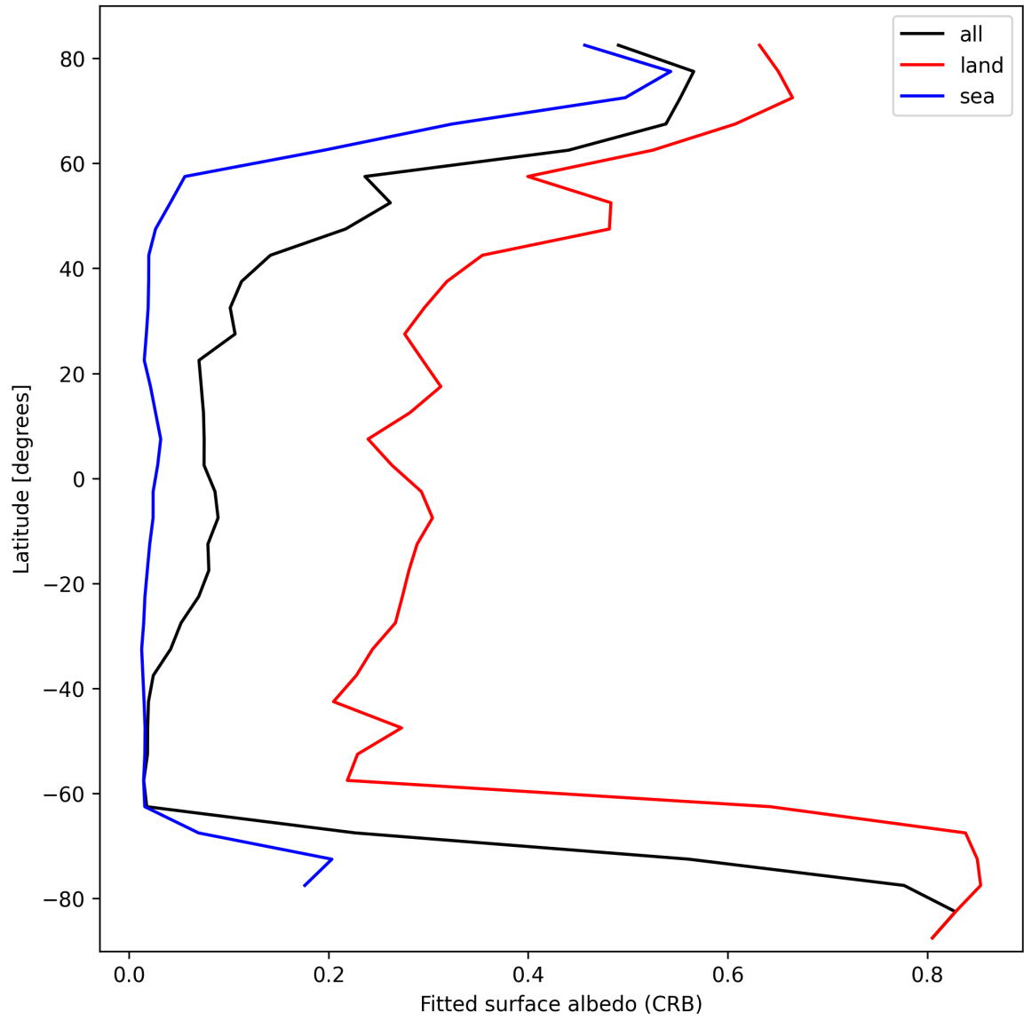
Figure 30: Zonal average of “Fitted surface albedo (CRB)” for 2025-02-25 to 2025-02-27.
