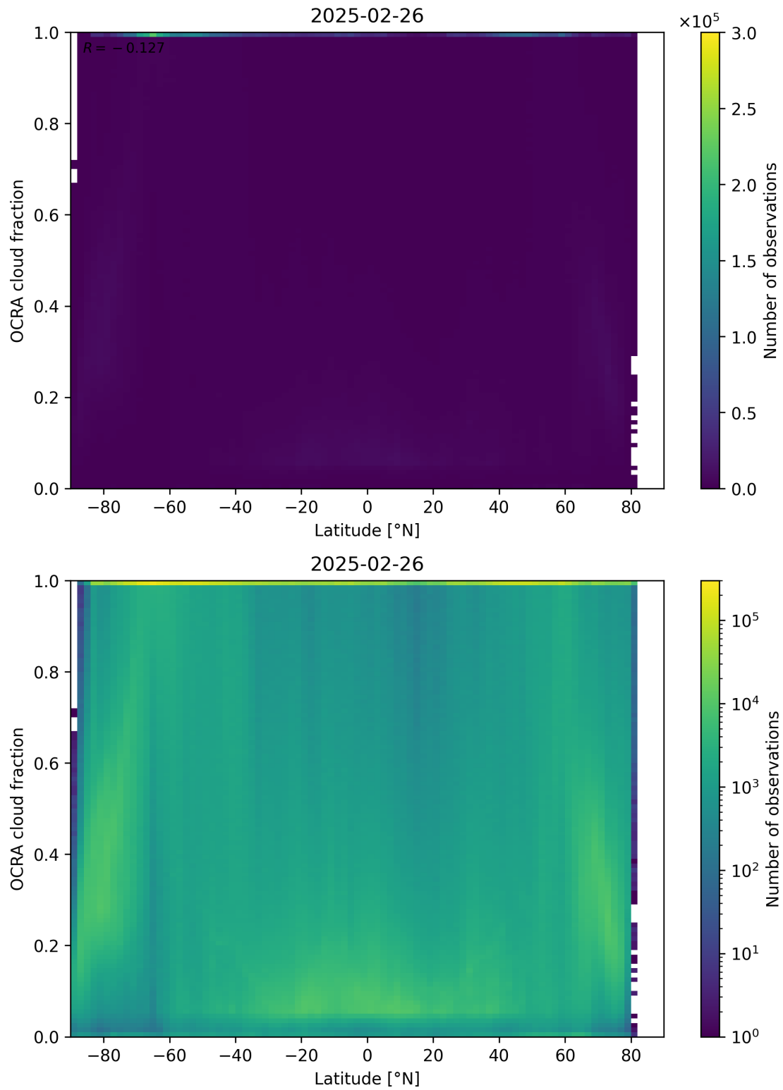
Figure 93: Scatter density plot of “Latitude” against “OCRA cloud fraction” for 2025-02-25 to 2025-02-27.
