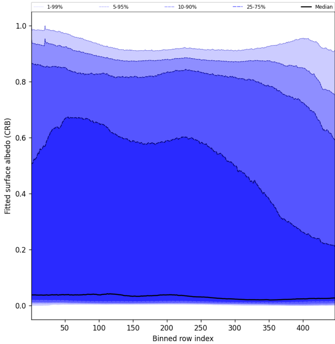
Figure 62: Along track statistics of “Fitted surface albedo (CRB)” for 2025-02-25 to 2025-02-27
