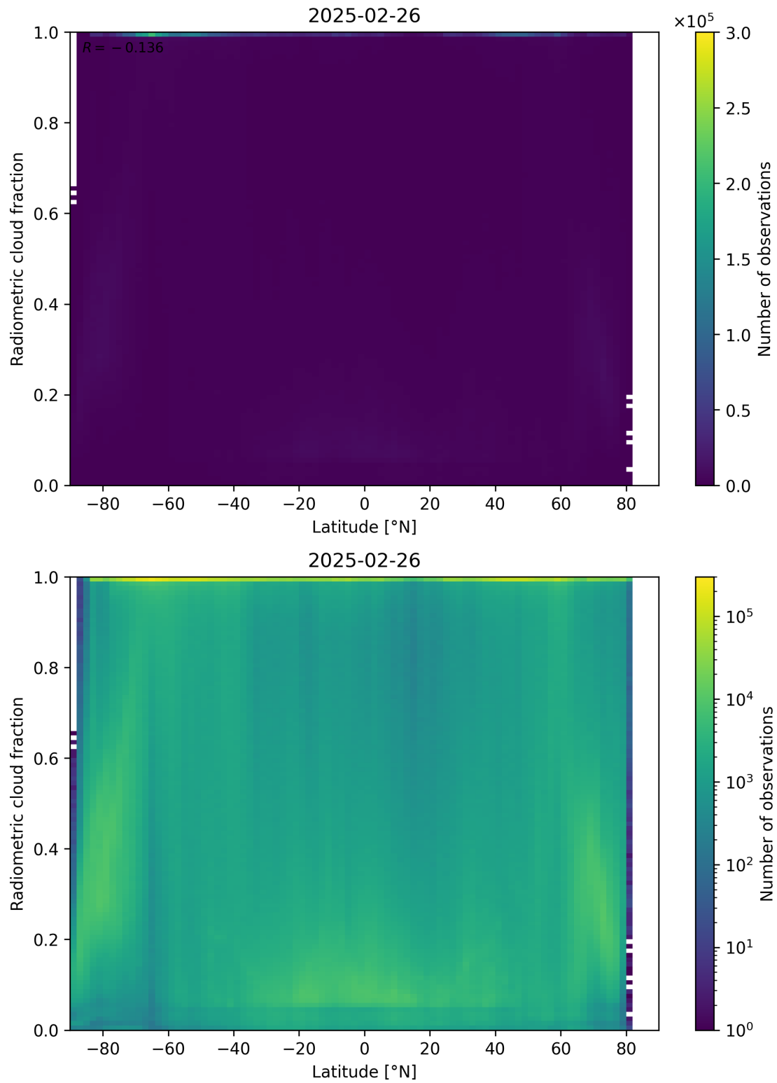
Figure 92: Scatter density plot of “Latitude” against “Radiometric cloud fraction” for 2025-02-25 to 2025-02-27.
