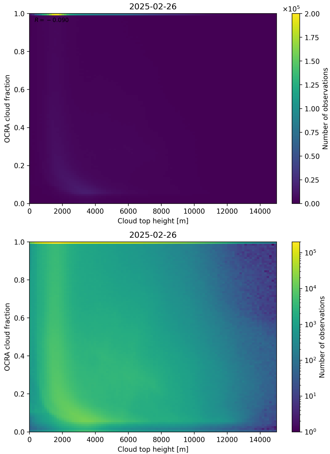
Figure 87: Scatter density plot of “Cloud top height” against “OCRA cloud fraction” for 2025-02-25 to 2025-02-27.
