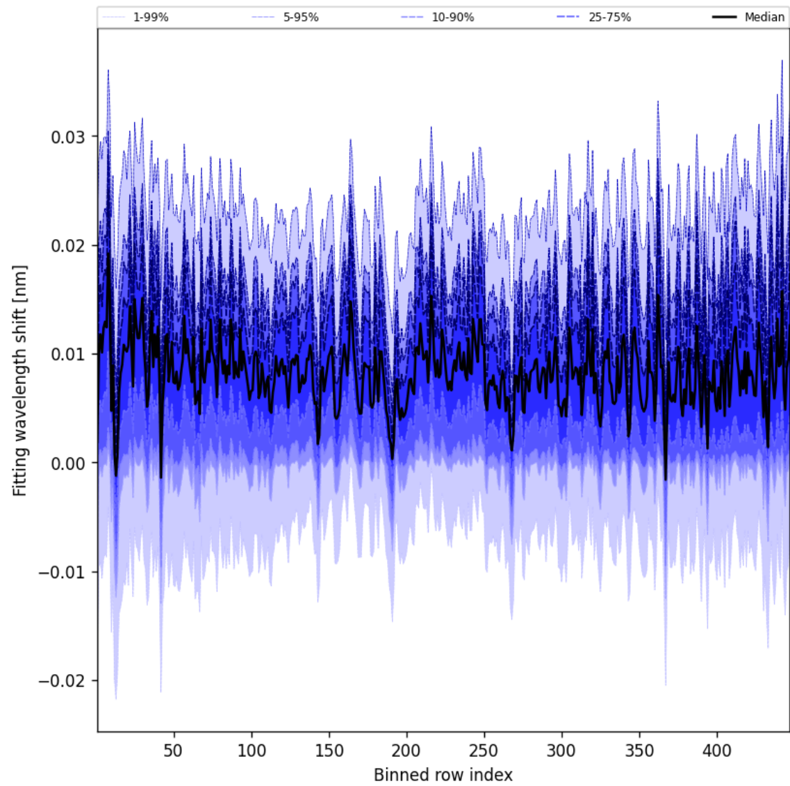
Figure 65: Along track statistics of “Fitting wavelength shift” for 2025-02-25 to 2025-02-27
