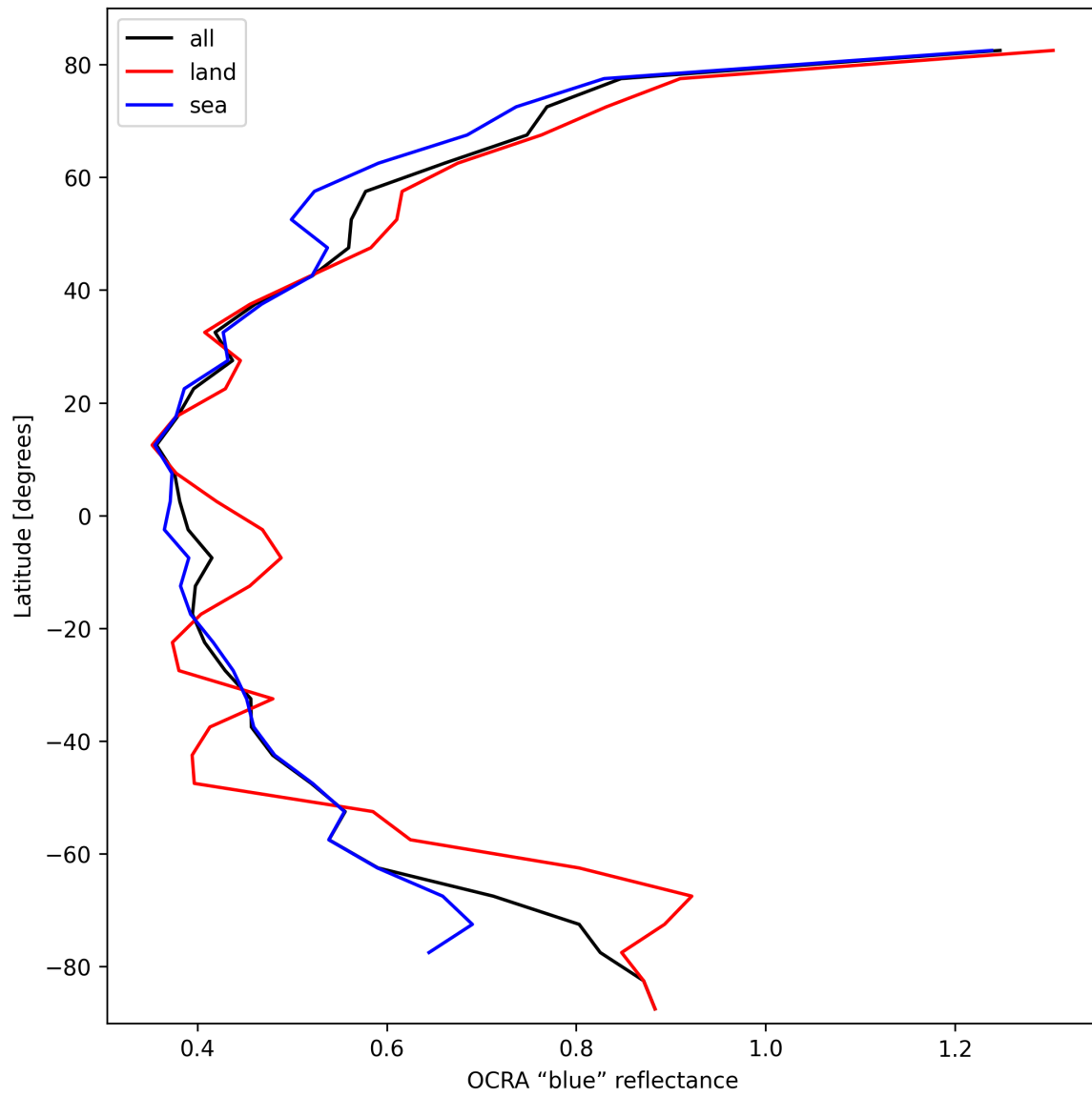
Figure 35: Zonal average of “OCRA “blue” reflectance” for 2025-02-25 to 2025-02-27.
