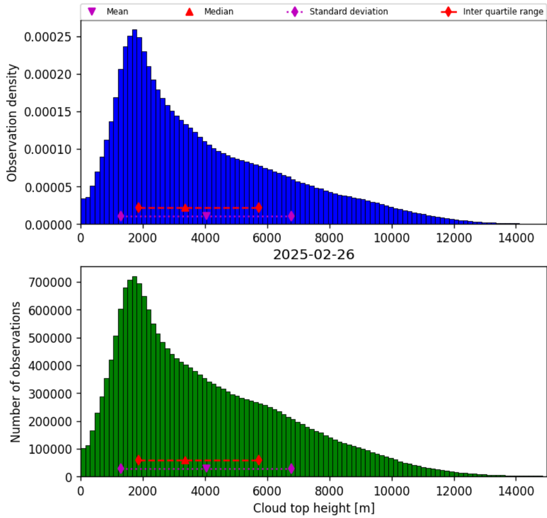
Figure 40: Histogram of “Cloud top height” for 2025-02-25 to 2025-02-27
