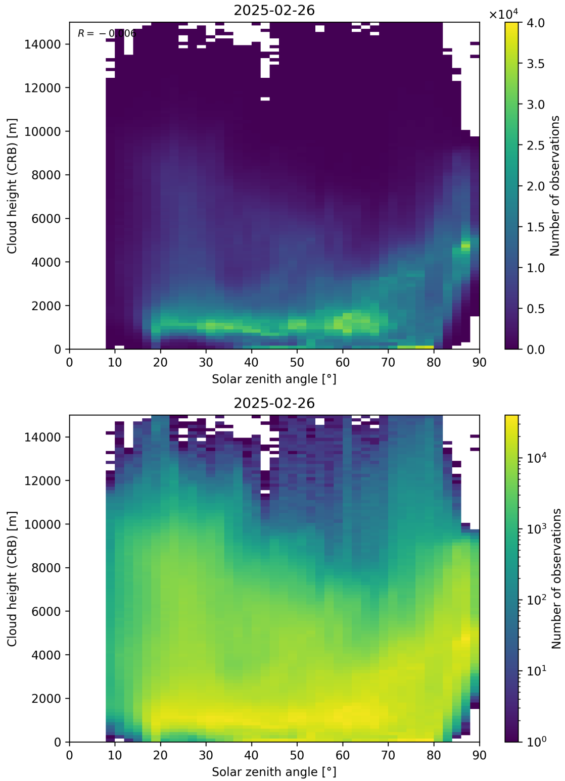
Figure 102: Scatter density plot of “Solar zenith angle” against “Cloud height (CRB)” for 2025-02-25 to 2025-02-27.
