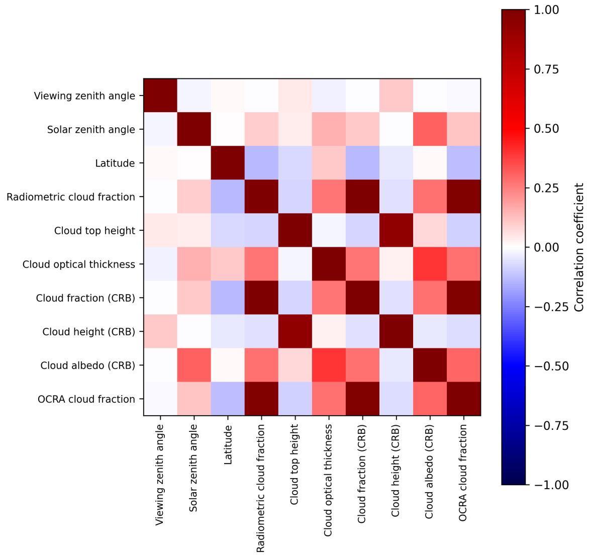
Figure 2: Map of correlation matrix for 2025-02-25 to 2025-02-27.
