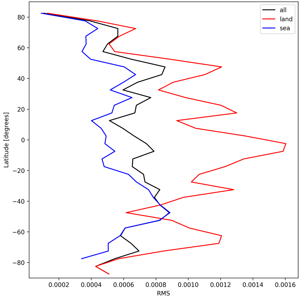
Figure 31: Zonal average of “RMS” for 2025-02-25 to 2025-02-27.
