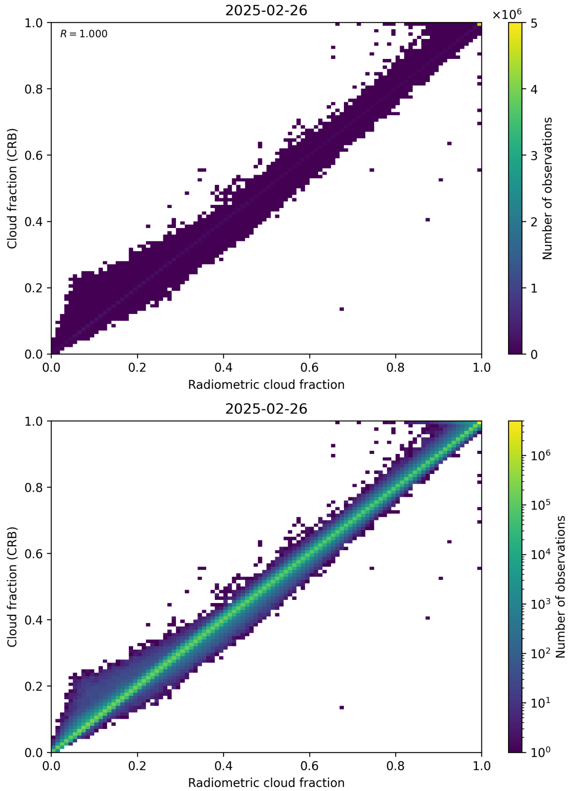
Figure 73: Scatter density plot of “Radiometric cloud fraction” against “Cloud fraction (CRB)” for 2025-02-25 to 2025-02-27.
