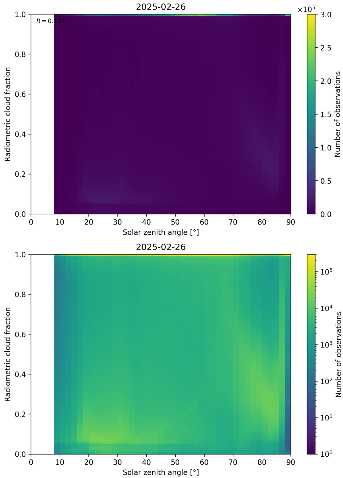
Figure 99: Scatter density plot of “Solar zenith angle” against “Radiometric cloud fraction” for 2025-02-25 to 2025-02-27.
