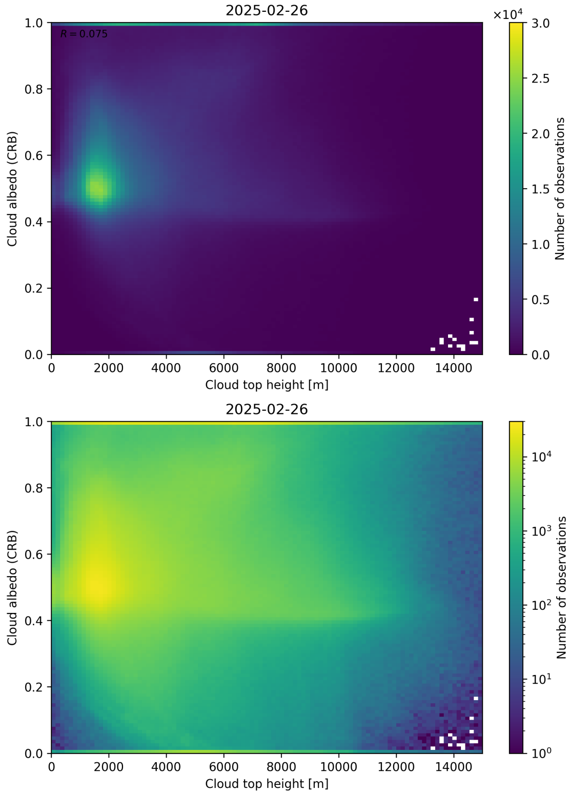
Figure 86: Scatter density plot of “Cloud top height” against “Cloud albedo (CRB)” for 2025-02-25 to 2025-02-27.
