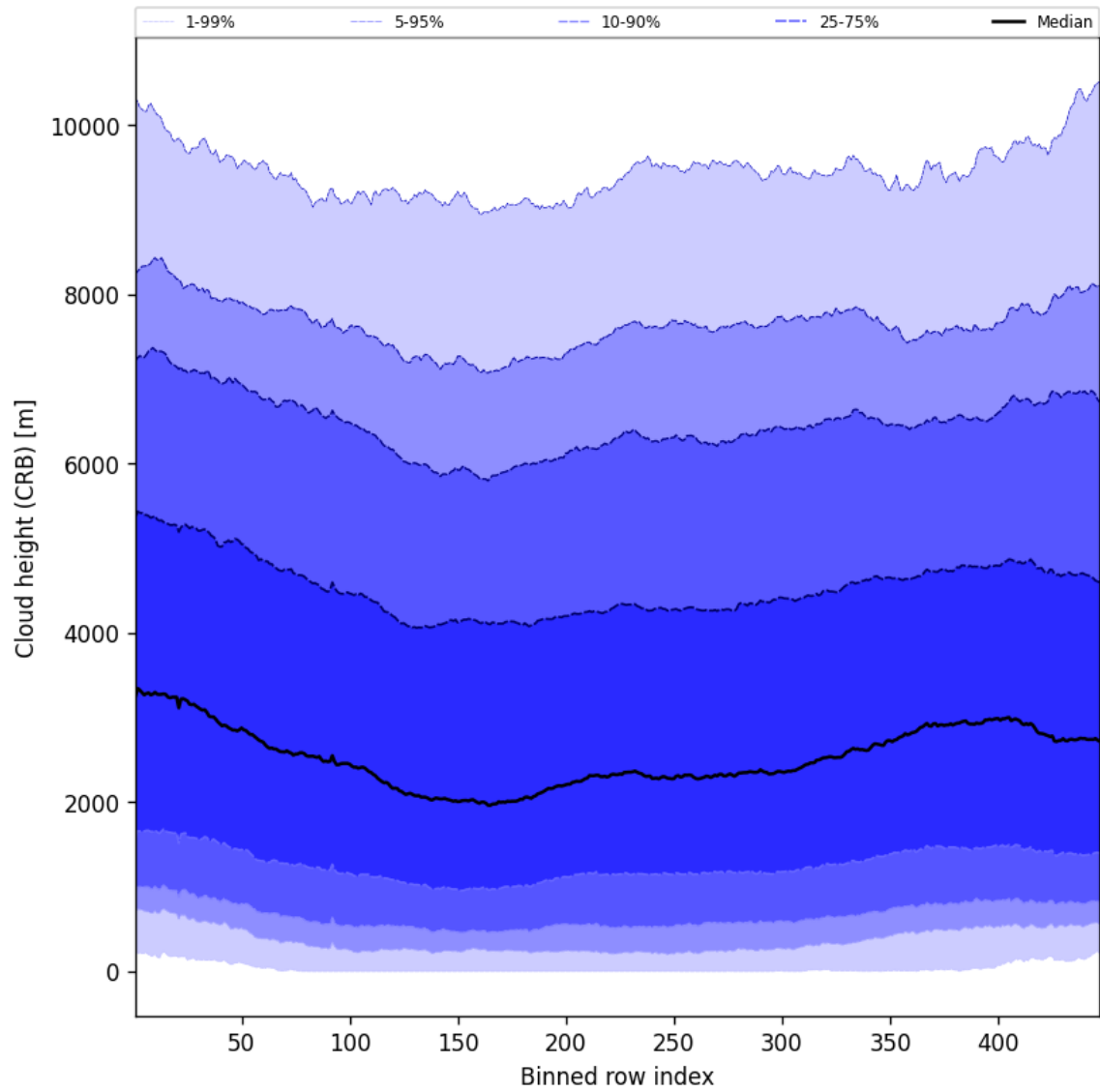
Figure 59: Along track statistics of “Cloud height (CRB)” for 2025-02-25 to 2025-02-27
