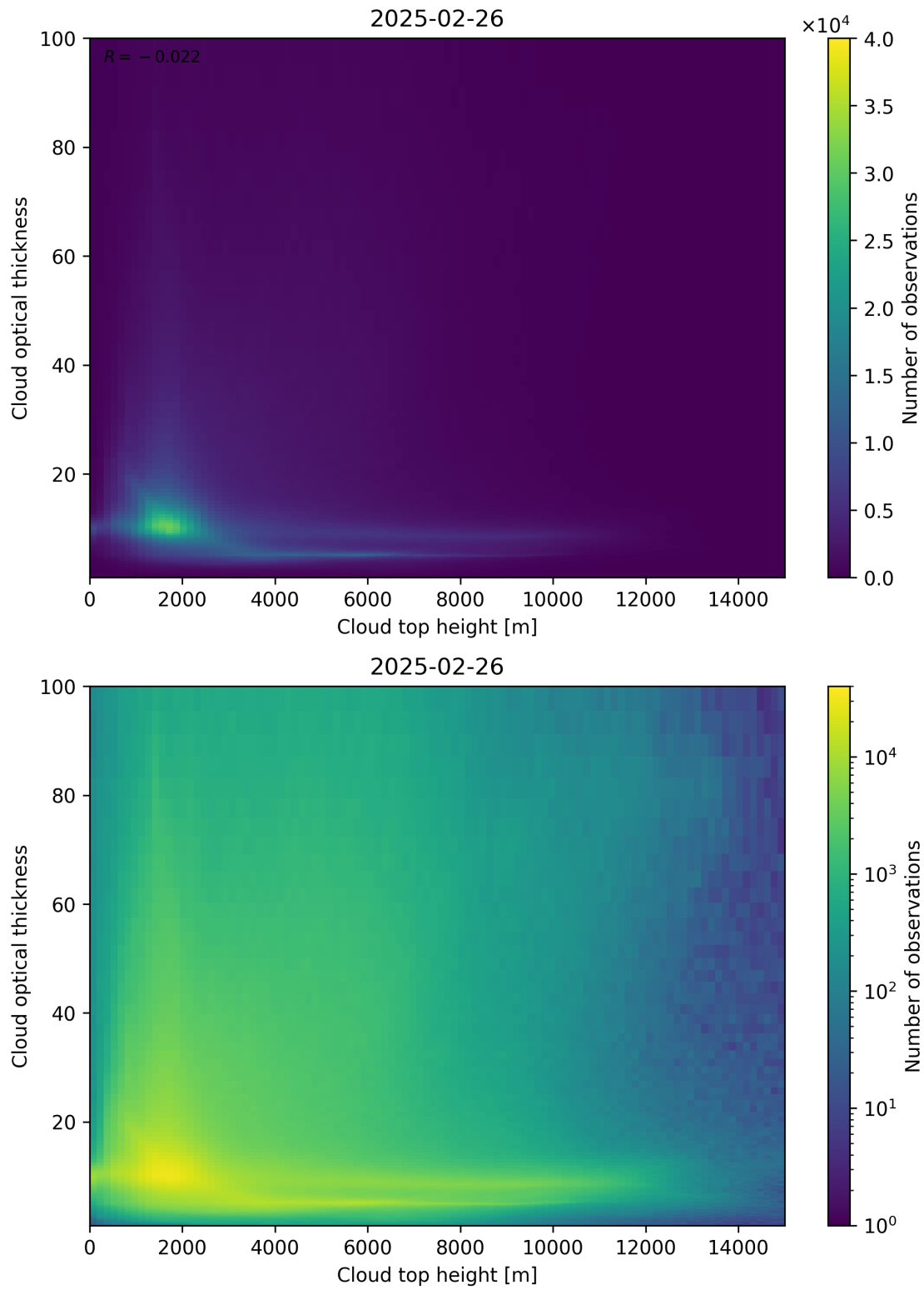
Figure 90: Scatter density plot of “Cloud top height” against “Cloud optical thickness” for 2025-02-25 to 2025-02-27.
