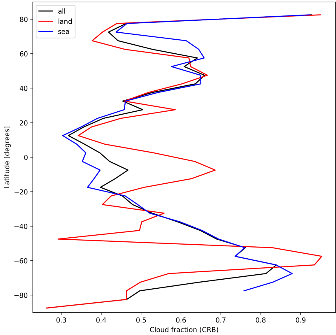
Figure 26: Zonal average of “Cloud fraction (CRB)” for 2025-02-25 to 2025-02-27.
