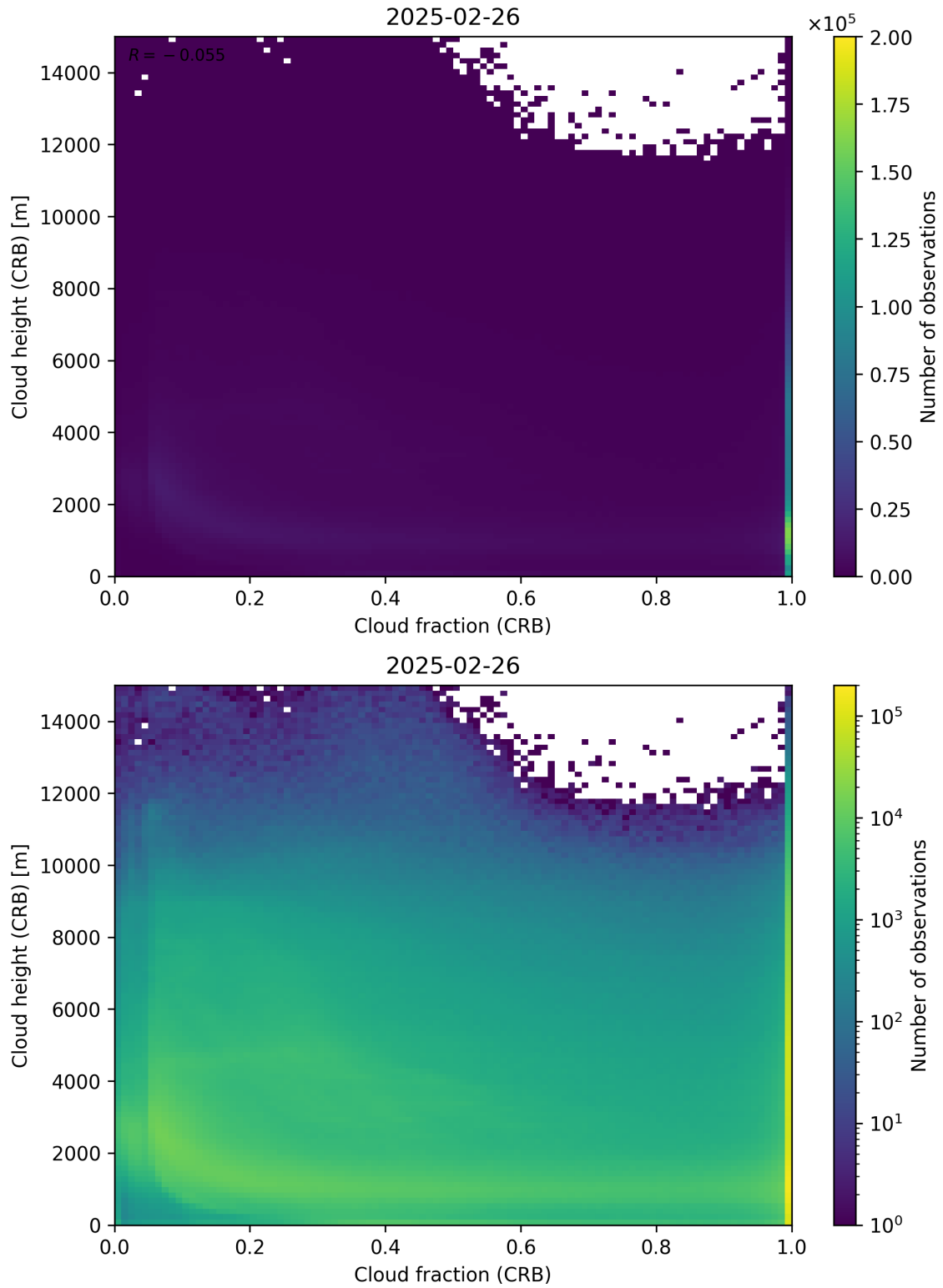
Figure 79: Scatter density plot of “Cloud fraction (CRB)” against “Cloud height (CRB)” for 2025-02-25 to 2025-02-27.
