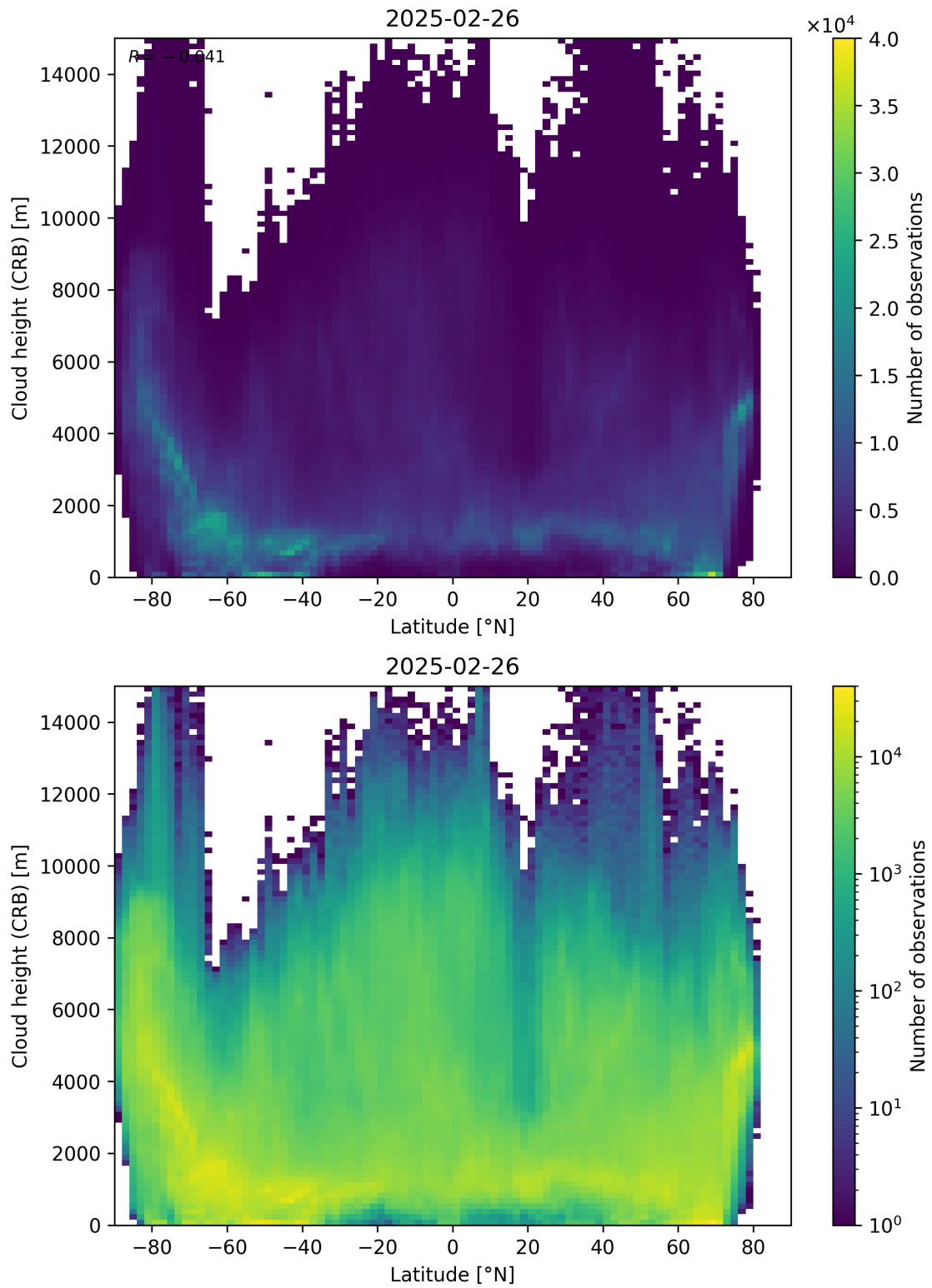
Figure 95: Scatter density plot of “Latitude” against “Cloud height (CRB)” for 2025-02-25 to 2025-02-27.
