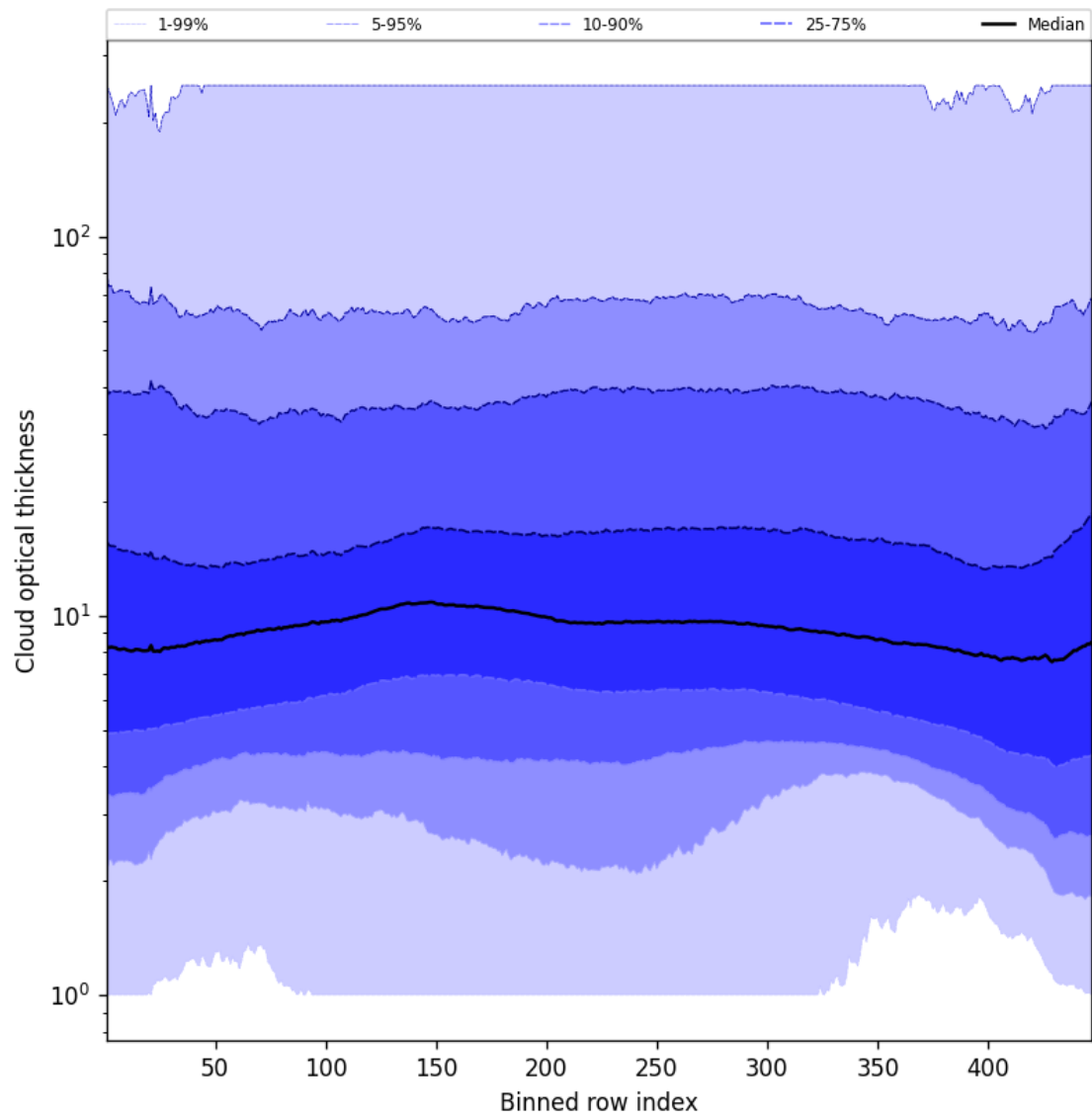
Figure 57: Along track statistics of “Cloud optical thickness” for 2025-02-25 to 2025-02-27
