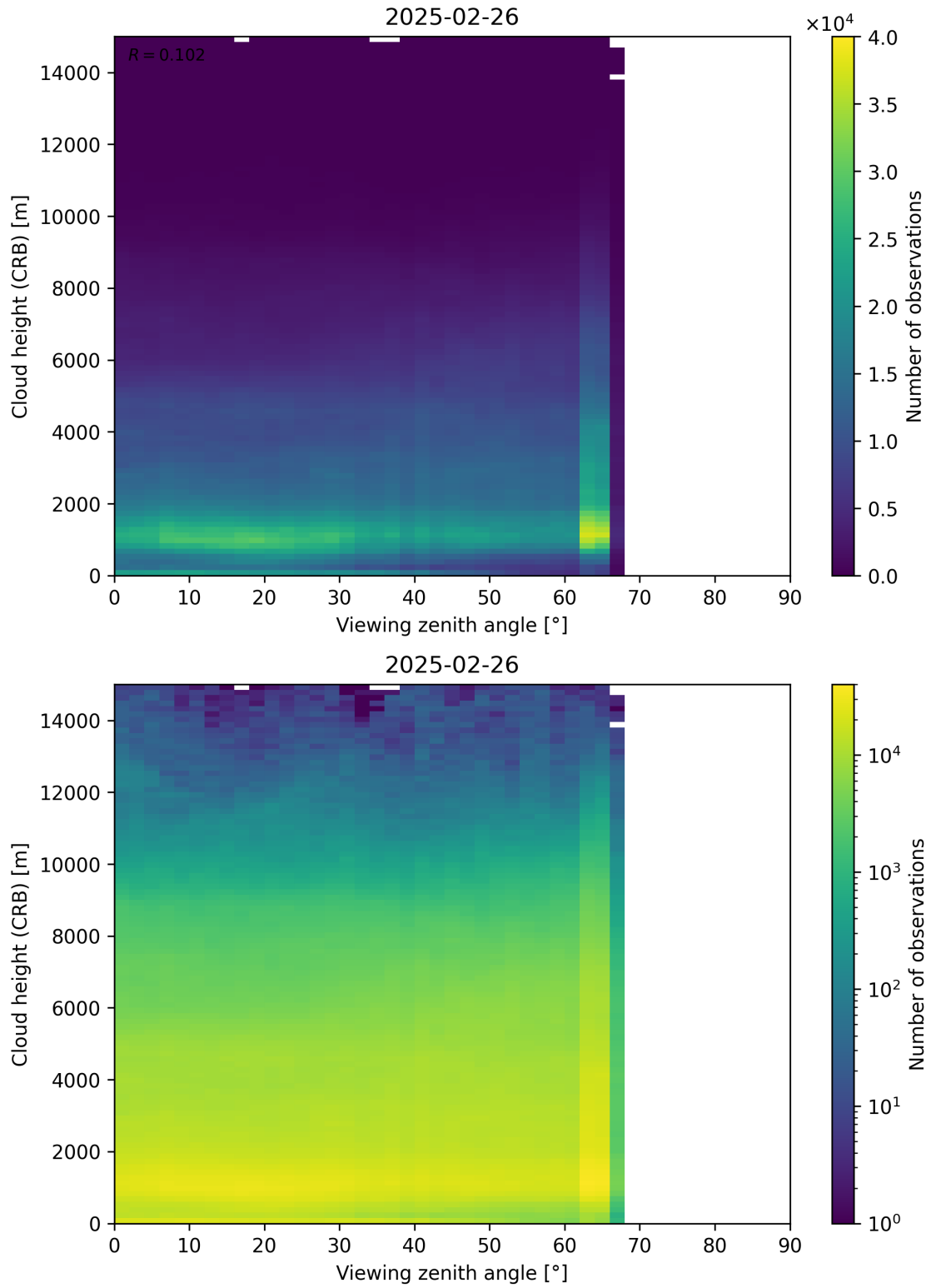
Figure 110: Scatter density plot of “Viewing zenith angle” against “Cloud height (CRB)” for 2025-02-25 to 2025-02-27.
