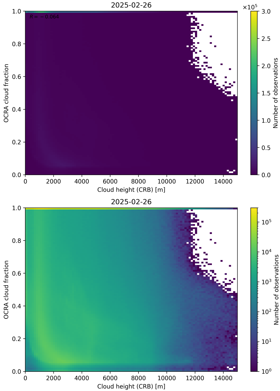
Figure 81: Scatter density plot of “Cloud height (CRB)” against “OCRA cloud fraction” for 2025-02-25 to 2025-02-27.
