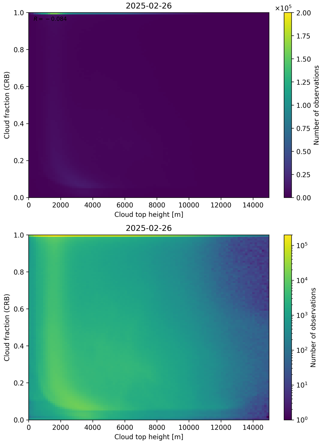
Figure 88: Scatter density plot of “Cloud top height” against “Cloud fraction (CRB)” for 2025-02-25 to 2025-02-27.
