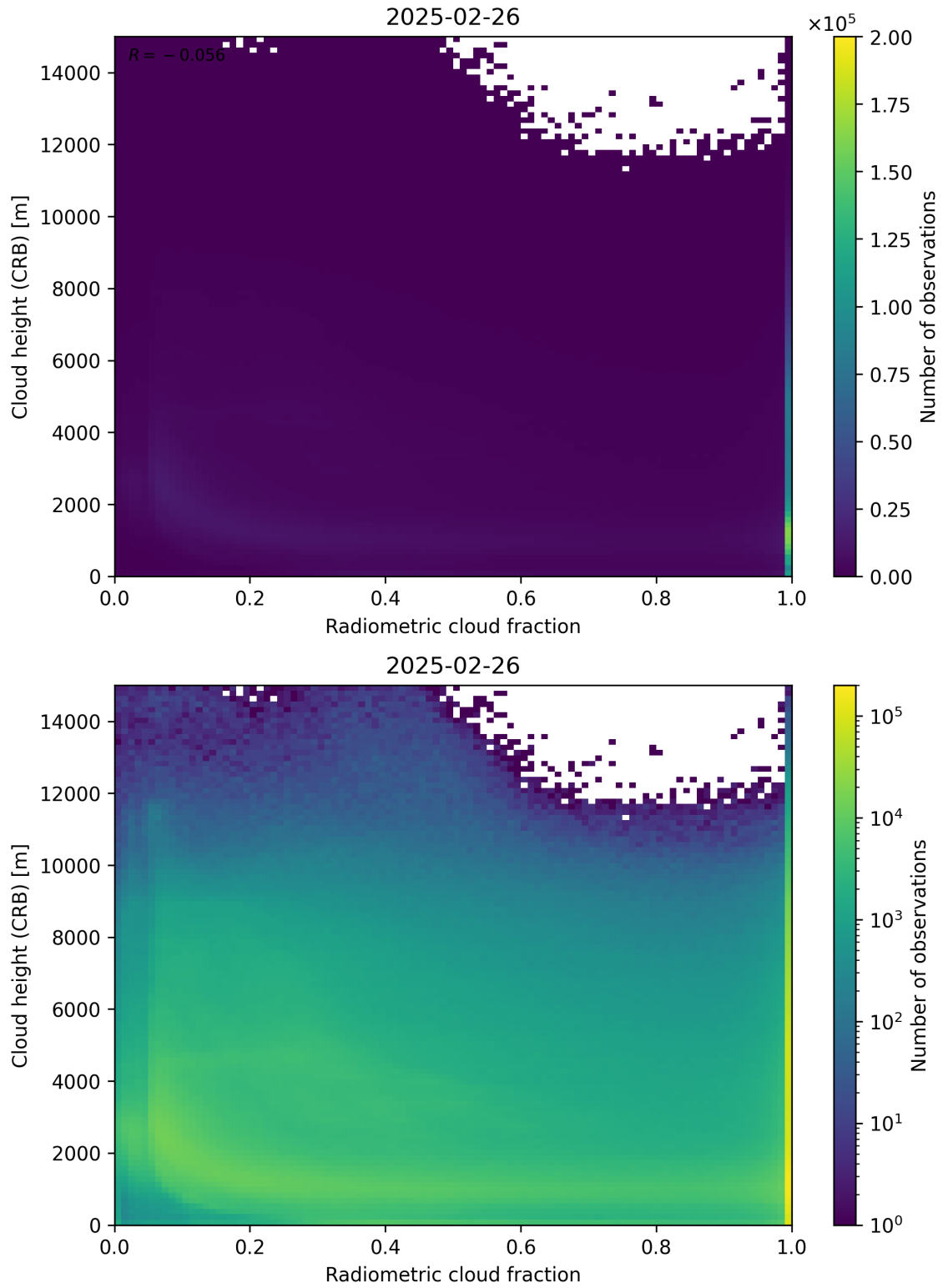
Figure 74: Scatter density plot of “Radiometric cloud fraction” against “Cloud height (CRB)” for 2025-02-25 to 2025-02-27.
