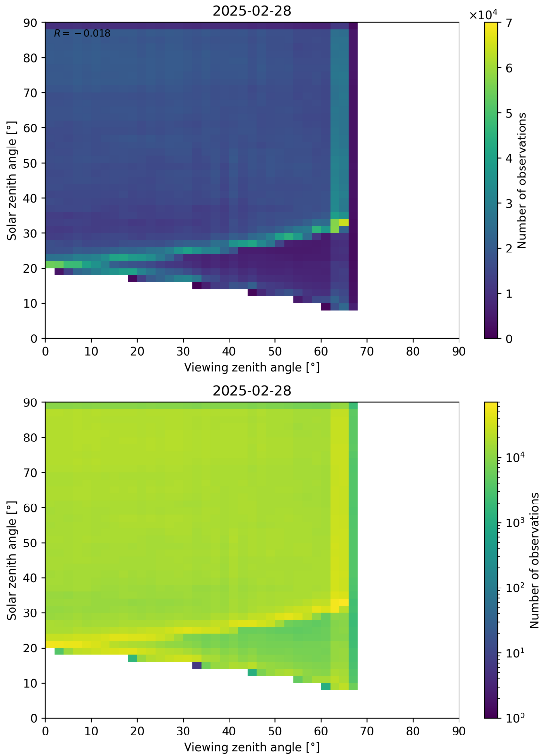
Figure 114: Scatter density plot of “Viewing zenith angle” against “Solar zenith angle” for 2025-02-27 to 2025-03-01.
