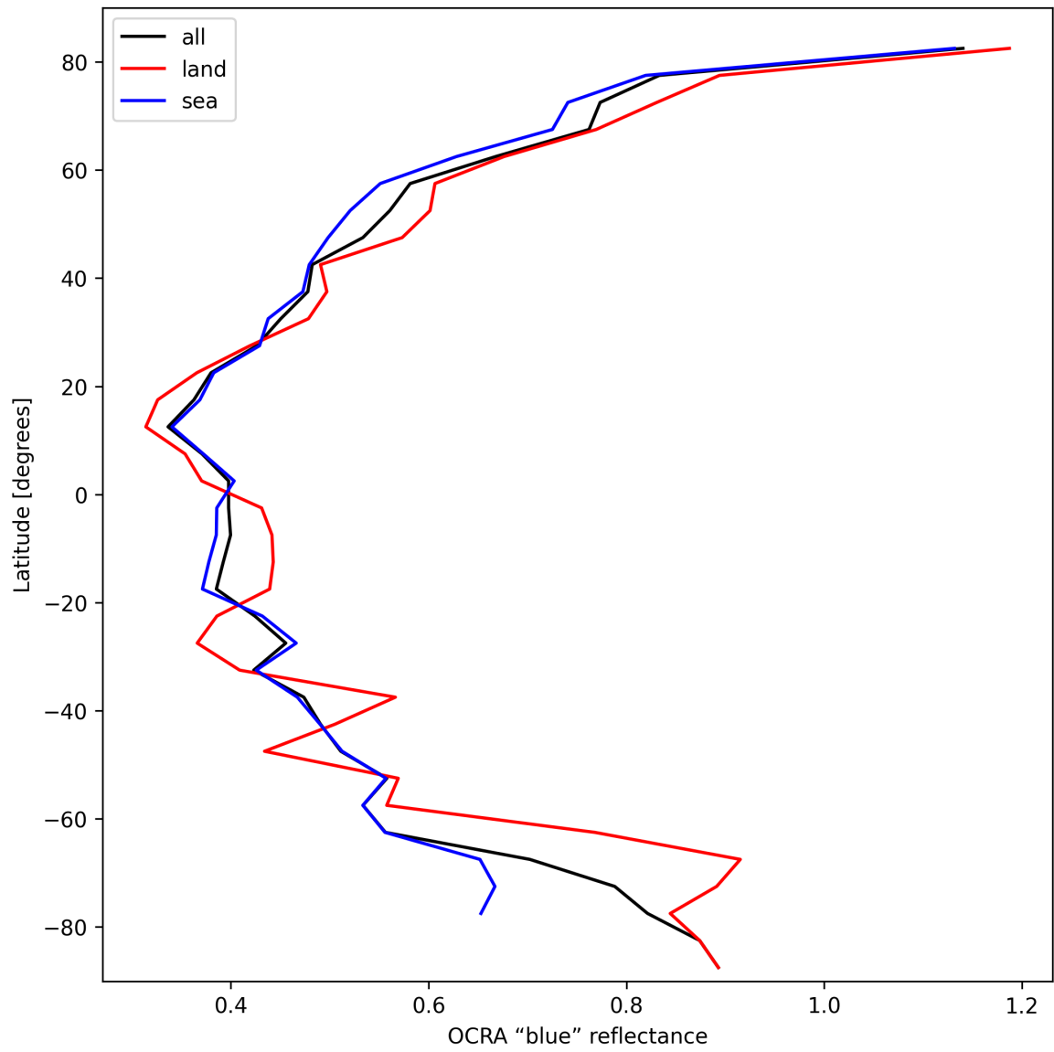
Figure 35: Zonal average of "OCRA "blue" reflectance" for 2025-02-27 to 2025-03-01.
