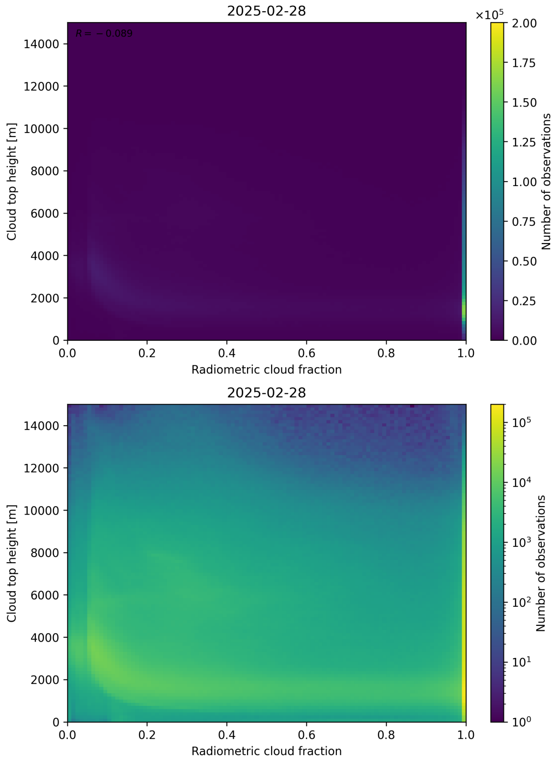
Figure 76: Scatter density plot of “Radiometric cloud fraction” against “Cloud top height” for 2025-02-27 to 2025-03-01.
