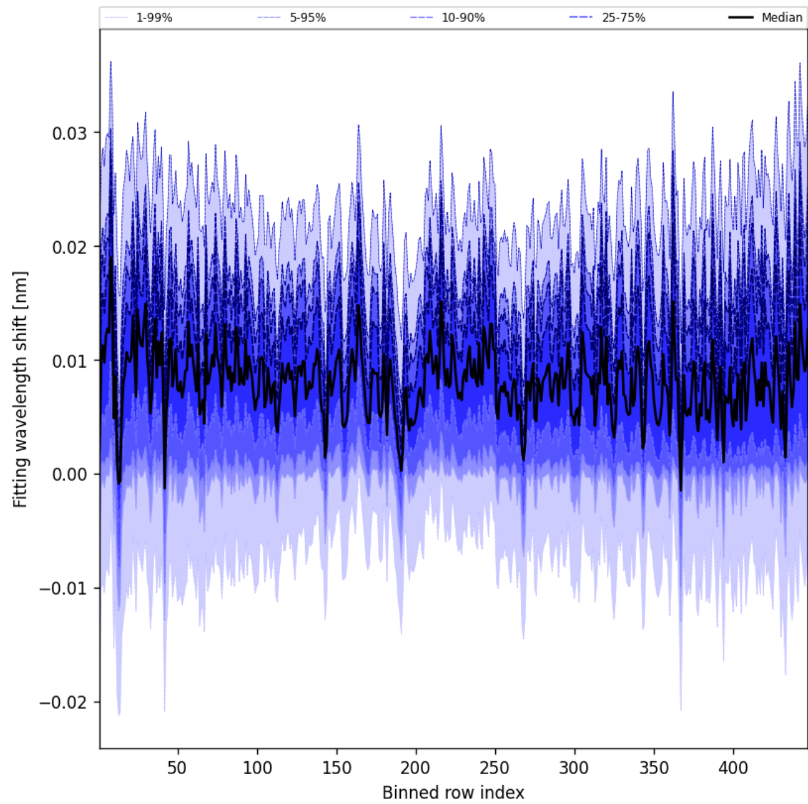
Figure 65: Along track statistics of “Fitting wavelength shift” for 2025-02-27 to 2025-03-01
