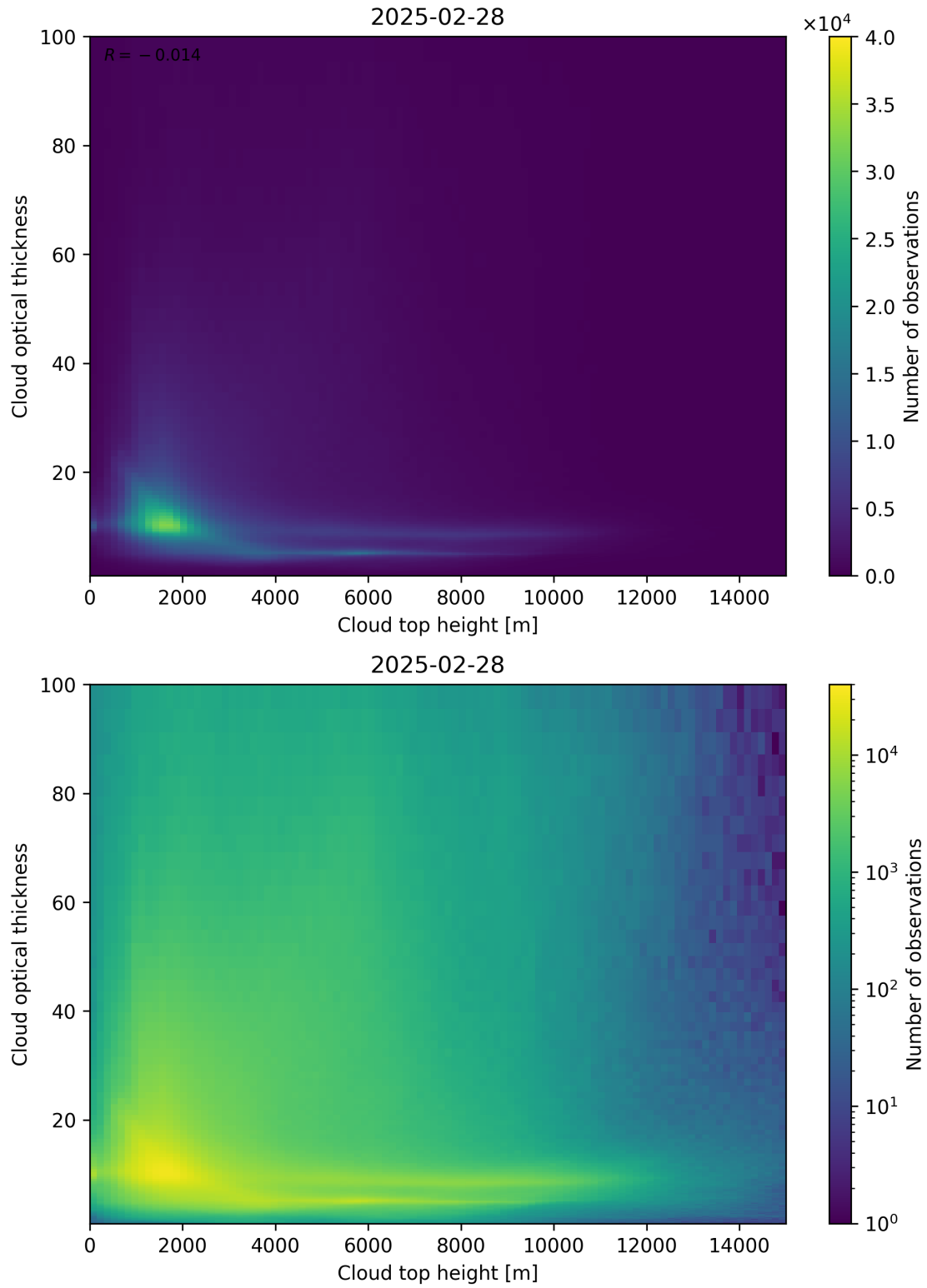
Figure 90: Scatter density plot of “Cloud top height” against “Cloud optical thickness” for 2025-02-27 to 2025-03-01.
