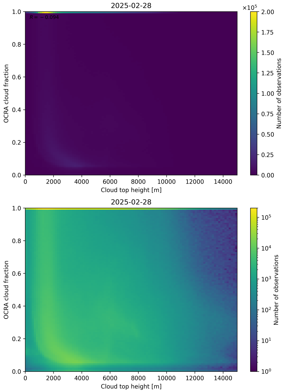
Figure 87: Scatter density plot of “Cloud top height” against “OCRA cloud fraction” for 2025-02-27 to 2025-03-01.
