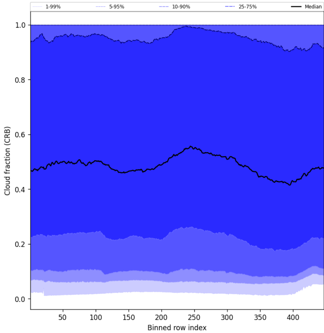
Figure 58: Along track statistics of “Cloud fraction (CRB)” for 2025-02-27 to 2025-03-01
