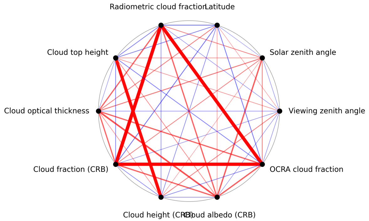
Figure 1: Map of correlation graph for 2025-02-27 to 2025-03-01.
