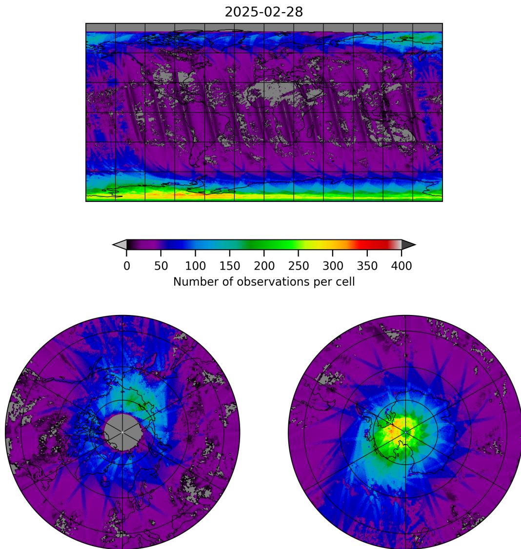
Figure 21: Map of the number of observations for 2025-02-27 to 2025-03-01
