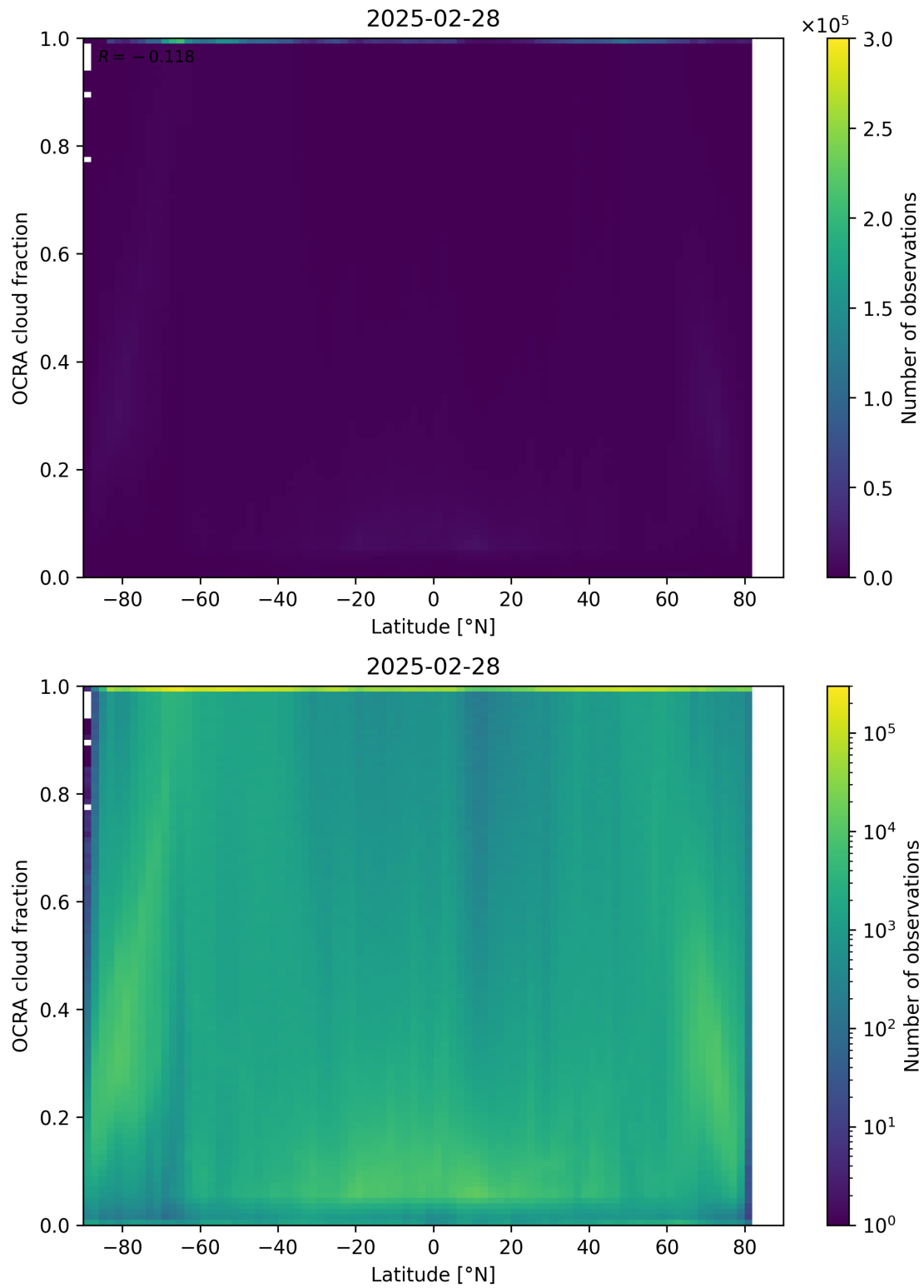
Figure 93: Scatter density plot of “Latitude” against “OCRA cloud fraction” for 2025-02-27 to 2025-03-01.
