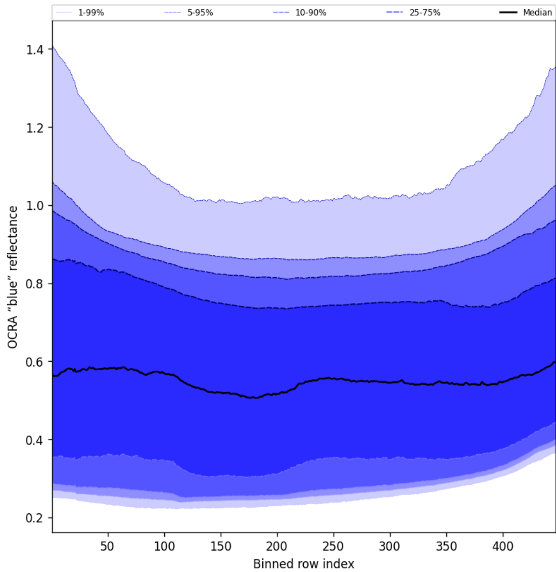
Figure 67: Along track statistics of “OCRA “blue” reflectance” for 2025-02-27 to 2025-03-01
