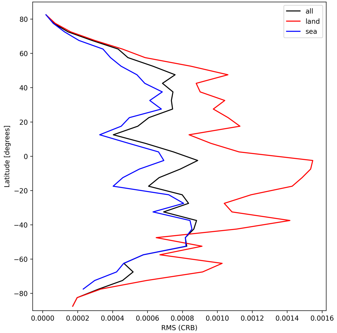
Figure 32: Zonal average of “RMS (CRB)” for 2025-02-27 to 2025-03-01.
