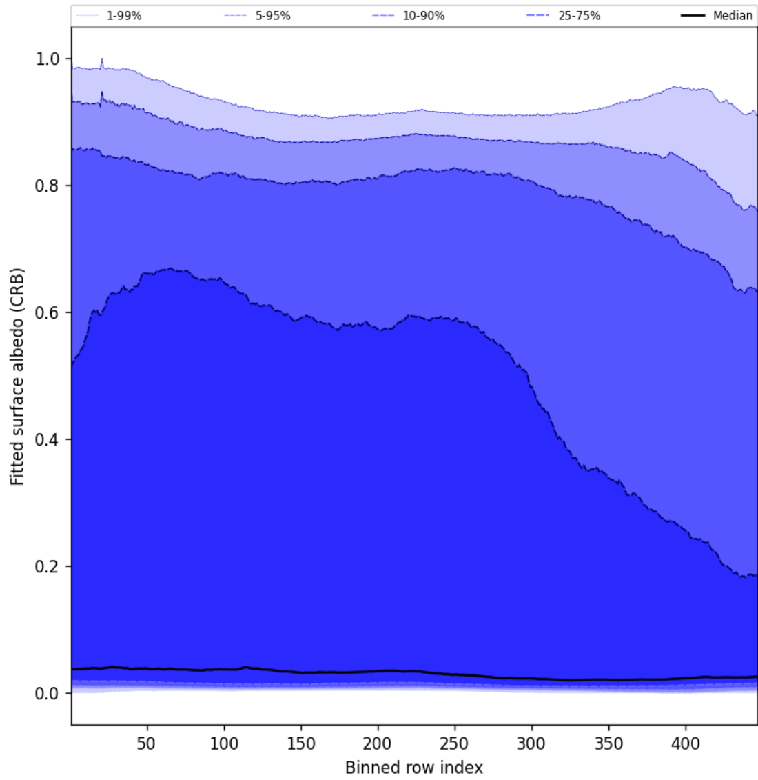
Figure 62: Along track statistics of “Fitted surface albedo (CRB)” for 2025-02-27 to 2025-03-01
