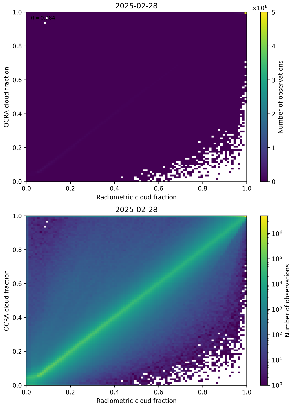
Figure 72: Scatter density plot of “Radiometric cloud fraction” against “OCRA cloud fraction” for 2025-02-27 to 2025-03-01.
