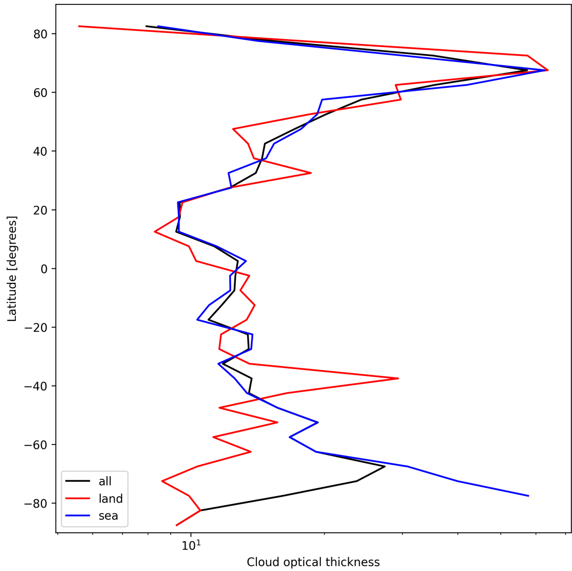
Figure 25: Zonal average of “Cloud optical thickness” for 2025-02-27 to 2025-03-01.
