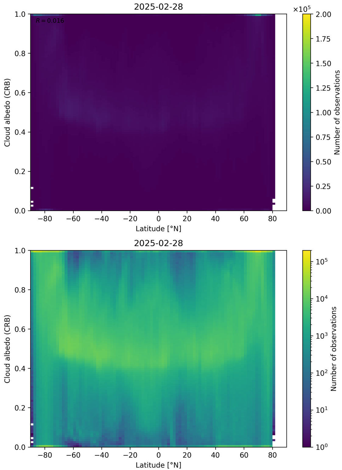
Figure 91: Scatter density plot of “Latitude” against “Cloud albedo (CRB)” for 2025-02-27 to 2025-03-01.
