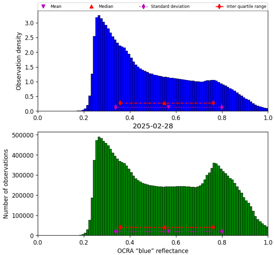
Figure 51: Histogram of “OCRA “blue” reflectance” for 2025-02-27 to 2025-03-01
