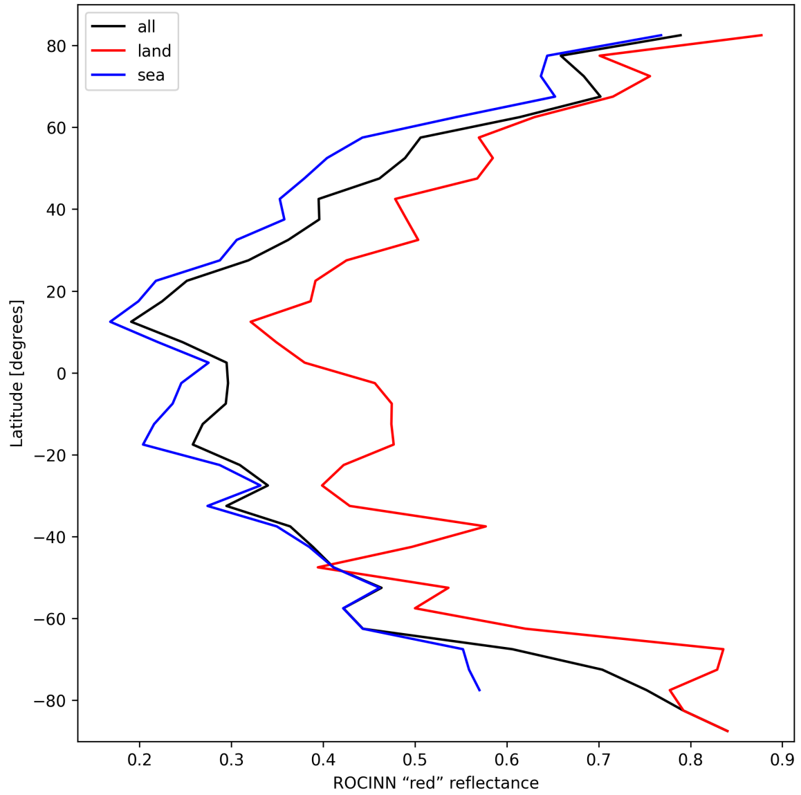
Figure 37: Zonal average of “ROCINN “red” reflectance” for 2025-02-27 to 2025-03-01.
