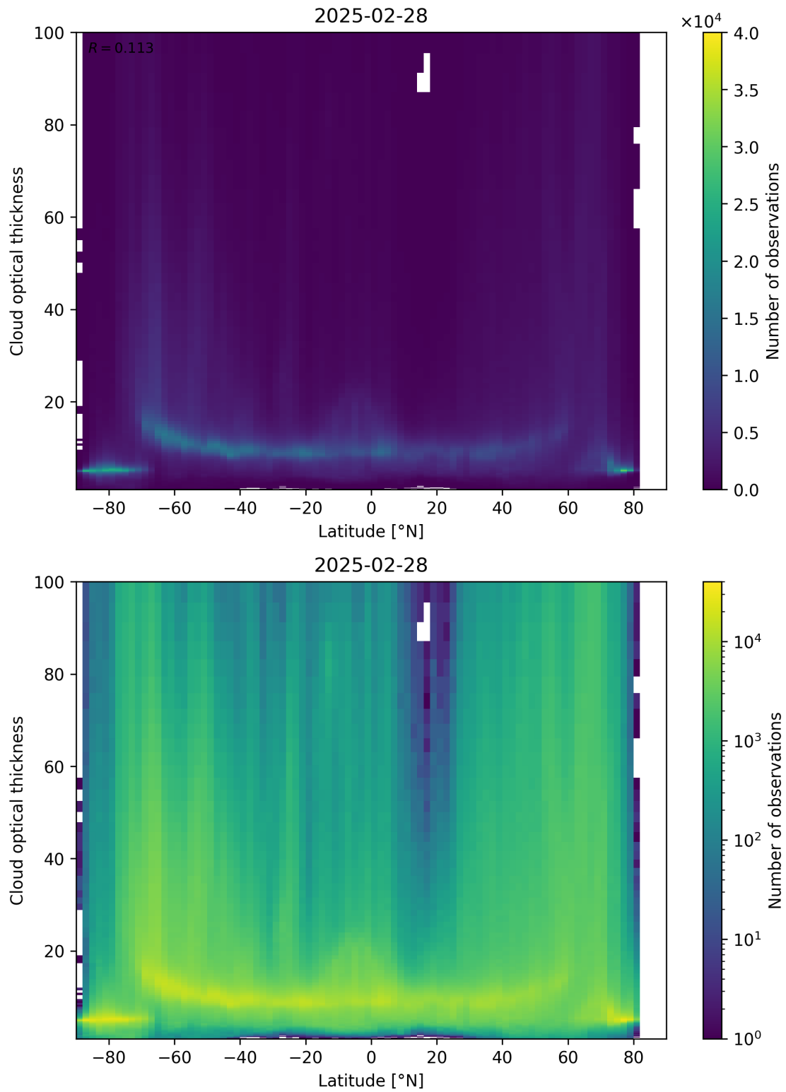
Figure 96: Scatter density plot of “Latitude” against “Cloud optical thickness” for 2025-02-27 to 2025-03-01.
