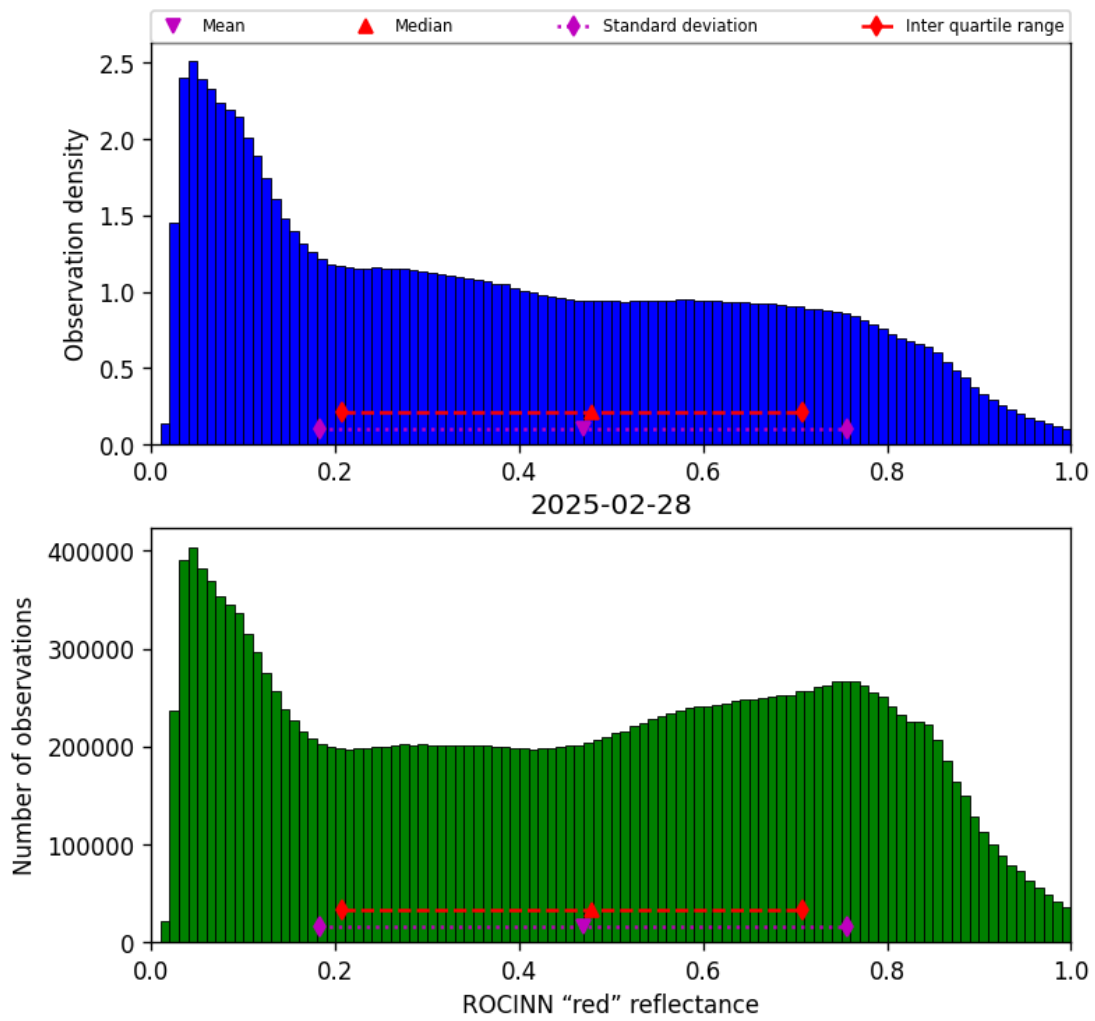
Figure 53: Histogram of “ROCINN “red” reflectance” for 2025-02-27 to 2025-03-01
