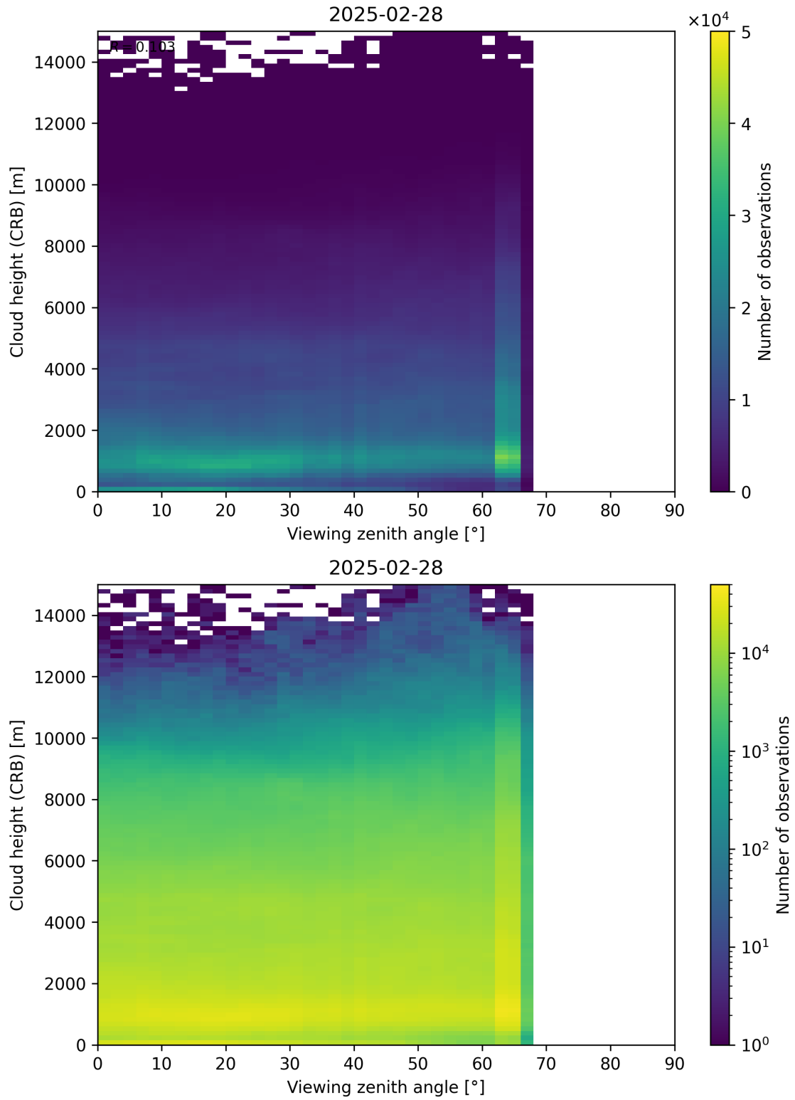
Figure 110: Scatter density plot of “Viewing zenith angle” against “Cloud height (CRB)” for 2025-02-27 to 2025-03-01.
