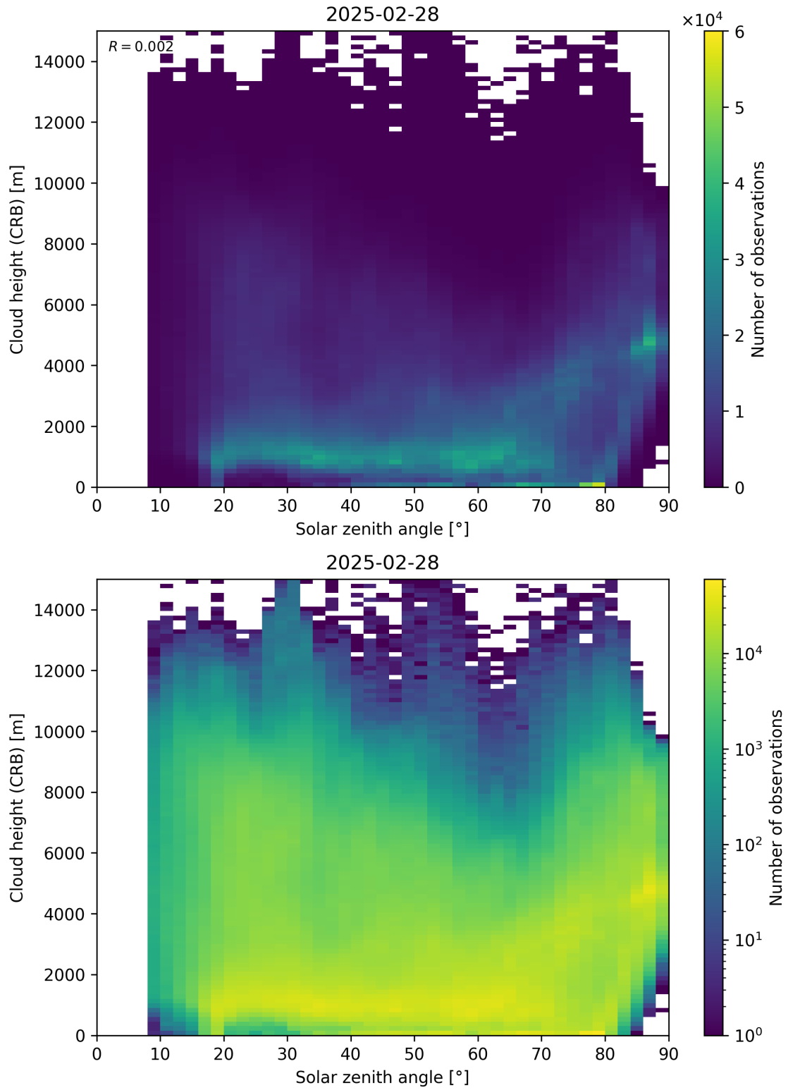
Figure 102: Scatter density plot of “Solar zenith angle” against “Cloud height (CRB)” for 2025-02-27 to 2025-03-01.
