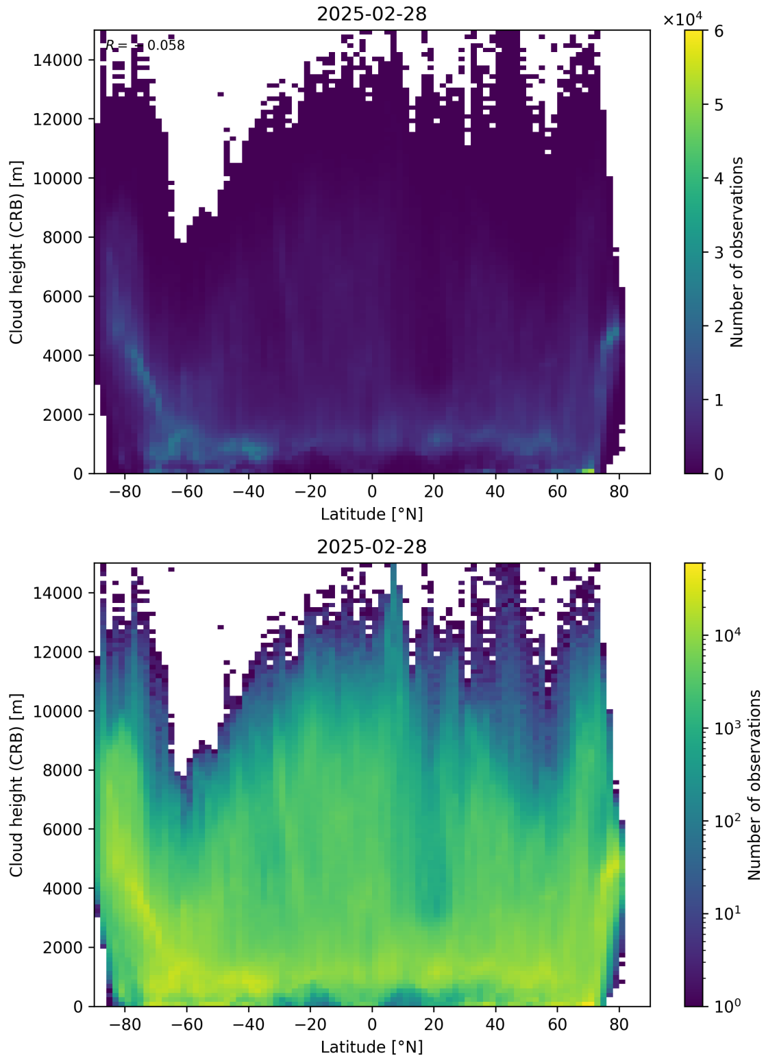
Figure 95: Scatter density plot of “Latitude” against “Cloud height (CRB)” for 2025-02-27 to 2025-03-01.
