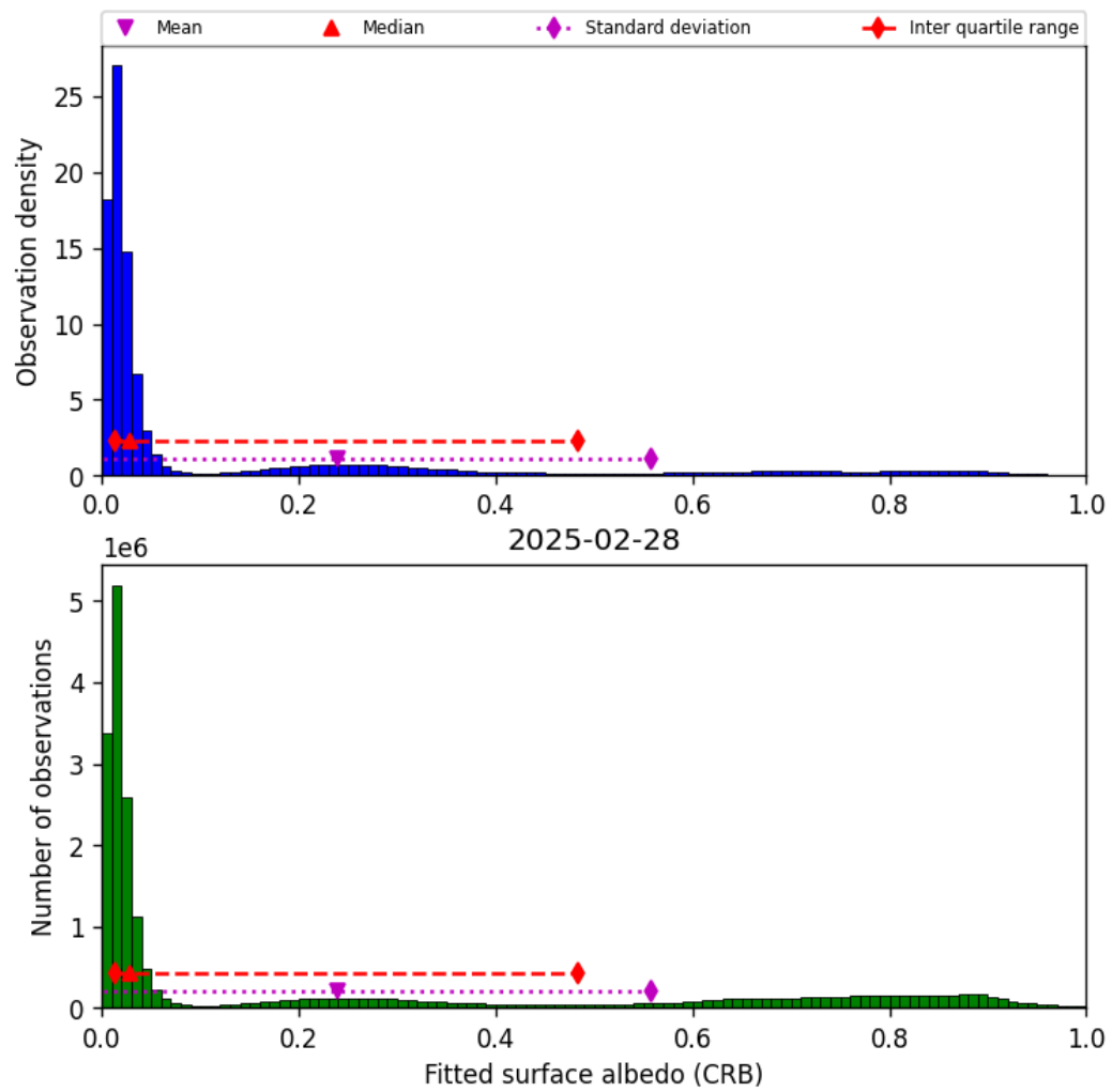
Figure 46: Histogram of “Fitted surface albedo (CRB)” for 2025-02-27 to 2025-03-01
