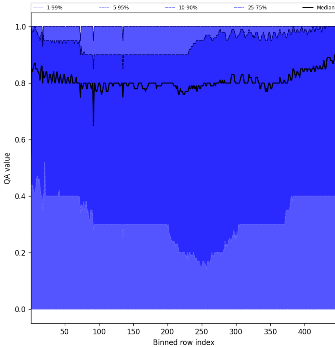
Figure 54: Along track statistics of “QA value” for 2025-02-27 to 2025-03-01
