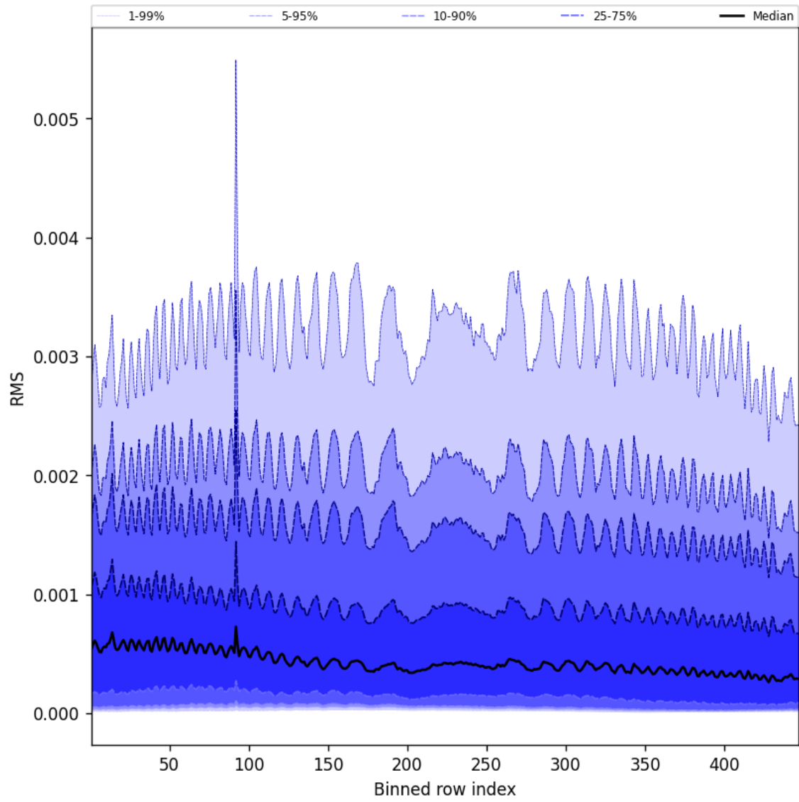
Figure 63: Along track statistics of “RMS” for 2025-02-27 to 2025-03-01
