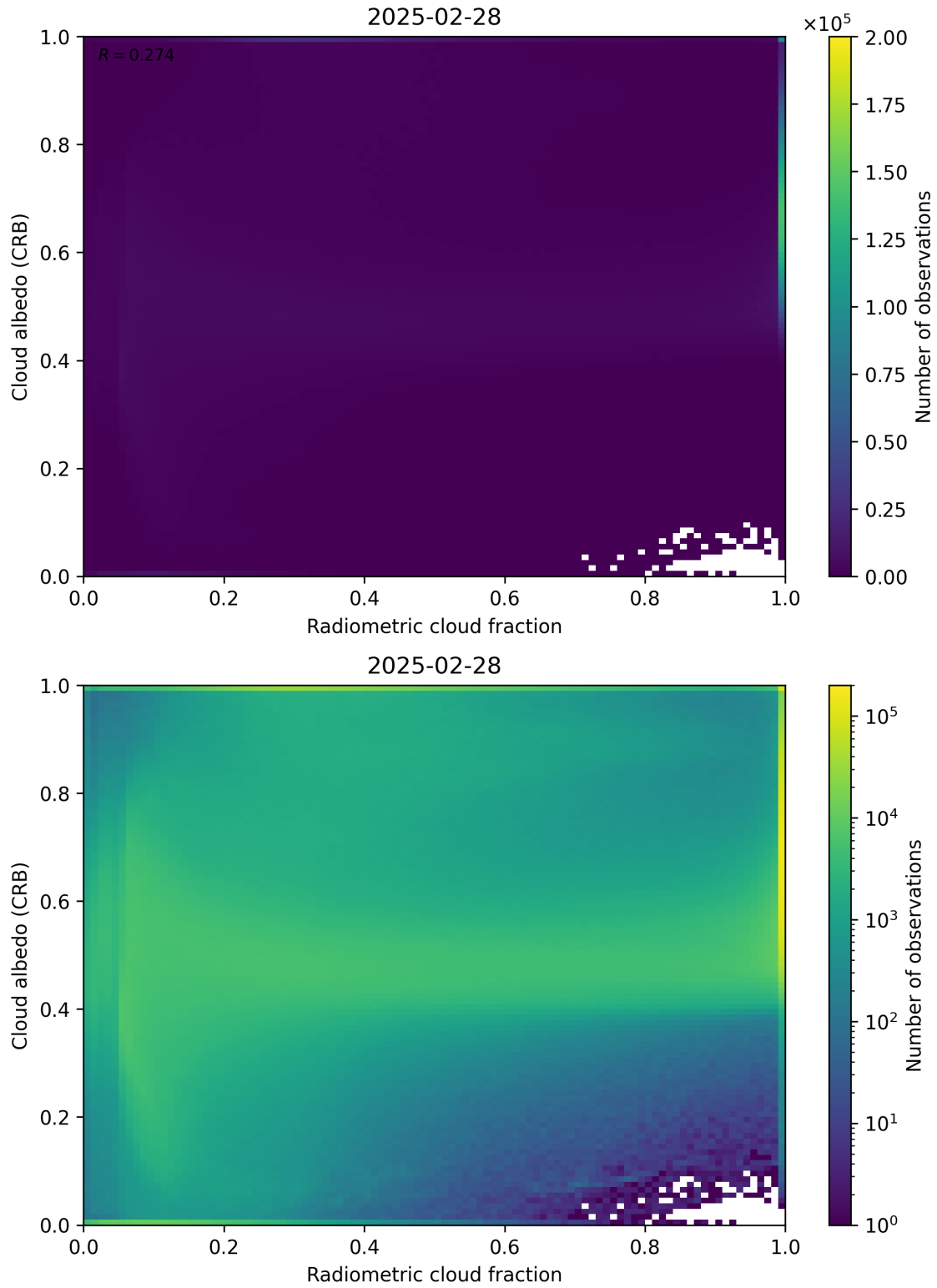
Figure 71: Scatter density plot of “Radiometric cloud fraction” against “Cloud albedo (CRB)” for 2025-02-27 to 2025-03-01.
