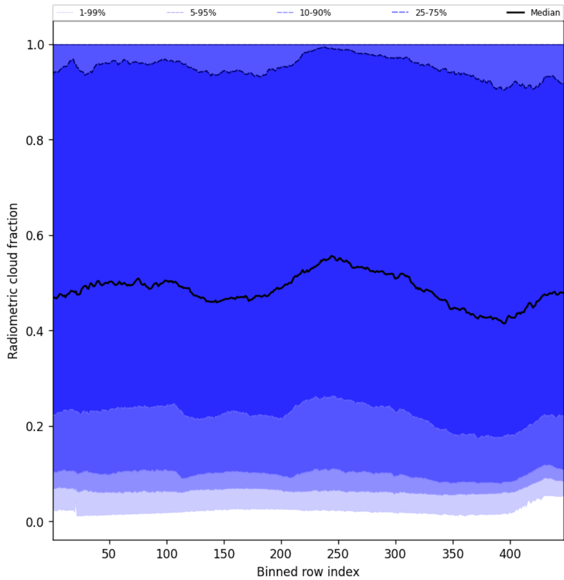
Figure 55: Along track statistics of “Radiometric cloud fraction” for 2025-02-27 to 2025-03-01
