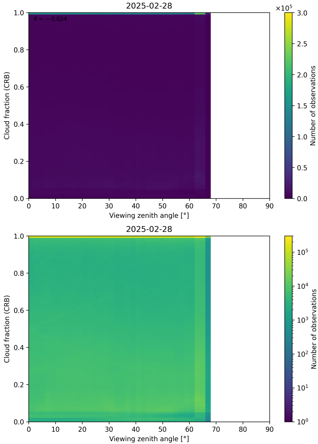
Figure 109: Scatter density plot of “Viewing zenith angle” against “Cloud fraction (CRB)” for 2025-02-27 to 2025-03-01.
