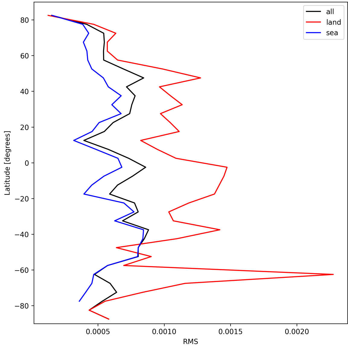
Figure 31: Zonal average of “RMS” for 2025-02-27 to 2025-03-01.
