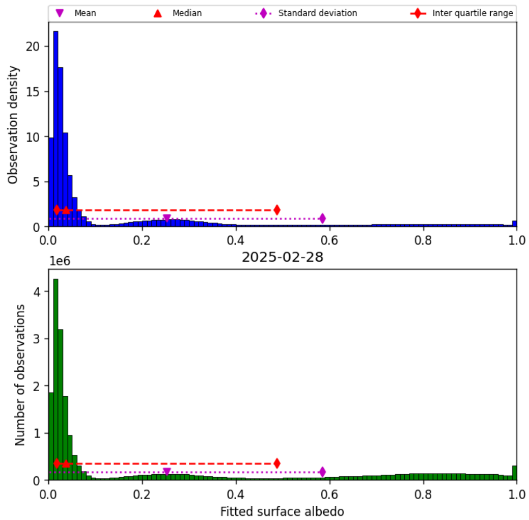
Figure 45: Histogram of “Fitted surface albedo” for 2025-02-27 to 2025-03-01
