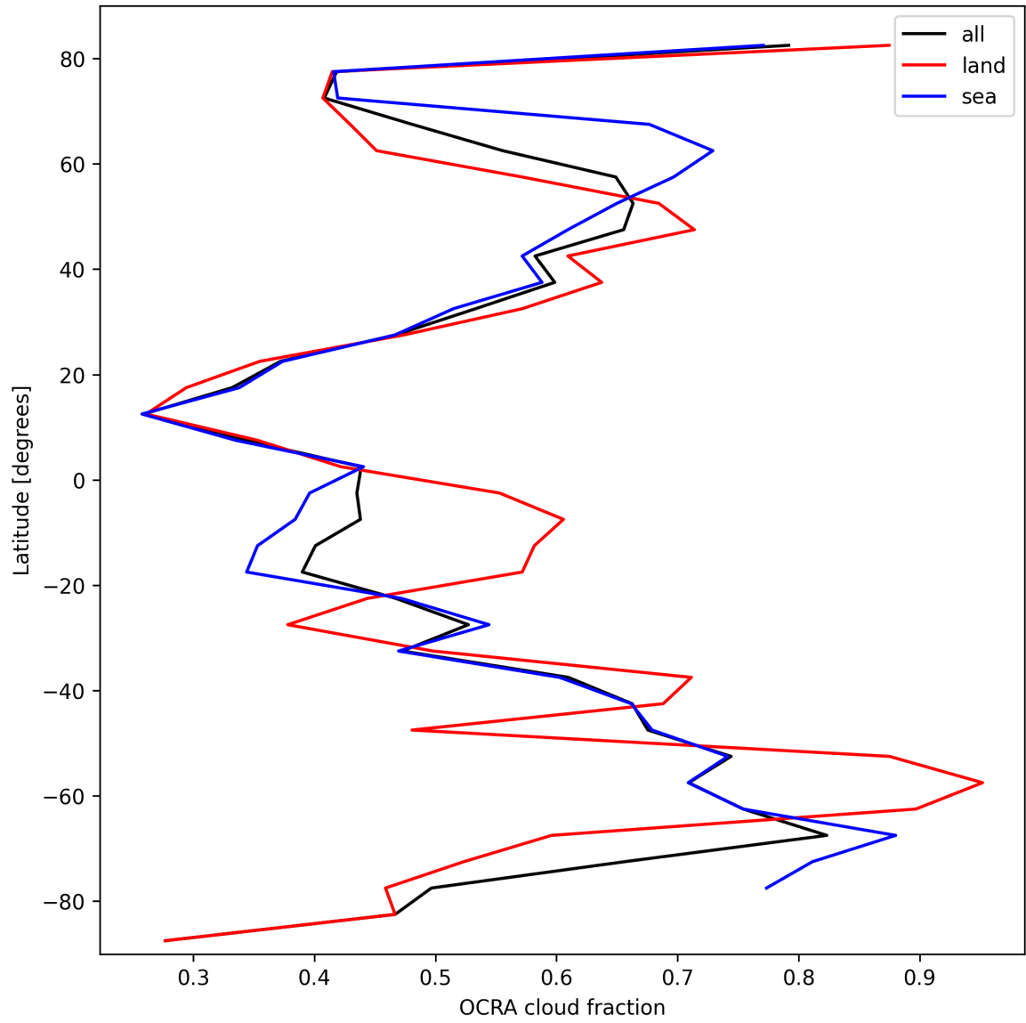
Figure 34: Zonal average of “OCRA cloud fraction” for 2025-02-27 to 2025-03-01.
