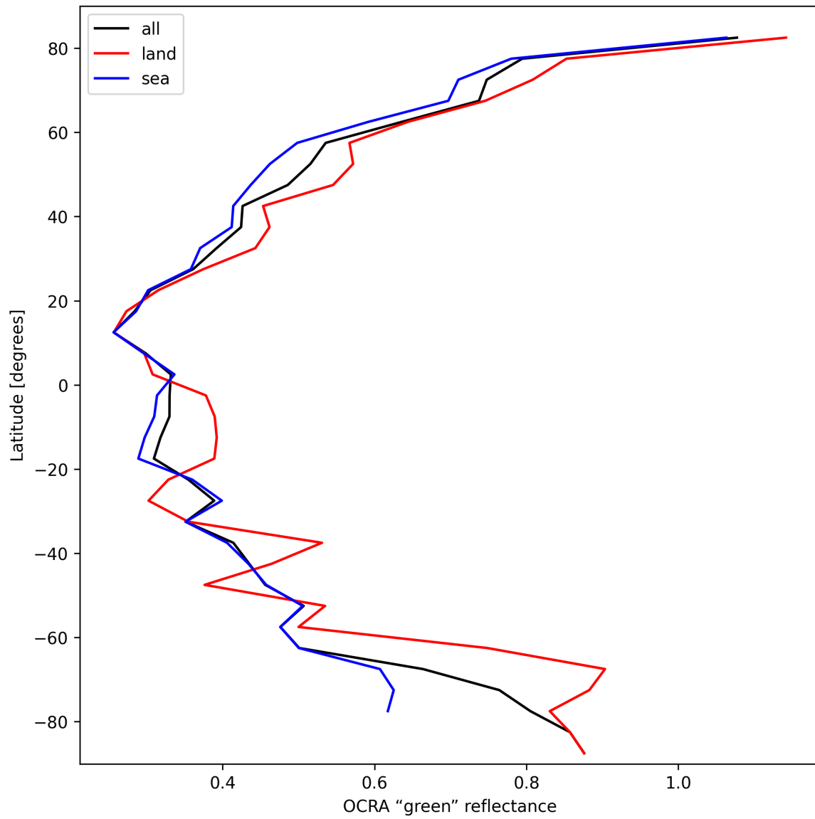
Figure 36: Zonal average of “OCRA “green” reflectance” for 2025-02-27 to 2025-03-01.
