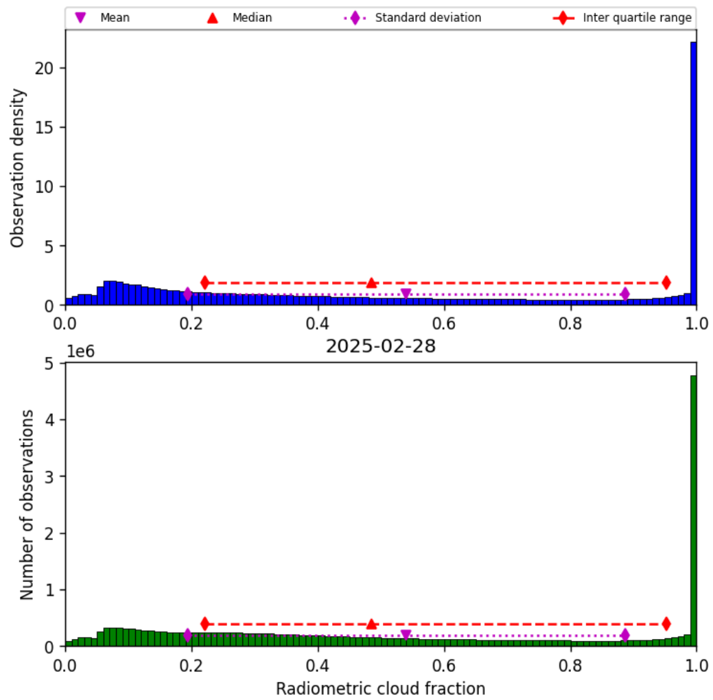
Figure 39: Histogram of “Radiometric cloud fraction” for 2025-02-27 to 2025-03-01
