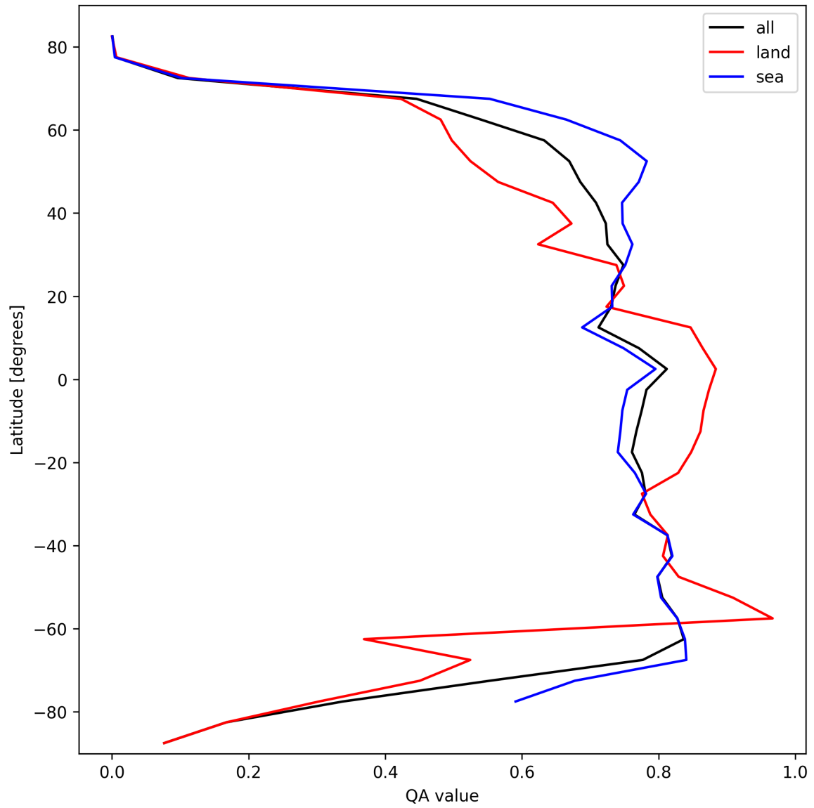
Figure 22: Zonal average of “QA value” for 2025-02-27 to 2025-03-01.
