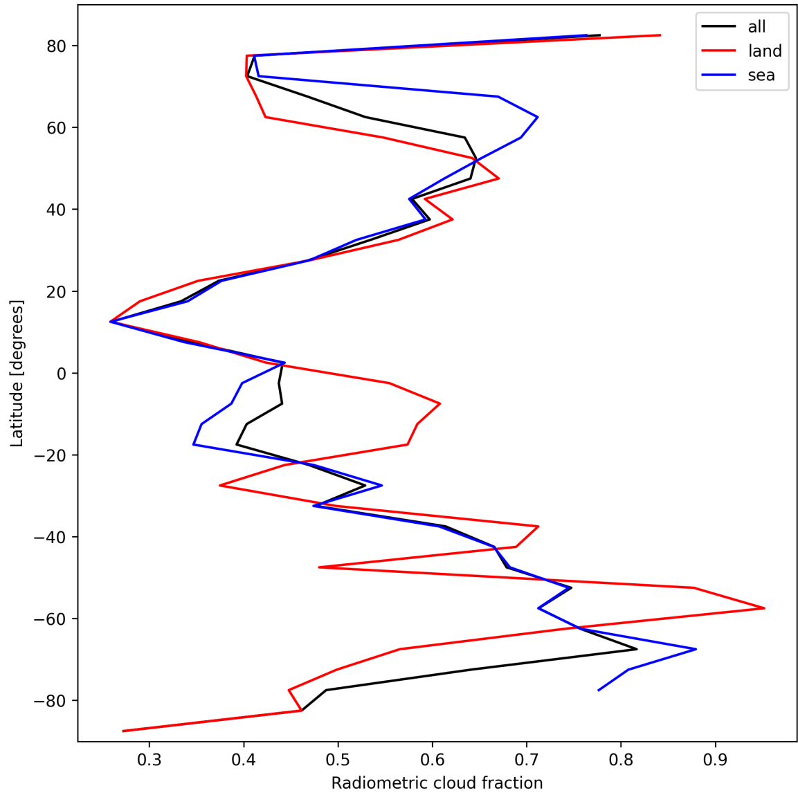
Figure 23: Zonal average of “Radiometric cloud fraction” for 2025-02-27 to 2025-03-01.
