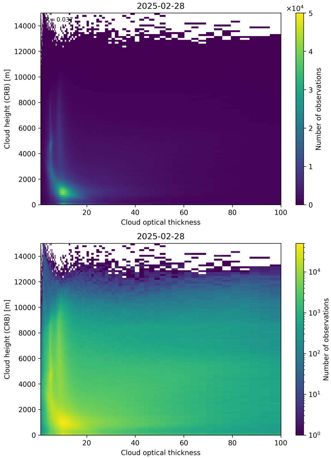
Figure 85: Scatter density plot of “Cloud optical thickness” against “Cloud height (CRB)” for 2025-02-27 to 2025-03-01.
