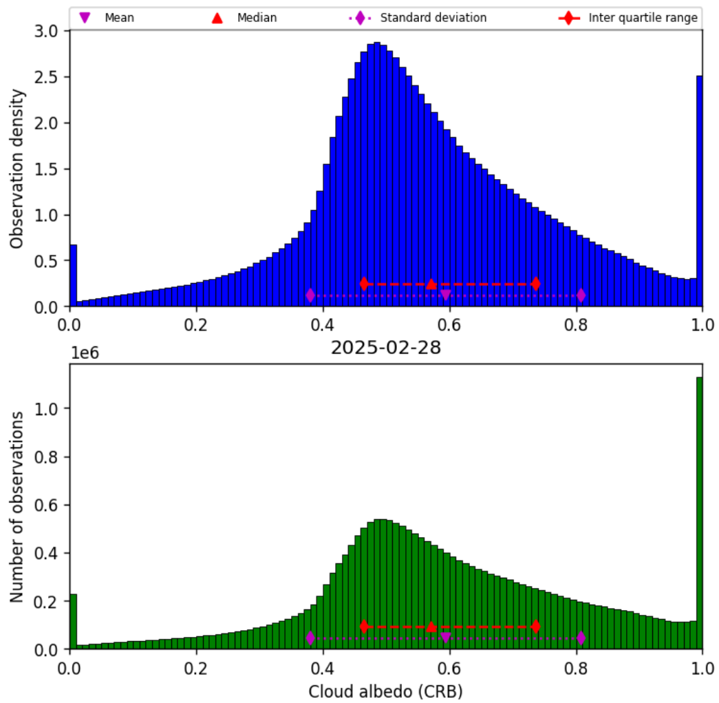
Figure 44: Histogram of “Cloud albedo (CRB)” for 2025-02-27 to 2025-03-01
