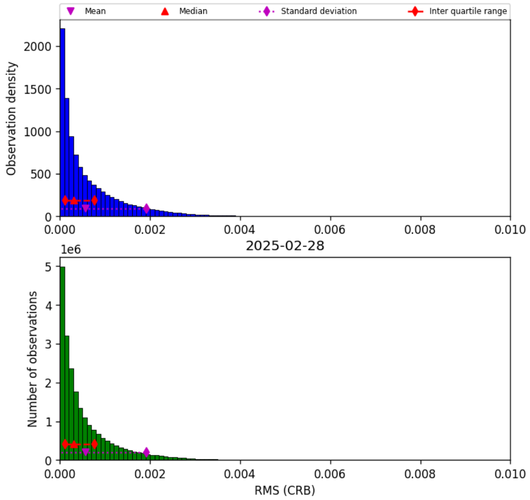
Figure 48: Histogram of “RMS (CRB)” for 2025-02-27 to 2025-03-01
