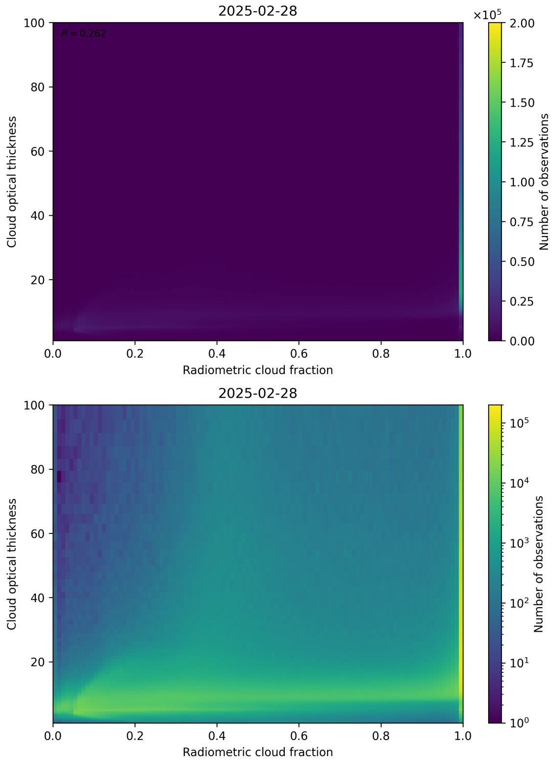
Figure 75: Scatter density plot of “Radiometric cloud fraction” against “Cloud optical thickness” for 2025-02-27 to 2025-03-01.
