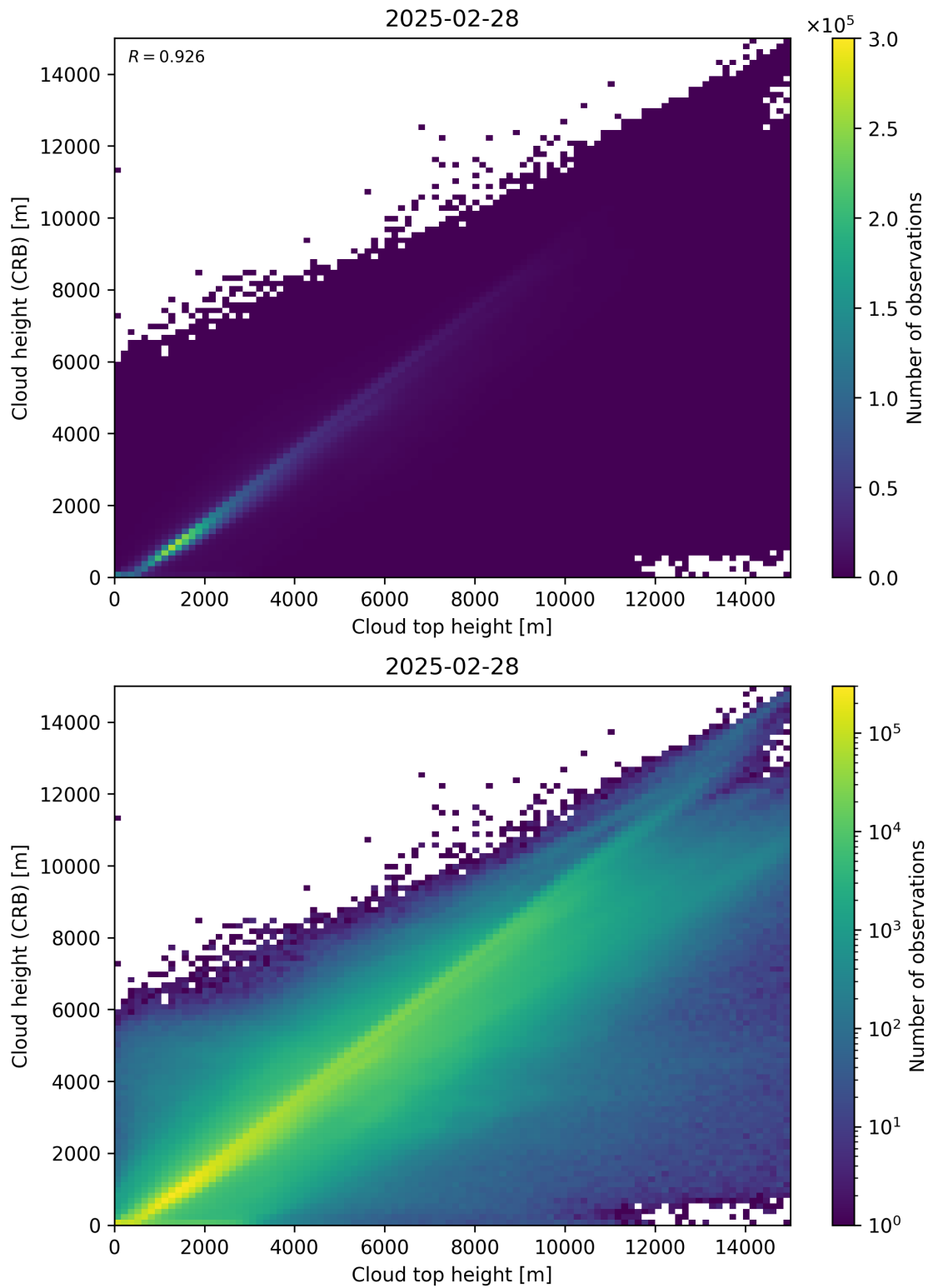
Figure 89: Scatter density plot of “Cloud top height” against “Cloud height (CRB)” for 2025-02-27 to 2025-03-01.
