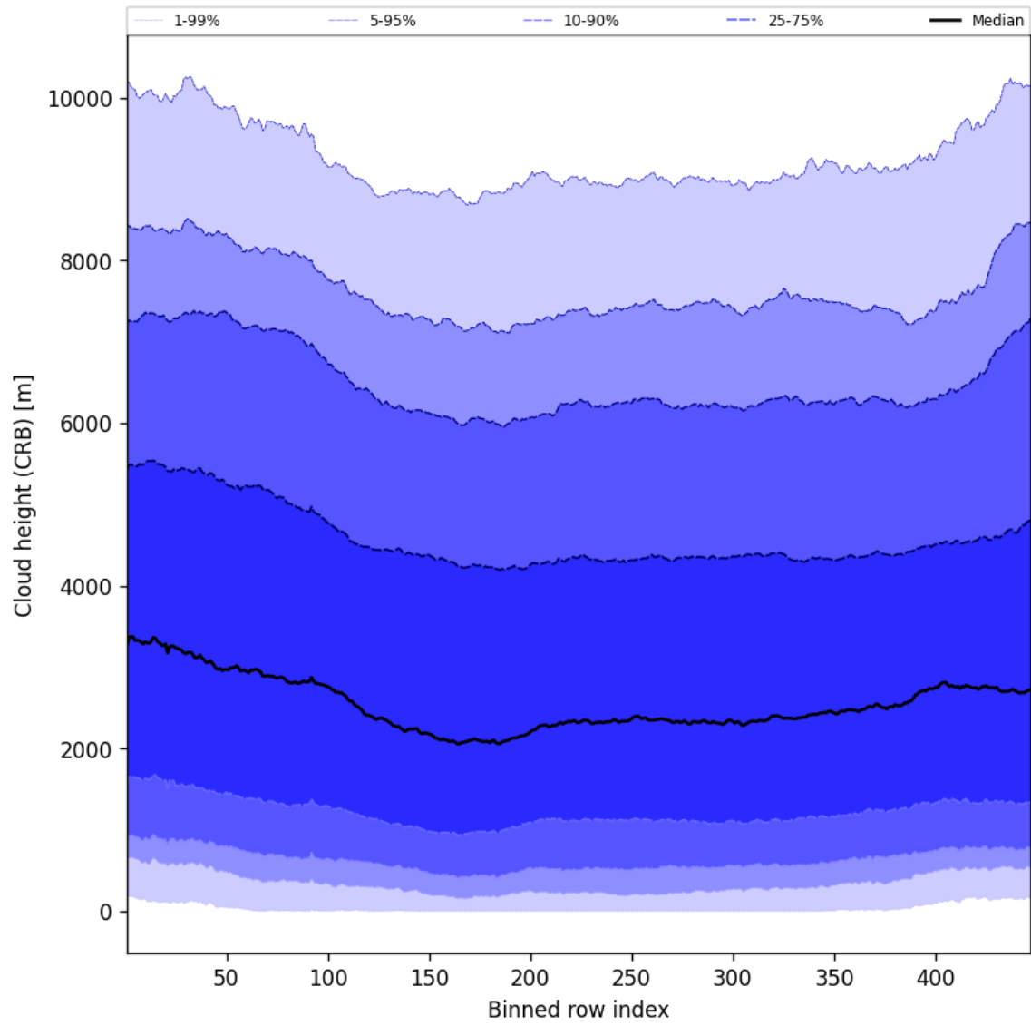
Figure 59: Along track statistics of “Cloud height (CRB)” for 2025-02-27 to 2025-03-01
