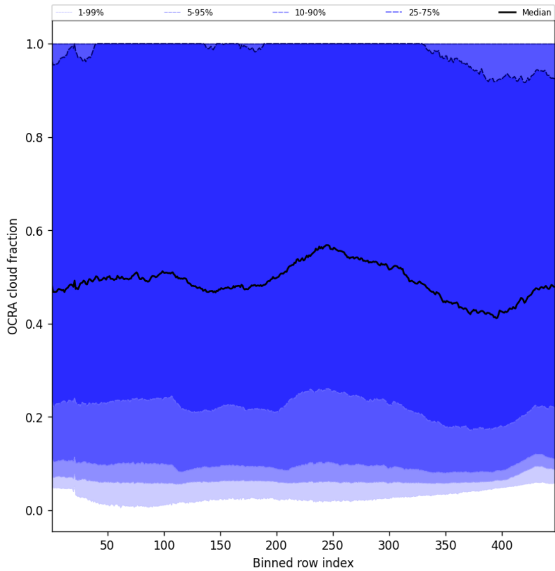
Figure 66: Along track statistics of “OCRA cloud fraction” for 2025-02-27 to 2025-03-01
