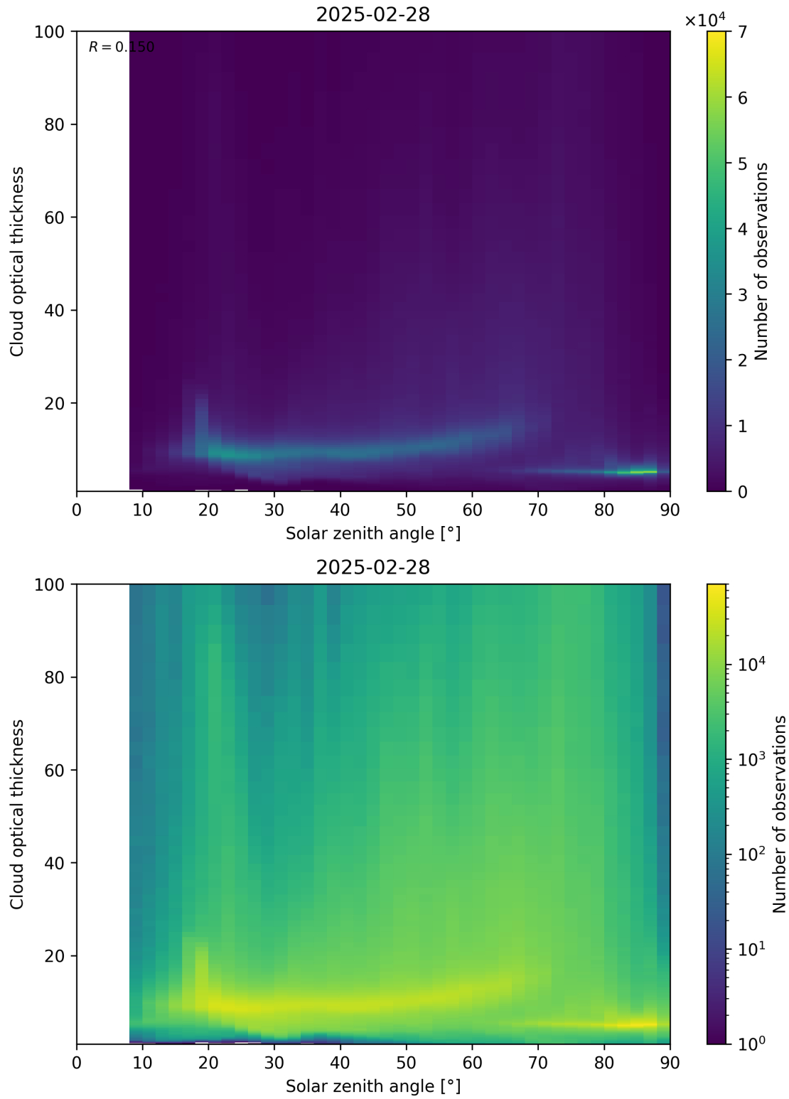
Figure 103: Scatter density plot of “Solar zenith angle” against “Cloud optical thickness” for 2025-02-27 to 2025-03-01.
