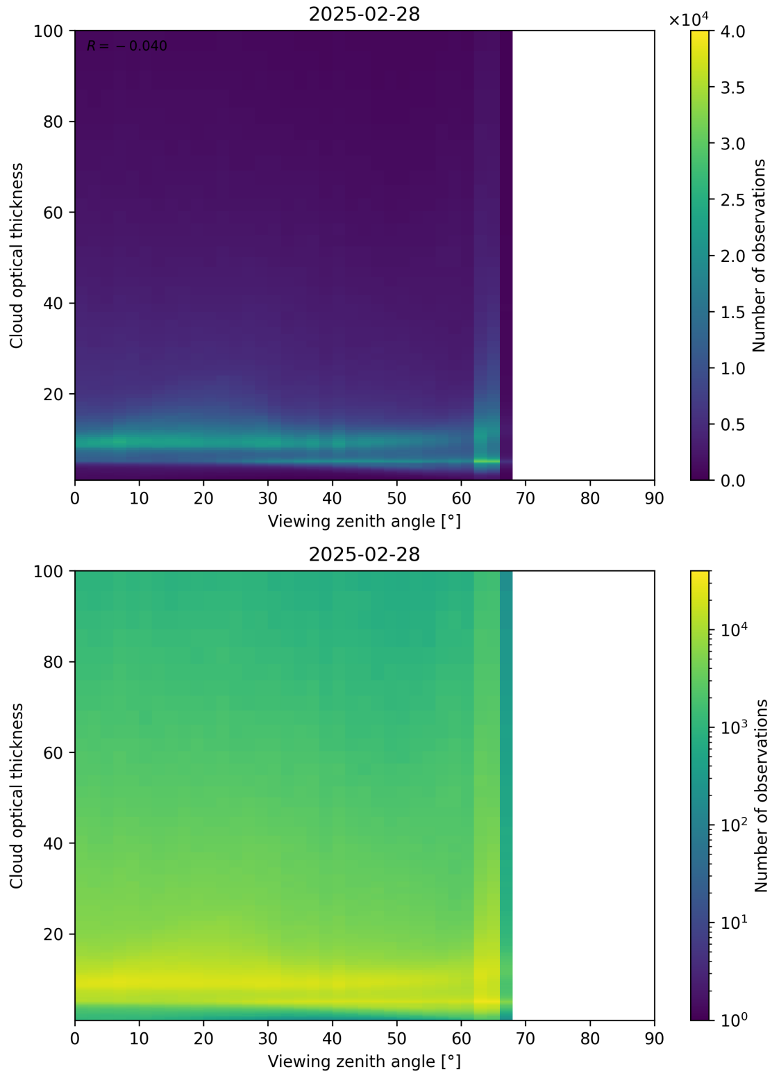
Figure 111: Scatter density plot of “Viewing zenith angle” against “Cloud optical thickness” for 2025-02-27 to 2025-03-01.
