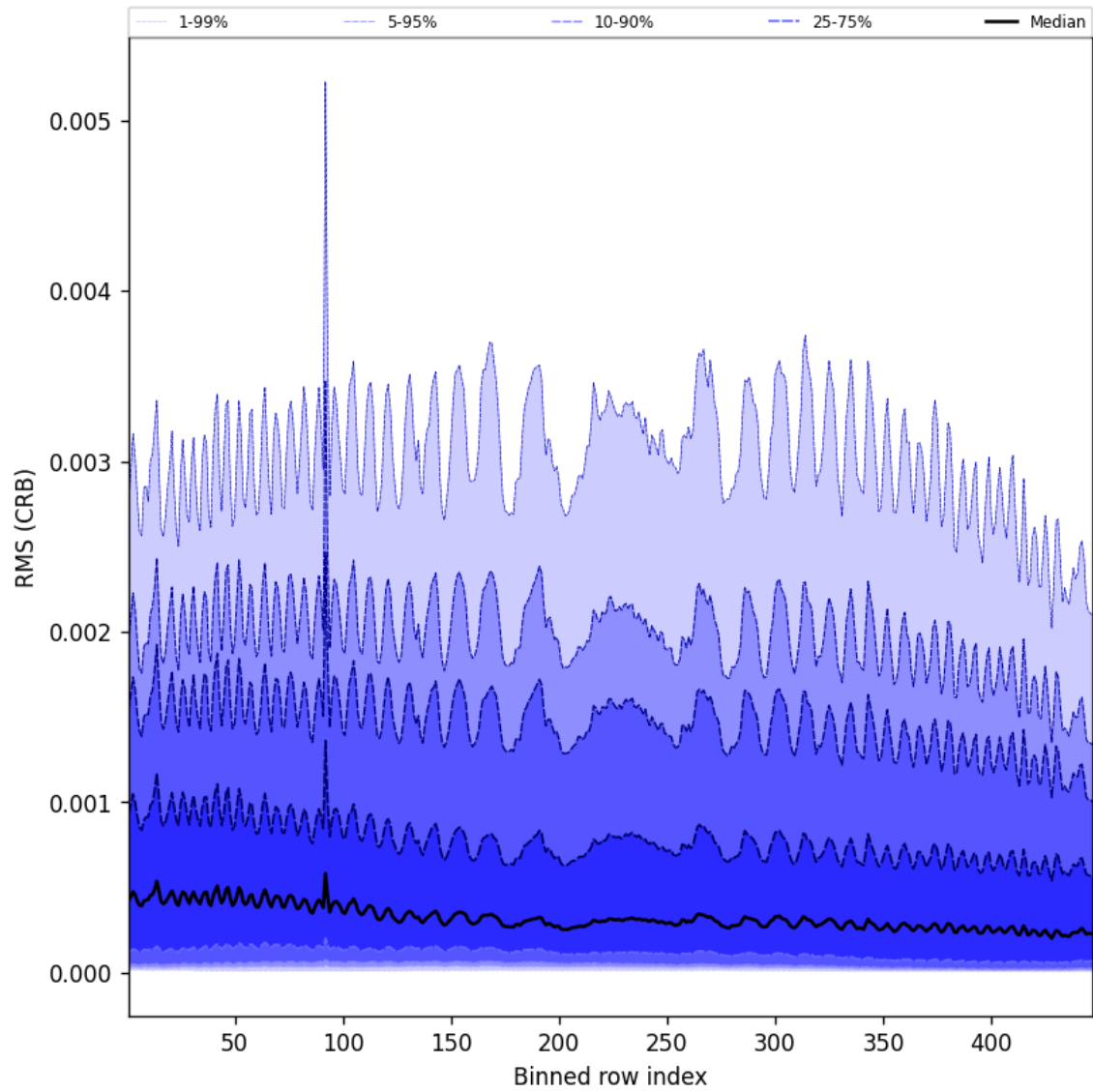
Figure 64: Along track statistics of “RMS (CRB)” for 2025-02-27 to 2025-03-01
