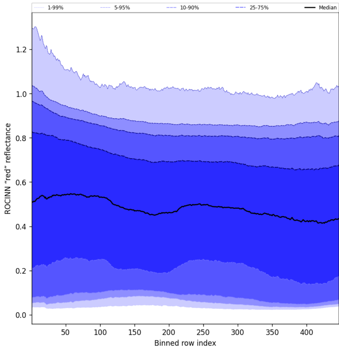
Figure 69: Along track statistics of "ROCINN "red" reflectance" for 2025-02-27 to 2025-03-01
