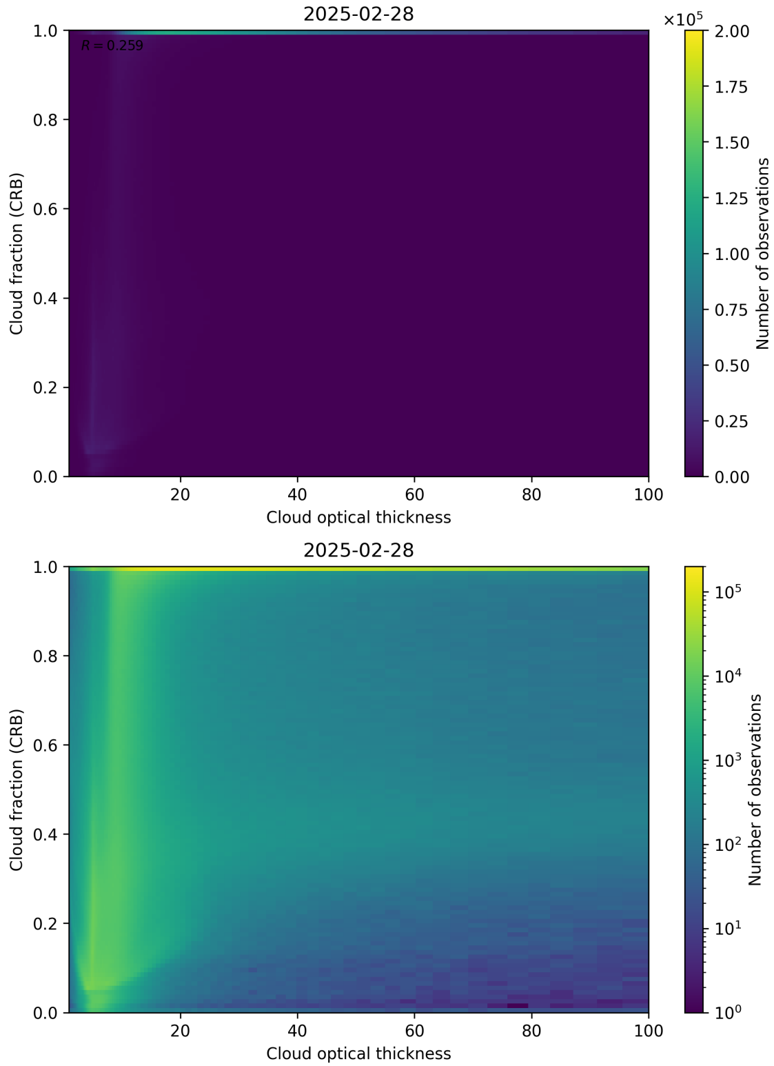
Figure 84: Scatter density plot of “Cloud optical thickness” against “Cloud fraction (CRB)” for 2025-02-27 to 2025-03-01.
