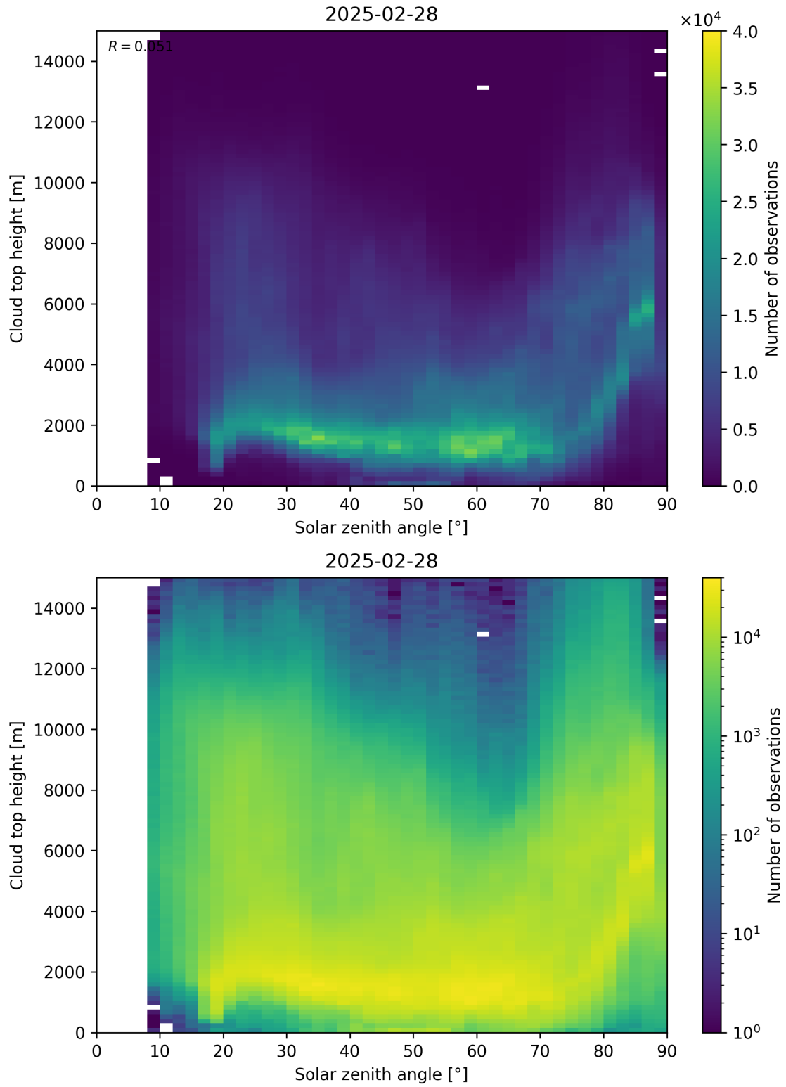
Figure 104: Scatter density plot of “Solar zenith angle” against “Cloud top height” for 2025-02-27 to 2025-03-01.
