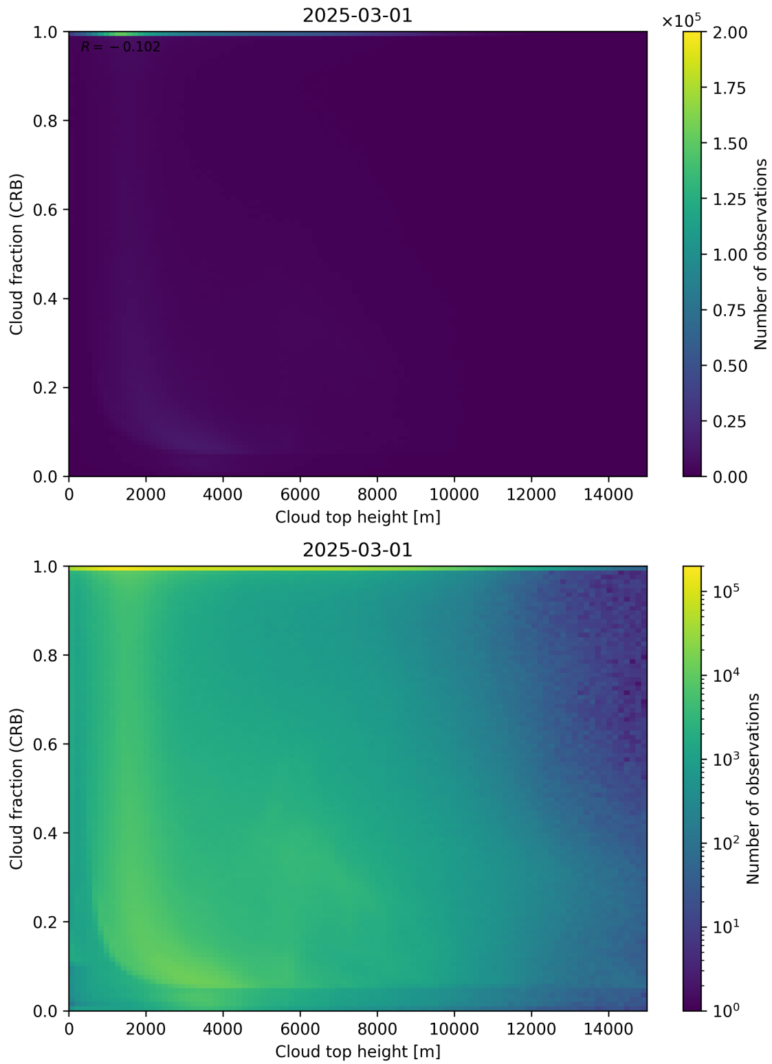
Figure 88: Scatter density plot of “Cloud top height” against “Cloud fraction (CRB)” for 2025-03-01 to 2025-03-02.
