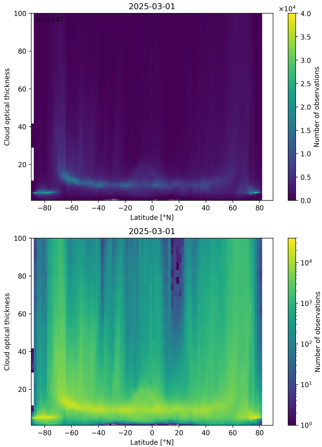
Figure 96: Scatter density plot of “Latitude” against “Cloud optical thickness” for 2025-03-01 to 2025-03-02.
