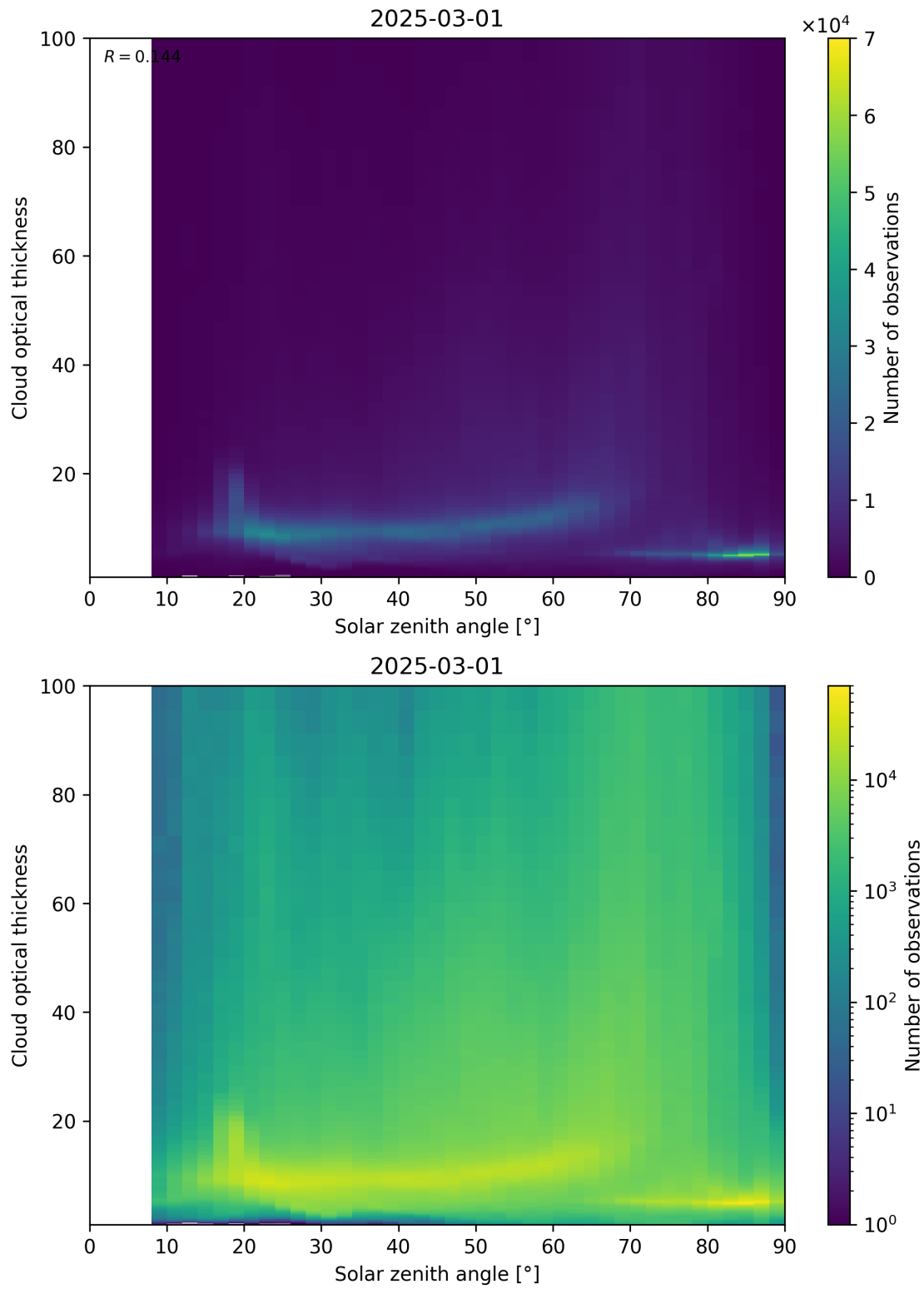
Figure 103: Scatter density plot of “Solar zenith angle” against “Cloud optical thickness” for 2025-03-01 to 2025-03-02.
