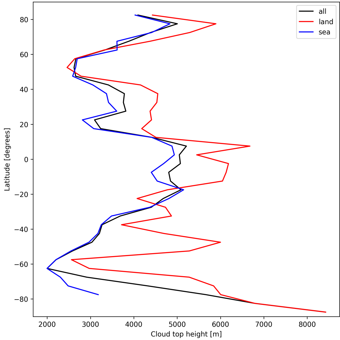
Figure 24: Zonal average of “Cloud top height” for 2025-03-01 to 2025-03-02.
