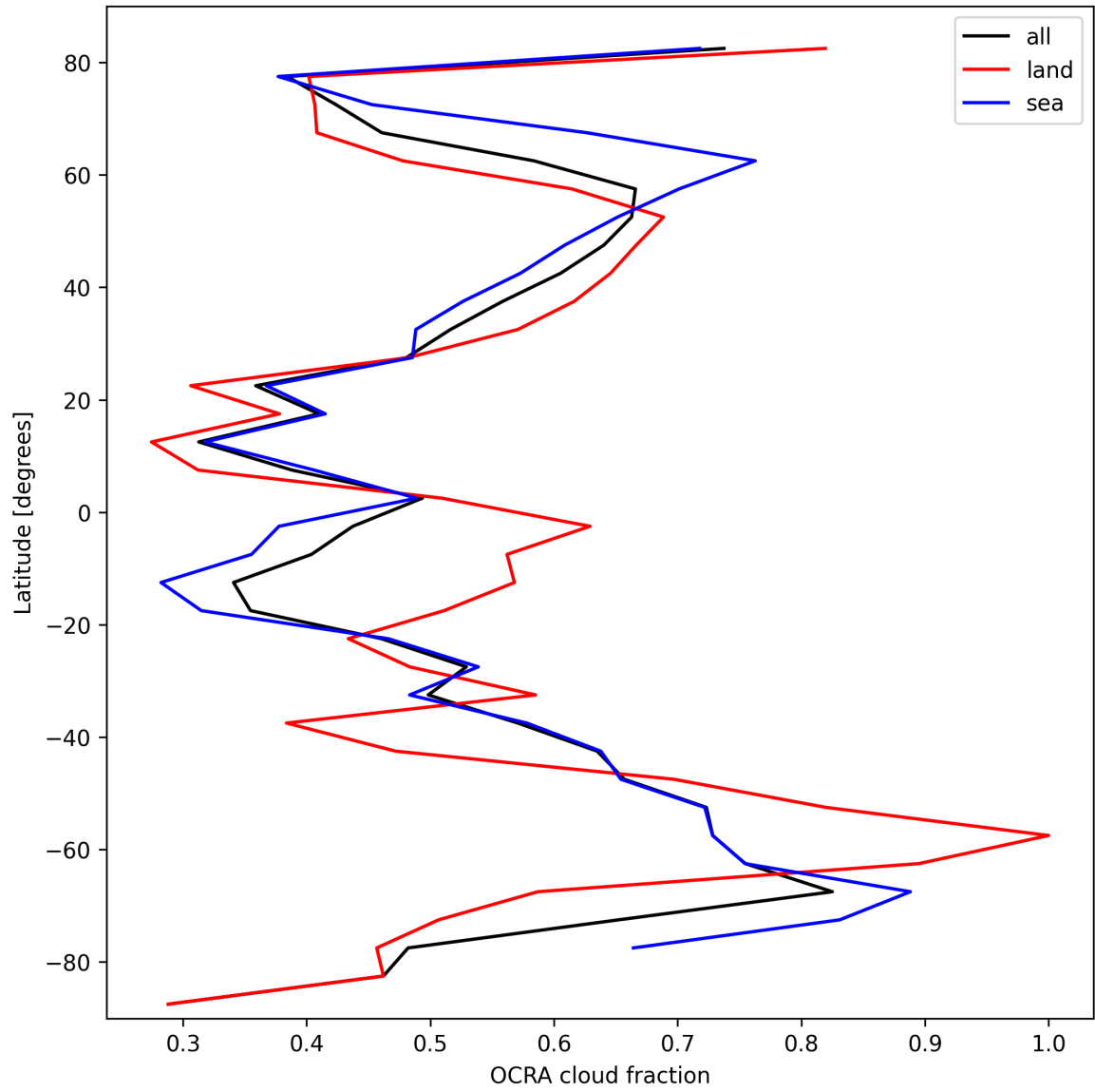
Figure 34: Zonal average of “OCRA cloud fraction” for 2025-03-01 to 2025-03-02.
