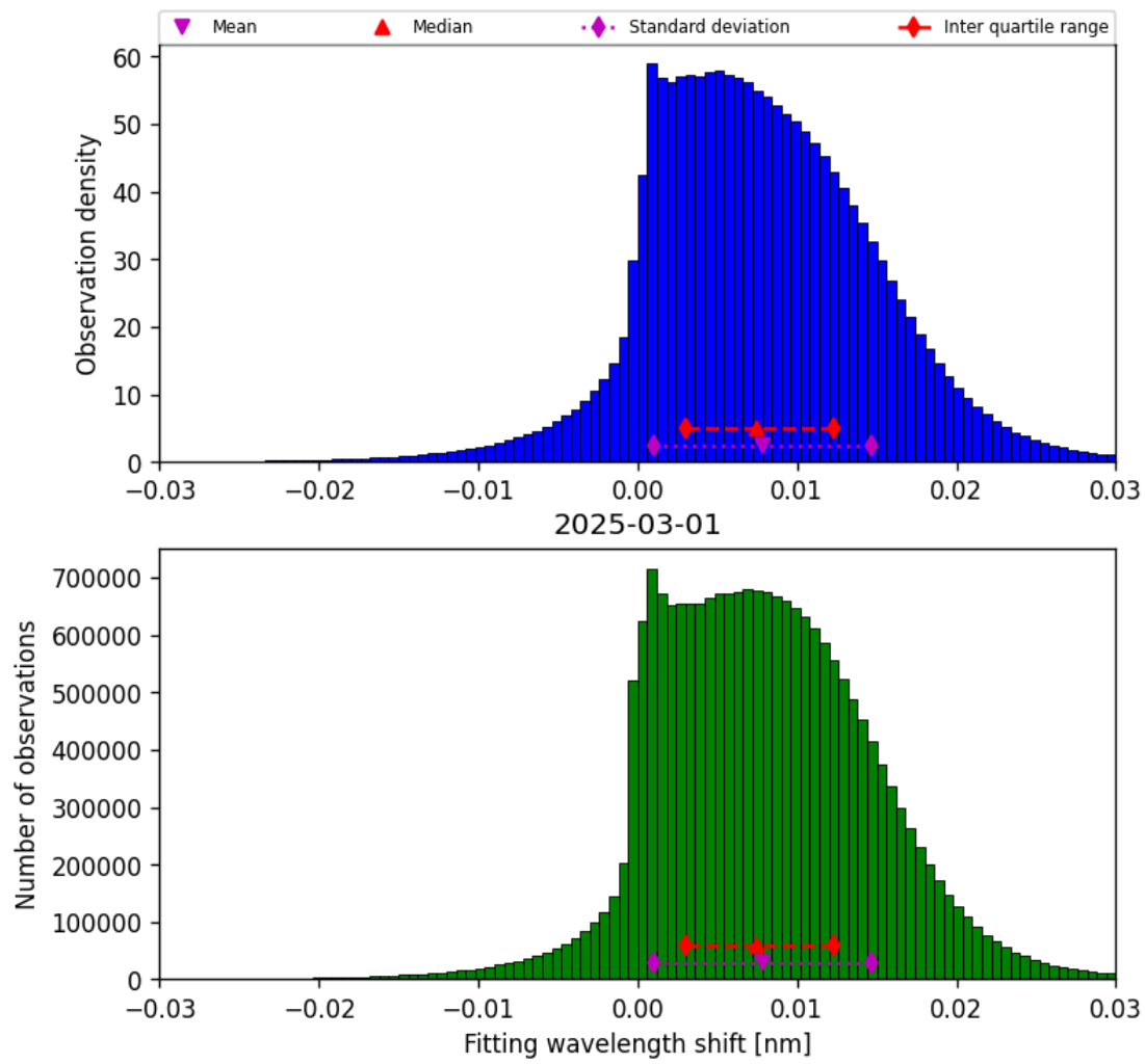
Figure 49: Histogram of “Fitting wavelength shift” for 2025-03-01 to 2025-03-02
