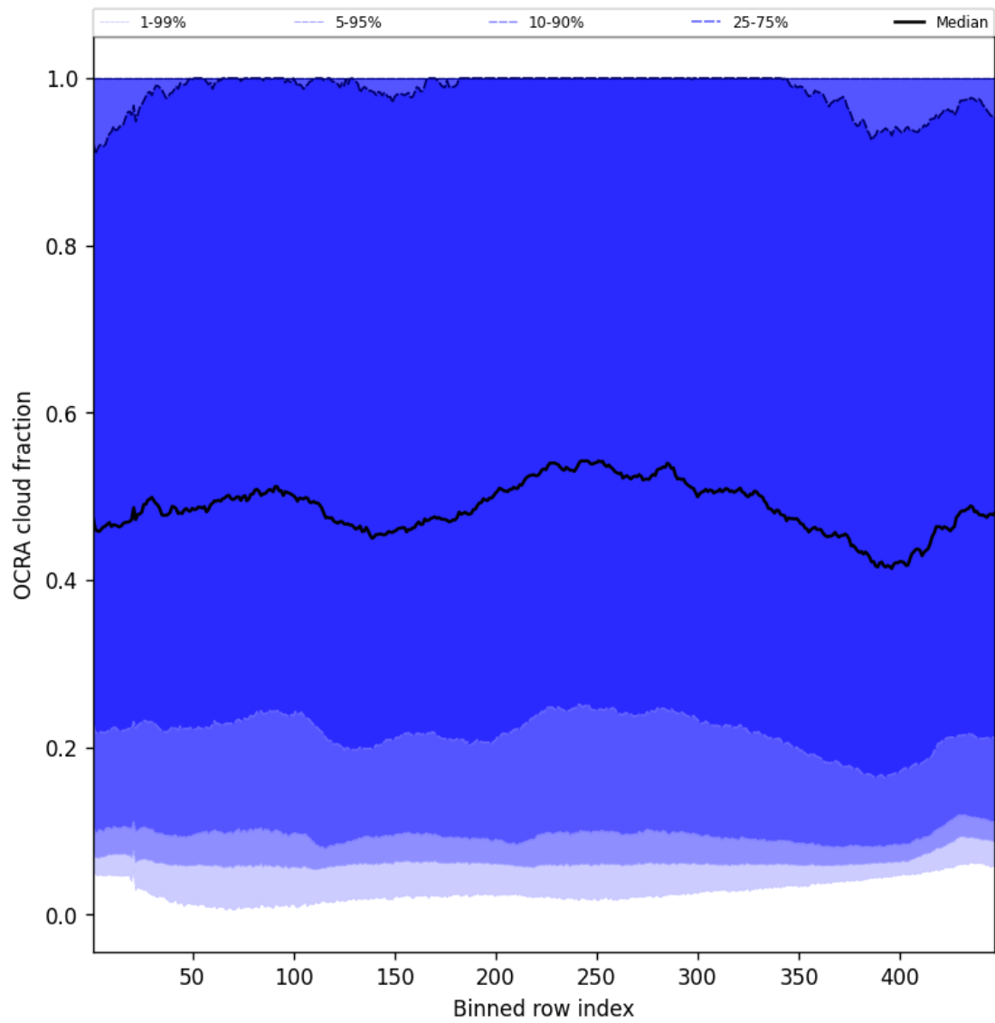
Figure 66: Along track statistics of “OCRA cloud fraction” for 2025-03-01 to 2025-03-02
