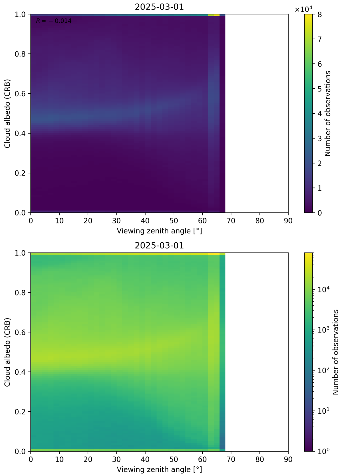
Figure 106: Scatter density plot of “Viewing zenith angle” against “Cloud albedo (CRB)” for 2025-03-01 to 2025-03-02.
