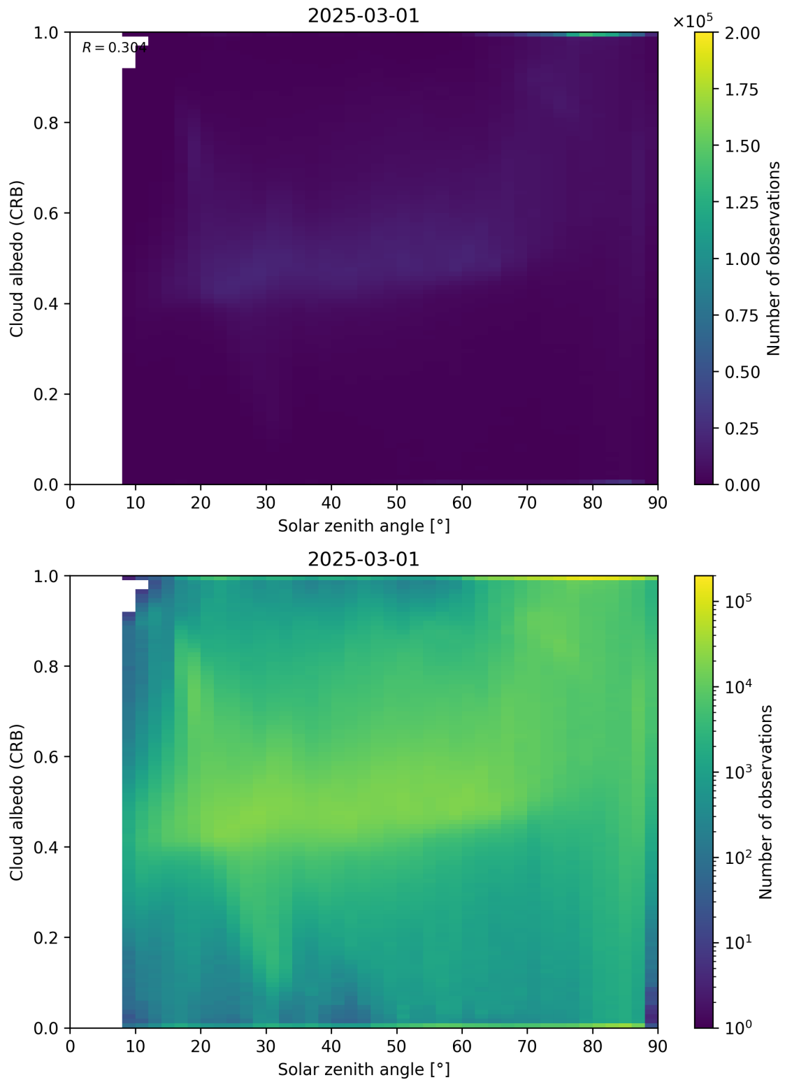
Figure 98: Scatter density plot of “Solar zenith angle” against “Cloud albedo (CRB)” for 2025-03-01 to 2025-03-02.
