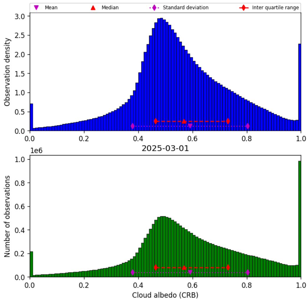
Figure 44: Histogram of “Cloud albedo (CRB)” for 2025-03-01 to 2025-03-02
