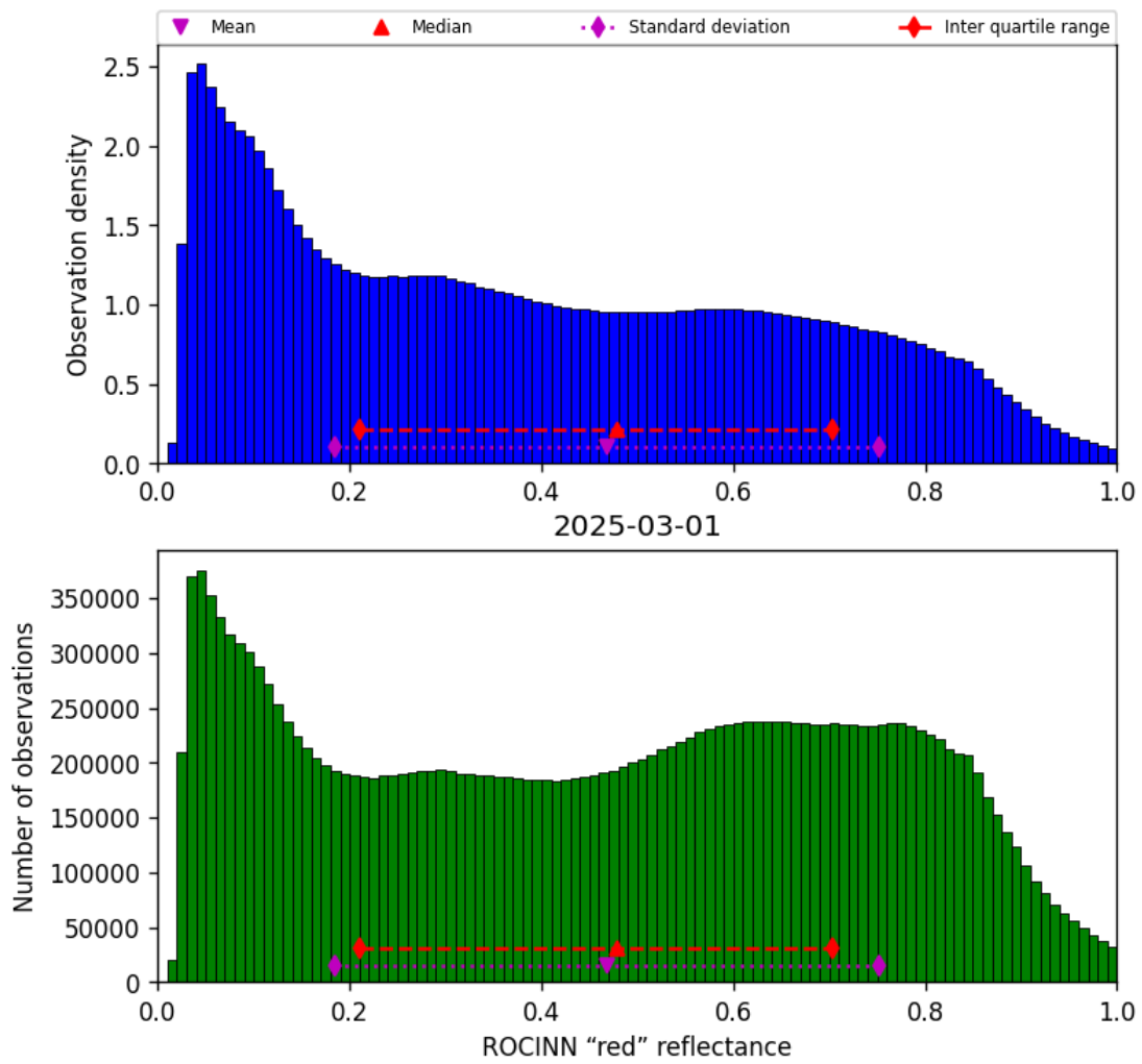
Figure 53: Histogram of “ROCINN “red” reflectance” for 2025-03-01 to 2025-03-02
