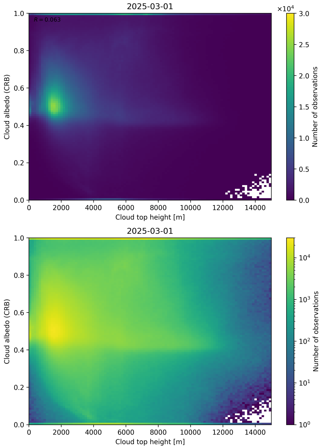
Figure 86: Scatter density plot of “Cloud top height” against “Cloud albedo (CRB)” for 2025-03-01 to 2025-03-02.
