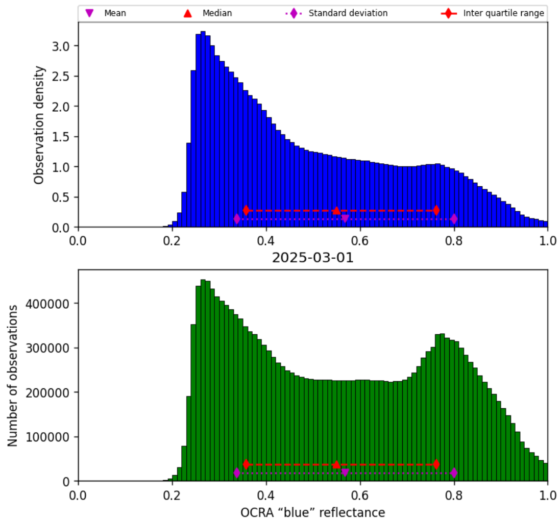
Figure 51: Histogram of “OCRA “blue” reflectance” for 2025-03-01 to 2025-03-02
