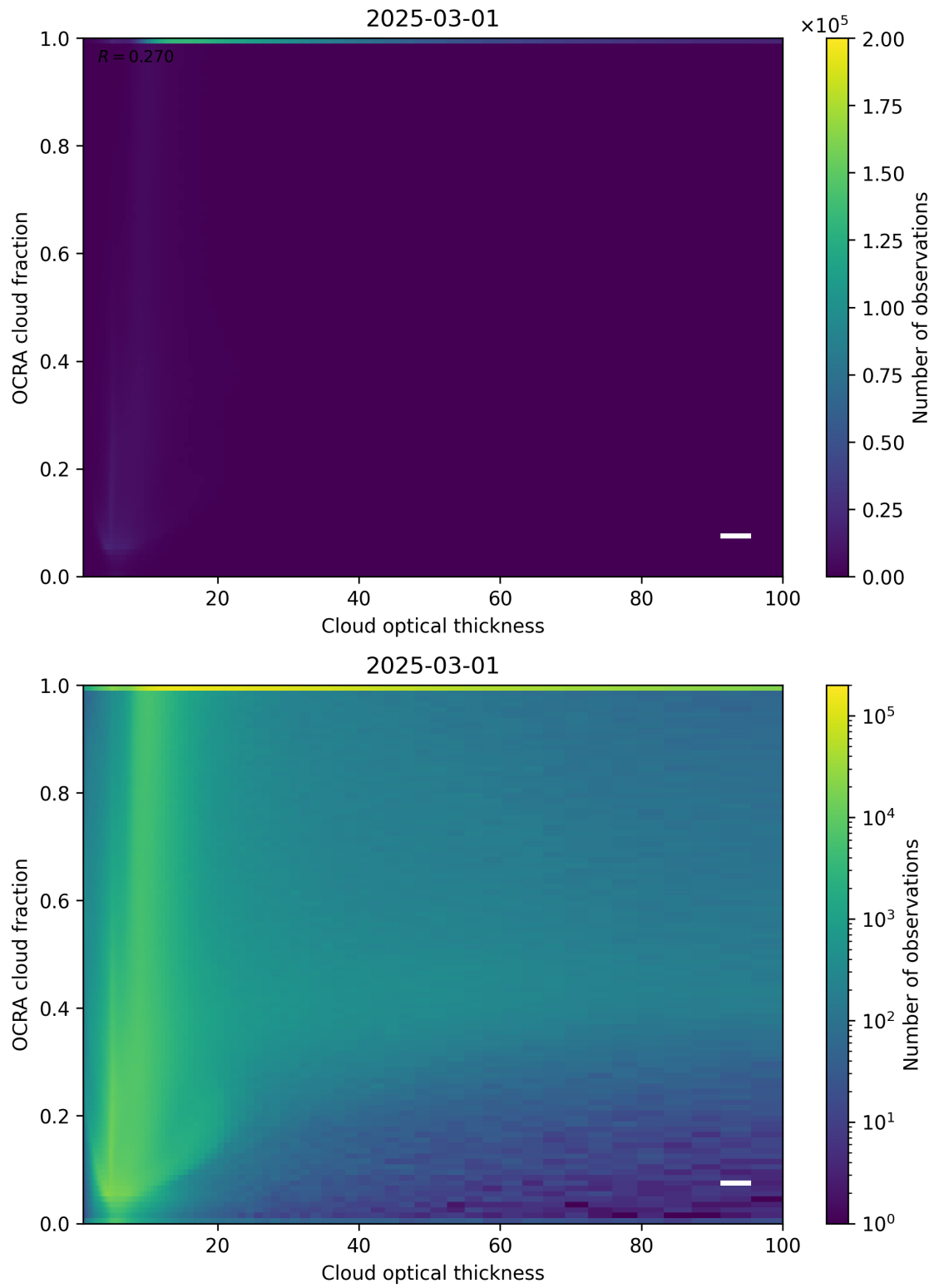
Figure 83: Scatter density plot of “Cloud optical thickness” against “OCRA cloud fraction” for 2025-03-01 to 2025-03-02.
