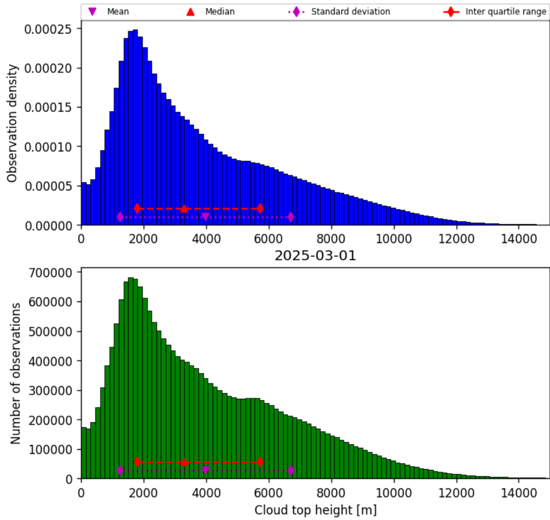
Figure 40: Histogram of “Cloud top height” for 2025-03-01 to 2025-03-02
