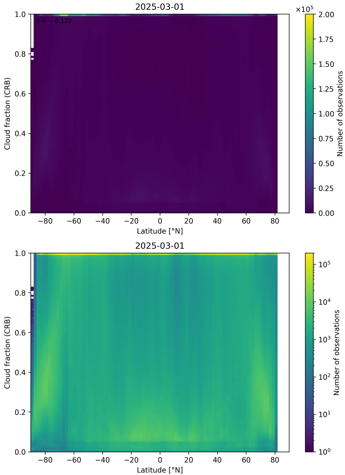
Figure 94: Scatter density plot of “Latitude” against “Cloud fraction (CRB)” for 2025-03-01 to 2025-03-02.
