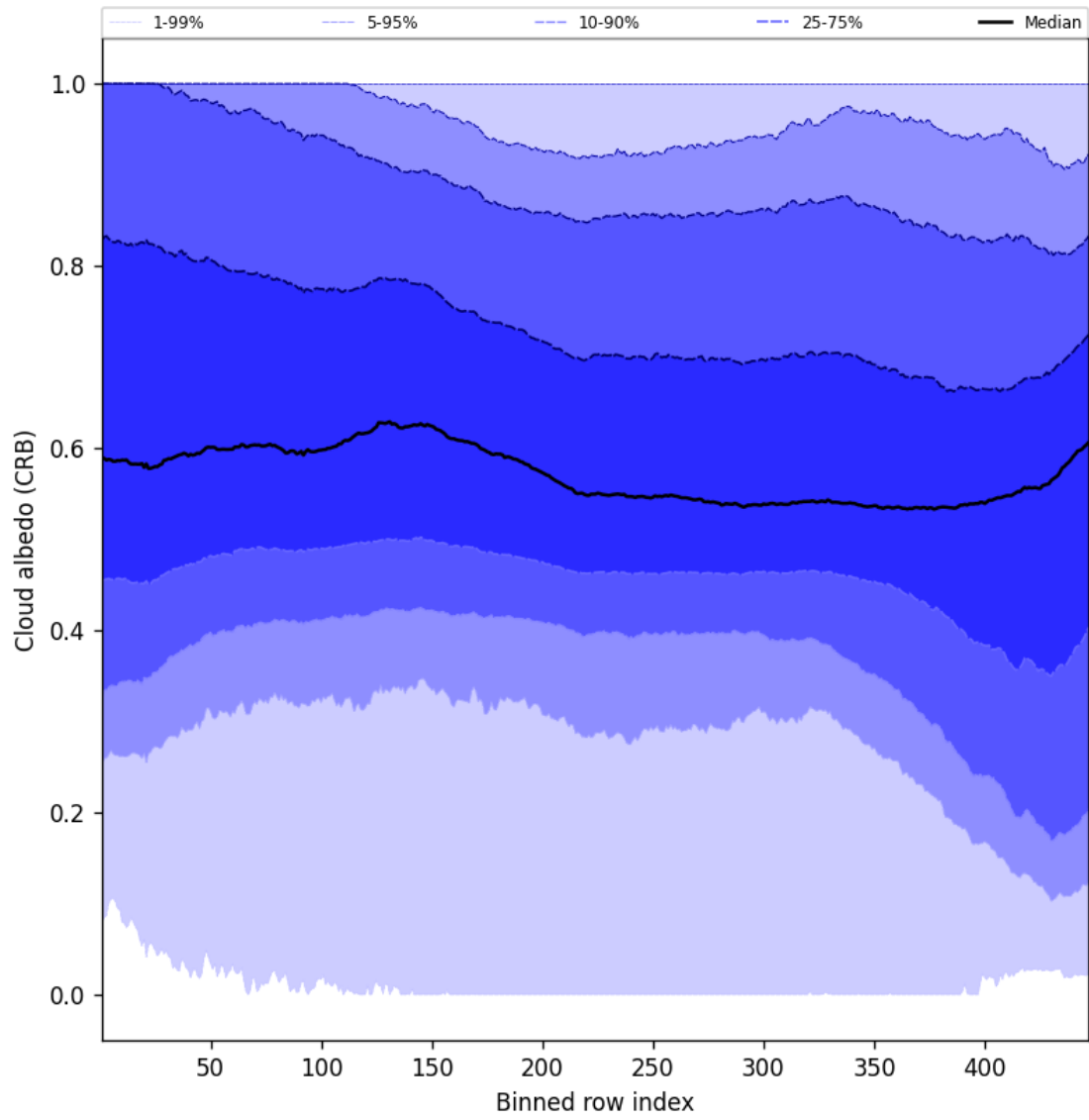
Figure 60: Along track statistics of “Cloud albedo (CRB)” for 2025-03-01 to 2025-03-02
