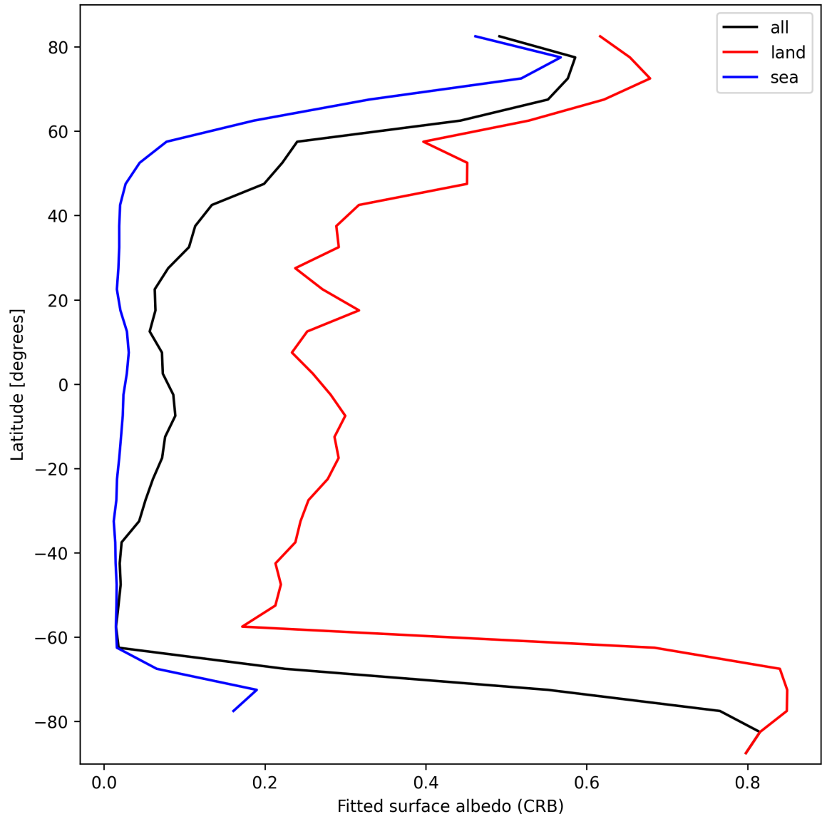
Figure 30: Zonal average of “Fitted surface albedo (CRB)” for 2025-03-01 to 2025-03-02.
