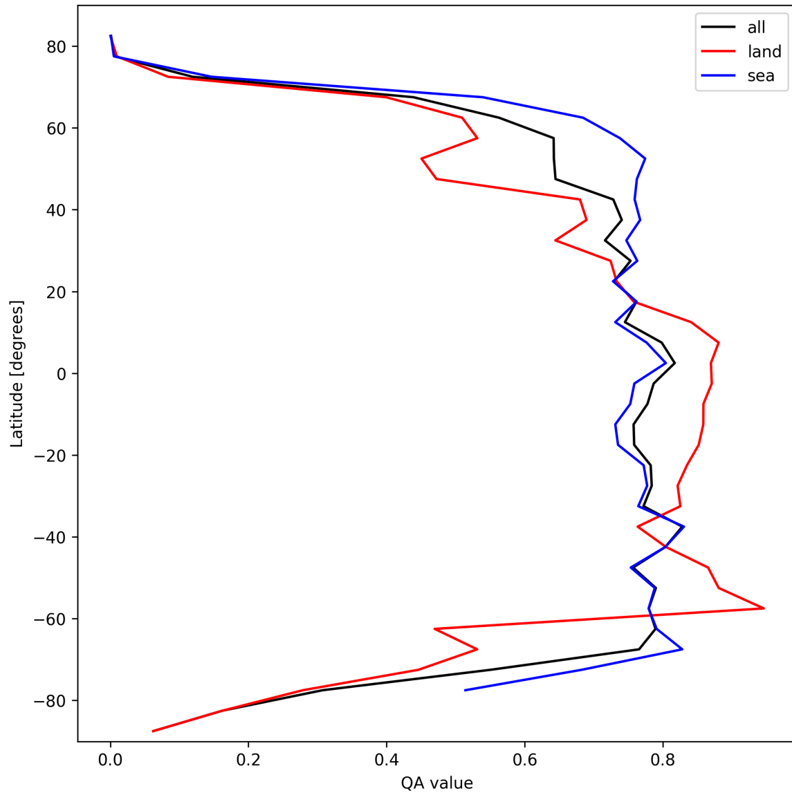
Figure 22: Zonal average of “QA value” for 2025-03-01 to 2025-03-02.
