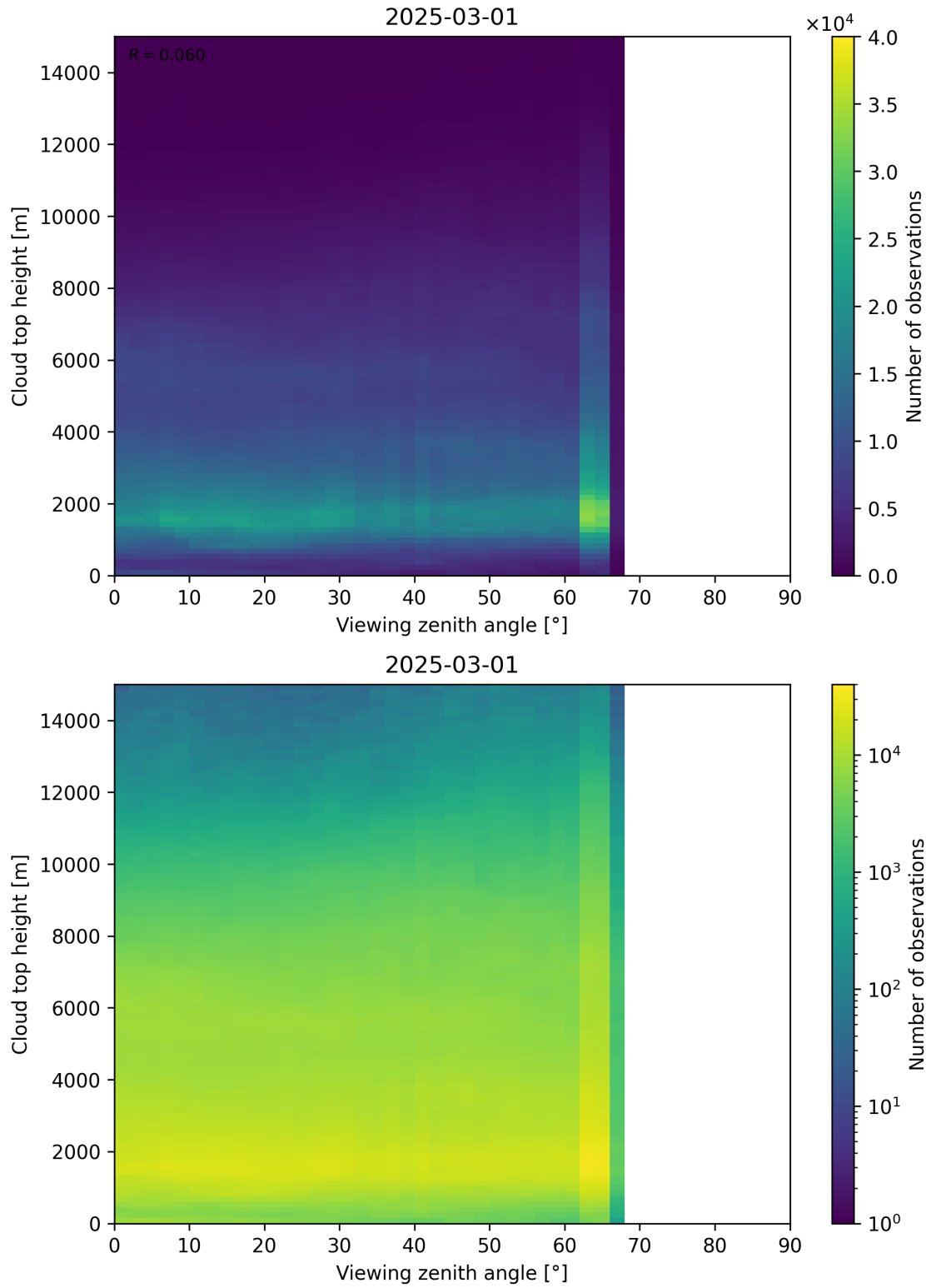
Figure 112: Scatter density plot of “Viewing zenith angle” against “Cloud top height” for 2025-03-01 to 2025-03-02.
