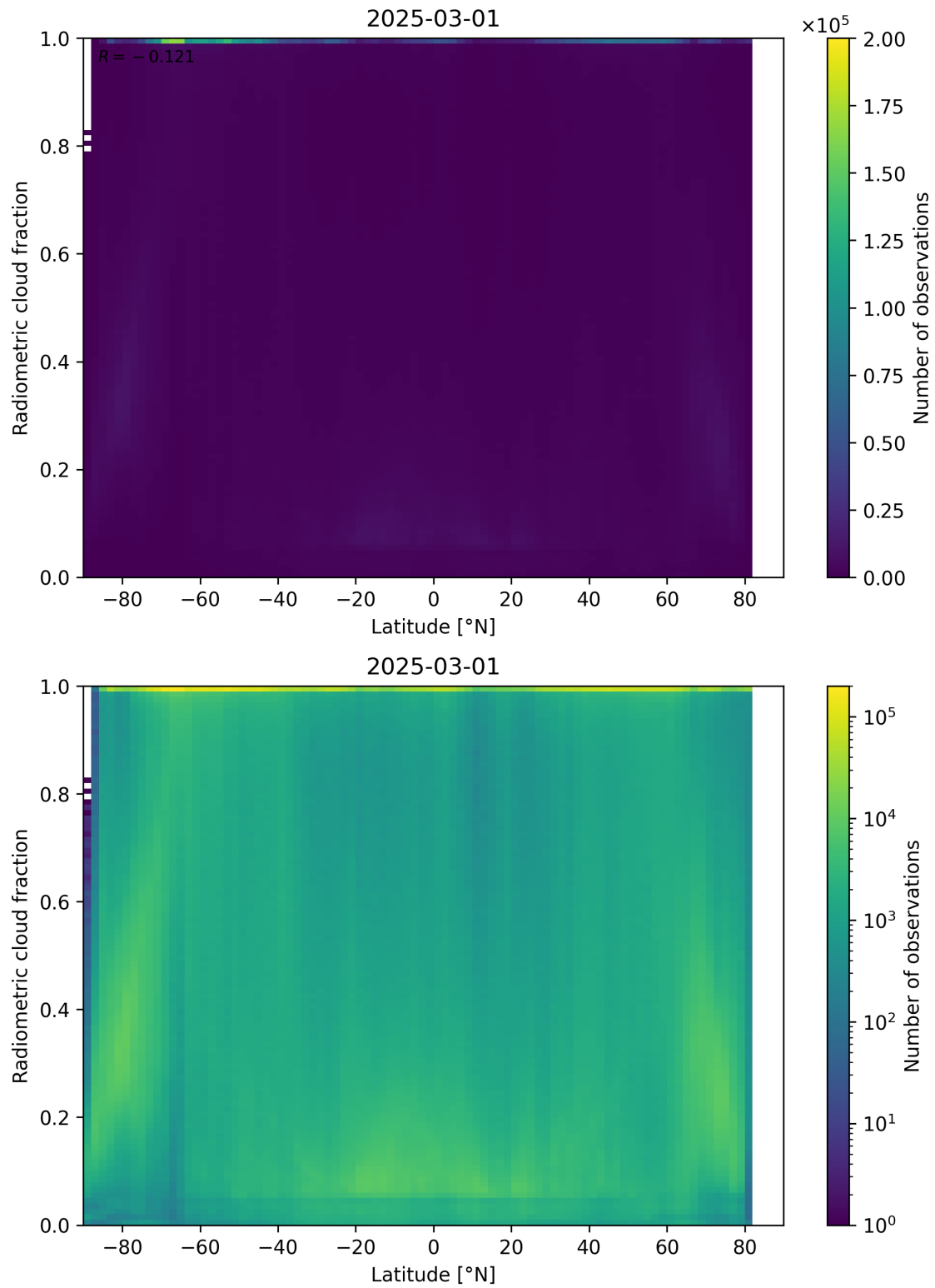
Figure 92: Scatter density plot of “Latitude” against “Radiometric cloud fraction” for 2025-03-01 to 2025-03-02.
