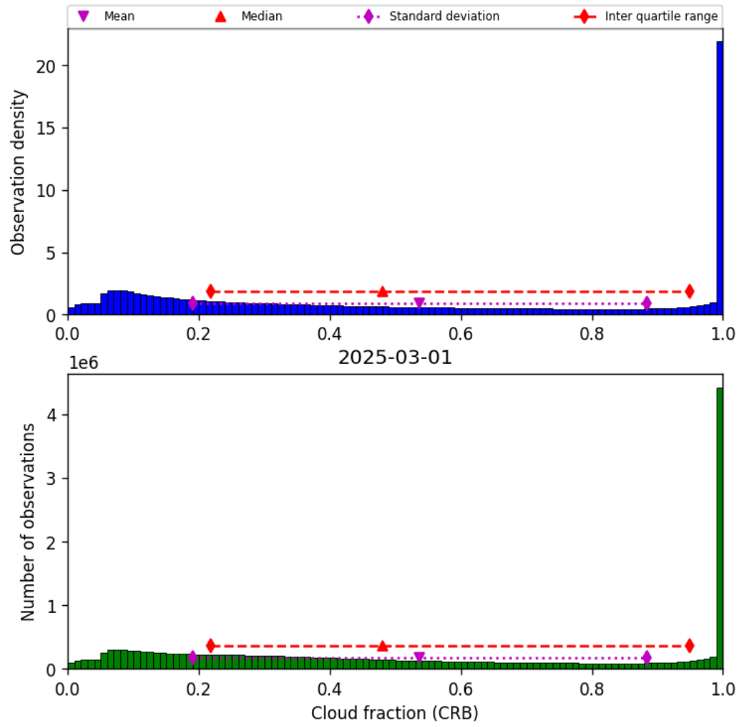
Figure 42: Histogram of “Cloud fraction (CRB)” for 2025-03-01 to 2025-03-02
