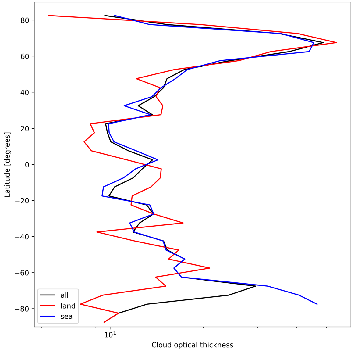
Figure 25: Zonal average of “Cloud optical thickness” for 2025-03-01 to 2025-03-02.
