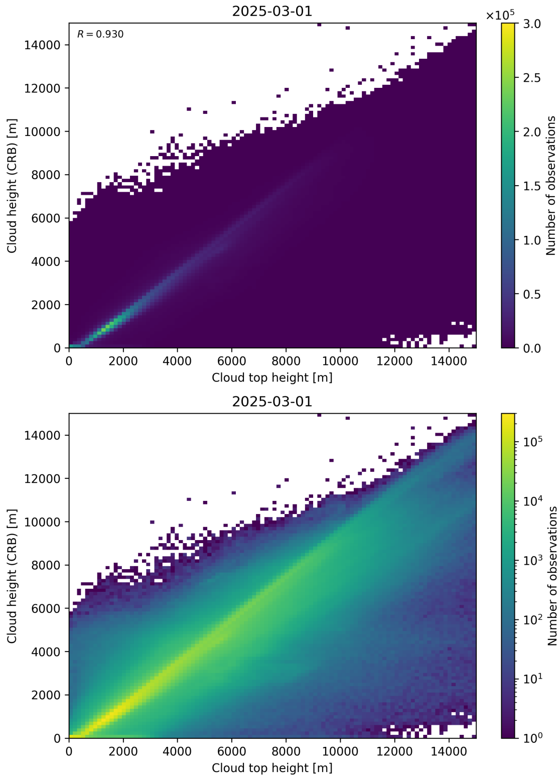
Figure 89: Scatter density plot of “Cloud top height” against “Cloud height (CRB)” for 2025-03-01 to 2025-03-02.
