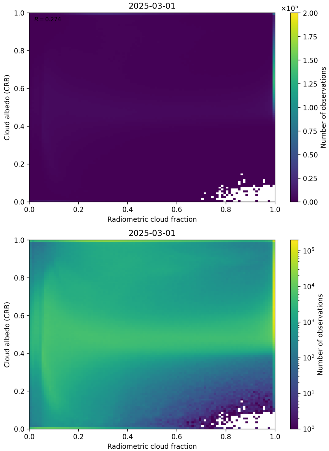
Figure 71: Scatter density plot of “Radiometric cloud fraction” against “Cloud albedo (CRB)” for 2025-03-01 to 2025-03-02.
