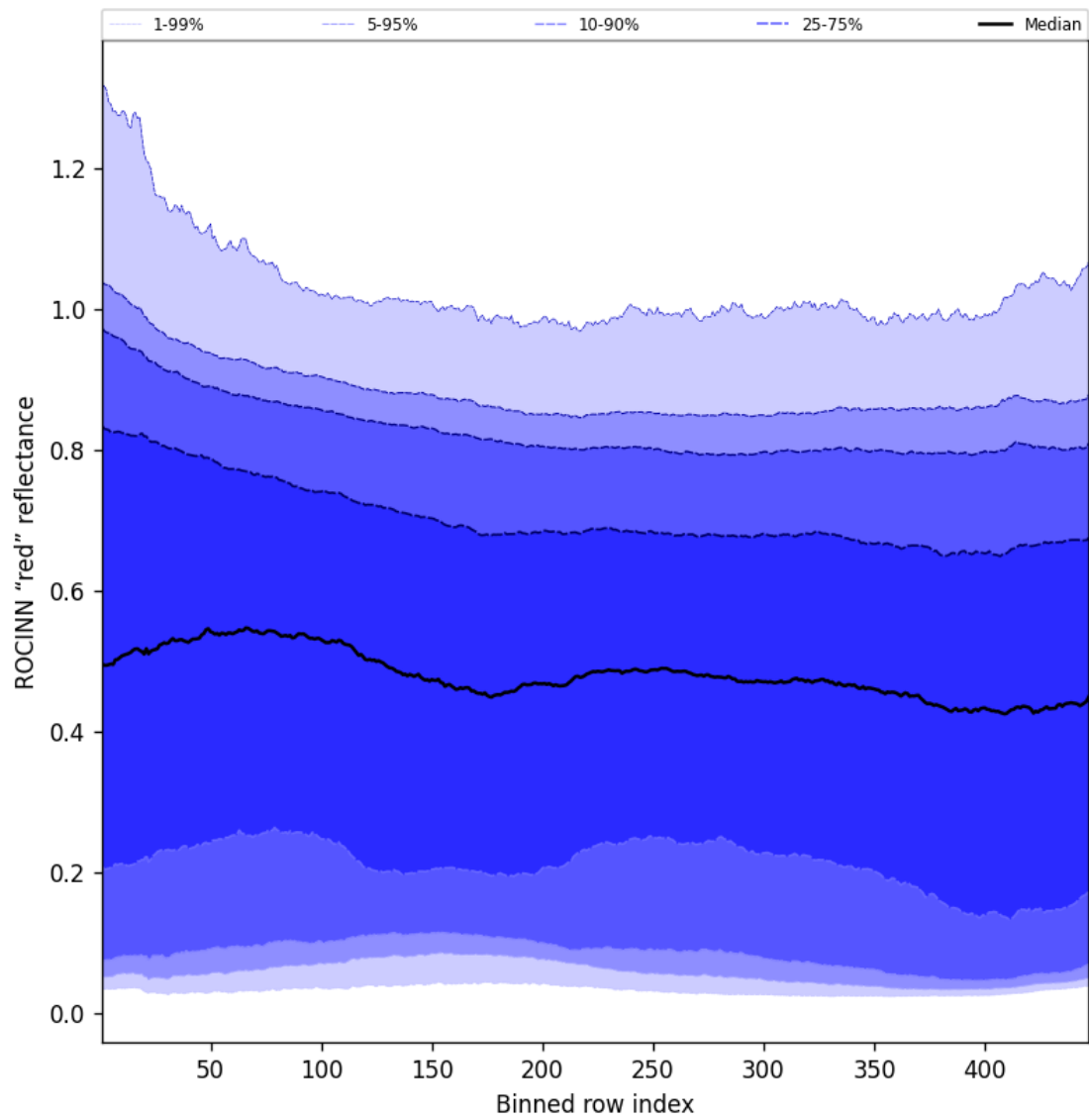
Figure 69: Along track statistics of “ROCINN “red” reflectance” for 2025-03-01 to 2025-03-02
