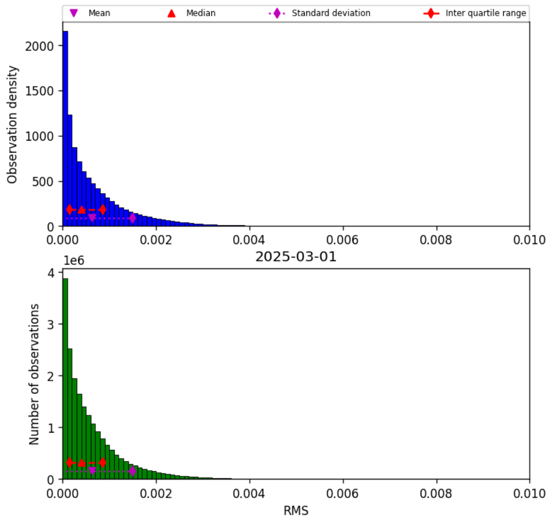
Figure 47: Histogram of “RMS” for 2025-03-01 to 2025-03-02
