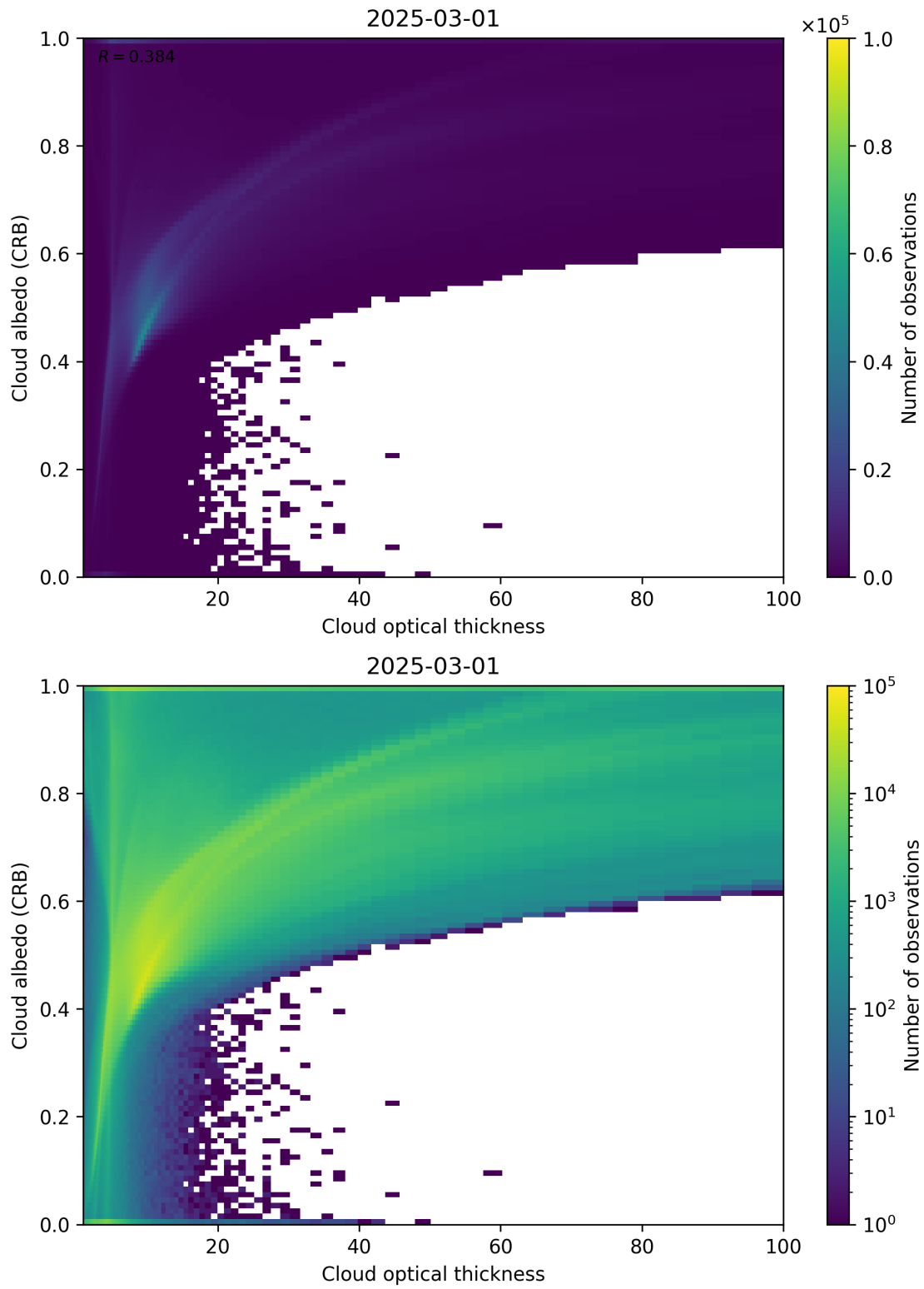
Figure 82: Scatter density plot of “Cloud optical thickness” against “Cloud albedo (CRB)” for 2025-03-01 to 2025-03-02.
