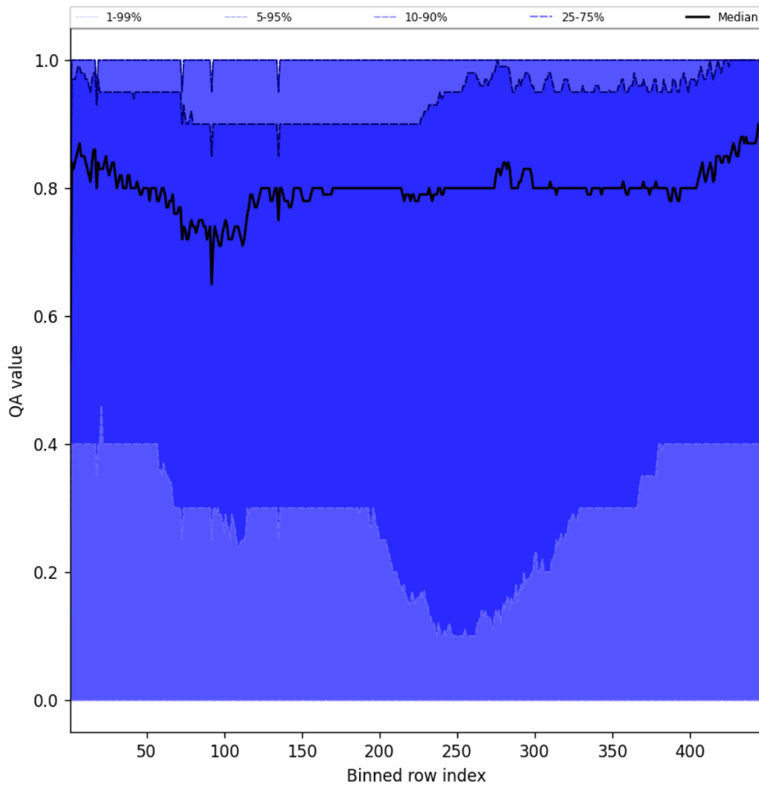
Figure 54: Along track statistics of “QA value” for 2025-03-01 to 2025-03-02
