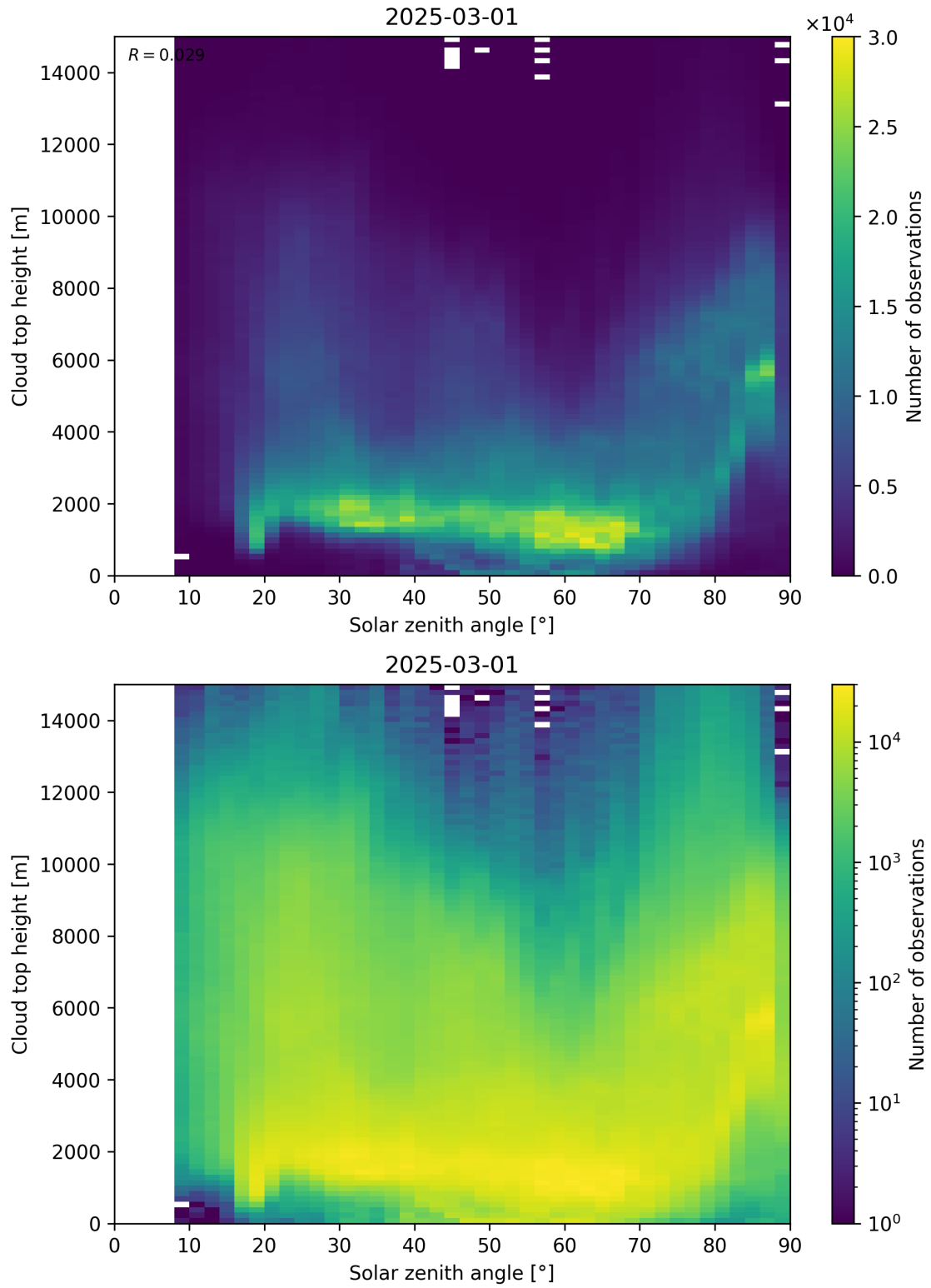
Figure 104: Scatter density plot of “Solar zenith angle” against “Cloud top height” for 2025-03-01 to 2025-03-02.
