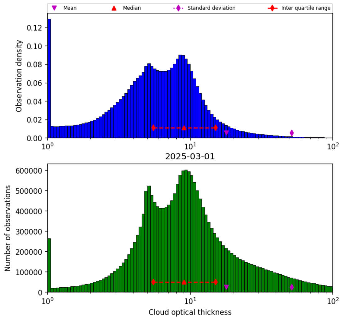
Figure 41: Histogram of “Cloud optical thickness” for 2025-03-01 to 2025-03-02
