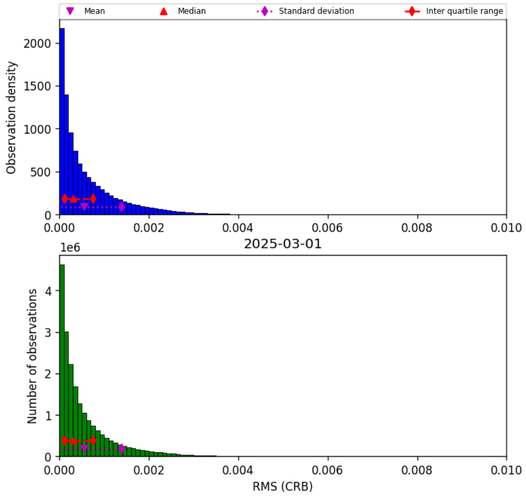
Figure 48: Histogram of “RMS (CRB)” for 2025-03-01 to 2025-03-02
