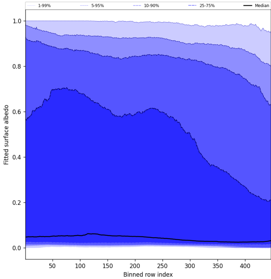
Figure 61: Along track statistics of “Fitted surface albedo” for 2025-03-01 to 2025-03-02
