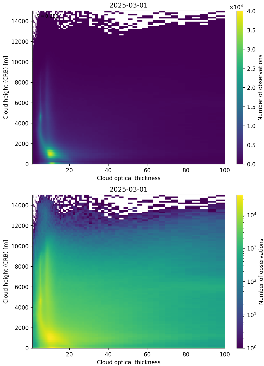
Figure 85: Scatter density plot of “Cloud optical thickness” against “Cloud height (CRB)” for 2025-03-01 to 2025-03-02.
