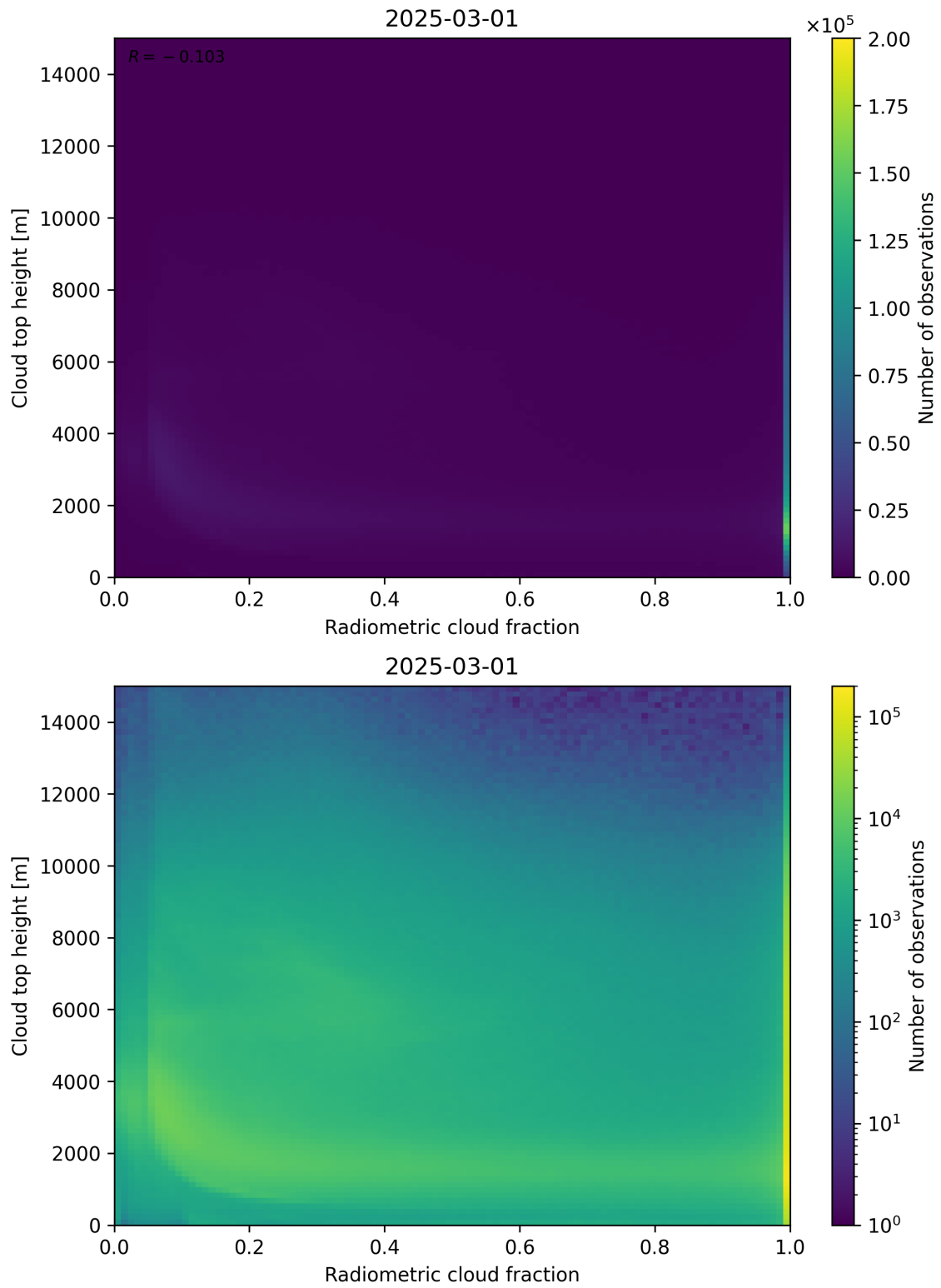
Figure 76: Scatter density plot of “Radiometric cloud fraction” against “Cloud top height” for 2025-03-01 to 2025-03-02.
