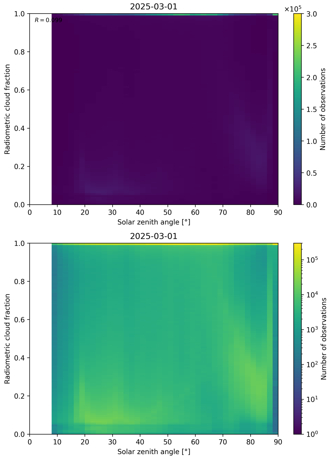
Figure 99: Scatter density plot of “Solar zenith angle” against “Radiometric cloud fraction” for 2025-03-01 to 2025-03-02.
