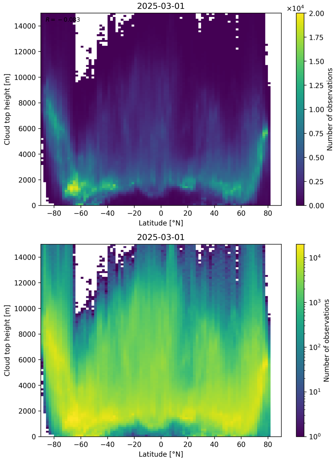
Figure 97: Scatter density plot of “Latitude” against “Cloud top height” for 2025-03-01 to 2025-03-02.
