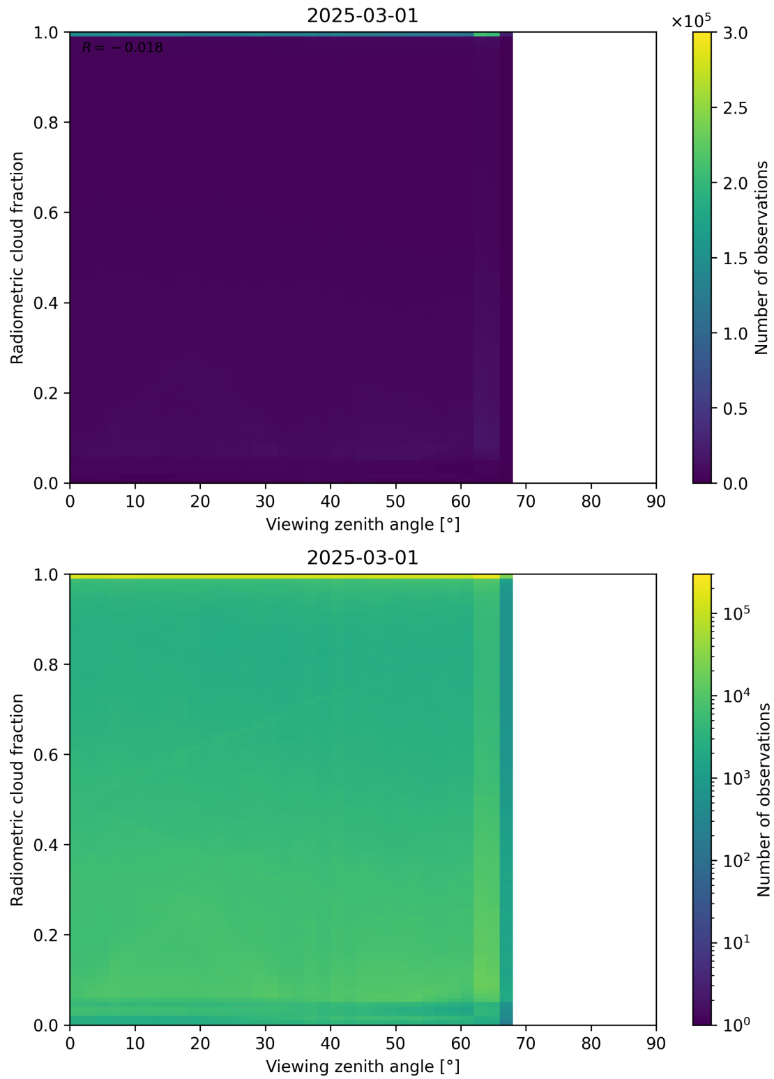
Figure 107: Scatter density plot of “Viewing zenith angle” against “Radiometric cloud fraction” for 2025-03-01 to 2025-03-02.
