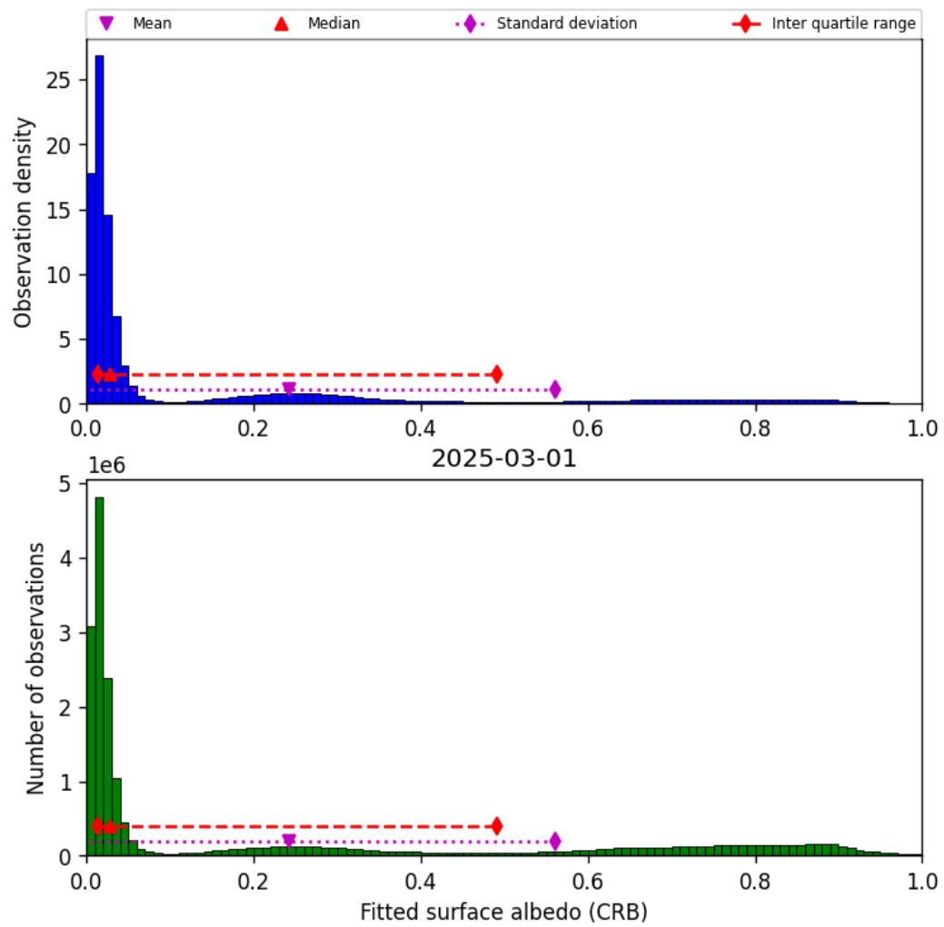
Figure 46: Histogram of “Fitted surface albedo (CRB)” for 2025-03-01 to 2025-03-02
