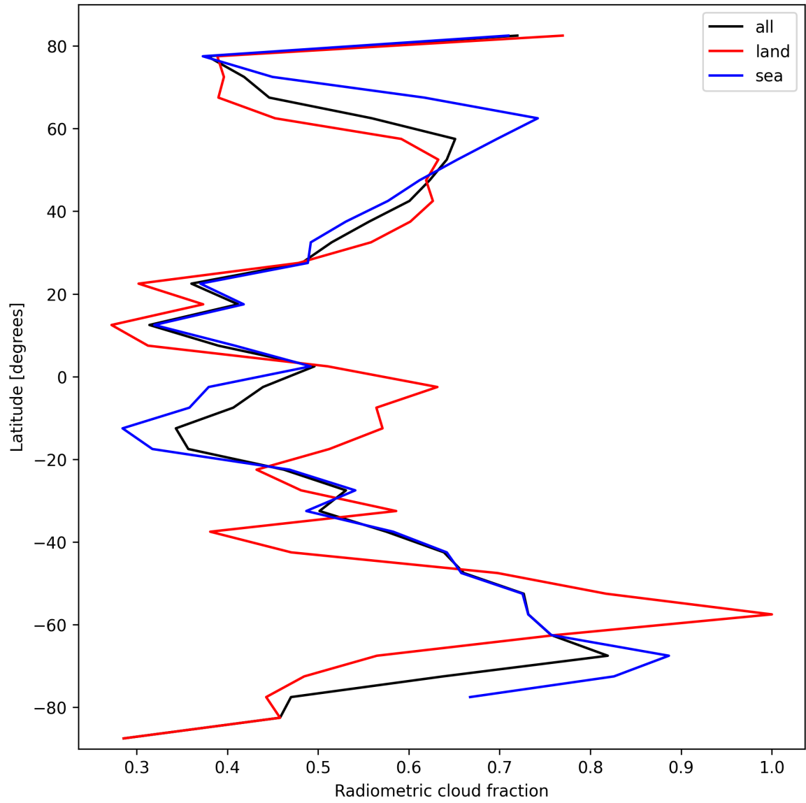
Figure 23: Zonal average of “Radiometric cloud fraction” for 2025-03-01 to 2025-03-02.
