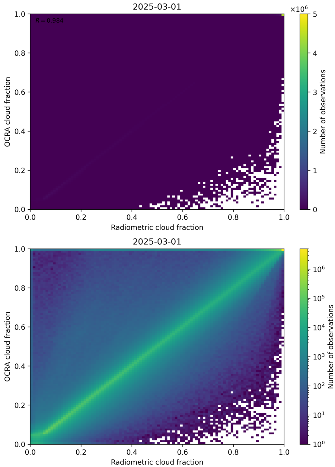
Figure 72: Scatter density plot of “Radiometric cloud fraction” against “OCRA cloud fraction” for 2025-03-01 to 2025-03-02.
