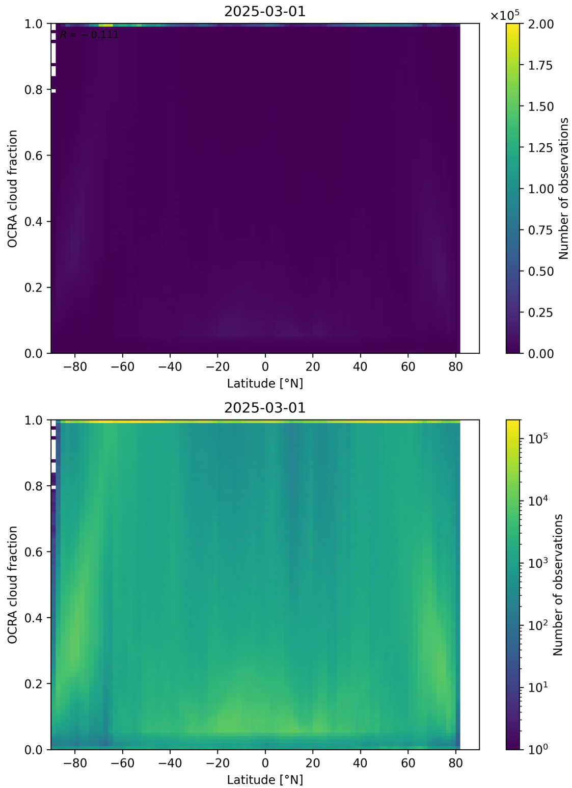
Figure 93: Scatter density plot of “Latitude” against “OCRA cloud fraction” for 2025-03-01 to 2025-03-02.
