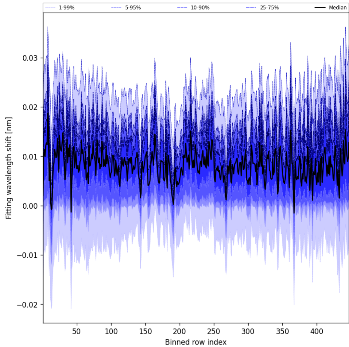
Figure 65: Along track statistics of “Fitting wavelength shift” for 2025-03-01 to 2025-03-02
