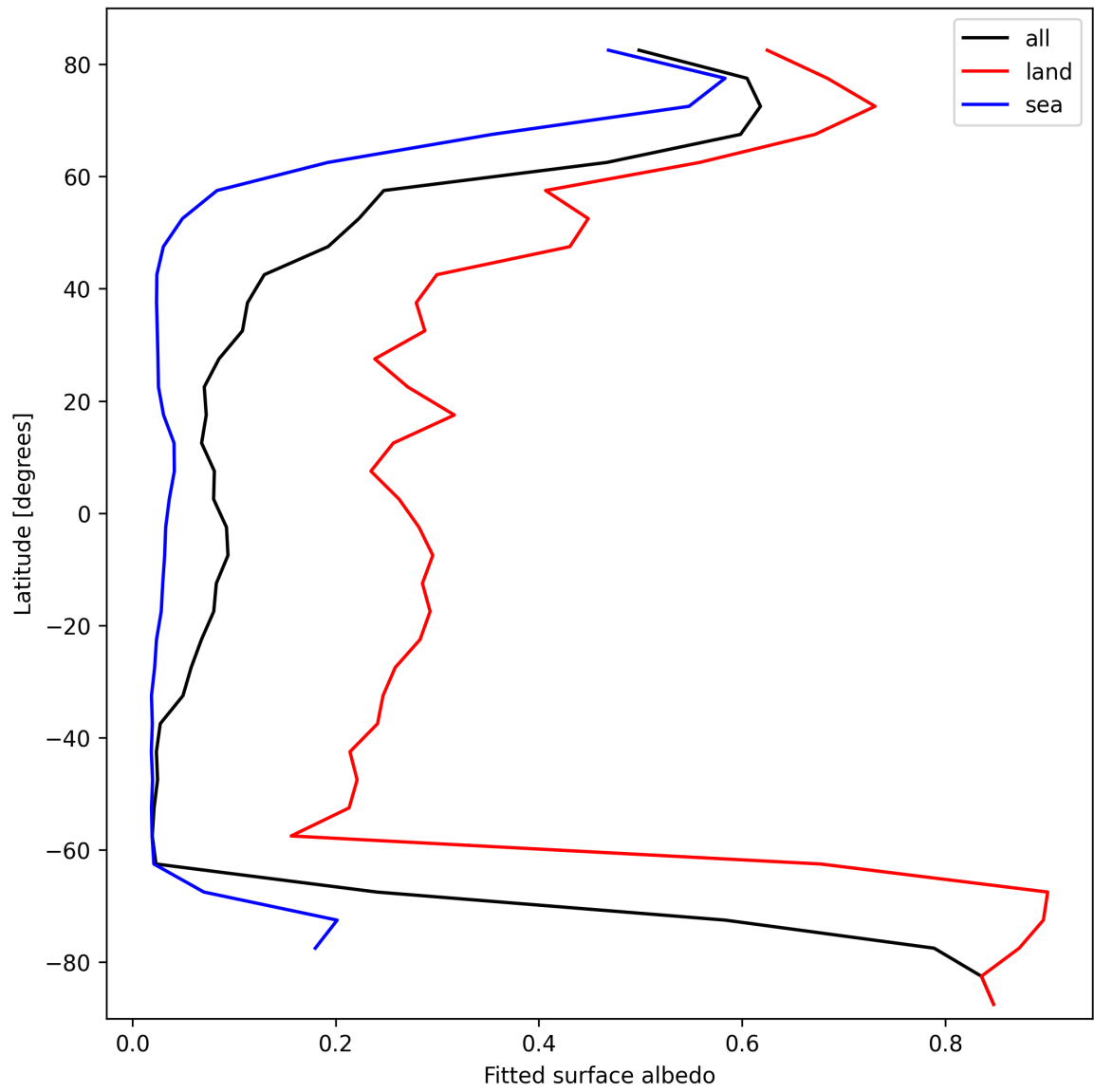
Figure 29: Zonal average of “Fitted surface albedo” for 2025-03-01 to 2025-03-02.
