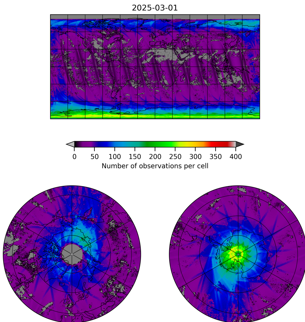
Figure 21: Map of the number of observations for 2025-03-01 to 2025-03-02
