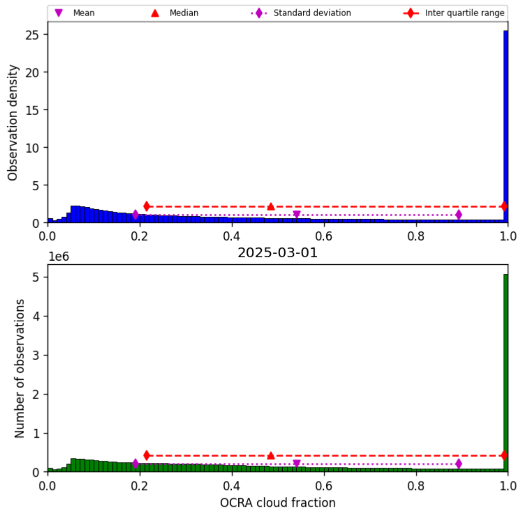
Figure 50: Histogram of “OCRA cloud fraction” for 2025-03-01 to 2025-03-02
