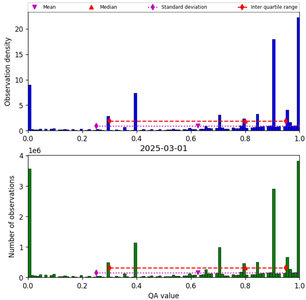
Figure 38: Histogram of “QA value” for 2025-03-01 to 2025-03-02
