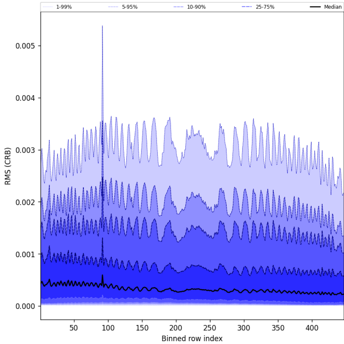
Figure 64: Along track statistics of “RMS (CRB)” for 2025-03-01 to 2025-03-02
