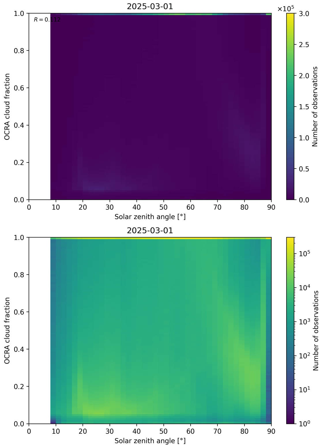
Figure 100: Scatter density plot of “Solar zenith angle” against “OCRA cloud fraction” for 2025-03-01 to 2025-03-02.
