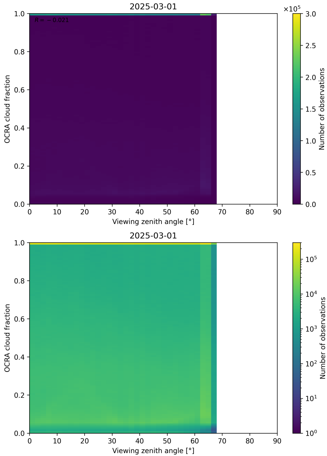
Figure 108: Scatter density plot of “Viewing zenith angle” against “OCRA cloud fraction” for 2025-03-01 to 2025-03-02.
