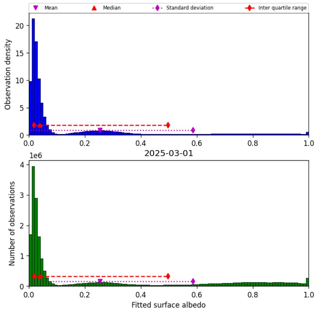
Figure 45: Histogram of “Fitted surface albedo” for 2025-03-01 to 2025-03-02
