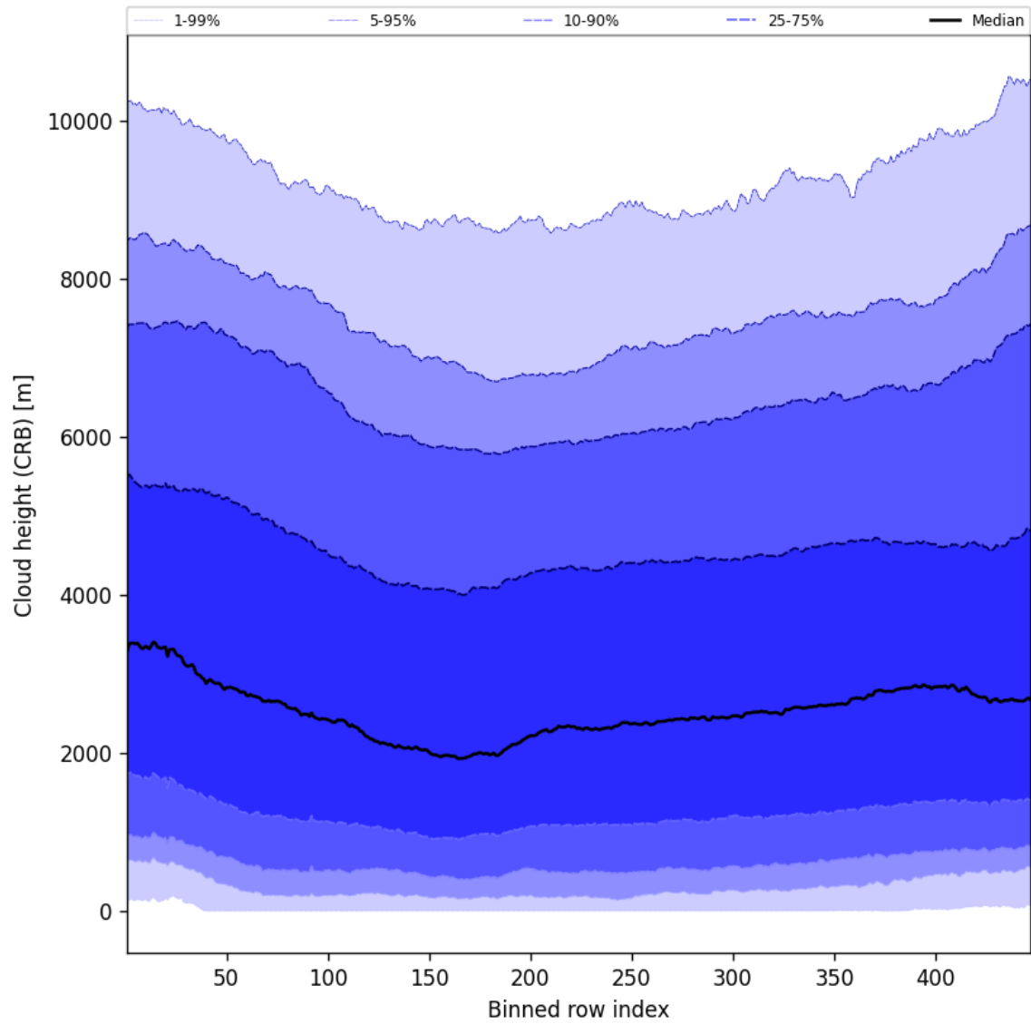
Figure 59: Along track statistics of “Cloud height (CRB)” for 2025-03-01 to 2025-03-02
