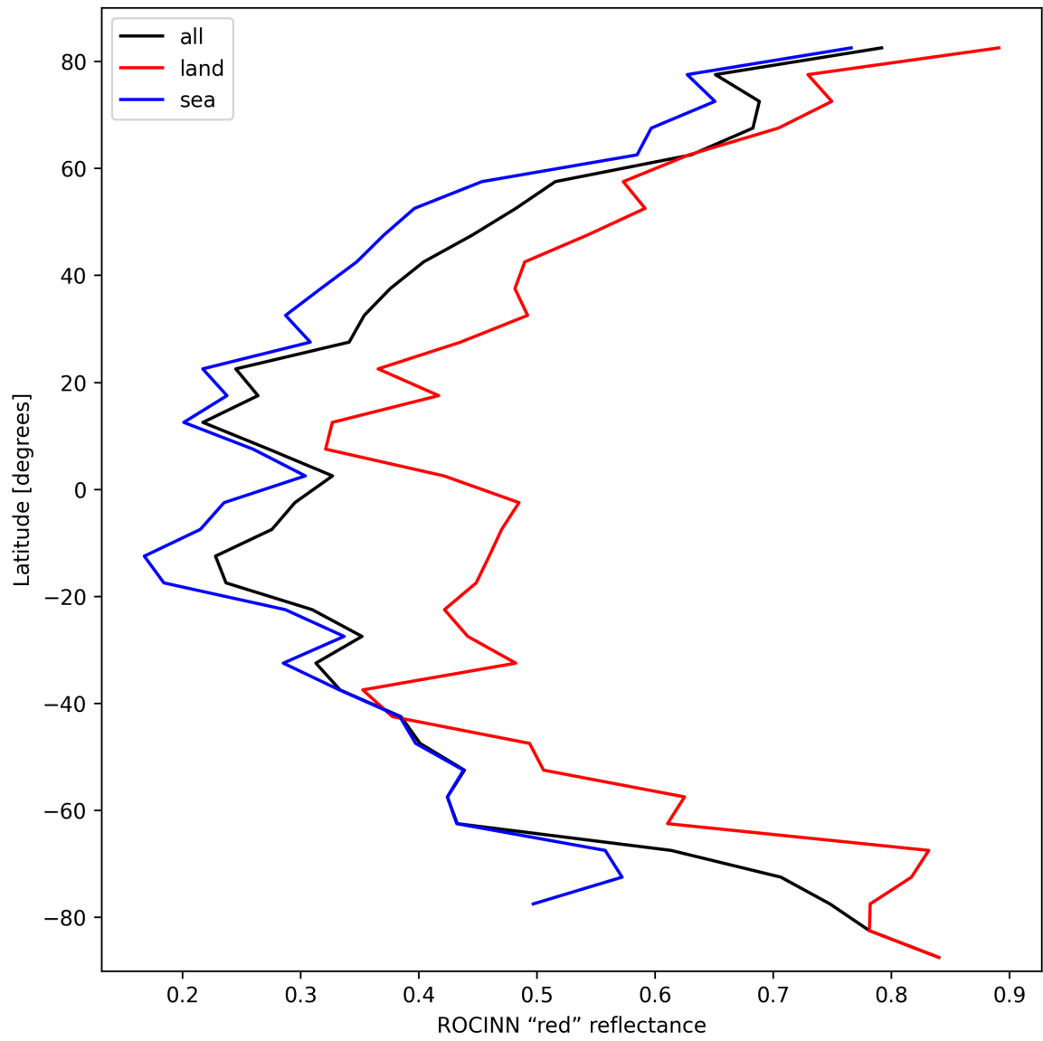
Figure 37: Zonal average of “ROCINN “red” reflectance” for 2025-03-01 to 2025-03-02.
