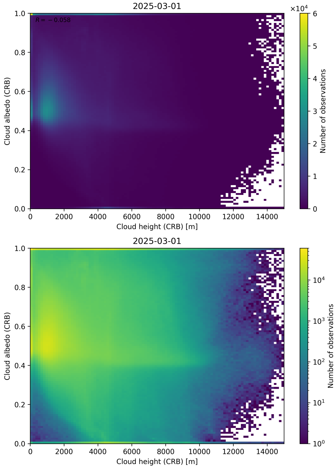
Figure 80: Scatter density plot of “Cloud height (CRB)” against “Cloud albedo (CRB)” for 2025-03-01 to 2025-03-02.
