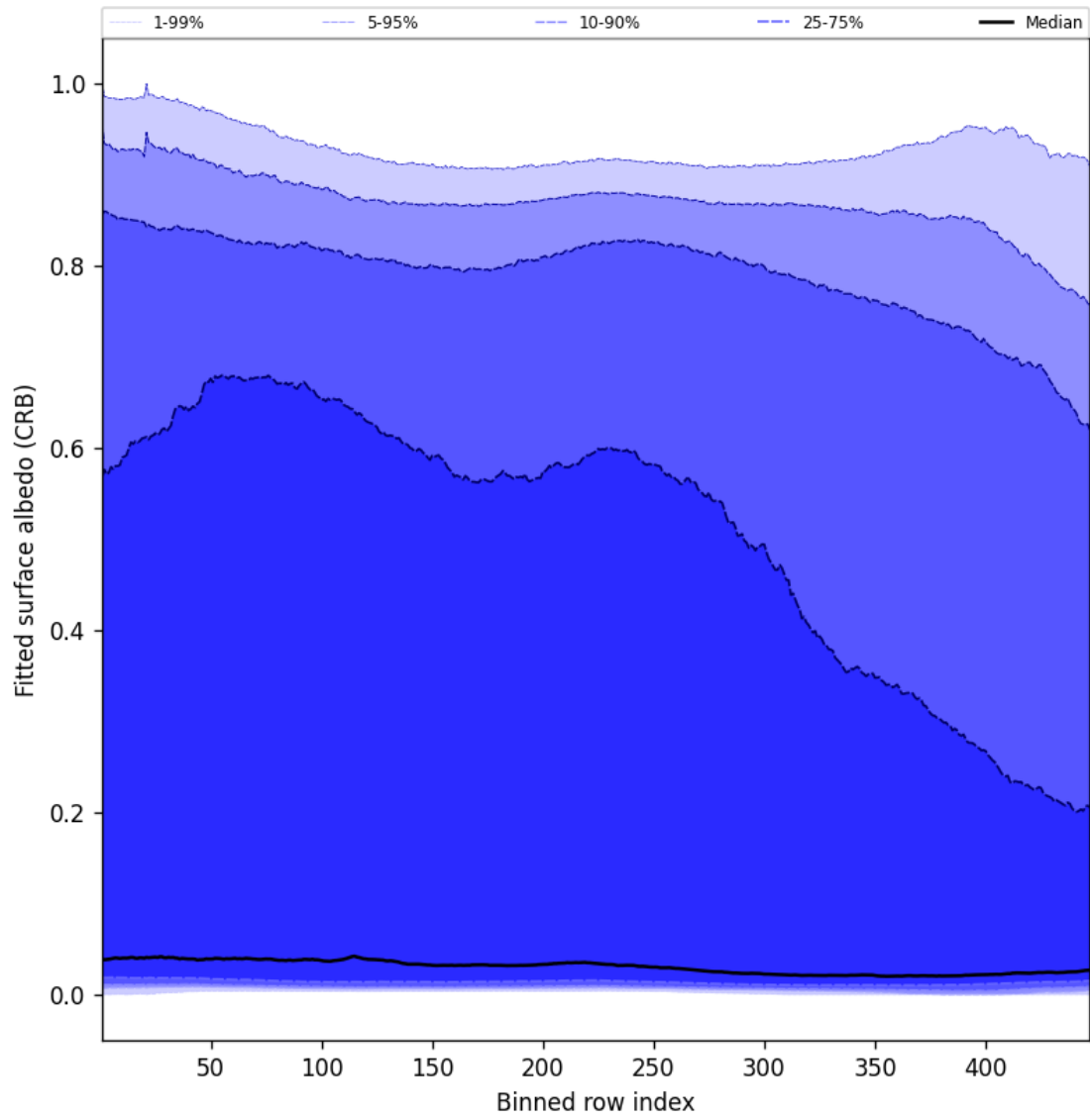
Figure 62: Along track statistics of “Fitted surface albedo (CRB)” for 2025-03-01 to 2025-03-02
