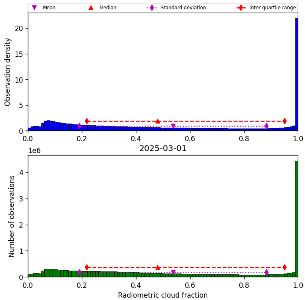
Figure 39: Histogram of “Radiometric cloud fraction” for 2025-03-01 to 2025-03-02
