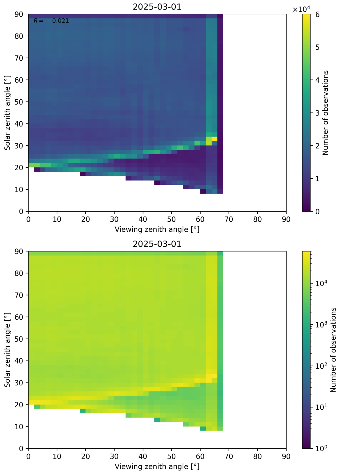
Figure 114: Scatter density plot of “Viewing zenith angle” against “Solar zenith angle” for 2025-03-01 to 2025-03-02.
