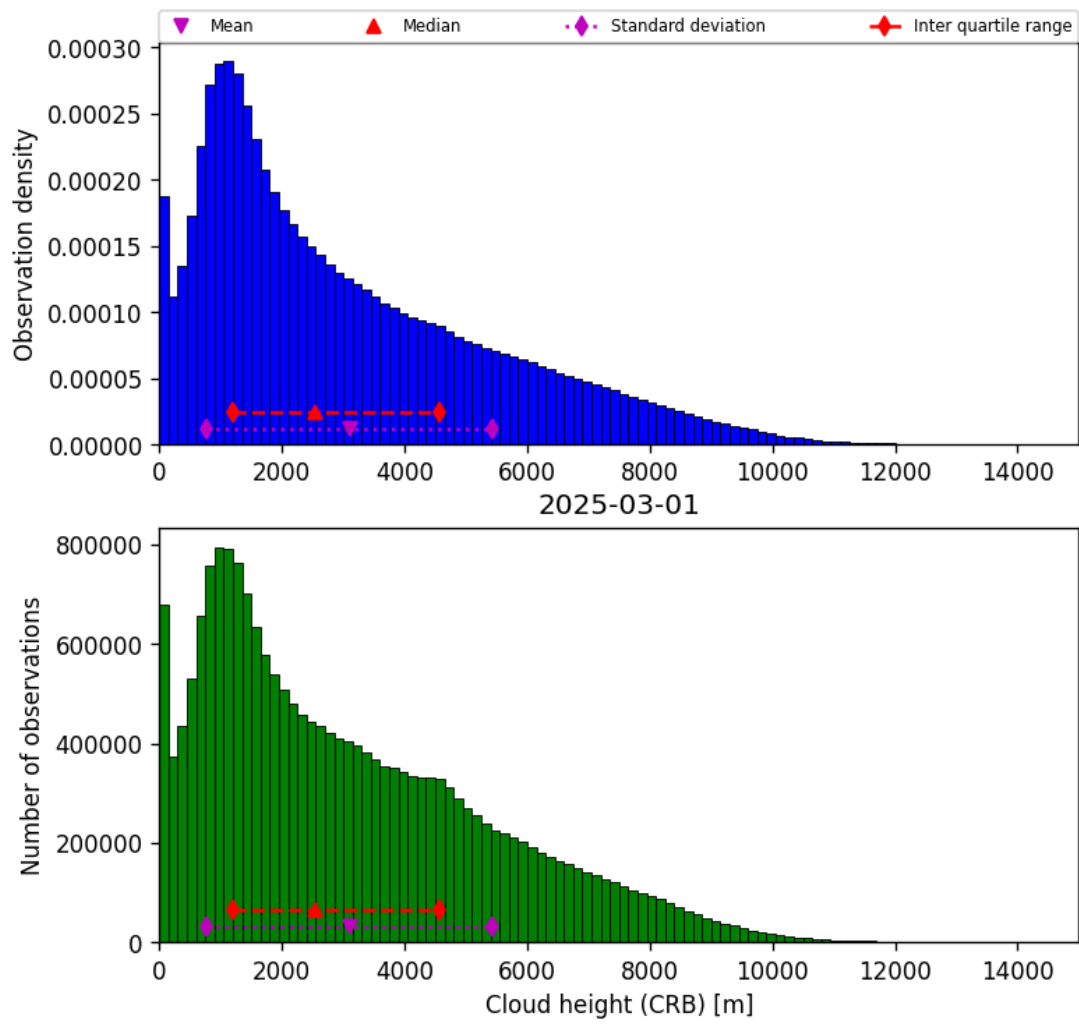
Figure 43: Histogram of “Cloud height (CRB)” for 2025-03-01 to 2025-03-02
