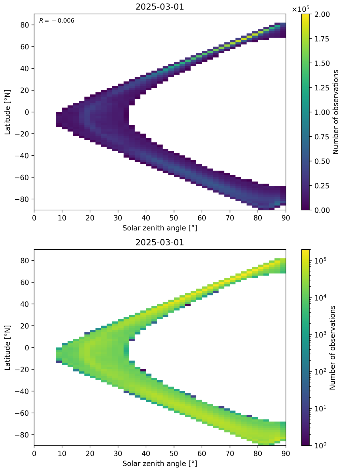
Figure 105: Scatter density plot of “Solar zenith angle” against “Latitude” for 2025-03-01 to 2025-03-02.
