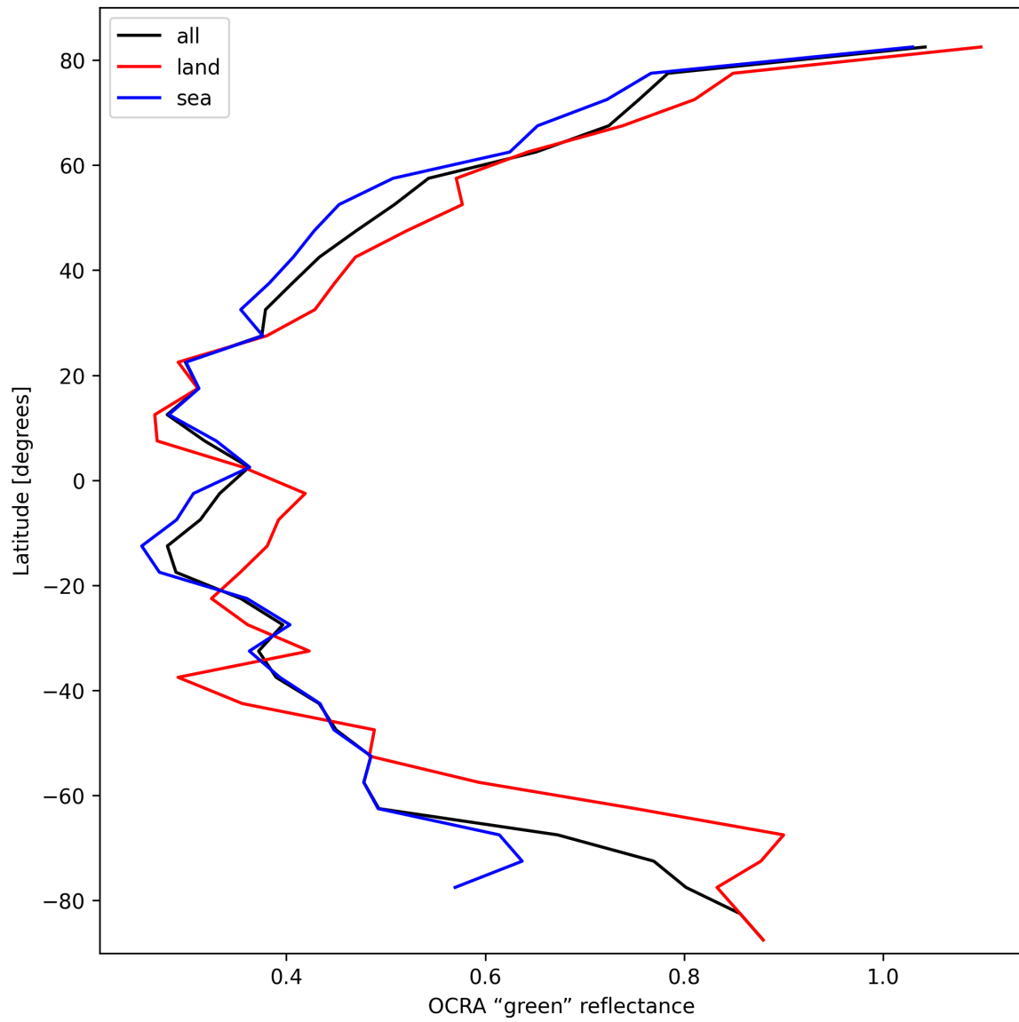
Figure 36: Zonal average of “OCRA “green” reflectance” for 2025-03-01 to 2025-03-02.
