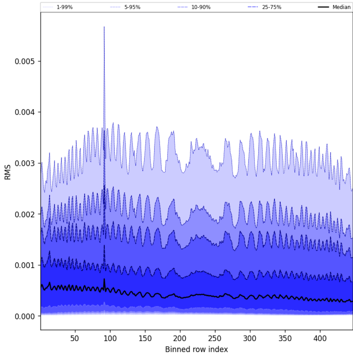
Figure 63: Along track statistics of “RMS” for 2025-03-01 to 2025-03-02
