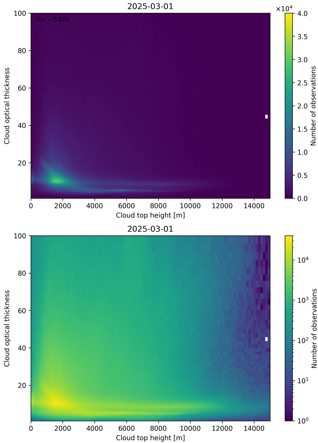
Figure 90: Scatter density plot of “Cloud top height” against “Cloud optical thickness” for 2025-03-01 to 2025-03-02.
