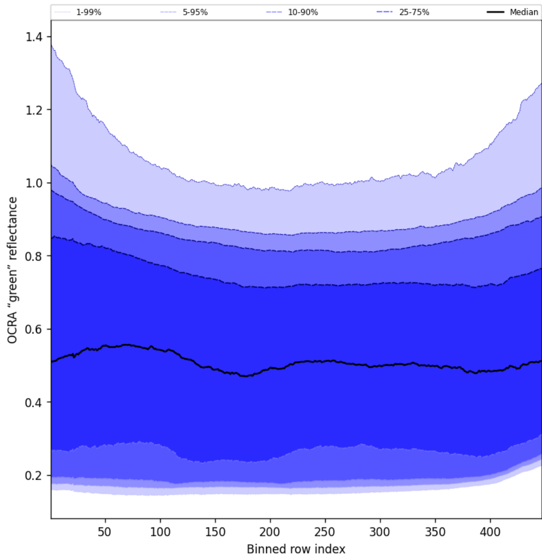
Figure 68: Along track statistics of “OCRA “green” reflectance” for 2025-03-01 to 2025-03-02
