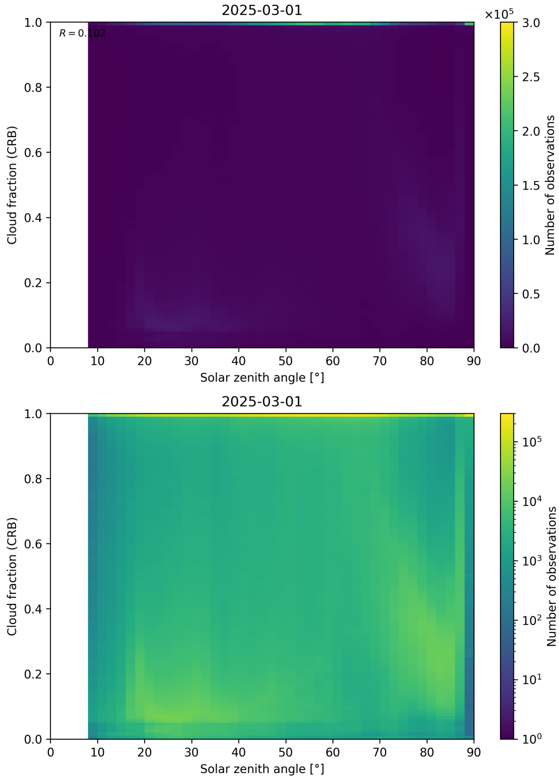
Figure 101: Scatter density plot of “Solar zenith angle” against “Cloud fraction (CRB)” for 2025-03-01 to 2025-03-02.
