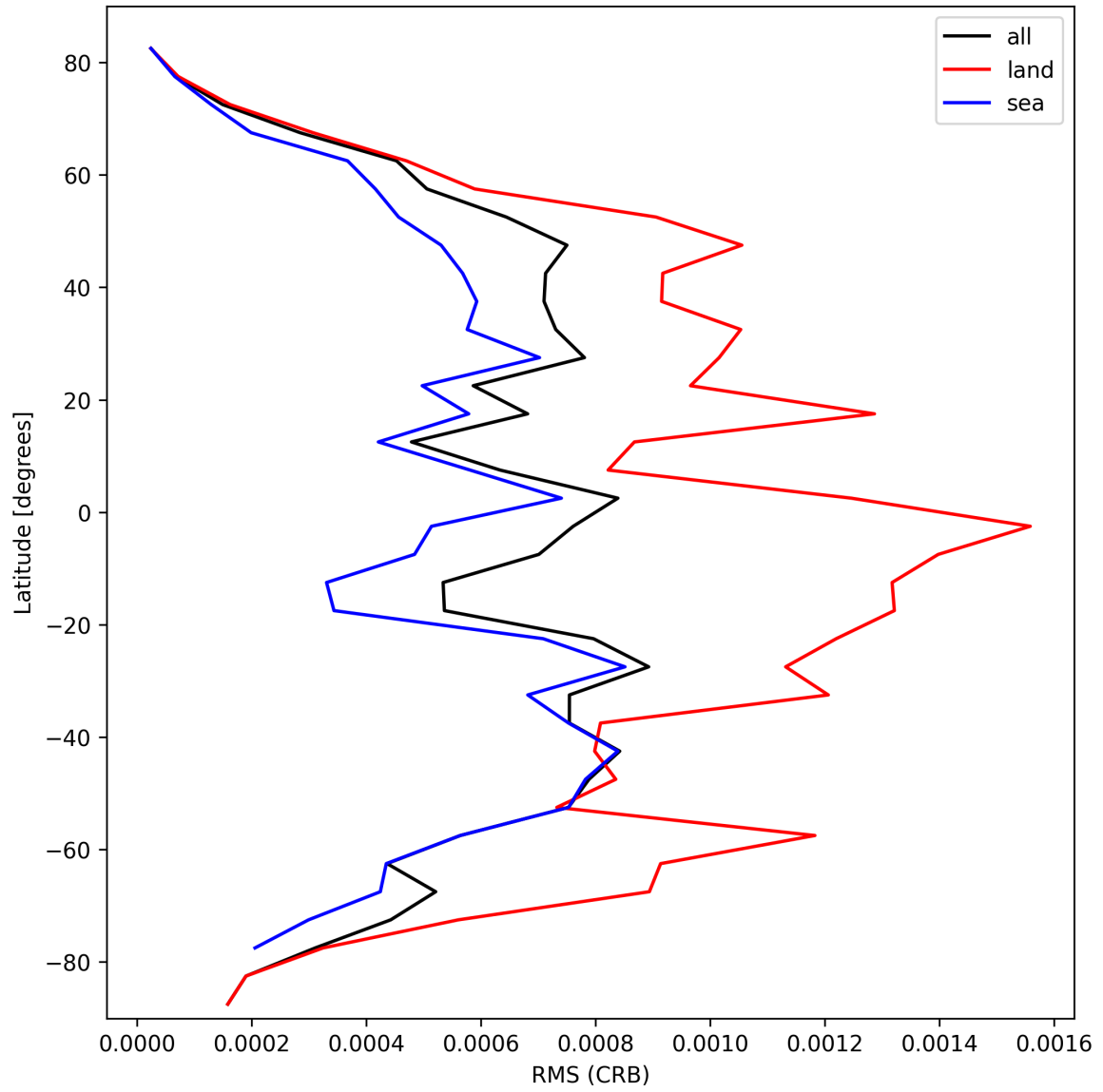
Figure 32: Zonal average of “RMS (CRB)” for 2025-03-01 to 2025-03-02.
