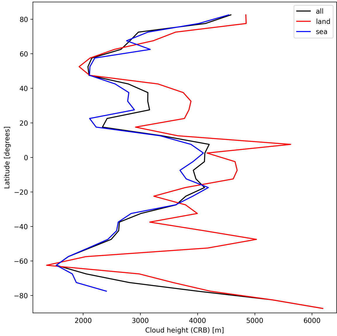
Figure 27: Zonal average of “Cloud height (CRB)” for 2025-03-01 to 2025-03-02.
