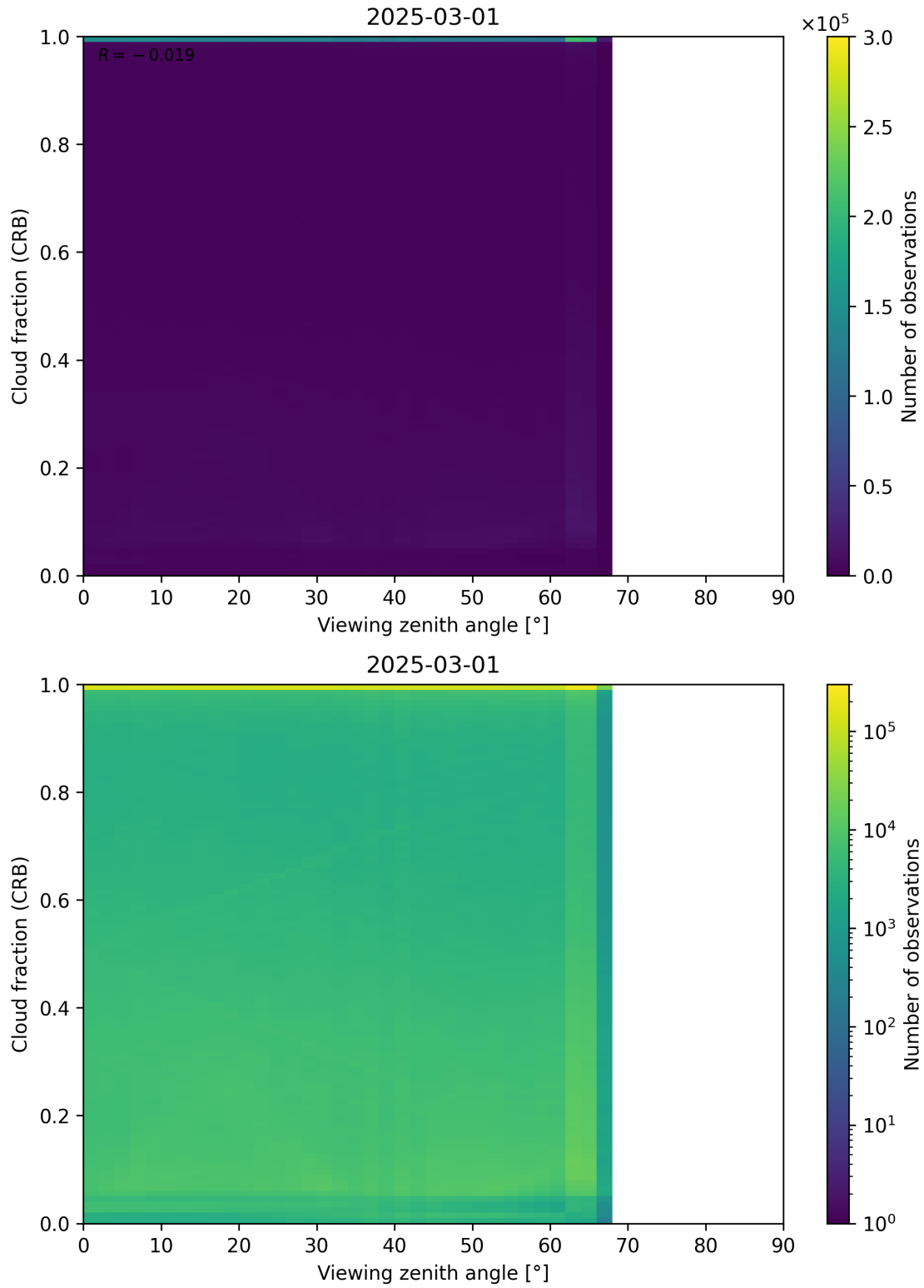
Figure 109: Scatter density plot of “Viewing zenith angle” against “Cloud fraction (CRB)” for 2025-03-01 to 2025-03-02.
