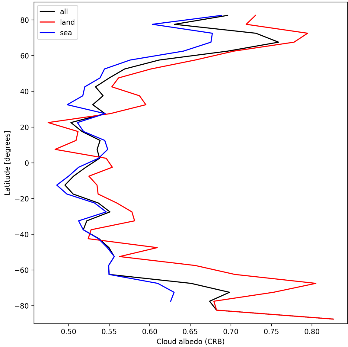
Figure 28: Zonal average of “Cloud albedo (CRB)” for 2025-03-01 to 2025-03-02.
