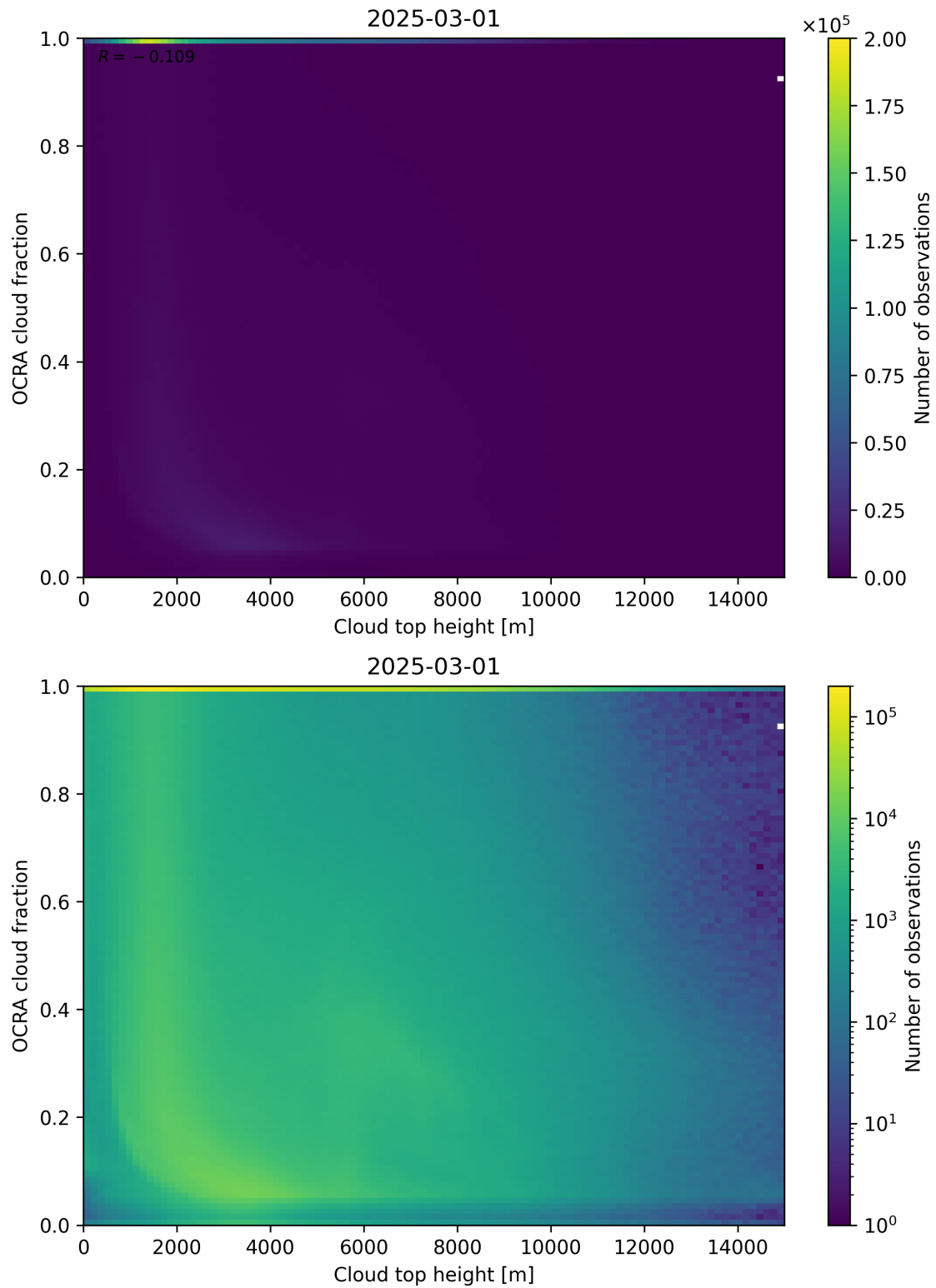
Figure 87: Scatter density plot of “Cloud top height” against “OCRA cloud fraction” for 2025-03-01 to 2025-03-02.
