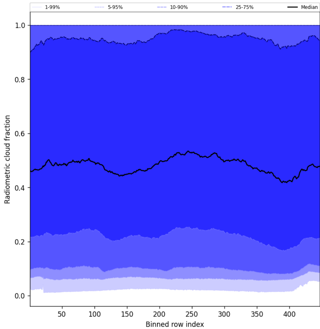
Figure 55: Along track statistics of “Radiometric cloud fraction” for 2025-03-01 to 2025-03-02
