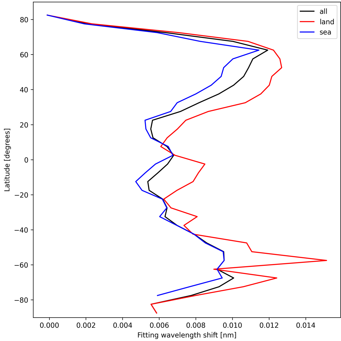
Figure 33: Zonal average of “Fitting wavelength shift” for 2025-03-01 to 2025-03-02.
