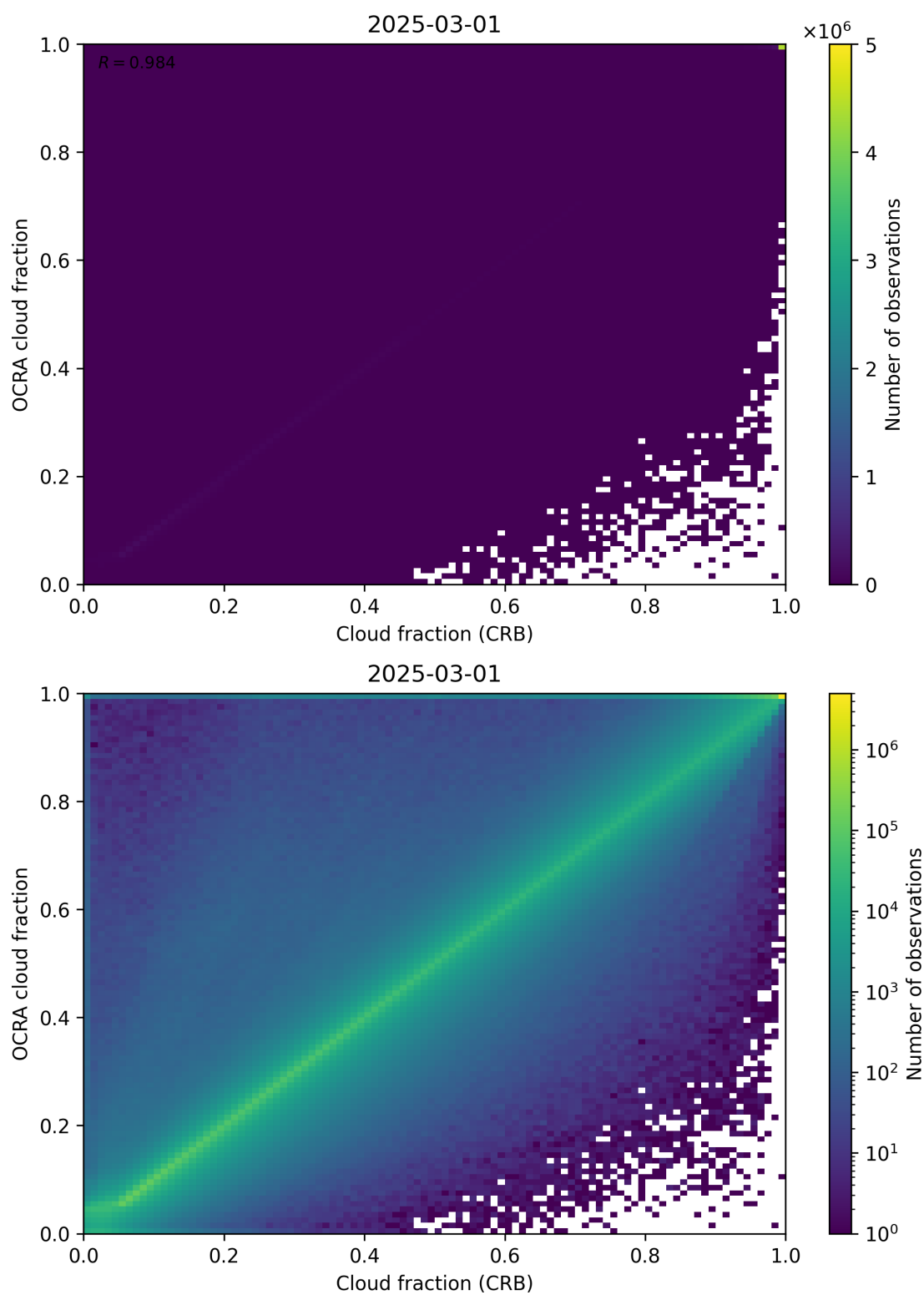
Figure 78: Scatter density plot of “Cloud fraction (CRB)” against “OCRA cloud fraction” for 2025-03-01 to 2025-03-02.
