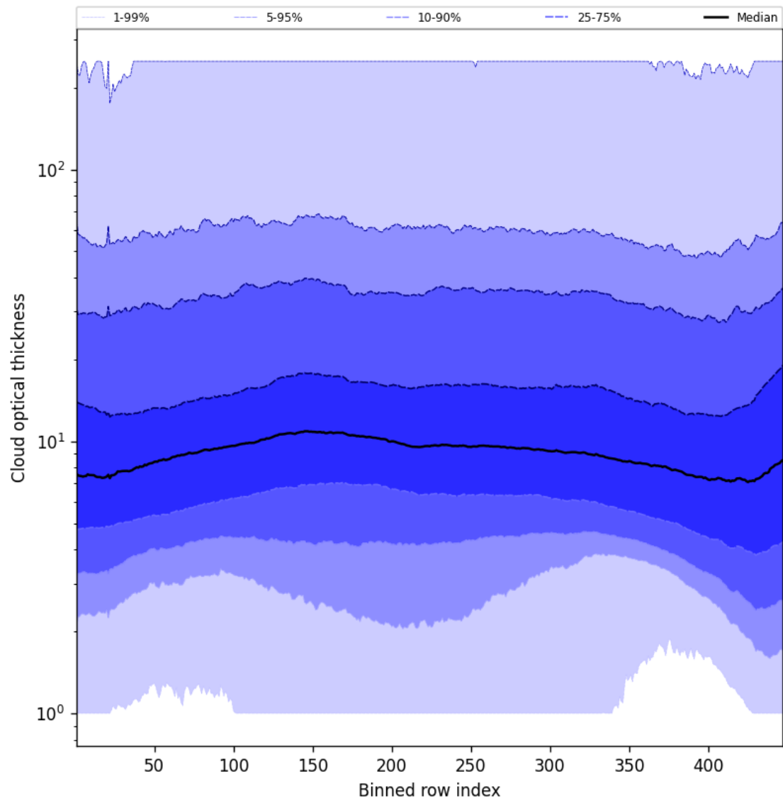
Figure 57: Along track statistics of “Cloud optical thickness” for 2025-03-01 to 2025-03-02
