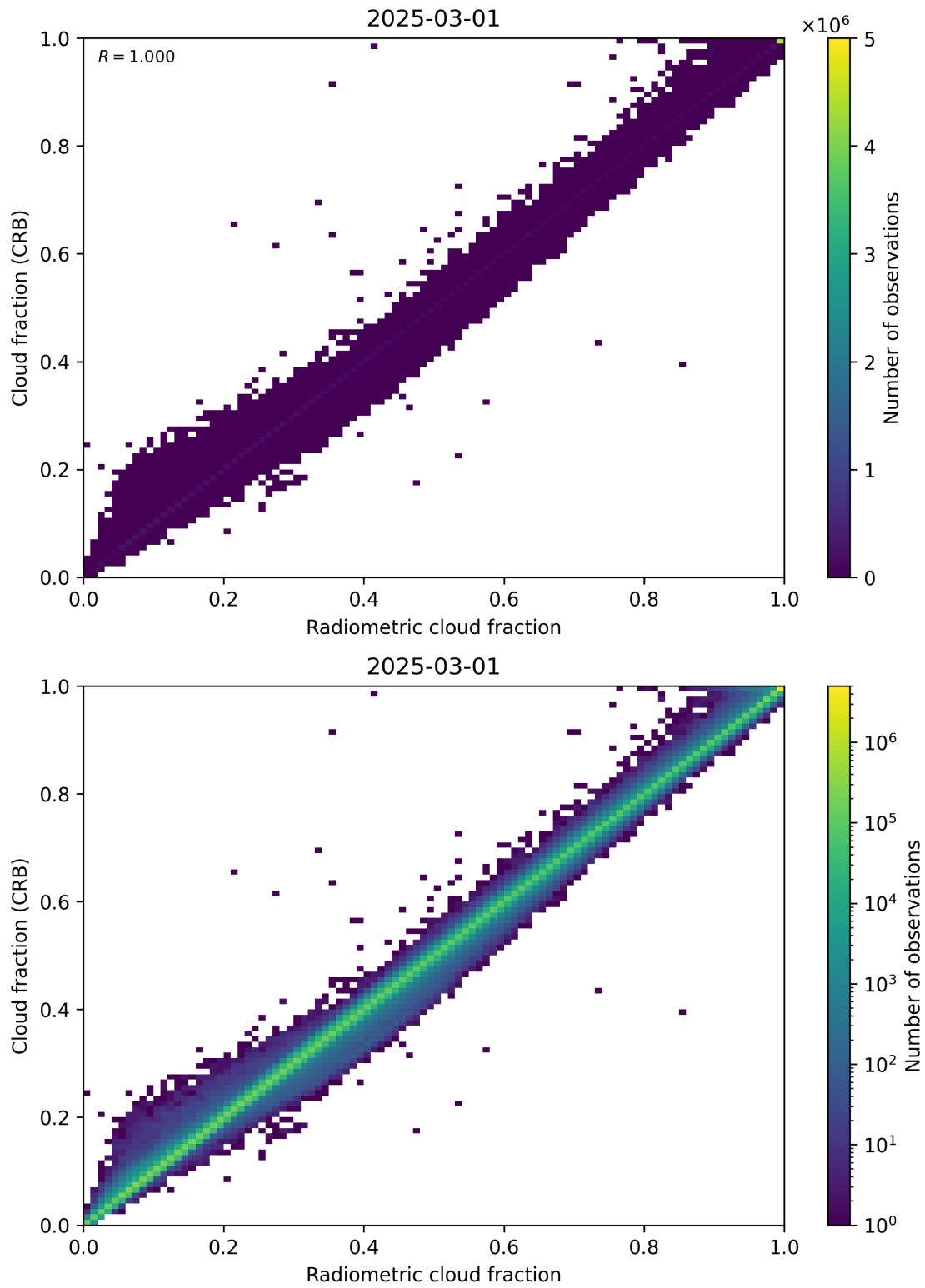
Figure 73: Scatter density plot of “Radiometric cloud fraction” against “Cloud fraction (CRB)” for 2025-03-01 to 2025-03-02.
