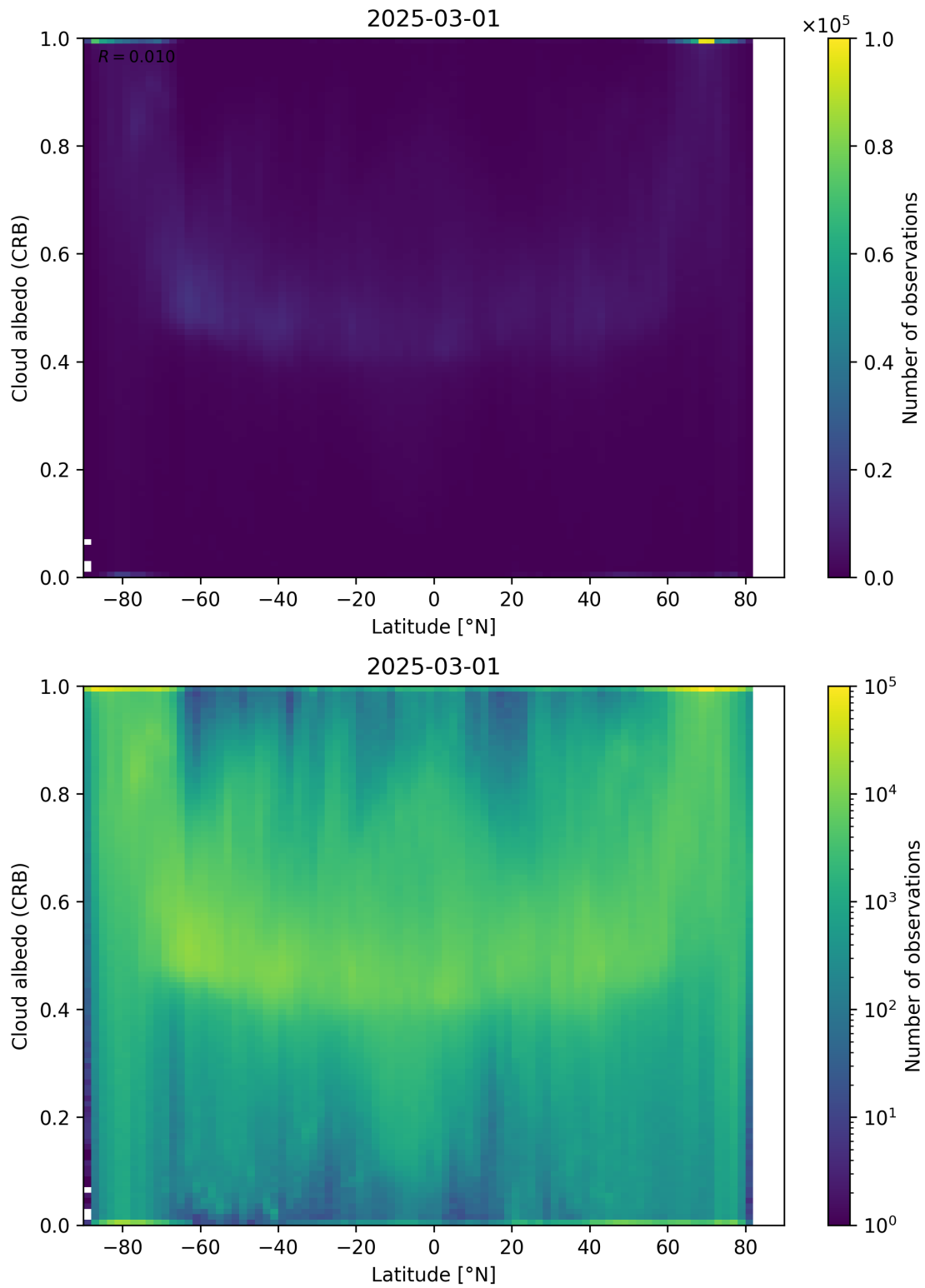
Figure 91: Scatter density plot of “Latitude” against “Cloud albedo (CRB)” for 2025-03-01 to 2025-03-02.
