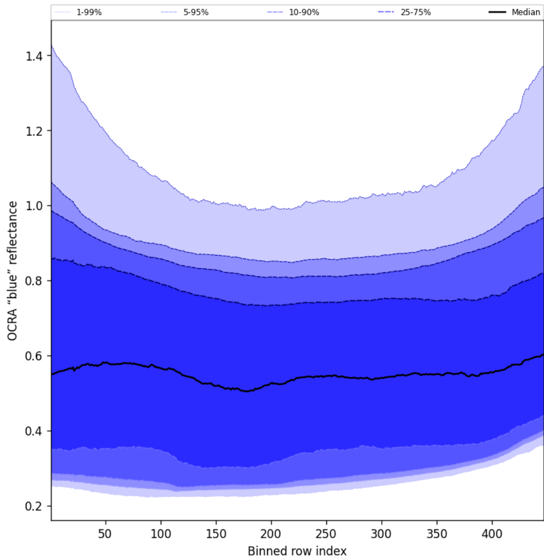
Figure 67: Along track statistics of "OCRA "blue" reflectance" for 2025-03-01 to 2025-03-02
