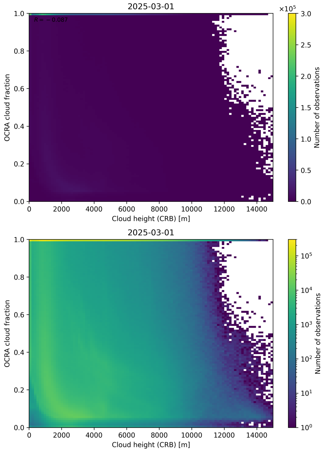
Figure 81: Scatter density plot of “Cloud height (CRB)” against “OCRA cloud fraction” for 2025-03-01 to 2025-03-02.
