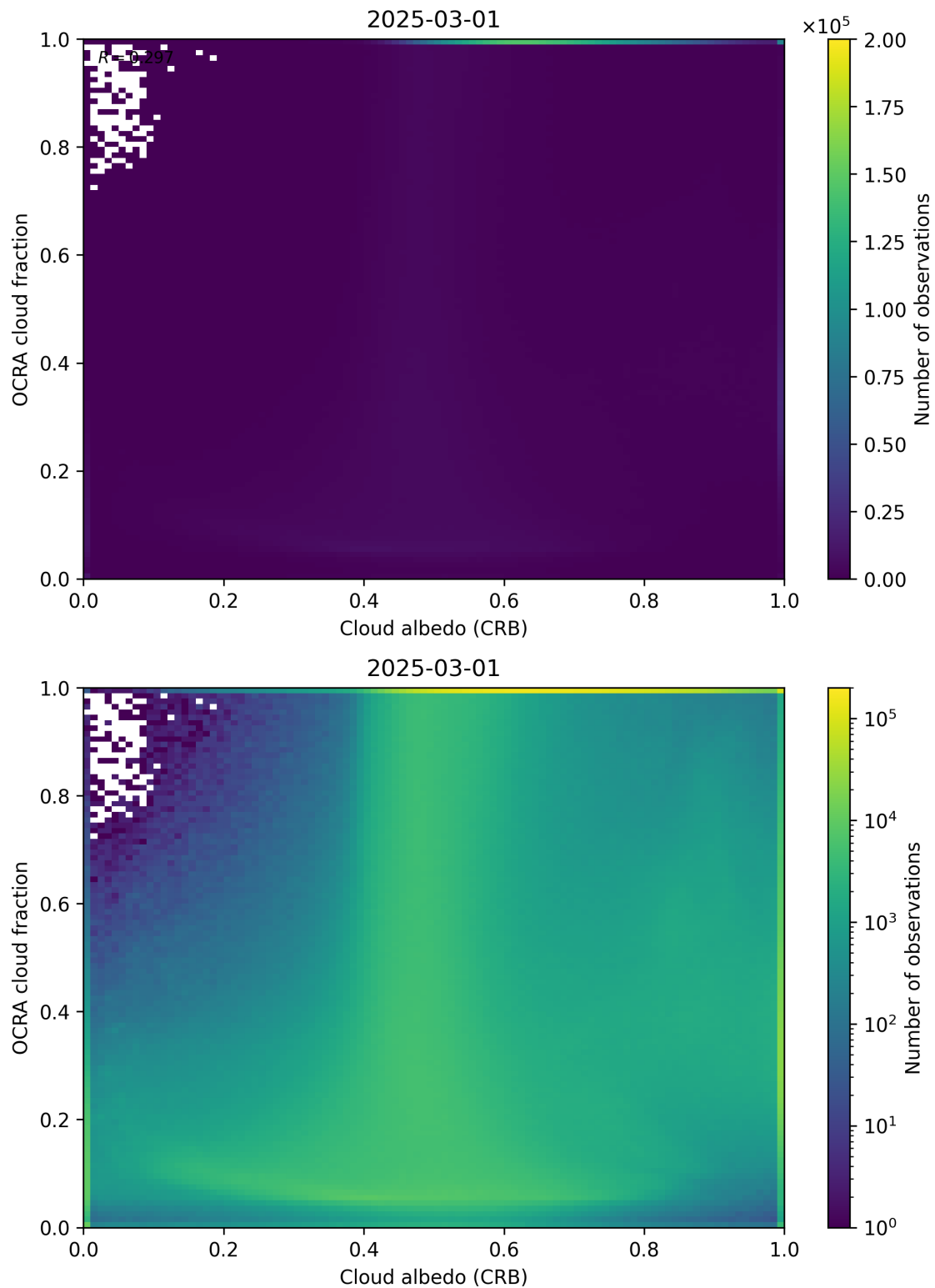
Figure 70: Scatter density plot of “Cloud albedo (CRB)” against “OCRA cloud fraction” for 2025-03-01 to 2025-03-02.
