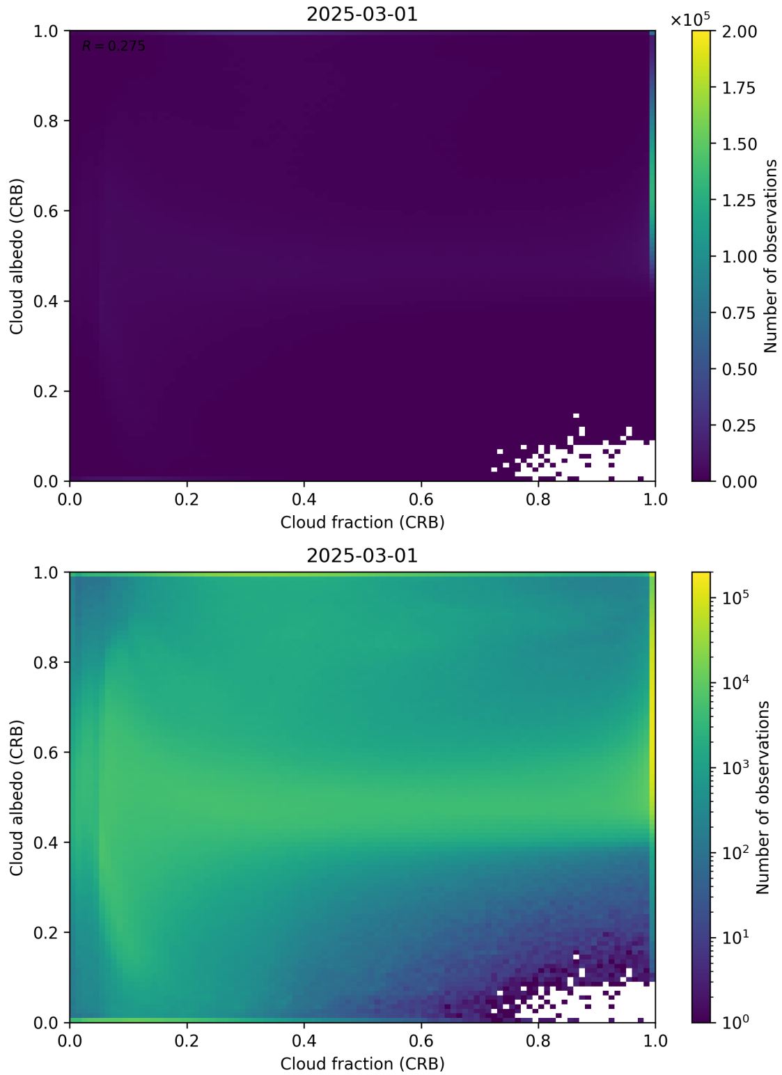
Figure 77: Scatter density plot of “Cloud fraction (CRB)” against “Cloud albedo (CRB)” for 2025-03-01 to 2025-03-02.
