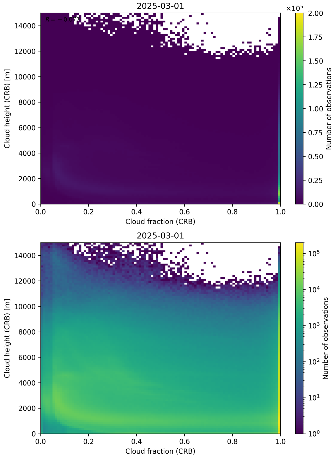
Figure 79: Scatter density plot of “Cloud fraction (CRB)” against “Cloud height (CRB)” for 2025-03-01 to 2025-03-02.
