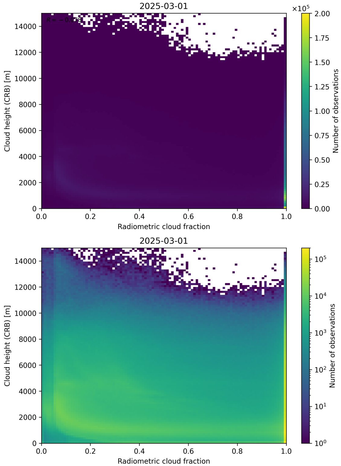
Figure 74: Scatter density plot of “Radiometric cloud fraction” against “Cloud height (CRB)” for 2025-03-01 to 2025-03-02.
