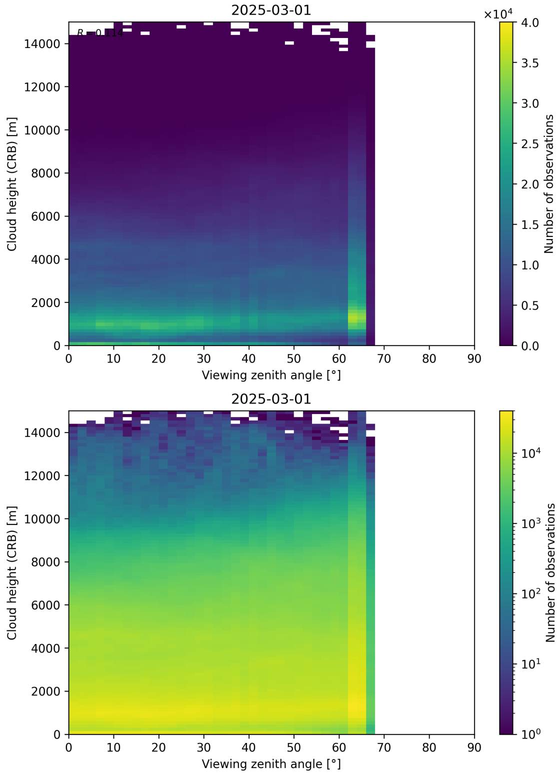
Figure 110: Scatter density plot of “Viewing zenith angle” against “Cloud height (CRB)” for 2025-03-01 to 2025-03-02.
