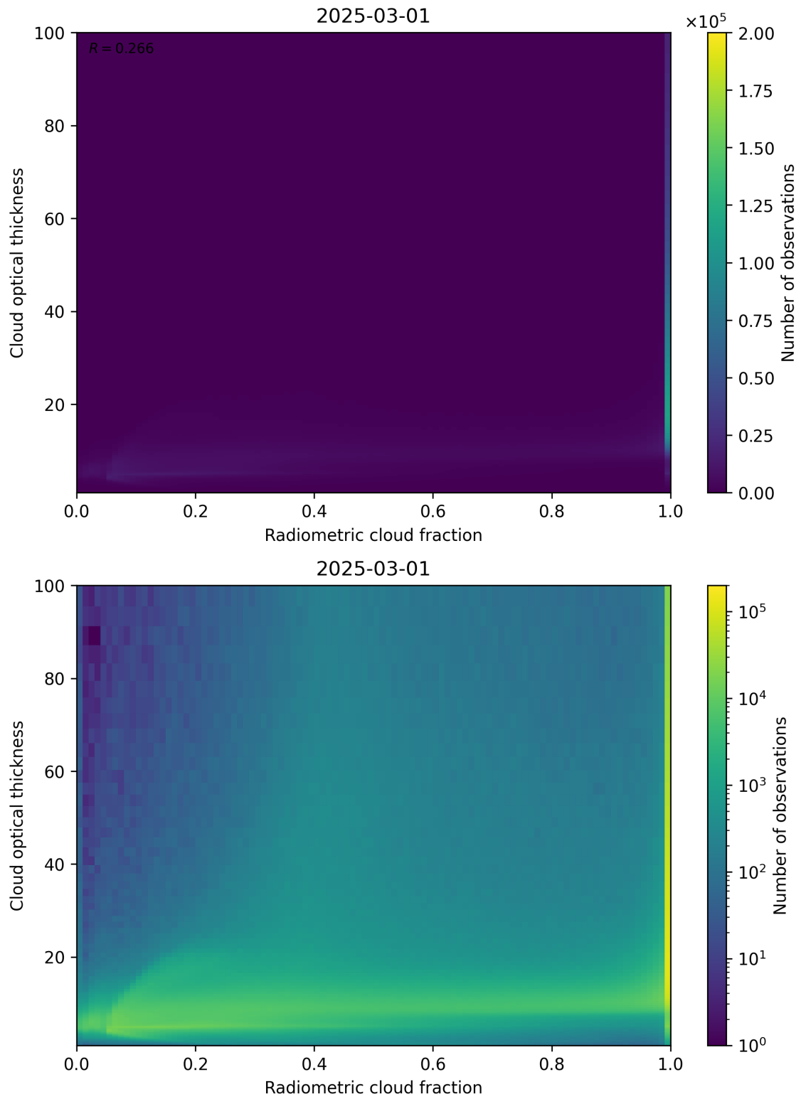
Figure 75: Scatter density plot of “Radiometric cloud fraction” against “Cloud optical thickness” for 2025-03-01 to 2025-03-02.
