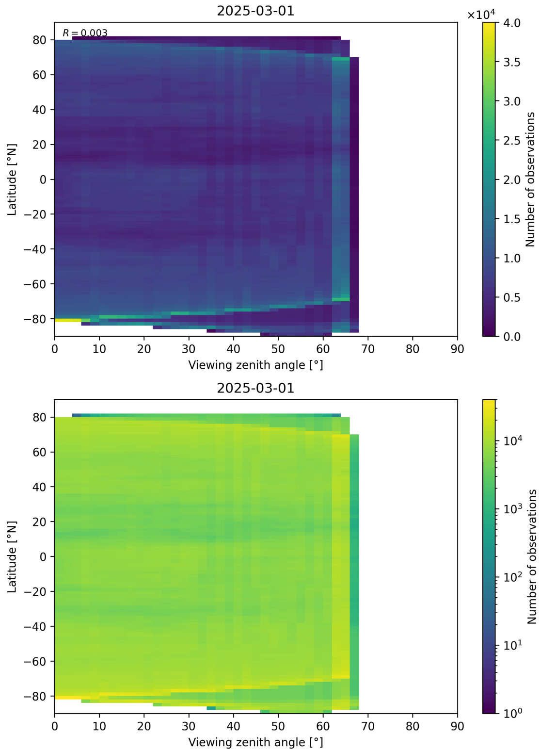
Figure 113: Scatter density plot of “Viewing zenith angle” against “Latitude” for 2025-03-01 to 2025-03-02.
