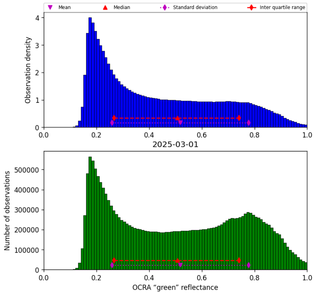
Figure 52: Histogram of “OCRA “green” reflectance” for 2025-03-01 to 2025-03-02
