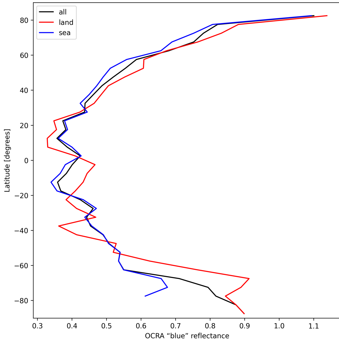
Figure 35: Zonal average of “OCRA “blue” reflectance” for 2025-03-01 to 2025-03-02.
