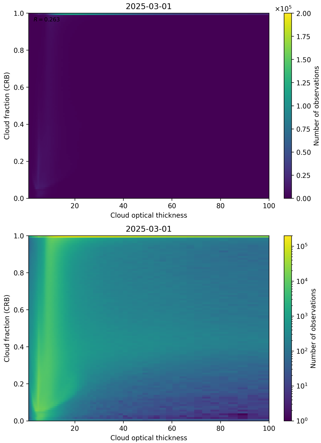
Figure 84: Scatter density plot of “Cloud optical thickness” against “Cloud fraction (CRB)” for 2025-03-01 to 2025-03-02.
