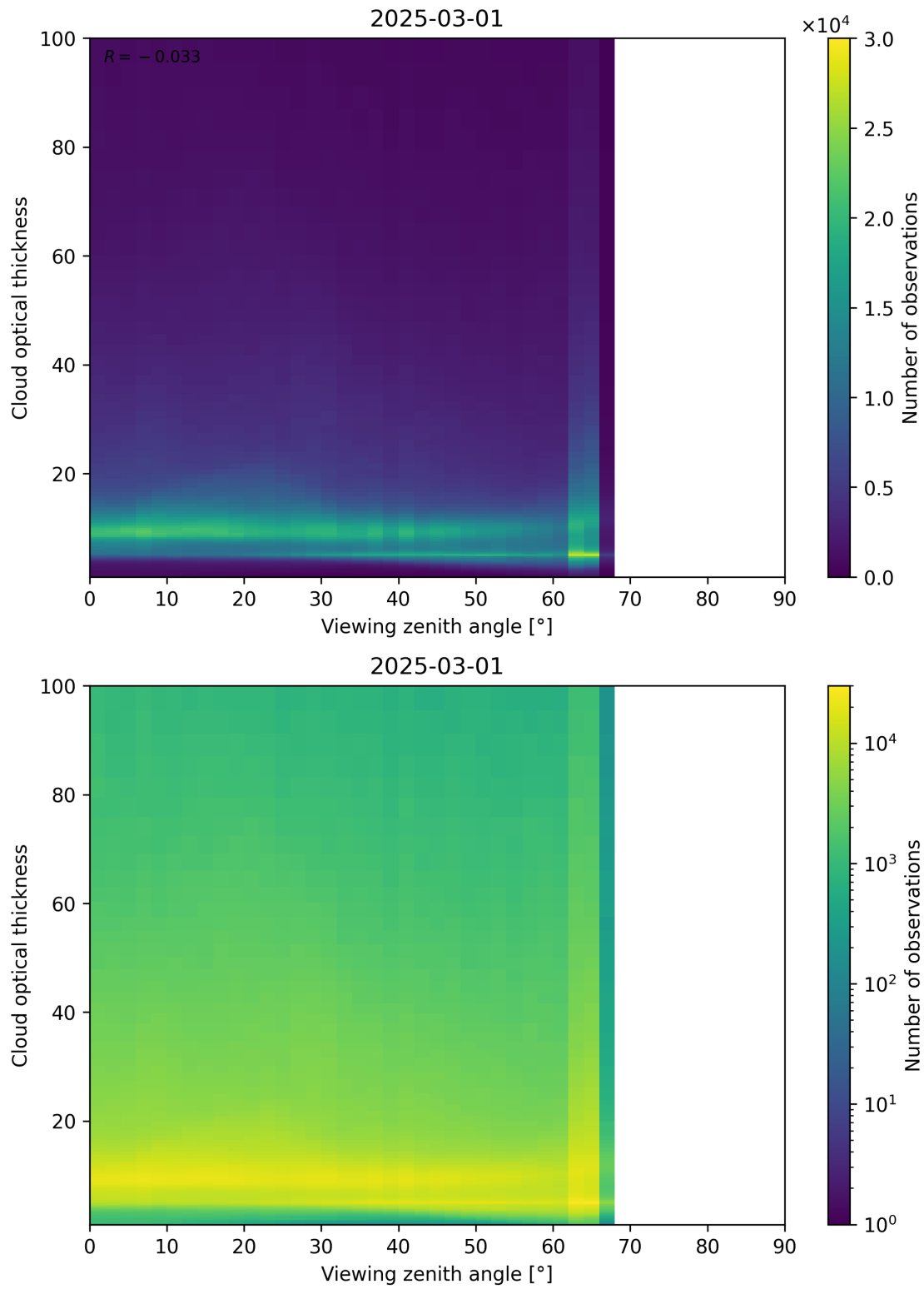
Figure 111: Scatter density plot of “Viewing zenith angle” against “Cloud optical thickness” for 2025-03-01 to 2025-03-02.
