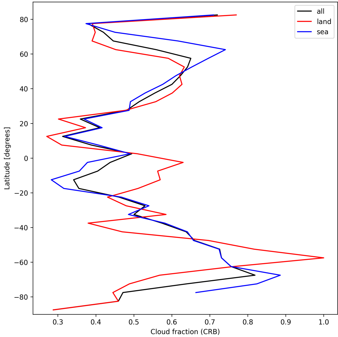
Figure 26: Zonal average of “Cloud fraction (CRB)” for 2025-03-01 to 2025-03-02.
