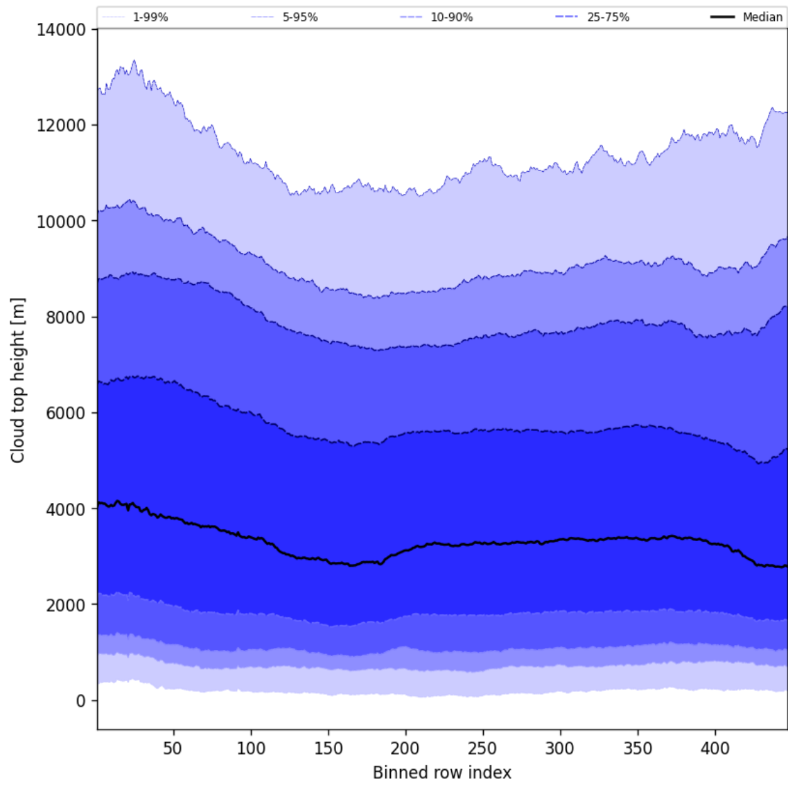
Figure 56: Along track statistics of “Cloud top height” for 2025-03-01 to 2025-03-02
