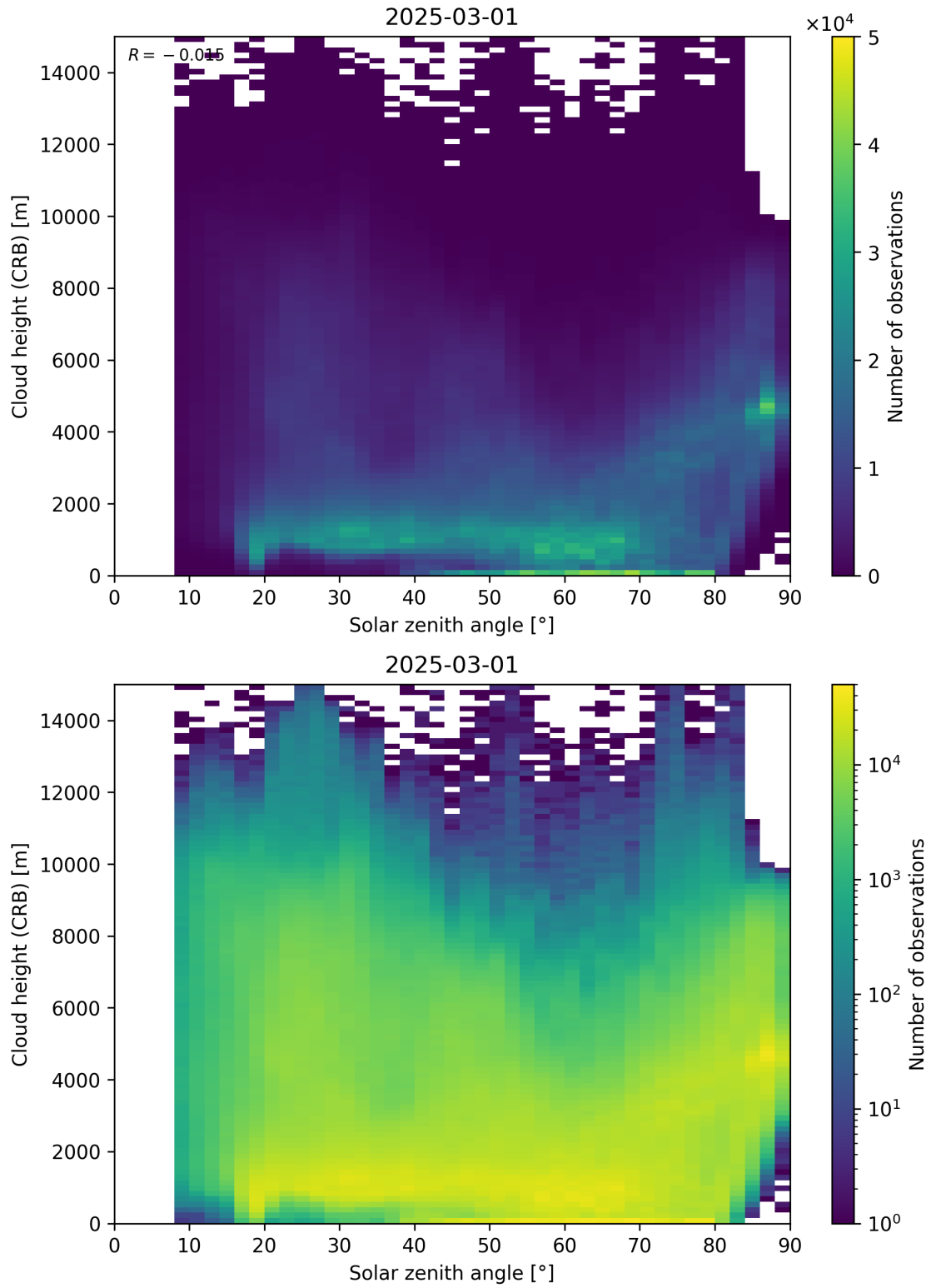
Figure 102: Scatter density plot of “Solar zenith angle” against “Cloud height (CRB)” for 2025-03-01 to 2025-03-02.
