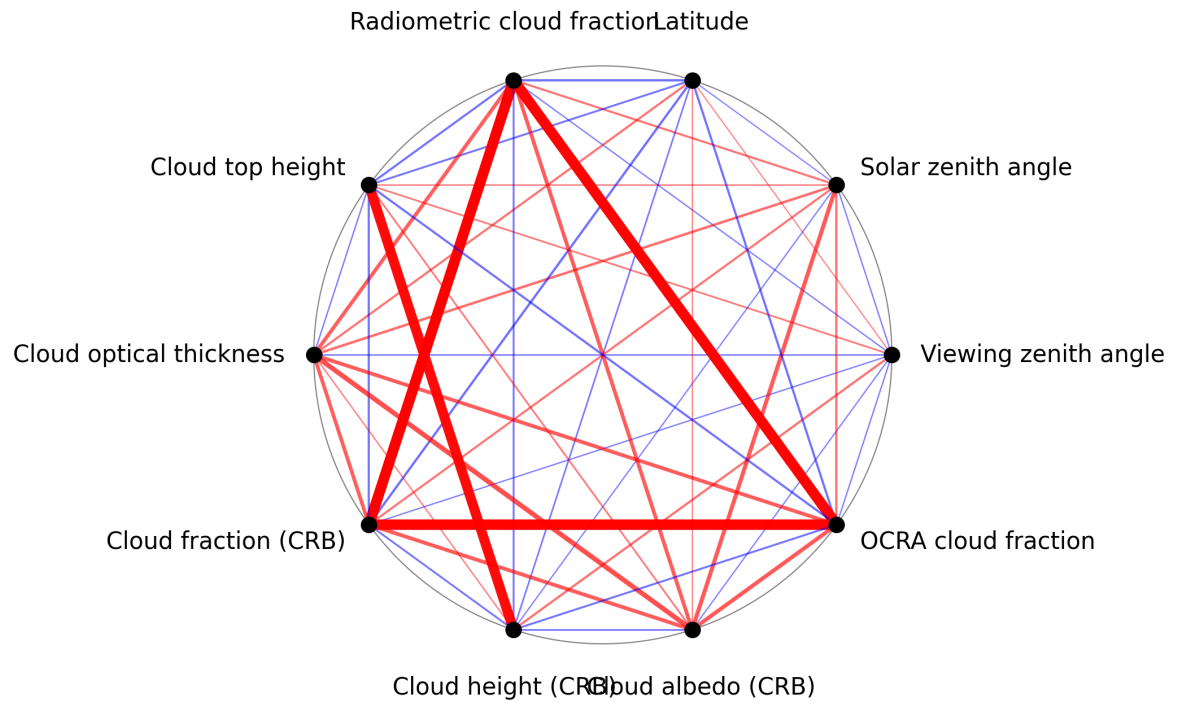
Figure 1: Map of correlation graph for 2025-03-01 to 2025-03-02.
