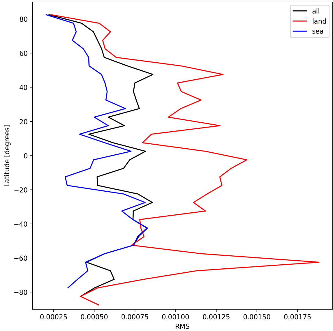
Figure 31: Zonal average of “RMS” for 2025-03-01 to 2025-03-02.
