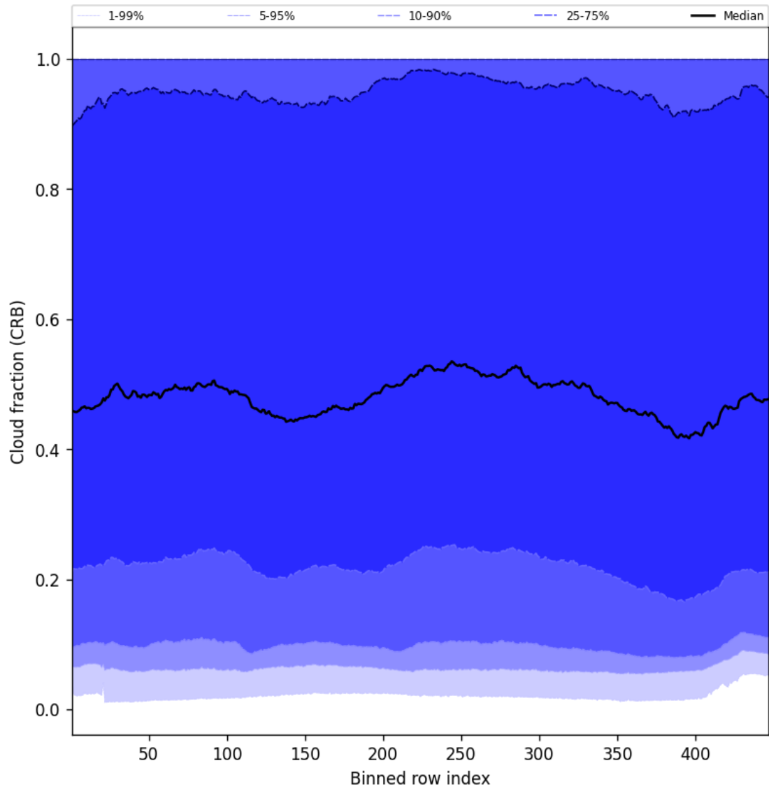
Figure 58: Along track statistics of “Cloud fraction (CRB)” for 2025-03-01 to 2025-03-02
