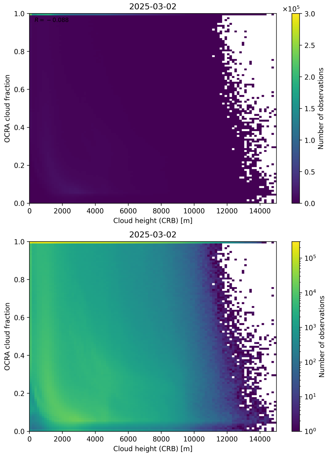
Figure 81: Scatter density plot of “Cloud height (CRB)” against “OCRA cloud fraction” for 2025-03-01 to 2025-03-03.
