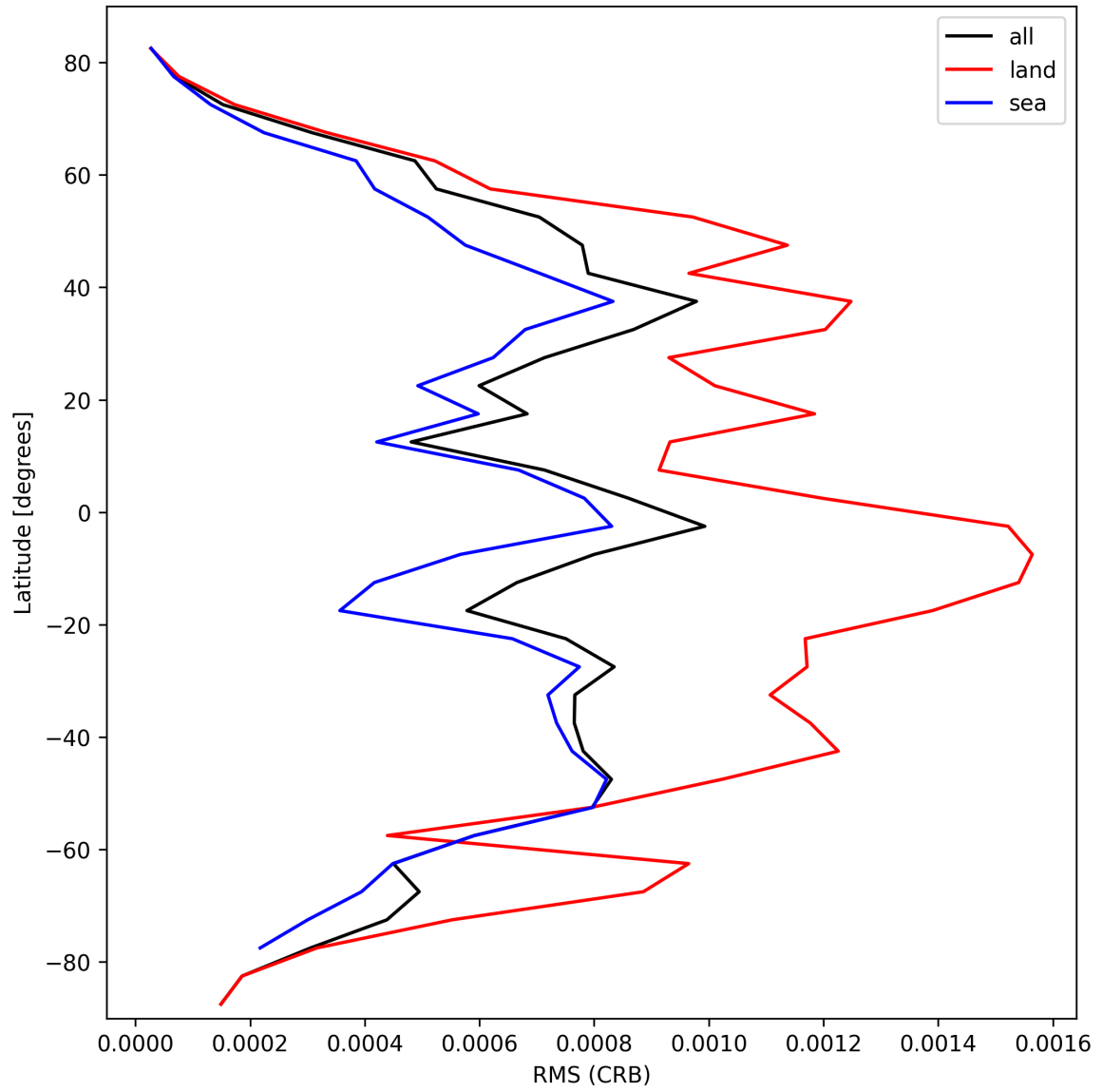
Figure 32: Zonal average of “RMS (CRB)” for 2025-03-01 to 2025-03-03.
