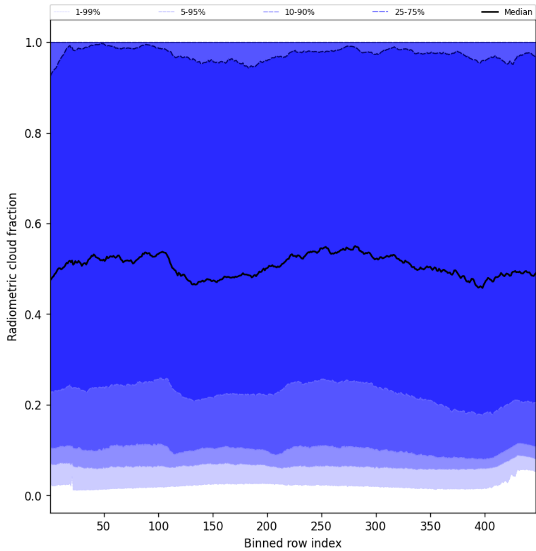
Figure 55: Along track statistics of “Radiometric cloud fraction” for 2025-03-01 to 2025-03-03
