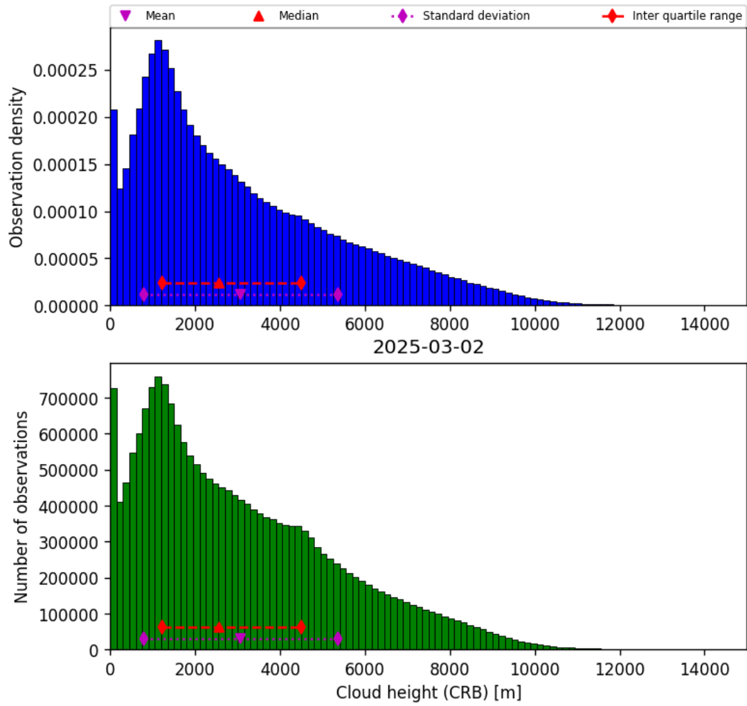
Figure 43: Histogram of “Cloud height (CRB)” for 2025-03-01 to 2025-03-03
