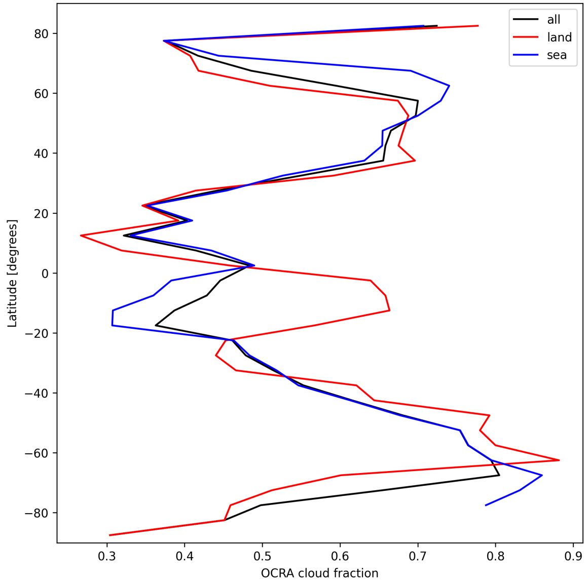
Figure 34: Zonal average of “OCRA cloud fraction” for 2025-03-01 to 2025-03-03.
