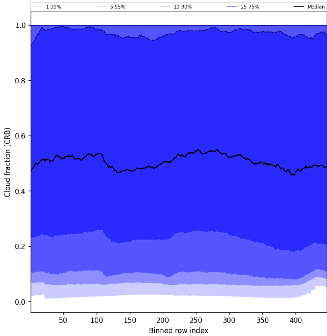
Figure 58: Along track statistics of “Cloud fraction (CRB)” for 2025-03-01 to 2025-03-03
