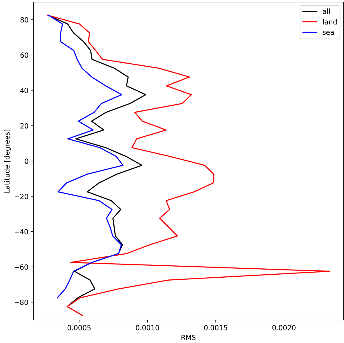
Figure 31: Zonal average of “RMS” for 2025-03-01 to 2025-03-03.
