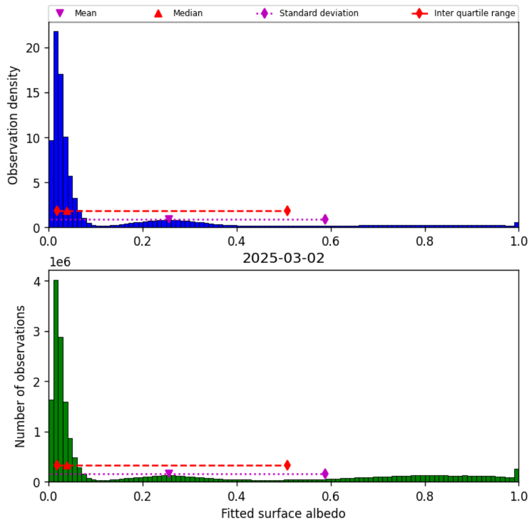
Figure 45: Histogram of “Fitted surface albedo” for 2025-03-01 to 2025-03-03
