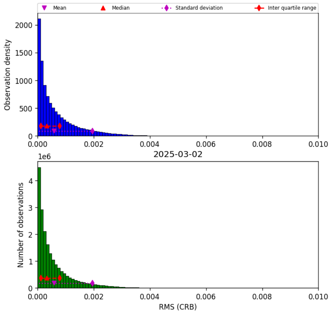
Figure 48: Histogram of “RMS (CRB)” for 2025-03-01 to 2025-03-03
