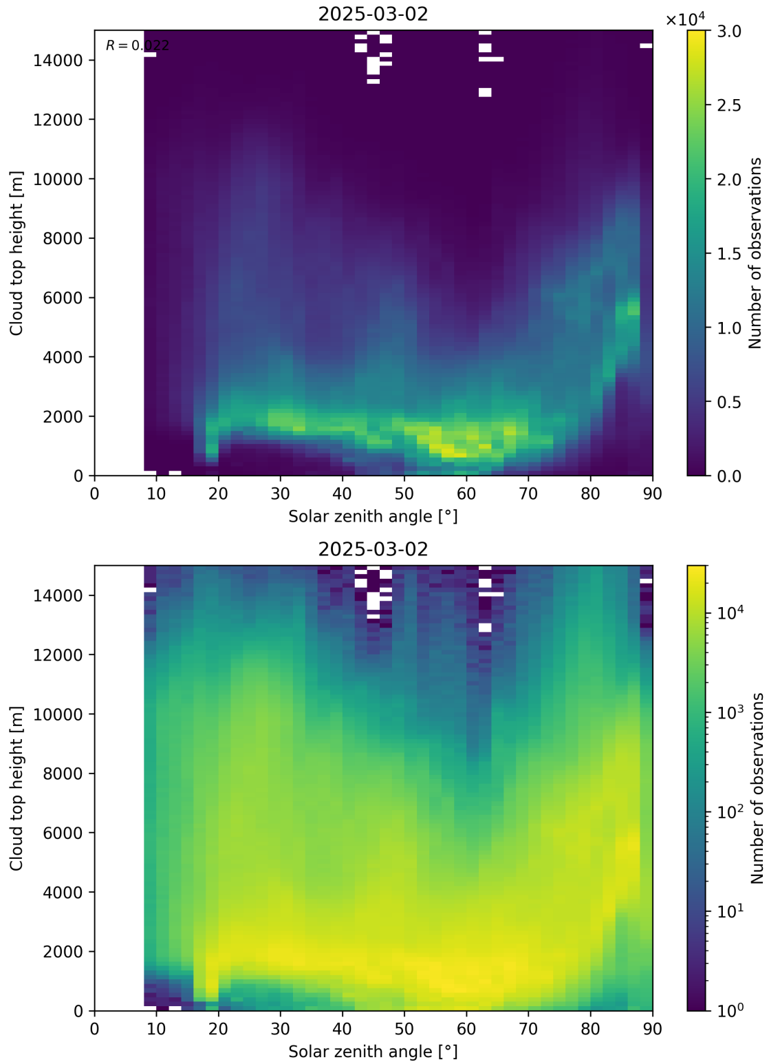
Figure 104: Scatter density plot of “Solar zenith angle” against “Cloud top height” for 2025-03-01 to 2025-03-03.
