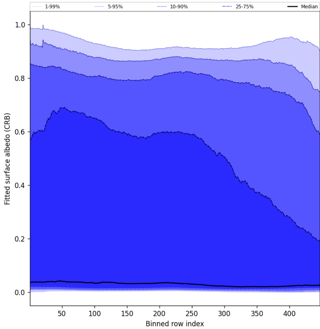
Figure 62: Along track statistics of “Fitted surface albedo (CRB)” for 2025-03-01 to 2025-03-03
