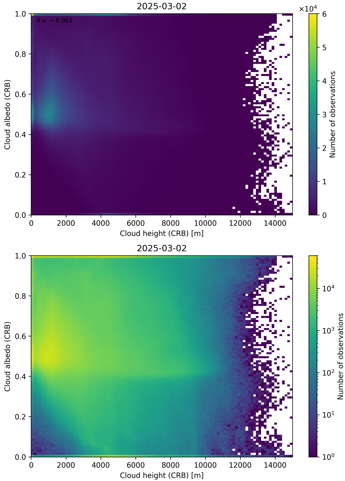
Figure 80: Scatter density plot of “Cloud height (CRB)” against “Cloud albedo (CRB)” for 2025-03-01 to 2025-03-03.
