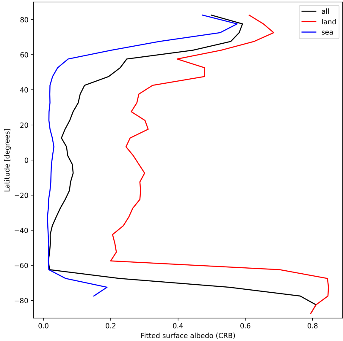
Figure 30: Zonal average of “Fitted surface albedo (CRB)” for 2025-03-01 to 2025-03-03.
