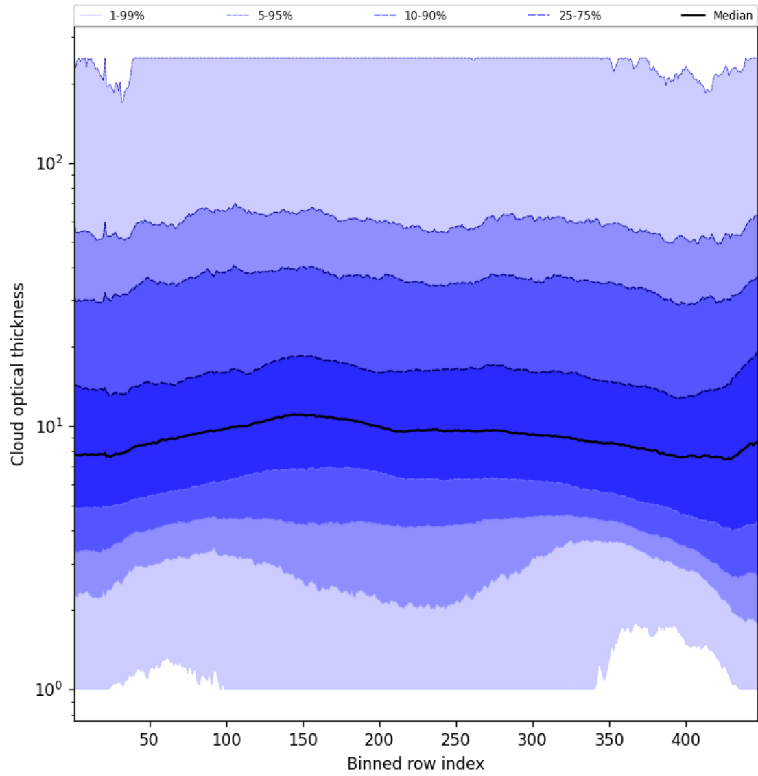
Figure 57: Along track statistics of “Cloud optical thickness” for 2025-03-01 to 2025-03-03
