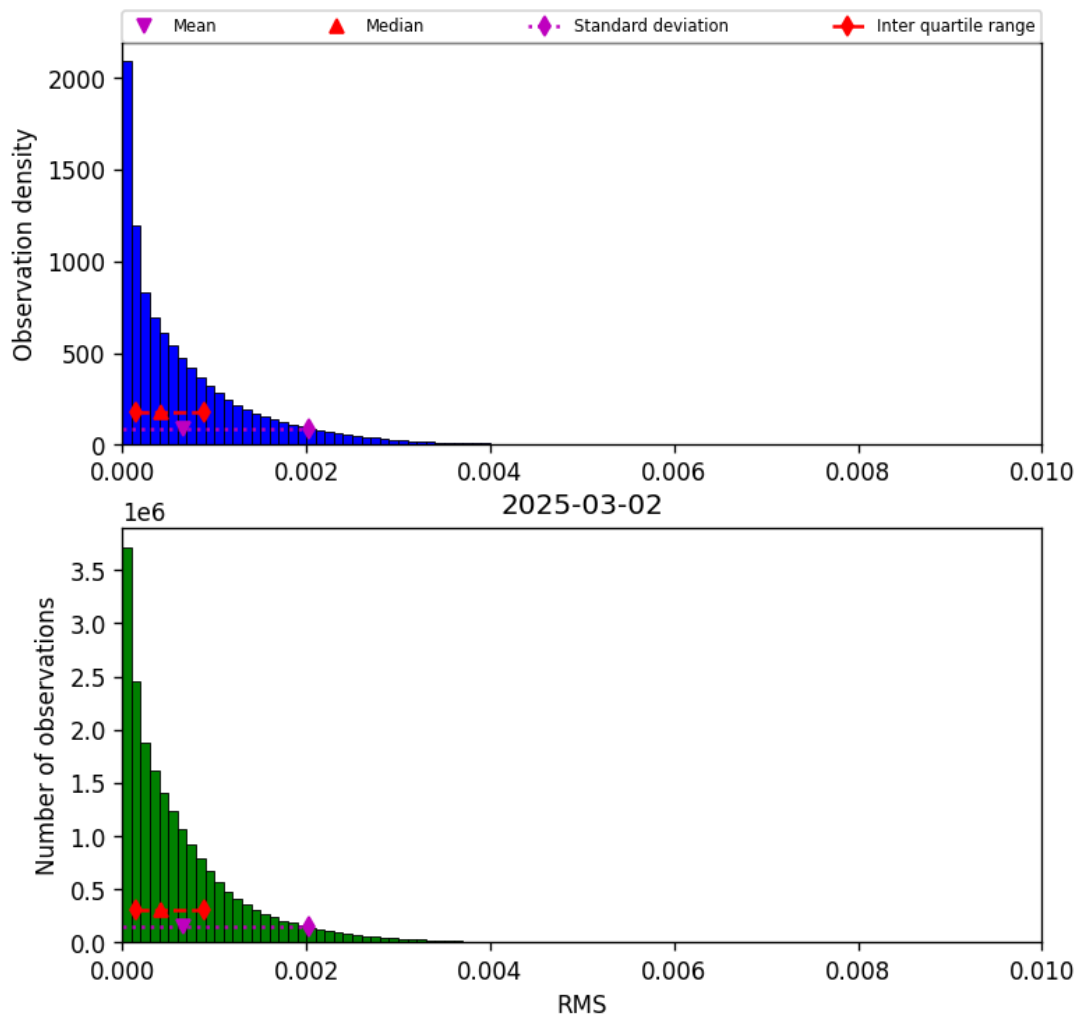
Figure 47: Histogram of “RMS” for 2025-03-01 to 2025-03-03
