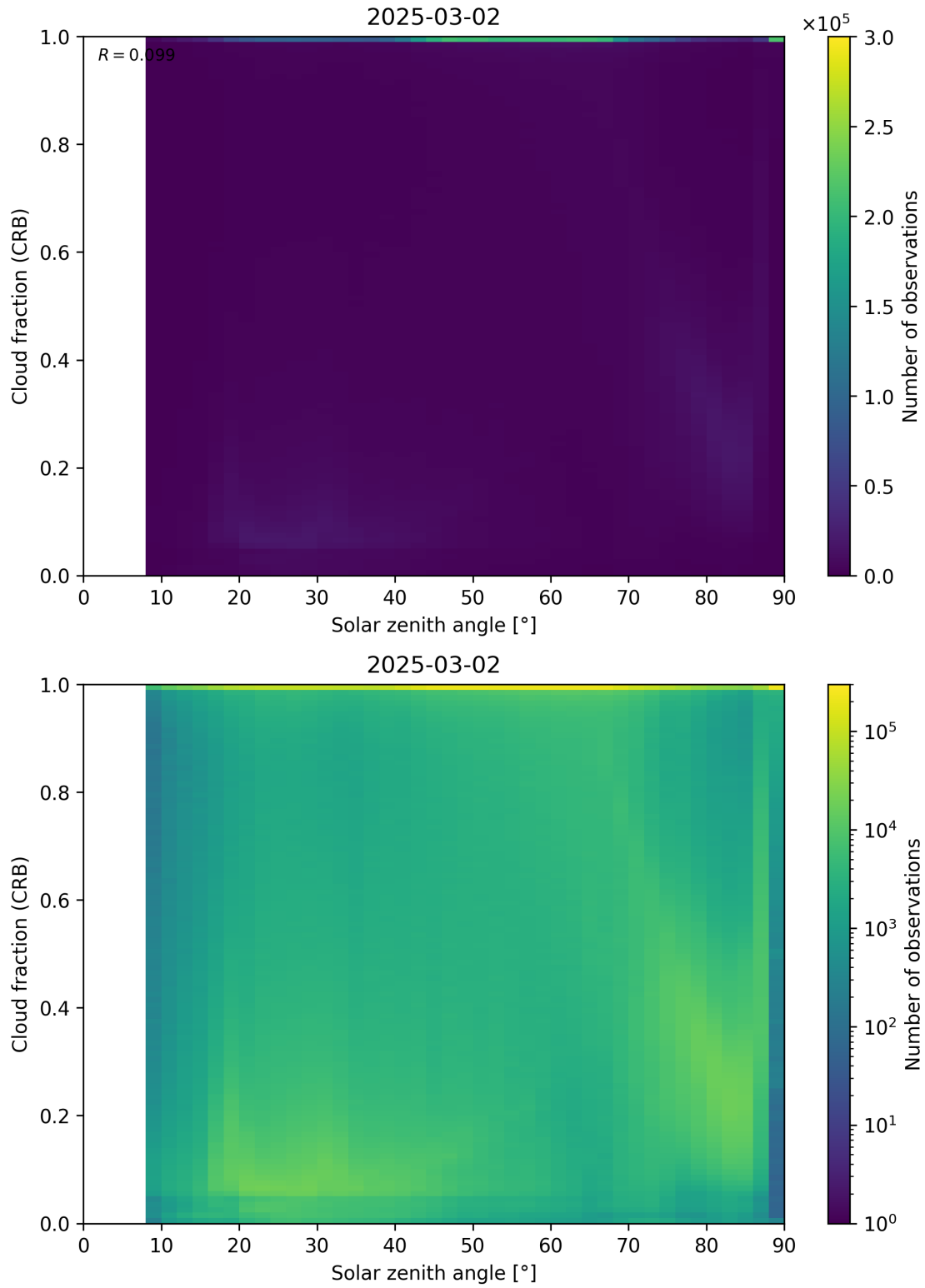
Figure 101: Scatter density plot of “Solar zenith angle” against “Cloud fraction (CRB)” for 2025-03-01 to 2025-03-03.
