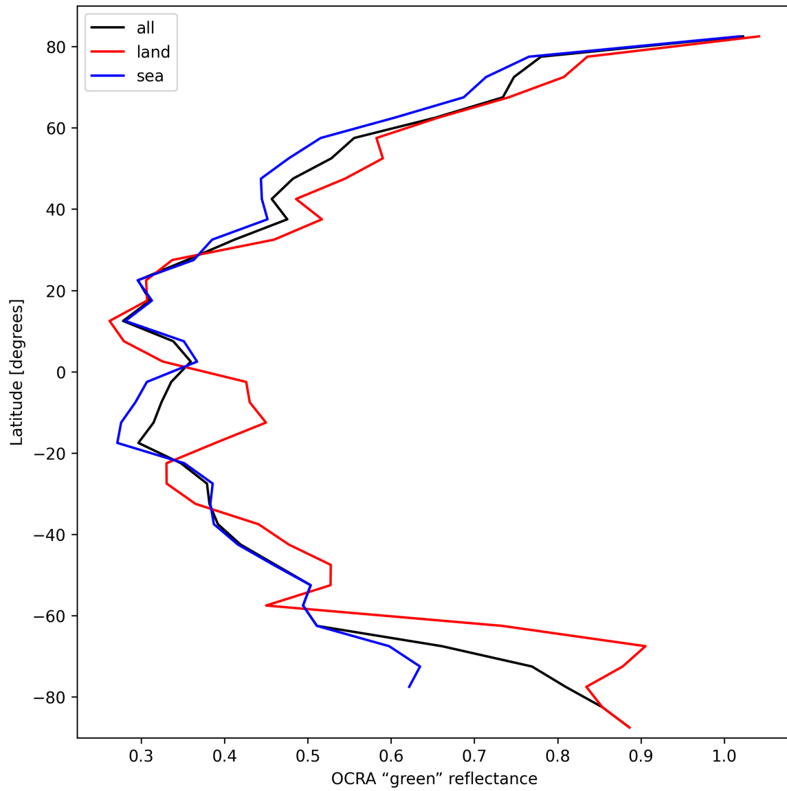
Figure 36: Zonal average of “OCRA “green” reflectance” for 2025-03-01 to 2025-03-03.
