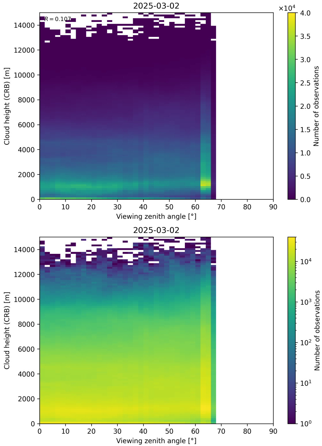
Figure 110: Scatter density plot of “Viewing zenith angle” against “Cloud height (CRB)” for 2025-03-01 to 2025-03-03.
