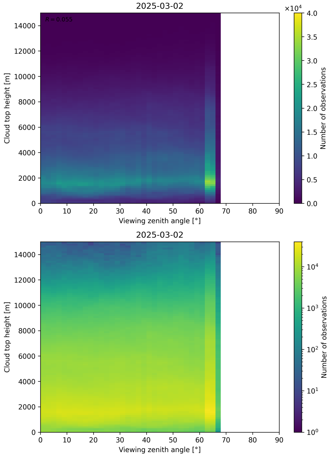
Figure 112: Scatter density plot of “Viewing zenith angle” against “Cloud top height” for 2025-03-01 to 2025-03-03.
