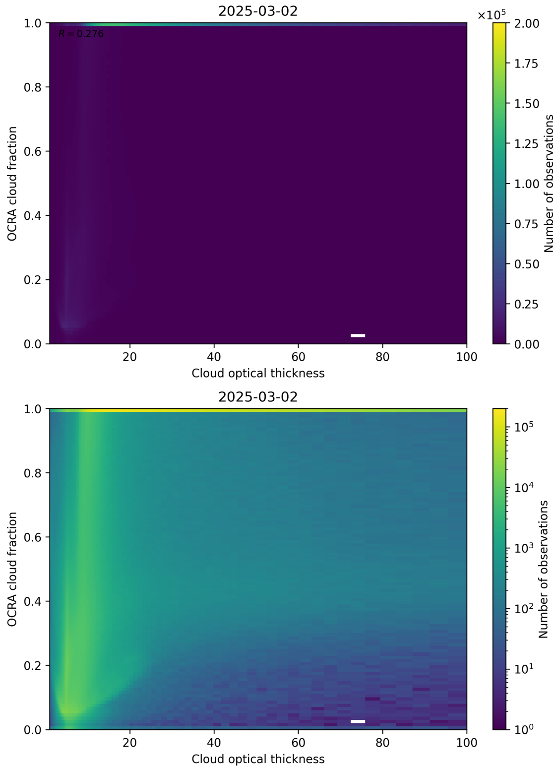
Figure 83: Scatter density plot of “Cloud optical thickness” against “OCRA cloud fraction” for 2025-03-01 to 2025-03-03.
