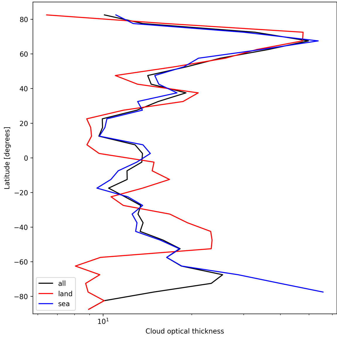
Figure 25: Zonal average of “Cloud optical thickness” for 2025-03-01 to 2025-03-03.
