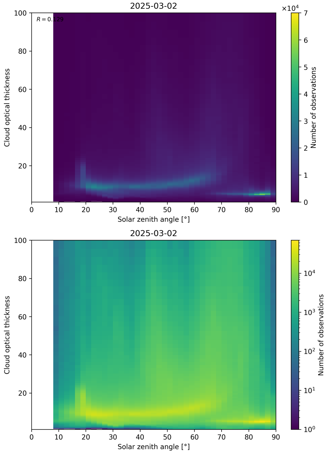
Figure 103: Scatter density plot of “Solar zenith angle” against “Cloud optical thickness” for 2025-03-01 to 2025-03-03.
