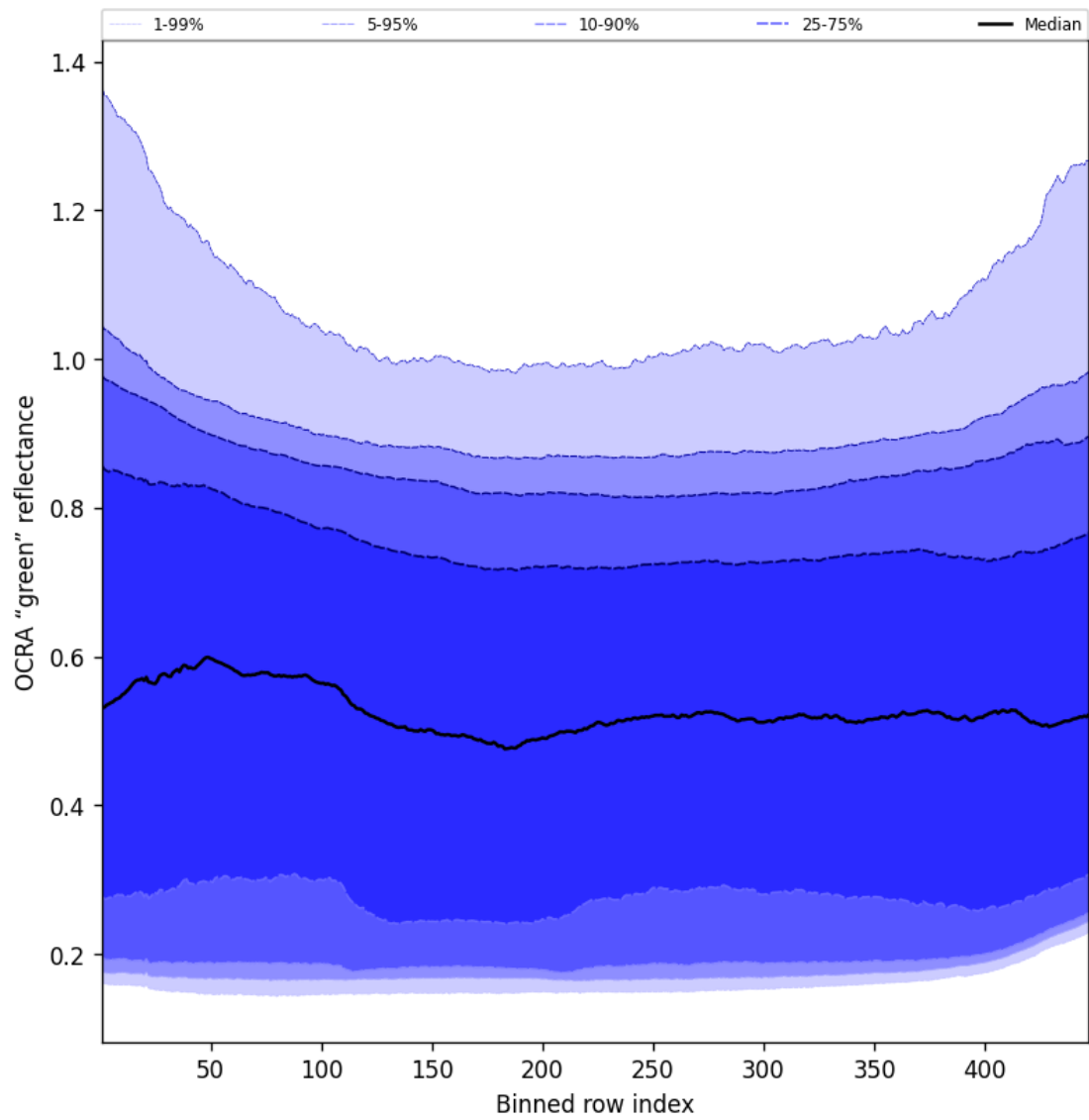
Figure 68: Along track statistics of “OCRA “green” reflectance” for 2025-03-01 to 2025-03-03
