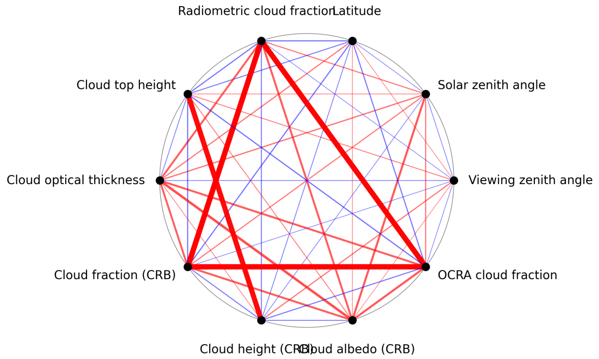
Figure 1: Map of correlation graph for 2025-03-01 to 2025-03-03.
