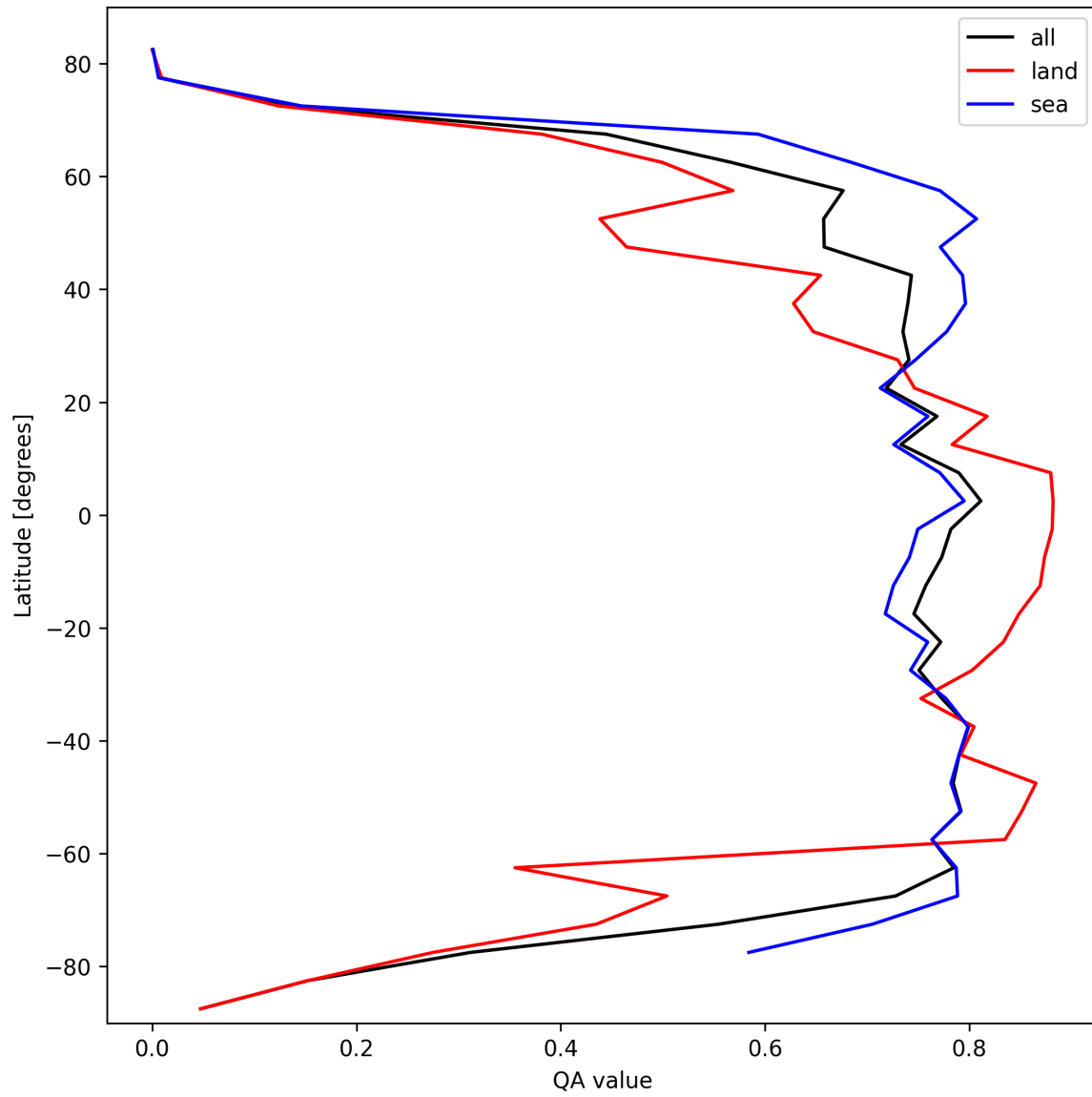
Figure 22: Zonal average of “QA value” for 2025-03-01 to 2025-03-03.
