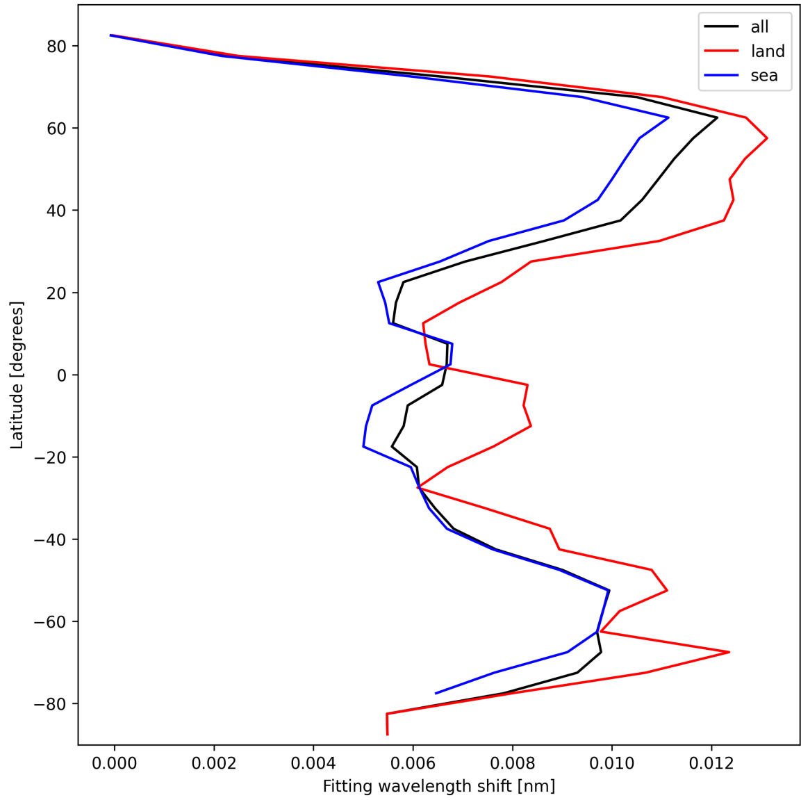
Figure 33: Zonal average of “Fitting wavelength shift” for 2025-03-01 to 2025-03-03.
