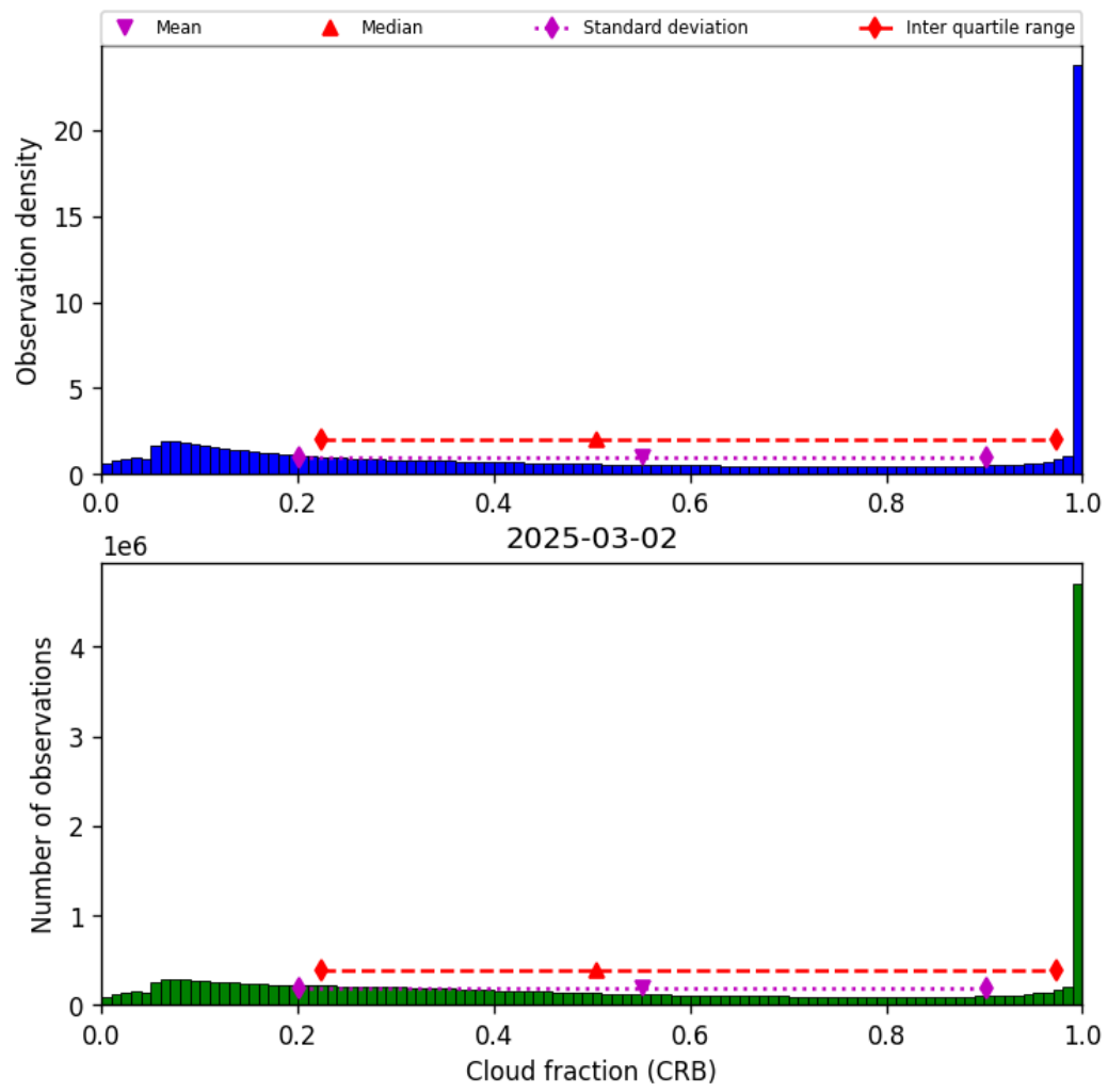
Figure 42: Histogram of “Cloud fraction (CRB)” for 2025-03-01 to 2025-03-03
