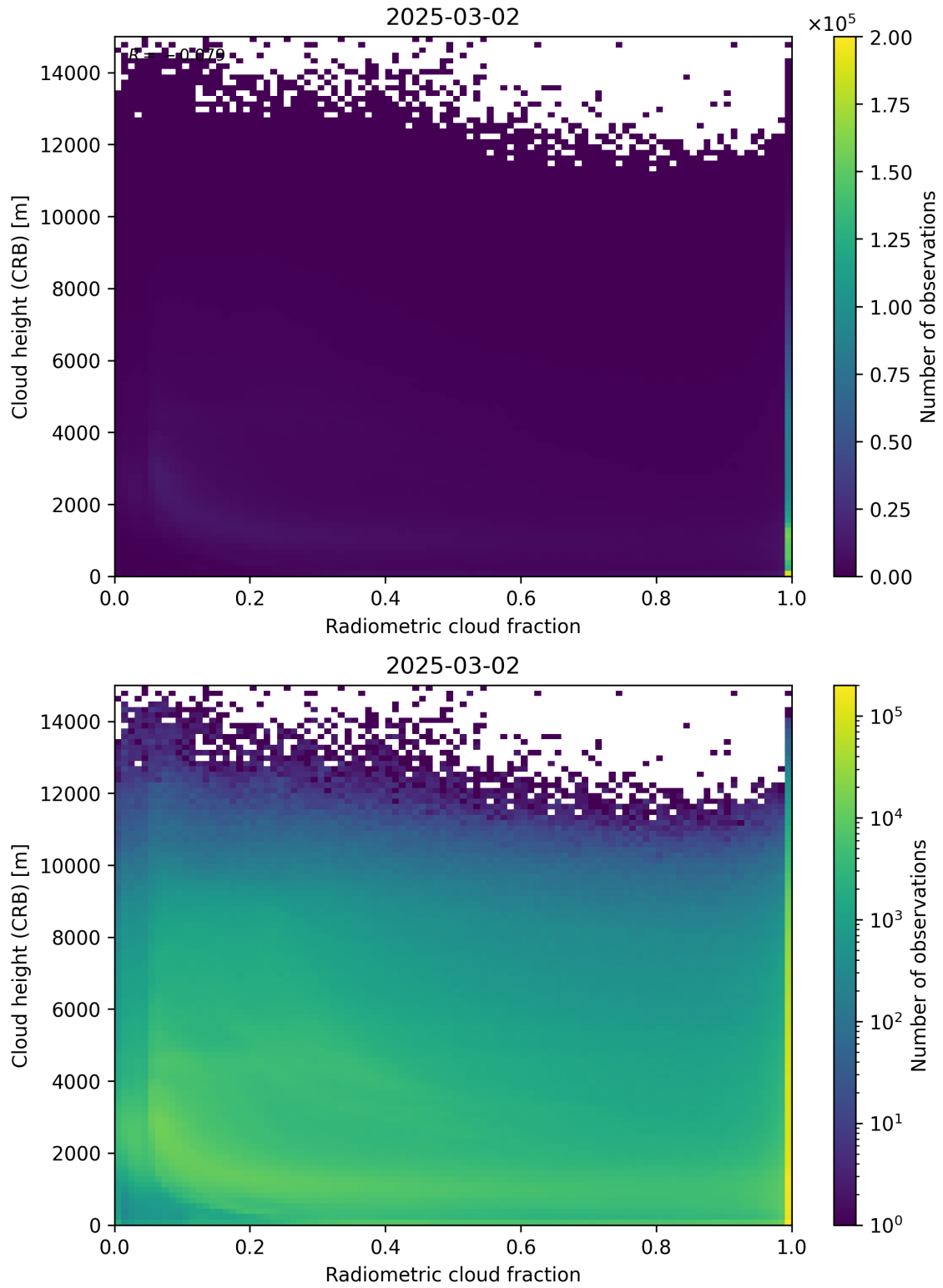
Figure 74: Scatter density plot of “Radiometric cloud fraction” against “Cloud height (CRB)” for 2025-03-01 to 2025-03-03.
