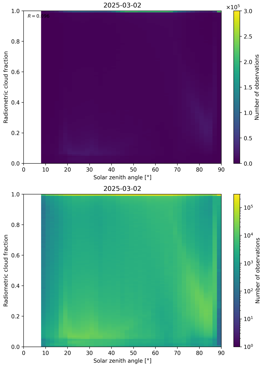
Figure 99: Scatter density plot of “Solar zenith angle” against “Radiometric cloud fraction” for 2025-03-01 to 2025-03-03.
