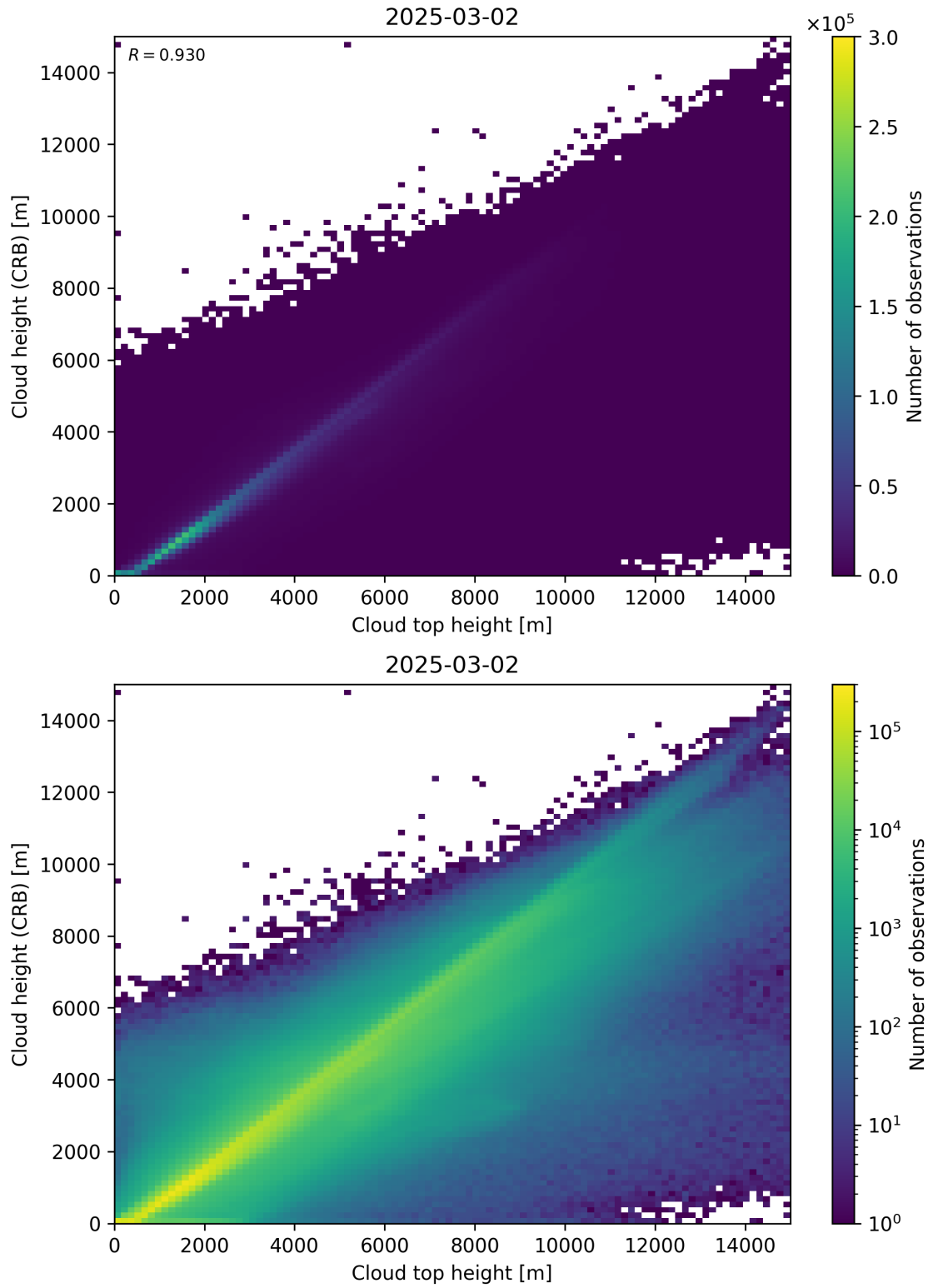
Figure 89: Scatter density plot of “Cloud top height” against “Cloud height (CRB)” for 2025-03-01 to 2025-03-03.
