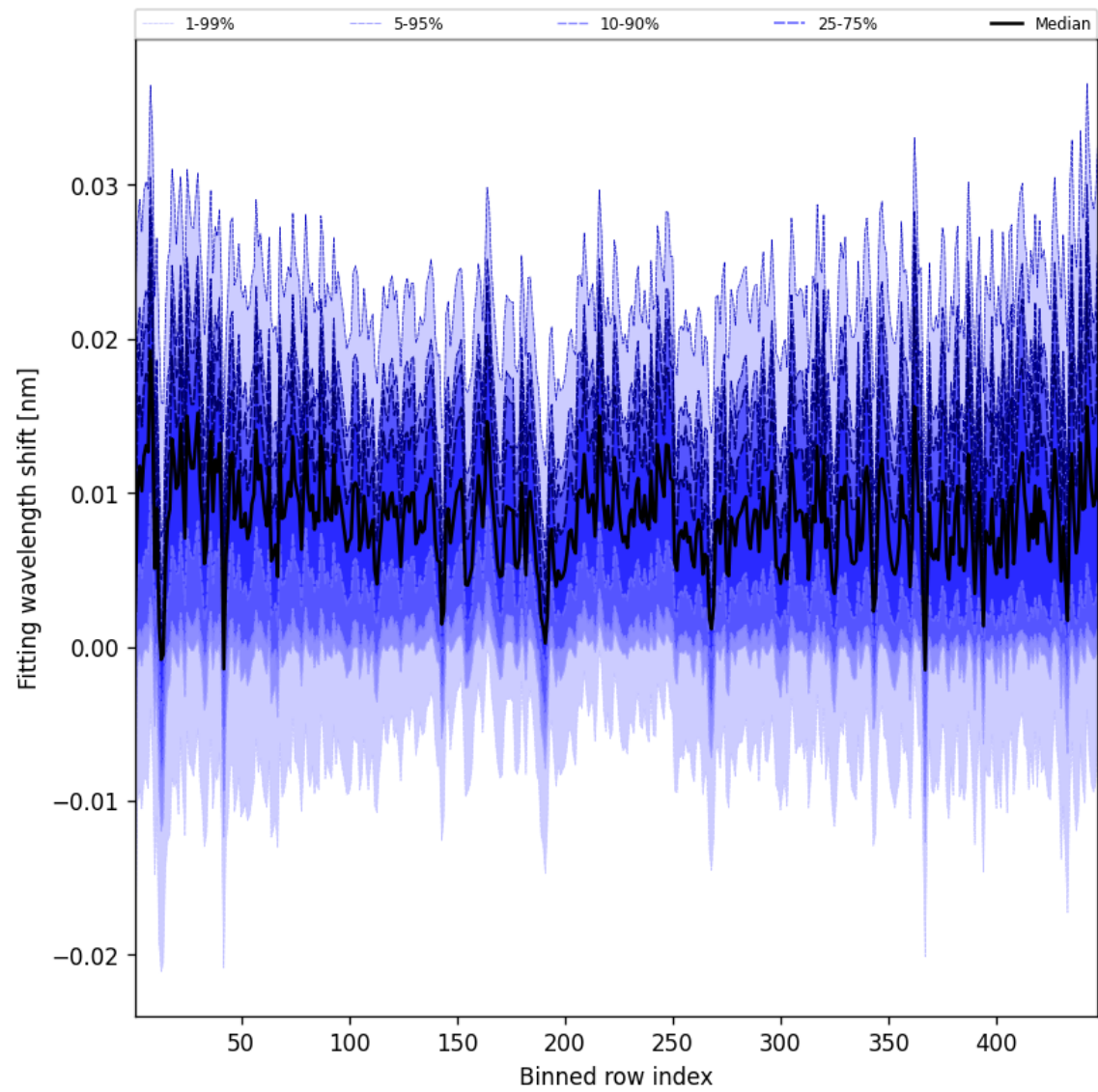
Figure 65: Along track statistics of “Fitting wavelength shift” for 2025-03-01 to 2025-03-03
