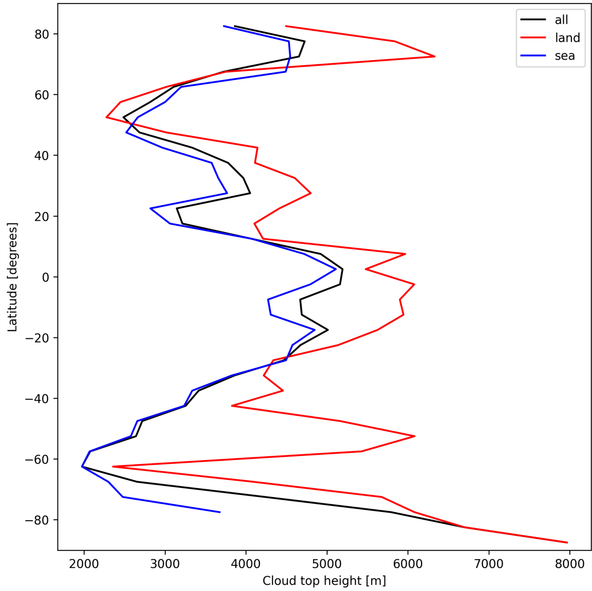
Figure 24: Zonal average of “Cloud top height” for 2025-03-01 to 2025-03-03.
