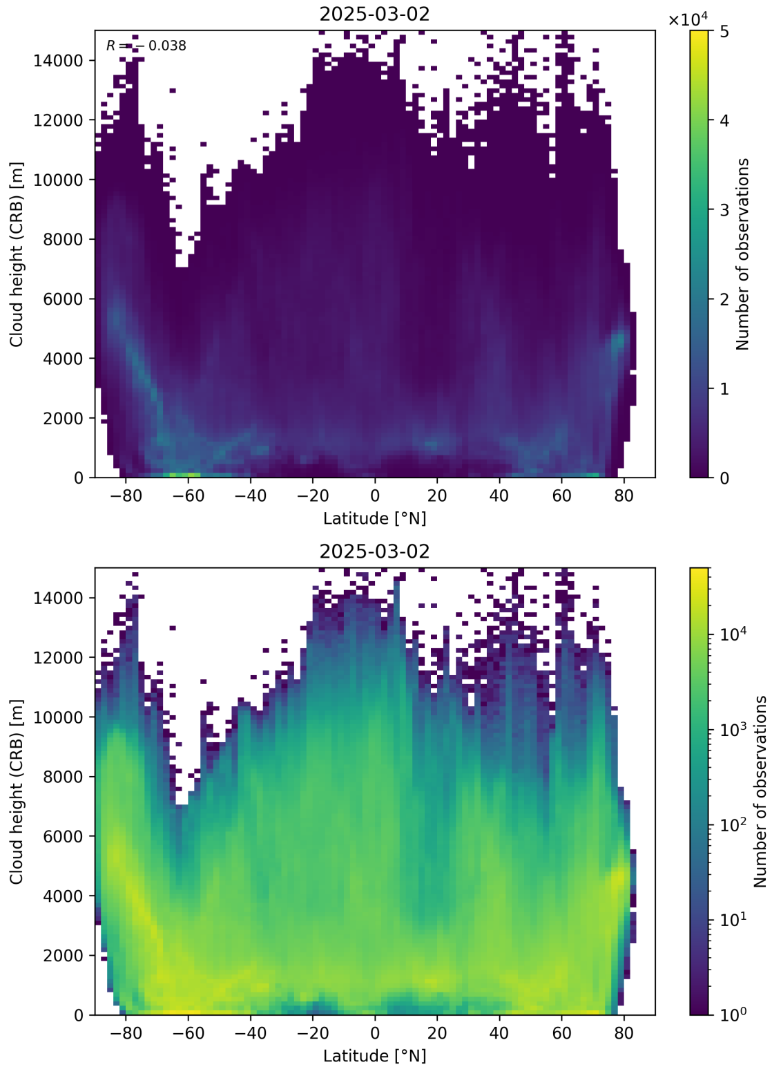
Figure 95: Scatter density plot of “Latitude” against “Cloud height (CRB)” for 2025-03-01 to 2025-03-03.
