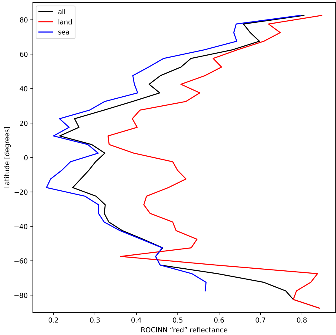
Figure 37: Zonal average of “ROCINN “red” reflectance” for 2025-03-01 to 2025-03-03.
