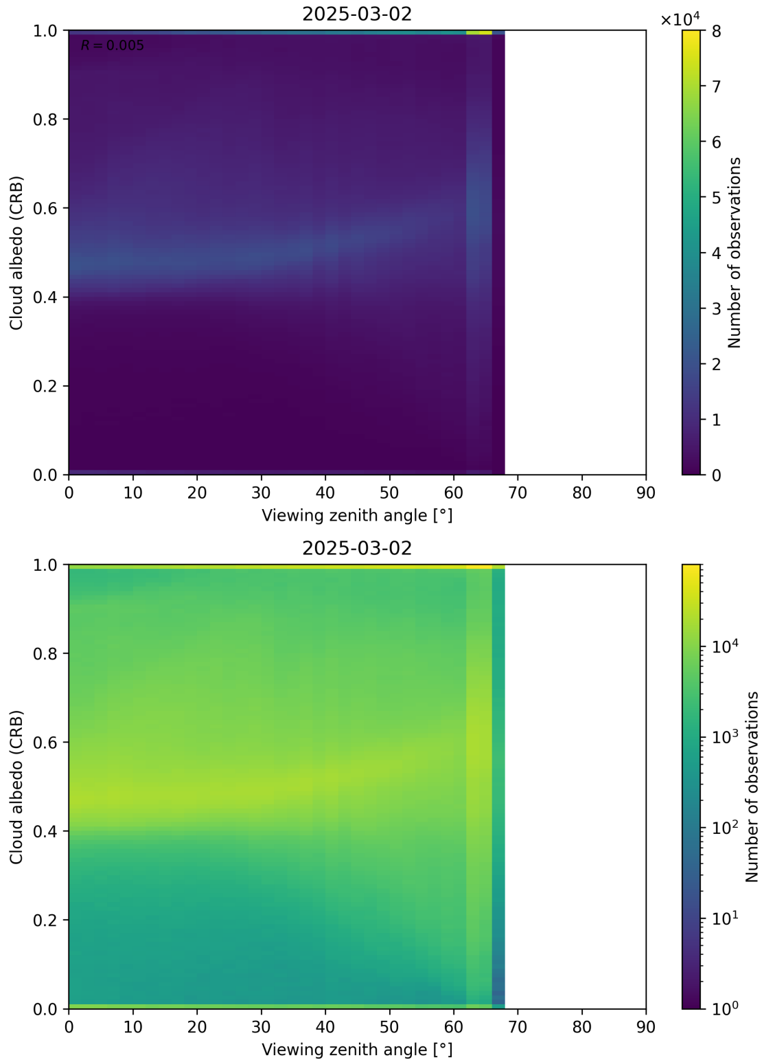
Figure 106: Scatter density plot of “Viewing zenith angle” against “Cloud albedo (CRB)” for 2025-03-01 to 2025-03-03.
