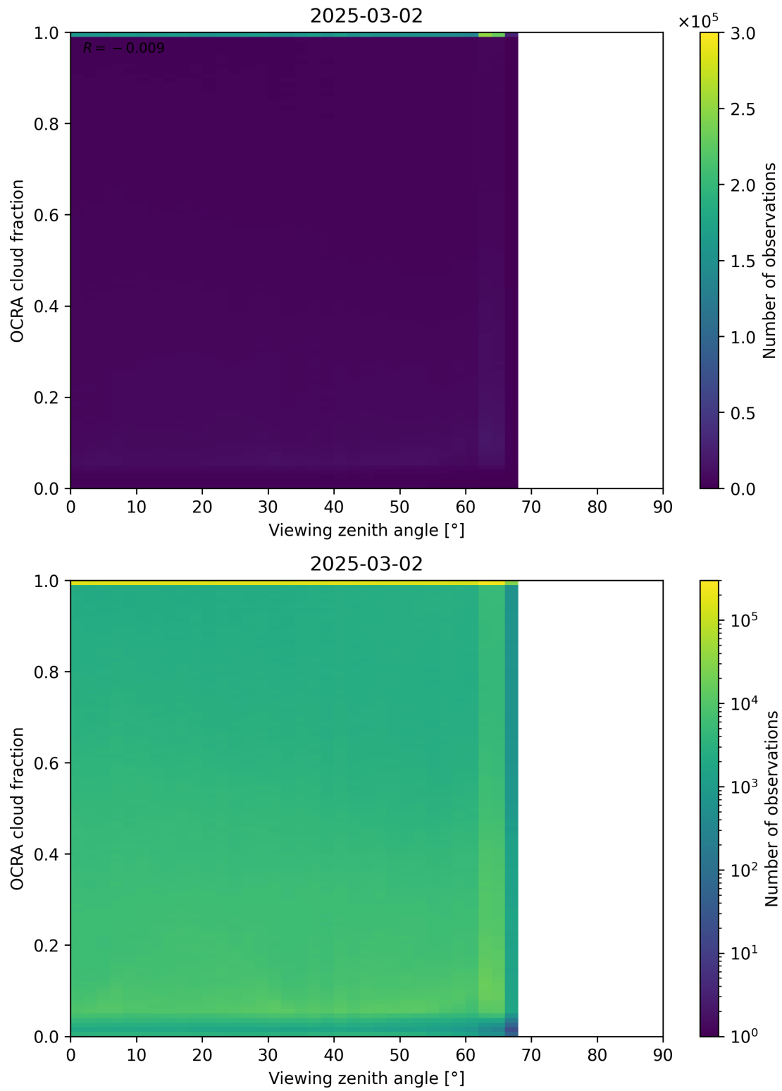
Figure 108: Scatter density plot of “Viewing zenith angle” against “OCRA cloud fraction” for 2025-03-01 to 2025-03-03.
