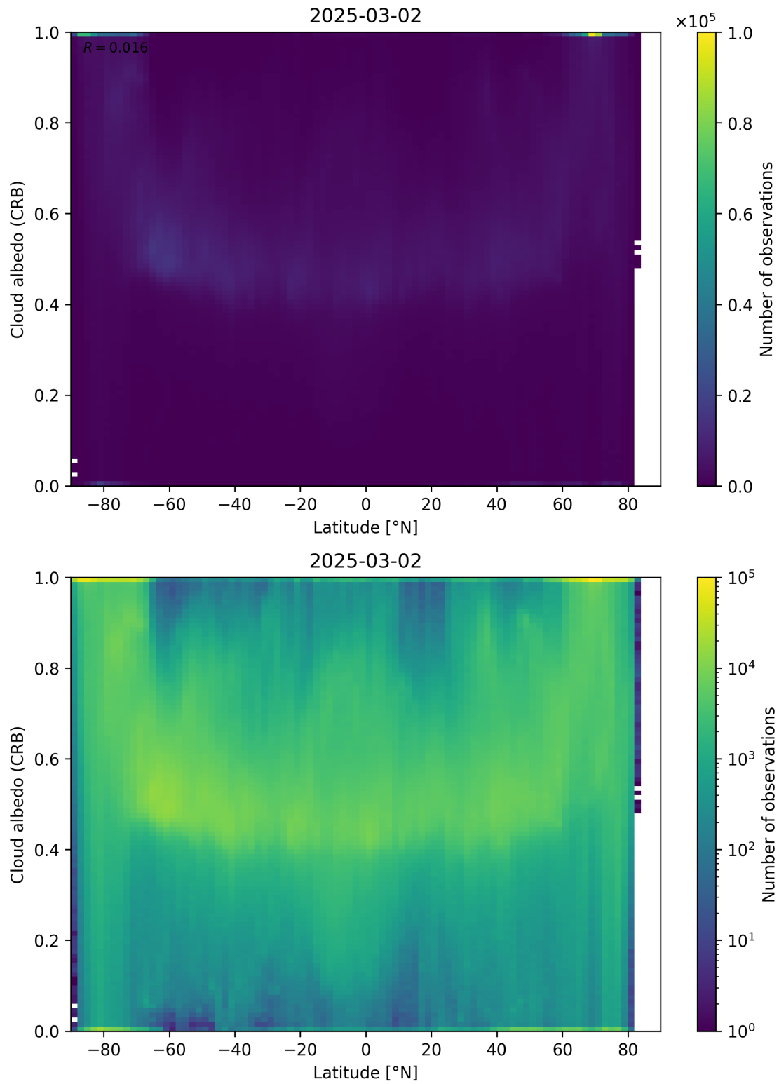
Figure 91: Scatter density plot of “Latitude” against “Cloud albedo (CRB)” for 2025-03-01 to 2025-03-03.
