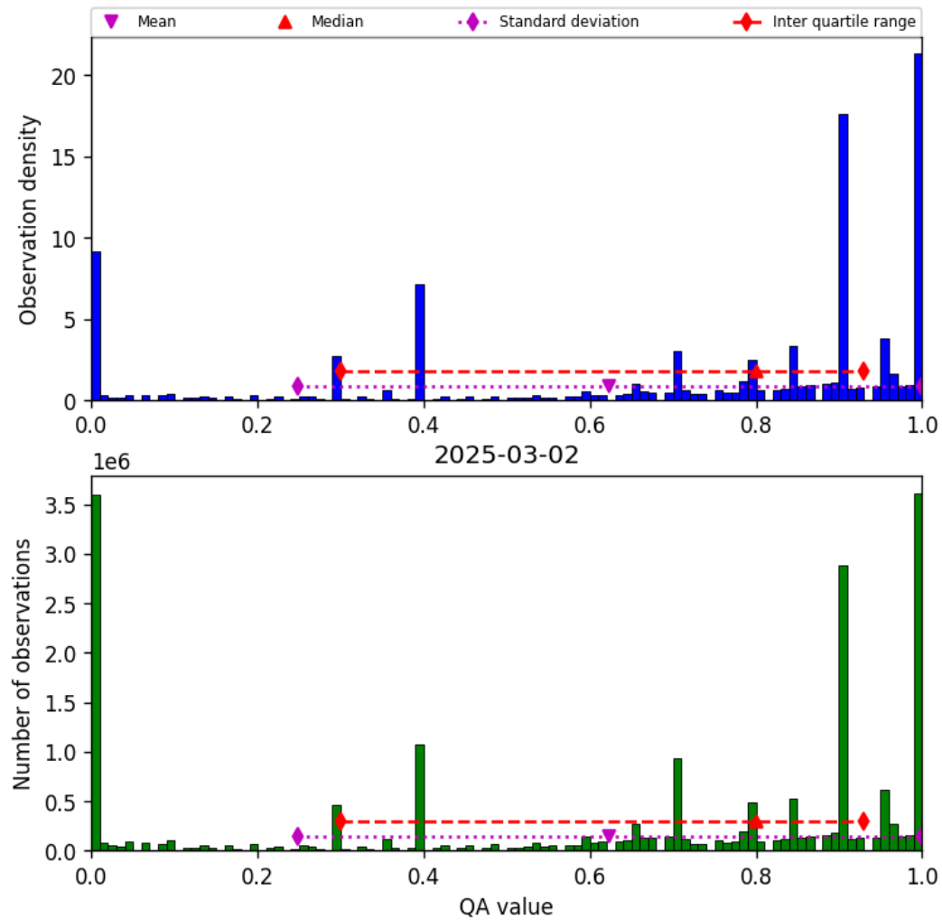
Figure 38: Histogram of “QA value” for 2025-03-01 to 2025-03-03
