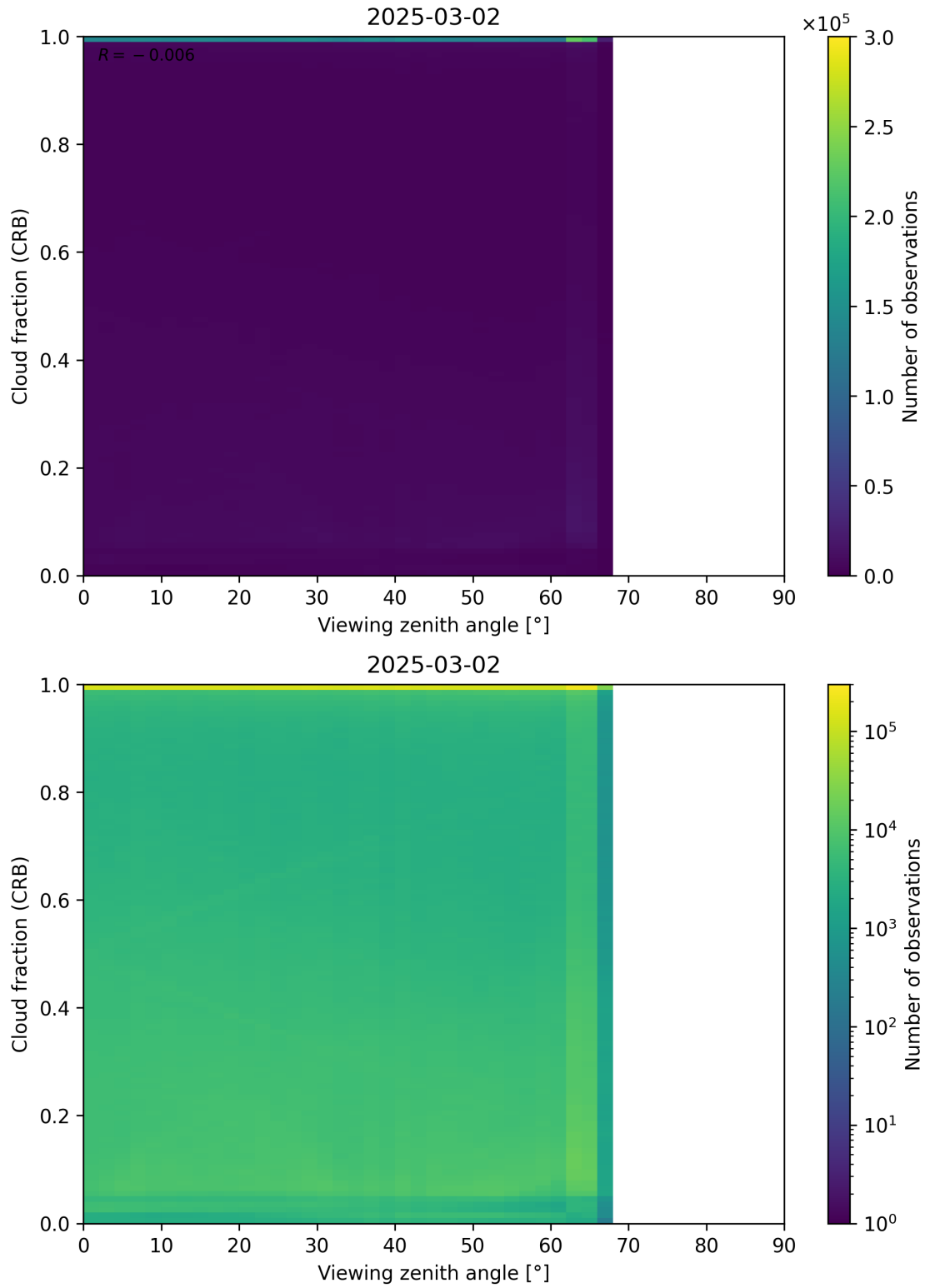
Figure 109: Scatter density plot of “Viewing zenith angle” against “Cloud fraction (CRB)” for 2025-03-01 to 2025-03-03.
