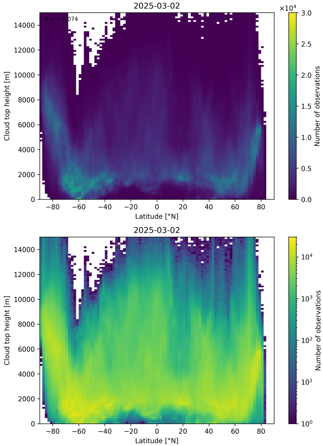
Figure 97: Scatter density plot of “Latitude” against “Cloud top height” for 2025-03-01 to 2025-03-03.
