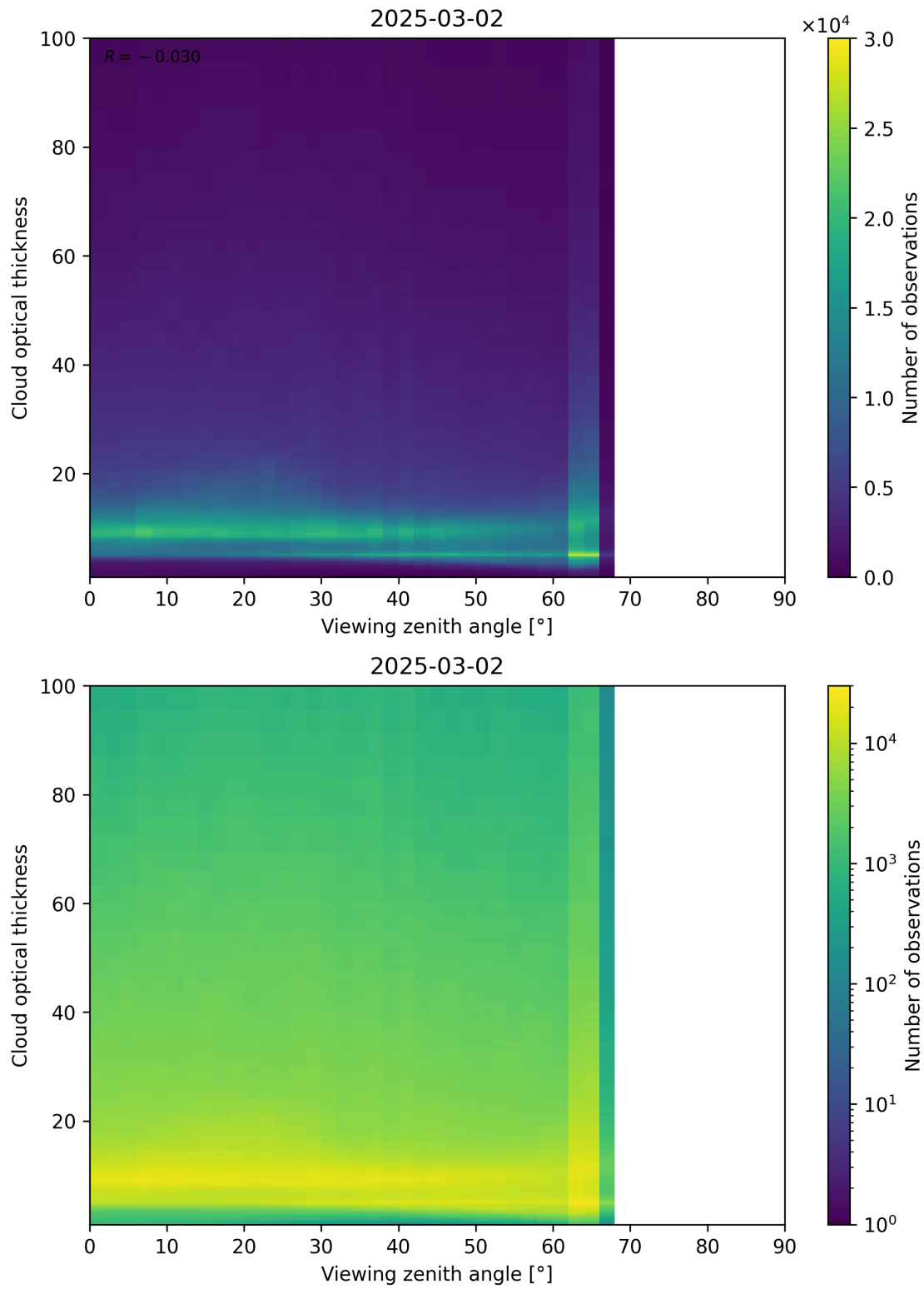
Figure 111: Scatter density plot of “Viewing zenith angle” against “Cloud optical thickness” for 2025-03-01 to 2025-03-03.
