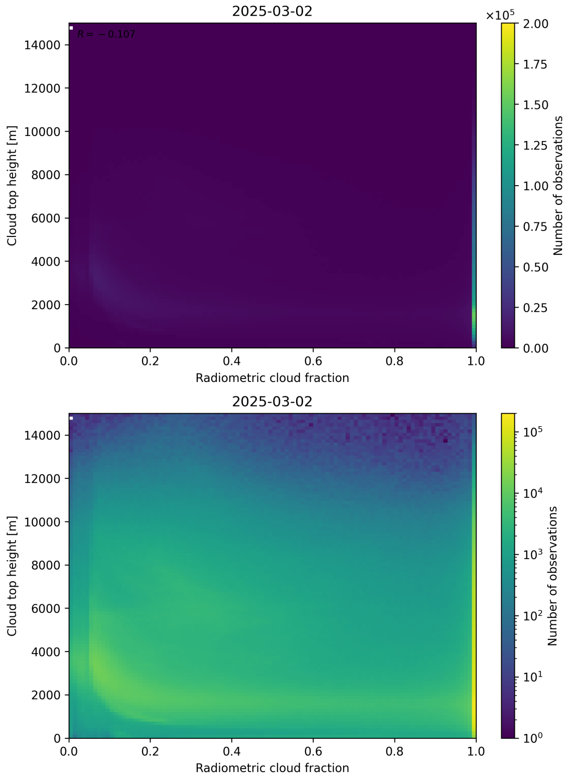
Figure 76: Scatter density plot of “Radiometric cloud fraction” against “Cloud top height” for 2025-03-01 to 2025-03-03.
