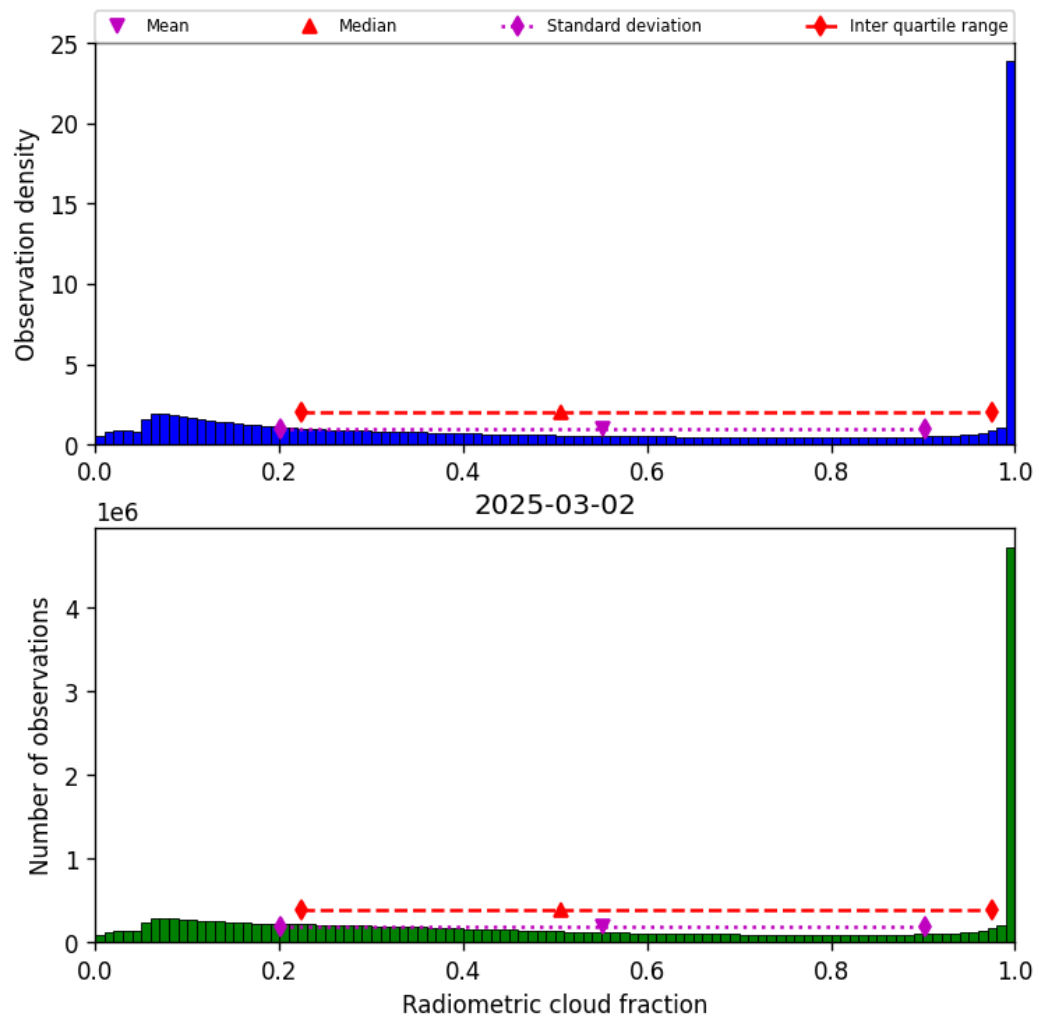
Figure 39: Histogram of “Radiometric cloud fraction” for 2025-03-01 to 2025-03-03
