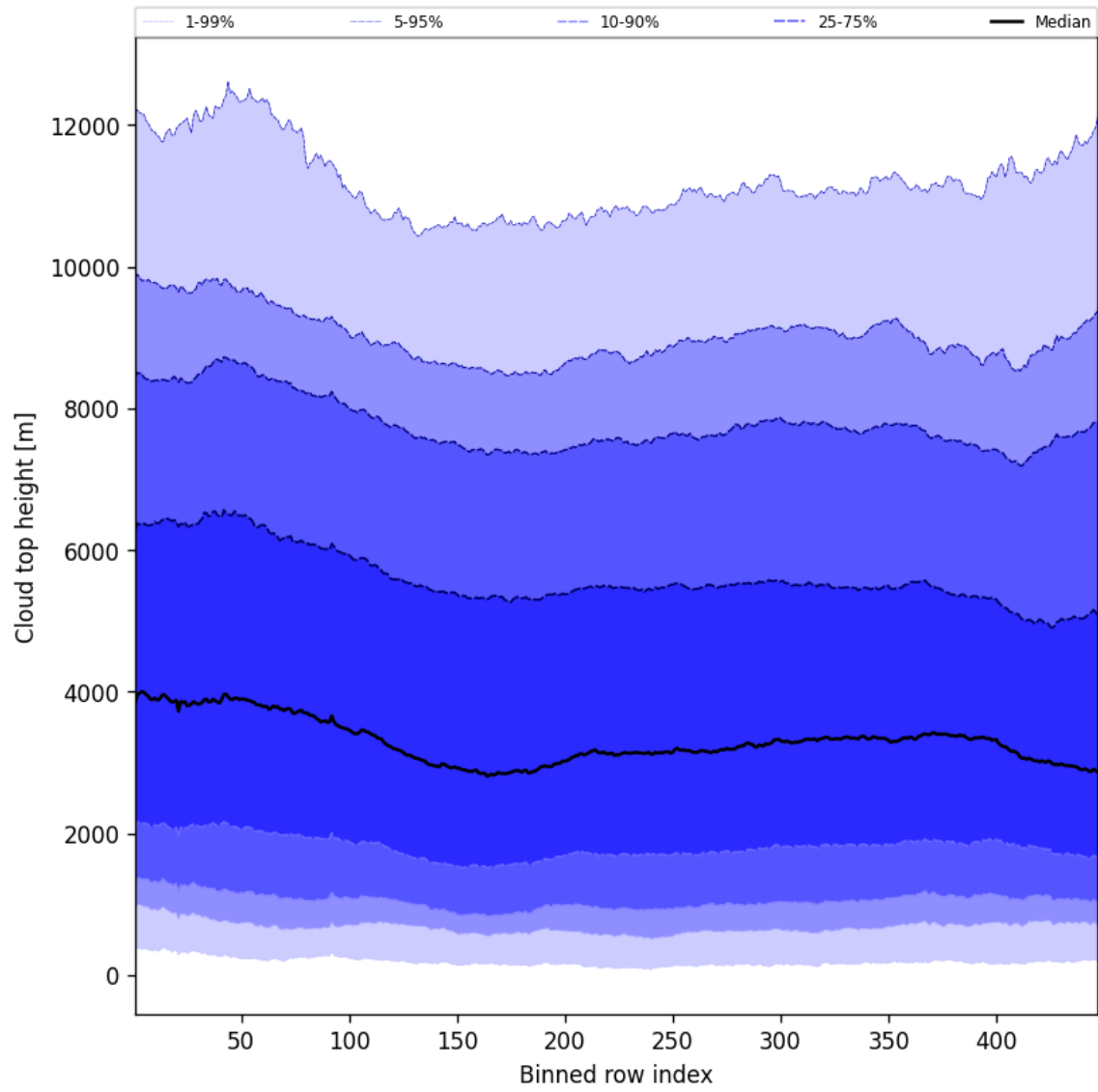
Figure 56: Along track statistics of “Cloud top height” for 2025-03-01 to 2025-03-03
