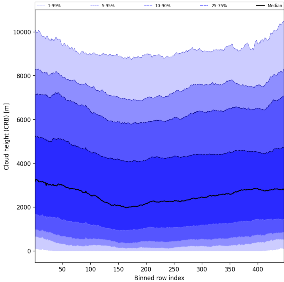
Figure 59: Along track statistics of “Cloud height (CRB)” for 2025-03-01 to 2025-03-03
