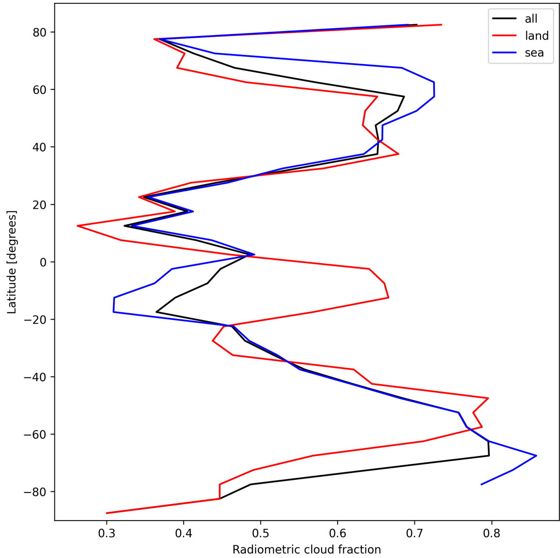
Figure 23: Zonal average of “Radiometric cloud fraction” for 2025-03-01 to 2025-03-03.
