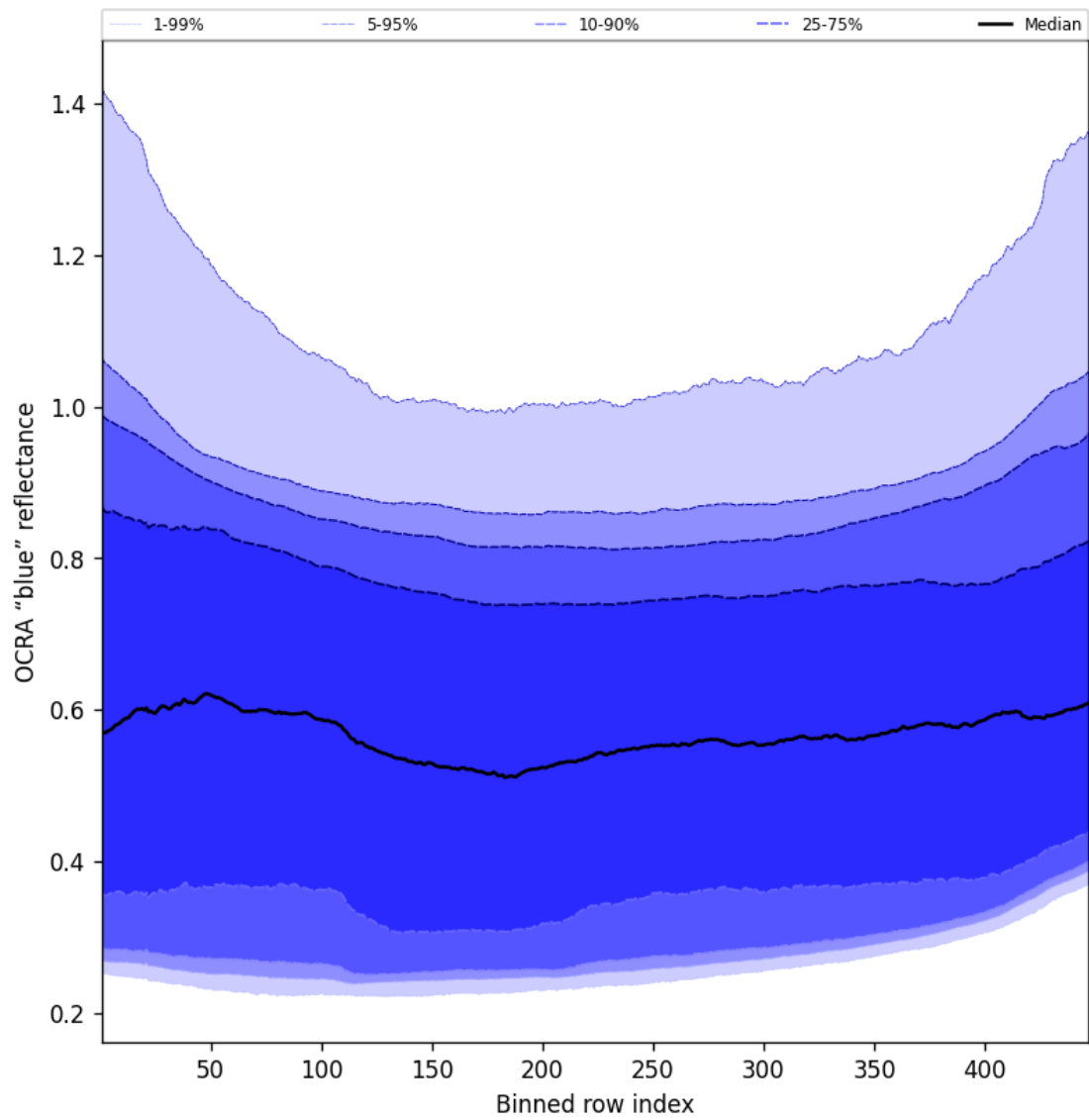
Figure 67: Along track statistics of “OCRA “blue” reflectance” for 2025-03-01 to 2025-03-03
