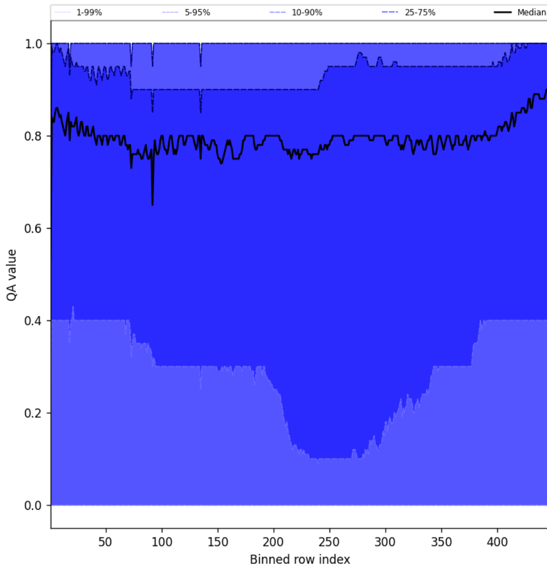
Figure 54: Along track statistics of “QA value” for 2025-03-01 to 2025-03-03
