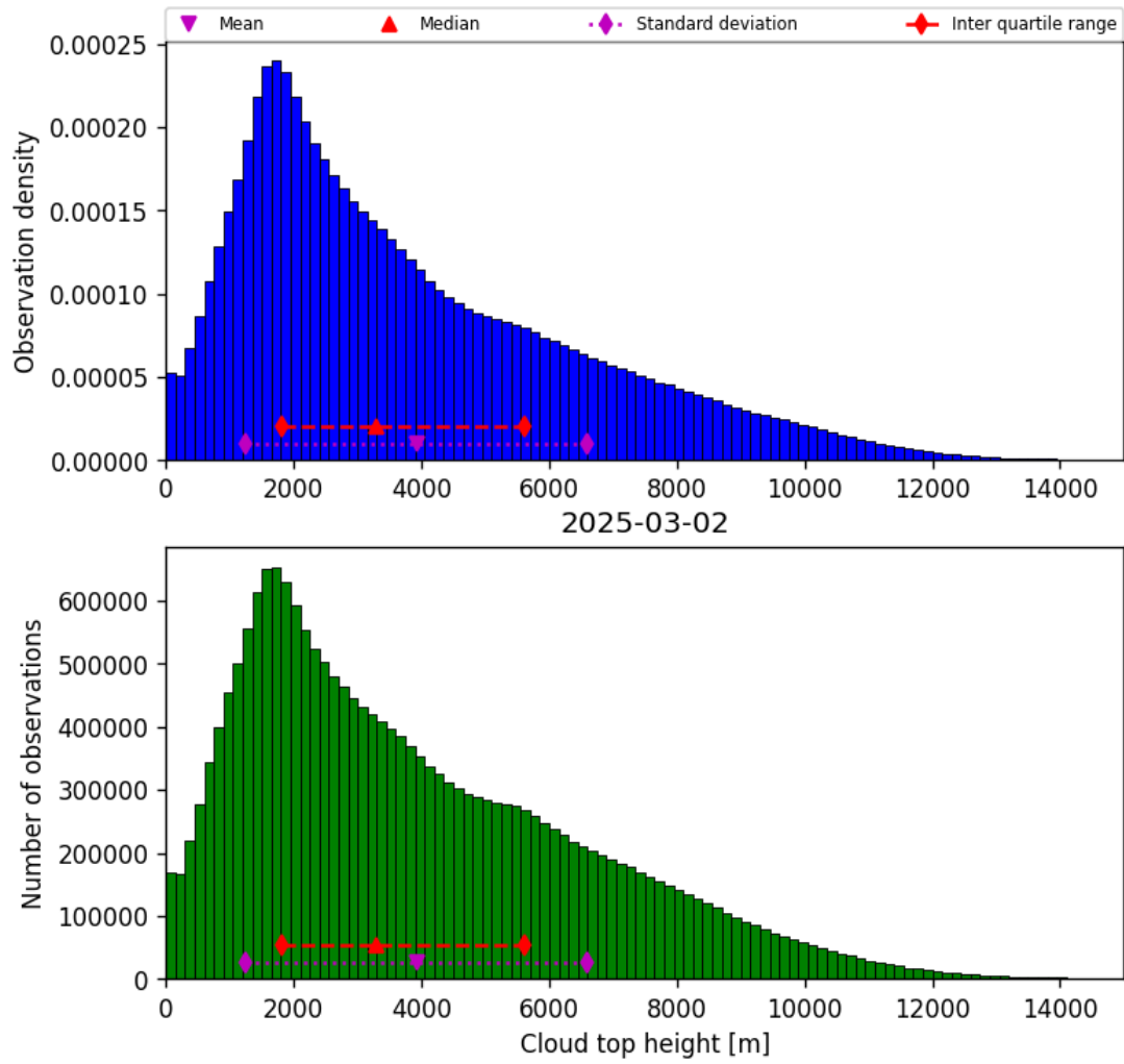
Figure 40: Histogram of “Cloud top height” for 2025-03-01 to 2025-03-03
