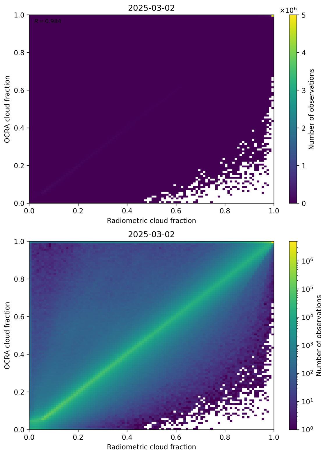
Figure 72: Scatter density plot of “Radiometric cloud fraction” against “OCRA cloud fraction” for 2025-03-01 to 2025-03-03.
