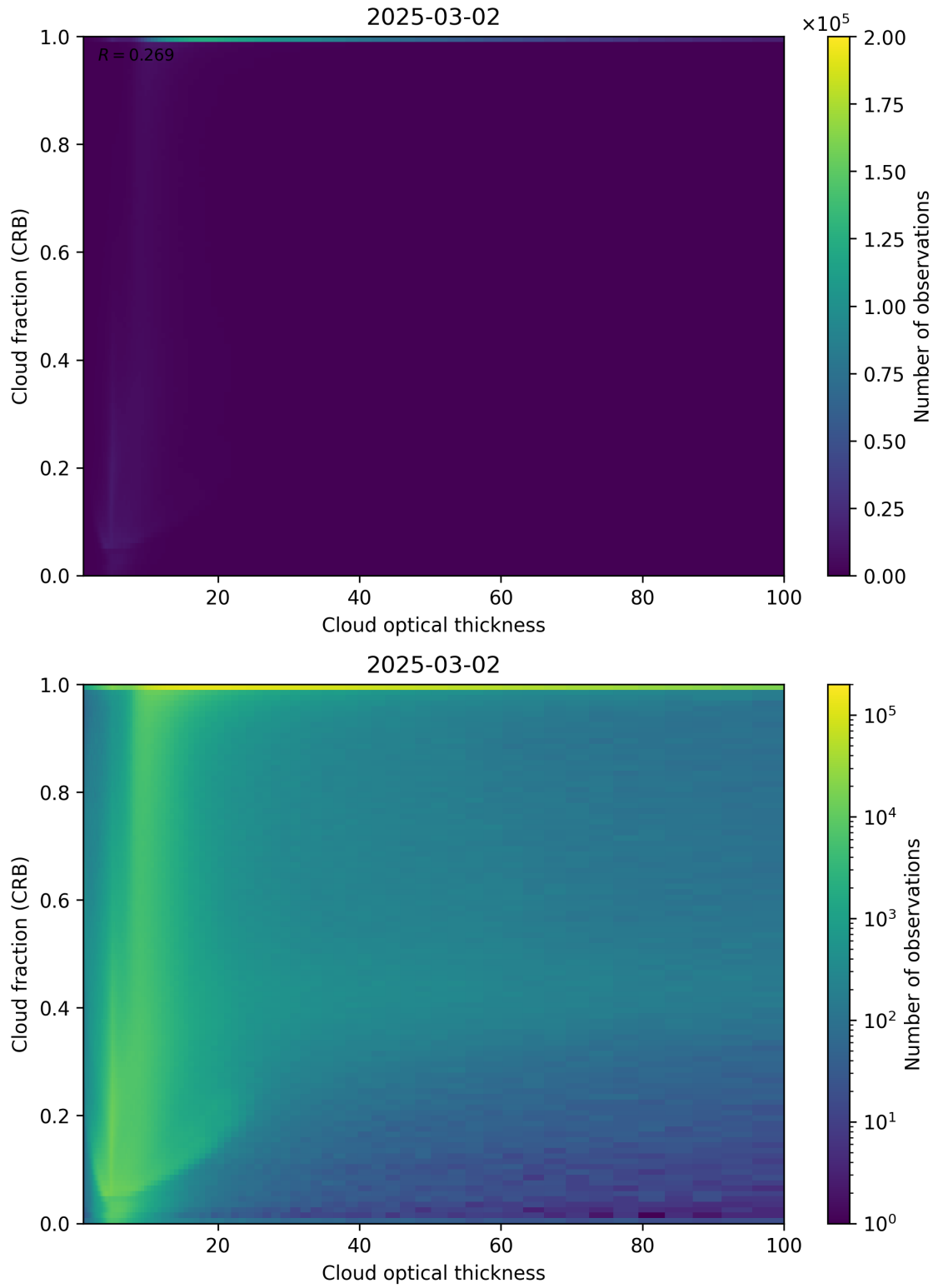
Figure 84: Scatter density plot of “Cloud optical thickness” against “Cloud fraction (CRB)” for 2025-03-01 to 2025-03-03.
