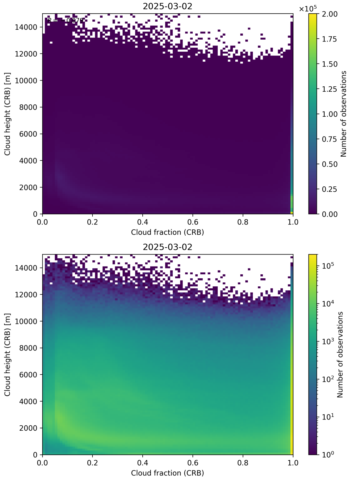
Figure 79: Scatter density plot of “Cloud fraction (CRB)” against “Cloud height (CRB)” for 2025-03-01 to 2025-03-03.
