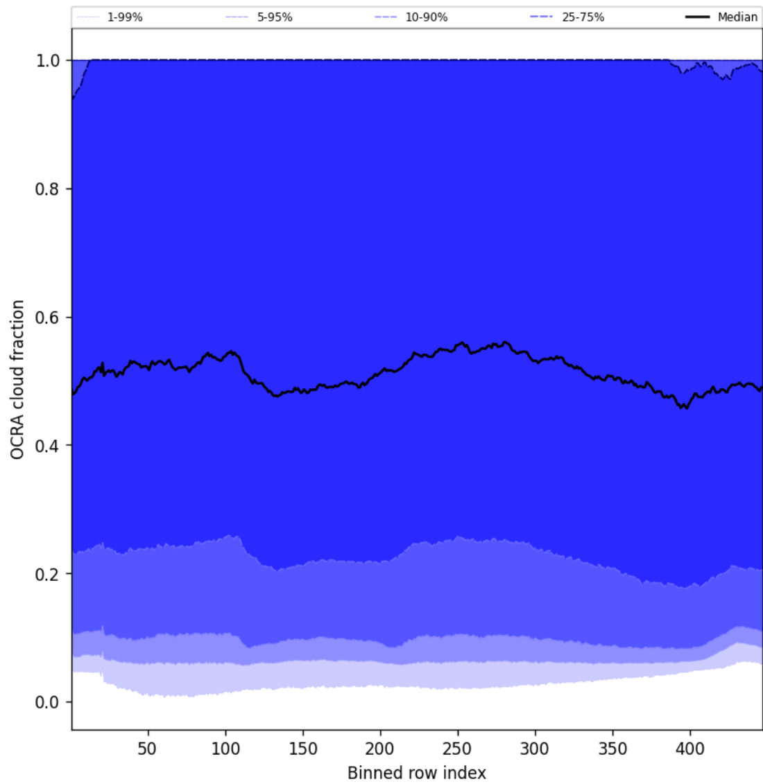
Figure 66: Along track statistics of “OCRA cloud fraction” for 2025-03-01 to 2025-03-03
