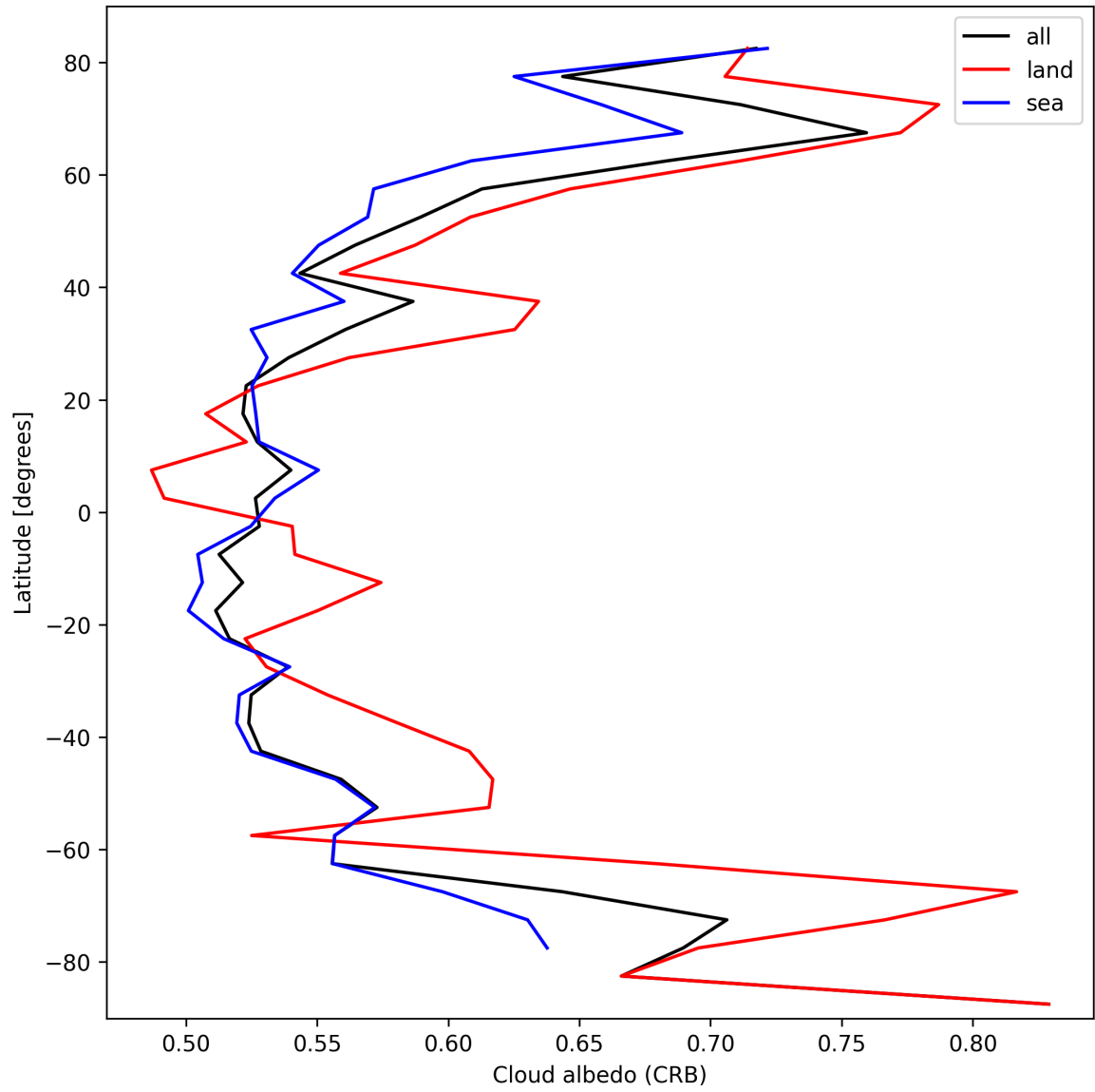
Figure 28: Zonal average of “Cloud albedo (CRB)” for 2025-03-01 to 2025-03-03.
