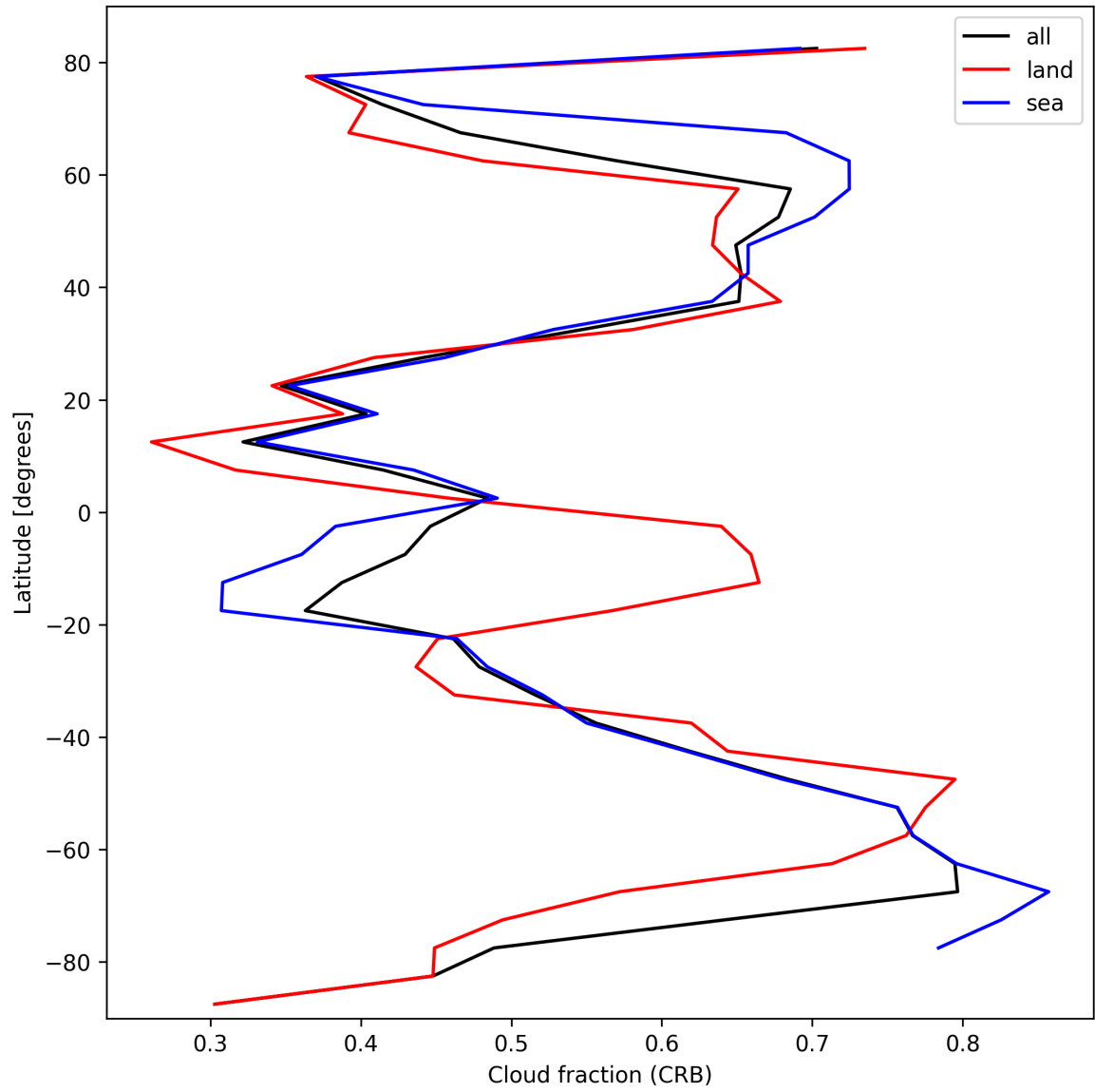
Figure 26: Zonal average of “Cloud fraction (CRB)” for 2025-03-01 to 2025-03-03.
