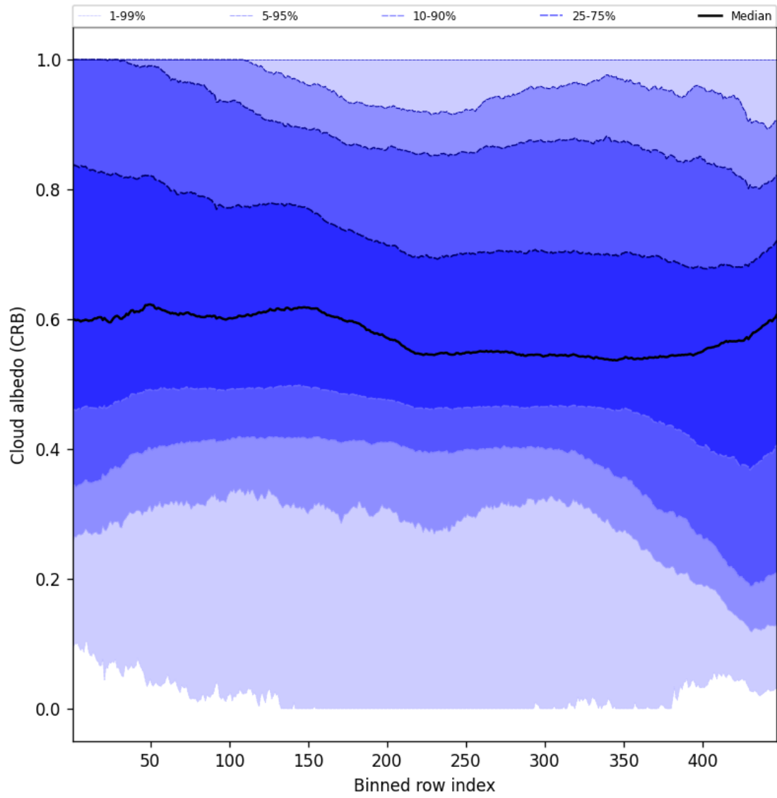
Figure 60: Along track statistics of “Cloud albedo (CRB)” for 2025-03-01 to 2025-03-03
