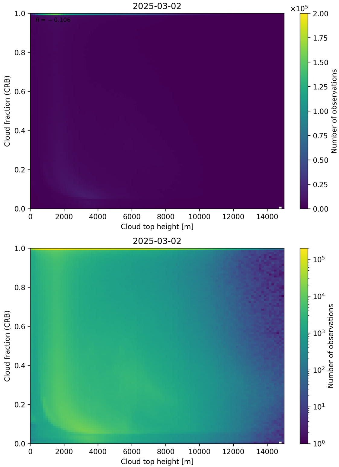
Figure 88: Scatter density plot of “Cloud top height” against “Cloud fraction (CRB)” for 2025-03-01 to 2025-03-03.
