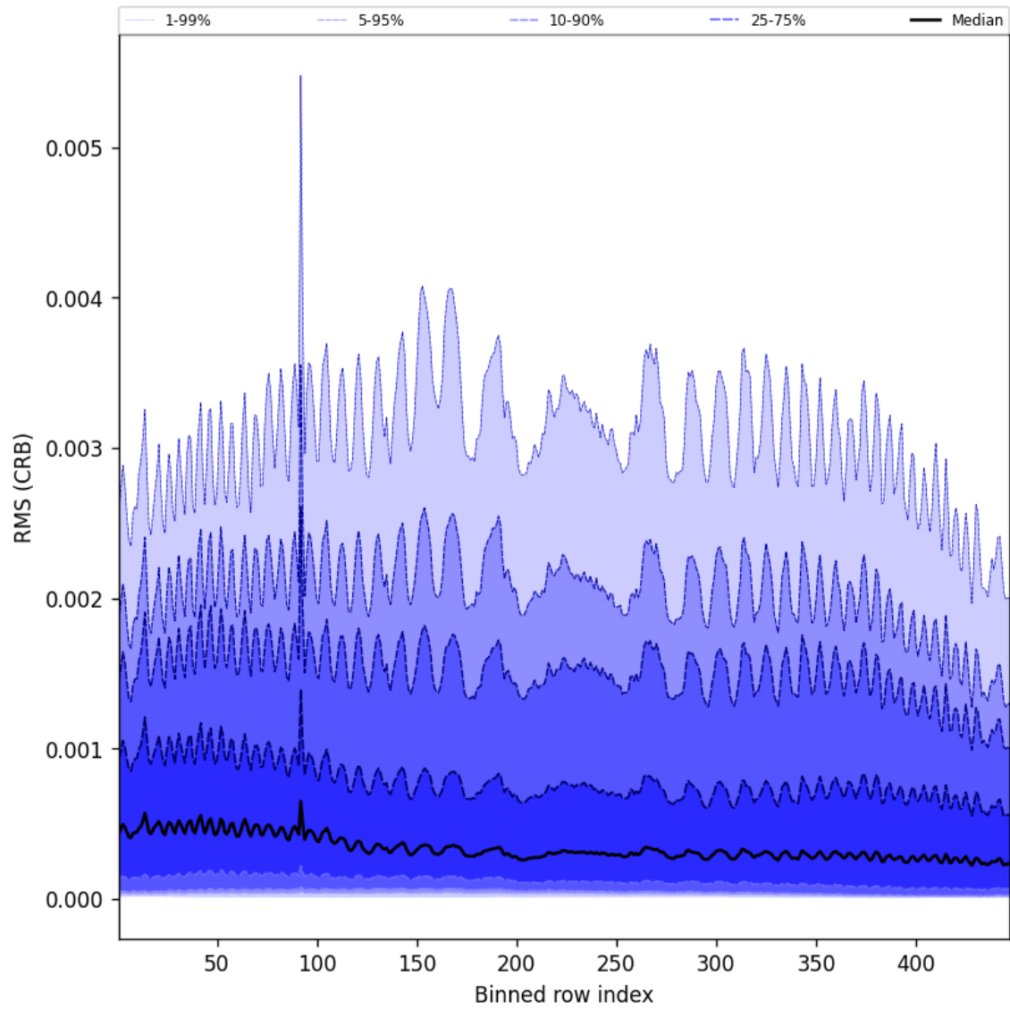
Figure 64: Along track statistics of “RMS (CRB)” for 2025-03-01 to 2025-03-03
