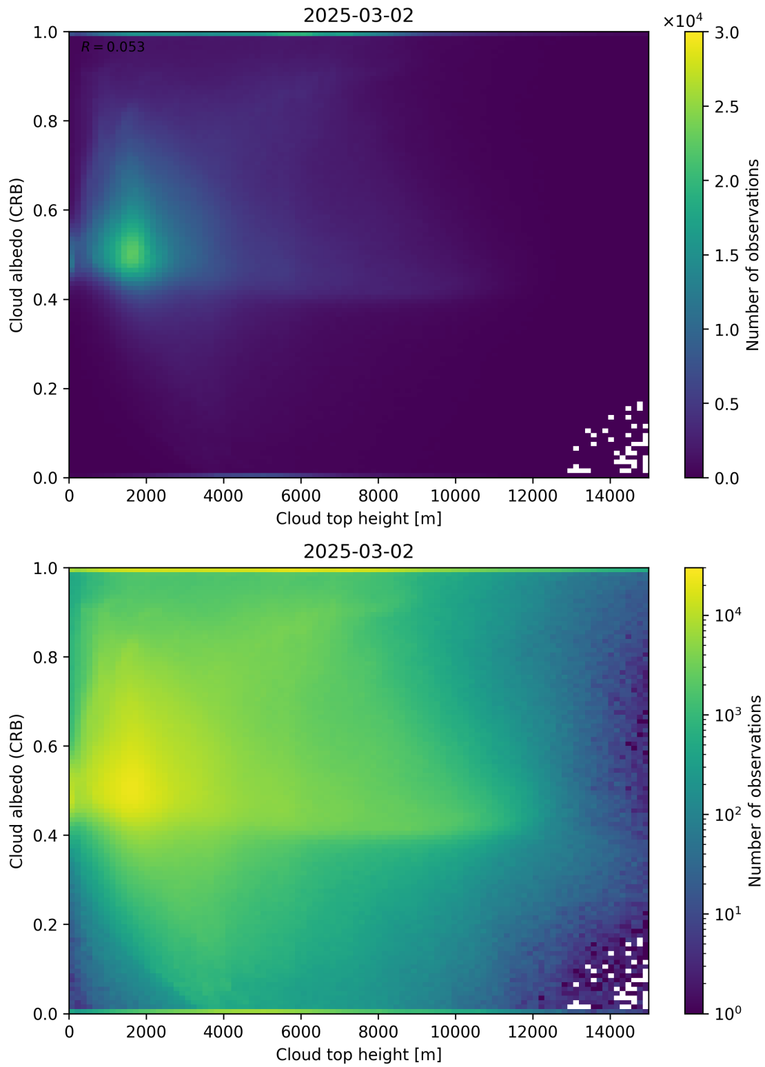
Figure 86: Scatter density plot of “Cloud top height” against “Cloud albedo (CRB)” for 2025-03-01 to 2025-03-03.
