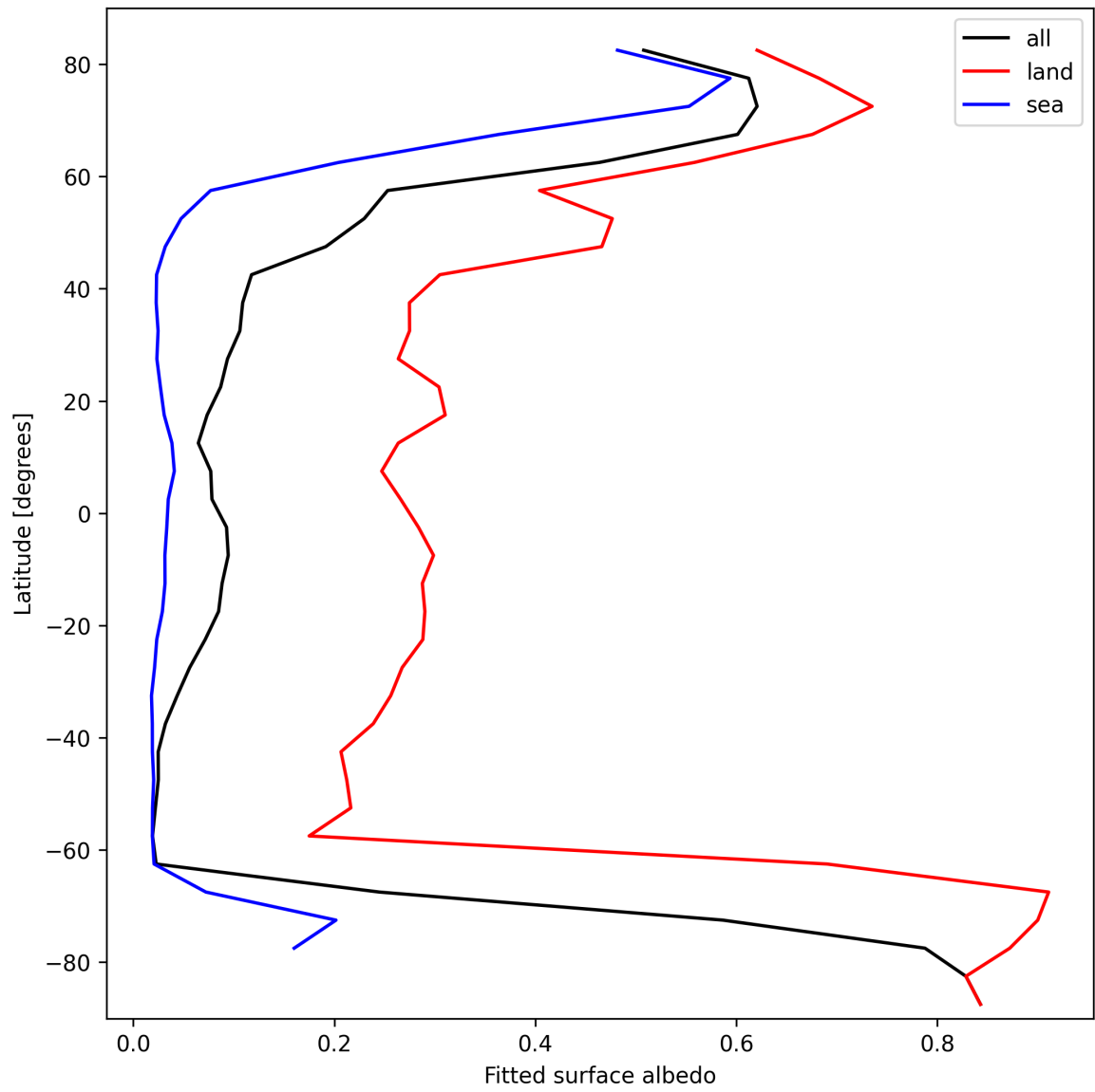
Figure 29: Zonal average of “Fitted surface albedo” for 2025-03-01 to 2025-03-03.
