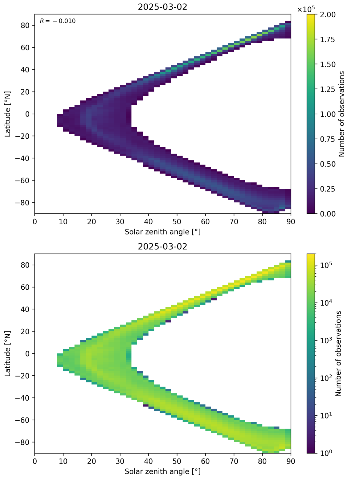
Figure 105: Scatter density plot of “Solar zenith angle” against “Latitude” for 2025-03-01 to 2025-03-03.
