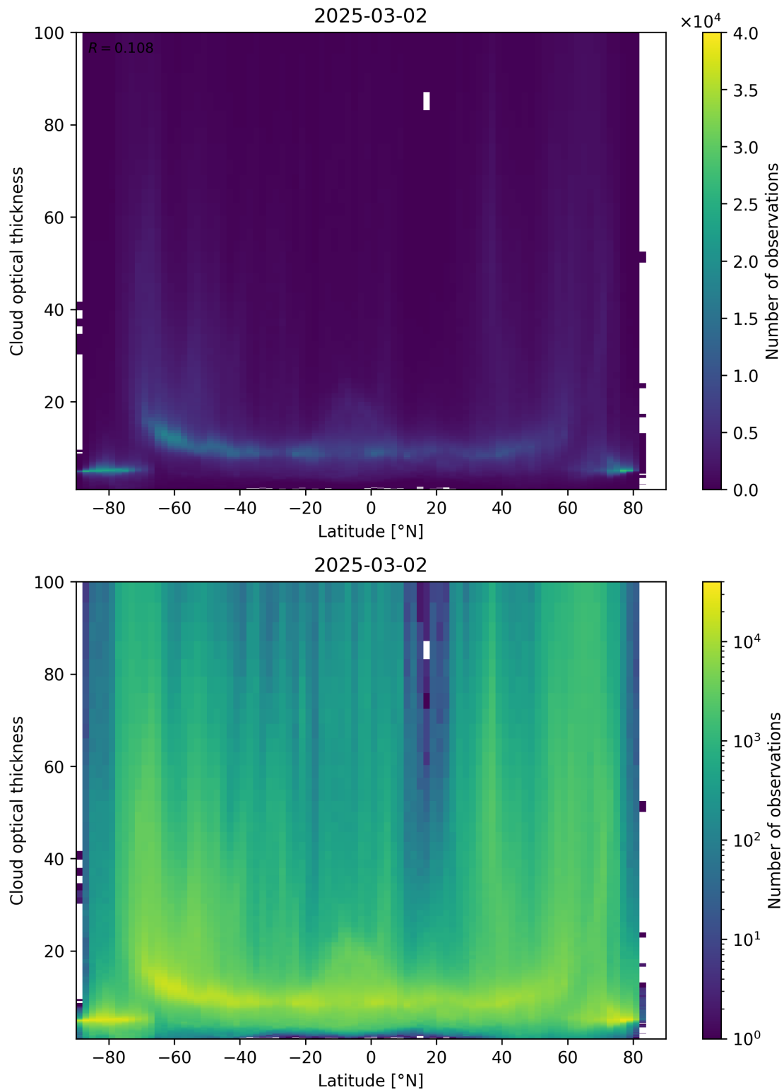
Figure 96: Scatter density plot of “Latitude” against “Cloud optical thickness” for 2025-03-01 to 2025-03-03.
