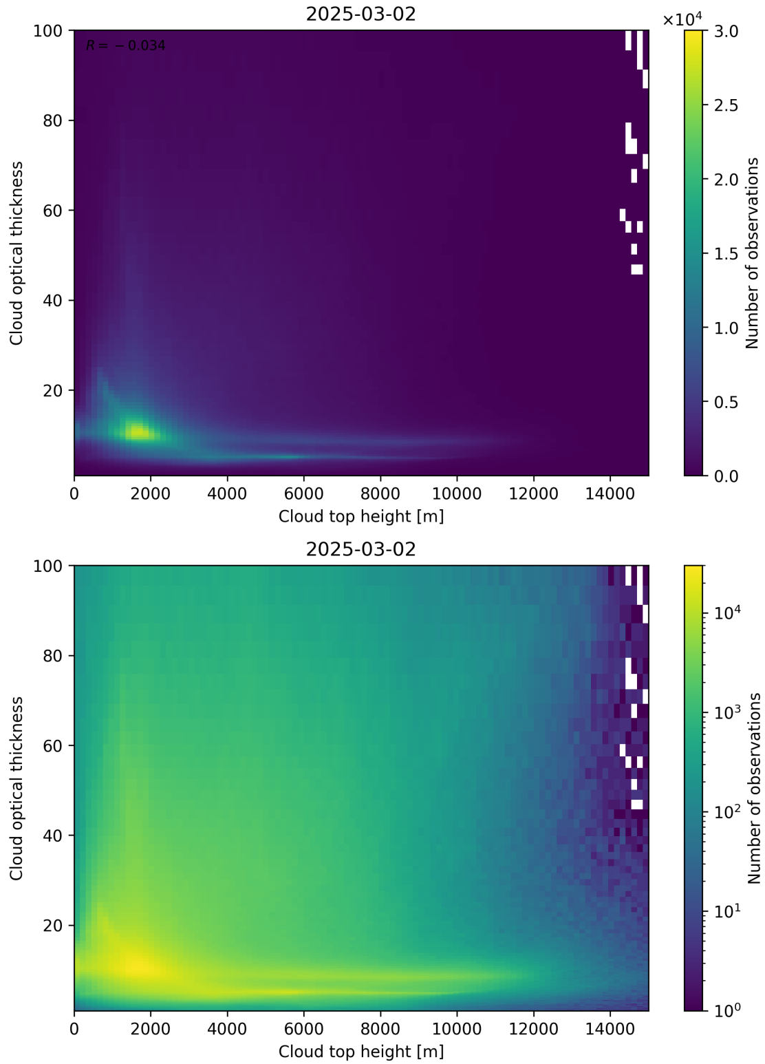
Figure 90: Scatter density plot of “Cloud top height” against “Cloud optical thickness” for 2025-03-01 to 2025-03-03.
