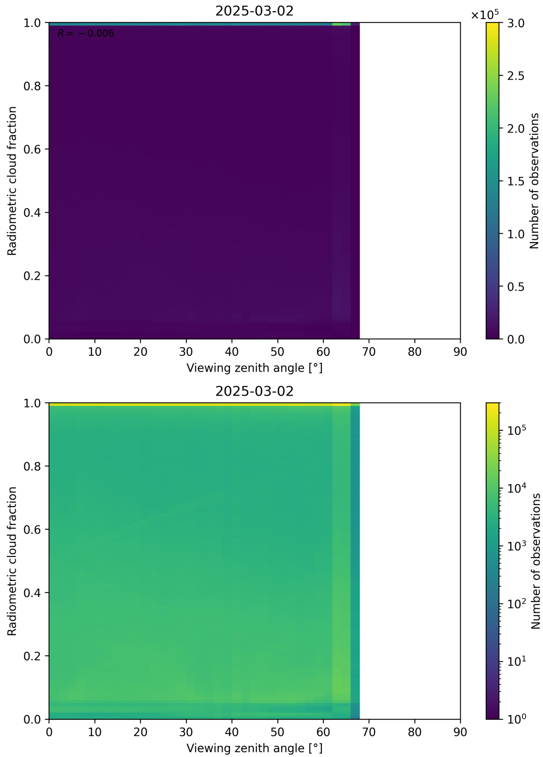
Figure 107: Scatter density plot of “Viewing zenith angle” against “Radiometric cloud fraction” for 2025-03-01 to 2025-03-03.
