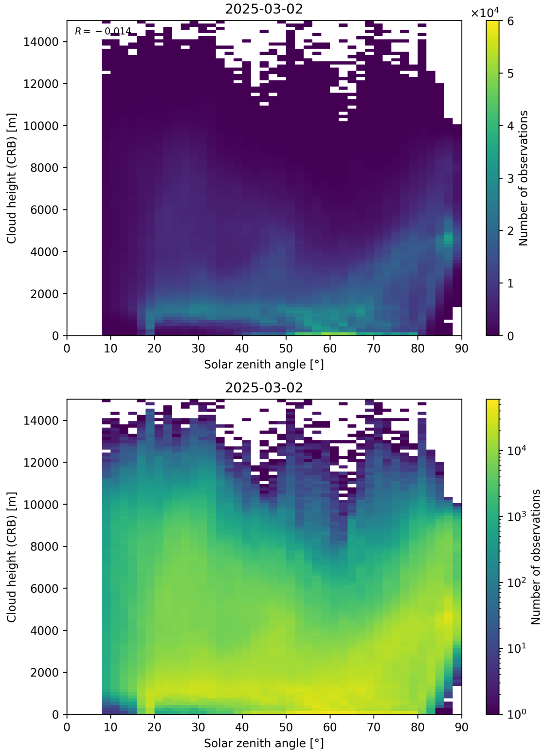
Figure 102: Scatter density plot of “Solar zenith angle” against “Cloud height (CRB)” for 2025-03-01 to 2025-03-03.
