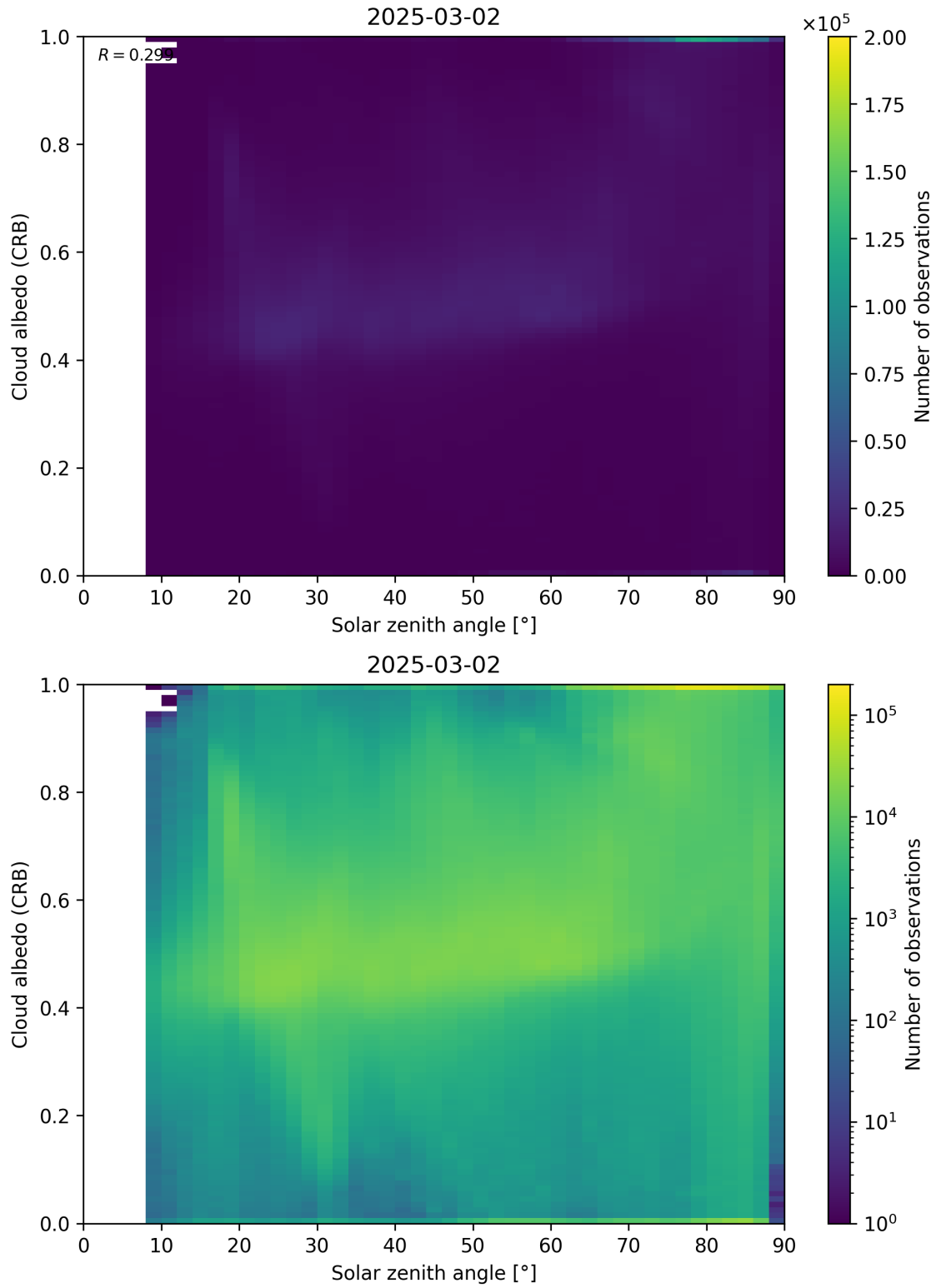
Figure 98: Scatter density plot of “Solar zenith angle” against “Cloud albedo (CRB)” for 2025-03-01 to 2025-03-03.
