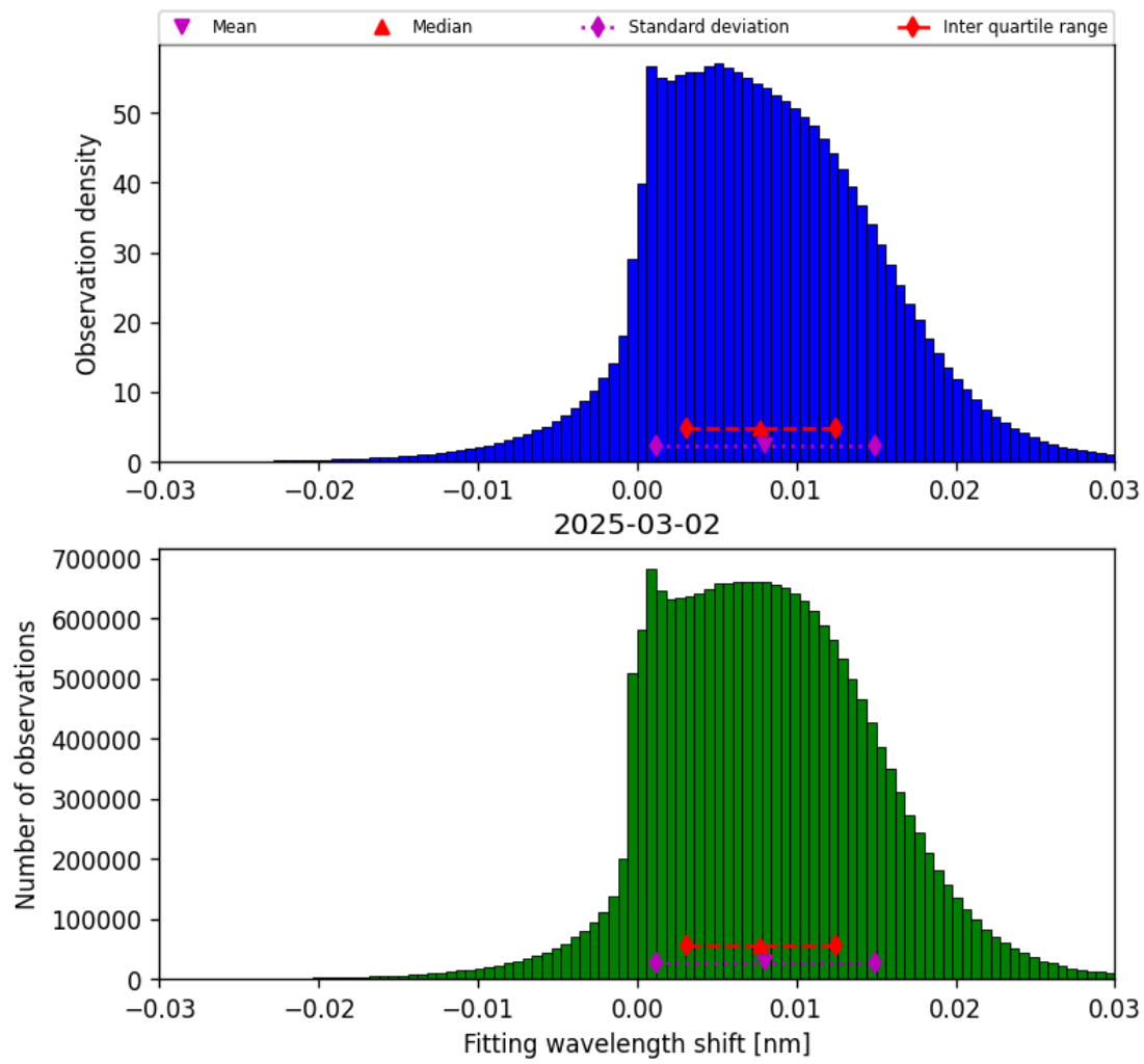
Figure 49: Histogram of “Fitting wavelength shift” for 2025-03-01 to 2025-03-03
