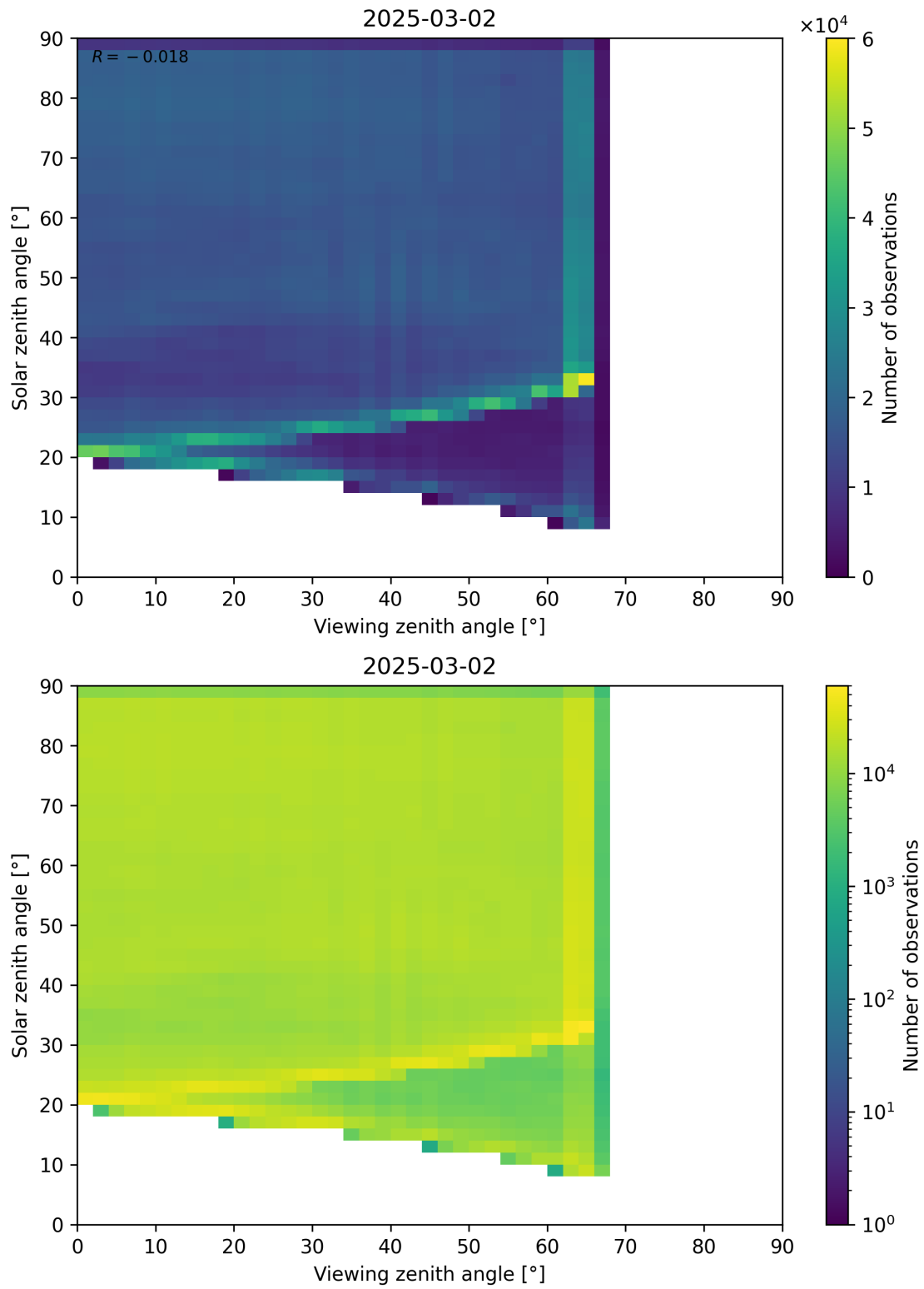
Figure 114: Scatter density plot of “Viewing zenith angle” against “Solar zenith angle” for 2025-03-01 to 2025-03-03.
