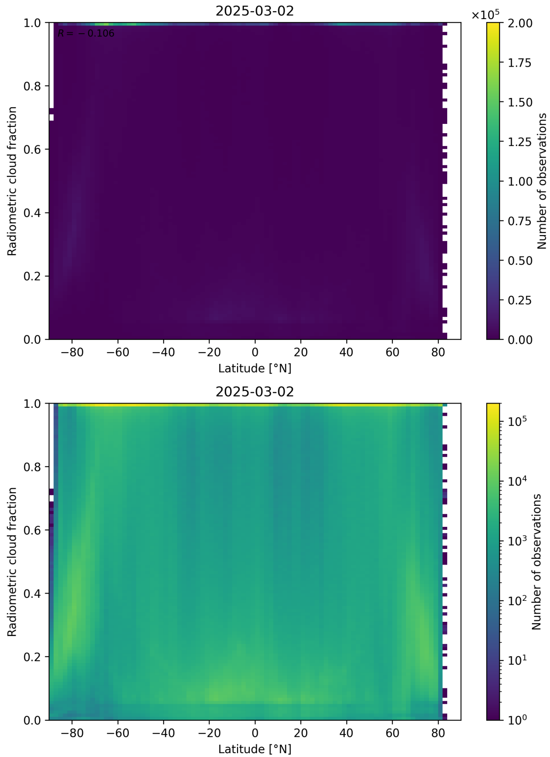
Figure 92: Scatter density plot of “Latitude” against “Radiometric cloud fraction” for 2025-03-01 to 2025-03-03.
