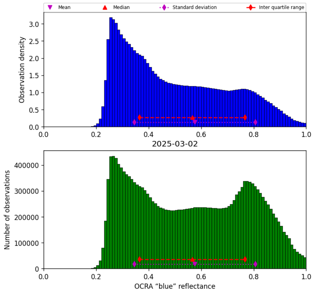
Figure 51: Histogram of “OCRA “blue” reflectance” for 2025-03-01 to 2025-03-03
