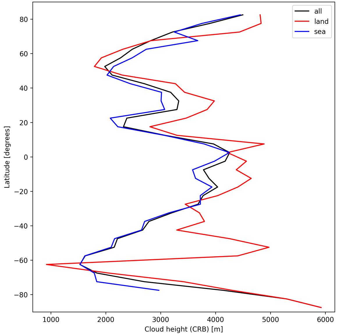
Figure 27: Zonal average of “Cloud height (CRB)” for 2025-03-01 to 2025-03-03.
