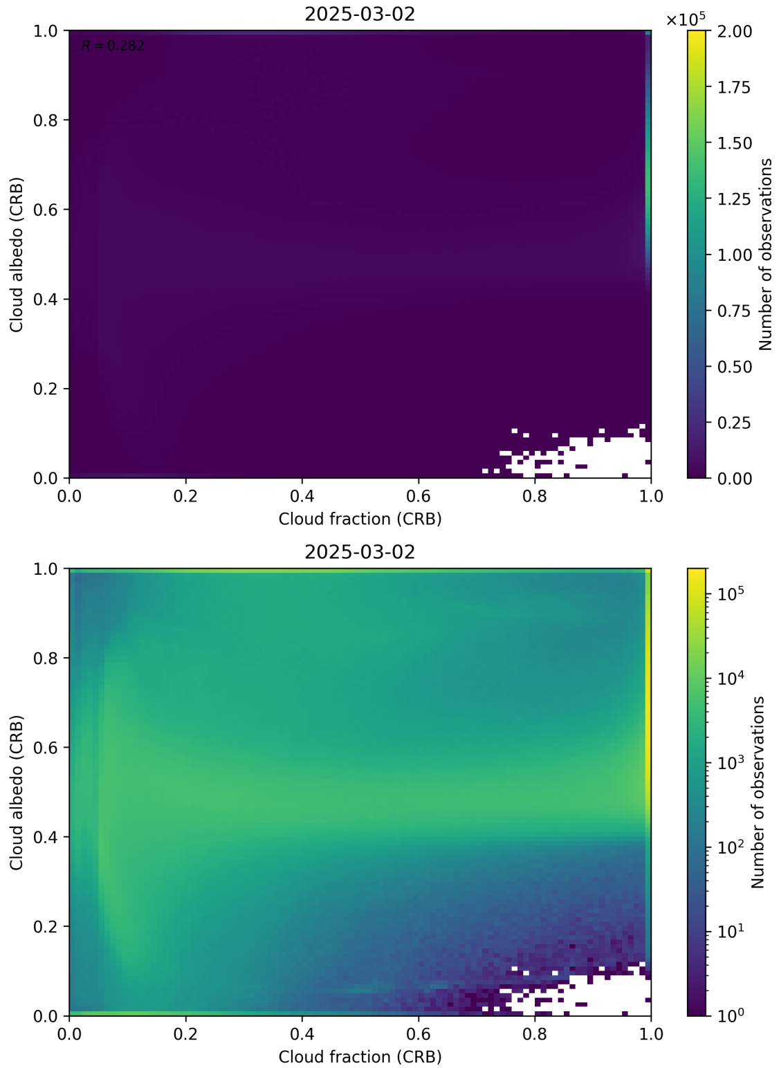
Figure 77: Scatter density plot of “Cloud fraction (CRB)” against “Cloud albedo (CRB)” for 2025-03-01 to 2025-03-03.
