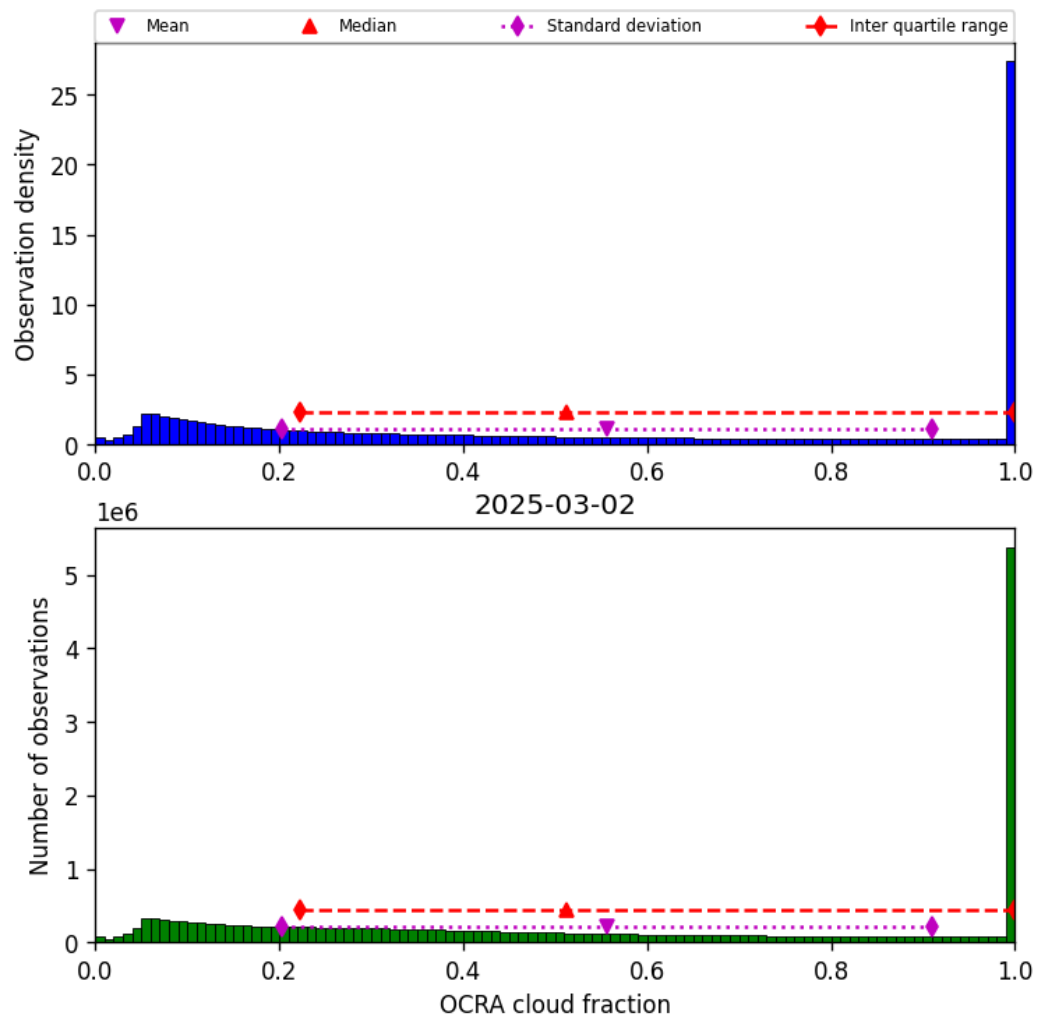
Figure 50: Histogram of “OCRA cloud fraction” for 2025-03-01 to 2025-03-03
