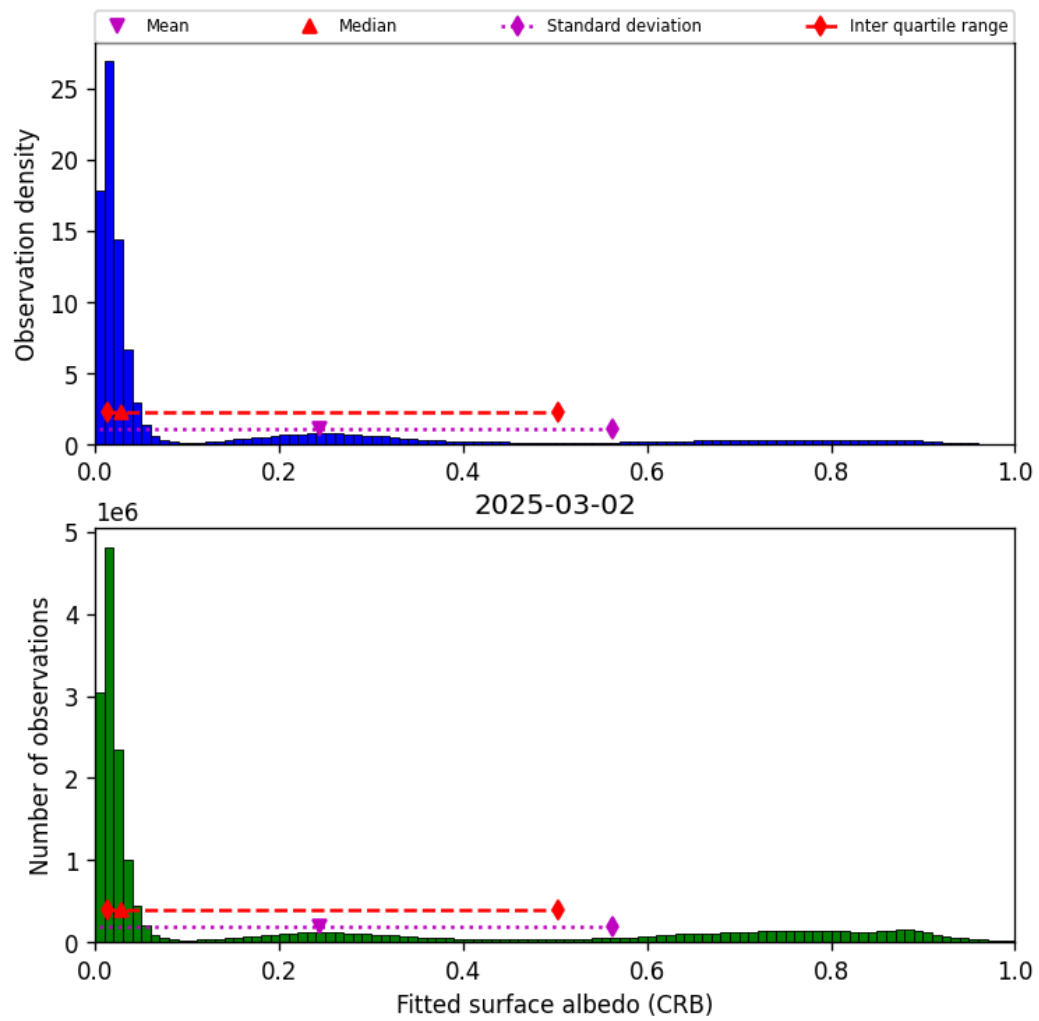
Figure 46: Histogram of “Fitted surface albedo (CRB)” for 2025-03-01 to 2025-03-03
