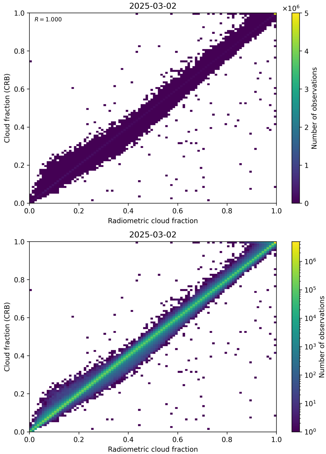
Figure 73: Scatter density plot of “Radiometric cloud fraction” against “Cloud fraction (CRB)” for 2025-03-01 to 2025-03-03.
