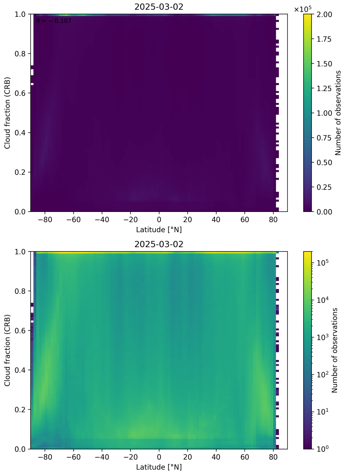
Figure 94: Scatter density plot of “Latitude” against “Cloud fraction (CRB)” for 2025-03-01 to 2025-03-03.
