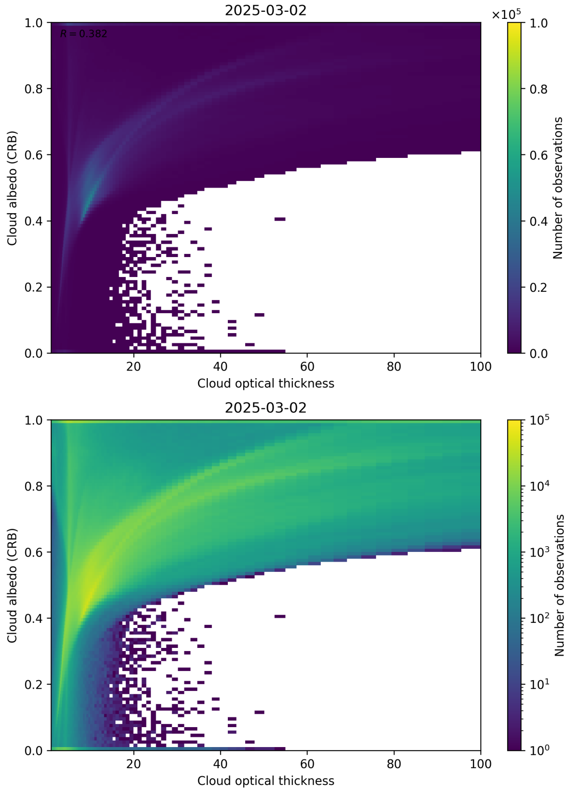
Figure 82: Scatter density plot of “Cloud optical thickness” against “Cloud albedo (CRB)” for 2025-03-01 to 2025-03-03.
