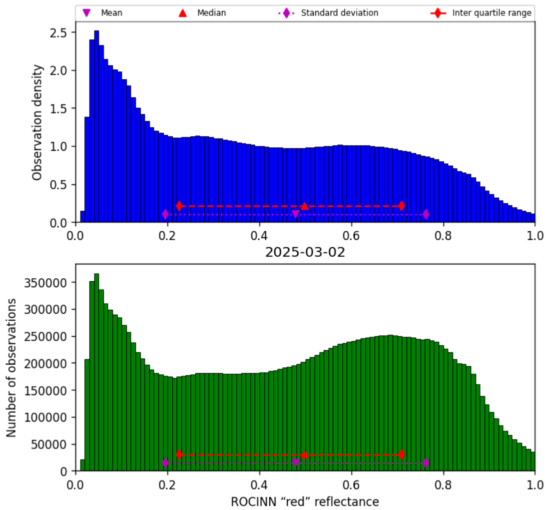
Figure 53: Histogram of “ROCINN “red” reflectance” for 2025-03-01 to 2025-03-03
