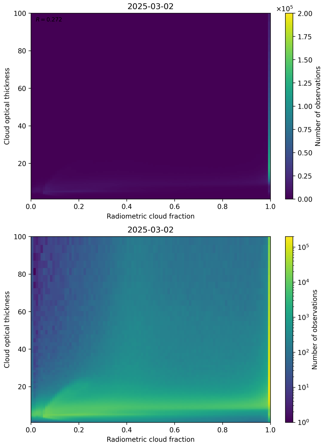
Figure 75: Scatter density plot of “Radiometric cloud fraction” against “Cloud optical thickness” for 2025-03-01 to 2025-03-03.
