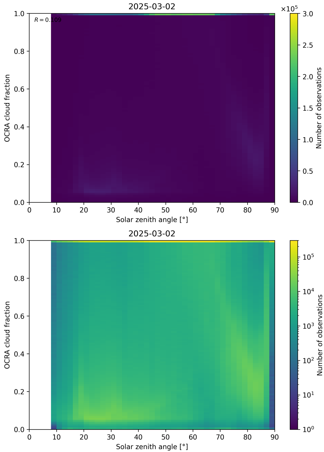
Figure 100: Scatter density plot of “Solar zenith angle” against “OCRA cloud fraction” for 2025-03-01 to 2025-03-03.
