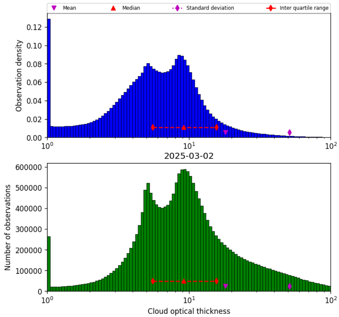
Figure 41: Histogram of “Cloud optical thickness” for 2025-03-01 to 2025-03-03
