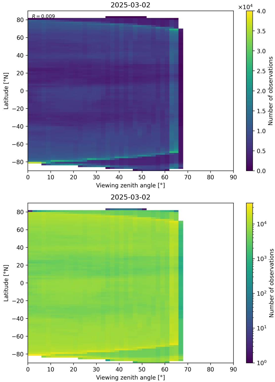
Figure 113: Scatter density plot of “Viewing zenith angle” against “Latitude” for 2025-03-01 to 2025-03-03.
