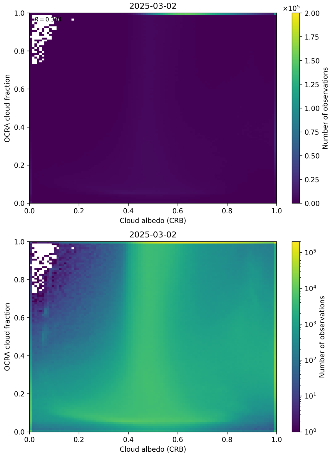
Figure 70: Scatter density plot of “Cloud albedo (CRB)” against “OCRA cloud fraction” for 2025-03-01 to 2025-03-03.
