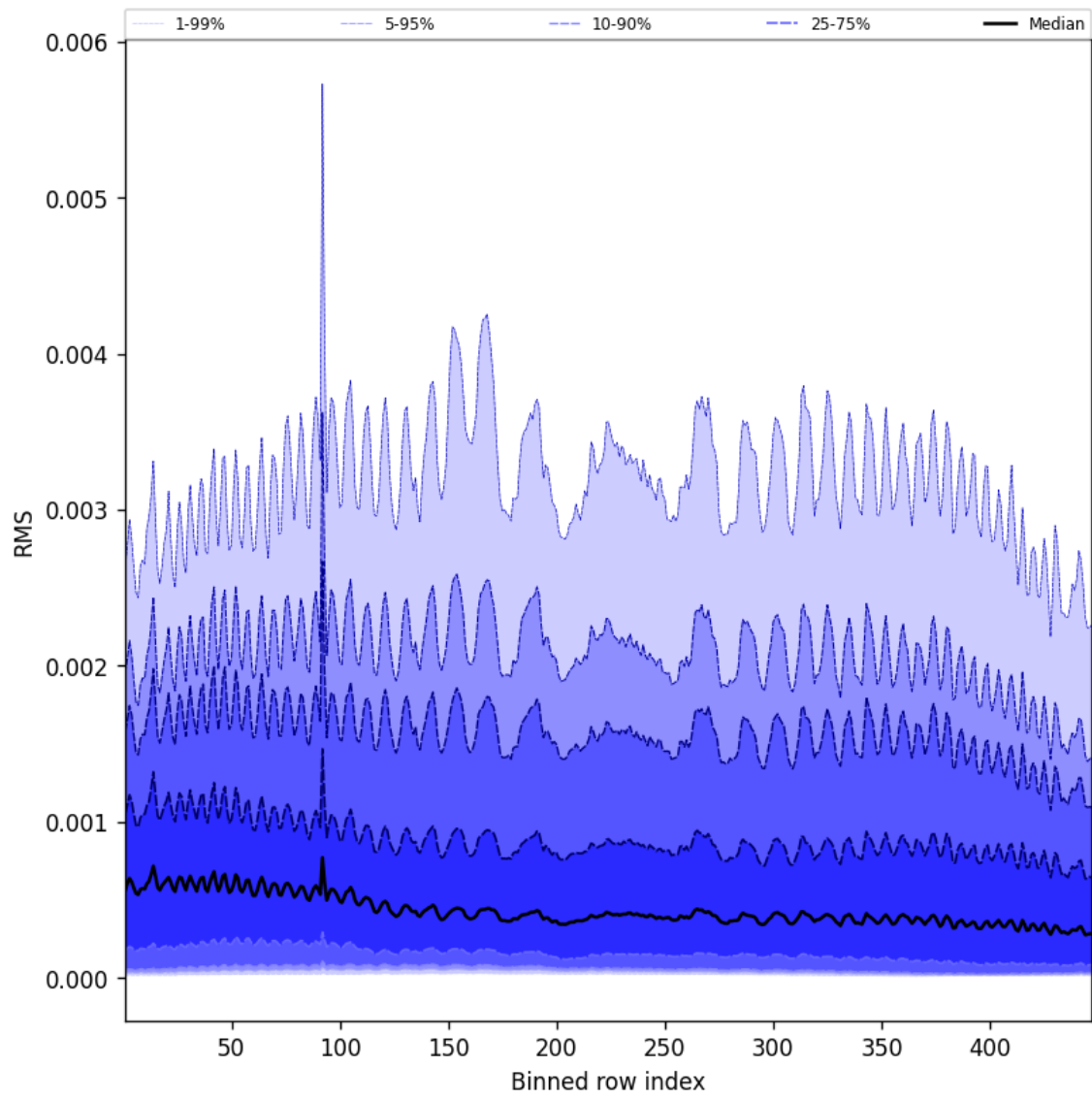
Figure 63: Along track statistics of “RMS” for 2025-03-01 to 2025-03-03
