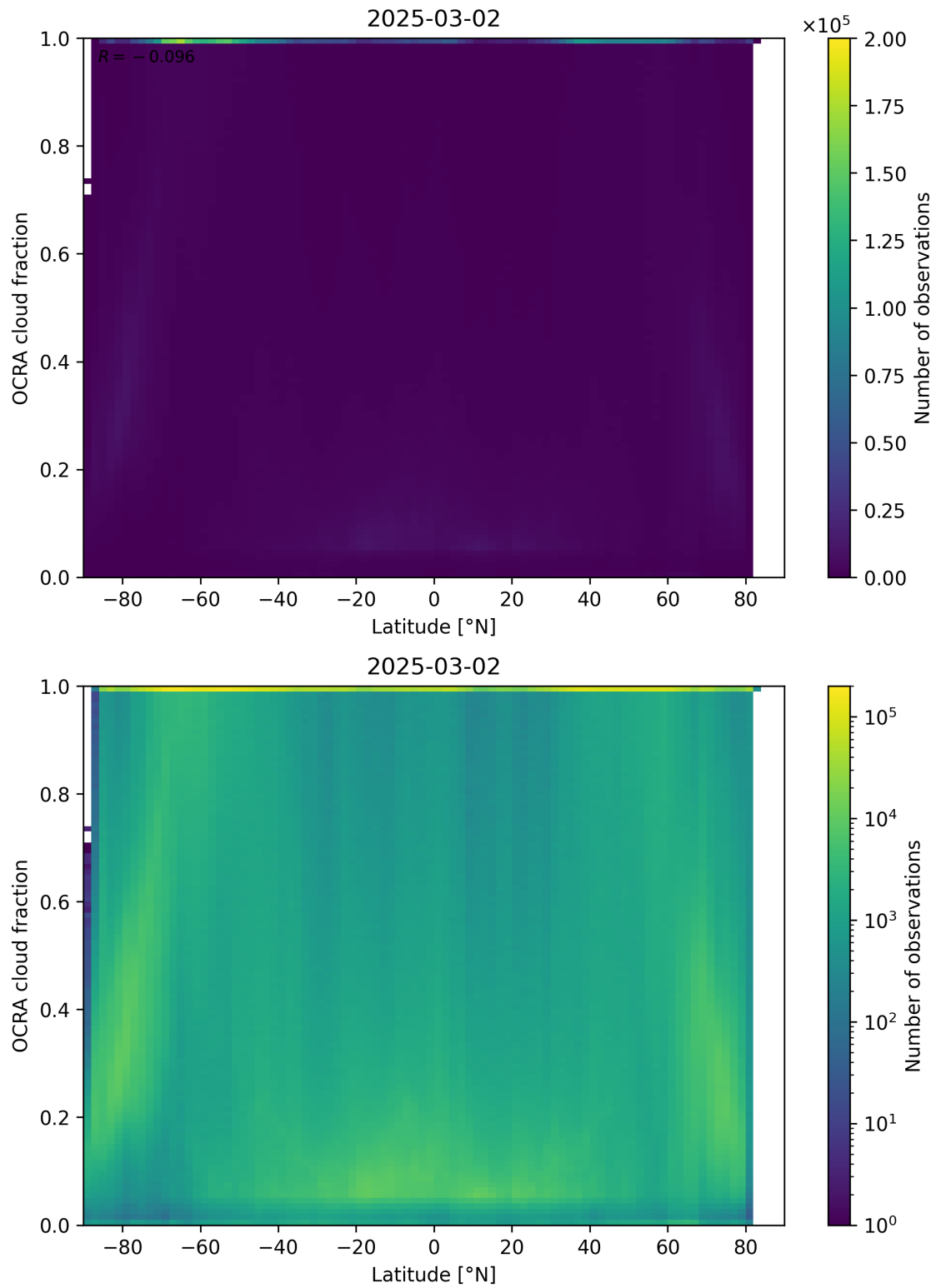
Figure 93: Scatter density plot of “Latitude” against “OCRA cloud fraction” for 2025-03-01 to 2025-03-03.
