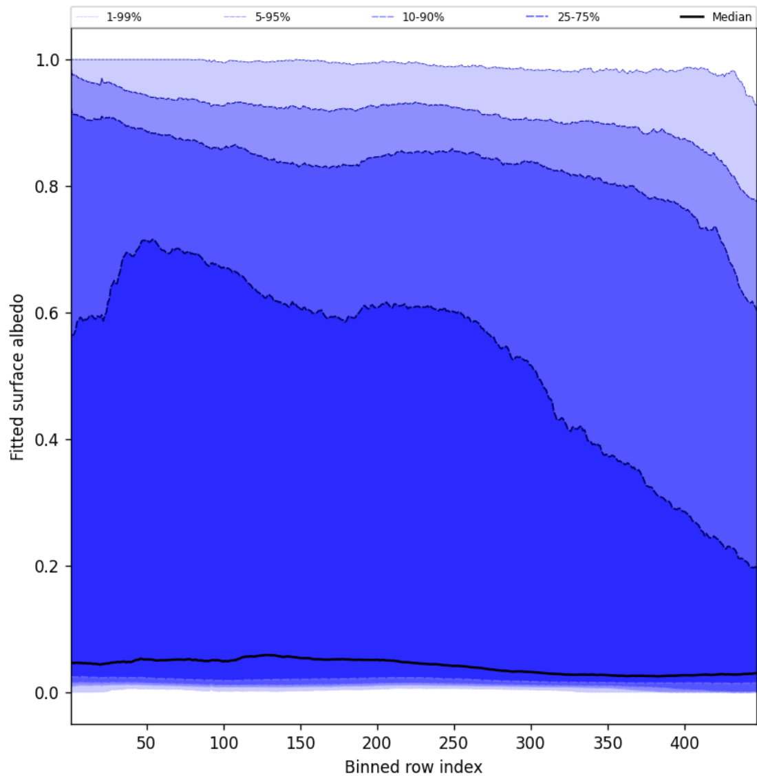
Figure 61: Along track statistics of “Fitted surface albedo” for 2025-03-01 to 2025-03-03
