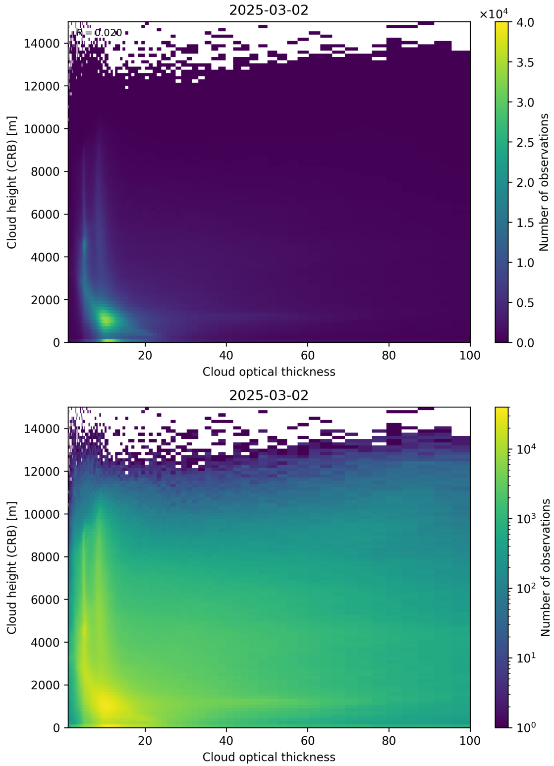
Figure 85: Scatter density plot of “Cloud optical thickness” against “Cloud height (CRB)” for 2025-03-01 to 2025-03-03.
