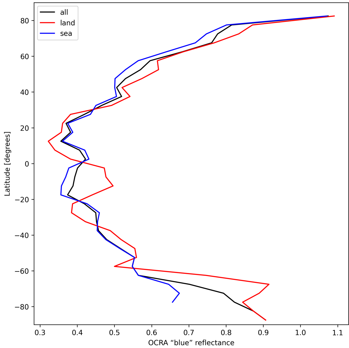
Figure 35: Zonal average of “OCRA “blue” reflectance” for 2025-03-01 to 2025-03-03.
