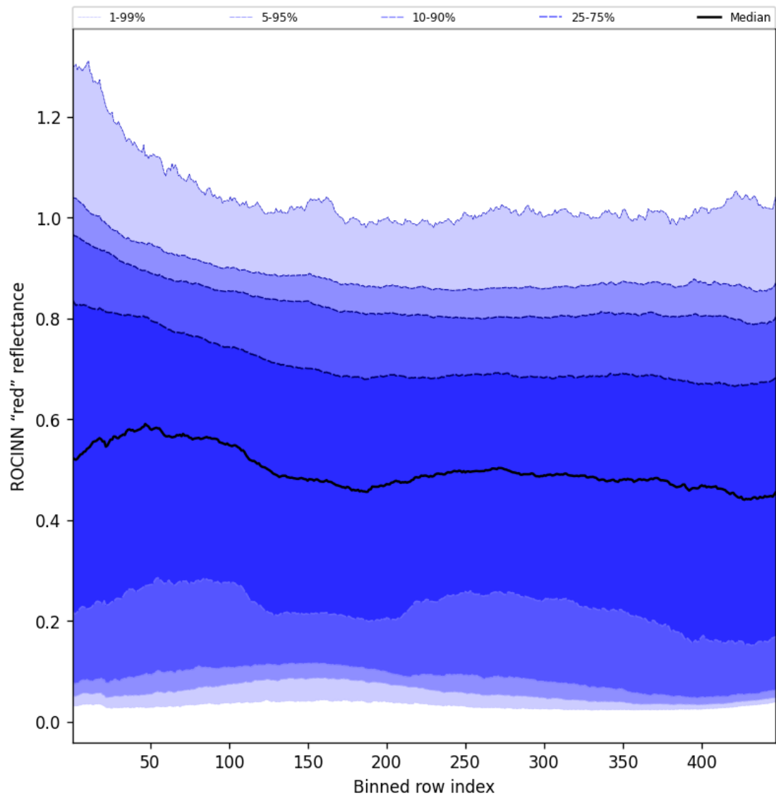
Figure 69: Along track statistics of "ROCINN "red" reflectance" for 2025-03-01 to 2025-03-03
