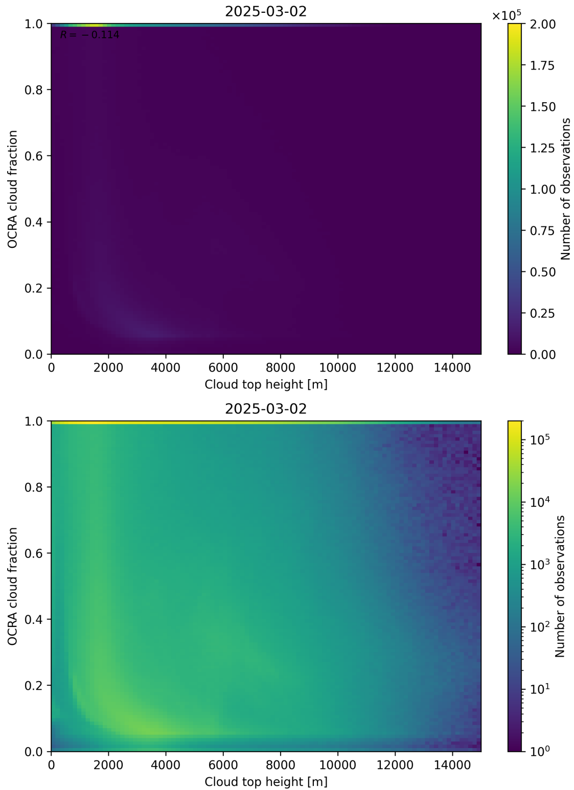
Figure 87: Scatter density plot of “Cloud top height” against “OCRA cloud fraction” for 2025-03-01 to 2025-03-03.
