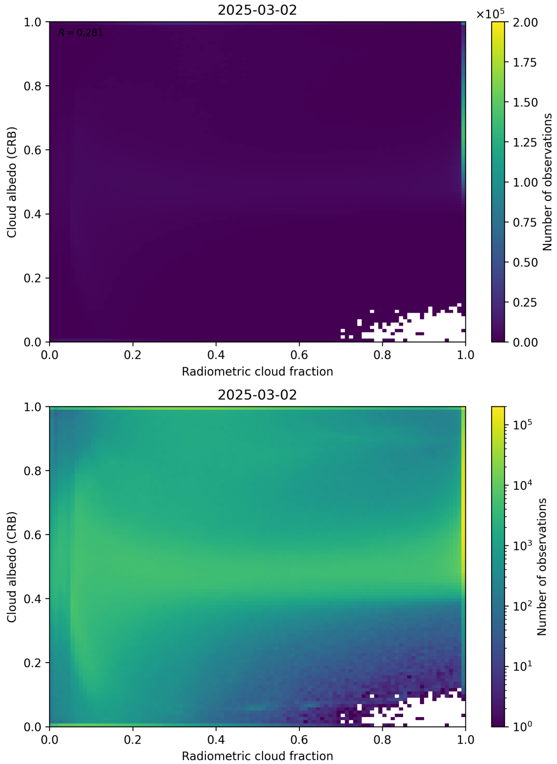
Figure 71: Scatter density plot of “Radiometric cloud fraction” against “Cloud albedo (CRB)” for 2025-03-01 to 2025-03-03.
