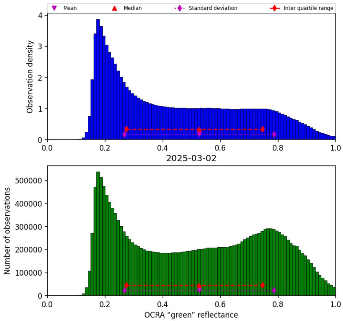
Figure 52: Histogram of “OCRA “green” reflectance” for 2025-03-01 to 2025-03-03
