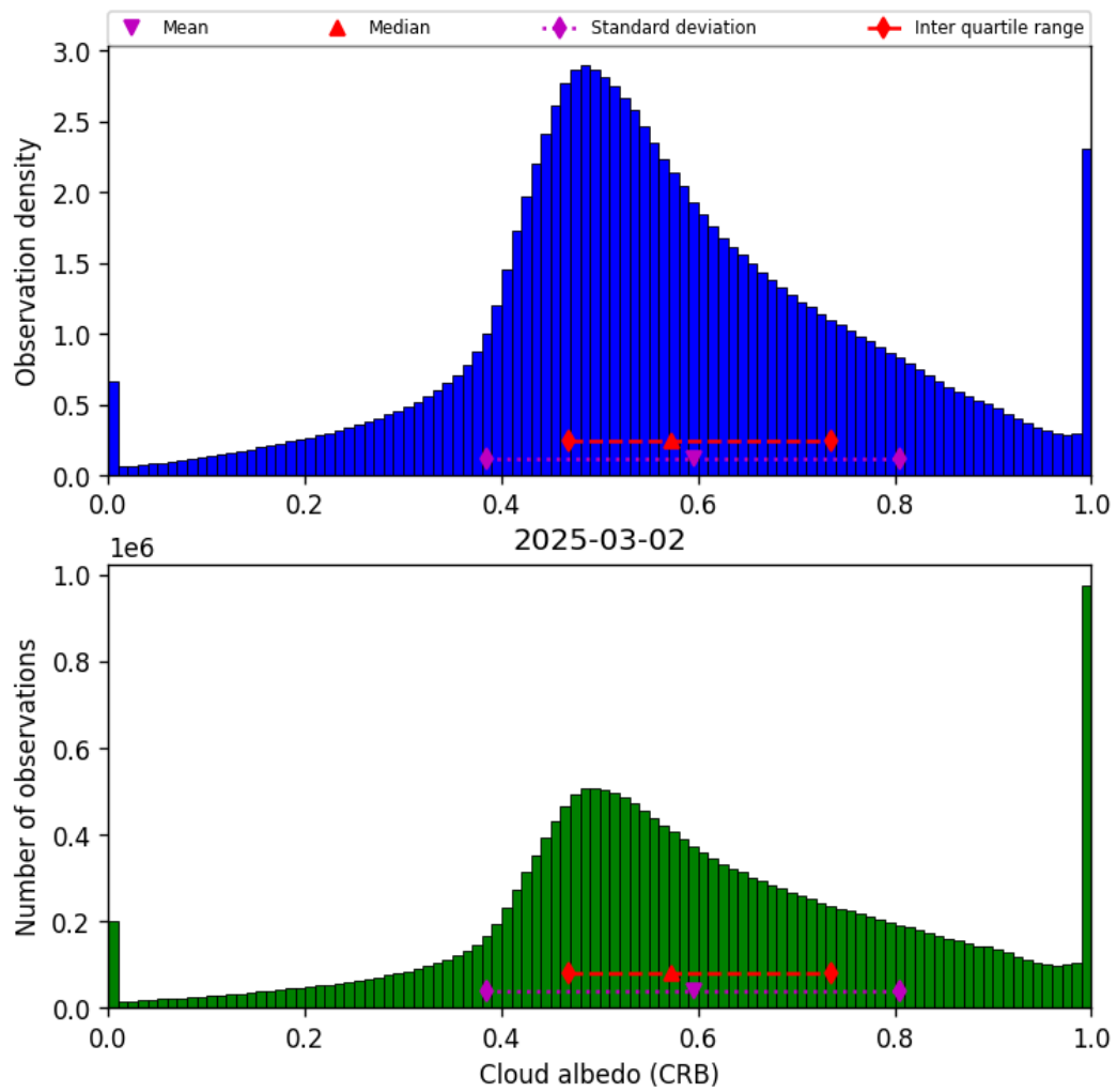
Figure 44: Histogram of “Cloud albedo (CRB)” for 2025-03-01 to 2025-03-03
