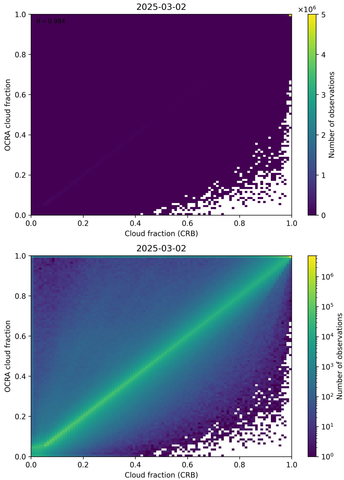
Figure 78: Scatter density plot of “Cloud fraction (CRB)” against “OCRA cloud fraction” for 2025-03-01 to 2025-03-03.
