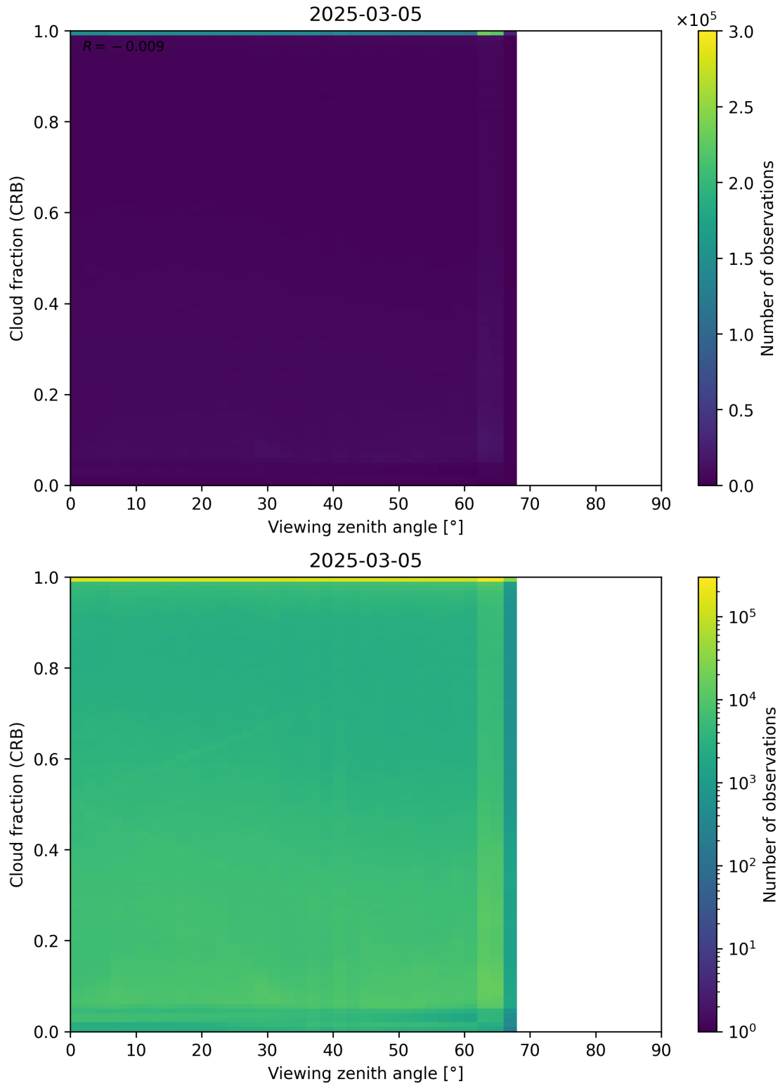
Figure 109: Scatter density plot of “Viewing zenith angle” against “Cloud fraction (CRB)” for 2025-03-04 to 2025-03-06.
