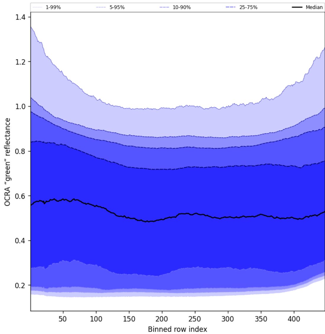
Figure 68: Along track statistics of “OCRA “green” reflectance” for 2025-03-04 to 2025-03-06
