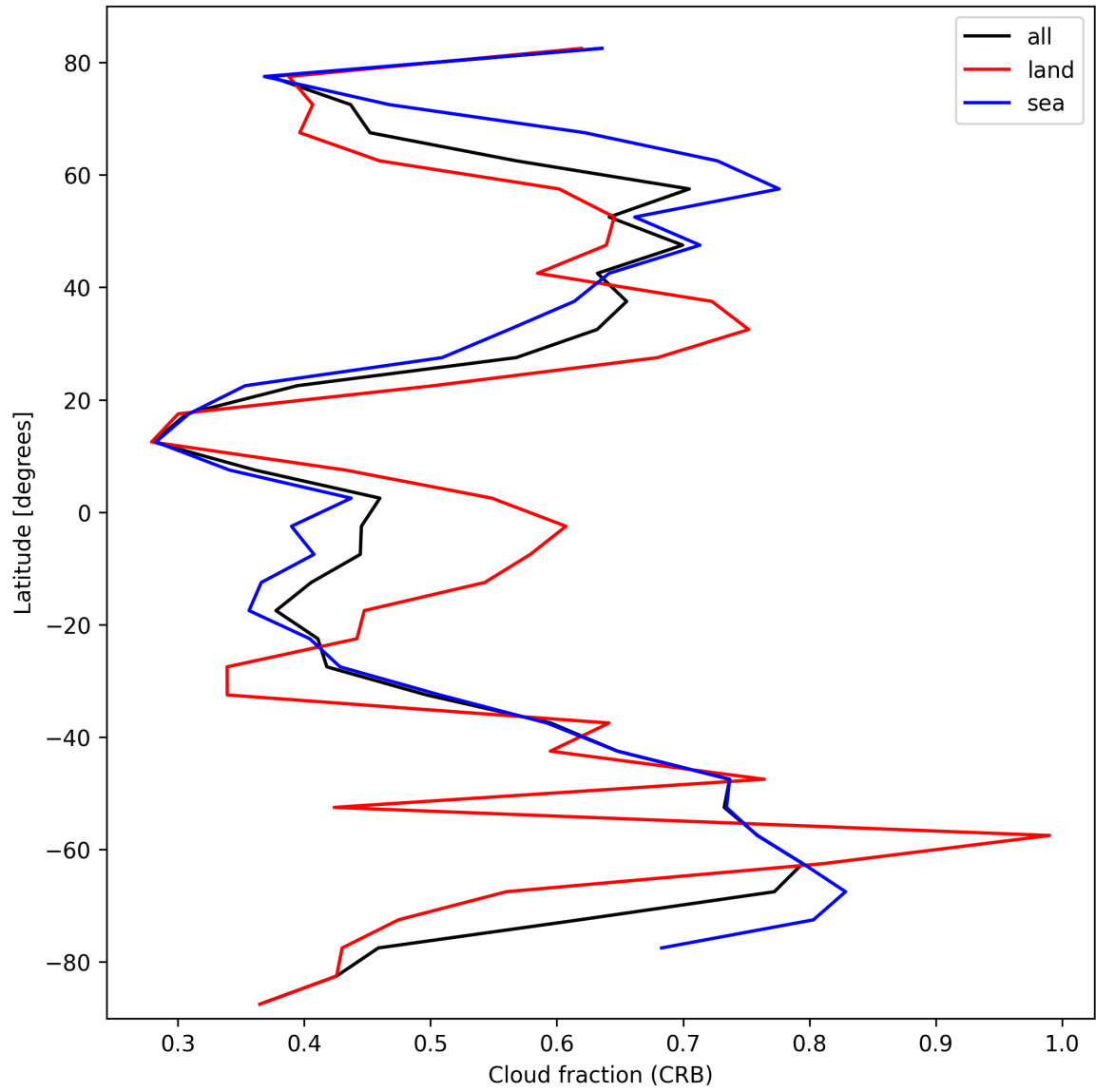
Figure 26: Zonal average of “Cloud fraction (CRB)” for 2025-03-04 to 2025-03-06.
