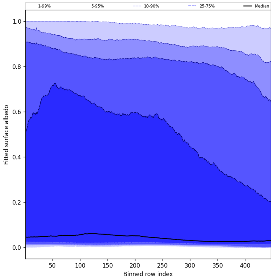
Figure 61: Along track statistics of “Fitted surface albedo” for 2025-03-04 to 2025-03-06
