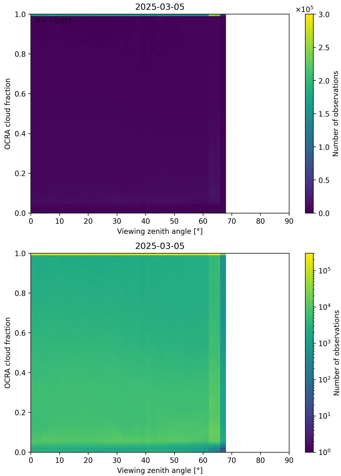
Figure 108: Scatter density plot of “Viewing zenith angle” against “OCRA cloud fraction” for 2025-03-04 to 2025-03-06.
