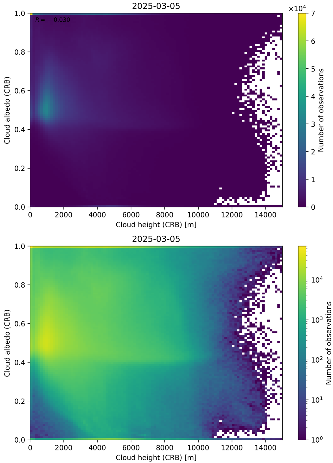
Figure 80: Scatter density plot of “Cloud height (CRB)” against “Cloud albedo (CRB)” for 2025-03-04 to 2025-03-06.
