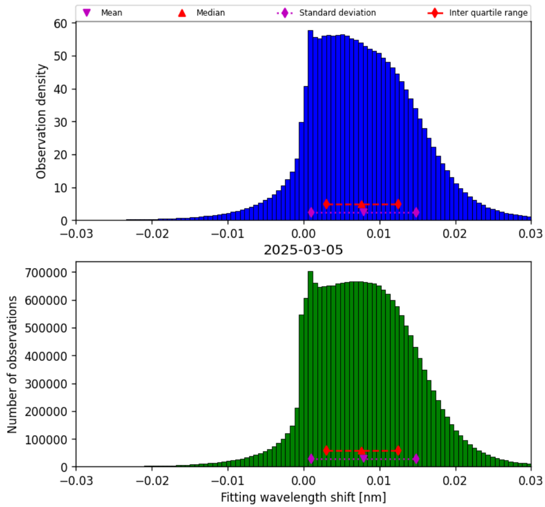
Figure 49: Histogram of “Fitting wavelength shift” for 2025-03-04 to 2025-03-06
