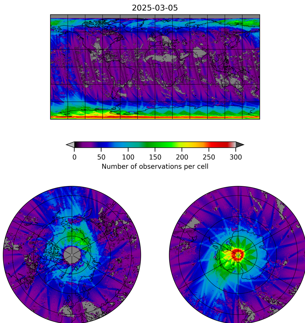
Figure 21: Map of the number of observations for 2025-03-04 to 2025-03-06
