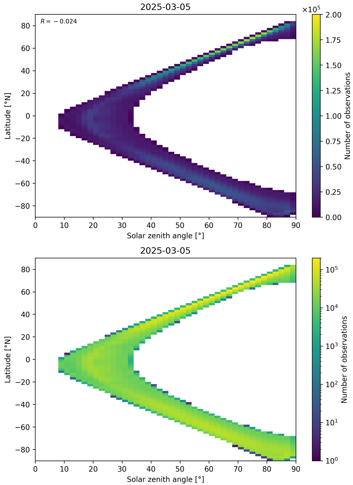
Figure 105: Scatter density plot of “Solar zenith angle” against “Latitude” for 2025-03-04 to 2025-03-06.
