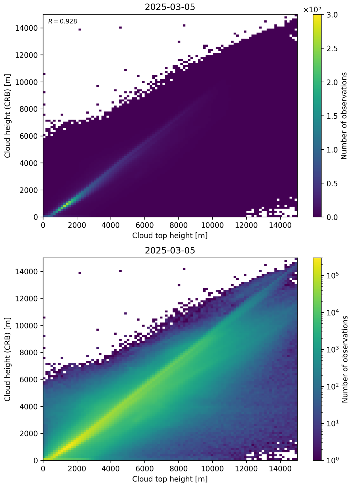
Figure 89: Scatter density plot of “Cloud top height” against “Cloud height (CRB)” for 2025-03-04 to 2025-03-06.
