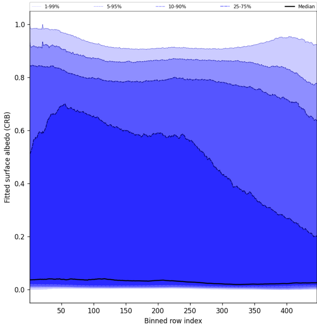
Figure 62: Along track statistics of “Fitted surface albedo (CRB)” for 2025-03-04 to 2025-03-06
