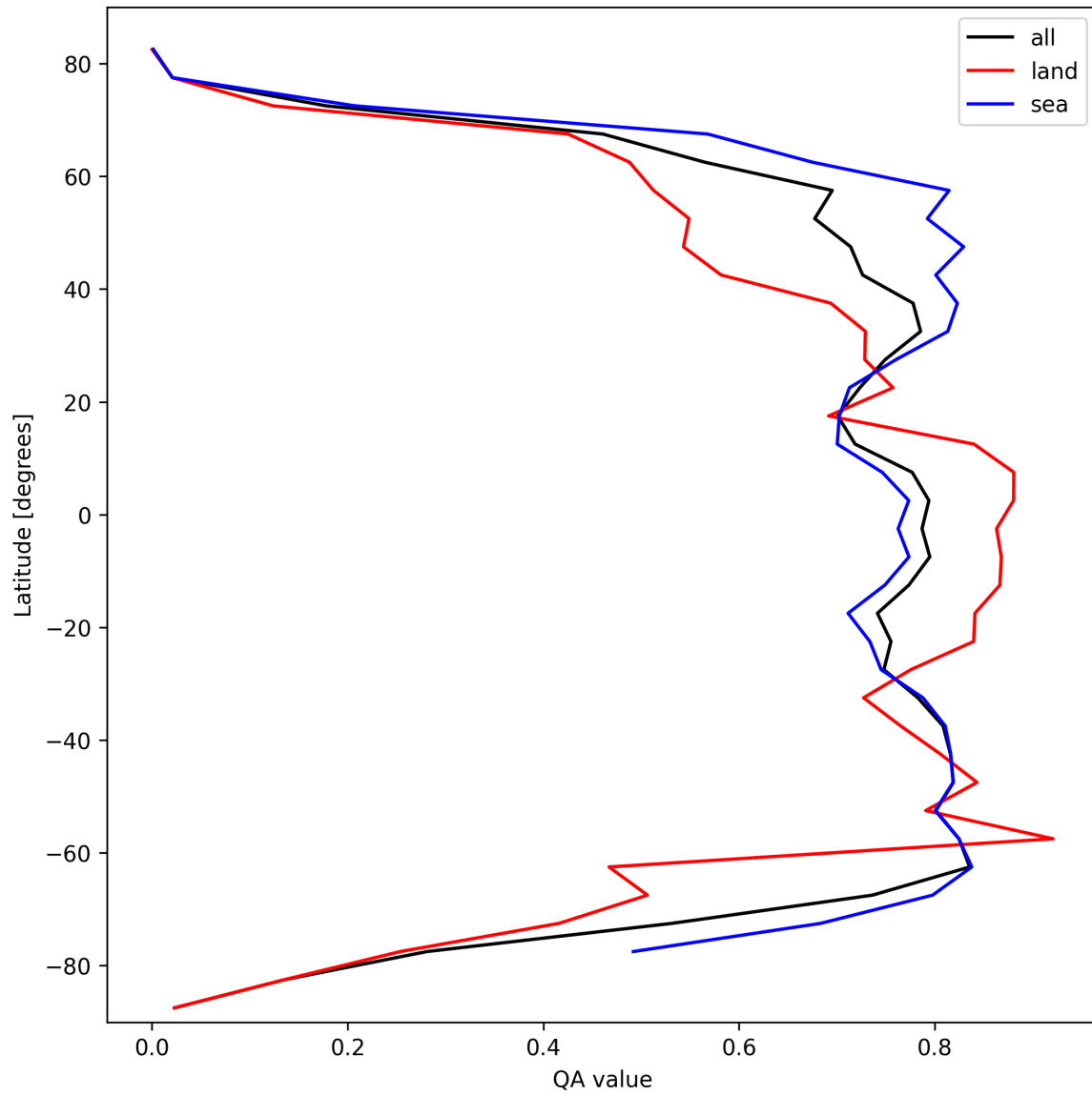
Figure 22: Zonal average of “QA value” for 2025-03-04 to 2025-03-06.
