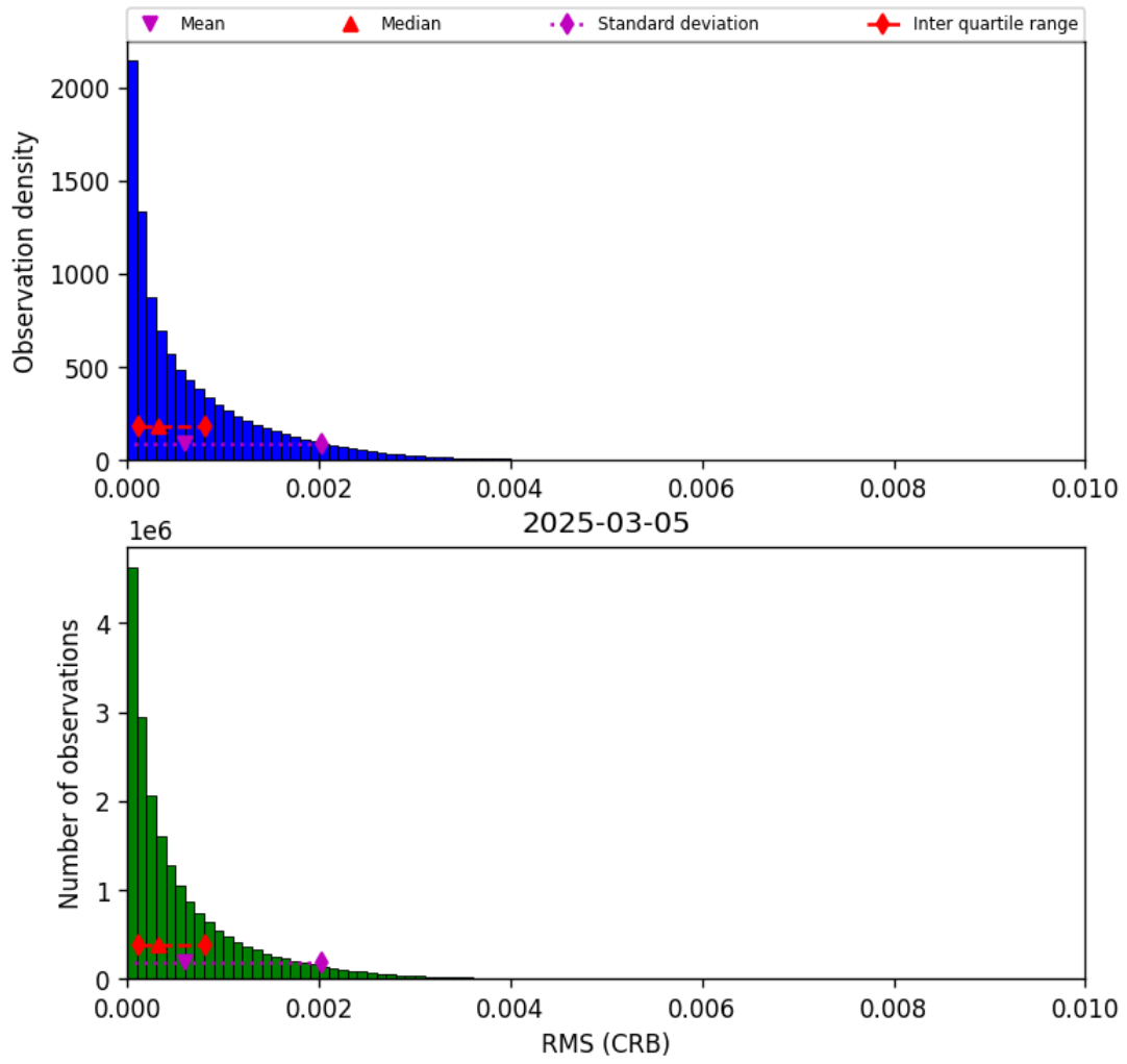
Figure 48: Histogram of “RMS (CRB)” for 2025-03-04 to 2025-03-06
