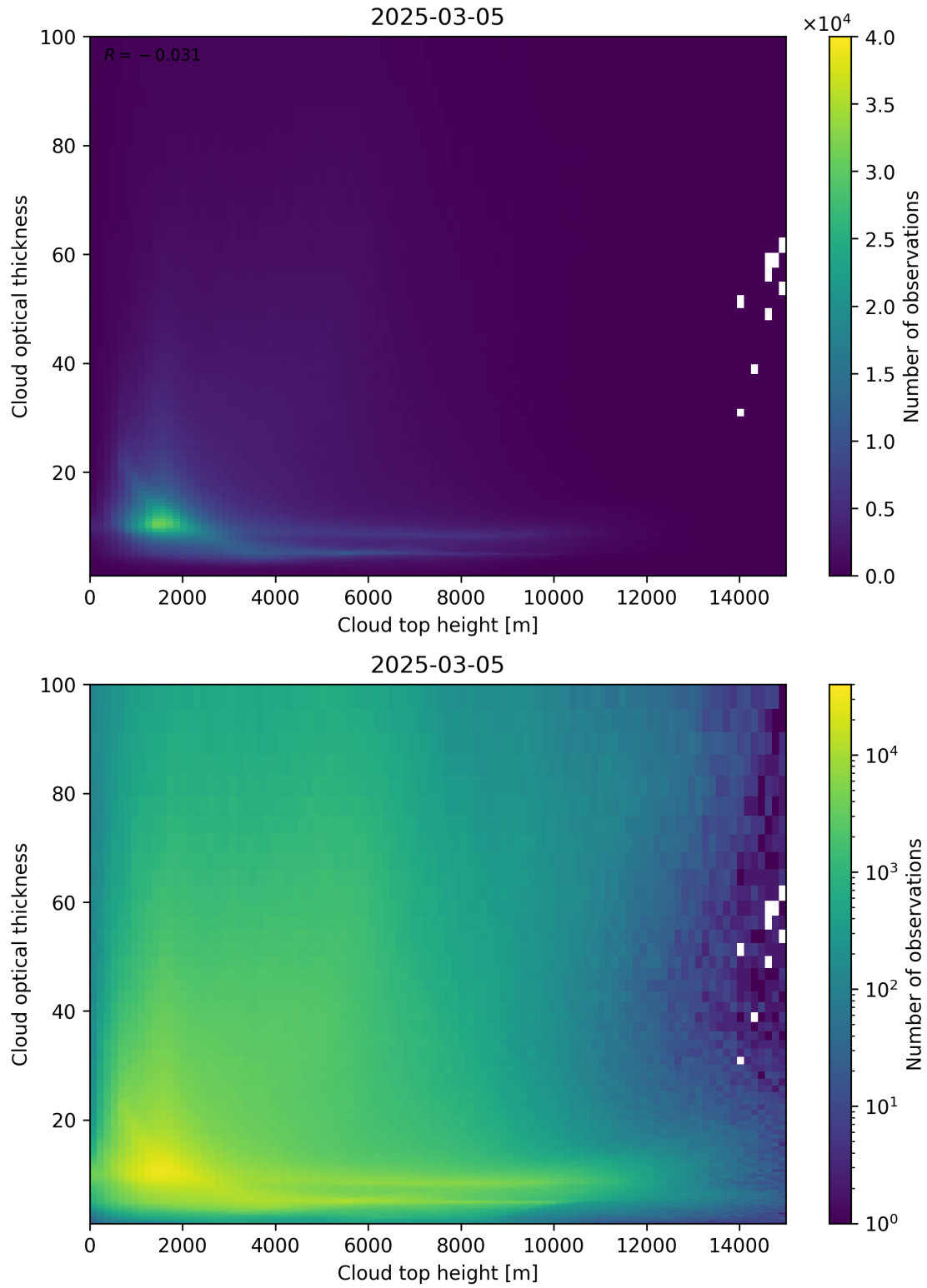
Figure 90: Scatter density plot of “Cloud top height” against “Cloud optical thickness” for 2025-03-04 to 2025-03-06.
