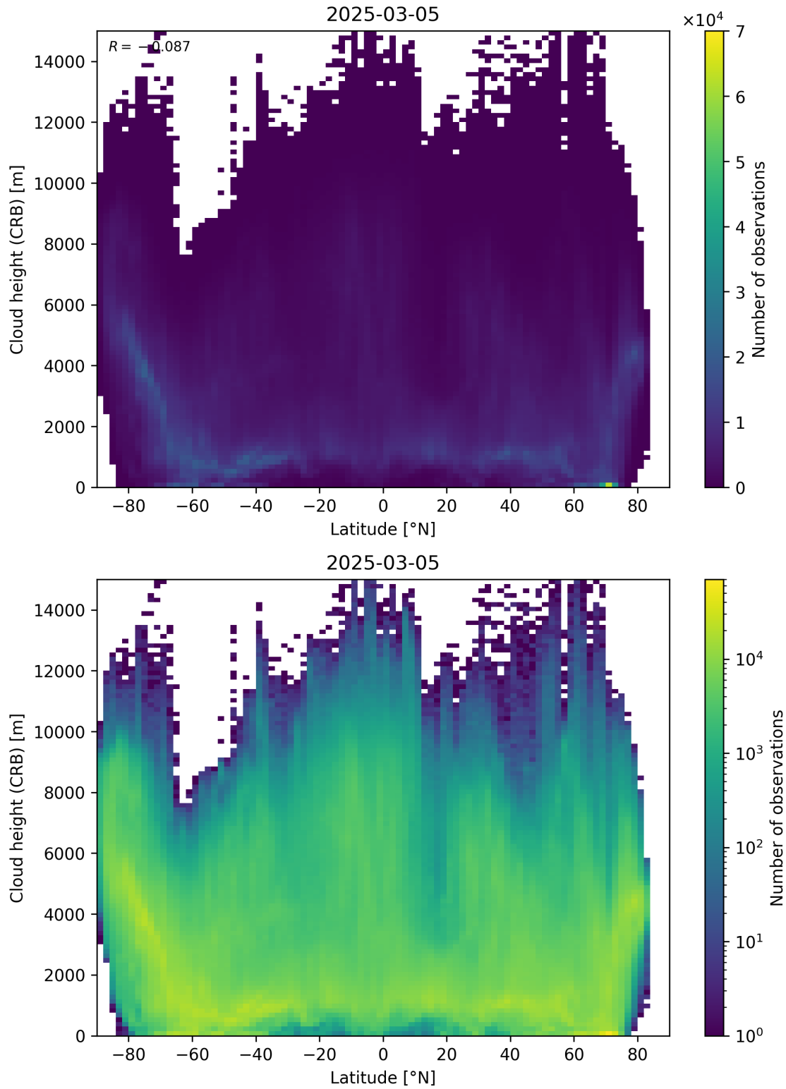
Figure 95: Scatter density plot of “Latitude” against “Cloud height (CRB)” for 2025-03-04 to 2025-03-06.
