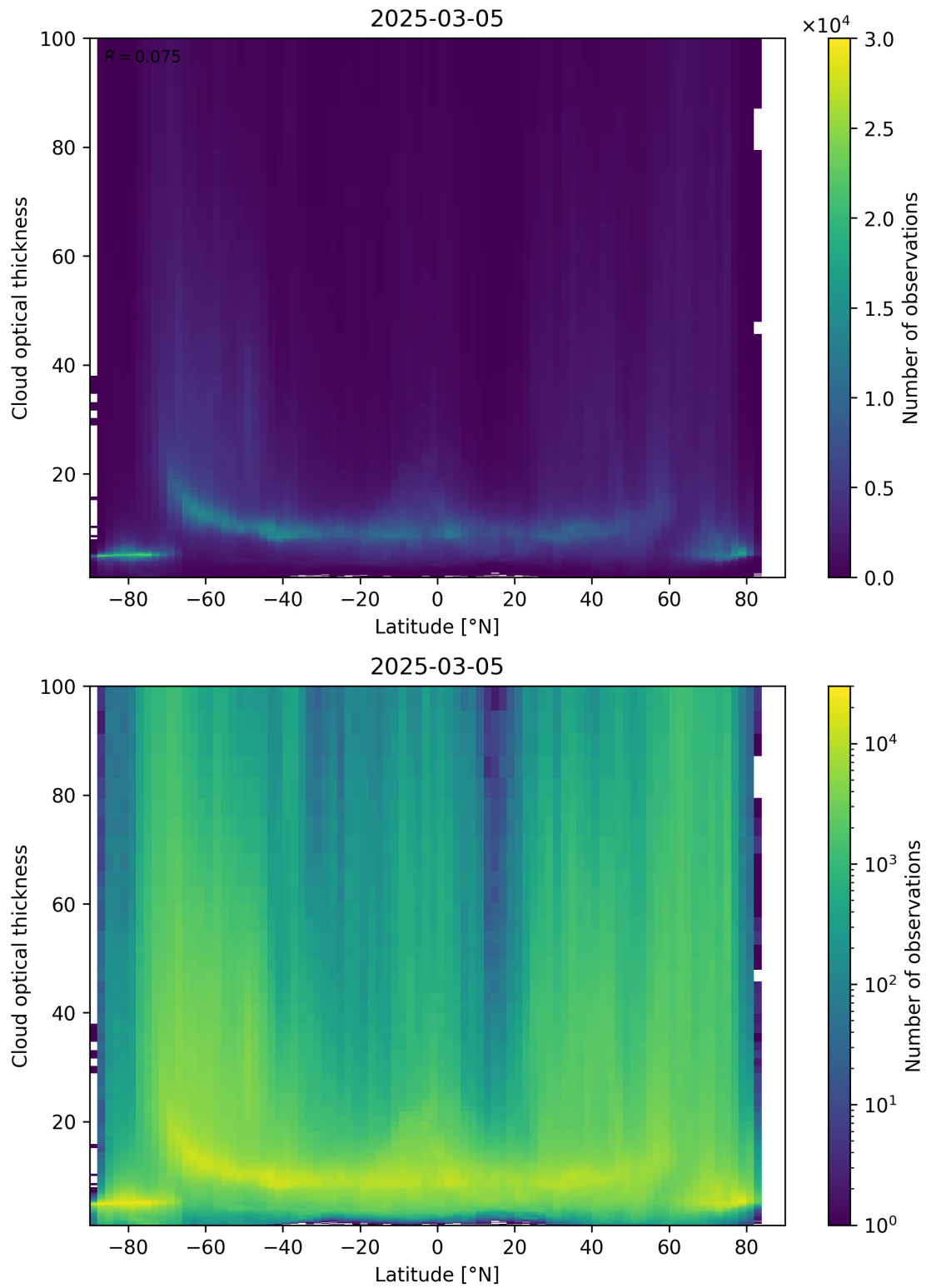
Figure 96: Scatter density plot of “Latitude” against “Cloud optical thickness” for 2025-03-04 to 2025-03-06.
