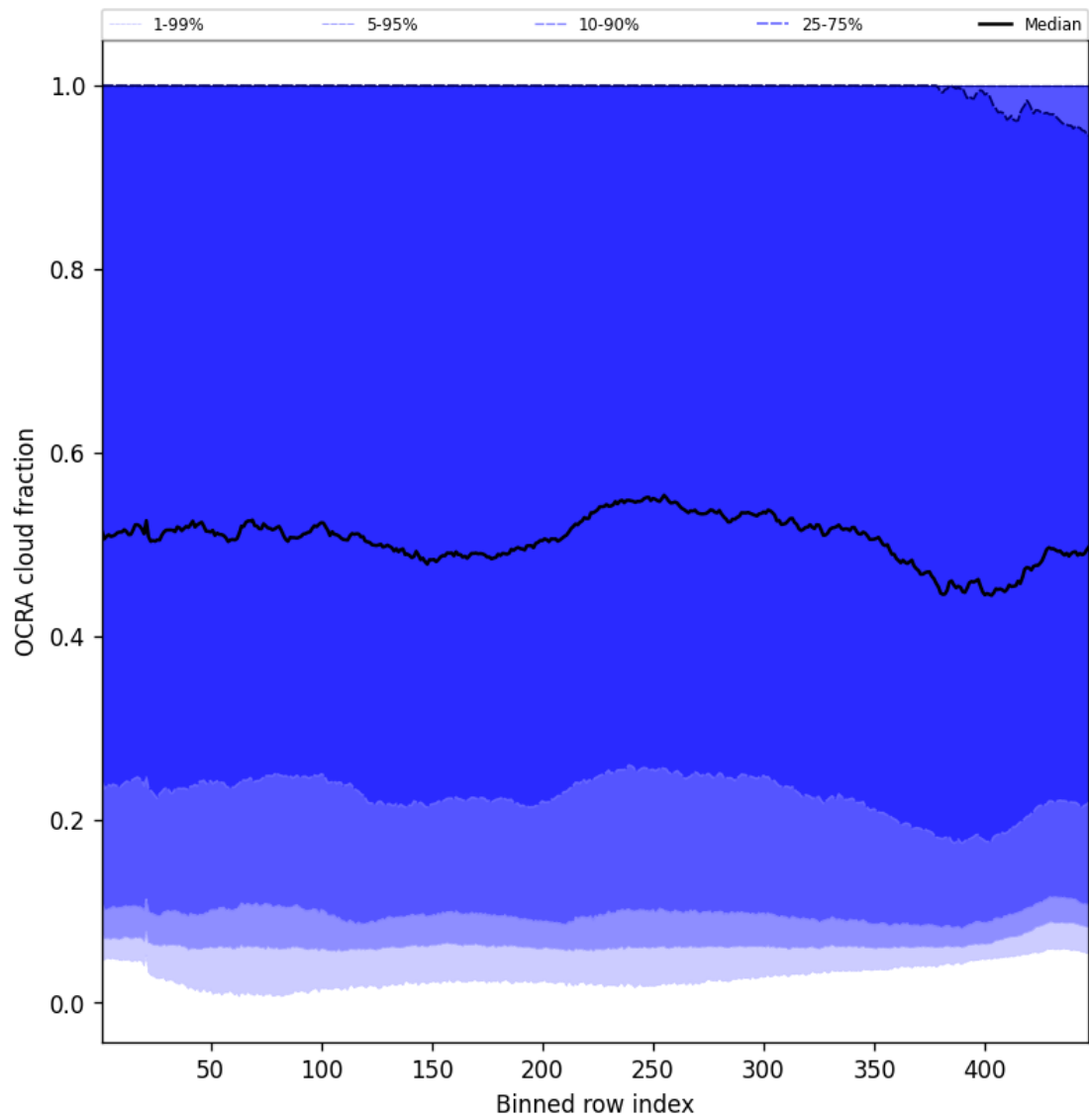
Figure 66: Along track statistics of “OCRA cloud fraction” for 2025-03-04 to 2025-03-06
