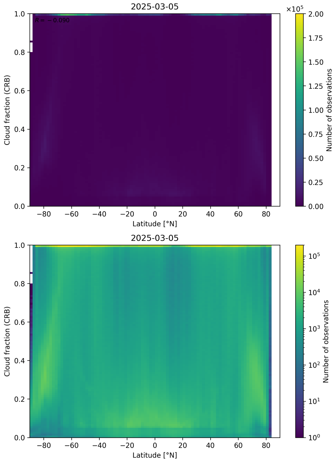
Figure 94: Scatter density plot of “Latitude” against “Cloud fraction (CRB)” for 2025-03-04 to 2025-03-06.
