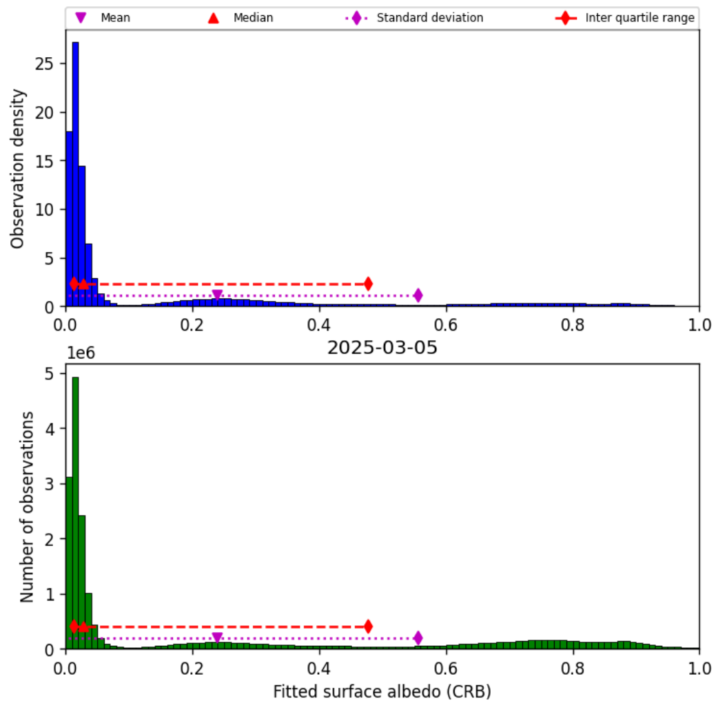
Figure 46: Histogram of “Fitted surface albedo (CRB)” for 2025-03-04 to 2025-03-06
