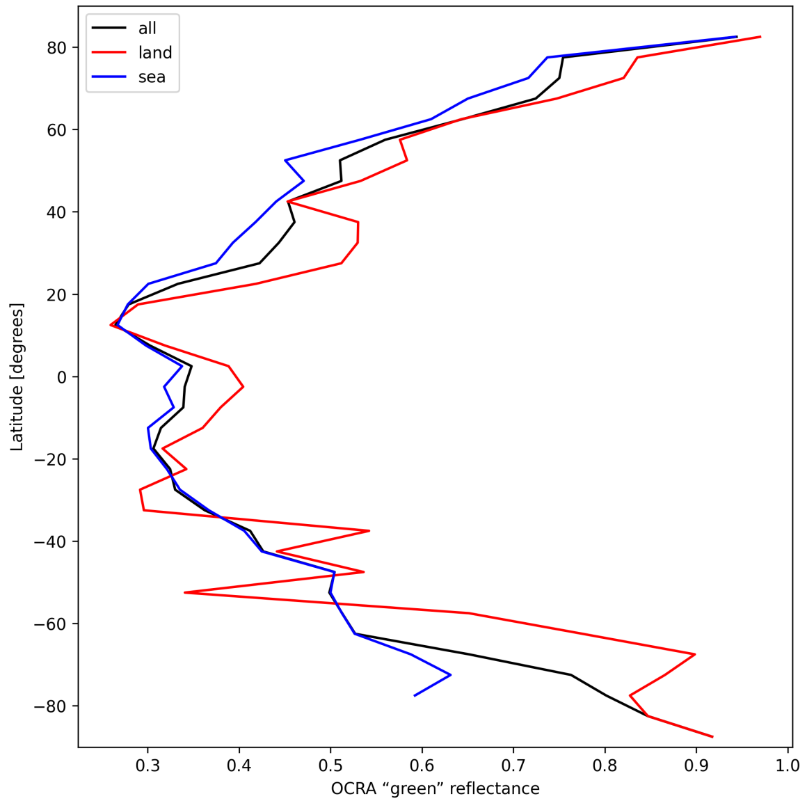
Figure 36: Zonal average of “OCRA “green” reflectance” for 2025-03-04 to 2025-03-06.
