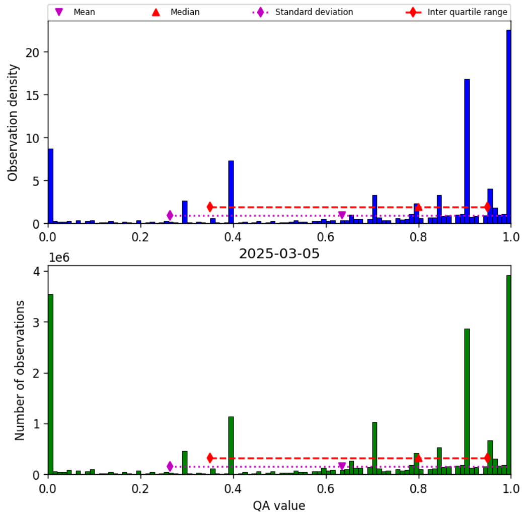
Figure 38: Histogram of “QA value” for 2025-03-04 to 2025-03-06
