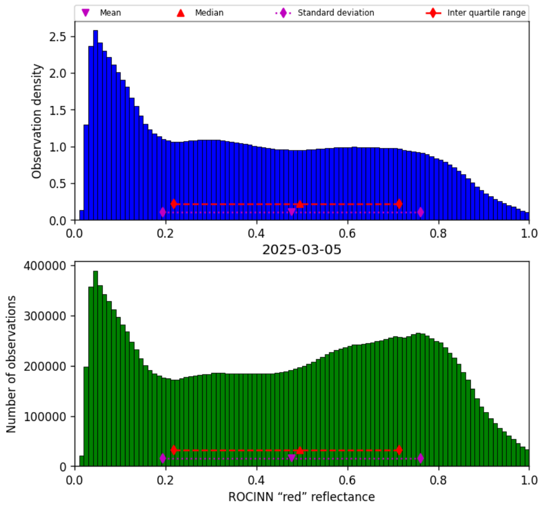
Figure 53: Histogram of “ROCINN “red” reflectance” for 2025-03-04 to 2025-03-06
