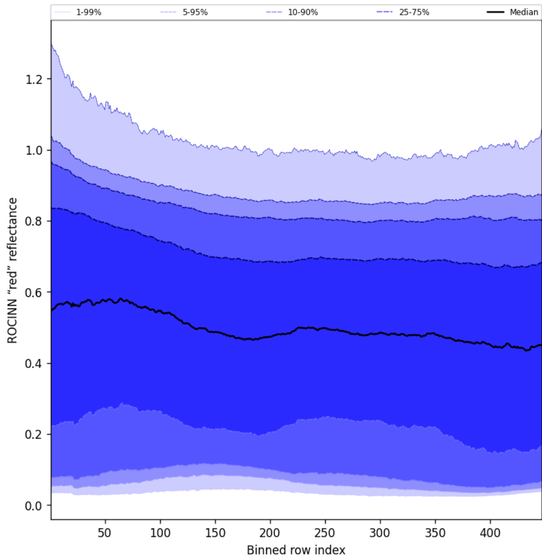
Figure 69: Along track statistics of “ROCINN “red” reflectance” for 2025-03-04 to 2025-03-06
