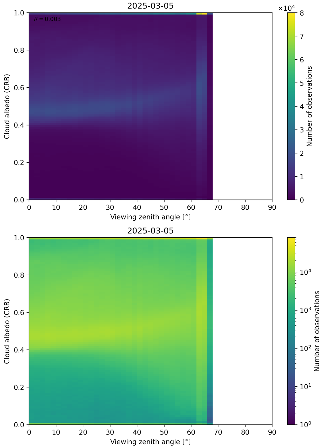
Figure 106: Scatter density plot of “Viewing zenith angle” against “Cloud albedo (CRB)” for 2025-03-04 to 2025-03-06.
