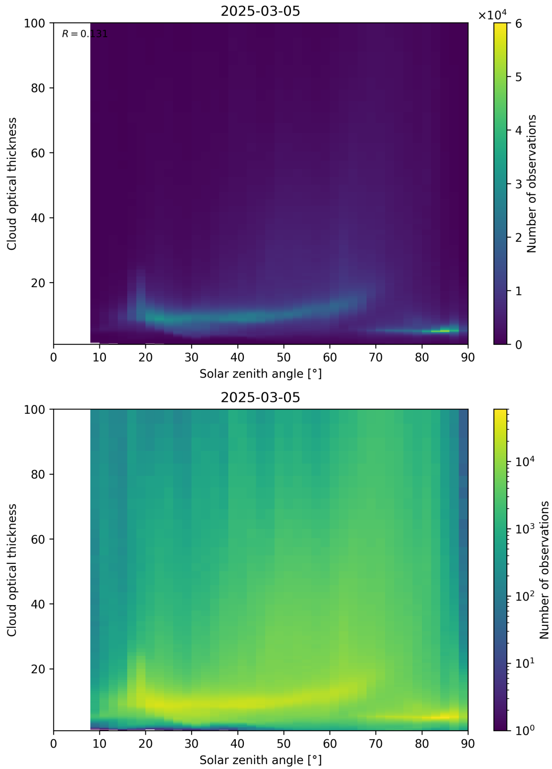
Figure 103: Scatter density plot of “Solar zenith angle” against “Cloud optical thickness” for 2025-03-04 to 2025-03-06.
