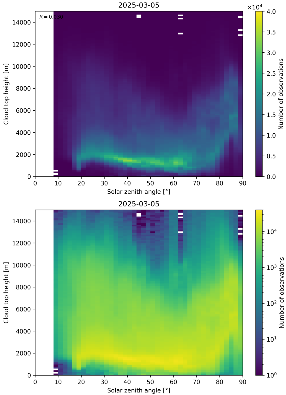
Figure 104: Scatter density plot of “Solar zenith angle” against “Cloud top height” for 2025-03-04 to 2025-03-06.
