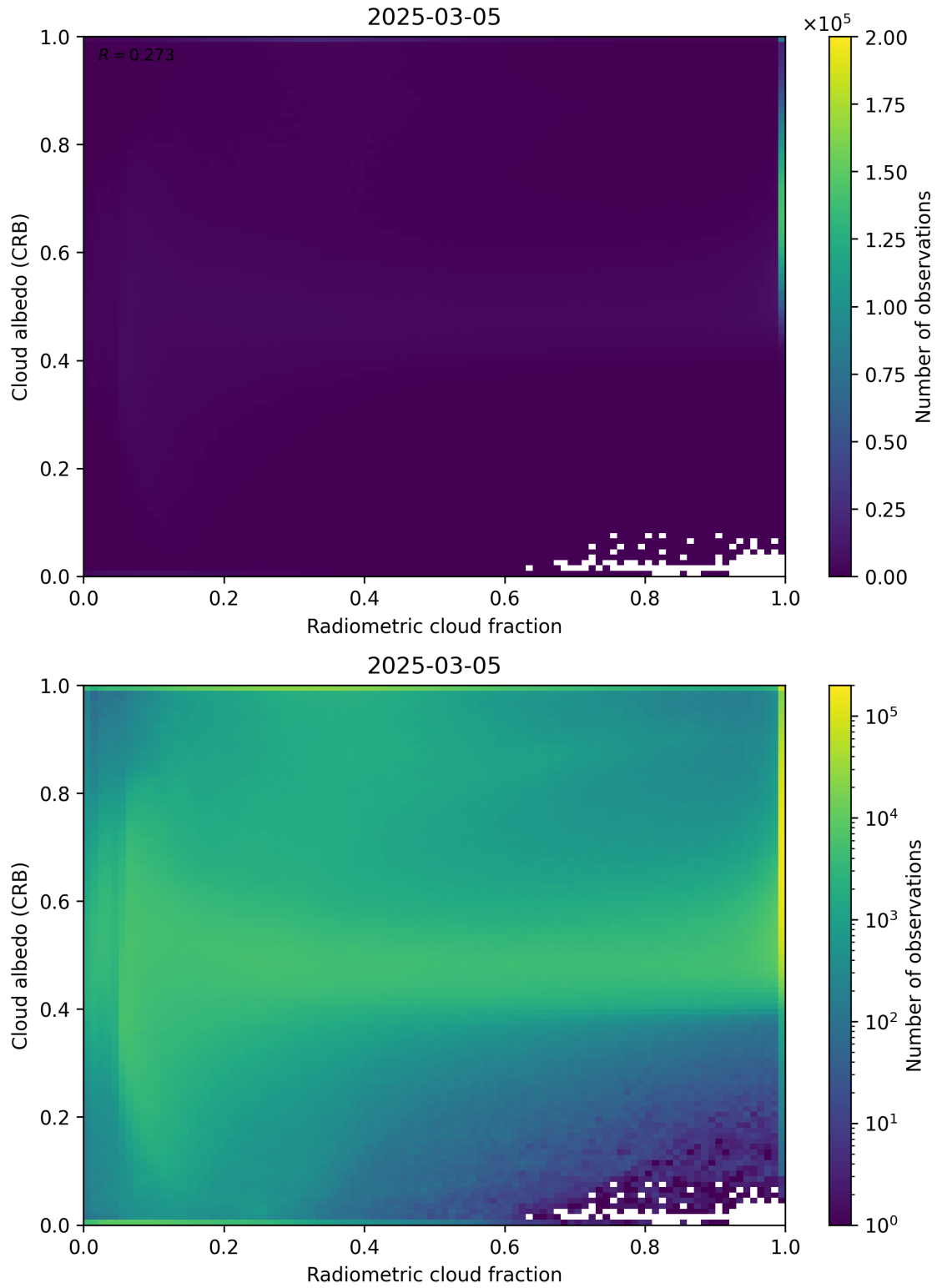
Figure 71: Scatter density plot of “Radiometric cloud fraction” against “Cloud albedo (CRB)” for 2025-03-04 to 2025-03-06.
