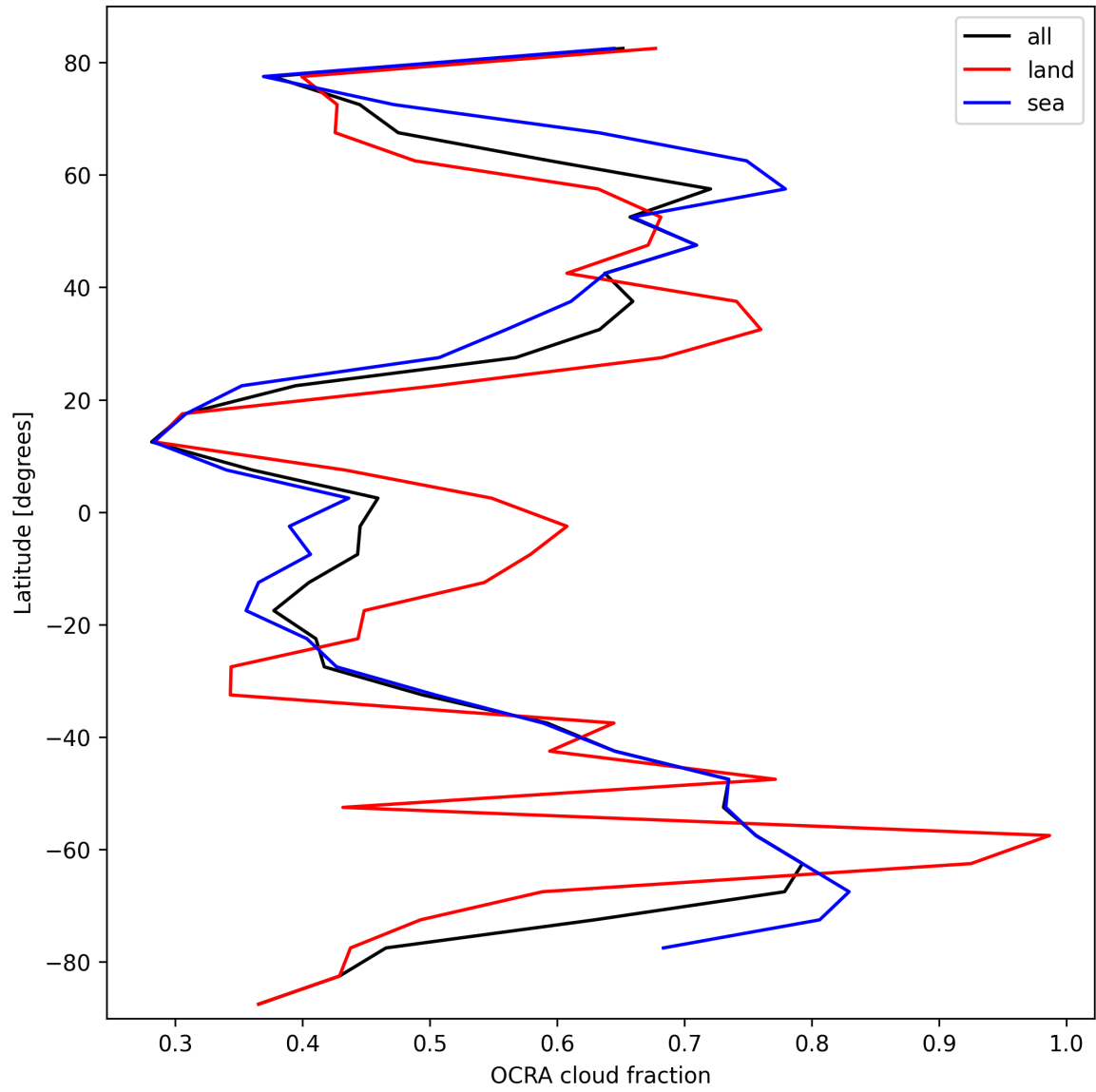
Figure 34: Zonal average of “OCRA cloud fraction” for 2025-03-04 to 2025-03-06.
