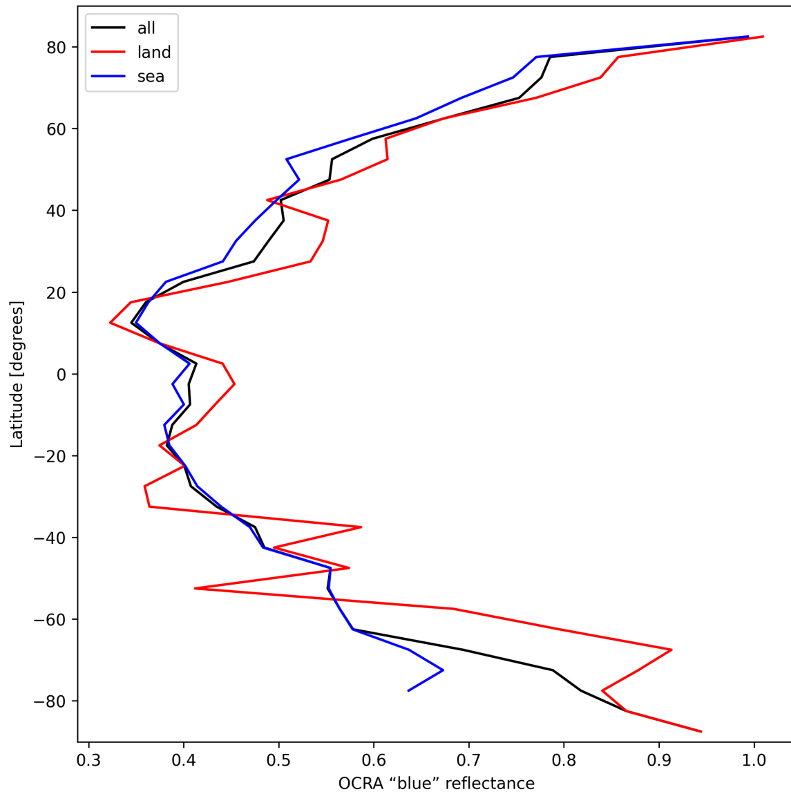
Figure 35: Zonal average of “OCRA “blue” reflectance” for 2025-03-04 to 2025-03-06.
