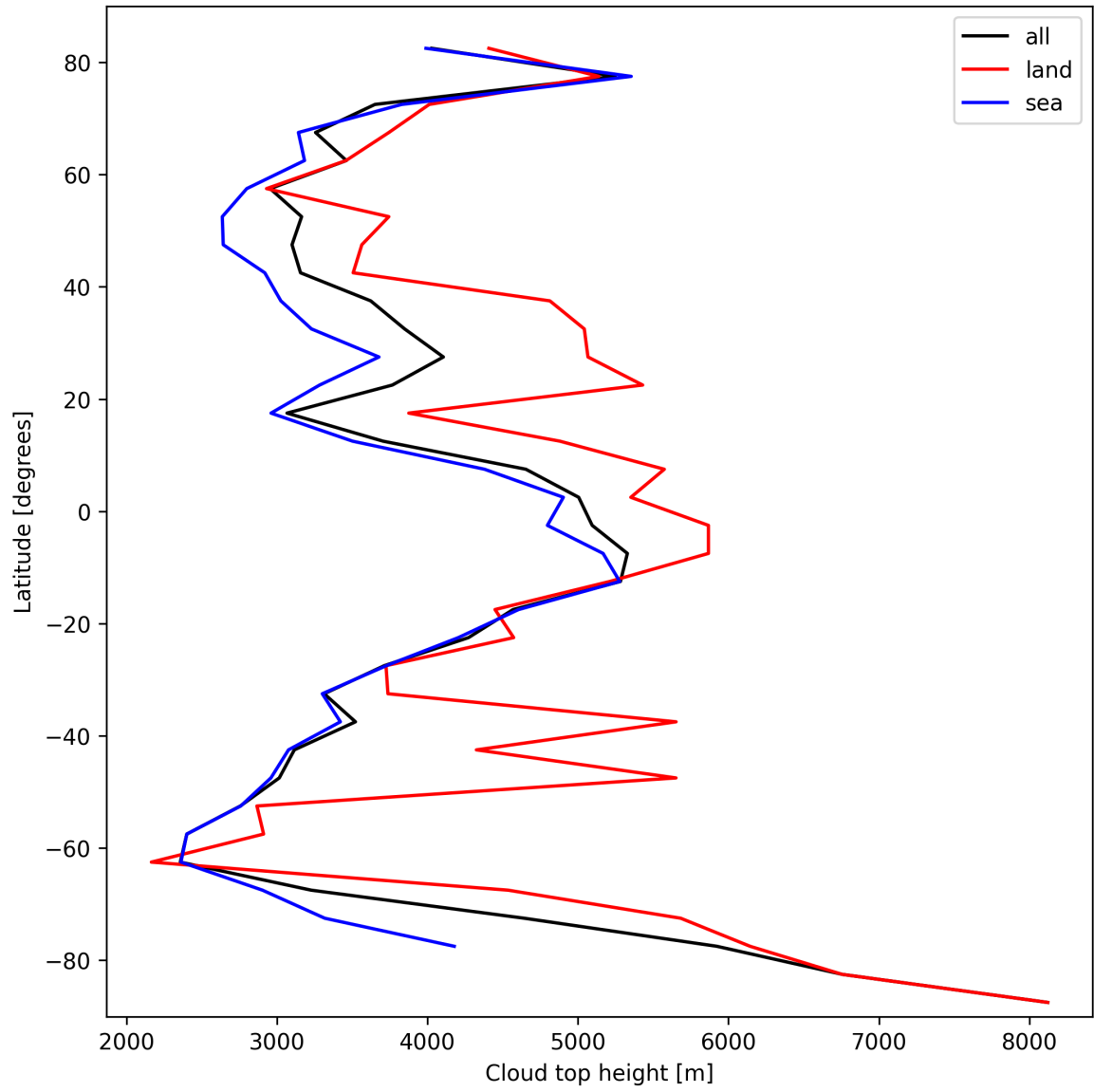
Figure 24: Zonal average of “Cloud top height” for 2025-03-04 to 2025-03-06.
