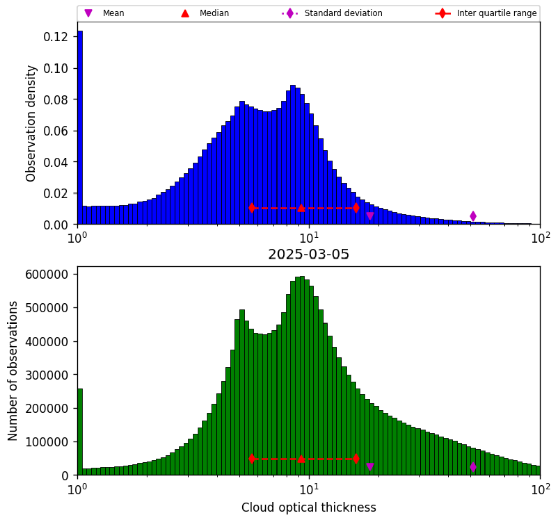
Figure 41: Histogram of “Cloud optical thickness” for 2025-03-04 to 2025-03-06
