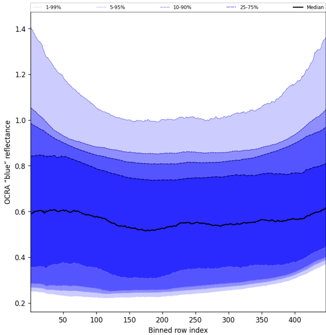
Figure 67: Along track statistics of “OCRA “blue” reflectance” for 2025-03-04 to 2025-03-06
