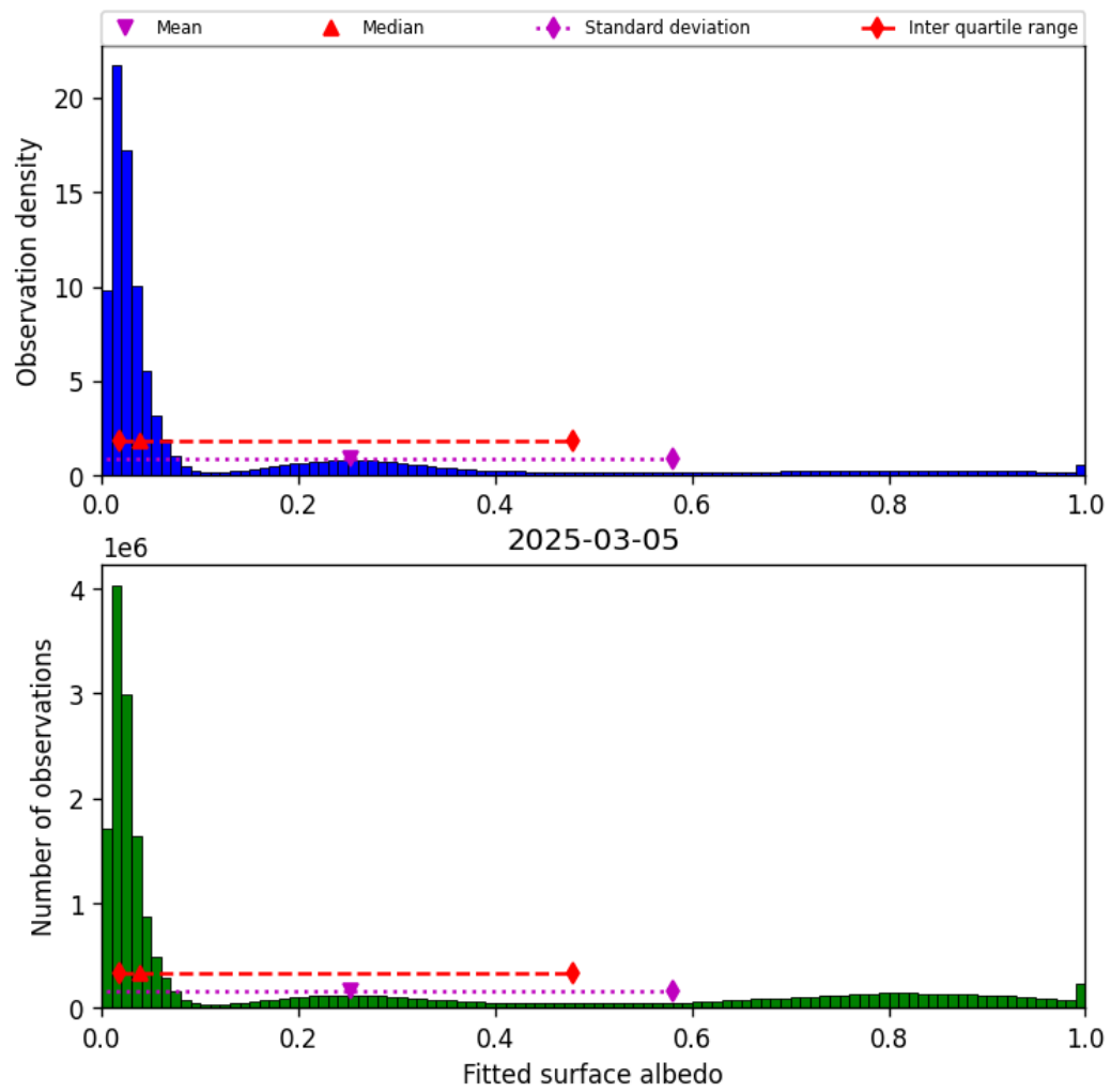
Figure 45: Histogram of “Fitted surface albedo” for 2025-03-04 to 2025-03-06
