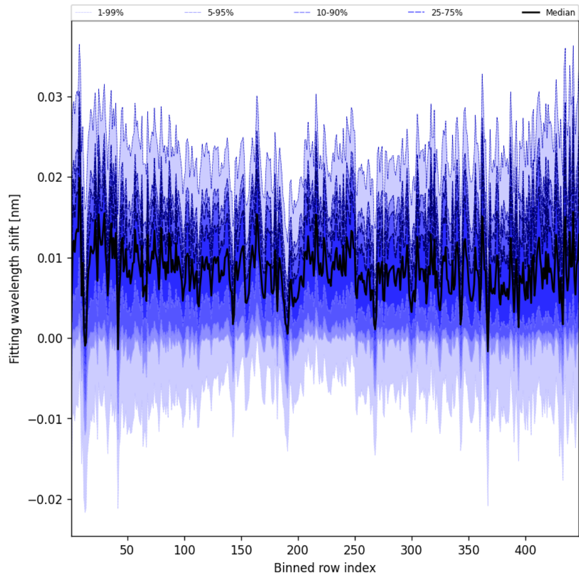
Figure 65: Along track statistics of “Fitting wavelength shift” for 2025-03-04 to 2025-03-06
