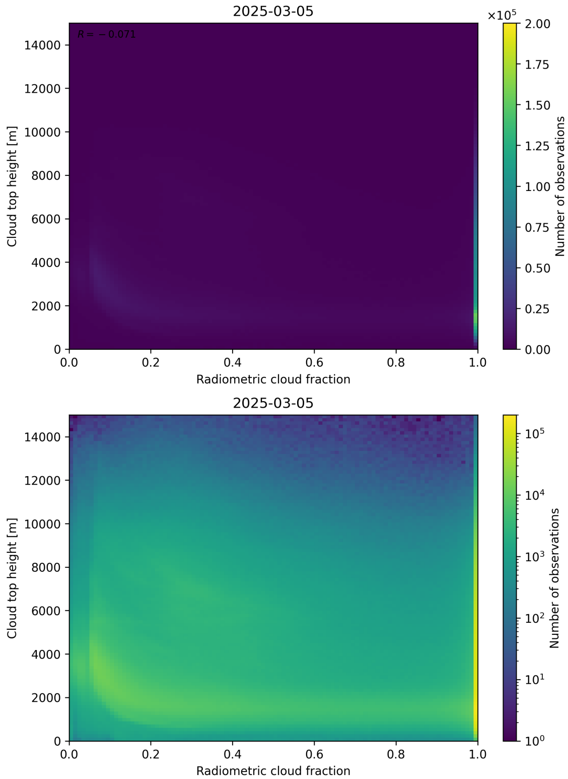
Figure 76: Scatter density plot of “Radiometric cloud fraction” against “Cloud top height” for 2025-03-04 to 2025-03-06.
