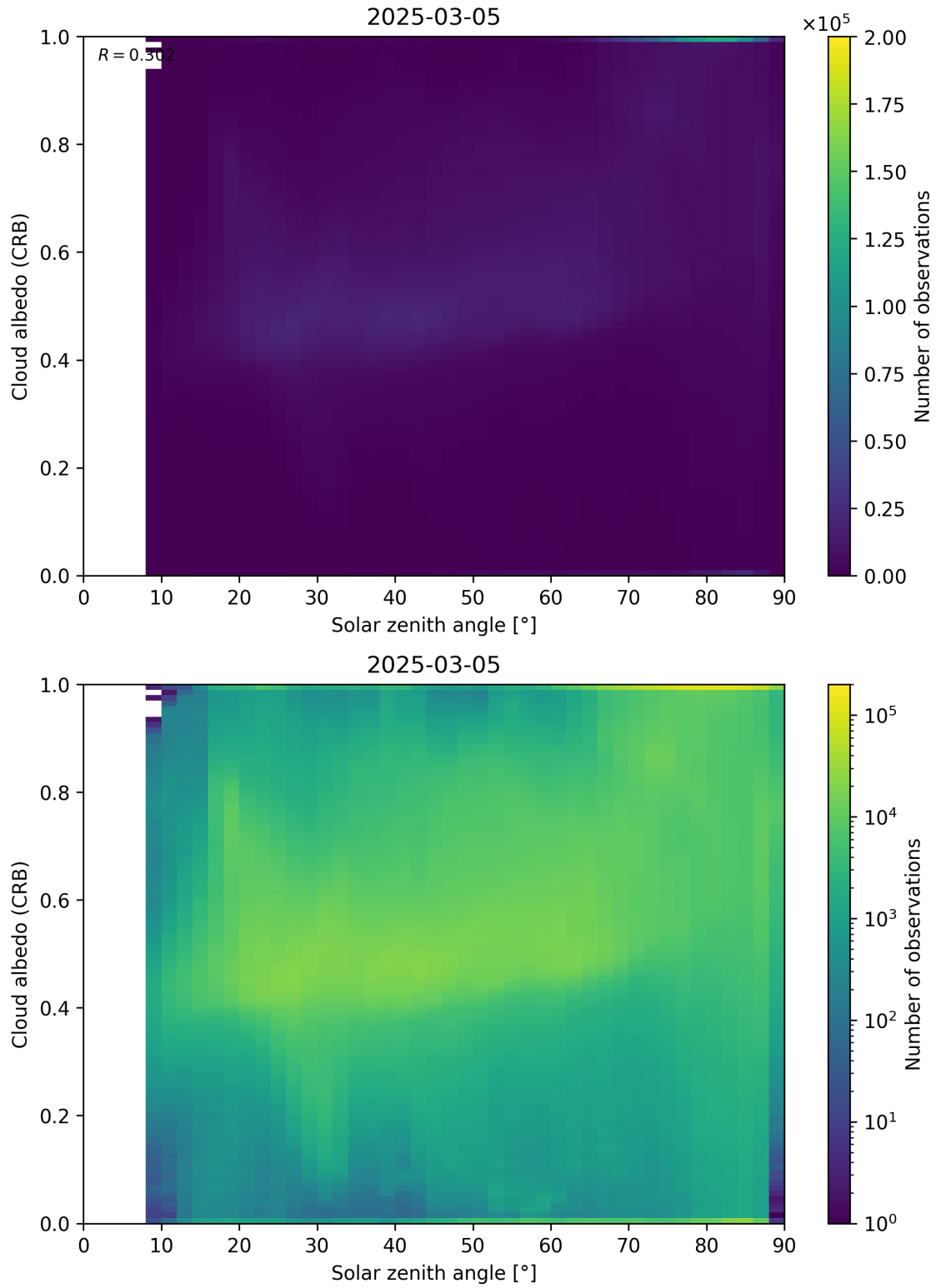
Figure 98: Scatter density plot of “Solar zenith angle” against “Cloud albedo (CRB)” for 2025-03-04 to 2025-03-06.
