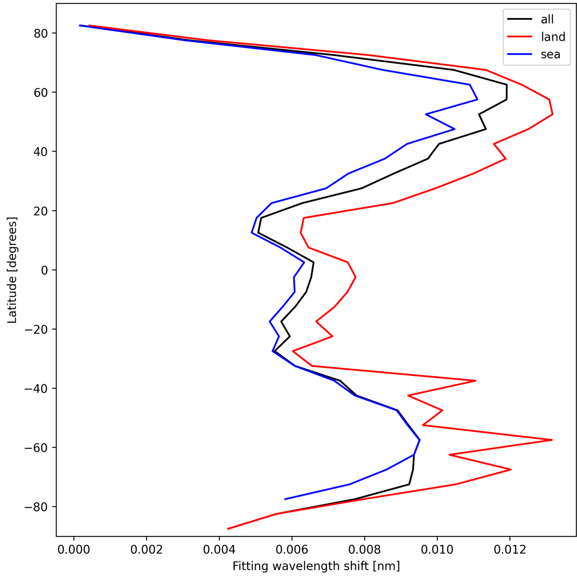
Figure 33: Zonal average of “Fitting wavelength shift” for 2025-03-04 to 2025-03-06.
