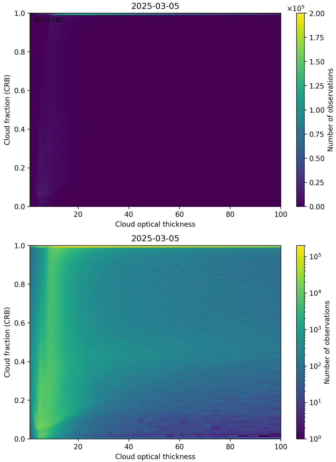
Figure 84: Scatter density plot of “Cloud optical thickness” against “Cloud fraction (CRB)” for 2025-03-04 to 2025-03-06.
