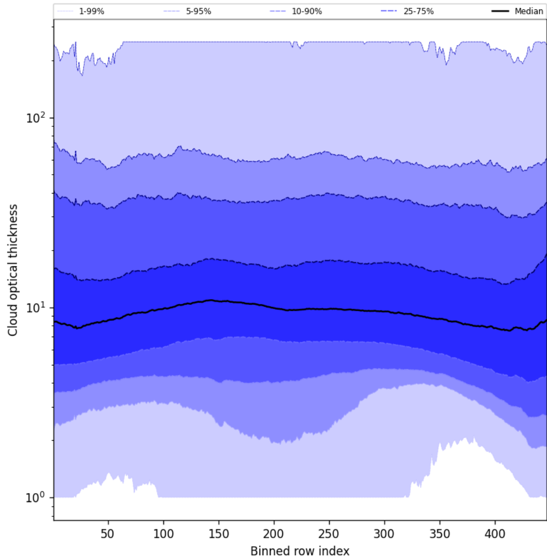
Figure 57: Along track statistics of “Cloud optical thickness” for 2025-03-04 to 2025-03-06
