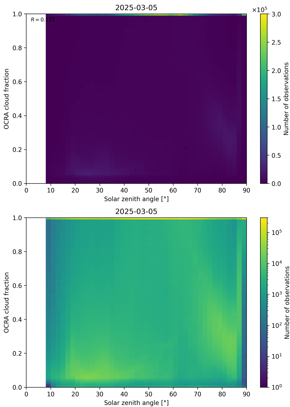
Figure 100: Scatter density plot of “Solar zenith angle” against “OCRA cloud fraction” for 2025-03-04 to 2025-03-06.
