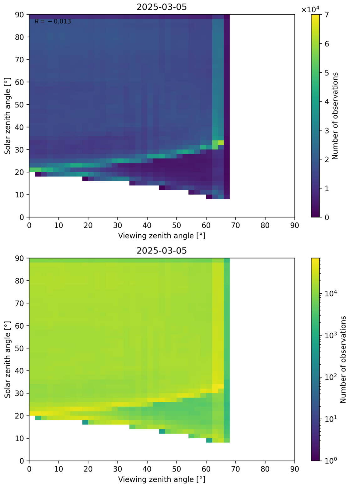
Figure 114: Scatter density plot of “Viewing zenith angle” against “Solar zenith angle” for 2025-03-04 to 2025-03-06.
