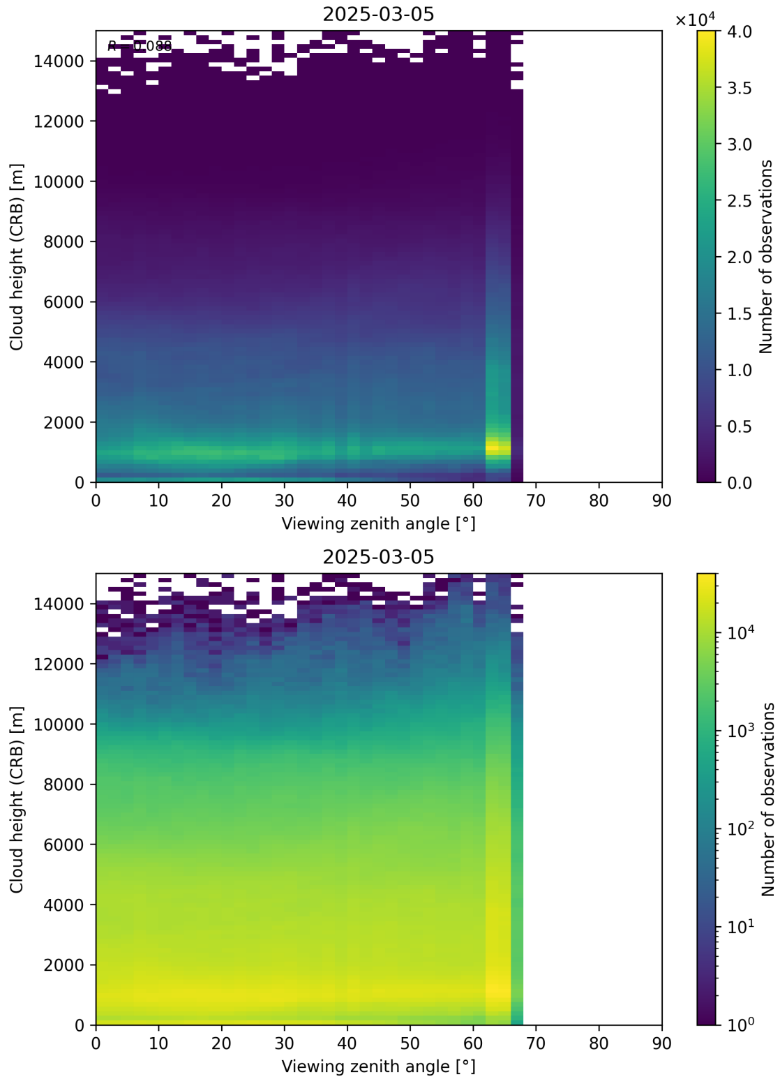
Figure 110: Scatter density plot of “Viewing zenith angle” against “Cloud height (CRB)” for 2025-03-04 to 2025-03-06.
