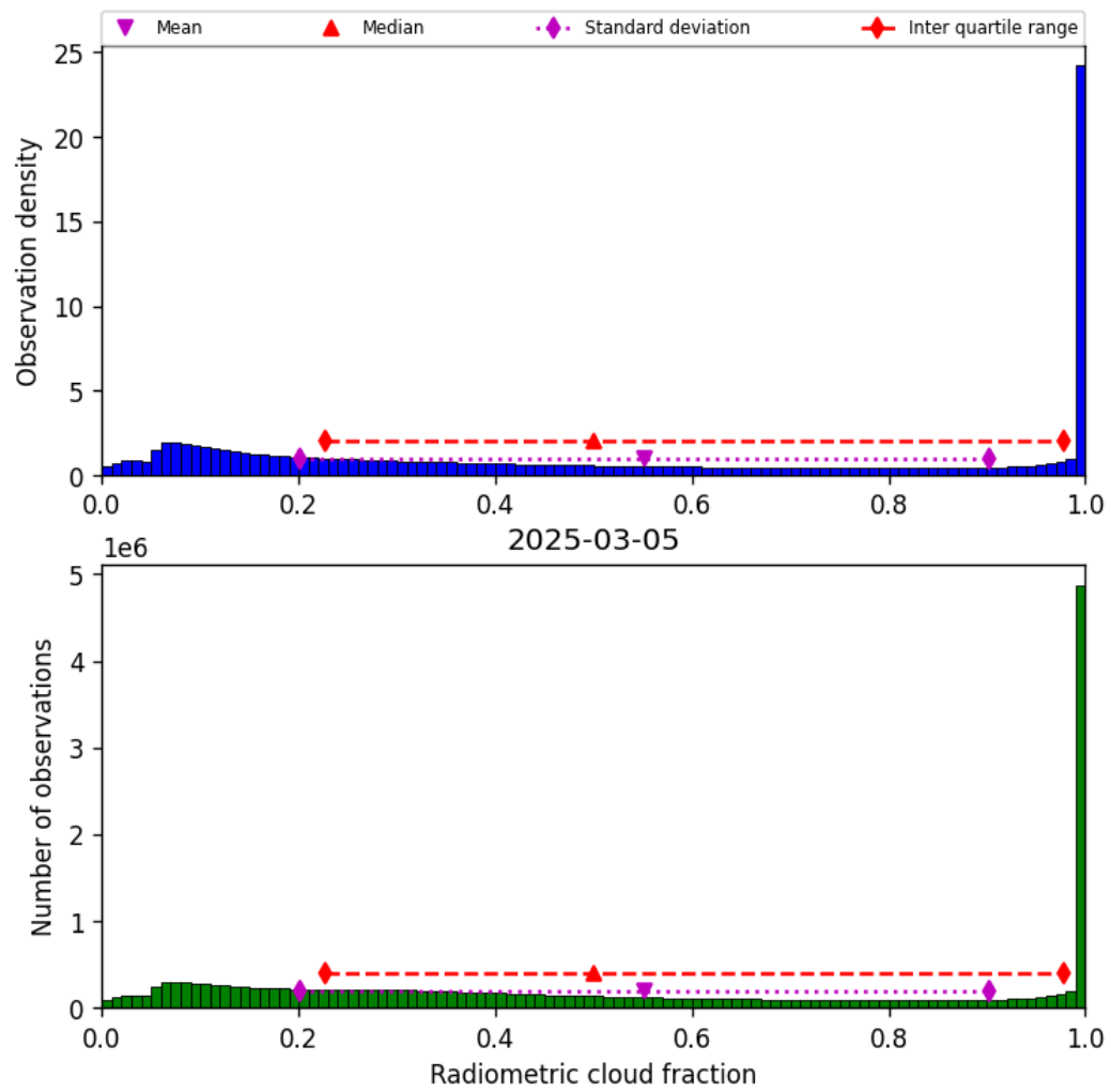
Figure 39: Histogram of “Radiometric cloud fraction” for 2025-03-04 to 2025-03-06
