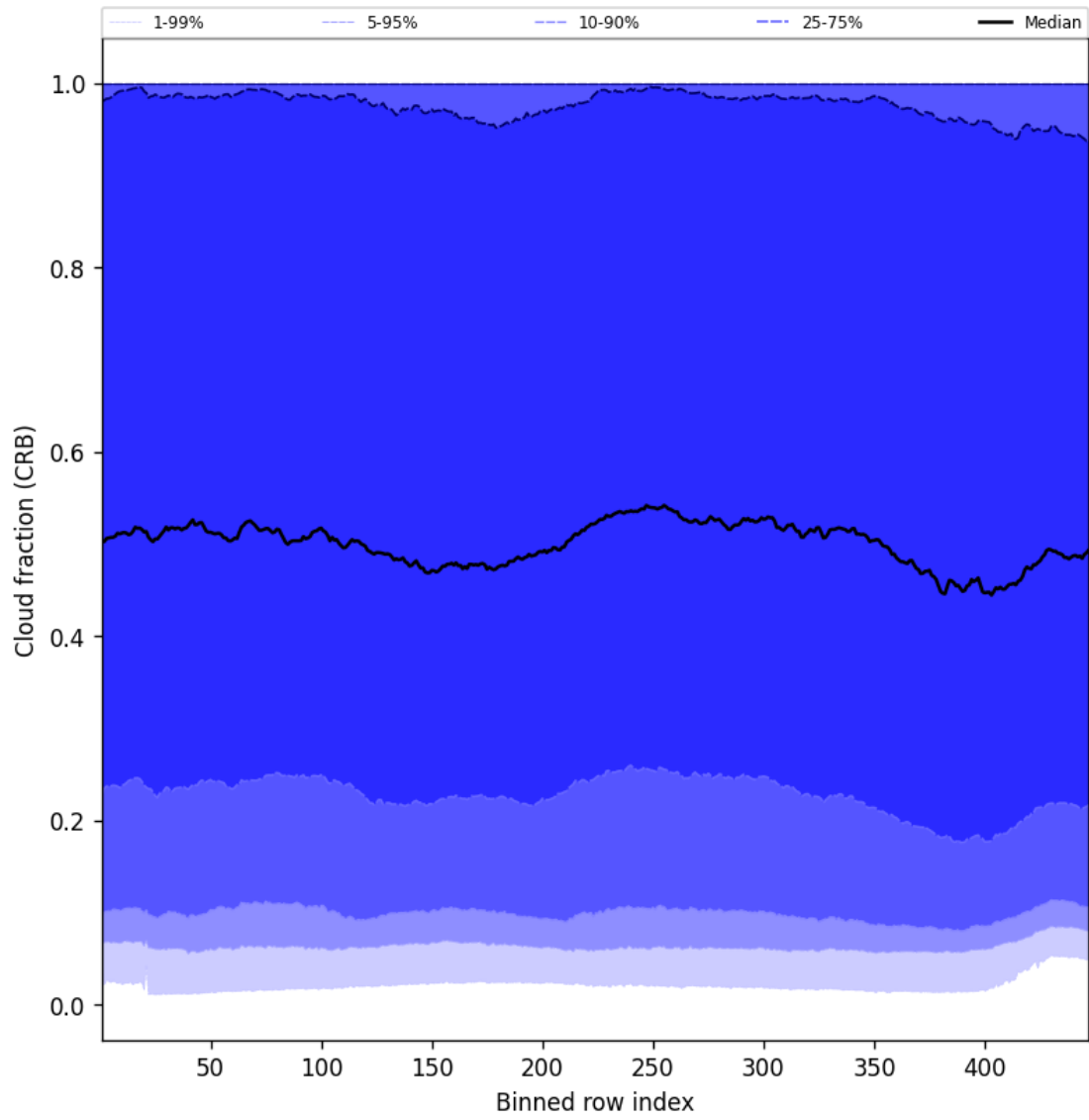
Figure 58: Along track statistics of “Cloud fraction (CRB)” for 2025-03-04 to 2025-03-06
