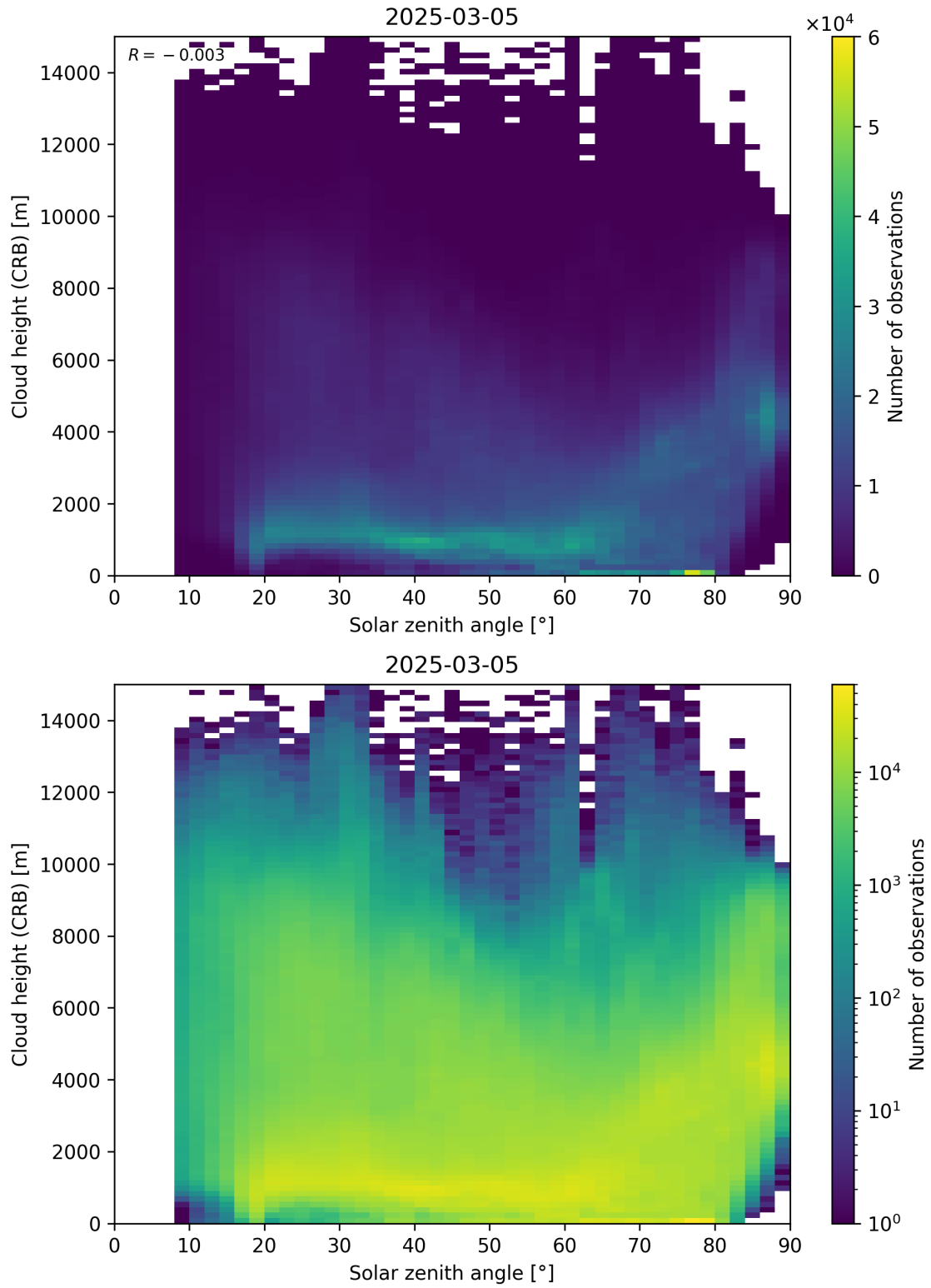
Figure 102: Scatter density plot of “Solar zenith angle” against “Cloud height (CRB)” for 2025-03-04 to 2025-03-06.
