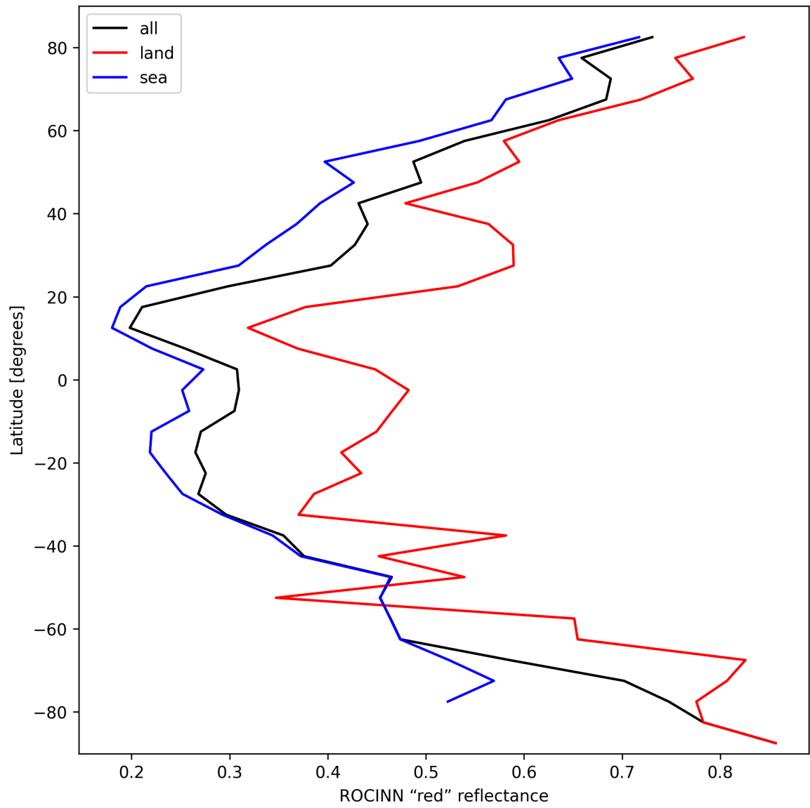
Figure 37: Zonal average of “ROCINN “red” reflectance” for 2025-03-04 to 2025-03-06.
