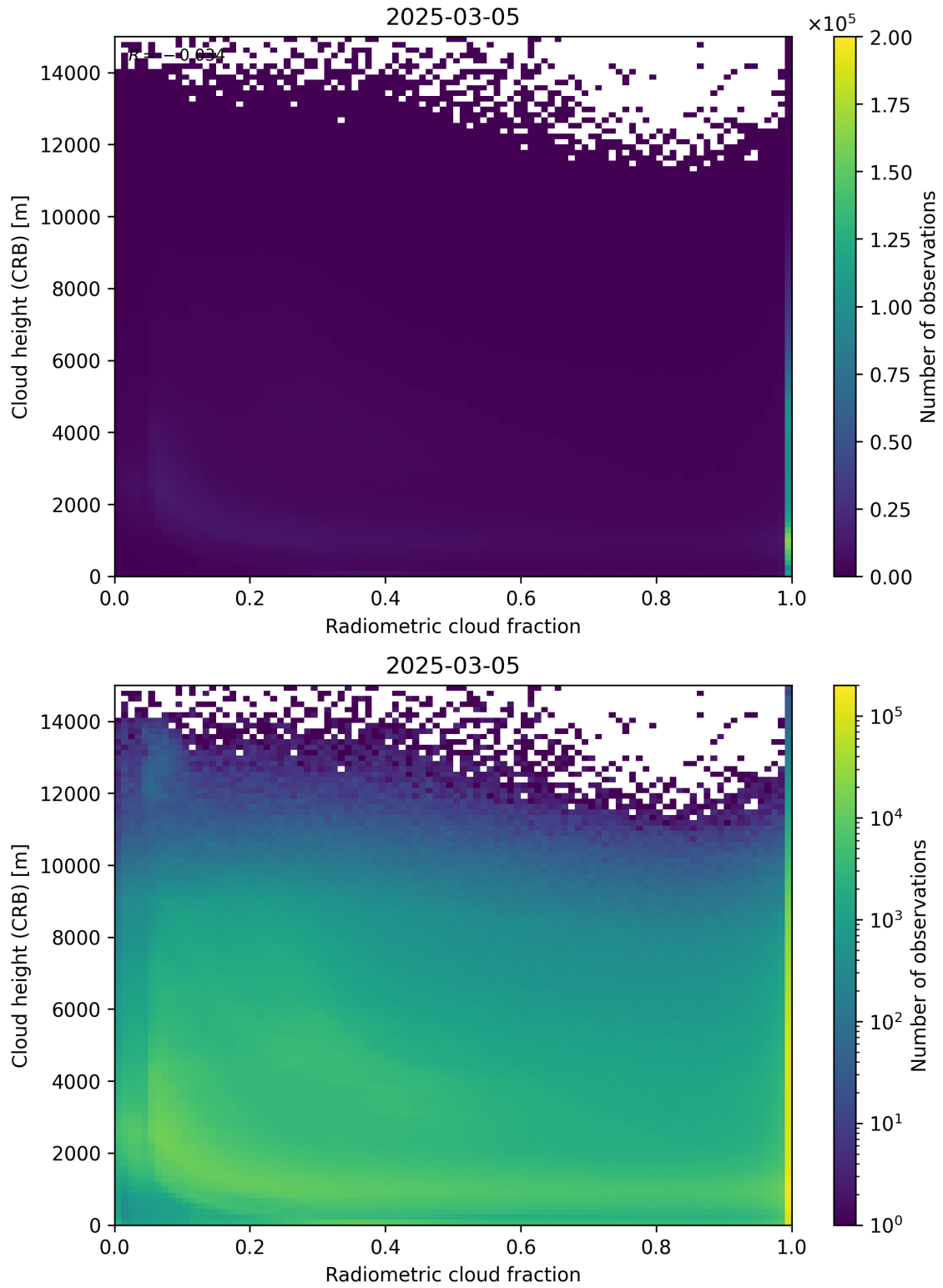
Figure 74: Scatter density plot of “Radiometric cloud fraction” against “Cloud height (CRB)” for 2025-03-04 to 2025-03-06.
