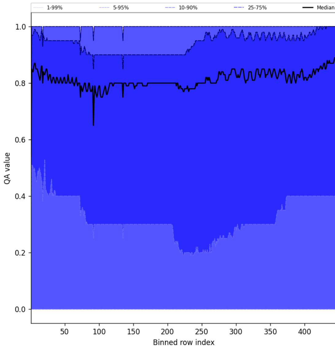
Figure 54: Along track statistics of “QA value” for 2025-03-04 to 2025-03-06
