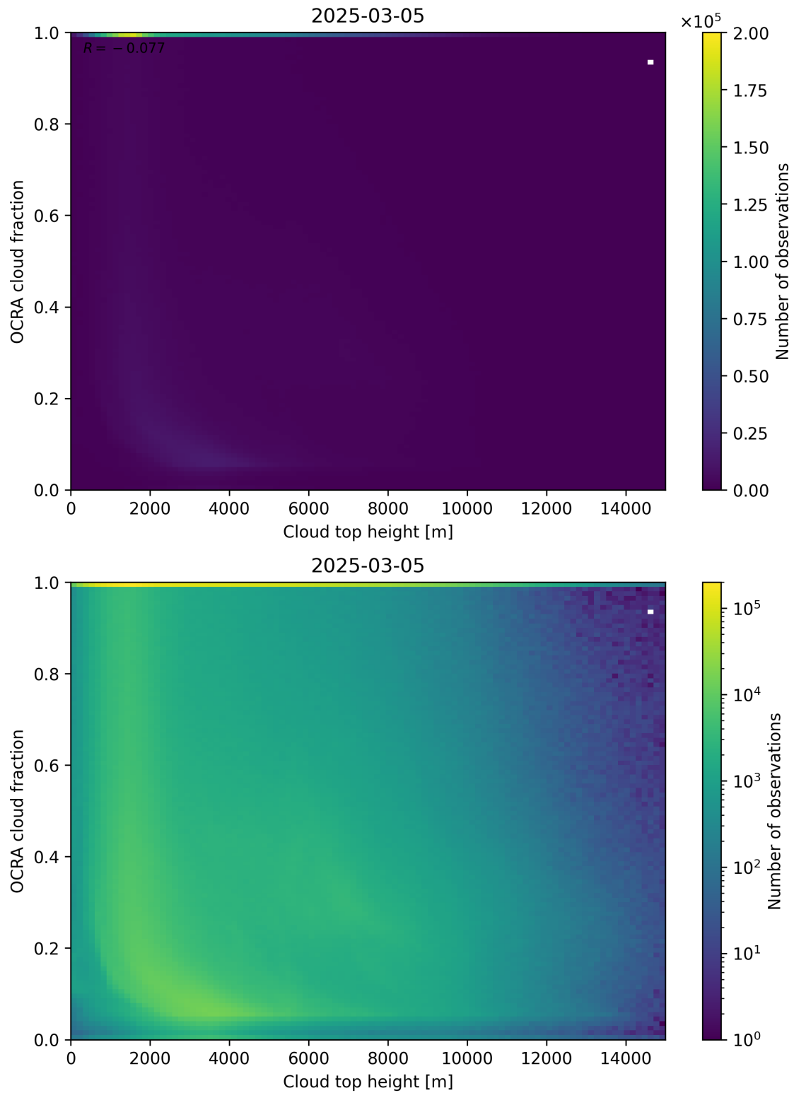
Figure 87: Scatter density plot of “Cloud top height” against “OCRA cloud fraction” for 2025-03-04 to 2025-03-06.
