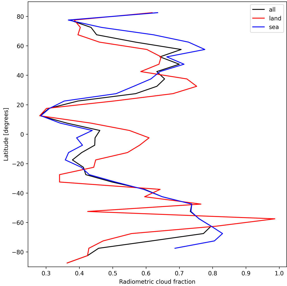
Figure 23: Zonal average of “Radiometric cloud fraction” for 2025-03-04 to 2025-03-06.
