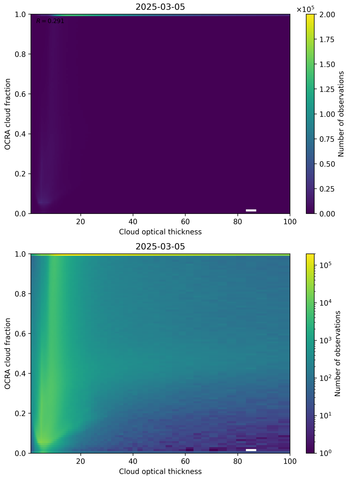
Figure 83: Scatter density plot of “Cloud optical thickness” against “OCRA cloud fraction” for 2025-03-04 to 2025-03-06.
