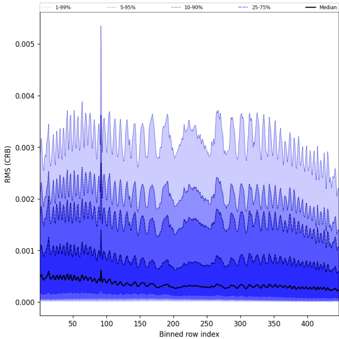
Figure 64: Along track statistics of “RMS (CRB)” for 2025-03-04 to 2025-03-06
