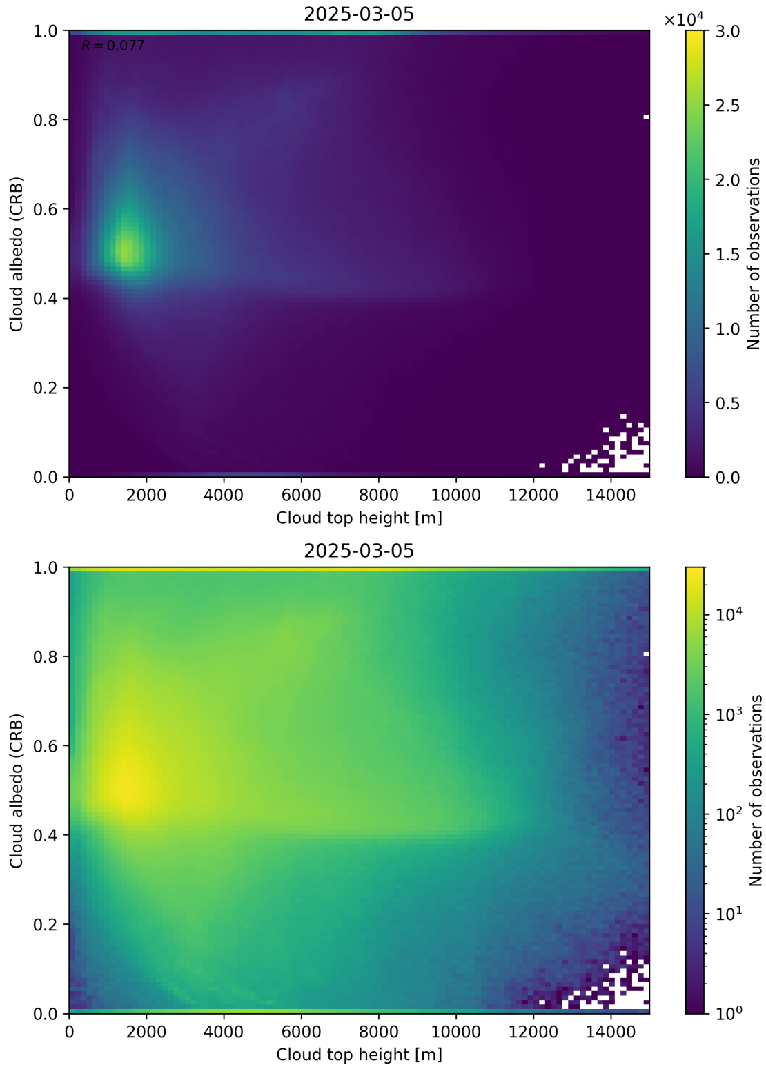
Figure 86: Scatter density plot of “Cloud top height” against “Cloud albedo (CRB)” for 2025-03-04 to 2025-03-06.
