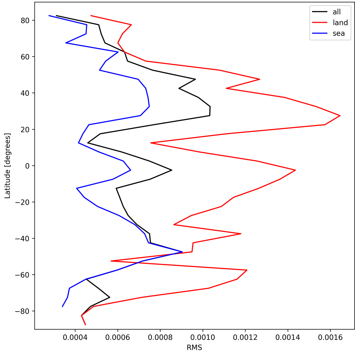
Figure 31: Zonal average of “RMS” for 2025-03-04 to 2025-03-06.
