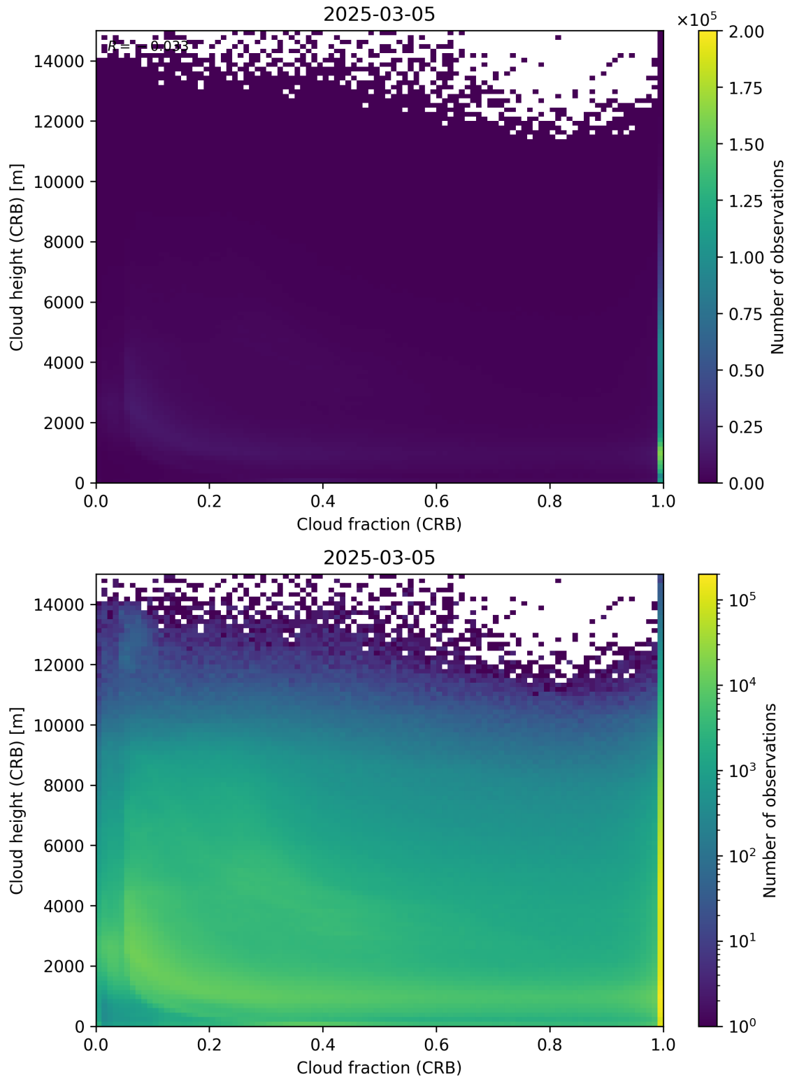
Figure 79: Scatter density plot of “Cloud fraction (CRB)” against “Cloud height (CRB)” for 2025-03-04 to 2025-03-06.
