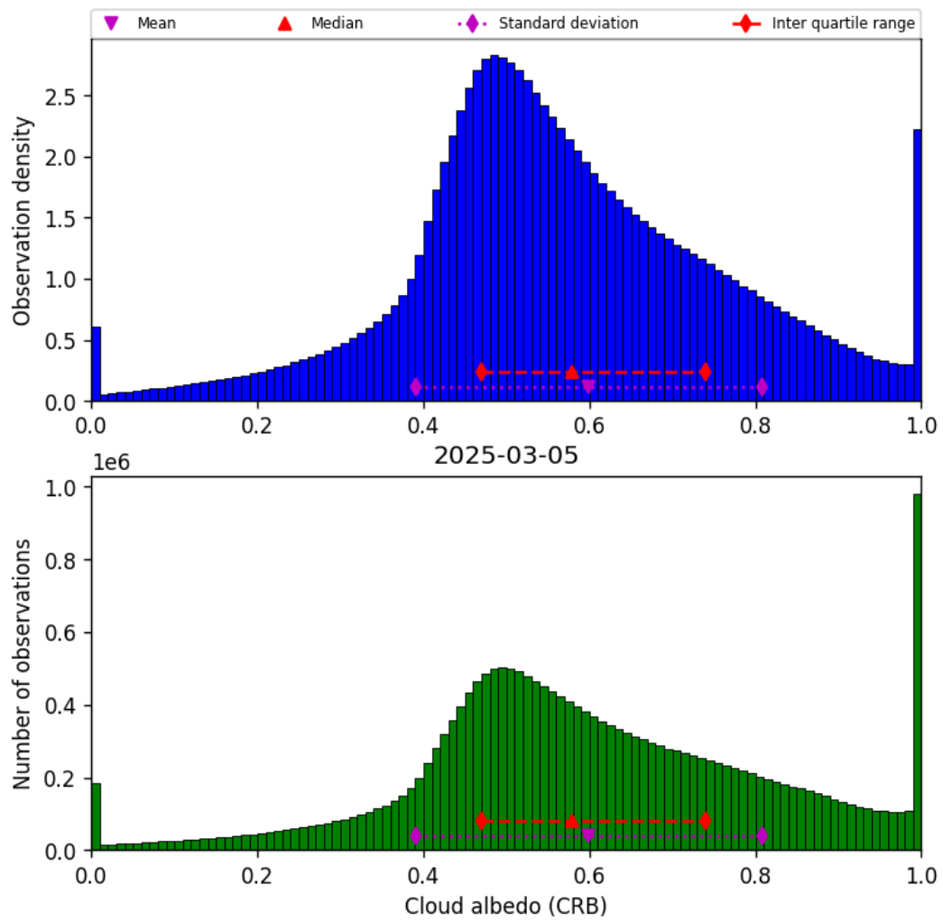
Figure 44: Histogram of “Cloud albedo (CRB)” for 2025-03-04 to 2025-03-06
