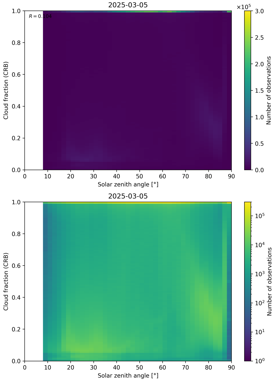
Figure 101: Scatter density plot of “Solar zenith angle” against “Cloud fraction (CRB)” for 2025-03-04 to 2025-03-06.
