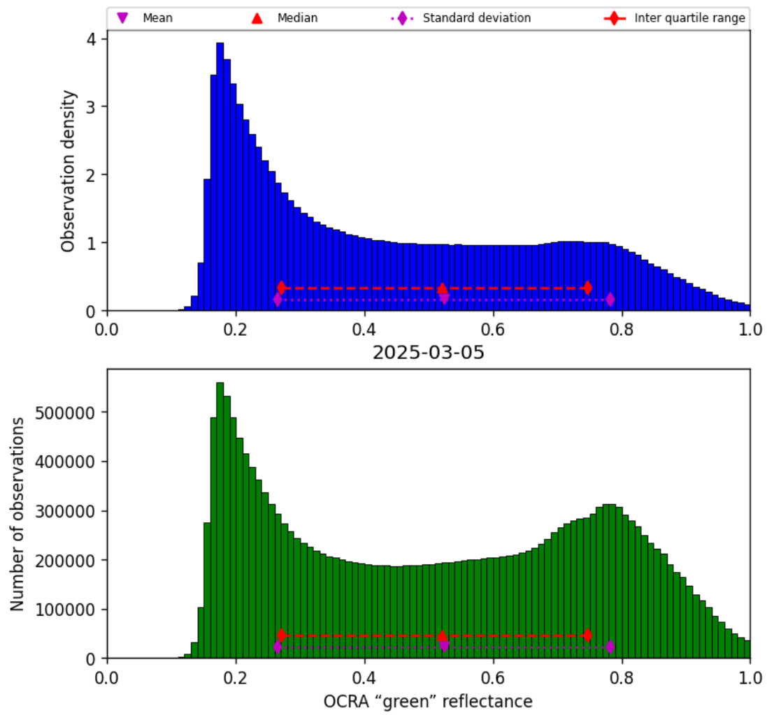
Figure 52: Histogram of “OCRA “green” reflectance” for 2025-03-04 to 2025-03-06
