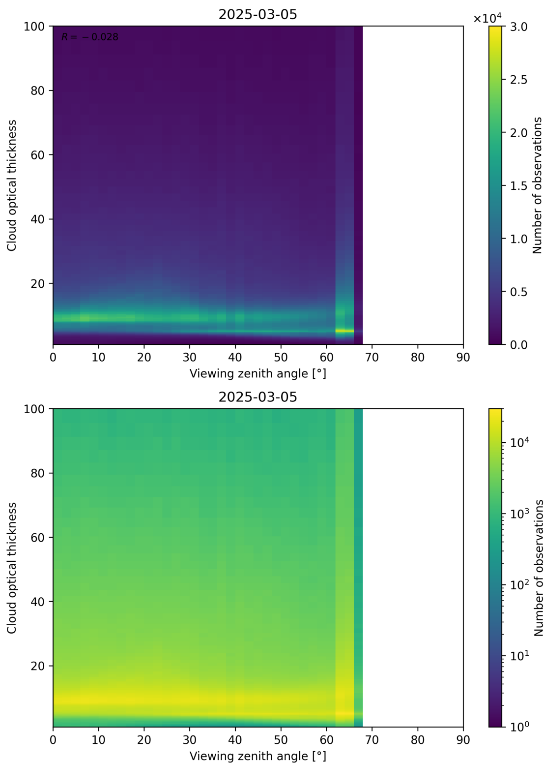
Figure 111: Scatter density plot of “Viewing zenith angle” against “Cloud optical thickness” for 2025-03-04 to 2025-03-06.
