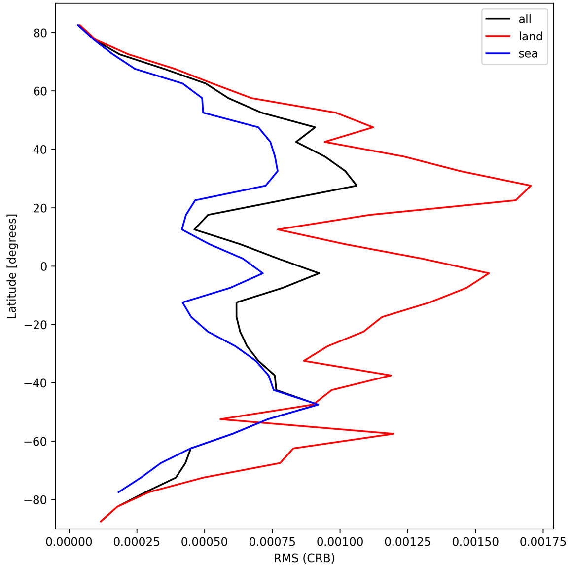
Figure 32: Zonal average of “RMS (CRB)” for 2025-03-04 to 2025-03-06.
