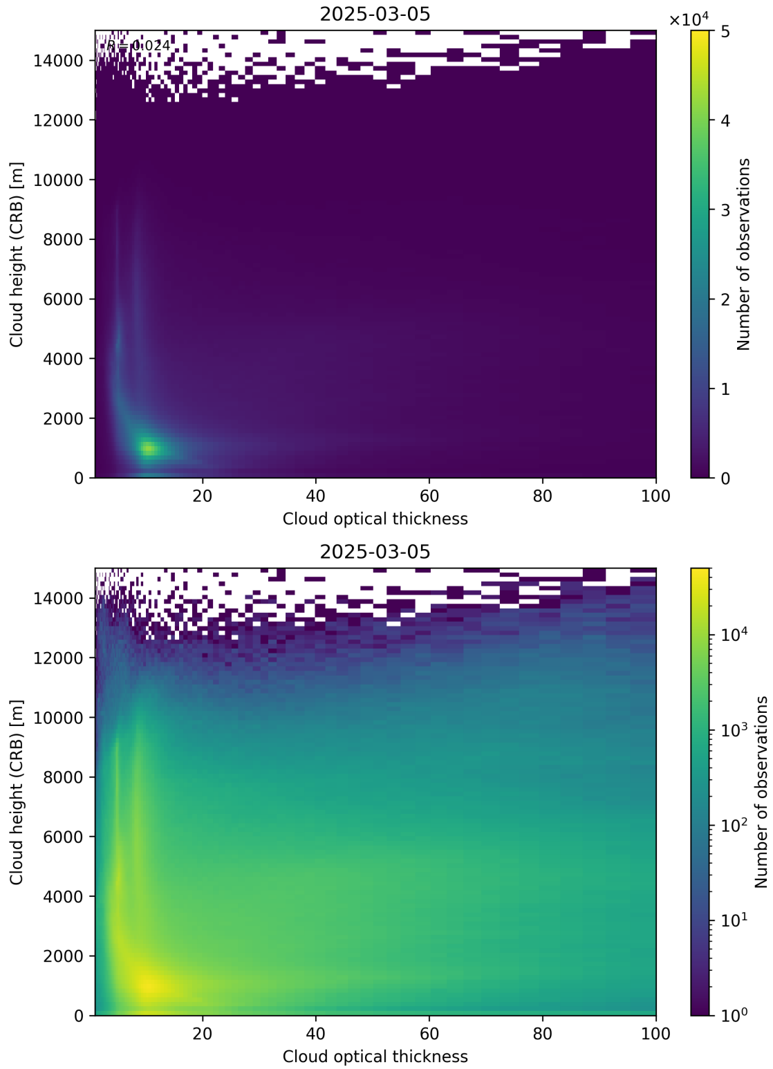
Figure 85: Scatter density plot of “Cloud optical thickness” against “Cloud height (CRB)” for 2025-03-04 to 2025-03-06.
