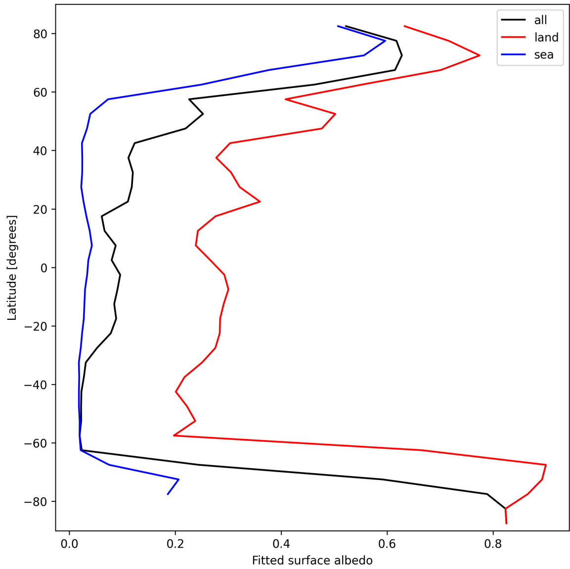
Figure 29: Zonal average of “Fitted surface albedo” for 2025-03-04 to 2025-03-06.
