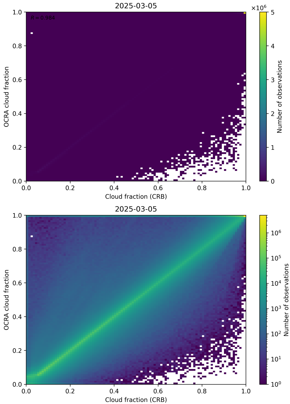
Figure 78: Scatter density plot of “Cloud fraction (CRB)” against “OCRA cloud fraction” for 2025-03-04 to 2025-03-06.
