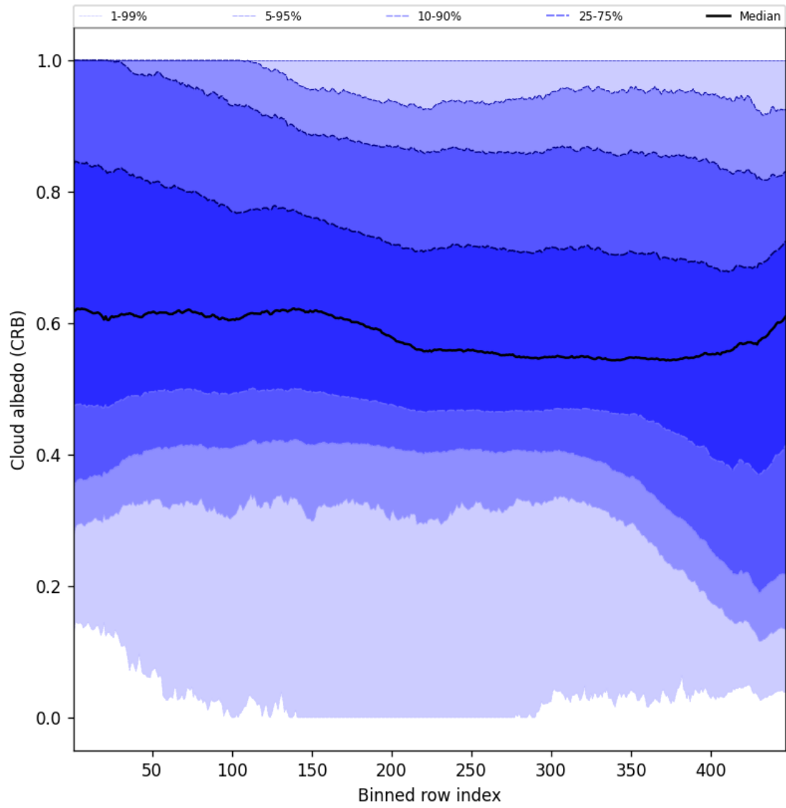
Figure 60: Along track statistics of “Cloud albedo (CRB)” for 2025-03-04 to 2025-03-06
