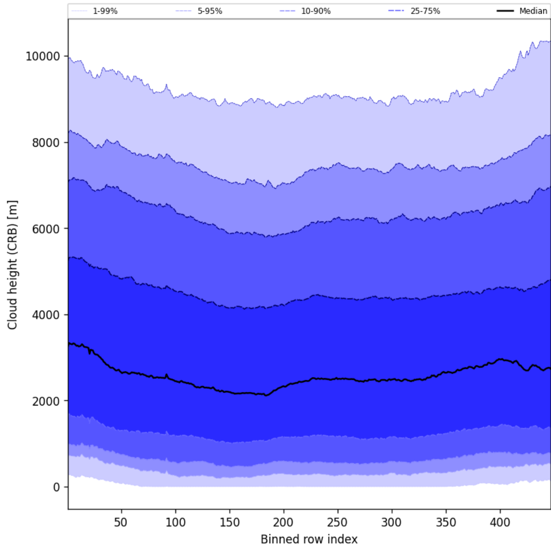
Figure 59: Along track statistics of “Cloud height (CRB)” for 2025-03-04 to 2025-03-06
