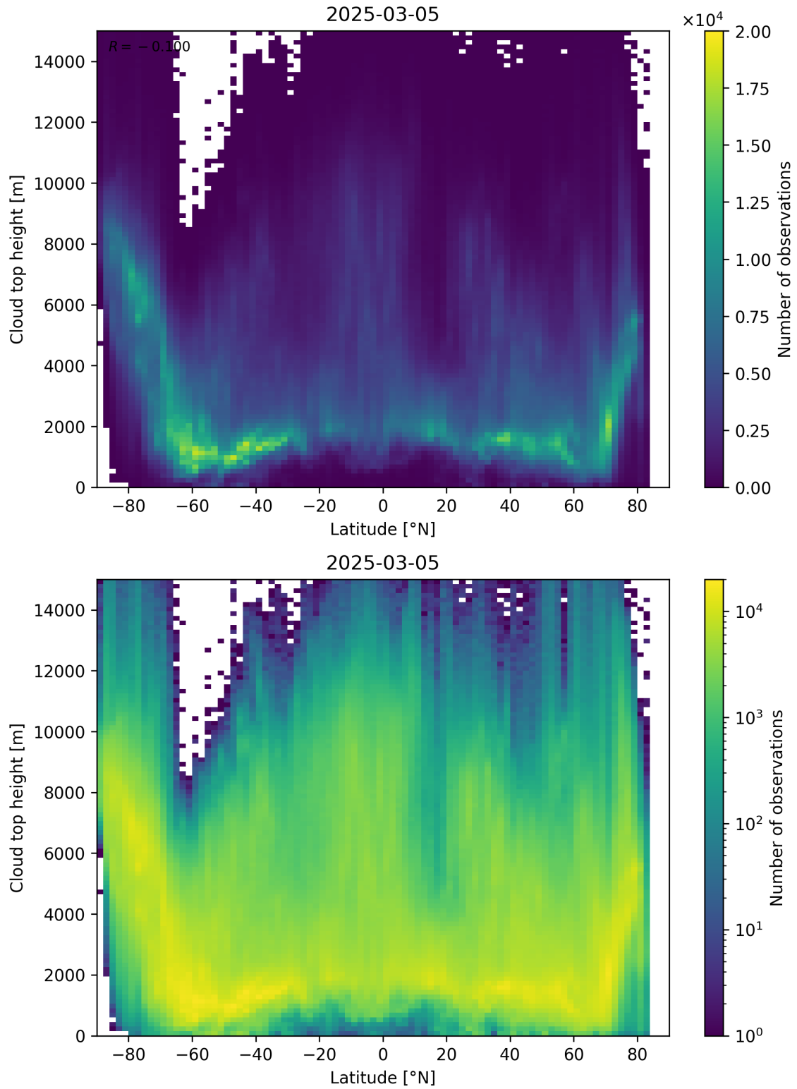
Figure 97: Scatter density plot of “Latitude” against “Cloud top height” for 2025-03-04 to 2025-03-06.
