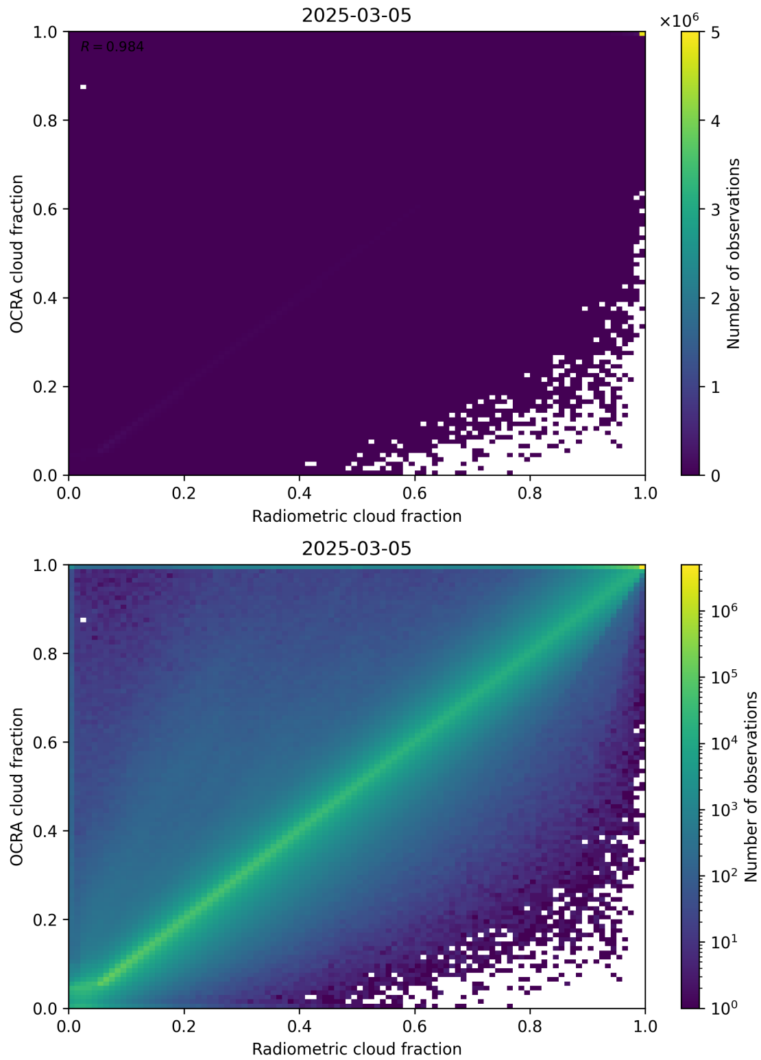
Figure 72: Scatter density plot of “Radiometric cloud fraction” against “OCRA cloud fraction” for 2025-03-04 to 2025-03-06.
