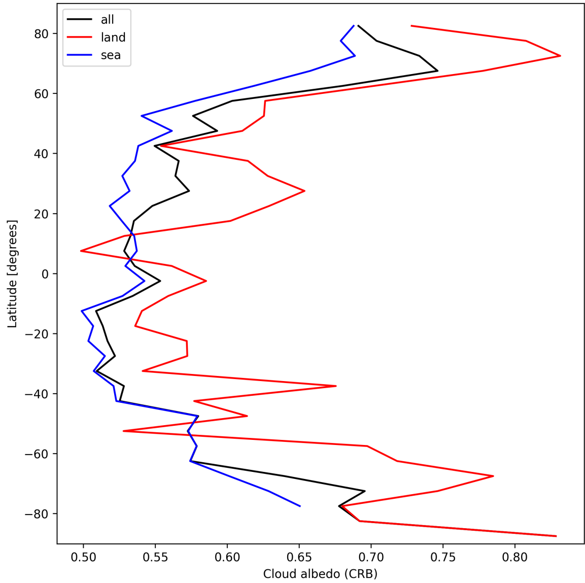
Figure 28: Zonal average of “Cloud albedo (CRB)” for 2025-03-04 to 2025-03-06.
