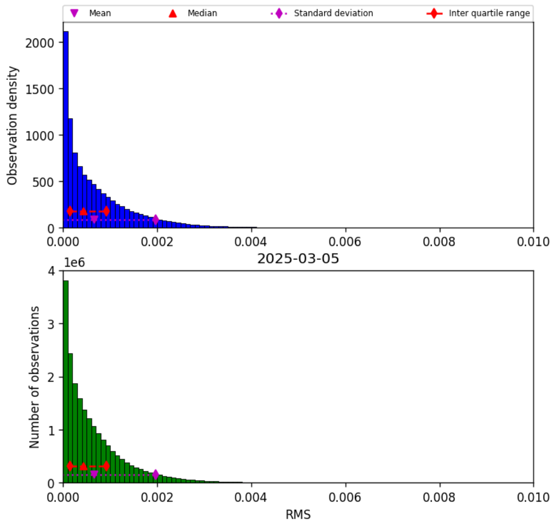
Figure 47: Histogram of “RMS” for 2025-03-04 to 2025-03-06
