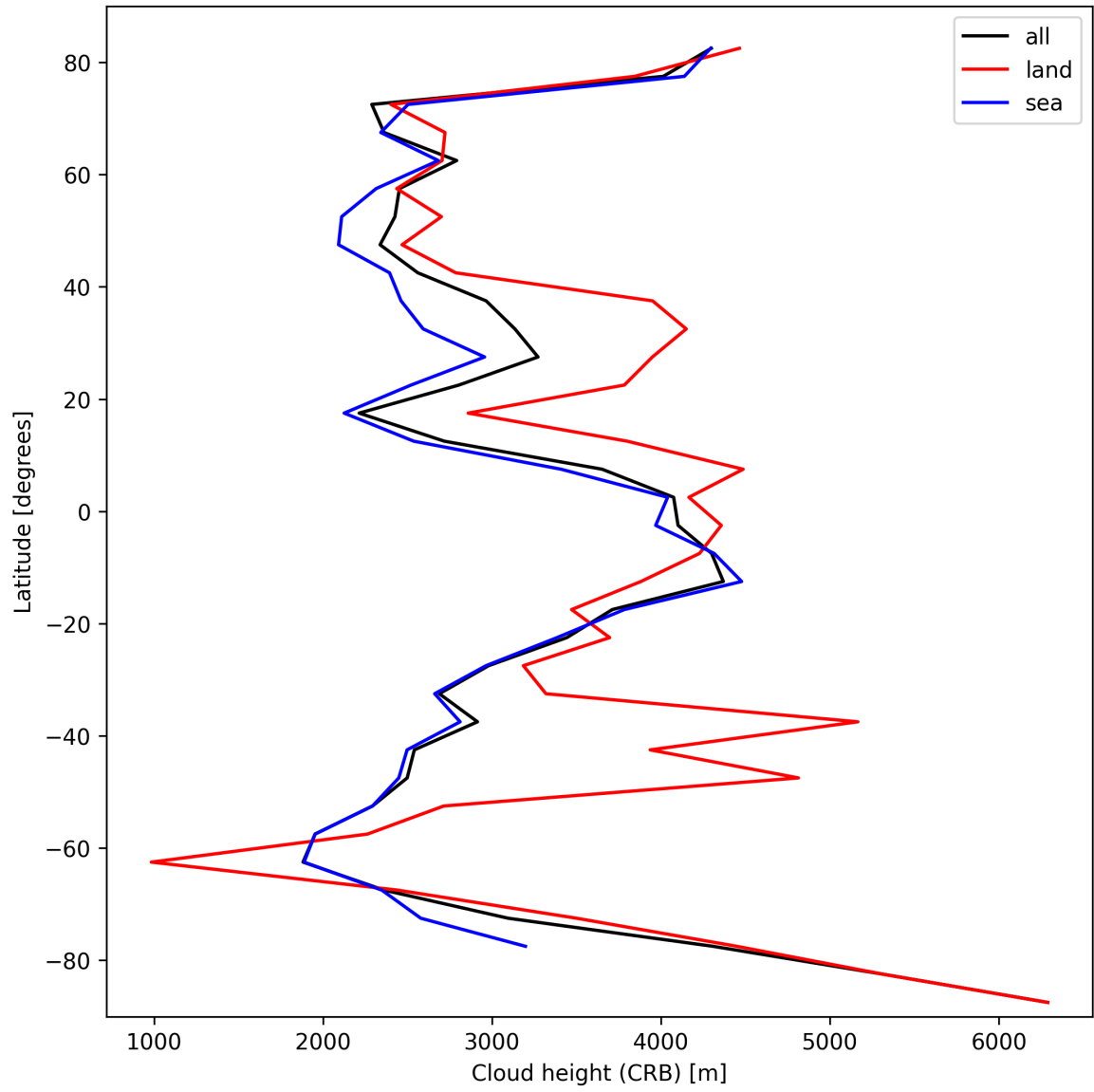
Figure 27: Zonal average of “Cloud height (CRB)” for 2025-03-04 to 2025-03-06.
