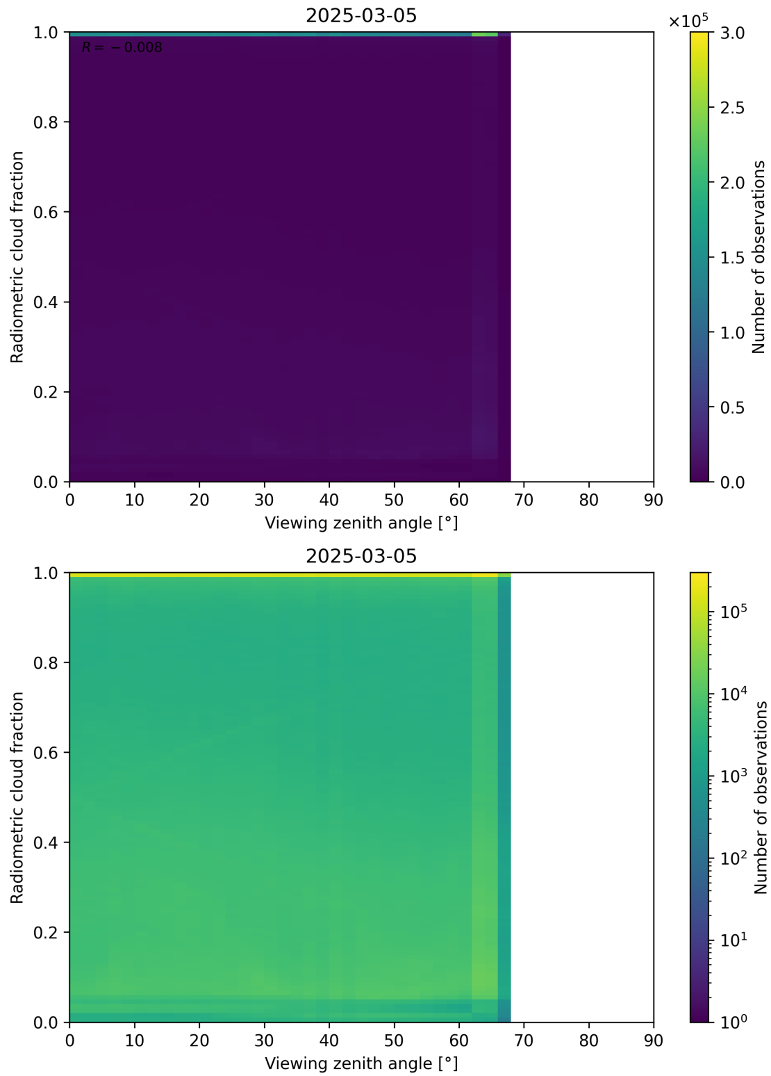
Figure 107: Scatter density plot of “Viewing zenith angle” against “Radiometric cloud fraction” for 2025-03-04 to 2025-03-06.
