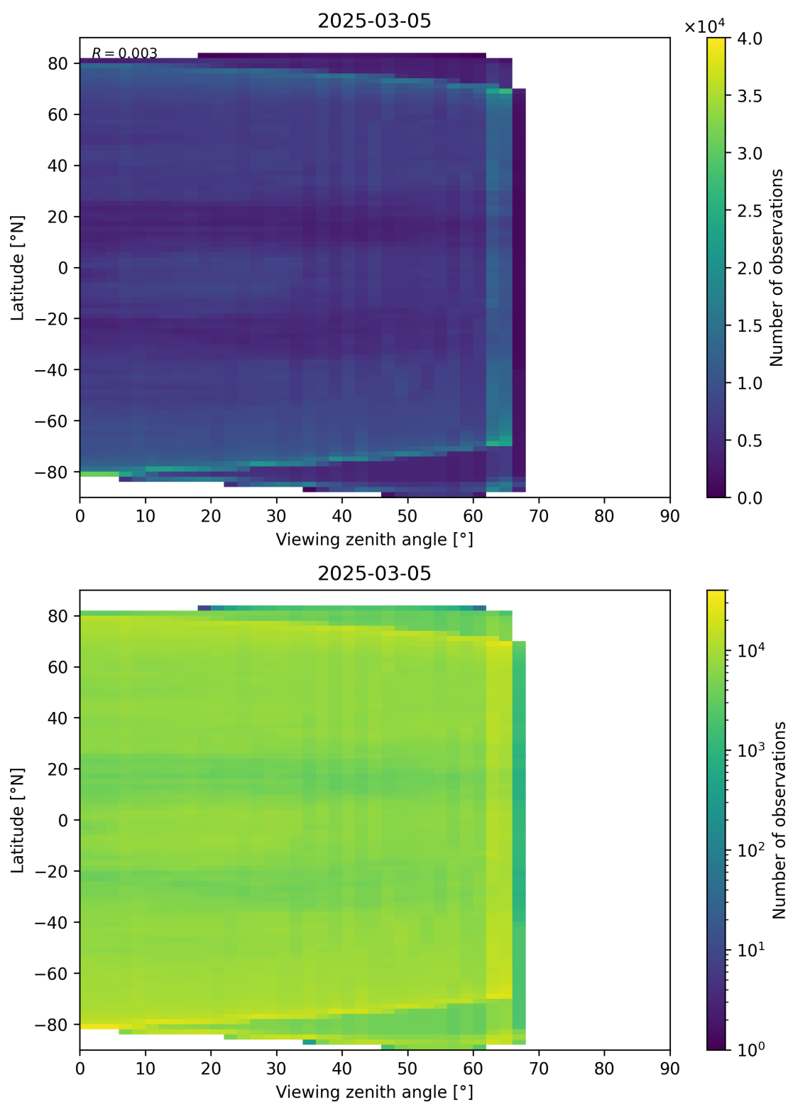
Figure 113: Scatter density plot of “Viewing zenith angle” against “Latitude” for 2025-03-04 to 2025-03-06.
