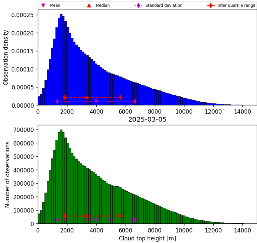
Figure 40: Histogram of “Cloud top height” for 2025-03-04 to 2025-03-06
