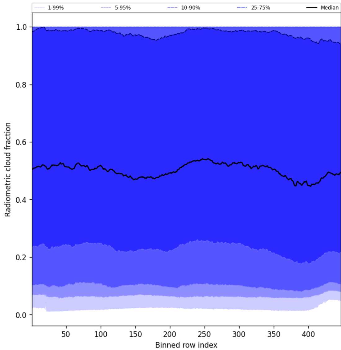
Figure 55: Along track statistics of “Radiometric cloud fraction” for 2025-03-04 to 2025-03-06
