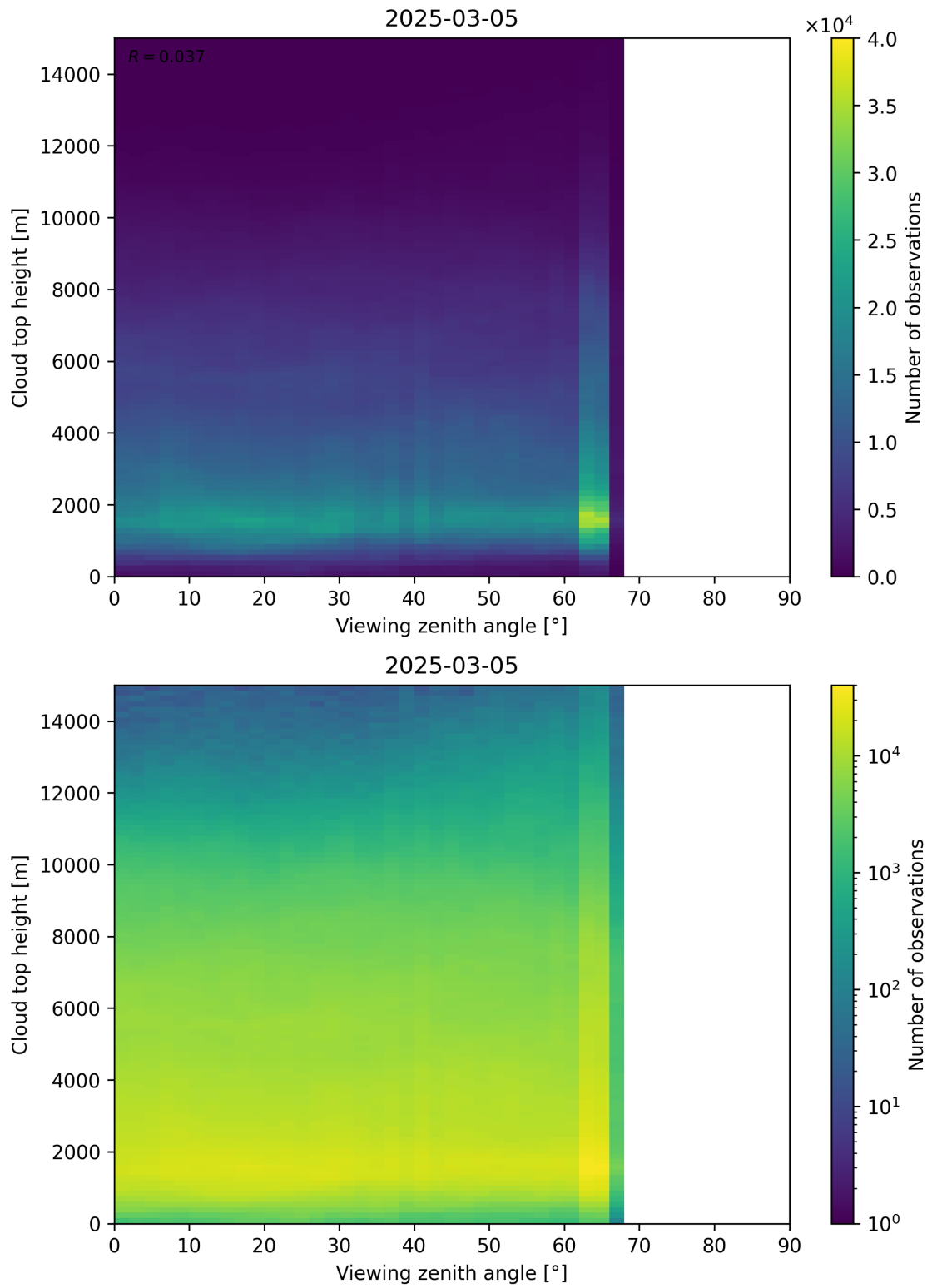
Figure 112: Scatter density plot of “Viewing zenith angle” against “Cloud top height” for 2025-03-04 to 2025-03-06.
