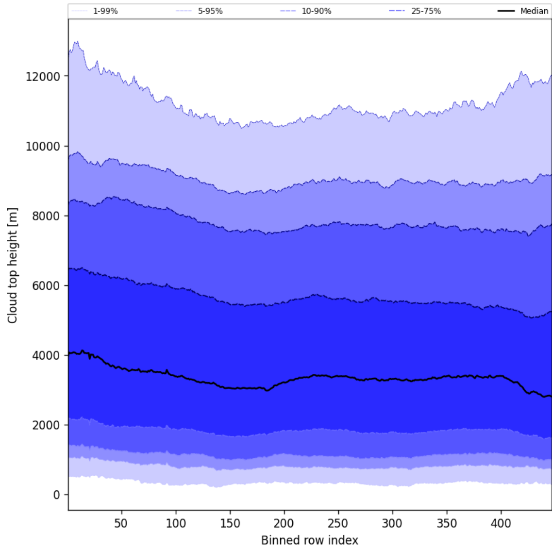
Figure 56: Along track statistics of “Cloud top height” for 2025-03-04 to 2025-03-06
