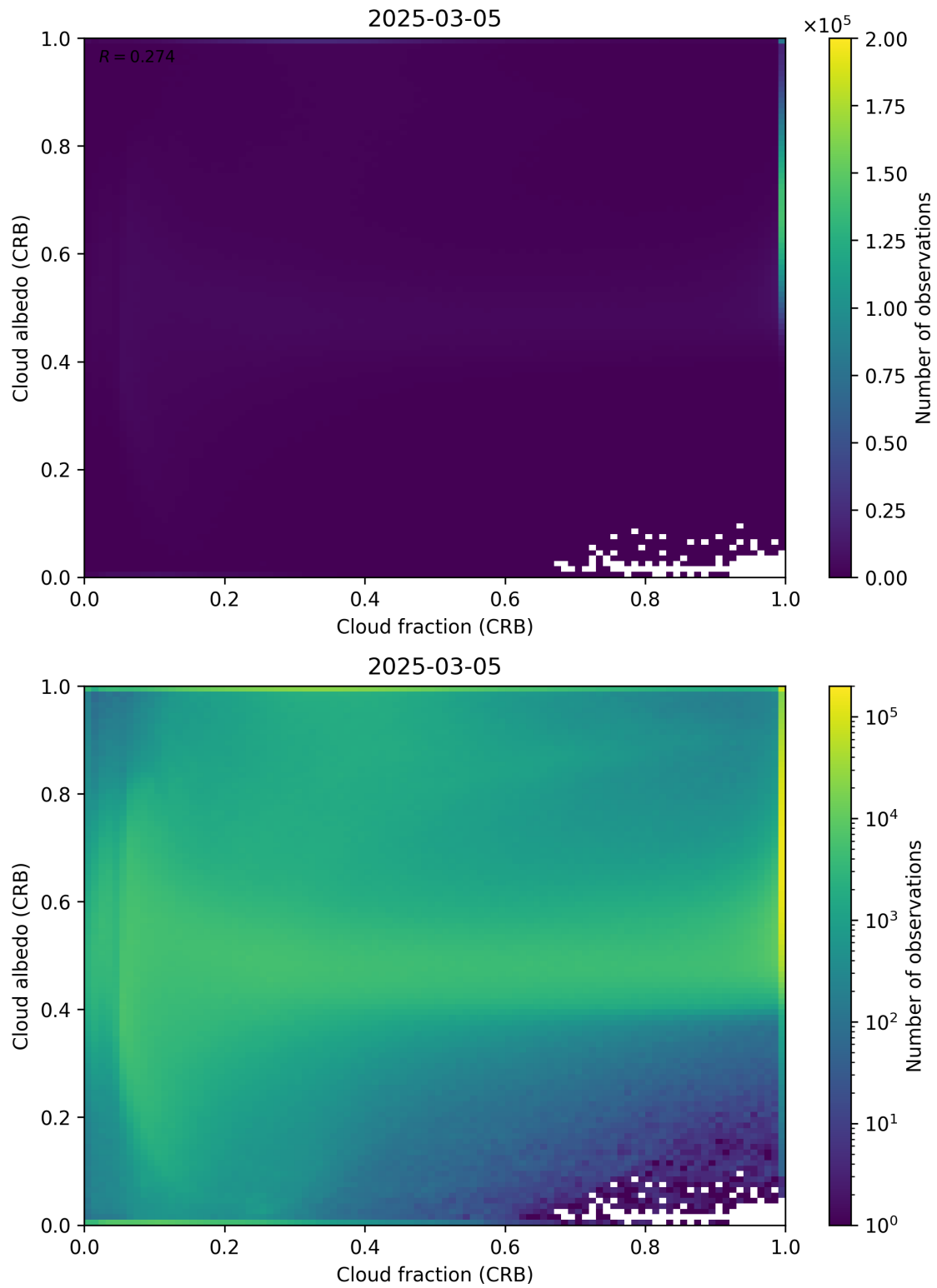
Figure 77: Scatter density plot of “Cloud fraction (CRB)” against “Cloud albedo (CRB)” for 2025-03-04 to 2025-03-06.
