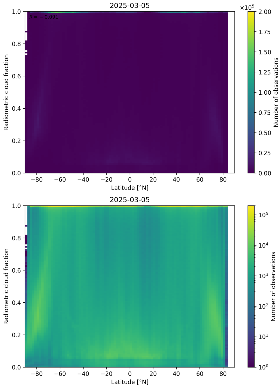
Figure 92: Scatter density plot of “Latitude” against “Radiometric cloud fraction” for 2025-03-04 to 2025-03-06.
