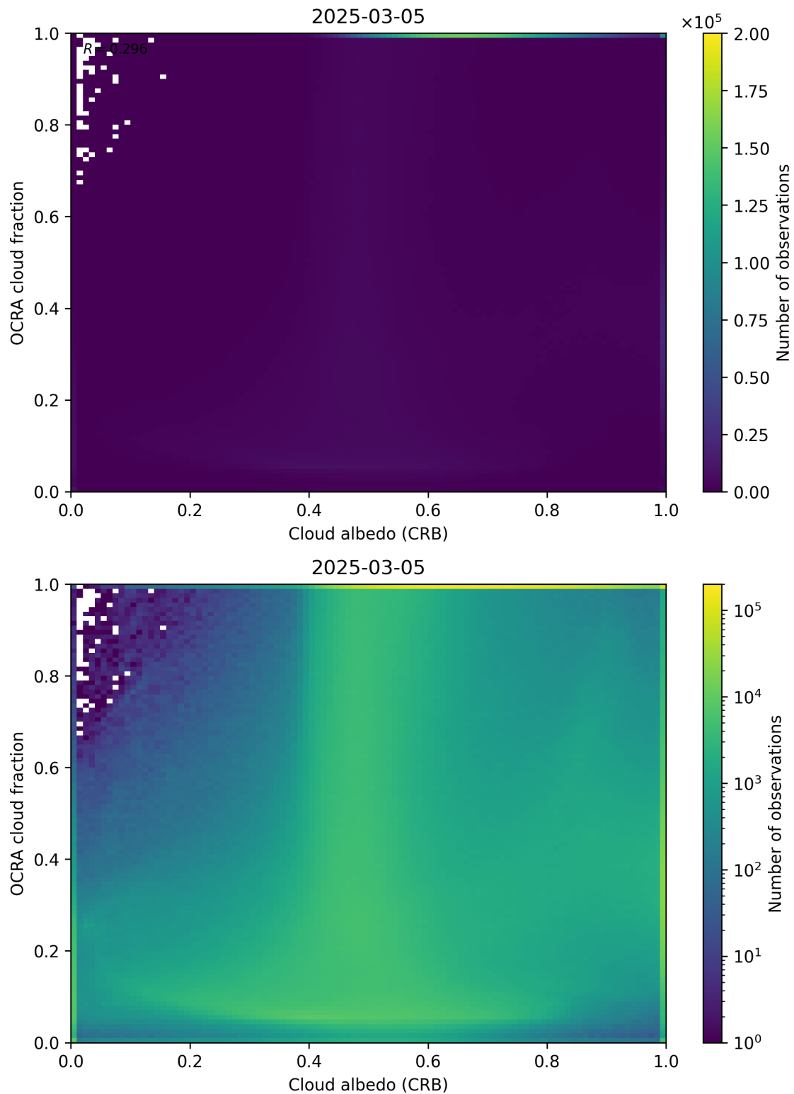
Figure 70: Scatter density plot of “Cloud albedo (CRB)” against “OCRA cloud fraction” for 2025-03-04 to 2025-03-06.
