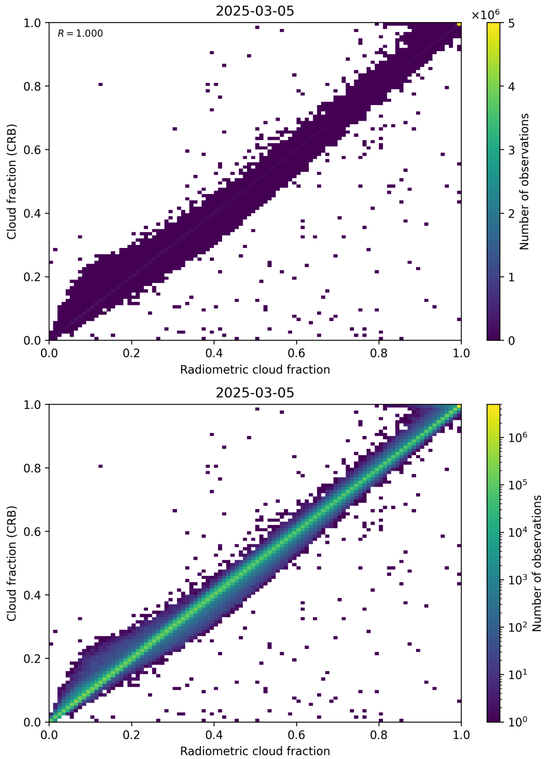
Figure 73: Scatter density plot of “Radiometric cloud fraction” against “Cloud fraction (CRB)” for 2025-03-04 to 2025-03-06.
