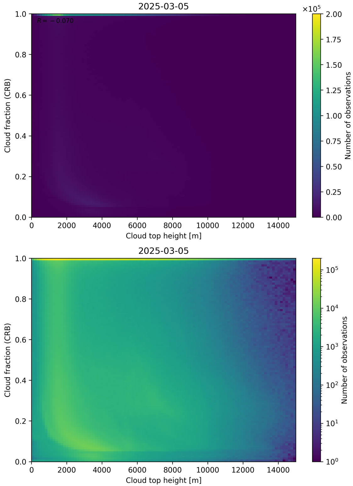
Figure 88: Scatter density plot of “Cloud top height” against “Cloud fraction (CRB)” for 2025-03-04 to 2025-03-06.
