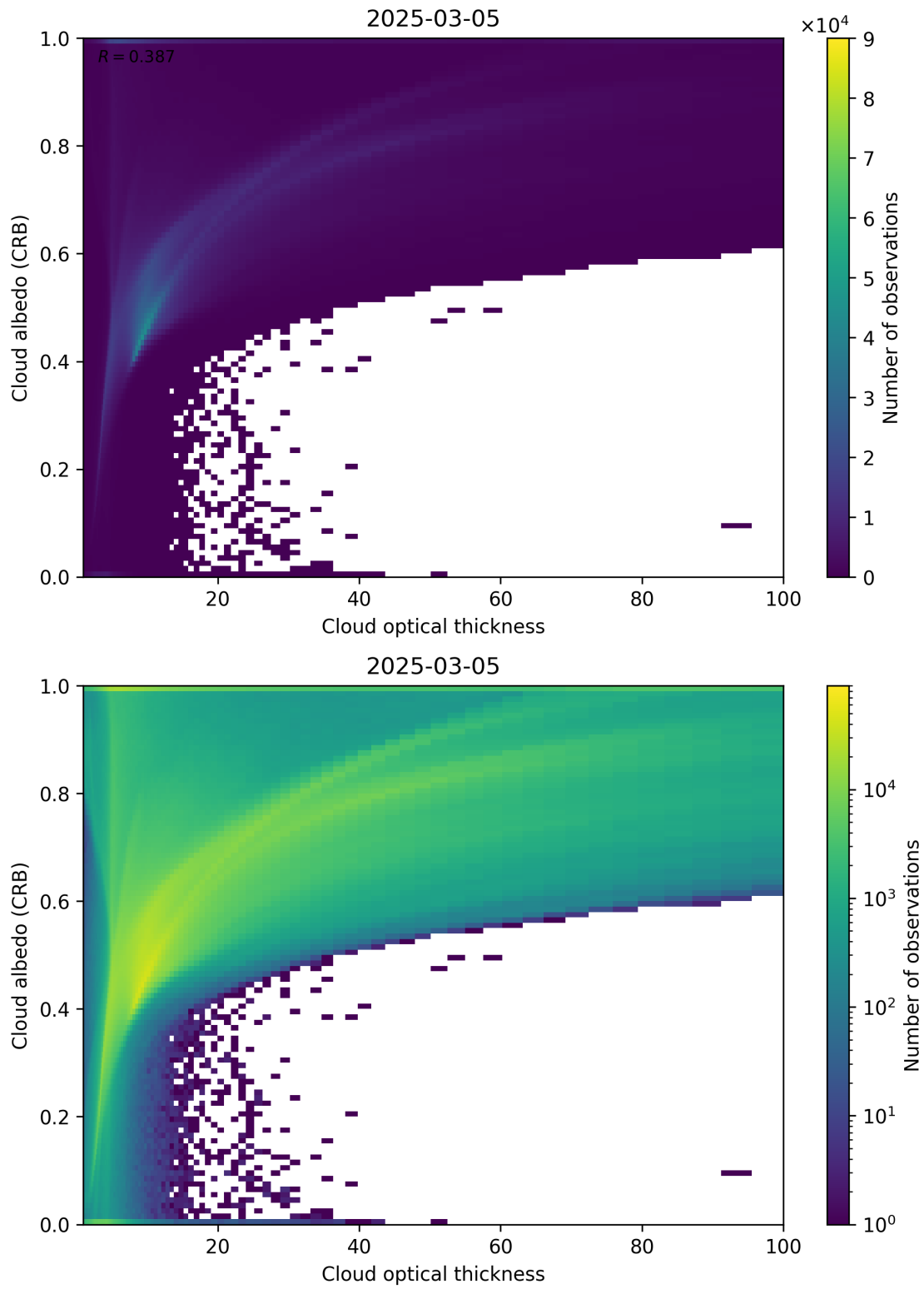
Figure 82: Scatter density plot of “Cloud optical thickness” against “Cloud albedo (CRB)” for 2025-03-04 to 2025-03-06.
