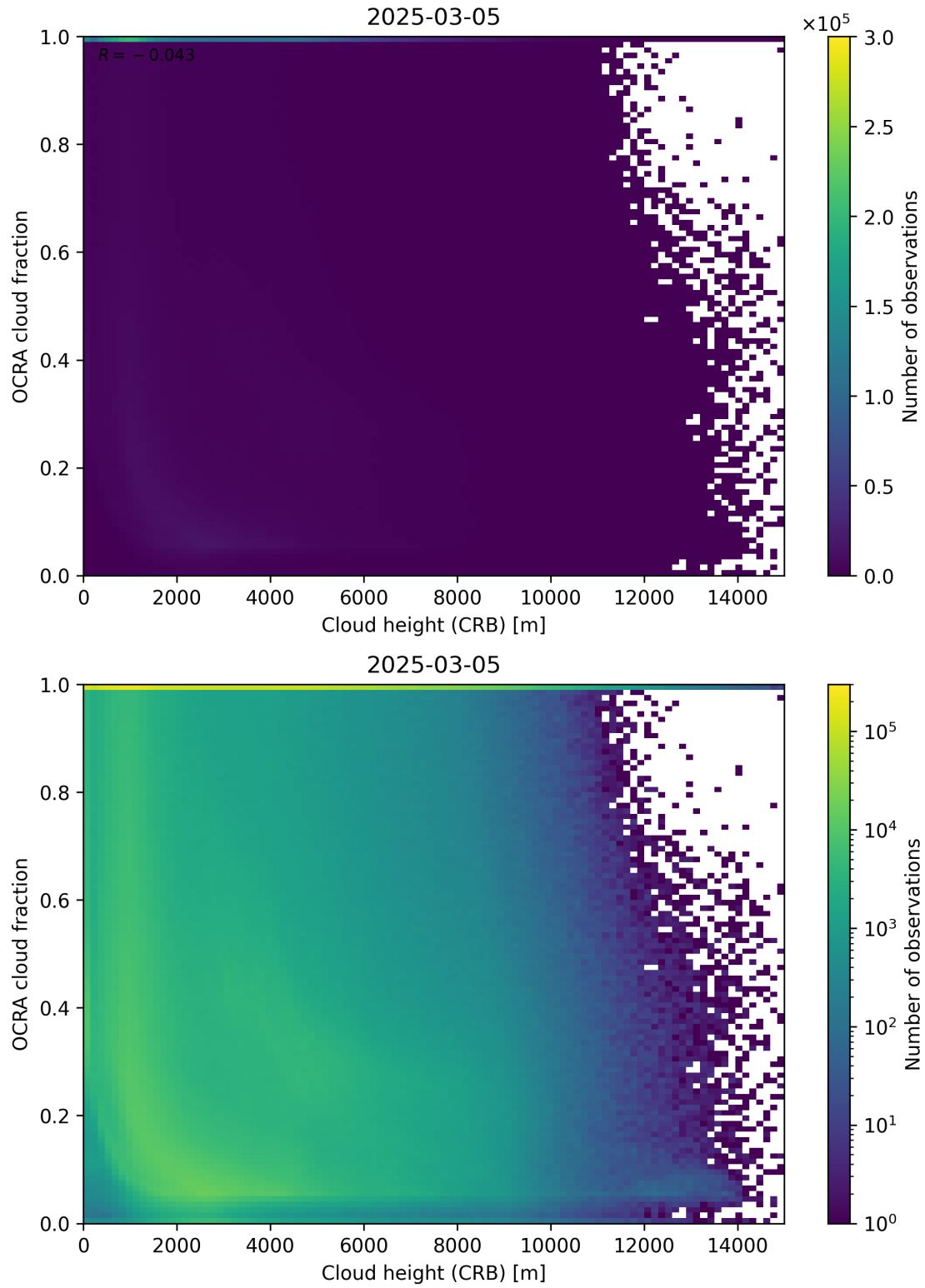
Figure 81: Scatter density plot of “Cloud height (CRB)” against “OCRA cloud fraction” for 2025-03-04 to 2025-03-06.
