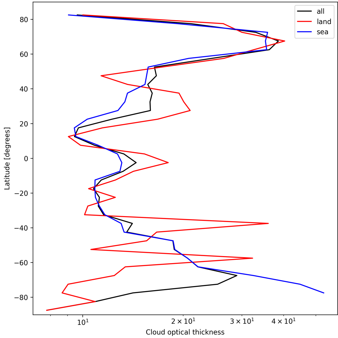
Figure 25: Zonal average of “Cloud optical thickness” for 2025-03-04 to 2025-03-06.
