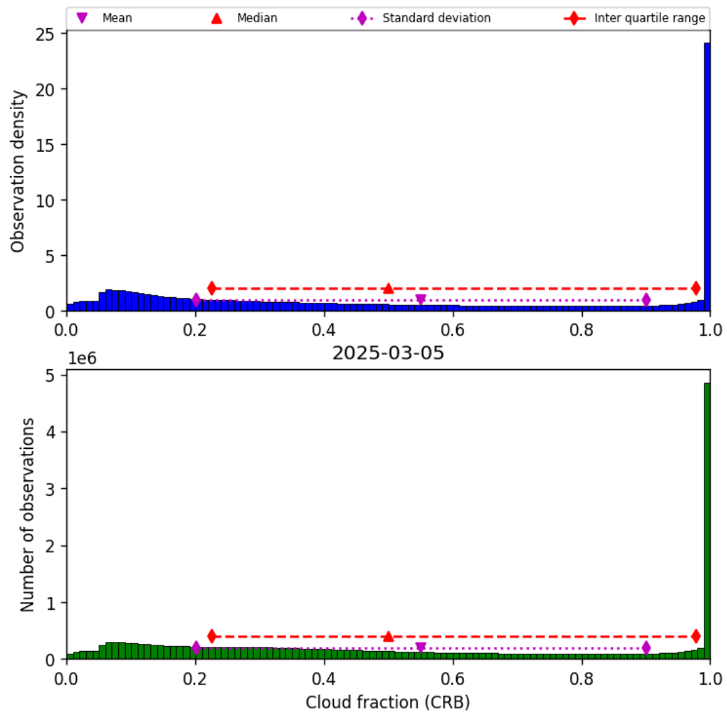
Figure 42: Histogram of “Cloud fraction (CRB)” for 2025-03-04 to 2025-03-06
