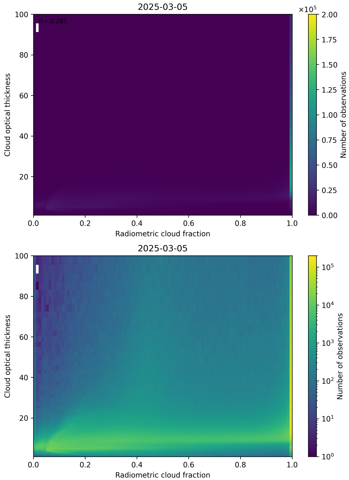
Figure 75: Scatter density plot of “Radiometric cloud fraction” against “Cloud optical thickness” for 2025-03-04 to 2025-03-06.
