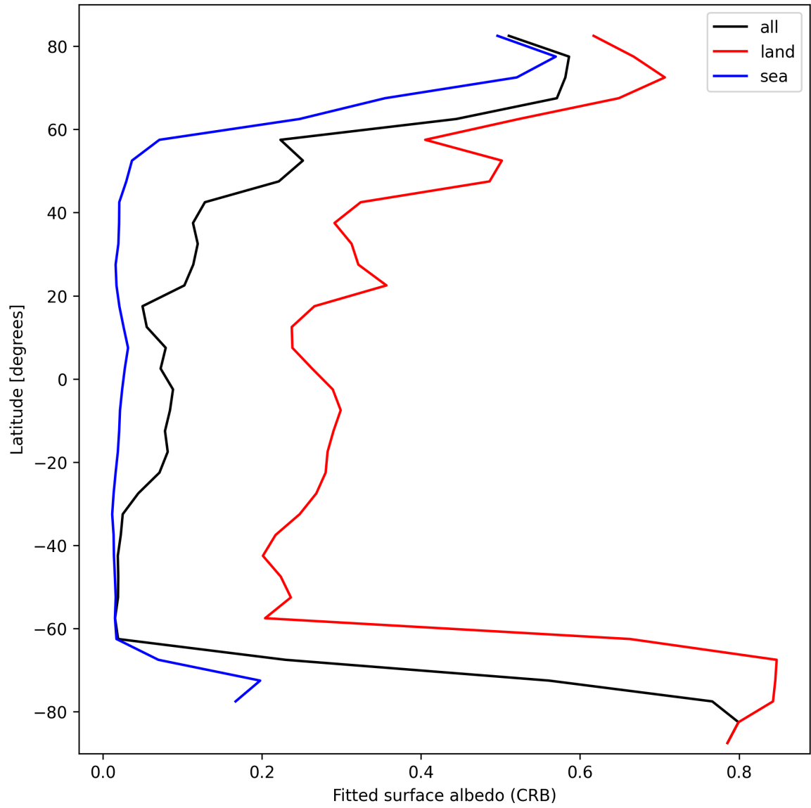
Figure 30: Zonal average of “Fitted surface albedo (CRB)” for 2025-03-04 to 2025-03-06.
