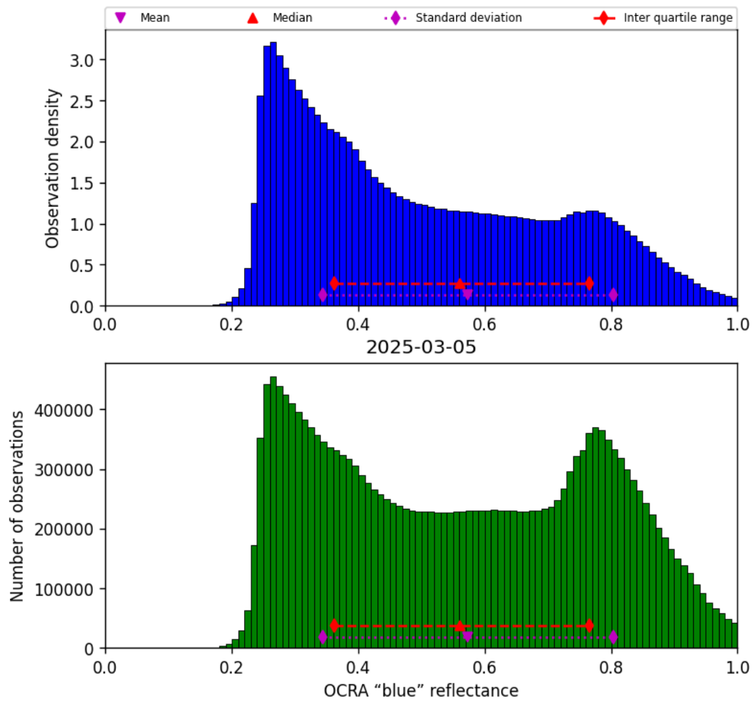
Figure 51: Histogram of “OCRA “blue” reflectance” for 2025-03-04 to 2025-03-06
