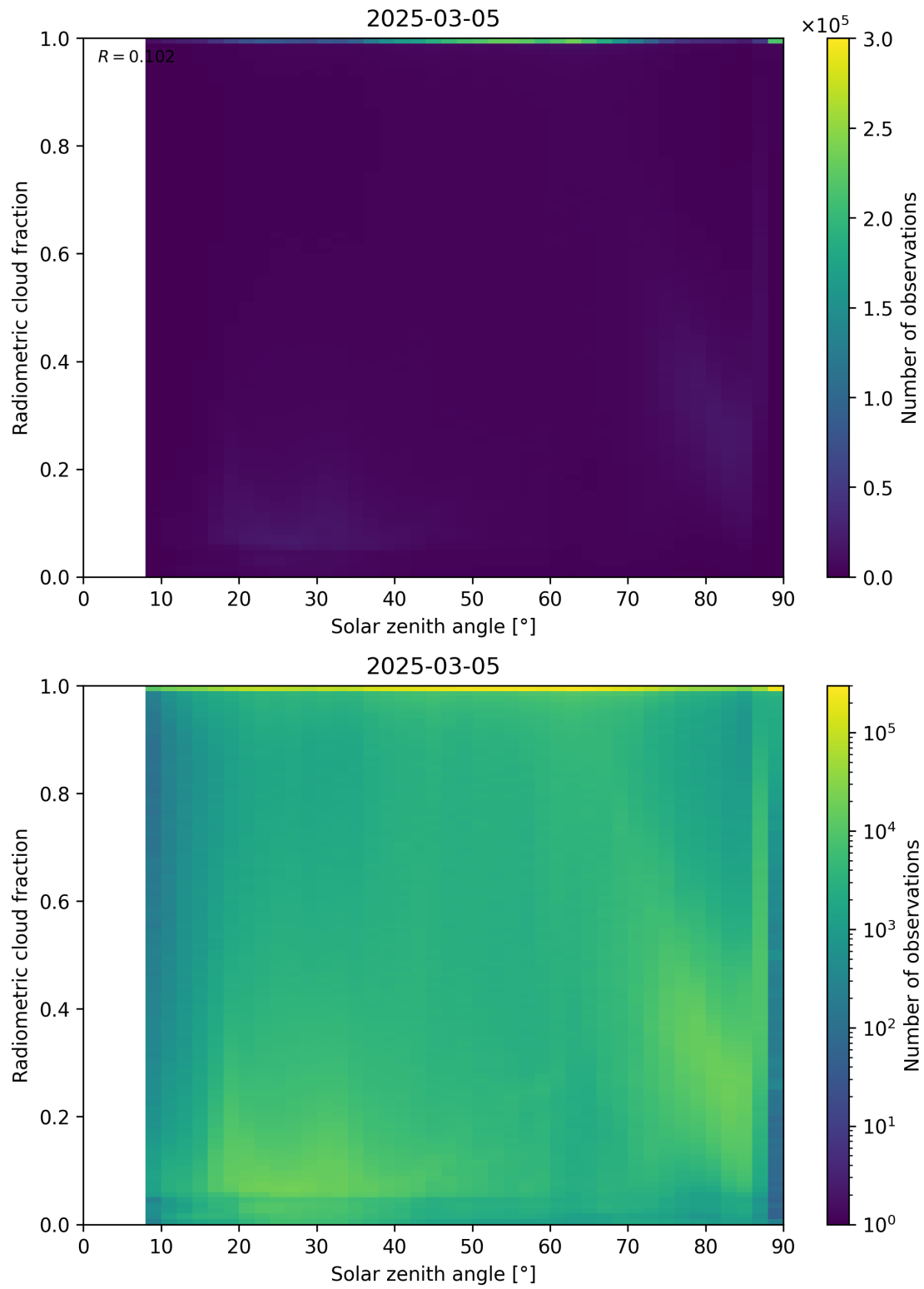
Figure 99: Scatter density plot of “Solar zenith angle” against “Radiometric cloud fraction” for 2025-03-04 to 2025-03-06.
