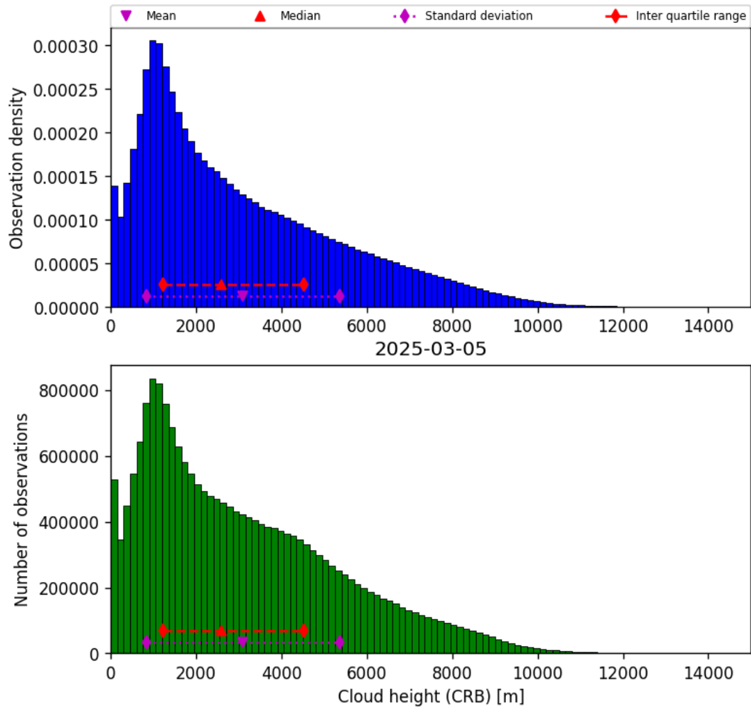
Figure 43: Histogram of “Cloud height (CRB)” for 2025-03-04 to 2025-03-06
