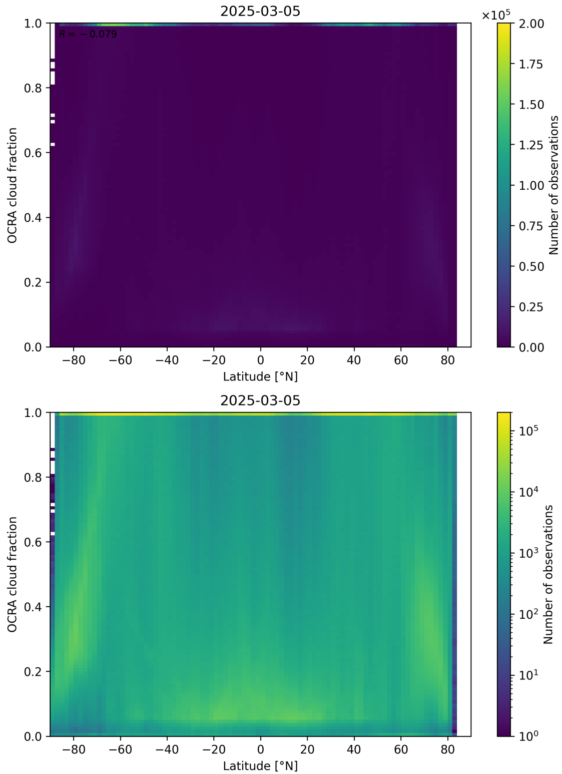
Figure 93: Scatter density plot of “Latitude” against “OCRA cloud fraction” for 2025-03-04 to 2025-03-06.
