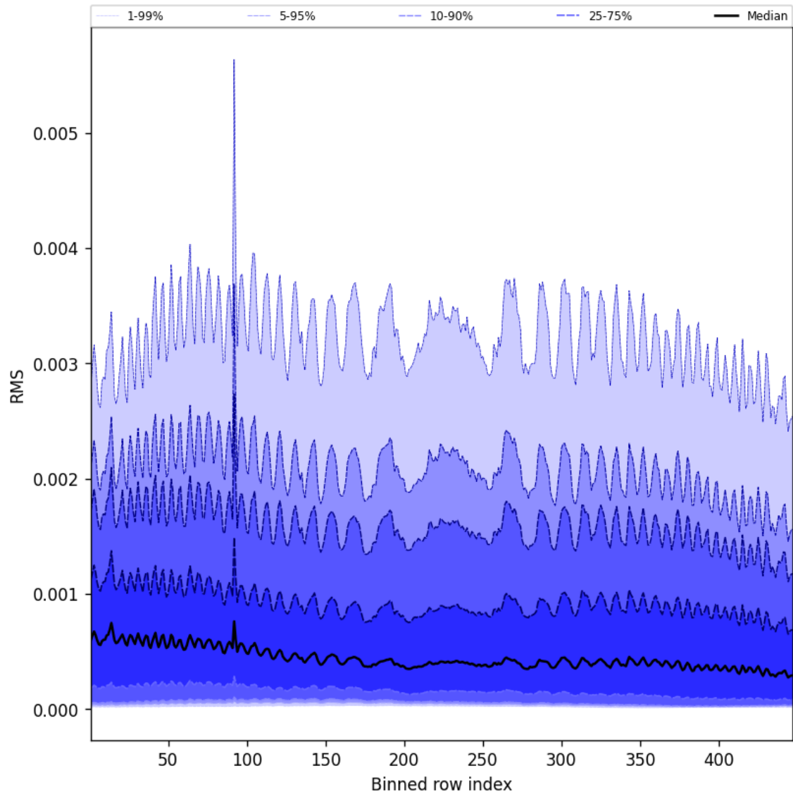
Figure 63: Along track statistics of “RMS” for 2025-03-04 to 2025-03-06
