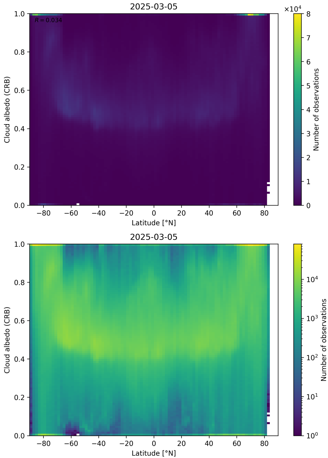
Figure 91: Scatter density plot of “Latitude” against “Cloud albedo (CRB)” for 2025-03-04 to 2025-03-06.
