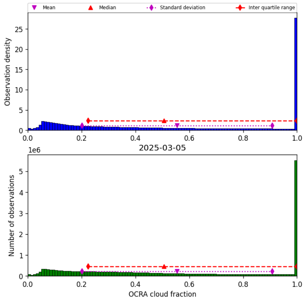
Figure 50: Histogram of “OCRA cloud fraction” for 2025-03-04 to 2025-03-06
