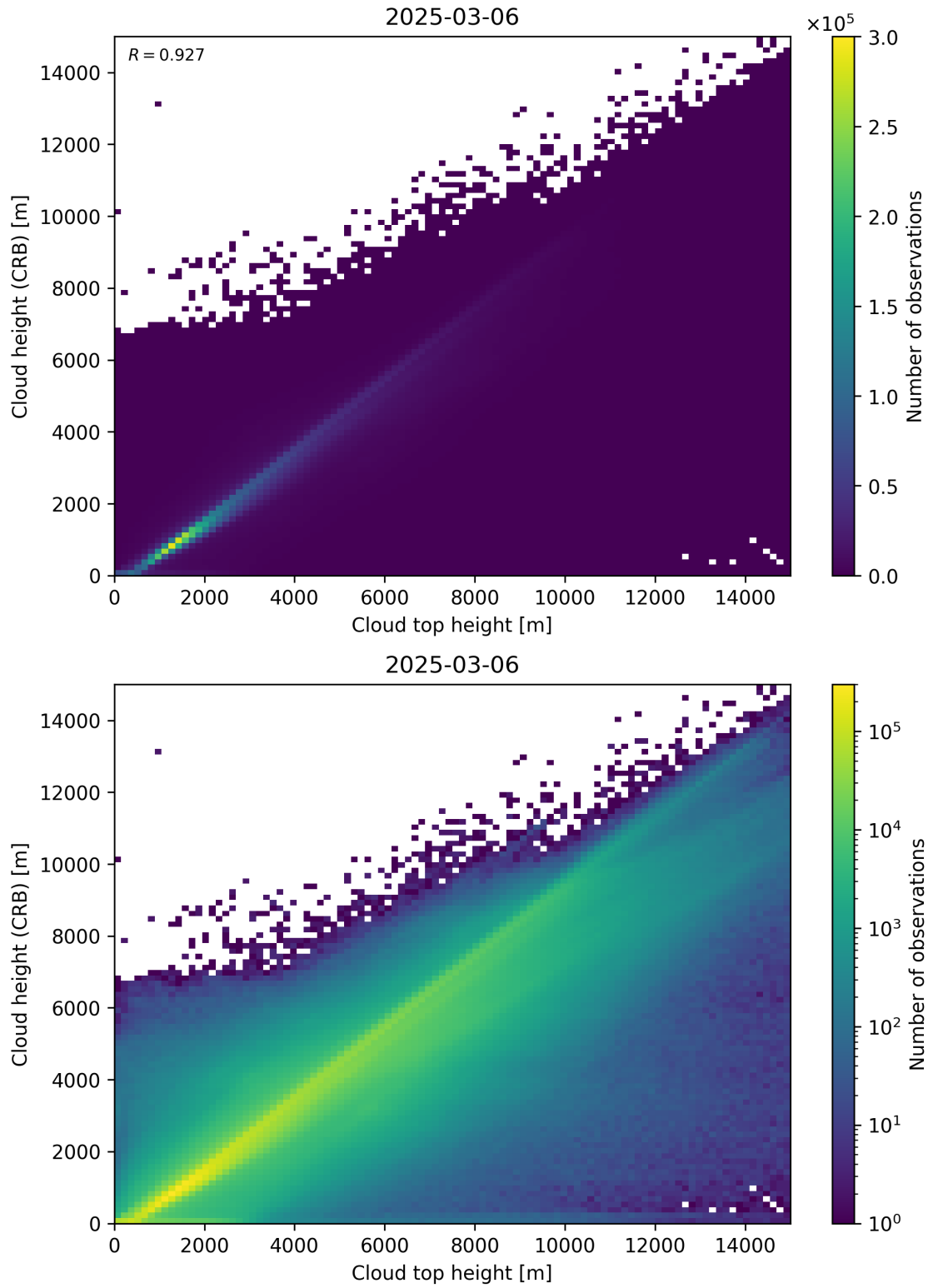
Figure 89: Scatter density plot of “Cloud top height” against “Cloud height (CRB)” for 2025-03-05 to 2025-03-07.
