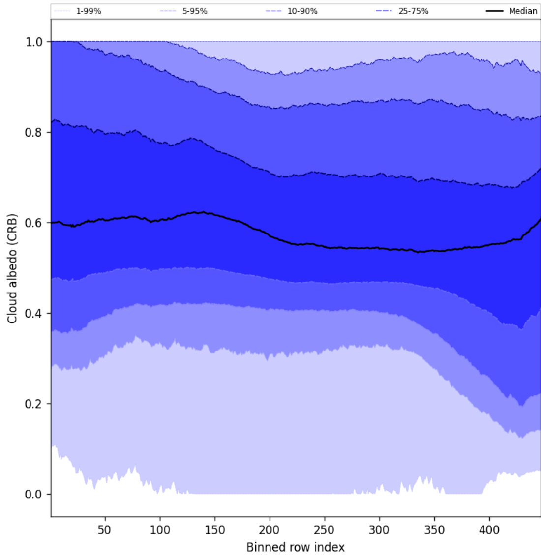
Figure 60: Along track statistics of “Cloud albedo (CRB)” for 2025-03-05 to 2025-03-07
