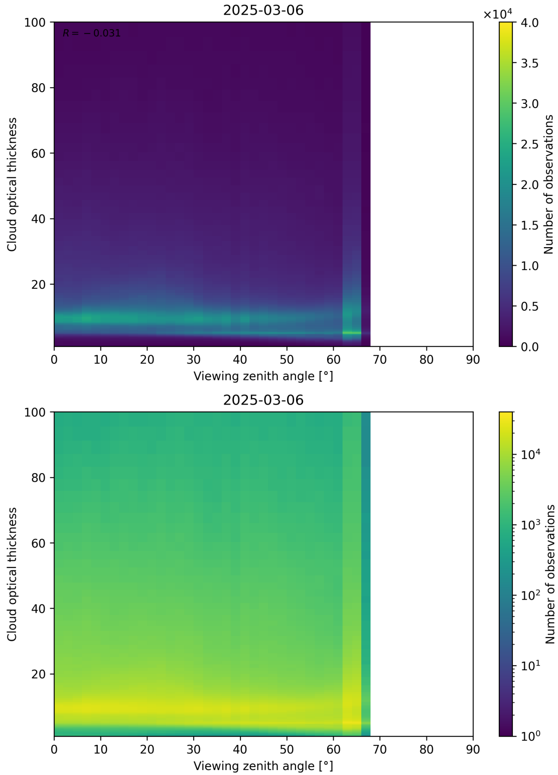
Figure 111: Scatter density plot of “Viewing zenith angle” against “Cloud optical thickness” for 2025-03-05 to 2025-03-07.
