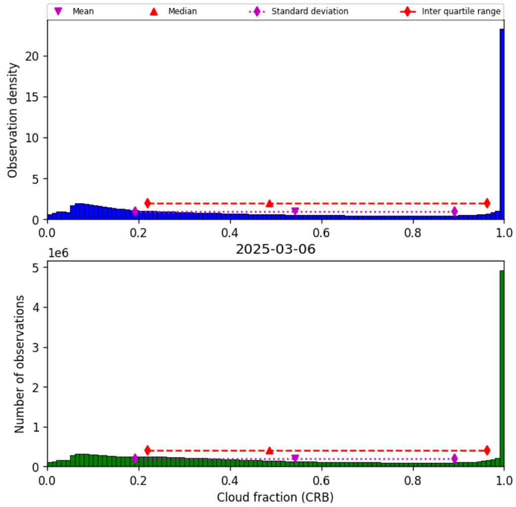
Figure 42: Histogram of “Cloud fraction (CRB)” for 2025-03-05 to 2025-03-07
