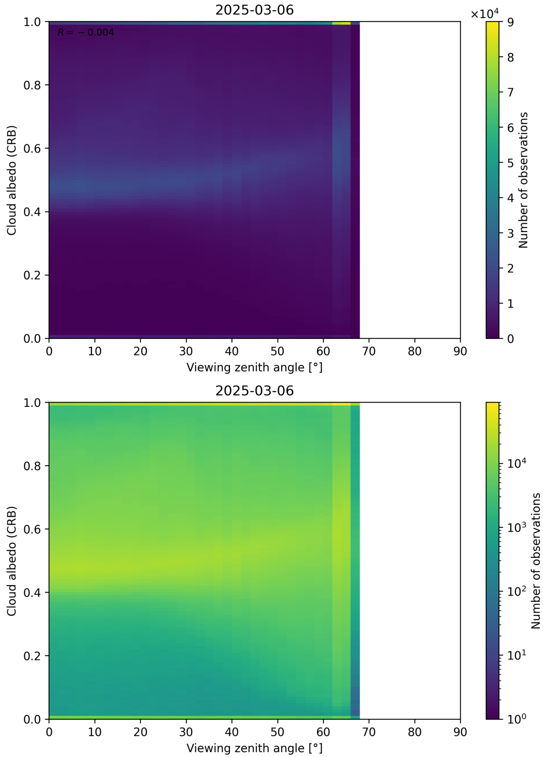
Figure 106: Scatter density plot of “Viewing zenith angle” against “Cloud albedo (CRB)” for 2025-03-05 to 2025-03-07.
