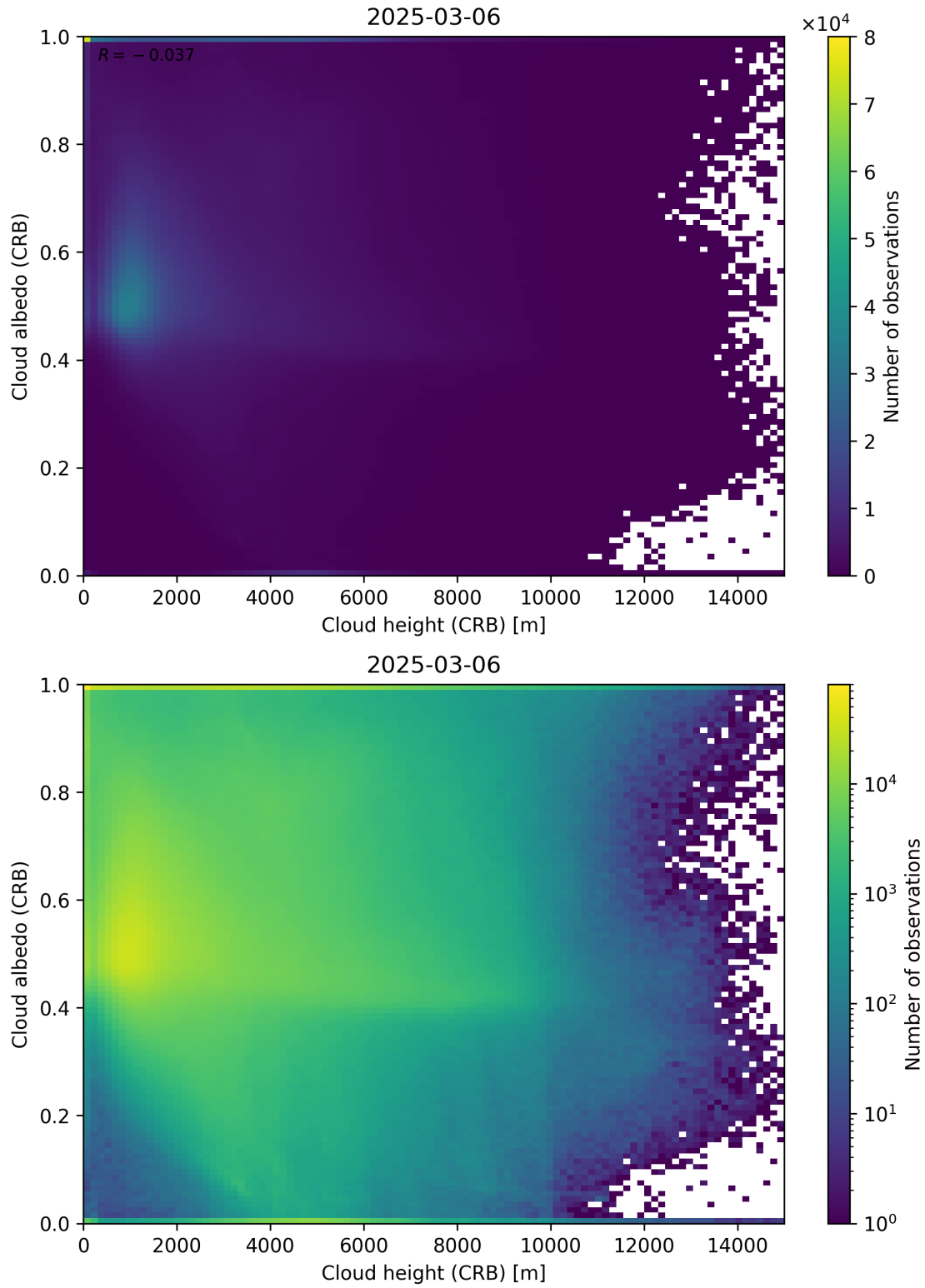
Figure 80: Scatter density plot of “Cloud height (CRB)” against “Cloud albedo (CRB)” for 2025-03-05 to 2025-03-07.
