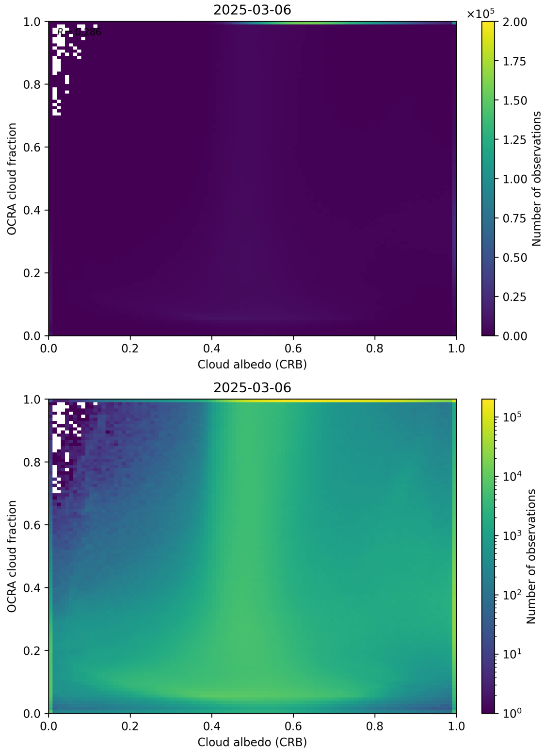
Figure 70: Scatter density plot of “Cloud albedo (CRB)” against “OCRA cloud fraction” for 2025-03-05 to 2025-03-07.
