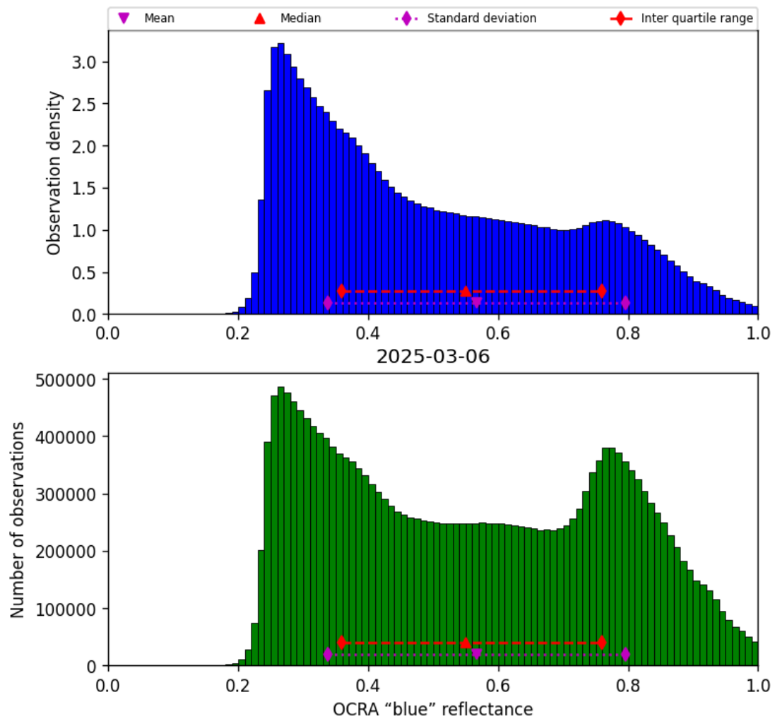
Figure 51: Histogram of “OCRA “blue” reflectance” for 2025-03-05 to 2025-03-07
