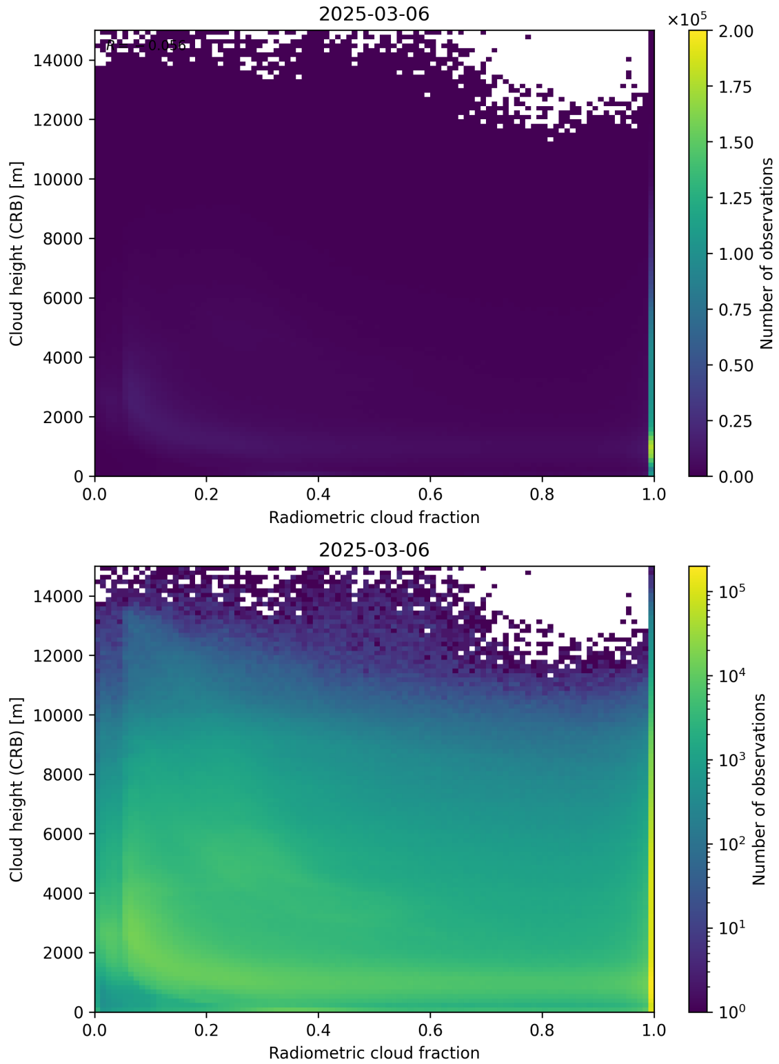
Figure 74: Scatter density plot of “Radiometric cloud fraction” against “Cloud height (CRB)” for 2025-03-05 to 2025-03-07.
