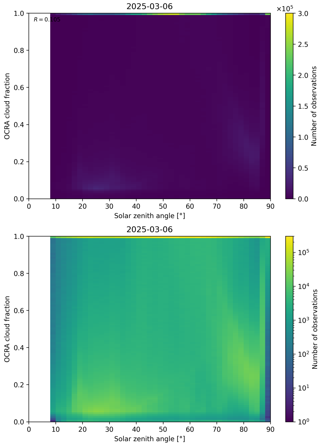
Figure 100: Scatter density plot of “Solar zenith angle” against “OCRA cloud fraction” for 2025-03-05 to 2025-03-07.
