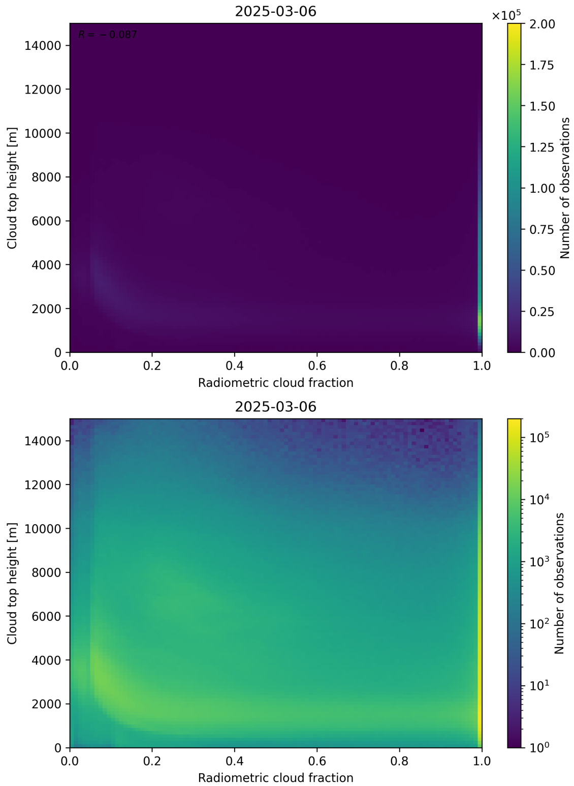
Figure 76: Scatter density plot of “Radiometric cloud fraction” against “Cloud top height” for 2025-03-05 to 2025-03-07.
