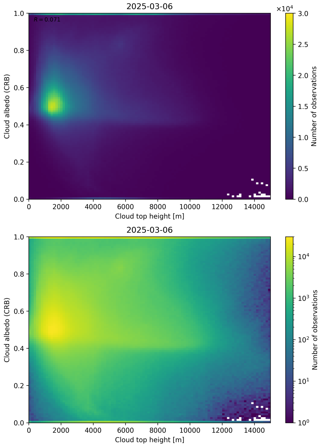
Figure 86: Scatter density plot of “Cloud top height” against “Cloud albedo (CRB)” for 2025-03-05 to 2025-03-07.
