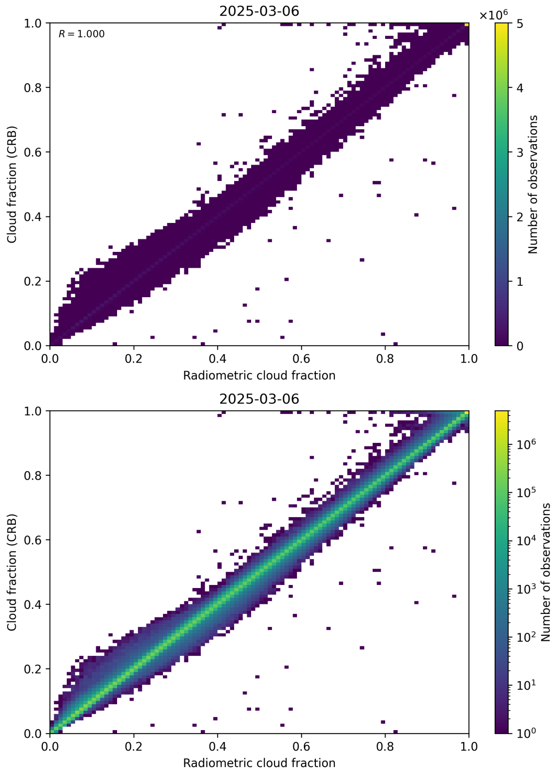
Figure 73: Scatter density plot of “Radiometric cloud fraction” against “Cloud fraction (CRB)” for 2025-03-05 to 2025-03-07.
