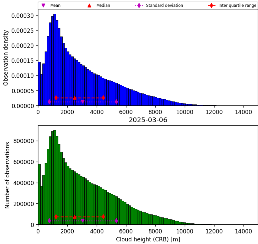
Figure 43: Histogram of “Cloud height (CRB)” for 2025-03-05 to 2025-03-07
