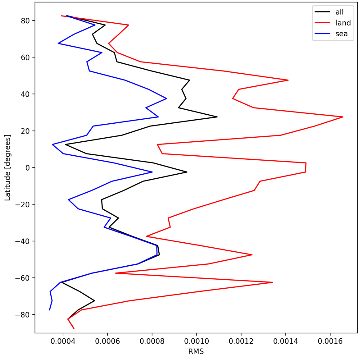
Figure 31: Zonal average of “RMS” for 2025-03-05 to 2025-03-07.
