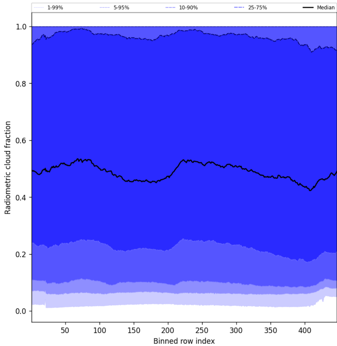
Figure 55: Along track statistics of “Radiometric cloud fraction” for 2025-03-05 to 2025-03-07
