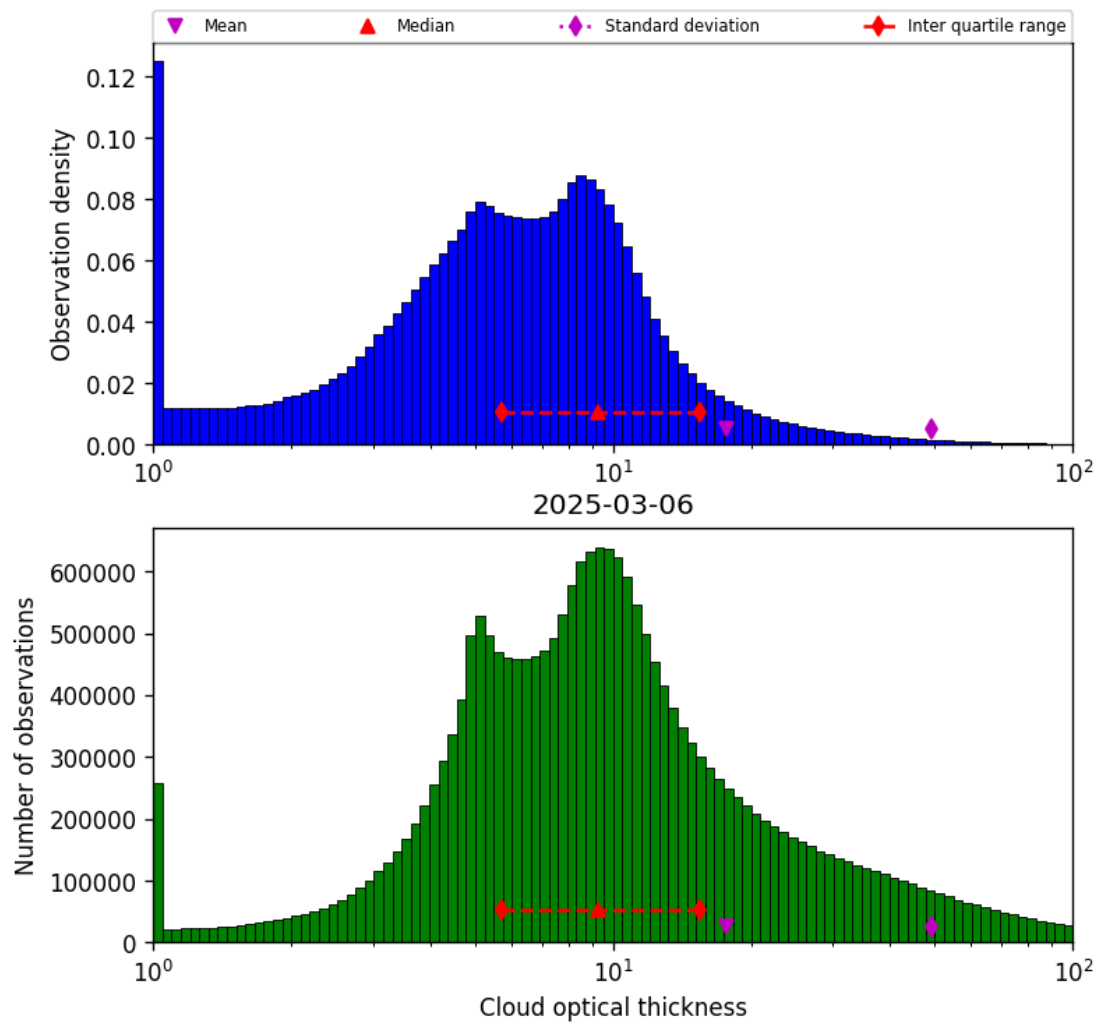
Figure 41: Histogram of “Cloud optical thickness” for 2025-03-05 to 2025-03-07
