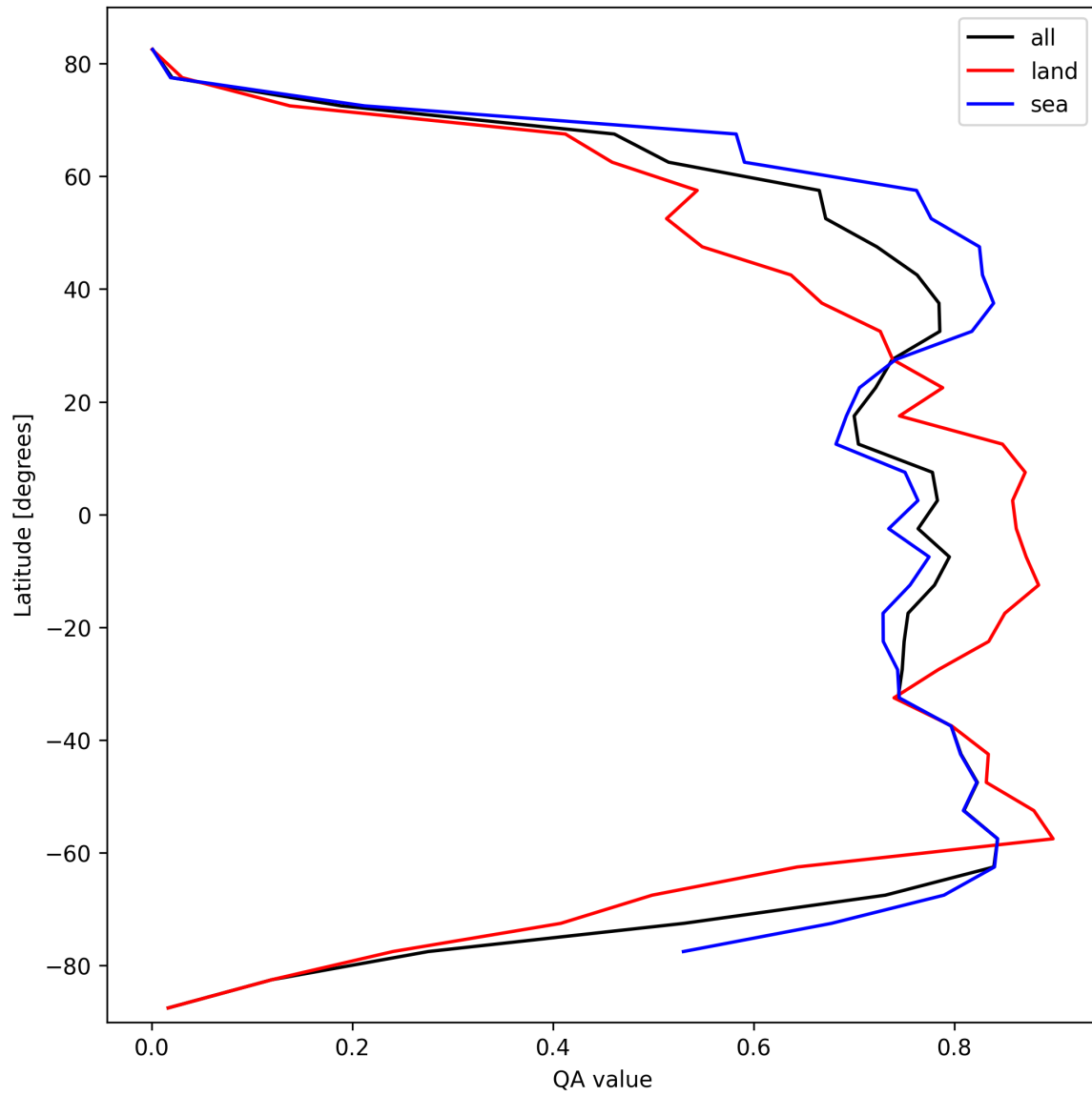
Figure 22: Zonal average of “QA value” for 2025-03-05 to 2025-03-07.
