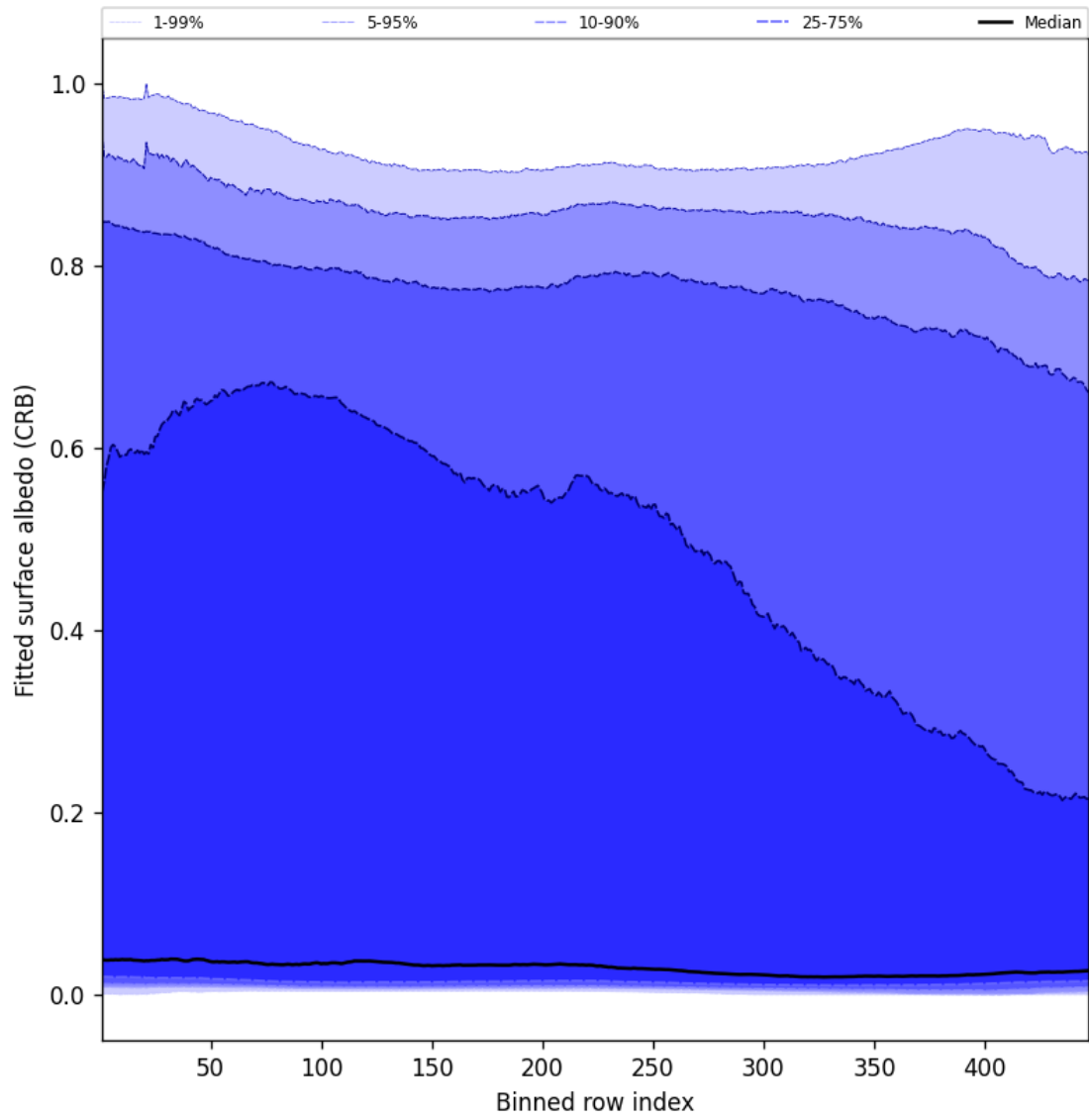
Figure 62: Along track statistics of “Fitted surface albedo (CRB)” for 2025-03-05 to 2025-03-07
