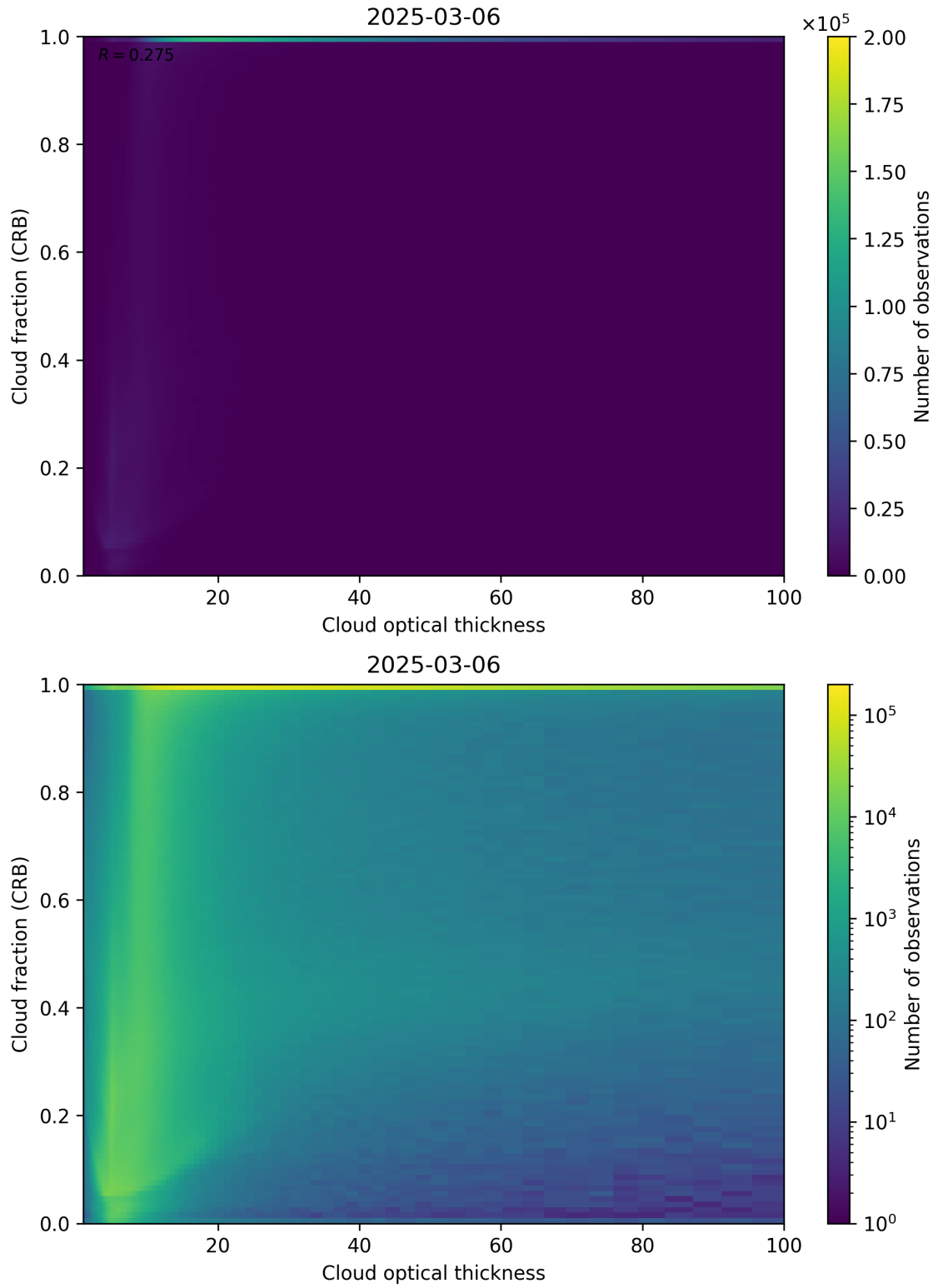
Figure 84: Scatter density plot of “Cloud optical thickness” against “Cloud fraction (CRB)” for 2025-03-05 to 2025-03-07.
