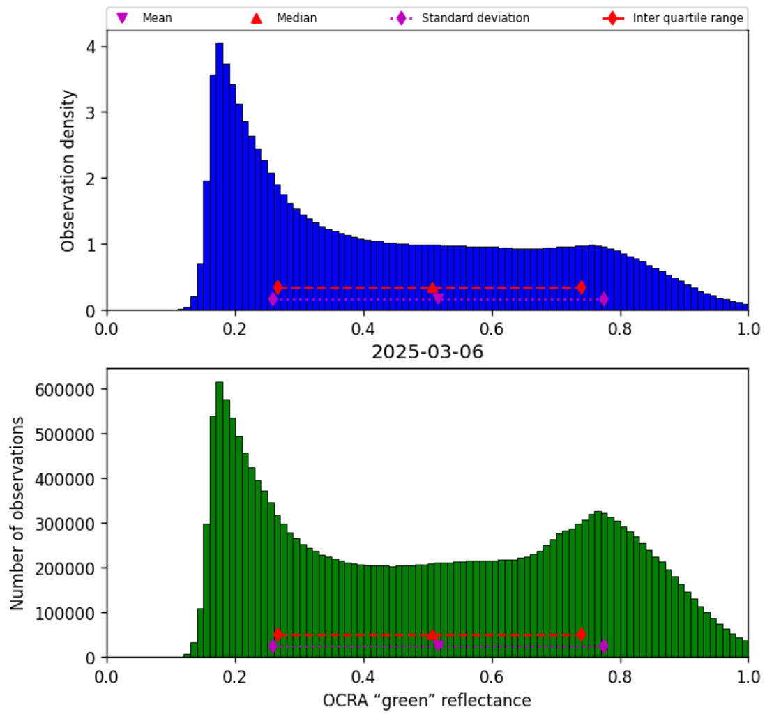
Figure 52: Histogram of “OCRA “green” reflectance” for 2025-03-05 to 2025-03-07
