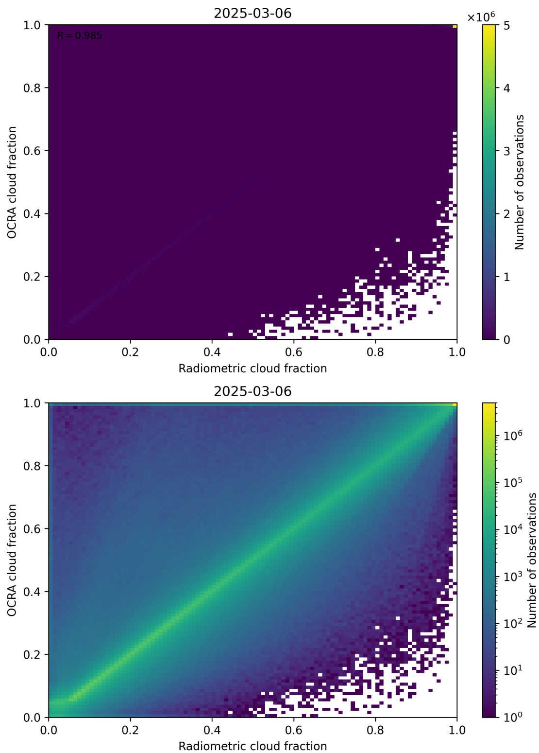
Figure 72: Scatter density plot of “Radiometric cloud fraction” against “OCRA cloud fraction” for 2025-03-05 to 2025-03-07.
