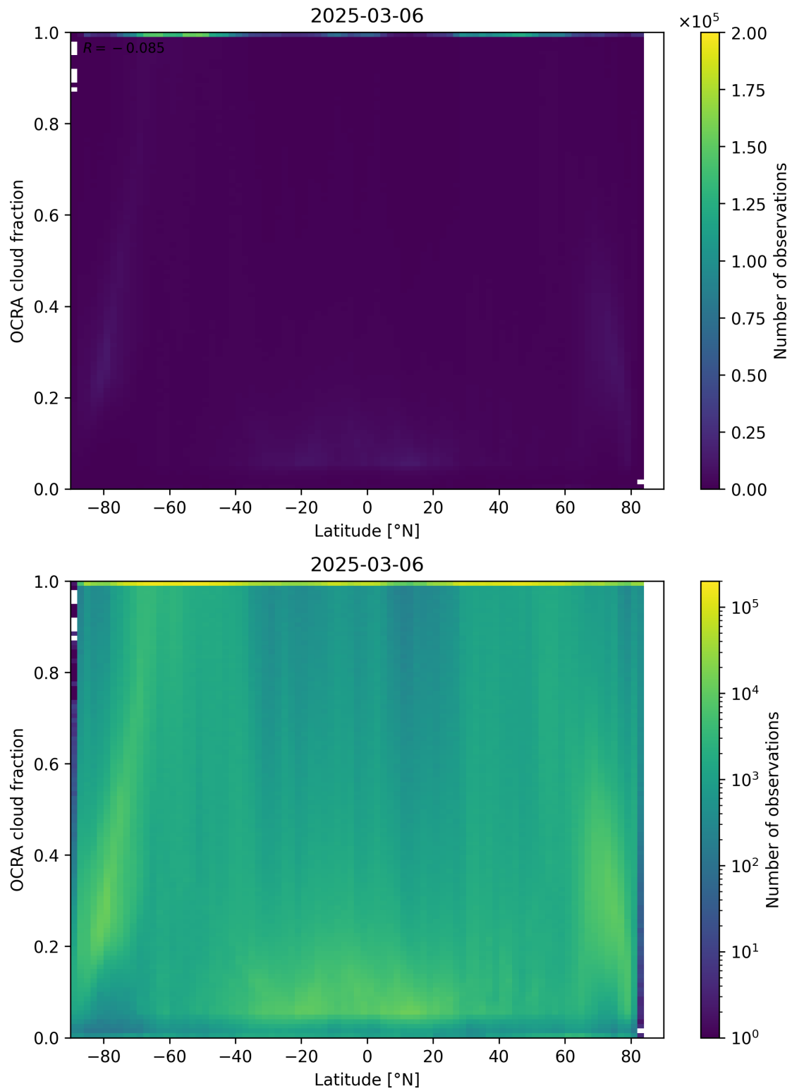
Figure 93: Scatter density plot of “Latitude” against “OCRA cloud fraction” for 2025-03-05 to 2025-03-07.
