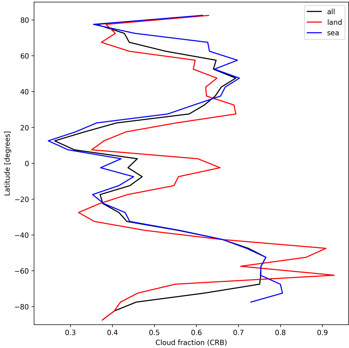
Figure 26: Zonal average of “Cloud fraction (CRB)” for 2025-03-05 to 2025-03-07.
