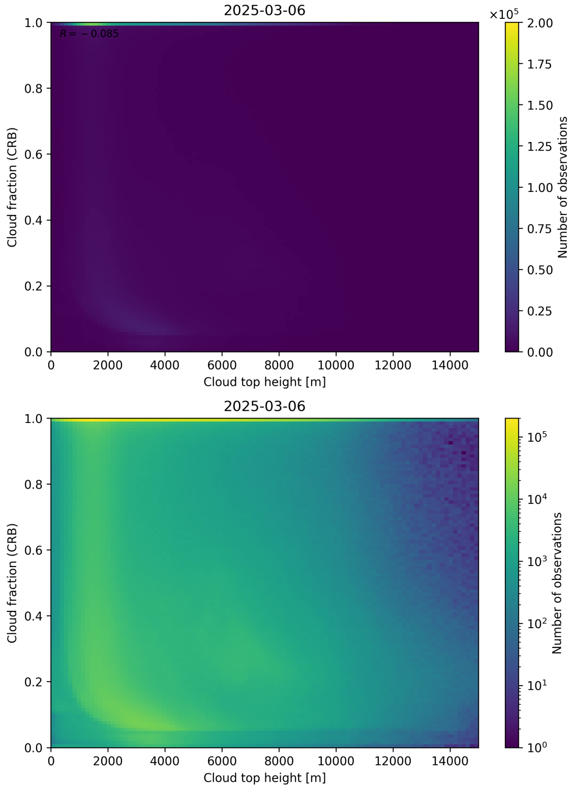
Figure 88: Scatter density plot of “Cloud top height” against “Cloud fraction (CRB)” for 2025-03-05 to 2025-03-07.
