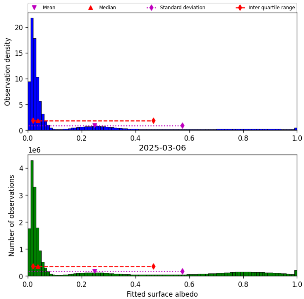
Figure 45: Histogram of “Fitted surface albedo” for 2025-03-05 to 2025-03-07
