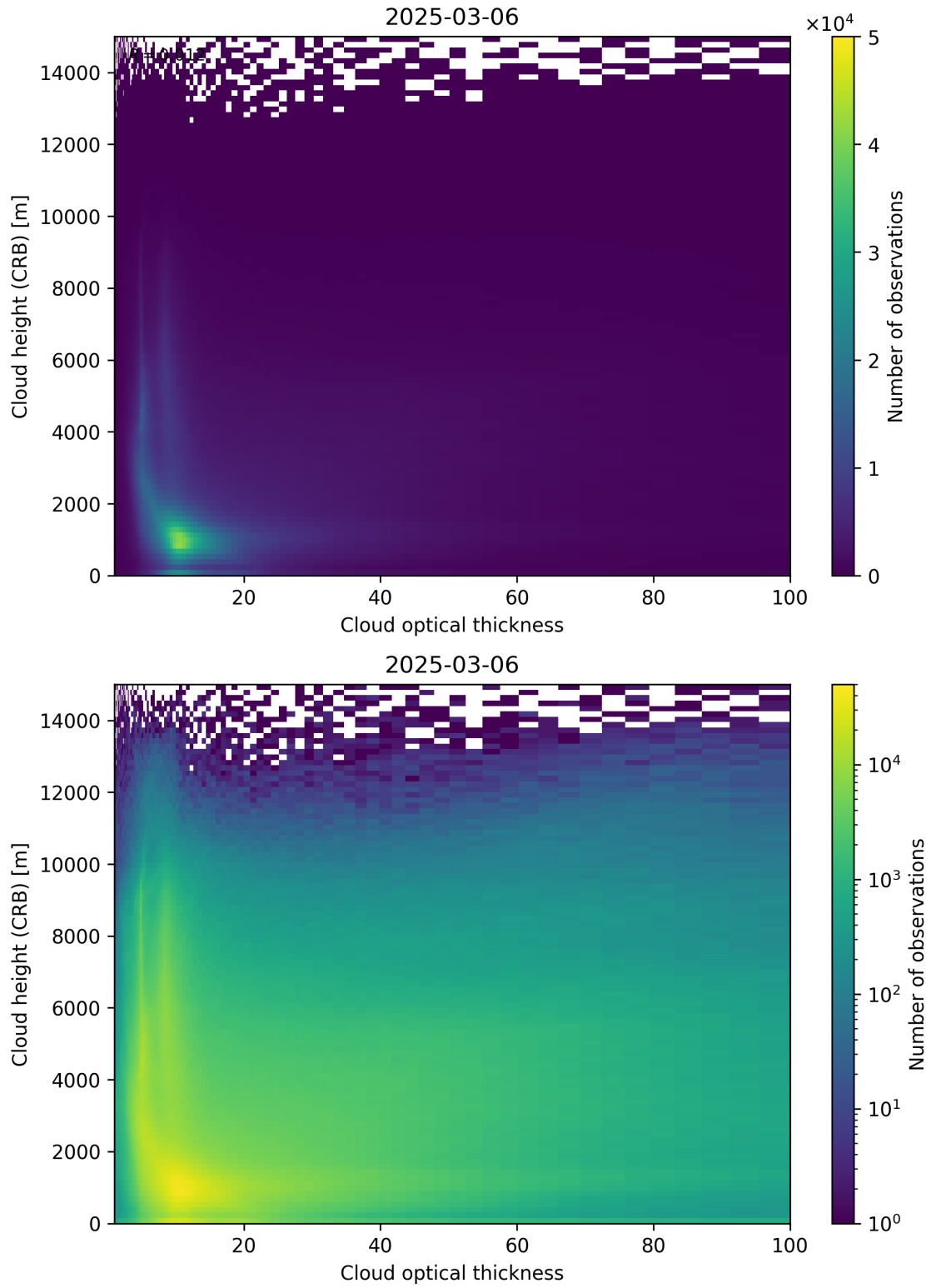
Figure 85: Scatter density plot of “Cloud optical thickness” against “Cloud height (CRB)” for 2025-03-05 to 2025-03-07.
