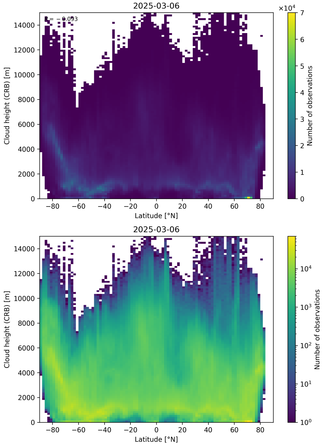
Figure 95: Scatter density plot of “Latitude” against “Cloud height (CRB)” for 2025-03-05 to 2025-03-07.
