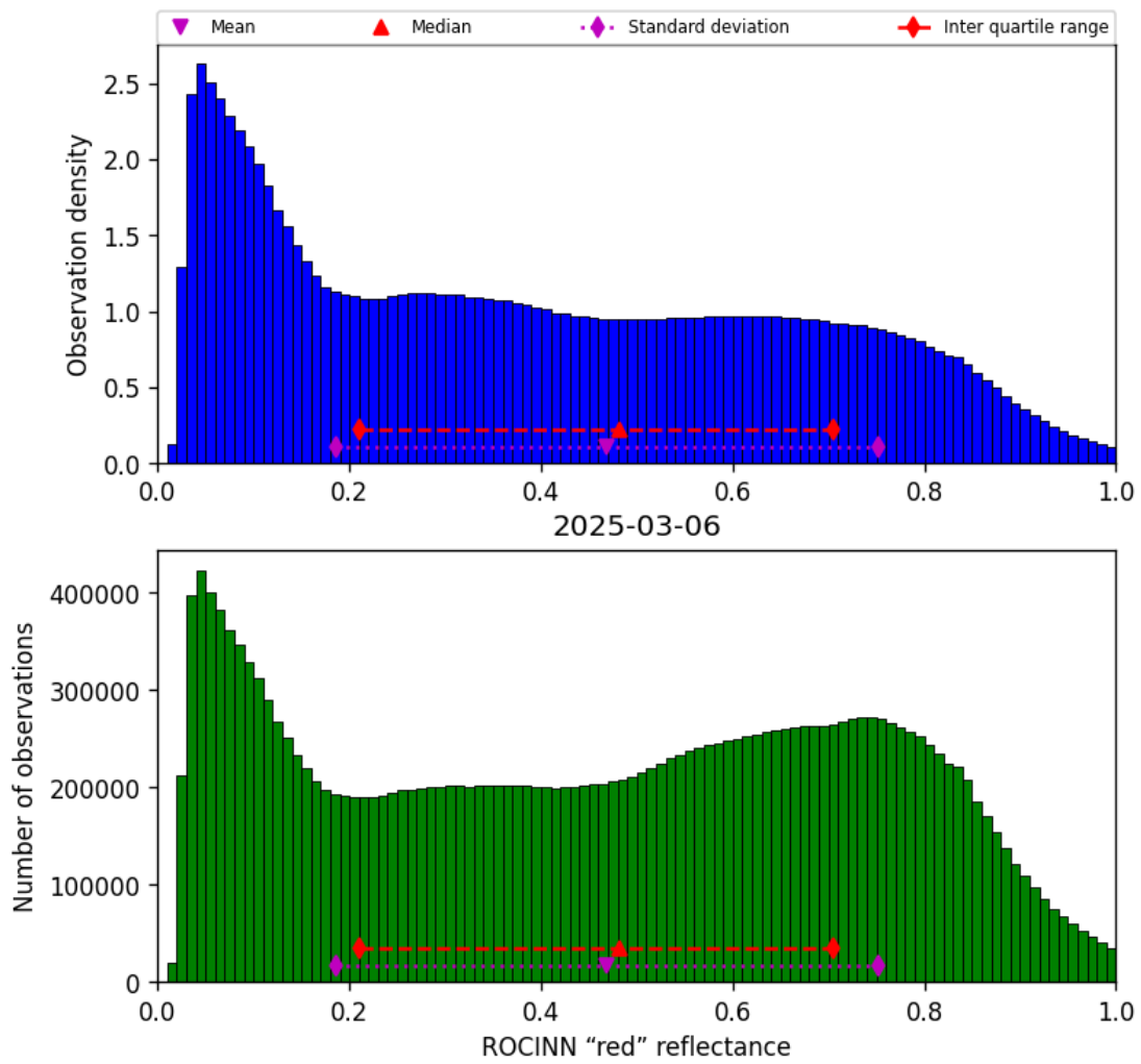
Figure 53: Histogram of “ROCINN “red” reflectance” for 2025-03-05 to 2025-03-07
