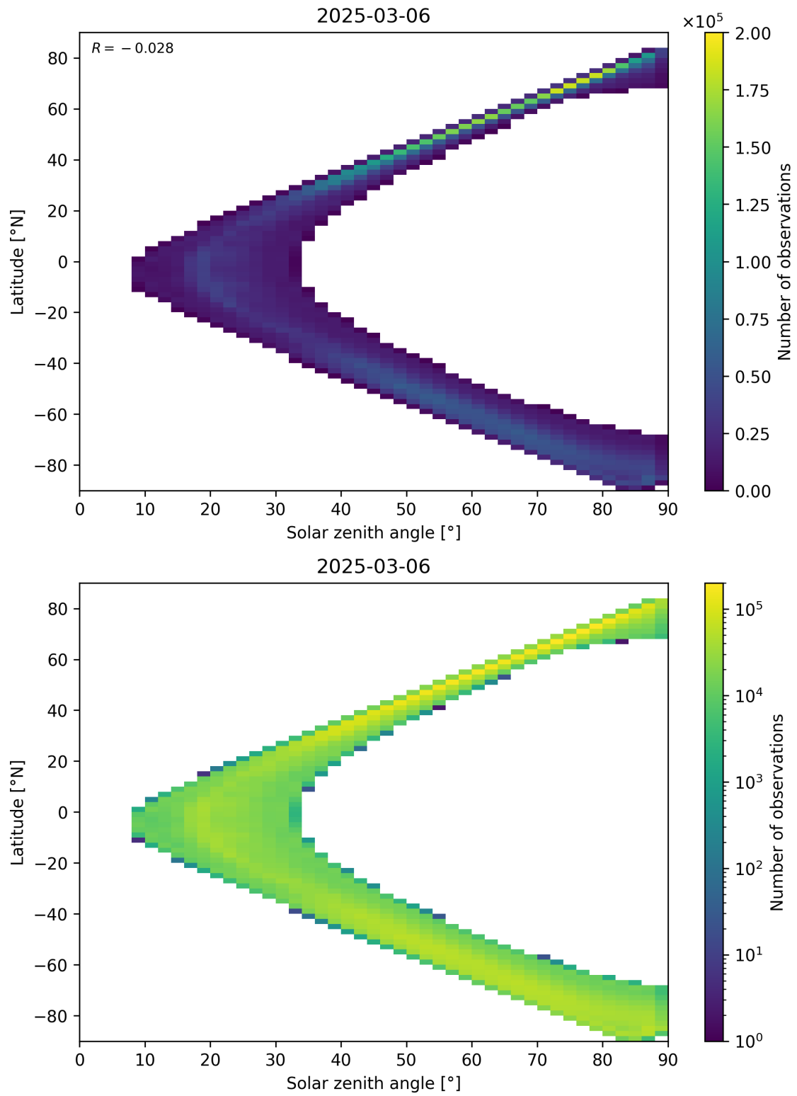
Figure 105: Scatter density plot of “Solar zenith angle” against “Latitude” for 2025-03-05 to 2025-03-07.
