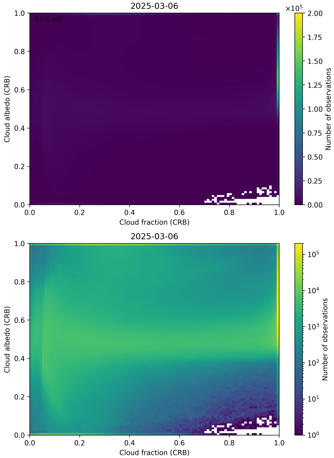
Figure 77: Scatter density plot of “Cloud fraction (CRB)” against “Cloud albedo (CRB)” for 2025-03-05 to 2025-03-07.
