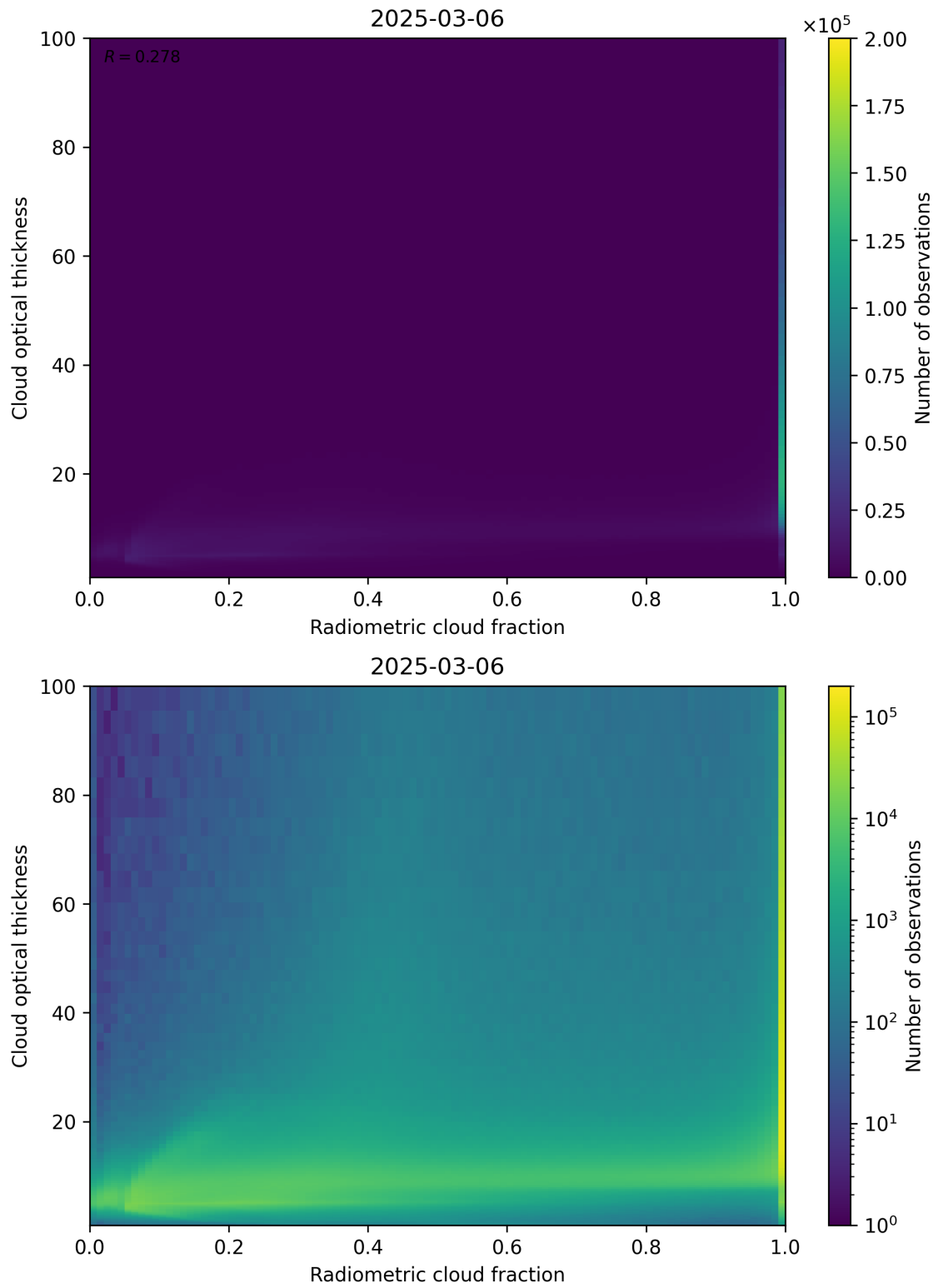
Figure 75: Scatter density plot of “Radiometric cloud fraction” against “Cloud optical thickness” for 2025-03-05 to 2025-03-07.
