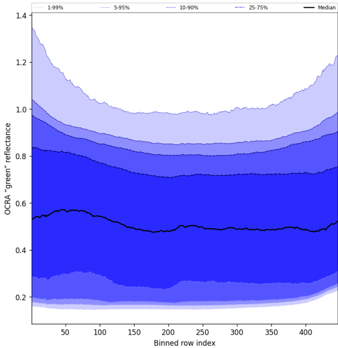
Figure 68: Along track statistics of "OCRA "green" reflectance" for 2025-03-05 to 2025-03-07
