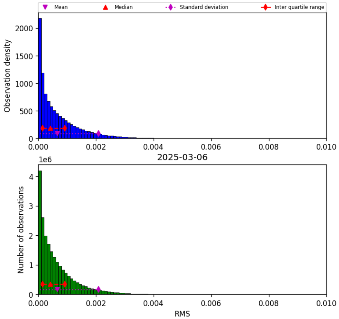
Figure 47: Histogram of “RMS” for 2025-03-05 to 2025-03-07
