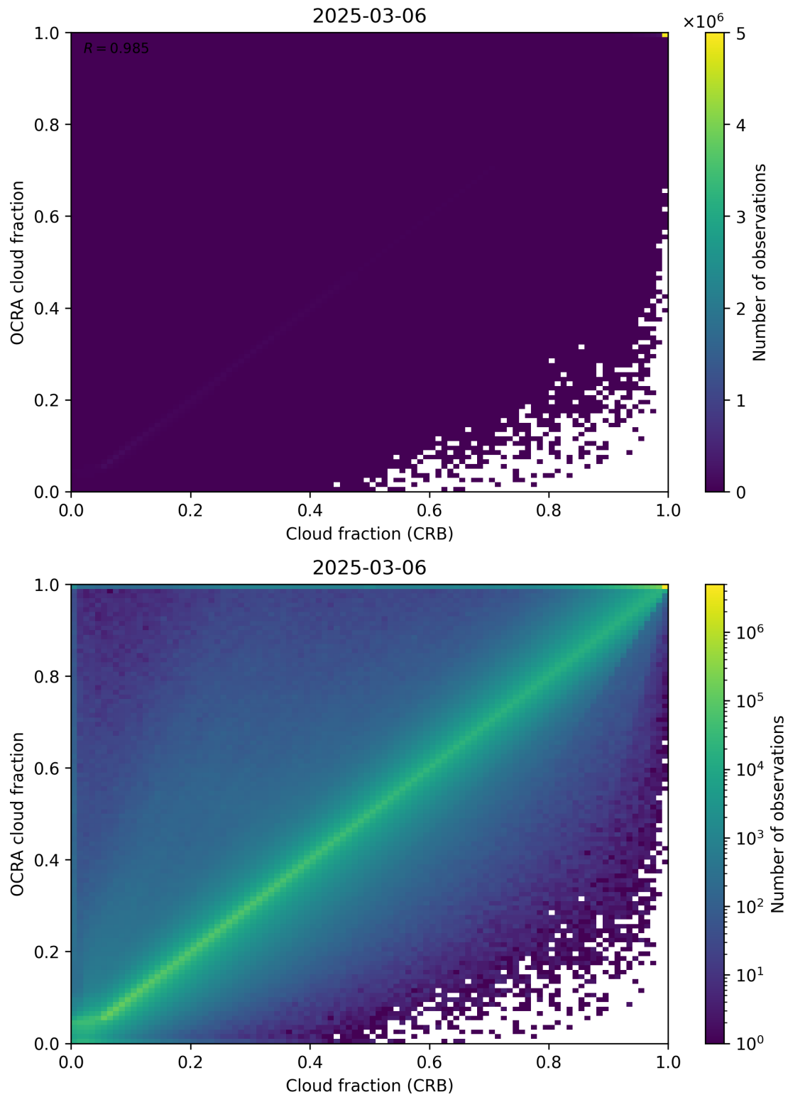
Figure 78: Scatter density plot of “Cloud fraction (CRB)” against “OCRA cloud fraction” for 2025-03-05 to 2025-03-07.
