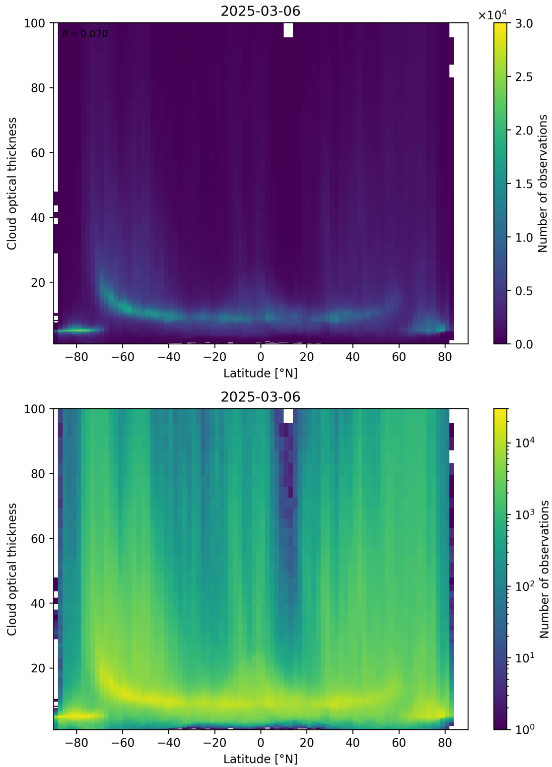
Figure 96: Scatter density plot of “Latitude” against “Cloud optical thickness” for 2025-03-05 to 2025-03-07.
