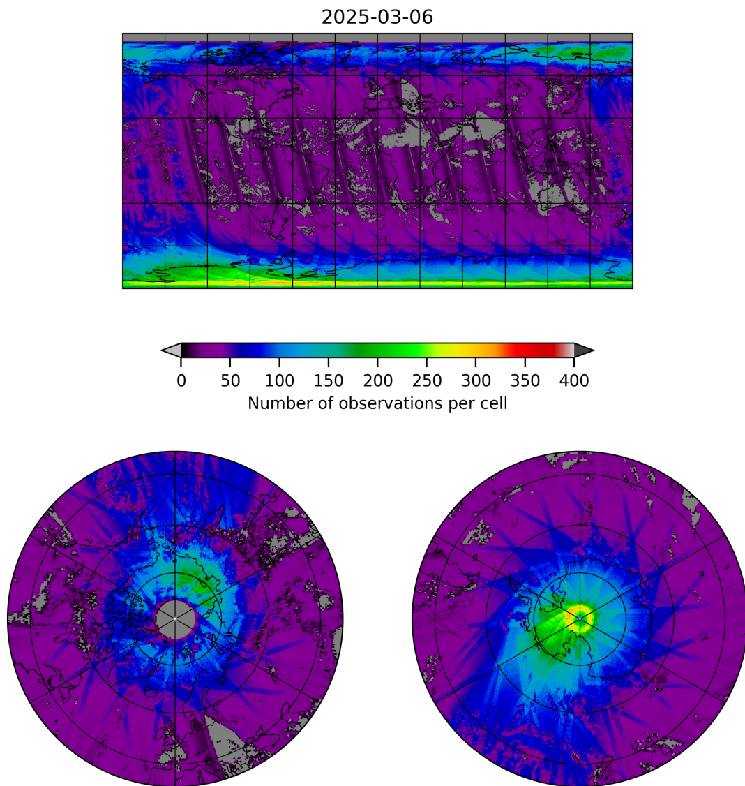
Figure 21: Map of the number of observations for 2025-03-05 to 2025-03-07
