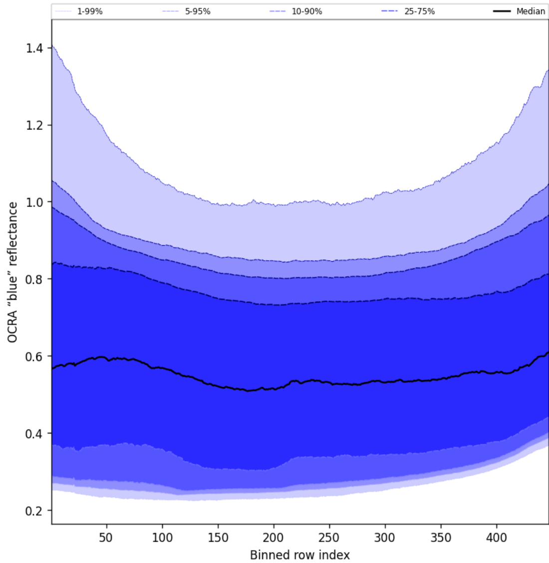
Figure 67: Along track statistics of “OCRA “blue” reflectance” for 2025-03-05 to 2025-03-07
