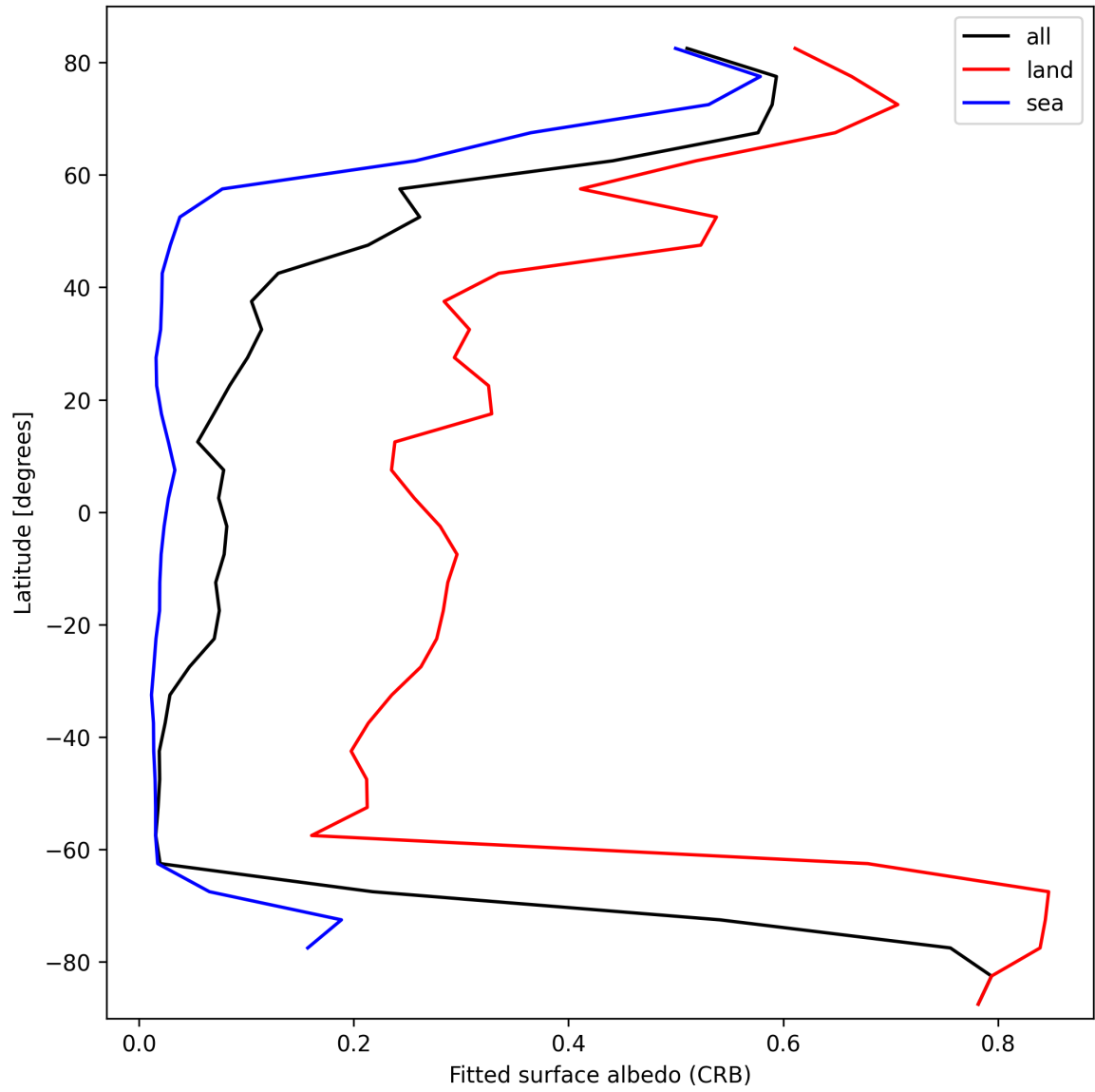
Figure 30: Zonal average of “Fitted surface albedo (CRB)” for 2025-03-05 to 2025-03-07.
