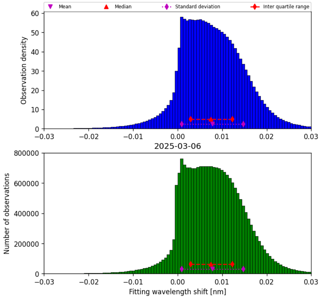
Figure 49: Histogram of “Fitting wavelength shift” for 2025-03-05 to 2025-03-07
