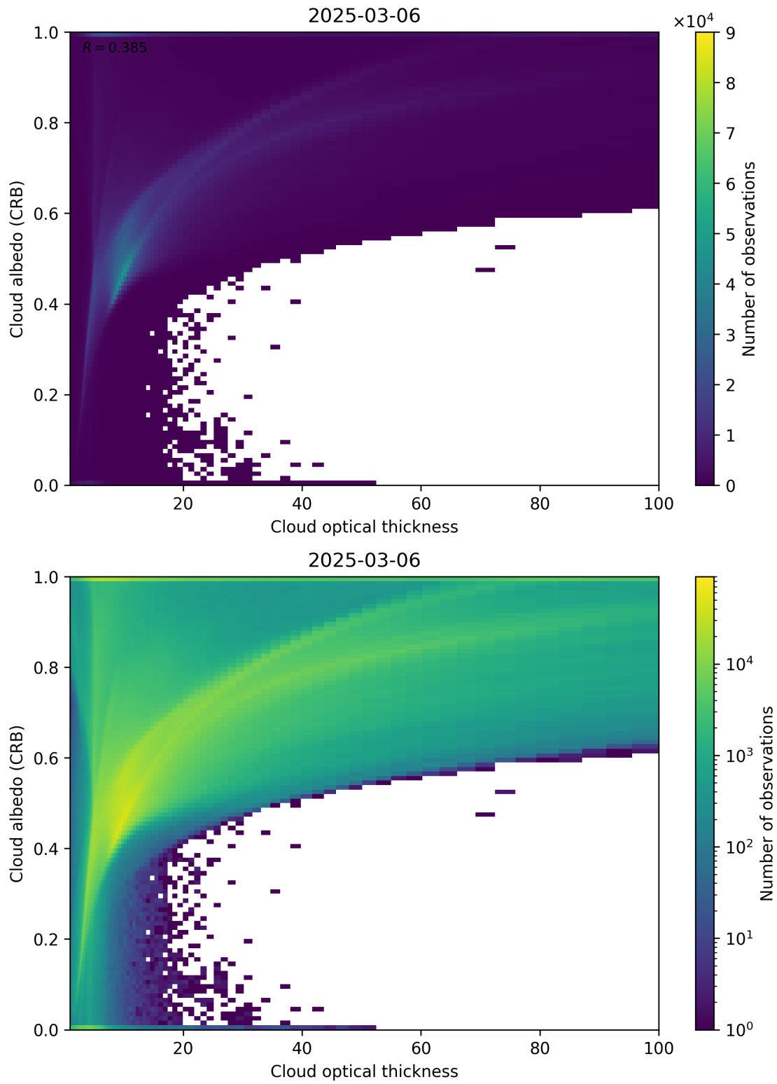
Figure 82: Scatter density plot of “Cloud optical thickness” against “Cloud albedo (CRB)” for 2025-03-05 to 2025-03-07.
