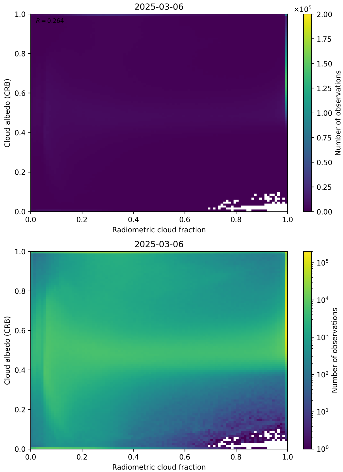
Figure 71: Scatter density plot of “Radiometric cloud fraction” against “Cloud albedo (CRB)” for 2025-03-05 to 2025-03-07.
