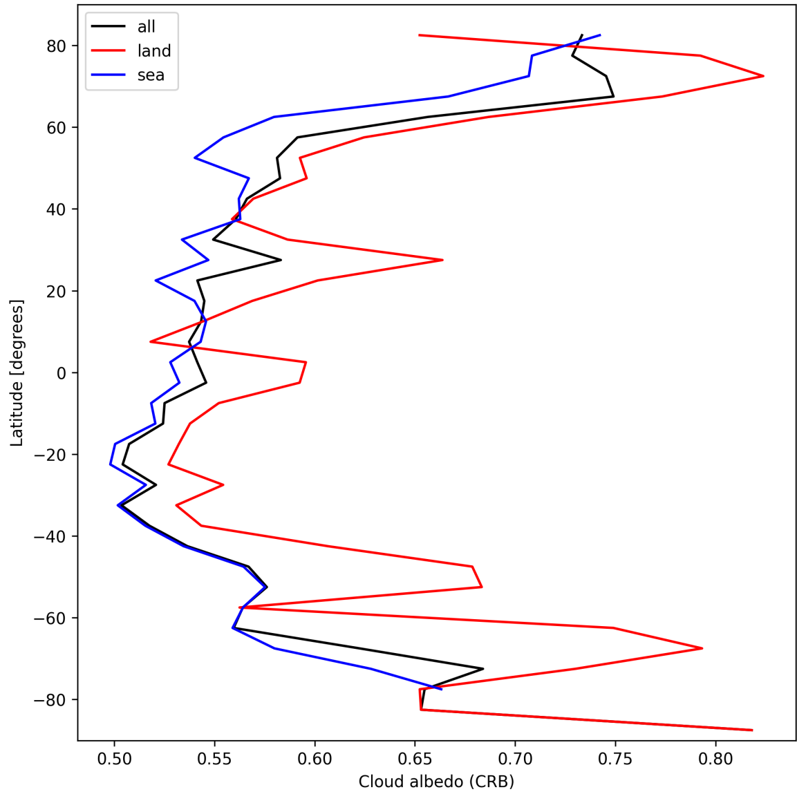
Figure 28: Zonal average of “Cloud albedo (CRB)” for 2025-03-05 to 2025-03-07.
