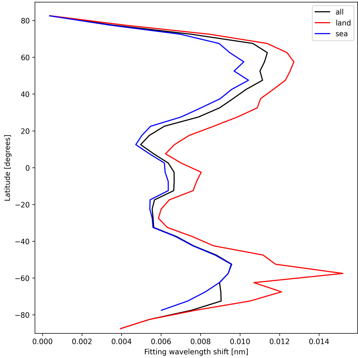
Figure 33: Zonal average of “Fitting wavelength shift” for 2025-03-05 to 2025-03-07.
