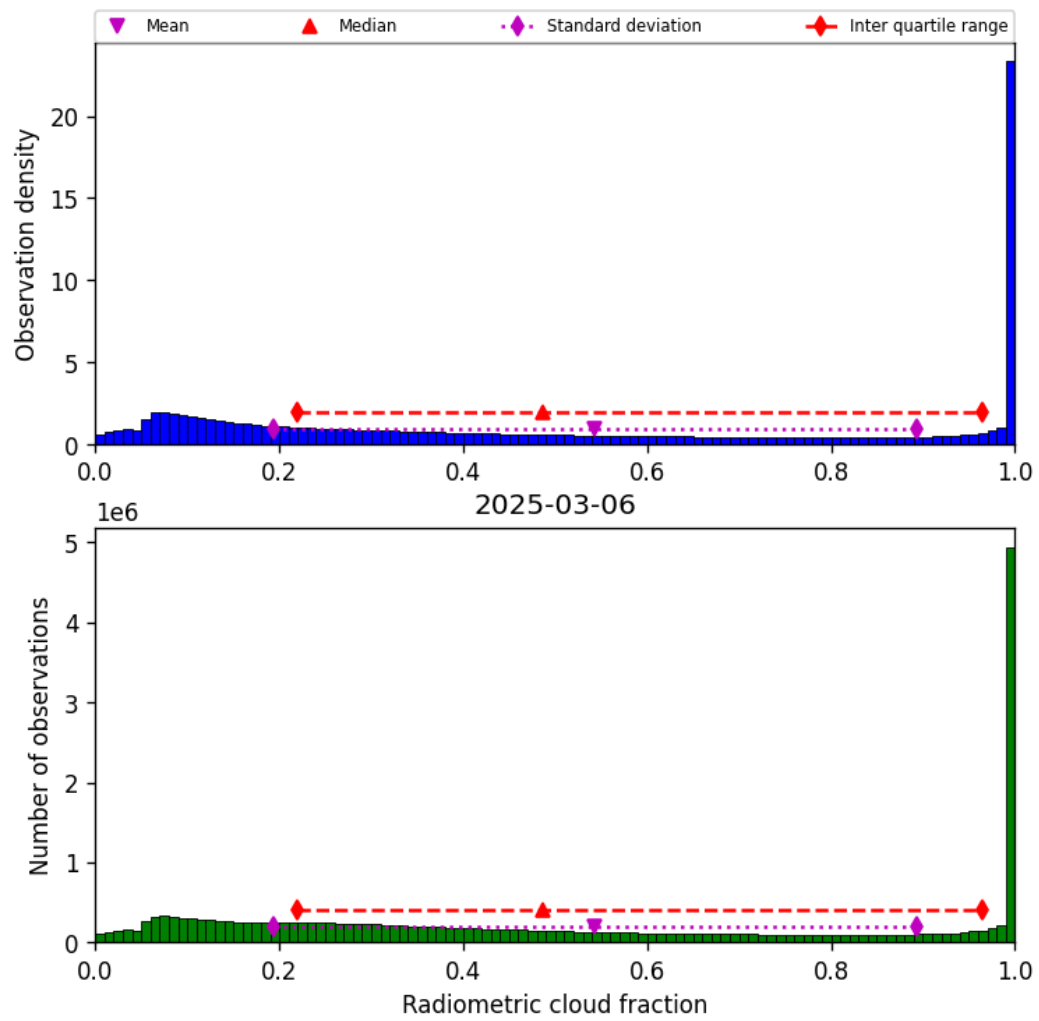
Figure 39: Histogram of “Radiometric cloud fraction” for 2025-03-05 to 2025-03-07
