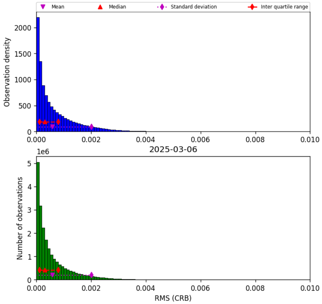
Figure 48: Histogram of “RMS (CRB)” for 2025-03-05 to 2025-03-07
