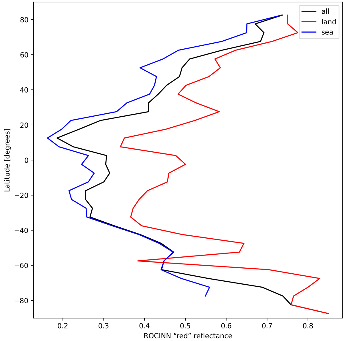
Figure 37: Zonal average of “ROCINN “red” reflectance” for 2025-03-05 to 2025-03-07.
