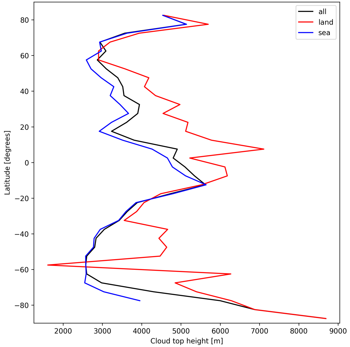
Figure 24: Zonal average of “Cloud top height” for 2025-03-05 to 2025-03-07.
