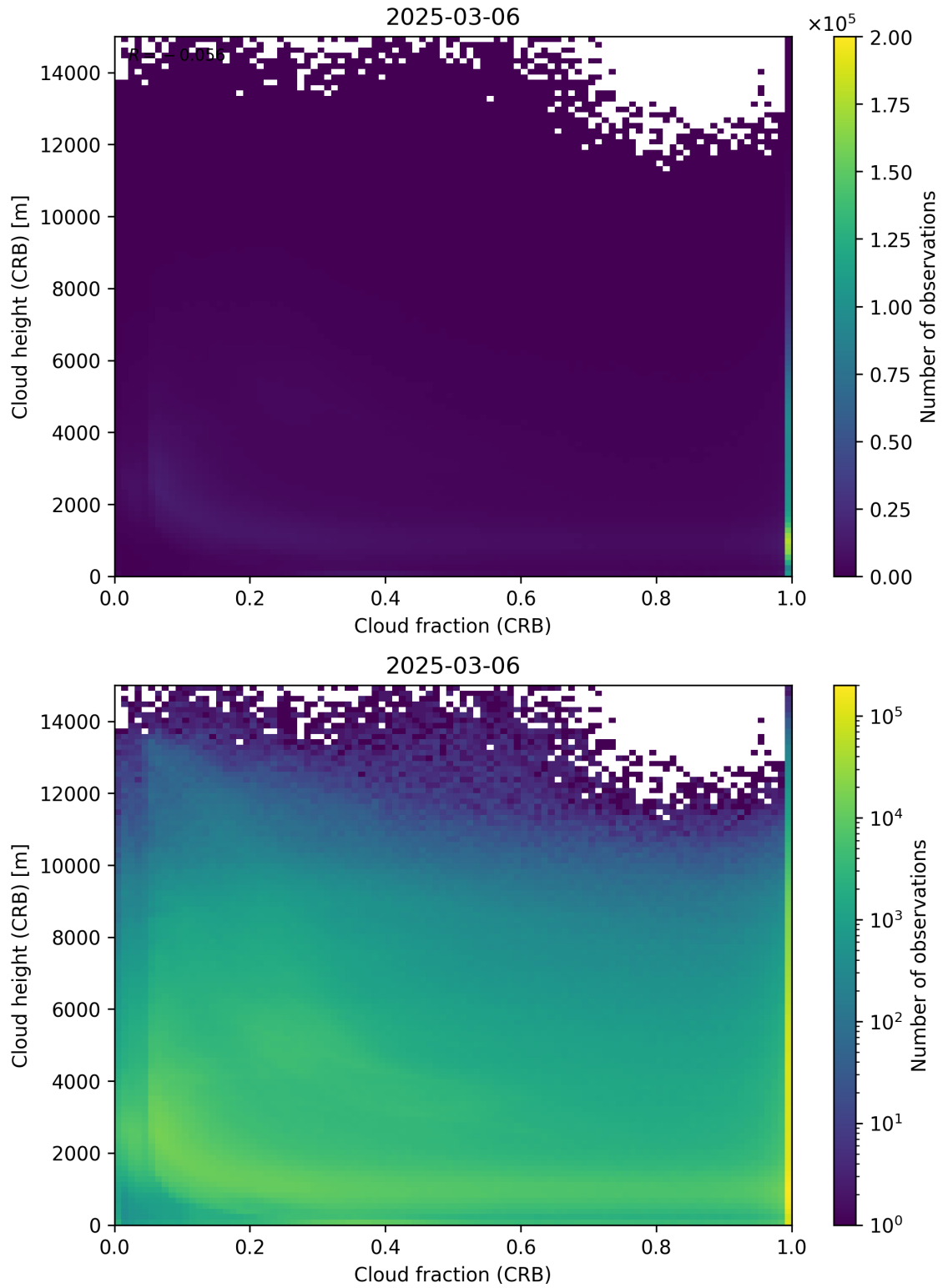
Figure 79: Scatter density plot of “Cloud fraction (CRB)” against “Cloud height (CRB)” for 2025-03-05 to 2025-03-07.
