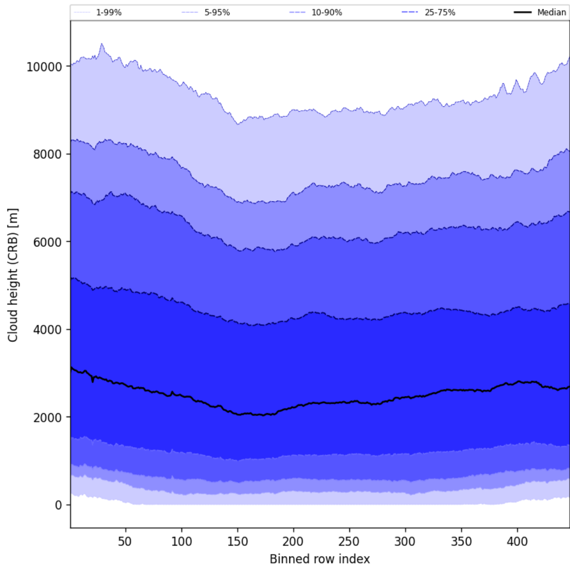
Figure 59: Along track statistics of “Cloud height (CRB)” for 2025-03-05 to 2025-03-07
