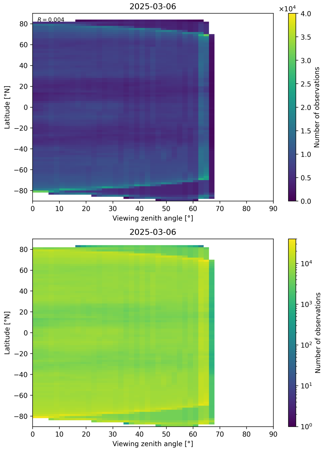
Figure 113: Scatter density plot of “Viewing zenith angle” against “Latitude” for 2025-03-05 to 2025-03-07.
