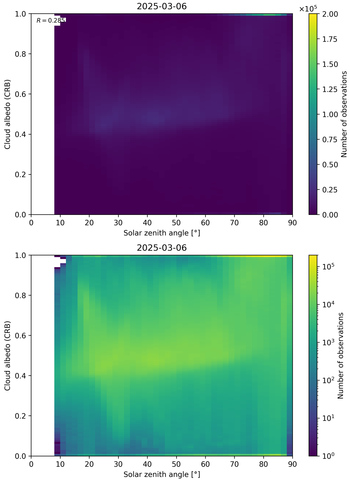
Figure 98: Scatter density plot of “Solar zenith angle” against “Cloud albedo (CRB)” for 2025-03-05 to 2025-03-07.
