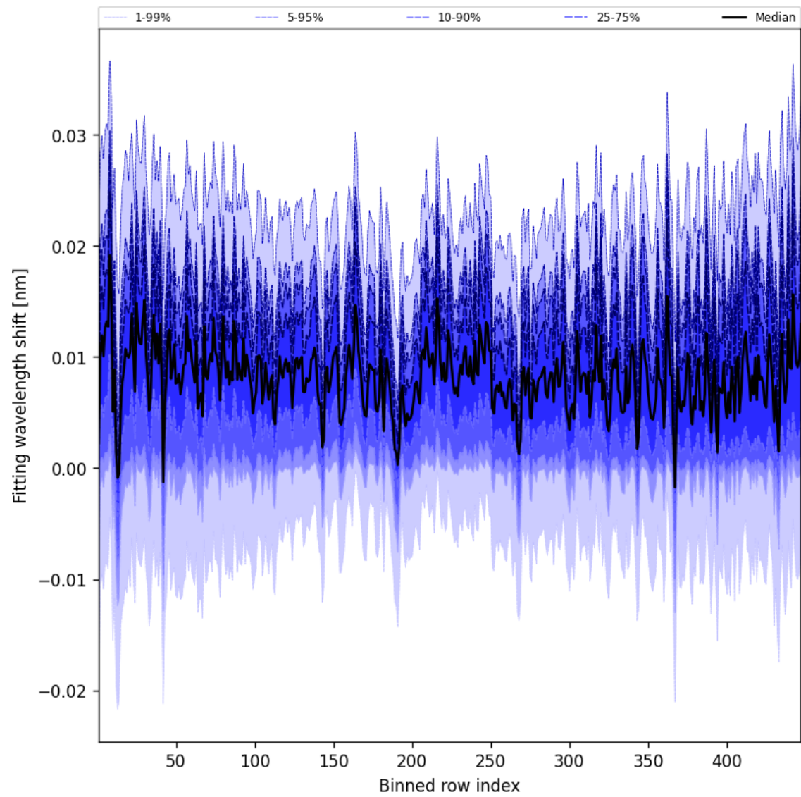
Figure 65: Along track statistics of “Fitting wavelength shift” for 2025-03-05 to 2025-03-07
