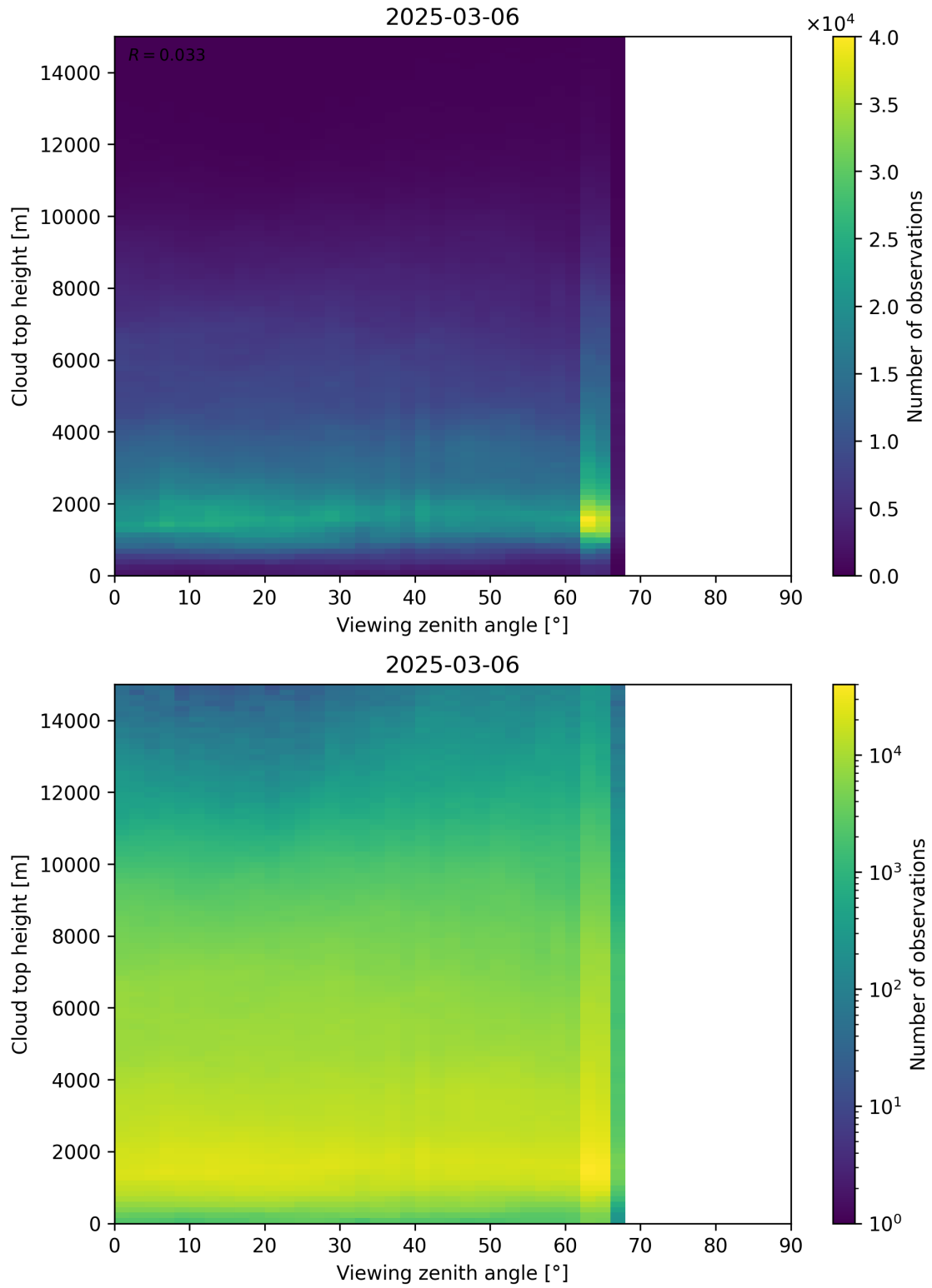
Figure 112: Scatter density plot of “Viewing zenith angle” against “Cloud top height” for 2025-03-05 to 2025-03-07.
