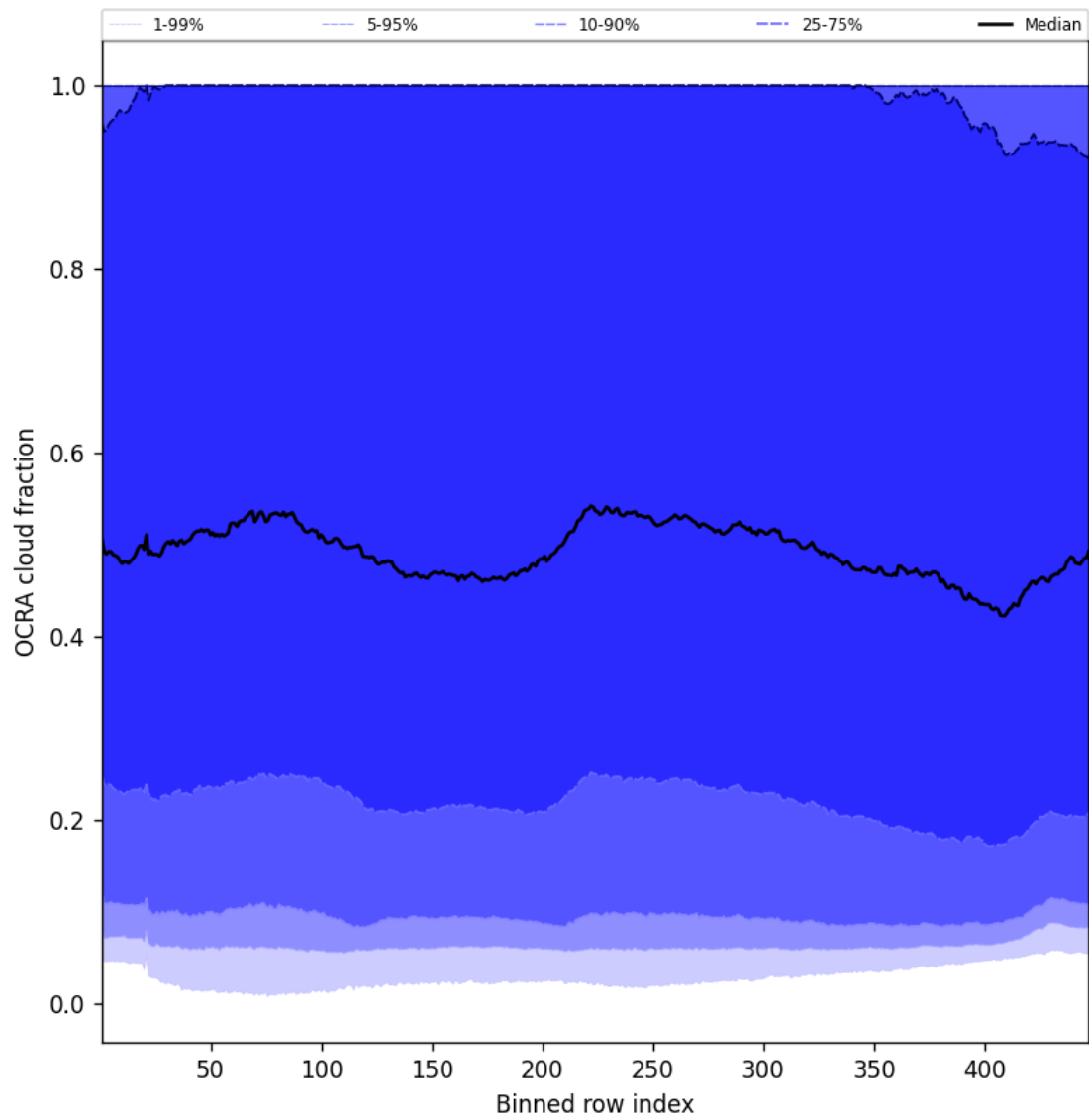
Figure 66: Along track statistics of “OCRA cloud fraction” for 2025-03-05 to 2025-03-07
