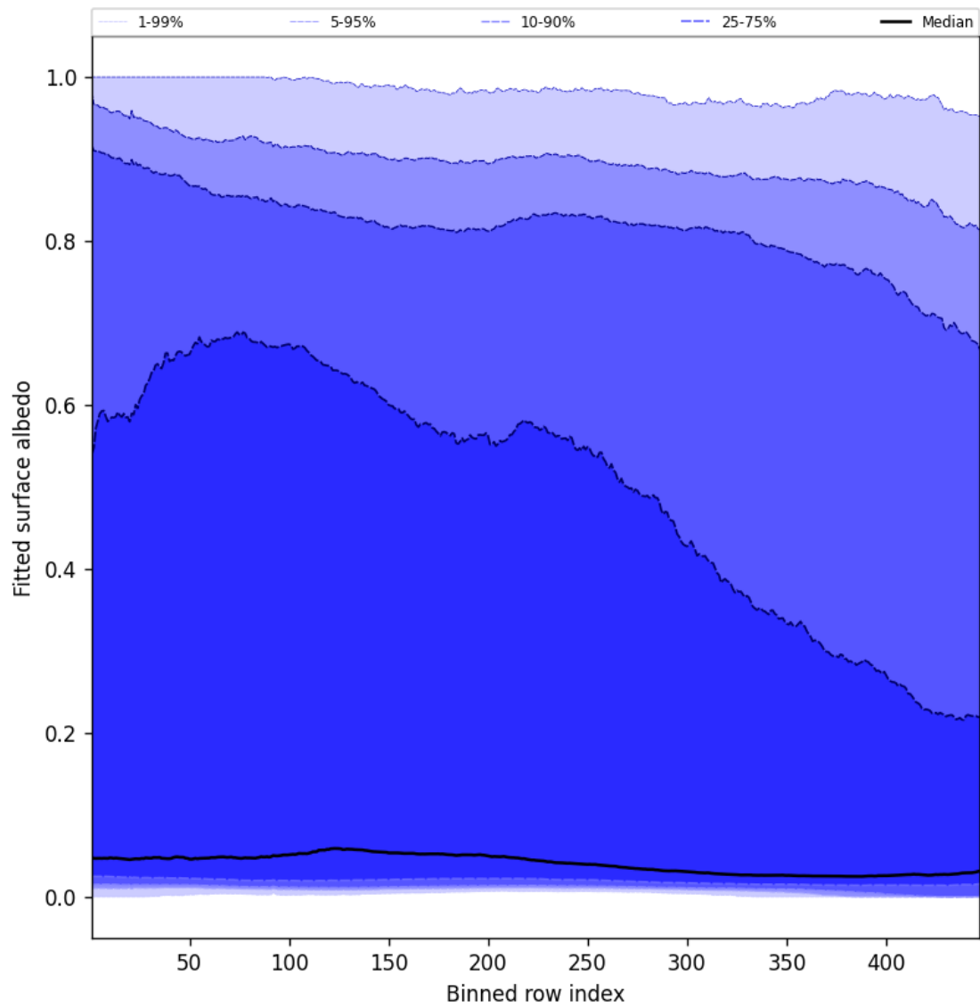
Figure 61: Along track statistics of “Fitted surface albedo” for 2025-03-05 to 2025-03-07
