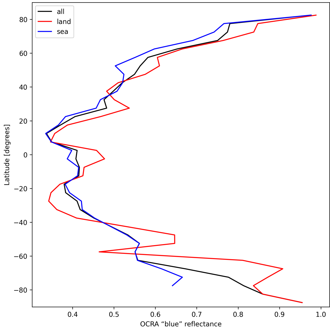
Figure 35: Zonal average of "OCRA "blue" reflectance" for 2025-03-05 to 2025-03-07.
