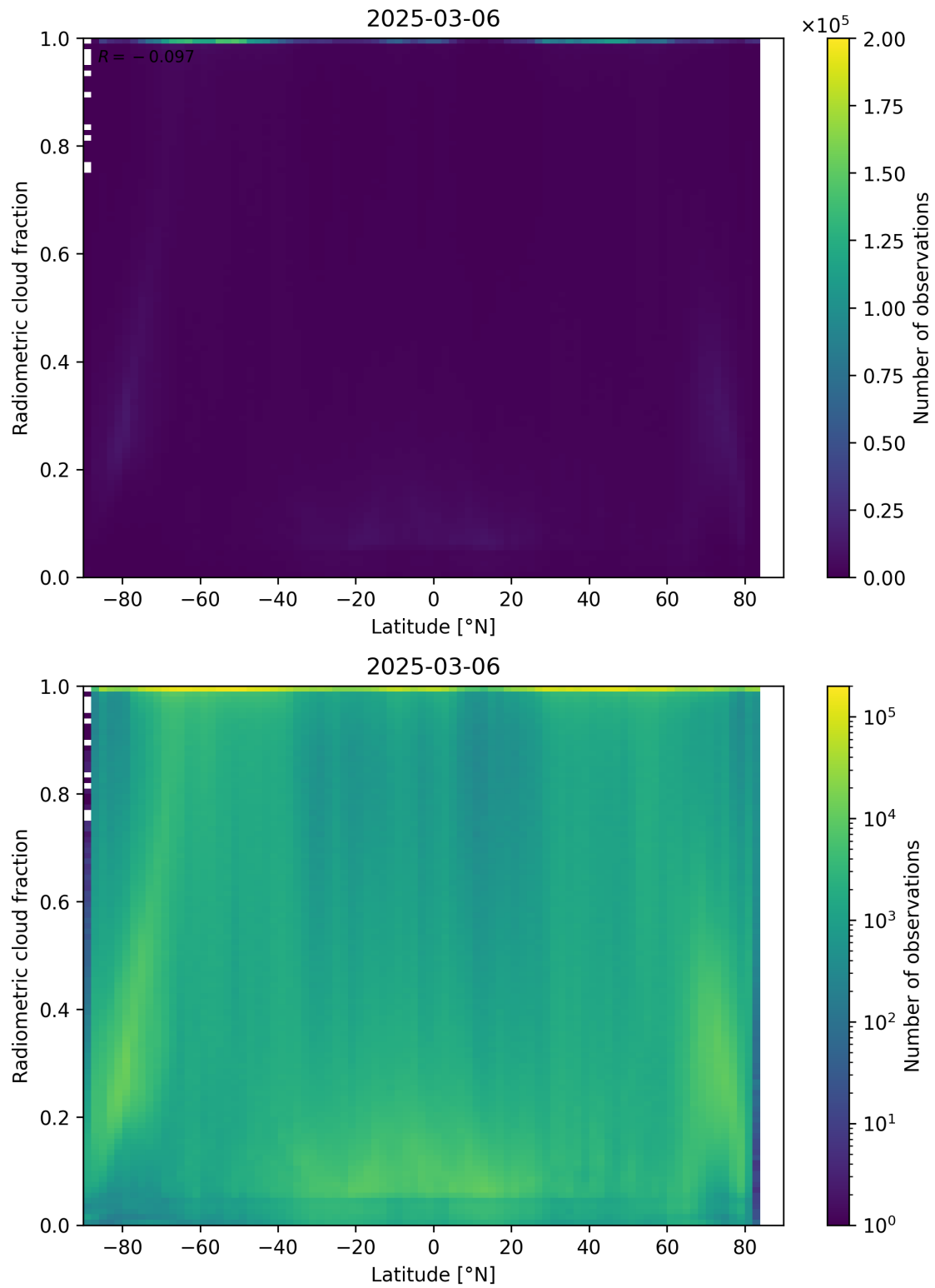
Figure 92: Scatter density plot of “Latitude” against “Radiometric cloud fraction” for 2025-03-05 to 2025-03-07.
