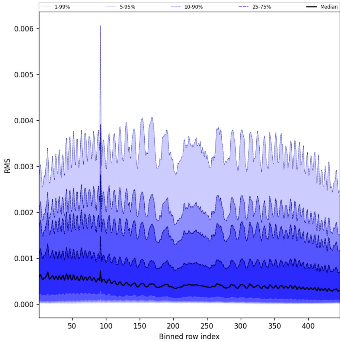
Figure 63: Along track statistics of “RMS” for 2025-03-05 to 2025-03-07
