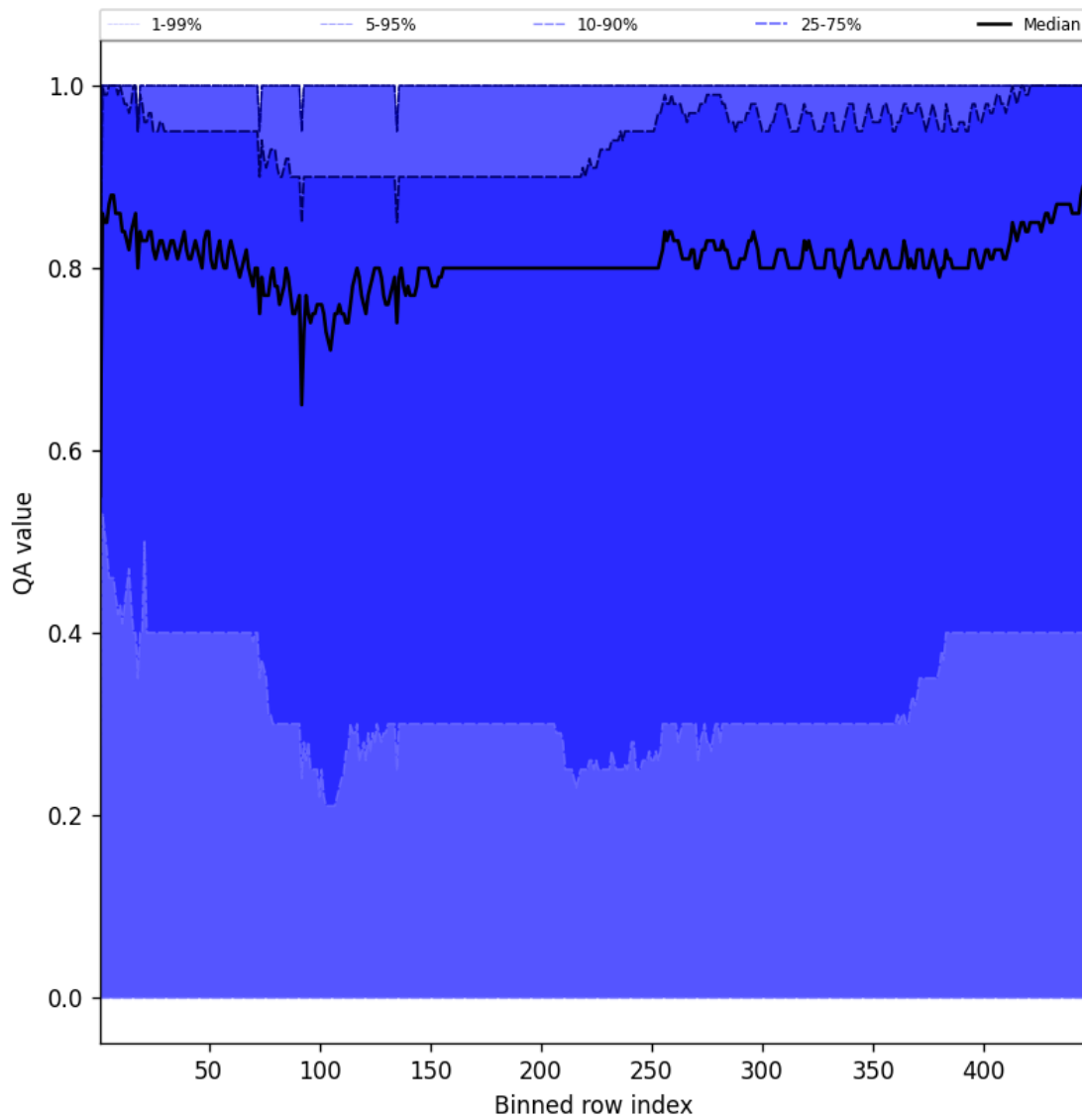
Figure 54: Along track statistics of “QA value” for 2025-03-05 to 2025-03-07
