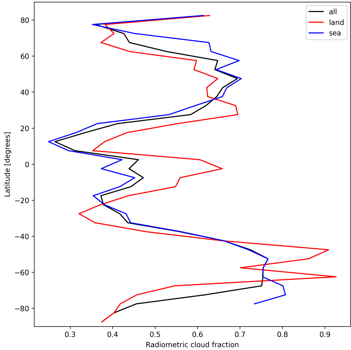
Figure 23: Zonal average of “Radiometric cloud fraction” for 2025-03-05 to 2025-03-07.
