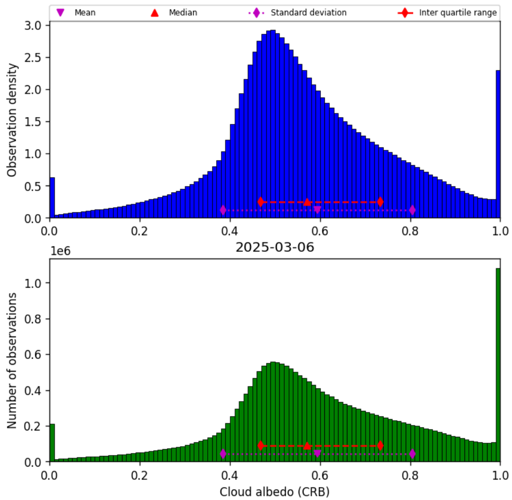
Figure 44: Histogram of “Cloud albedo (CRB)” for 2025-03-05 to 2025-03-07
