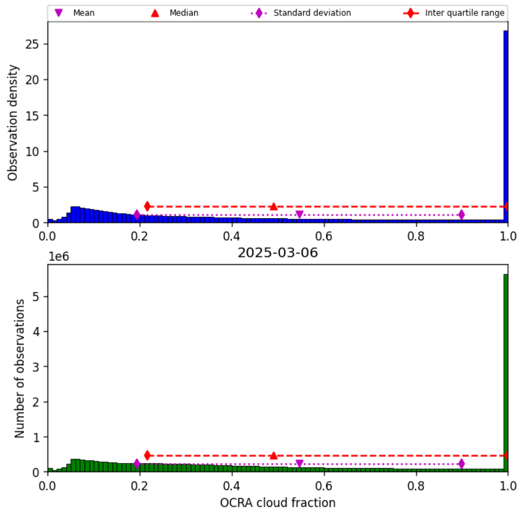
Figure 50: Histogram of “OCRA cloud fraction” for 2025-03-05 to 2025-03-07
