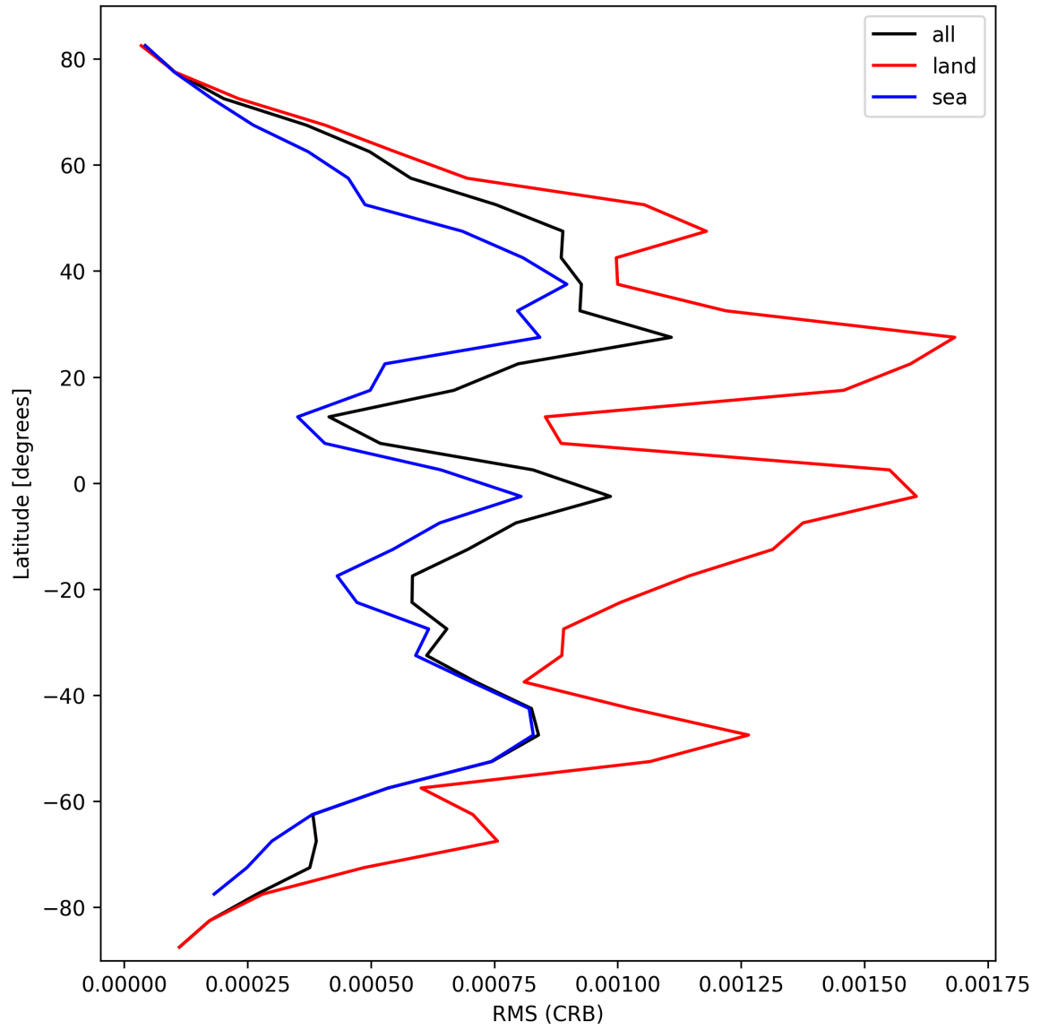
Figure 32: Zonal average of “RMS (CRB)” for 2025-03-05 to 2025-03-07.
