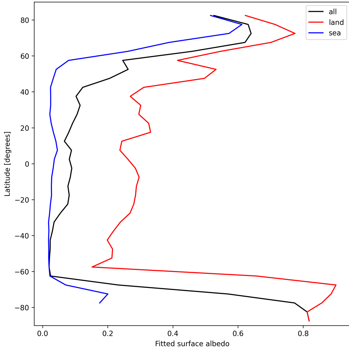
Figure 29: Zonal average of “Fitted surface albedo” for 2025-03-05 to 2025-03-07.
