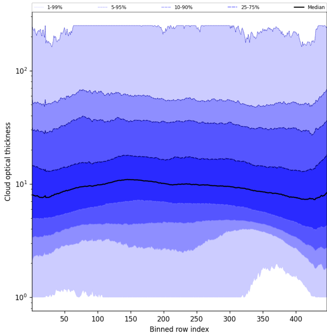
Figure 57: Along track statistics of “Cloud optical thickness” for 2025-03-05 to 2025-03-07
