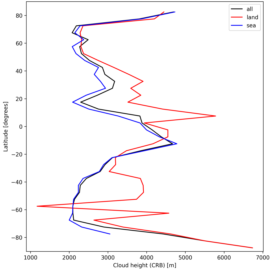
Figure 27: Zonal average of “Cloud height (CRB)” for 2025-03-05 to 2025-03-07.
