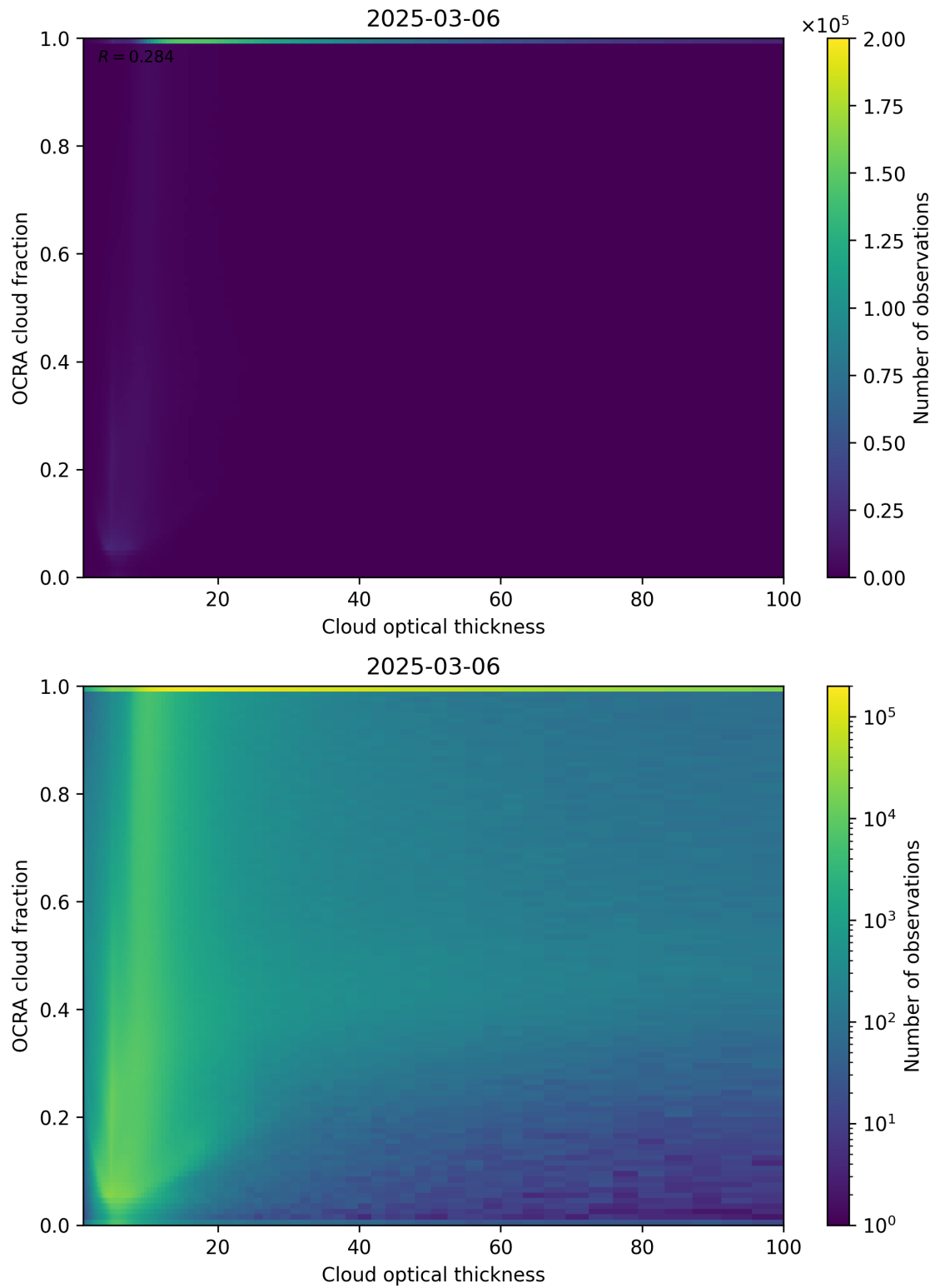
Figure 83: Scatter density plot of “Cloud optical thickness” against “OCRA cloud fraction” for 2025-03-05 to 2025-03-07.
