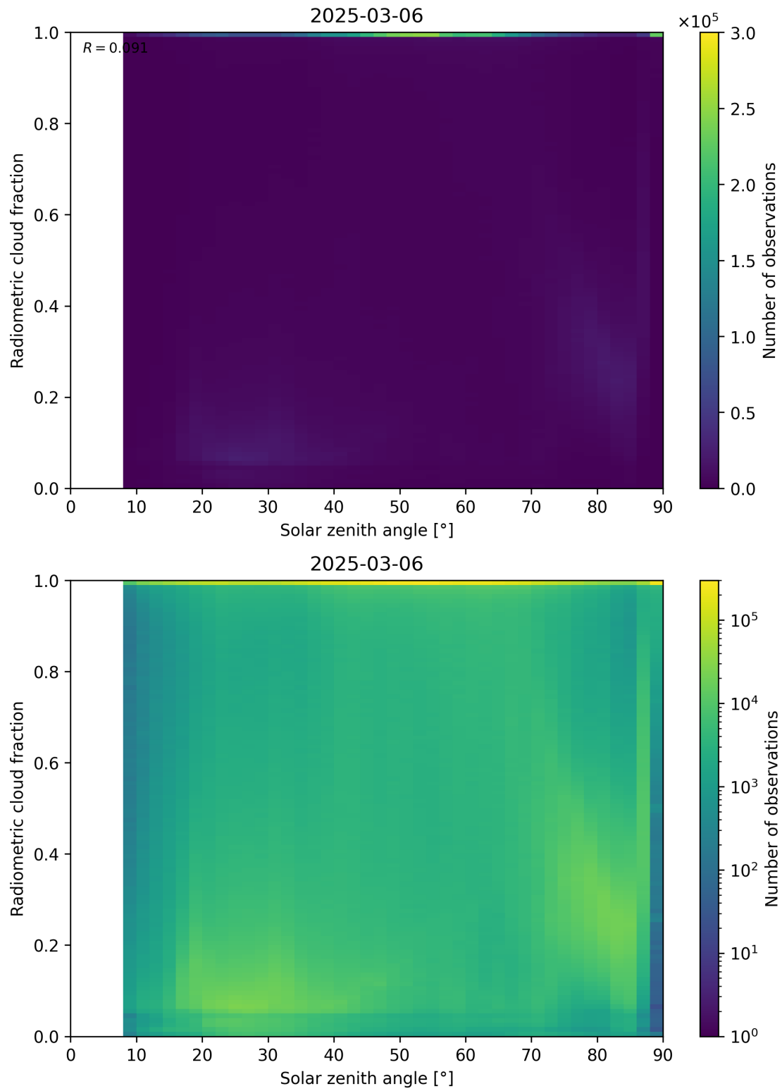
Figure 99: Scatter density plot of “Solar zenith angle” against “Radiometric cloud fraction” for 2025-03-05 to 2025-03-07.
