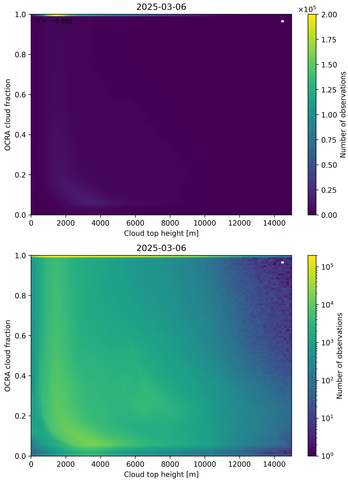
Figure 87: Scatter density plot of “Cloud top height” against “OCRA cloud fraction” for 2025-03-05 to 2025-03-07.
