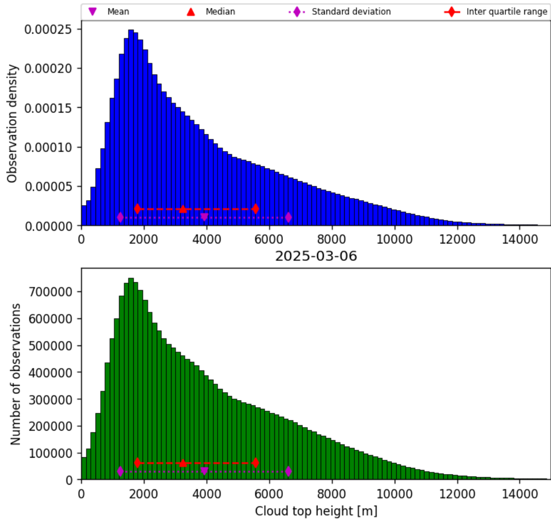
Figure 40: Histogram of “Cloud top height” for 2025-03-05 to 2025-03-07
