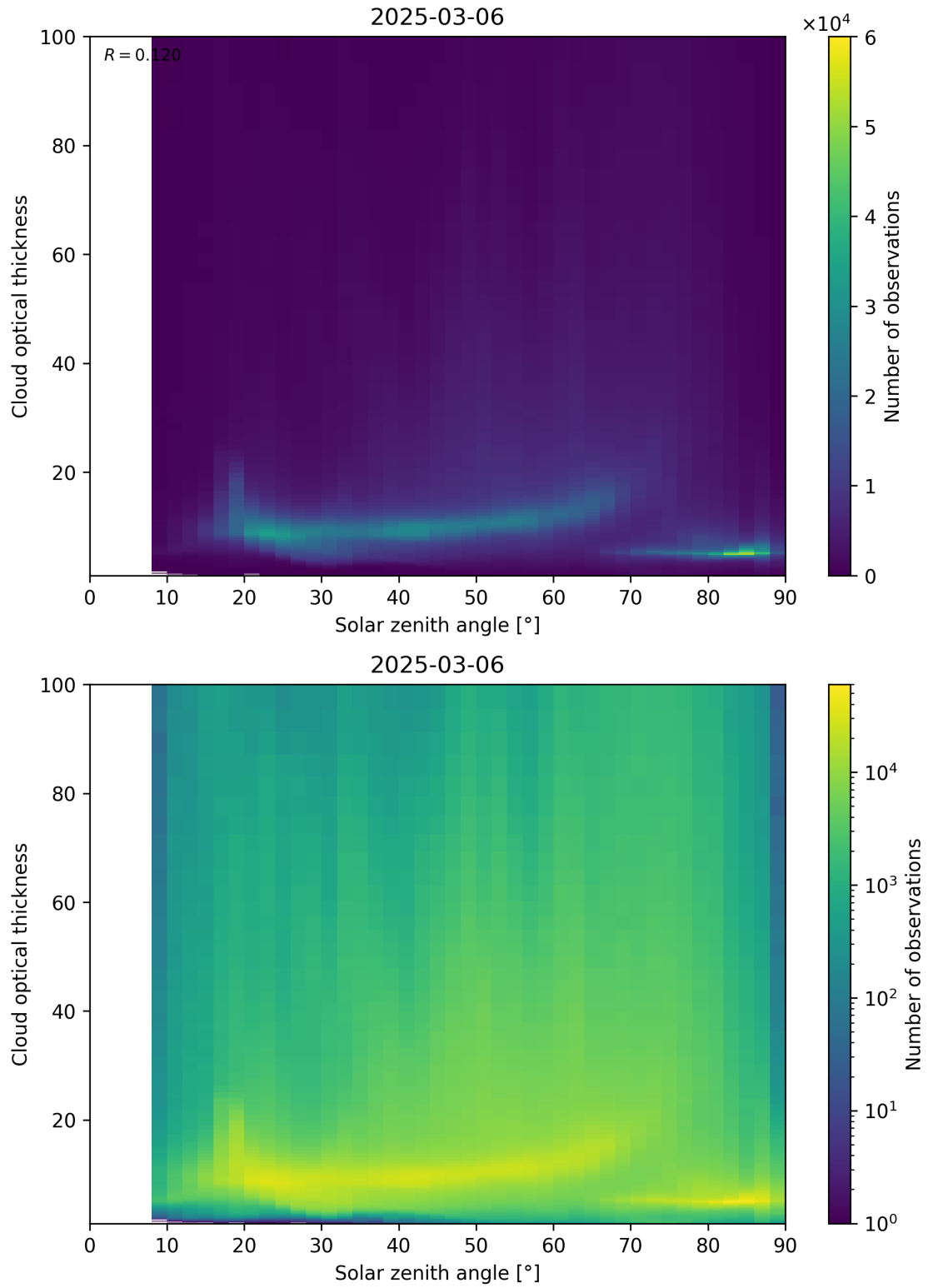
Figure 103: Scatter density plot of “Solar zenith angle” against “Cloud optical thickness” for 2025-03-05 to 2025-03-07.
