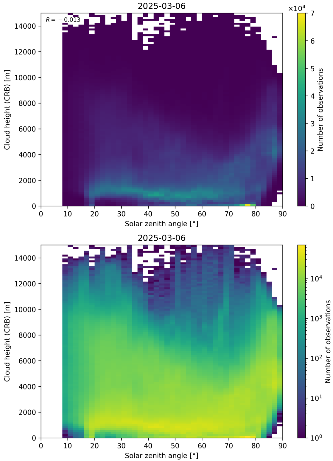
Figure 102: Scatter density plot of “Solar zenith angle” against “Cloud height (CRB)” for 2025-03-05 to 2025-03-07.
