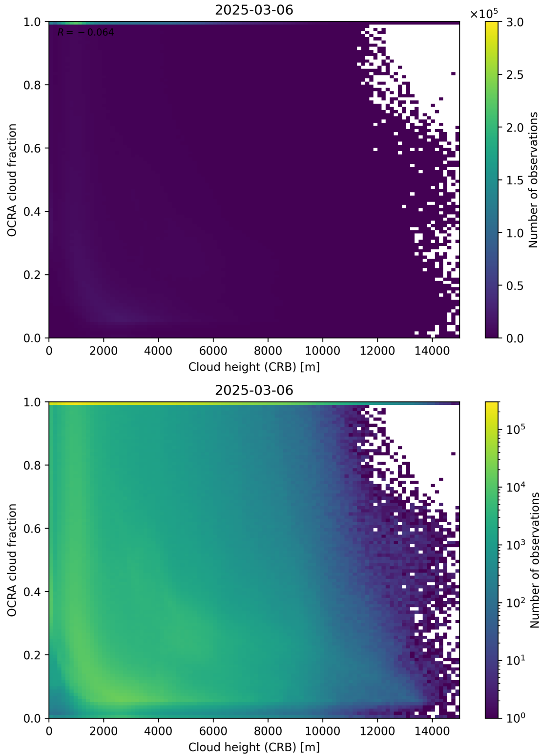
Figure 81: Scatter density plot of “Cloud height (CRB)” against “OCRA cloud fraction” for 2025-03-05 to 2025-03-07.
