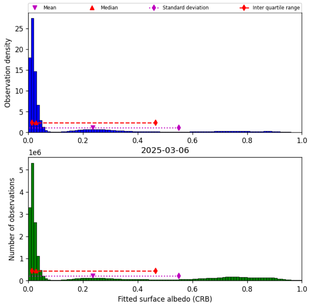
Figure 46: Histogram of “Fitted surface albedo (CRB)” for 2025-03-05 to 2025-03-07
