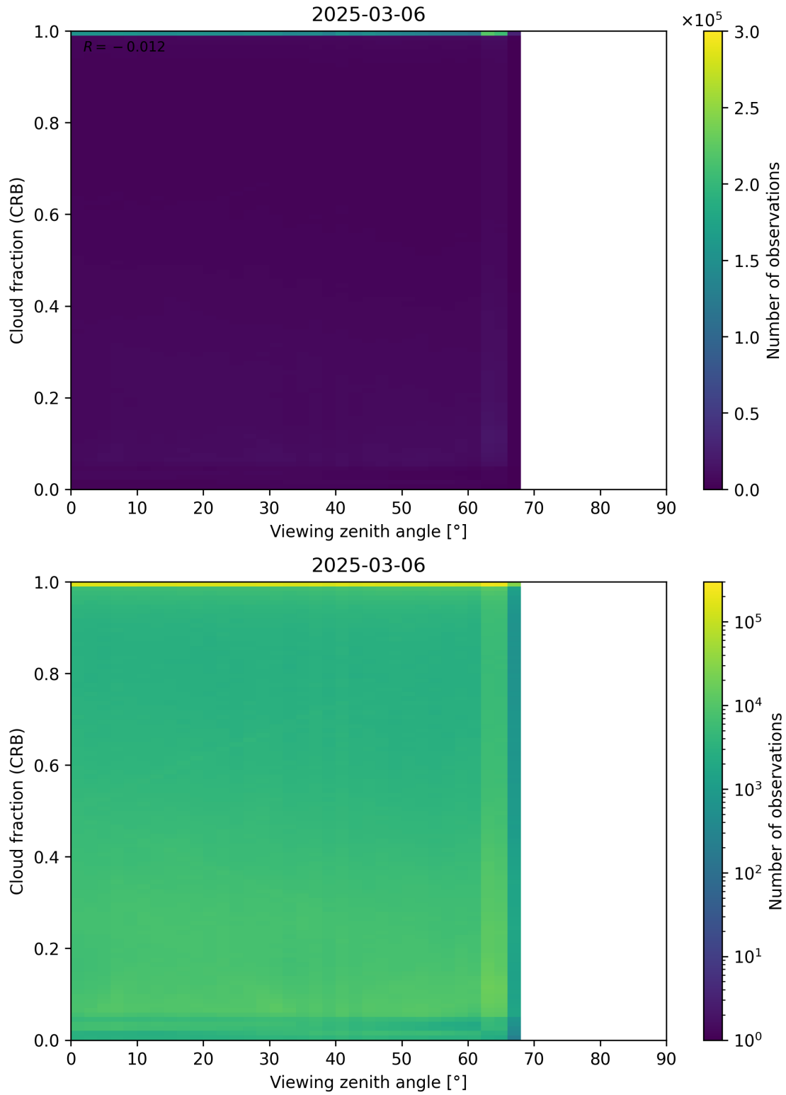
Figure 109: Scatter density plot of “Viewing zenith angle” against “Cloud fraction (CRB)” for 2025-03-05 to 2025-03-07.
