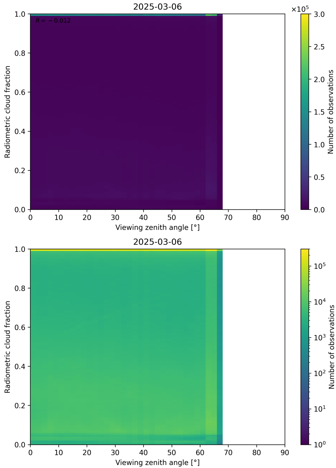
Figure 107: Scatter density plot of “Viewing zenith angle” against “Radiometric cloud fraction” for 2025-03-05 to 2025-03-07.
