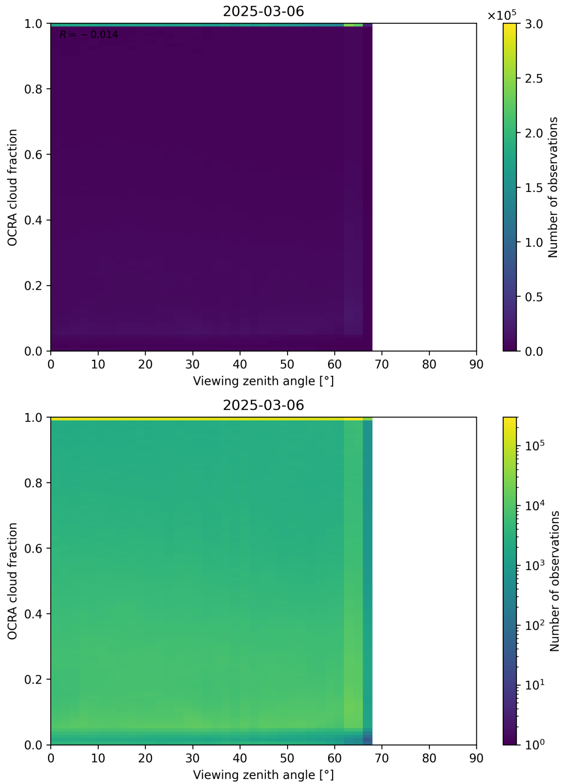
Figure 108: Scatter density plot of “Viewing zenith angle” against “OCRA cloud fraction” for 2025-03-05 to 2025-03-07.
