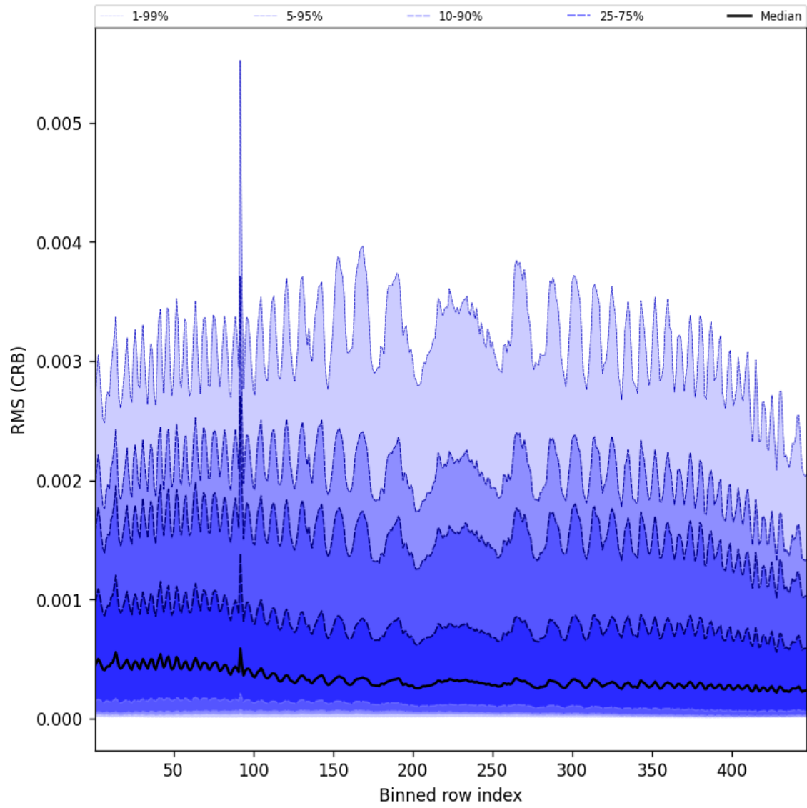
Figure 64: Along track statistics of “RMS (CRB)” for 2025-03-05 to 2025-03-07
