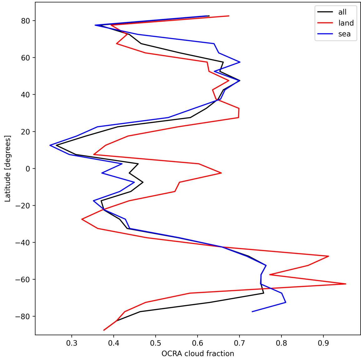
Figure 34: Zonal average of “OCRA cloud fraction” for 2025-03-05 to 2025-03-07.
