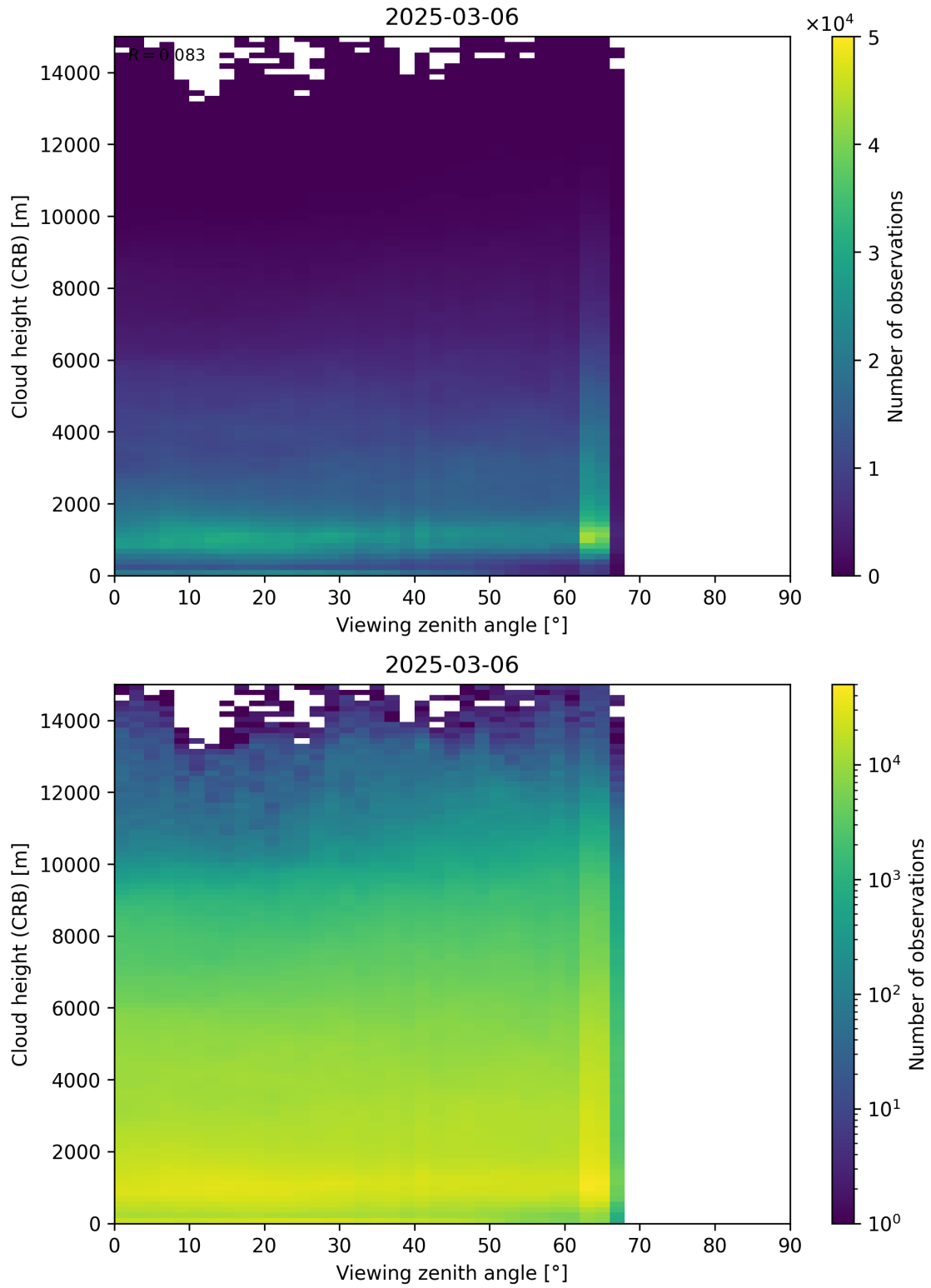
Figure 110: Scatter density plot of “Viewing zenith angle” against “Cloud height (CRB)” for 2025-03-05 to 2025-03-07.
