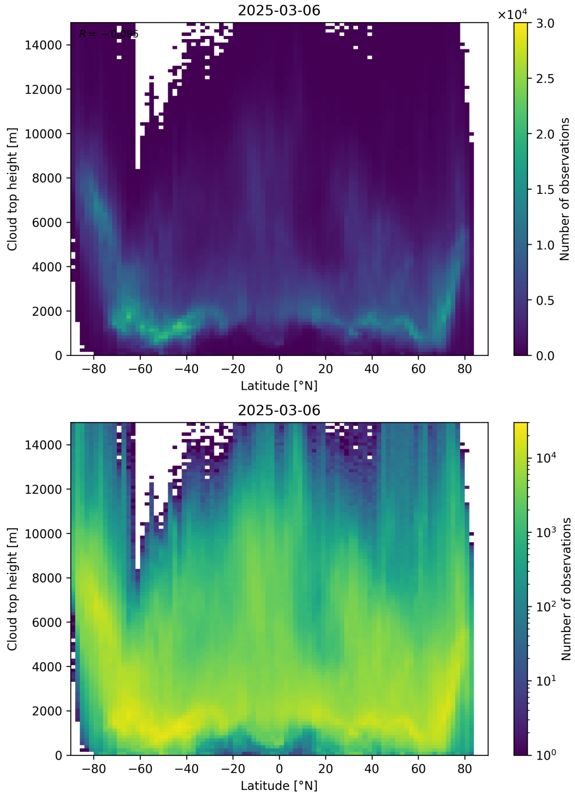
Figure 97: Scatter density plot of “Latitude” against “Cloud top height” for 2025-03-05 to 2025-03-07.
