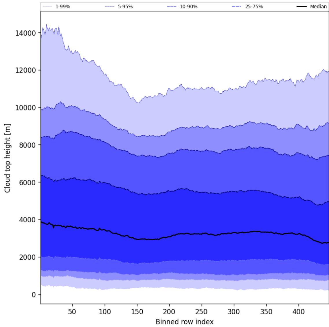
Figure 56: Along track statistics of “Cloud top height” for 2025-03-05 to 2025-03-07
