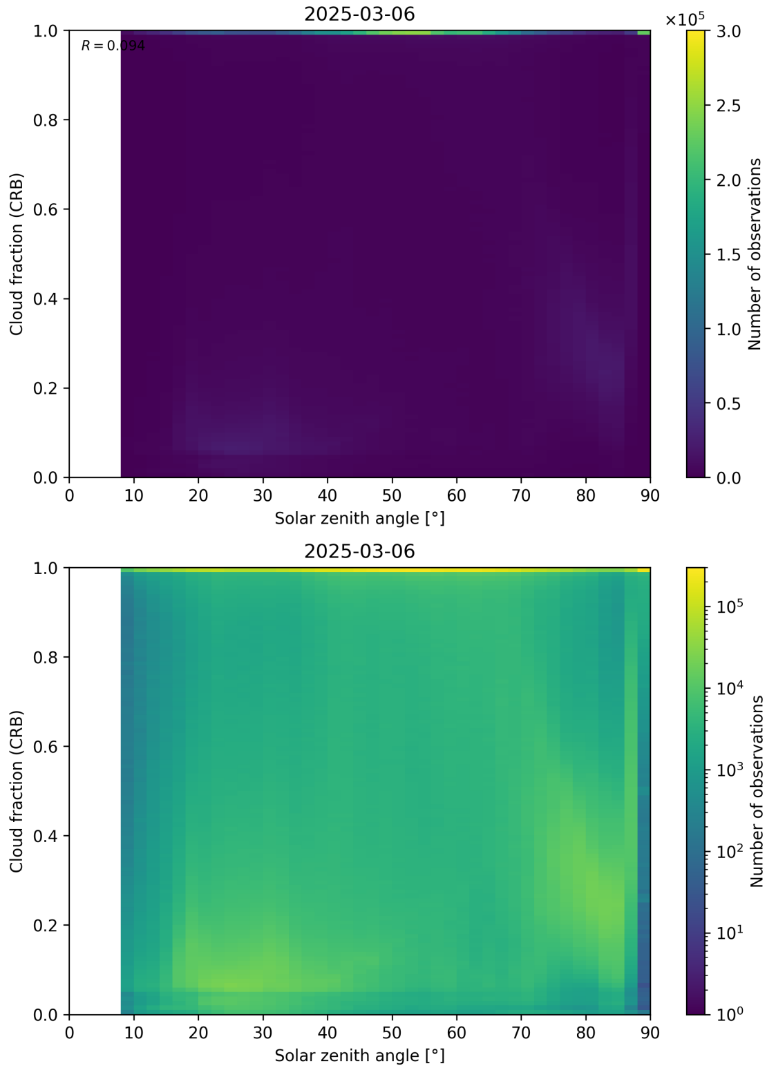
Figure 101: Scatter density plot of “Solar zenith angle” against “Cloud fraction (CRB)” for 2025-03-05 to 2025-03-07.
