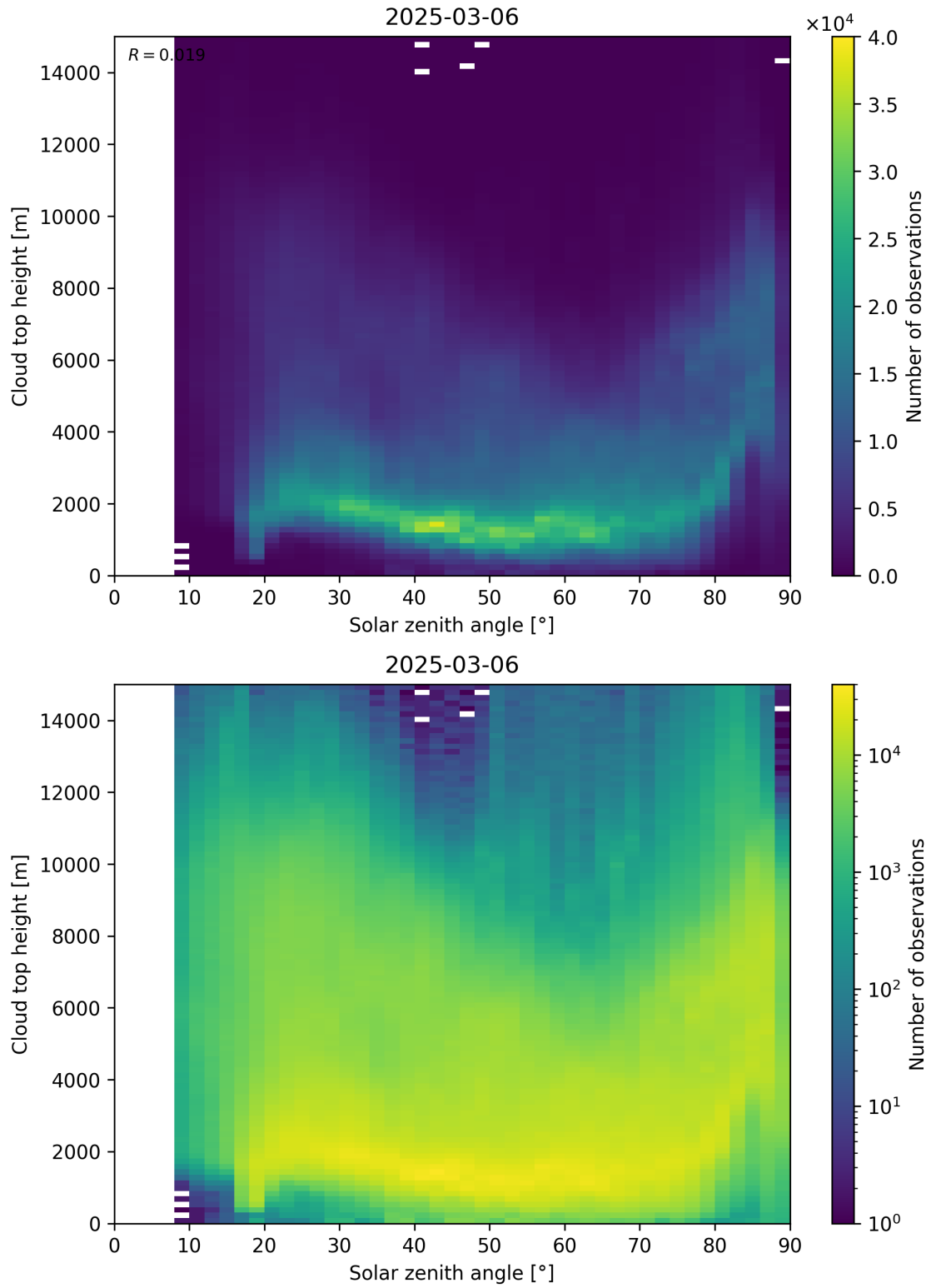
Figure 104: Scatter density plot of “Solar zenith angle” against “Cloud top height” for 2025-03-05 to 2025-03-07.
