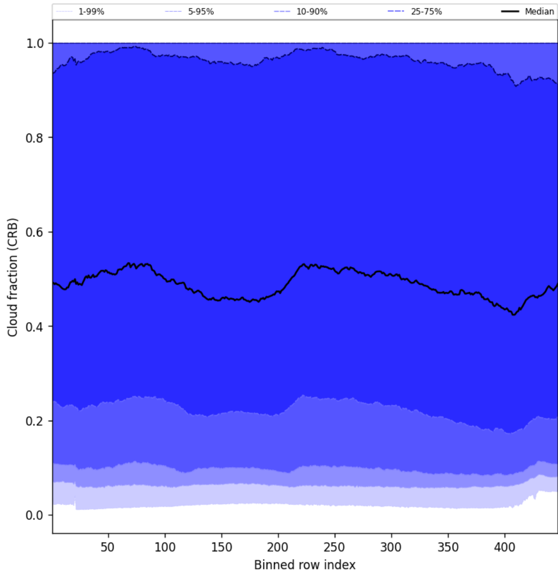
Figure 58: Along track statistics of “Cloud fraction (CRB)” for 2025-03-05 to 2025-03-07
