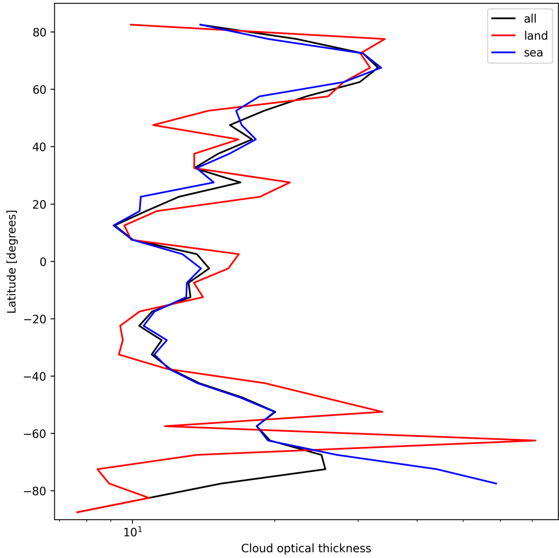
Figure 25: Zonal average of “Cloud optical thickness” for 2025-03-05 to 2025-03-07.
