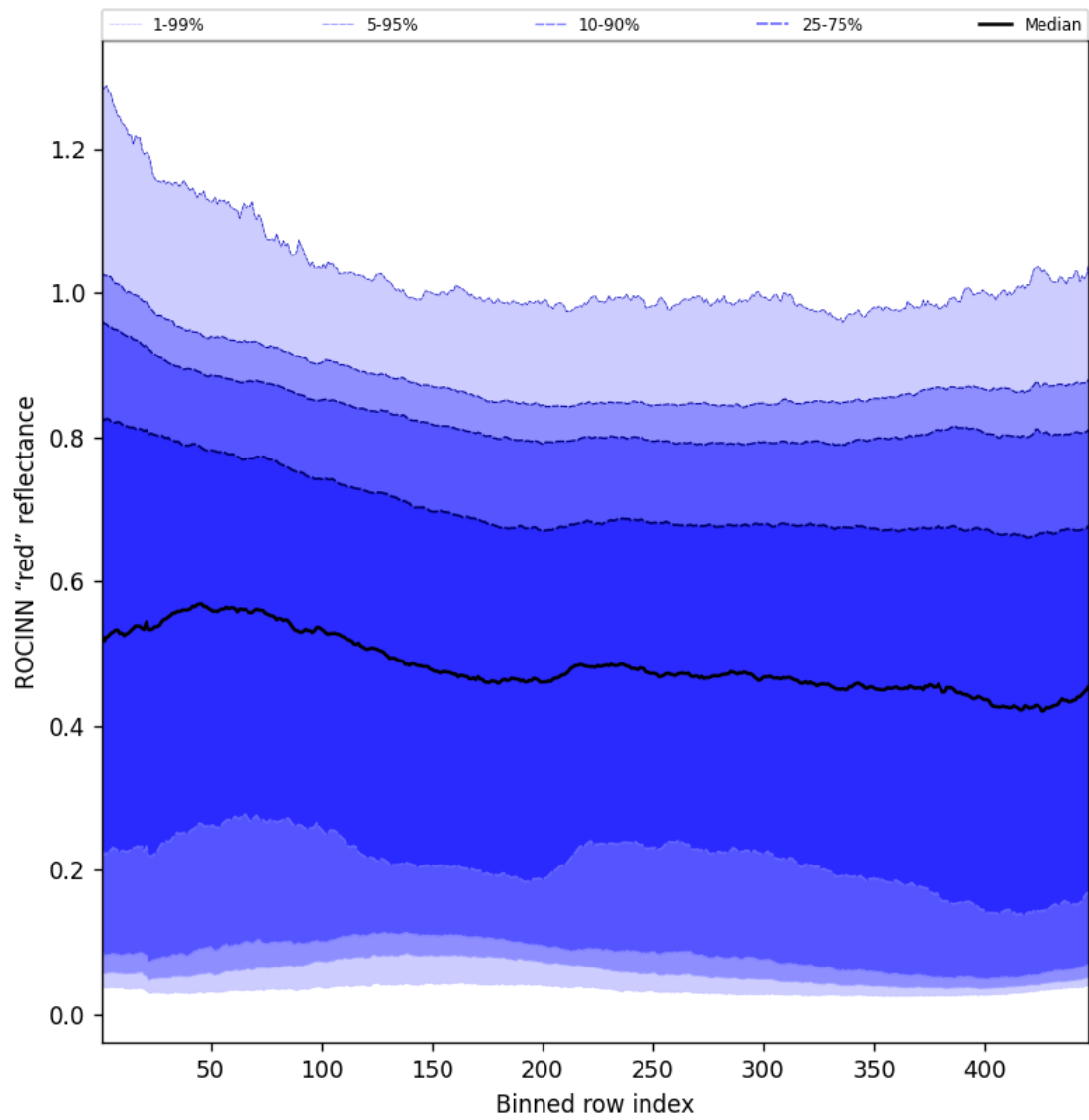
Figure 69: Along track statistics of “ROCINN “red” reflectance” for 2025-03-05 to 2025-03-07
