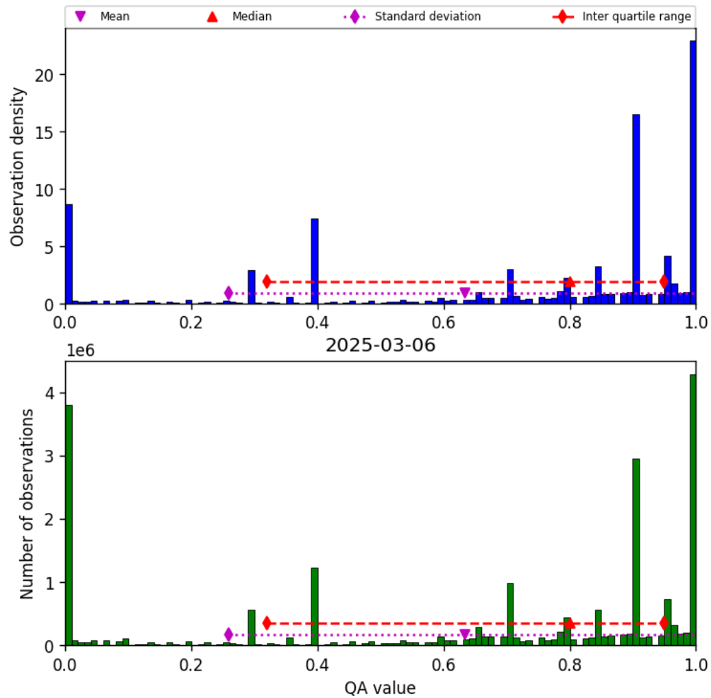
Figure 38: Histogram of “QA value” for 2025-03-05 to 2025-03-07
