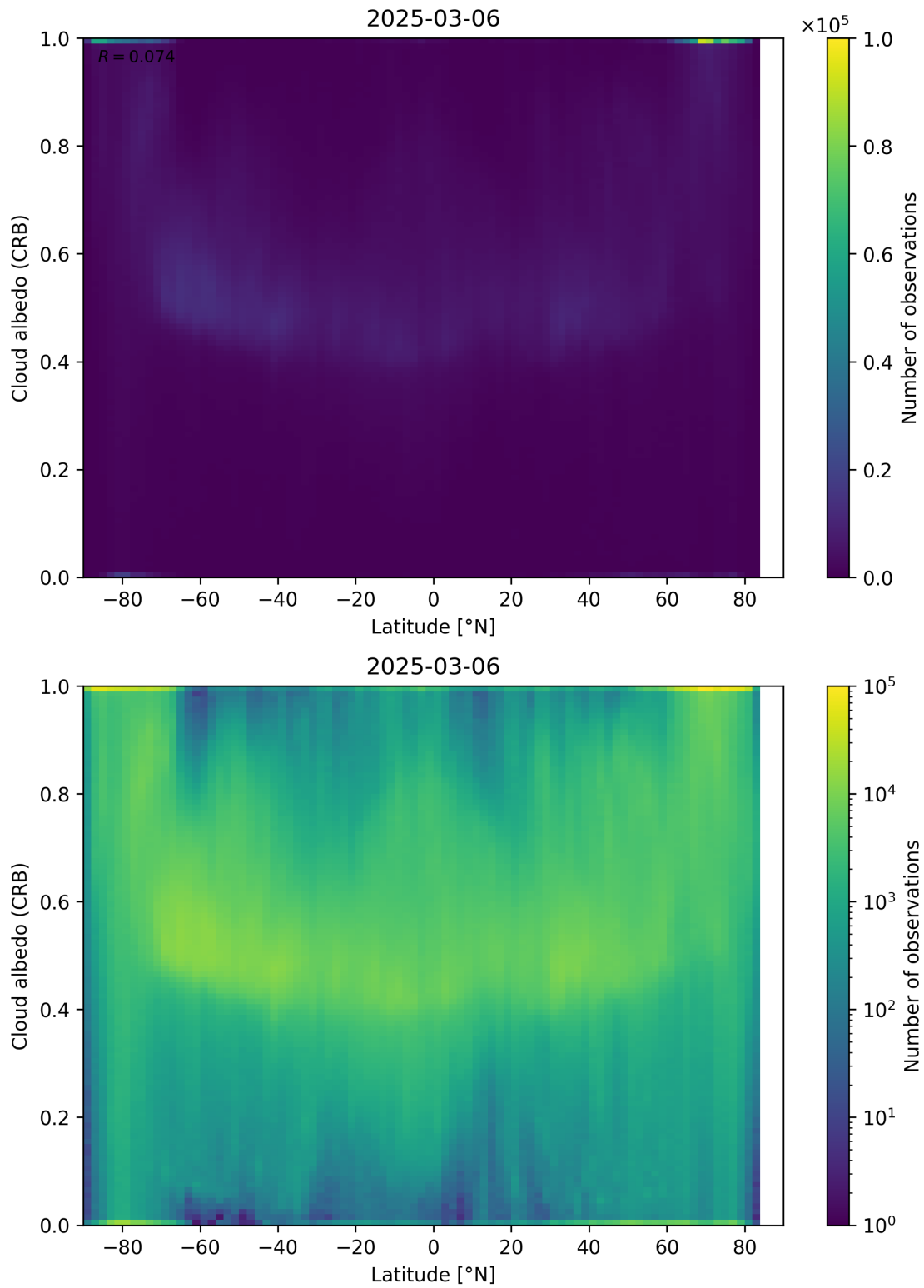
Figure 91: Scatter density plot of “Latitude” against “Cloud albedo (CRB)” for 2025-03-05 to 2025-03-07.
