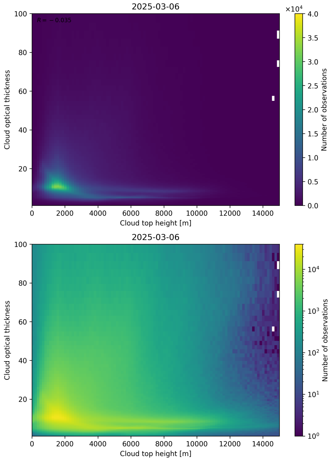
Figure 90: Scatter density plot of “Cloud top height” against “Cloud optical thickness” for 2025-03-05 to 2025-03-07.
