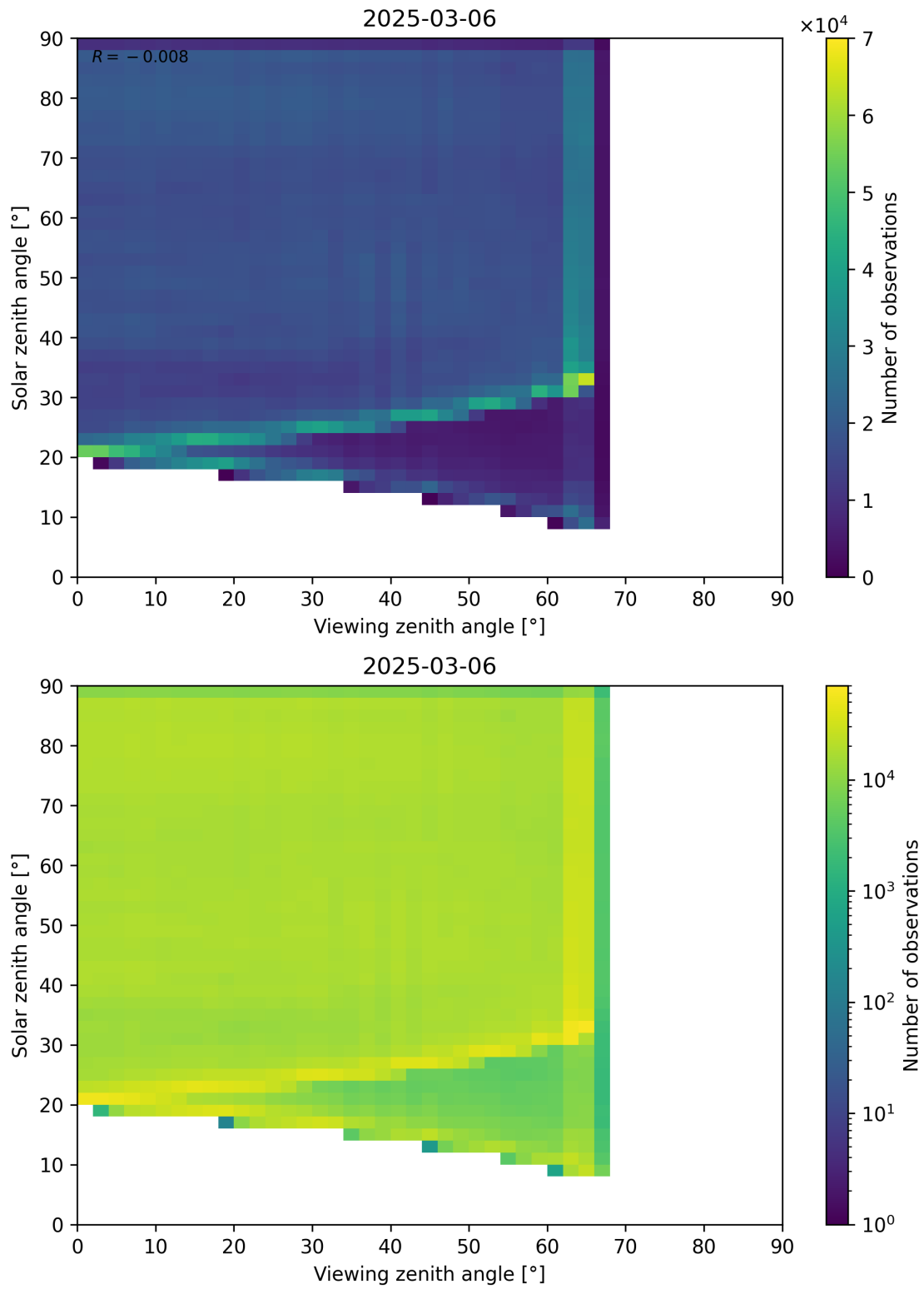
Figure 114: Scatter density plot of “Viewing zenith angle” against “Solar zenith angle” for 2025-03-05 to 2025-03-07.
