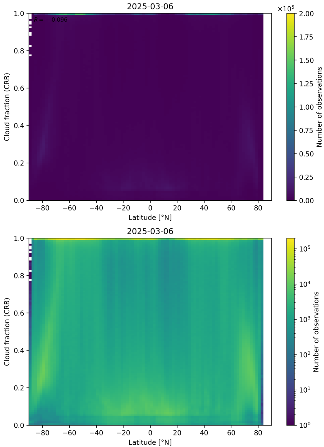
Figure 94: Scatter density plot of “Latitude” against “Cloud fraction (CRB)” for 2025-03-05 to 2025-03-07.
