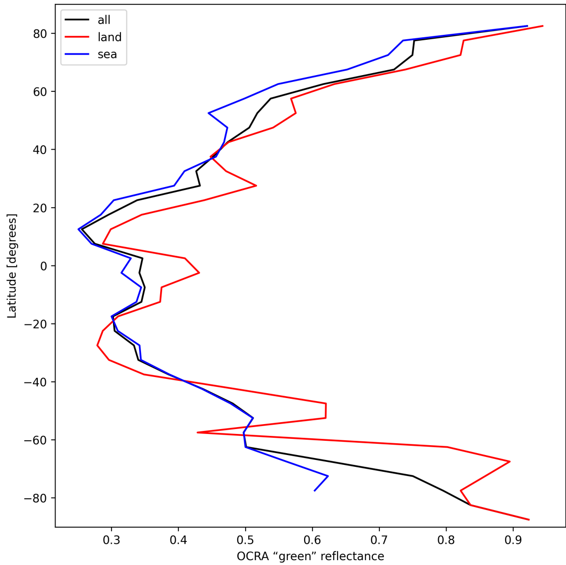
Figure 36: Zonal average of “OCRA “green” reflectance” for 2025-03-05 to 2025-03-07.
