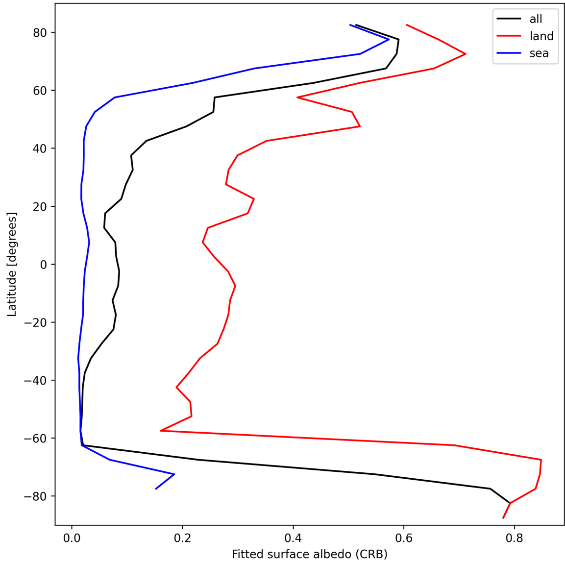
Figure 30: Zonal average of “Fitted surface albedo (CRB)” for 2025-03-07 to 2025-03-08.
