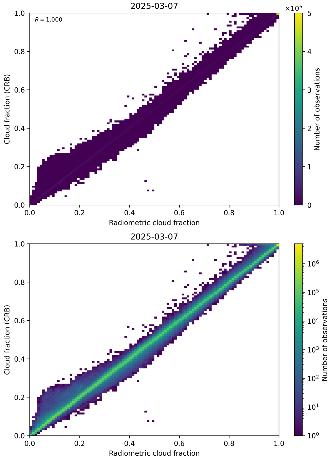
Figure 73: Scatter density plot of “Radiometric cloud fraction” against “Cloud fraction (CRB)” for 2025-03-07 to 2025-03-08.
