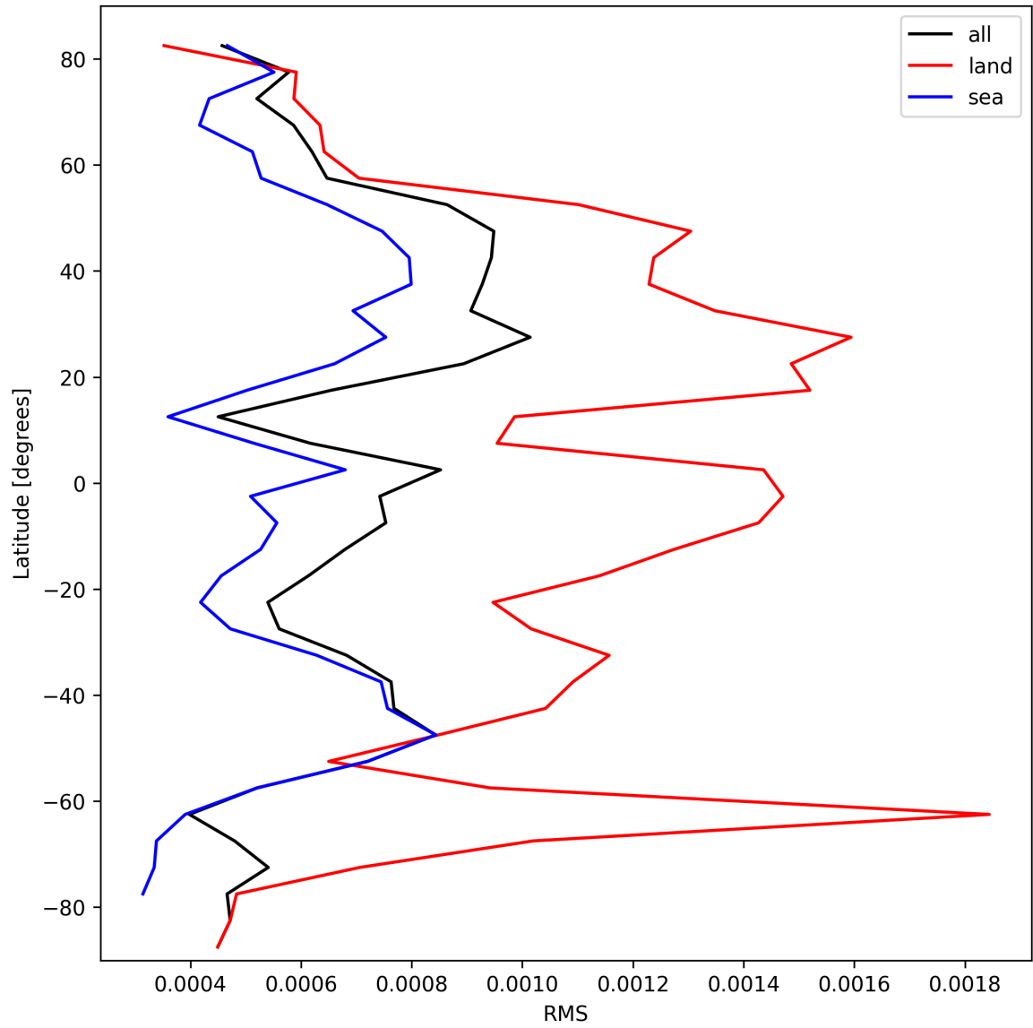
Figure 31: Zonal average of “RMS” for 2025-03-07 to 2025-03-08.
