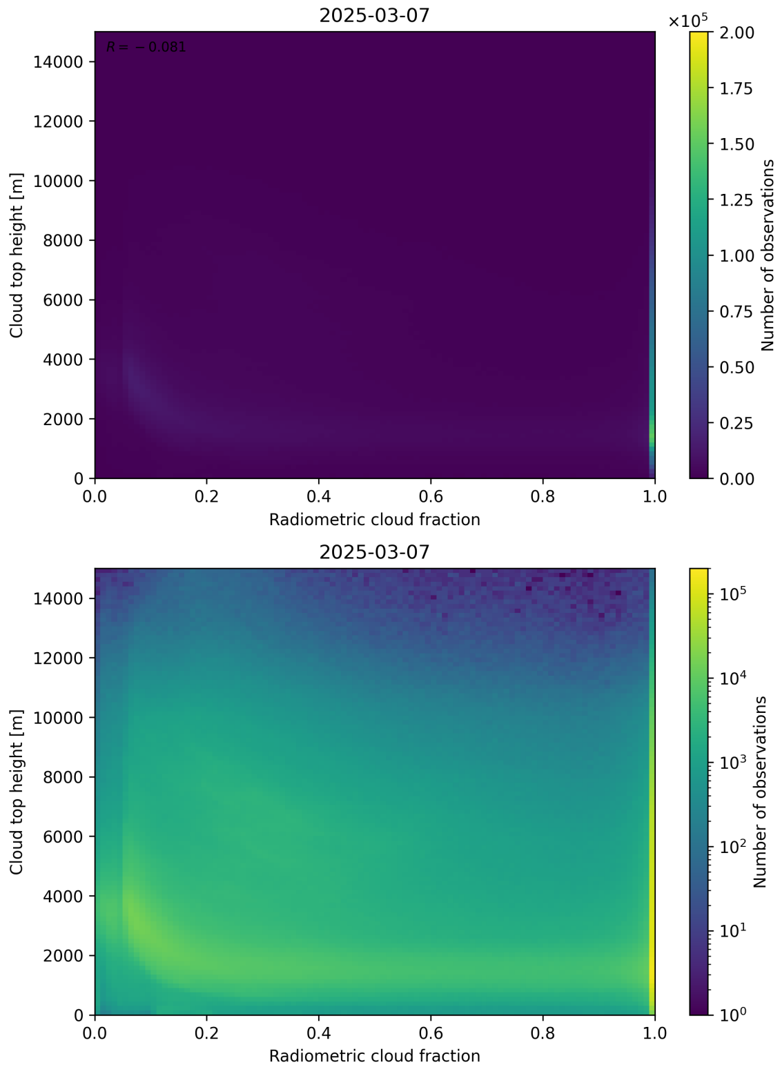
Figure 76: Scatter density plot of “Radiometric cloud fraction” against “Cloud top height” for 2025-03-07 to 2025-03-08.
