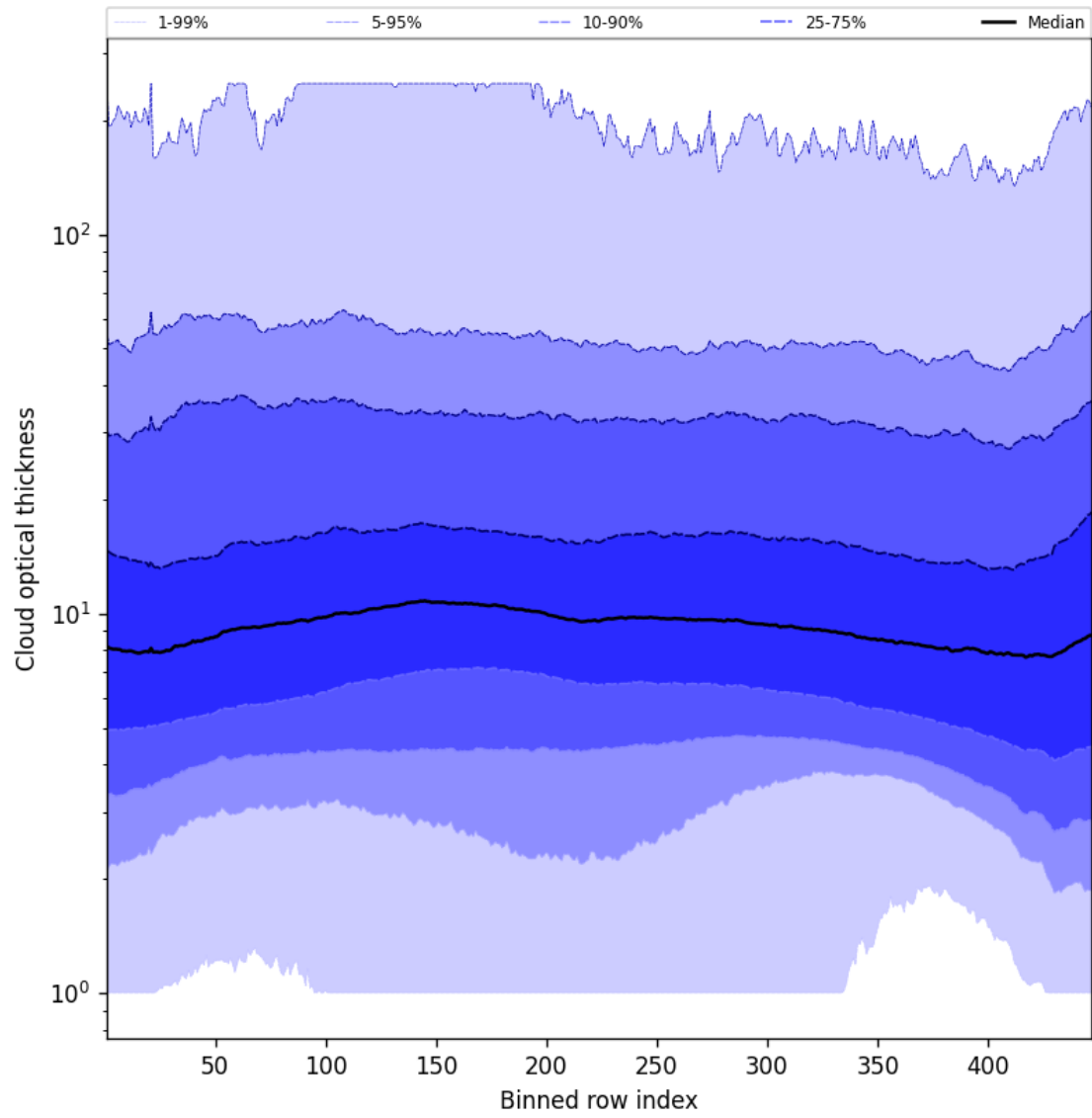
Figure 57: Along track statistics of “Cloud optical thickness” for 2025-03-07 to 2025-03-08
