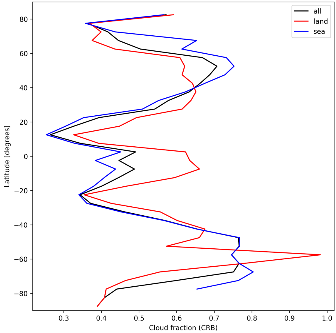
Figure 26: Zonal average of “Cloud fraction (CRB)” for 2025-03-07 to 2025-03-08.
