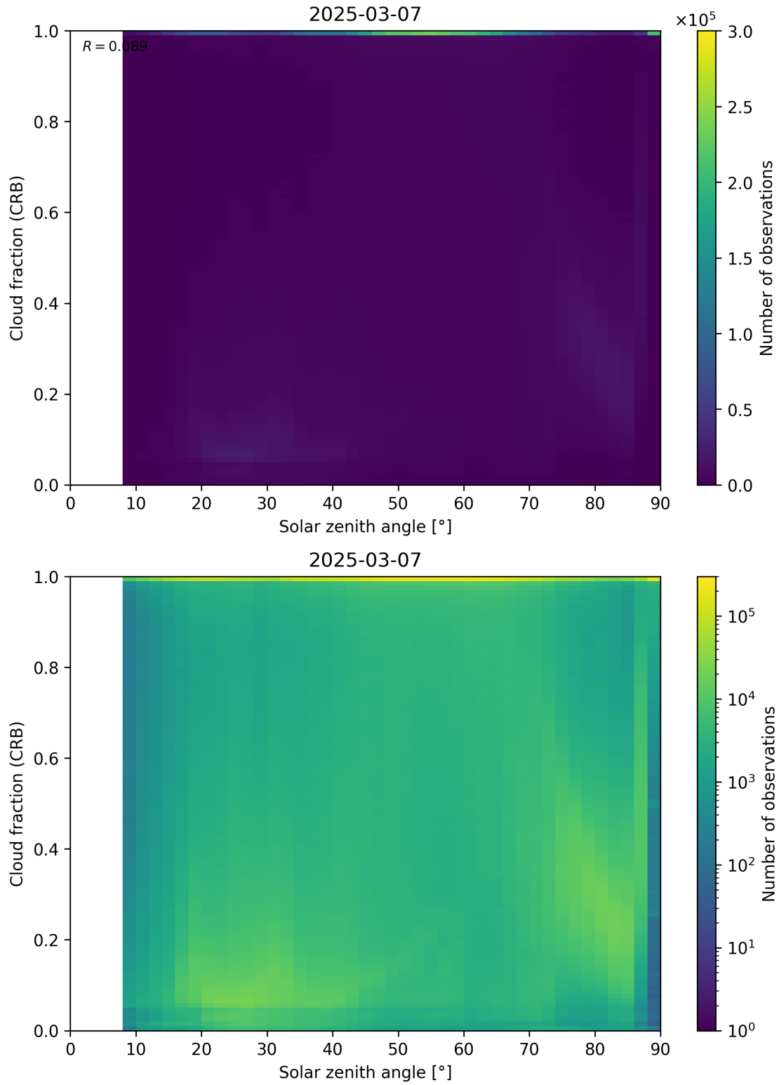
Figure 101: Scatter density plot of “Solar zenith angle” against “Cloud fraction (CRB)” for 2025-03-07 to 2025-03-08.
