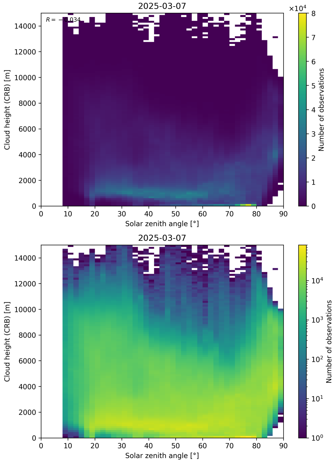
Figure 102: Scatter density plot of “Solar zenith angle” against “Cloud height (CRB)” for 2025-03-07 to 2025-03-08.
