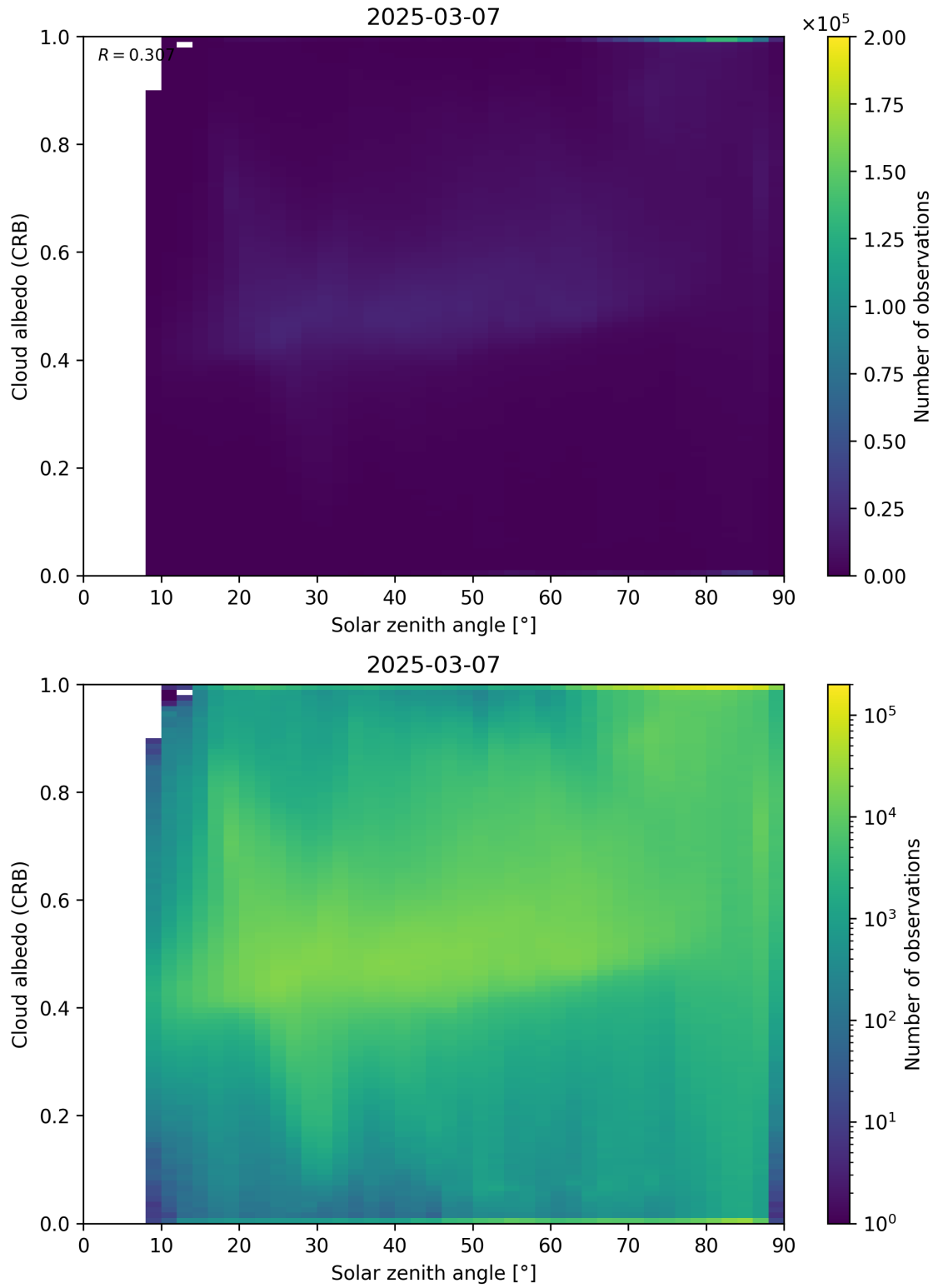
Figure 98: Scatter density plot of “Solar zenith angle” against “Cloud albedo (CRB)” for 2025-03-07 to 2025-03-08.
