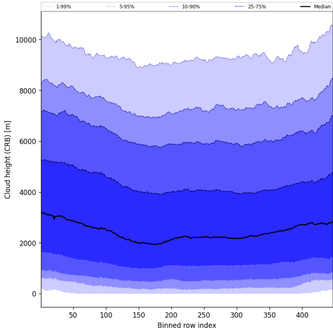
Figure 59: Along track statistics of “Cloud height (CRB)” for 2025-03-07 to 2025-03-08
