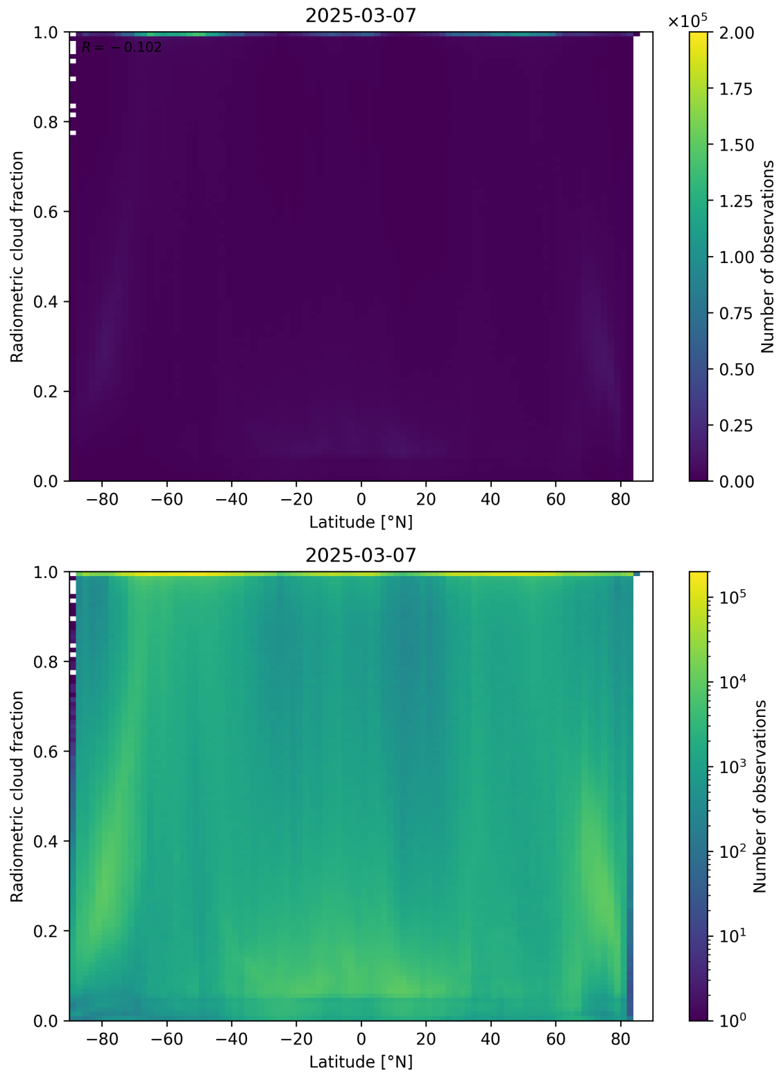
Figure 92: Scatter density plot of “Latitude” against “Radiometric cloud fraction” for 2025-03-07 to 2025-03-08.
