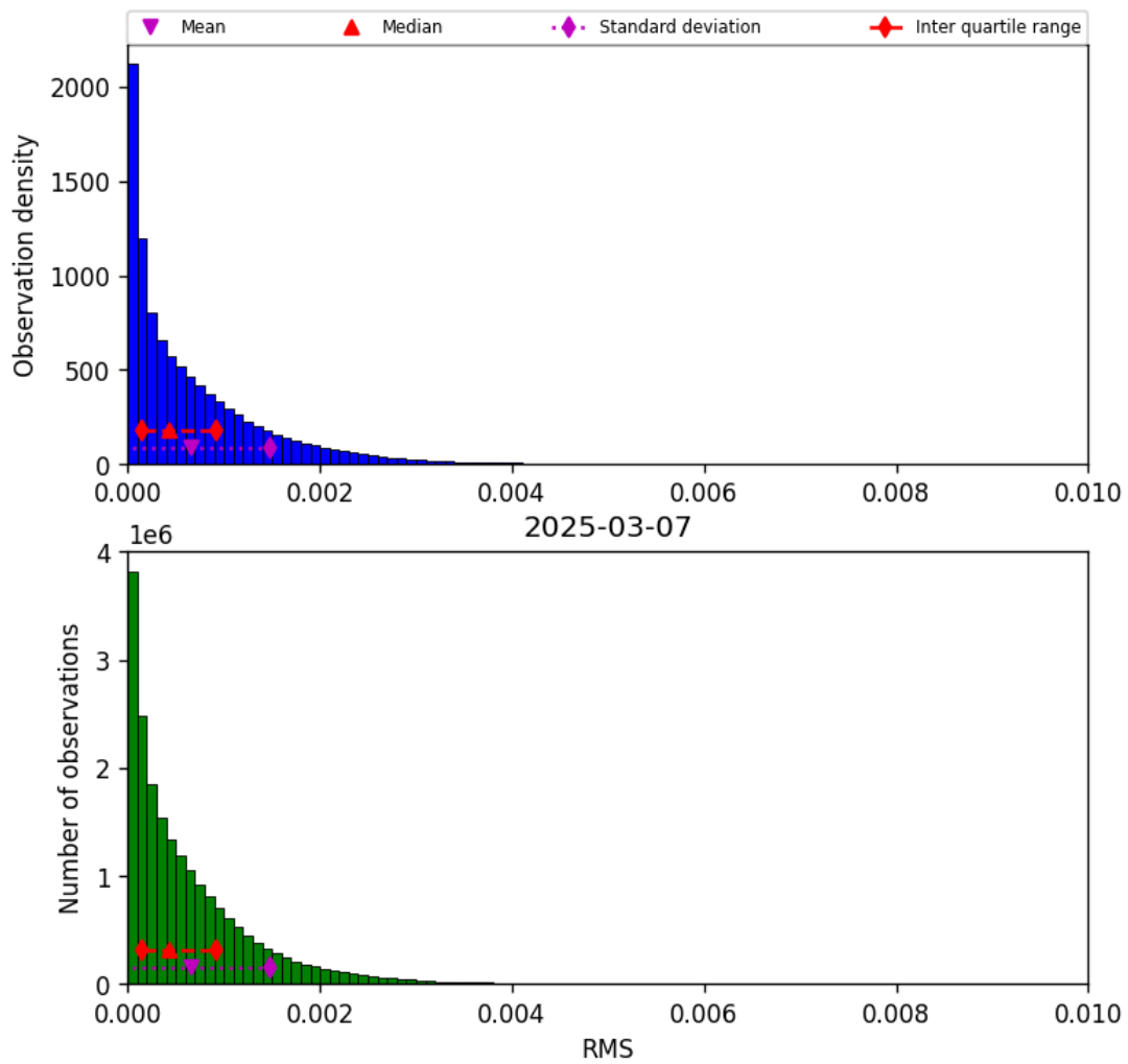
Figure 47: Histogram of “RMS” for 2025-03-07 to 2025-03-08
