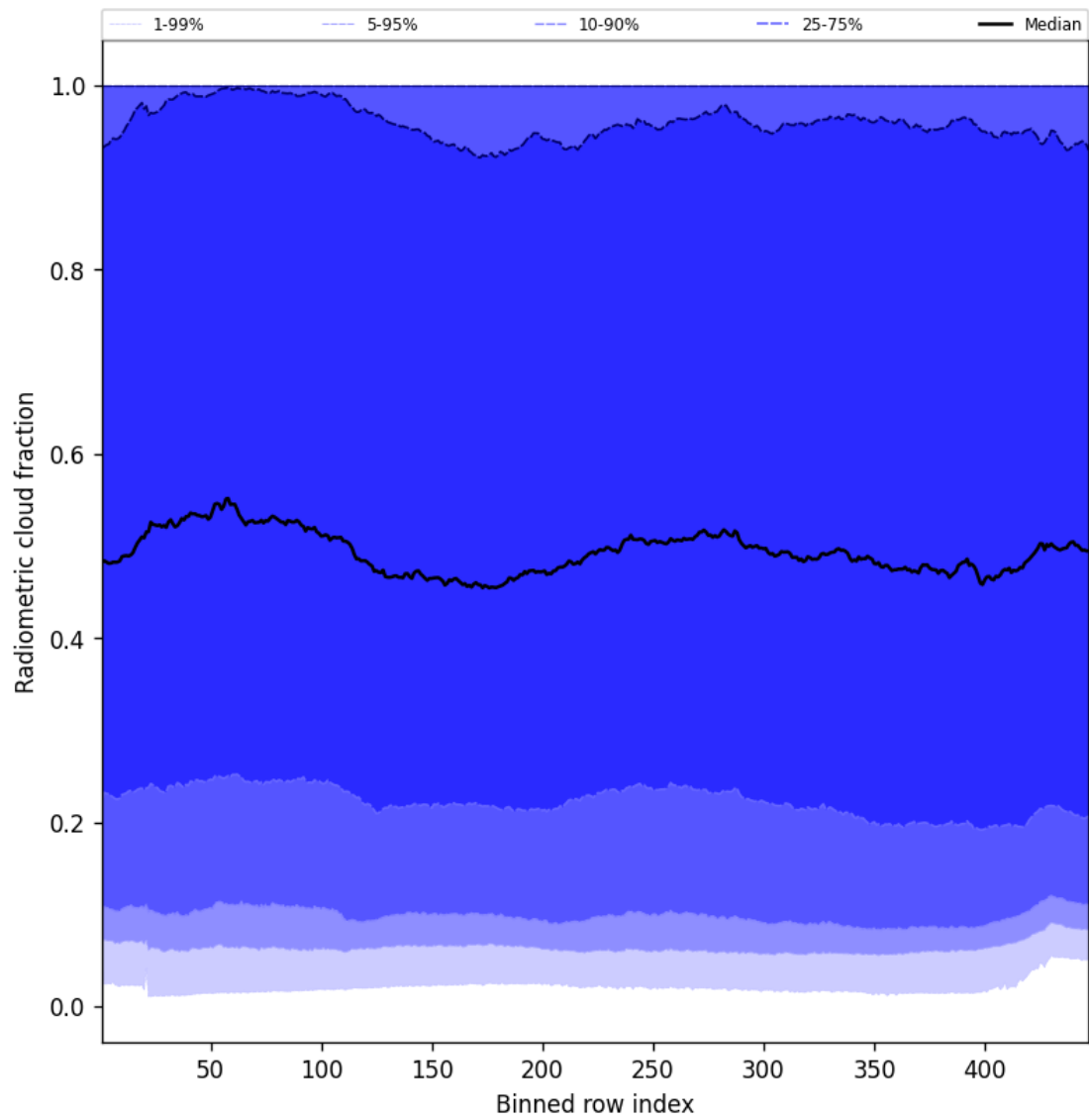
Figure 55: Along track statistics of “Radiometric cloud fraction” for 2025-03-07 to 2025-03-08
