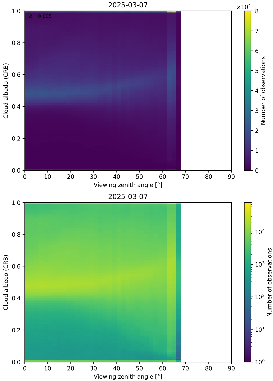
Figure 106: Scatter density plot of “Viewing zenith angle” against “Cloud albedo (CRB)” for 2025-03-07 to 2025-03-08.
