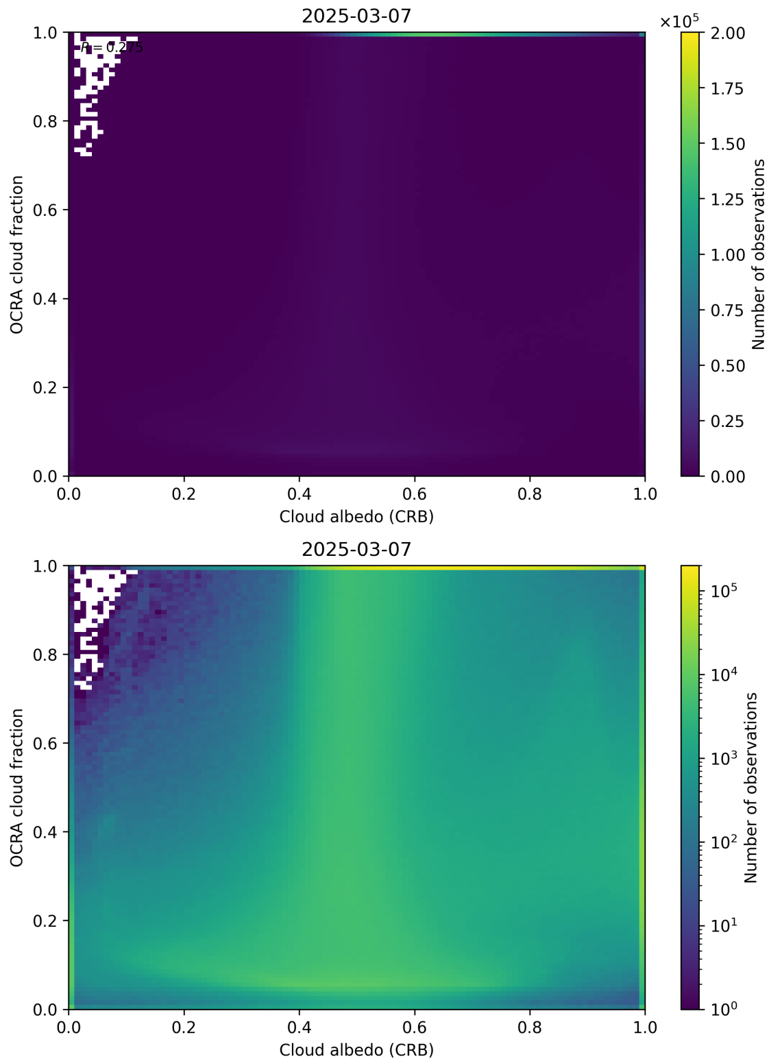
Figure 70: Scatter density plot of “Cloud albedo (CRB)” against “OCRA cloud fraction” for 2025-03-07 to 2025-03-08.
