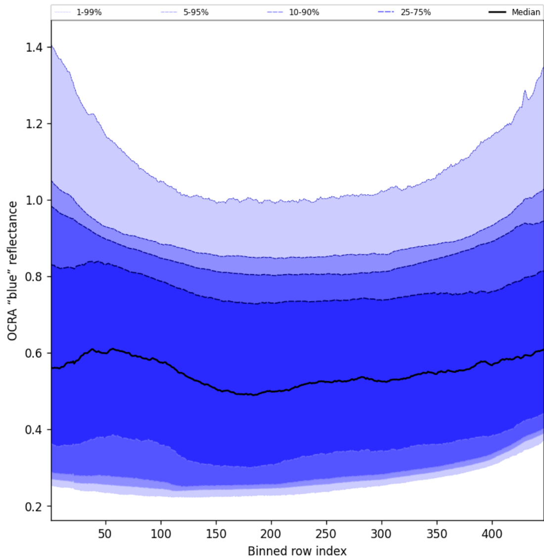
Figure 67: Along track statistics of “OCRA “blue” reflectance” for 2025-03-07 to 2025-03-08
