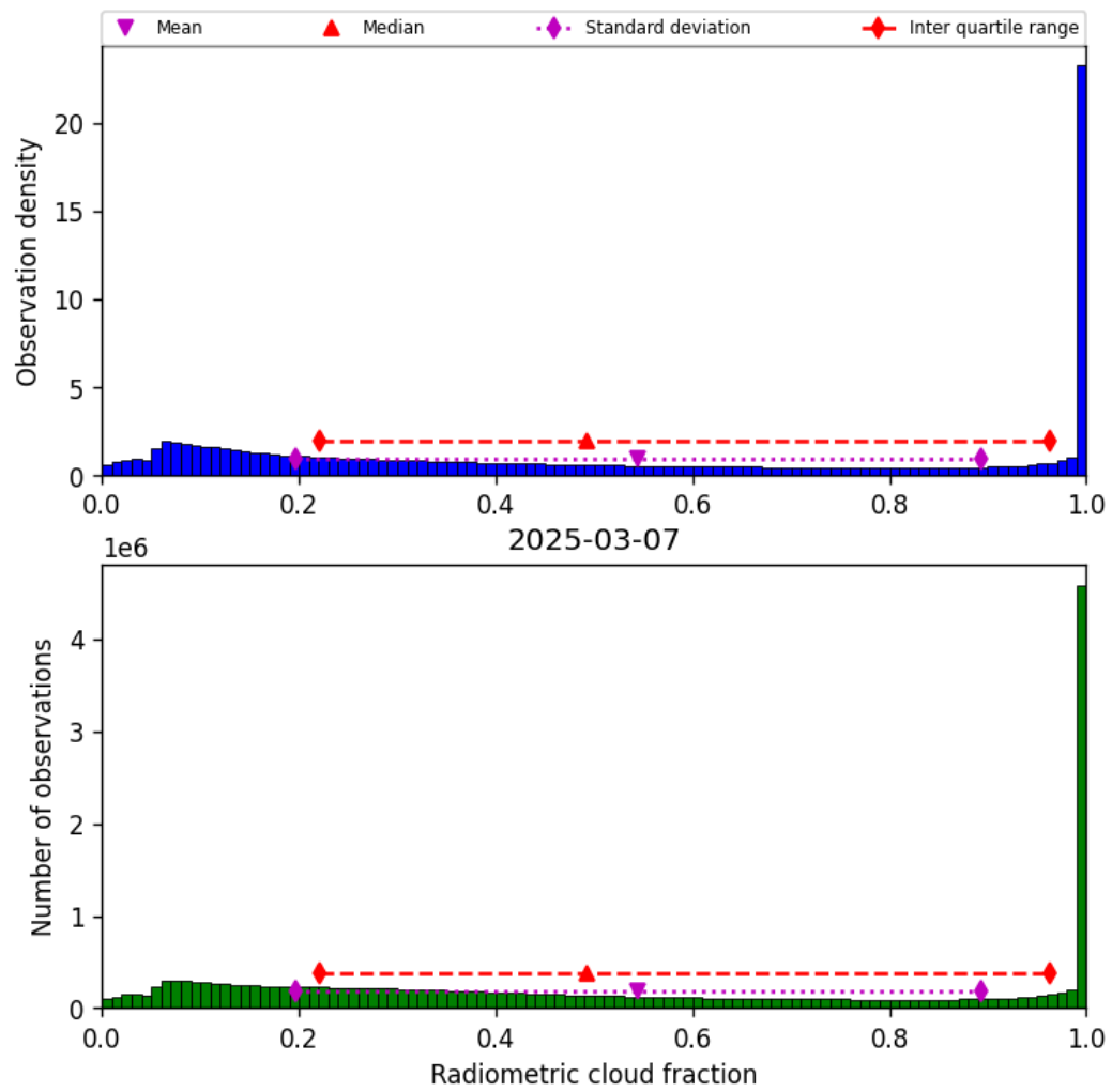
Figure 39: Histogram of “Radiometric cloud fraction” for 2025-03-07 to 2025-03-08
