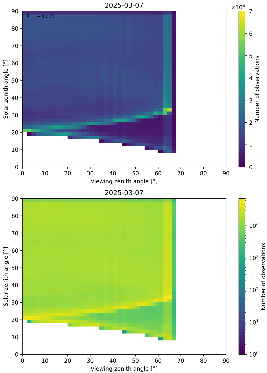
Figure 114: Scatter density plot of “Viewing zenith angle” against “Solar zenith angle” for 2025-03-07 to 2025-03-08.
