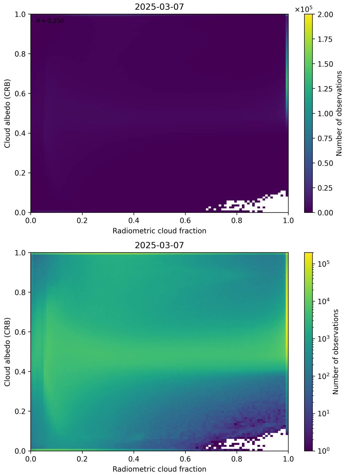
Figure 71: Scatter density plot of “Radiometric cloud fraction” against “Cloud albedo (CRB)” for 2025-03-07 to 2025-03-08.
