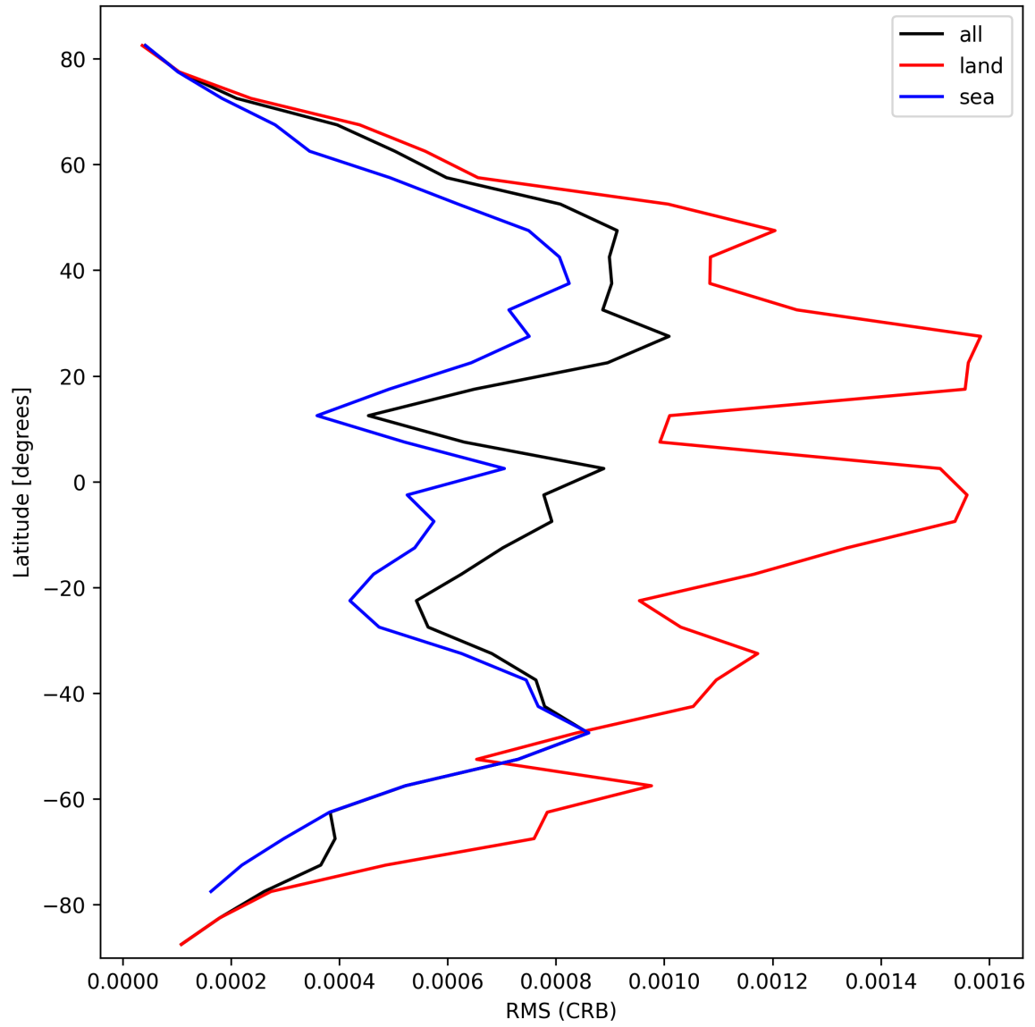
Figure 32: Zonal average of “RMS (CRB)” for 2025-03-07 to 2025-03-08.
