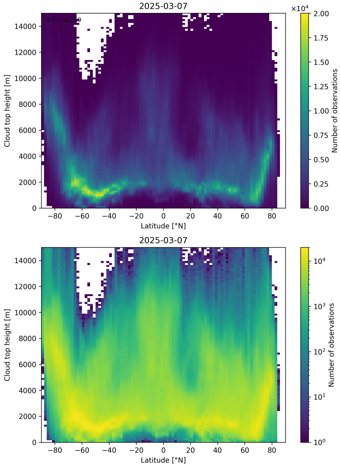
Figure 97: Scatter density plot of “Latitude” against “Cloud top height” for 2025-03-07 to 2025-03-08.
