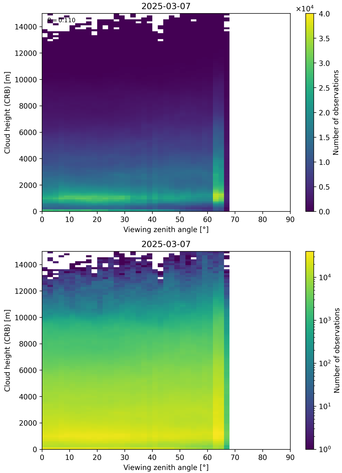
Figure 110: Scatter density plot of “Viewing zenith angle” against “Cloud height (CRB)” for 2025-03-07 to 2025-03-08.
