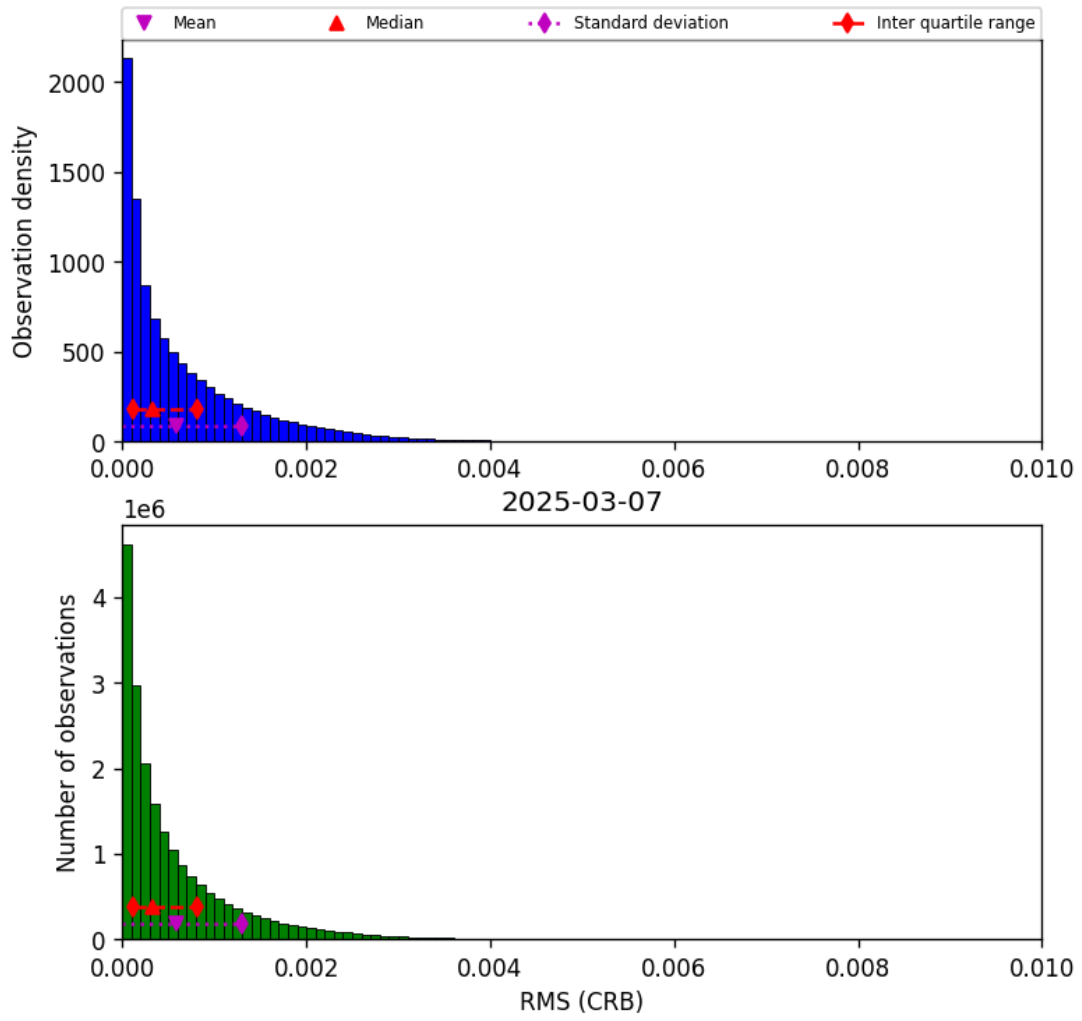
Figure 48: Histogram of "RMS (CRB)" for 2025-03-07 to 2025-03-08
