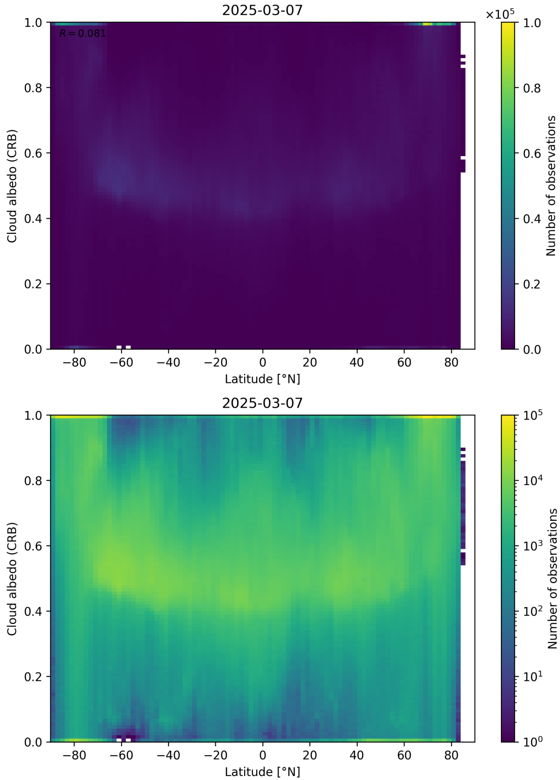
Figure 91: Scatter density plot of “Latitude” against “Cloud albedo (CRB)” for 2025-03-07 to 2025-03-08.
