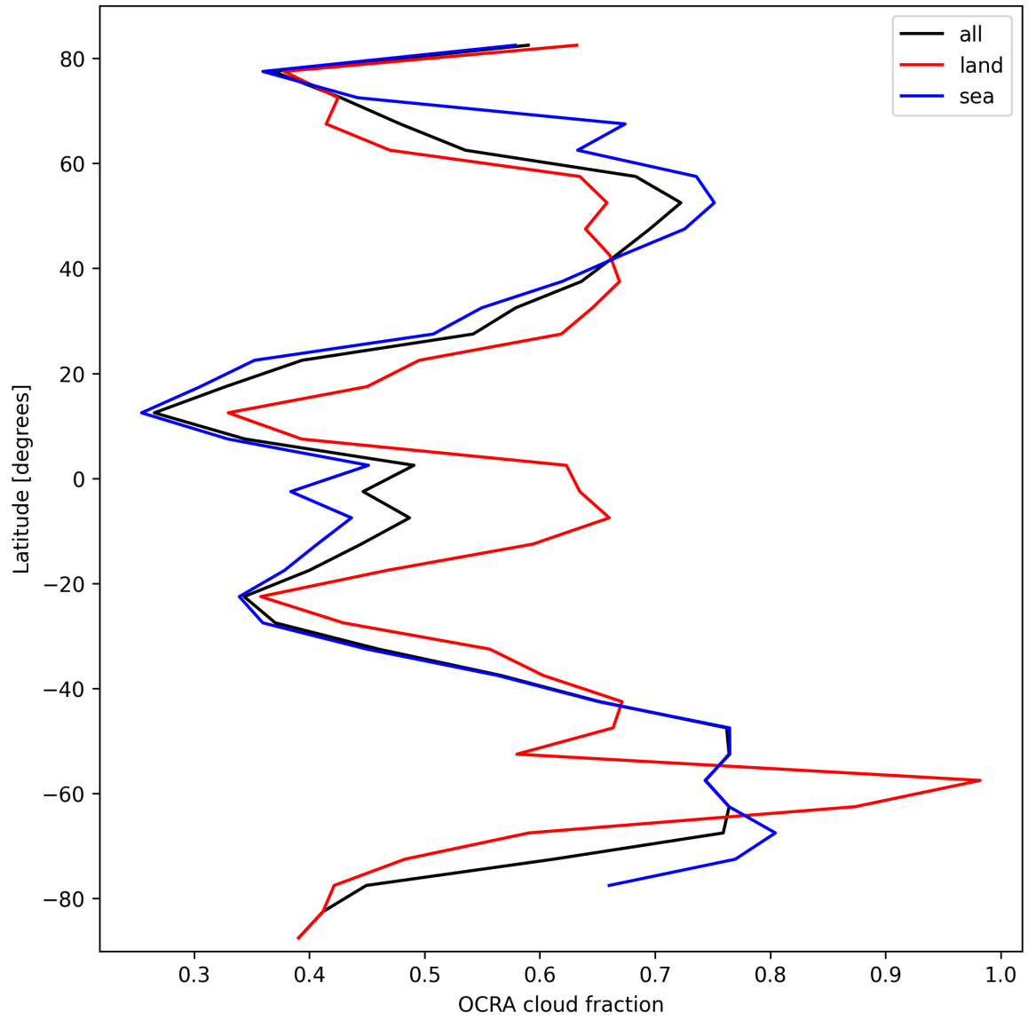
Figure 34: Zonal average of “OCRA cloud fraction” for 2025-03-07 to 2025-03-08.
