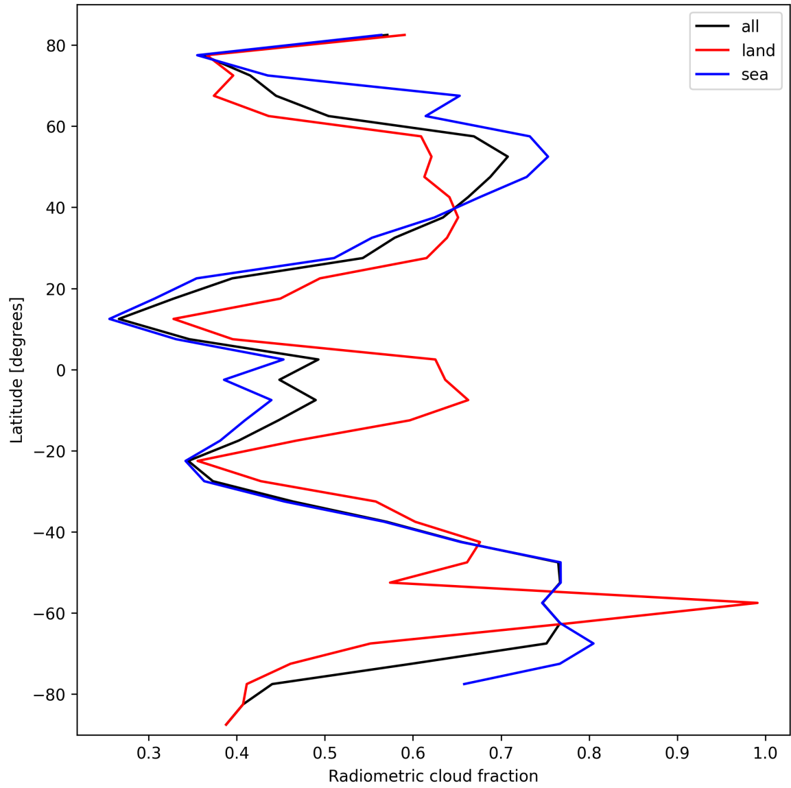
Figure 23: Zonal average of “Radiometric cloud fraction” for 2025-03-07 to 2025-03-08.
