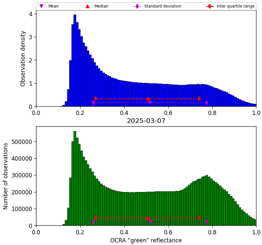
Figure 52: Histogram of “OCRA “green” reflectance” for 2025-03-07 to 2025-03-08
