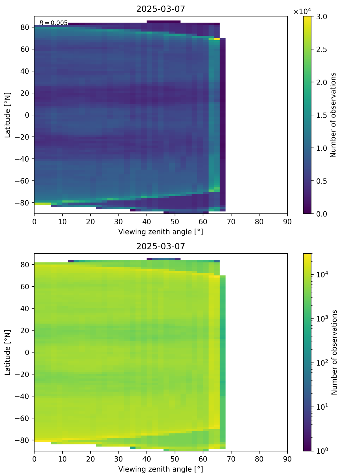
Figure 113: Scatter density plot of “Viewing zenith angle” against “Latitude” for 2025-03-07 to 2025-03-08.
