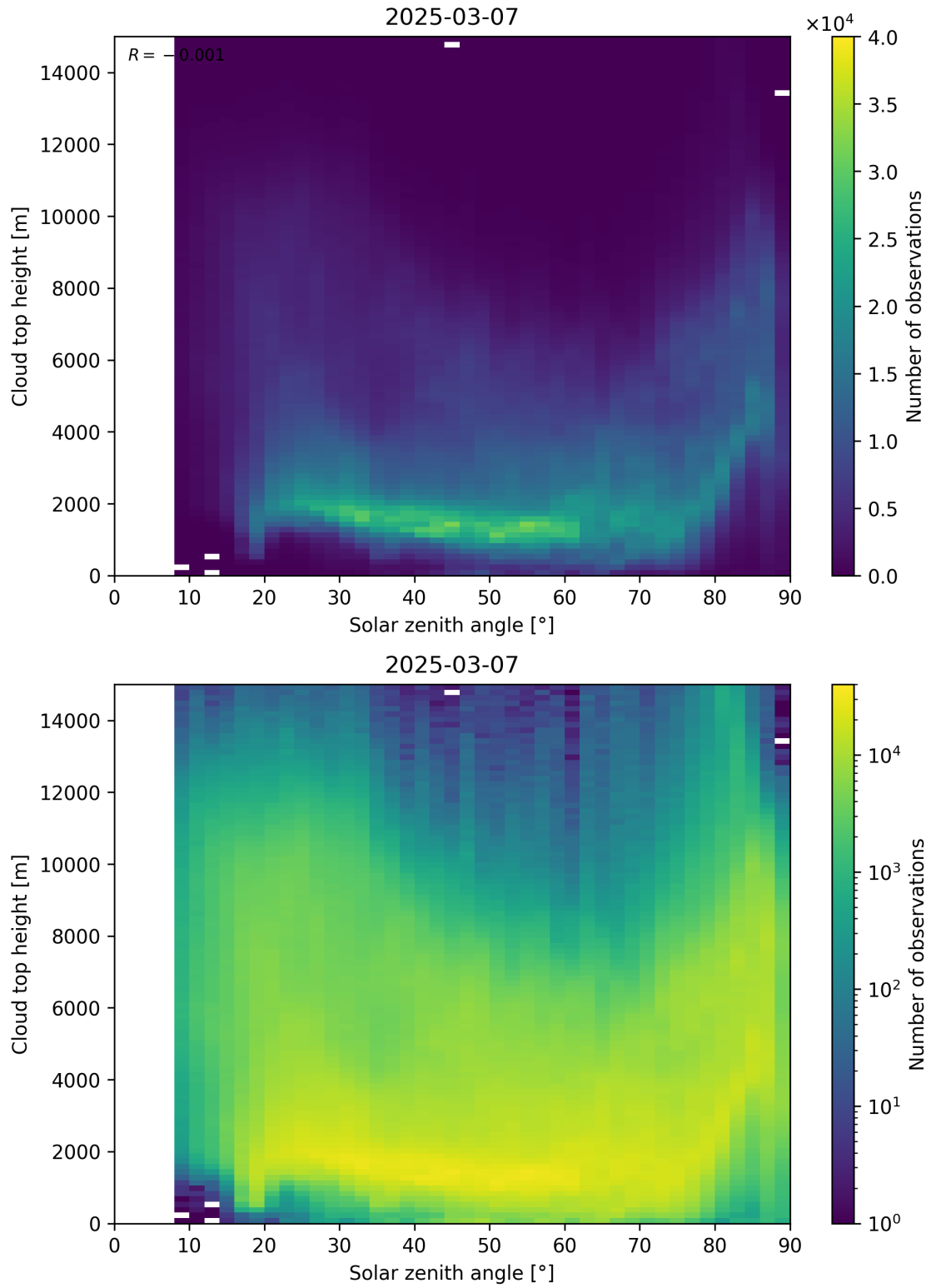
Figure 104: Scatter density plot of “Solar zenith angle” against “Cloud top height” for 2025-03-07 to 2025-03-08.
