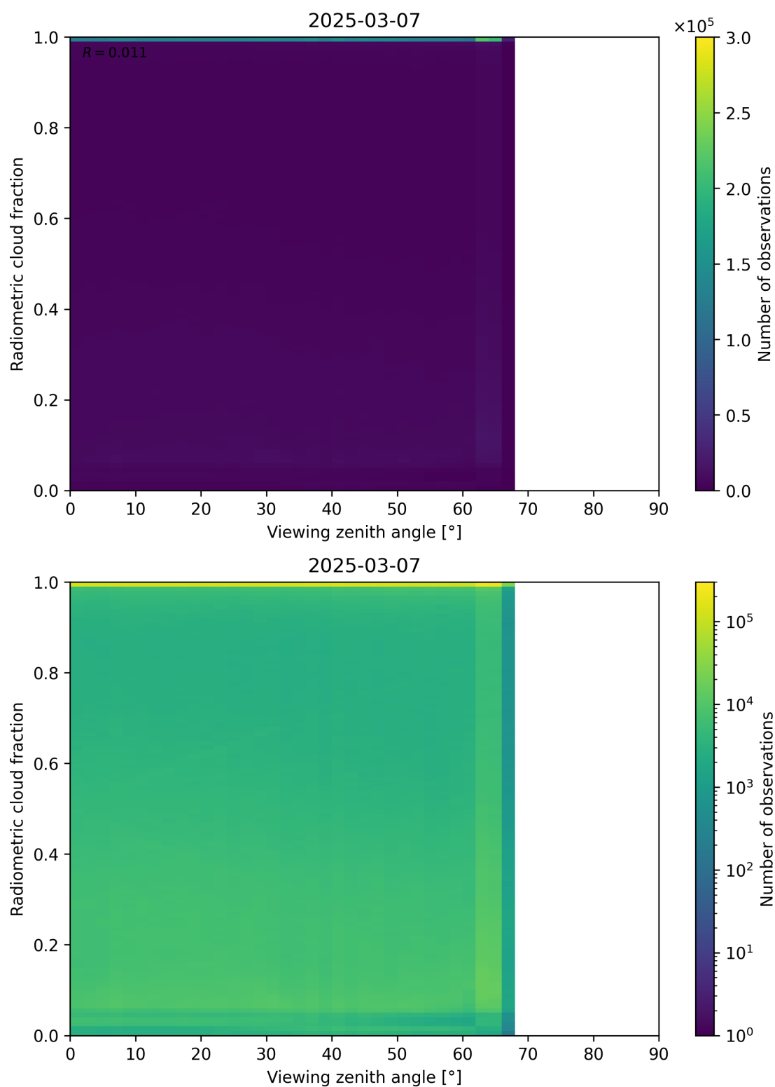
Figure 107: Scatter density plot of “Viewing zenith angle” against “Radiometric cloud fraction” for 2025-03-07 to 2025-03-08.
