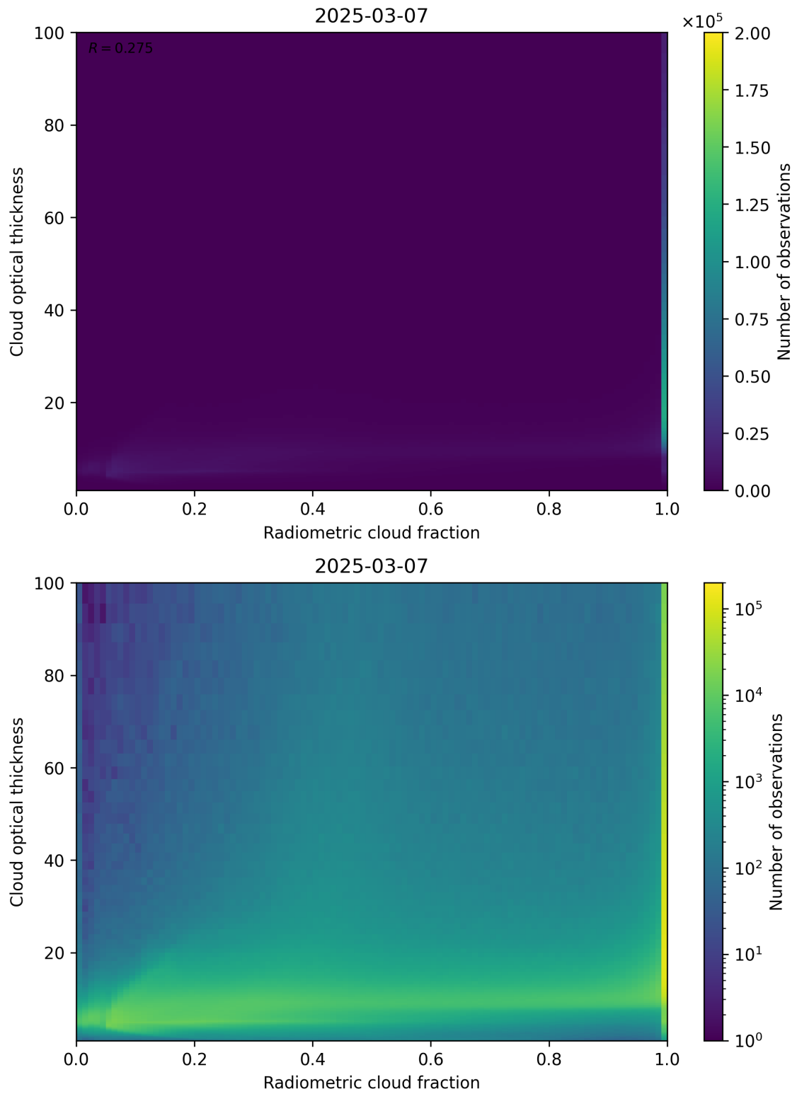
Figure 75: Scatter density plot of “Radiometric cloud fraction” against “Cloud optical thickness” for 2025-03-07 to 2025-03-08.
