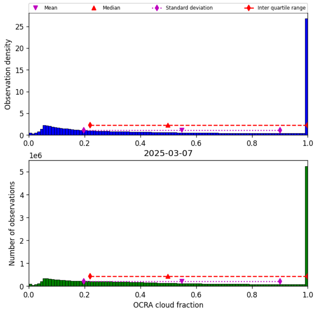
Figure 50: Histogram of “OCRA cloud fraction” for 2025-03-07 to 2025-03-08
