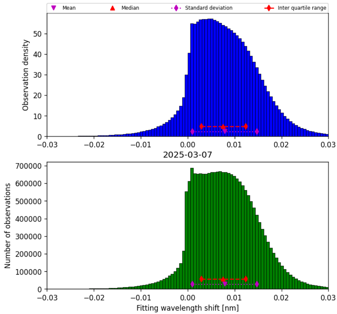
Figure 49: Histogram of “Fitting wavelength shift” for 2025-03-07 to 2025-03-08
