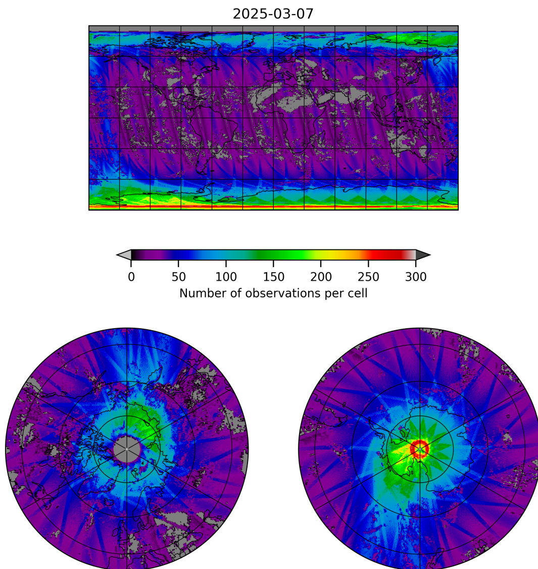
Figure 21: Map of the number of observations for 2025-03-07 to 2025-03-08
