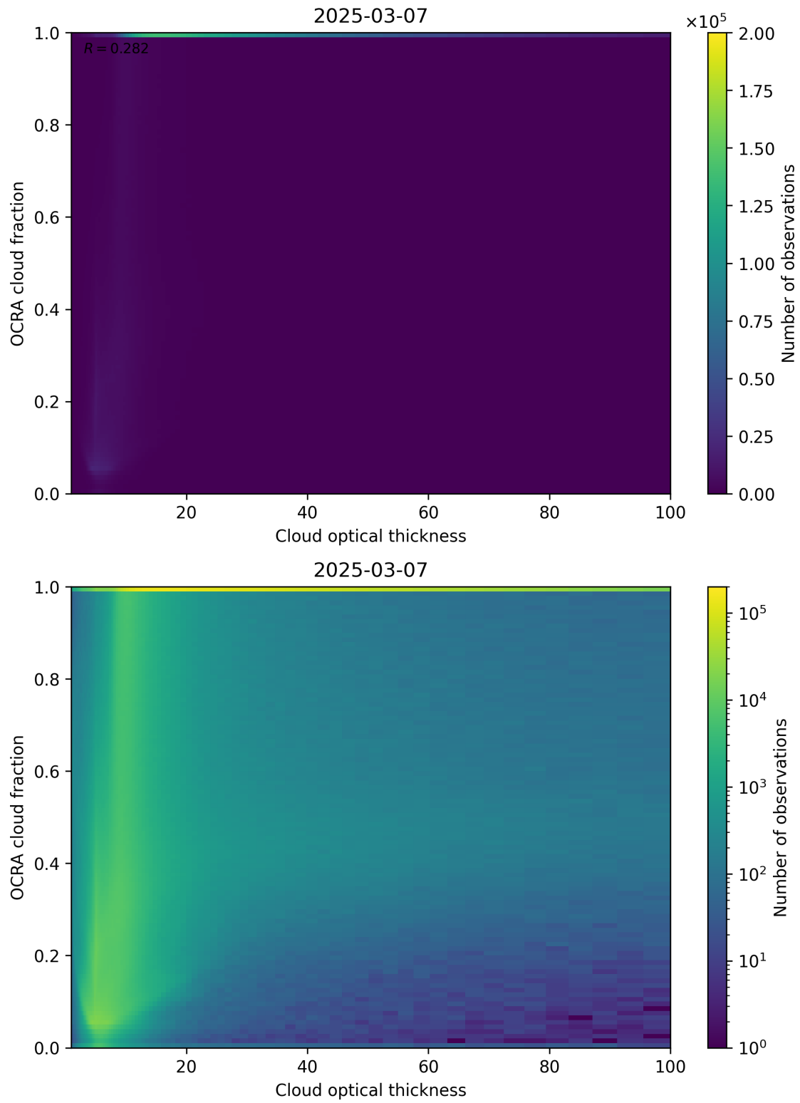
Figure 83: Scatter density plot of “Cloud optical thickness” against “OCRA cloud fraction” for 2025-03-07 to 2025-03-08.
