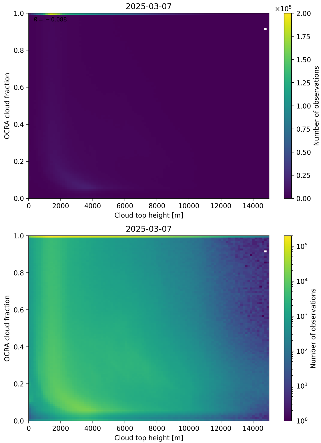
Figure 87: Scatter density plot of “Cloud top height” against “OCRA cloud fraction” for 2025-03-07 to 2025-03-08.
