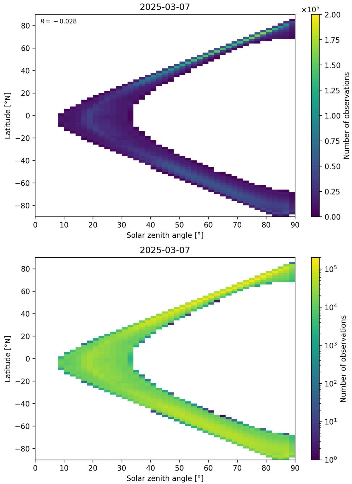
Figure 105: Scatter density plot of “Solar zenith angle” against “Latitude” for 2025-03-07 to 2025-03-08.
