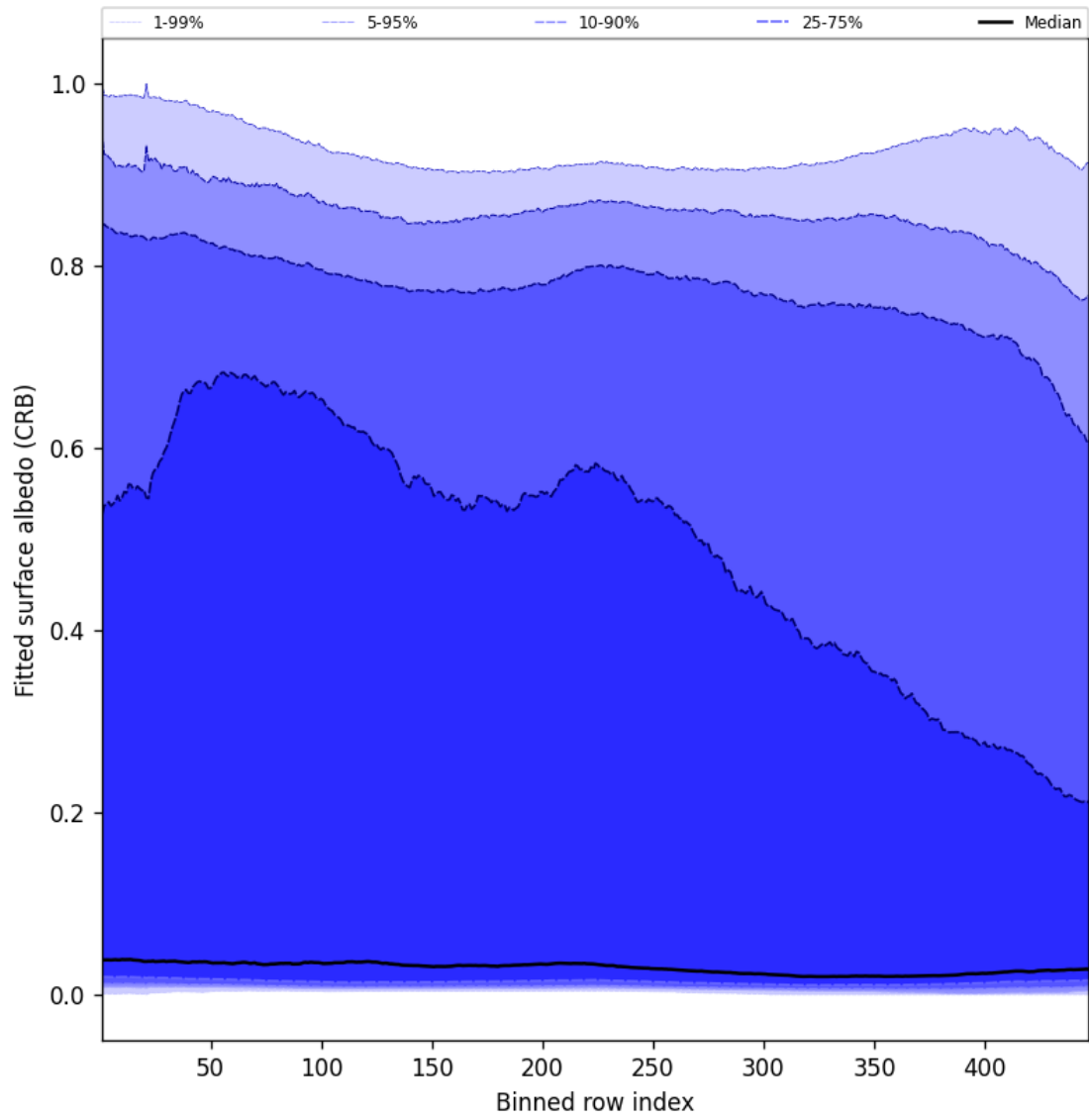
Figure 62: Along track statistics of “Fitted surface albedo (CRB)” for 2025-03-07 to 2025-03-08
