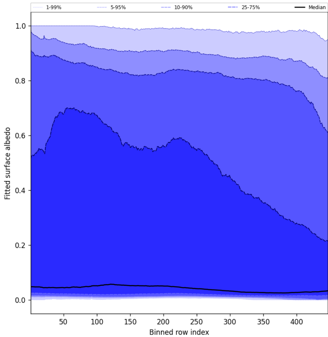
Figure 61: Along track statistics of “Fitted surface albedo” for 2025-03-07 to 2025-03-08
