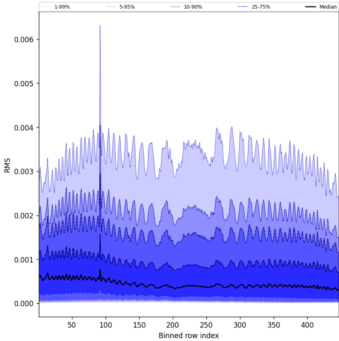
Figure 63: Along track statistics of “RMS” for 2025-03-07 to 2025-03-08
