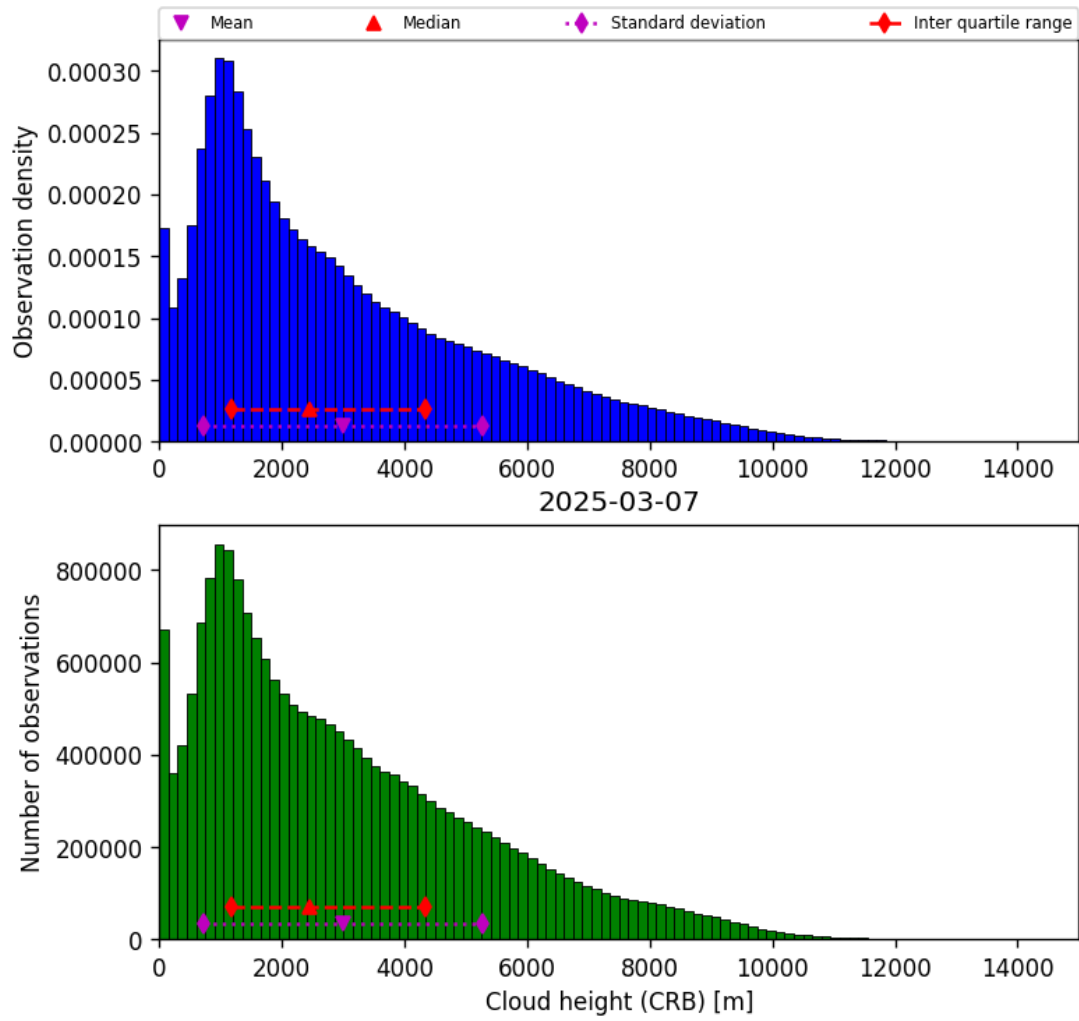
Figure 43: Histogram of “Cloud height (CRB)” for 2025-03-07 to 2025-03-08
