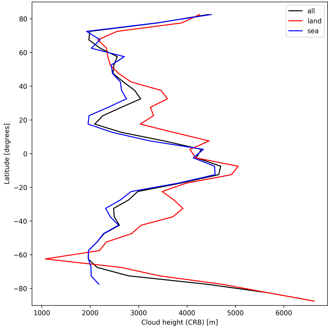
Figure 27: Zonal average of “Cloud height (CRB)” for 2025-03-07 to 2025-03-08.
