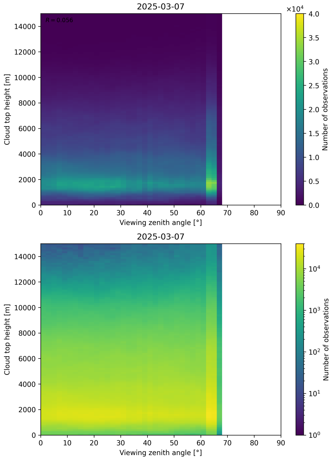
Figure 112: Scatter density plot of “Viewing zenith angle” against “Cloud top height” for 2025-03-07 to 2025-03-08.
