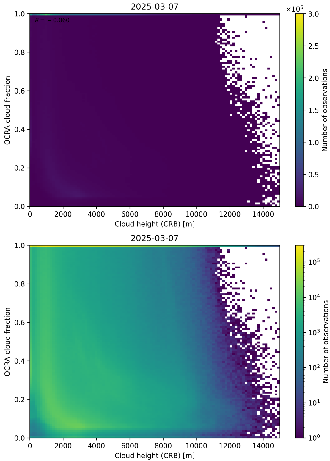
Figure 81: Scatter density plot of “Cloud height (CRB)” against “OCRA cloud fraction” for 2025-03-07 to 2025-03-08.
