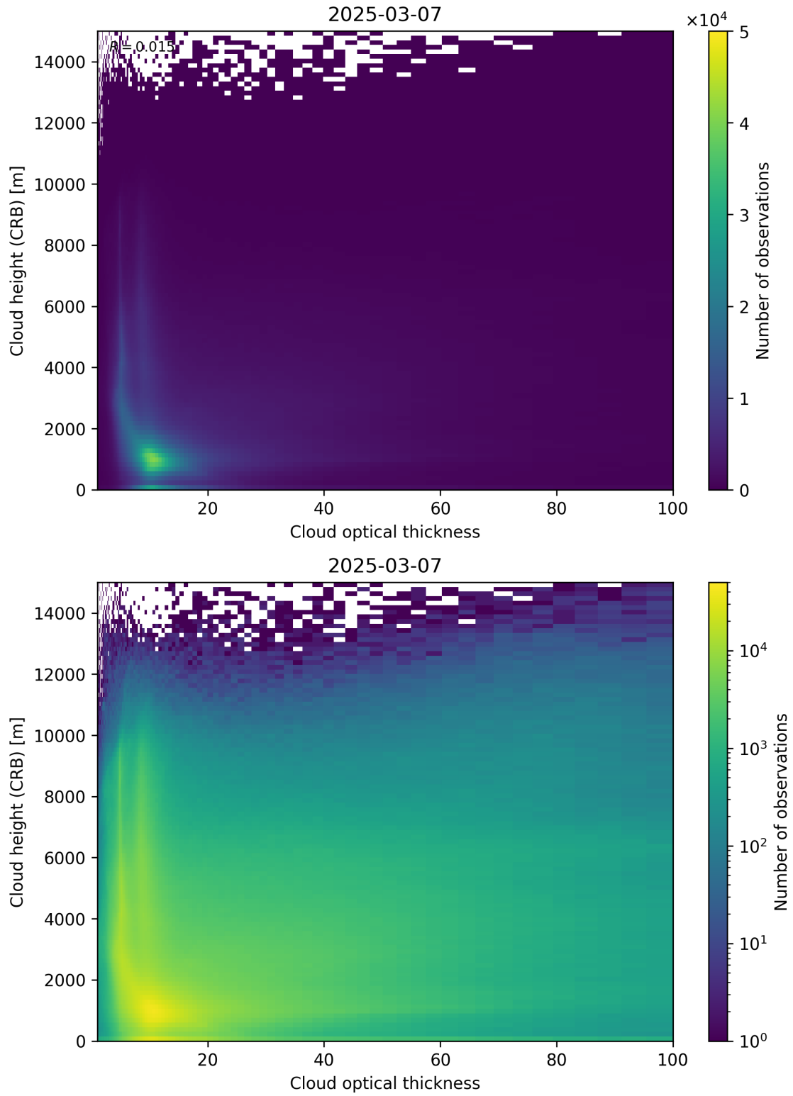
Figure 85: Scatter density plot of “Cloud optical thickness” against “Cloud height (CRB)” for 2025-03-07 to 2025-03-08.
