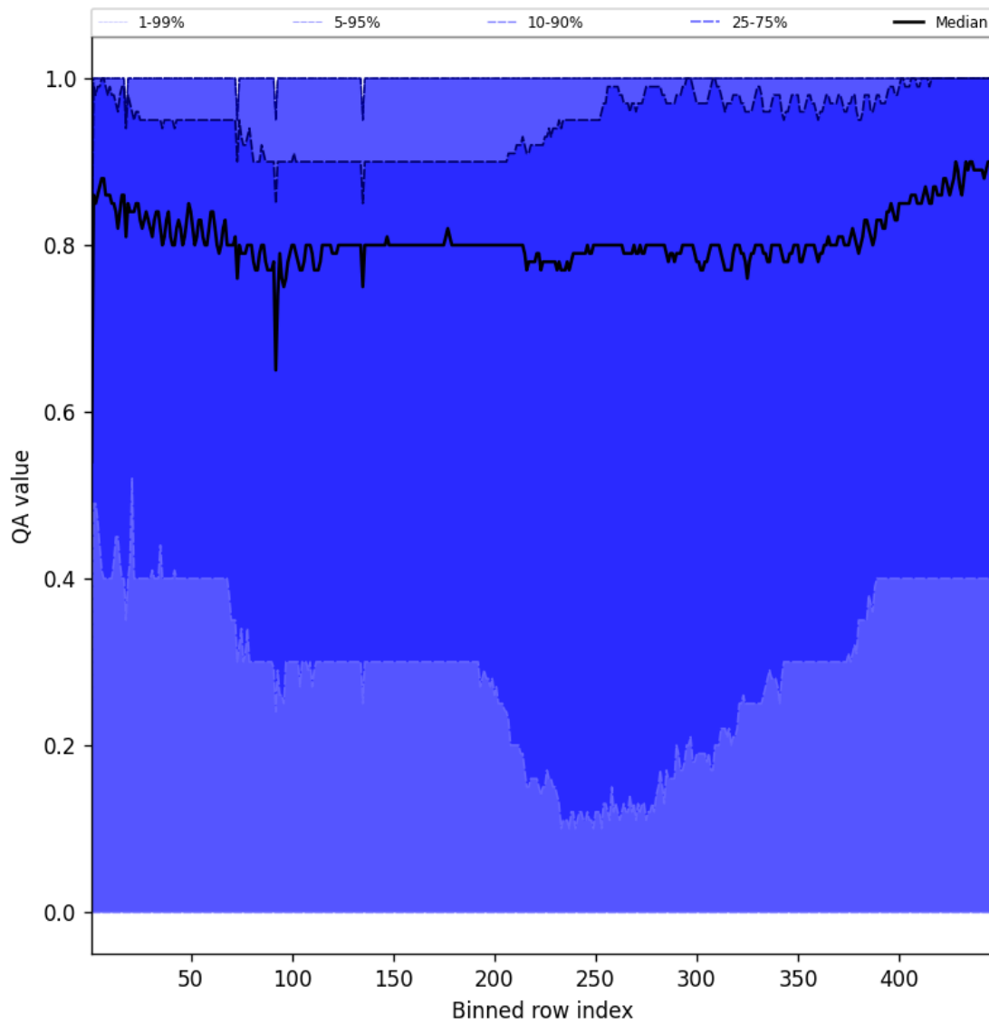
Figure 54: Along track statistics of “QA value” for 2025-03-07 to 2025-03-08
