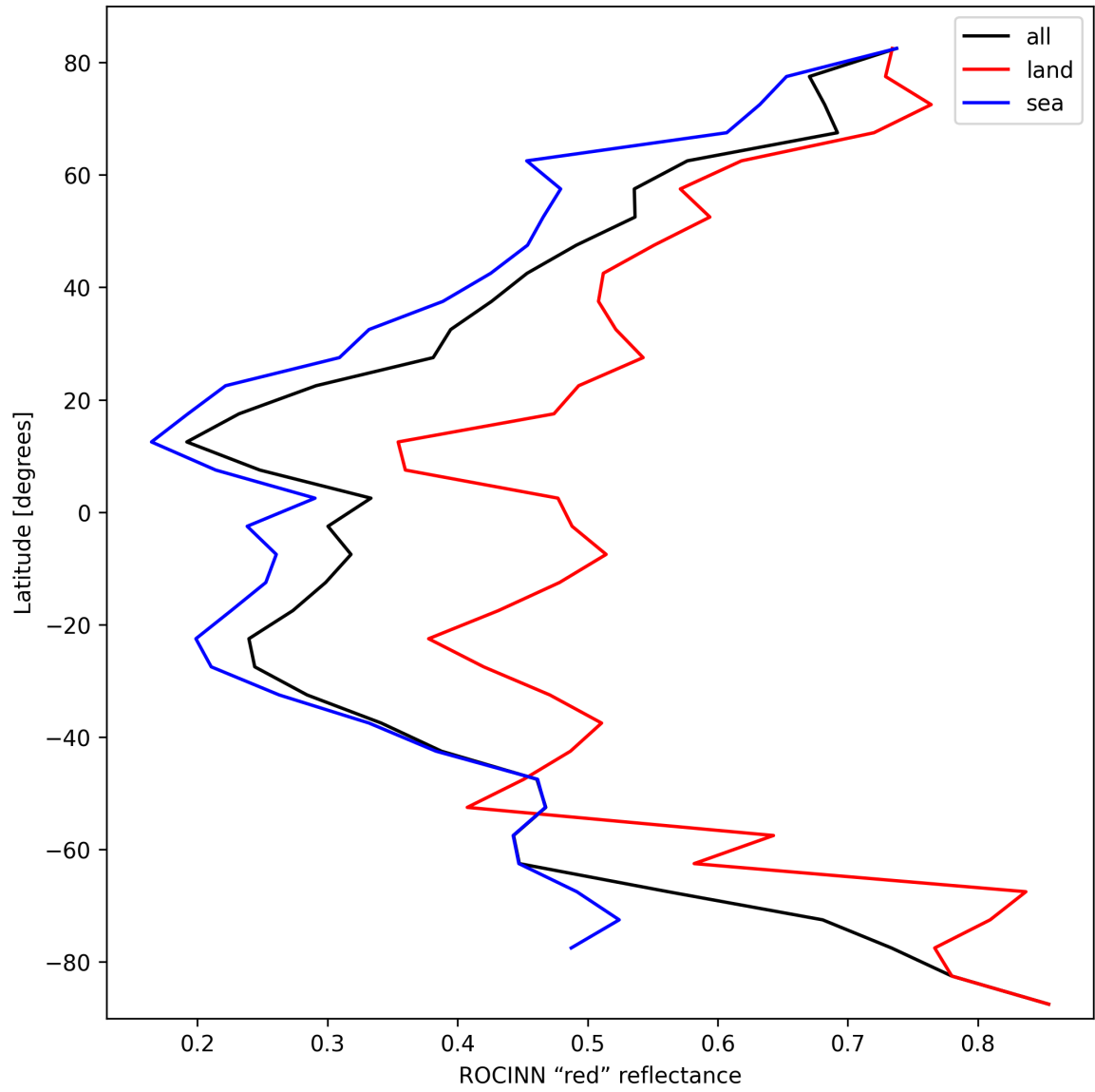
Figure 37: Zonal average of "ROCINN "red" reflectance" for 2025-03-07 to 2025-03-08.
