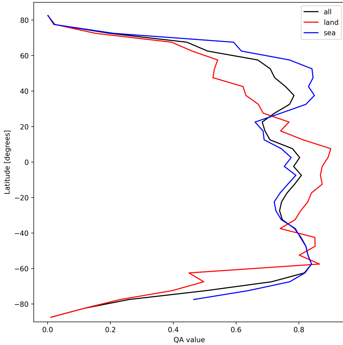
Figure 22: Zonal average of “QA value” for 2025-03-07 to 2025-03-08.
