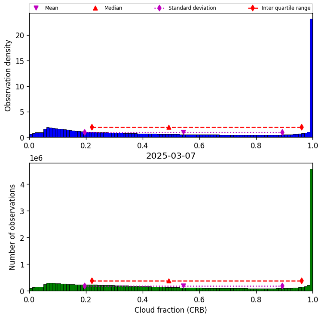
Figure 42: Histogram of “Cloud fraction (CRB)” for 2025-03-07 to 2025-03-08
