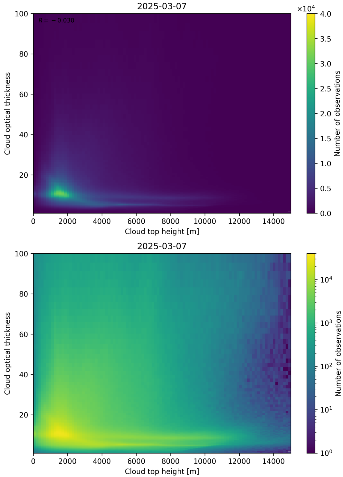
Figure 90: Scatter density plot of “Cloud top height” against “Cloud optical thickness” for 2025-03-07 to 2025-03-08.
