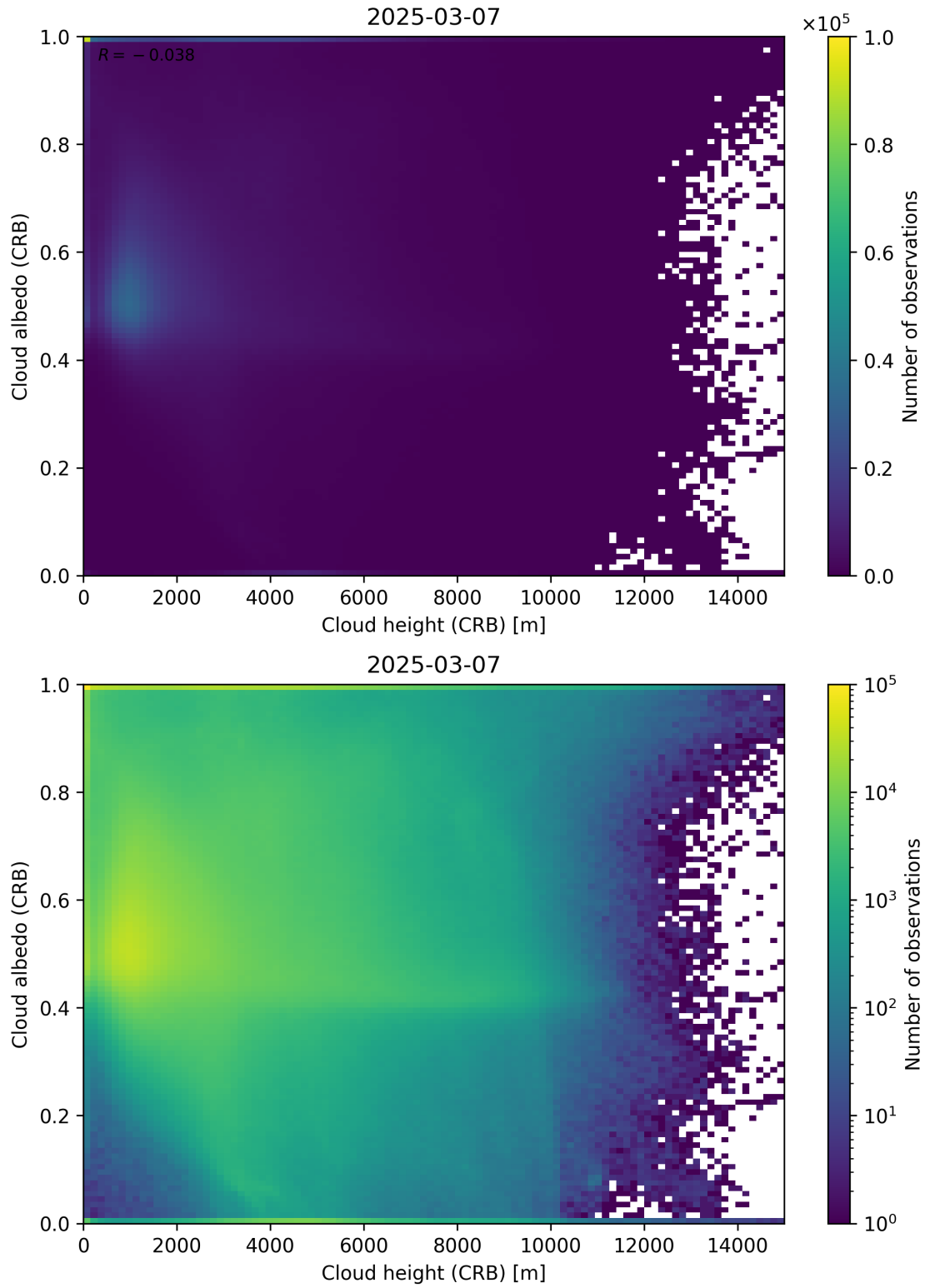
Figure 80: Scatter density plot of “Cloud height (CRB)” against “Cloud albedo (CRB)” for 2025-03-07 to 2025-03-08.
