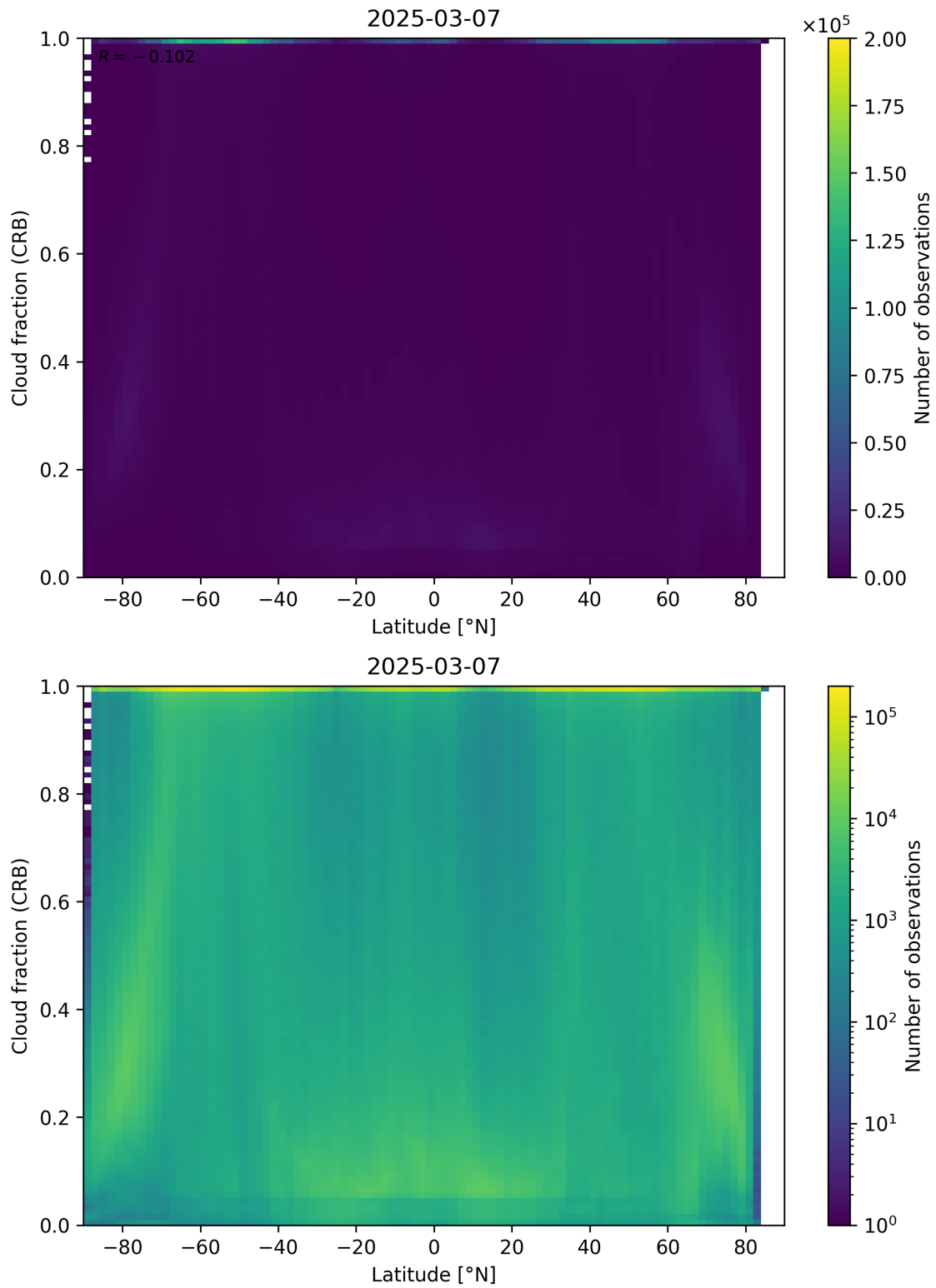
Figure 94: Scatter density plot of “Latitude” against “Cloud fraction (CRB)” for 2025-03-07 to 2025-03-08.
