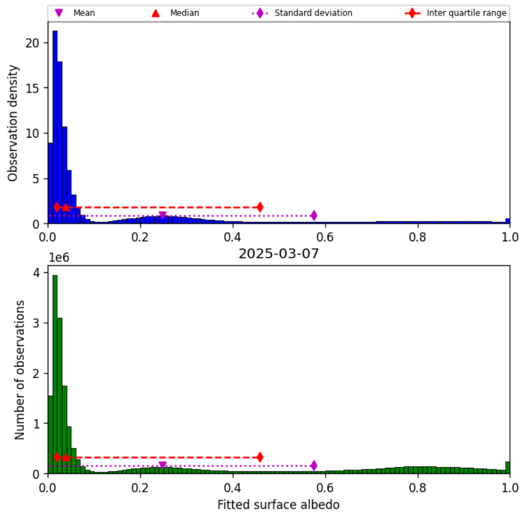
Figure 45: Histogram of “Fitted surface albedo” for 2025-03-07 to 2025-03-08
