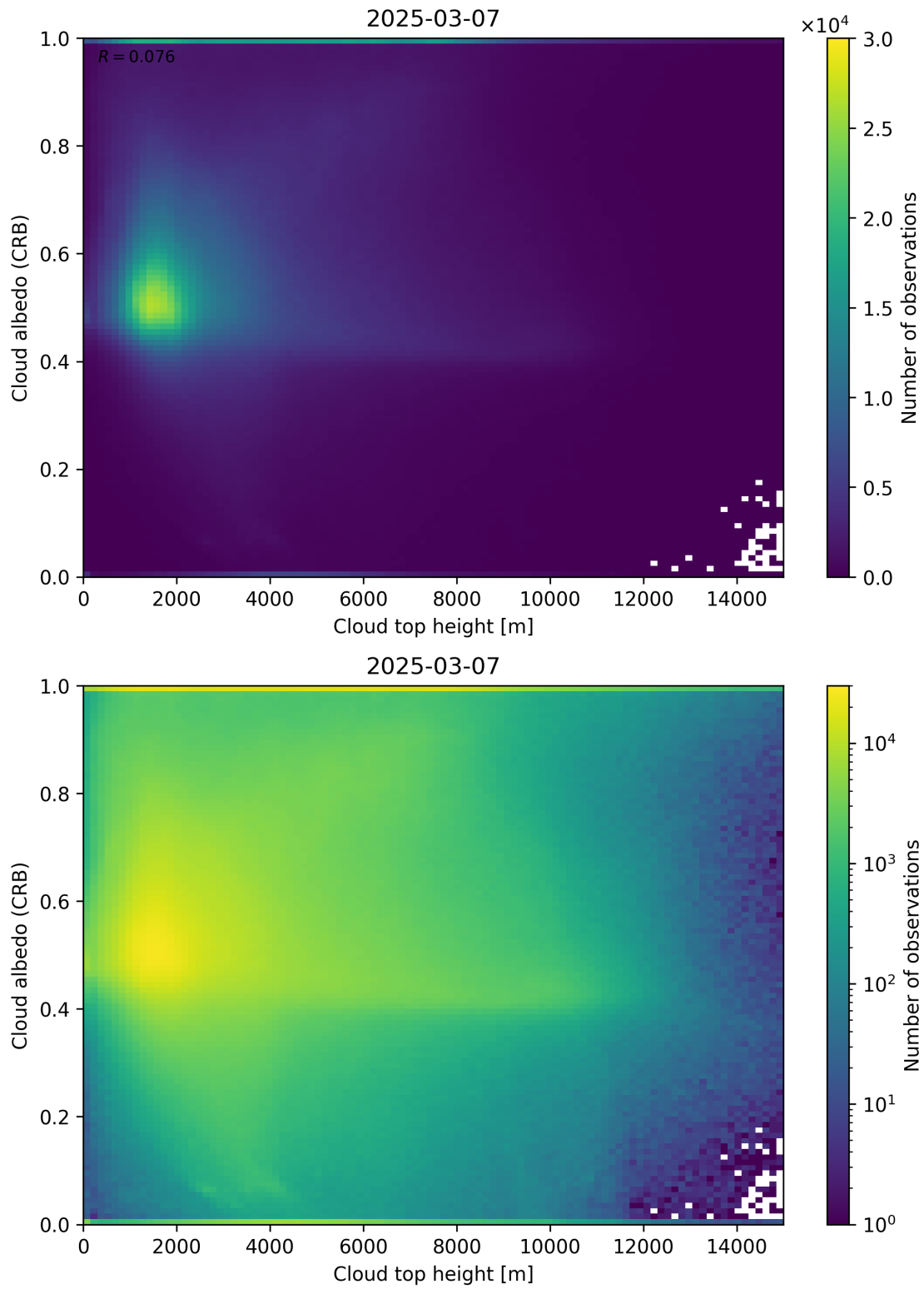
Figure 86: Scatter density plot of “Cloud top height” against “Cloud albedo (CRB)” for 2025-03-07 to 2025-03-08.
