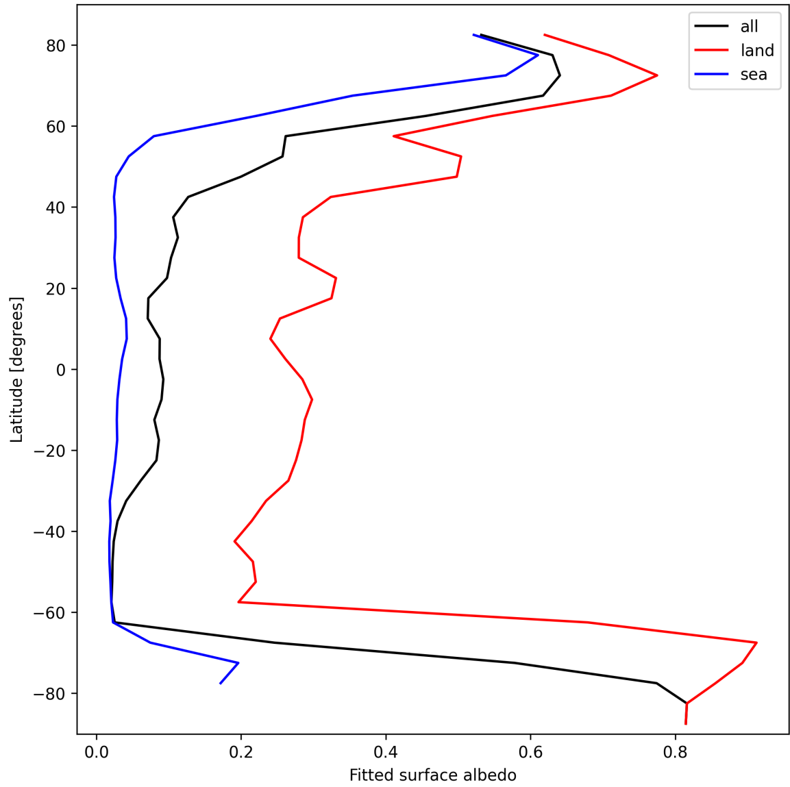
Figure 29: Zonal average of “Fitted surface albedo” for 2025-03-07 to 2025-03-08.
