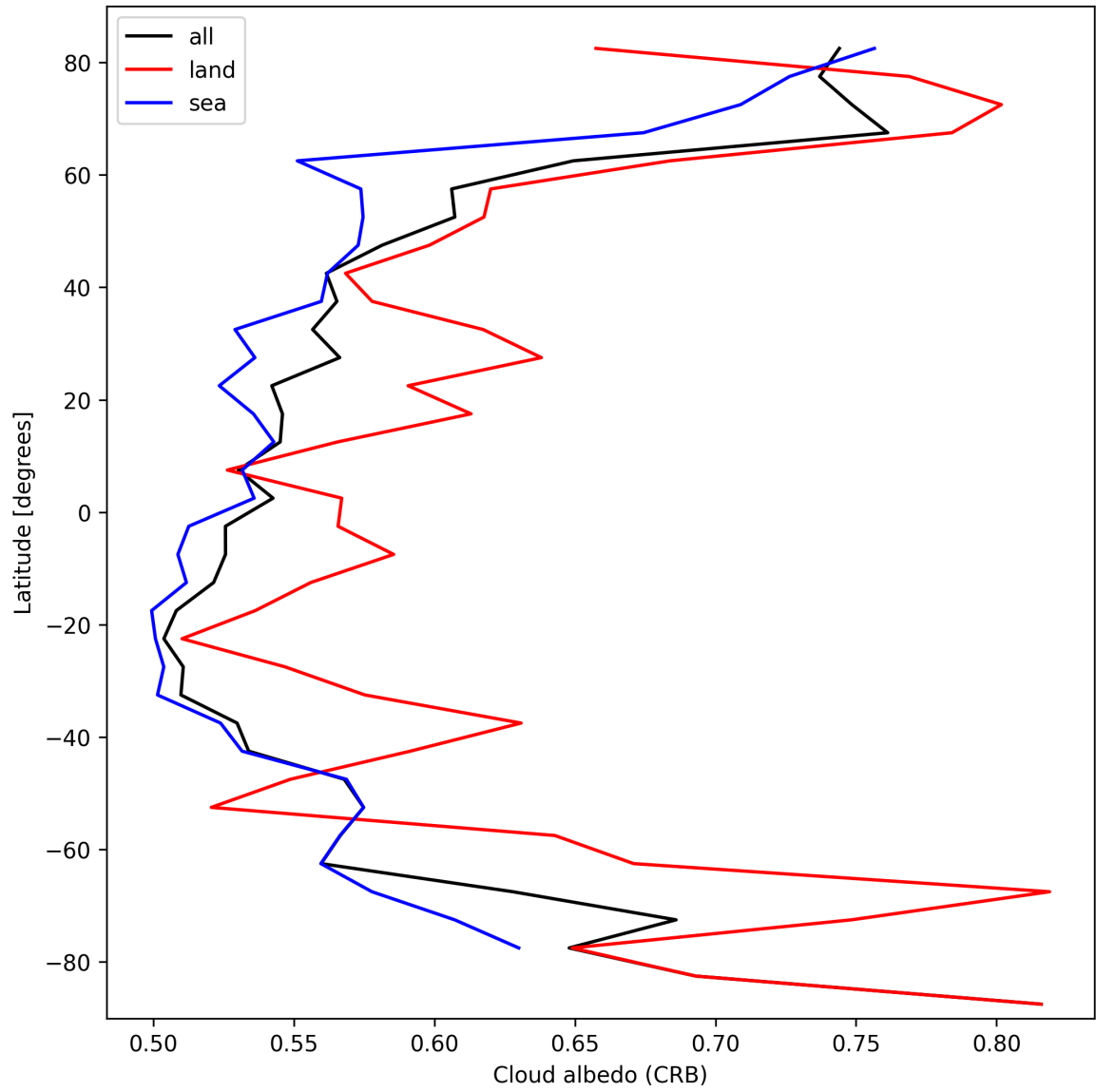
Figure 28: Zonal average of “Cloud albedo (CRB)” for 2025-03-07 to 2025-03-08.
