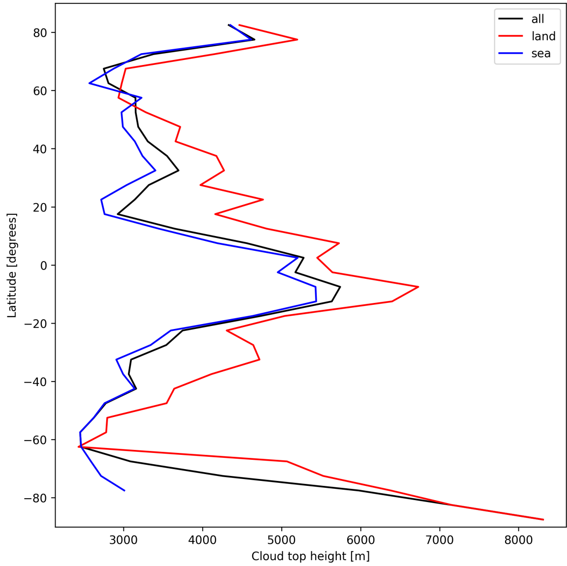
Figure 24: Zonal average of “Cloud top height” for 2025-03-07 to 2025-03-08.
