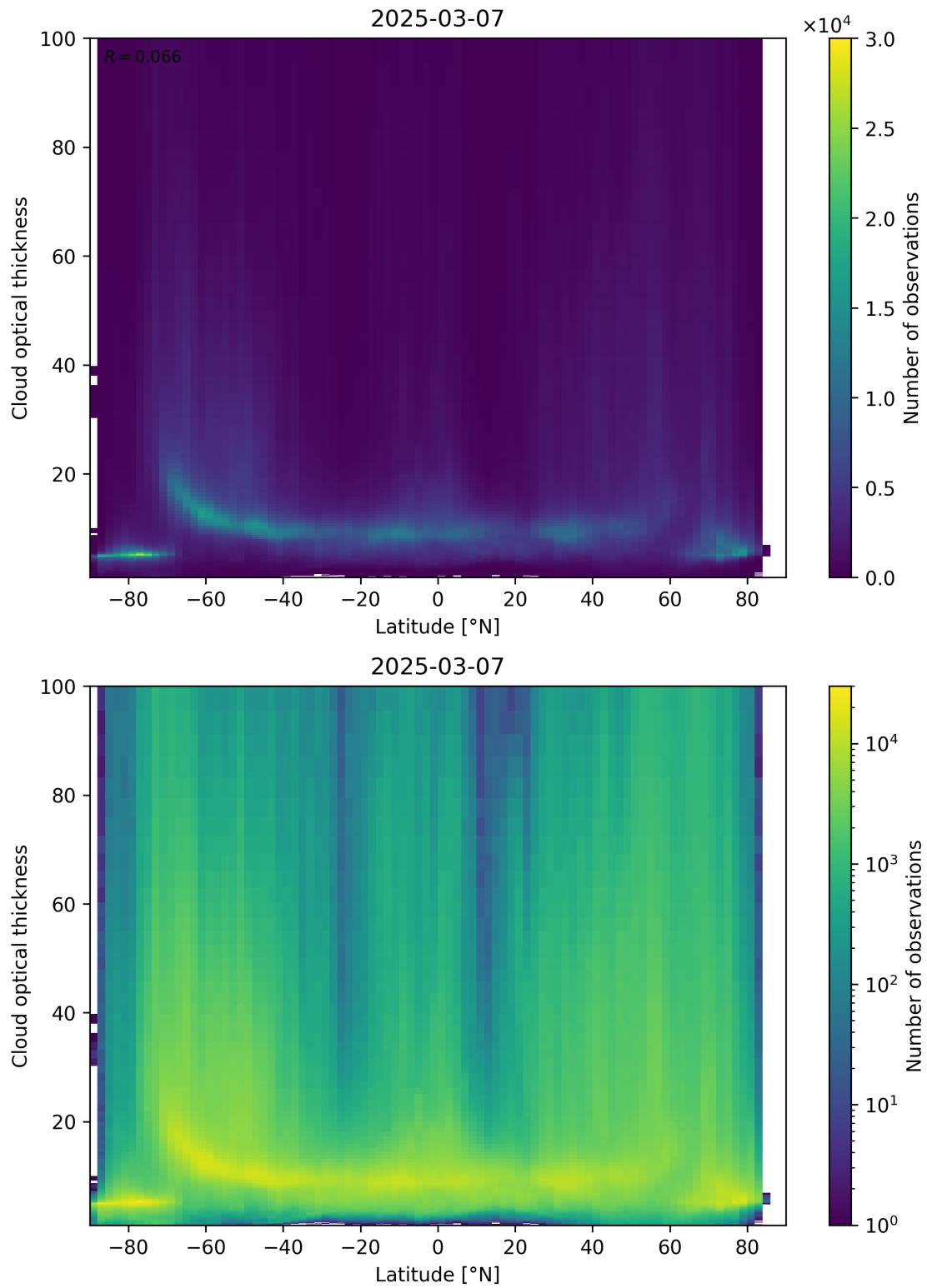
Figure 96: Scatter density plot of “Latitude” against “Cloud optical thickness” for 2025-03-07 to 2025-03-08.
