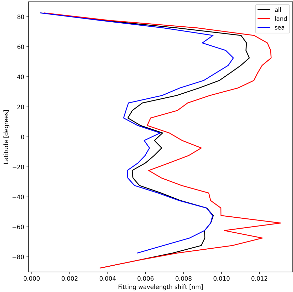
Figure 33: Zonal average of “Fitting wavelength shift” for 2025-03-07 to 2025-03-08.
