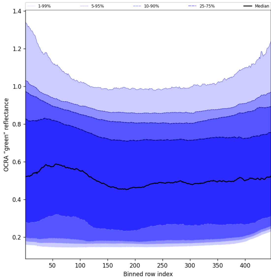
Figure 68: Along track statistics of “OCRA “green” reflectance” for 2025-03-07 to 2025-03-08
