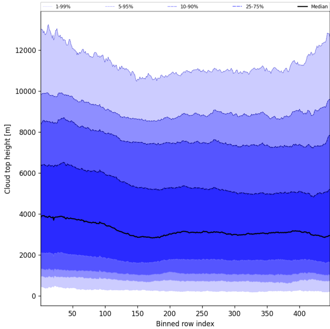
Figure 56: Along track statistics of “Cloud top height” for 2025-03-07 to 2025-03-08
