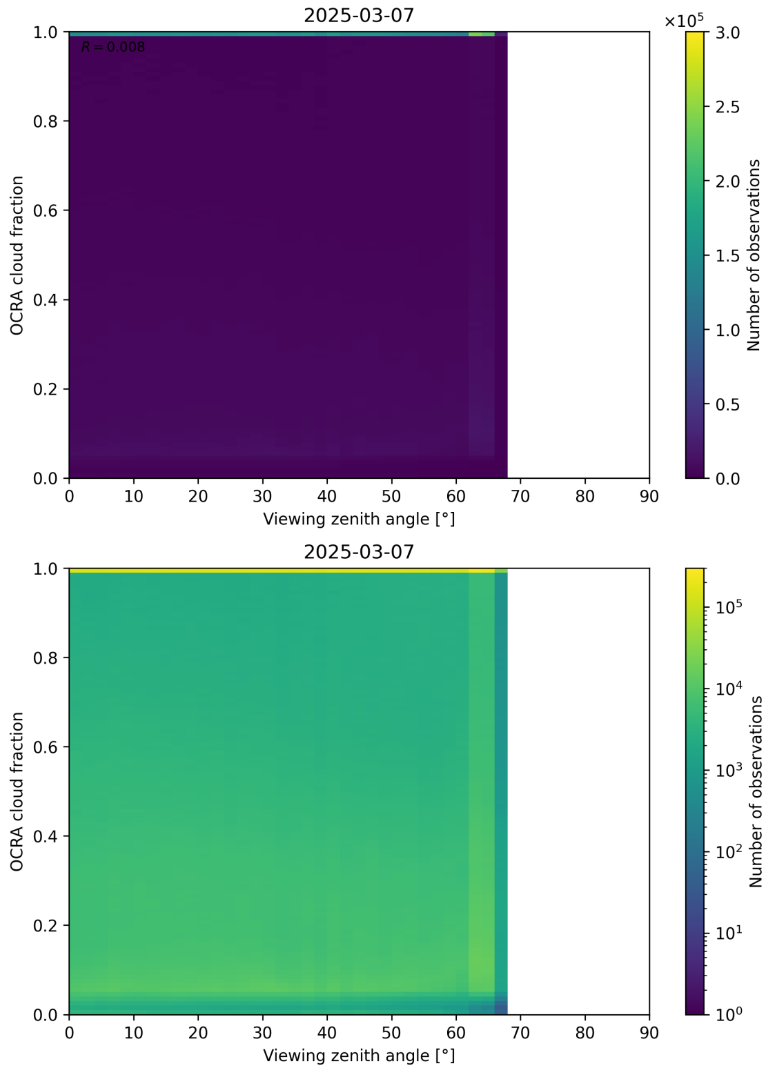
Figure 108: Scatter density plot of “Viewing zenith angle” against “OCRA cloud fraction” for 2025-03-07 to 2025-03-08.
