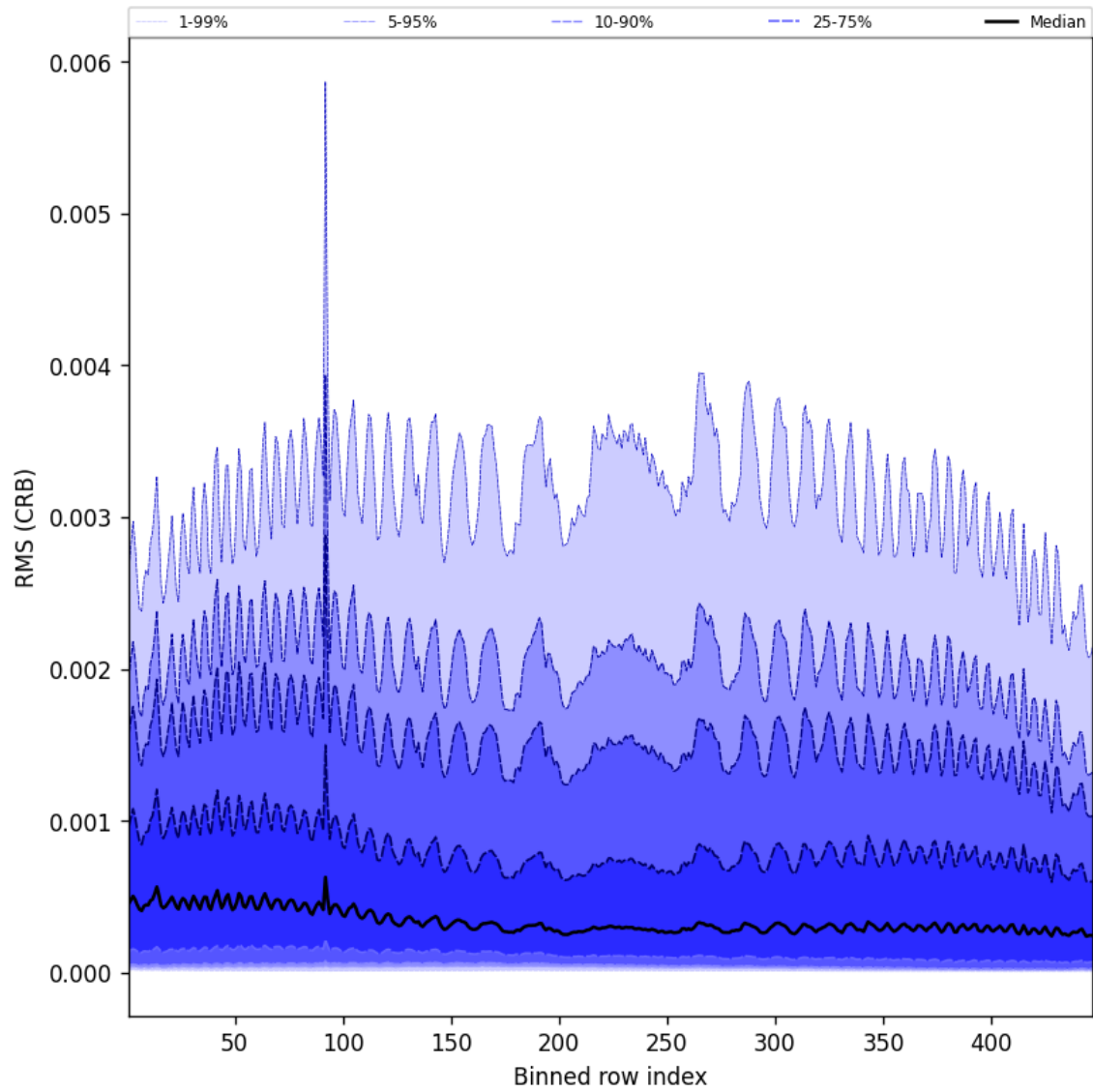
Figure 64: Along track statistics of “RMS (CRB)” for 2025-03-07 to 2025-03-08
