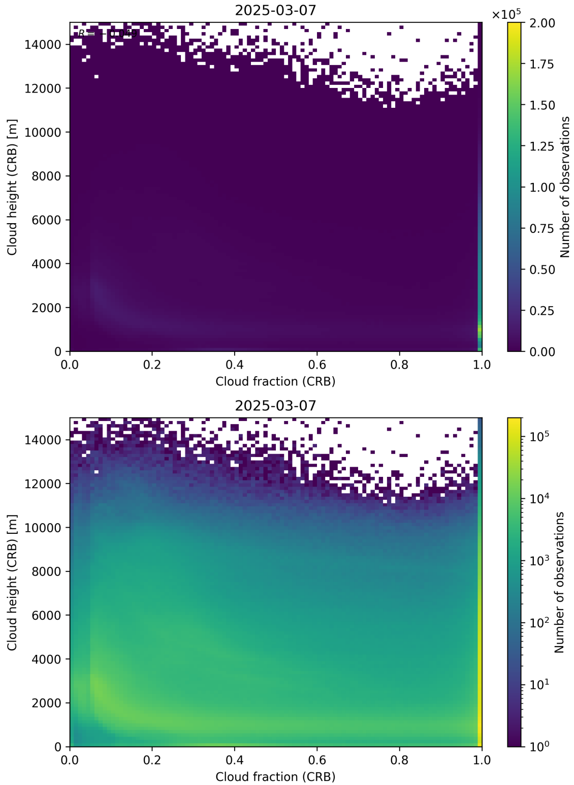
Figure 79: Scatter density plot of “Cloud fraction (CRB)” against “Cloud height (CRB)” for 2025-03-07 to 2025-03-08.
