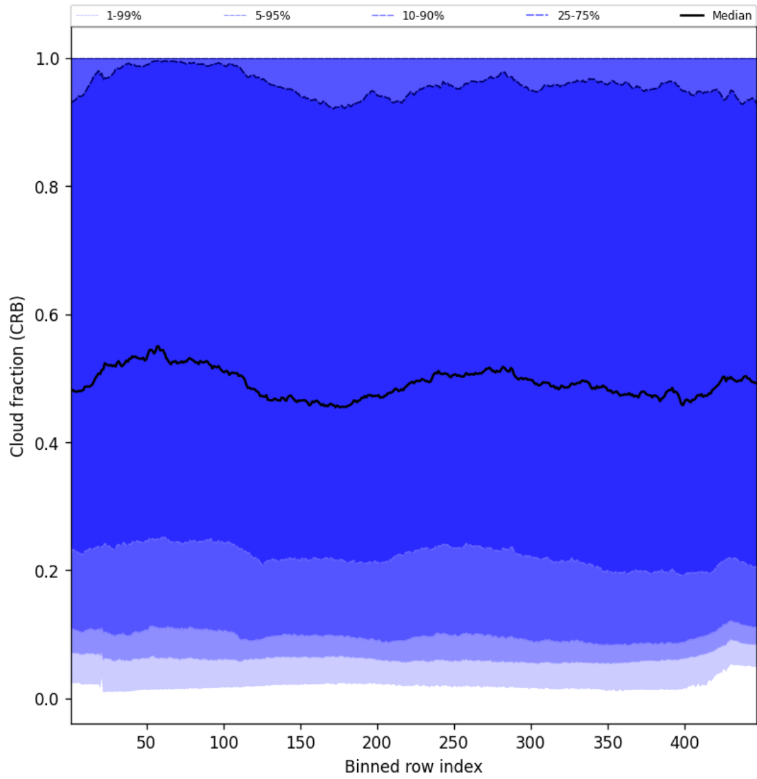
Figure 58: Along track statistics of “Cloud fraction (CRB)” for 2025-03-07 to 2025-03-08
