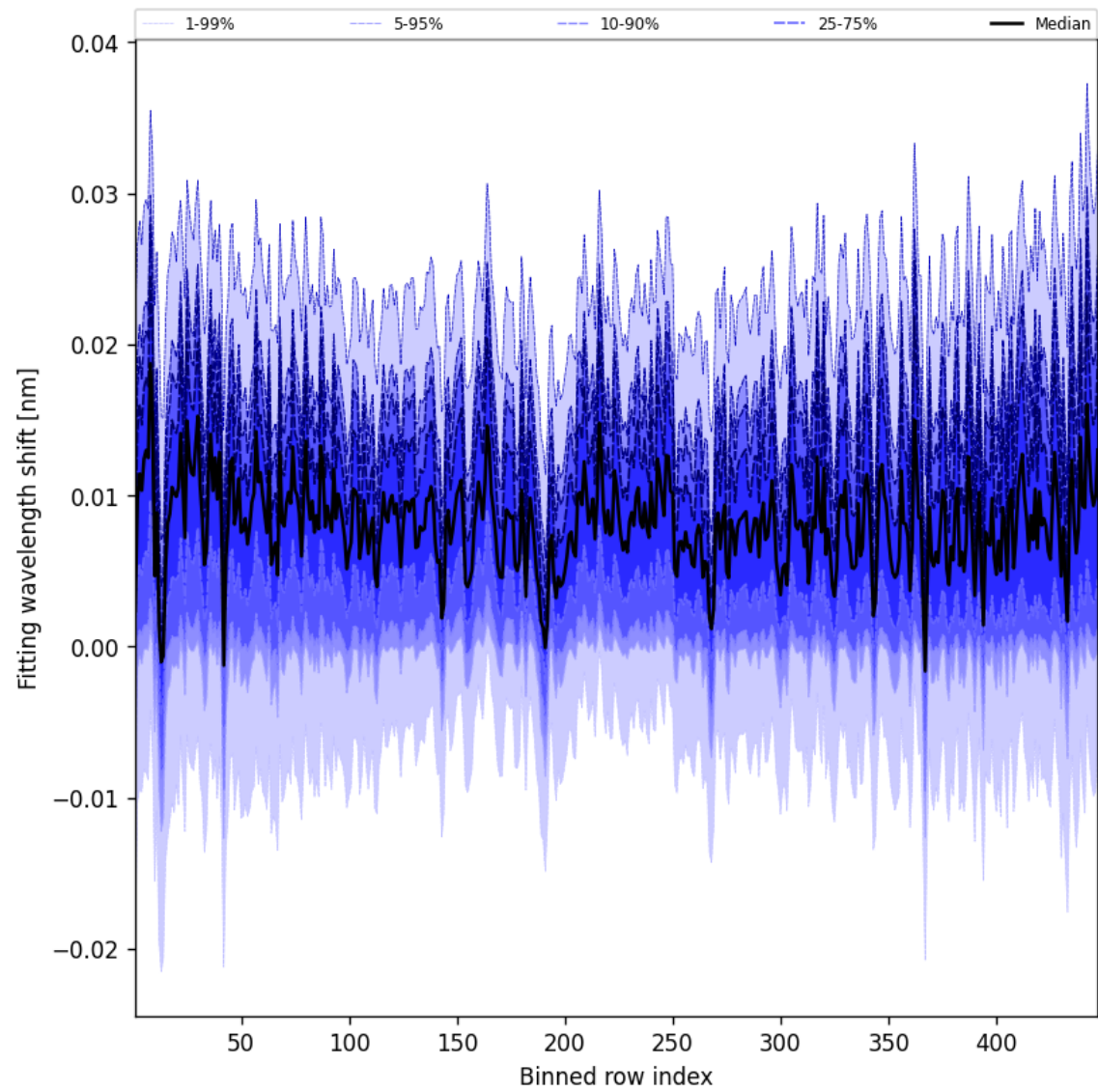
Figure 65: Along track statistics of “Fitting wavelength shift” for 2025-03-07 to 2025-03-08
