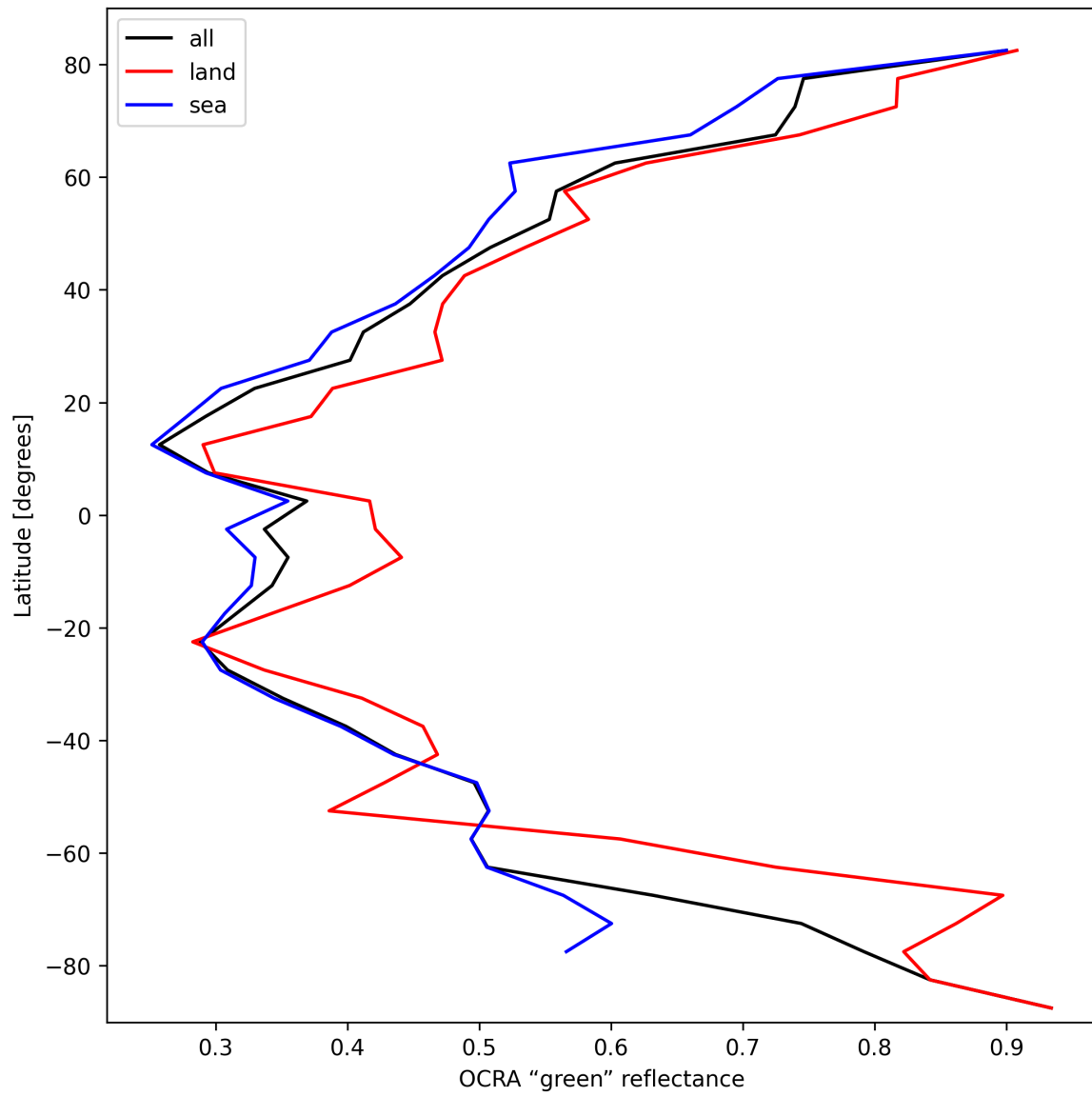
Figure 36: Zonal average of “OCRA “green” reflectance” for 2025-03-07 to 2025-03-08.
