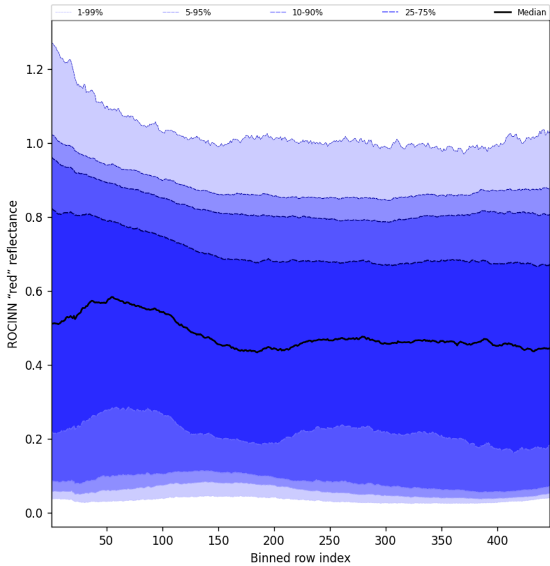
Figure 69: Along track statistics of “ROCINN “red” reflectance” for 2025-03-07 to 2025-03-08
