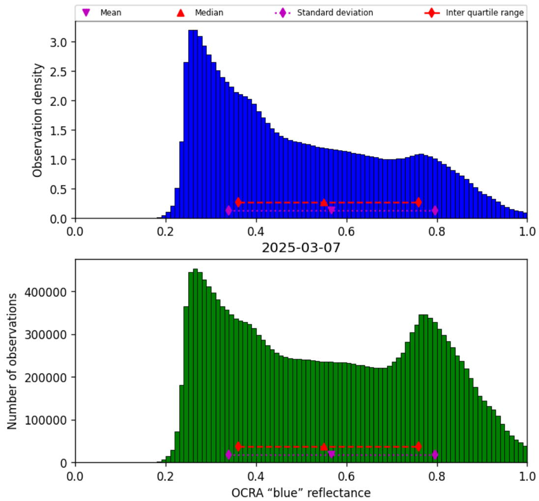
Figure 51: Histogram of “OCRA “blue” reflectance” for 2025-03-07 to 2025-03-08
