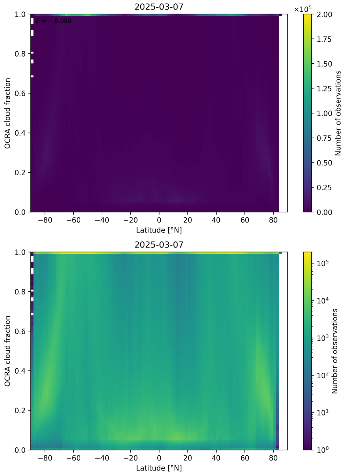
Figure 93: Scatter density plot of “Latitude” against “OCRA cloud fraction” for 2025-03-07 to 2025-03-08.
