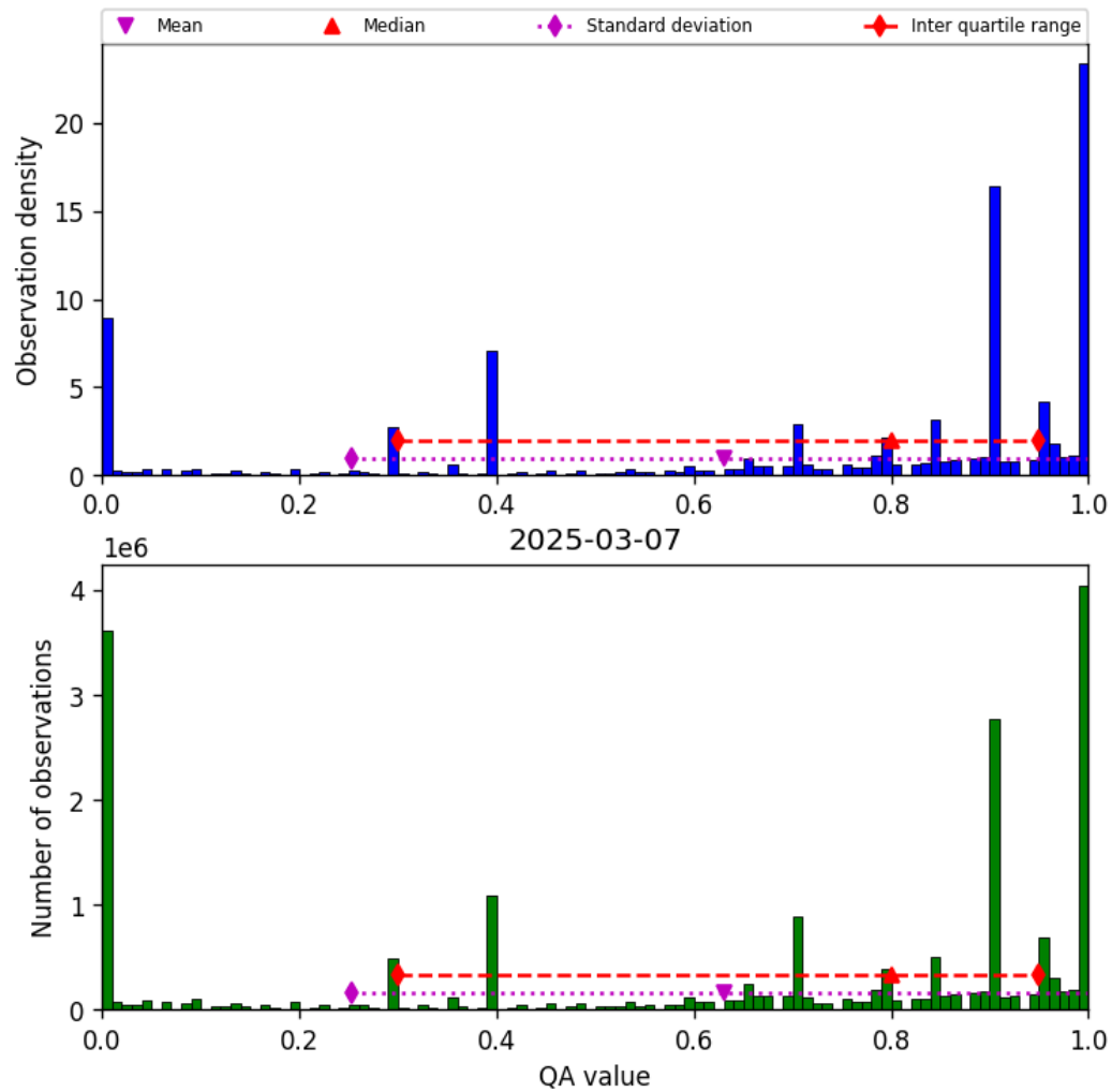
Figure 38: Histogram of “QA value” for 2025-03-07 to 2025-03-08
