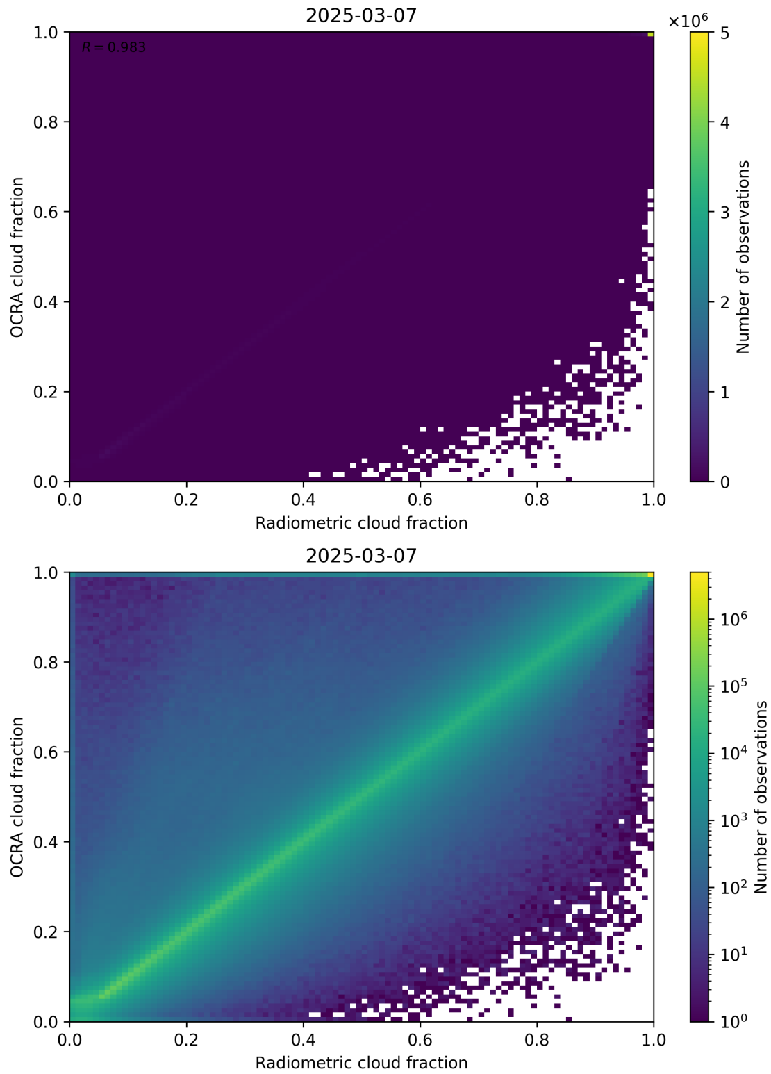
Figure 72: Scatter density plot of “Radiometric cloud fraction” against “OCRA cloud fraction” for 2025-03-07 to 2025-03-08.
