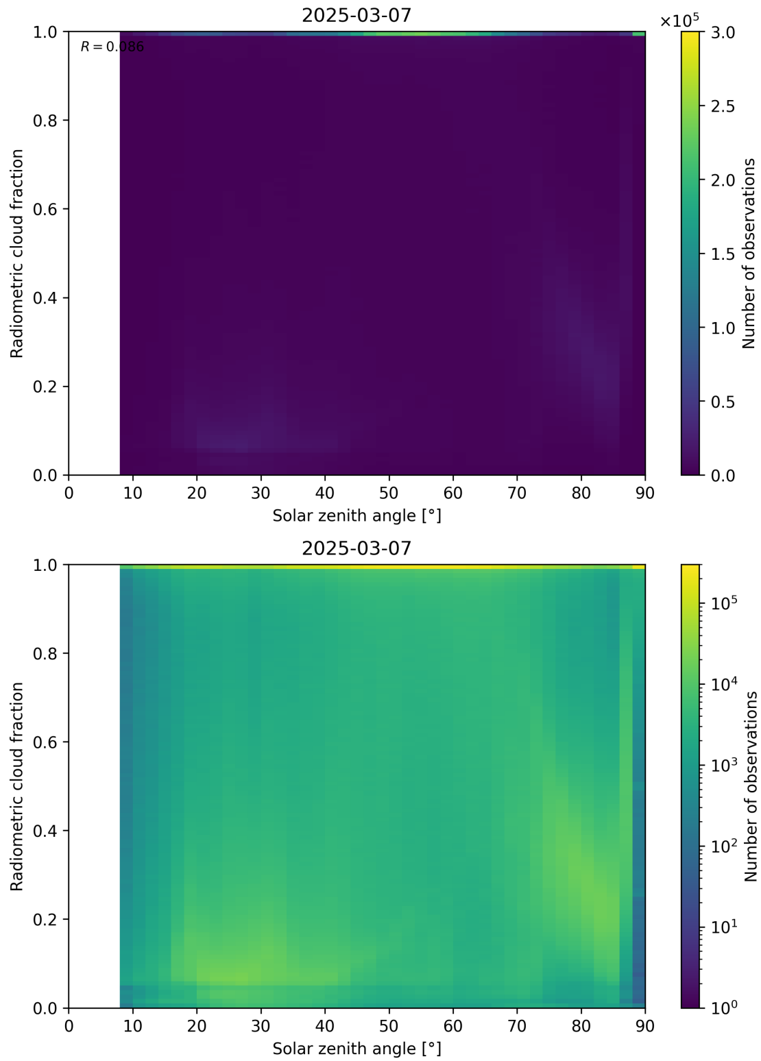
Figure 99: Scatter density plot of “Solar zenith angle” against “Radiometric cloud fraction” for 2025-03-07 to 2025-03-08.
