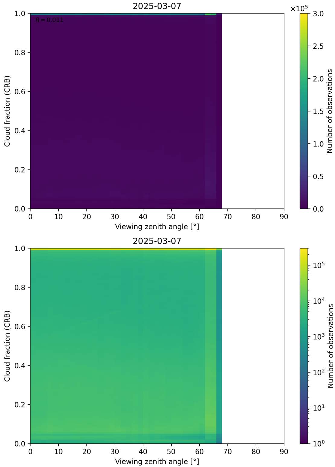
Figure 109: Scatter density plot of “Viewing zenith angle” against “Cloud fraction (CRB)” for 2025-03-07 to 2025-03-08.
