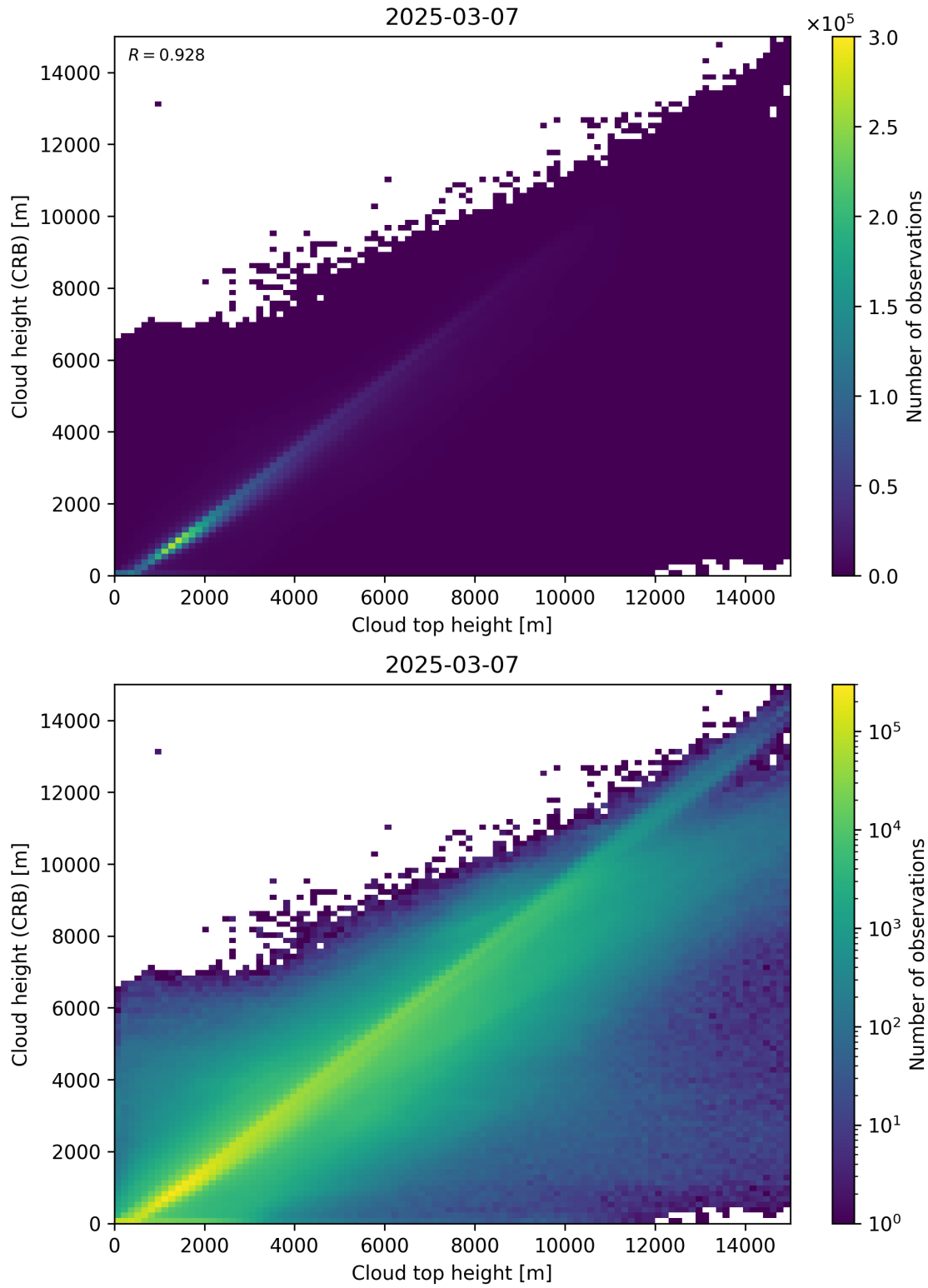
Figure 89: Scatter density plot of “Cloud top height” against “Cloud height (CRB)” for 2025-03-07 to 2025-03-08.
