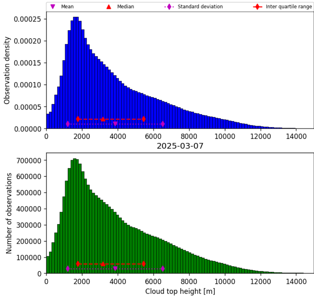
Figure 40: Histogram of “Cloud top height” for 2025-03-07 to 2025-03-08
