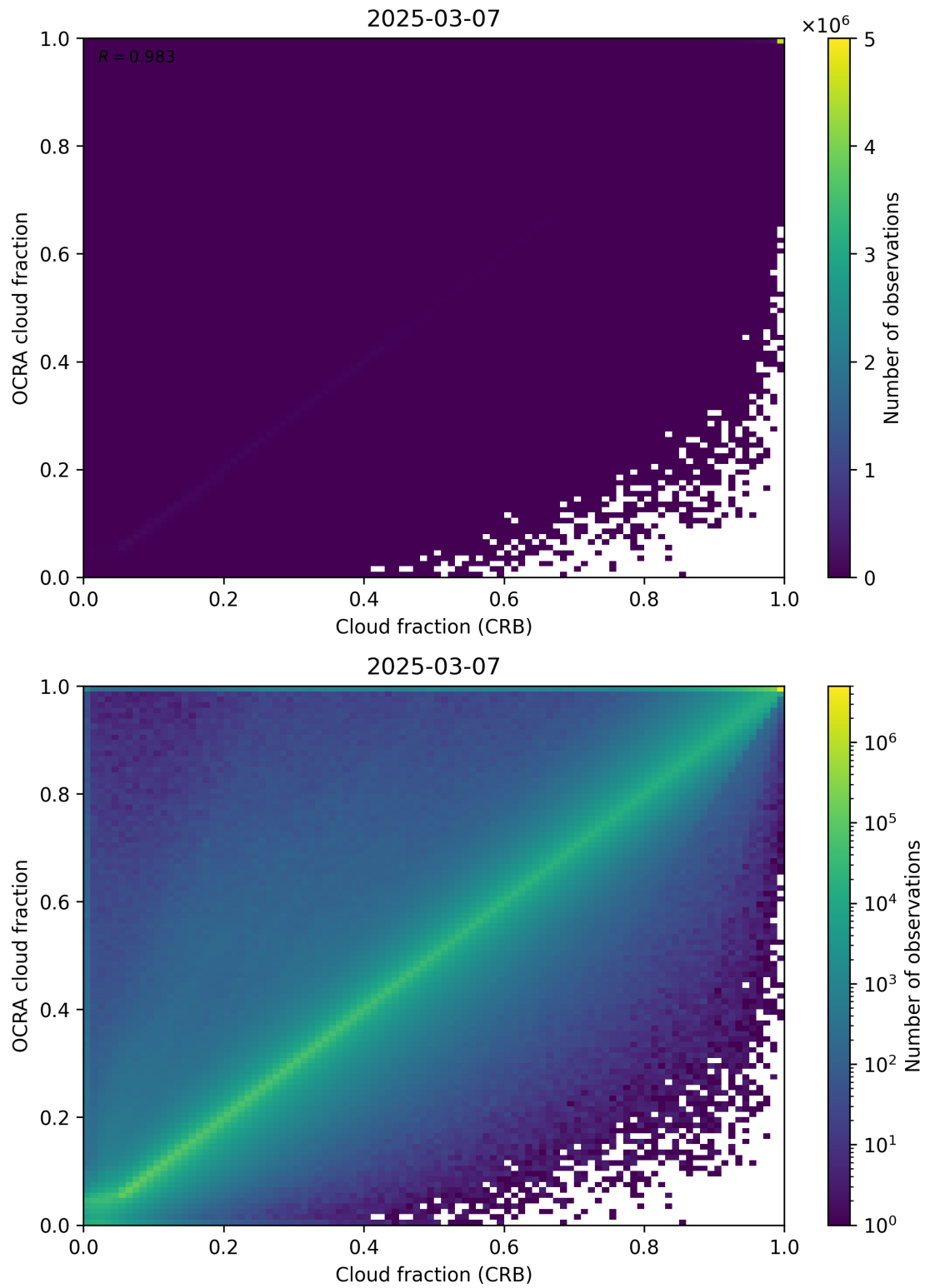
Figure 78: Scatter density plot of “Cloud fraction (CRB)” against “OCRA cloud fraction” for 2025-03-07 to 2025-03-08.
