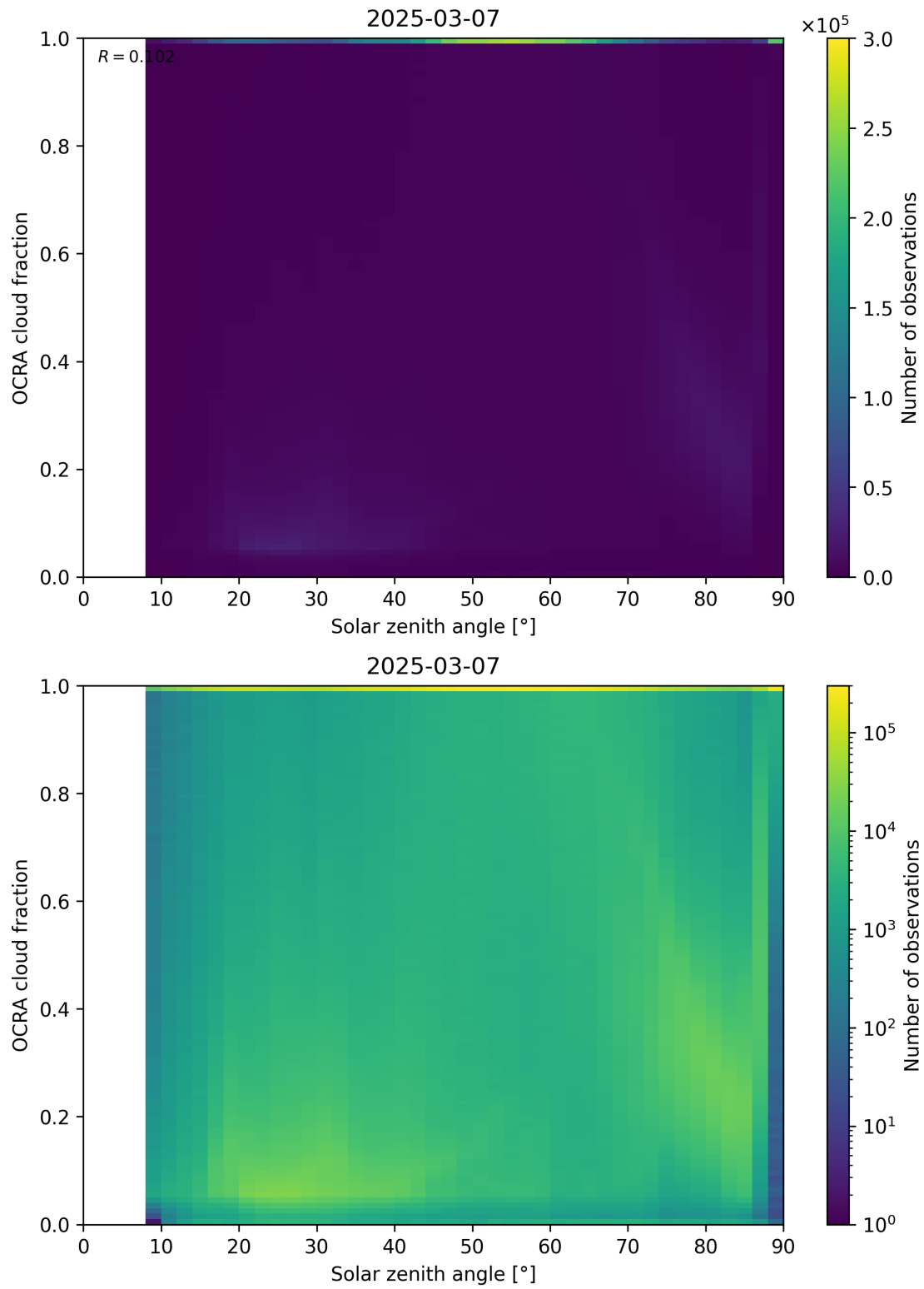
Figure 100: Scatter density plot of “Solar zenith angle” against “OCRA cloud fraction” for 2025-03-07 to 2025-03-08.
