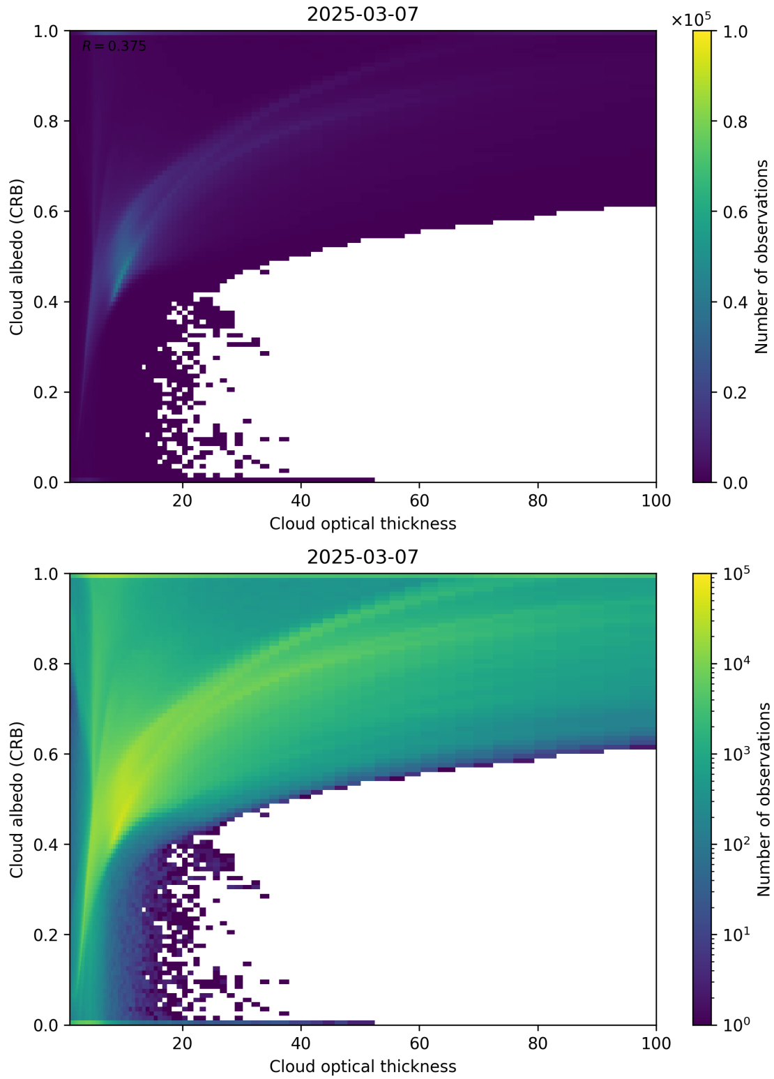
Figure 82: Scatter density plot of “Cloud optical thickness” against “Cloud albedo (CRB)” for 2025-03-07 to 2025-03-08.
