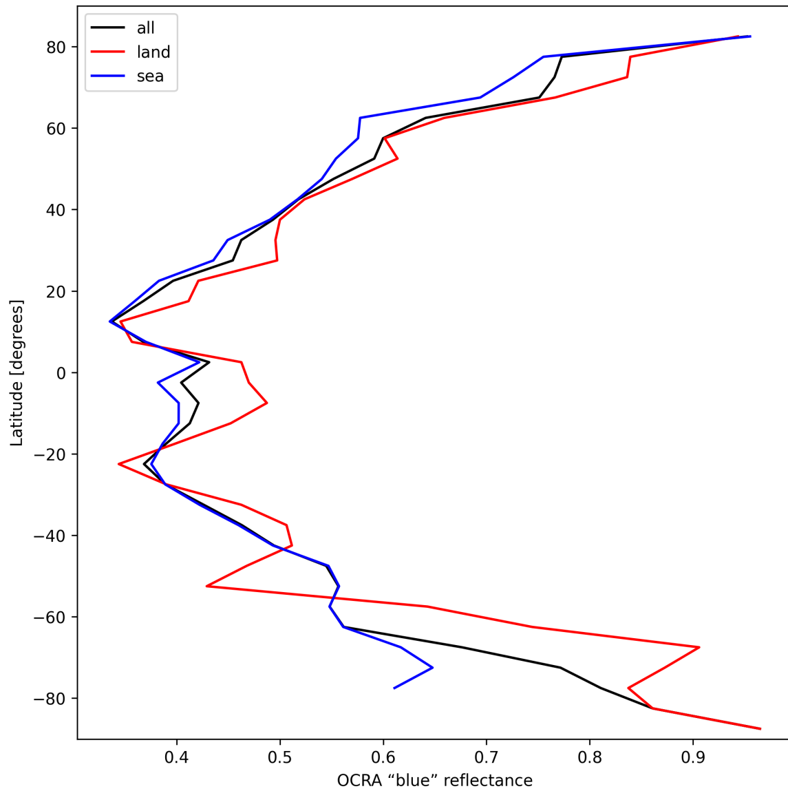
Figure 35: Zonal average of “OCRA “blue” reflectance” for 2025-03-07 to 2025-03-08.
