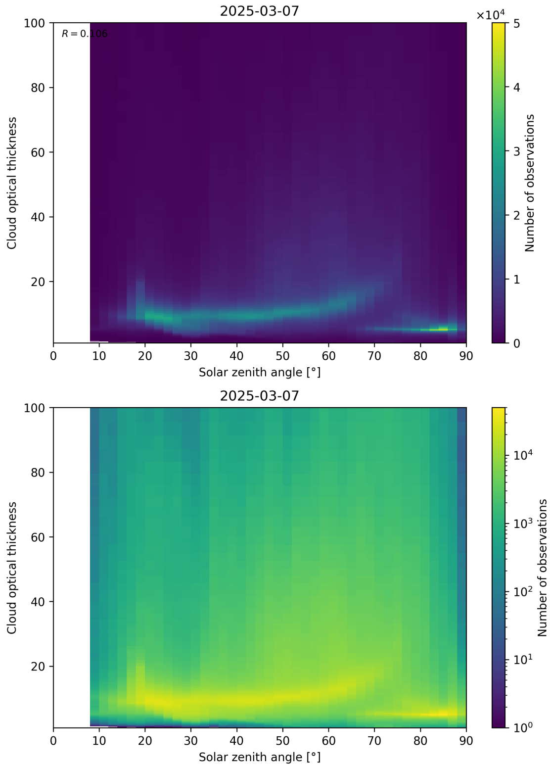
Figure 103: Scatter density plot of “Solar zenith angle” against “Cloud optical thickness” for 2025-03-07 to 2025-03-08.
