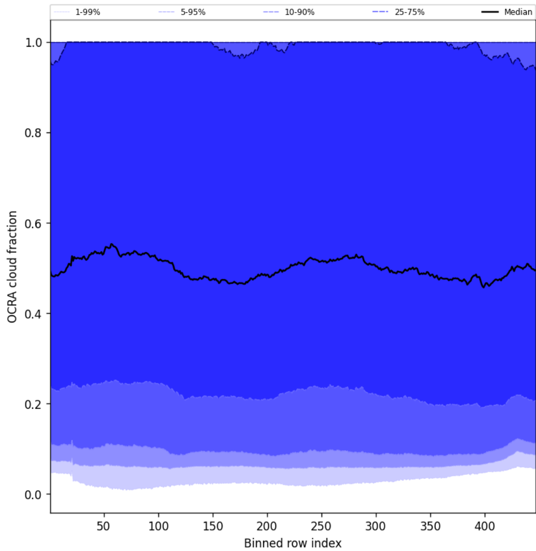
Figure 66: Along track statistics of “OCRA cloud fraction” for 2025-03-07 to 2025-03-08
