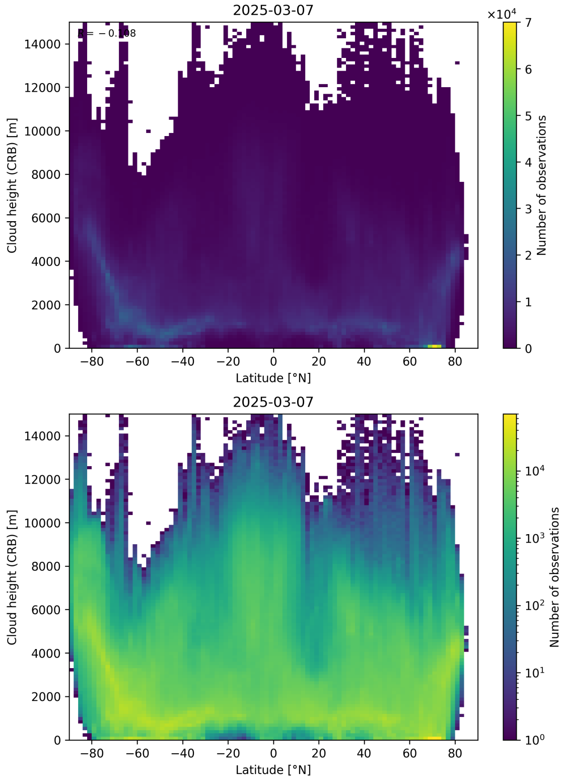
Figure 95: Scatter density plot of “Latitude” against “Cloud height (CRB)” for 2025-03-07 to 2025-03-08.
