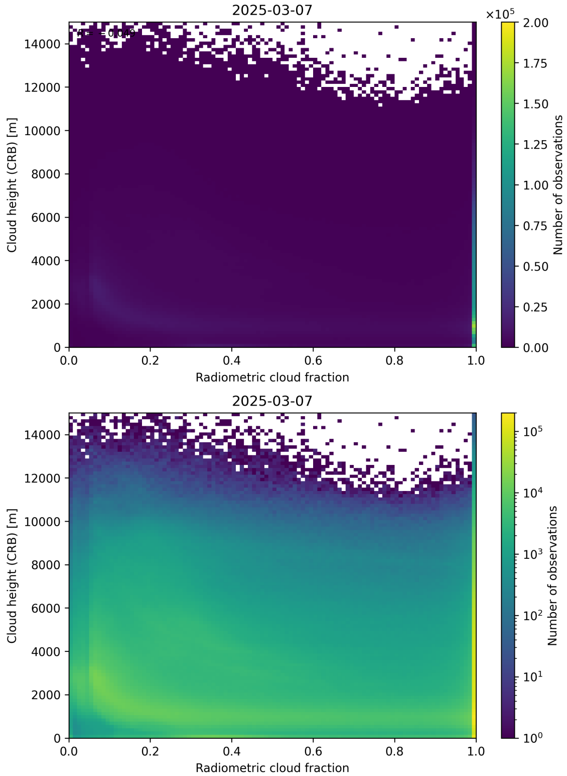
Figure 74: Scatter density plot of “Radiometric cloud fraction” against “Cloud height (CRB)” for 2025-03-07 to 2025-03-08.
