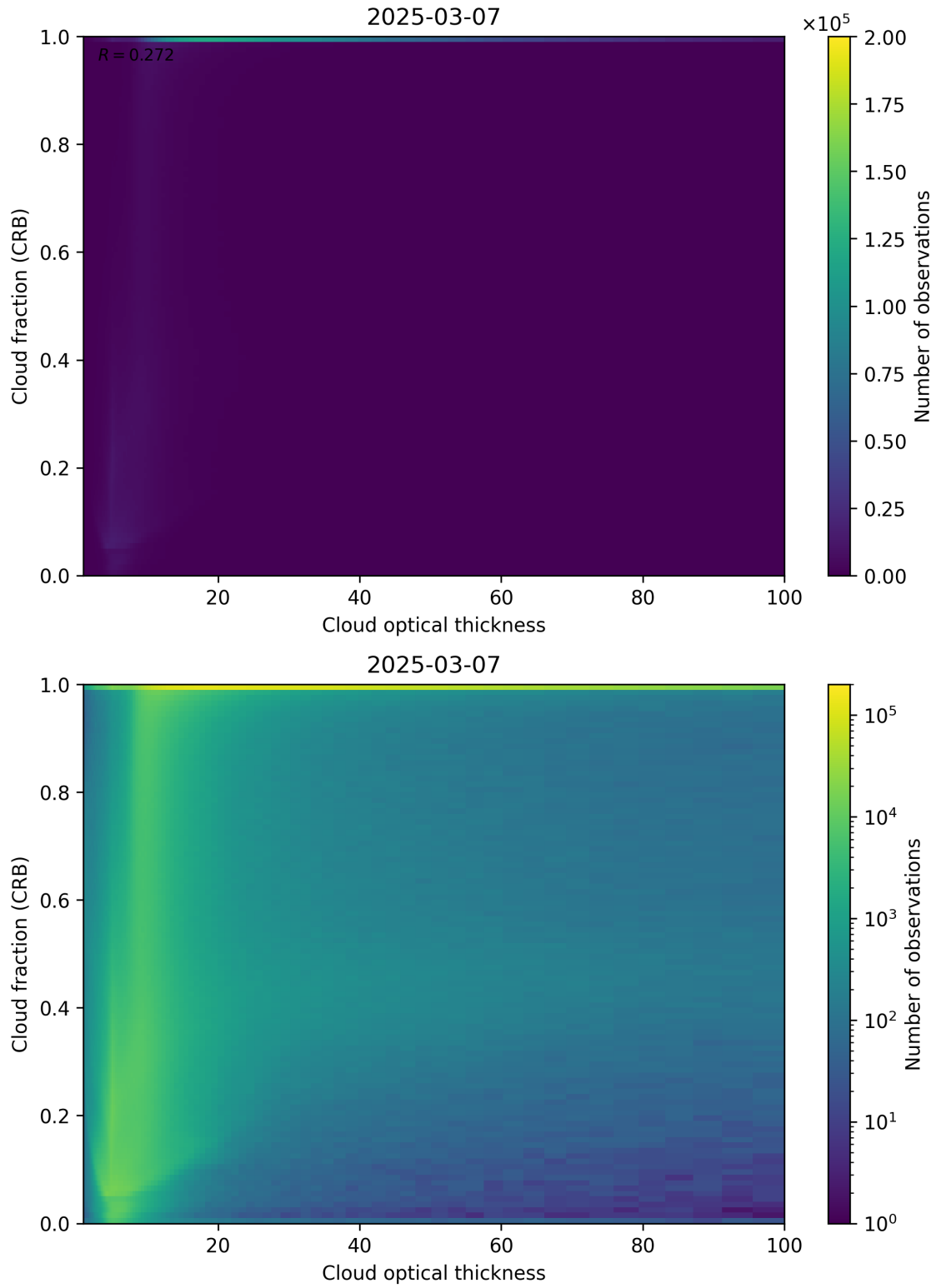
Figure 84: Scatter density plot of “Cloud optical thickness” against “Cloud fraction (CRB)” for 2025-03-07 to 2025-03-08.
