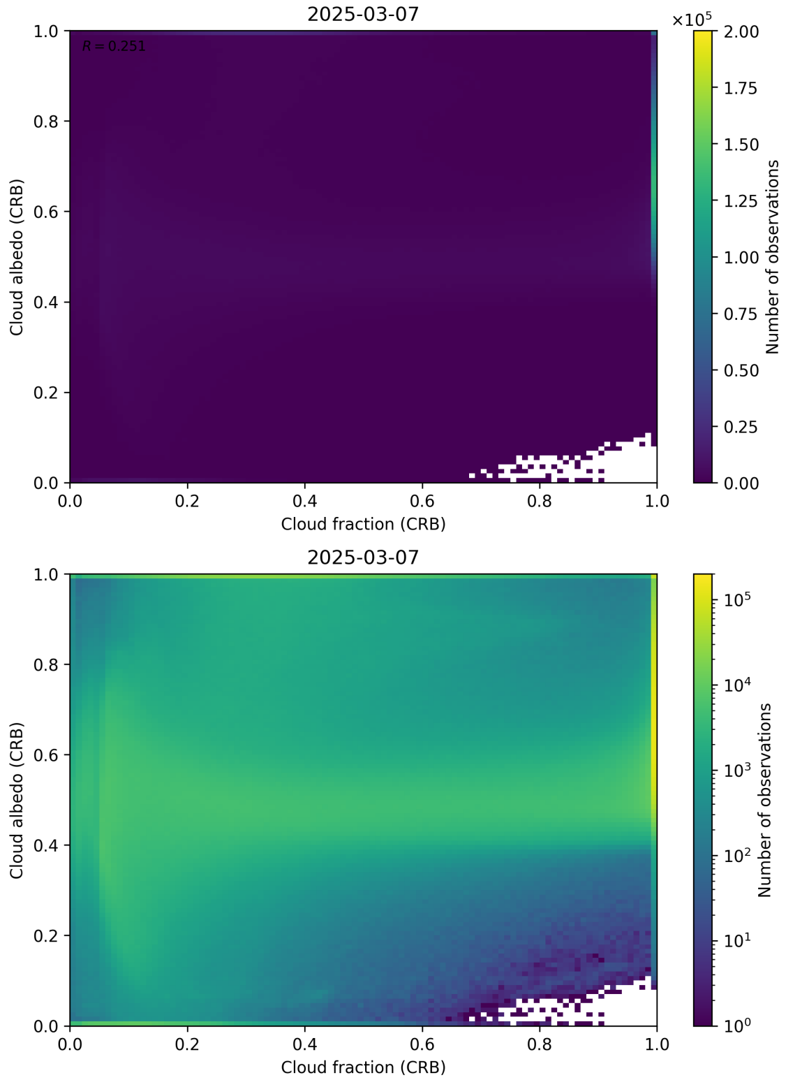
Figure 77: Scatter density plot of “Cloud fraction (CRB)” against “Cloud albedo (CRB)” for 2025-03-07 to 2025-03-08.
