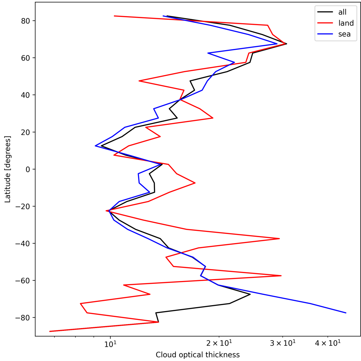
Figure 25: Zonal average of “Cloud optical thickness” for 2025-03-07 to 2025-03-08.
