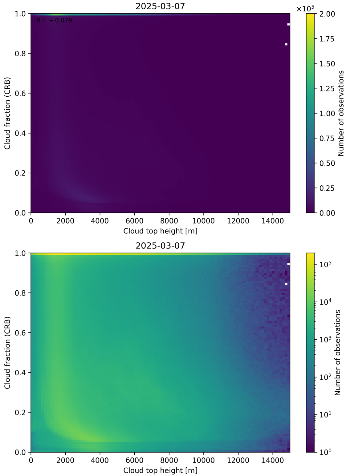
Figure 88: Scatter density plot of “Cloud top height” against “Cloud fraction (CRB)” for 2025-03-07 to 2025-03-08.
