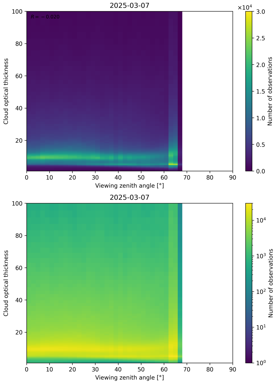
Figure 111: Scatter density plot of “Viewing zenith angle” against “Cloud optical thickness” for 2025-03-07 to 2025-03-08.
