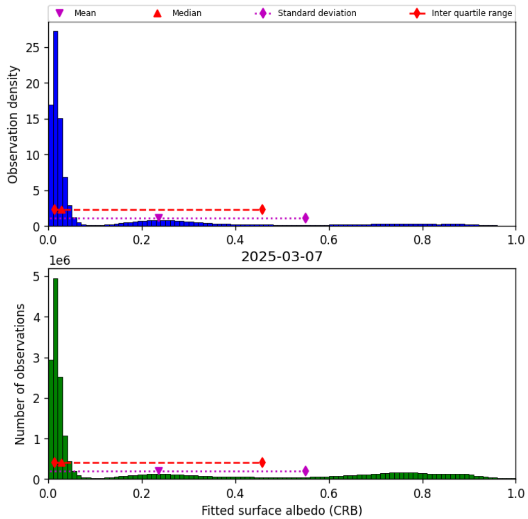
Figure 46: Histogram of “Fitted surface albedo (CRB)” for 2025-03-07 to 2025-03-08
