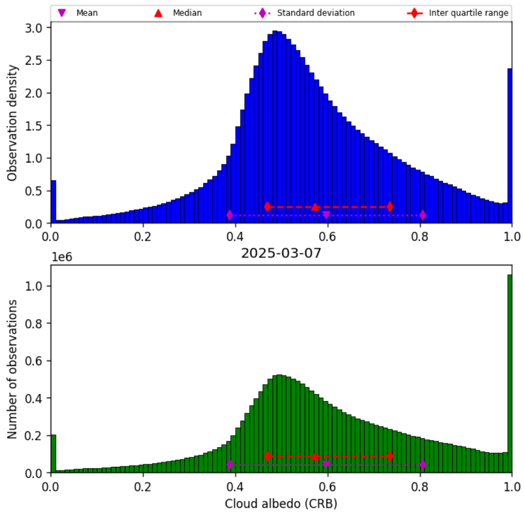
Figure 44: Histogram of “Cloud albedo (CRB)” for 2025-03-07 to 2025-03-08
