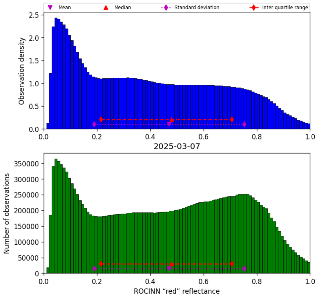
Figure 53: Histogram of “ROCINN “red” reflectance” for 2025-03-07 to 2025-03-08
