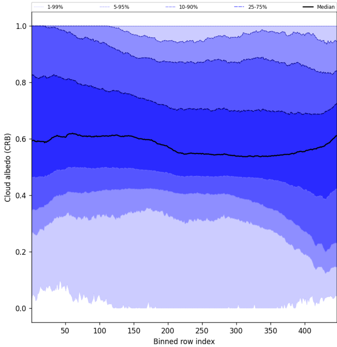
Figure 60: Along track statistics of “Cloud albedo (CRB)” for 2025-03-07 to 2025-03-08
