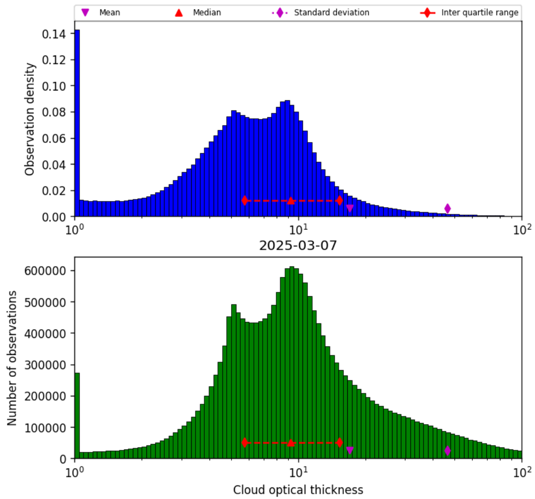
Figure 41: Histogram of “Cloud optical thickness” for 2025-03-07 to 2025-03-08
