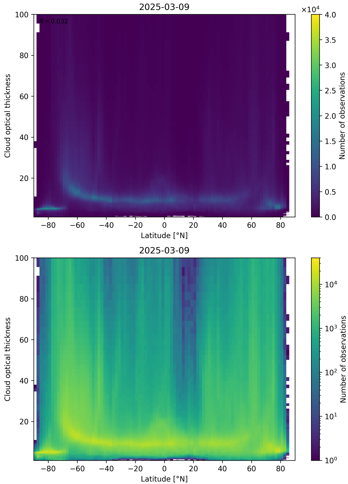
Figure 96: Scatter density plot of “Latitude” against “Cloud optical thickness” for 2025-03-08 to 2025-03-10.
