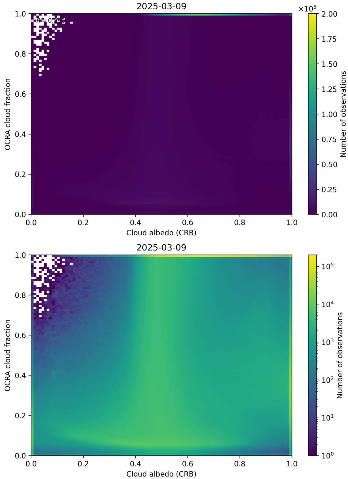
Figure 70: Scatter density plot of “Cloud albedo (CRB)” against “OCRA cloud fraction” for 2025-03-08 to 2025-03-10.
