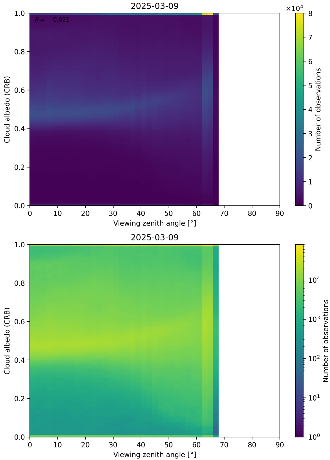
Figure 106: Scatter density plot of “Viewing zenith angle” against “Cloud albedo (CRB)” for 2025-03-08 to 2025-03-10.
