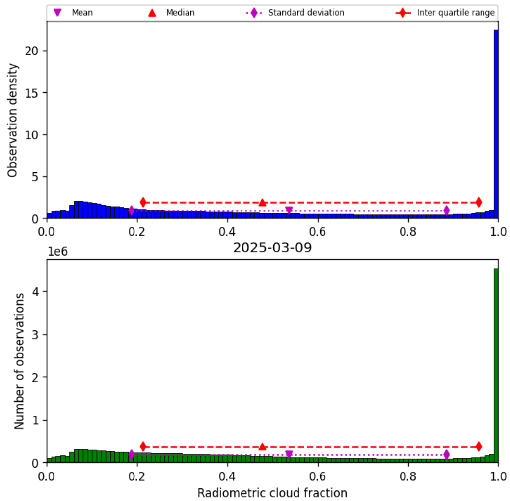
Figure 39: Histogram of “Radiometric cloud fraction” for 2025-03-08 to 2025-03-10
