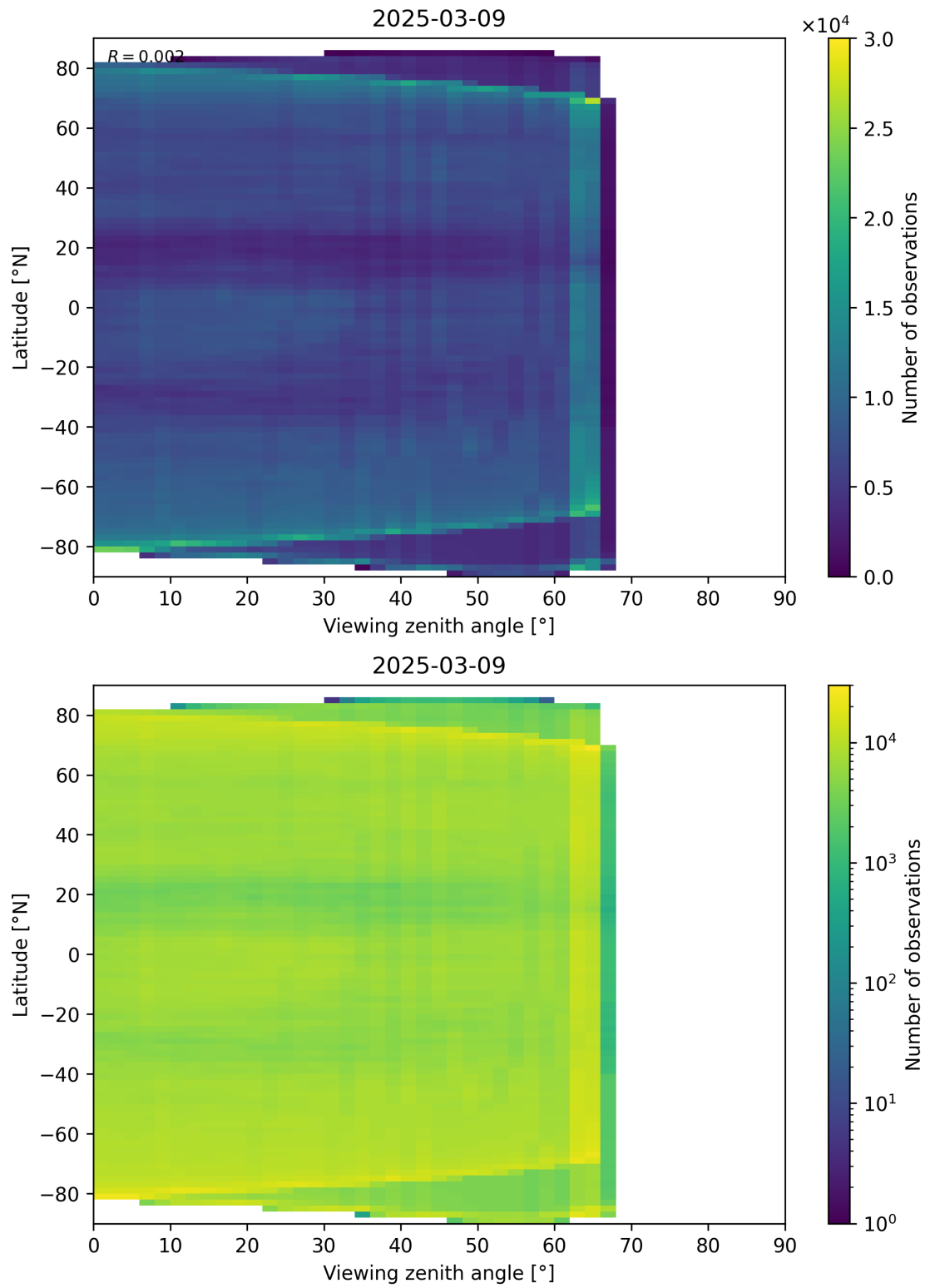
Figure 113: Scatter density plot of “Viewing zenith angle” against “Latitude” for 2025-03-08 to 2025-03-10.
