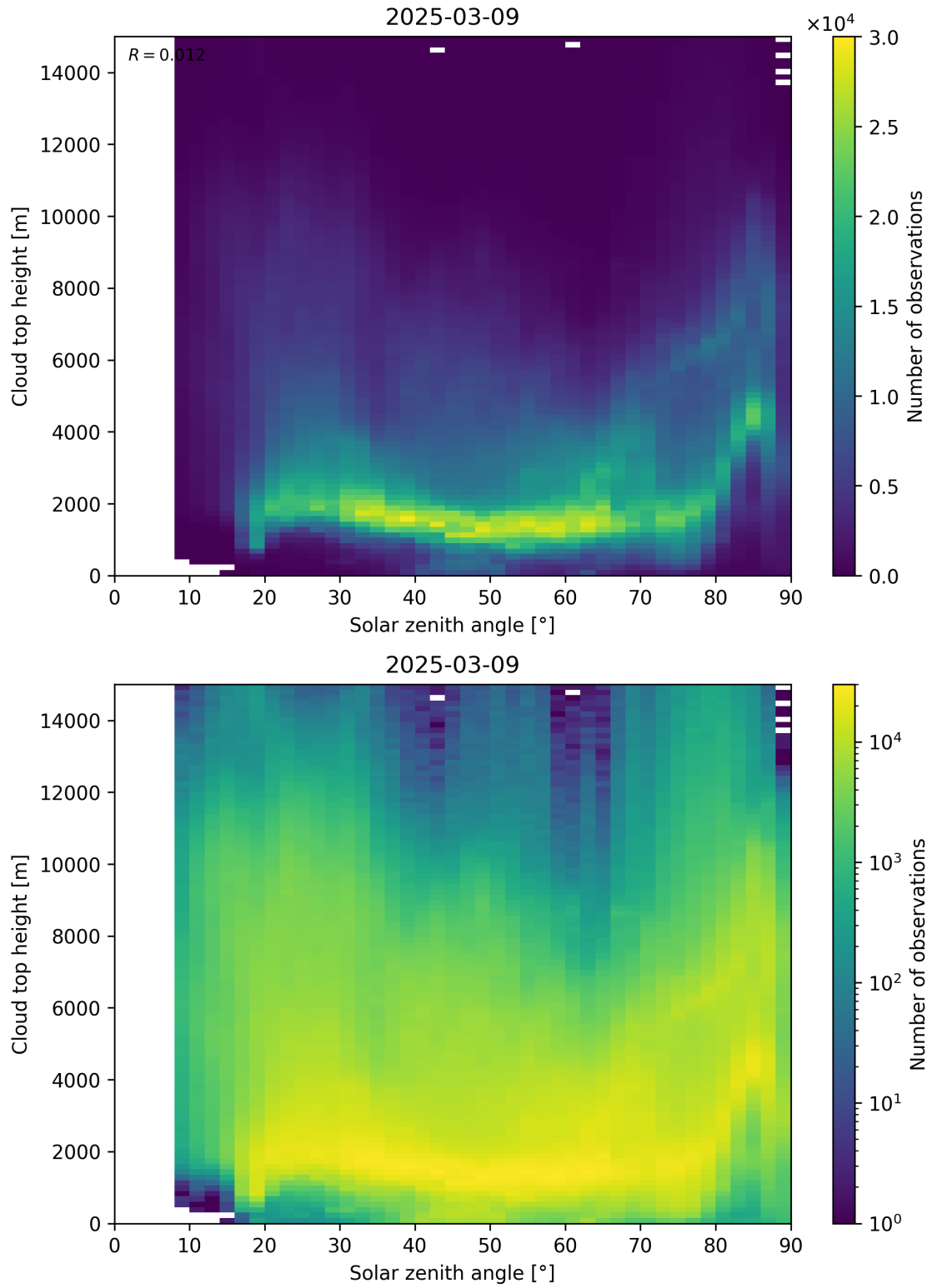
Figure 104: Scatter density plot of “Solar zenith angle” against “Cloud top height” for 2025-03-08 to 2025-03-10.
