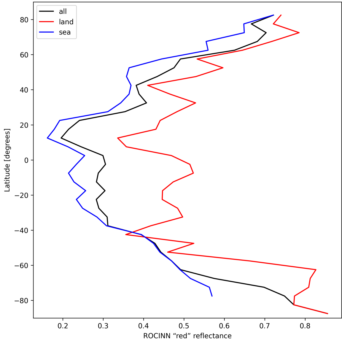
Figure 37: Zonal average of “ROCINN “red” reflectance” for 2025-03-08 to 2025-03-10.
