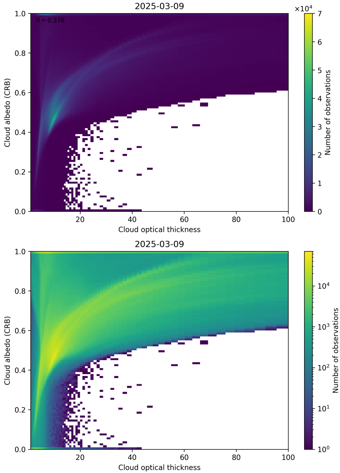
Figure 82: Scatter density plot of “Cloud optical thickness” against “Cloud albedo (CRB)” for 2025-03-08 to 2025-03-10.
