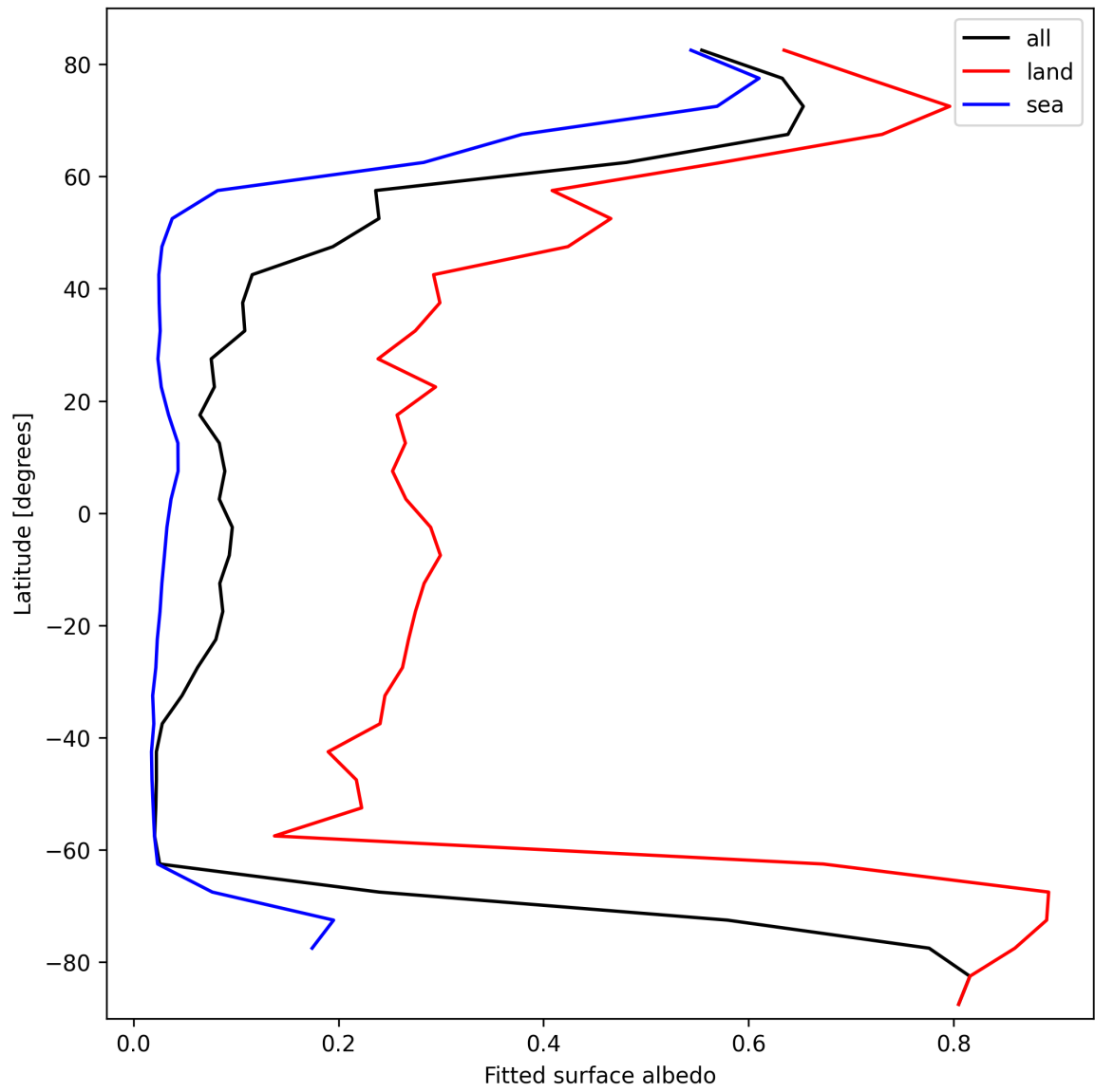
Figure 29: Zonal average of “Fitted surface albedo” for 2025-03-08 to 2025-03-10.
