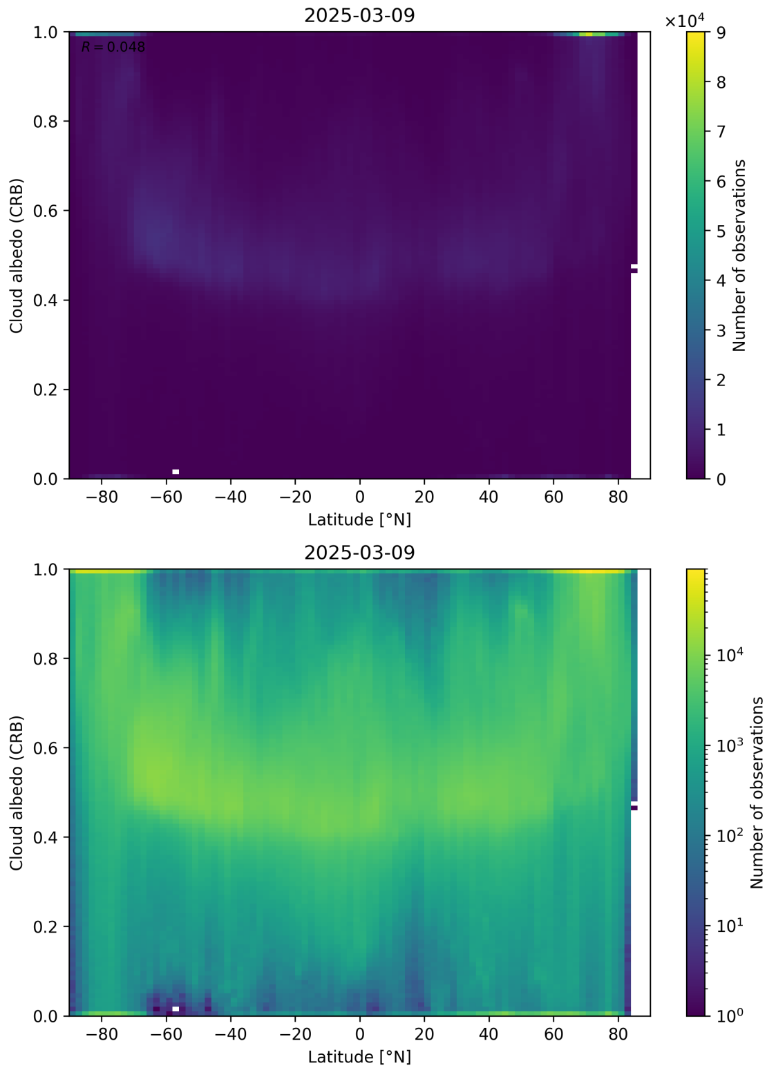
Figure 91: Scatter density plot of “Latitude” against “Cloud albedo (CRB)” for 2025-03-08 to 2025-03-10.
