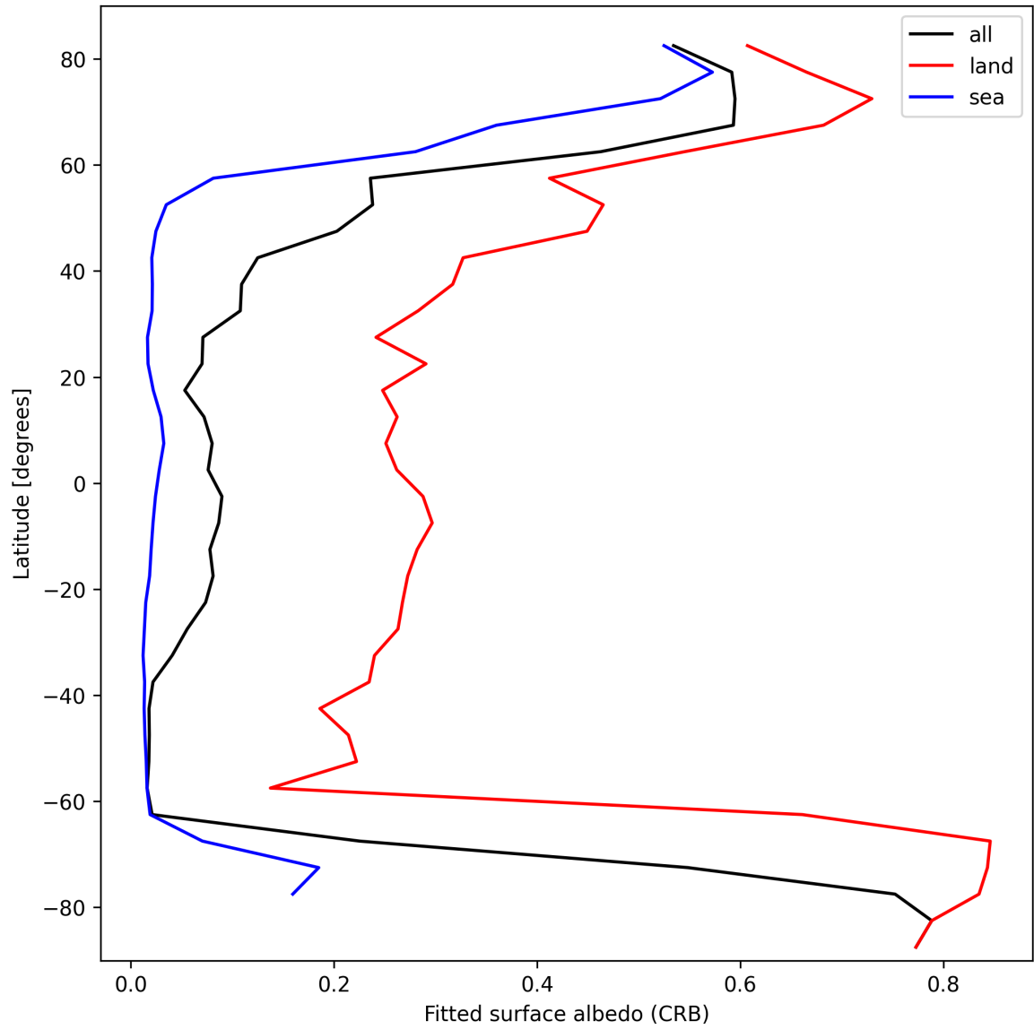
Figure 30: Zonal average of “Fitted surface albedo (CRB)” for 2025-03-08 to 2025-03-10.
