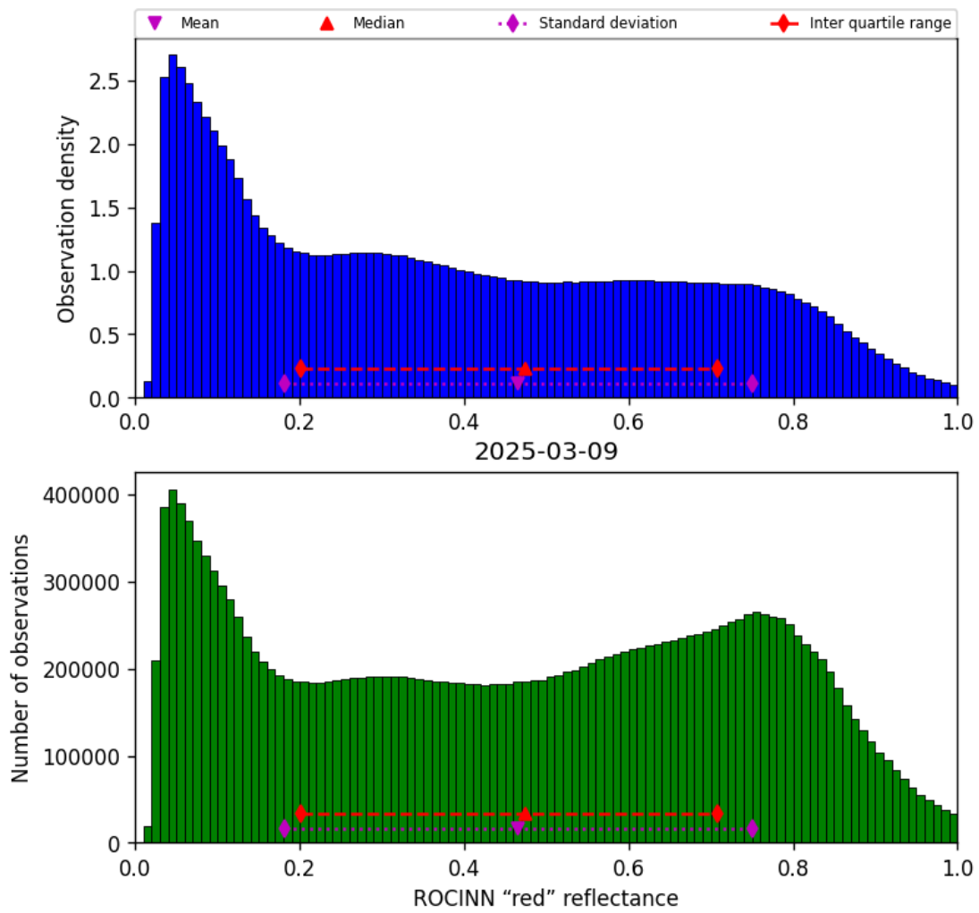
Figure 53: Histogram of “ROCINN “red” reflectance” for 2025-03-08 to 2025-03-10
