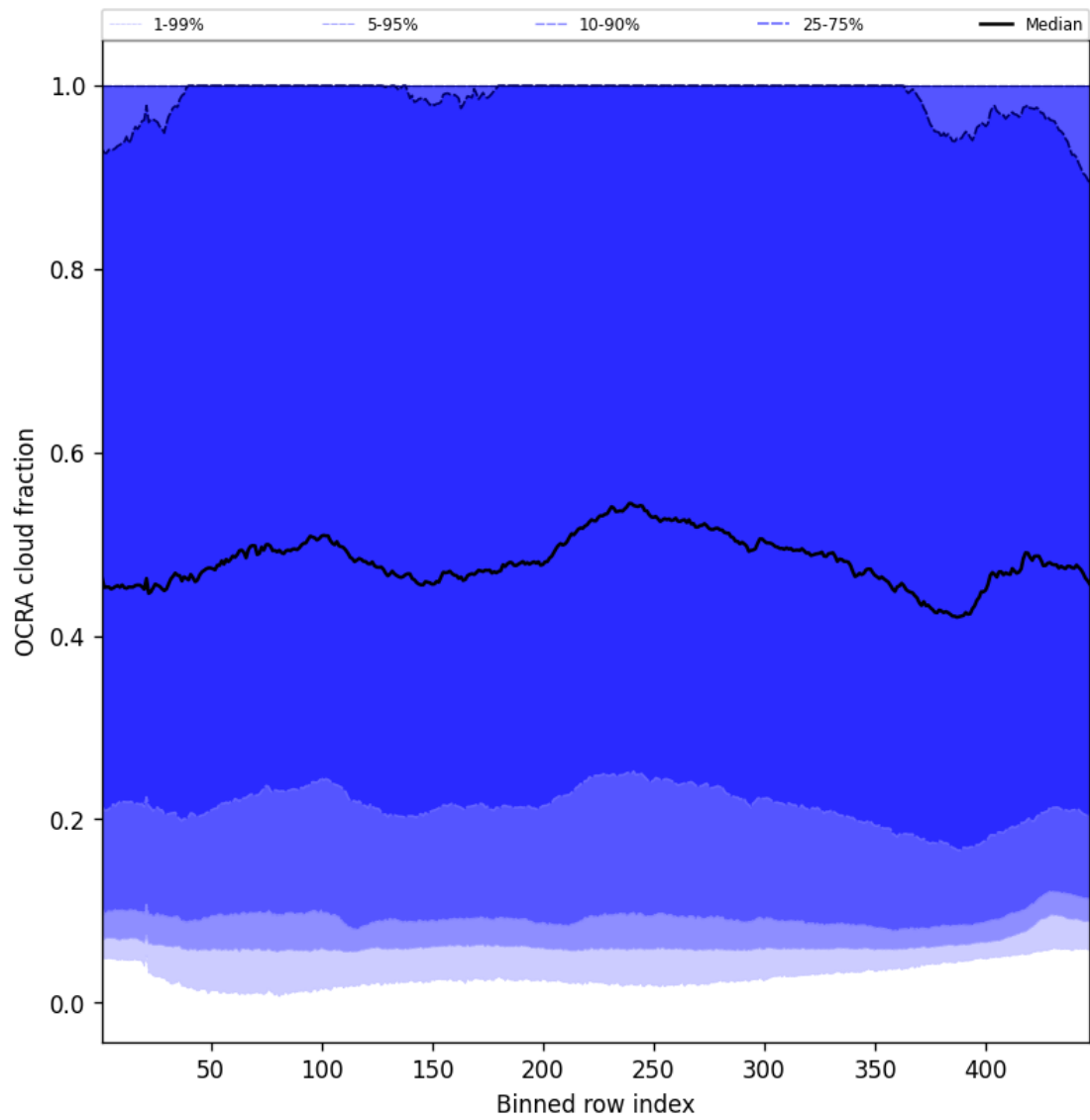
Figure 66: Along track statistics of “OCRA cloud fraction” for 2025-03-08 to 2025-03-10
