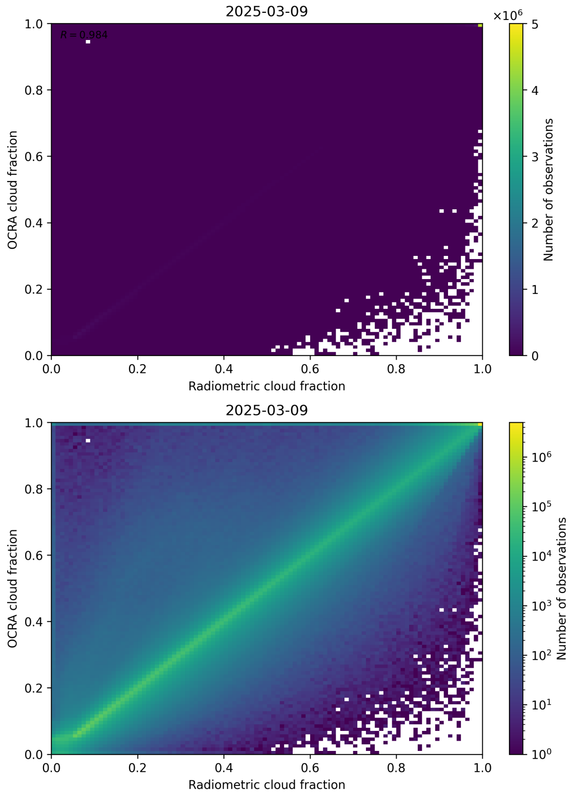
Figure 72: Scatter density plot of “Radiometric cloud fraction” against “OCRA cloud fraction” for 2025-03-08 to 2025-03-10.
