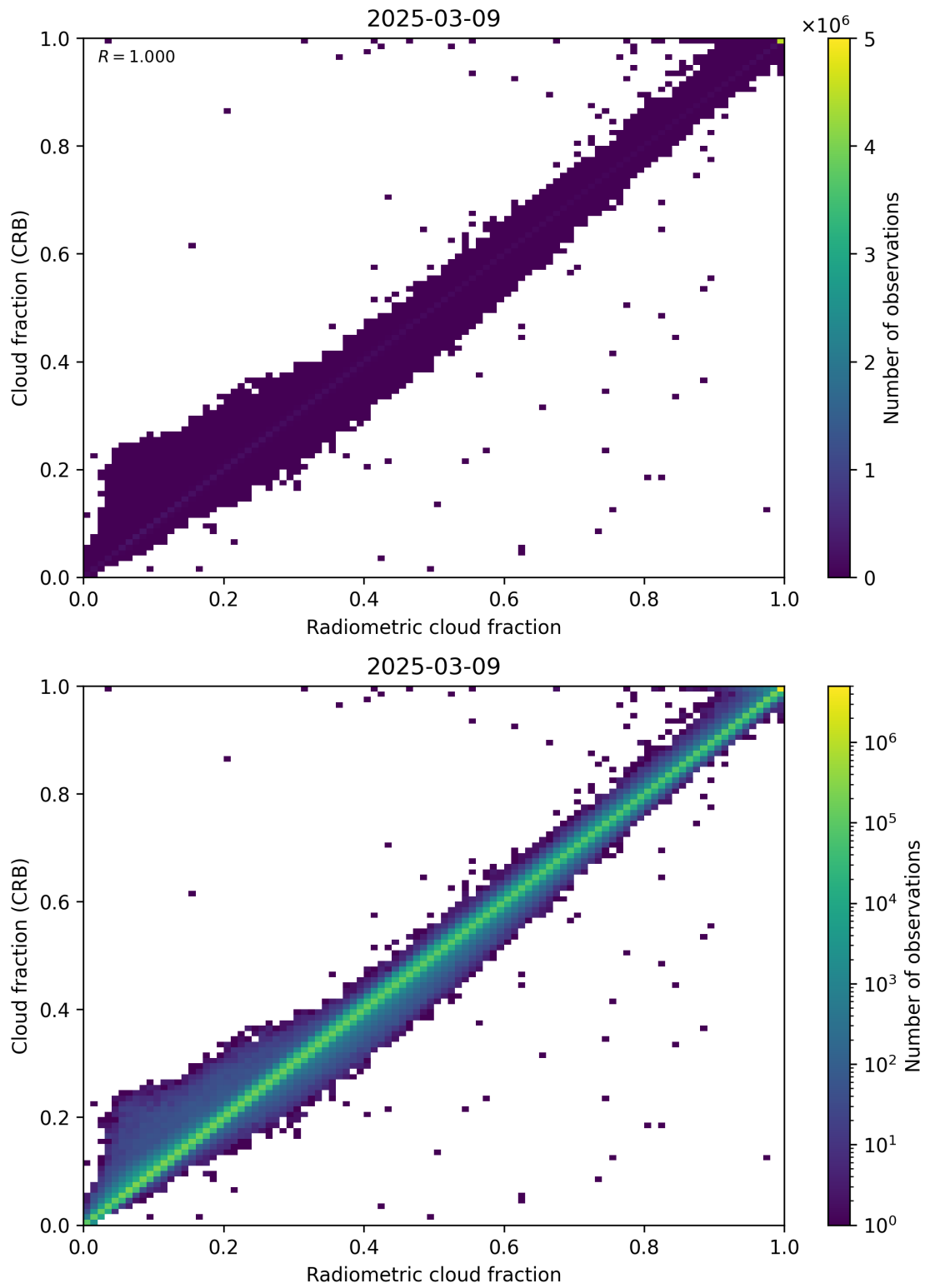
Figure 73: Scatter density plot of “Radiometric cloud fraction” against “Cloud fraction (CRB)” for 2025-03-08 to 2025-03-10.
