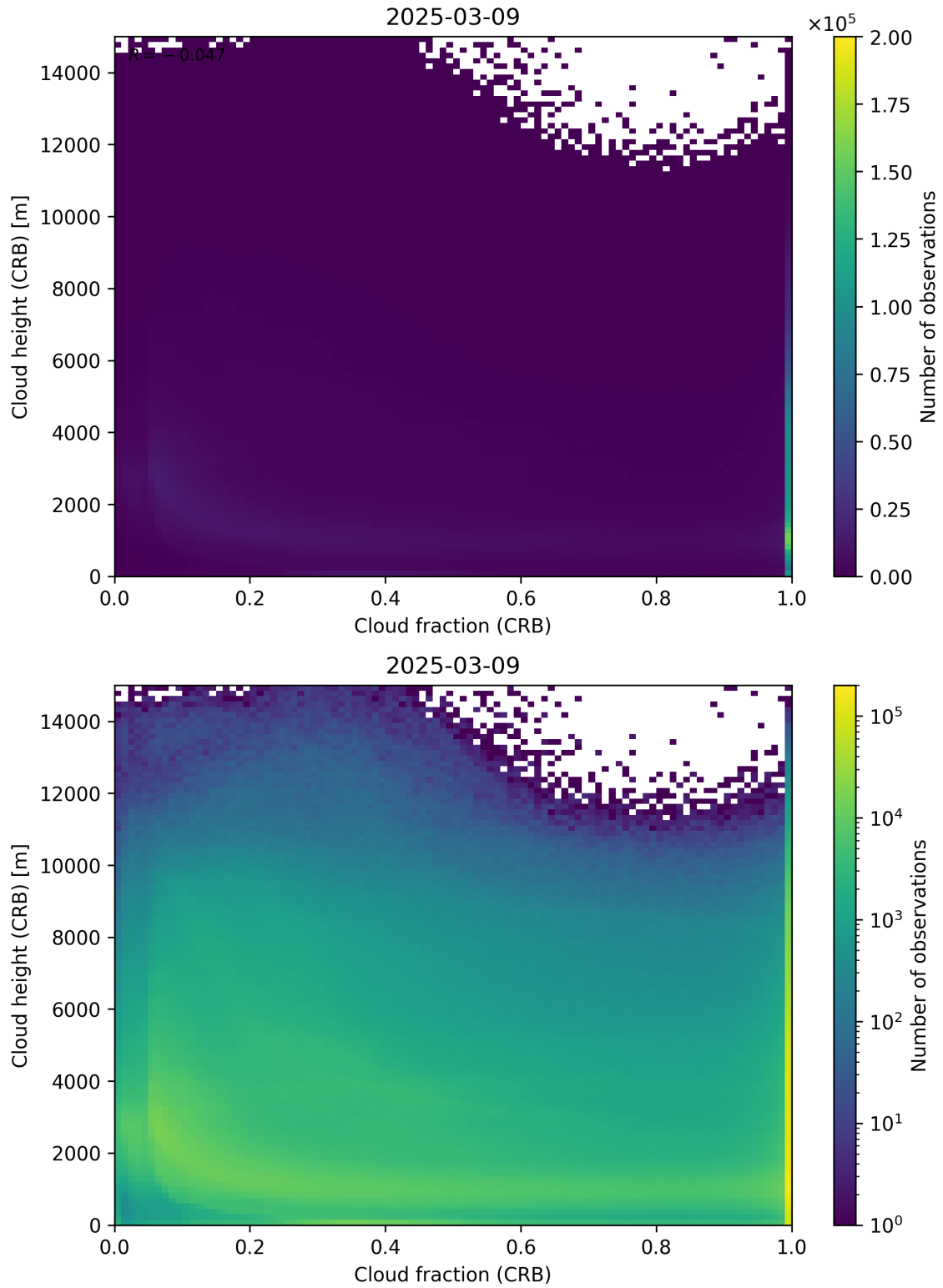
Figure 79: Scatter density plot of “Cloud fraction (CRB)” against “Cloud height (CRB)” for 2025-03-08 to 2025-03-10.
