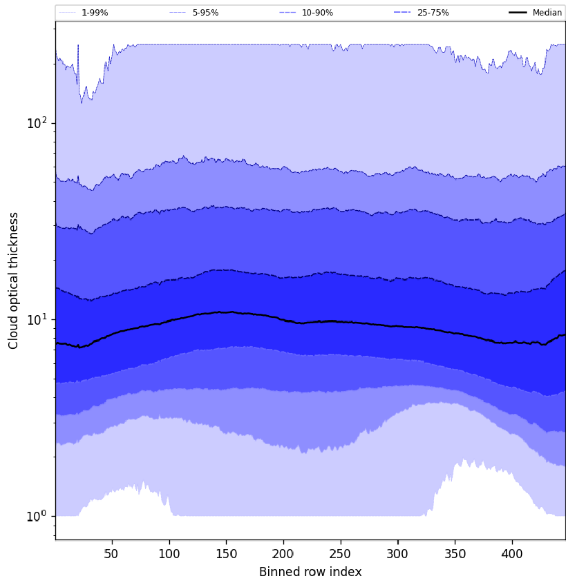
Figure 57: Along track statistics of “Cloud optical thickness” for 2025-03-08 to 2025-03-10
