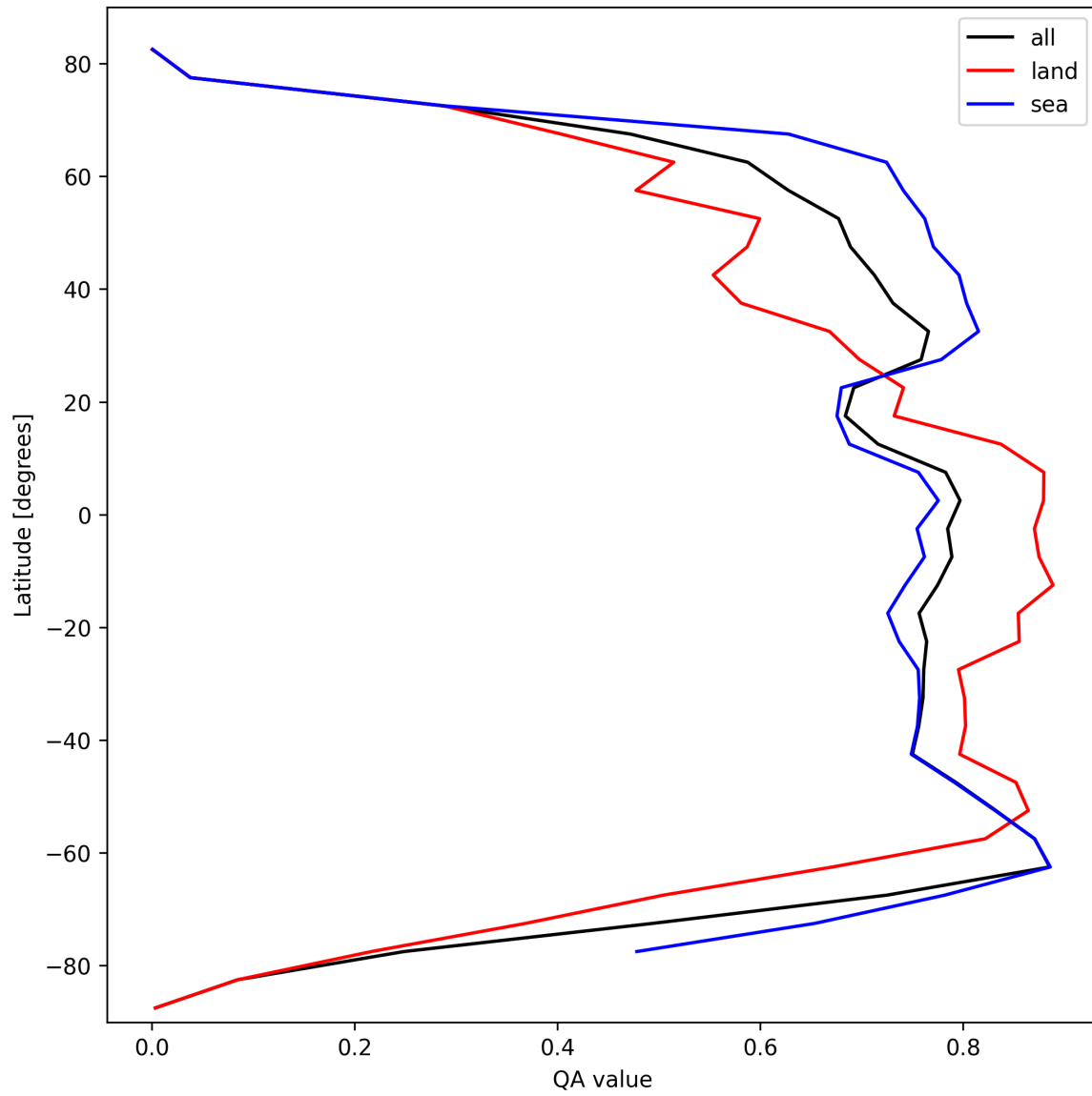
Figure 22: Zonal average of “QA value” for 2025-03-08 to 2025-03-10.
