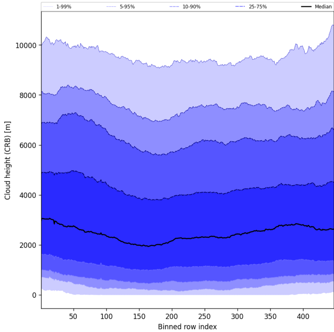
Figure 59: Along track statistics of “Cloud height (CRB)” for 2025-03-08 to 2025-03-10
