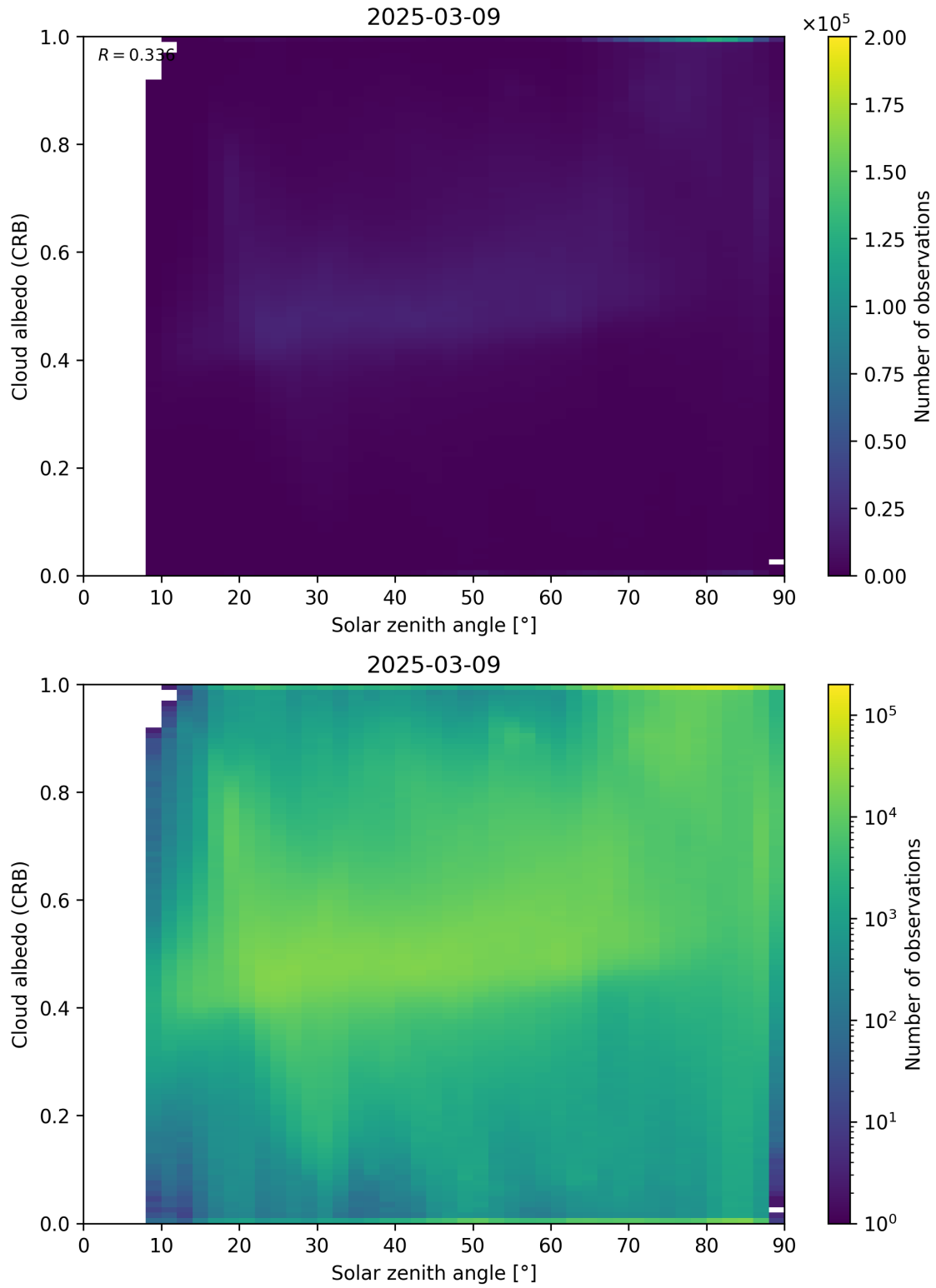
Figure 98: Scatter density plot of “Solar zenith angle” against “Cloud albedo (CRB)” for 2025-03-08 to 2025-03-10.
