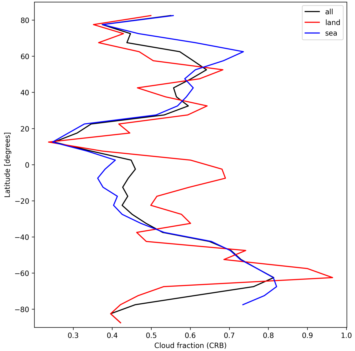
Figure 26: Zonal average of “Cloud fraction (CRB)” for 2025-03-08 to 2025-03-10.
