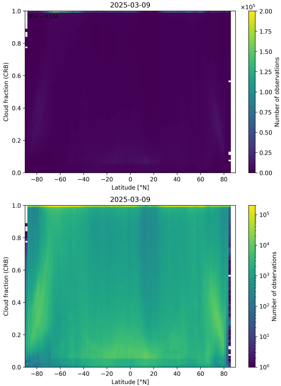
Figure 94: Scatter density plot of “Latitude” against “Cloud fraction (CRB)” for 2025-03-08 to 2025-03-10.
