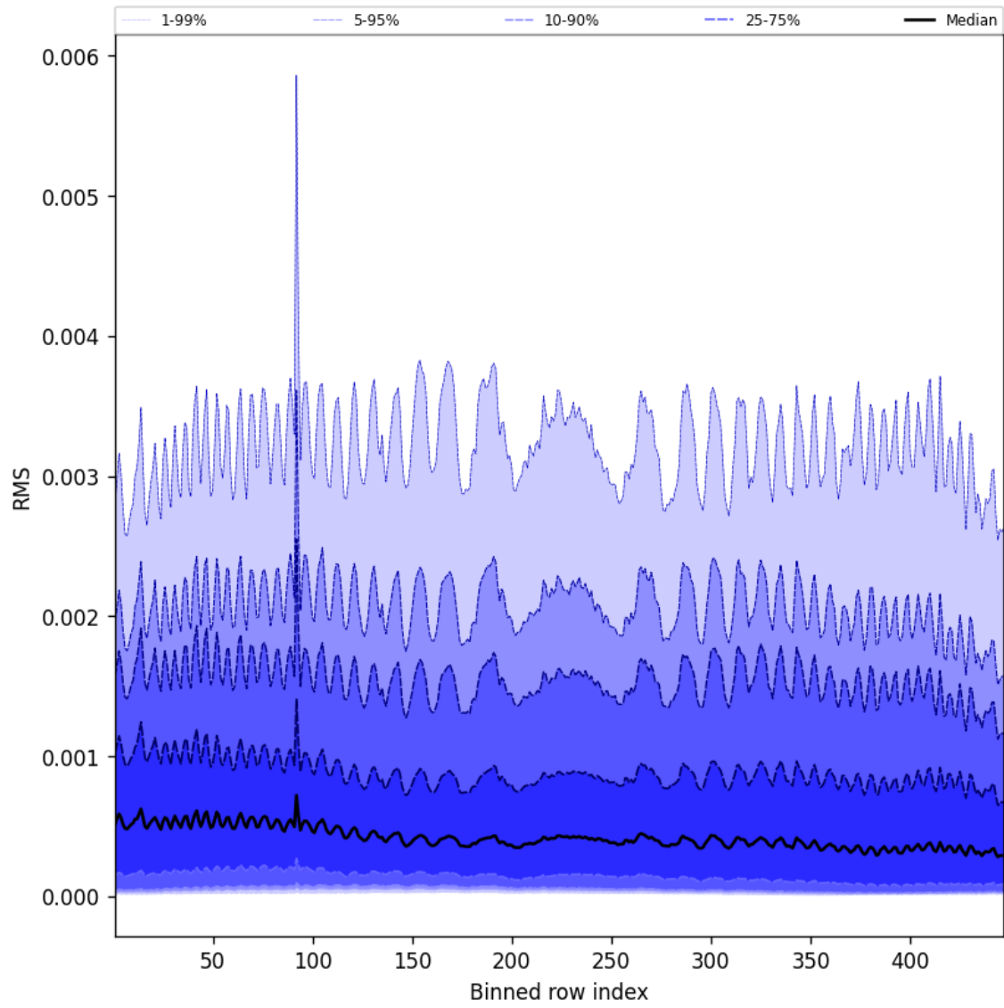
Figure 63: Along track statistics of “RMS” for 2025-03-08 to 2025-03-10
