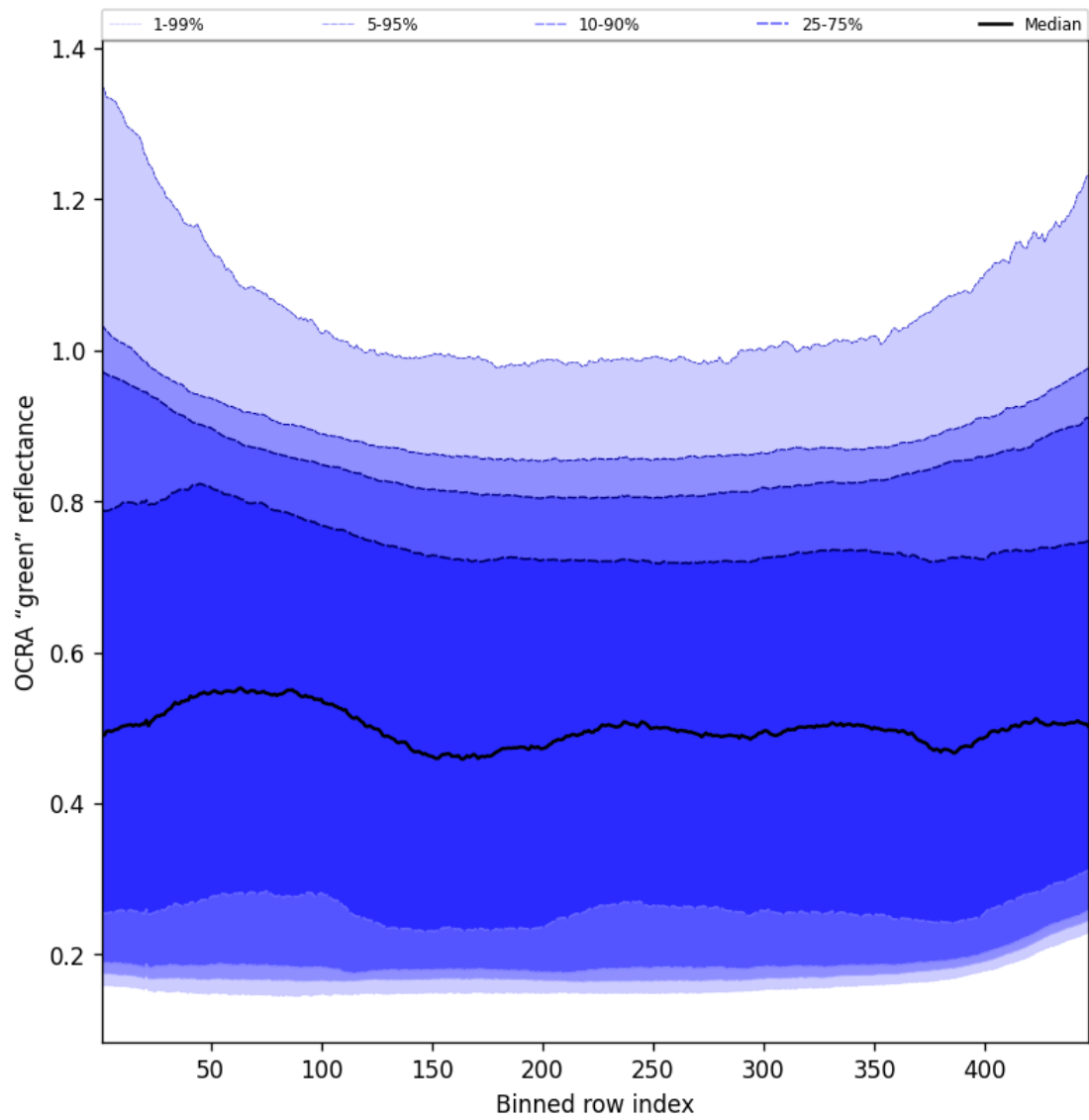
Figure 68: Along track statistics of “OCRA “green” reflectance” for 2025-03-08 to 2025-03-10
