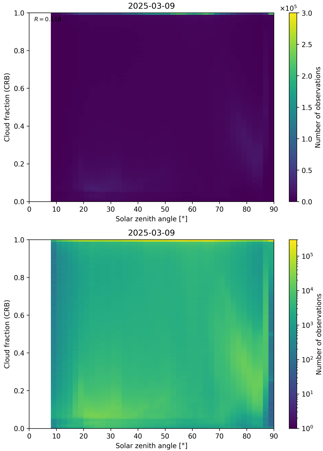
Figure 101: Scatter density plot of “Solar zenith angle” against “Cloud fraction (CRB)” for 2025-03-08 to 2025-03-10.
