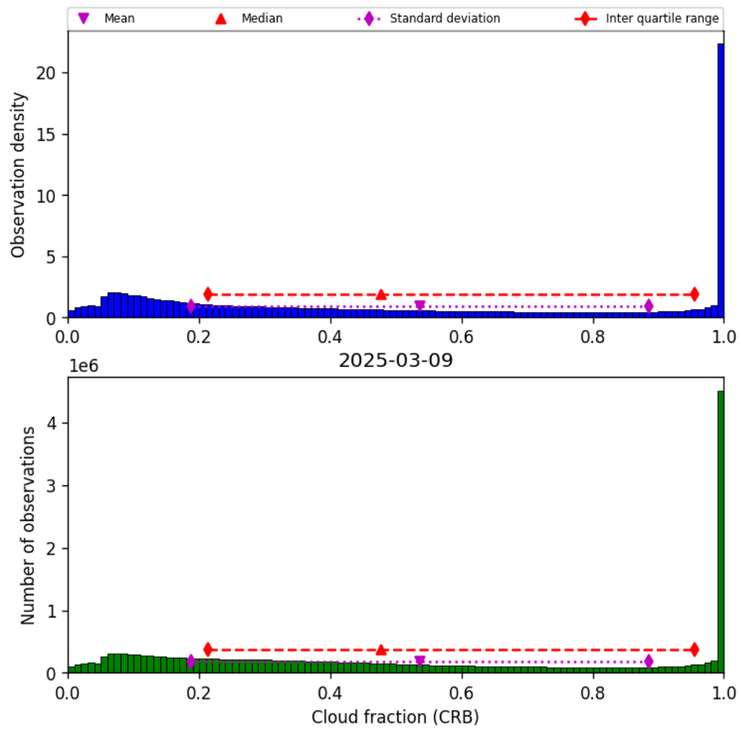
Figure 42: Histogram of “Cloud fraction (CRB)” for 2025-03-08 to 2025-03-10
