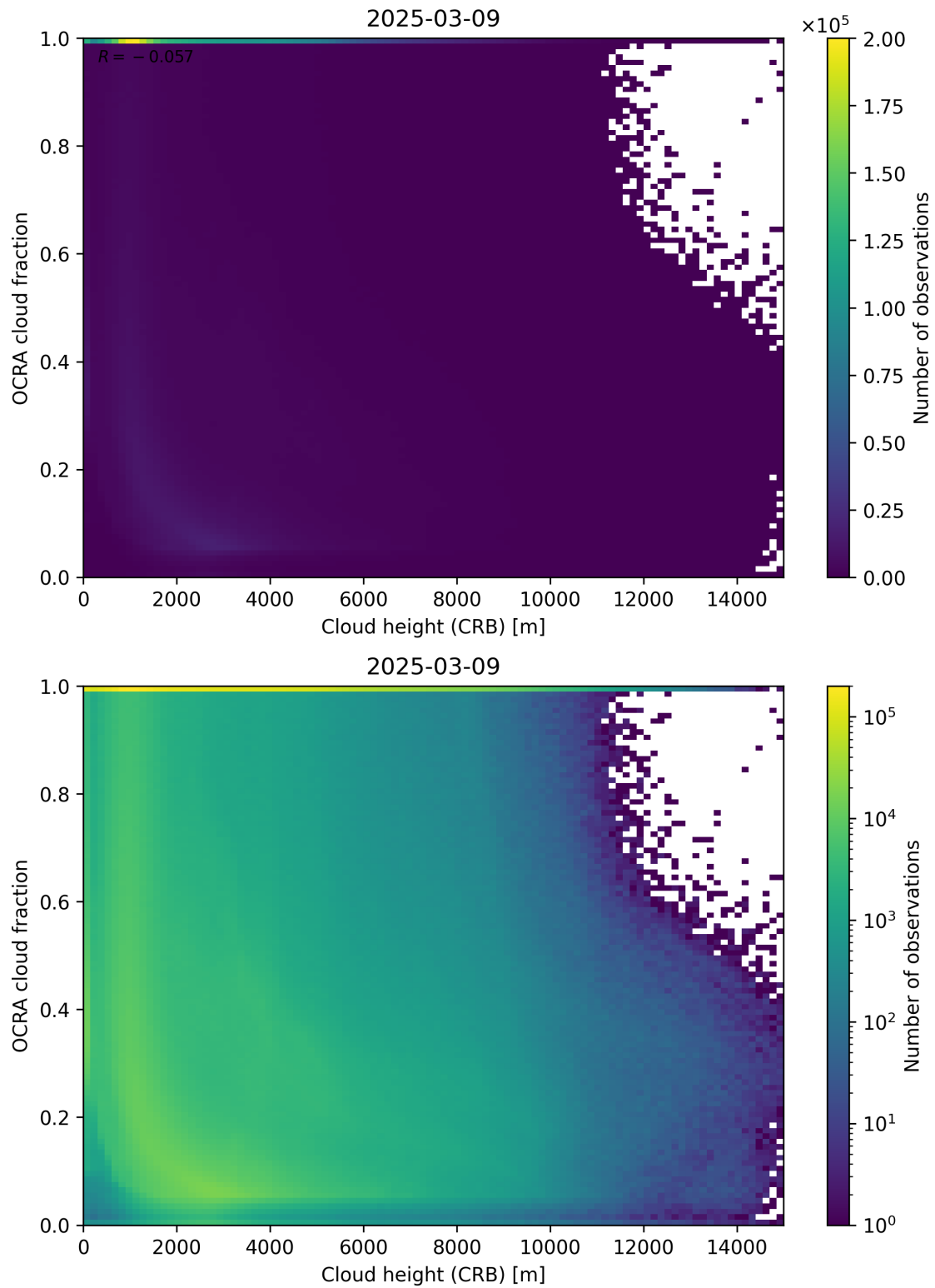
Figure 81: Scatter density plot of “Cloud height (CRB)” against “OCRA cloud fraction” for 2025-03-08 to 2025-03-10.
