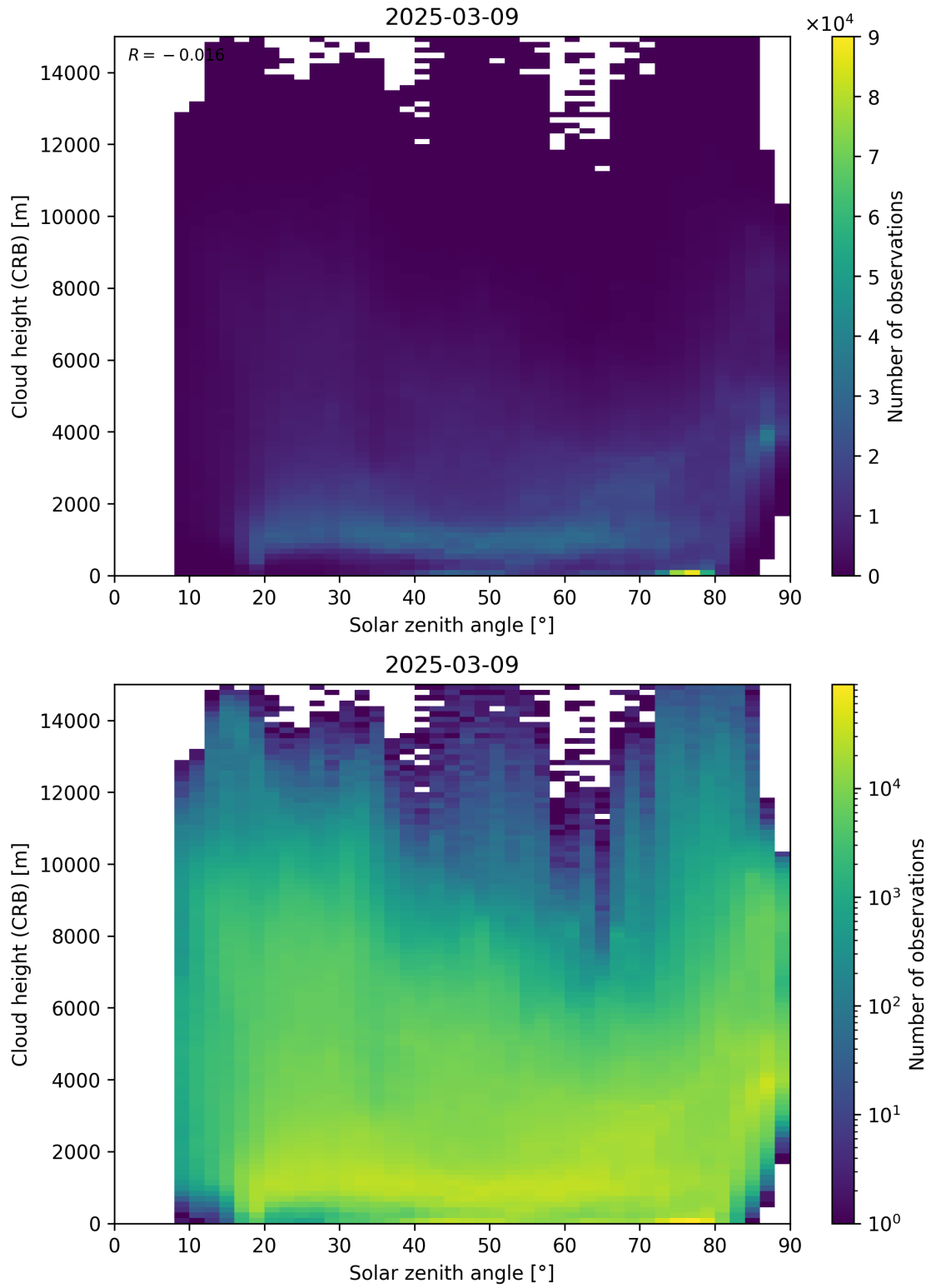
Figure 102: Scatter density plot of “Solar zenith angle” against “Cloud height (CRB)” for 2025-03-08 to 2025-03-10.
