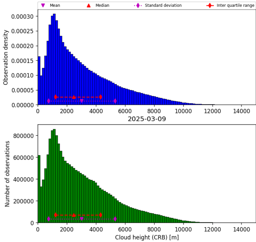
Figure 43: Histogram of “Cloud height (CRB)” for 2025-03-08 to 2025-03-10
