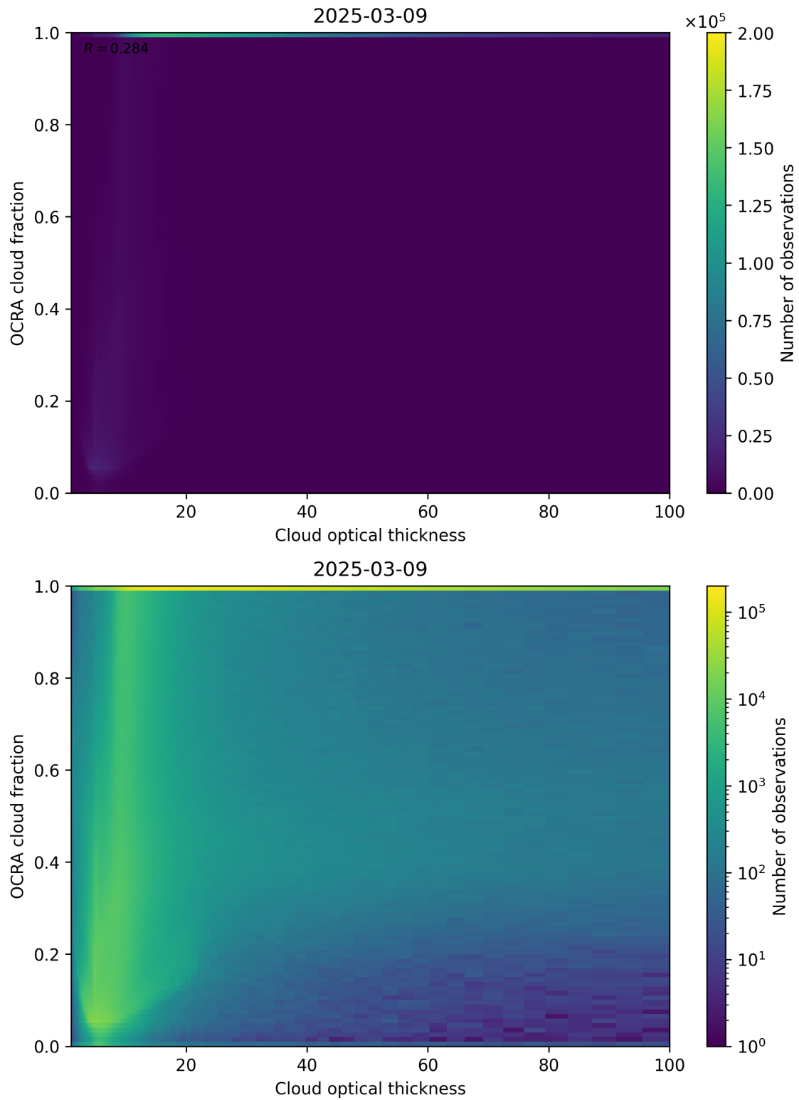
Figure 83: Scatter density plot of “Cloud optical thickness” against “OCRA cloud fraction” for 2025-03-08 to 2025-03-10.
