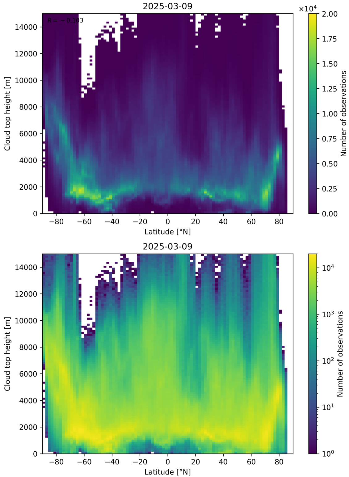
Figure 97: Scatter density plot of “Latitude” against “Cloud top height” for 2025-03-08 to 2025-03-10.
