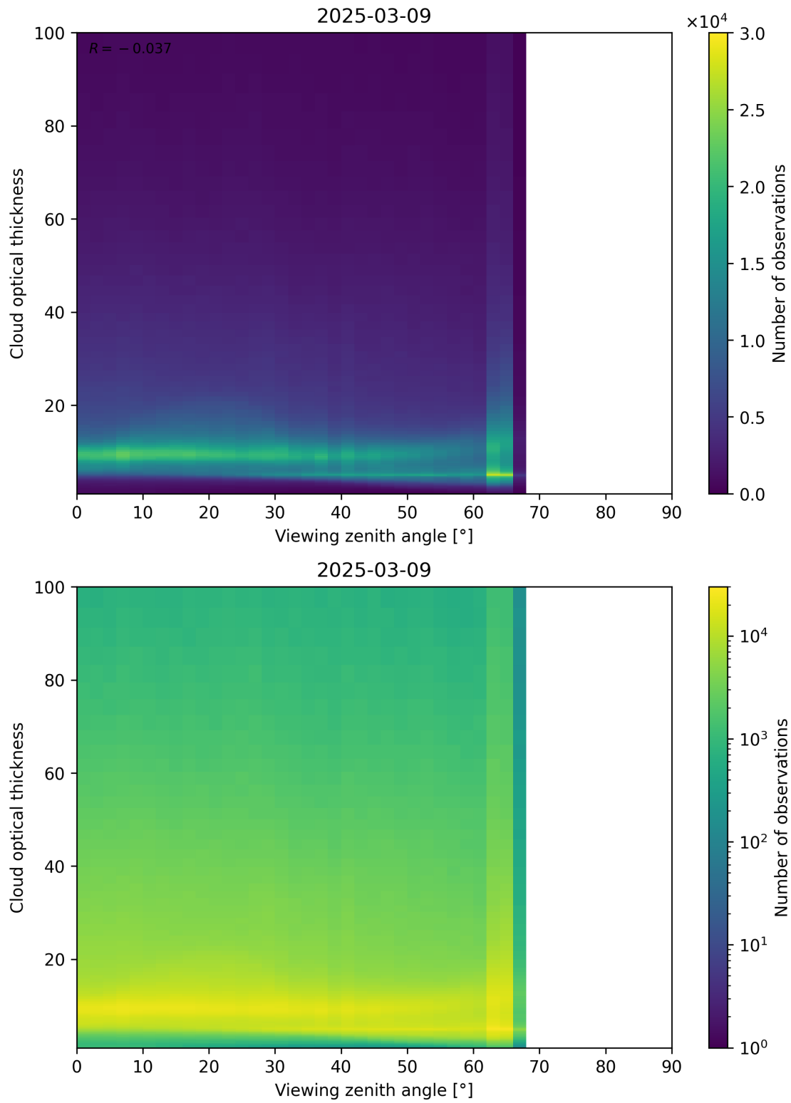
Figure 111: Scatter density plot of “Viewing zenith angle” against “Cloud optical thickness” for 2025-03-08 to 2025-03-10.
