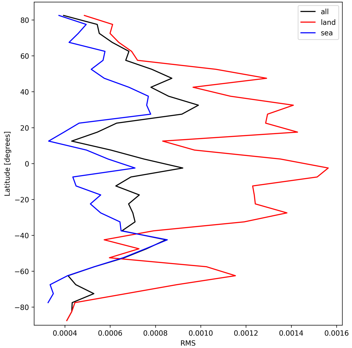
Figure 31: Zonal average of “RMS” for 2025-03-08 to 2025-03-10.
