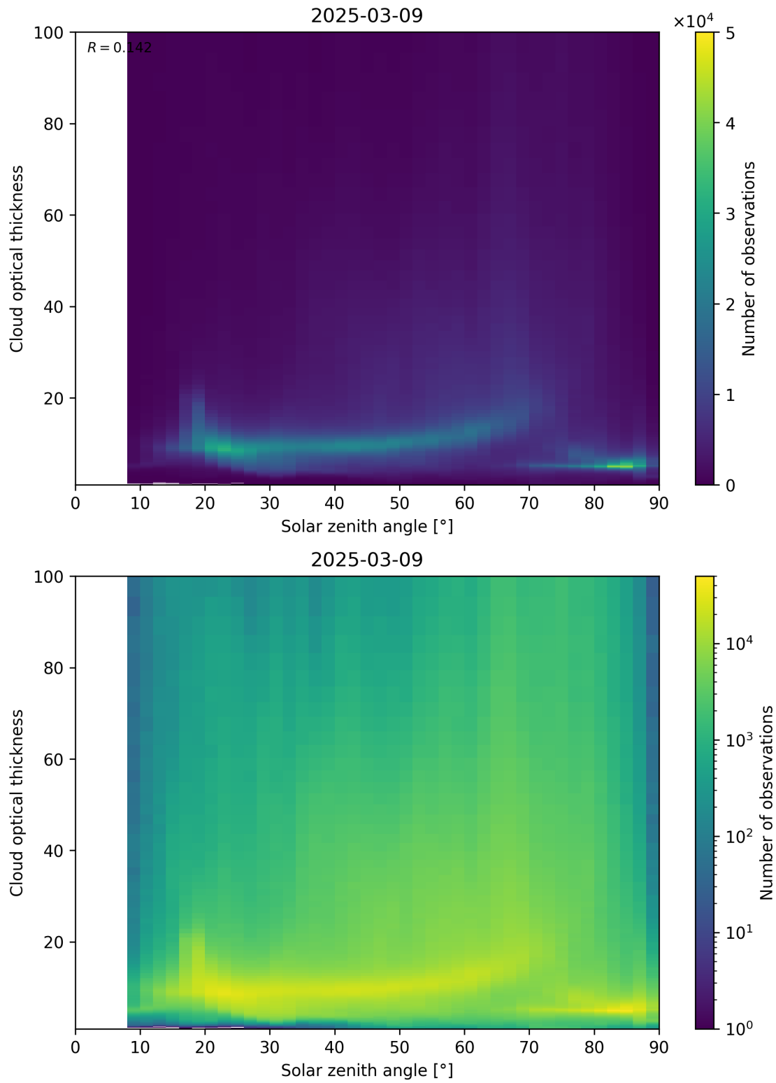
Figure 103: Scatter density plot of “Solar zenith angle” against “Cloud optical thickness” for 2025-03-08 to 2025-03-10.
