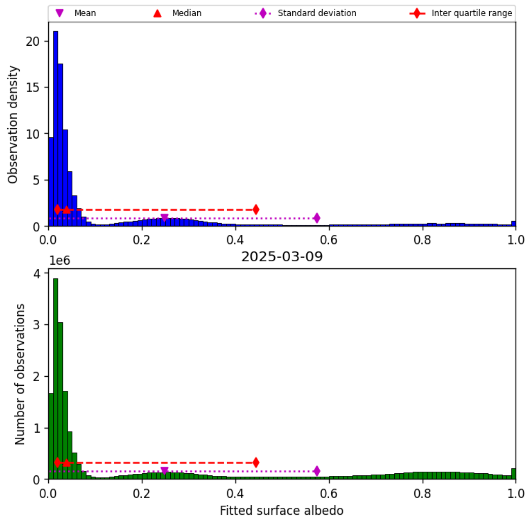
Figure 45: Histogram of “Fitted surface albedo” for 2025-03-08 to 2025-03-10
