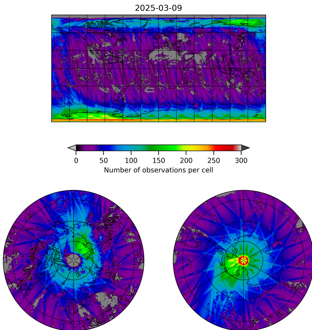
Figure 21: Map of the number of observations for 2025-03-08 to 2025-03-10
