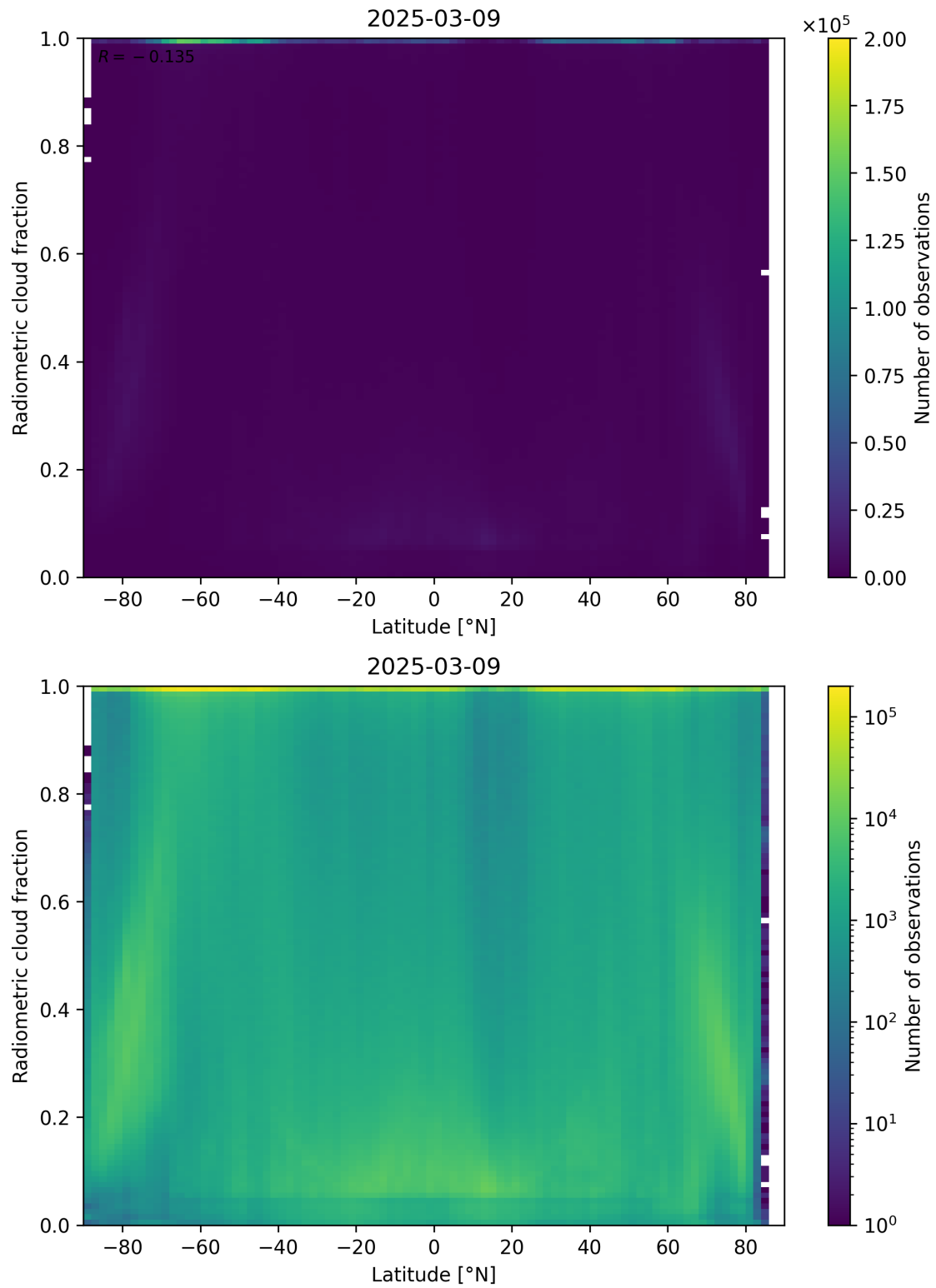
Figure 92: Scatter density plot of “Latitude” against “Radiometric cloud fraction” for 2025-03-08 to 2025-03-10.
