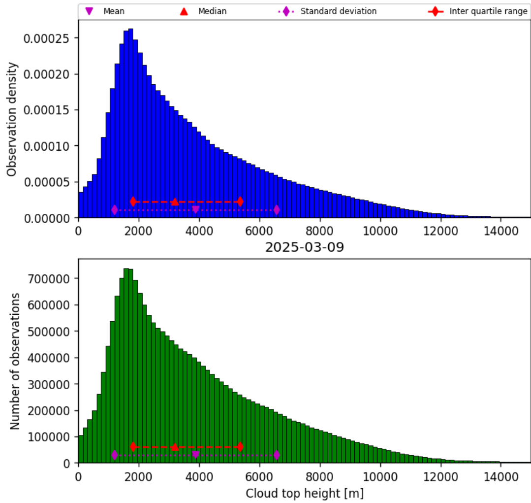
Figure 40: Histogram of “Cloud top height” for 2025-03-08 to 2025-03-10
