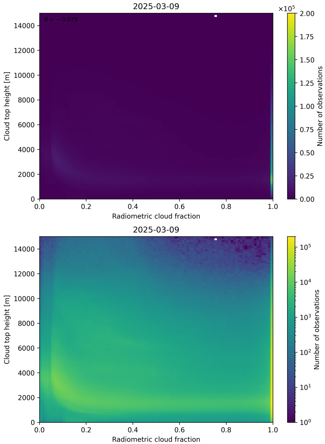
Figure 76: Scatter density plot of “Radiometric cloud fraction” against “Cloud top height” for 2025-03-08 to 2025-03-10.
