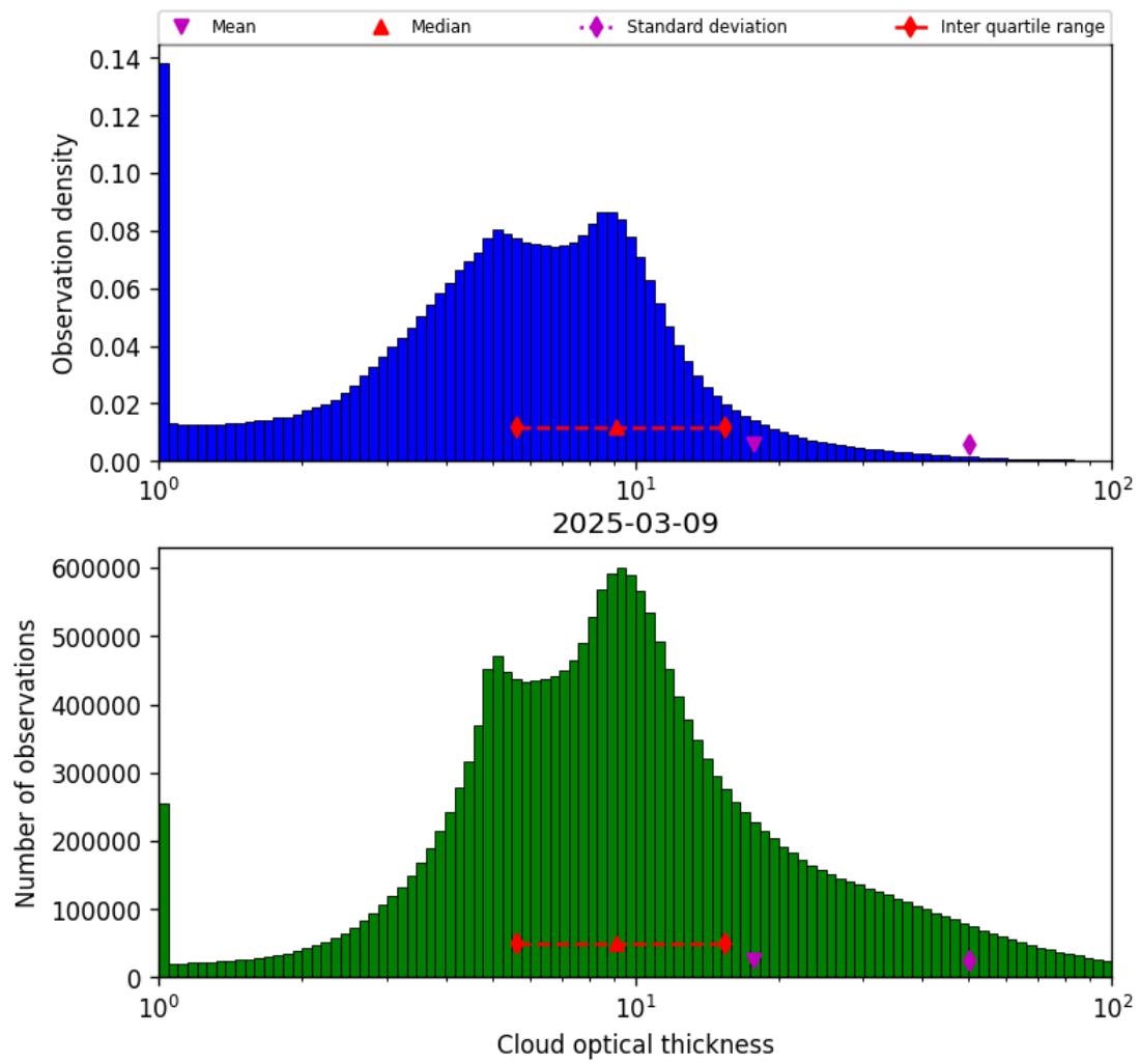
Figure 41: Histogram of “Cloud optical thickness” for 2025-03-08 to 2025-03-10
