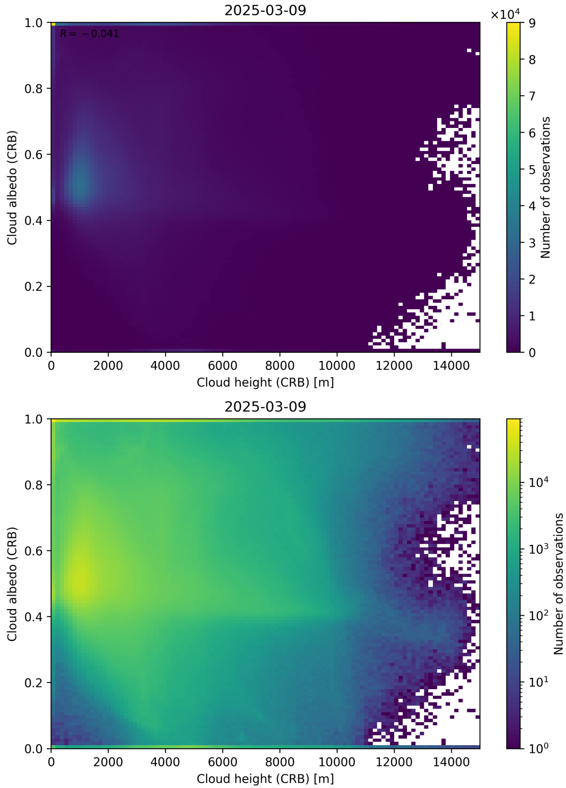
Figure 80: Scatter density plot of “Cloud height (CRB)” against “Cloud albedo (CRB)” for 2025-03-08 to 2025-03-10.
