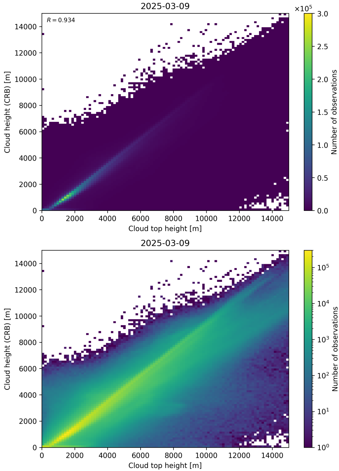
Figure 89: Scatter density plot of “Cloud top height” against “Cloud height (CRB)” for 2025-03-08 to 2025-03-10.
