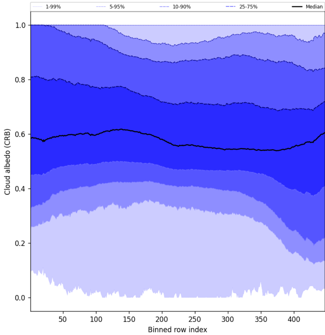
Figure 60: Along track statistics of “Cloud albedo (CRB)” for 2025-03-08 to 2025-03-10
