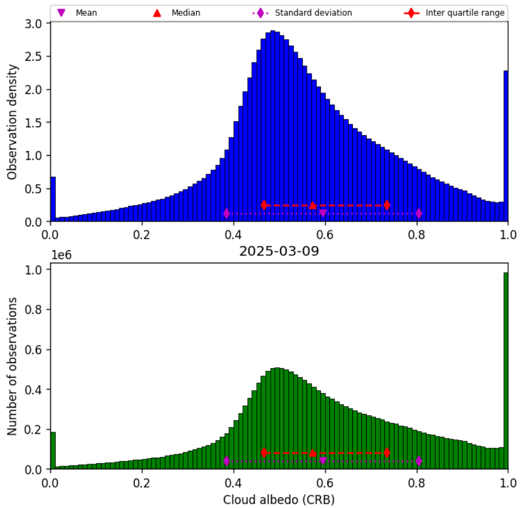
Figure 44: Histogram of “Cloud albedo (CRB)” for 2025-03-08 to 2025-03-10
