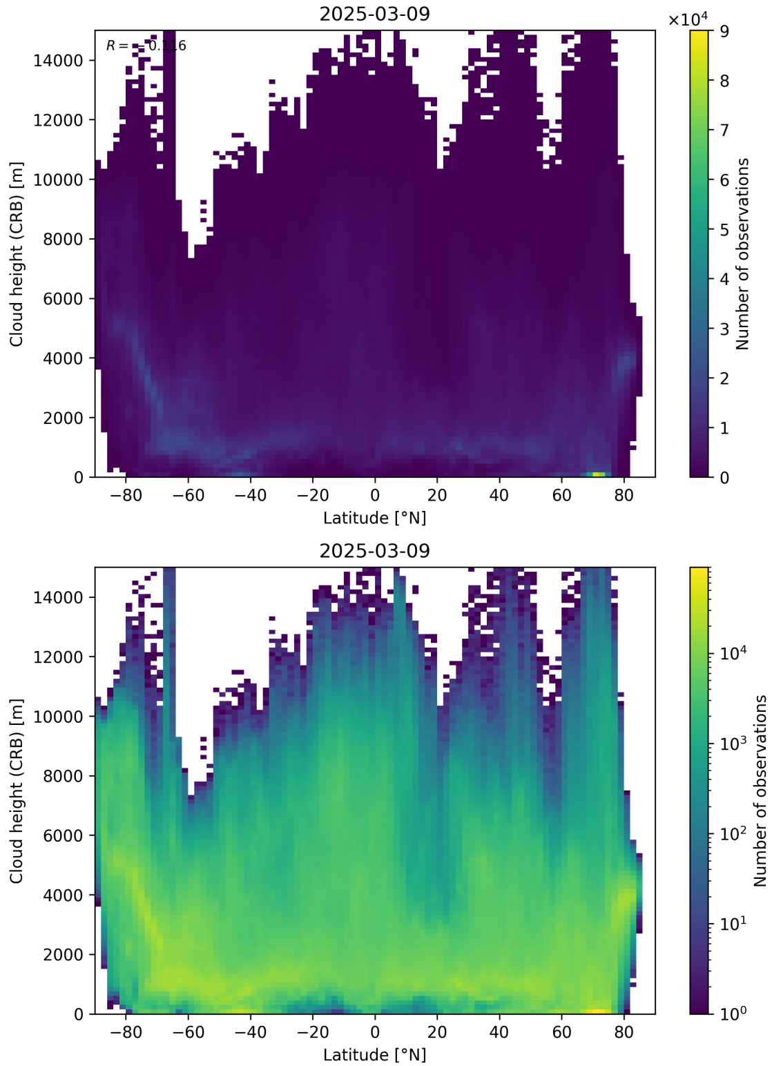
Figure 95: Scatter density plot of “Latitude” against “Cloud height (CRB)” for 2025-03-08 to 2025-03-10.
