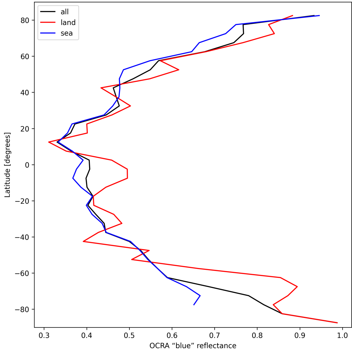
Figure 35: Zonal average of “OCRA “blue” reflectance” for 2025-03-08 to 2025-03-10.
