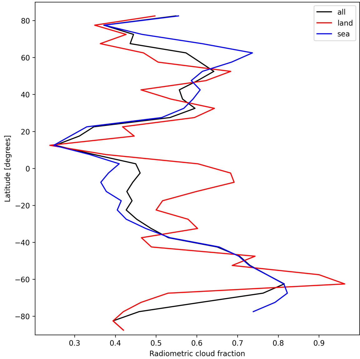
Figure 23: Zonal average of “Radiometric cloud fraction” for 2025-03-08 to 2025-03-10.
