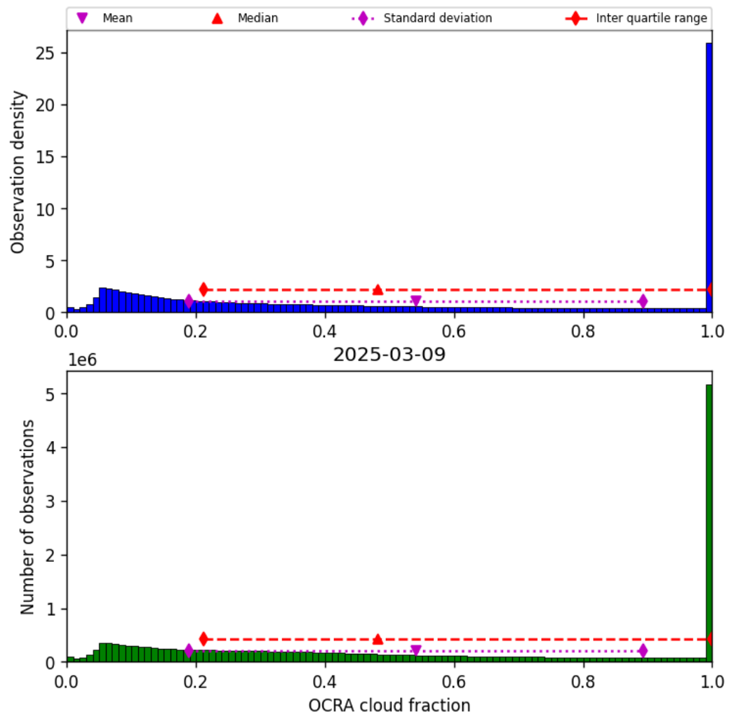
Figure 50: Histogram of “OCRA cloud fraction” for 2025-03-08 to 2025-03-10
