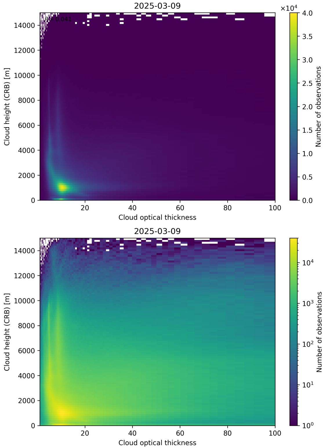
Figure 85: Scatter density plot of “Cloud optical thickness” against “Cloud height (CRB)” for 2025-03-08 to 2025-03-10.
