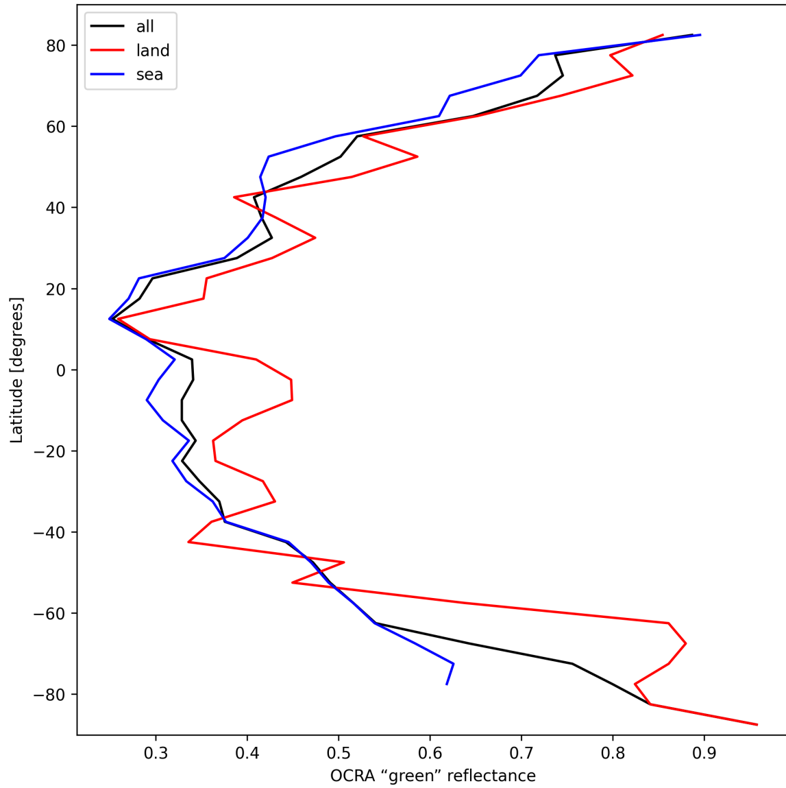
Figure 36: Zonal average of “OCRA “green” reflectance” for 2025-03-08 to 2025-03-10.
