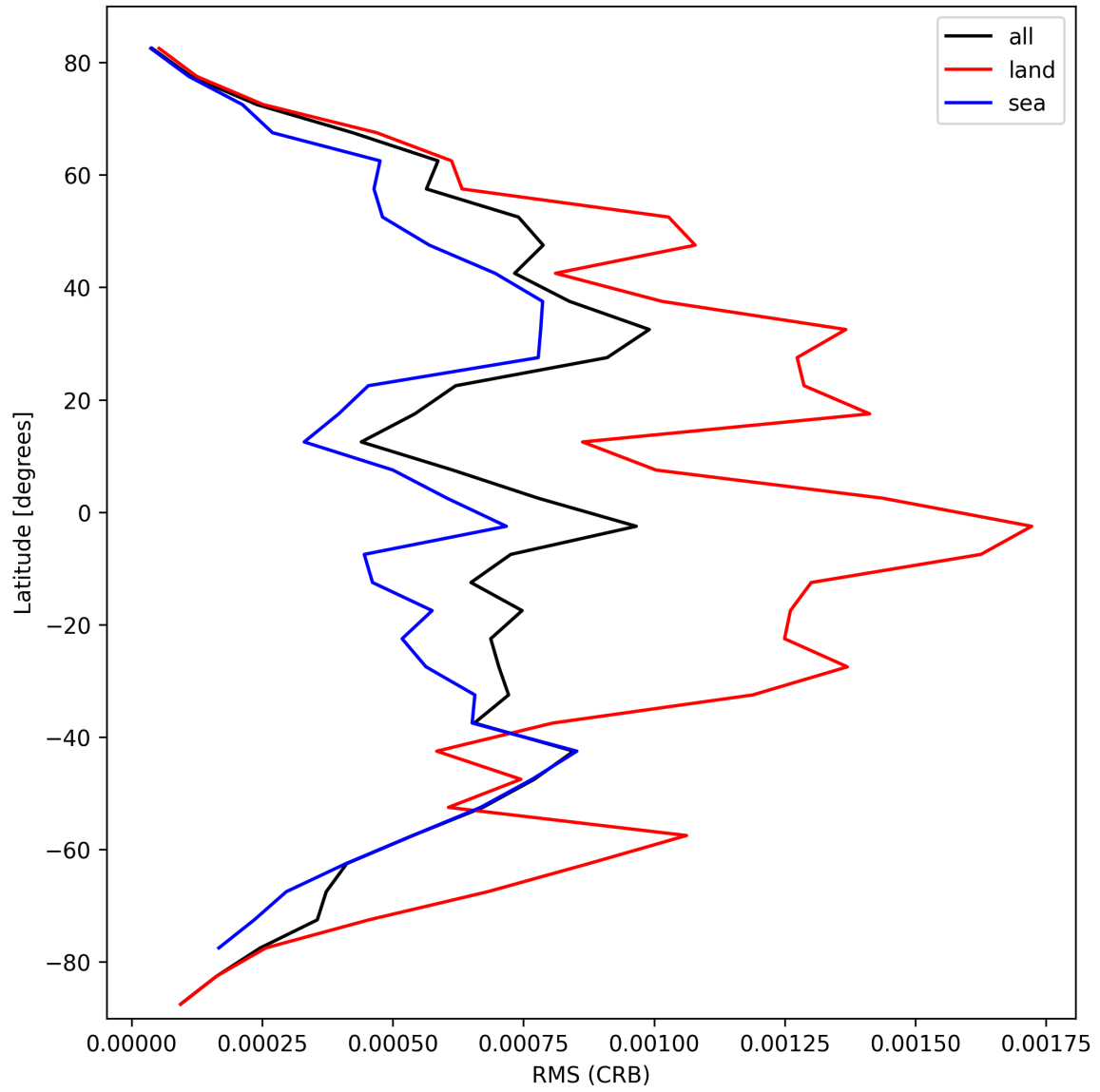
Figure 32: Zonal average of “RMS (CRB)” for 2025-03-08 to 2025-03-10.
