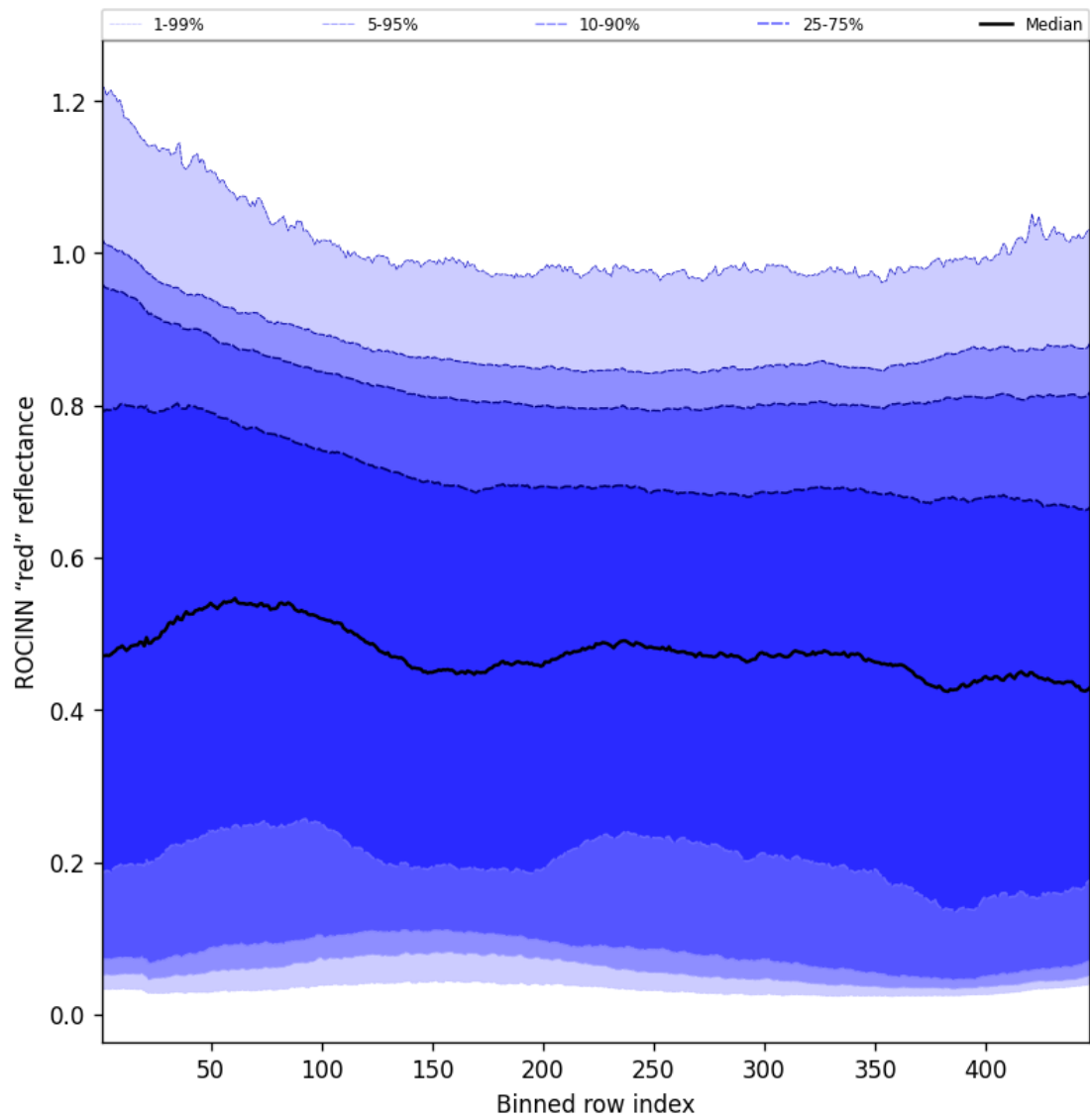
Figure 69: Along track statistics of “ROCINN “red” reflectance” for 2025-03-08 to 2025-03-10
