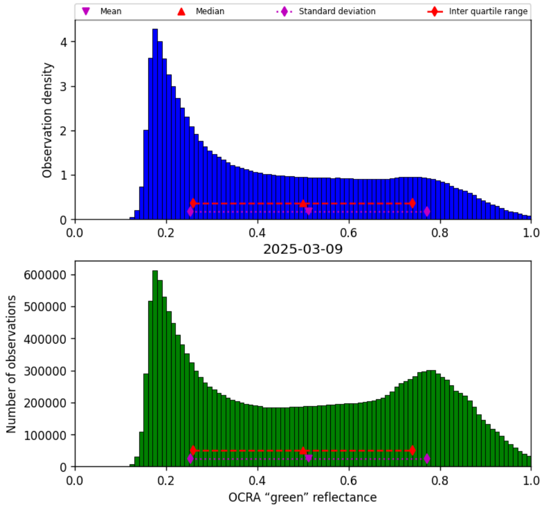
Figure 52: Histogram of “OCRA “green” reflectance” for 2025-03-08 to 2025-03-10
