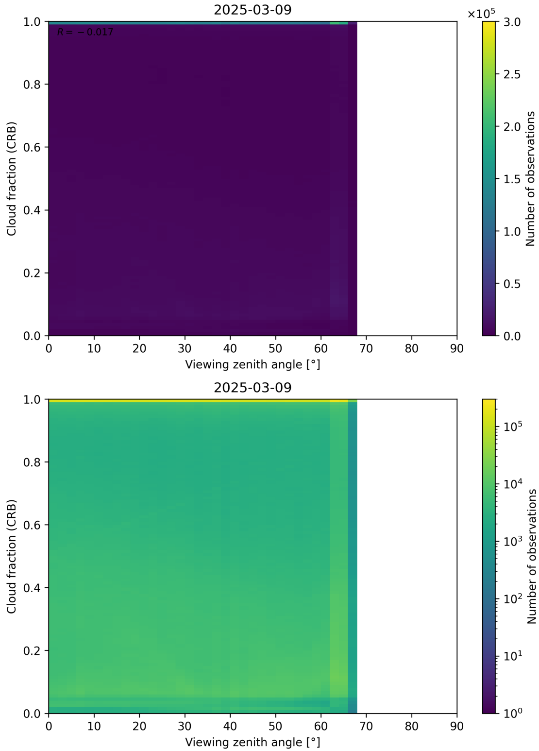
Figure 109: Scatter density plot of “Viewing zenith angle” against “Cloud fraction (CRB)” for 2025-03-08 to 2025-03-10.
