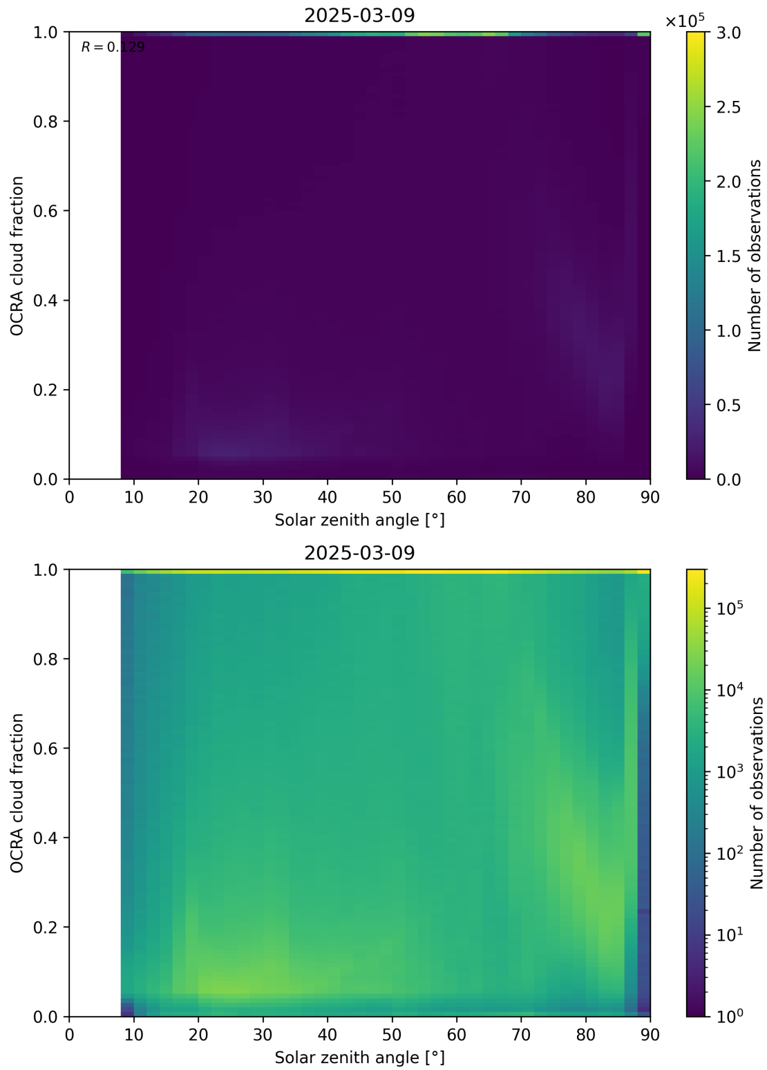
Figure 100: Scatter density plot of “Solar zenith angle” against “OCRA cloud fraction” for 2025-03-08 to 2025-03-10.
