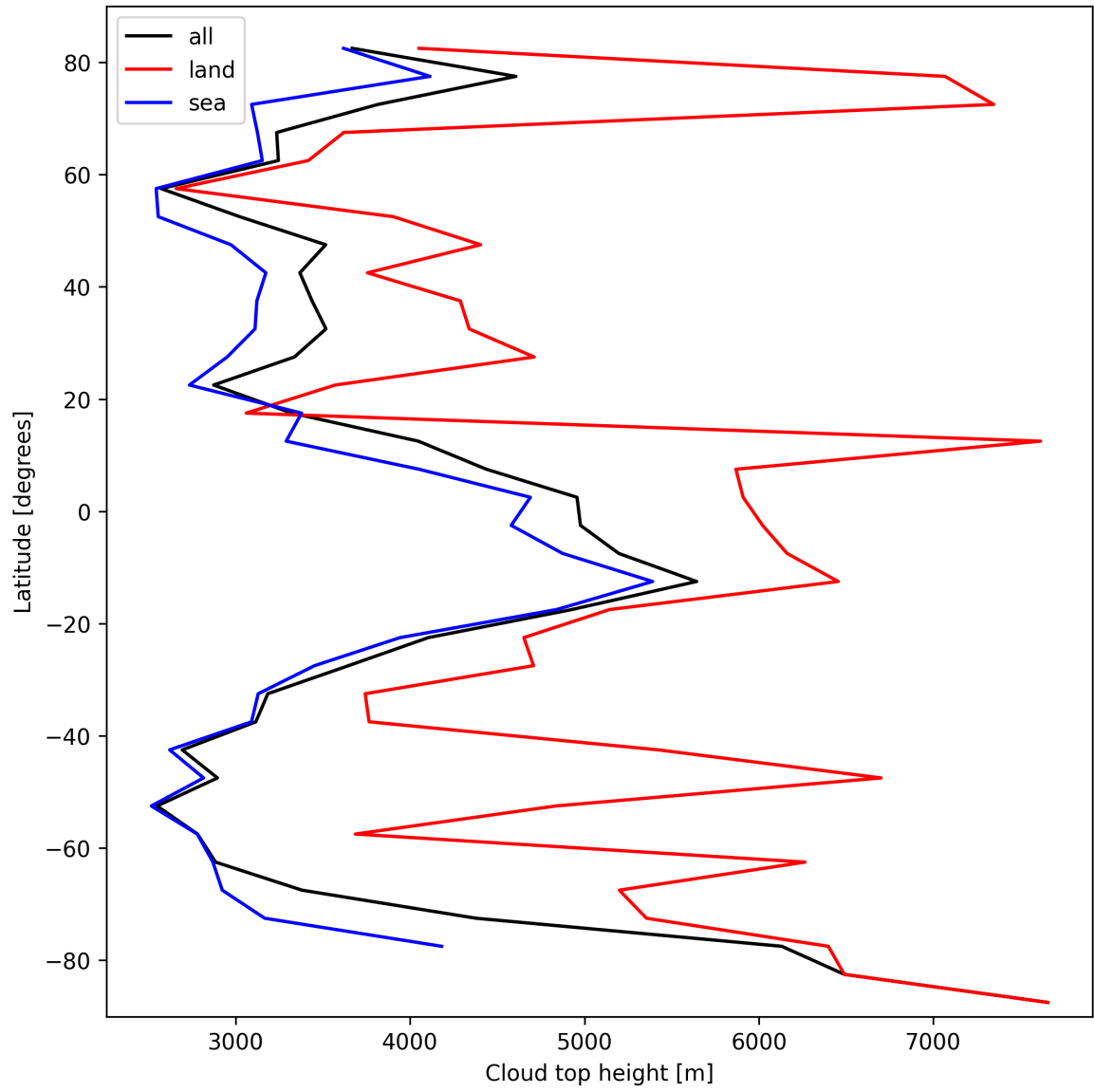
Figure 24: Zonal average of “Cloud top height” for 2025-03-08 to 2025-03-10.
