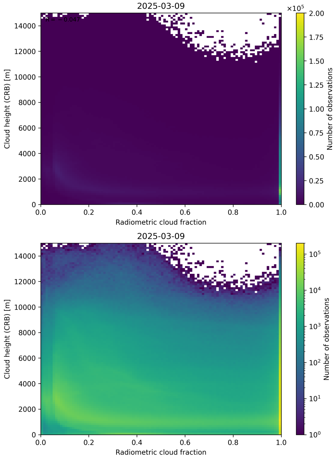
Figure 74: Scatter density plot of “Radiometric cloud fraction” against “Cloud height (CRB)” for 2025-03-08 to 2025-03-10.
