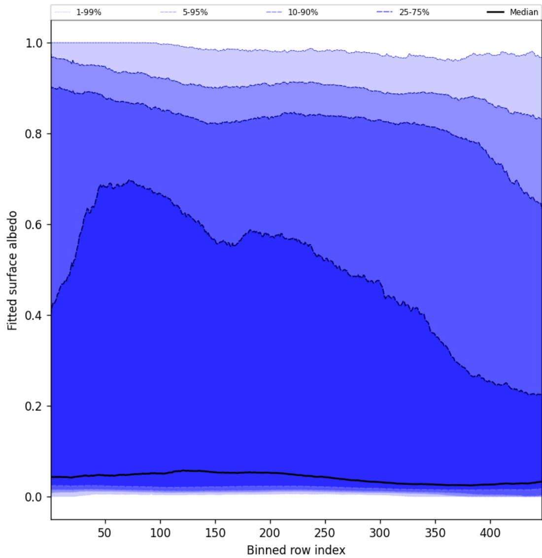
Figure 61: Along track statistics of “Fitted surface albedo” for 2025-03-08 to 2025-03-10
