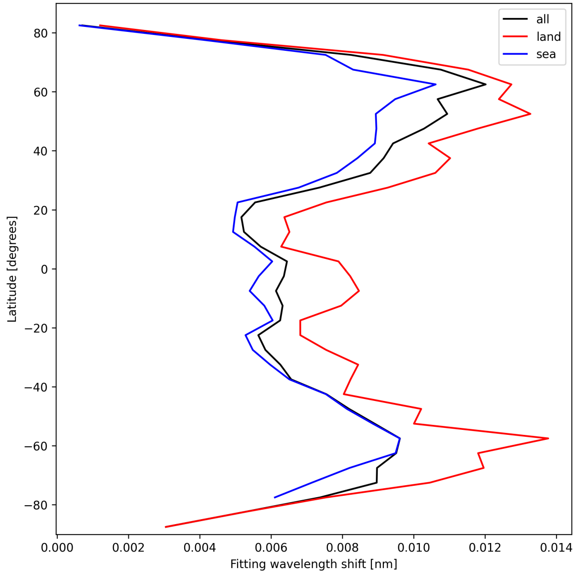
Figure 33: Zonal average of “Fitting wavelength shift” for 2025-03-08 to 2025-03-10.
