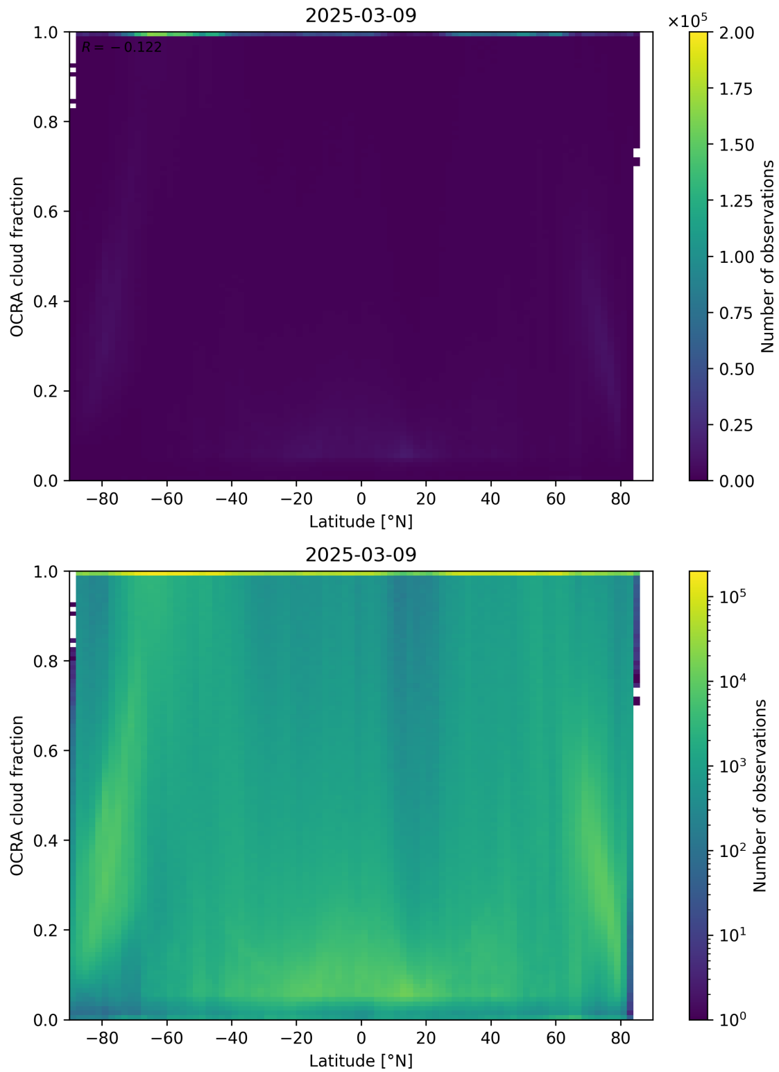
Figure 93: Scatter density plot of “Latitude” against “OCRA cloud fraction” for 2025-03-08 to 2025-03-10.
