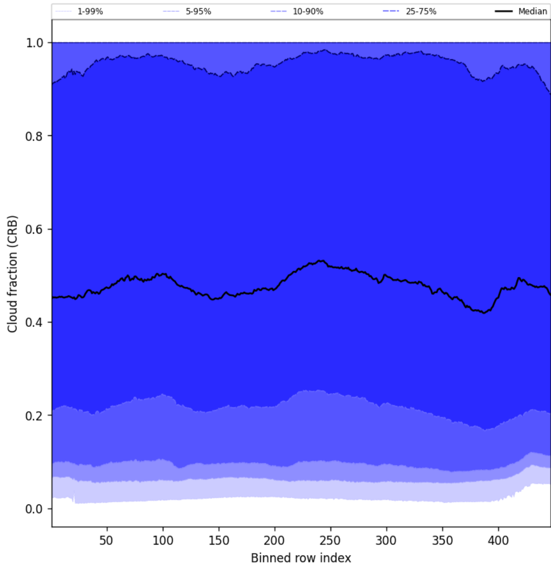
Figure 58: Along track statistics of “Cloud fraction (CRB)” for 2025-03-08 to 2025-03-10
