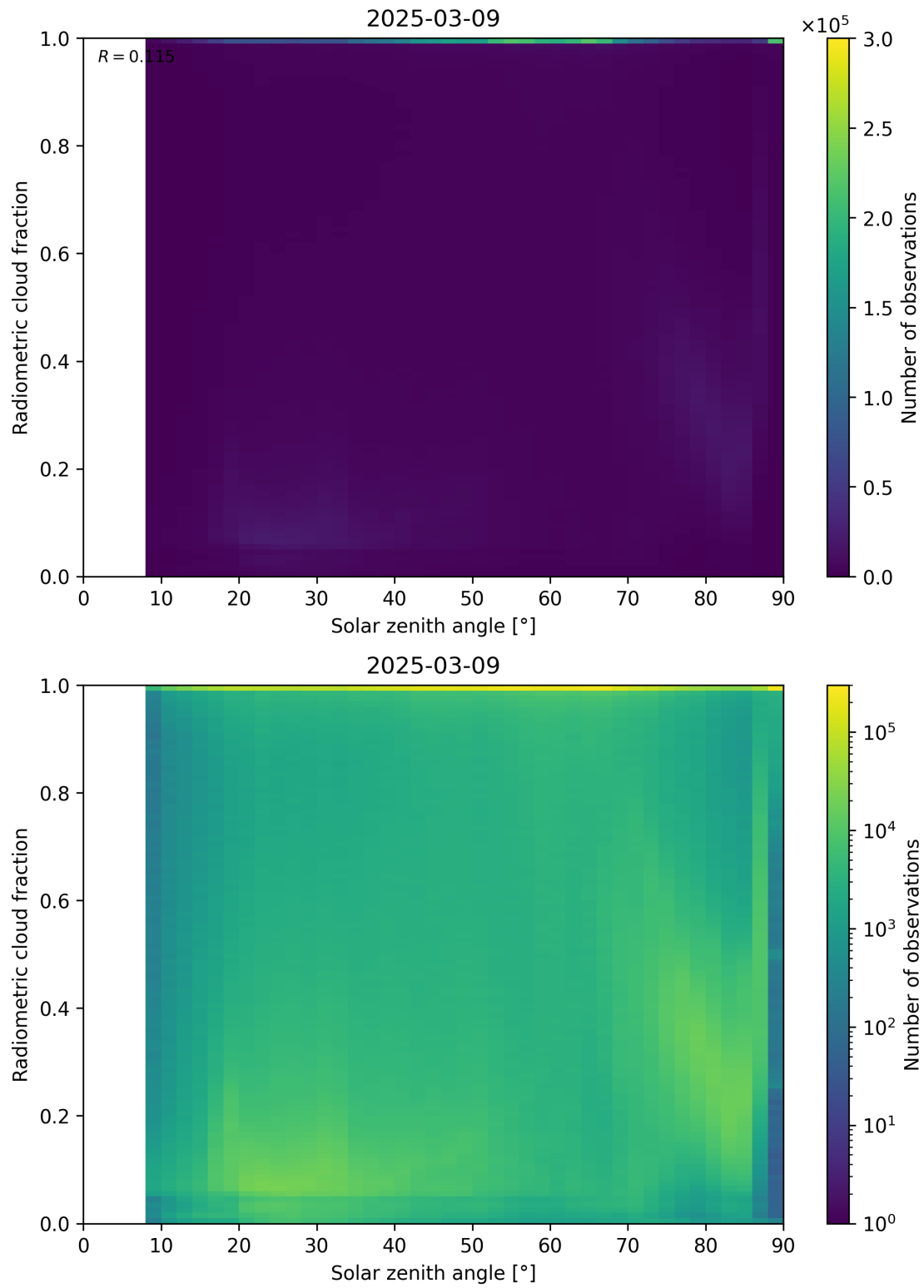
Figure 99: Scatter density plot of “Solar zenith angle” against “Radiometric cloud fraction” for 2025-03-08 to 2025-03-10.
