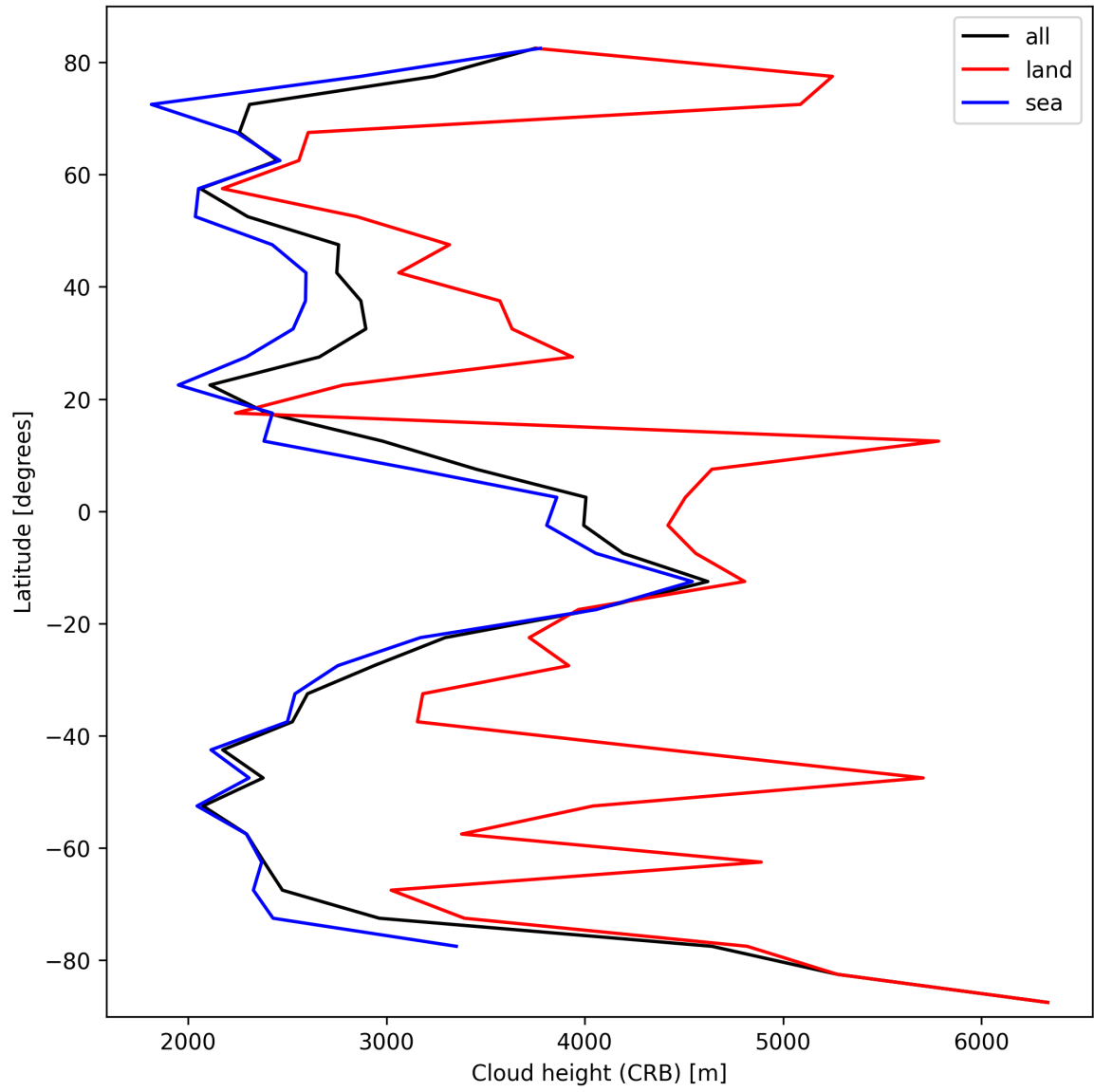
Figure 27: Zonal average of “Cloud height (CRB)” for 2025-03-08 to 2025-03-10.
