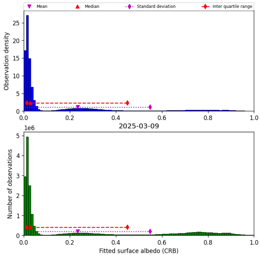
Figure 46: Histogram of “Fitted surface albedo (CRB)” for 2025-03-08 to 2025-03-10
