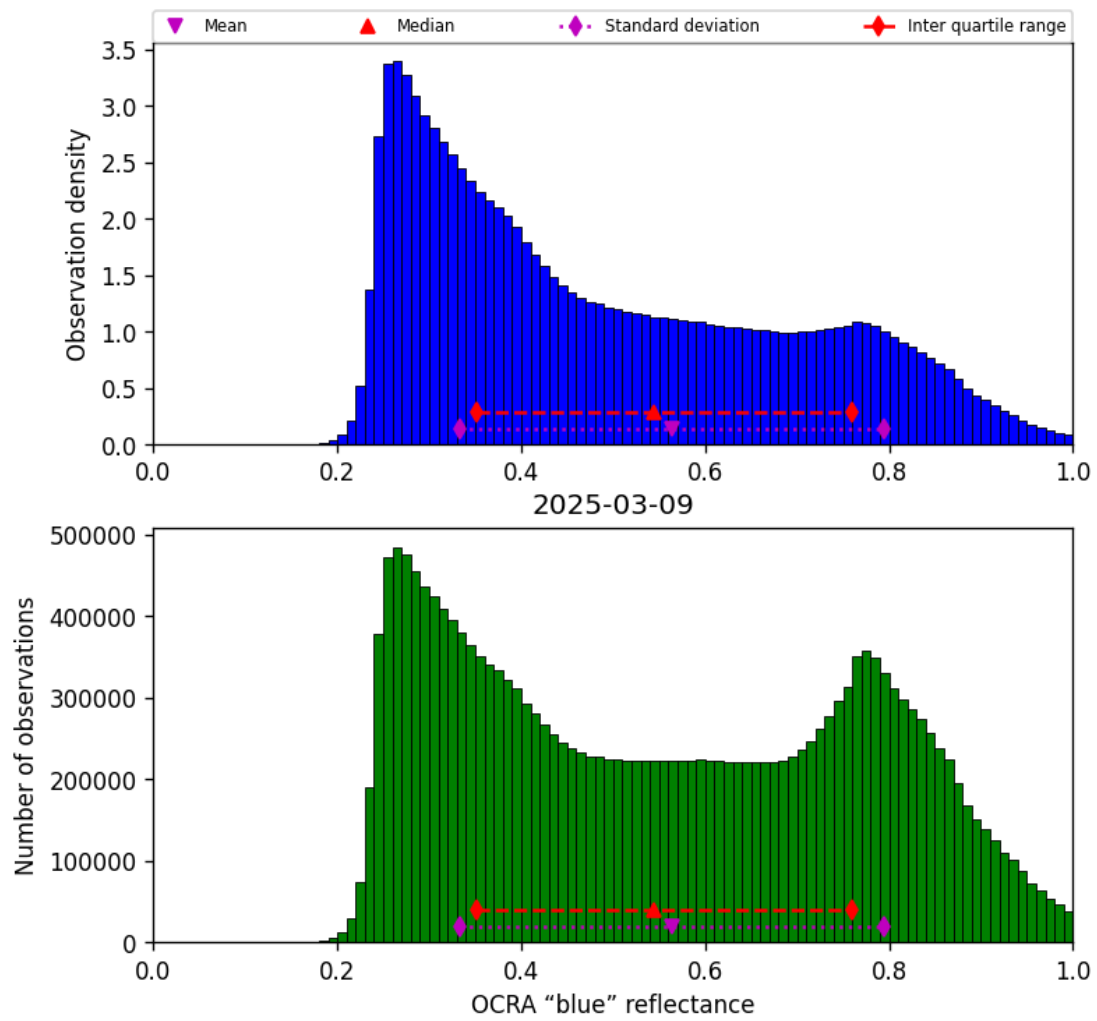
Figure 51: Histogram of “OCRA “blue” reflectance” for 2025-03-08 to 2025-03-10
