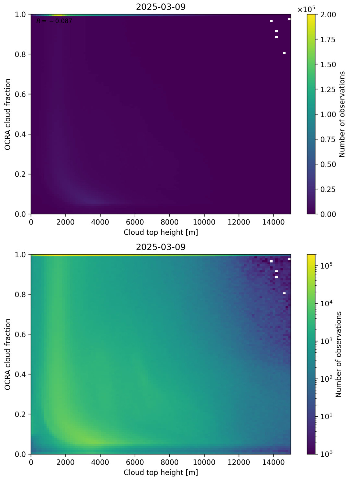
Figure 87: Scatter density plot of “Cloud top height” against “OCRA cloud fraction” for 2025-03-08 to 2025-03-10.
