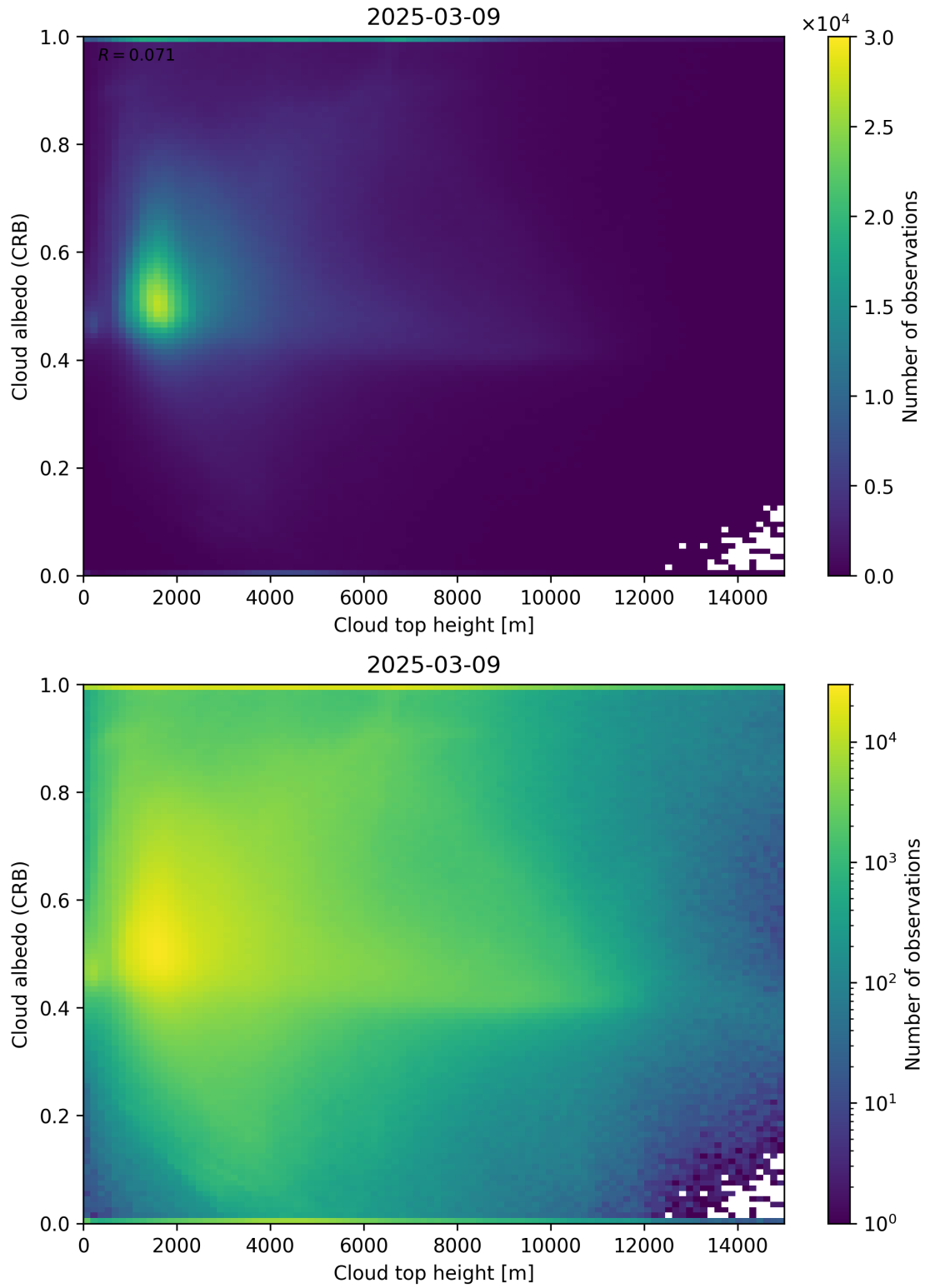
Figure 86: Scatter density plot of “Cloud top height” against “Cloud albedo (CRB)” for 2025-03-08 to 2025-03-10.
