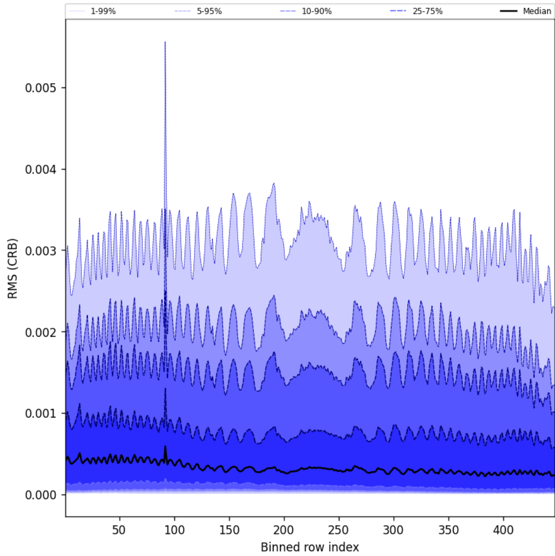
Figure 64: Along track statistics of “RMS (CRB)” for 2025-03-08 to 2025-03-10
