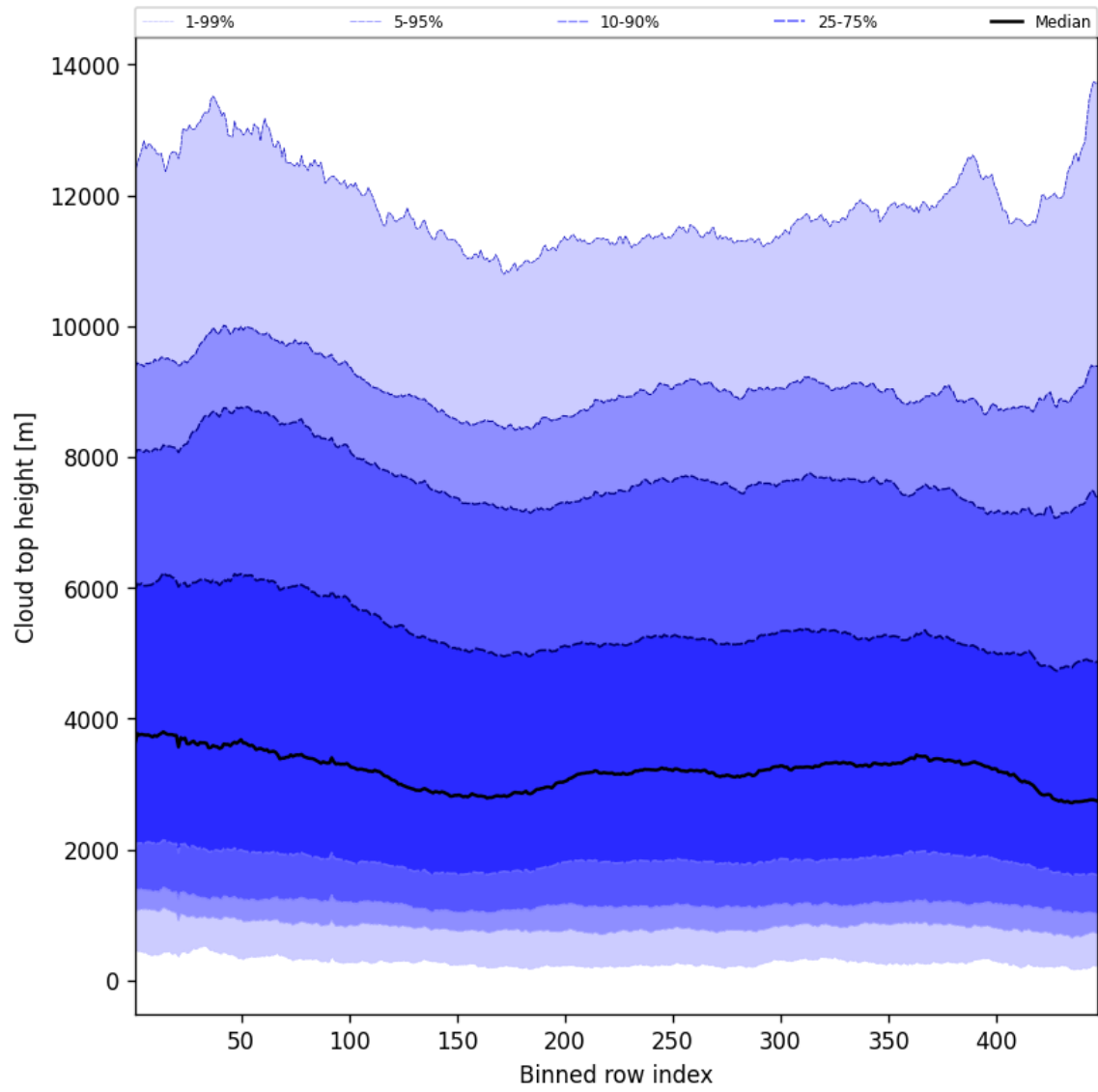
Figure 56: Along track statistics of “Cloud top height” for 2025-03-08 to 2025-03-10
