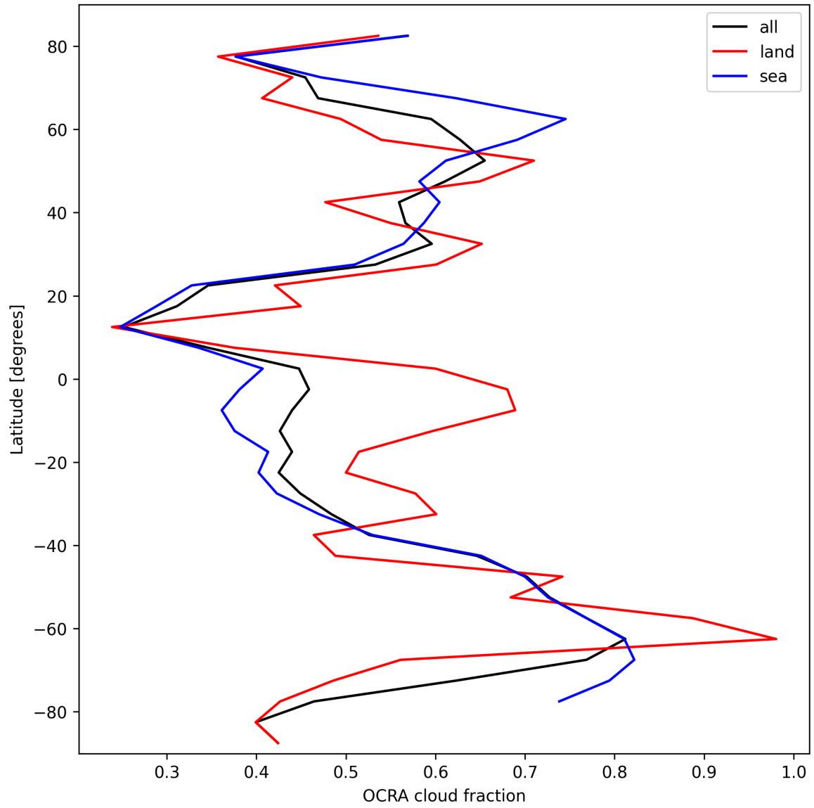
Figure 34: Zonal average of “OCRA cloud fraction” for 2025-03-08 to 2025-03-10.
