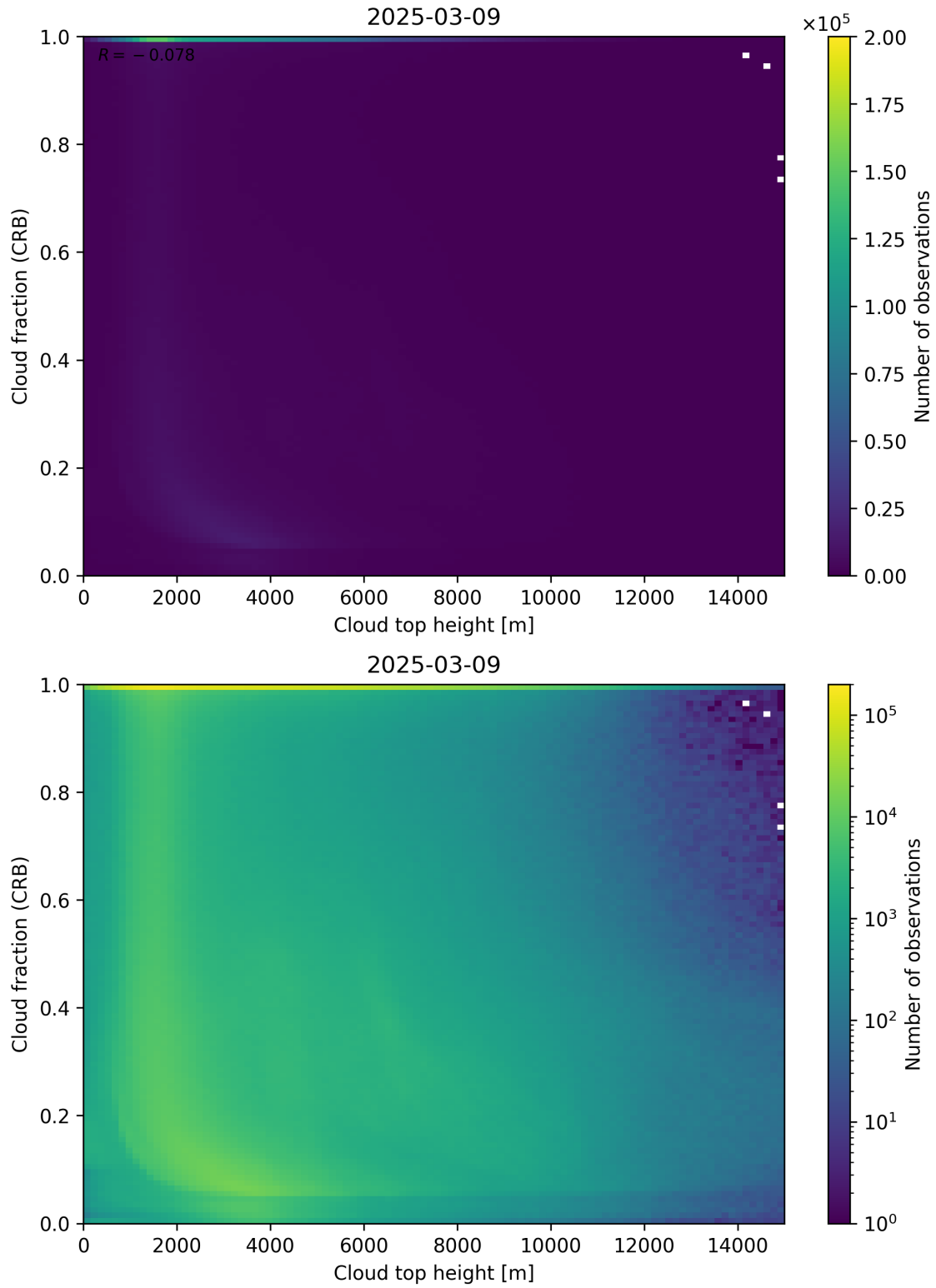
Figure 88: Scatter density plot of “Cloud top height” against “Cloud fraction (CRB)” for 2025-03-08 to 2025-03-10.
