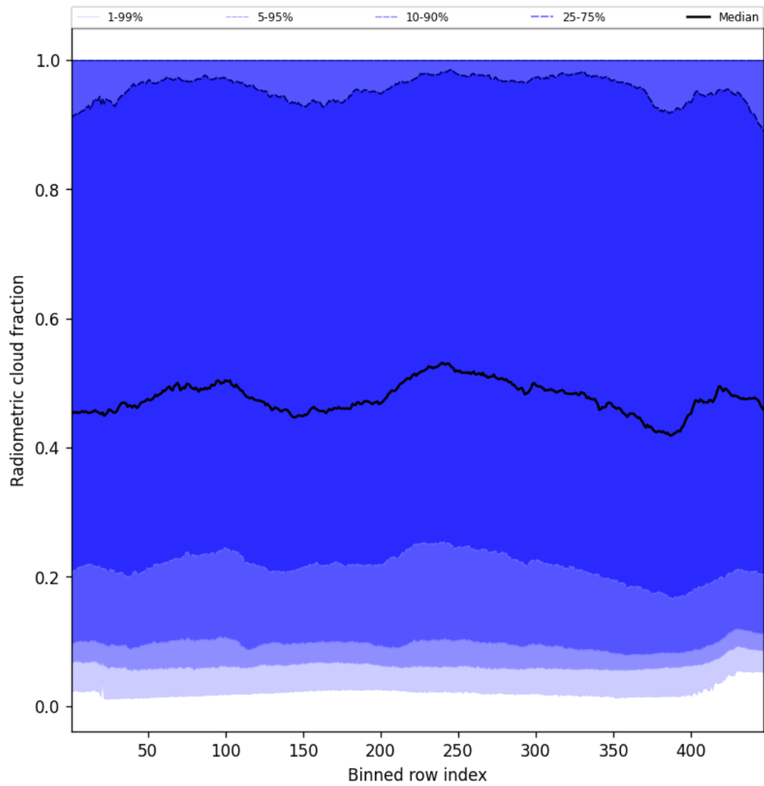
Figure 55: Along track statistics of “Radiometric cloud fraction” for 2025-03-08 to 2025-03-10
