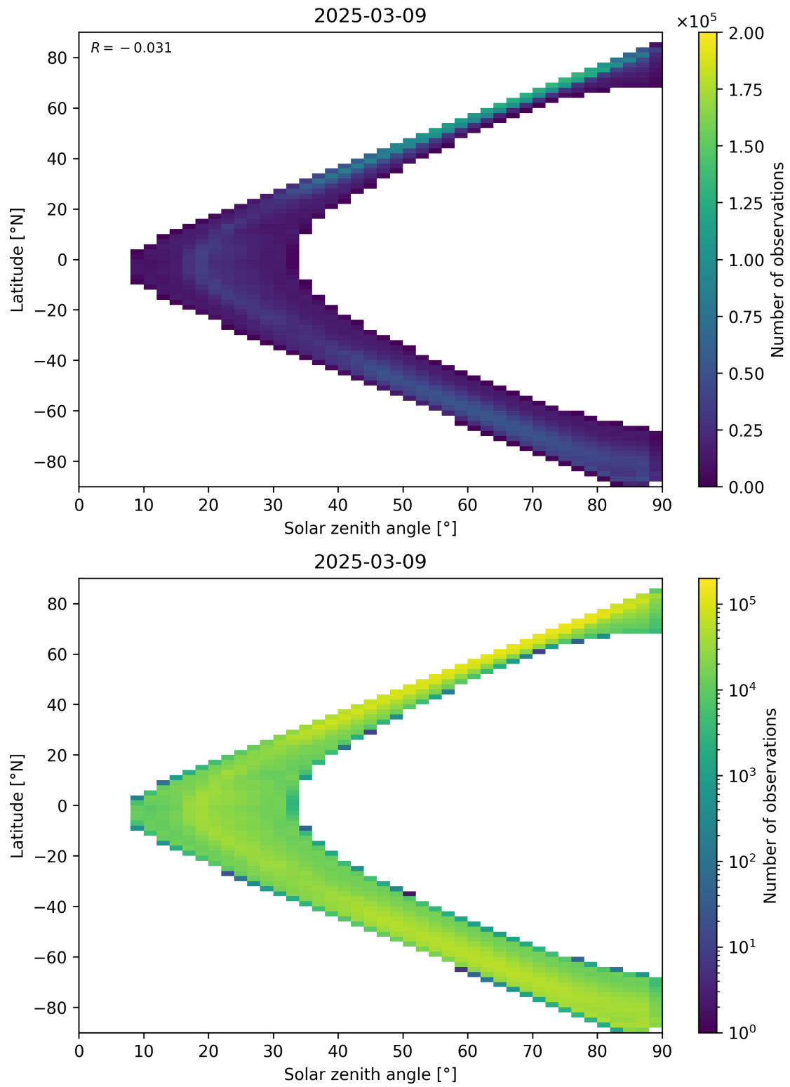
Figure 105: Scatter density plot of “Solar zenith angle” against “Latitude” for 2025-03-08 to 2025-03-10.
