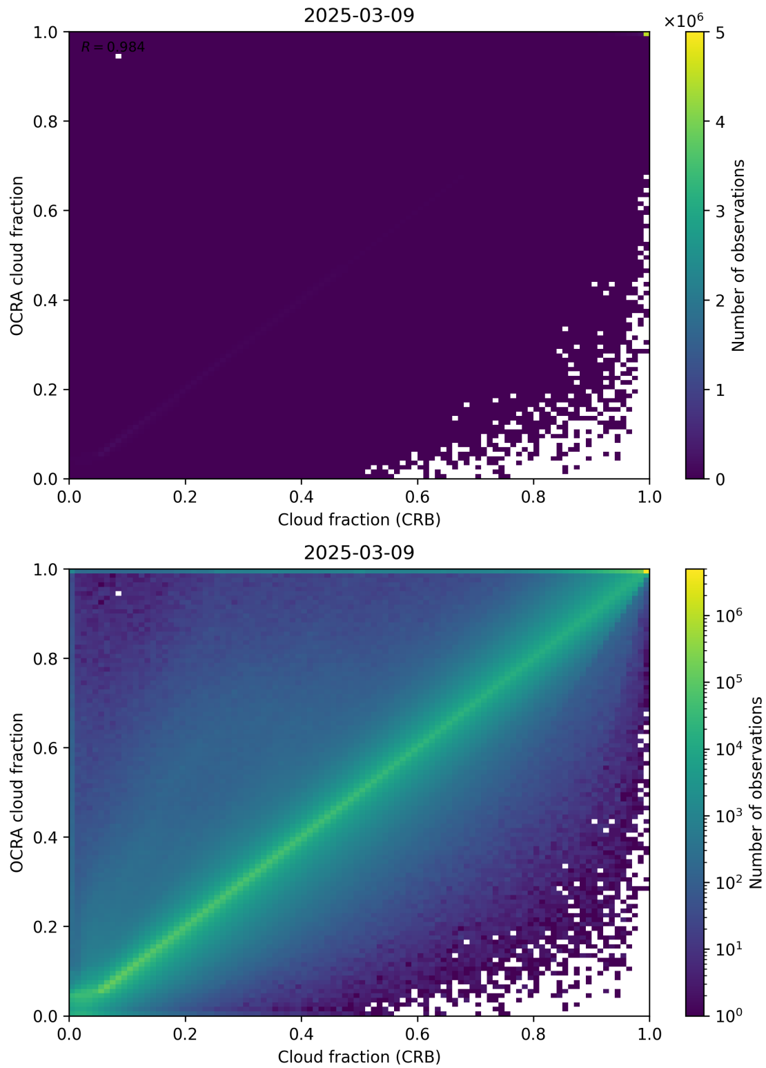
Figure 78: Scatter density plot of “Cloud fraction (CRB)” against “OCRA cloud fraction” for 2025-03-08 to 2025-03-10.
