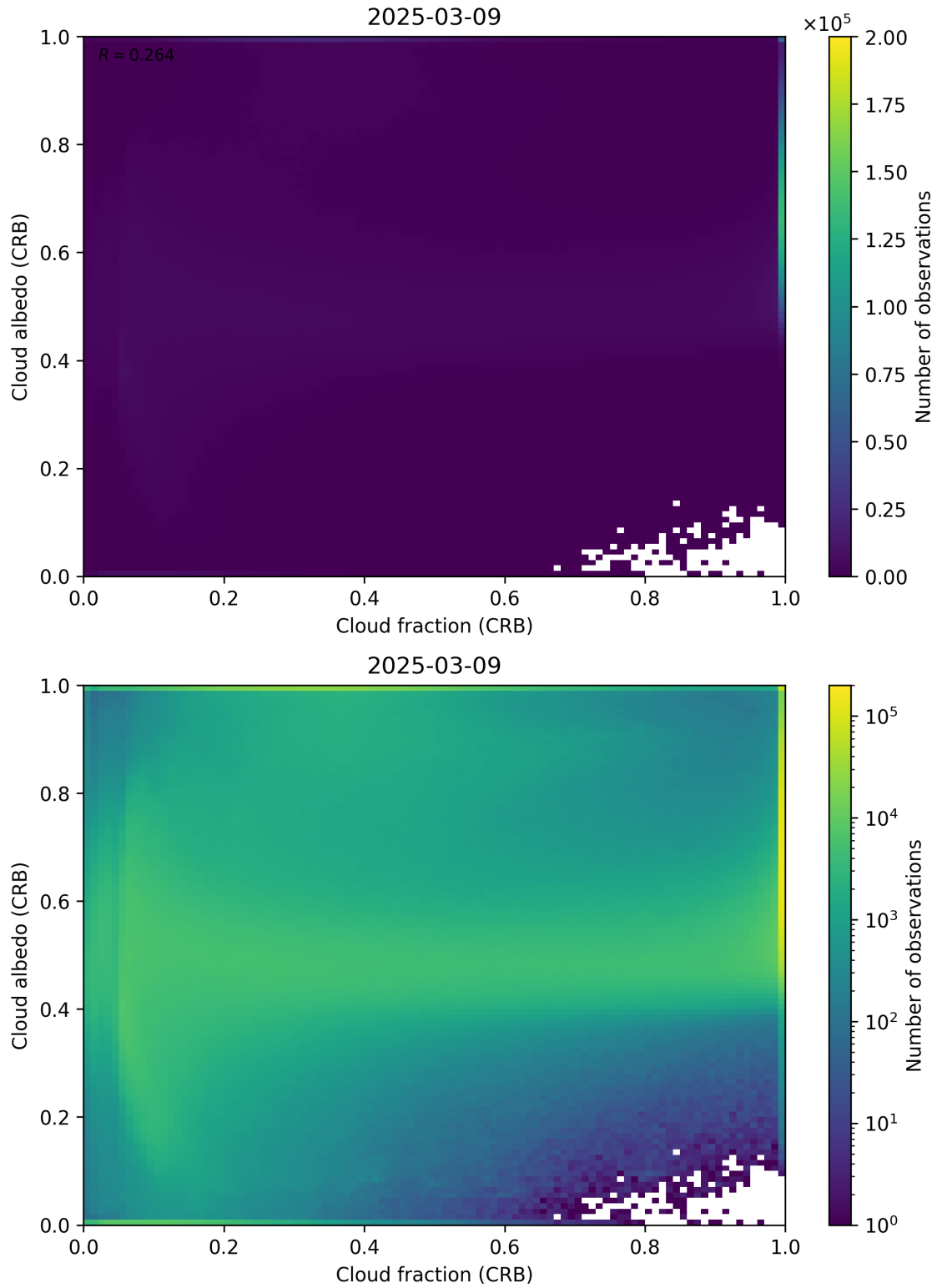
Figure 77: Scatter density plot of “Cloud fraction (CRB)” against “Cloud albedo (CRB)” for 2025-03-08 to 2025-03-10.
