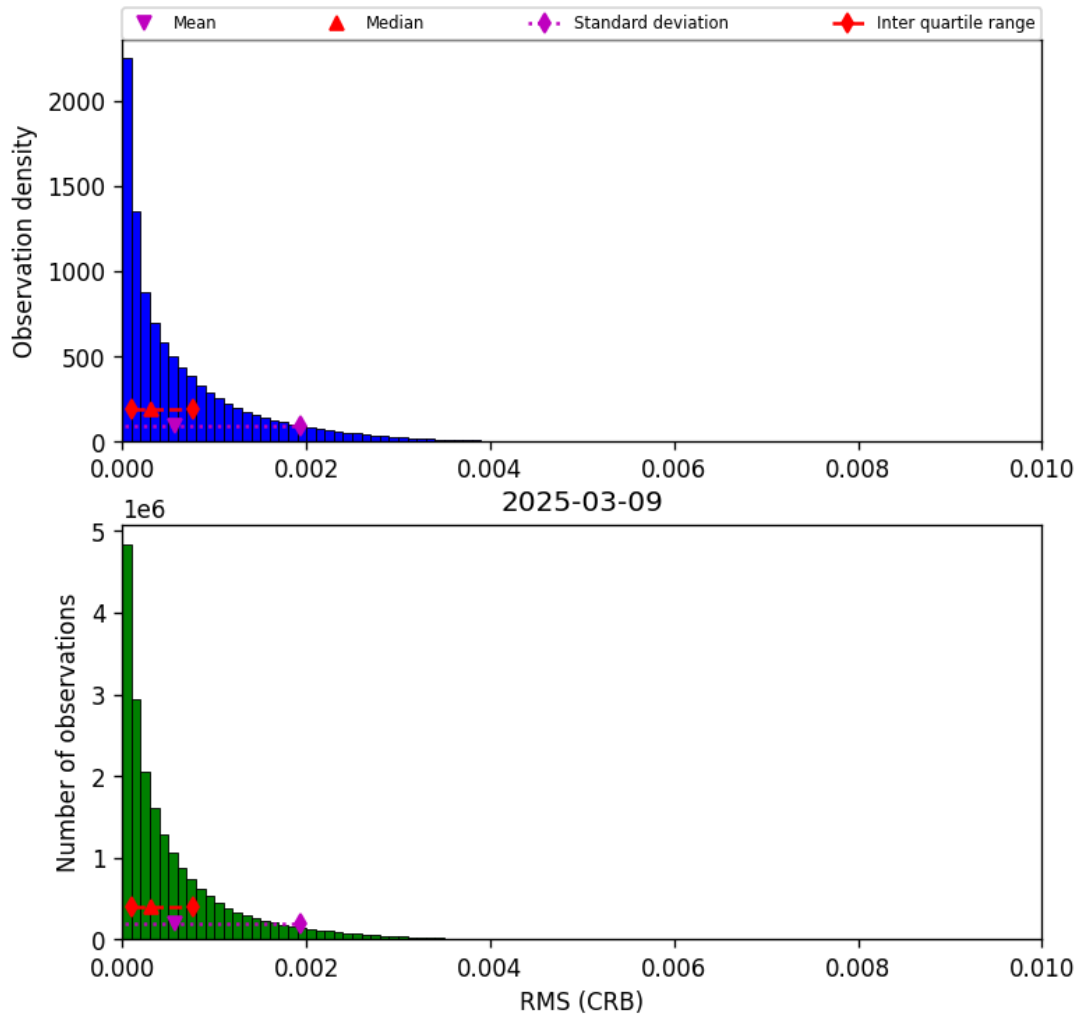
Figure 48: Histogram of “RMS (CRB)” for 2025-03-08 to 2025-03-10
