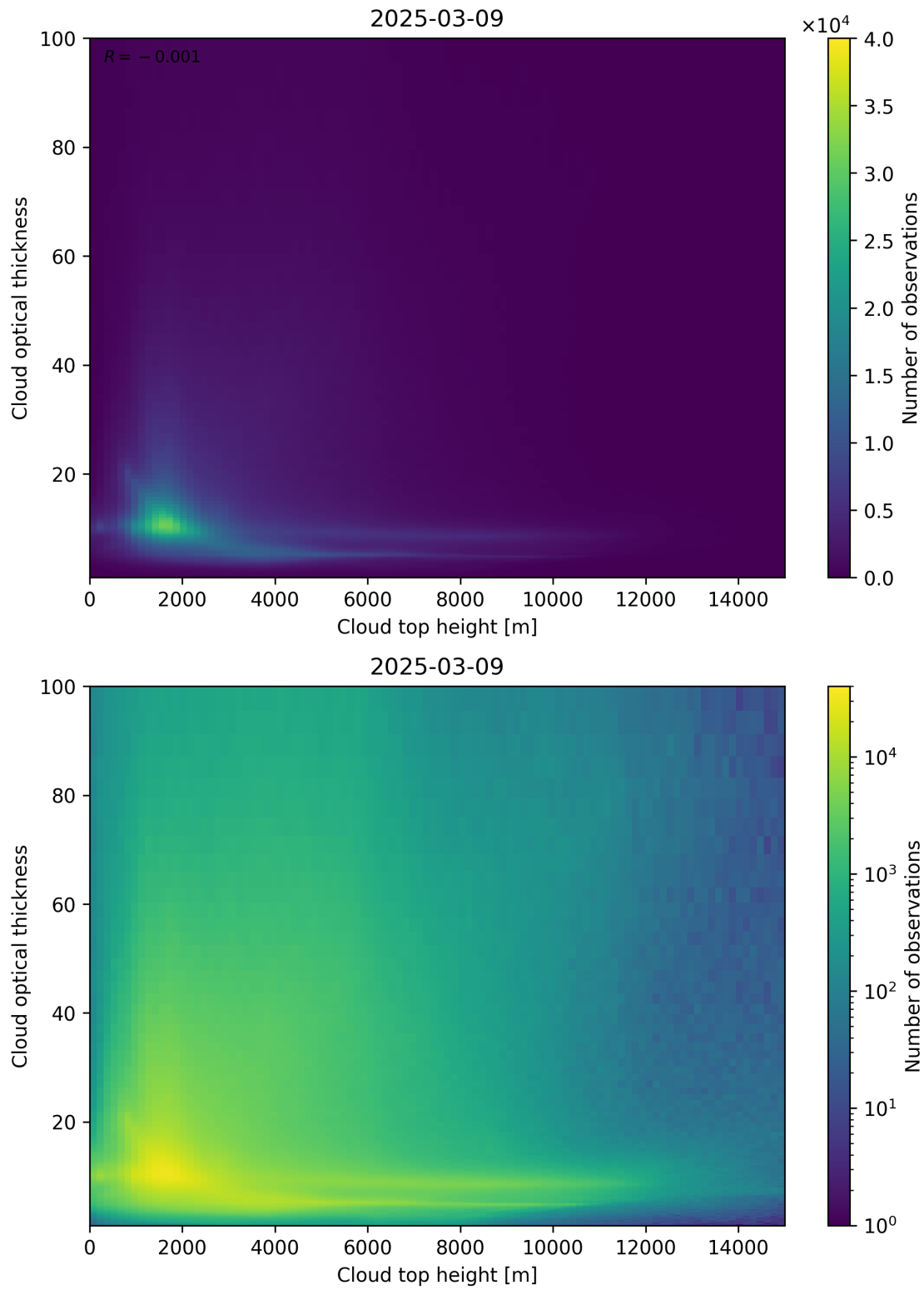
Figure 90: Scatter density plot of “Cloud top height” against “Cloud optical thickness” for 2025-03-08 to 2025-03-10.
