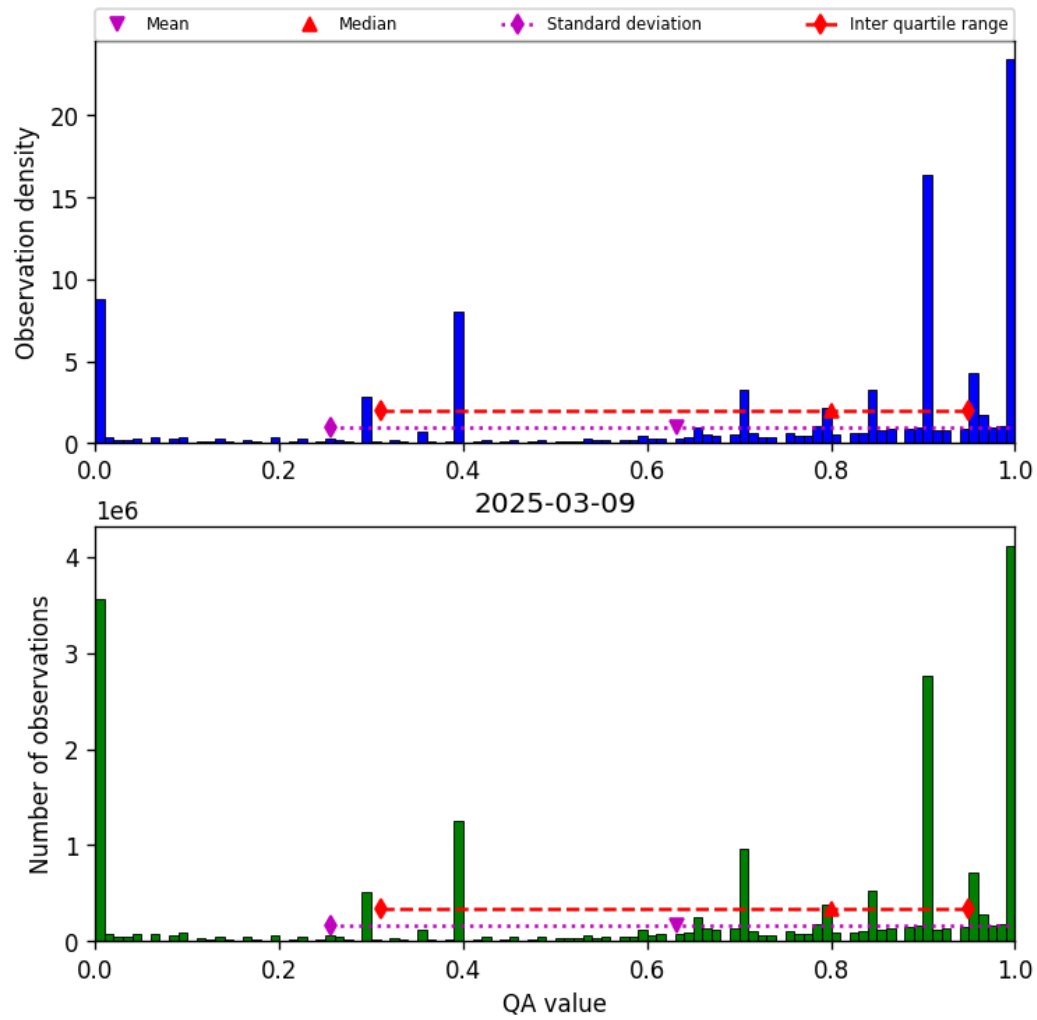
Figure 38: Histogram of “QA value” for 2025-03-08 to 2025-03-10
