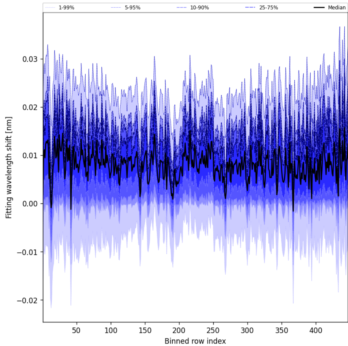
Figure 65: Along track statistics of “Fitting wavelength shift” for 2025-03-08 to 2025-03-10
