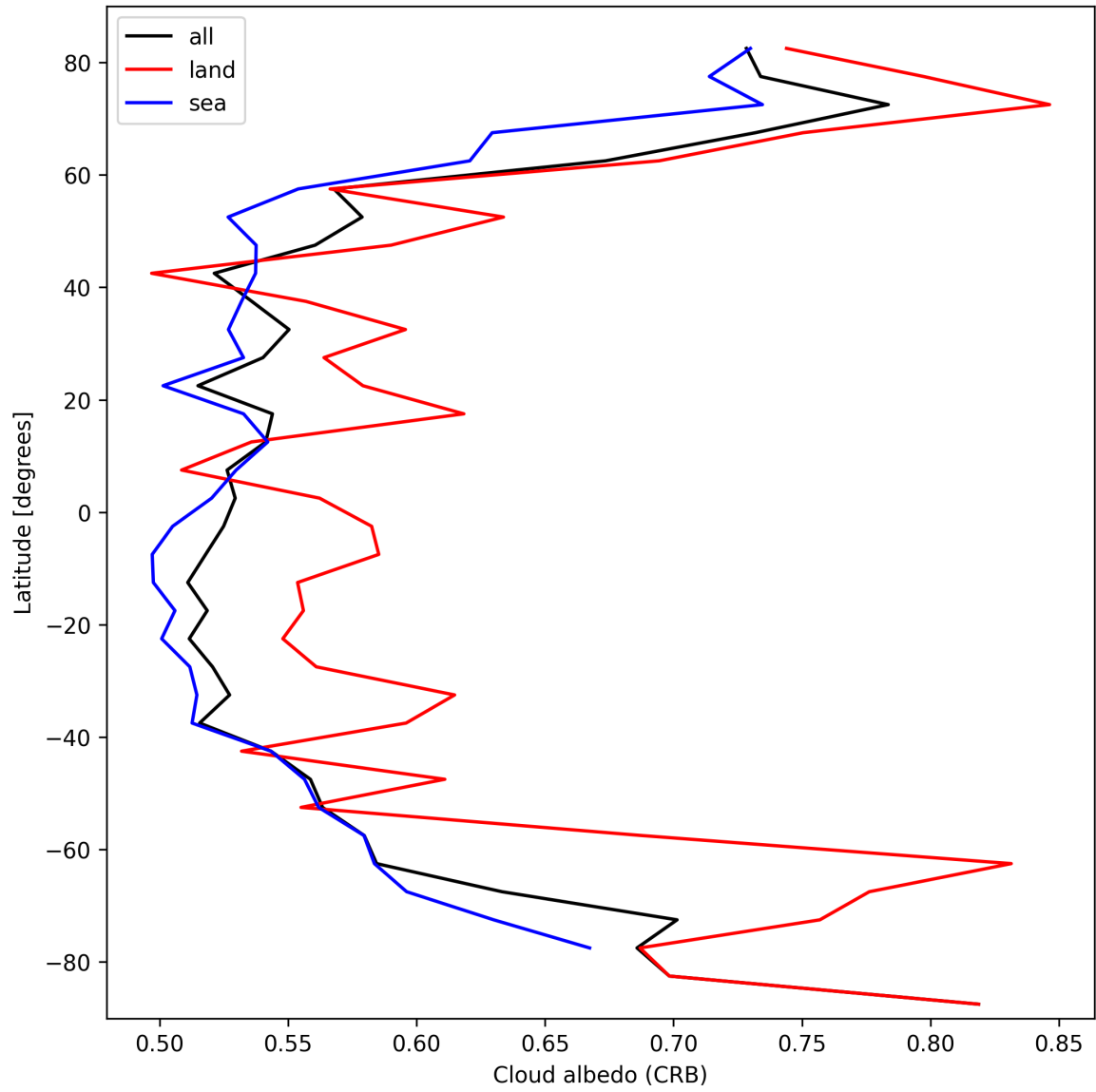
Figure 28: Zonal average of “Cloud albedo (CRB)” for 2025-03-08 to 2025-03-10.
