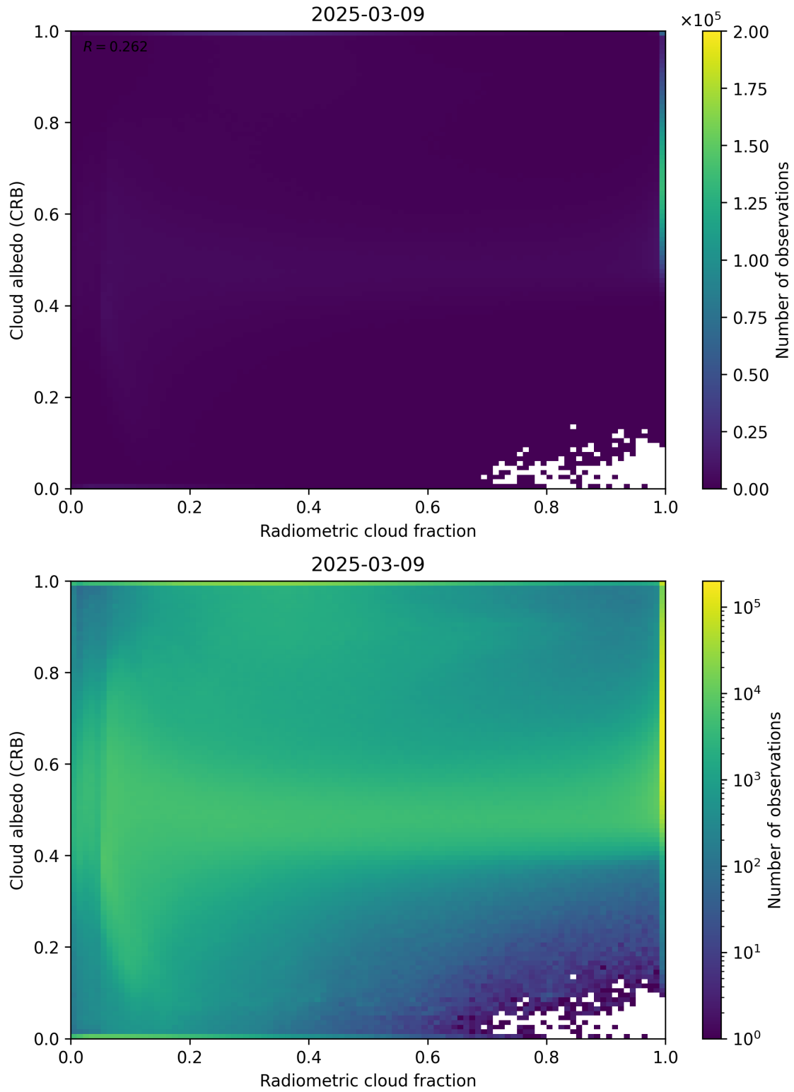
Figure 71: Scatter density plot of “Radiometric cloud fraction” against “Cloud albedo (CRB)” for 2025-03-08 to 2025-03-10.
