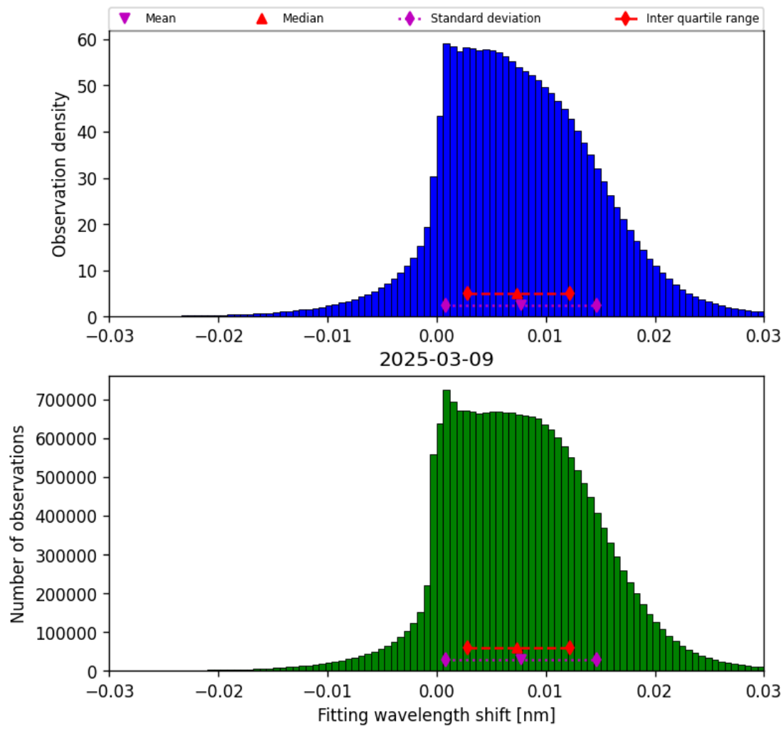
Figure 49: Histogram of “Fitting wavelength shift” for 2025-03-08 to 2025-03-10
