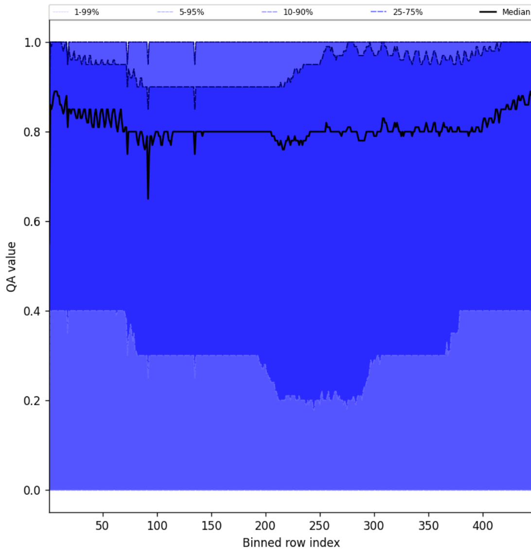
Figure 54: Along track statistics of “QA value” for 2025-03-08 to 2025-03-10
