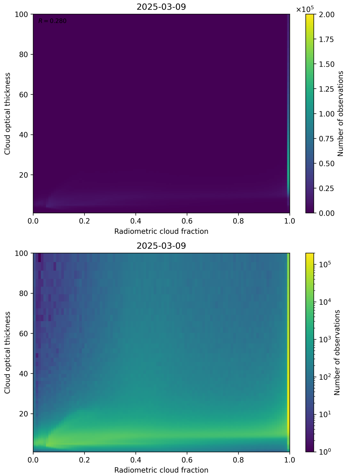
Figure 75: Scatter density plot of “Radiometric cloud fraction” against “Cloud optical thickness” for 2025-03-08 to 2025-03-10.
