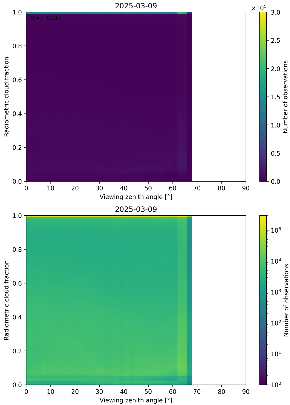
Figure 107: Scatter density plot of “Viewing zenith angle” against “Radiometric cloud fraction” for 2025-03-08 to 2025-03-10.
