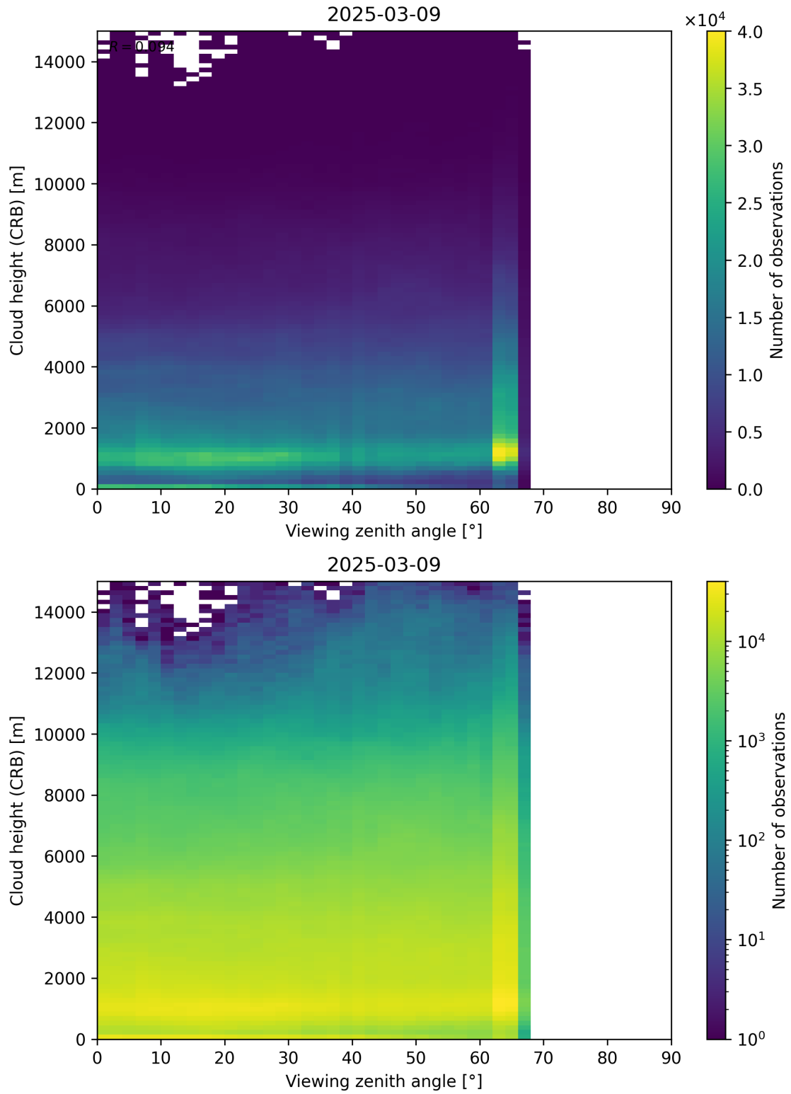
Figure 110: Scatter density plot of “Viewing zenith angle” against “Cloud height (CRB)” for 2025-03-08 to 2025-03-10.
