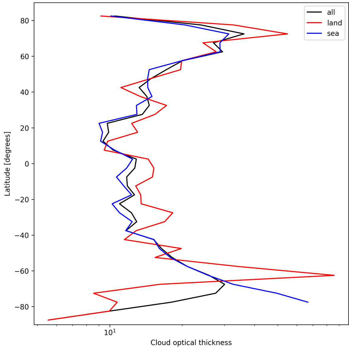
Figure 25: Zonal average of “Cloud optical thickness” for 2025-03-08 to 2025-03-10.
