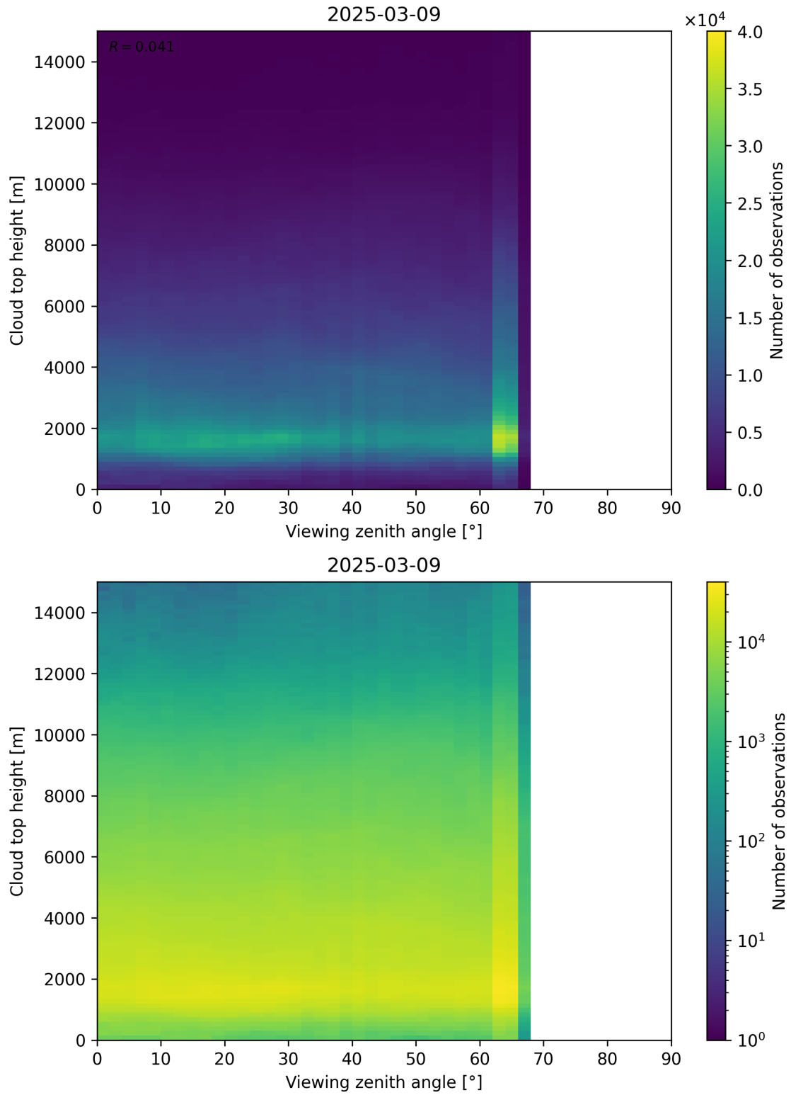
Figure 112: Scatter density plot of “Viewing zenith angle” against “Cloud top height” for 2025-03-08 to 2025-03-10.
