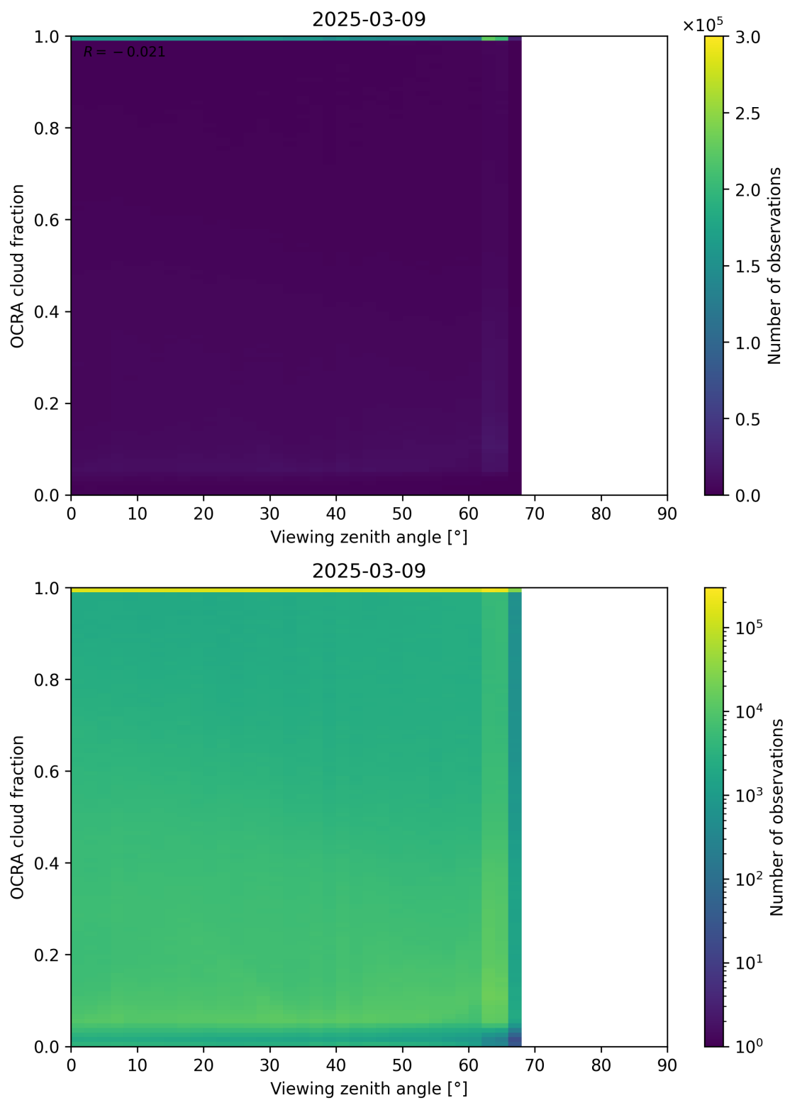
Figure 108: Scatter density plot of “Viewing zenith angle” against “OCRA cloud fraction” for 2025-03-08 to 2025-03-10.
