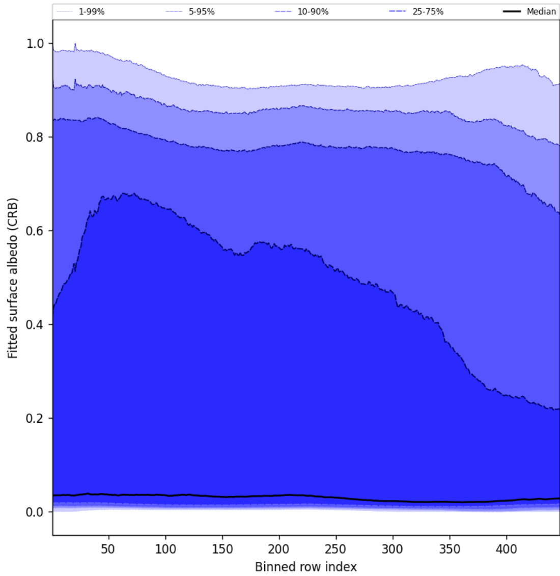
Figure 62: Along track statistics of “Fitted surface albedo (CRB)” for 2025-03-08 to 2025-03-10
