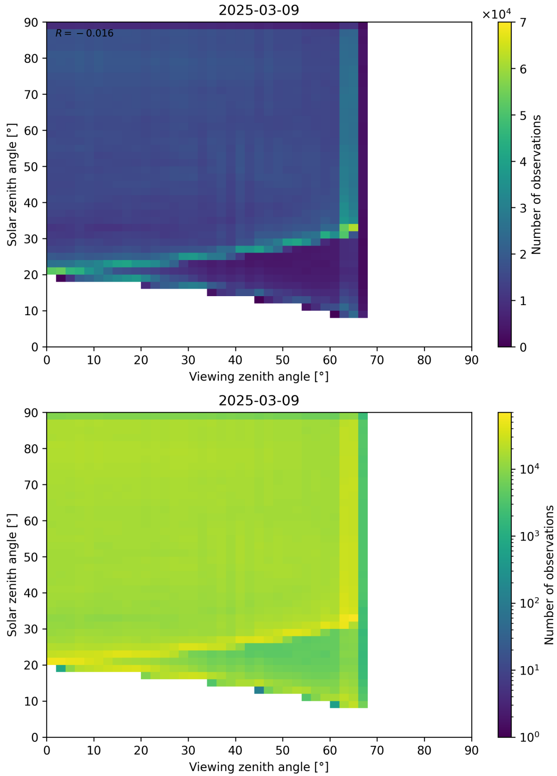
Figure 114: Scatter density plot of “Viewing zenith angle” against “Solar zenith angle” for 2025-03-08 to 2025-03-10.
