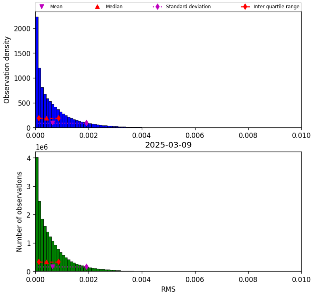
Figure 47: Histogram of “RMS” for 2025-03-08 to 2025-03-10
