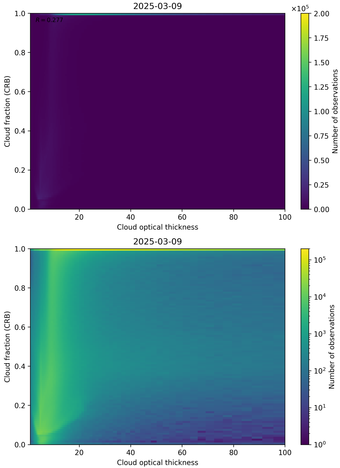
Figure 84: Scatter density plot of “Cloud optical thickness” against “Cloud fraction (CRB)” for 2025-03-08 to 2025-03-10.
