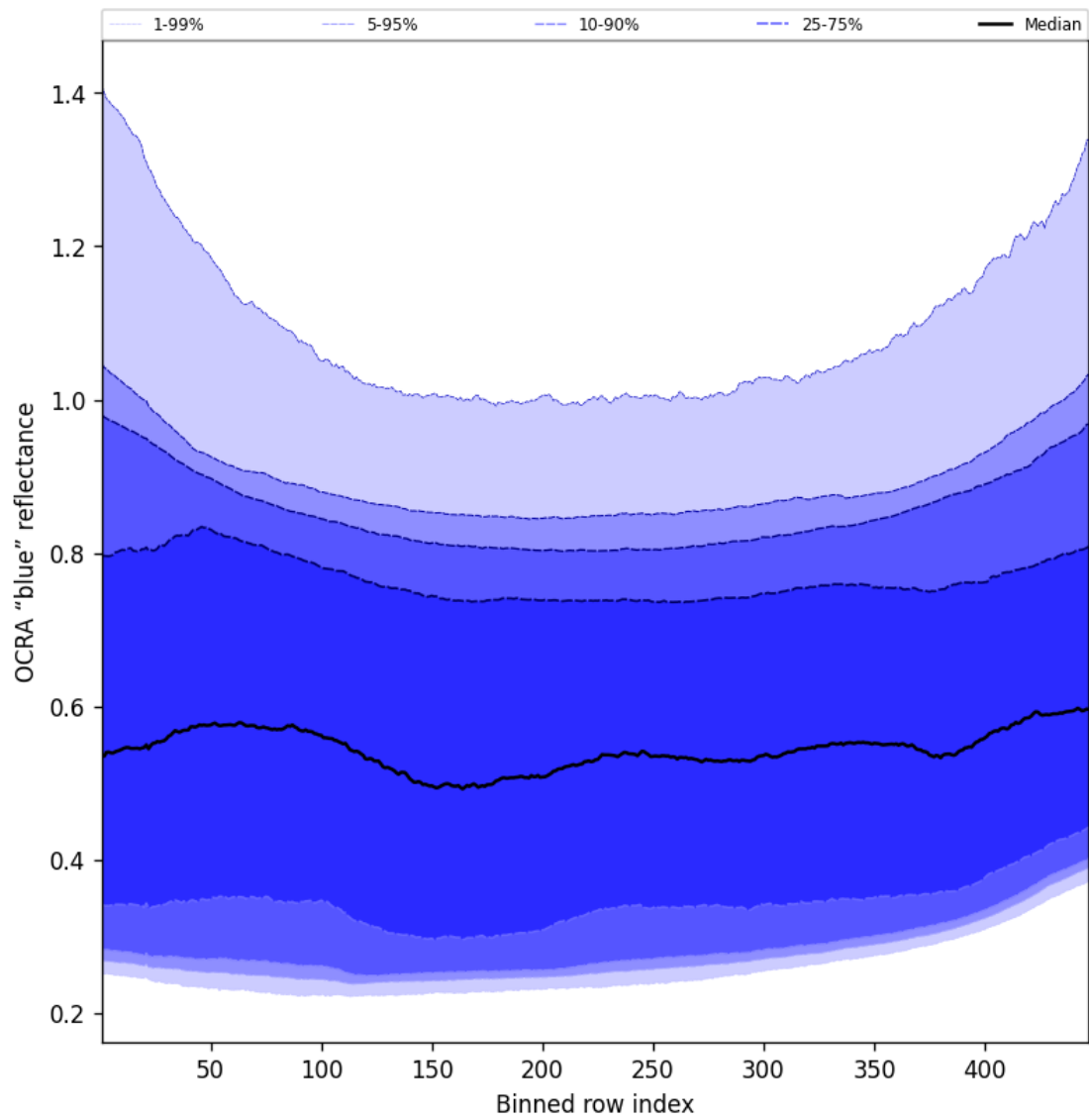
Figure 67: Along track statistics of “OCRA “blue” reflectance” for 2025-03-08 to 2025-03-10
