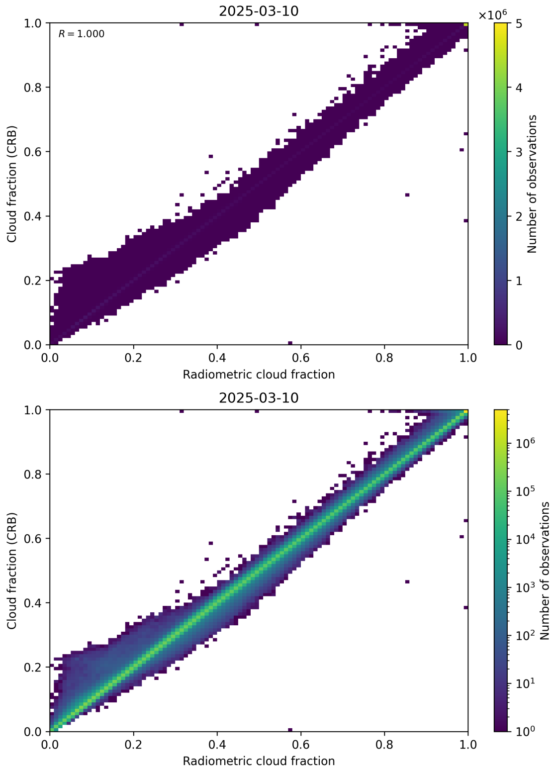
Figure 73: Scatter density plot of “Radiometric cloud fraction” against “Cloud fraction (CRB)” for 2025-03-09 to 2025-03-11.
