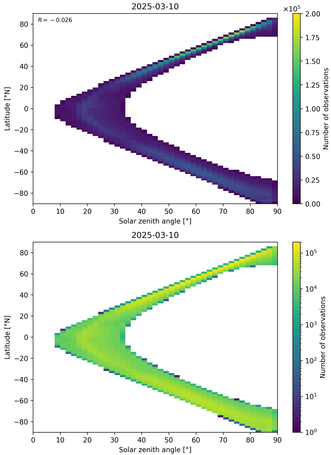
Figure 105: Scatter density plot of “Solar zenith angle” against “Latitude” for 2025-03-09 to 2025-03-11.
