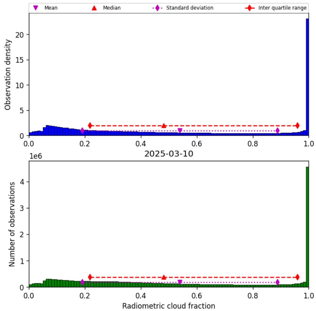
Figure 39: Histogram of “Radiometric cloud fraction” for 2025-03-09 to 2025-03-11
