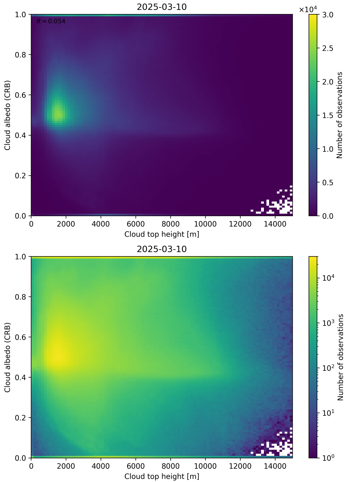
Figure 86: Scatter density plot of “Cloud top height” against “Cloud albedo (CRB)” for 2025-03-09 to 2025-03-11.
