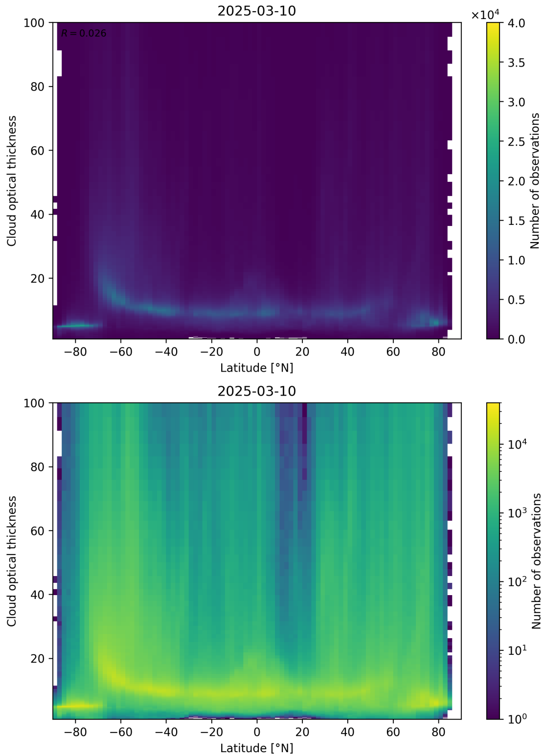
Figure 96: Scatter density plot of “Latitude” against “Cloud optical thickness” for 2025-03-09 to 2025-03-11.
