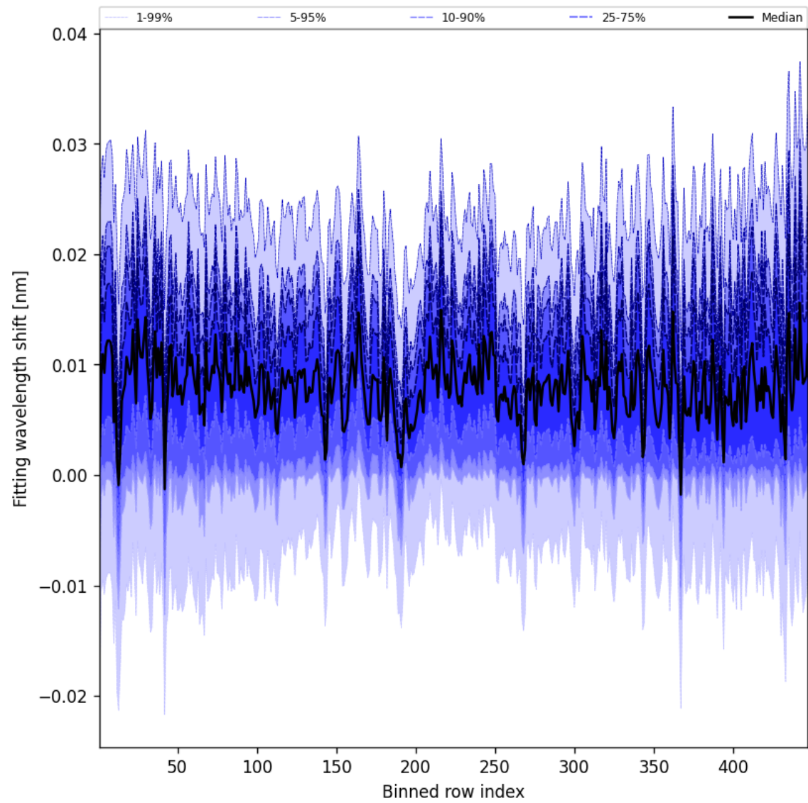
Figure 65: Along track statistics of “Fitting wavelength shift” for 2025-03-09 to 2025-03-11
