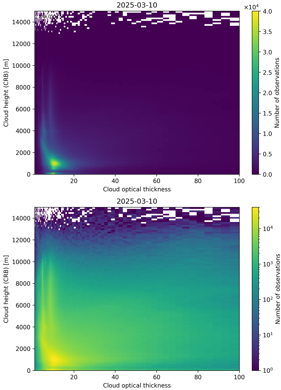
Figure 85: Scatter density plot of “Cloud optical thickness” against “Cloud height (CRB)” for 2025-03-09 to 2025-03-11.
