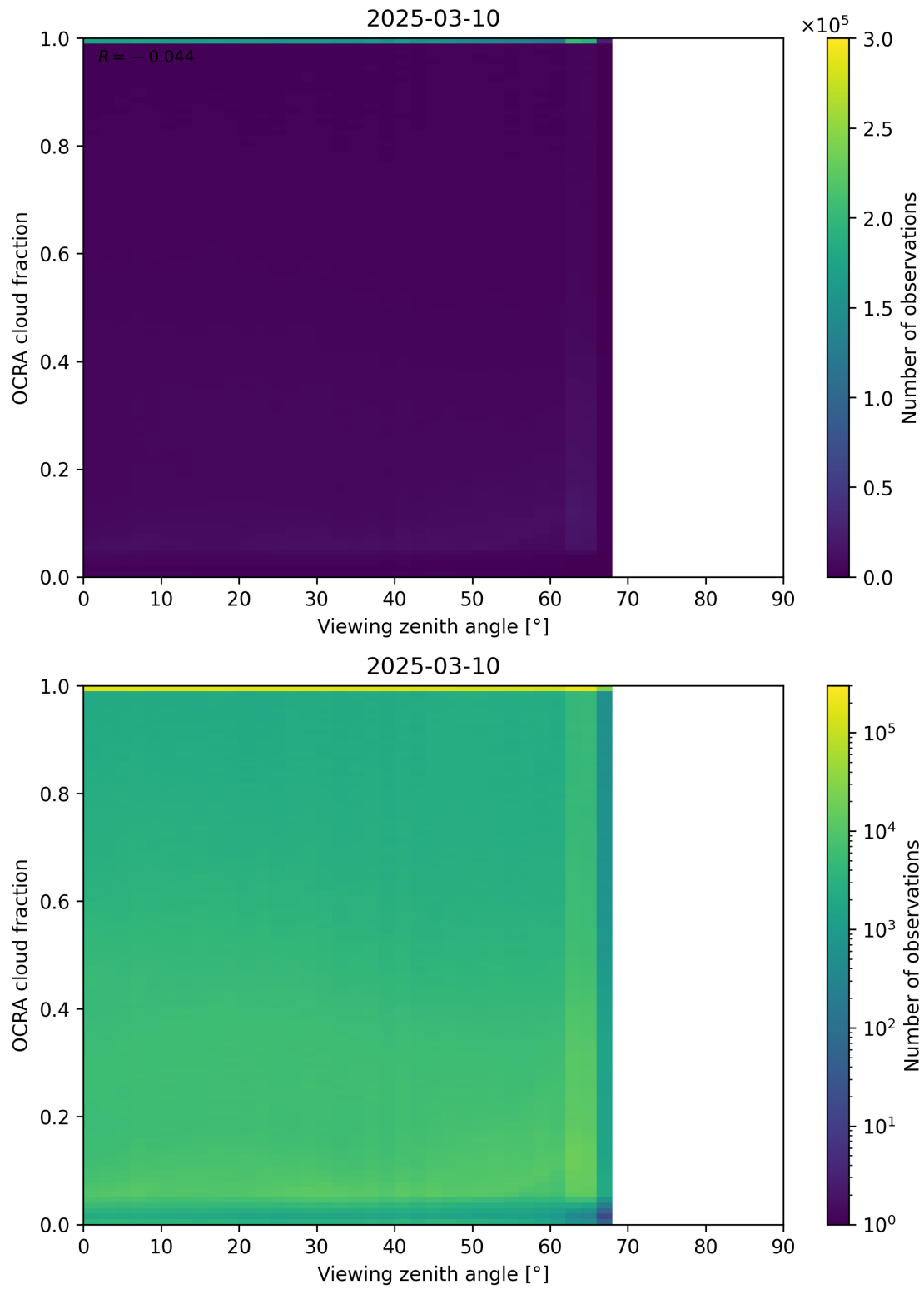
Figure 108: Scatter density plot of “Viewing zenith angle” against “OCRA cloud fraction” for 2025-03-09 to 2025-03-11.
