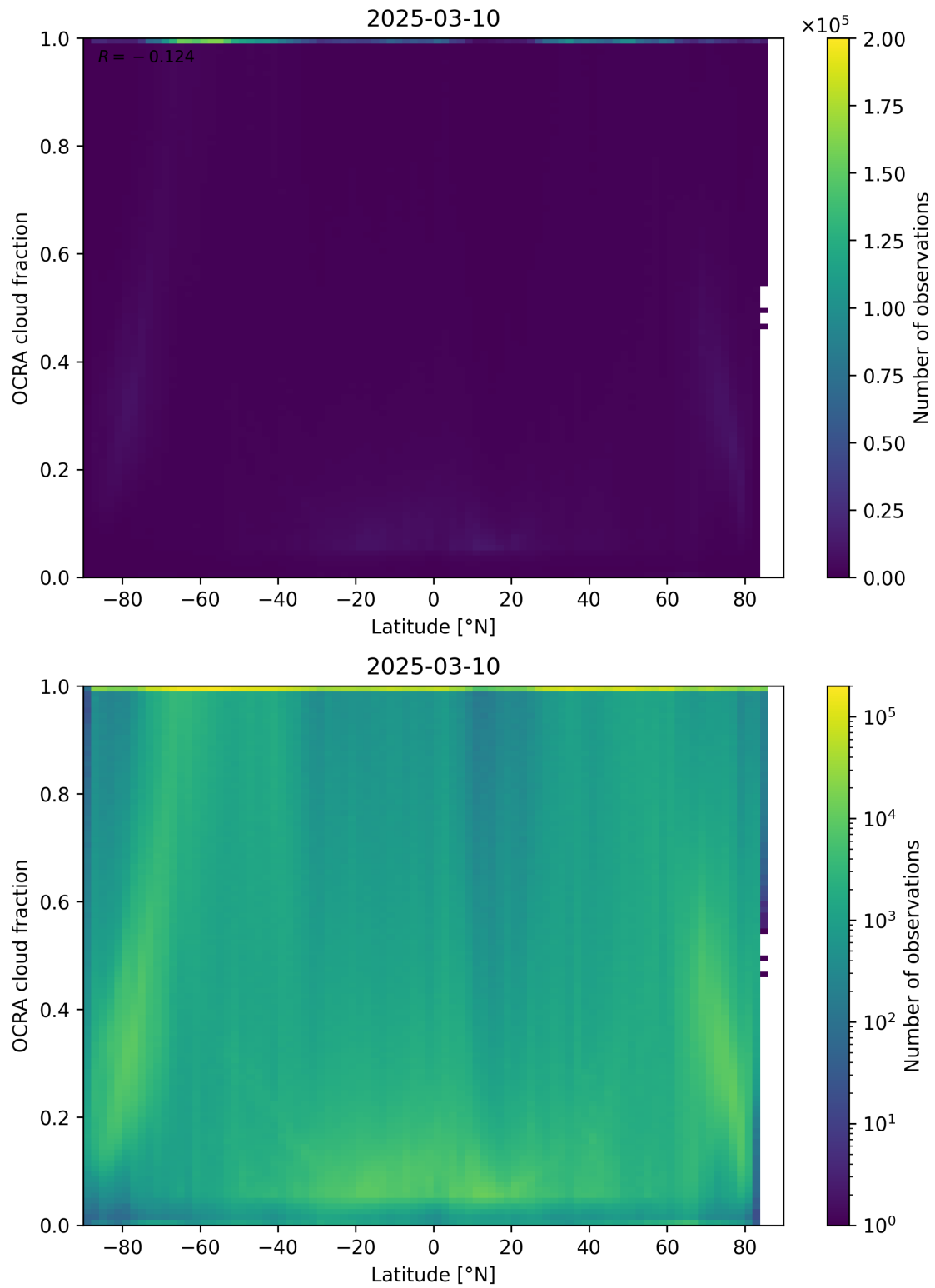
Figure 93: Scatter density plot of “Latitude” against “OCRA cloud fraction” for 2025-03-09 to 2025-03-11.
