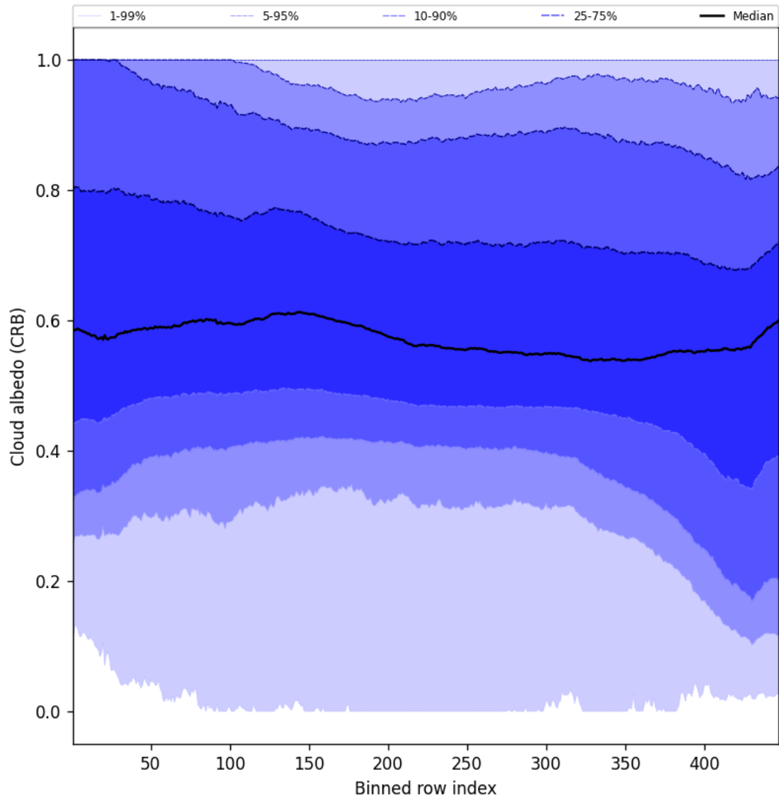
Figure 60: Along track statistics of “Cloud albedo (CRB)” for 2025-03-09 to 2025-03-11
