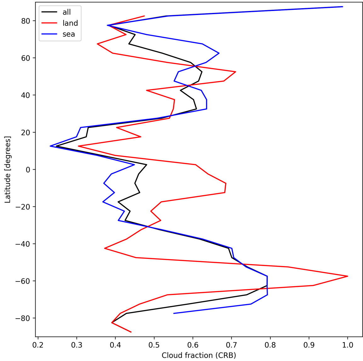
Figure 26: Zonal average of “Cloud fraction (CRB)” for 2025-03-09 to 2025-03-11.
