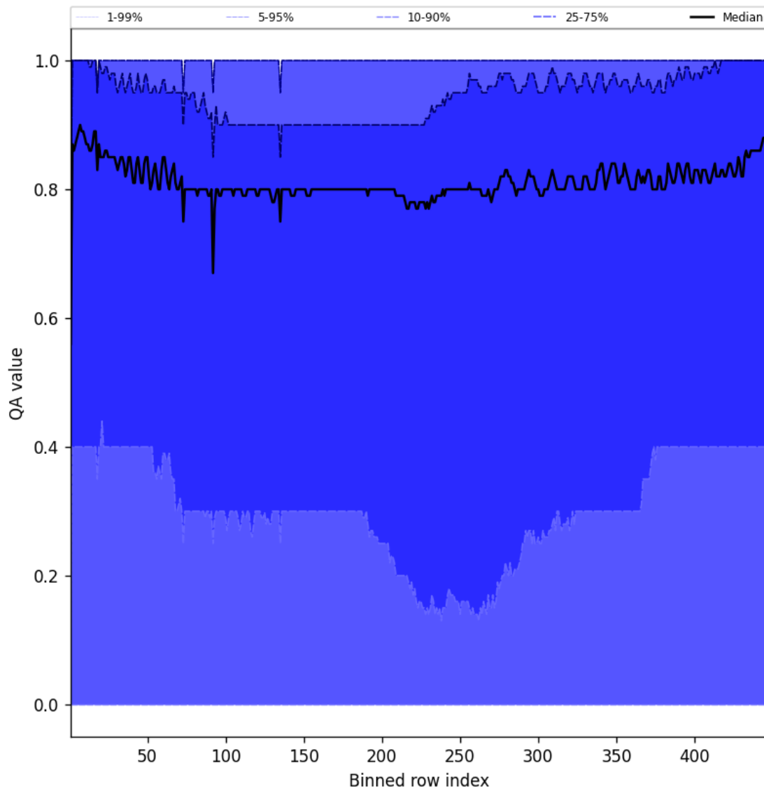
Figure 54: Along track statistics of “QA value” for 2025-03-09 to 2025-03-11
