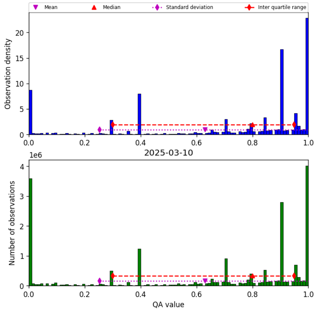
Figure 38: Histogram of “QA value” for 2025-03-09 to 2025-03-11
