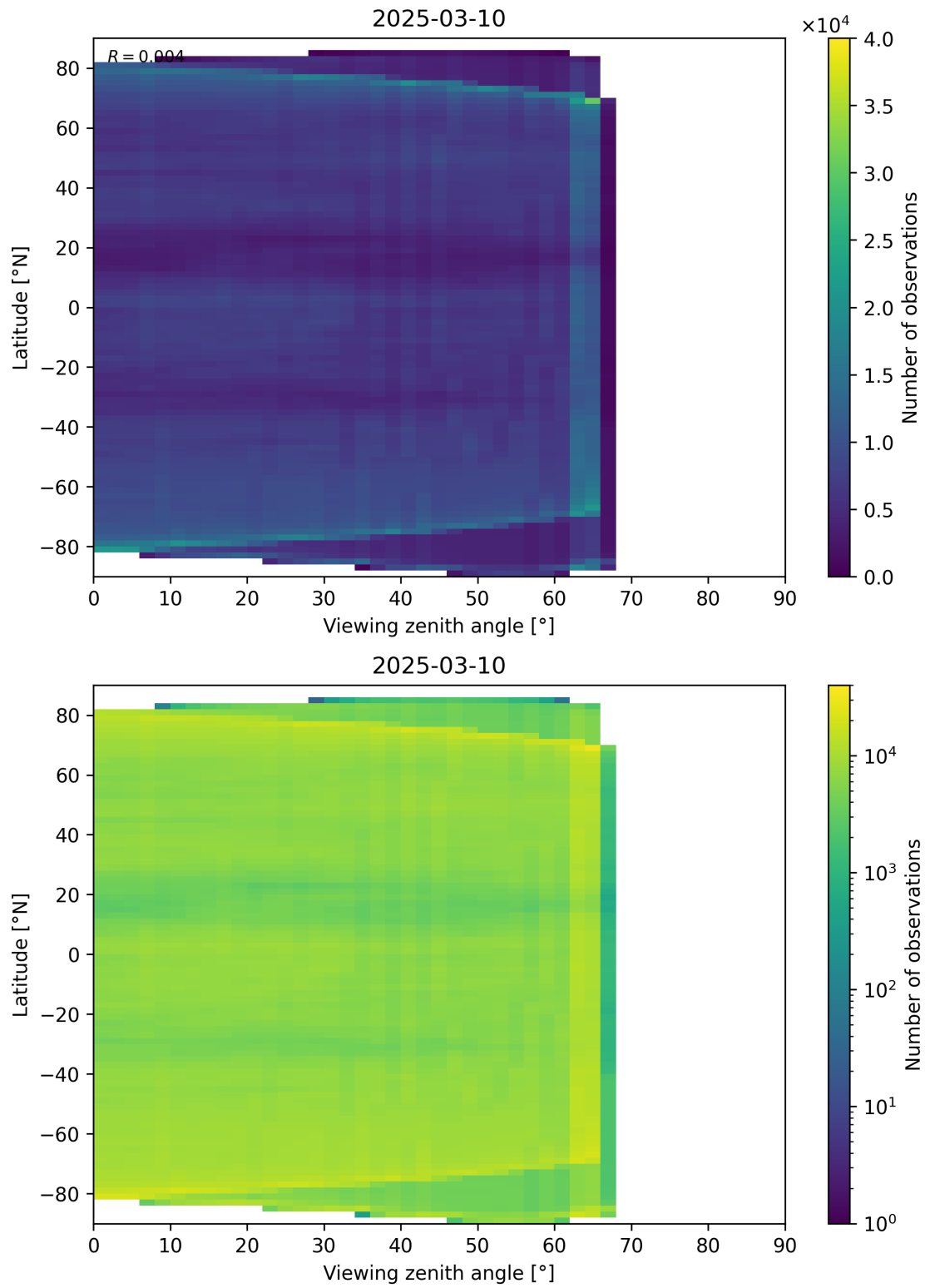
Figure 113: Scatter density plot of “Viewing zenith angle” against “Latitude” for 2025-03-09 to 2025-03-11.
