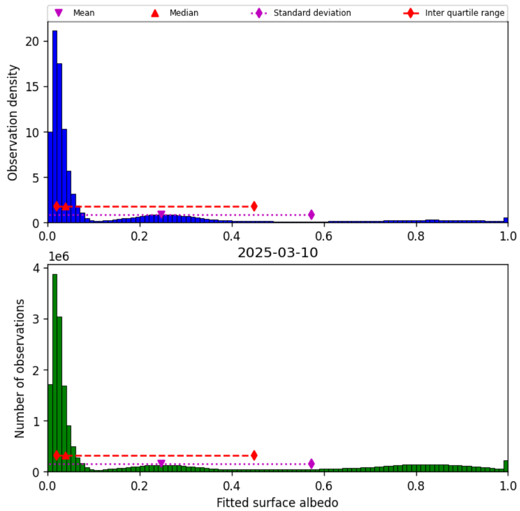
Figure 45: Histogram of “Fitted surface albedo” for 2025-03-09 to 2025-03-11
