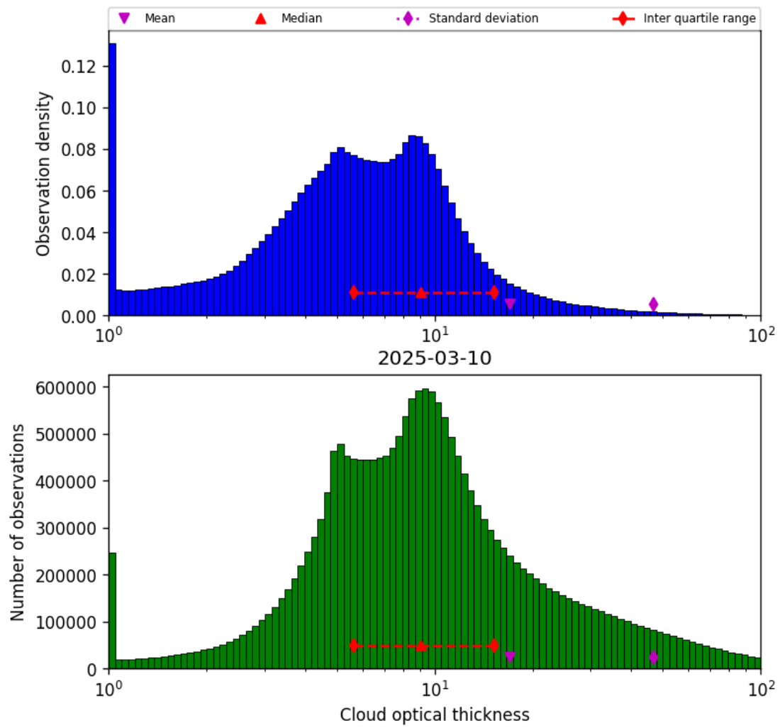
Figure 41: Histogram of “Cloud optical thickness” for 2025-03-09 to 2025-03-11
