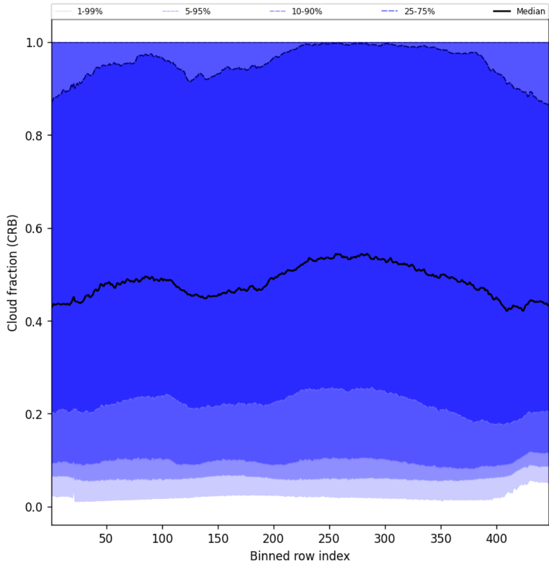
Figure 58: Along track statistics of “Cloud fraction (CRB)” for 2025-03-09 to 2025-03-11
