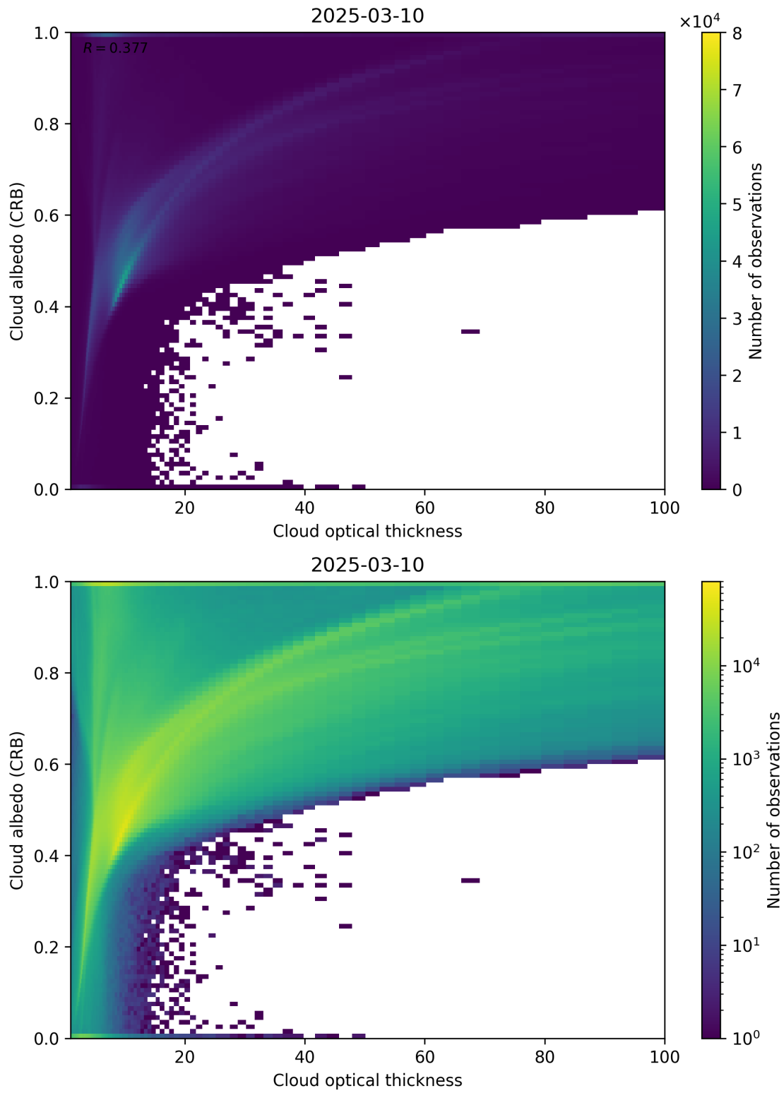
Figure 82: Scatter density plot of “Cloud optical thickness” against “Cloud albedo (CRB)” for 2025-03-09 to 2025-03-11.
