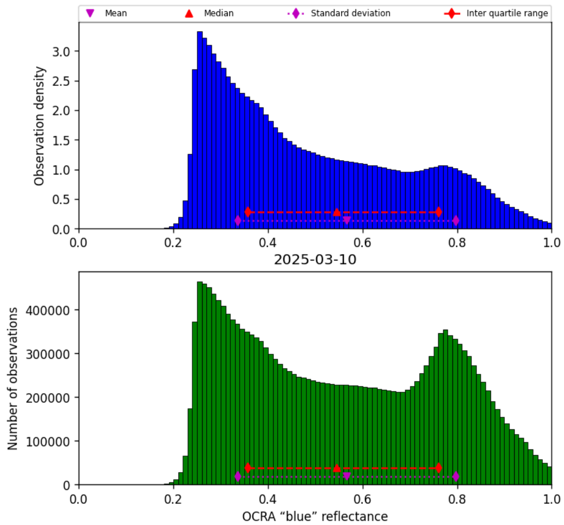
Figure 51: Histogram of “OCRA “blue” reflectance” for 2025-03-09 to 2025-03-11
