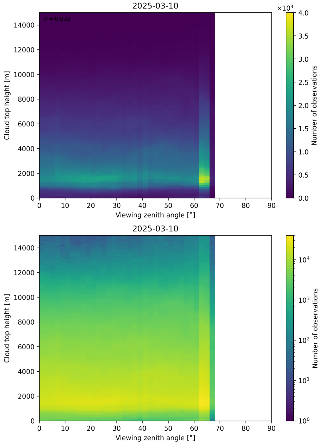
Figure 112: Scatter density plot of “Viewing zenith angle” against “Cloud top height” for 2025-03-09 to 2025-03-11.
