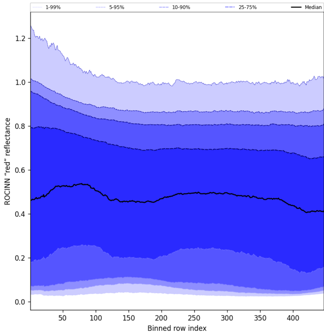
Figure 69: Along track statistics of “ROCINN “red” reflectance” for 2025-03-09 to 2025-03-11
