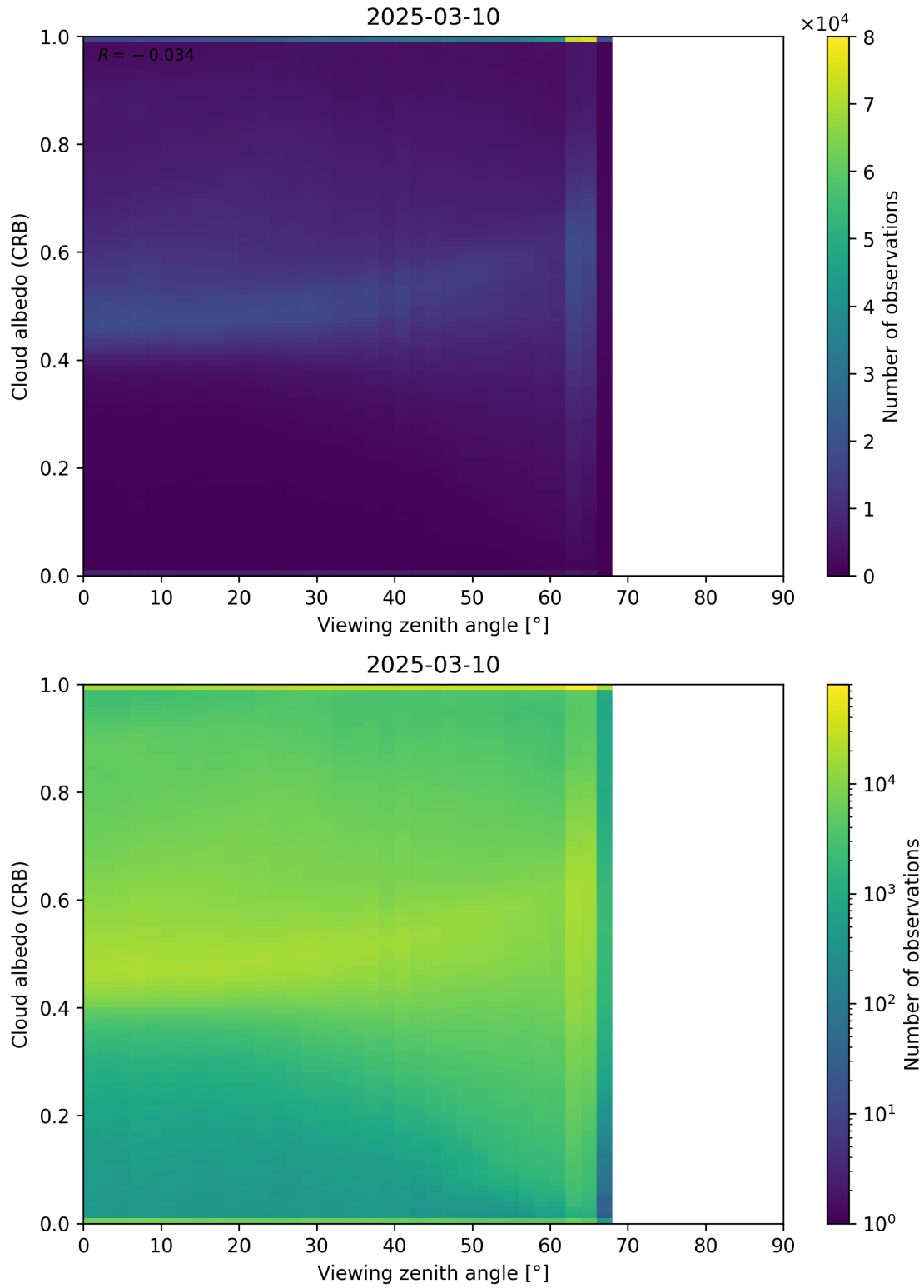
Figure 106: Scatter density plot of “Viewing zenith angle” against “Cloud albedo (CRB)” for 2025-03-09 to 2025-03-11.
