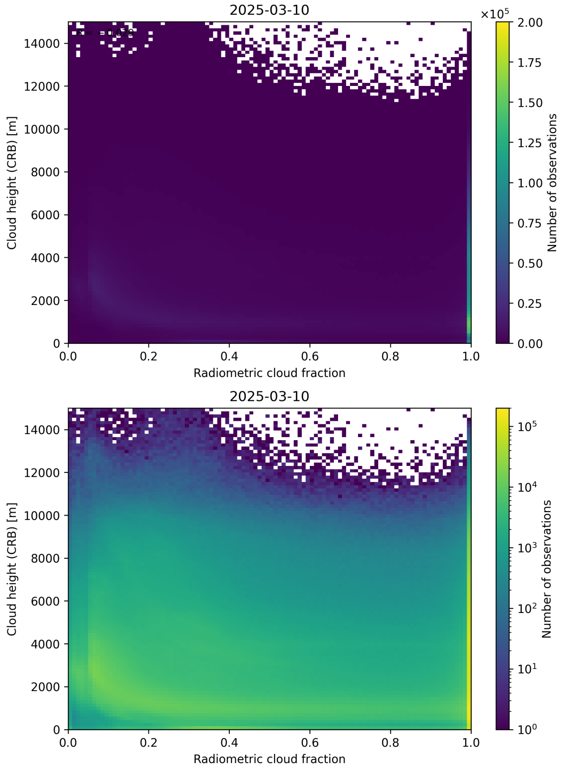
Figure 74: Scatter density plot of “Radiometric cloud fraction” against “Cloud height (CRB)” for 2025-03-09 to 2025-03-11.
