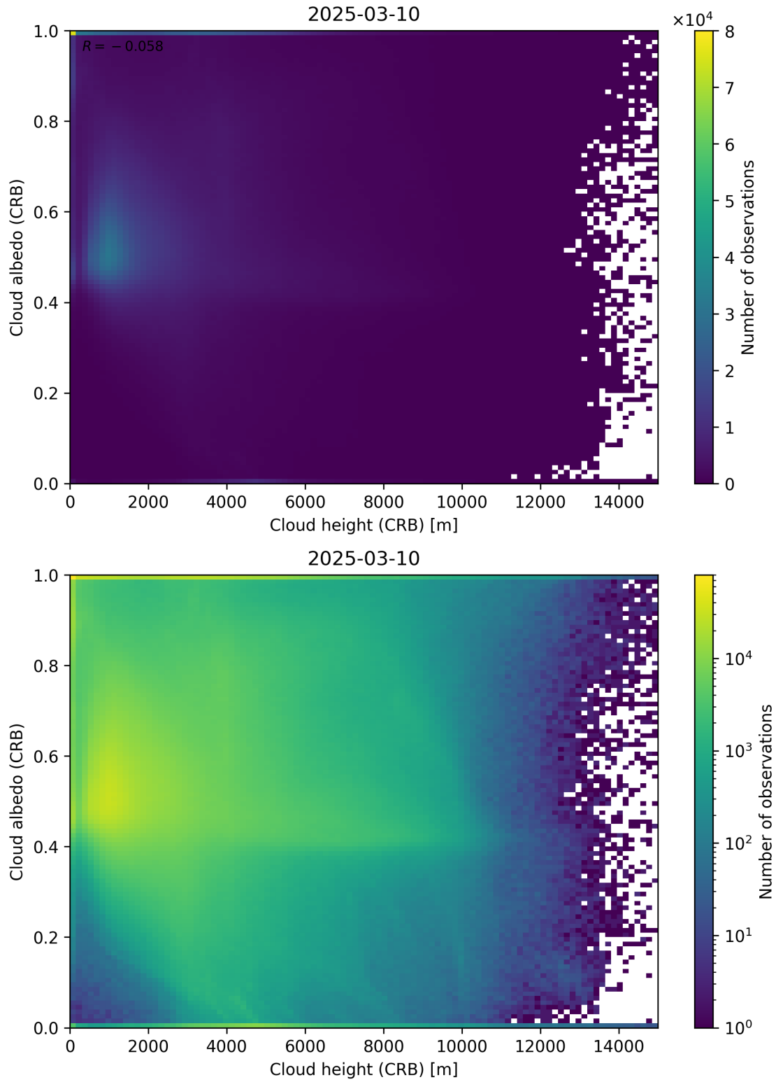
Figure 80: Scatter density plot of “Cloud height (CRB)” against “Cloud albedo (CRB)” for 2025-03-09 to 2025-03-11.
