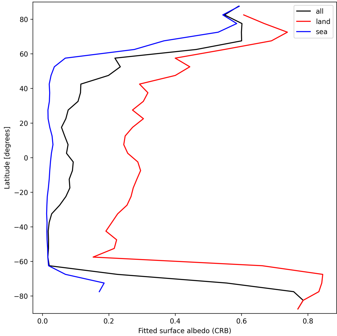
Figure 30: Zonal average of “Fitted surface albedo (CRB)” for 2025-03-09 to 2025-03-11.
