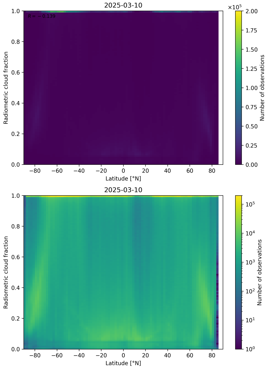
Figure 92: Scatter density plot of “Latitude” against “Radiometric cloud fraction” for 2025-03-09 to 2025-03-11.
