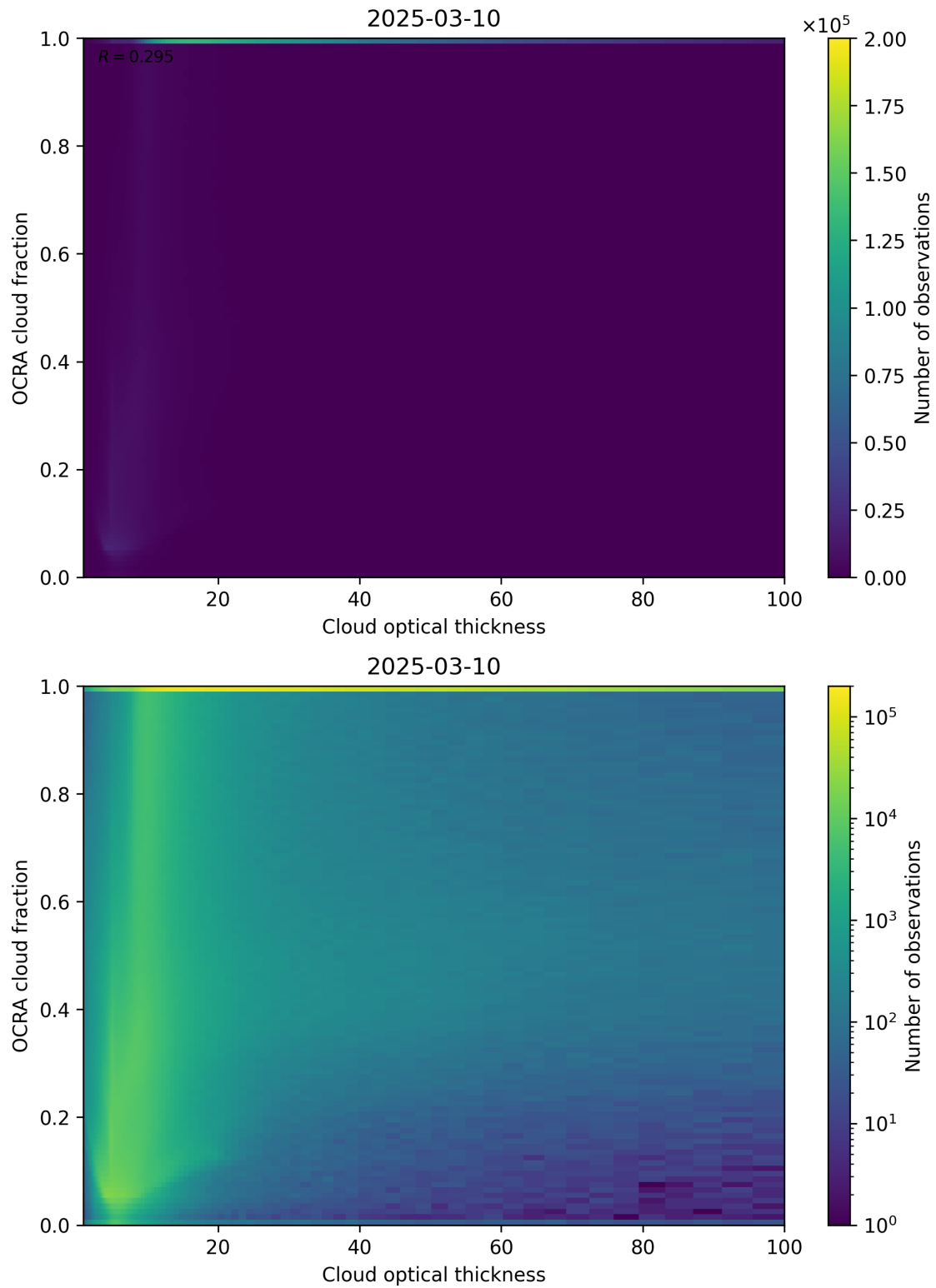
Figure 83: Scatter density plot of “Cloud optical thickness” against “OCRA cloud fraction” for 2025-03-09 to 2025-03-11.
