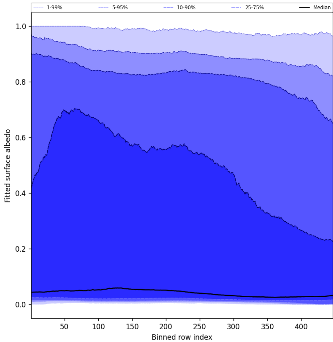
Figure 61: Along track statistics of “Fitted surface albedo” for 2025-03-09 to 2025-03-11
