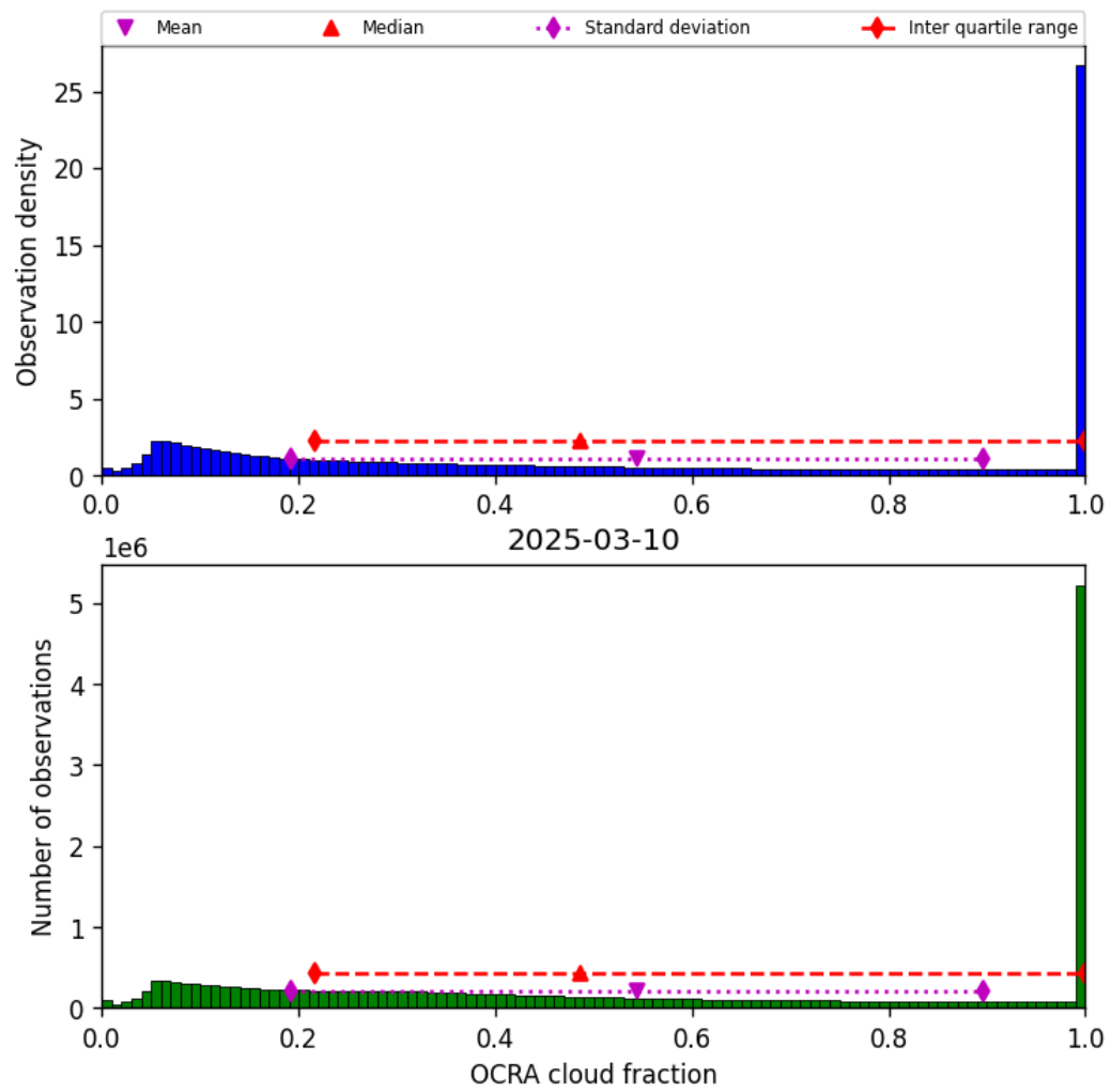
Figure 50: Histogram of “OCRA cloud fraction” for 2025-03-09 to 2025-03-11
