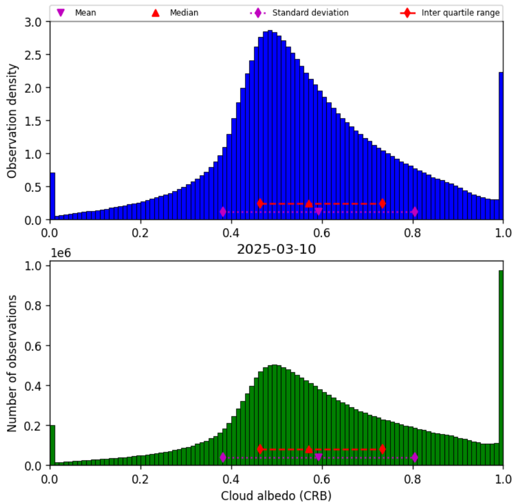
Figure 44: Histogram of “Cloud albedo (CRB)” for 2025-03-09 to 2025-03-11
