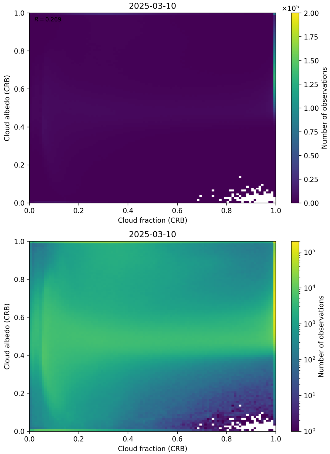
Figure 77: Scatter density plot of “Cloud fraction (CRB)” against “Cloud albedo (CRB)” for 2025-03-09 to 2025-03-11.
