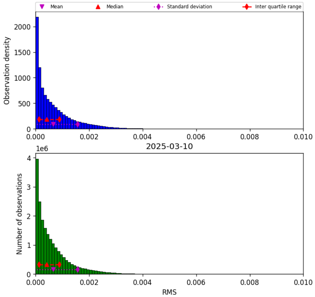
Figure 47: Histogram of “RMS” for 2025-03-09 to 2025-03-11
