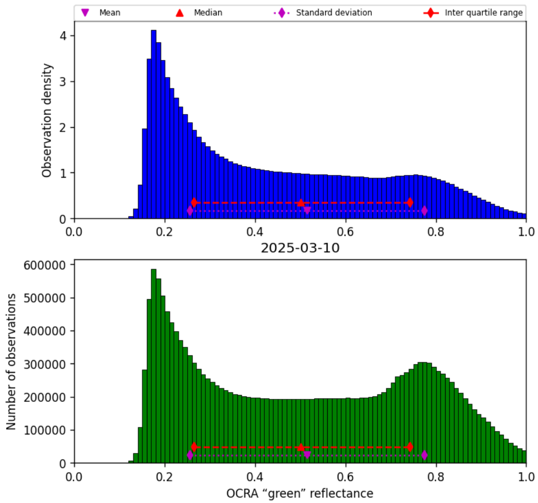
Figure 52: Histogram of “OCRA “green” reflectance” for 2025-03-09 to 2025-03-11
