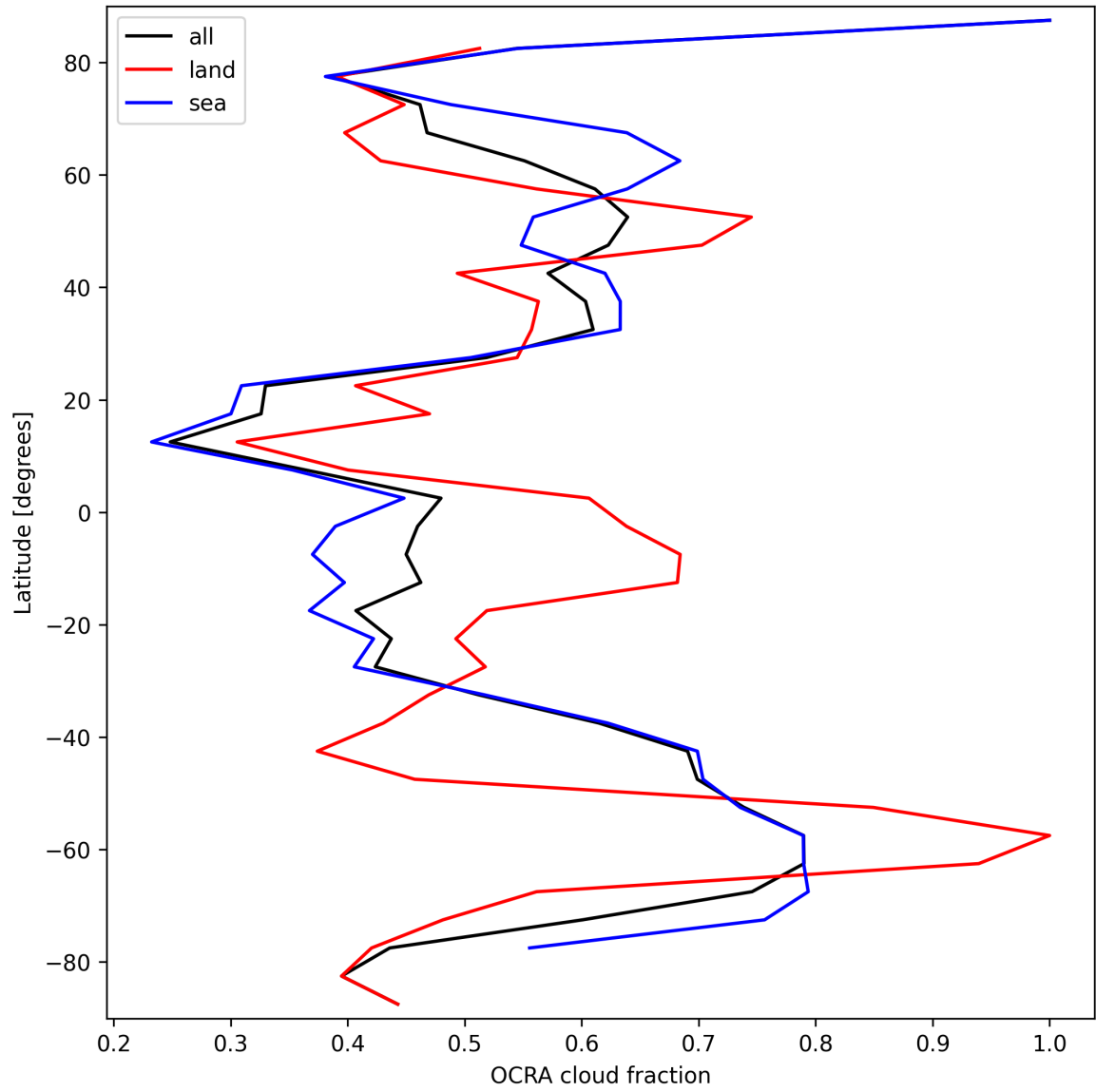
Figure 34: Zonal average of “OCRA cloud fraction” for 2025-03-09 to 2025-03-11.
