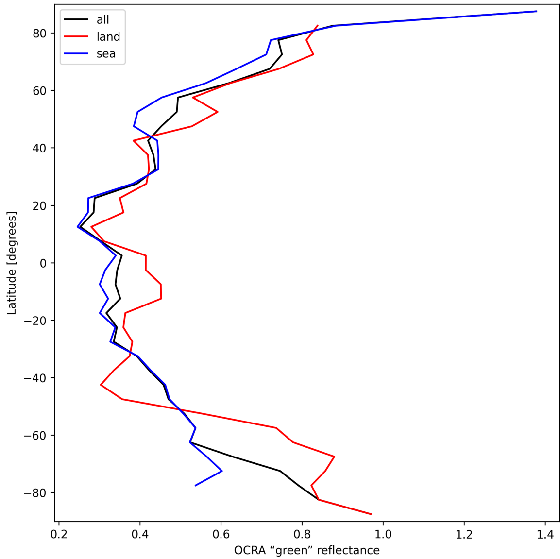
Figure 36: Zonal average of “OCRA “green” reflectance” for 2025-03-09 to 2025-03-11.
