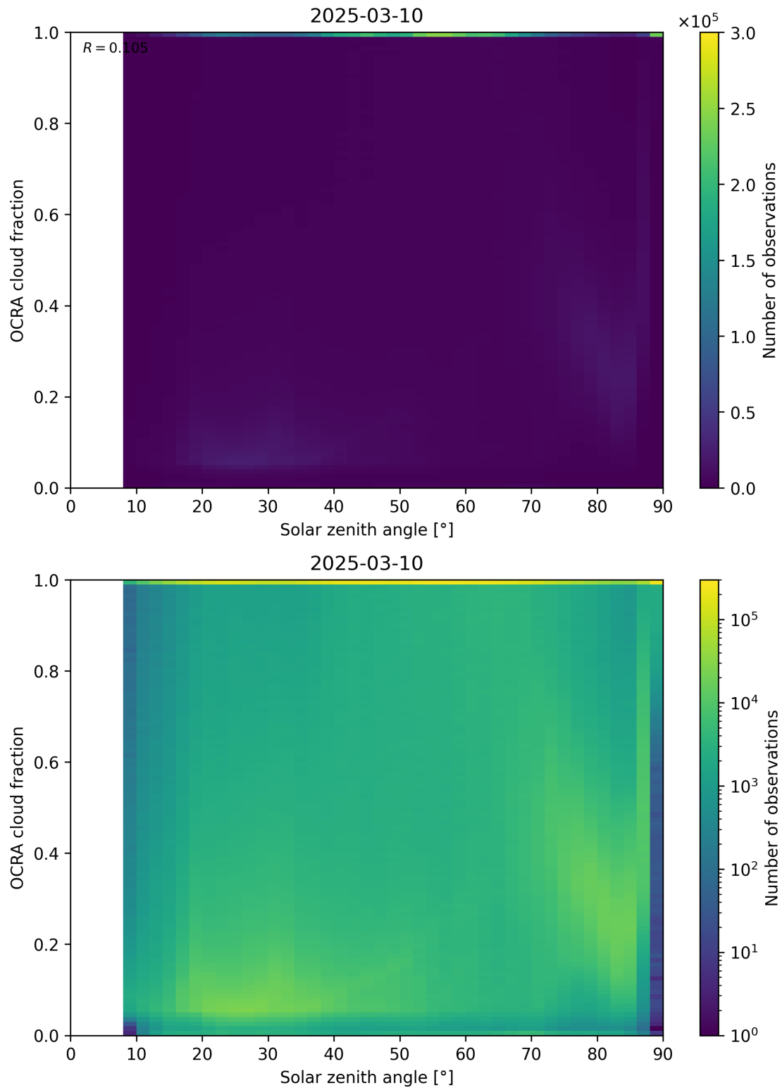
Figure 100: Scatter density plot of “Solar zenith angle” against “OCRA cloud fraction” for 2025-03-09 to 2025-03-11.
