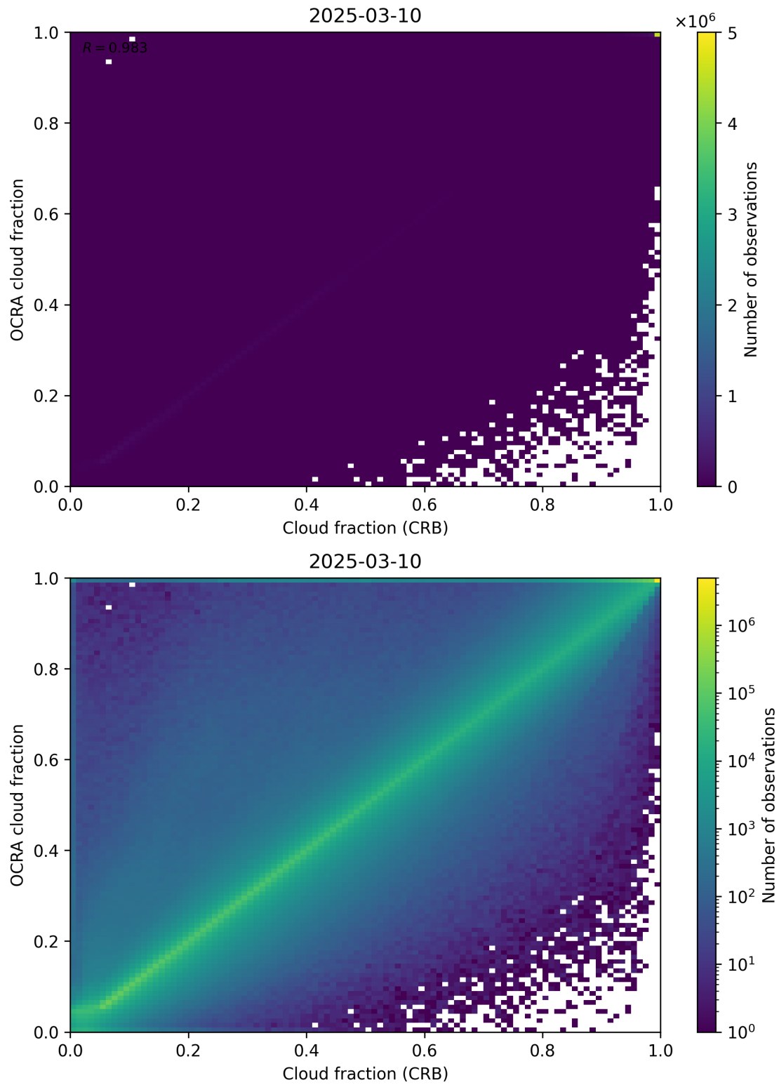
Figure 78: Scatter density plot of “Cloud fraction (CRB)” against “OCRA cloud fraction” for 2025-03-09 to 2025-03-11.
