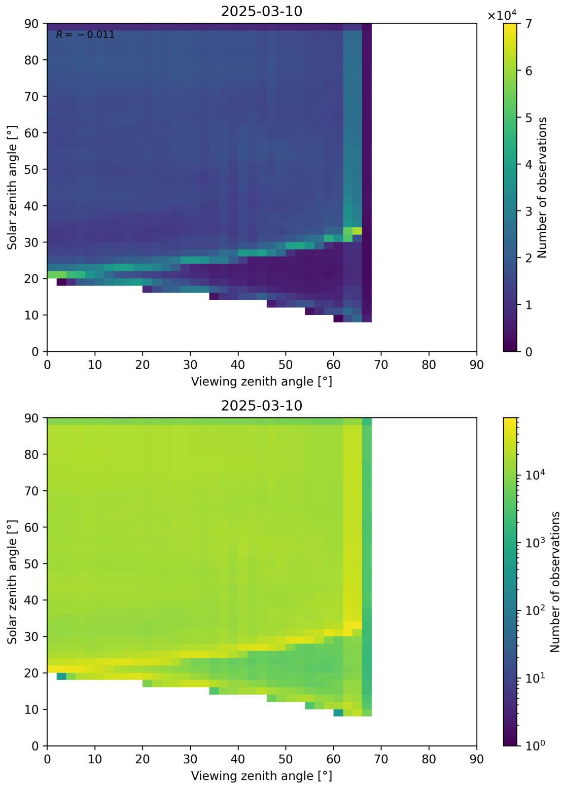
Figure 114: Scatter density plot of “Viewing zenith angle” against “Solar zenith angle” for 2025-03-09 to 2025-03-11.
