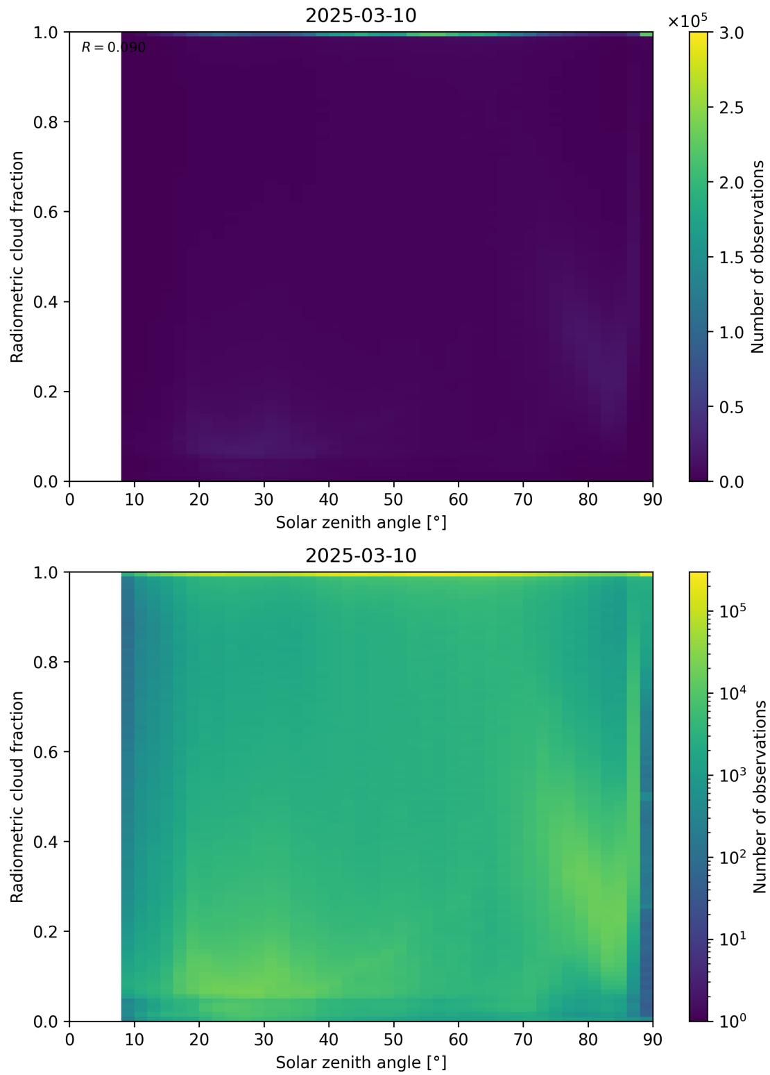
Figure 99: Scatter density plot of “Solar zenith angle” against “Radiometric cloud fraction” for 2025-03-09 to 2025-03-11.
