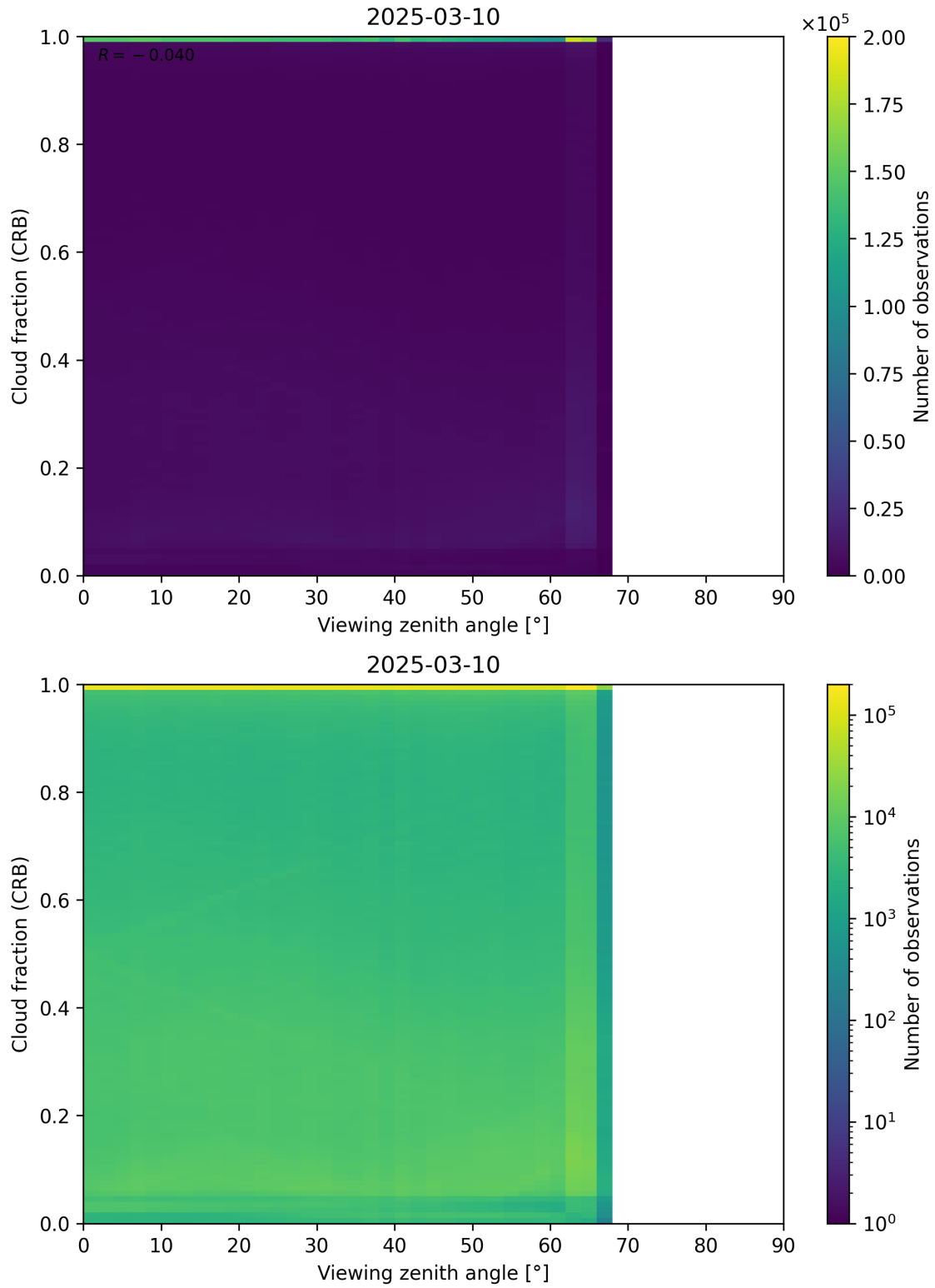
Figure 109: Scatter density plot of “Viewing zenith angle” against “Cloud fraction (CRB)” for 2025-03-09 to 2025-03-11.
