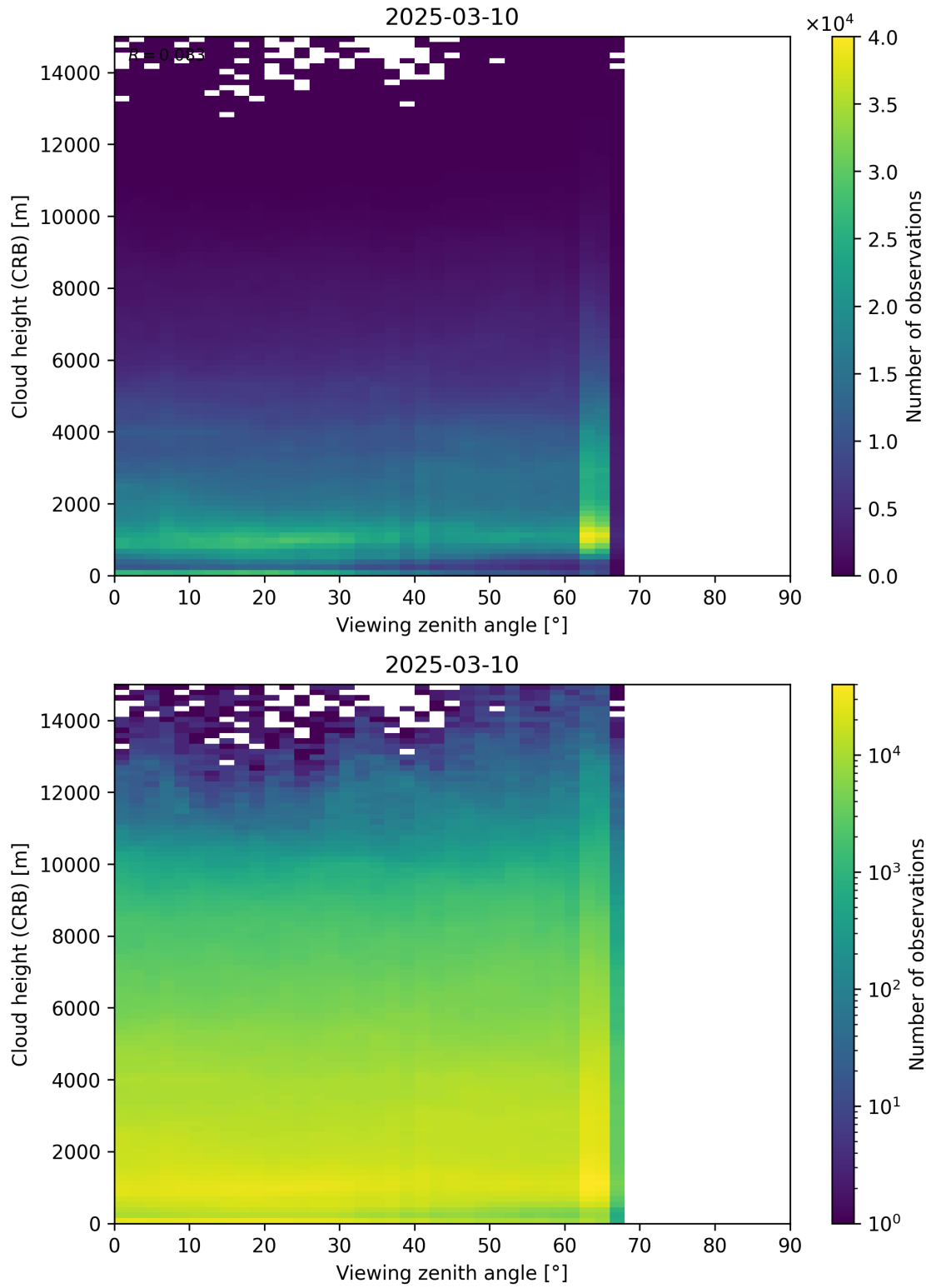
Figure 110: Scatter density plot of “Viewing zenith angle” against “Cloud height (CRB)” for 2025-03-09 to 2025-03-11.
