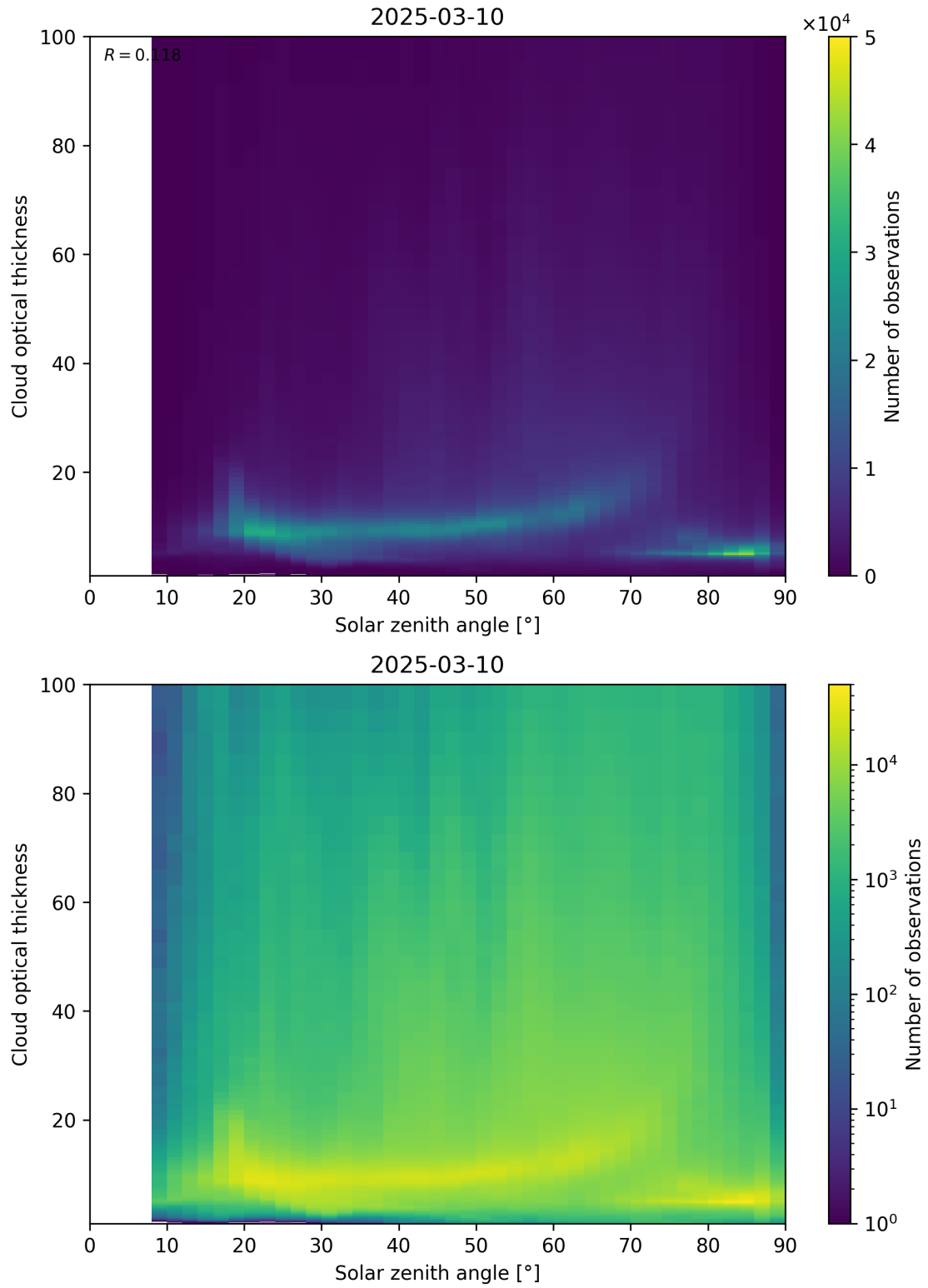
Figure 103: Scatter density plot of “Solar zenith angle” against “Cloud optical thickness” for 2025-03-09 to 2025-03-11.
