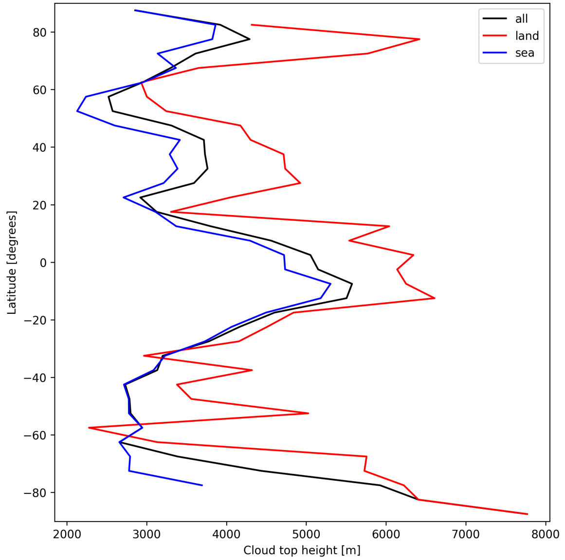
Figure 24: Zonal average of “Cloud top height” for 2025-03-09 to 2025-03-11.
