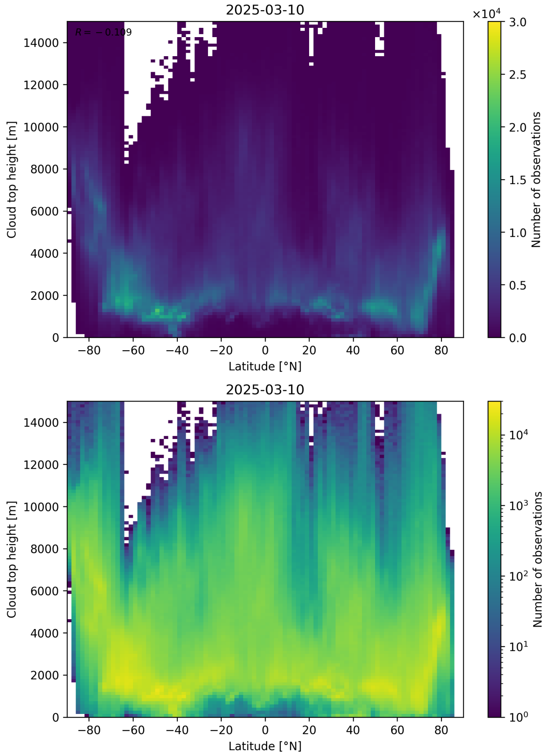
Figure 97: Scatter density plot of “Latitude” against “Cloud top height” for 2025-03-09 to 2025-03-11.
