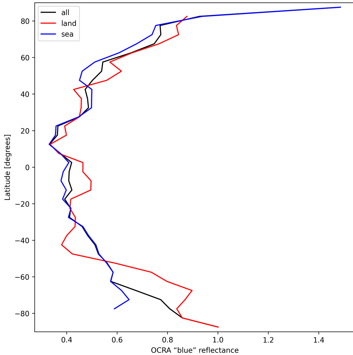
Figure 35: Zonal average of “OCRA “blue” reflectance” for 2025-03-09 to 2025-03-11.
