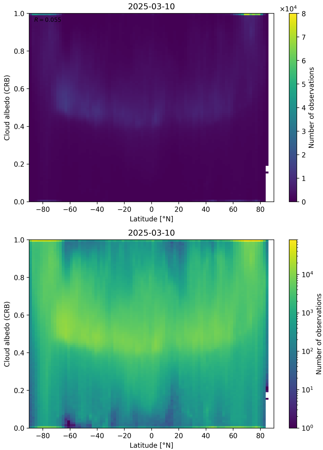
Figure 91: Scatter density plot of “Latitude” against “Cloud albedo (CRB)” for 2025-03-09 to 2025-03-11.
