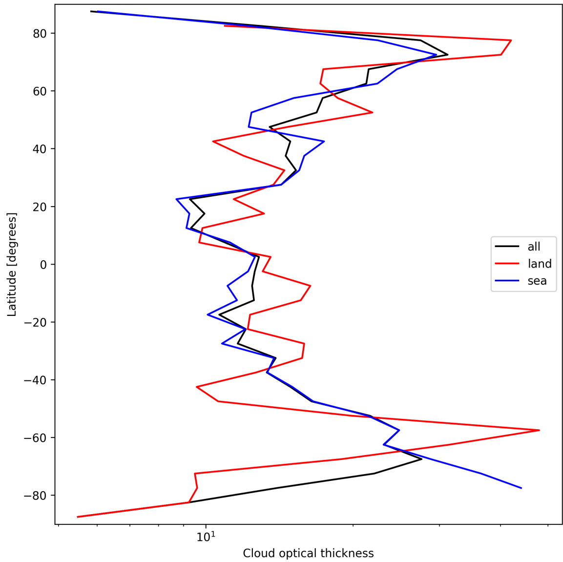
Figure 25: Zonal average of “Cloud optical thickness” for 2025-03-09 to 2025-03-11.
