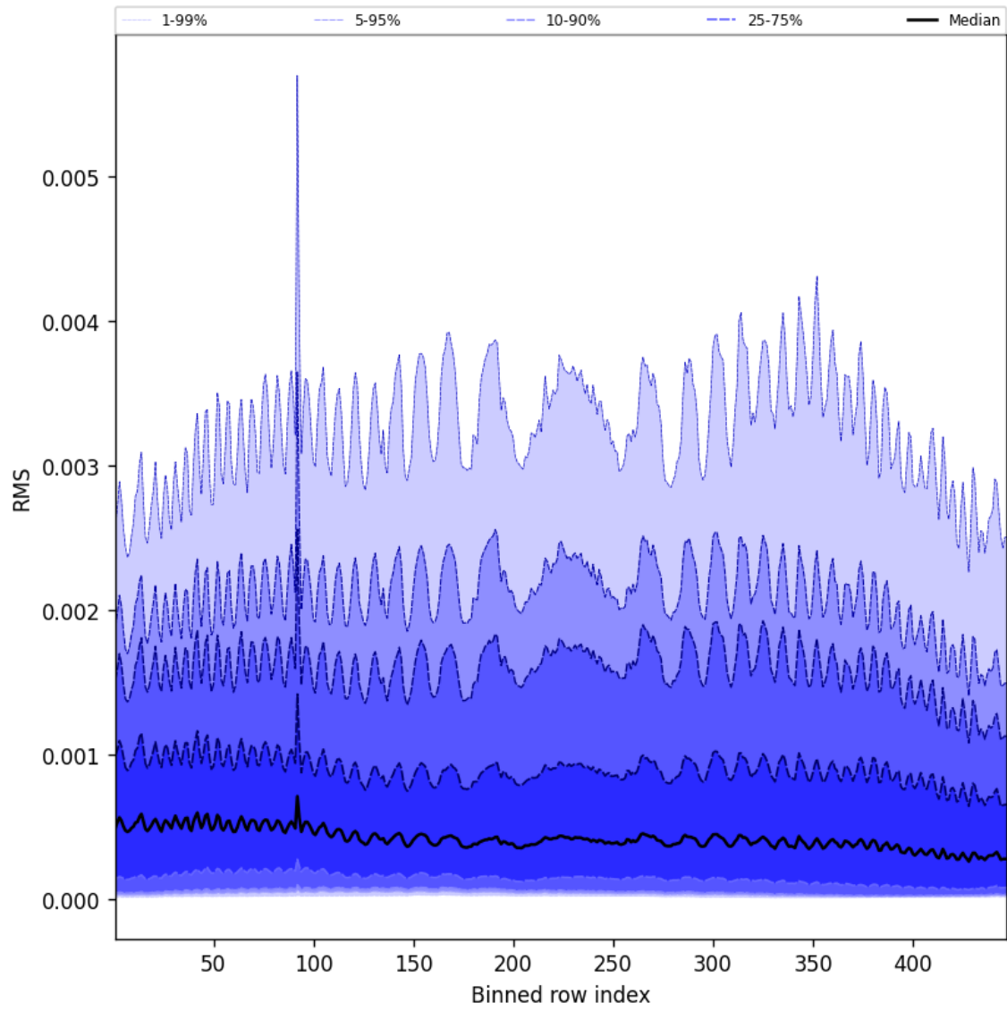
Figure 63: Along track statistics of “RMS” for 2025-03-09 to 2025-03-11
