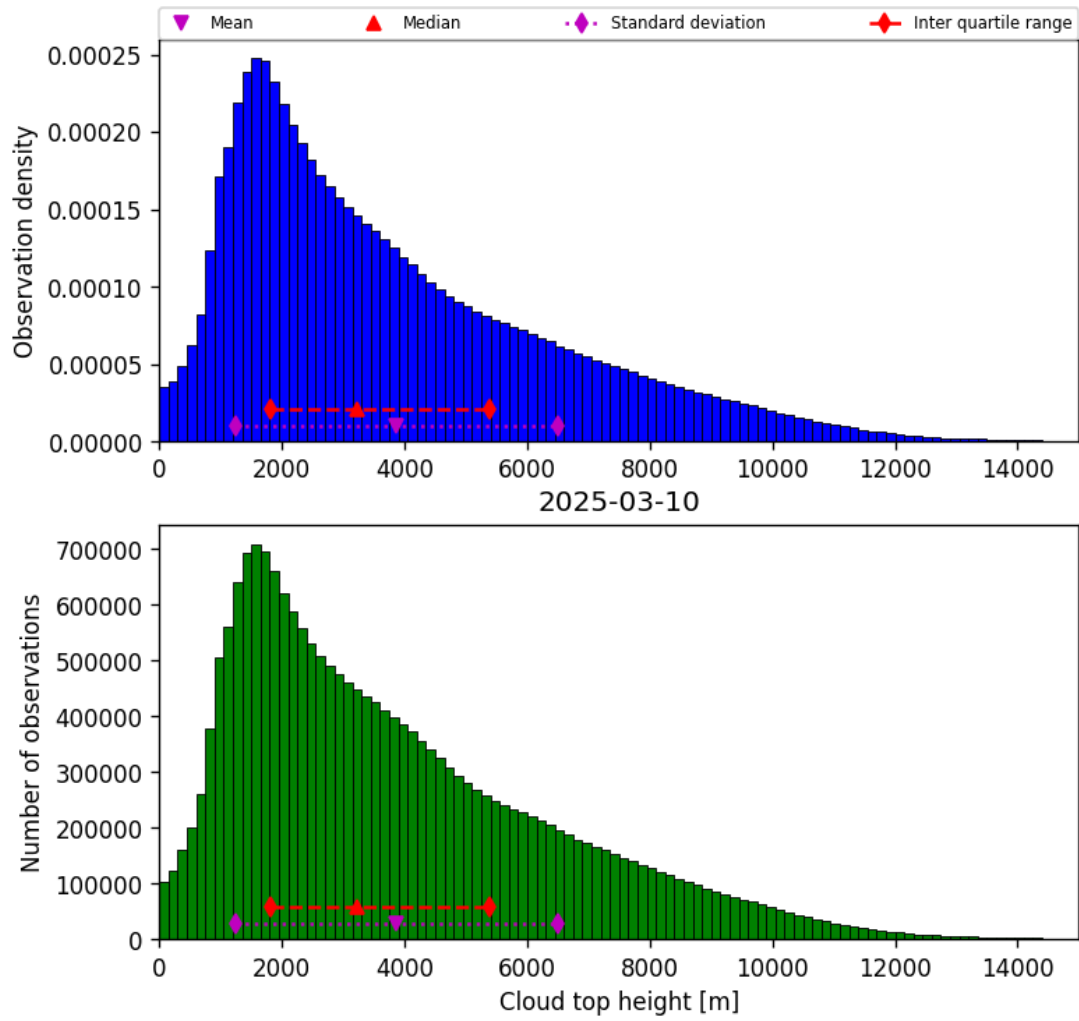
Figure 40: Histogram of “Cloud top height” for 2025-03-09 to 2025-03-11
