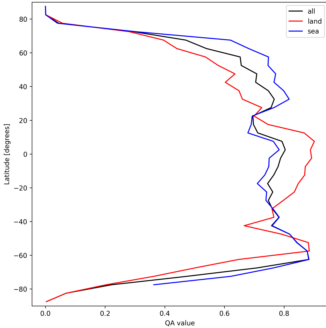
Figure 22: Zonal average of “QA value” for 2025-03-09 to 2025-03-11.
