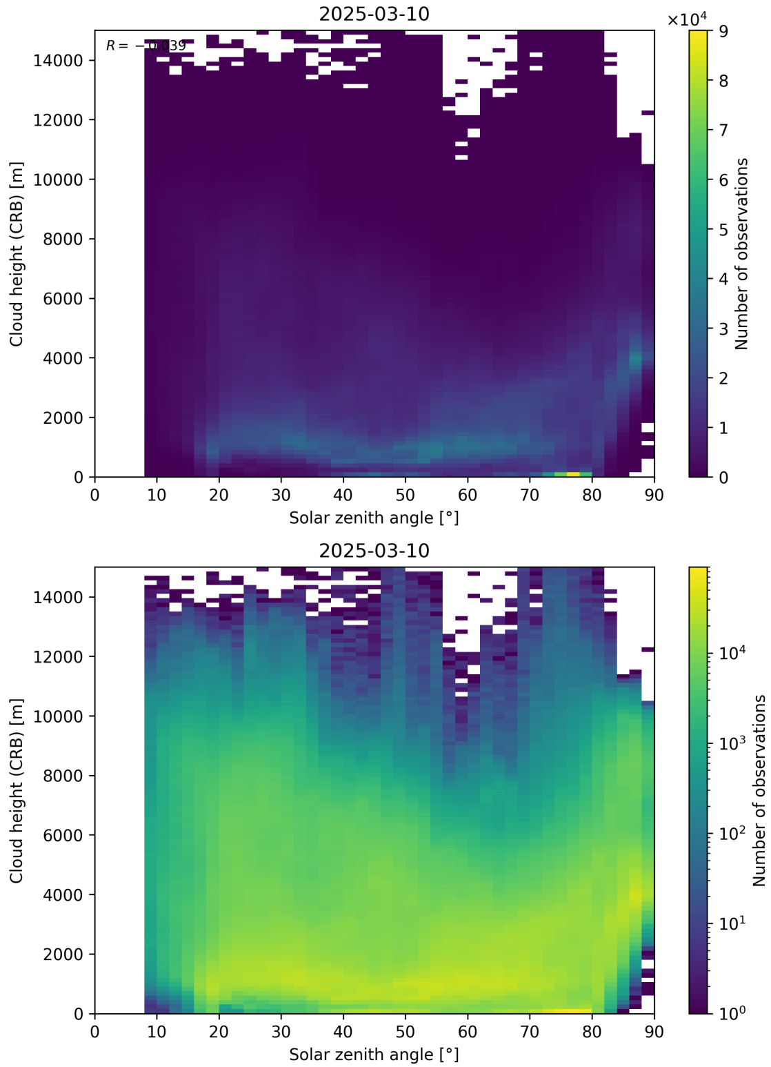
Figure 102: Scatter density plot of “Solar zenith angle” against “Cloud height (CRB)” for 2025-03-09 to 2025-03-11.
