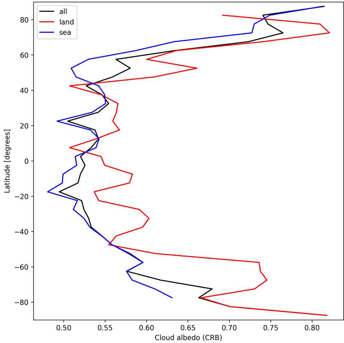
Figure 28: Zonal average of “Cloud albedo (CRB)” for 2025-03-09 to 2025-03-11.
