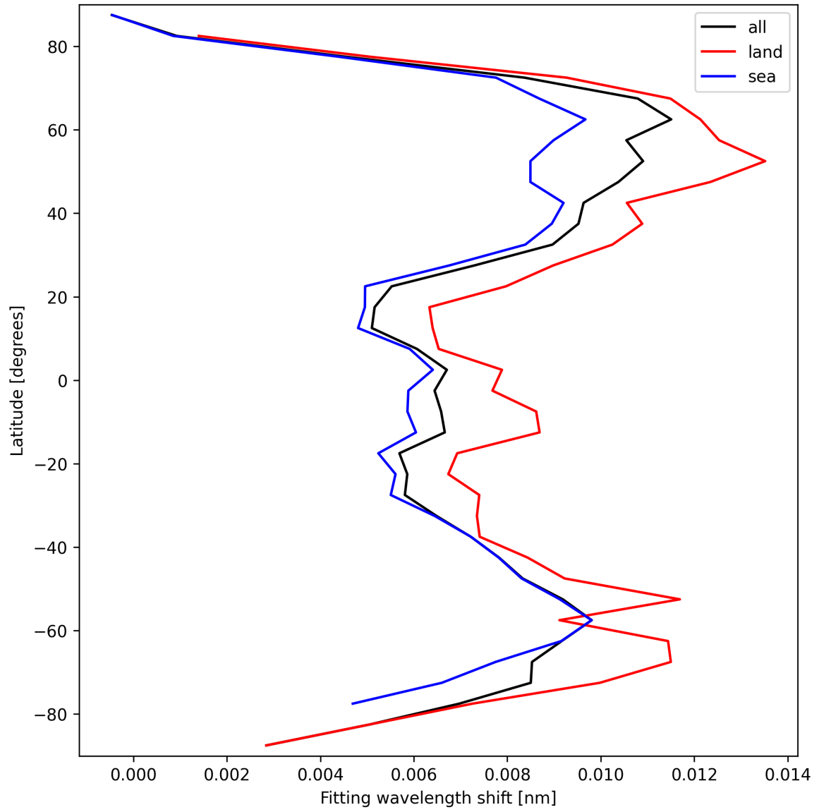
Figure 33: Zonal average of “Fitting wavelength shift” for 2025-03-09 to 2025-03-11.
