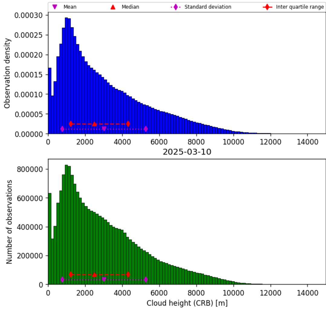
Figure 43: Histogram of “Cloud height (CRB)” for 2025-03-09 to 2025-03-11
