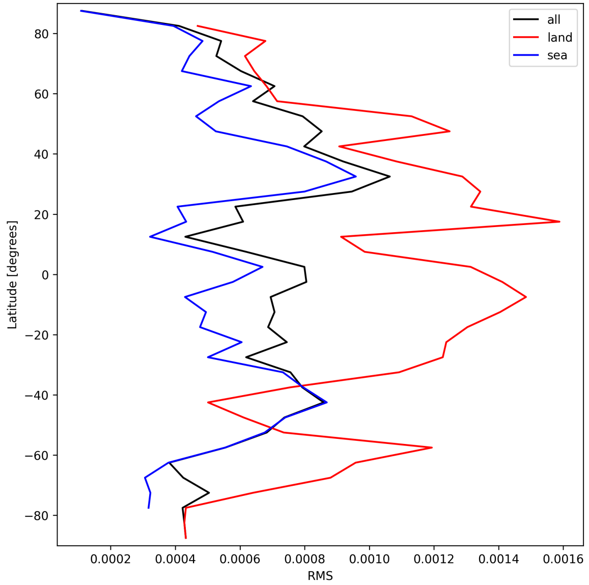
Figure 31: Zonal average of “RMS” for 2025-03-09 to 2025-03-11.
