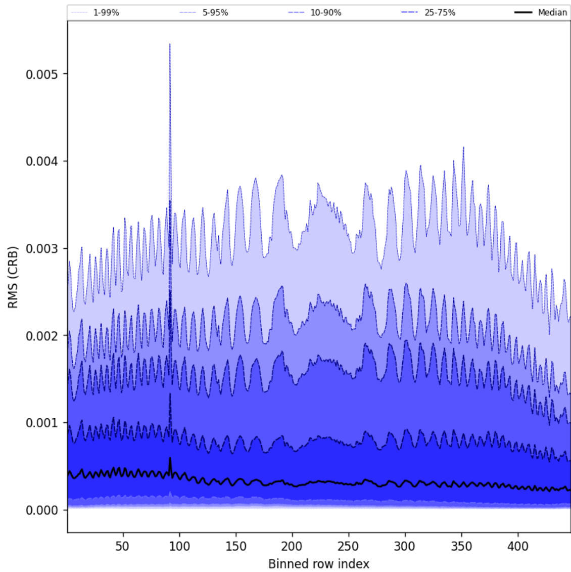
Figure 64: Along track statistics of “RMS (CRB)” for 2025-03-09 to 2025-03-11
