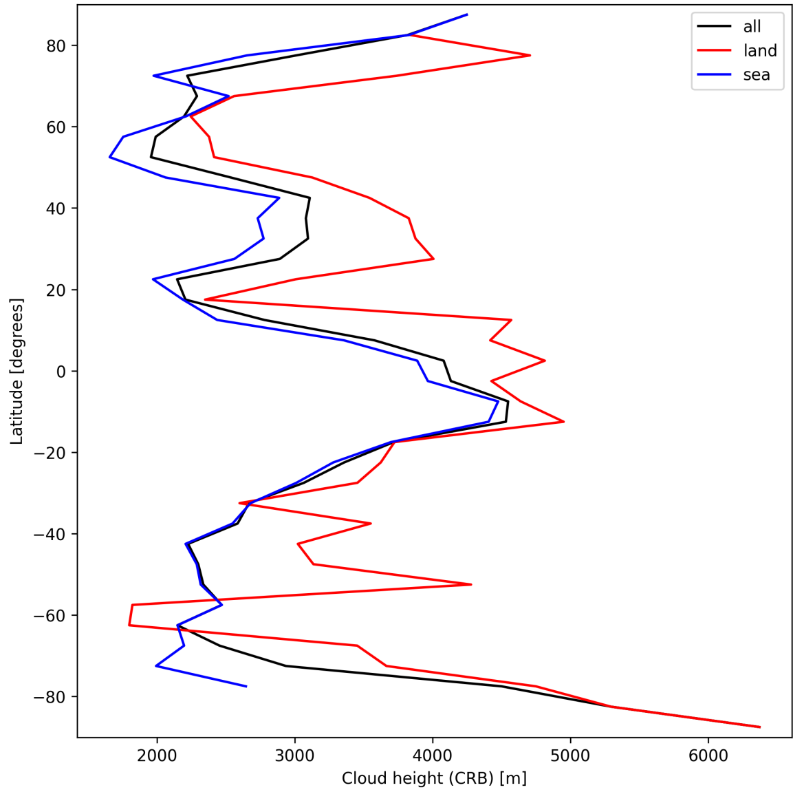
Figure 27: Zonal average of “Cloud height (CRB)” for 2025-03-09 to 2025-03-11.
