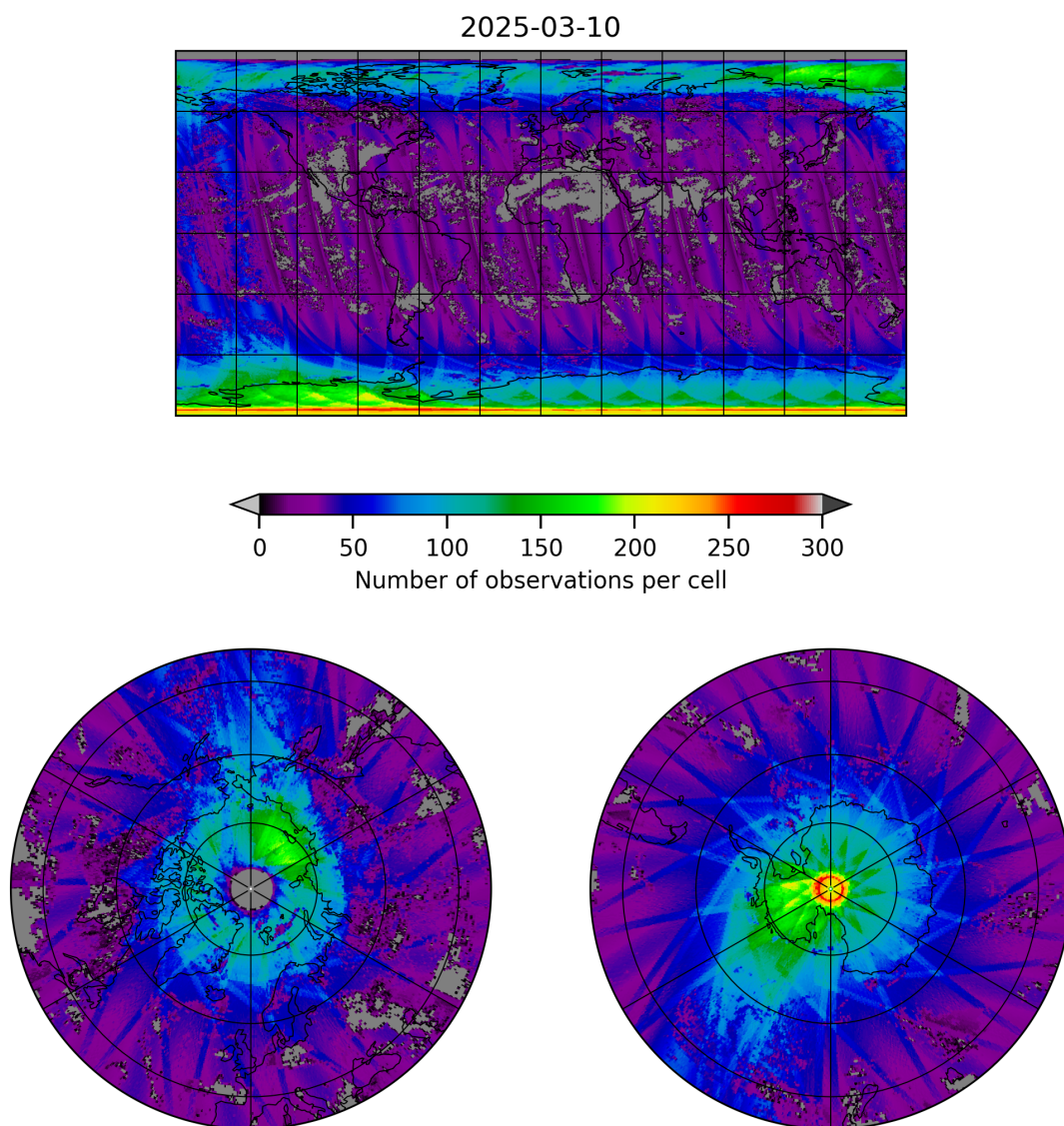
Figure 21: Map of the number of observations for 2025-03-09 to 2025-03-11
