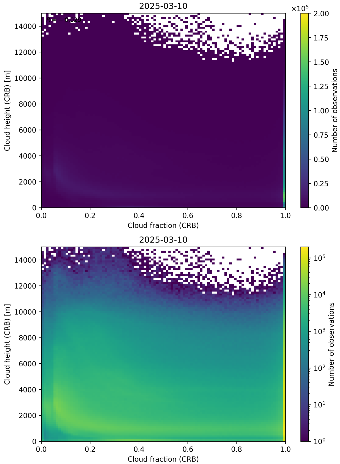
Figure 79: Scatter density plot of “Cloud fraction (CRB)” against “Cloud height (CRB)” for 2025-03-09 to 2025-03-11.
