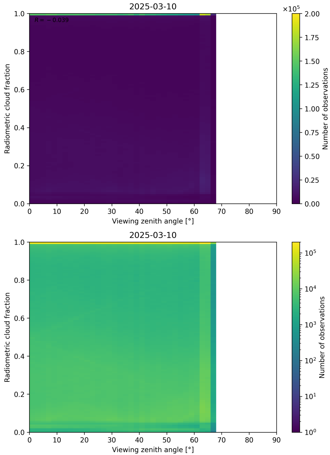
Figure 107: Scatter density plot of “Viewing zenith angle” against “Radiometric cloud fraction” for 2025-03-09 to 2025-03-11.
