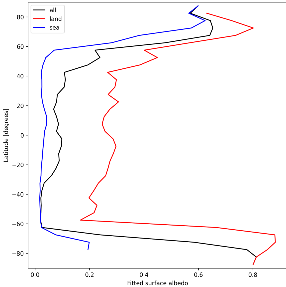
Figure 29: Zonal average of “Fitted surface albedo” for 2025-03-09 to 2025-03-11.
