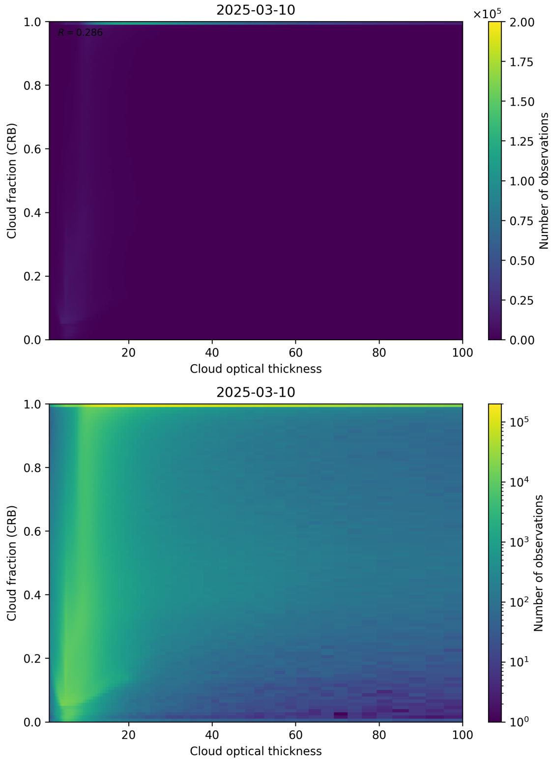
Figure 84: Scatter density plot of “Cloud optical thickness” against “Cloud fraction (CRB)” for 2025-03-09 to 2025-03-11.
