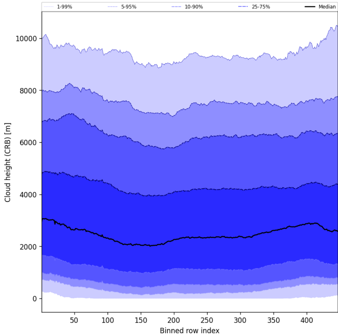
Figure 59: Along track statistics of “Cloud height (CRB)” for 2025-03-09 to 2025-03-11
