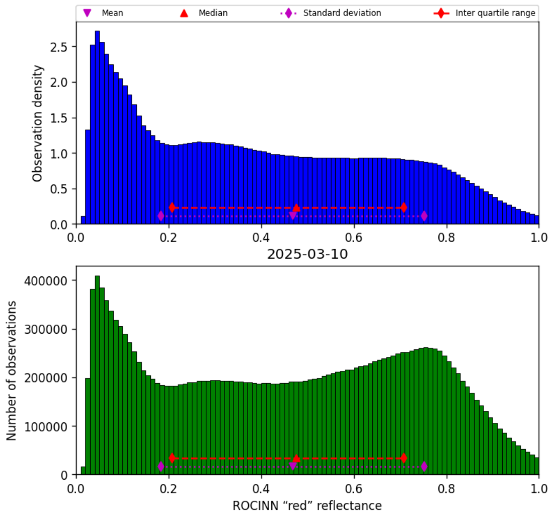
Figure 53: Histogram of “ROCINN “red” reflectance” for 2025-03-09 to 2025-03-11
