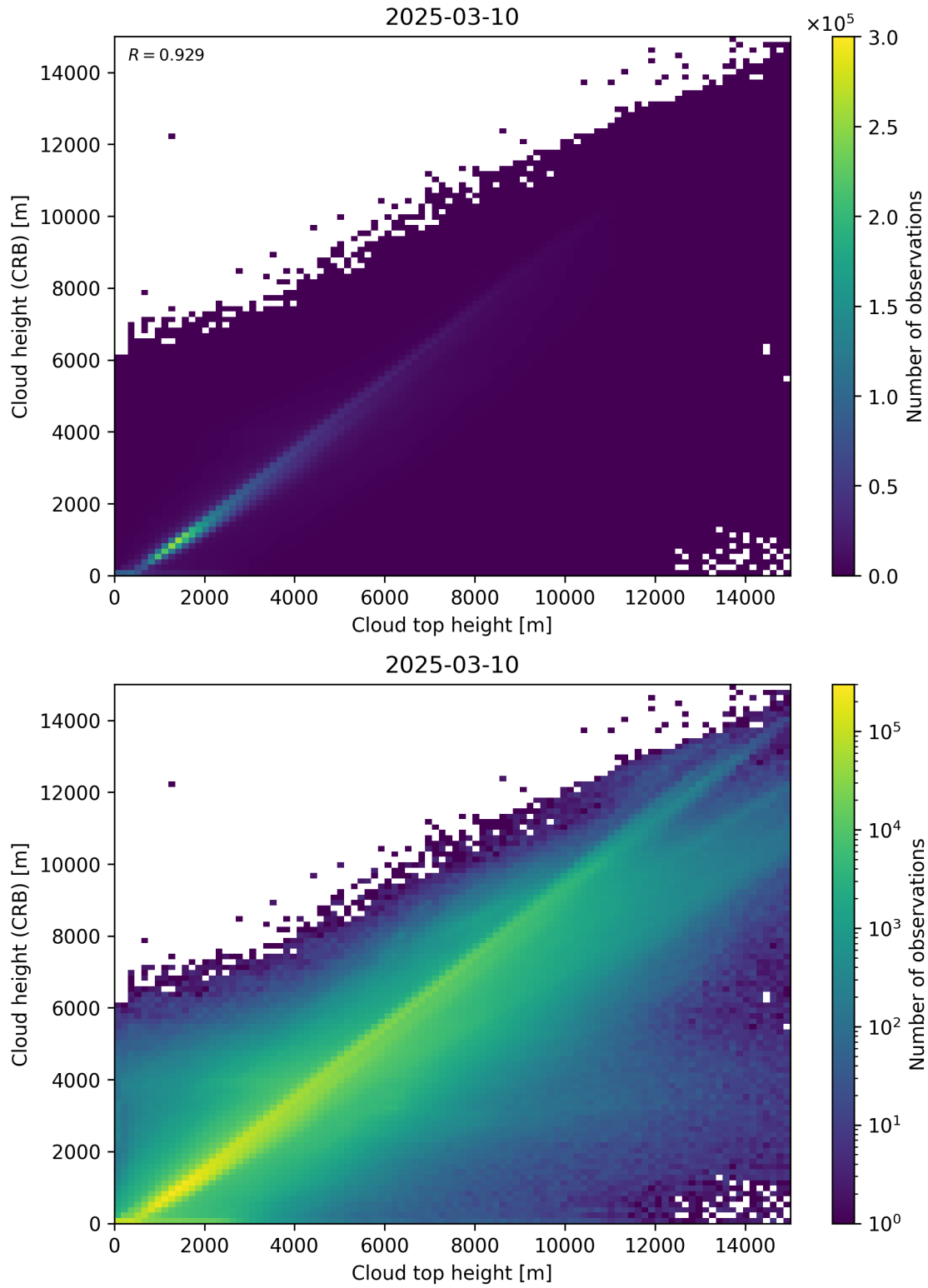
Figure 89: Scatter density plot of “Cloud top height” against “Cloud height (CRB)” for 2025-03-09 to 2025-03-11.
