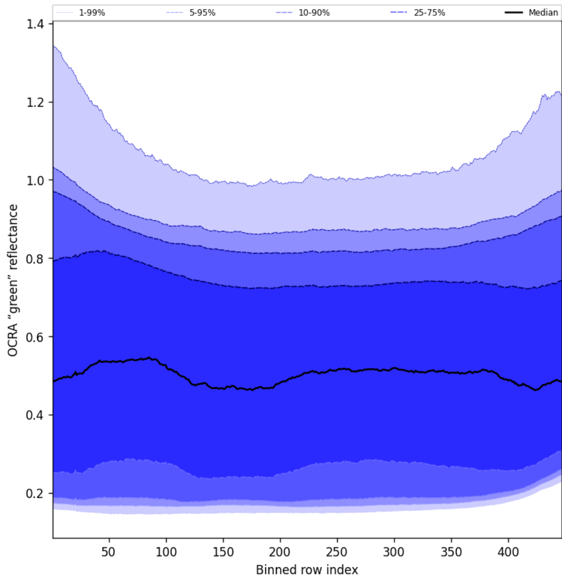
Figure 68: Along track statistics of “OCRA “green” reflectance” for 2025-03-09 to 2025-03-11
