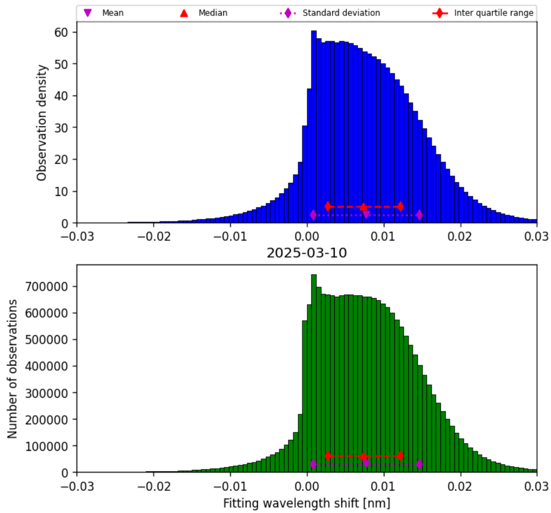
Figure 49: Histogram of “Fitting wavelength shift” for 2025-03-09 to 2025-03-11
