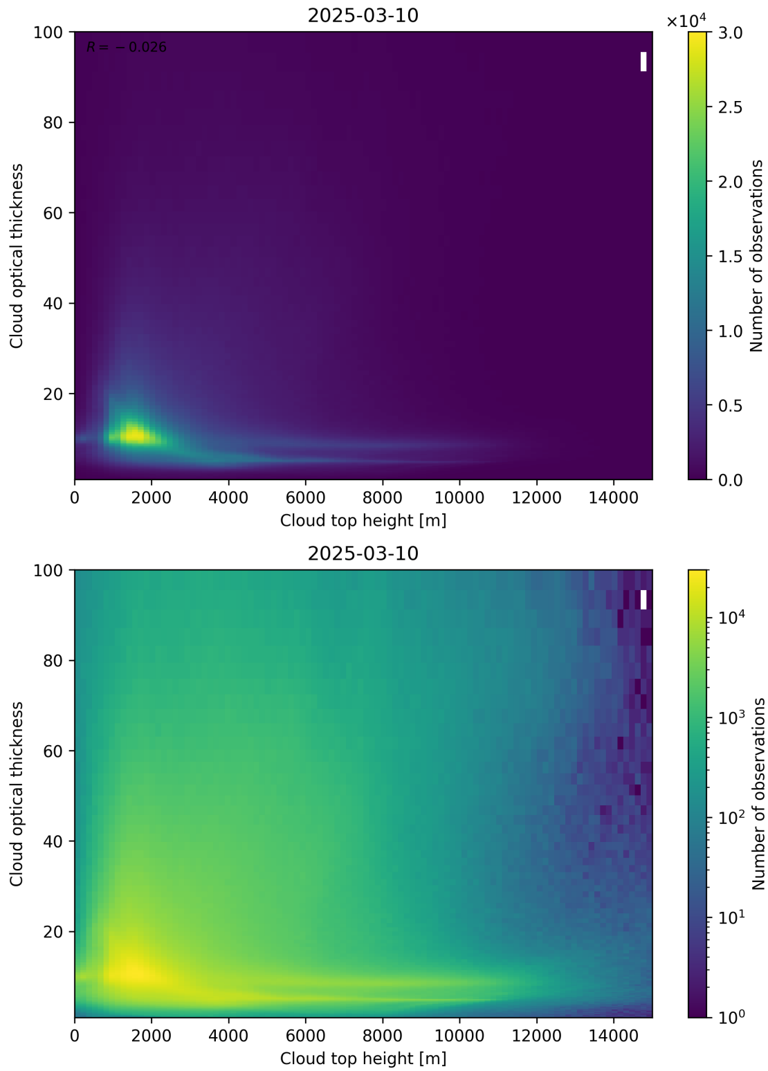
Figure 90: Scatter density plot of “Cloud top height” against “Cloud optical thickness” for 2025-03-09 to 2025-03-11.
