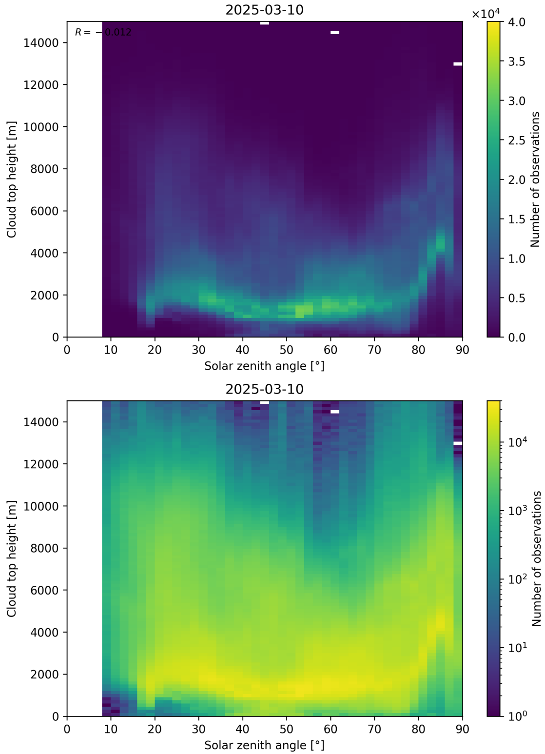
Figure 104: Scatter density plot of “Solar zenith angle” against “Cloud top height” for 2025-03-09 to 2025-03-11.
