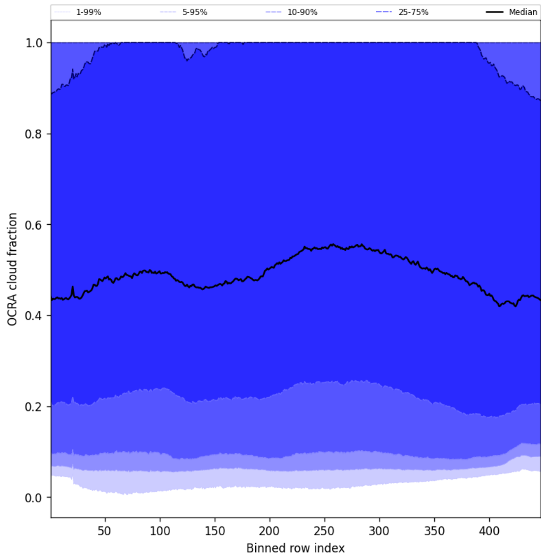
Figure 66: Along track statistics of “OCRA cloud fraction” for 2025-03-09 to 2025-03-11
