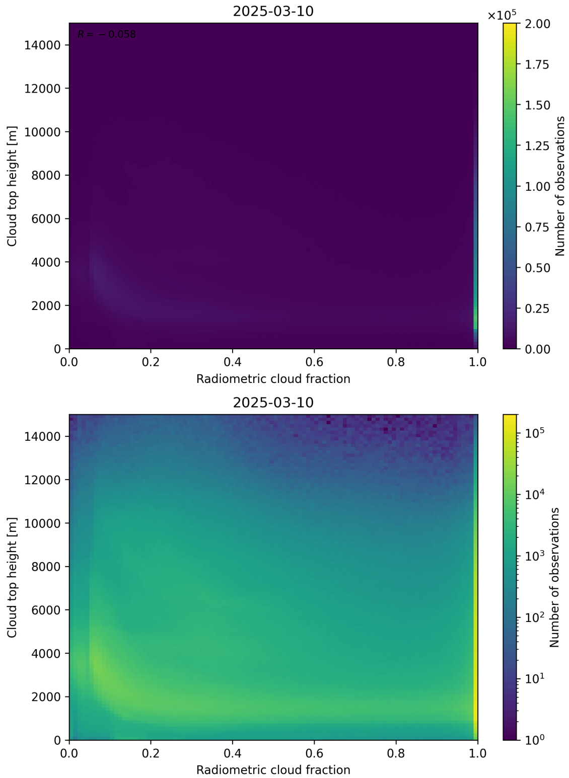
Figure 76: Scatter density plot of “Radiometric cloud fraction” against “Cloud top height” for 2025-03-09 to 2025-03-11.
