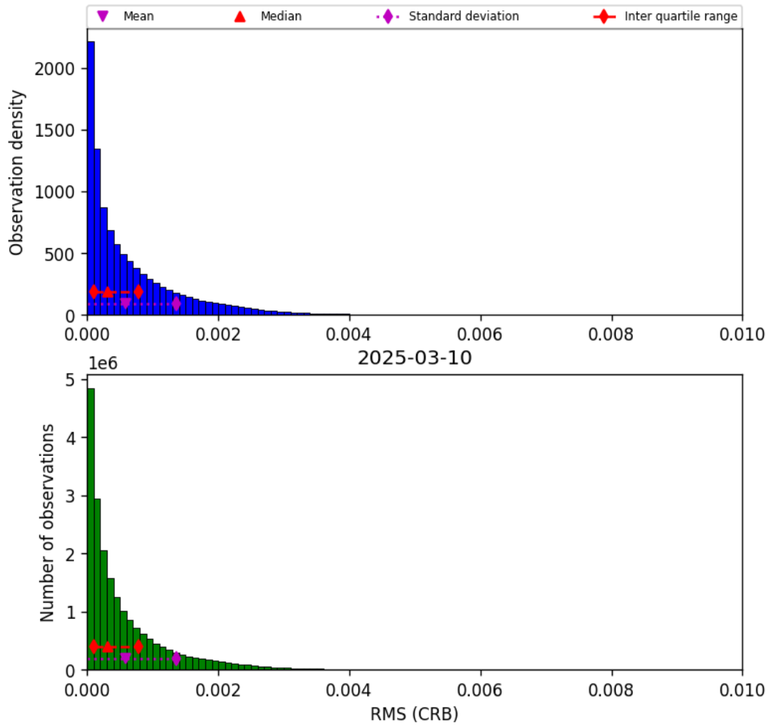
Figure 48: Histogram of “RMS (CRB)” for 2025-03-09 to 2025-03-11
