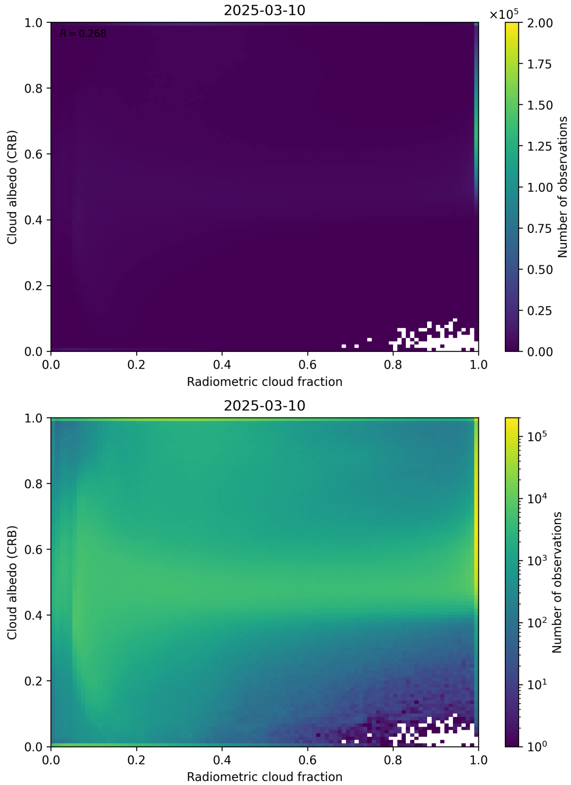
Figure 71: Scatter density plot of “Radiometric cloud fraction” against “Cloud albedo (CRB)” for 2025-03-09 to 2025-03-11.
