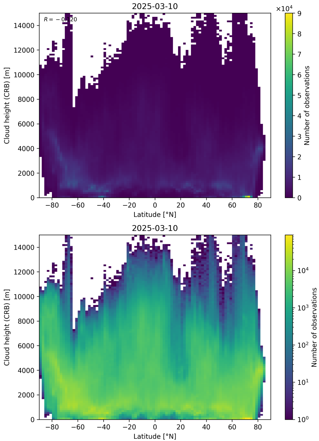
Figure 95: Scatter density plot of “Latitude” against “Cloud height (CRB)” for 2025-03-09 to 2025-03-11.
