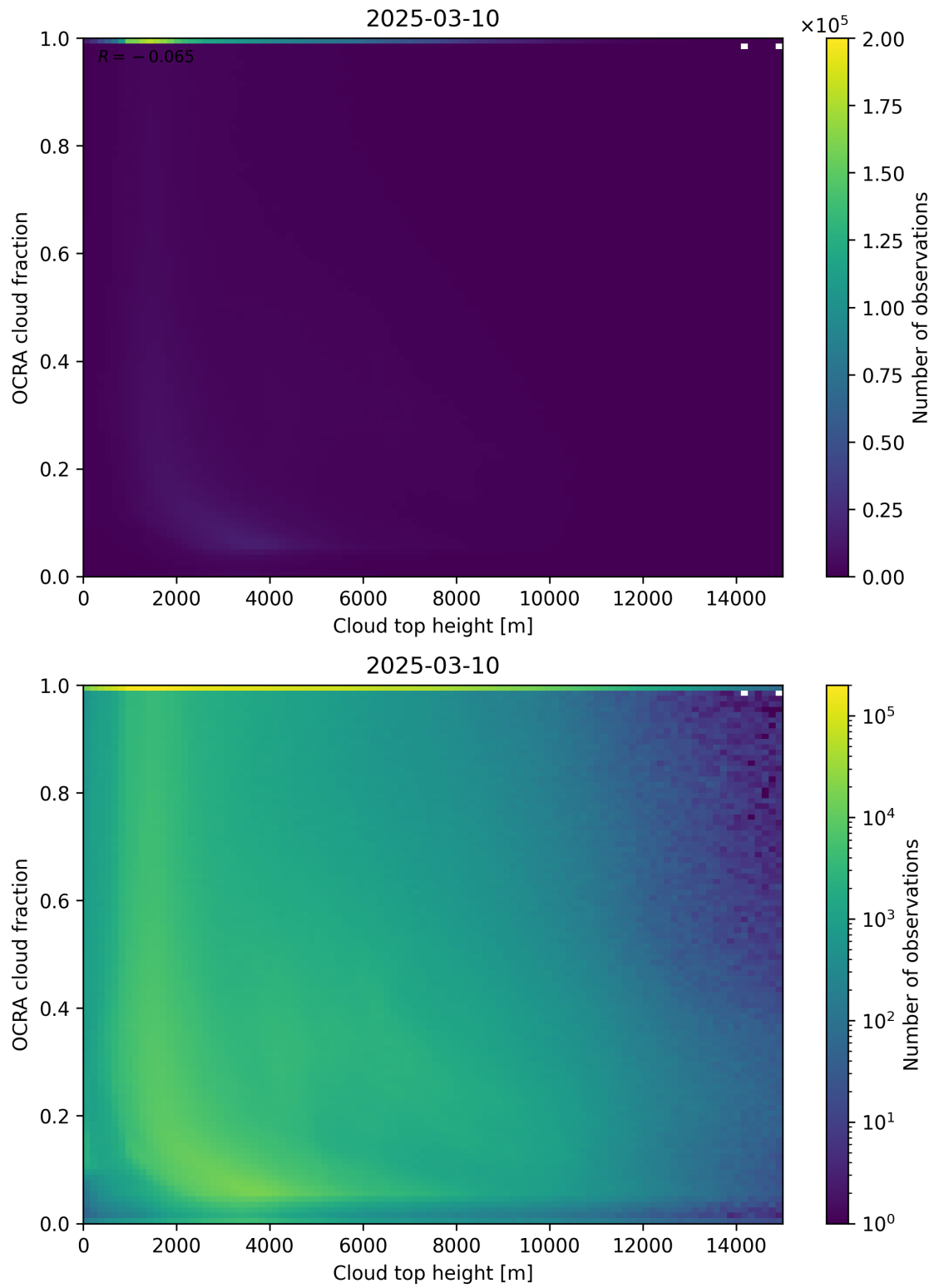
Figure 87: Scatter density plot of “Cloud top height” against “OCRA cloud fraction” for 2025-03-09 to 2025-03-11.
