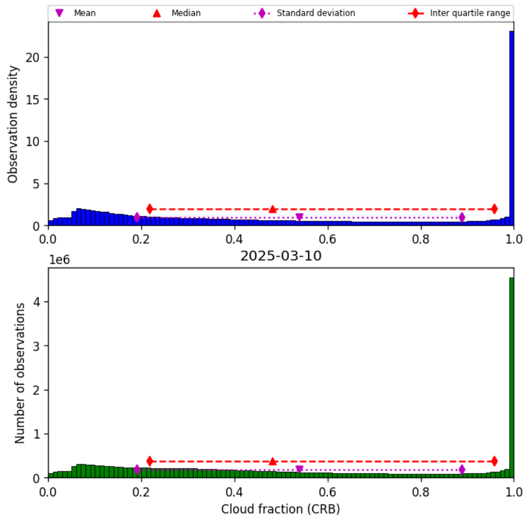
Figure 42: Histogram of “Cloud fraction (CRB)” for 2025-03-09 to 2025-03-11
