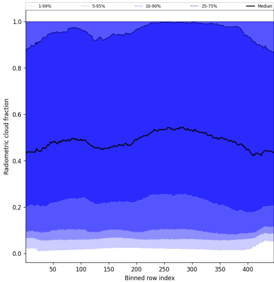
Figure 55: Along track statistics of “Radiometric cloud fraction” for 2025-03-09 to 2025-03-11
