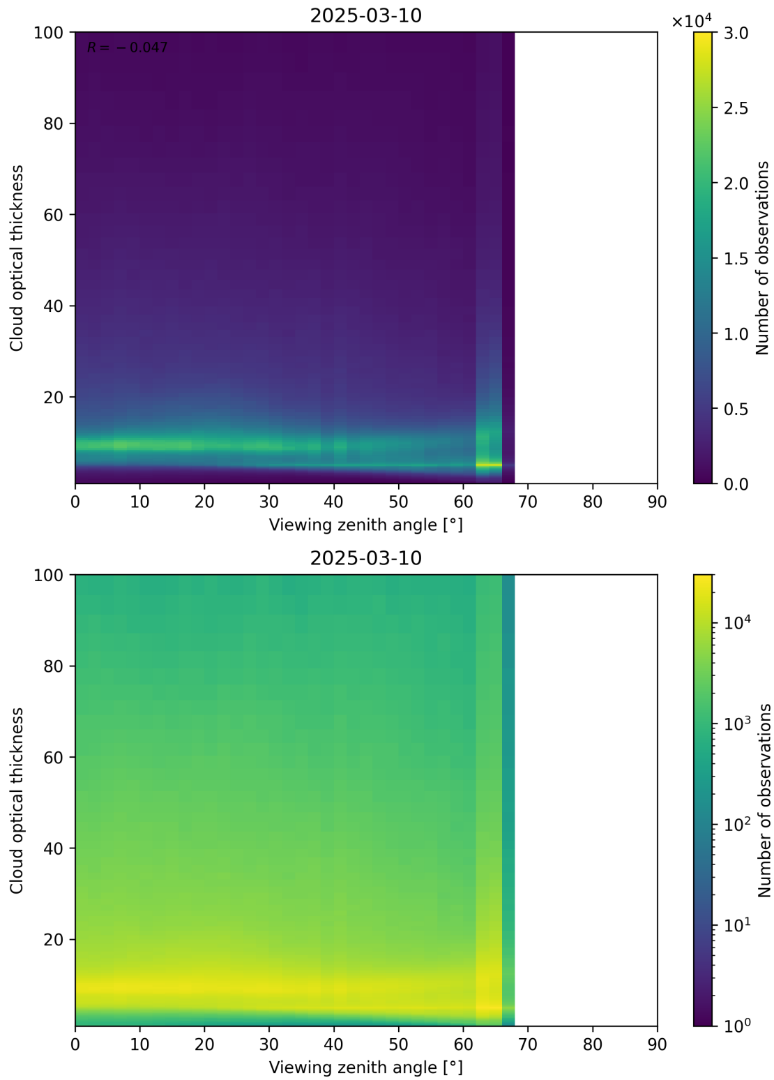
Figure 111: Scatter density plot of “Viewing zenith angle” against “Cloud optical thickness” for 2025-03-09 to 2025-03-11.
