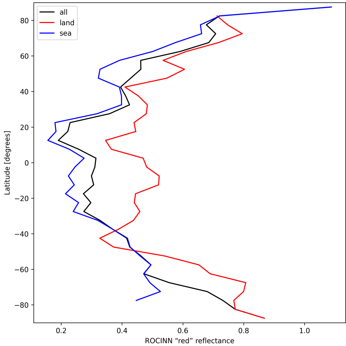
Figure 37: Zonal average of “ROCINN “red” reflectance” for 2025-03-09 to 2025-03-11.
