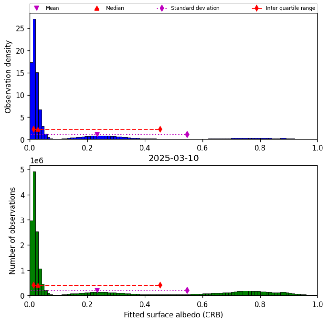
Figure 46: Histogram of “Fitted surface albedo (CRB)” for 2025-03-09 to 2025-03-11
