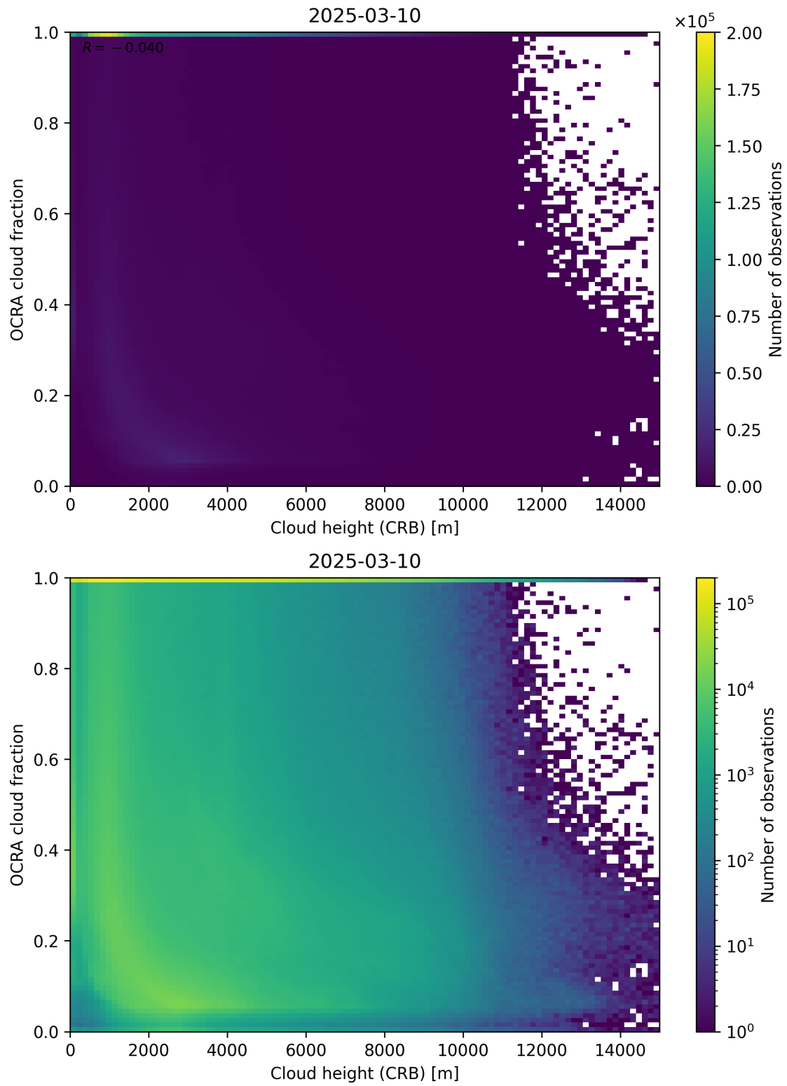
Figure 81: Scatter density plot of “Cloud height (CRB)” against “OCRA cloud fraction” for 2025-03-09 to 2025-03-11.
