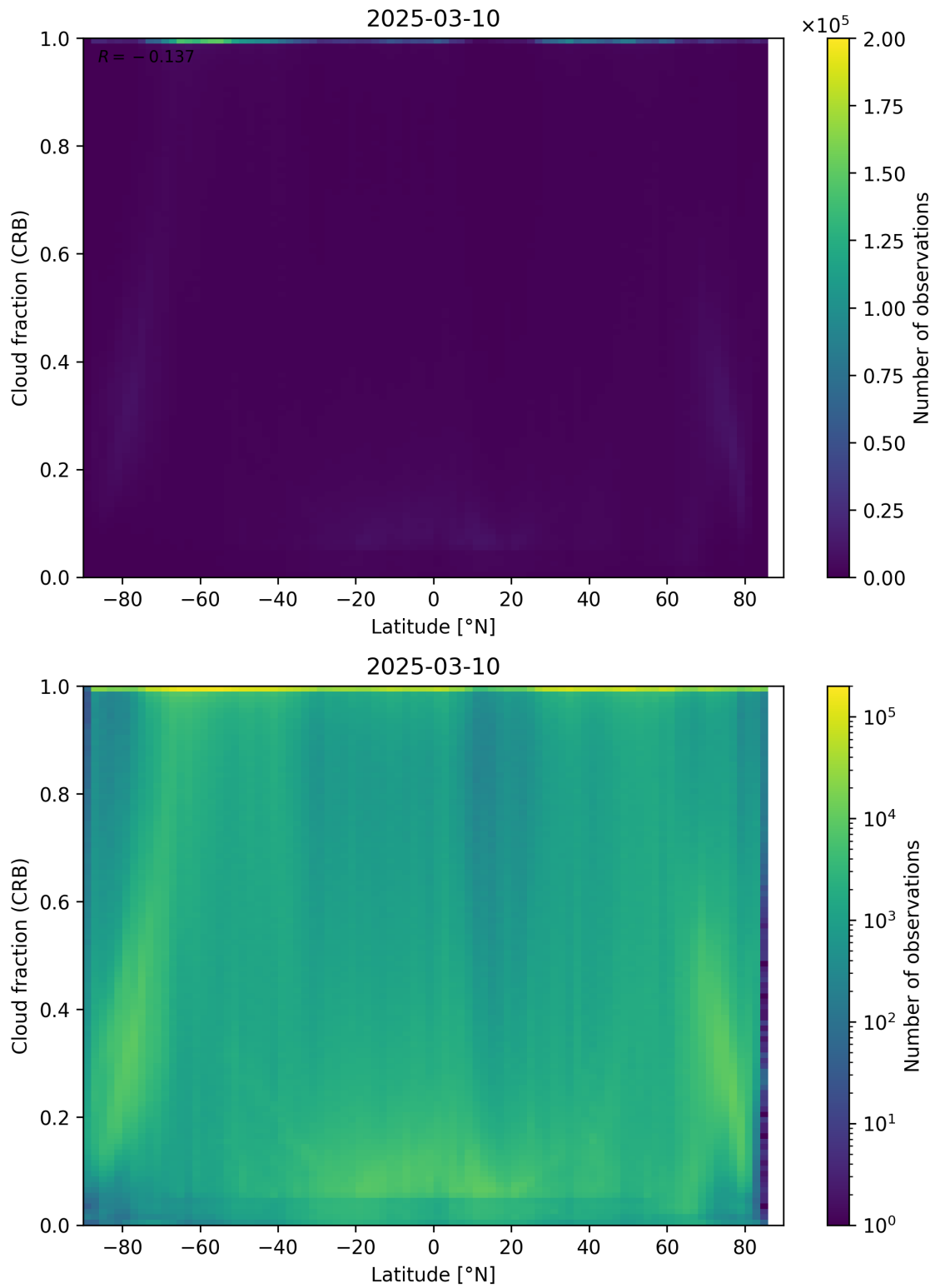
Figure 94: Scatter density plot of “Latitude” against “Cloud fraction (CRB)” for 2025-03-09 to 2025-03-11.
