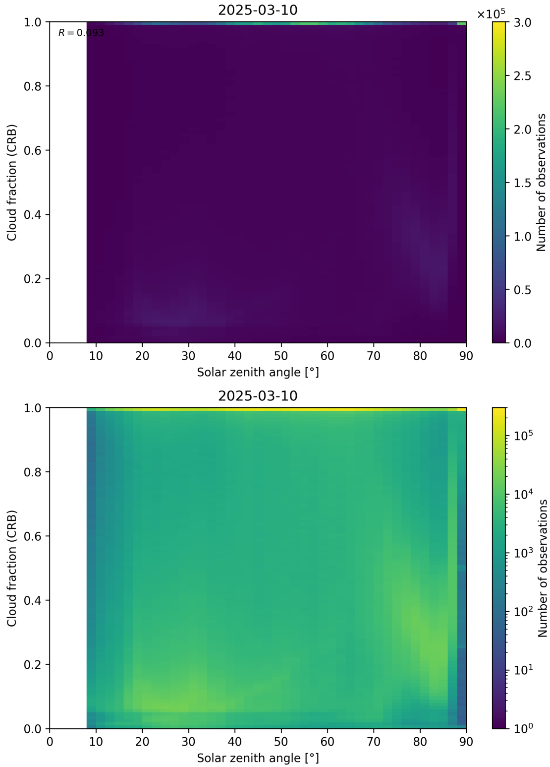
Figure 101: Scatter density plot of “Solar zenith angle” against “Cloud fraction (CRB)” for 2025-03-09 to 2025-03-11.
