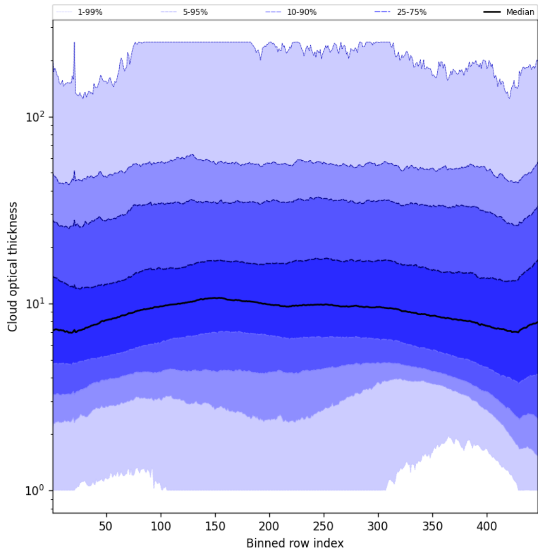
Figure 57: Along track statistics of “Cloud optical thickness” for 2025-03-09 to 2025-03-11
