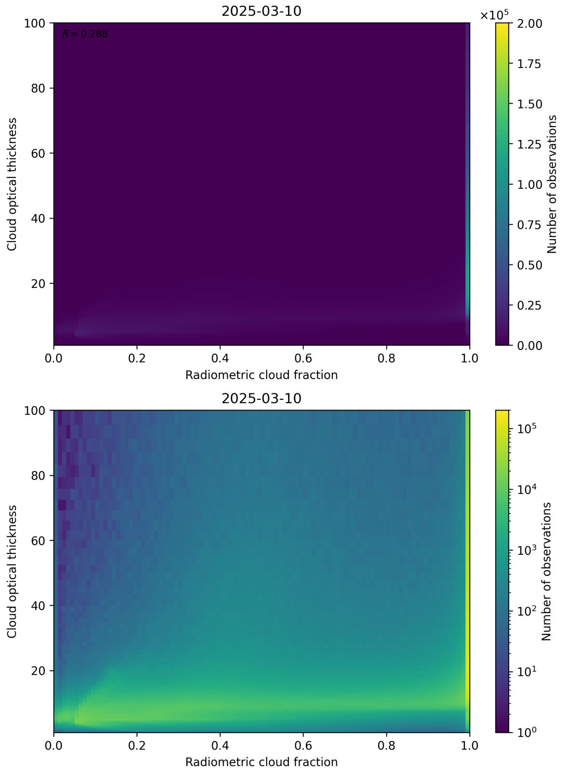
Figure 75: Scatter density plot of “Radiometric cloud fraction” against “Cloud optical thickness” for 2025-03-09 to 2025-03-11.
