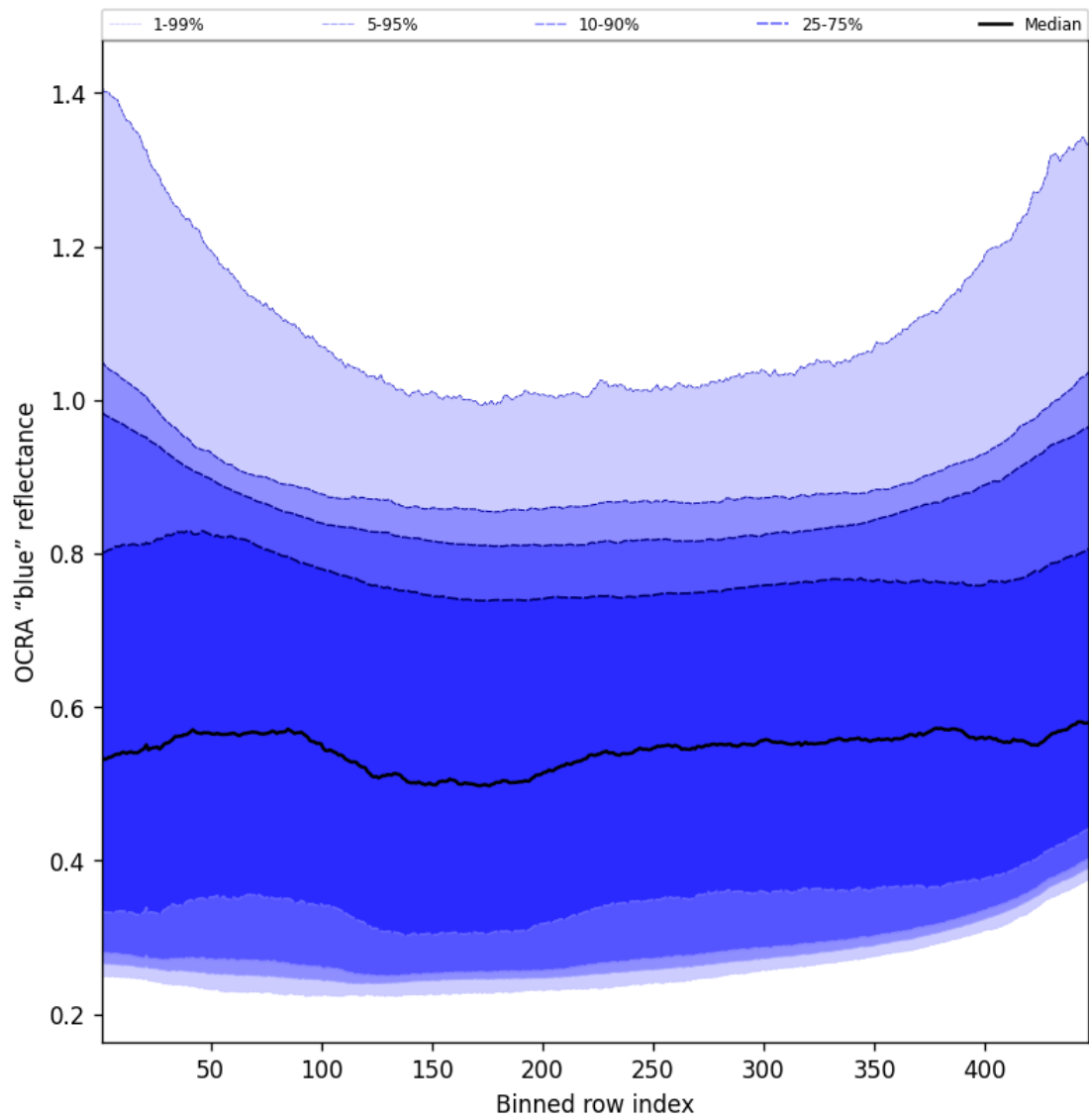
Figure 67: Along track statistics of “OCRA “blue” reflectance” for 2025-03-09 to 2025-03-11
