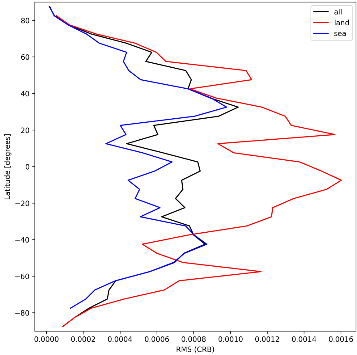
Figure 32: Zonal average of “RMS (CRB)” for 2025-03-09 to 2025-03-11.
