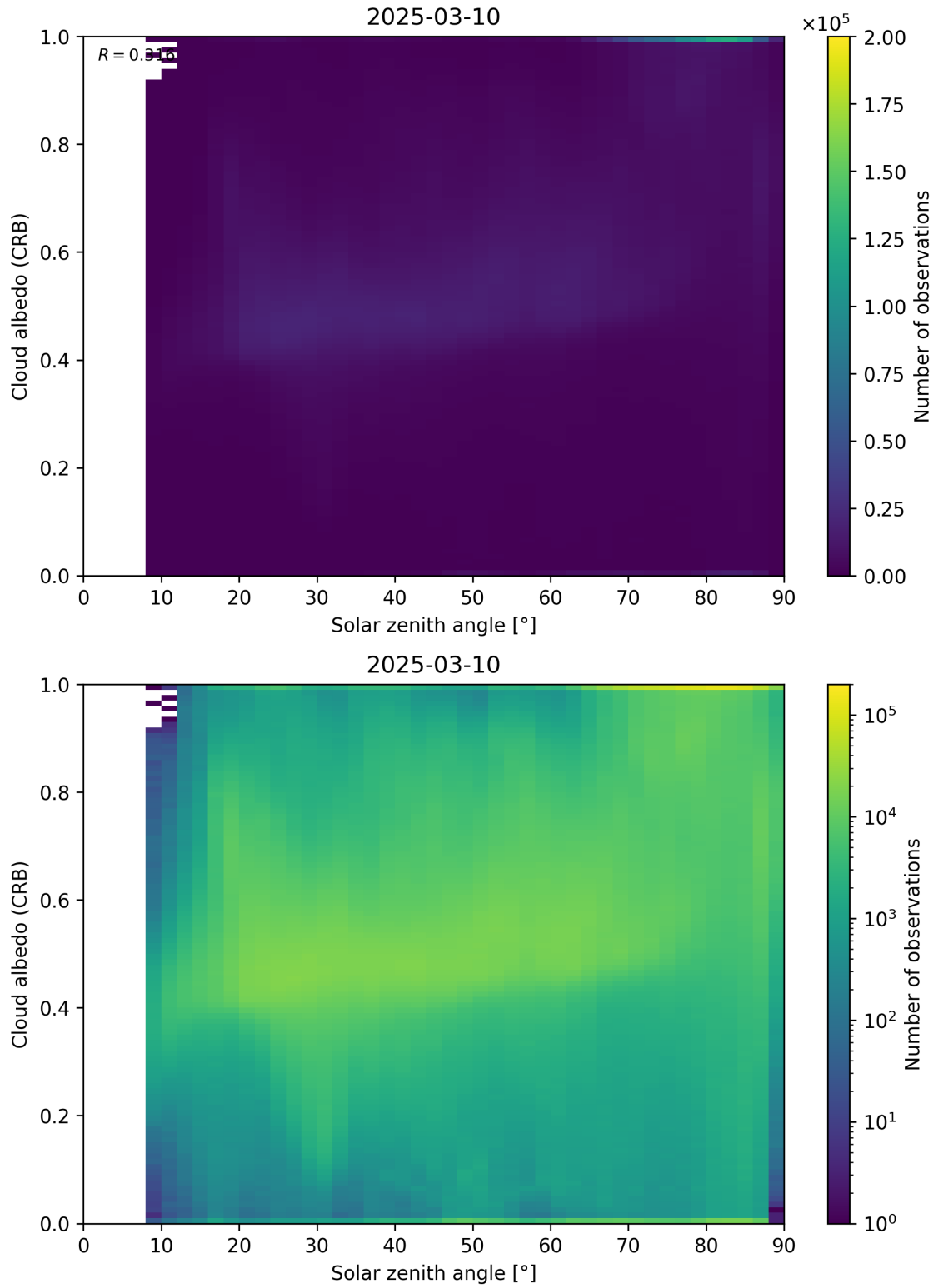
Figure 98: Scatter density plot of “Solar zenith angle” against “Cloud albedo (CRB)” for 2025-03-09 to 2025-03-11.
