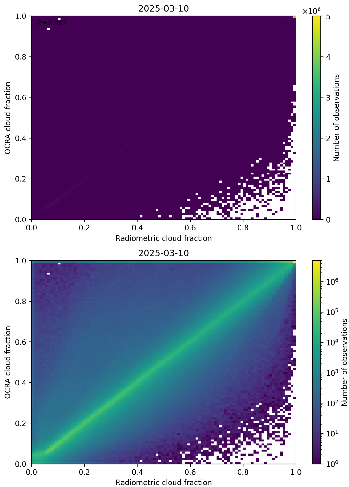
Figure 72: Scatter density plot of “Radiometric cloud fraction” against “OCRA cloud fraction” for 2025-03-09 to 2025-03-11.
