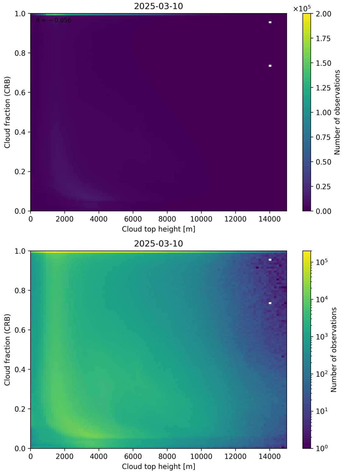
Figure 88: Scatter density plot of “Cloud top height” against “Cloud fraction (CRB)” for 2025-03-09 to 2025-03-11.
