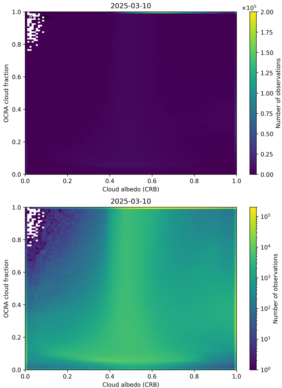
Figure 70: Scatter density plot of “Cloud albedo (CRB)” against “OCRA cloud fraction” for 2025-03-09 to 2025-03-11.
