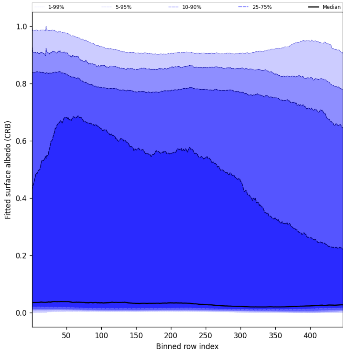
Figure 62: Along track statistics of “Fitted surface albedo (CRB)” for 2025-03-09 to 2025-03-11
