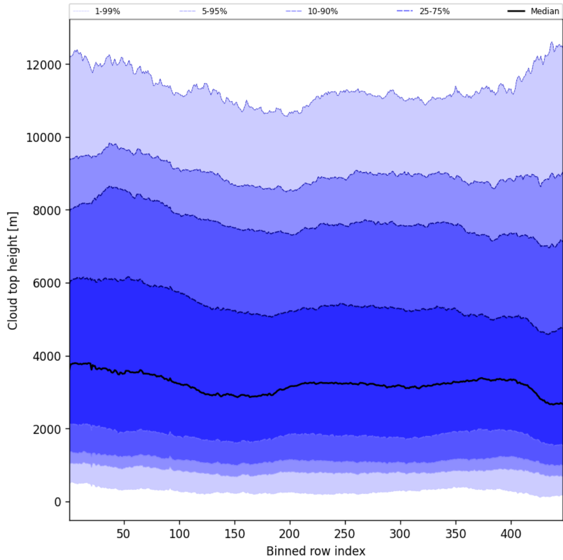
Figure 56: Along track statistics of “Cloud top height” for 2025-03-09 to 2025-03-11
