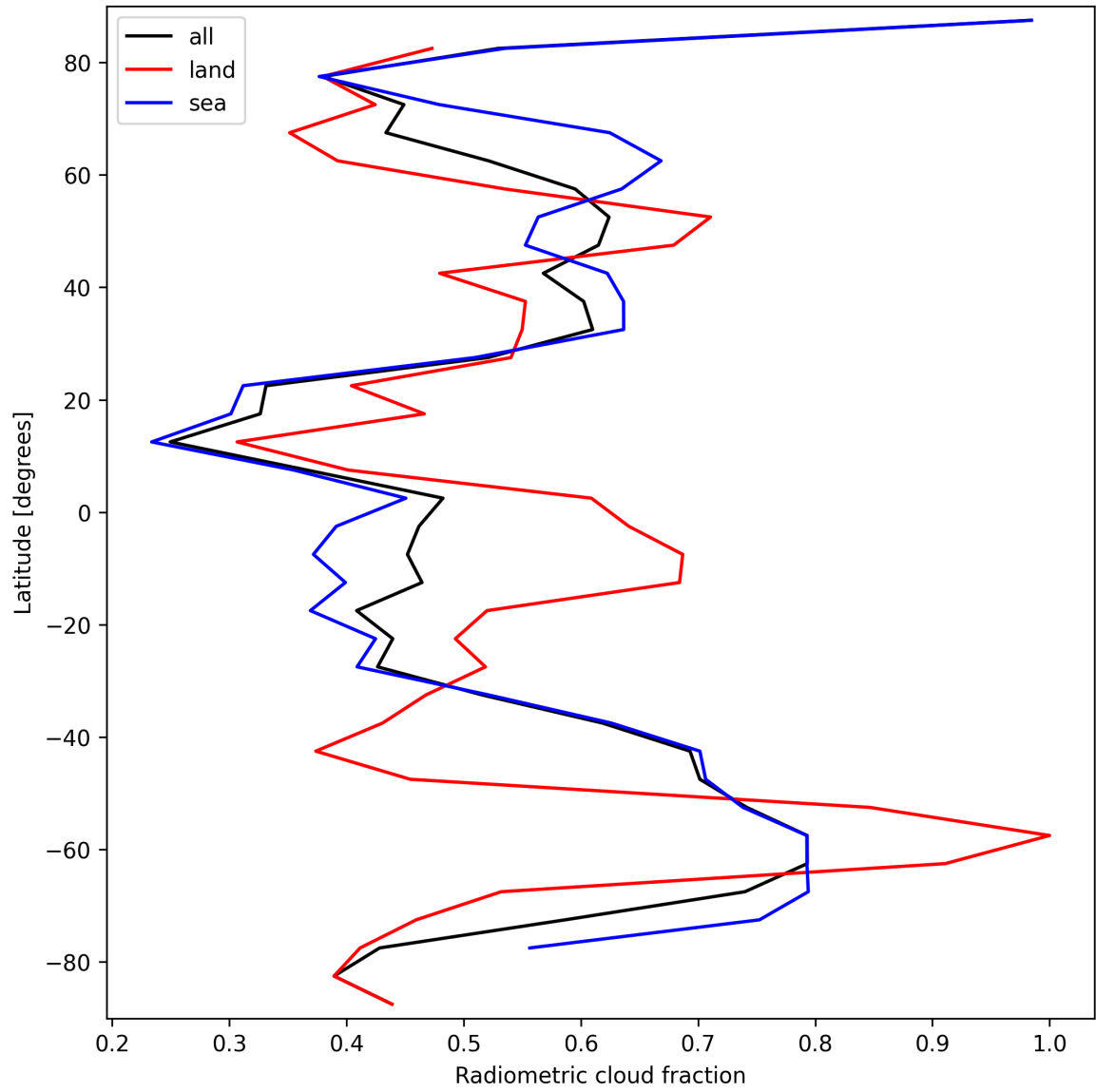
Figure 23: Zonal average of “Radiometric cloud fraction” for 2025-03-09 to 2025-03-11.
