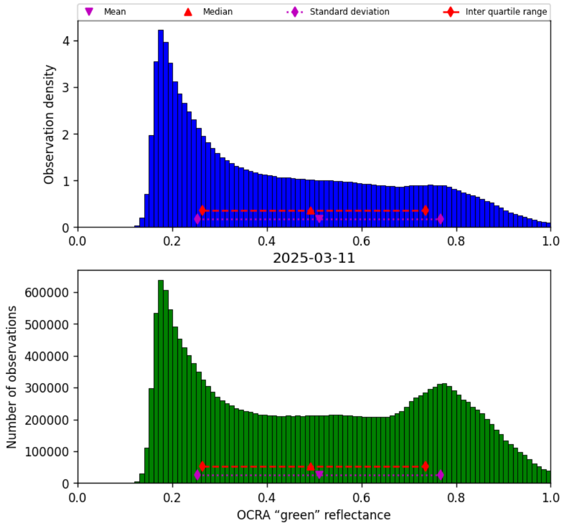
Figure 52: Histogram of “OCRA “green” reflectance” for 2025-03-10 to 2025-03-12
