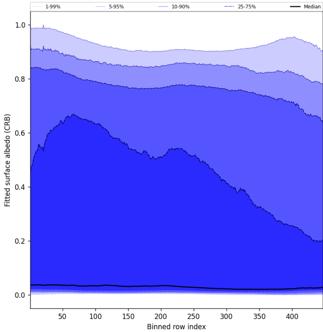
Figure 62: Along track statistics of “Fitted surface albedo (CRB)” for 2025-03-10 to 2025-03-12
