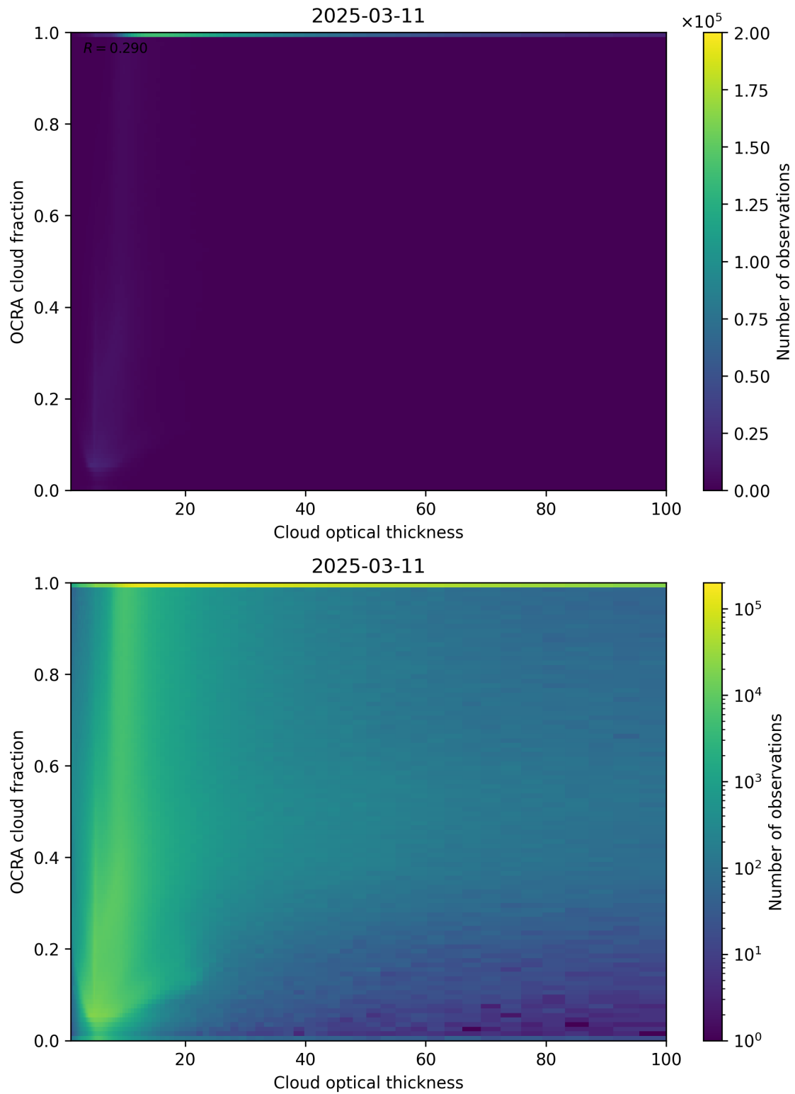
Figure 83: Scatter density plot of “Cloud optical thickness” against “OCRA cloud fraction” for 2025-03-10 to 2025-03-12.
