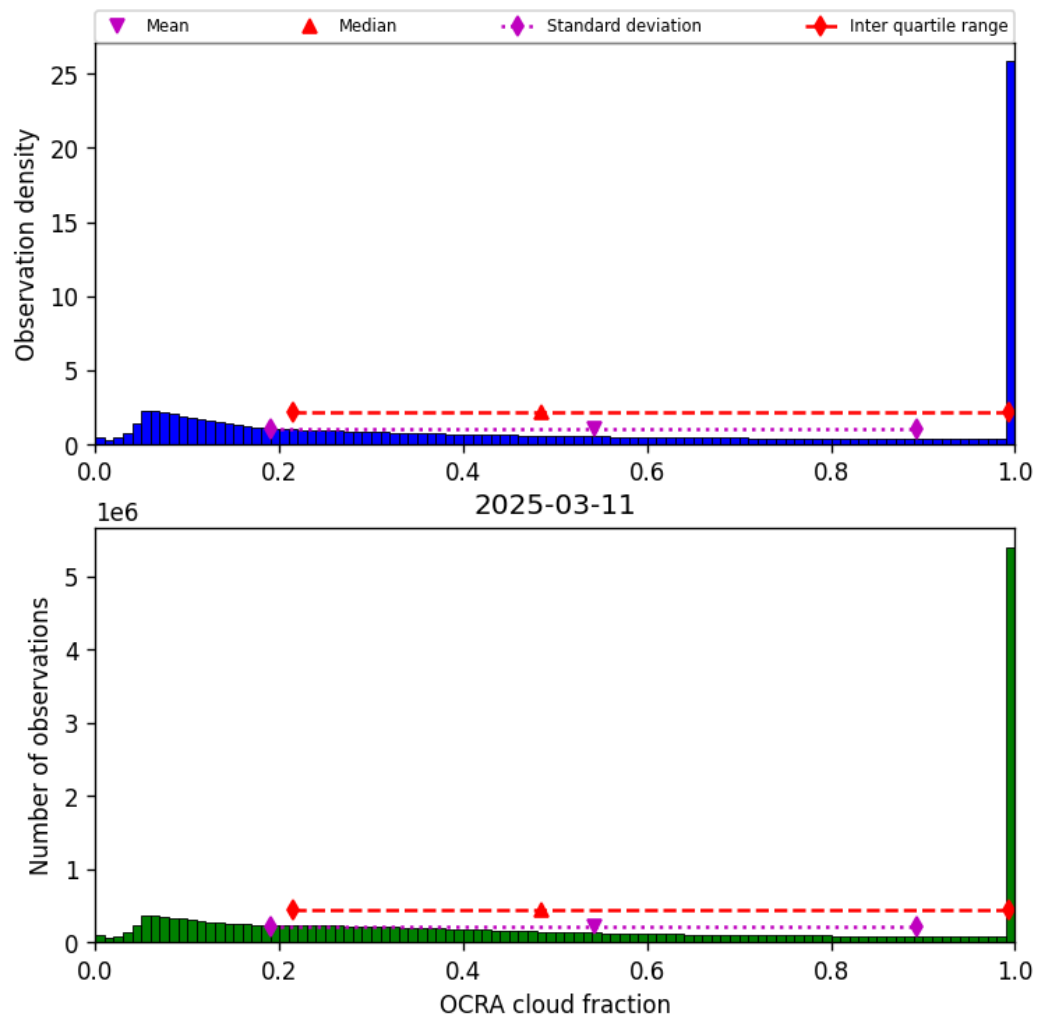
Figure 50: Histogram of “OCRA cloud fraction” for 2025-03-10 to 2025-03-12
