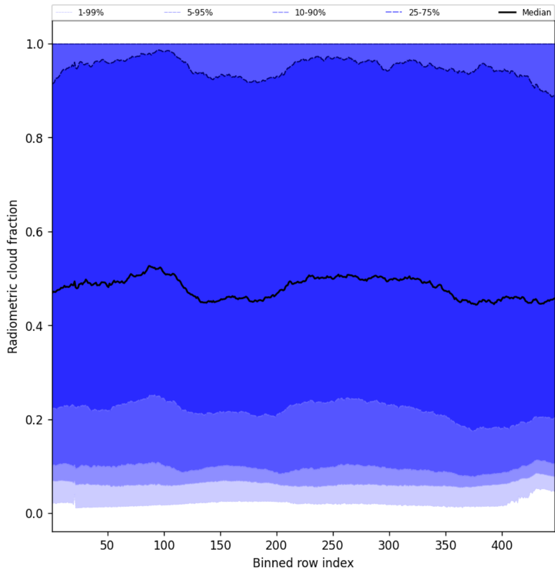
Figure 55: Along track statistics of “Radiometric cloud fraction” for 2025-03-10 to 2025-03-12
