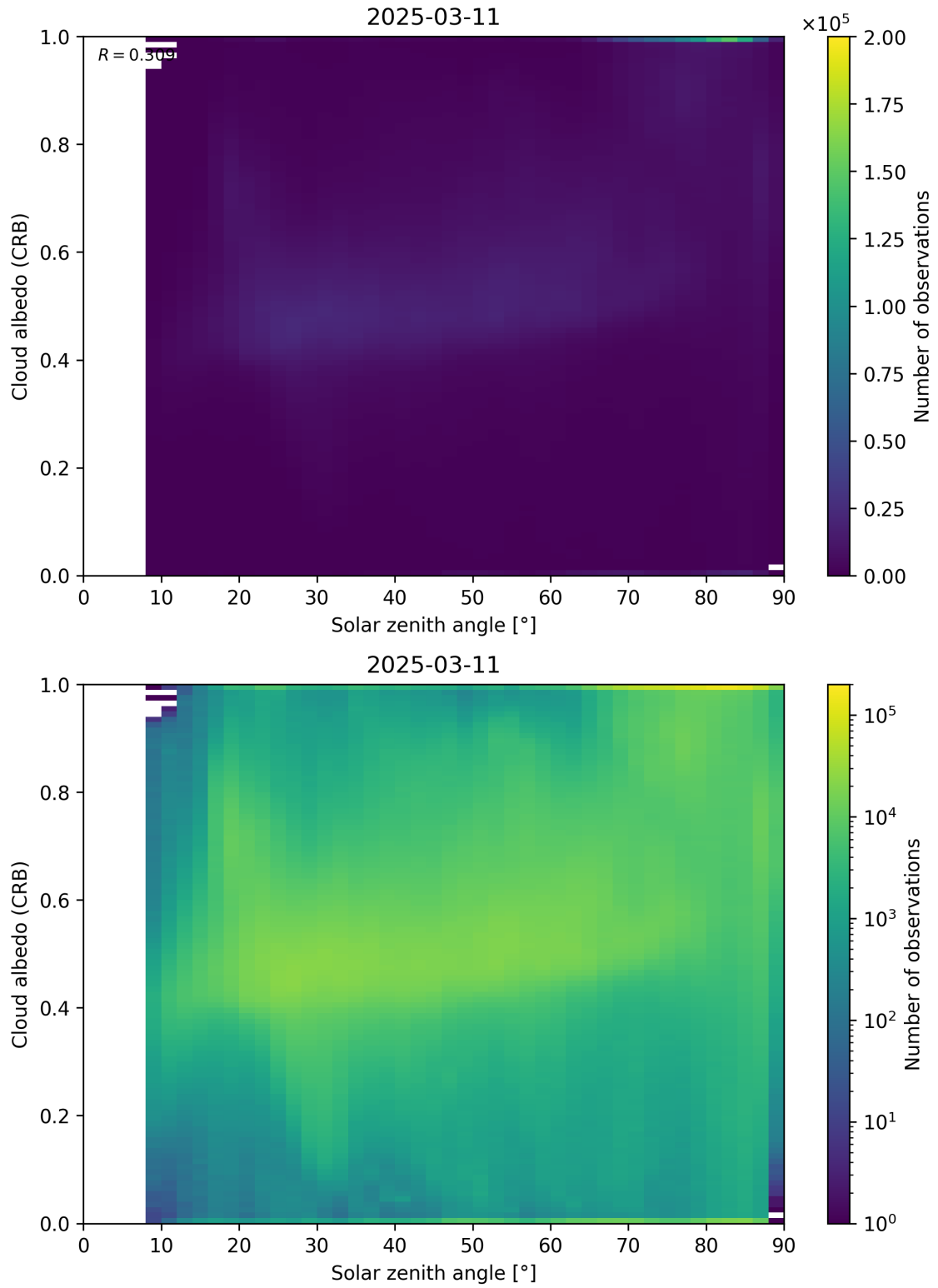
Figure 98: Scatter density plot of “Solar zenith angle” against “Cloud albedo (CRB)” for 2025-03-10 to 2025-03-12.
