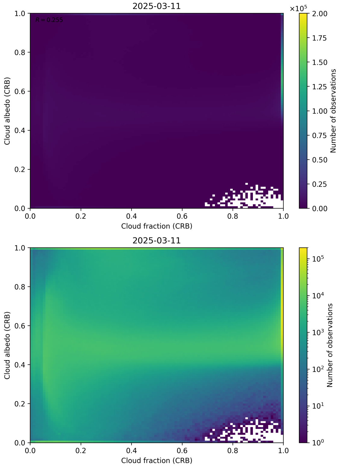
Figure 77: Scatter density plot of “Cloud fraction (CRB)” against “Cloud albedo (CRB)” for 2025-03-10 to 2025-03-12.
