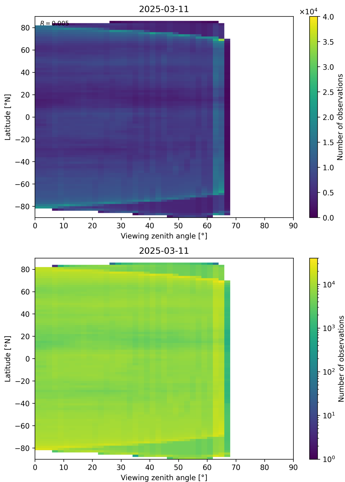
Figure 113: Scatter density plot of “Viewing zenith angle” against “Latitude” for 2025-03-10 to 2025-03-12.
