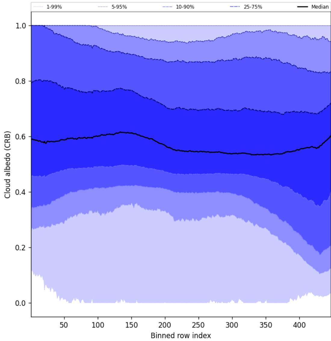
Figure 60: Along track statistics of “Cloud albedo (CRB)” for 2025-03-10 to 2025-03-12
