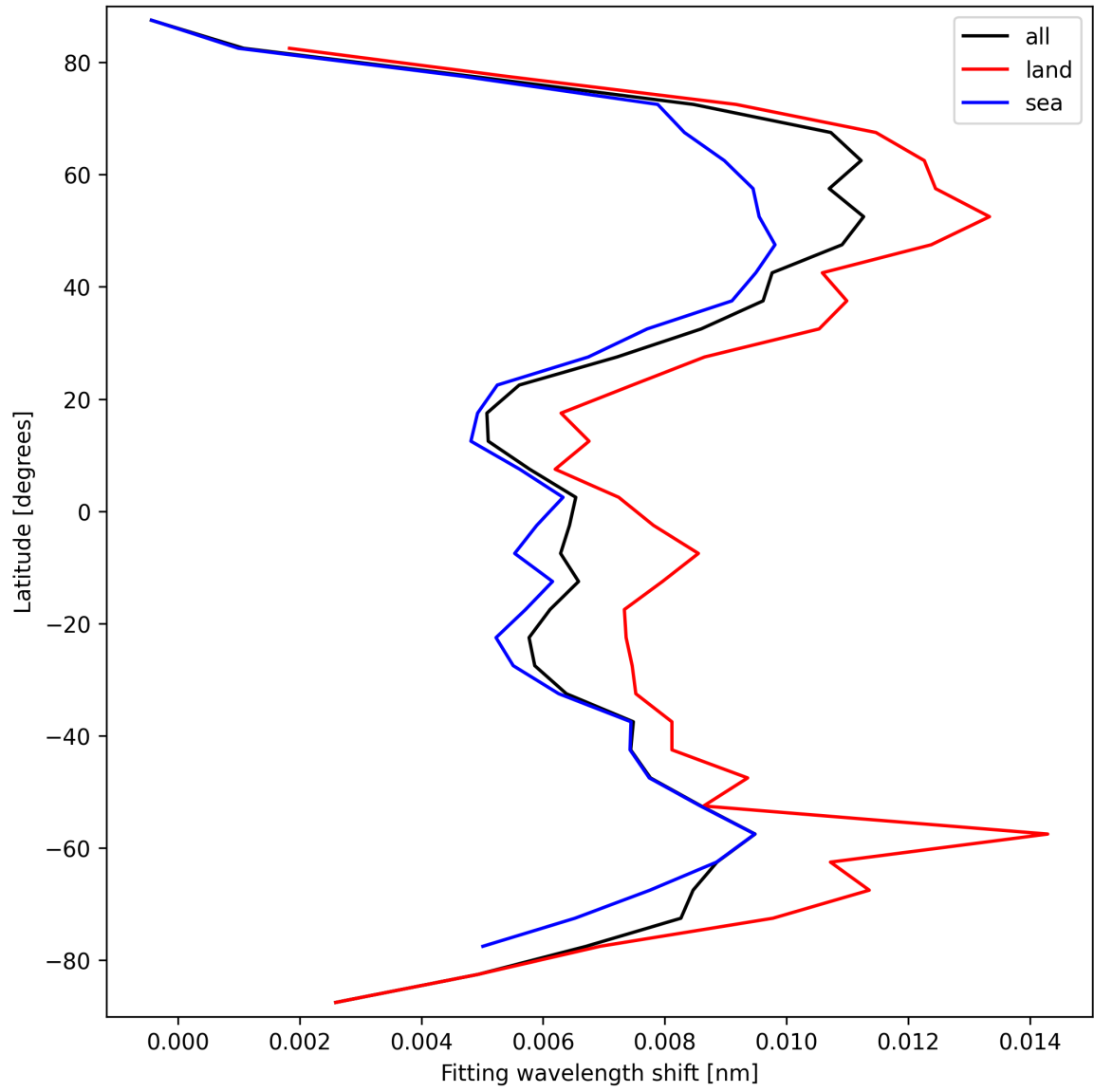
Figure 33: Zonal average of “Fitting wavelength shift” for 2025-03-10 to 2025-03-12.
