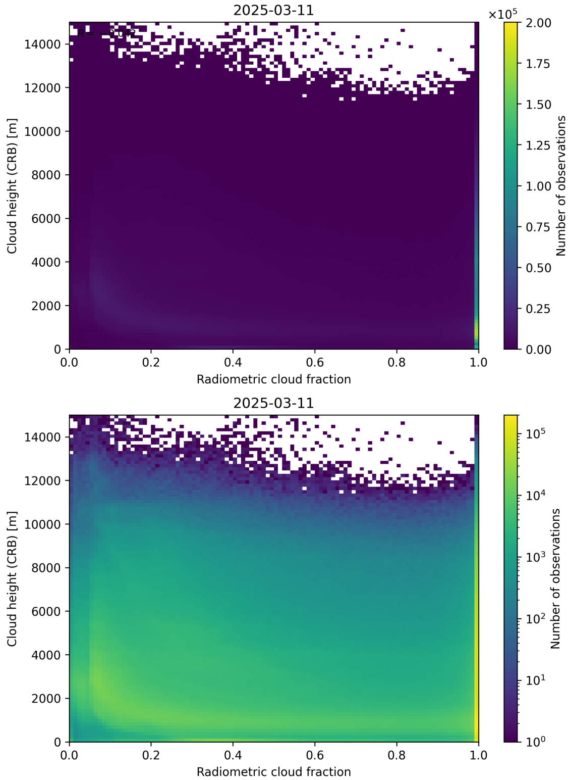
Figure 74: Scatter density plot of “Radiometric cloud fraction” against “Cloud height (CRB)” for 2025-03-10 to 2025-03-12.
