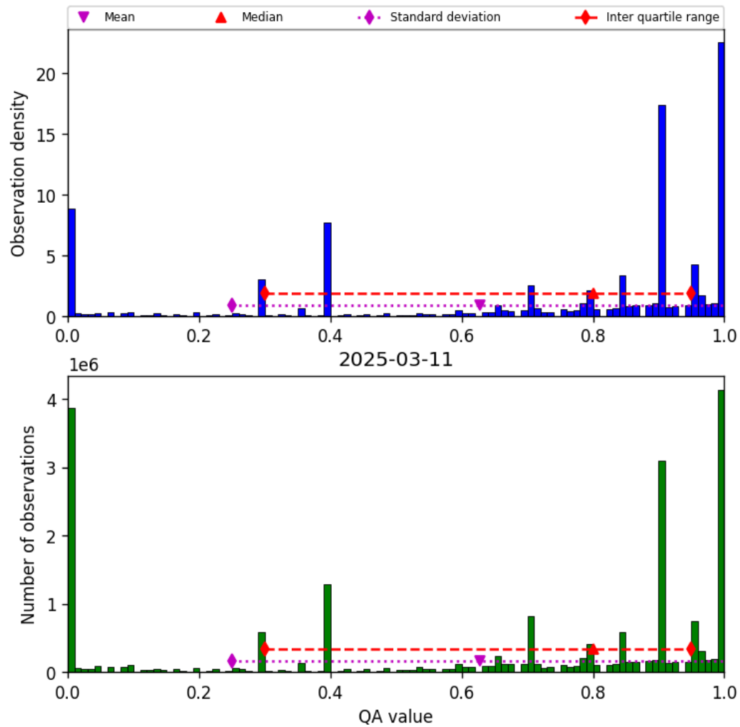
Figure 38: Histogram of “QA value” for 2025-03-10 to 2025-03-12
