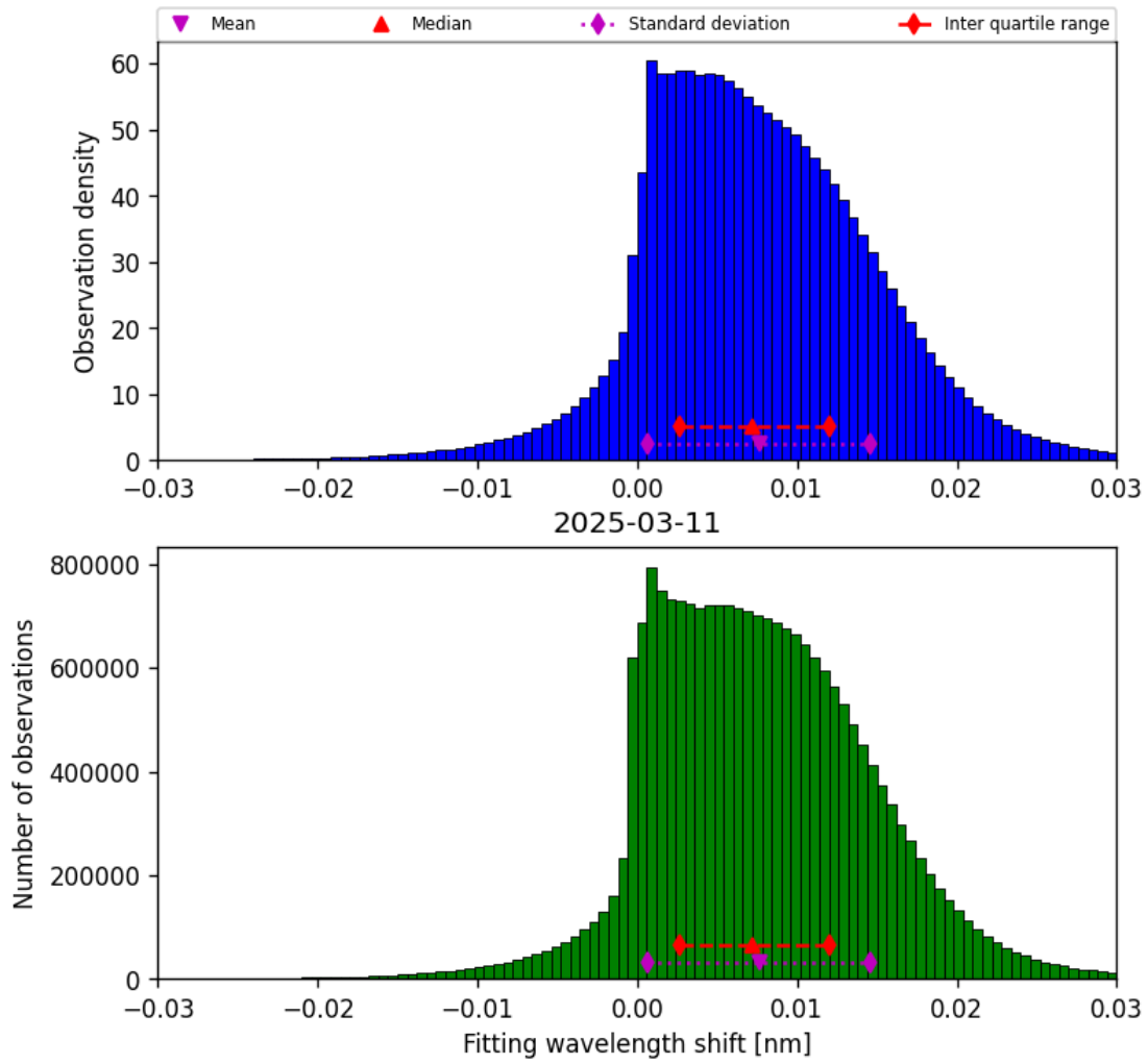
Figure 49: Histogram of “Fitting wavelength shift” for 2025-03-10 to 2025-03-12
