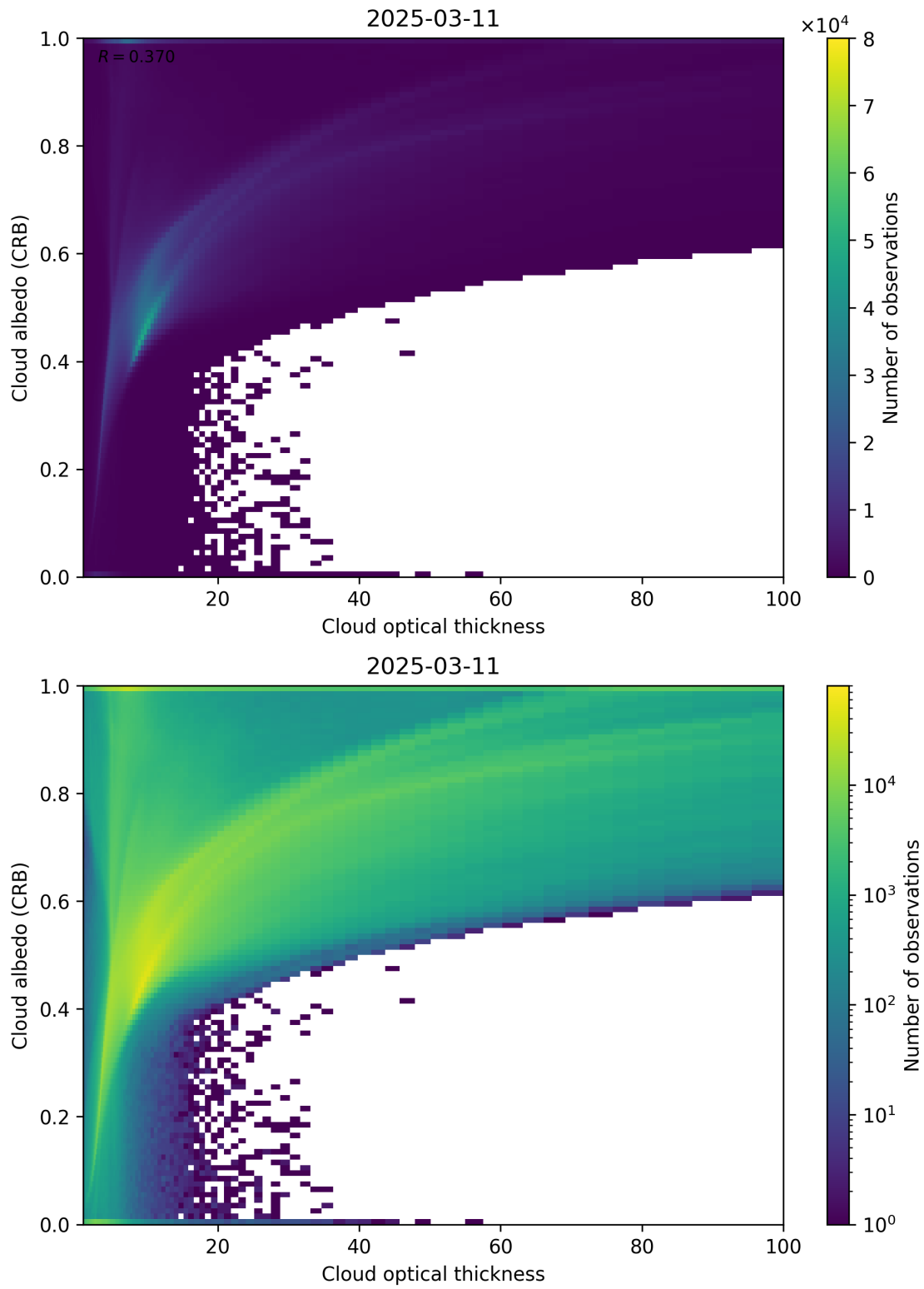
Figure 82: Scatter density plot of “Cloud optical thickness” against “Cloud albedo (CRB)” for 2025-03-10 to 2025-03-12.
