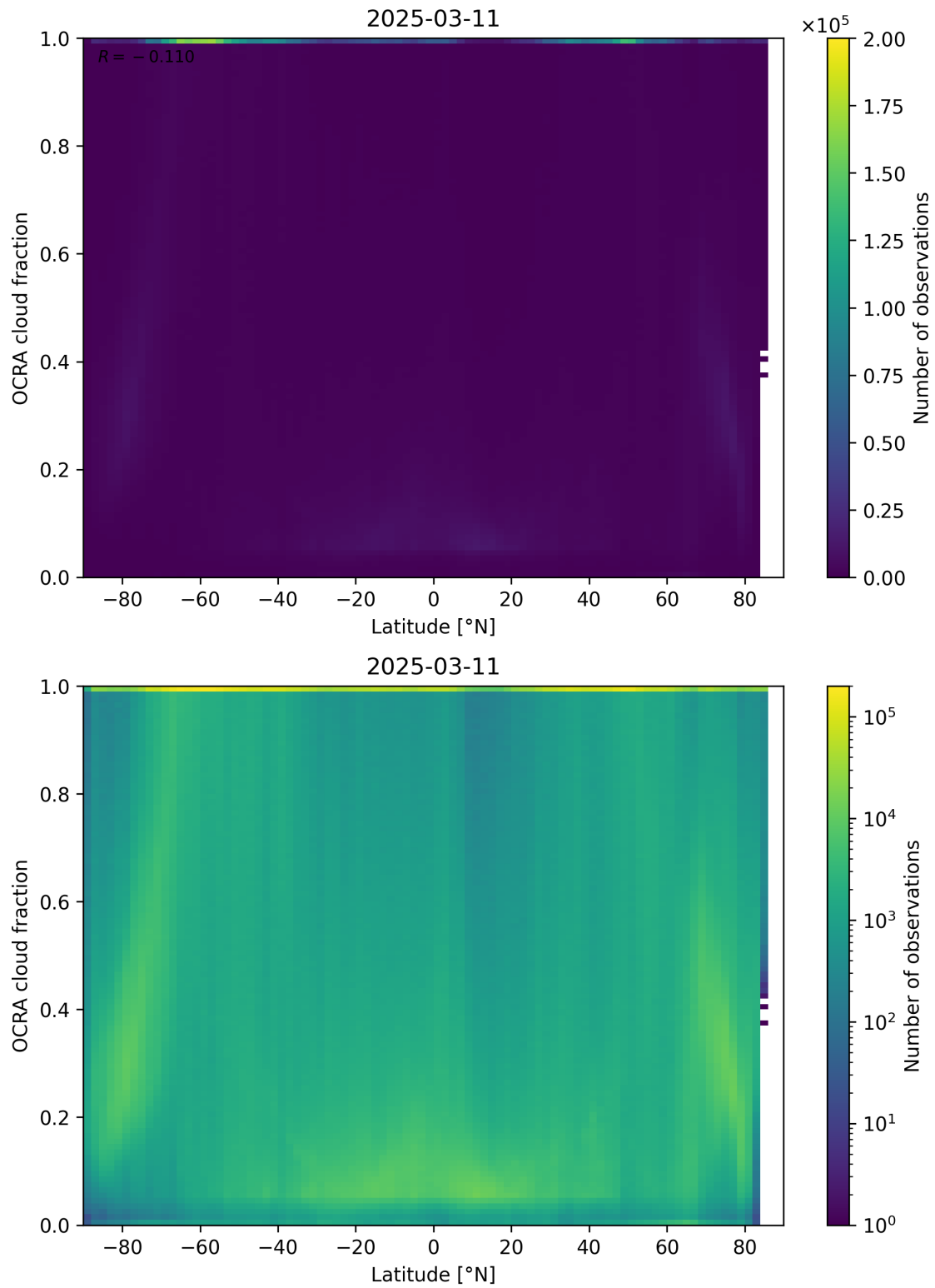
Figure 93: Scatter density plot of “Latitude” against “OCRA cloud fraction” for 2025-03-10 to 2025-03-12.
