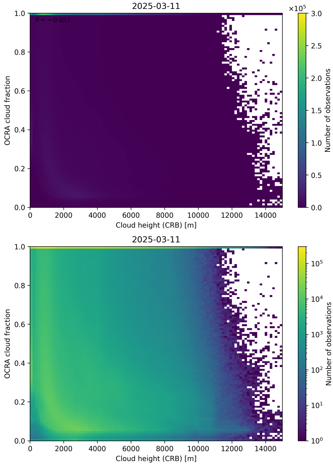
Figure 81: Scatter density plot of “Cloud height (CRB)” against “OCRA cloud fraction” for 2025-03-10 to 2025-03-12.
