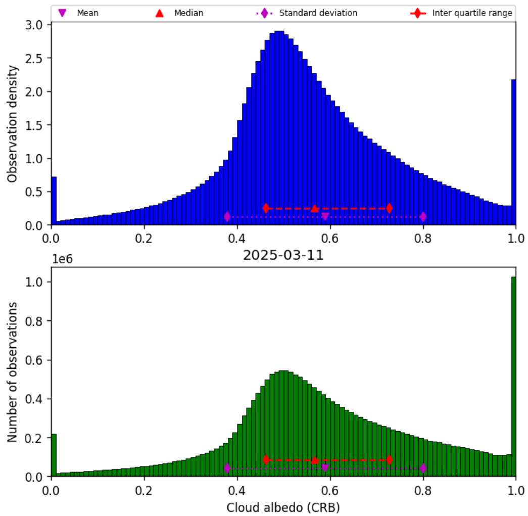
Figure 44: Histogram of “Cloud albedo (CRB)” for 2025-03-10 to 2025-03-12
