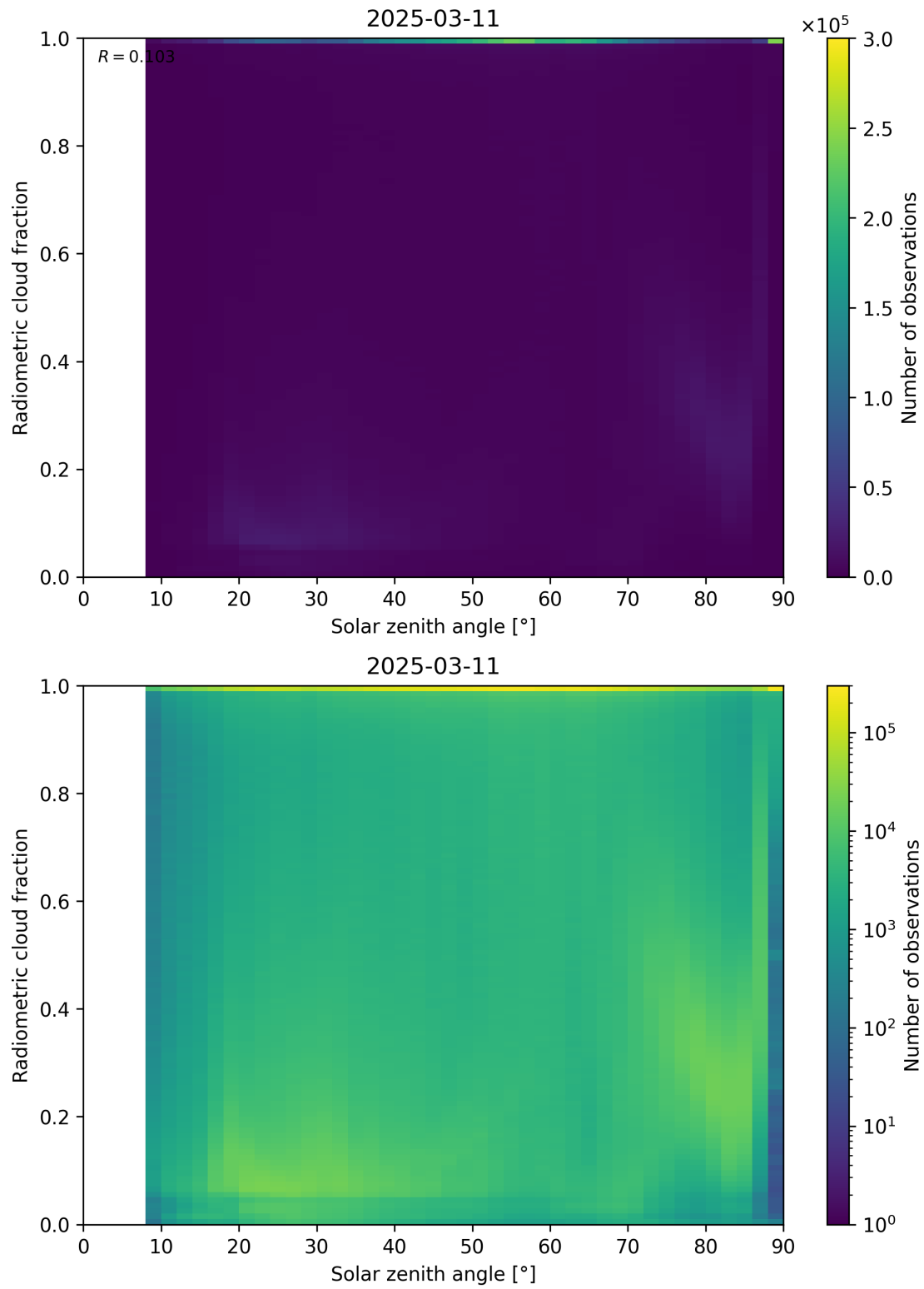
Figure 99: Scatter density plot of “Solar zenith angle” against “Radiometric cloud fraction” for 2025-03-10 to 2025-03-12.
