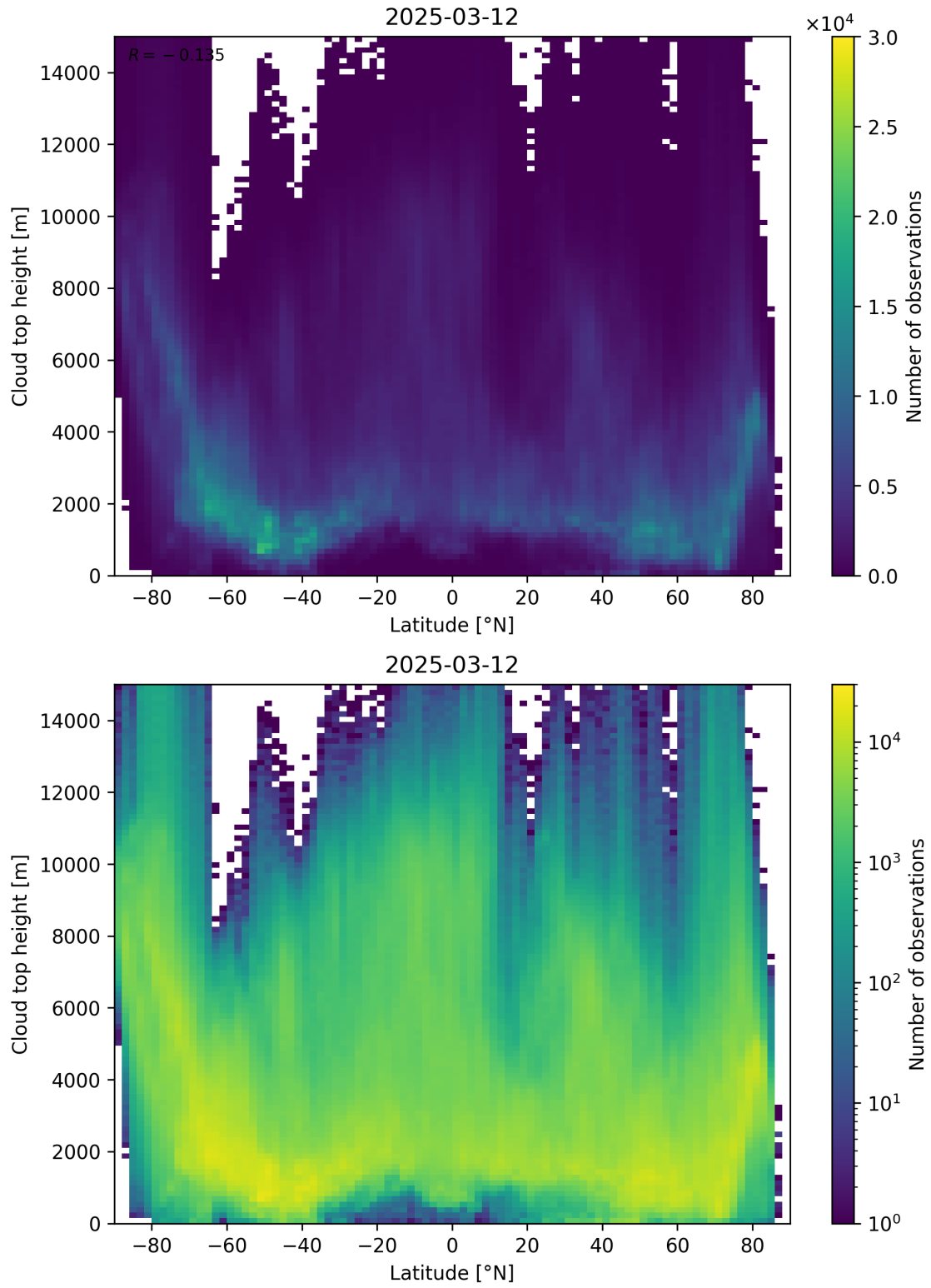
Figure 97: Scatter density plot of “Latitude” against “Cloud top height” for 2025-03-12 to 2025-03-13.
