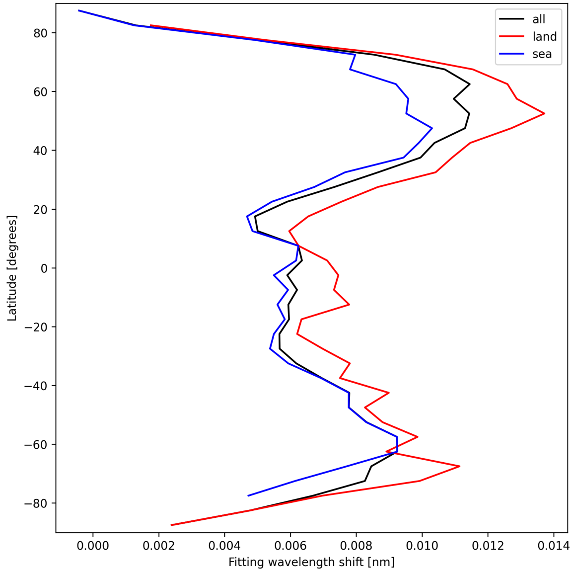
Figure 33: Zonal average of “Fitting wavelength shift” for 2025-03-12 to 2025-03-13.
