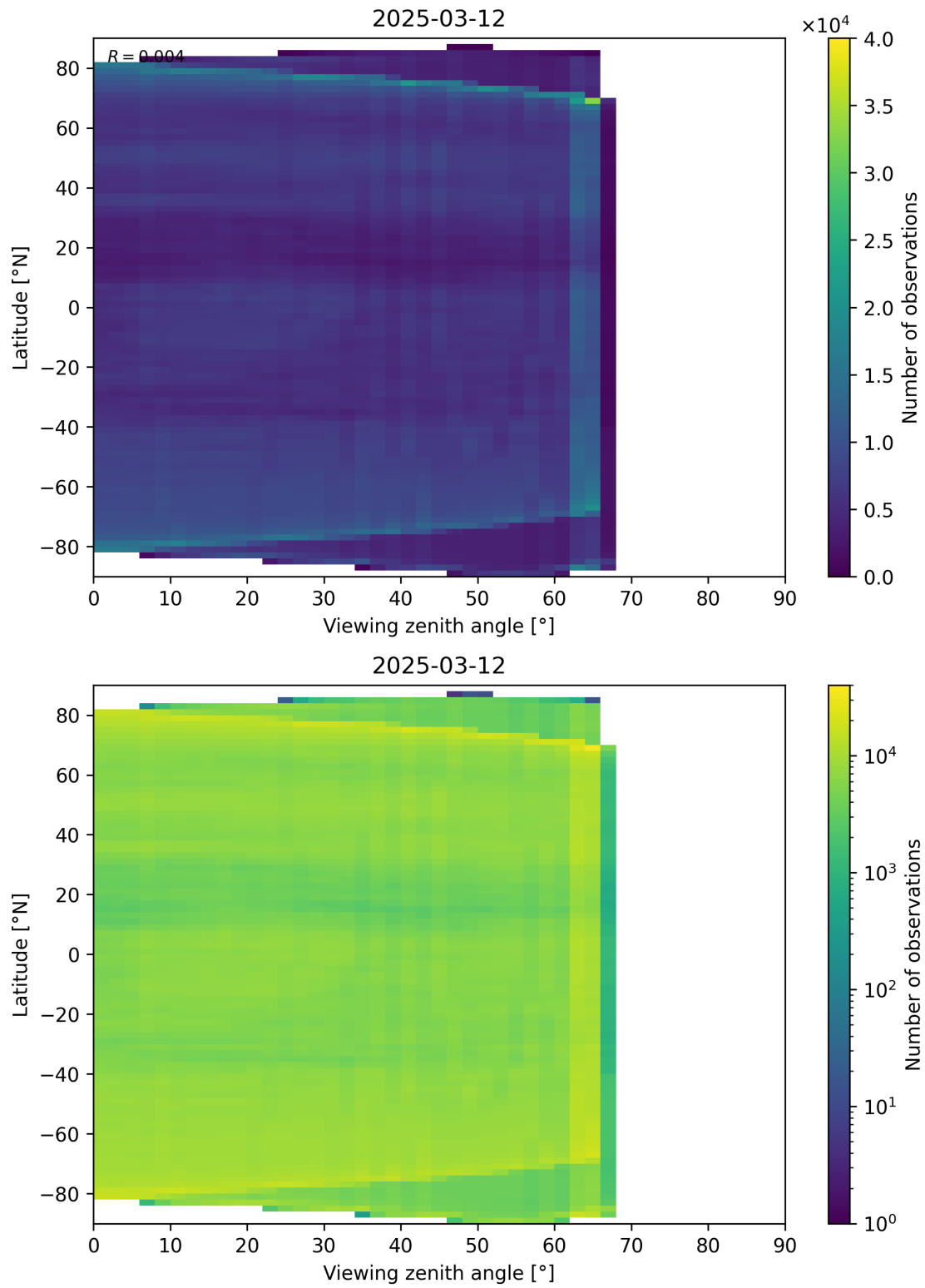
Figure 113: Scatter density plot of “Viewing zenith angle” against “Latitude” for 2025-03-12 to 2025-03-13.
