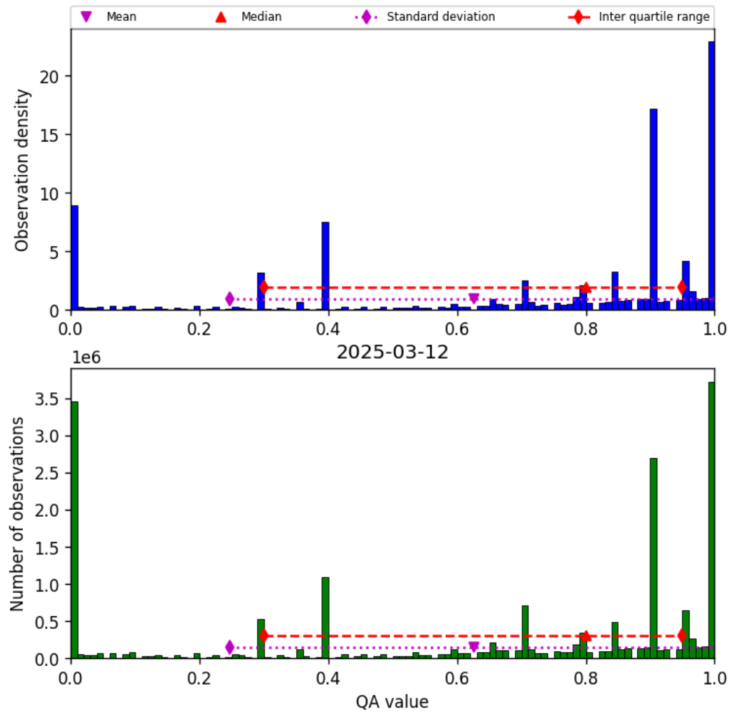
Figure 38: Histogram of “QA value” for 2025-03-12 to 2025-03-13
