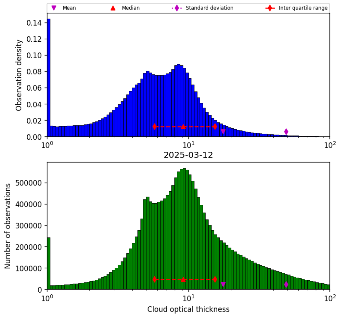
Figure 41: Histogram of “Cloud optical thickness” for 2025-03-12 to 2025-03-13
