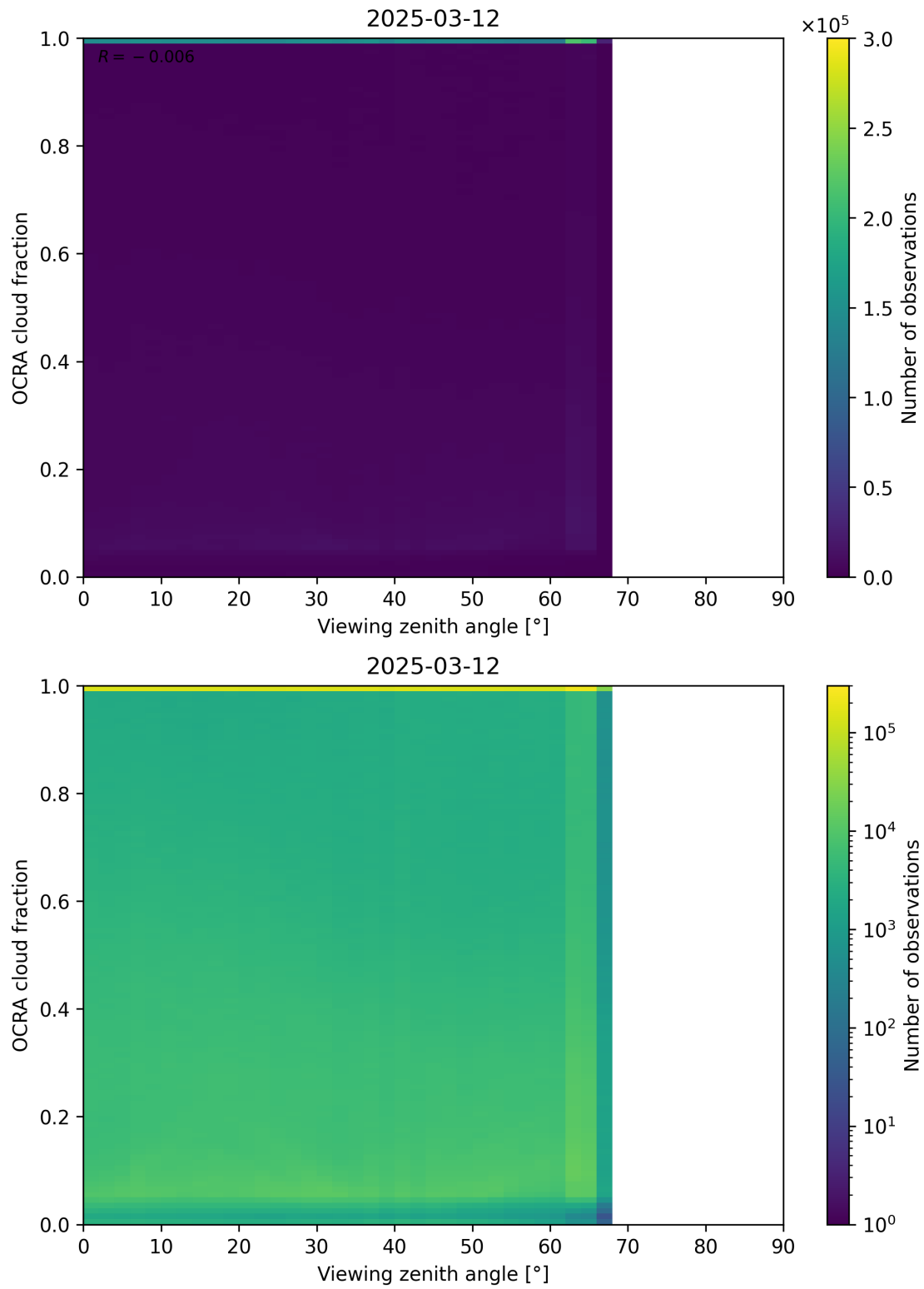
Figure 108: Scatter density plot of “Viewing zenith angle” against “OCRA cloud fraction” for 2025-03-12 to 2025-03-13.
