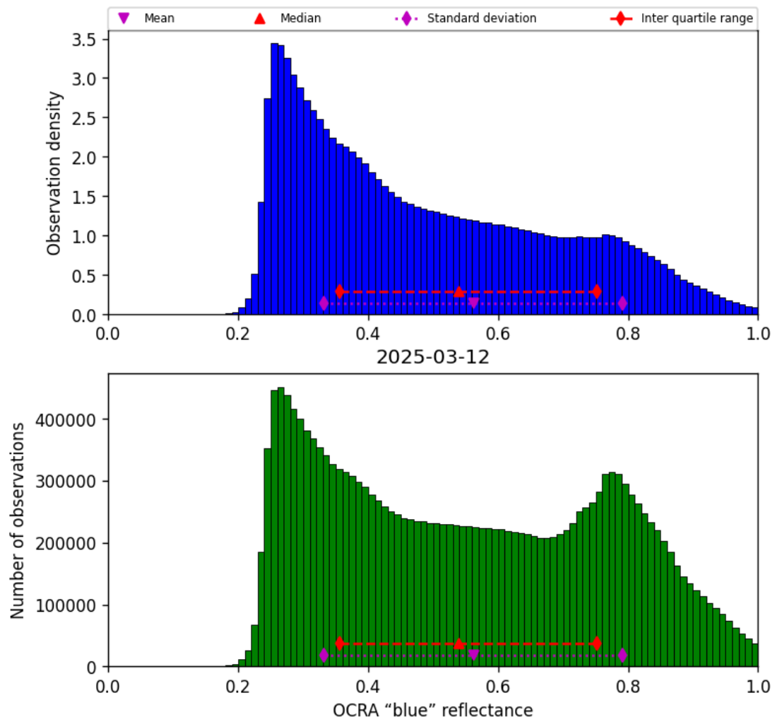
Figure 51: Histogram of “OCRA “blue” reflectance” for 2025-03-12 to 2025-03-13
