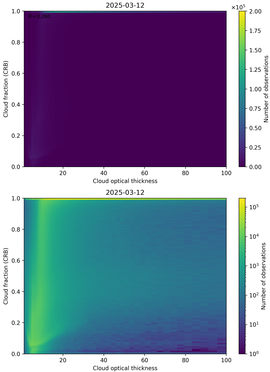
Figure 84: Scatter density plot of “Cloud optical thickness” against “Cloud fraction (CRB)” for 2025-03-12 to 2025-03-13.
