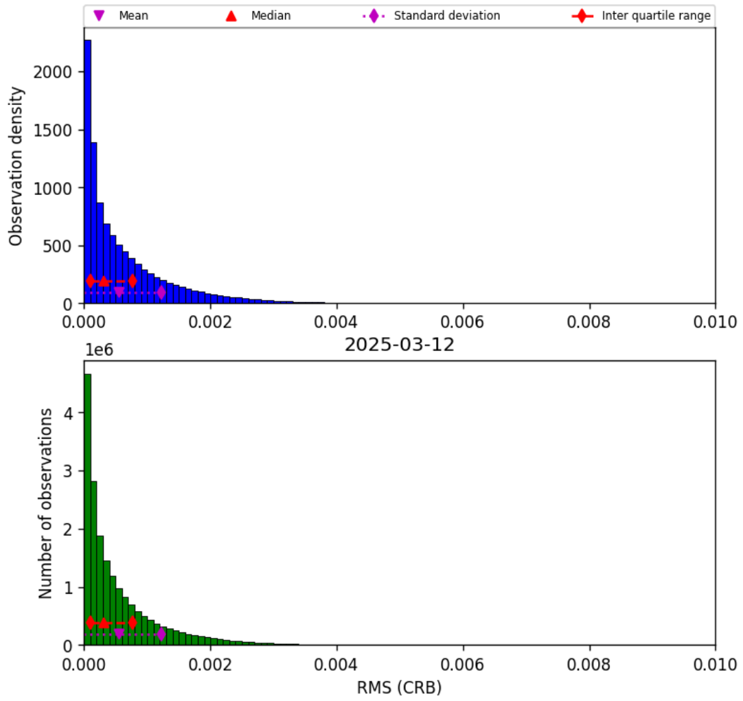
Figure 48: Histogram of "RMS (CRB)" for 2025-03-12 to 2025-03-13
