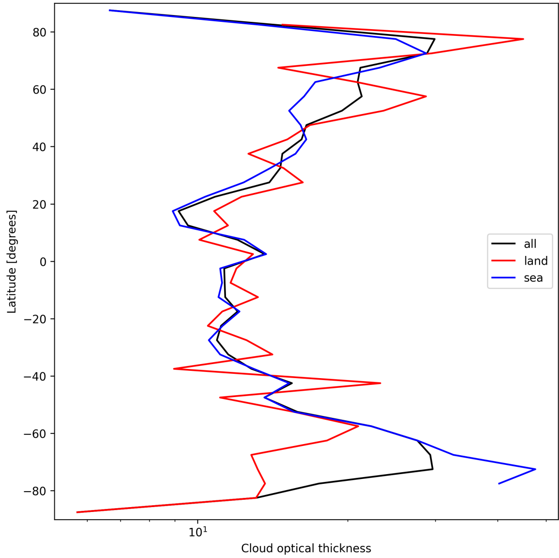
Figure 25: Zonal average of “Cloud optical thickness” for 2025-03-12 to 2025-03-13.
