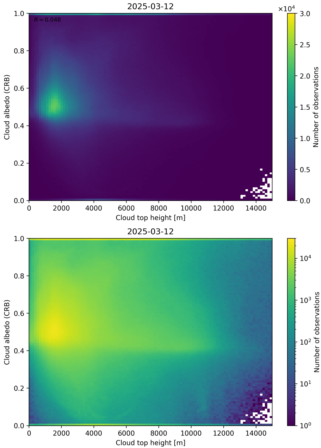
Figure 86: Scatter density plot of “Cloud top height” against “Cloud albedo (CRB)” for 2025-03-12 to 2025-03-13.
