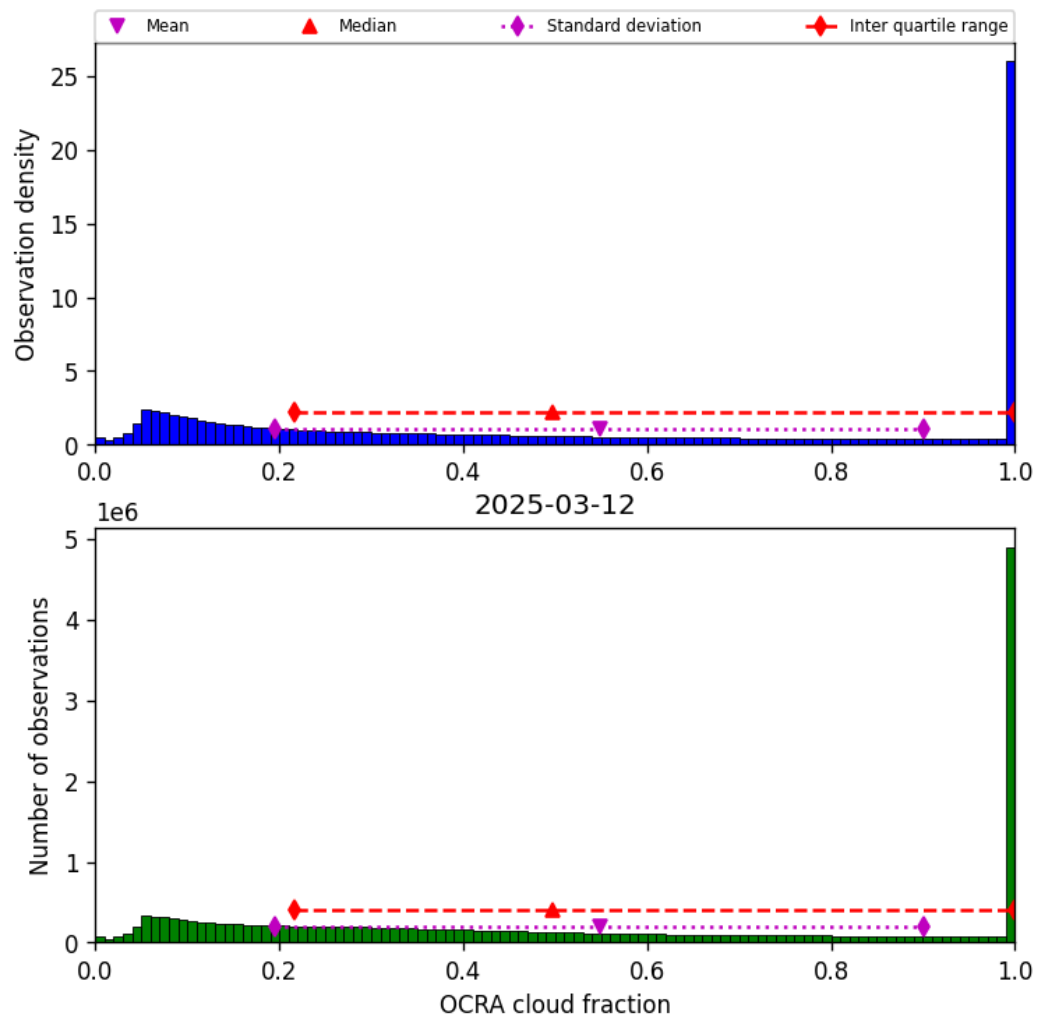
Figure 50: Histogram of “OCRA cloud fraction” for 2025-03-12 to 2025-03-13
