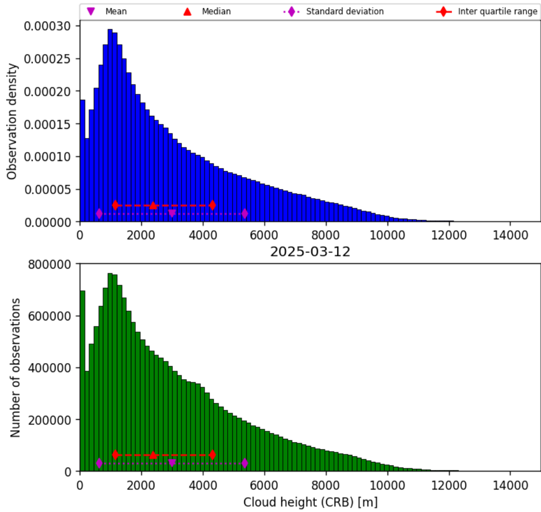
Figure 43: Histogram of “Cloud height (CRB)” for 2025-03-12 to 2025-03-13
