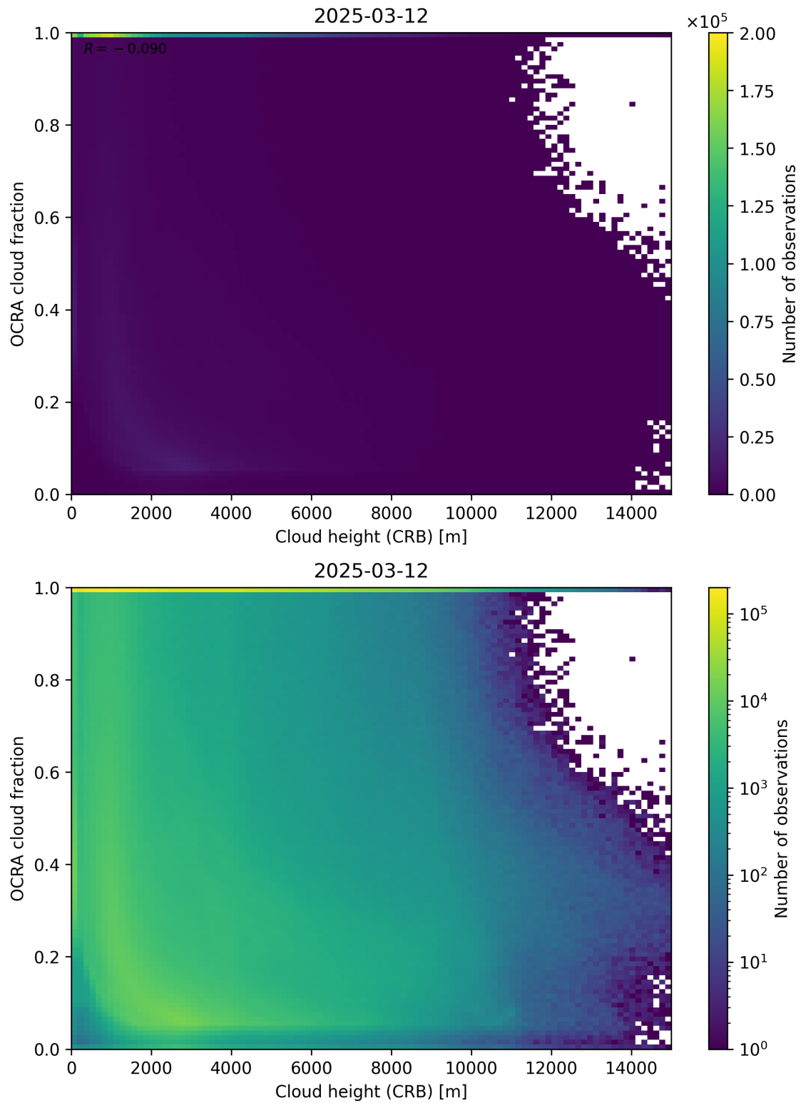
Figure 81: Scatter density plot of “Cloud height (CRB)” against “OCRA cloud fraction” for 2025-03-12 to 2025-03-13.
