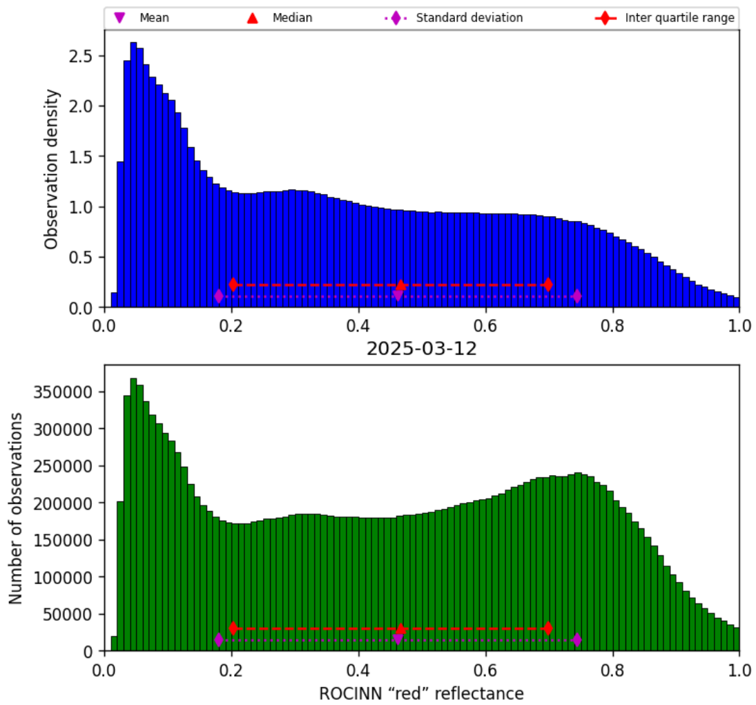
Figure 53: Histogram of “ROCINN “red” reflectance” for 2025-03-12 to 2025-03-13
