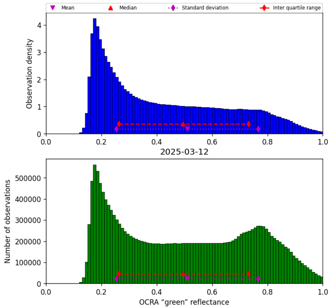
Figure 52: Histogram of “OCRA “green” reflectance” for 2025-03-12 to 2025-03-13
