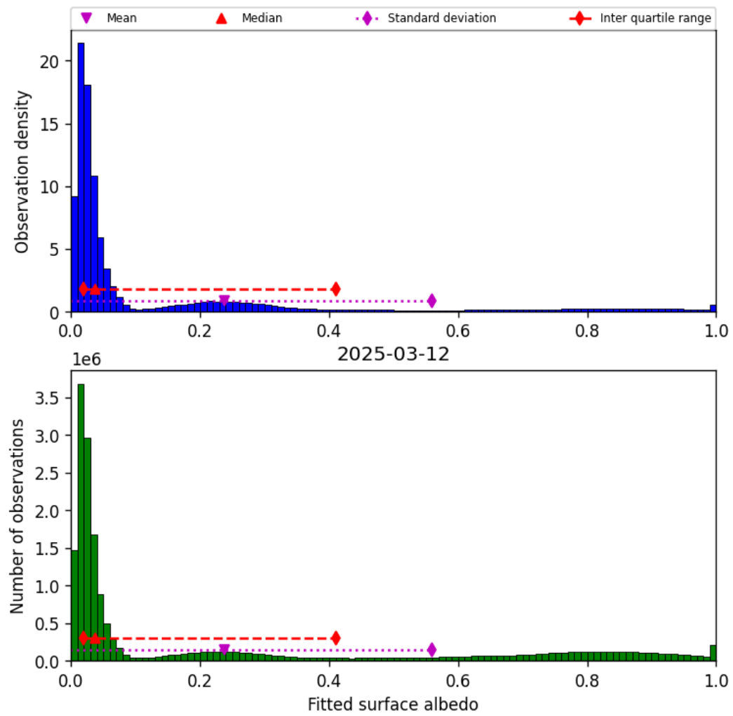
Figure 45: Histogram of “Fitted surface albedo” for 2025-03-12 to 2025-03-13
