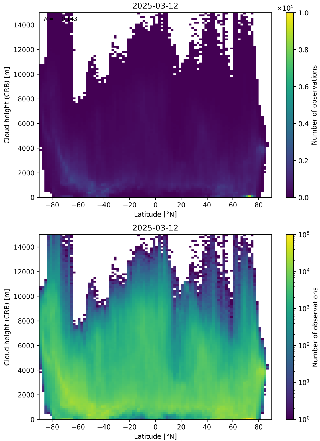
Figure 95: Scatter density plot of “Latitude” against “Cloud height (CRB)” for 2025-03-12 to 2025-03-13.
