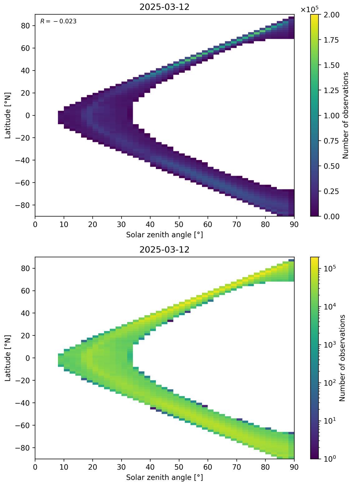
Figure 105: Scatter density plot of “Solar zenith angle” against “Latitude” for 2025-03-12 to 2025-03-13.
