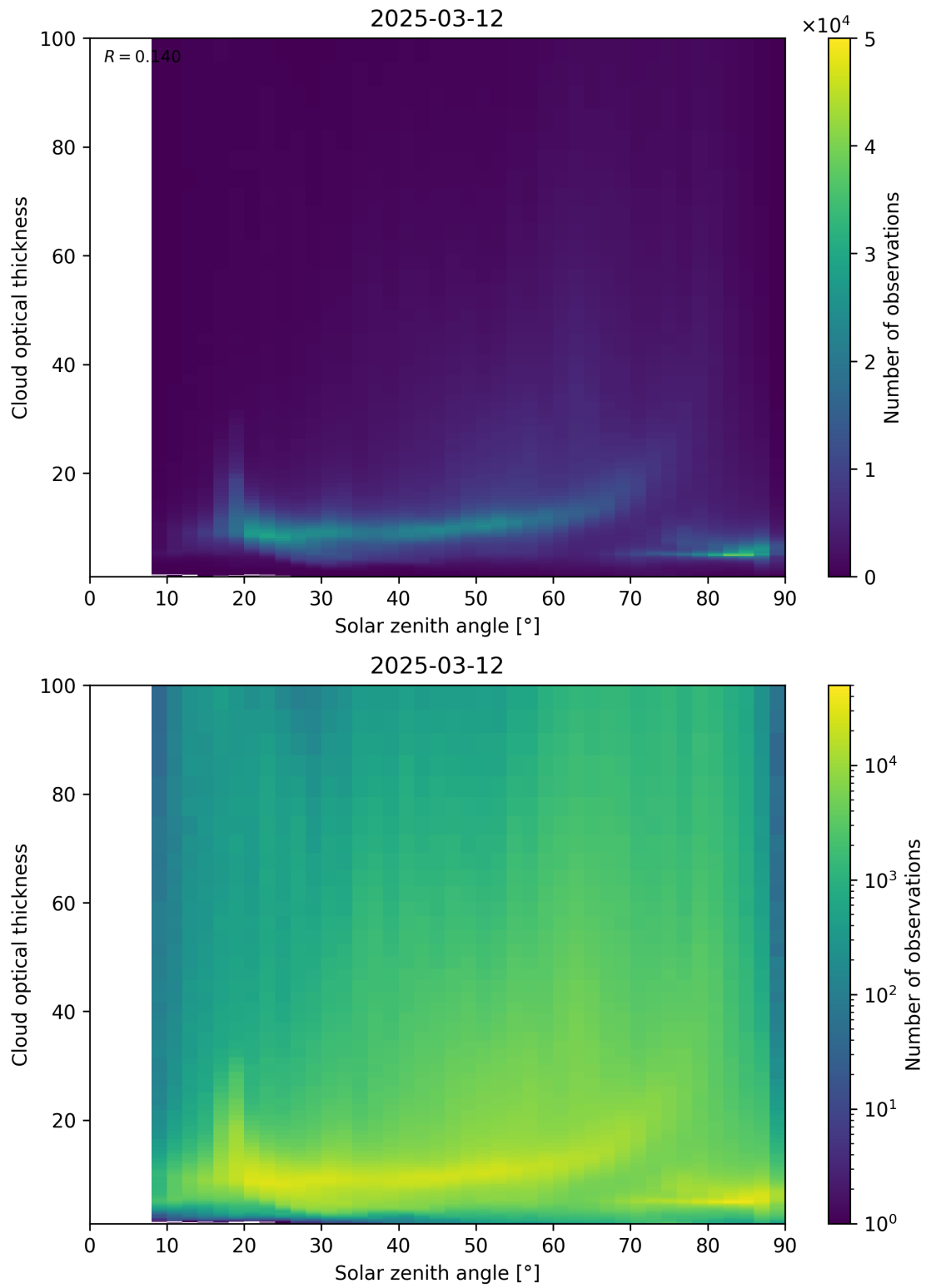
Figure 103: Scatter density plot of “Solar zenith angle” against “Cloud optical thickness” for 2025-03-12 to 2025-03-13.
