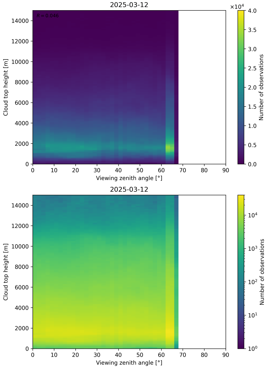
Figure 112: Scatter density plot of “Viewing zenith angle” against “Cloud top height” for 2025-03-12 to 2025-03-13.
