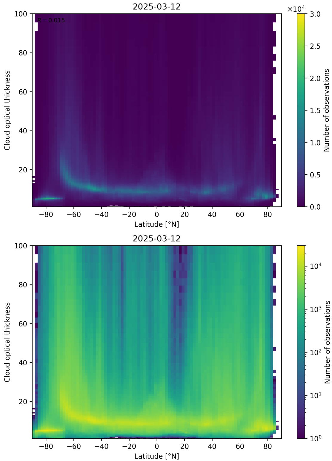
Figure 96: Scatter density plot of “Latitude” against “Cloud optical thickness” for 2025-03-12 to 2025-03-13.
