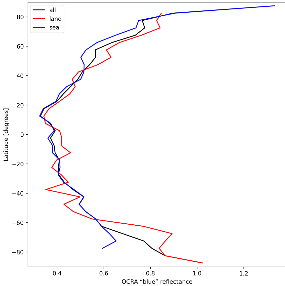
Figure 35: Zonal average of "OCRA "blue" reflectance" for 2025-03-12 to 2025-03-13.
