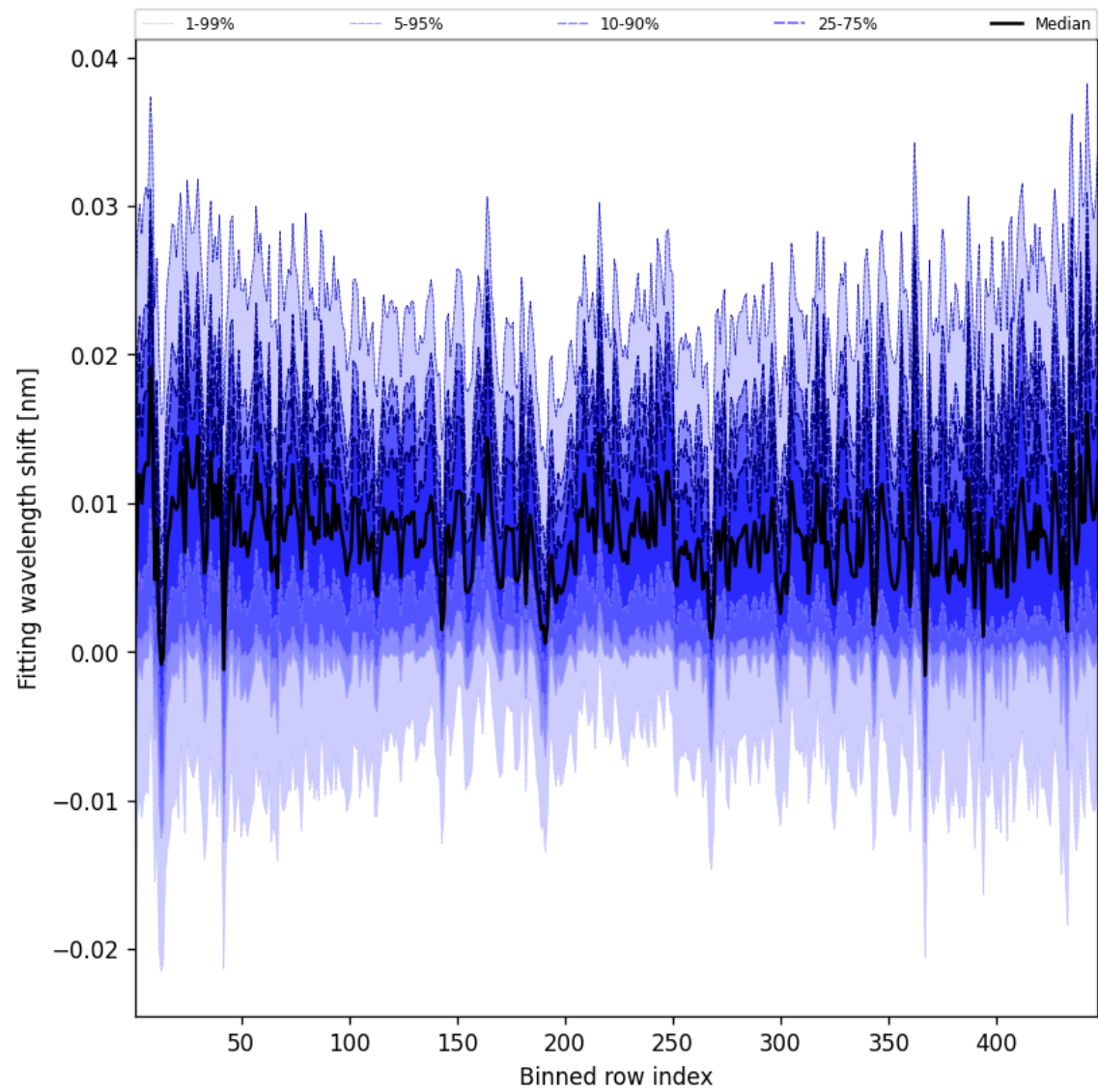
Figure 65: Along track statistics of “Fitting wavelength shift” for 2025-03-12 to 2025-03-13
