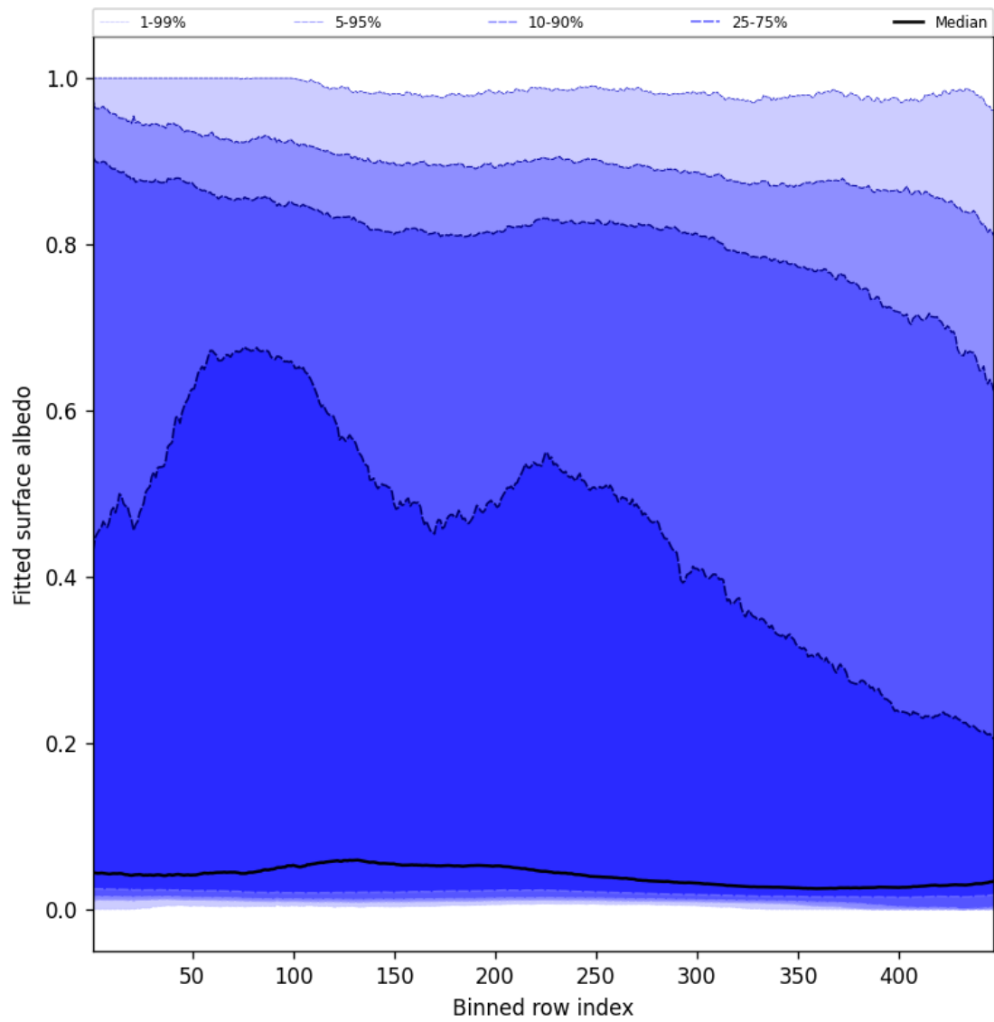
Figure 61: Along track statistics of “Fitted surface albedo” for 2025-03-12 to 2025-03-13
