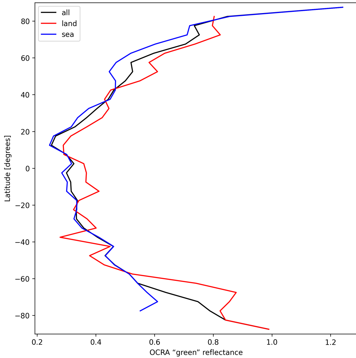
Figure 36: Zonal average of “OCRA “green” reflectance” for 2025-03-12 to 2025-03-13.
