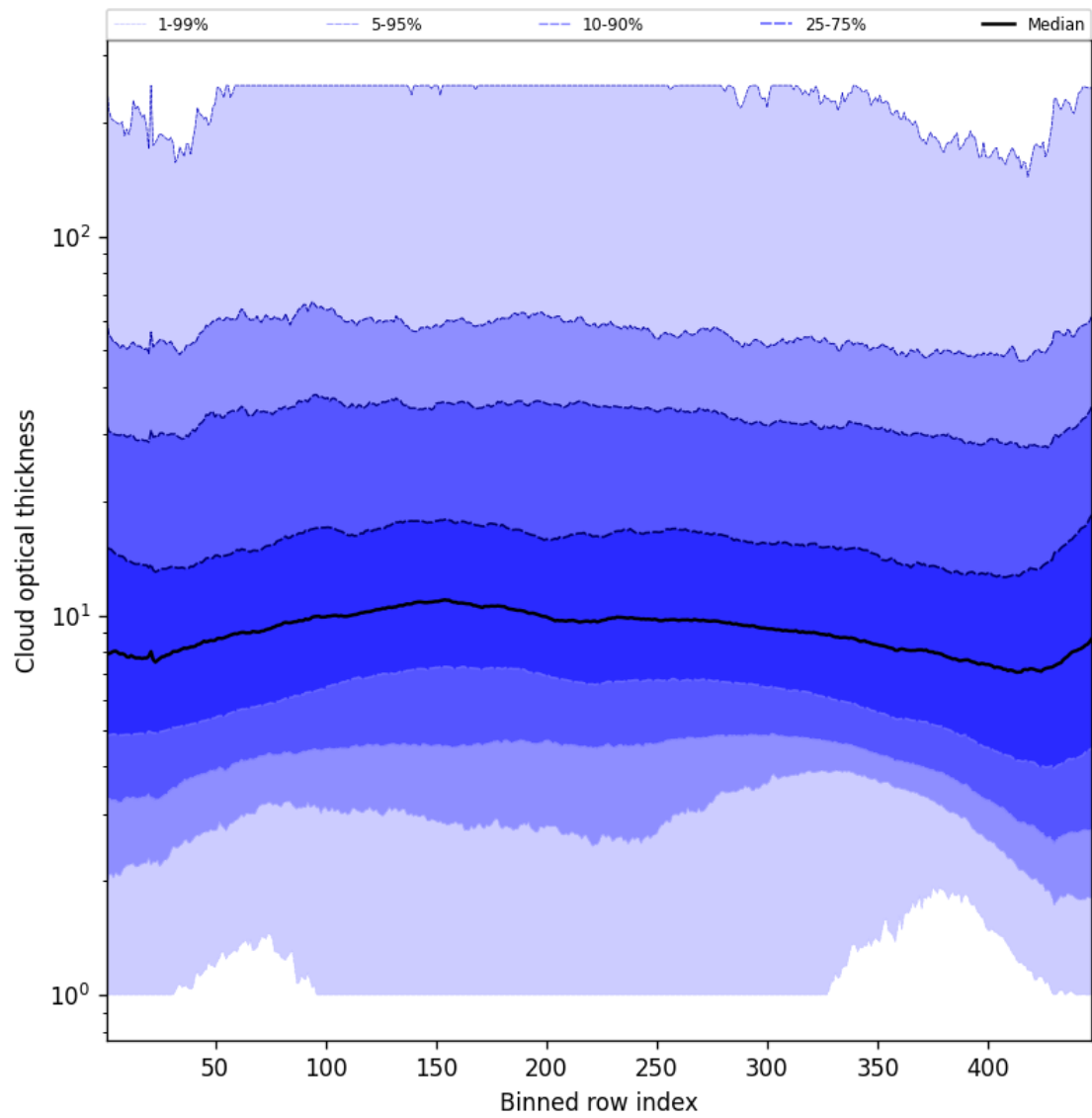
Figure 57: Along track statistics of “Cloud optical thickness” for 2025-03-12 to 2025-03-13
