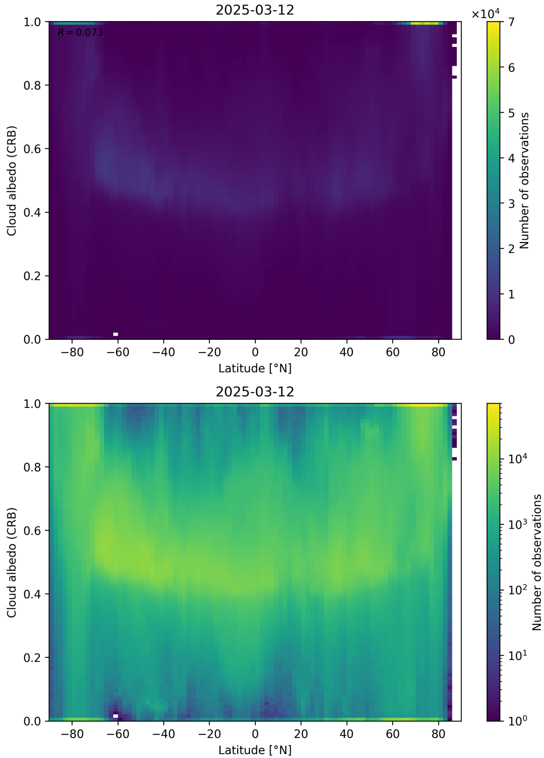
Figure 91: Scatter density plot of “Latitude” against “Cloud albedo (CRB)” for 2025-03-12 to 2025-03-13.
