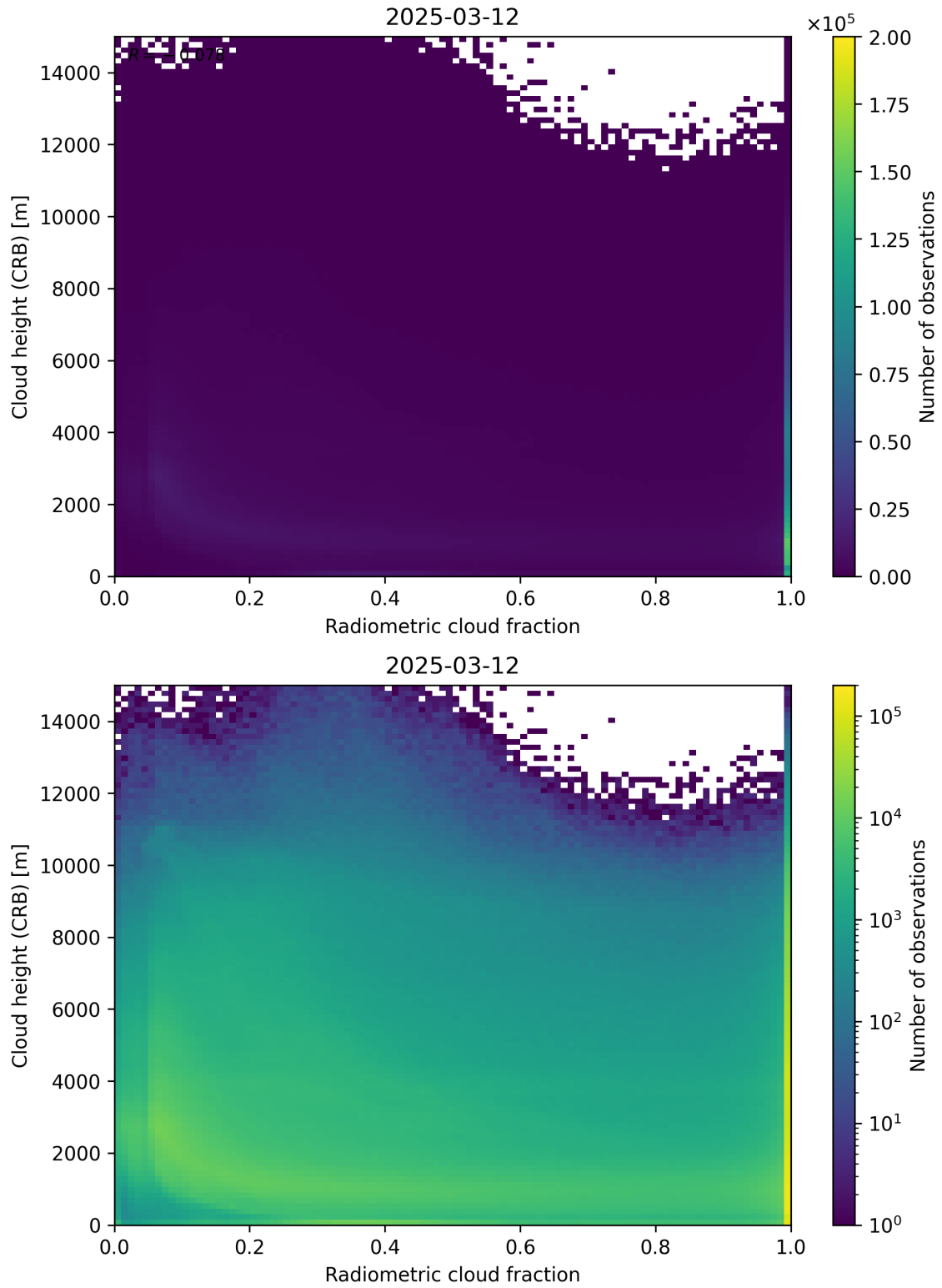
Figure 74: Scatter density plot of “Radiometric cloud fraction” against “Cloud height (CRB)” for 2025-03-12 to 2025-03-13.
