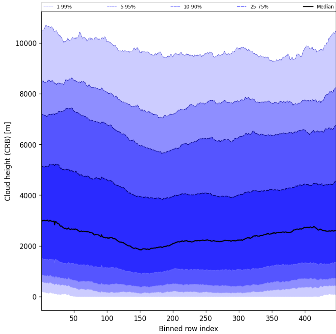
Figure 59: Along track statistics of “Cloud height (CRB)” for 2025-03-12 to 2025-03-13
