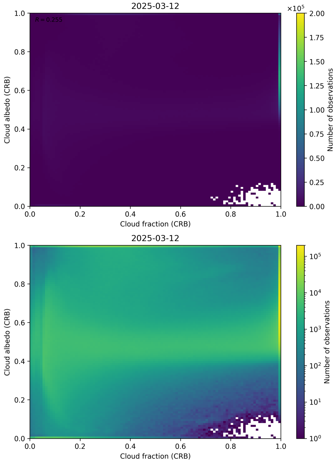
Figure 77: Scatter density plot of “Cloud fraction (CRB)” against “Cloud albedo (CRB)” for 2025-03-12 to 2025-03-13.
