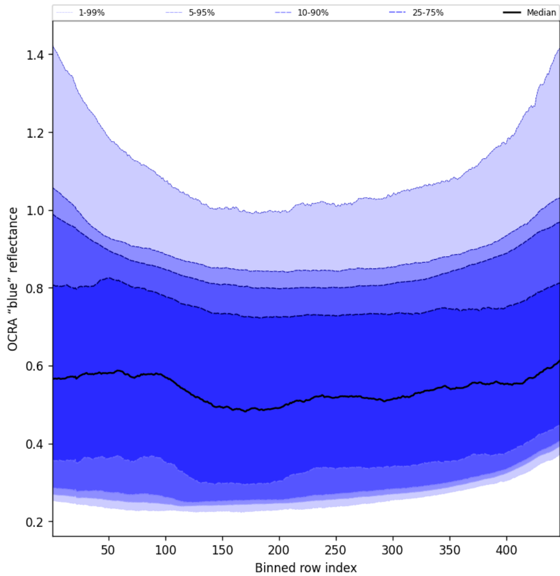
Figure 67: Along track statistics of “OCRA “blue” reflectance” for 2025-03-12 to 2025-03-13
