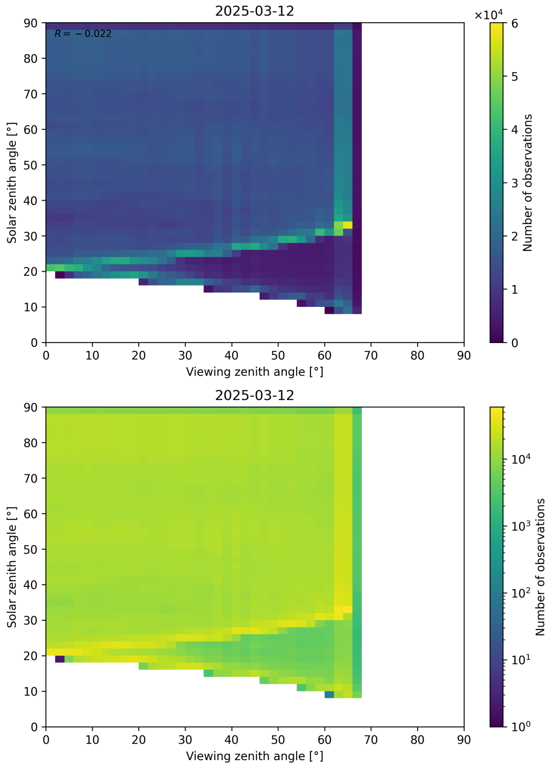
Figure 114: Scatter density plot of “Viewing zenith angle” against “Solar zenith angle” for 2025-03-12 to 2025-03-13.
