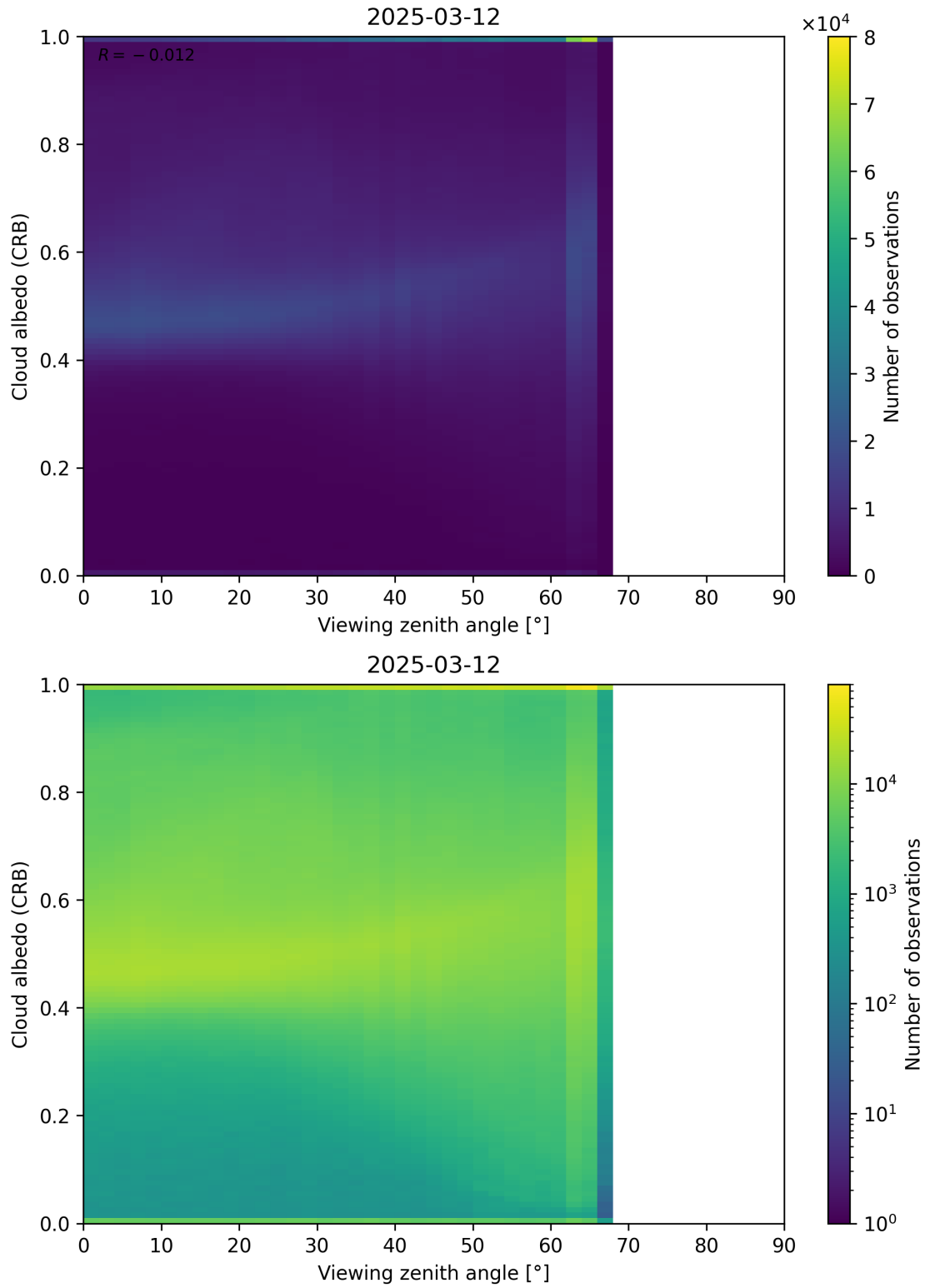
Figure 106: Scatter density plot of “Viewing zenith angle” against “Cloud albedo (CRB)” for 2025-03-12 to 2025-03-13.
