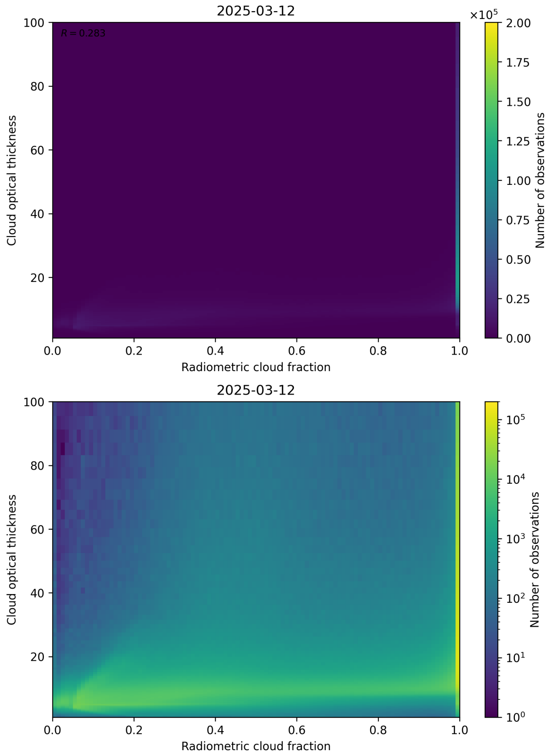
Figure 75: Scatter density plot of “Radiometric cloud fraction” against “Cloud optical thickness” for 2025-03-12 to 2025-03-13.
