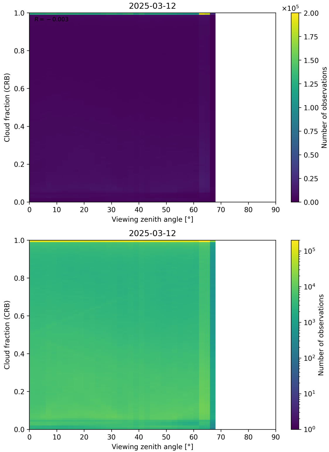
Figure 109: Scatter density plot of “Viewing zenith angle” against “Cloud fraction (CRB)” for 2025-03-12 to 2025-03-13.
