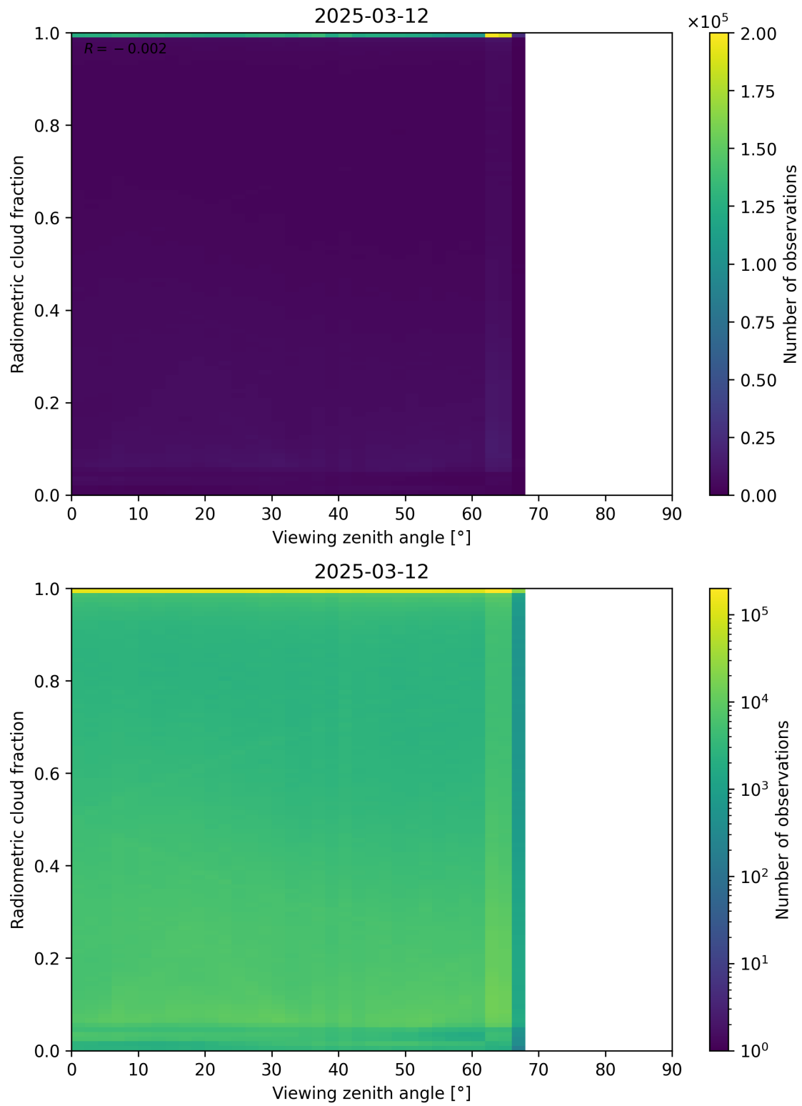
Figure 107: Scatter density plot of “Viewing zenith angle” against “Radiometric cloud fraction” for 2025-03-12 to 2025-03-13.
