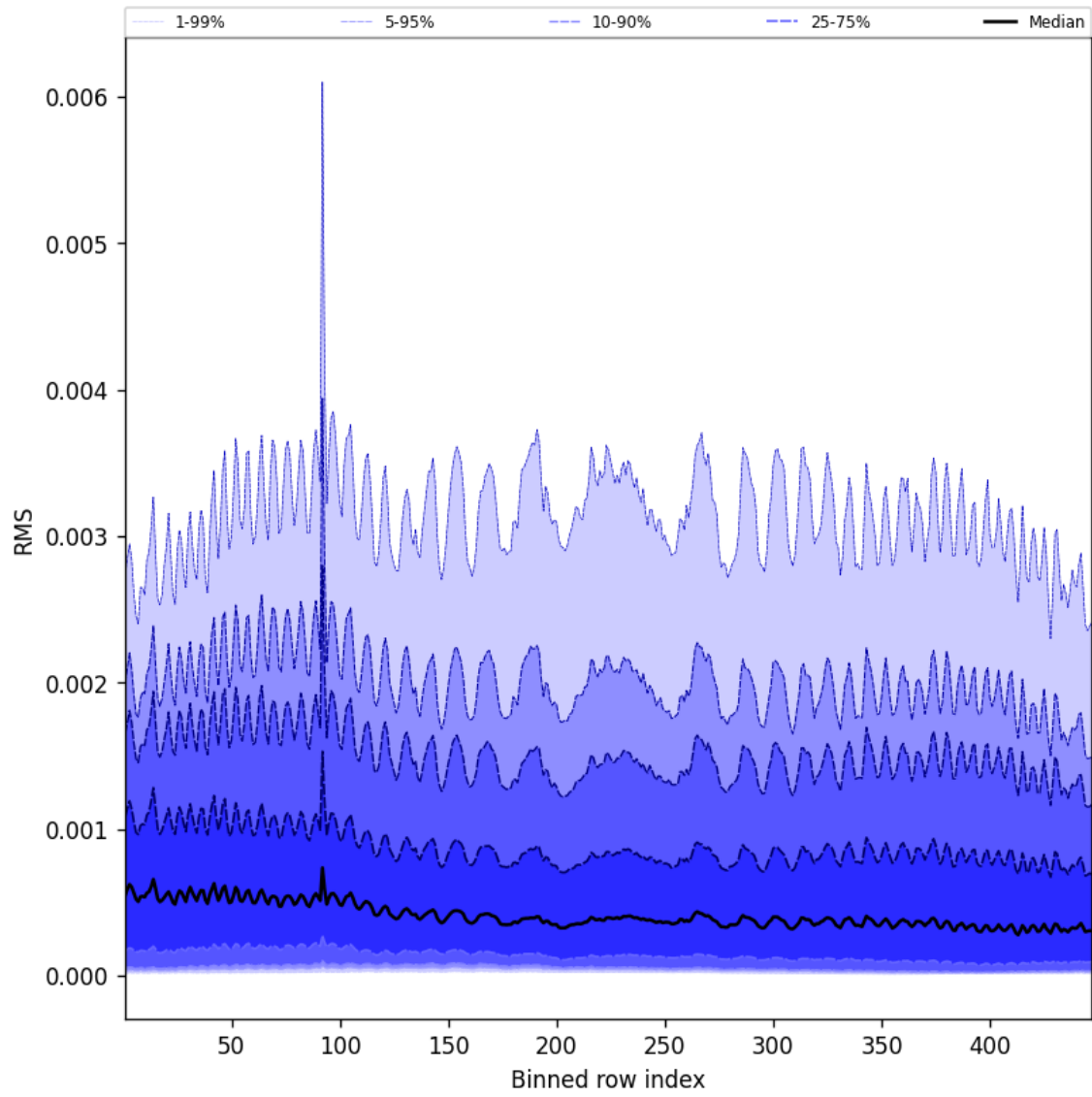
Figure 63: Along track statistics of “RMS” for 2025-03-12 to 2025-03-13
