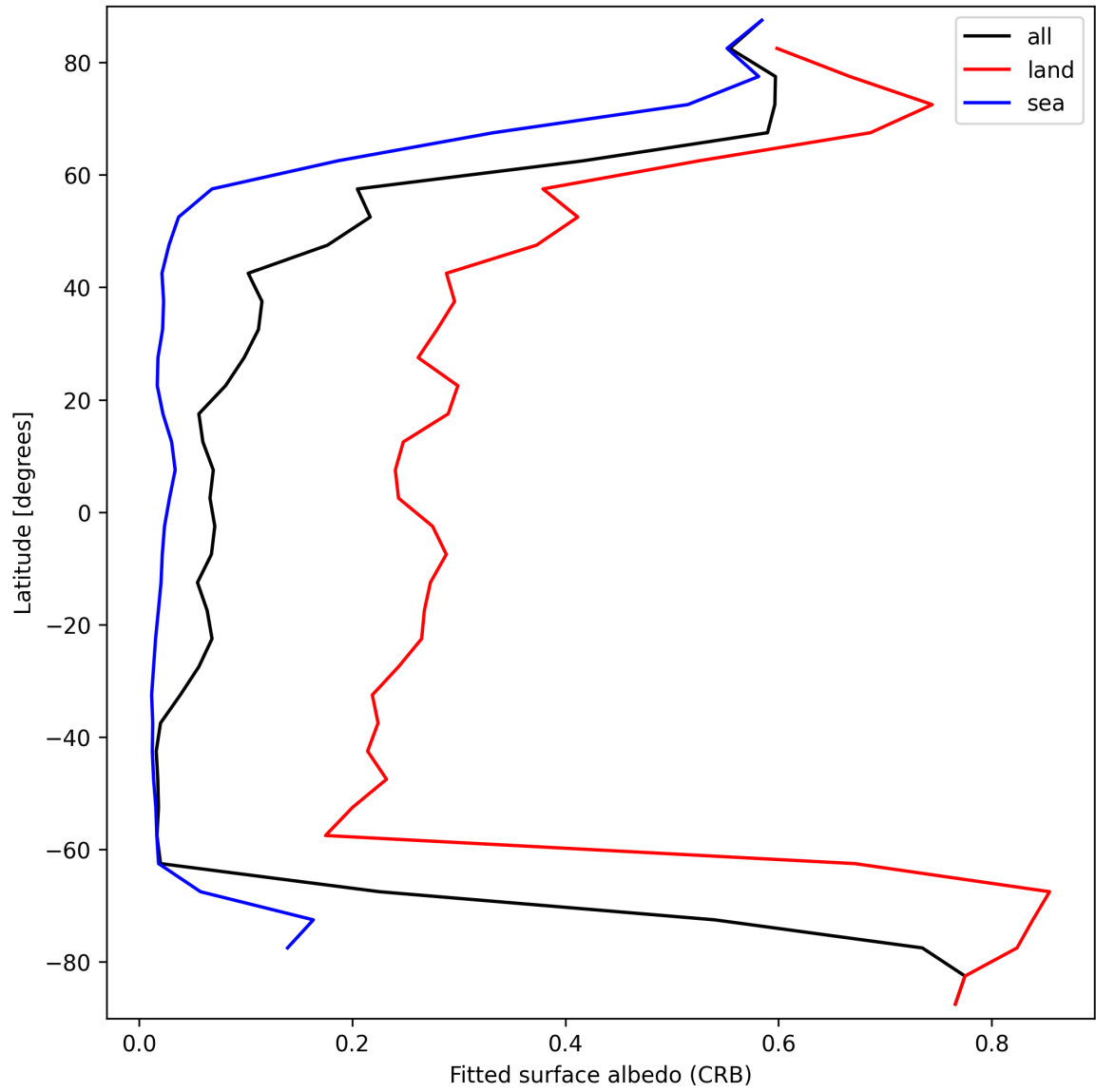
Figure 30: Zonal average of “Fitted surface albedo (CRB)” for 2025-03-12 to 2025-03-13.
