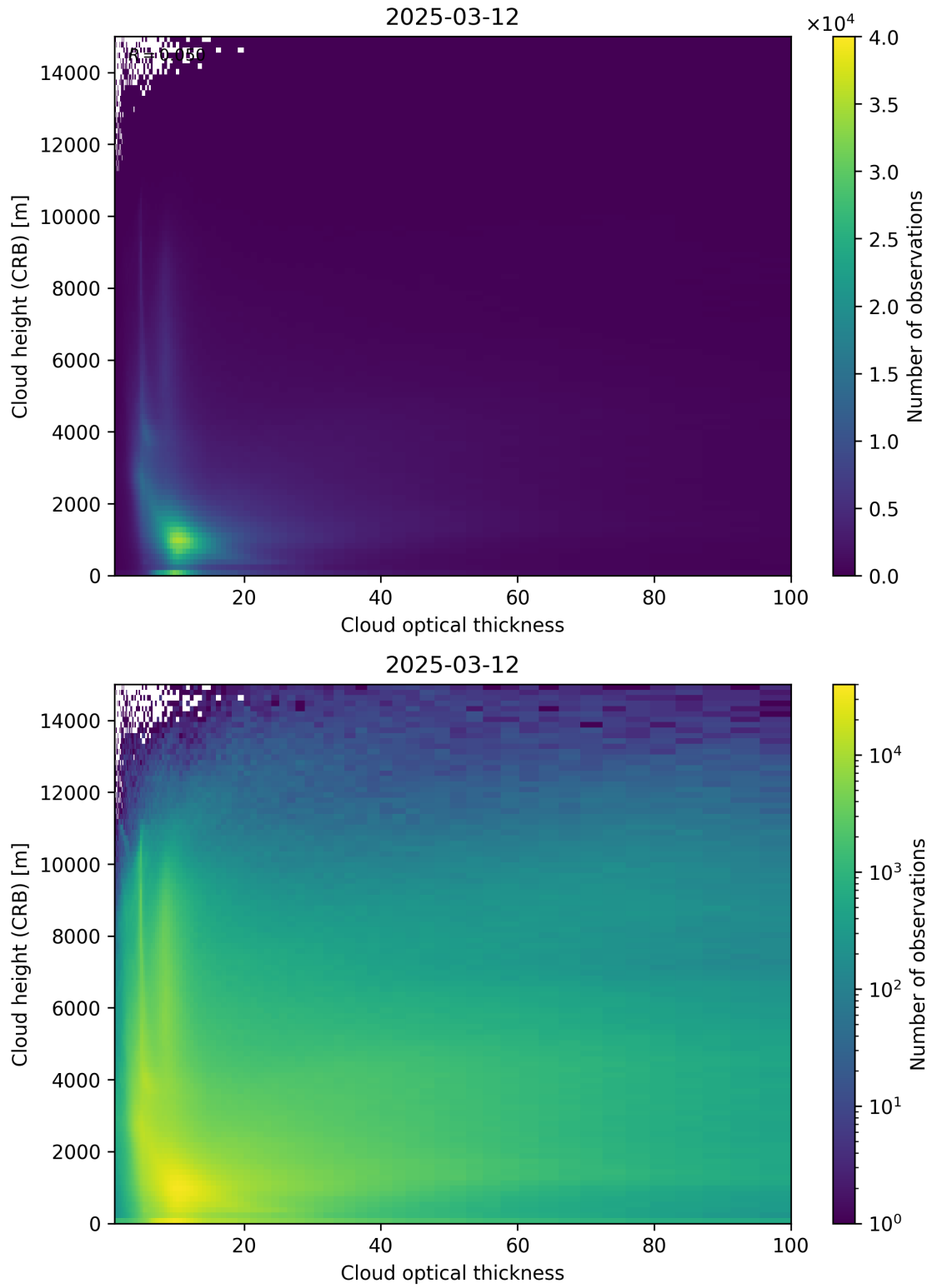
Figure 85: Scatter density plot of “Cloud optical thickness” against “Cloud height (CRB)” for 2025-03-12 to 2025-03-13.
