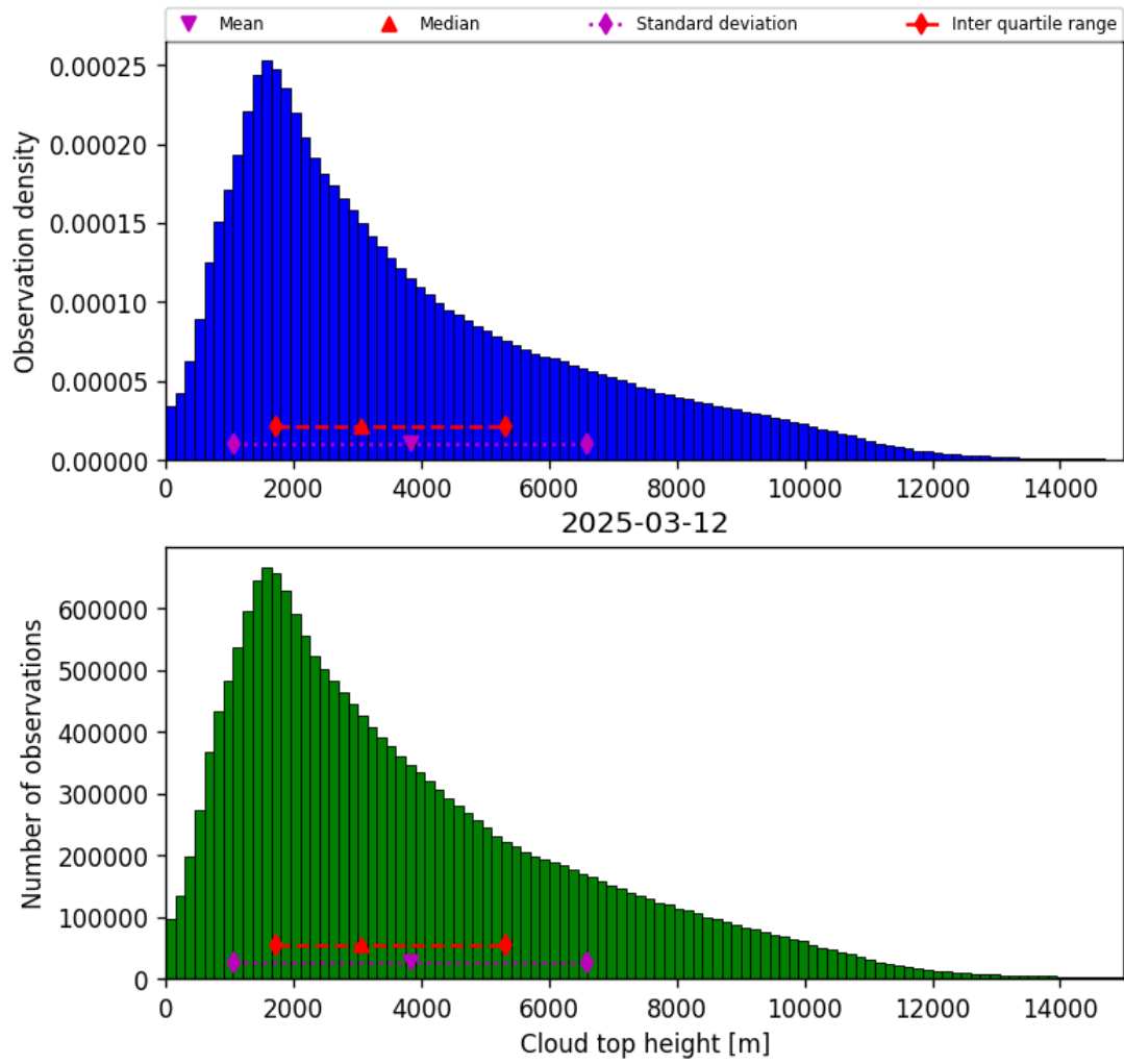
Figure 40: Histogram of “Cloud top height” for 2025-03-12 to 2025-03-13
