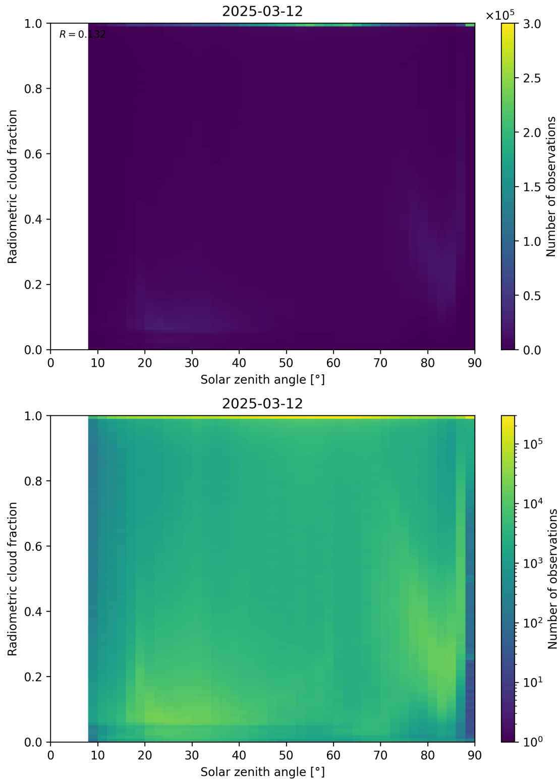
Figure 99: Scatter density plot of “Solar zenith angle” against “Radiometric cloud fraction” for 2025-03-12 to 2025-03-13.
