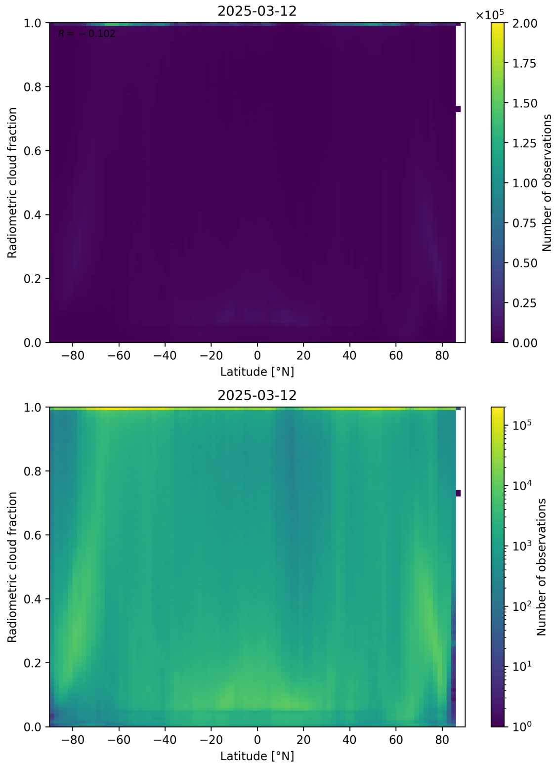
Figure 92: Scatter density plot of “Latitude” against “Radiometric cloud fraction” for 2025-03-12 to 2025-03-13.
