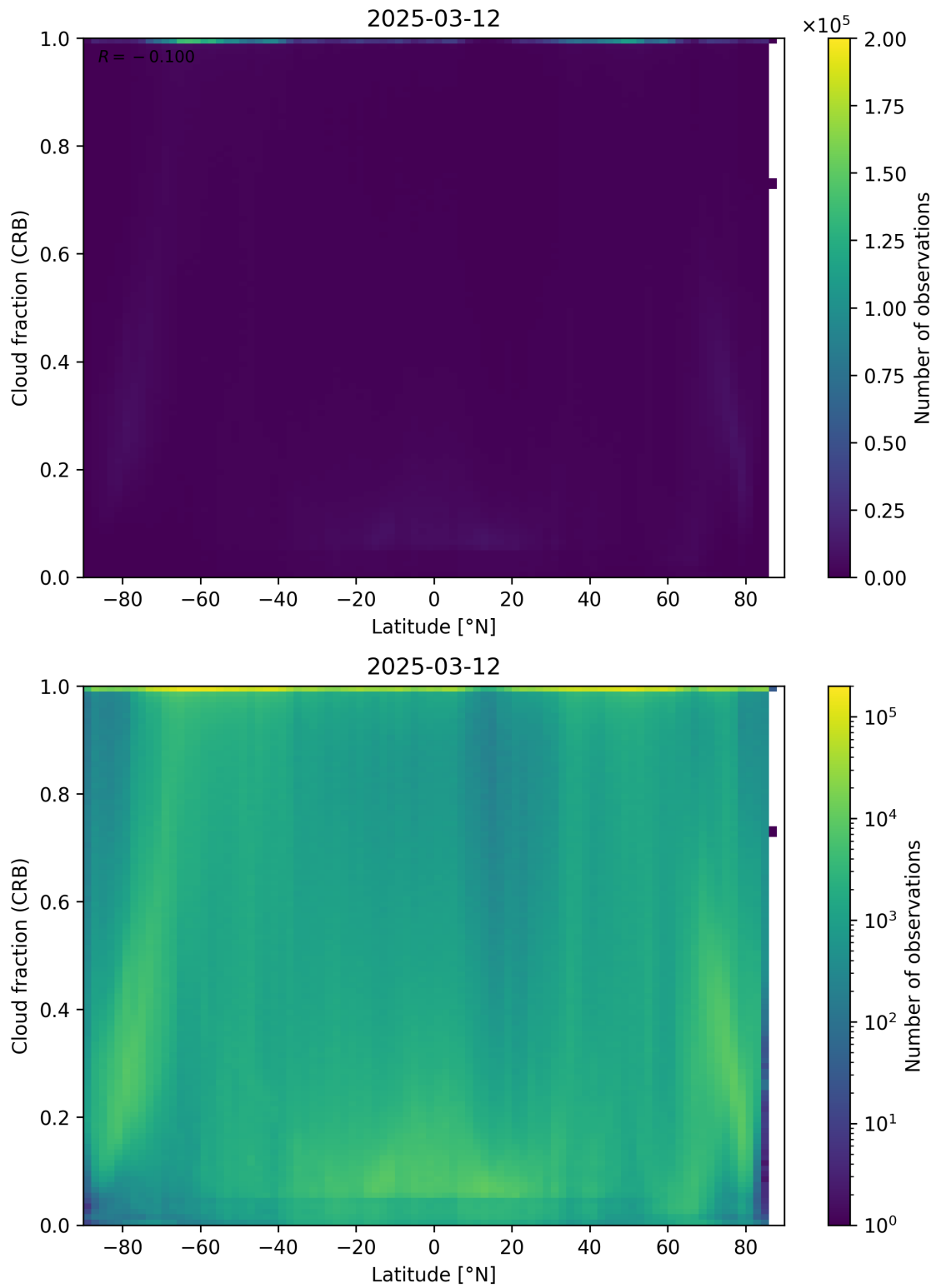
Figure 94: Scatter density plot of “Latitude” against “Cloud fraction (CRB)” for 2025-03-12 to 2025-03-13.
