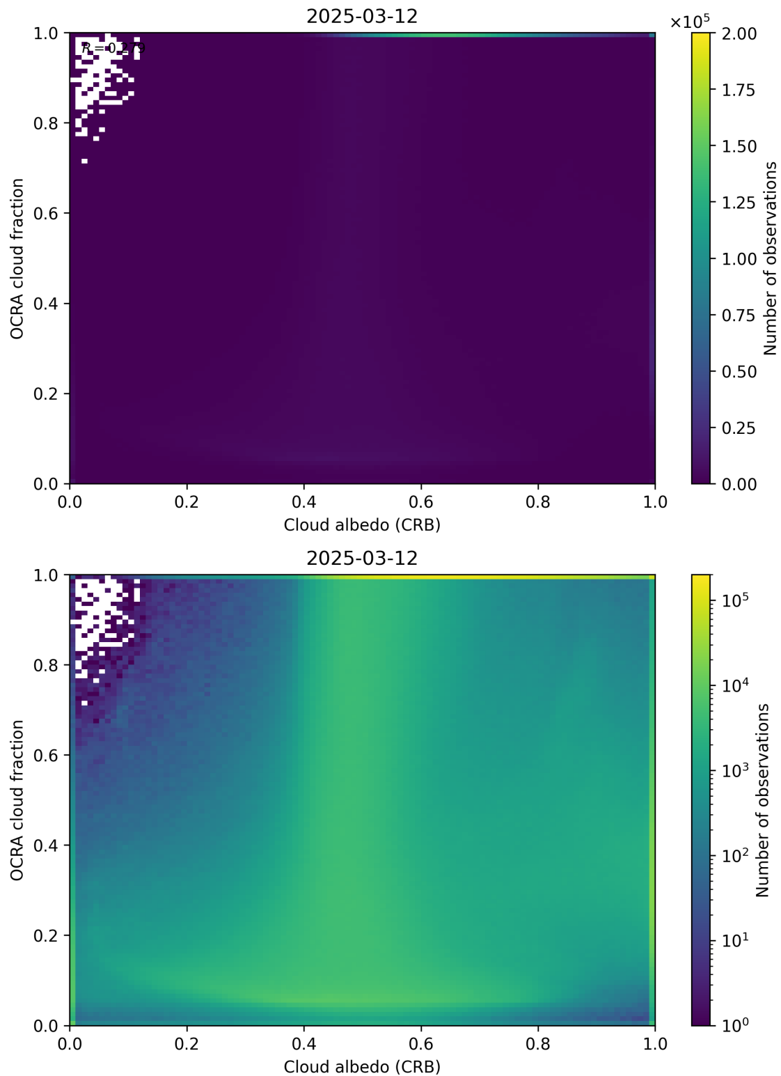
Figure 70: Scatter density plot of “Cloud albedo (CRB)” against “OCRA cloud fraction” for 2025-03-12 to 2025-03-13.
