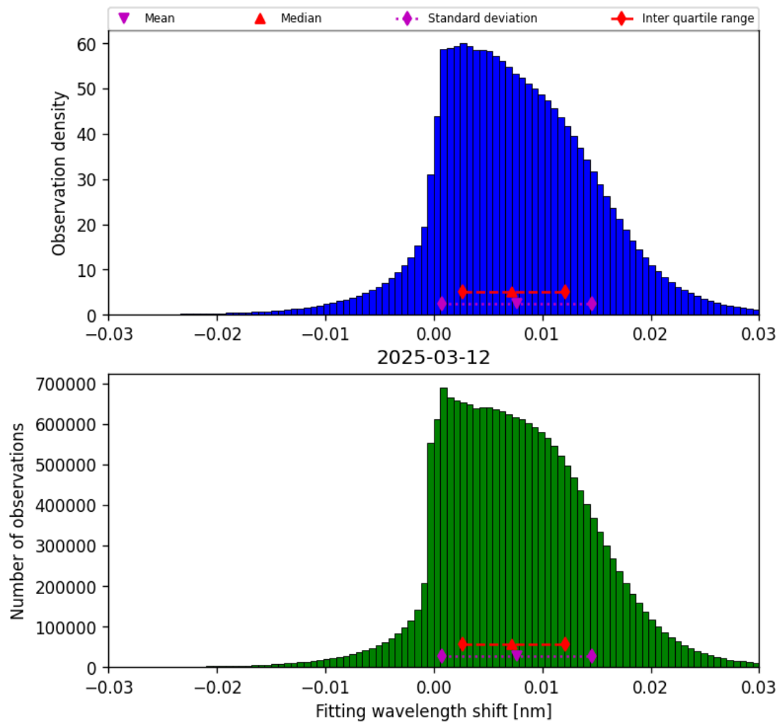
Figure 49: Histogram of “Fitting wavelength shift” for 2025-03-12 to 2025-03-13
