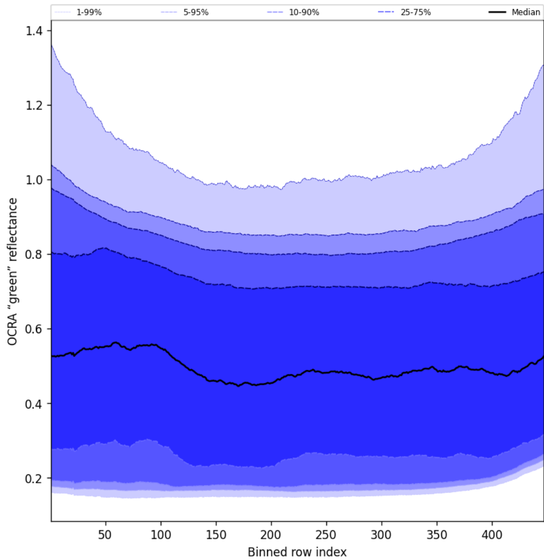
Figure 68: Along track statistics of "OCRA "green" reflectance" for 2025-03-12 to 2025-03-13
