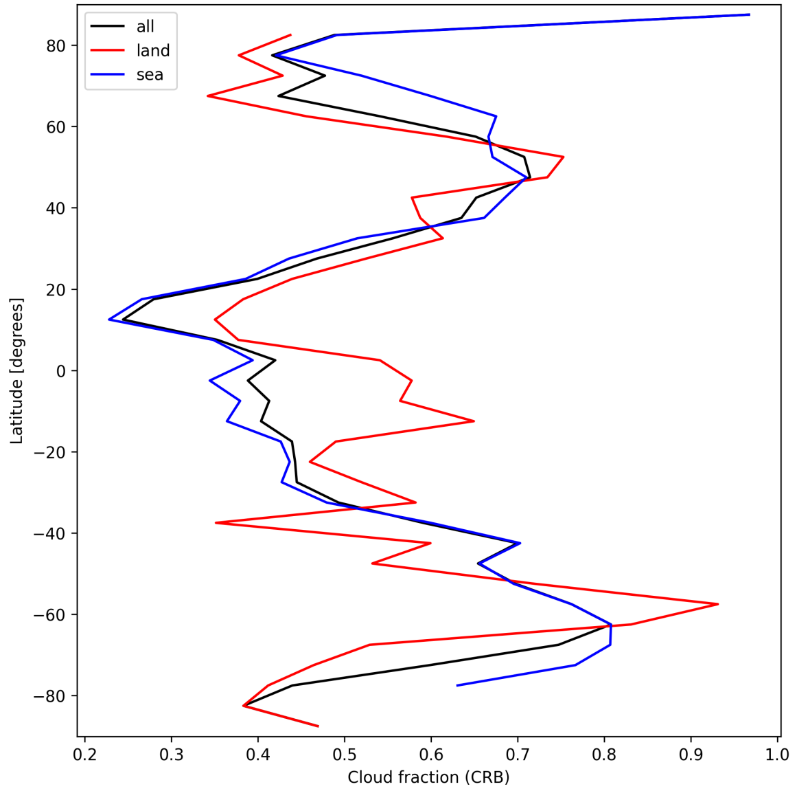
Figure 26: Zonal average of “Cloud fraction (CRB)” for 2025-03-12 to 2025-03-13.
