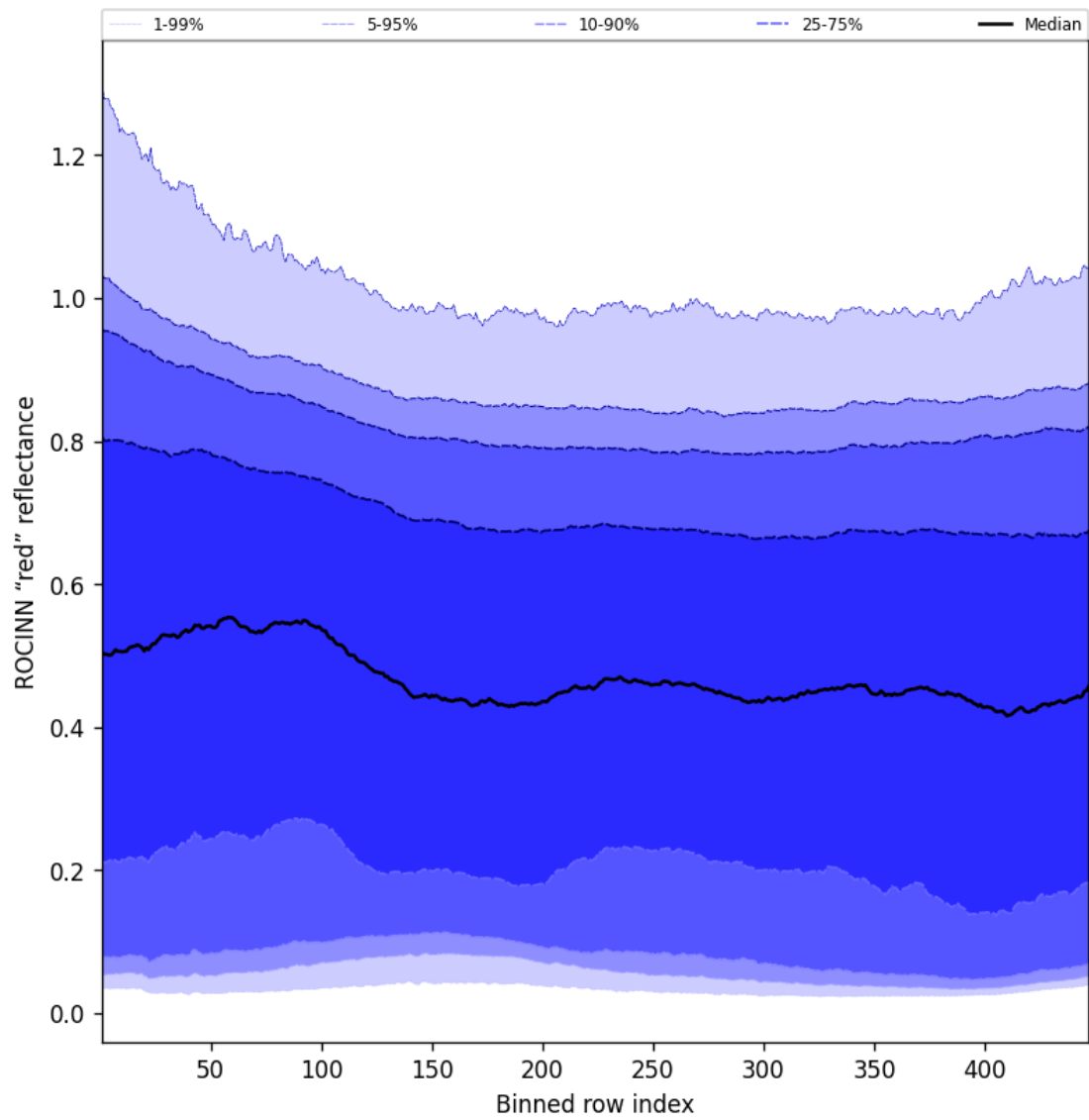
Figure 69: Along track statistics of “ROCINN “red” reflectance” for 2025-03-12 to 2025-03-13
