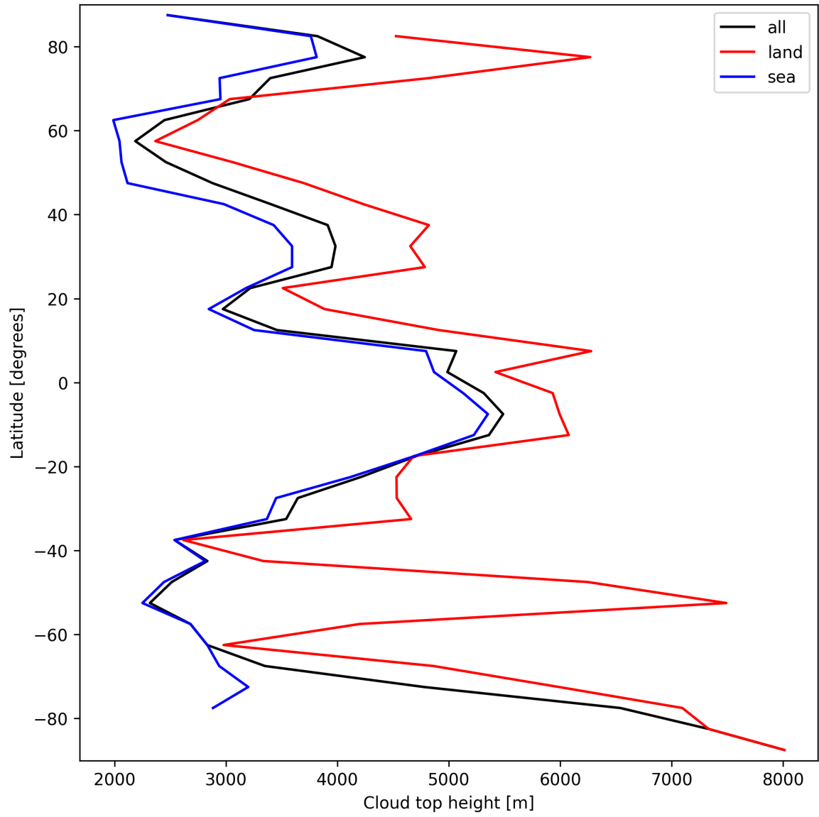
Figure 24: Zonal average of “Cloud top height” for 2025-03-12 to 2025-03-13.
