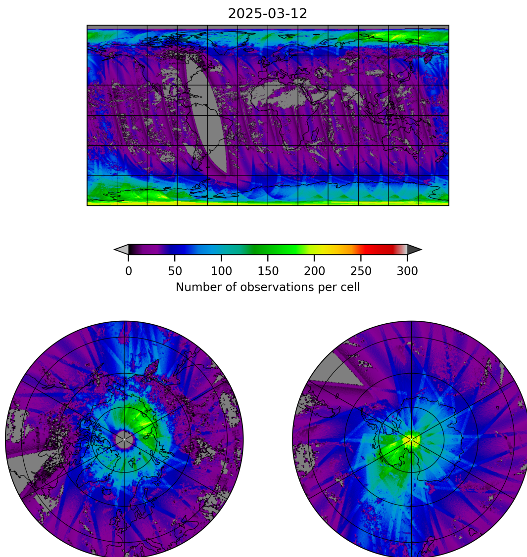
Figure 21: Map of the number of observations for 2025-03-12 to 2025-03-13
