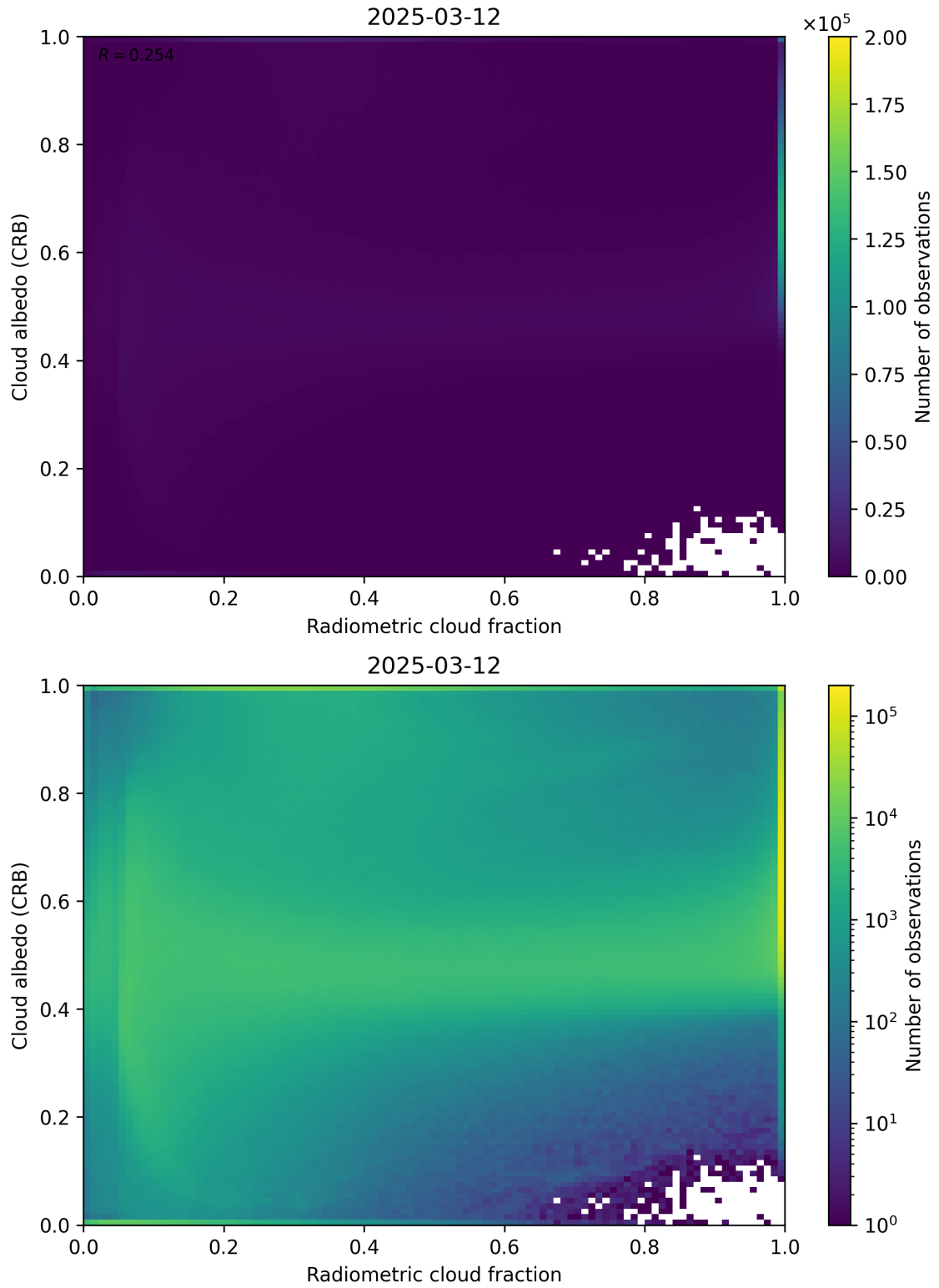
Figure 71: Scatter density plot of “Radiometric cloud fraction” against “Cloud albedo (CRB)” for 2025-03-12 to 2025-03-13.
