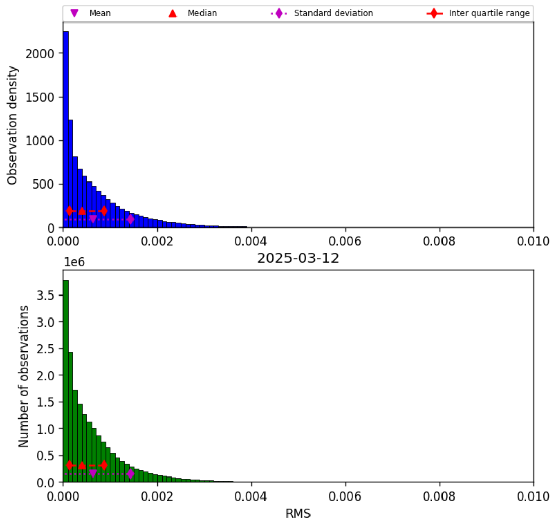
Figure 47: Histogram of “RMS” for 2025-03-12 to 2025-03-13
