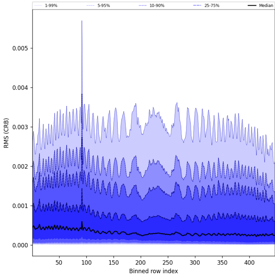
Figure 64: Along track statistics of “RMS (CRB)” for 2025-03-12 to 2025-03-13
