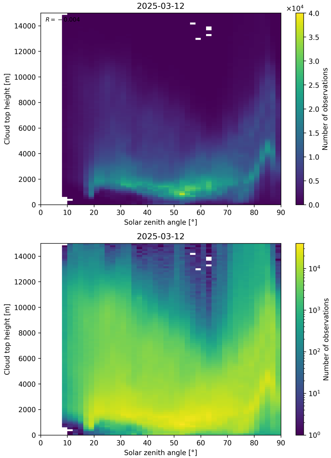
Figure 104: Scatter density plot of “Solar zenith angle” against “Cloud top height” for 2025-03-12 to 2025-03-13.
