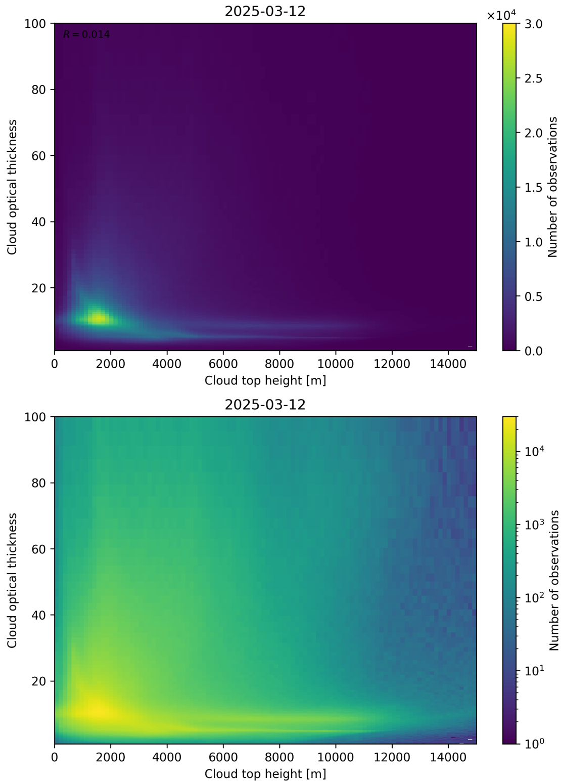
Figure 90: Scatter density plot of “Cloud top height” against “Cloud optical thickness” for 2025-03-12 to 2025-03-13.
