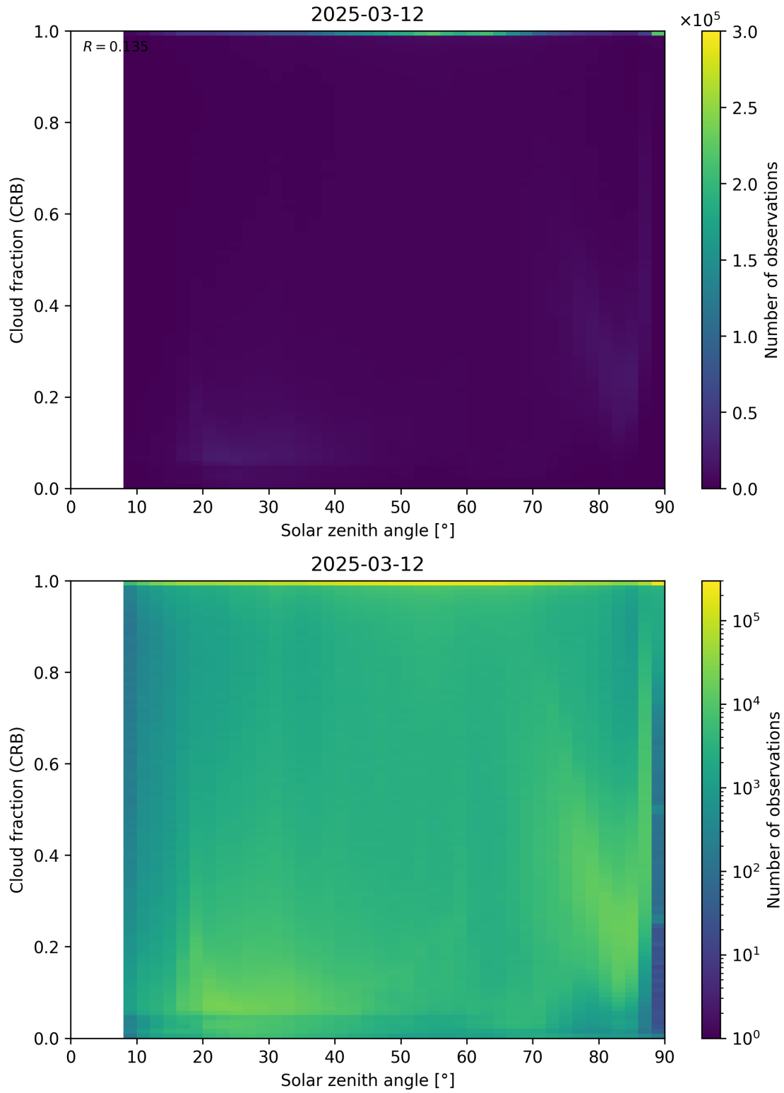
Figure 101: Scatter density plot of “Solar zenith angle” against “Cloud fraction (CRB)” for 2025-03-12 to 2025-03-13.
