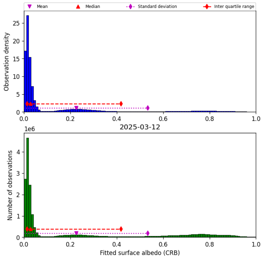
Figure 46: Histogram of “Fitted surface albedo (CRB)” for 2025-03-12 to 2025-03-13
