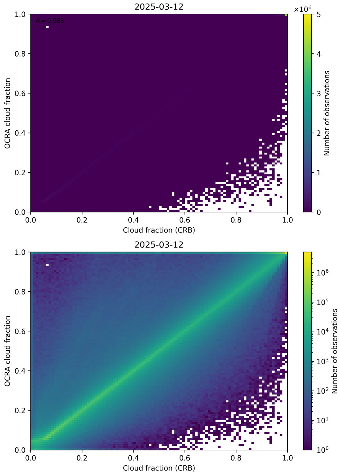
Figure 78: Scatter density plot of “Cloud fraction (CRB)” against “OCRA cloud fraction” for 2025-03-12 to 2025-03-13.
