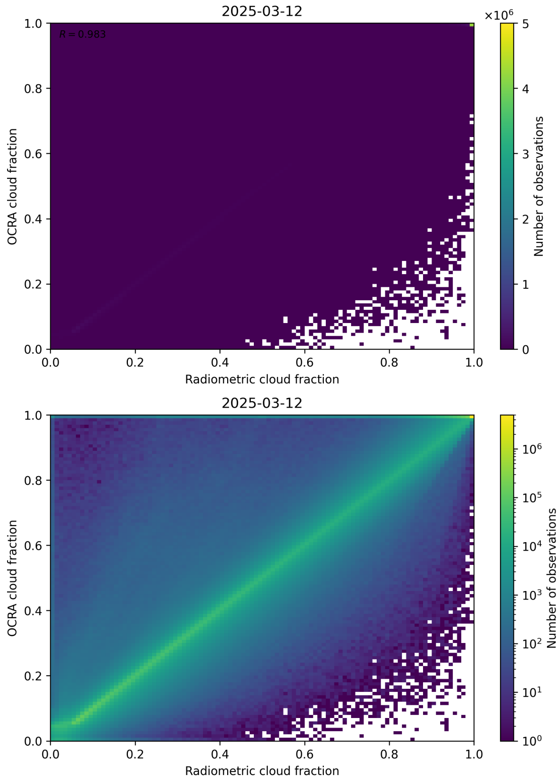
Figure 72: Scatter density plot of “Radiometric cloud fraction” against “OCRA cloud fraction” for 2025-03-12 to 2025-03-13.
