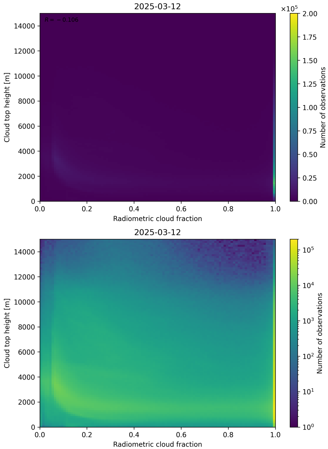
Figure 76: Scatter density plot of “Radiometric cloud fraction” against “Cloud top height” for 2025-03-12 to 2025-03-13.
