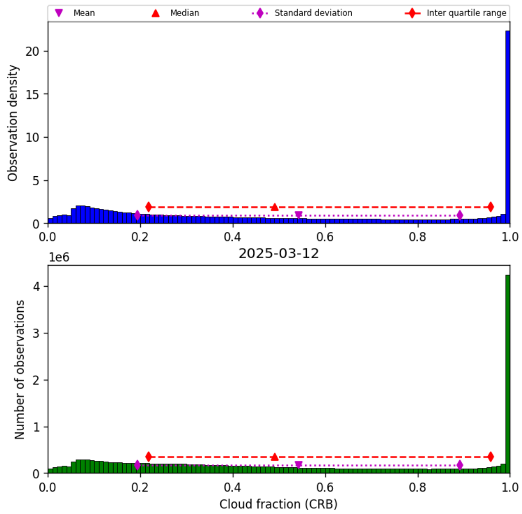
Figure 42: Histogram of “Cloud fraction (CRB)” for 2025-03-12 to 2025-03-13
