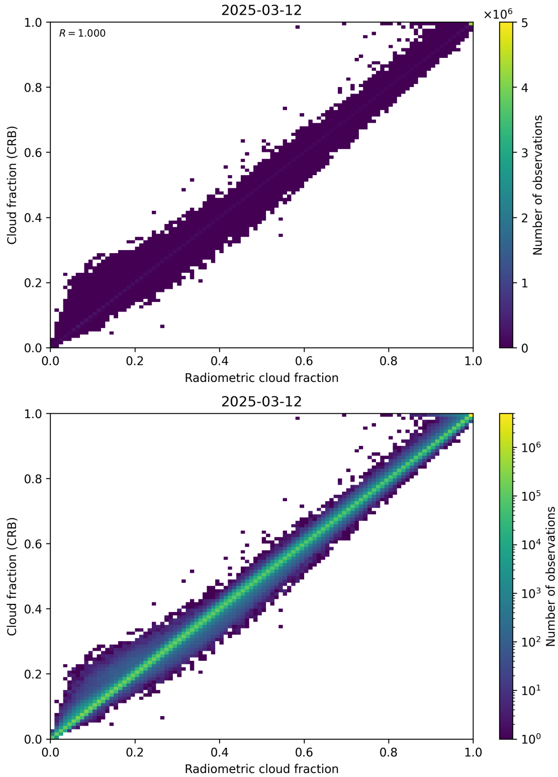
Figure 73: Scatter density plot of “Radiometric cloud fraction” against “Cloud fraction (CRB)” for 2025-03-12 to 2025-03-13.
