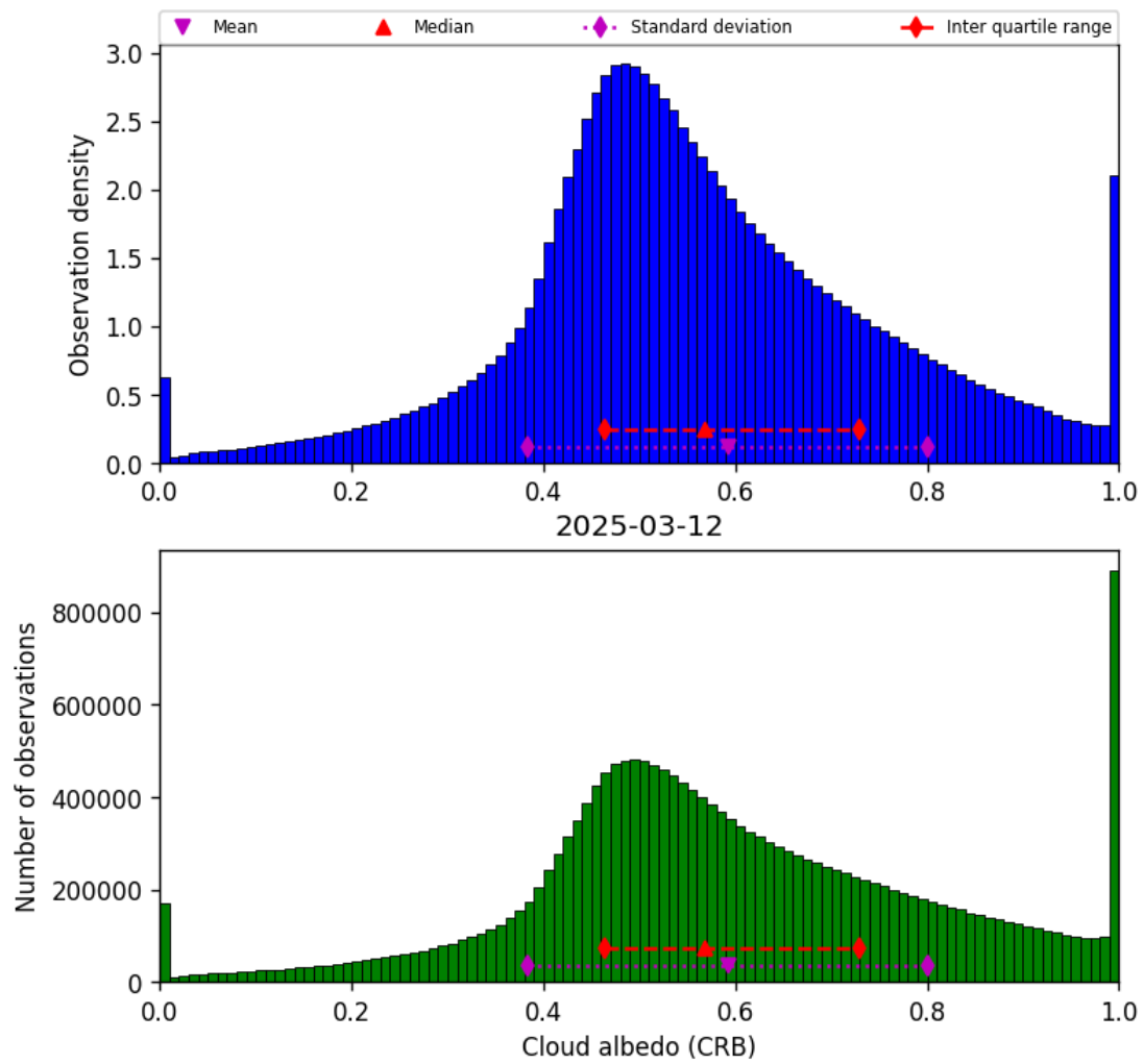
Figure 44: Histogram of “Cloud albedo (CRB)” for 2025-03-12 to 2025-03-13
