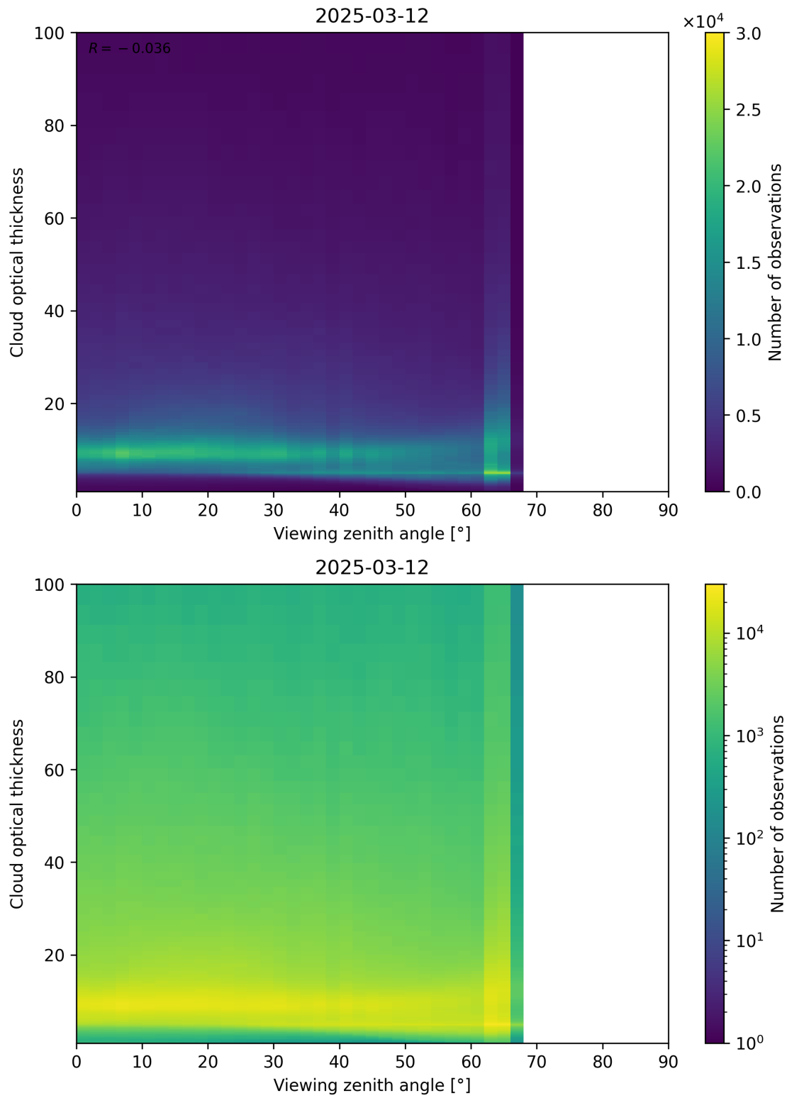
Figure 111: Scatter density plot of “Viewing zenith angle” against “Cloud optical thickness” for 2025-03-12 to 2025-03-13.
