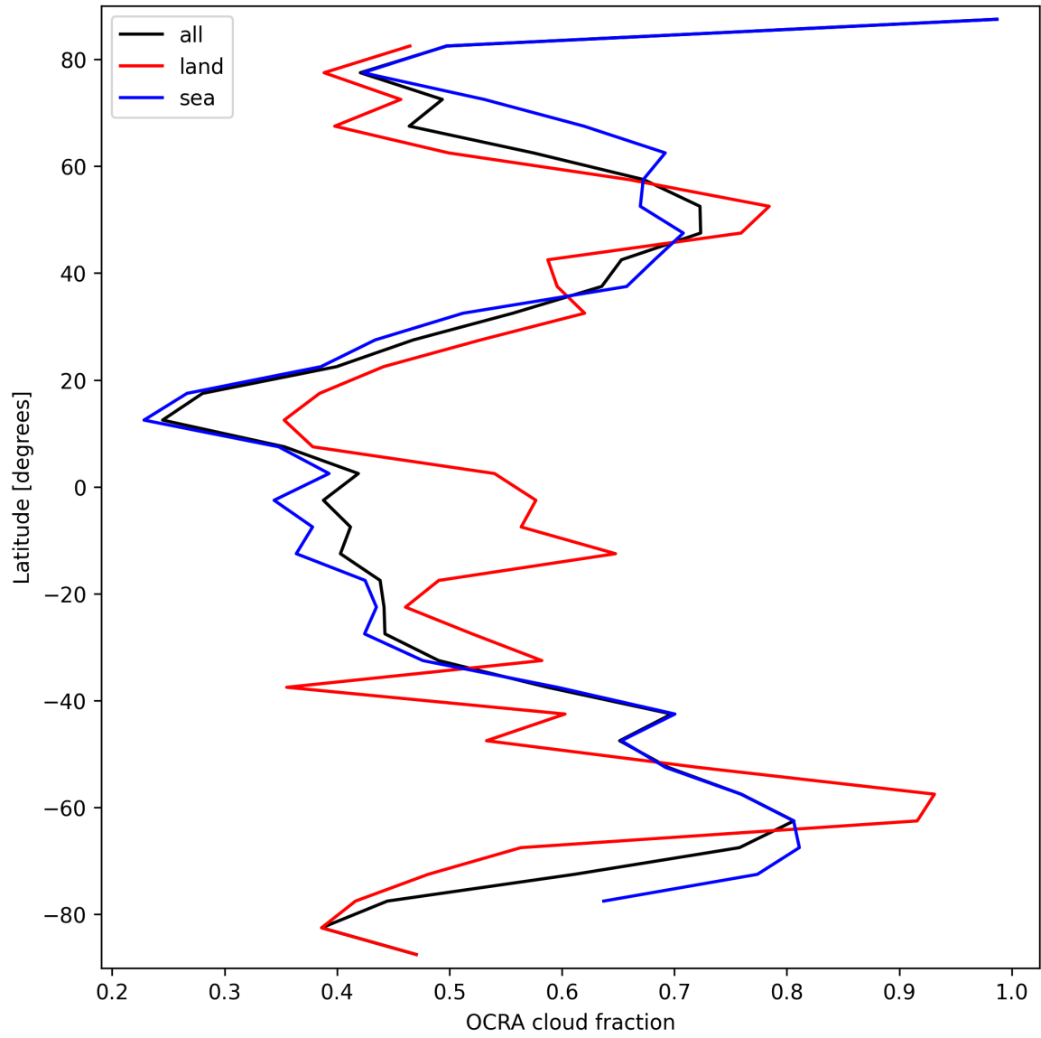
Figure 34: Zonal average of “OCRA cloud fraction” for 2025-03-12 to 2025-03-13.
