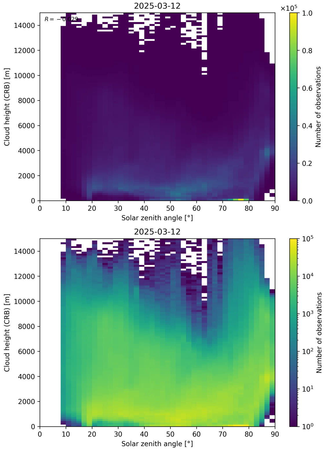
Figure 102: Scatter density plot of “Solar zenith angle” against “Cloud height (CRB)” for 2025-03-12 to 2025-03-13.
