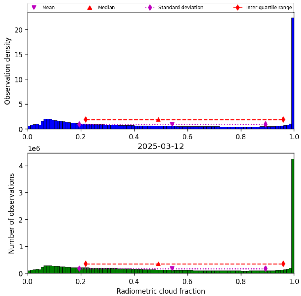
Figure 39: Histogram of “Radiometric cloud fraction” for 2025-03-12 to 2025-03-13
