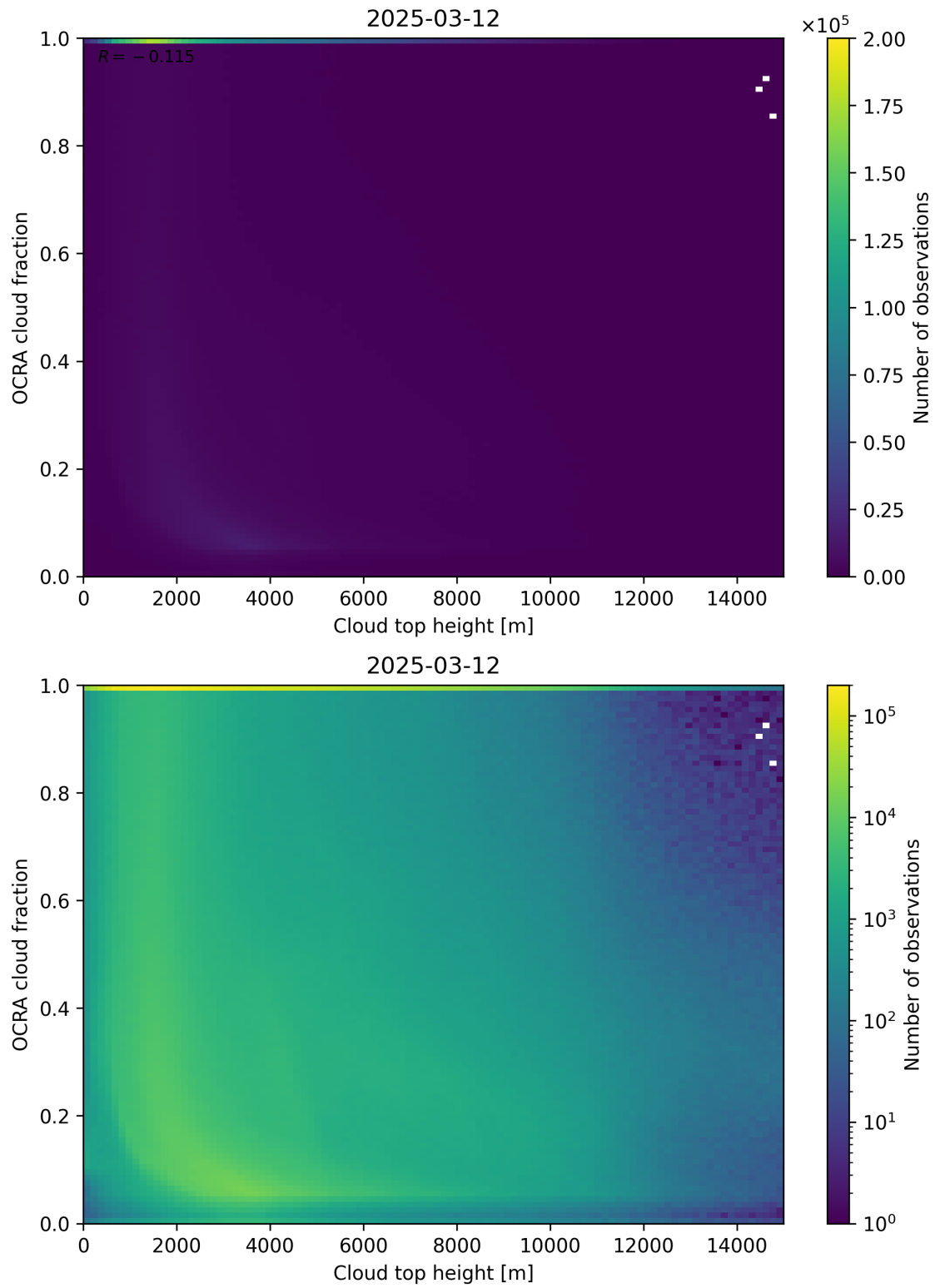
Figure 87: Scatter density plot of “Cloud top height” against “OCRA cloud fraction” for 2025-03-12 to 2025-03-13.
