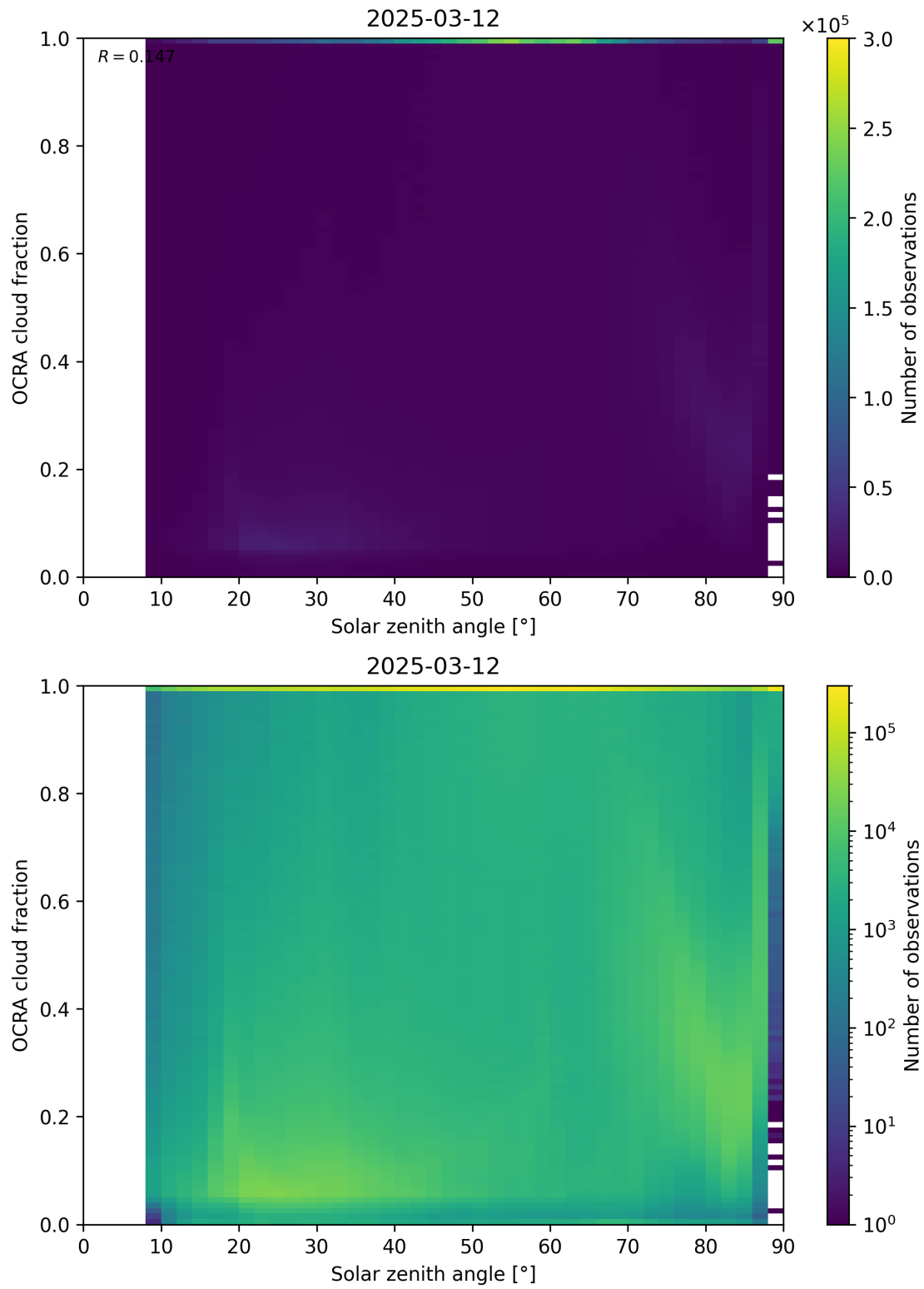
Figure 100: Scatter density plot of “Solar zenith angle” against “OCRA cloud fraction” for 2025-03-12 to 2025-03-13.
