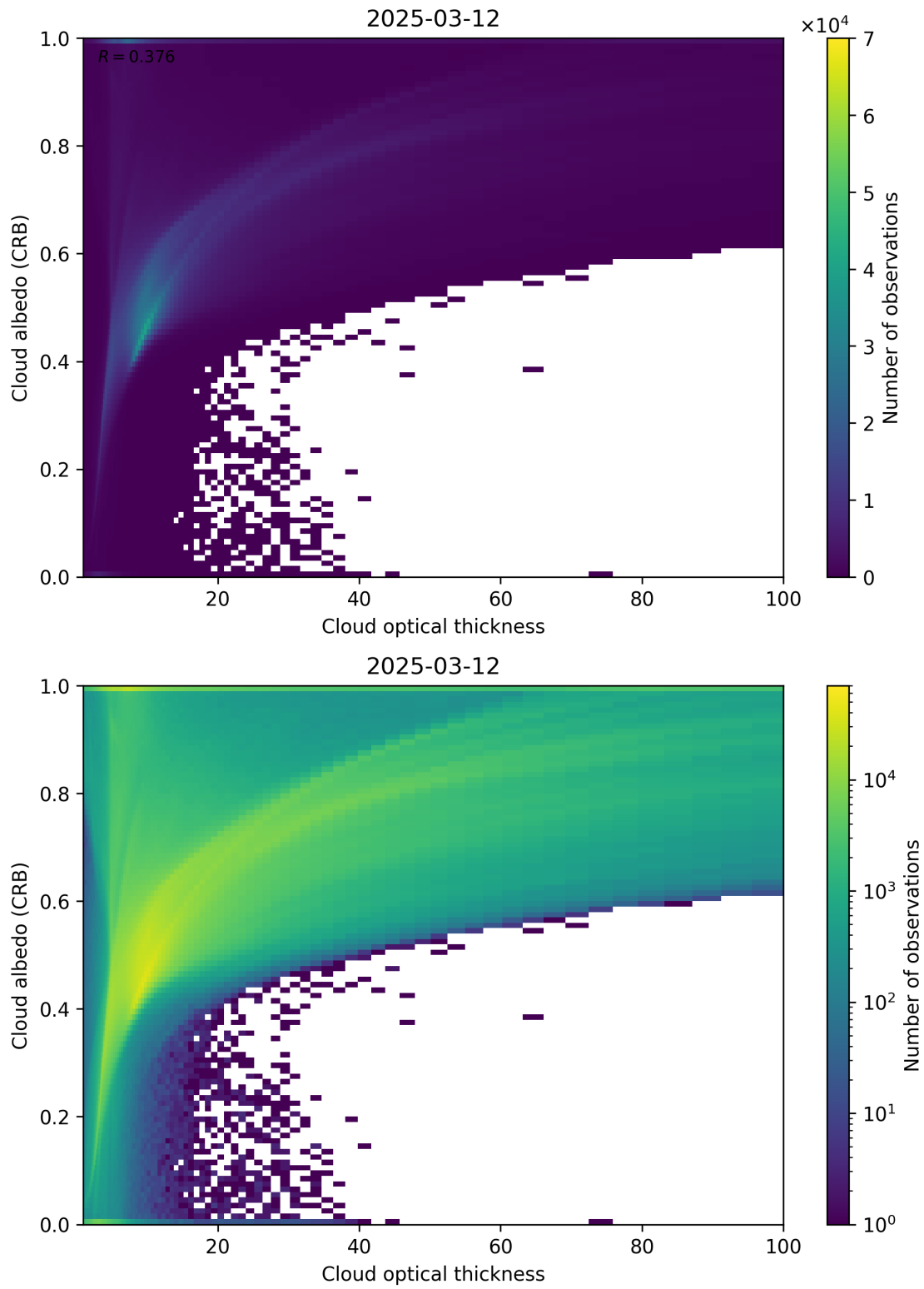
Figure 82: Scatter density plot of “Cloud optical thickness” against “Cloud albedo (CRB)” for 2025-03-12 to 2025-03-13.
