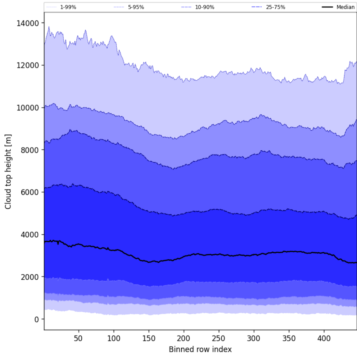
Figure 56: Along track statistics of “Cloud top height” for 2025-03-12 to 2025-03-13
