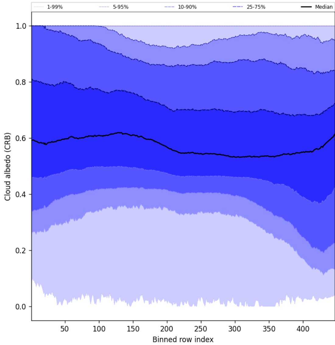
Figure 60: Along track statistics of “Cloud albedo (CRB)” for 2025-03-12 to 2025-03-13
