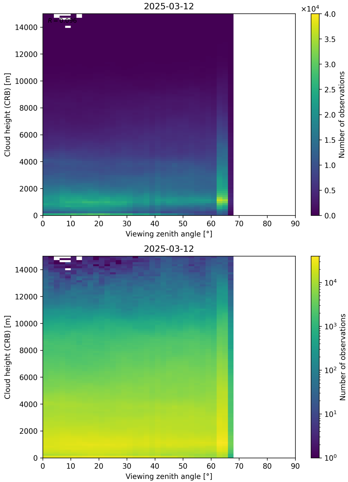
Figure 110: Scatter density plot of “Viewing zenith angle” against “Cloud height (CRB)” for 2025-03-12 to 2025-03-13.
