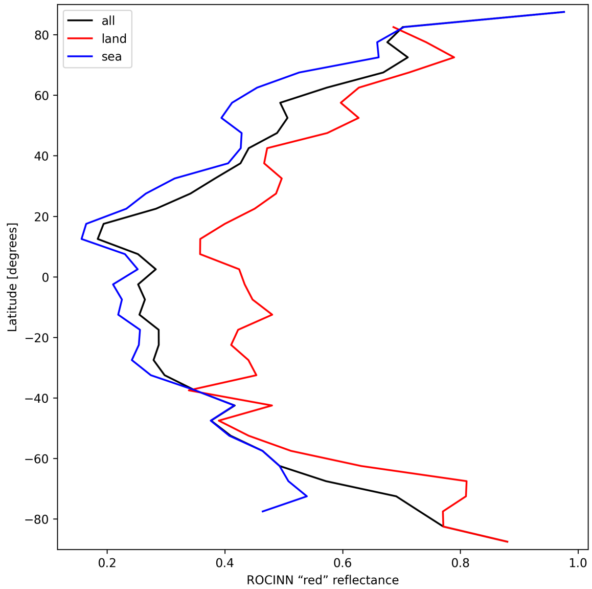
Figure 37: Zonal average of “ROCINN “red” reflectance” for 2025-03-12 to 2025-03-13.
