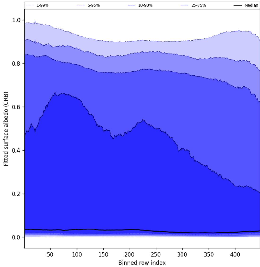
Figure 62: Along track statistics of “Fitted surface albedo (CRB)” for 2025-03-12 to 2025-03-13
