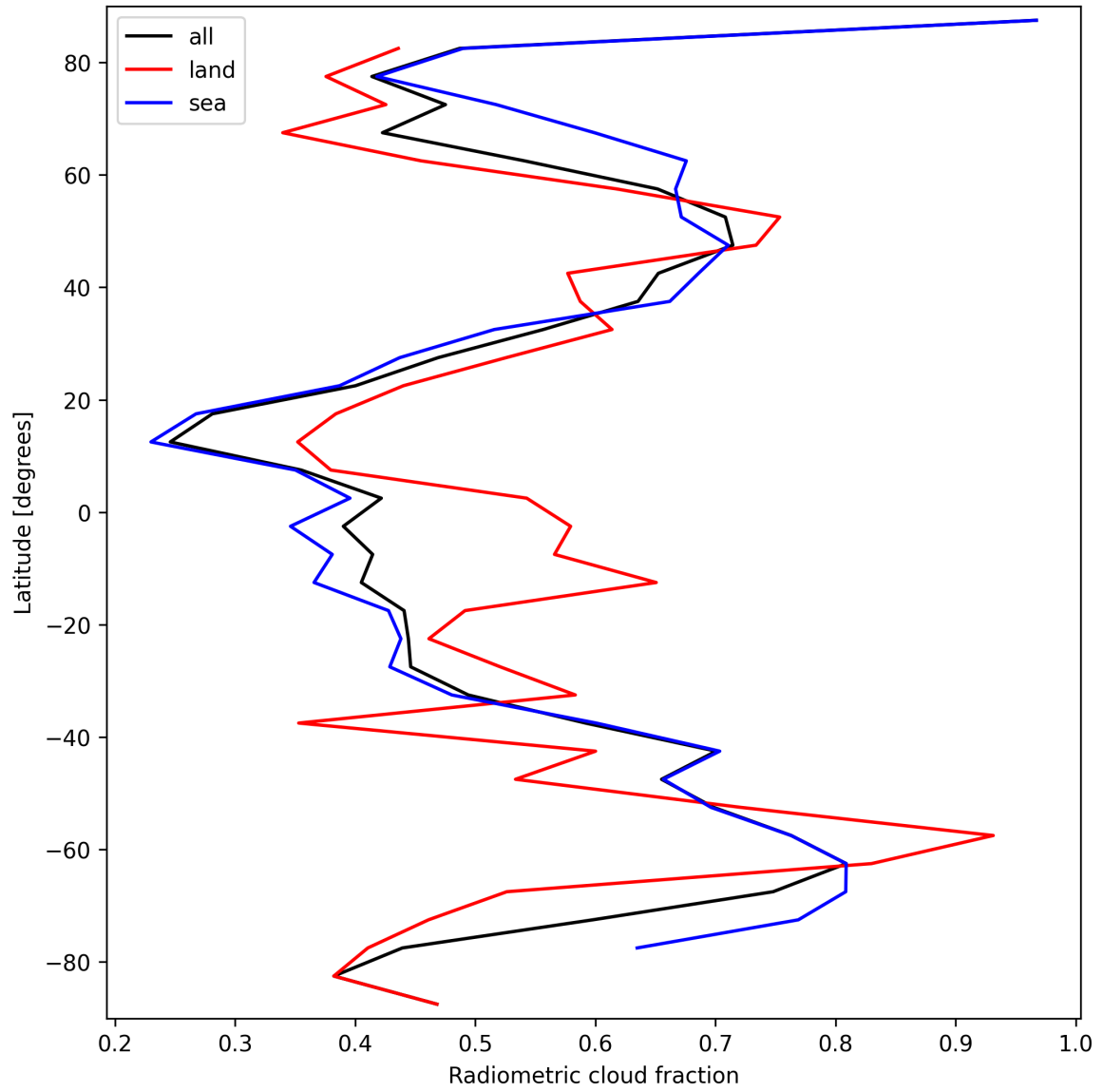
Figure 23: Zonal average of “Radiometric cloud fraction” for 2025-03-12 to 2025-03-13.
