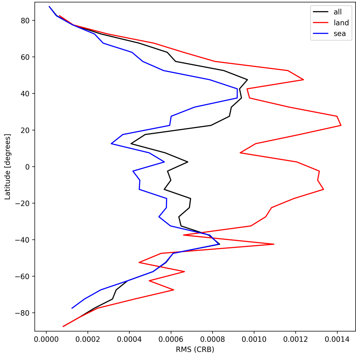
Figure 32: Zonal average of “RMS (CRB)” for 2025-03-12 to 2025-03-13.
