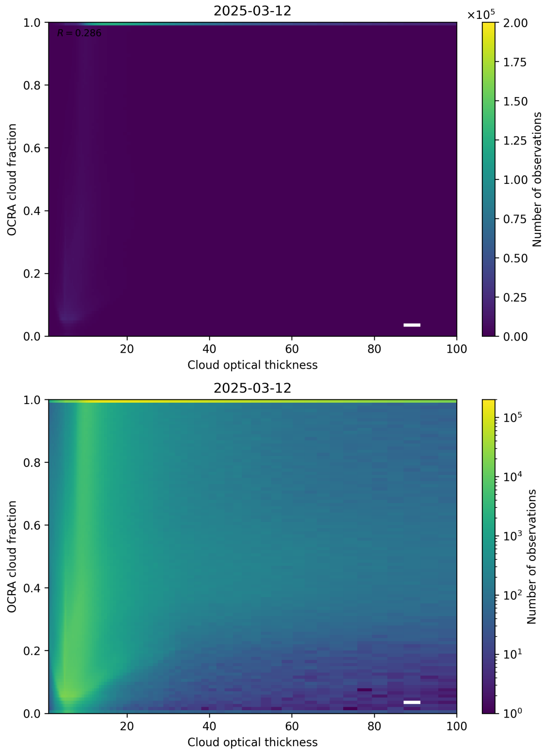
Figure 83: Scatter density plot of “Cloud optical thickness” against “OCRA cloud fraction” for 2025-03-12 to 2025-03-13.
