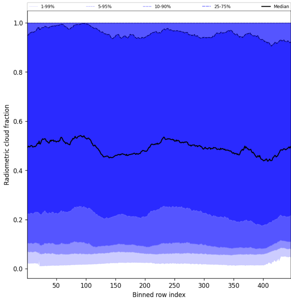
Figure 55: Along track statistics of “Radiometric cloud fraction” for 2025-03-12 to 2025-03-13
