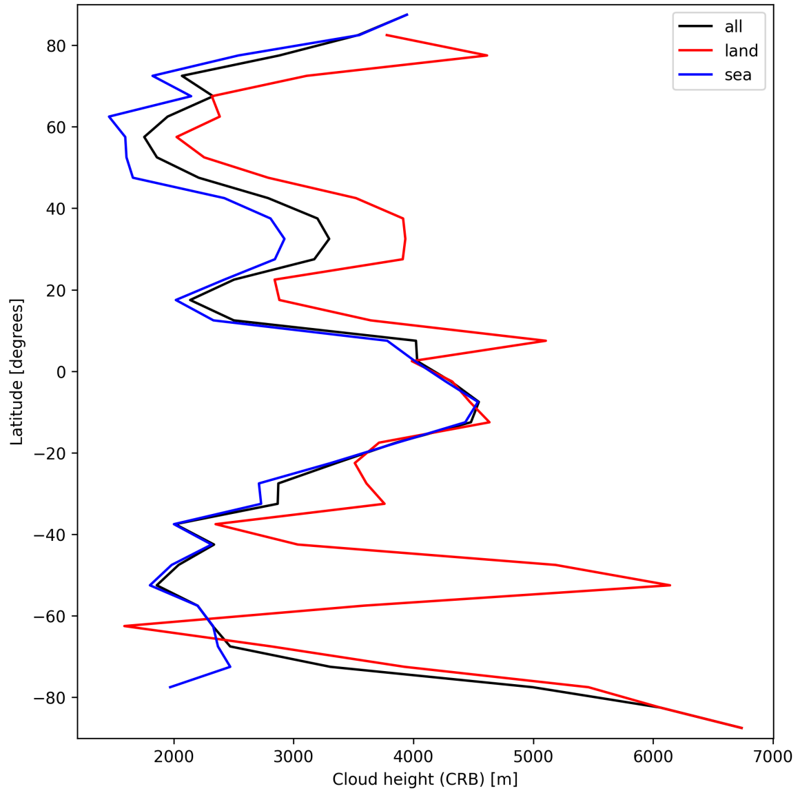
Figure 27: Zonal average of “Cloud height (CRB)” for 2025-03-12 to 2025-03-13.
