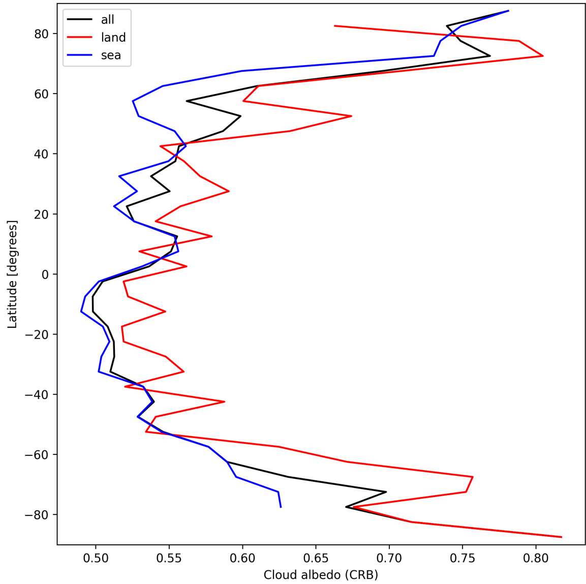
Figure 28: Zonal average of “Cloud albedo (CRB)” for 2025-03-12 to 2025-03-13.
