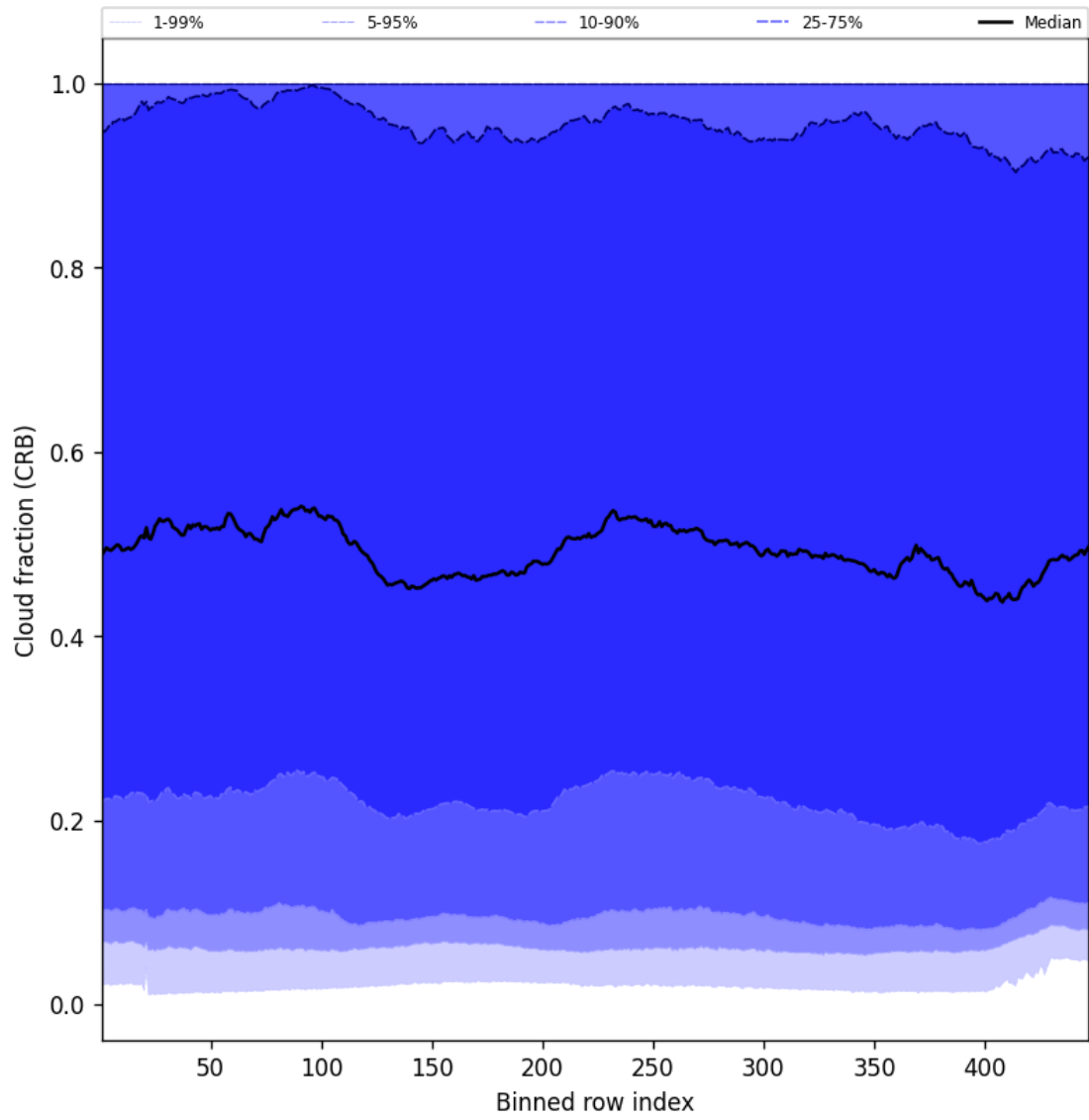
Figure 58: Along track statistics of “Cloud fraction (CRB)” for 2025-03-12 to 2025-03-13
