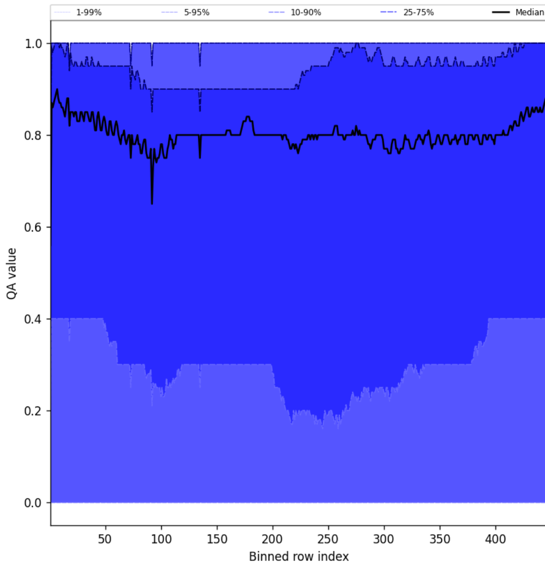
Figure 54: Along track statistics of “QA value” for 2025-03-12 to 2025-03-13
