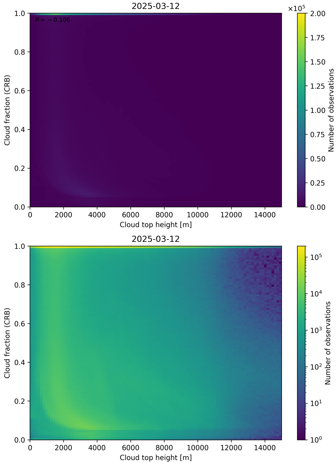
Figure 88: Scatter density plot of “Cloud top height” against “Cloud fraction (CRB)” for 2025-03-12 to 2025-03-13.
