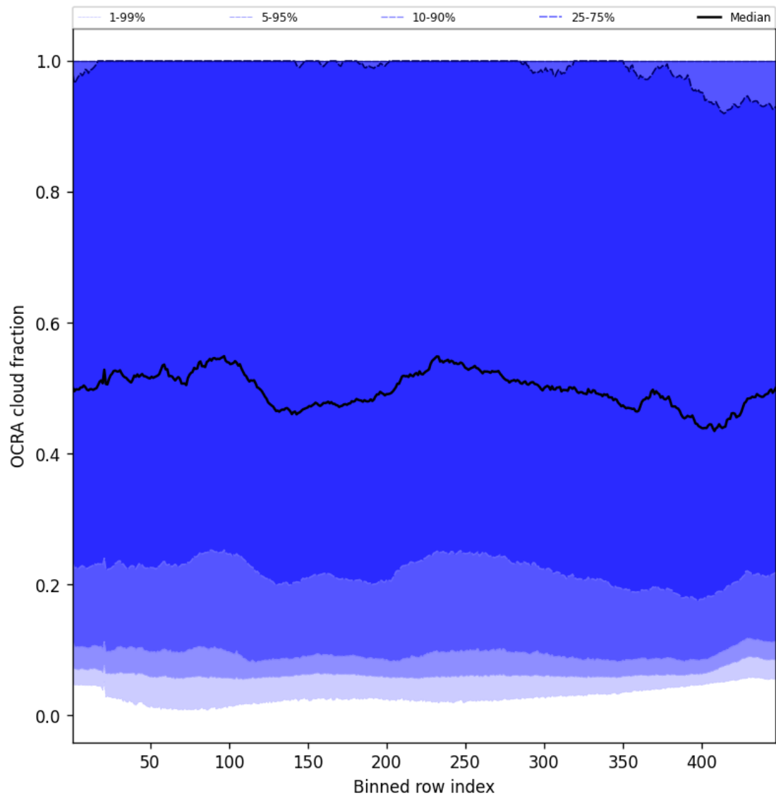
Figure 66: Along track statistics of “OCRA cloud fraction” for 2025-03-12 to 2025-03-13
