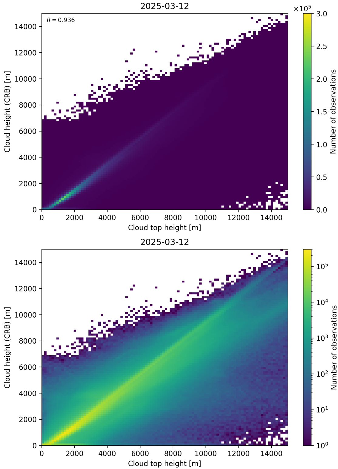
Figure 89: Scatter density plot of “Cloud top height” against “Cloud height (CRB)” for 2025-03-12 to 2025-03-13.
