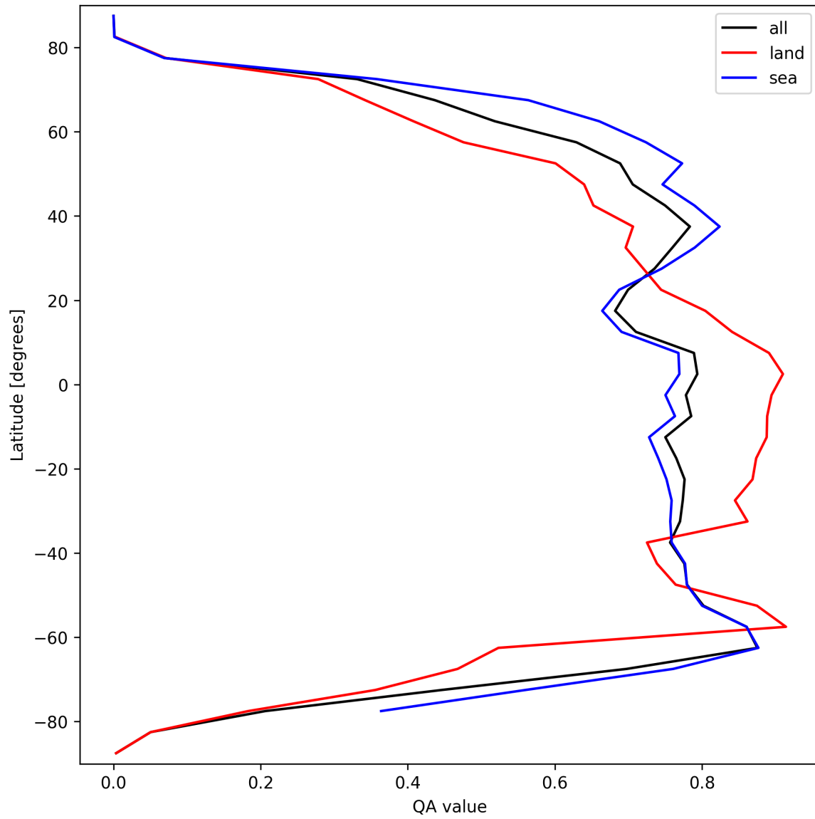
Figure 22: Zonal average of “QA value” for 2025-03-12 to 2025-03-13.
