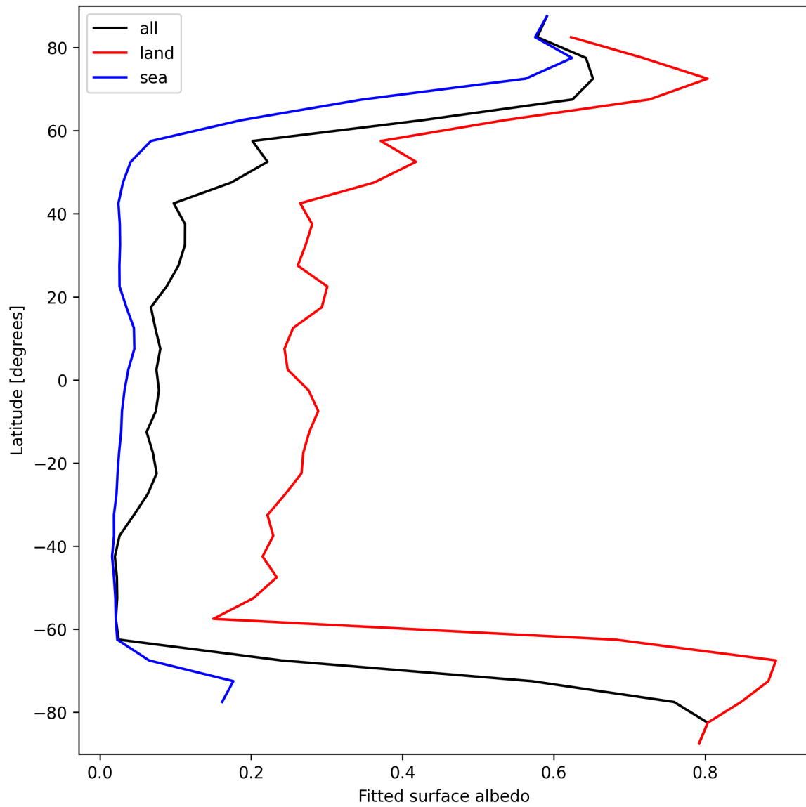
Figure 29: Zonal average of “Fitted surface albedo” for 2025-03-12 to 2025-03-13.
