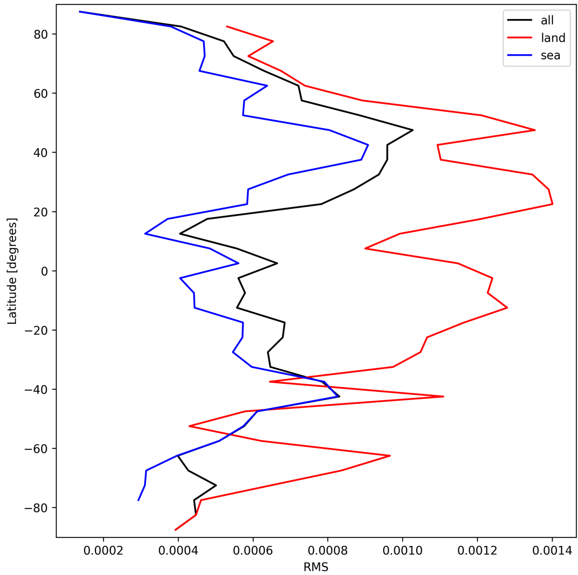
Figure 31: Zonal average of “RMS” for 2025-03-12 to 2025-03-13.
