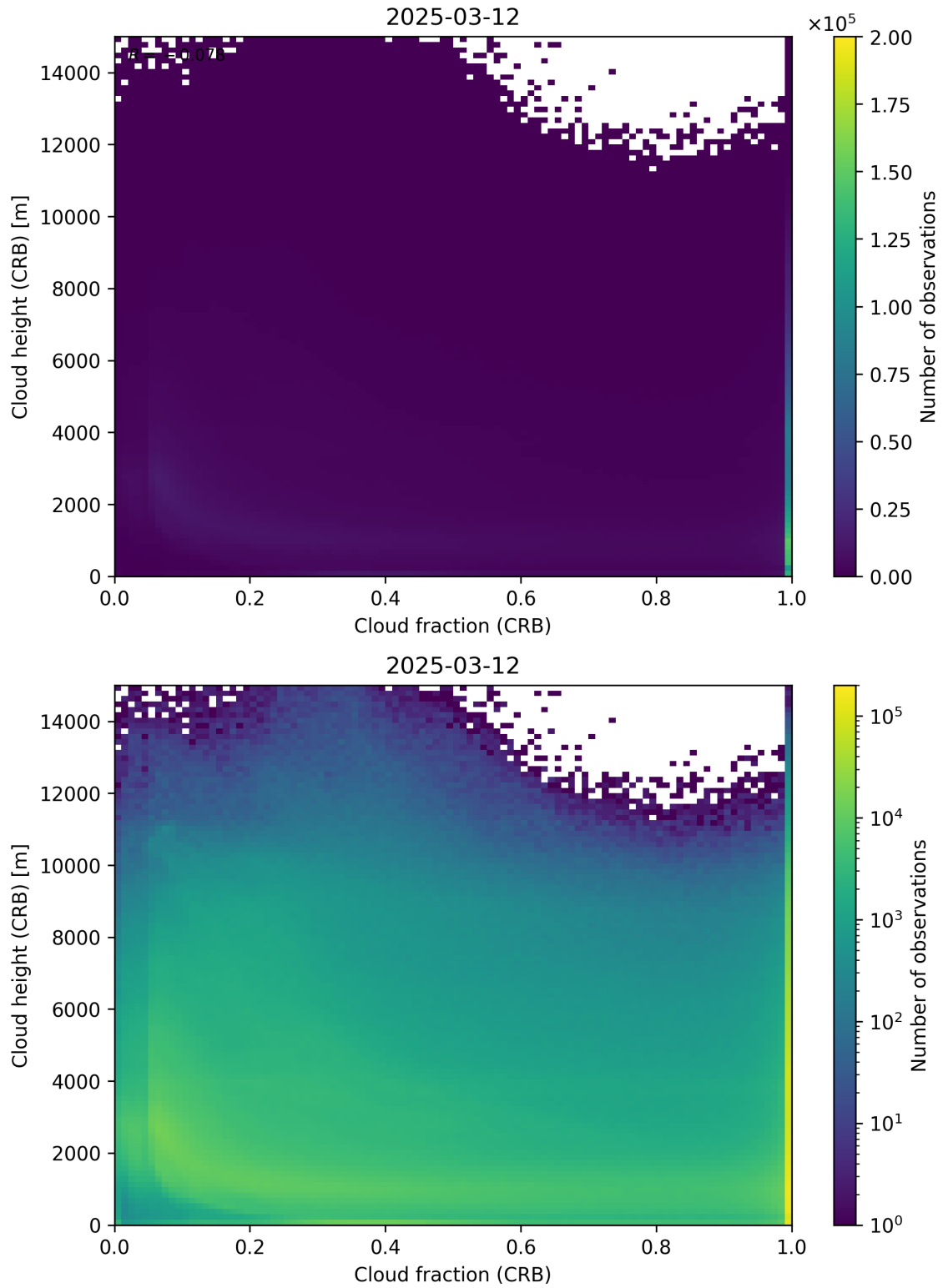
Figure 79: Scatter density plot of “Cloud fraction (CRB)” against “Cloud height (CRB)” for 2025-03-12 to 2025-03-13.
