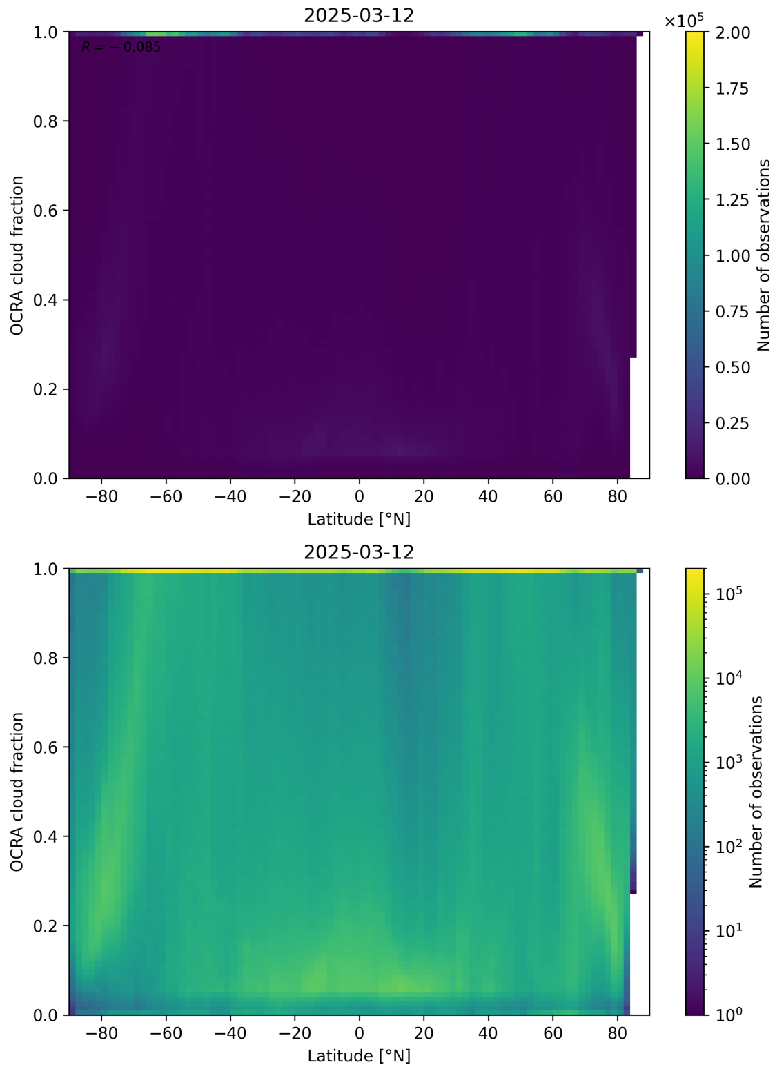
Figure 93: Scatter density plot of “Latitude” against “OCRA cloud fraction” for 2025-03-12 to 2025-03-13.
