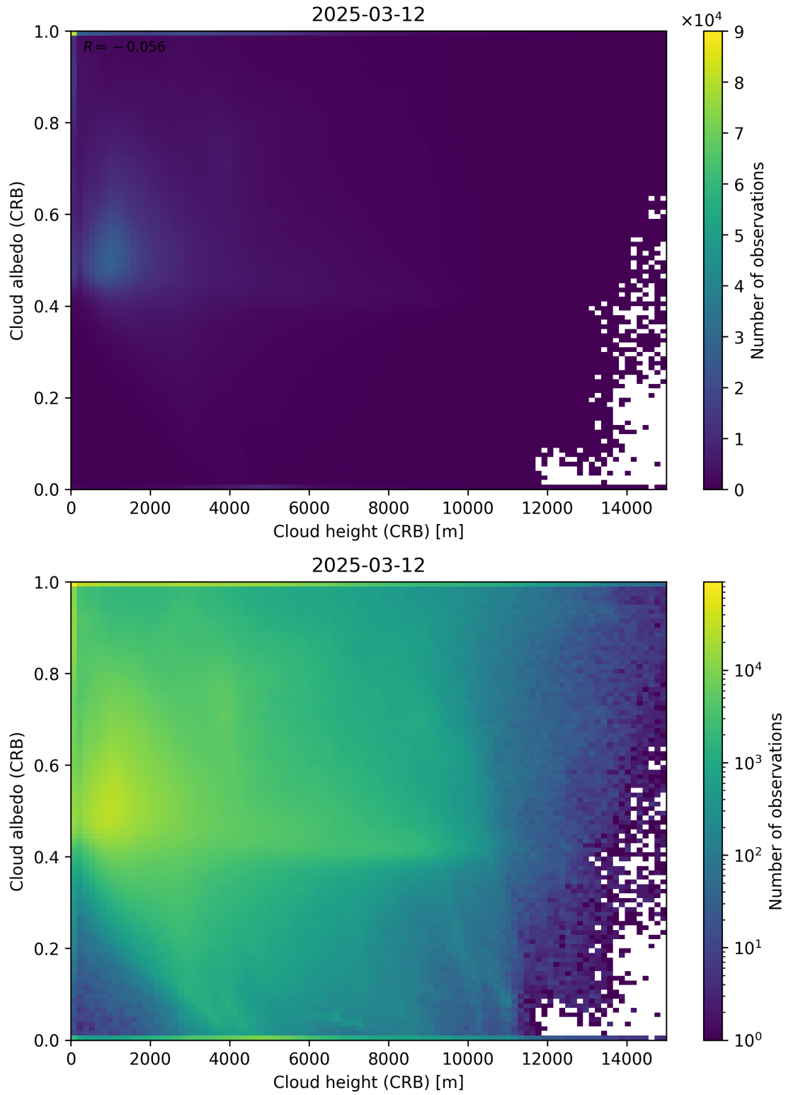
Figure 80: Scatter density plot of “Cloud height (CRB)” against “Cloud albedo (CRB)” for 2025-03-12 to 2025-03-13.
