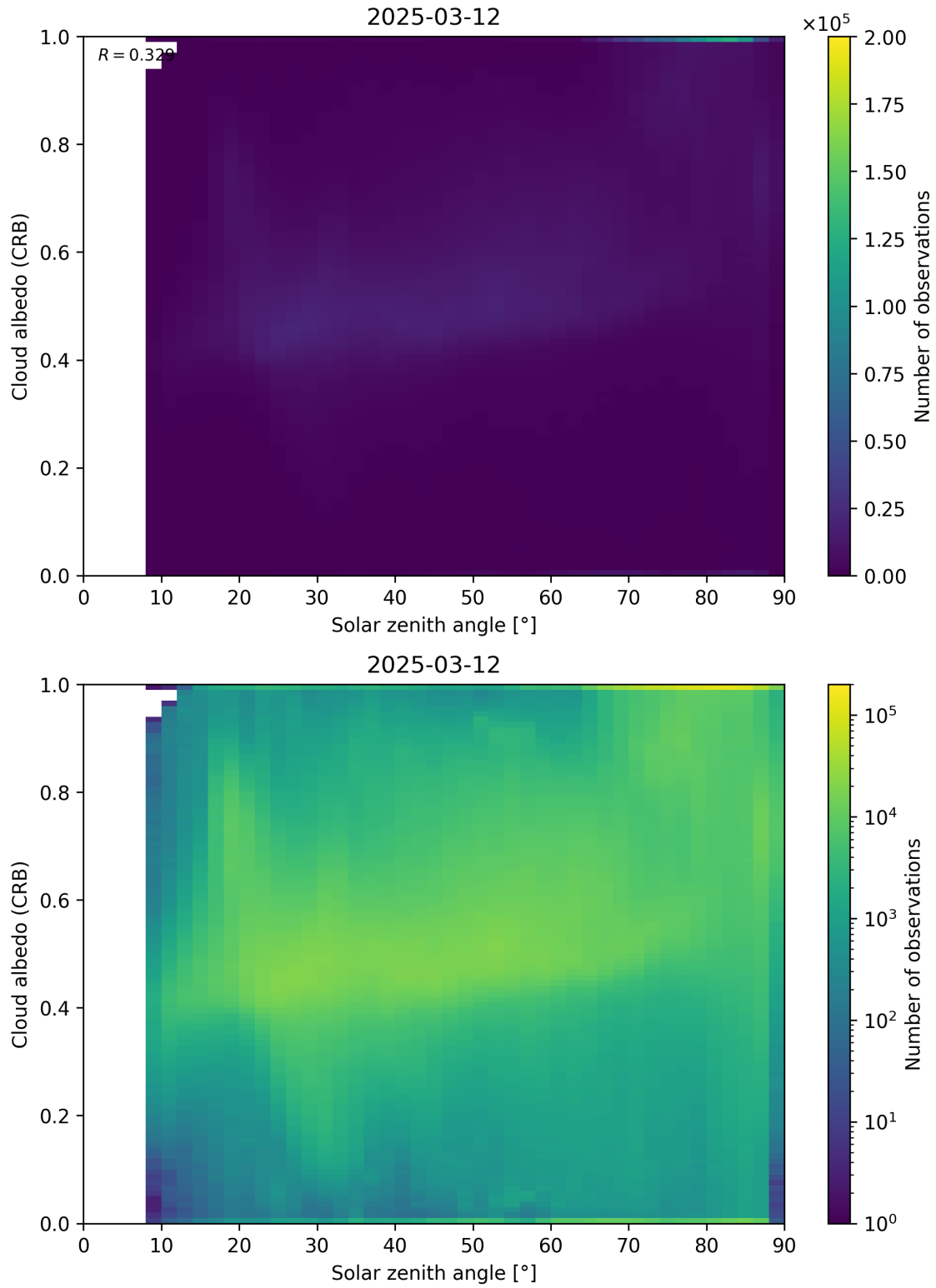
Figure 98: Scatter density plot of “Solar zenith angle” against “Cloud albedo (CRB)” for 2025-03-12 to 2025-03-13.
