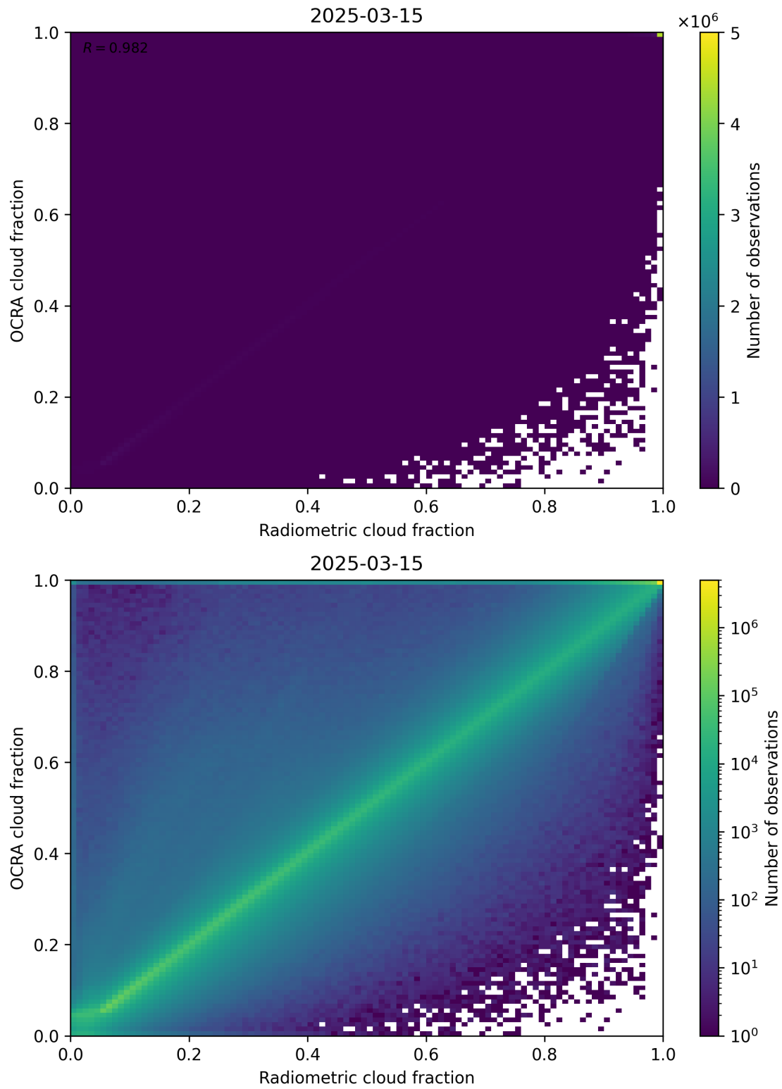
Figure 72: Scatter density plot of “Radiometric cloud fraction” against “OCRA cloud fraction” for 2025-03-14 to 2025-03-16.
