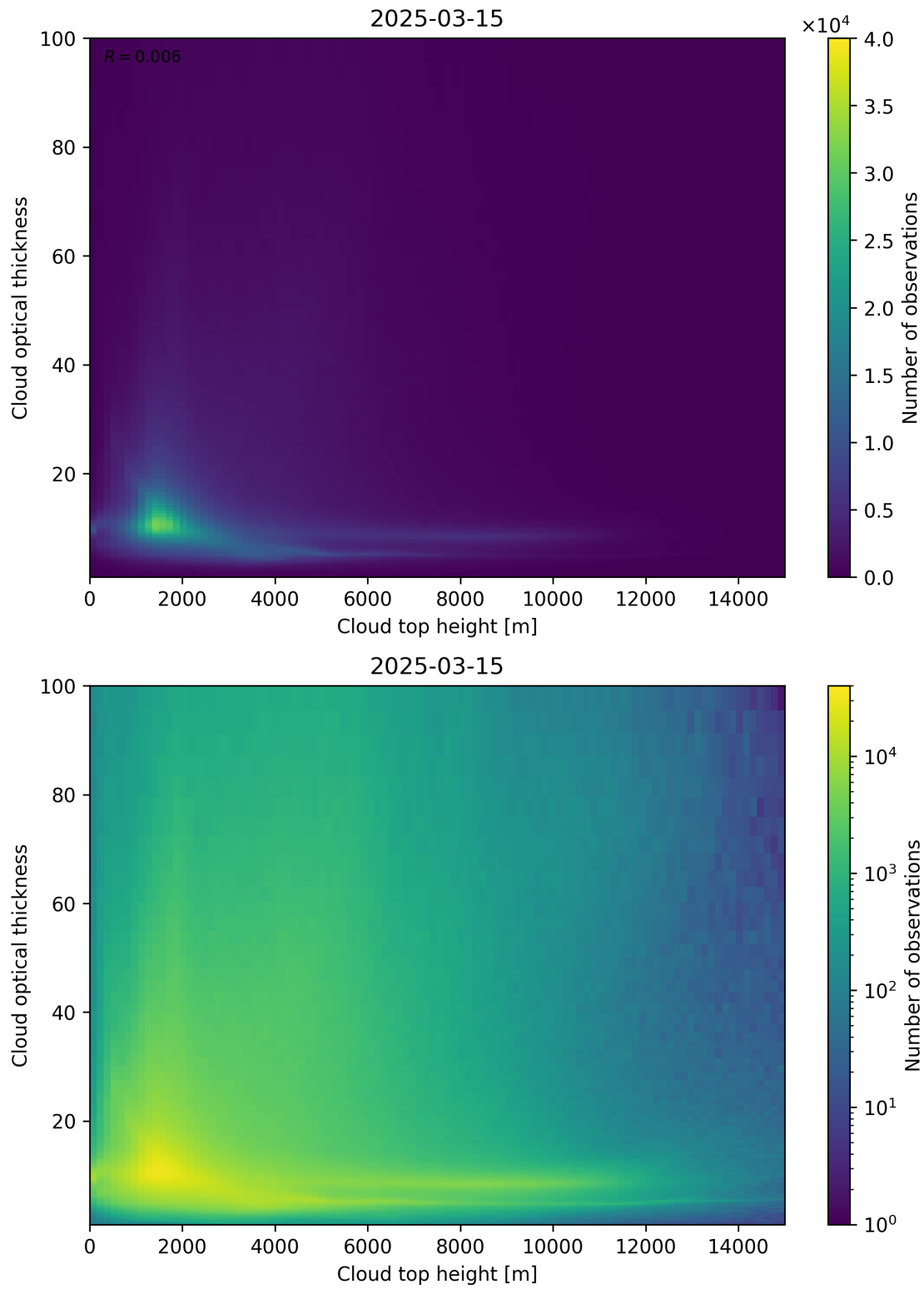
Figure 90: Scatter density plot of “Cloud top height” against “Cloud optical thickness” for 2025-03-14 to 2025-03-16.
