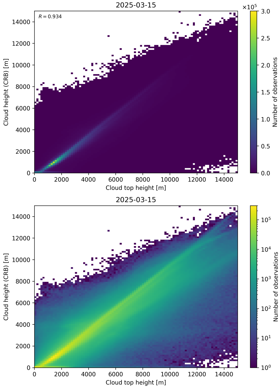
Figure 89: Scatter density plot of “Cloud top height” against “Cloud height (CRB)” for 2025-03-14 to 2025-03-16.
