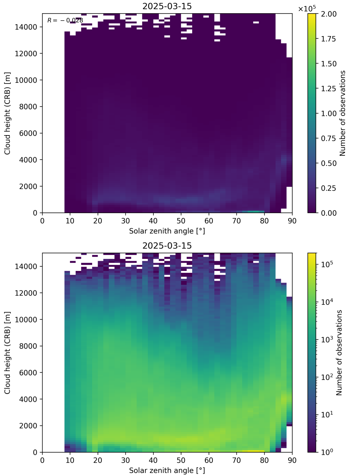
Figure 102: Scatter density plot of “Solar zenith angle” against “Cloud height (CRB)” for 2025-03-14 to 2025-03-16.
