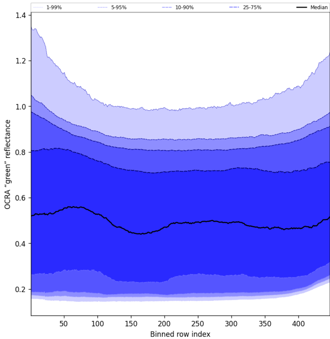
Figure 68: Along track statistics of "OCRA "green" reflectance" for 2025-03-14 to 2025-03-16
