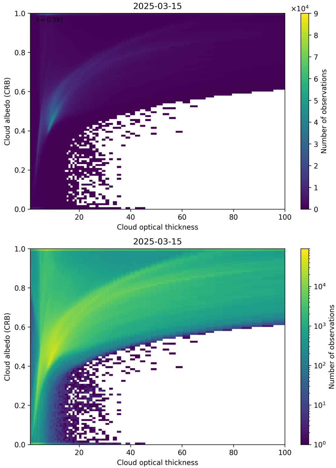
Figure 82: Scatter density plot of “Cloud optical thickness” against “Cloud albedo (CRB)” for 2025-03-14 to 2025-03-16.
