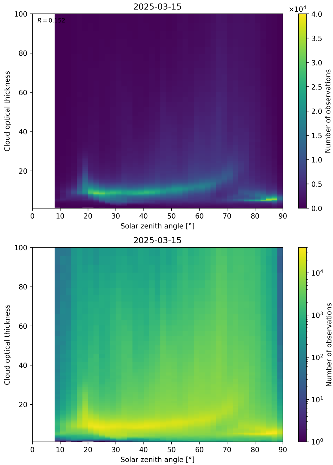
Figure 103: Scatter density plot of “Solar zenith angle” against “Cloud optical thickness” for 2025-03-14 to 2025-03-16.
