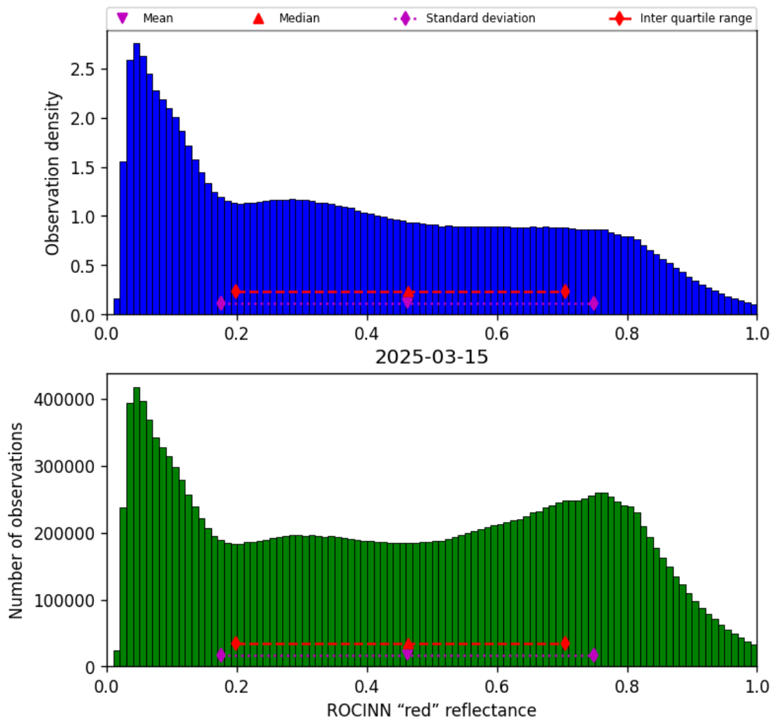
Figure 53: Histogram of “ROCINN “red” reflectance” for 2025-03-14 to 2025-03-16
