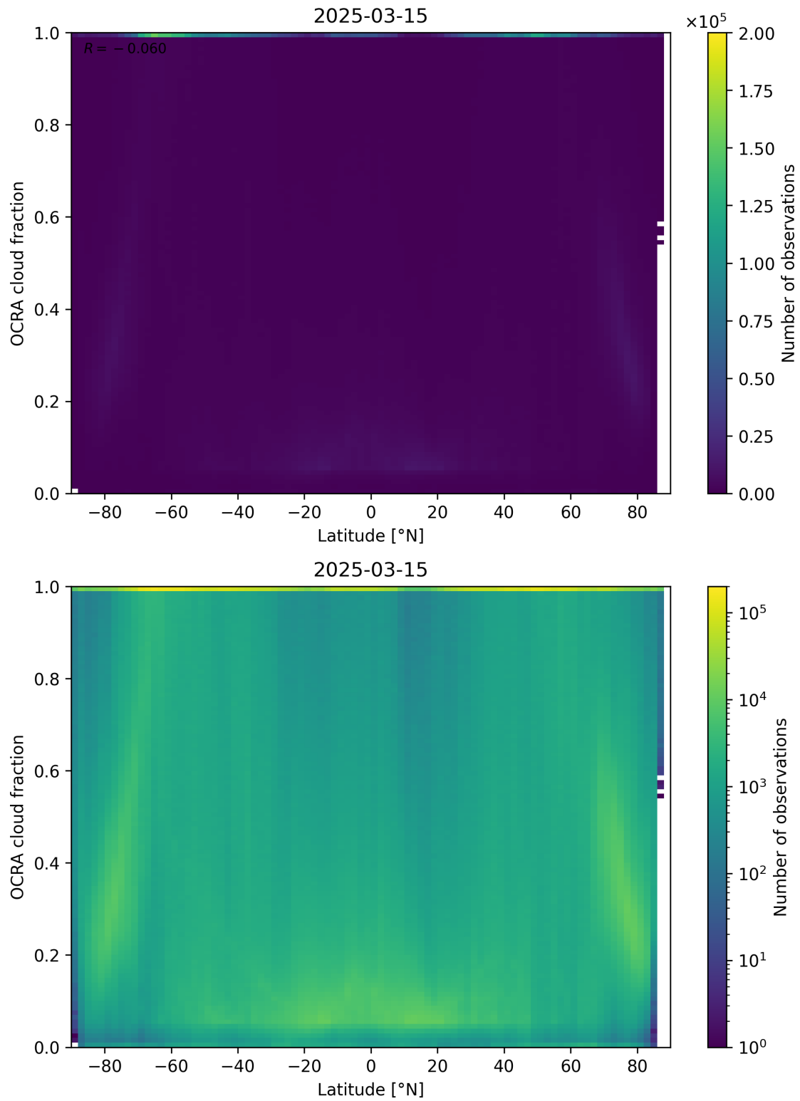
Figure 93: Scatter density plot of “Latitude” against “OCRA cloud fraction” for 2025-03-14 to 2025-03-16.
