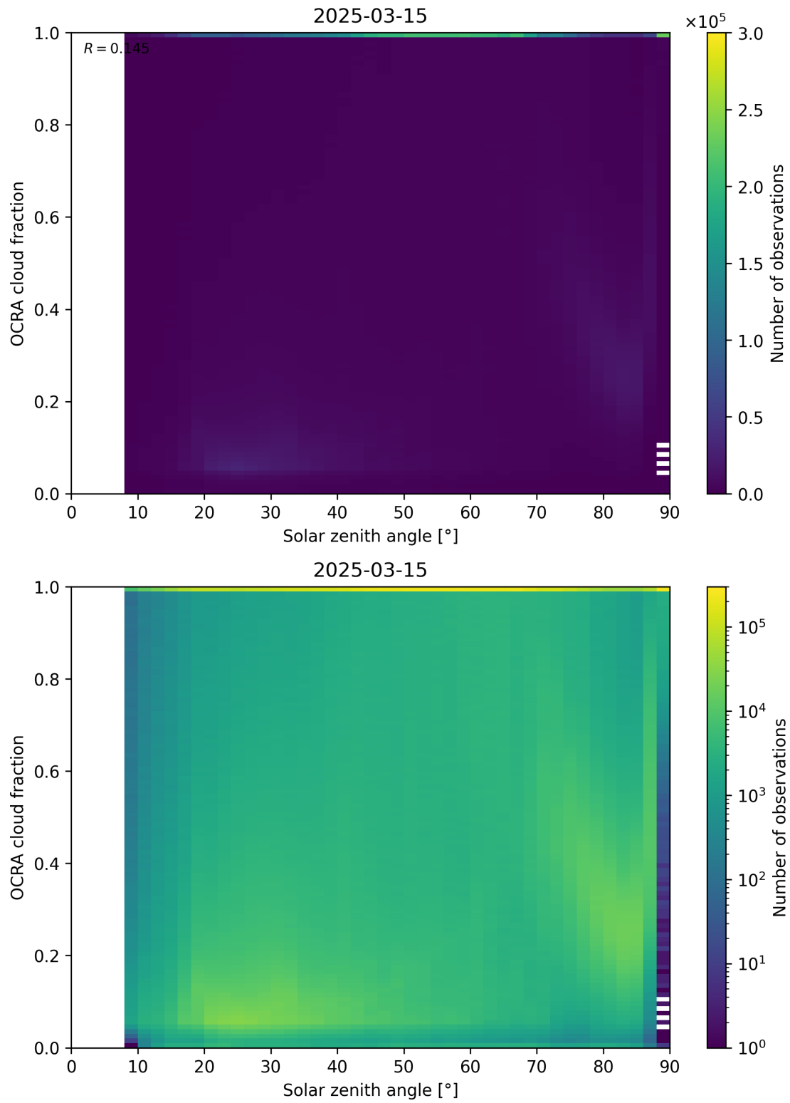
Figure 100: Scatter density plot of “Solar zenith angle” against “OCRA cloud fraction” for 2025-03-14 to 2025-03-16.
