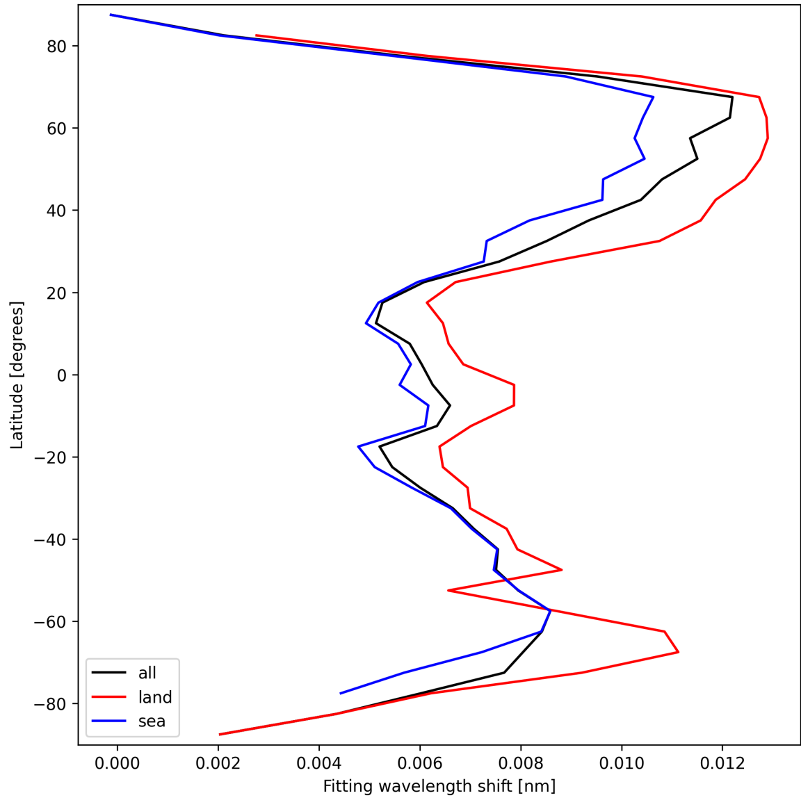
Figure 33: Zonal average of “Fitting wavelength shift” for 2025-03-14 to 2025-03-16.
