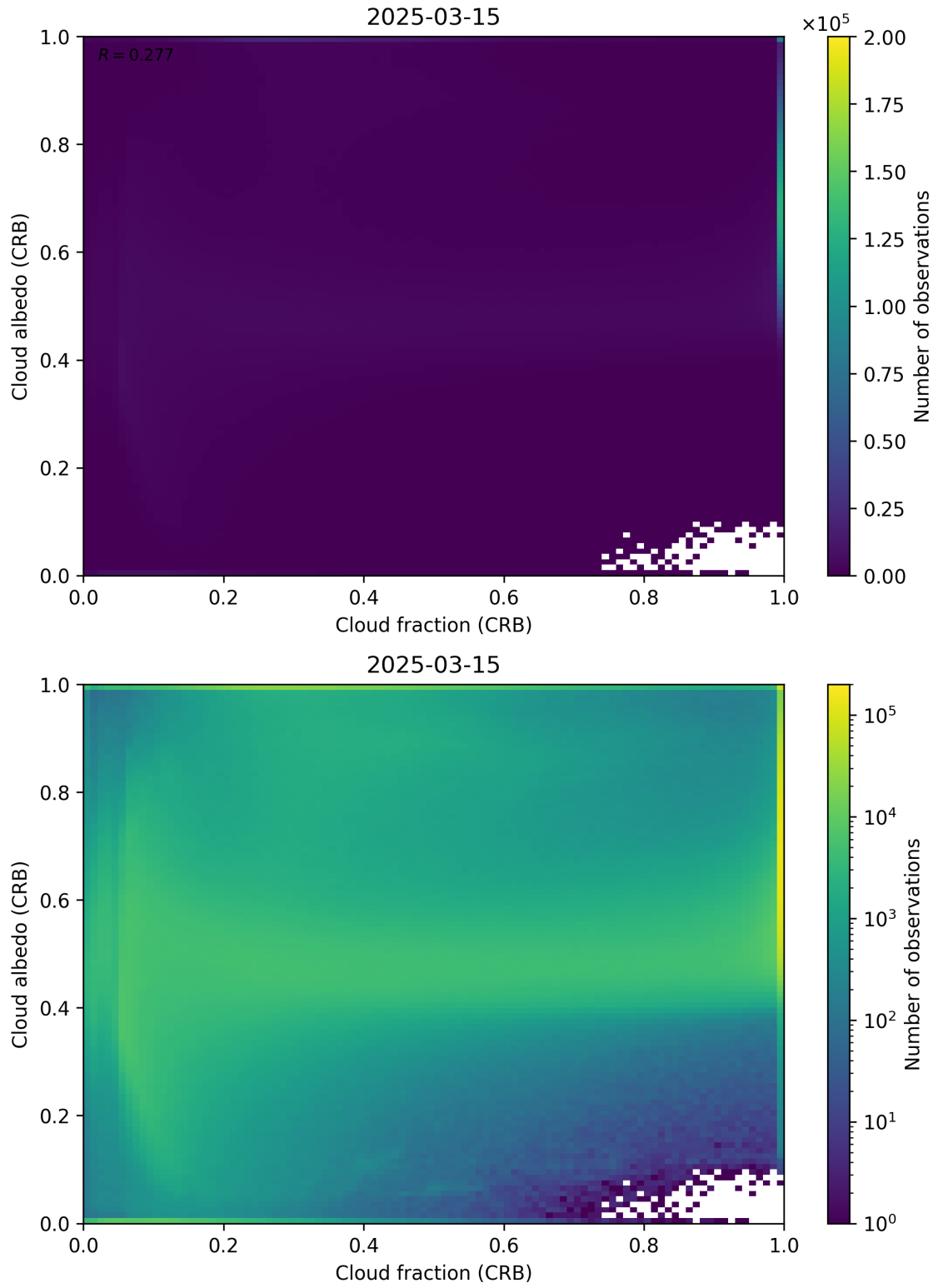
Figure 77: Scatter density plot of “Cloud fraction (CRB)” against “Cloud albedo (CRB)” for 2025-03-14 to 2025-03-16.
