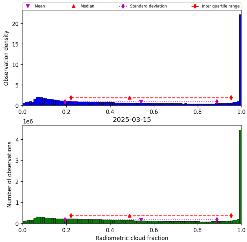
Figure 39: Histogram of “Radiometric cloud fraction” for 2025-03-14 to 2025-03-16
