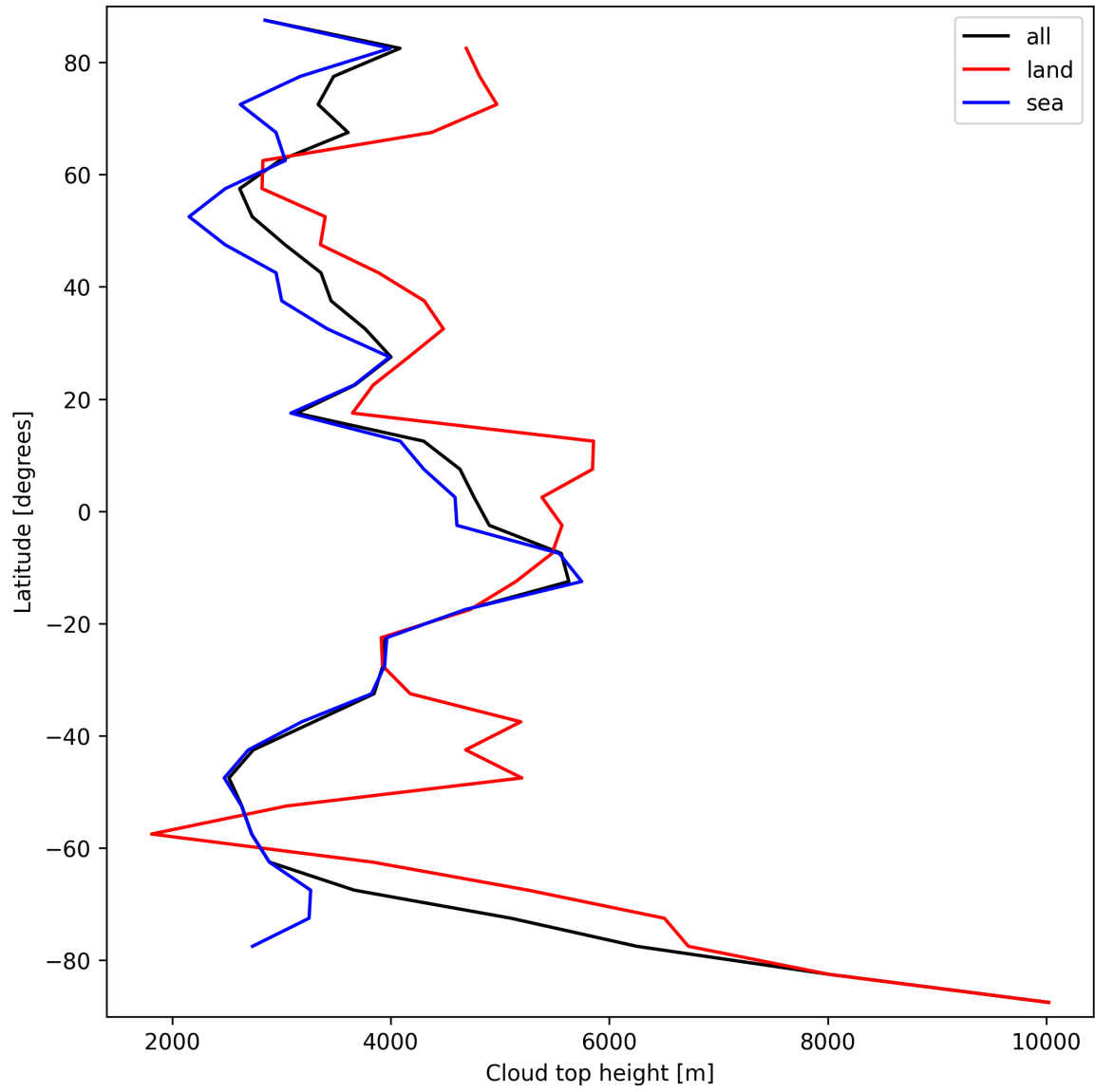
Figure 24: Zonal average of “Cloud top height” for 2025-03-14 to 2025-03-16.
