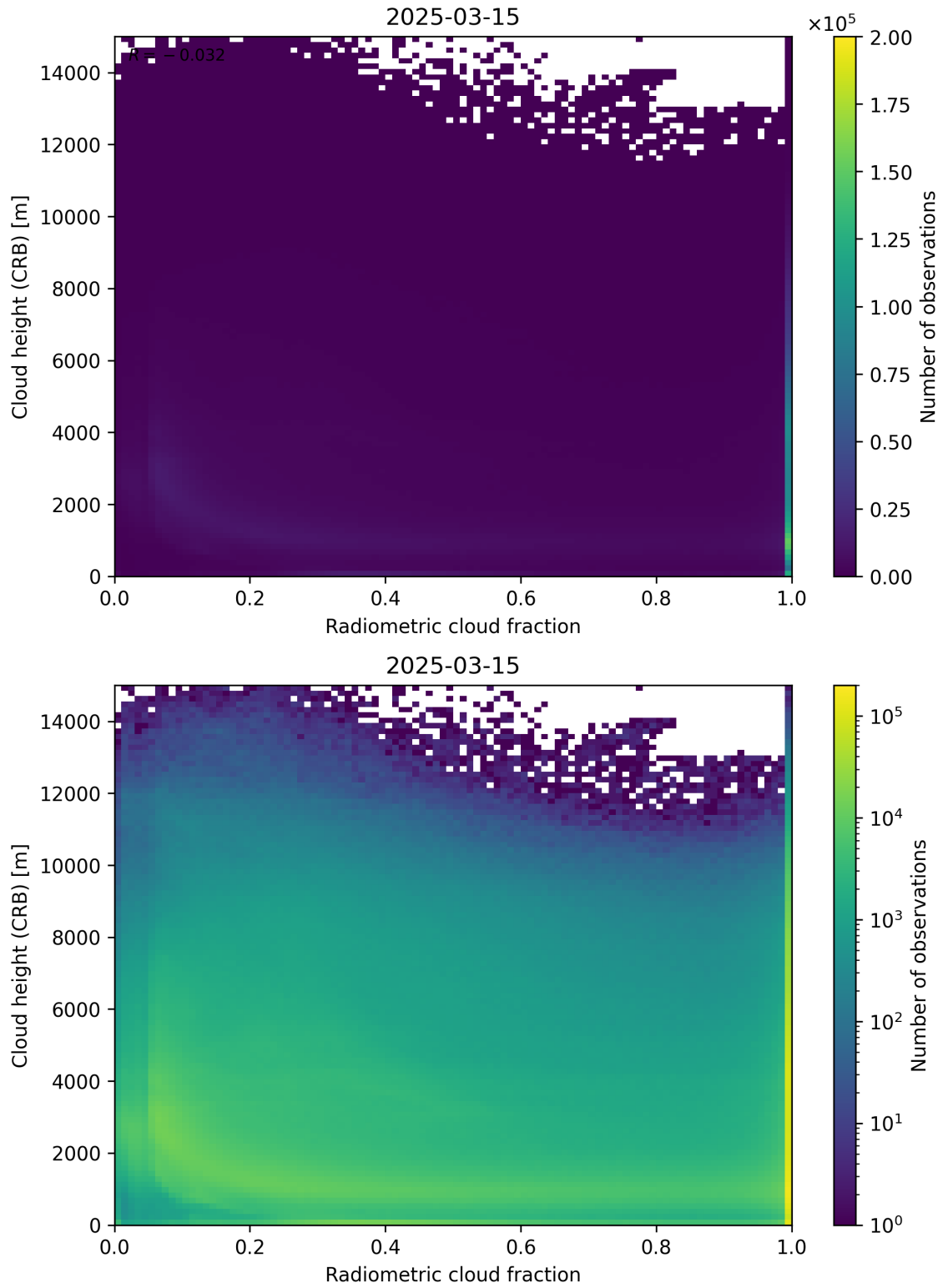
Figure 74: Scatter density plot of “Radiometric cloud fraction” against “Cloud height (CRB)” for 2025-03-14 to 2025-03-16.
