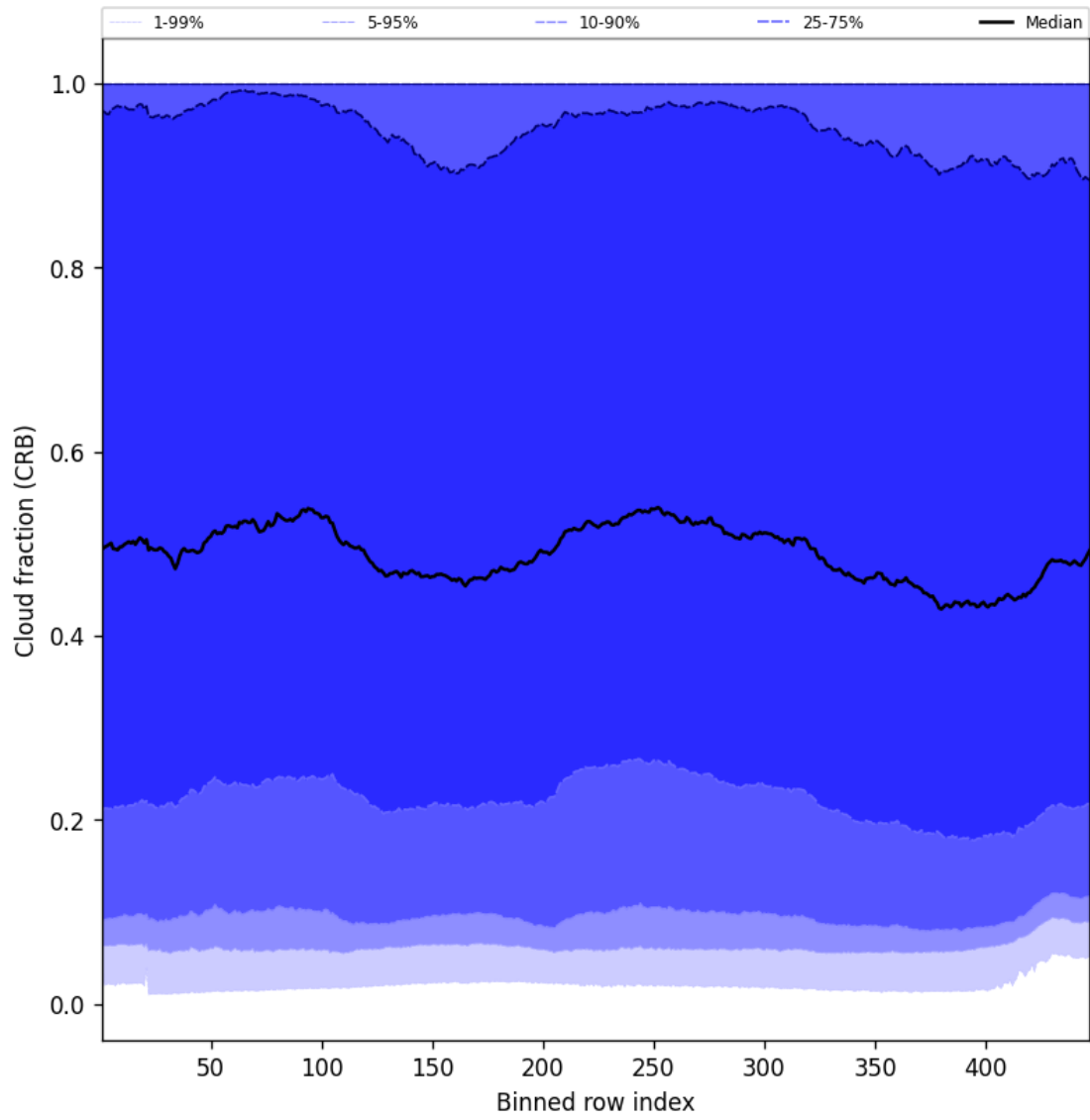
Figure 58: Along track statistics of “Cloud fraction (CRB)” for 2025-03-14 to 2025-03-16
