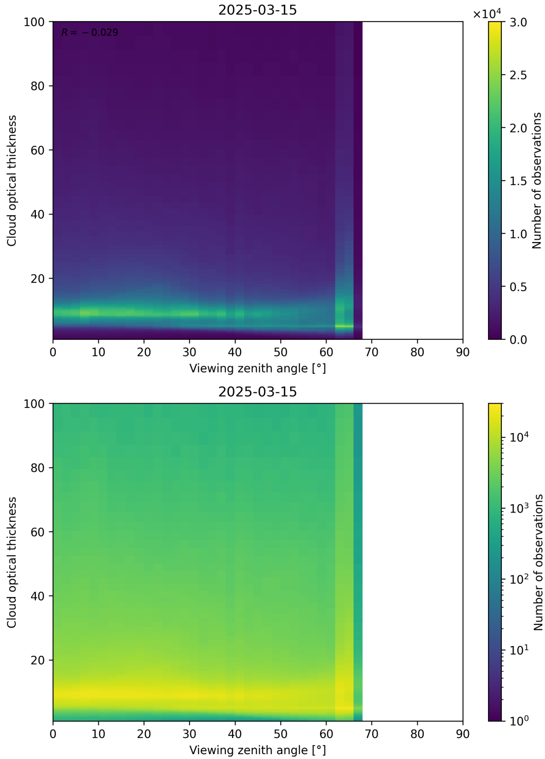
Figure 111: Scatter density plot of “Viewing zenith angle” against “Cloud optical thickness” for 2025-03-14 to 2025-03-16.
