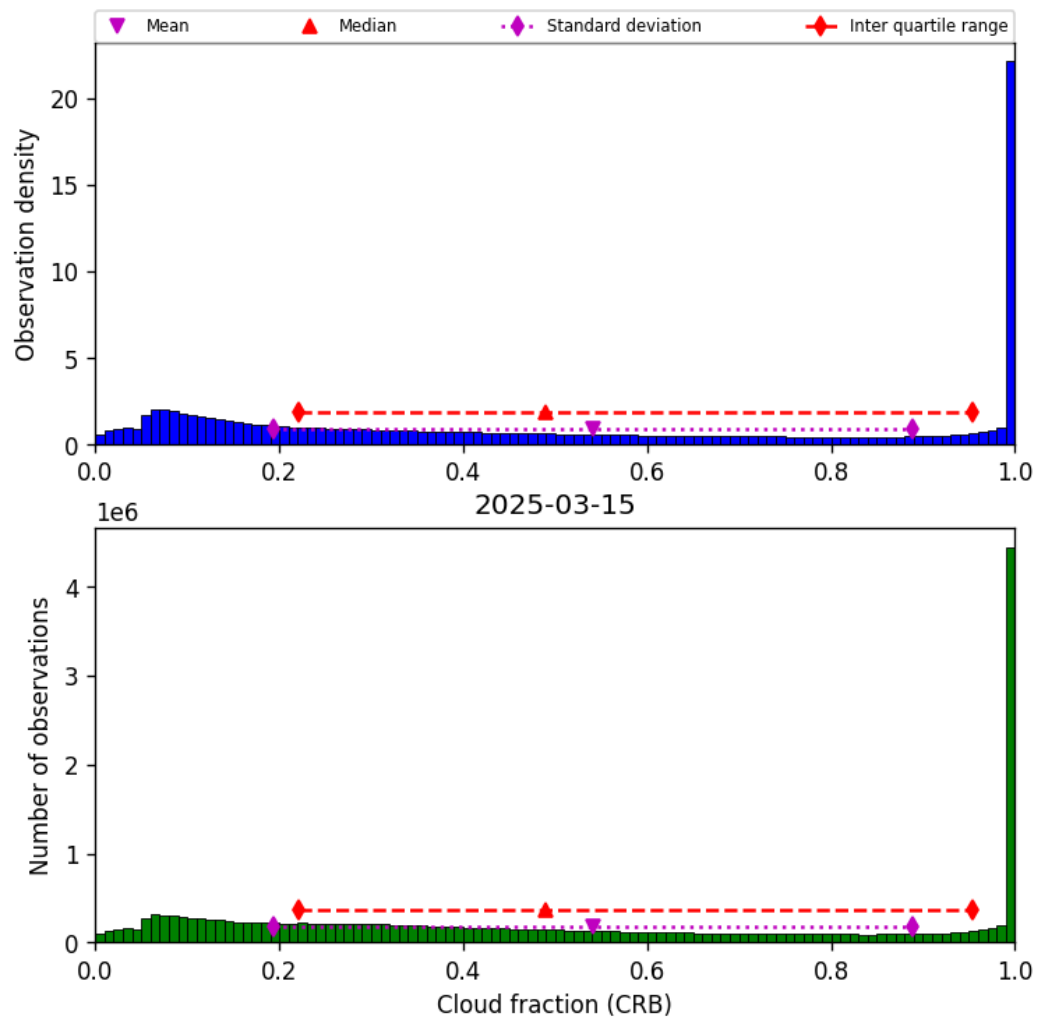
Figure 42: Histogram of “Cloud fraction (CRB)” for 2025-03-14 to 2025-03-16
