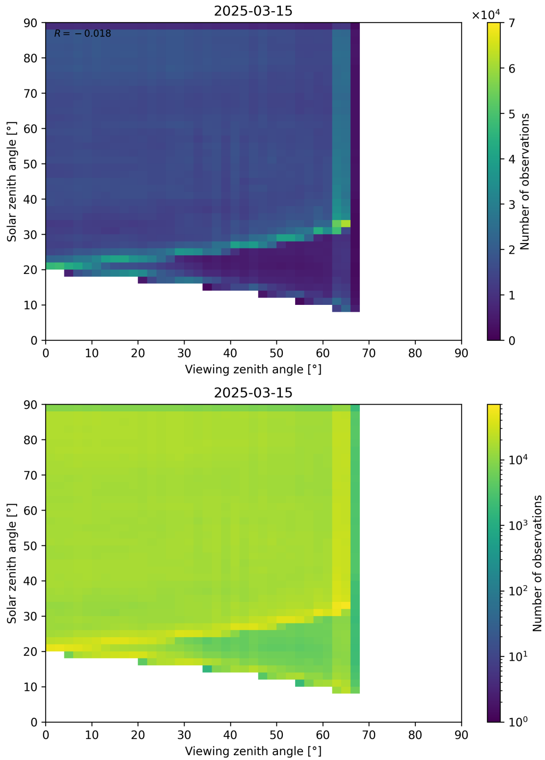
Figure 114: Scatter density plot of “Viewing zenith angle” against “Solar zenith angle” for 2025-03-14 to 2025-03-16.
