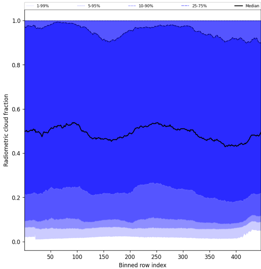
Figure 55: Along track statistics of “Radiometric cloud fraction” for 2025-03-14 to 2025-03-16
