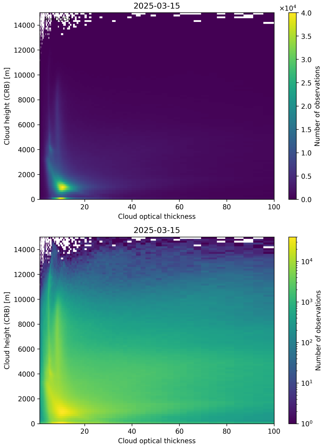
Figure 85: Scatter density plot of “Cloud optical thickness” against “Cloud height (CRB)” for 2025-03-14 to 2025-03-16.
