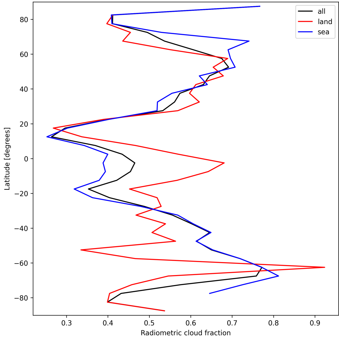
Figure 23: Zonal average of “Radiometric cloud fraction” for 2025-03-14 to 2025-03-16.
