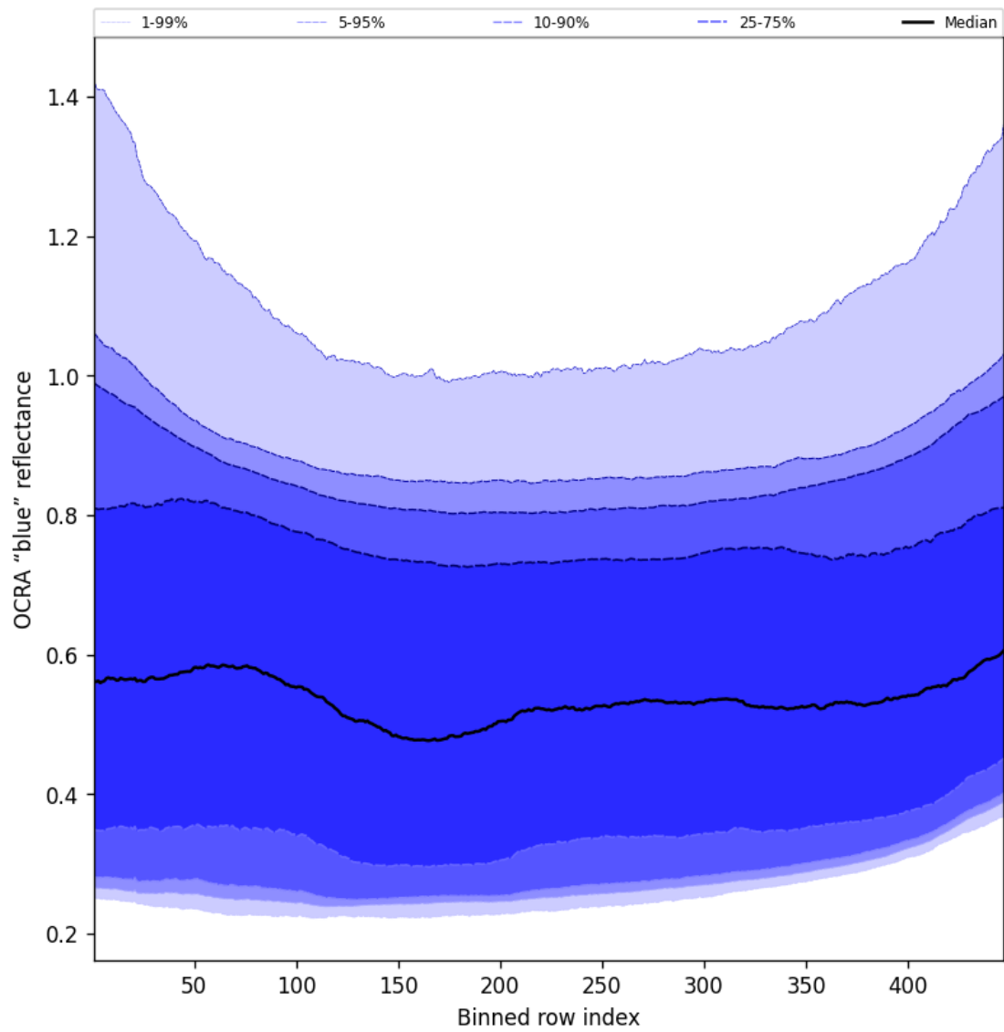
Figure 67: Along track statistics of “OCRA “blue” reflectance” for 2025-03-14 to 2025-03-16
