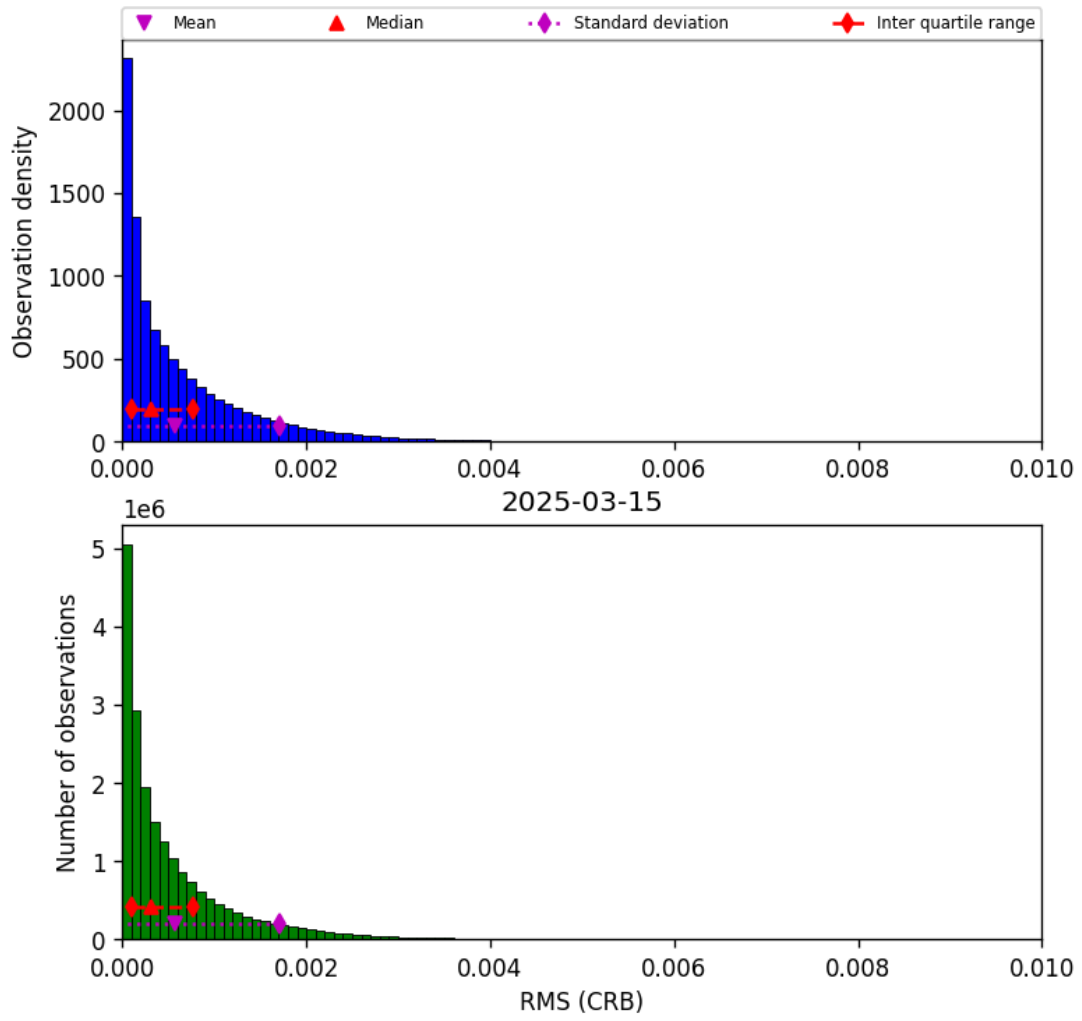
Figure 48: Histogram of “RMS (CRB)” for 2025-03-14 to 2025-03-16
