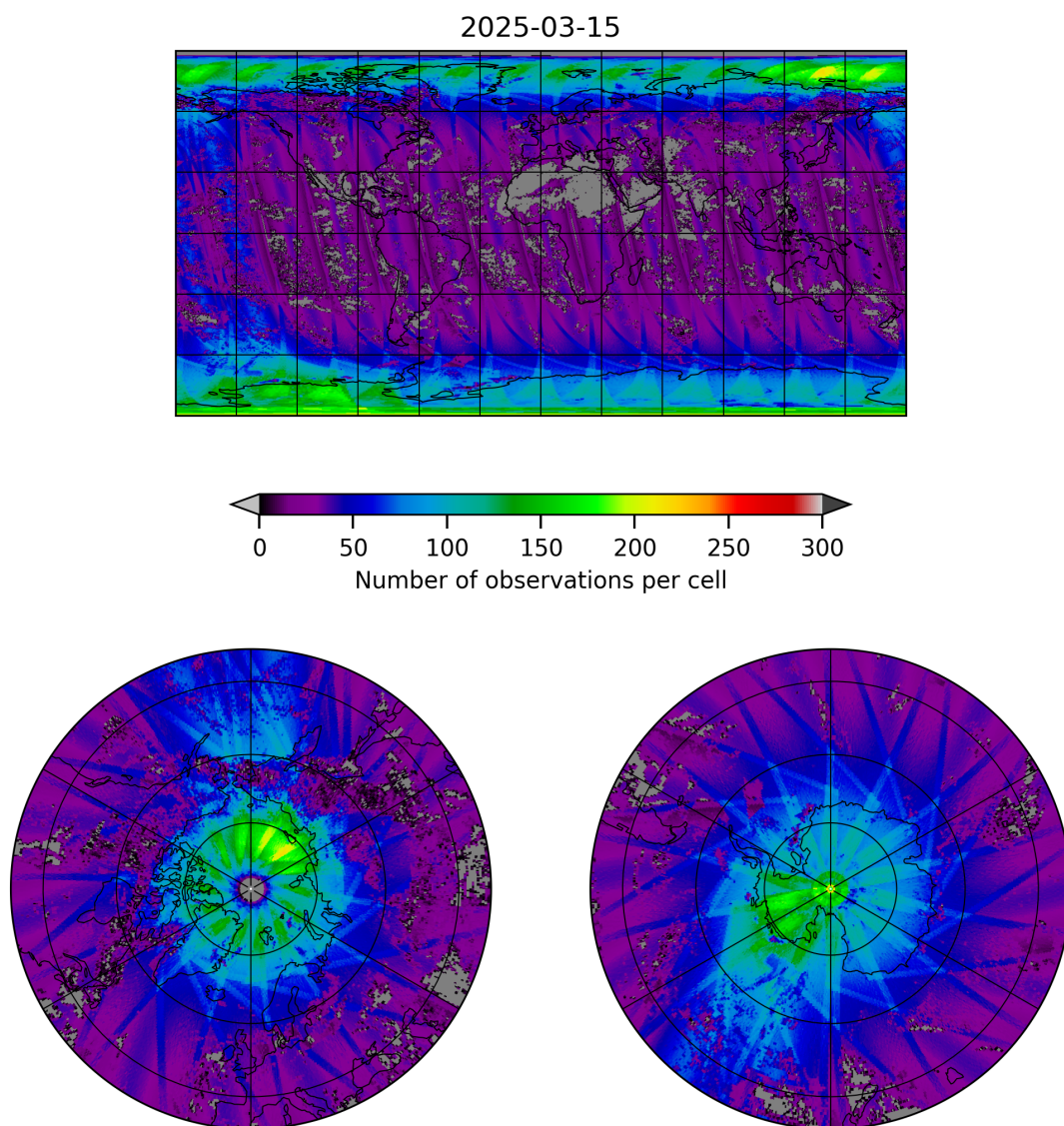
Figure 21: Map of the number of observations for 2025-03-14 to 2025-03-16
