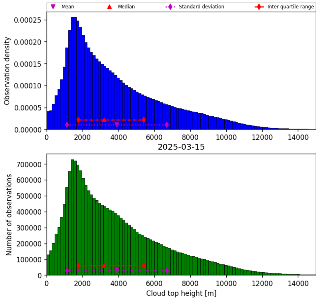
Figure 40: Histogram of “Cloud top height” for 2025-03-14 to 2025-03-16
