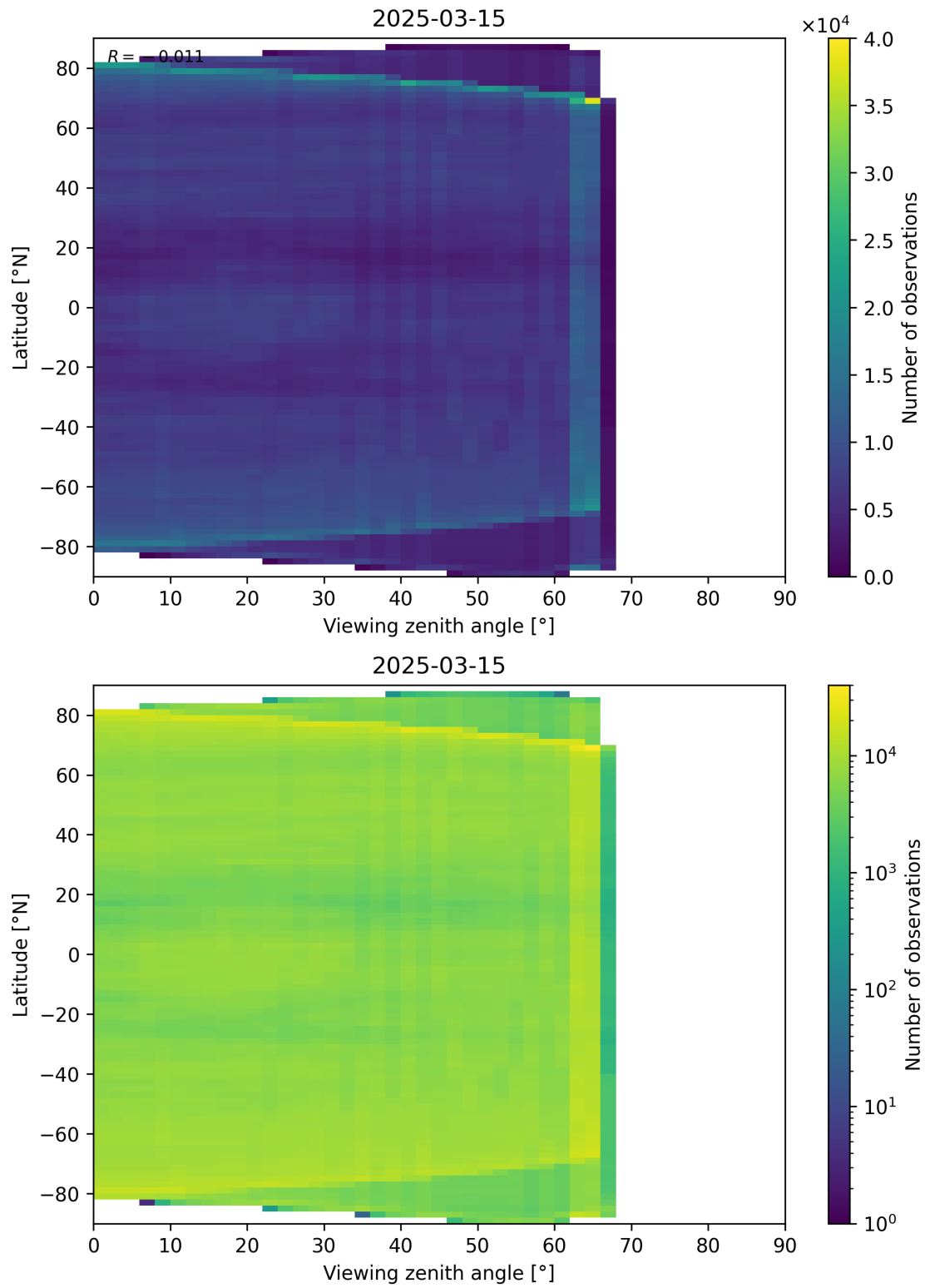
Figure 113: Scatter density plot of “Viewing zenith angle” against “Latitude” for 2025-03-14 to 2025-03-16.
