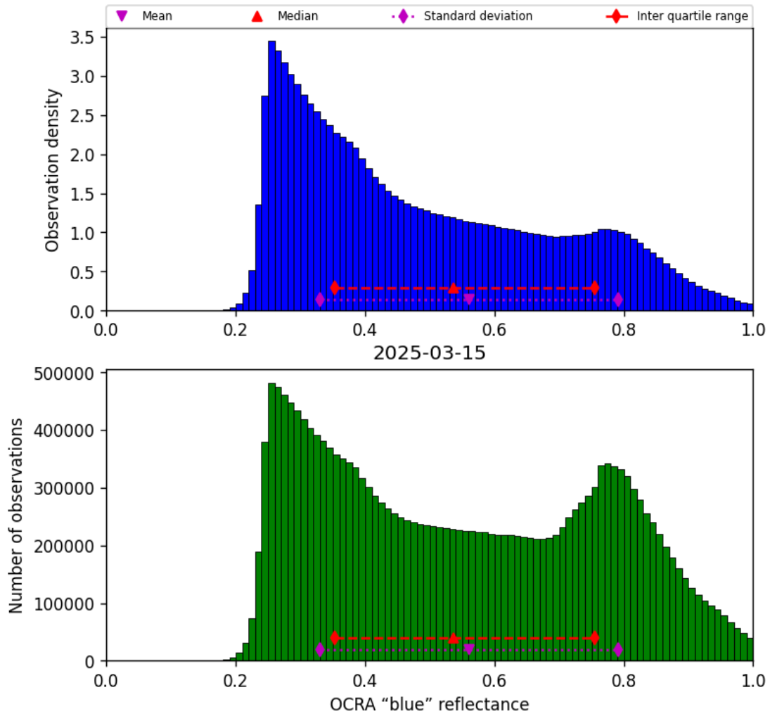
Figure 51: Histogram of “OCRA “blue” reflectance” for 2025-03-14 to 2025-03-16
