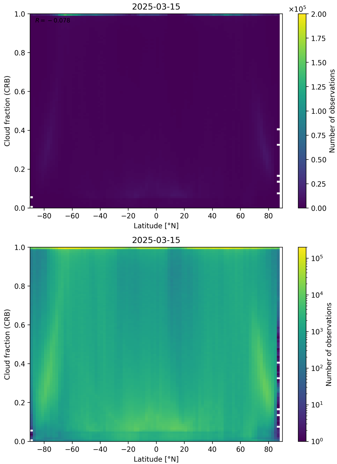
Figure 94: Scatter density plot of “Latitude” against “Cloud fraction (CRB)” for 2025-03-14 to 2025-03-16.
