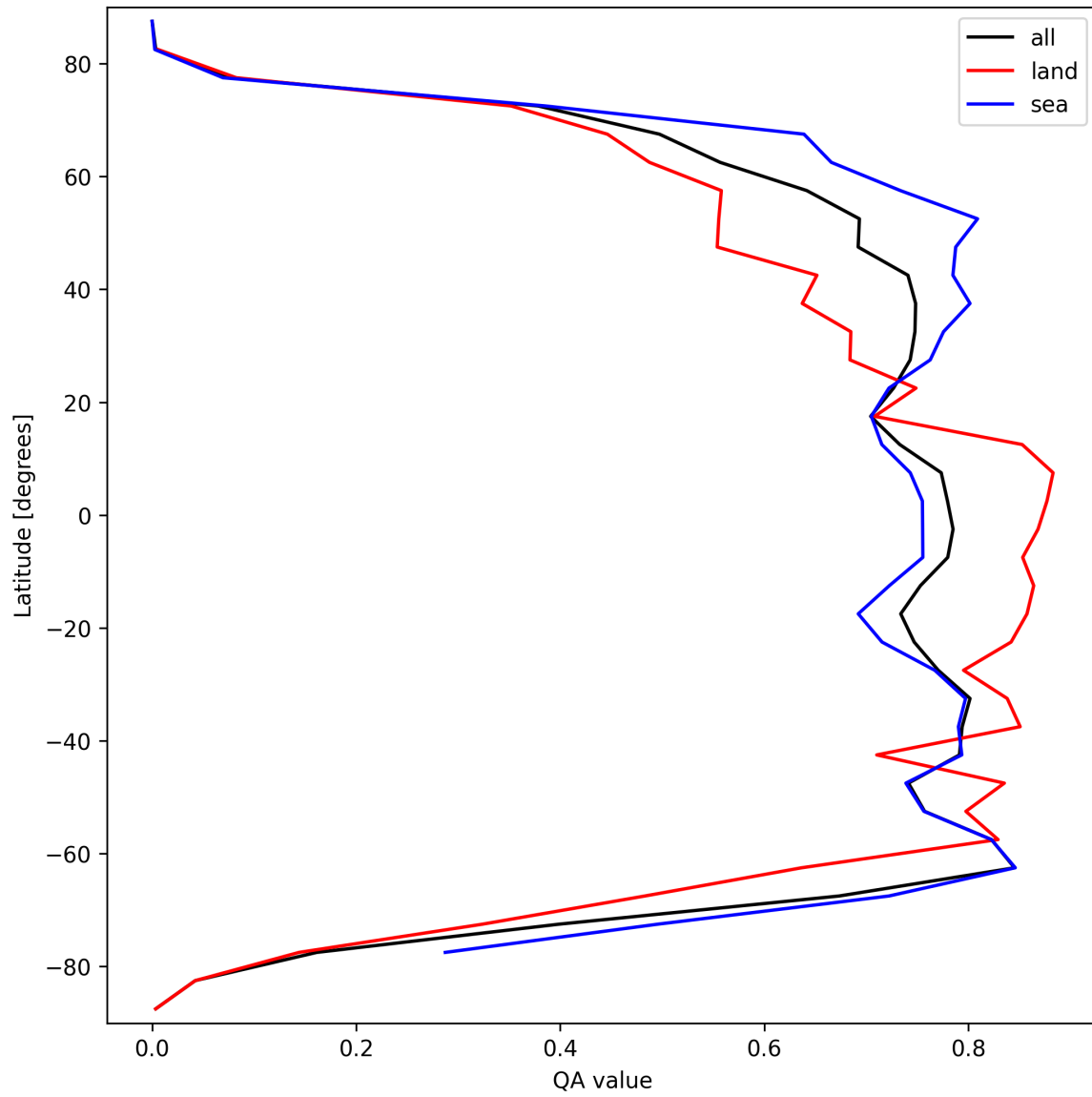
Figure 22: Zonal average of “QA value” for 2025-03-14 to 2025-03-16.
