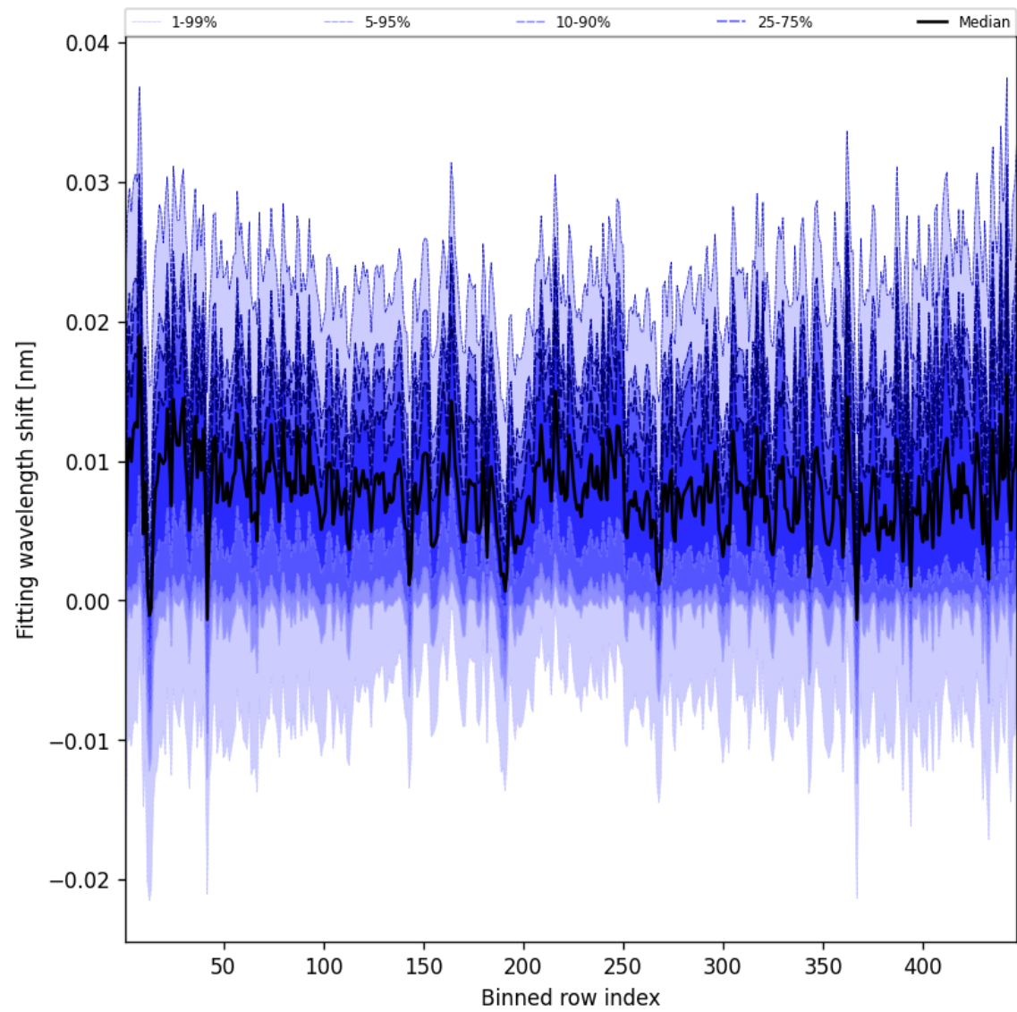
Figure 65: Along track statistics of “Fitting wavelength shift” for 2025-03-14 to 2025-03-16
