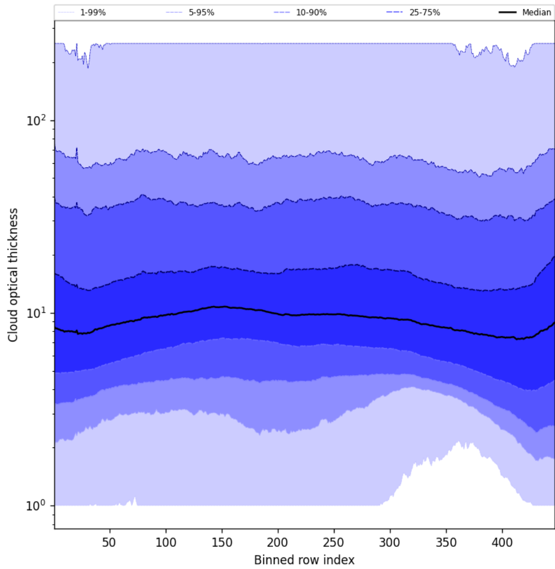
Figure 57: Along track statistics of “Cloud optical thickness” for 2025-03-14 to 2025-03-16
