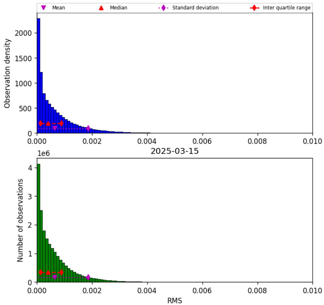
Figure 47: Histogram of “RMS” for 2025-03-14 to 2025-03-16
