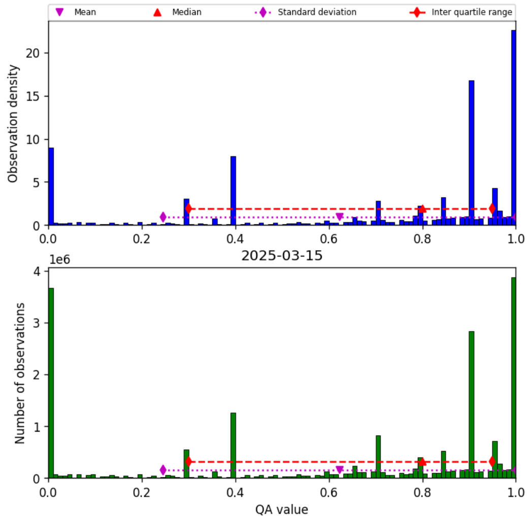
Figure 38: Histogram of “QA value” for 2025-03-14 to 2025-03-16
