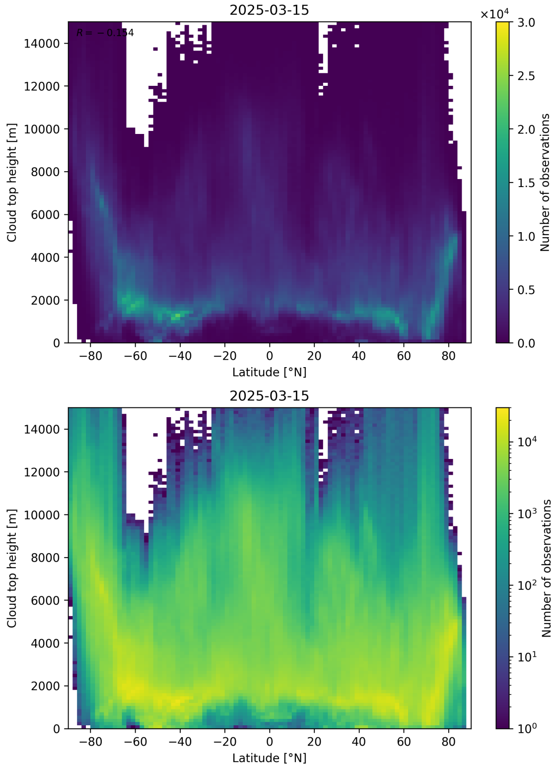
Figure 97: Scatter density plot of “Latitude” against “Cloud top height” for 2025-03-14 to 2025-03-16.
