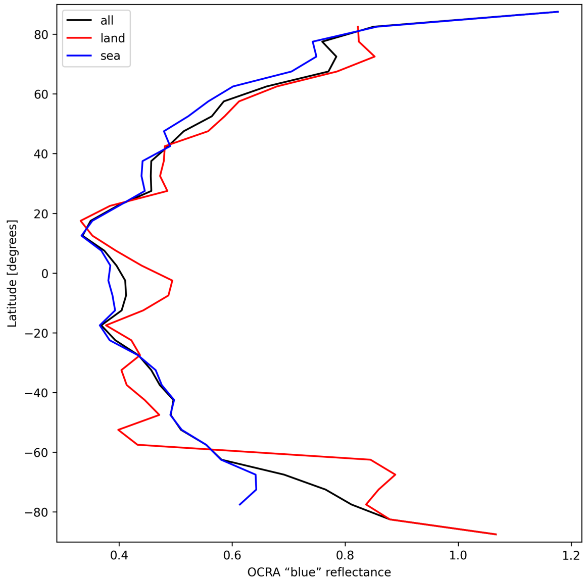
Figure 35: Zonal average of “OCRA “blue” reflectance” for 2025-03-14 to 2025-03-16.
