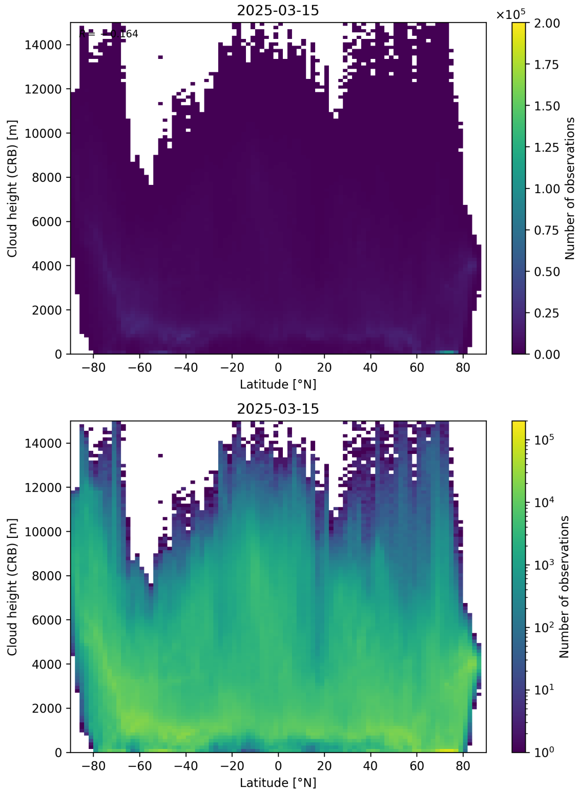
Figure 95: Scatter density plot of “Latitude” against “Cloud height (CRB)” for 2025-03-14 to 2025-03-16.
