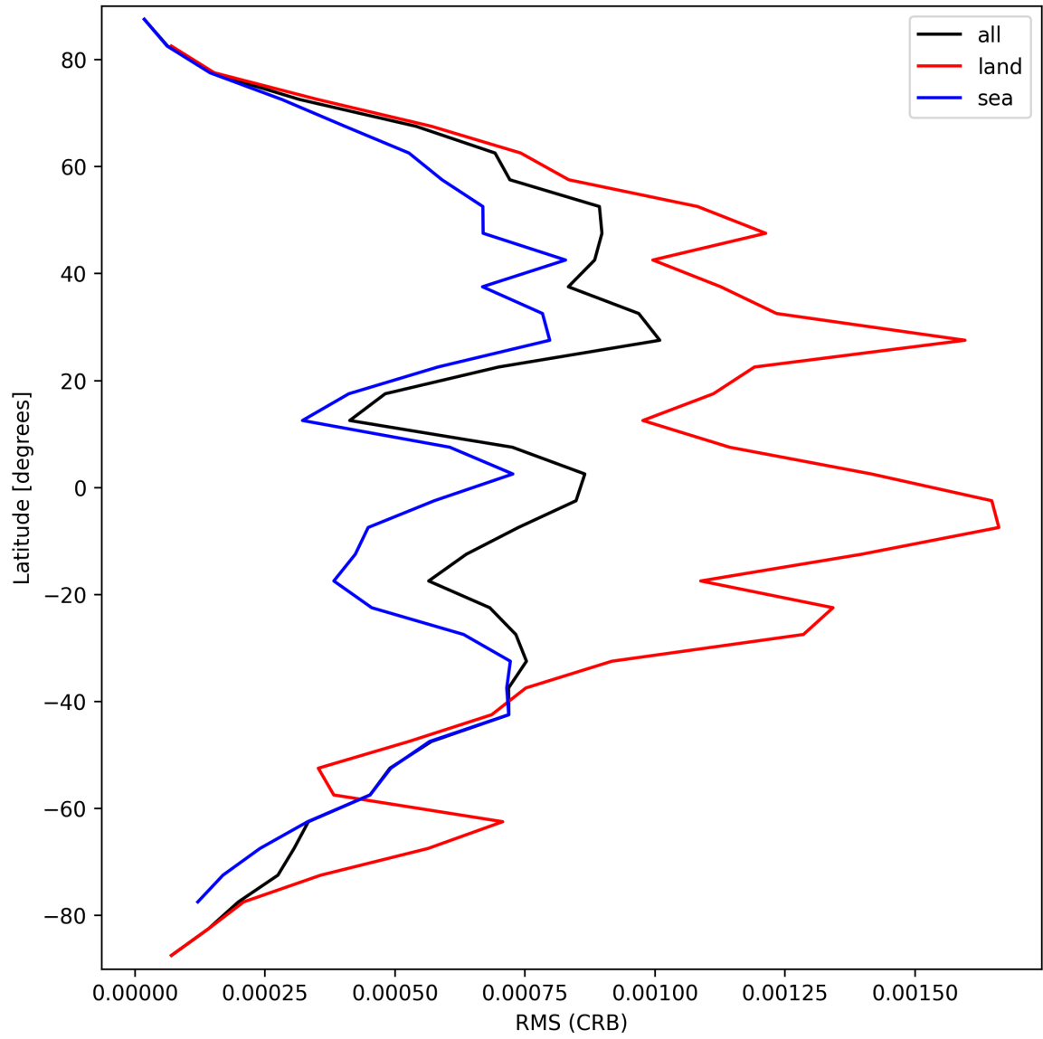
Figure 32: Zonal average of “RMS (CRB)” for 2025-03-14 to 2025-03-16.
