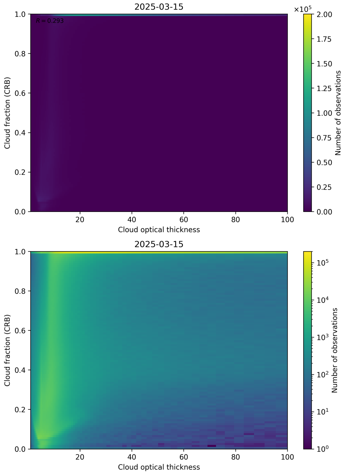
Figure 84: Scatter density plot of “Cloud optical thickness” against “Cloud fraction (CRB)” for 2025-03-14 to 2025-03-16.
