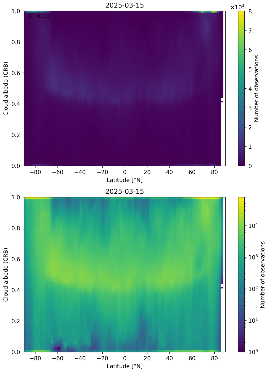
Figure 91: Scatter density plot of “Latitude” against “Cloud albedo (CRB)” for 2025-03-14 to 2025-03-16.
