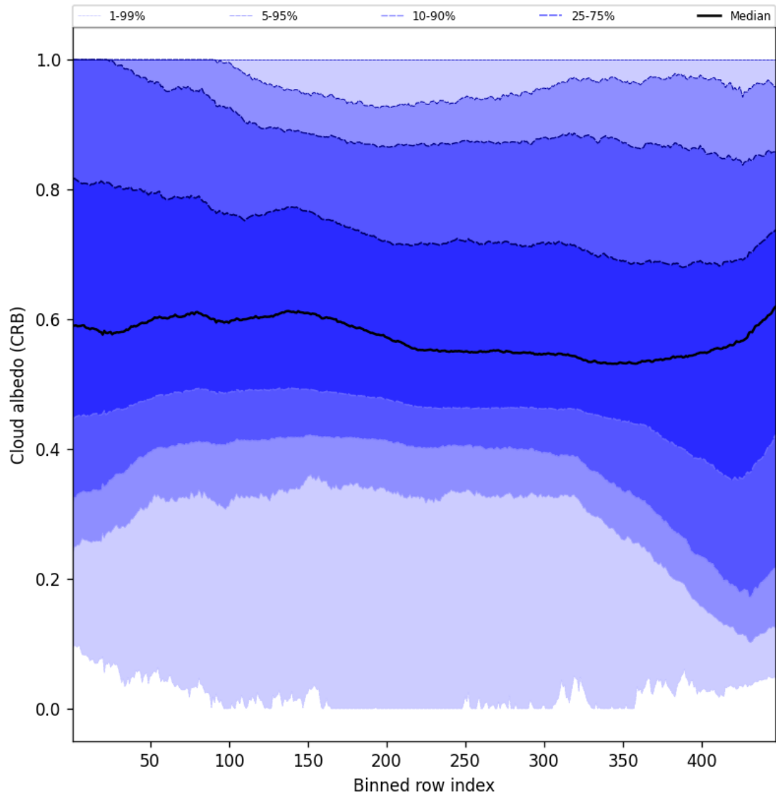
Figure 60: Along track statistics of “Cloud albedo (CRB)” for 2025-03-14 to 2025-03-16
