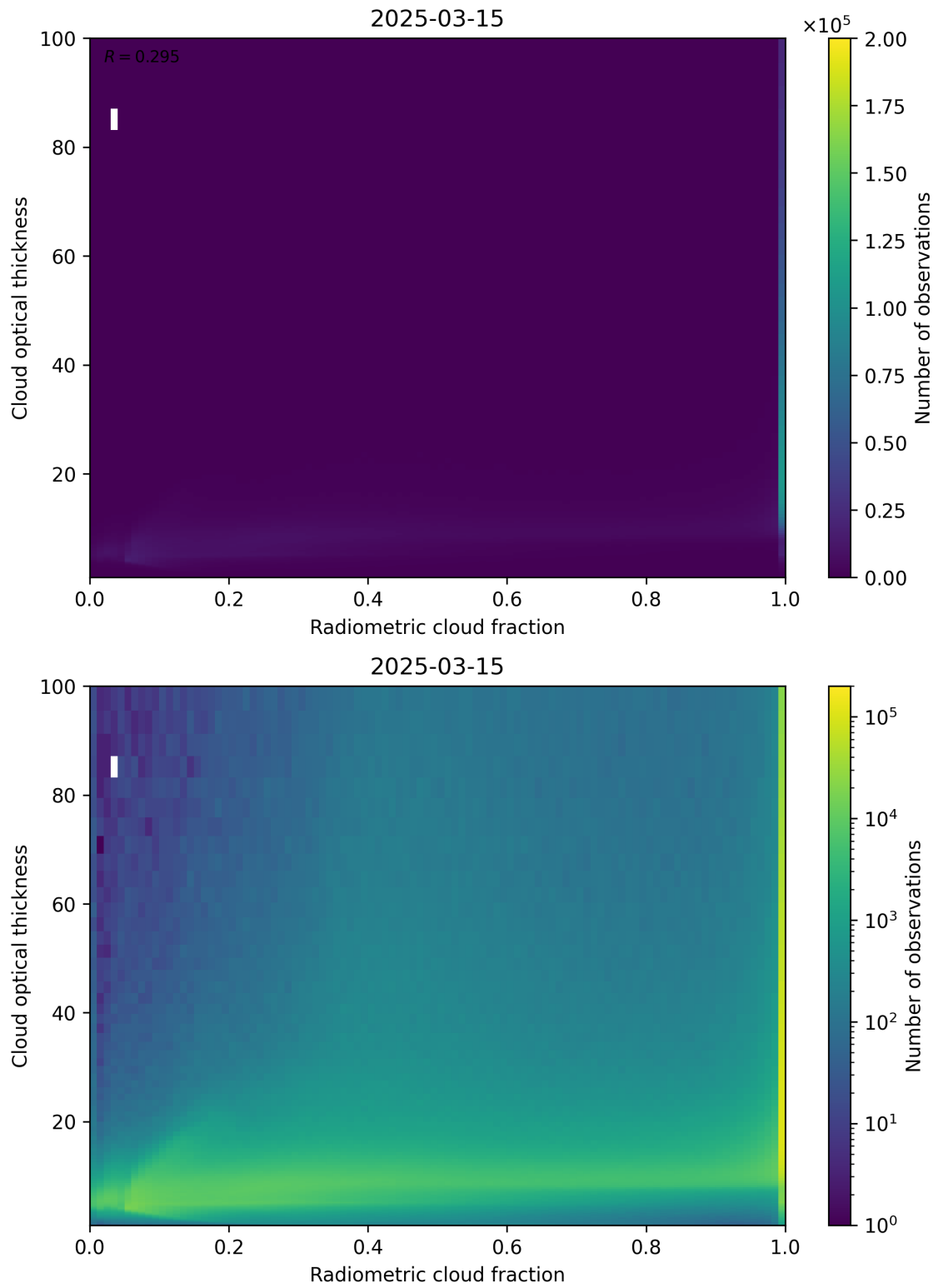
Figure 75: Scatter density plot of “Radiometric cloud fraction” against “Cloud optical thickness” for 2025-03-14 to 2025-03-16.
