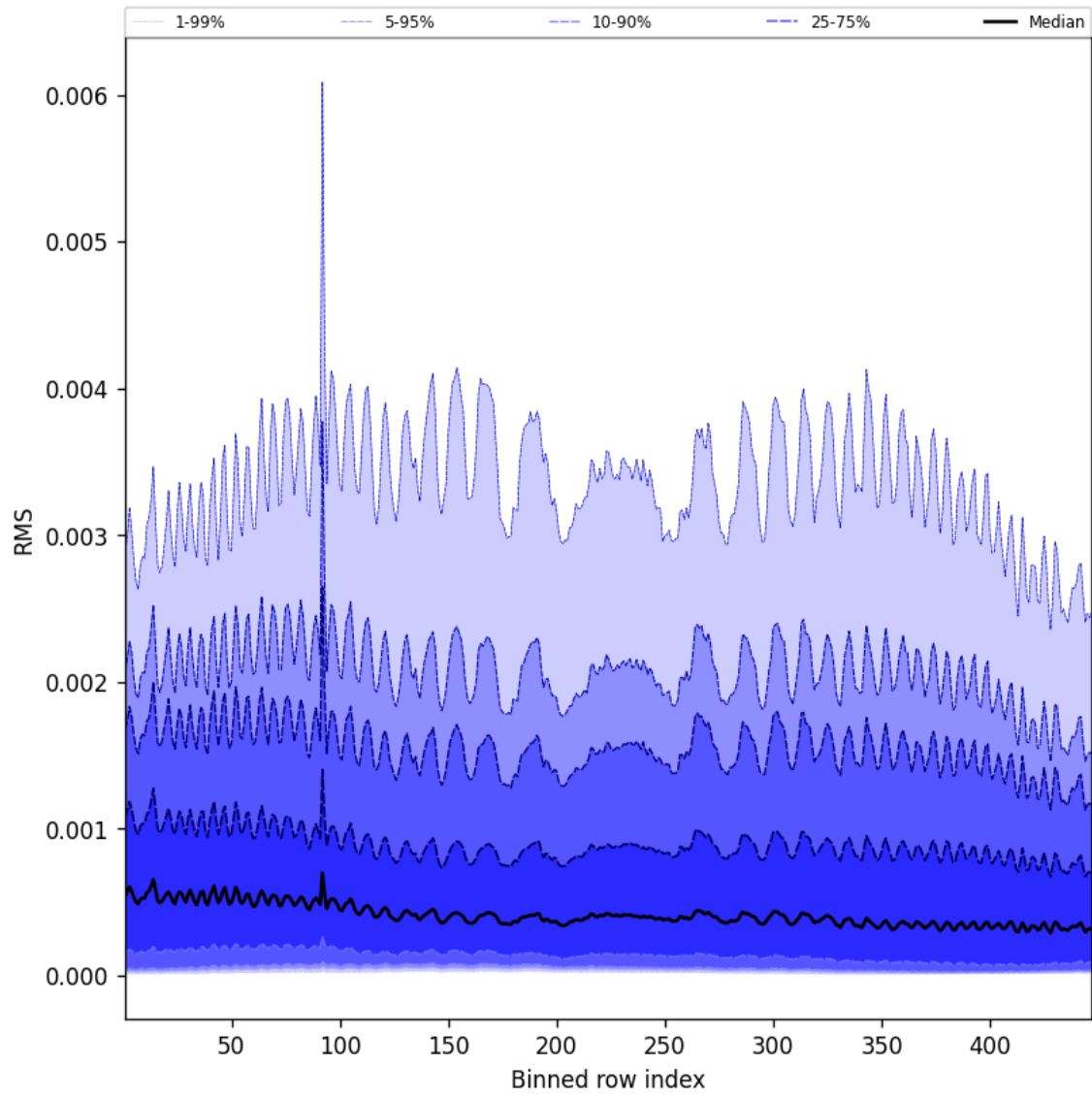
Figure 63: Along track statistics of “RMS” for 2025-03-14 to 2025-03-16
