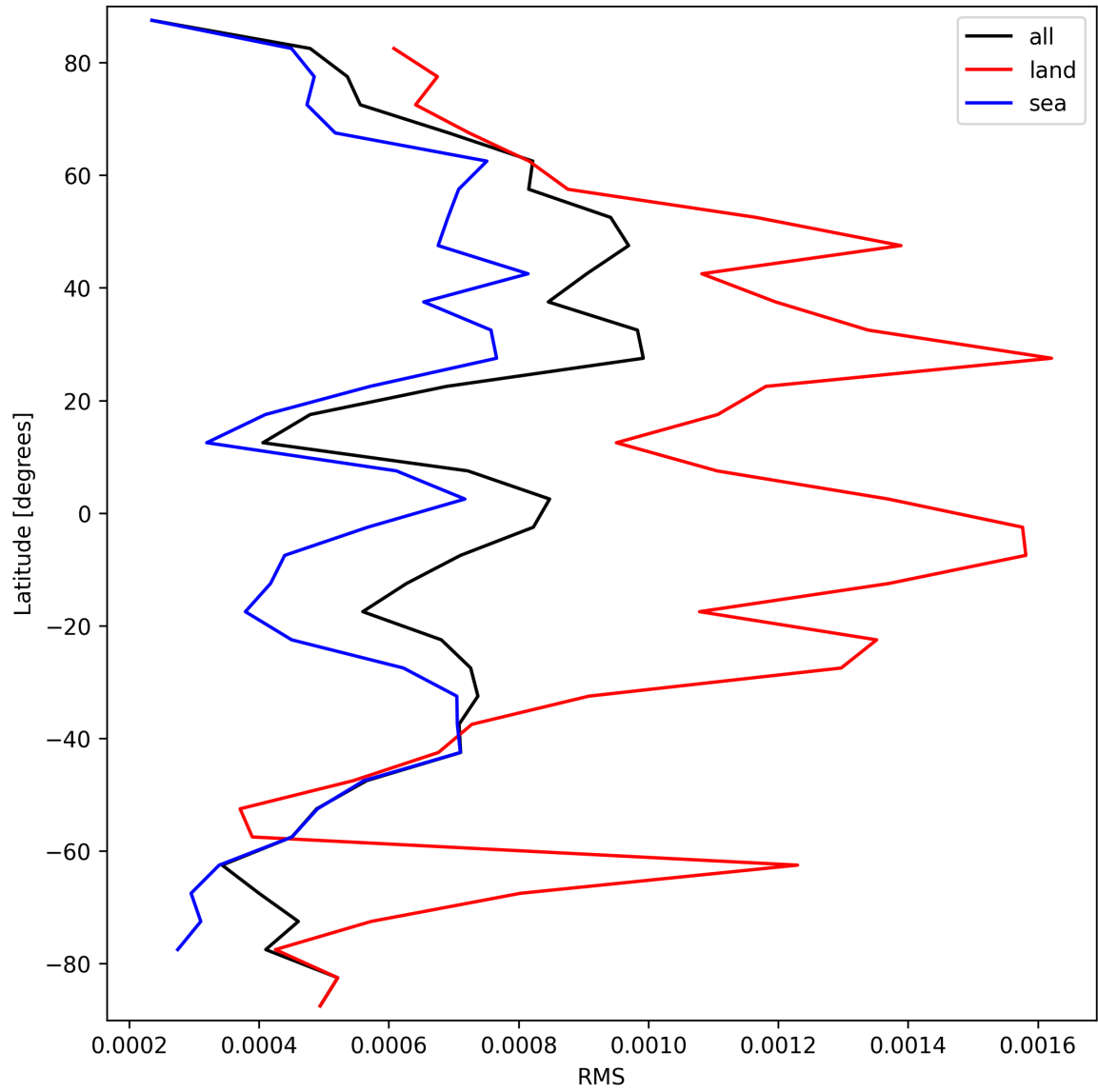
Figure 31: Zonal average of “RMS” for 2025-03-14 to 2025-03-16.
