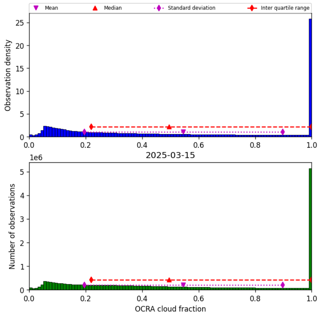
Figure 50: Histogram of “OCRA cloud fraction” for 2025-03-14 to 2025-03-16
