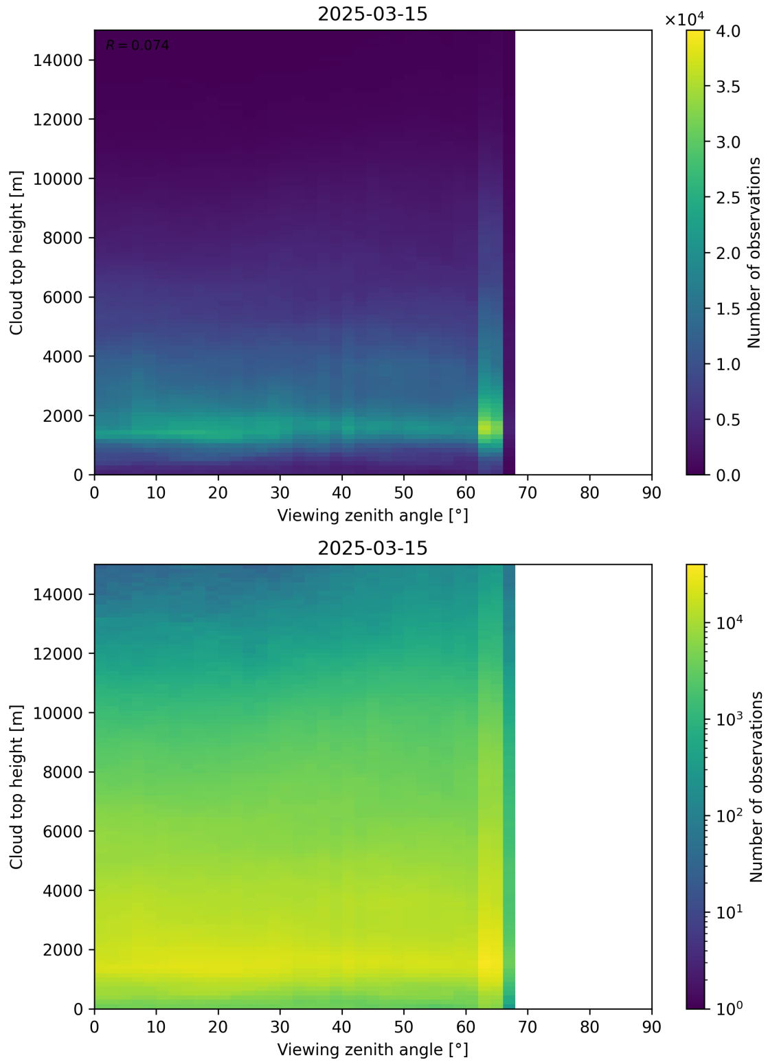
Figure 112: Scatter density plot of “Viewing zenith angle” against “Cloud top height” for 2025-03-14 to 2025-03-16.
