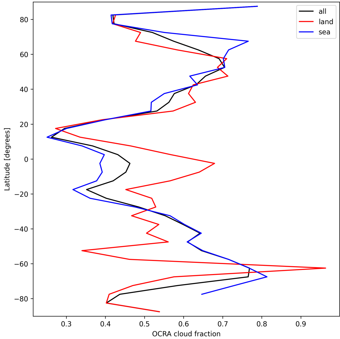
Figure 34: Zonal average of “OCRA cloud fraction” for 2025-03-14 to 2025-03-16.
