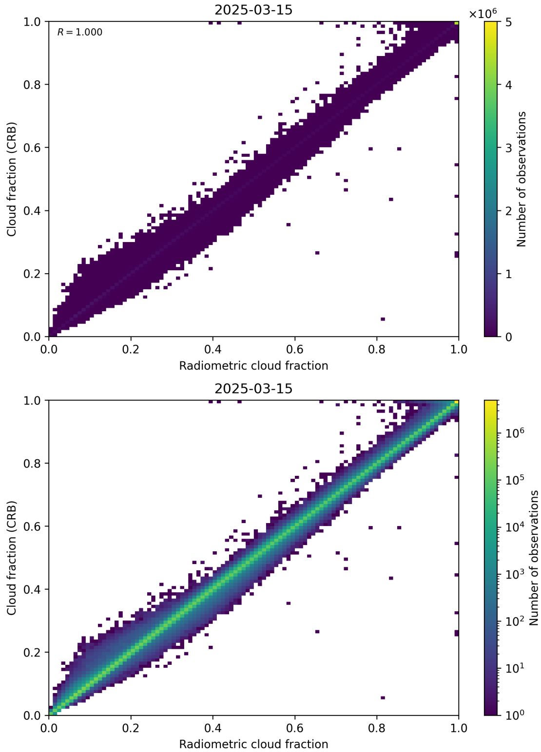
Figure 73: Scatter density plot of “Radiometric cloud fraction” against “Cloud fraction (CRB)” for 2025-03-14 to 2025-03-16.
