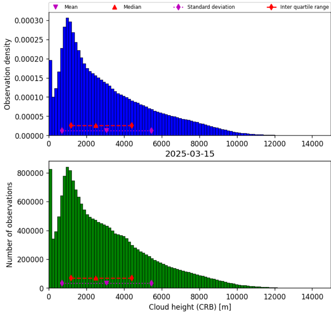
Figure 43: Histogram of “Cloud height (CRB)” for 2025-03-14 to 2025-03-16
