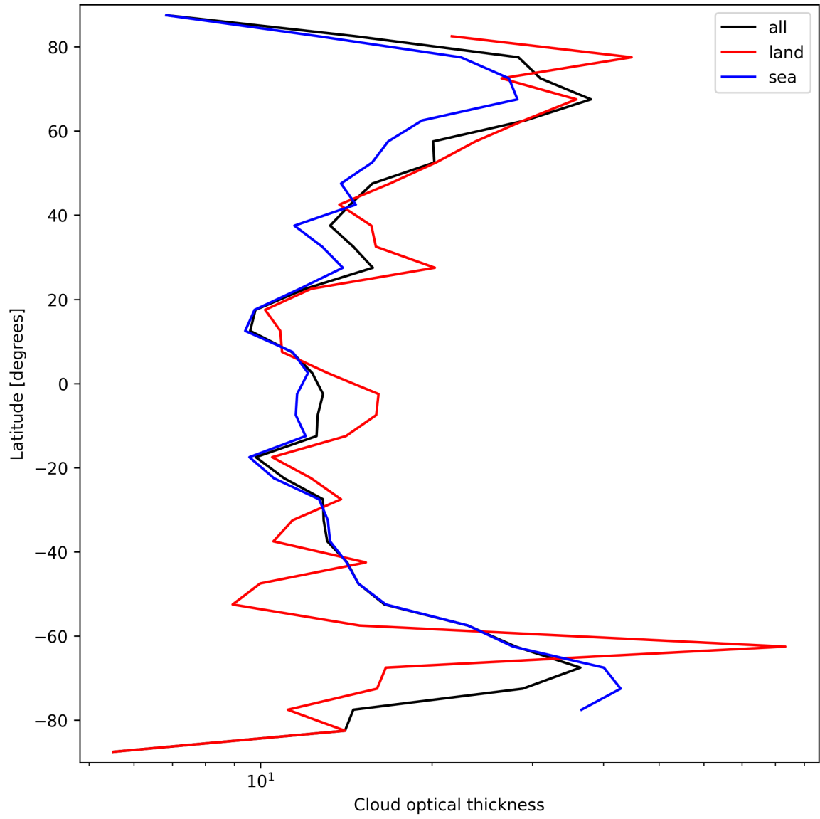
Figure 25: Zonal average of “Cloud optical thickness” for 2025-03-14 to 2025-03-16.
