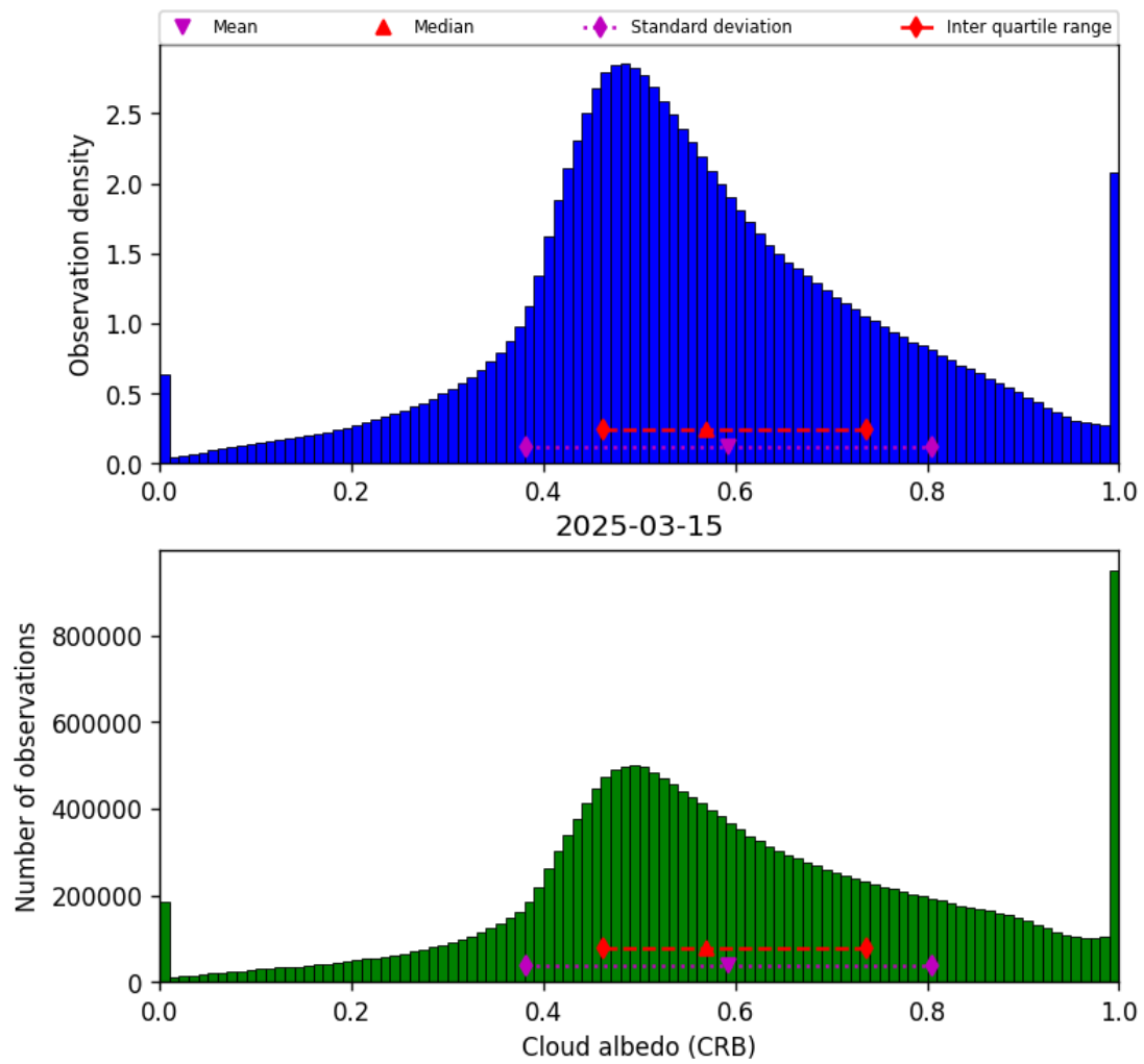
Figure 44: Histogram of “Cloud albedo (CRB)” for 2025-03-14 to 2025-03-16
