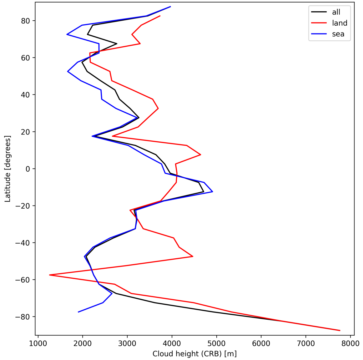
Figure 27: Zonal average of “Cloud height (CRB)” for 2025-03-14 to 2025-03-16.
