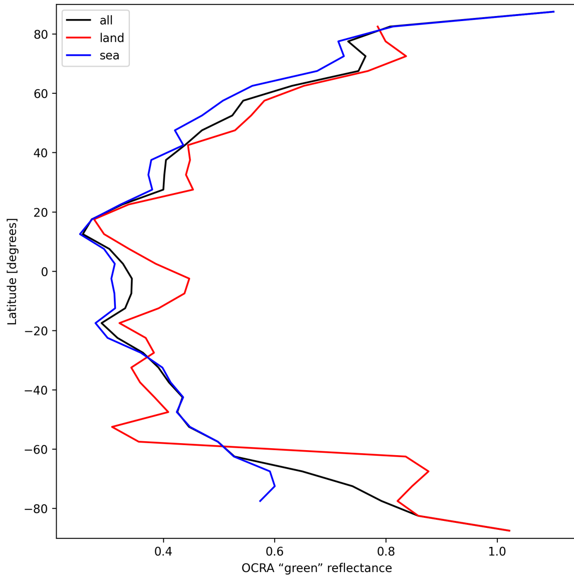
Figure 36: Zonal average of “OCRA “green” reflectance” for 2025-03-14 to 2025-03-16.
