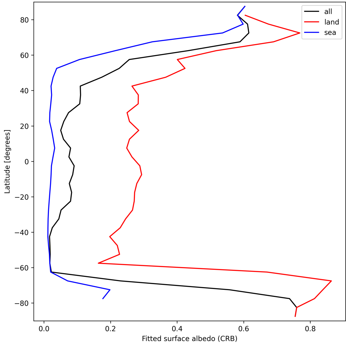
Figure 30: Zonal average of “Fitted surface albedo (CRB)” for 2025-03-14 to 2025-03-16.
