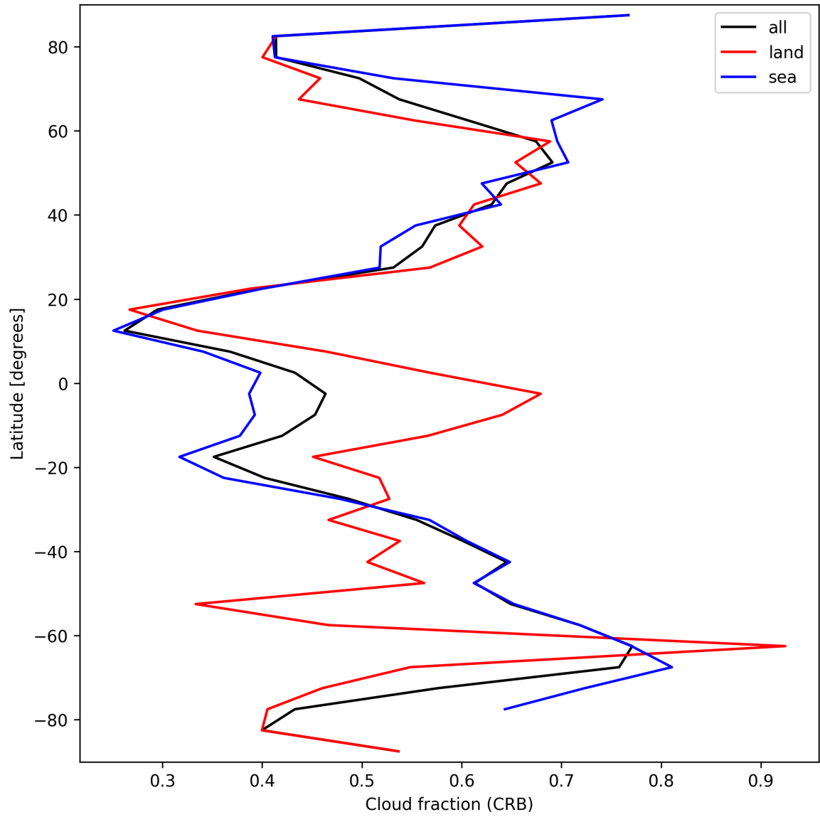
Figure 26: Zonal average of “Cloud fraction (CRB)” for 2025-03-14 to 2025-03-16.
