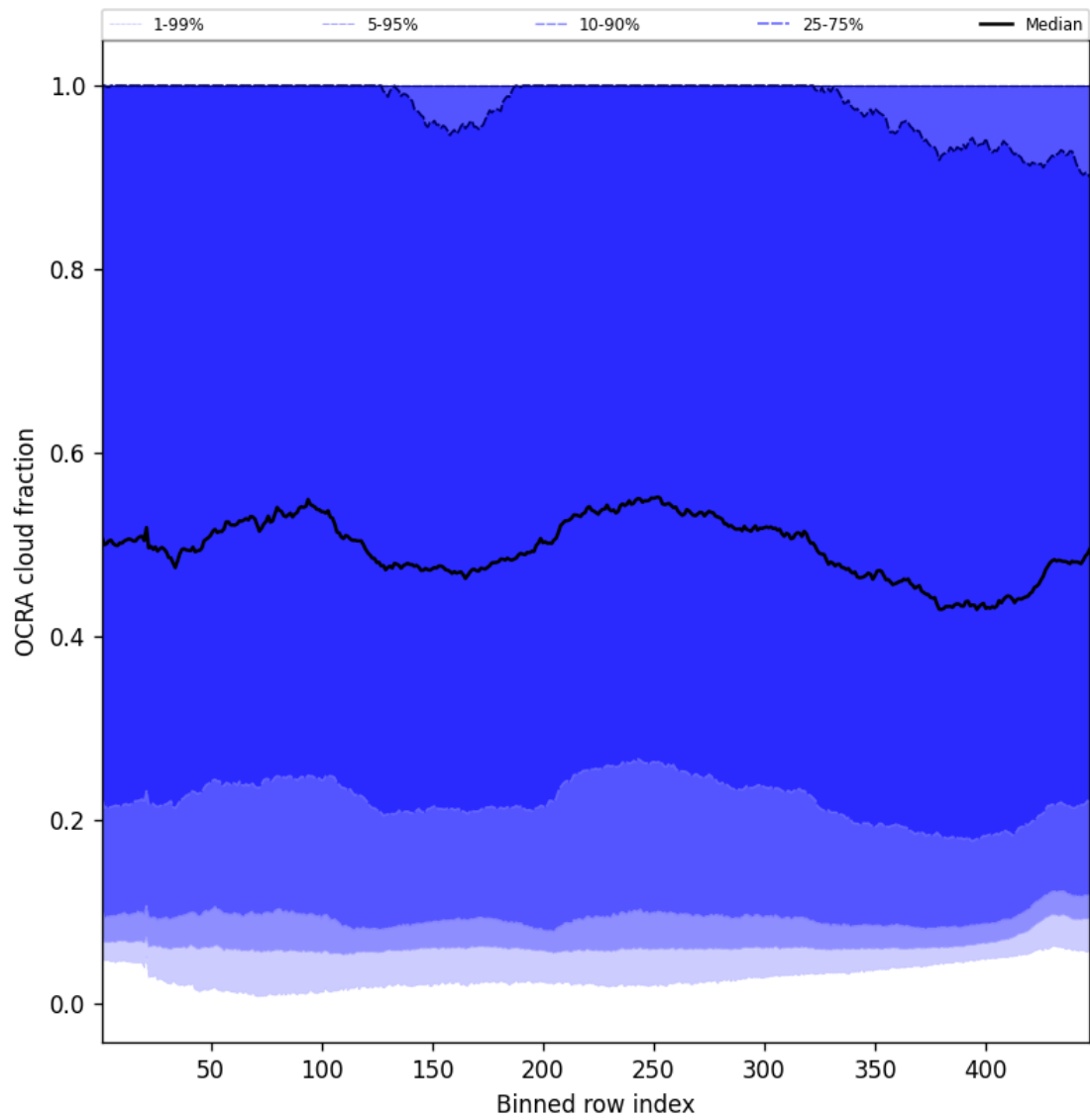
Figure 66: Along track statistics of “OCRA cloud fraction” for 2025-03-14 to 2025-03-16
