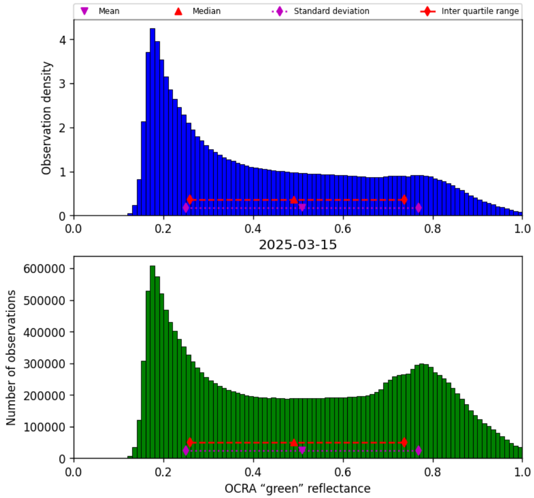
Figure 52: Histogram of “OCRA “green” reflectance” for 2025-03-14 to 2025-03-16
