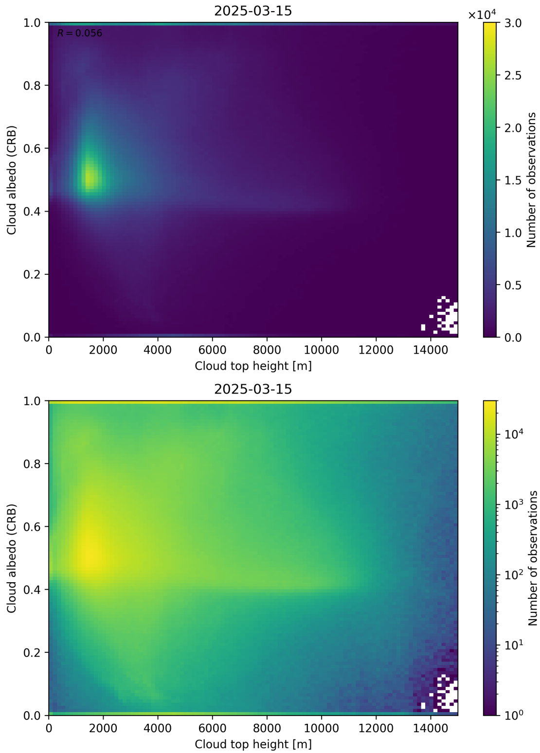
Figure 86: Scatter density plot of “Cloud top height” against “Cloud albedo (CRB)” for 2025-03-14 to 2025-03-16.
