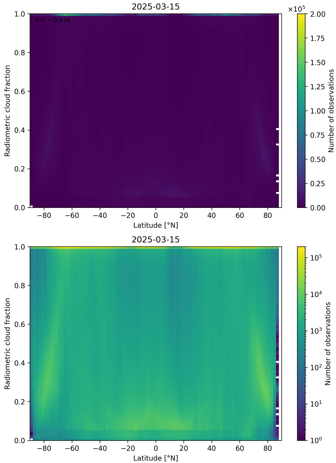
Figure 92: Scatter density plot of “Latitude” against “Radiometric cloud fraction” for 2025-03-14 to 2025-03-16.
