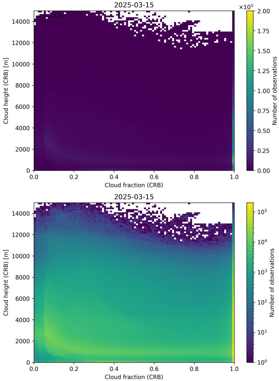
Figure 79: Scatter density plot of “Cloud fraction (CRB)” against “Cloud height (CRB)” for 2025-03-14 to 2025-03-16.
