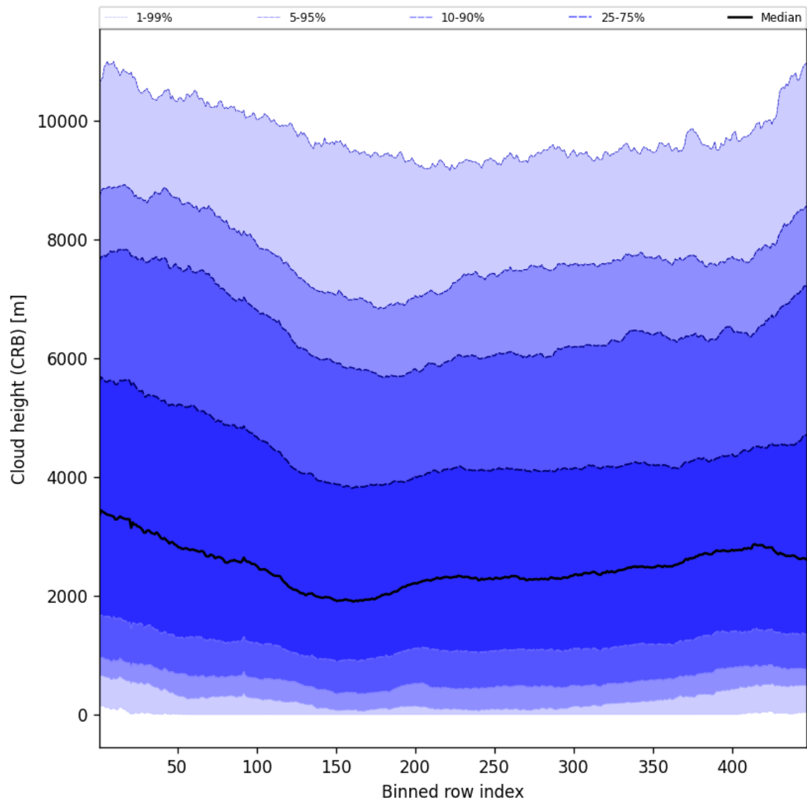
Figure 59: Along track statistics of “Cloud height (CRB)” for 2025-03-14 to 2025-03-16
