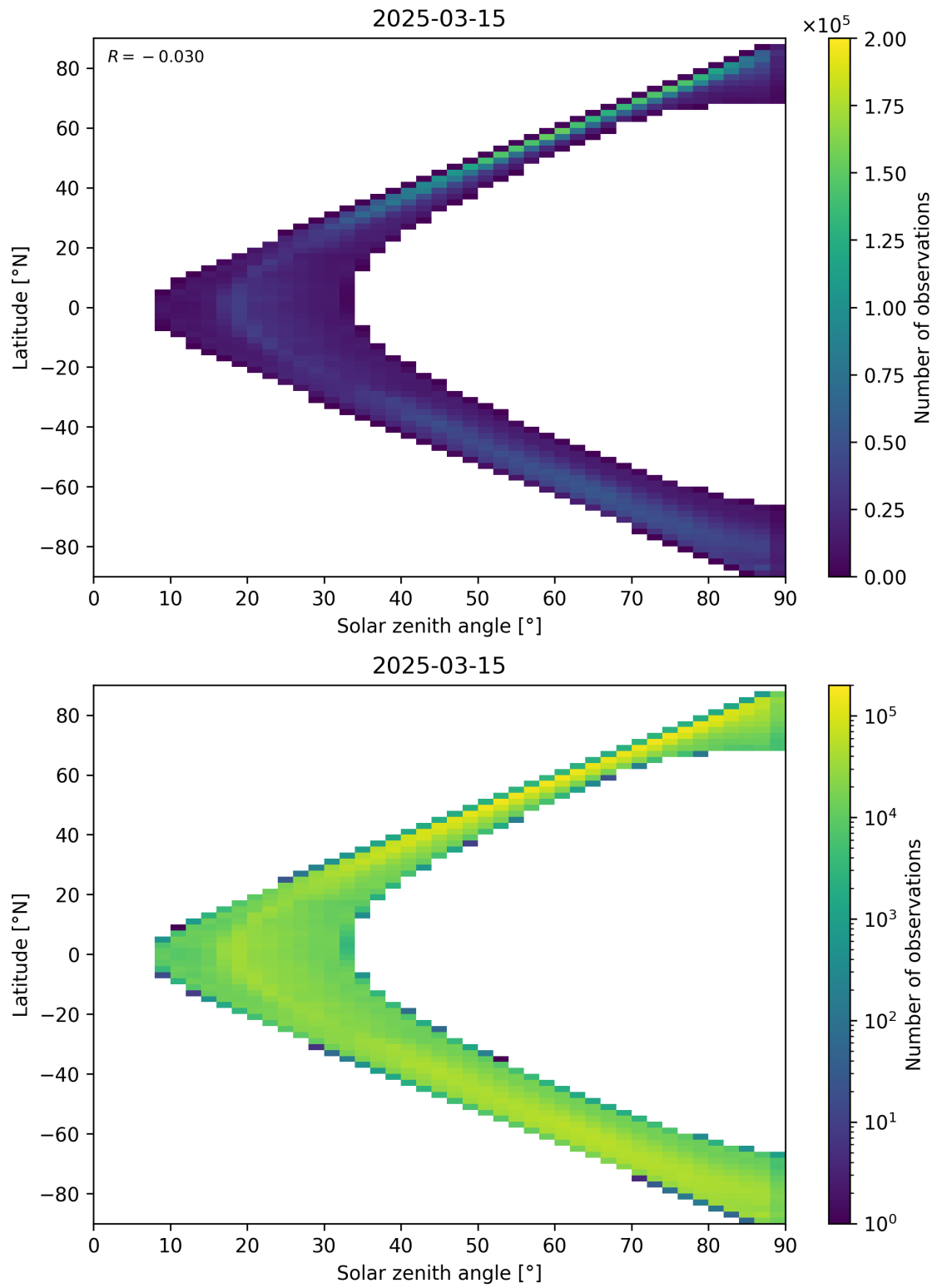
Figure 105: Scatter density plot of “Solar zenith angle” against “Latitude” for 2025-03-14 to 2025-03-16.
