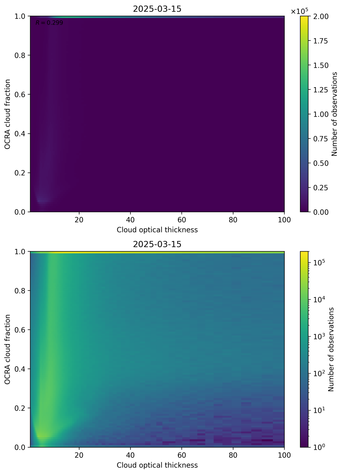
Figure 83: Scatter density plot of “Cloud optical thickness” against “OCRA cloud fraction” for 2025-03-14 to 2025-03-16.
