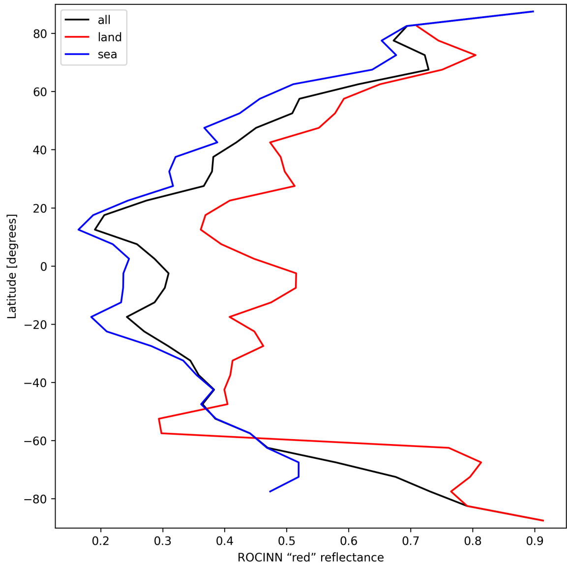
Figure 37: Zonal average of “ROCINN “red” reflectance” for 2025-03-14 to 2025-03-16.
