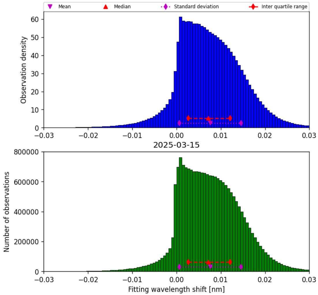
Figure 49: Histogram of “Fitting wavelength shift” for 2025-03-14 to 2025-03-16
