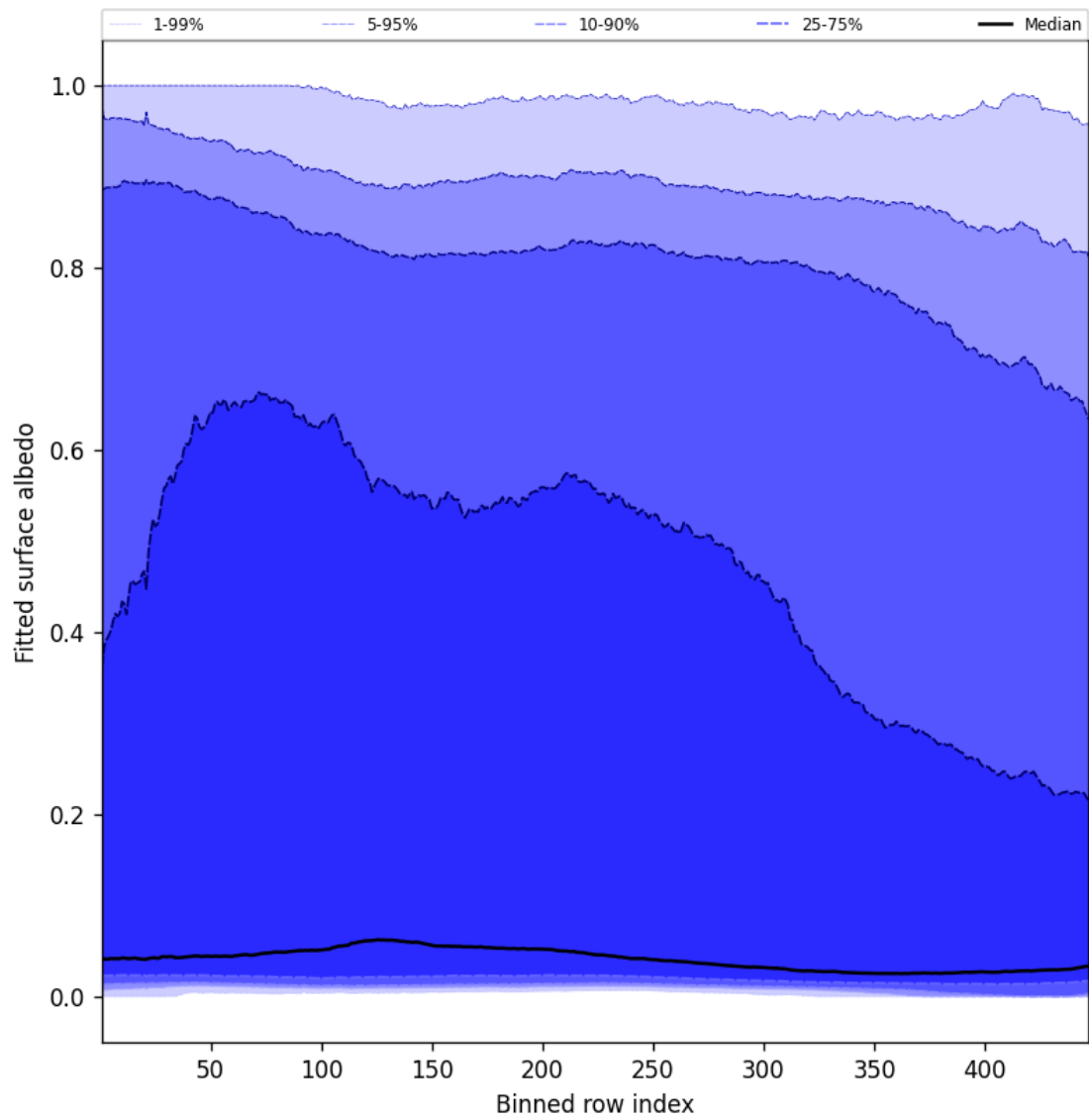
Figure 61: Along track statistics of “Fitted surface albedo” for 2025-03-14 to 2025-03-16
