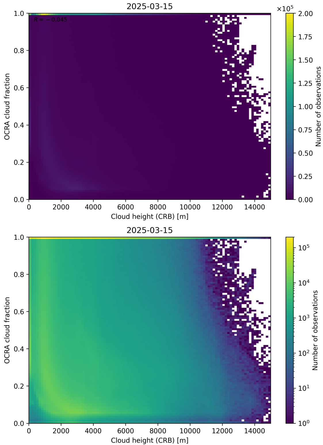
Figure 81: Scatter density plot of “Cloud height (CRB)” against “OCRA cloud fraction” for 2025-03-14 to 2025-03-16.
