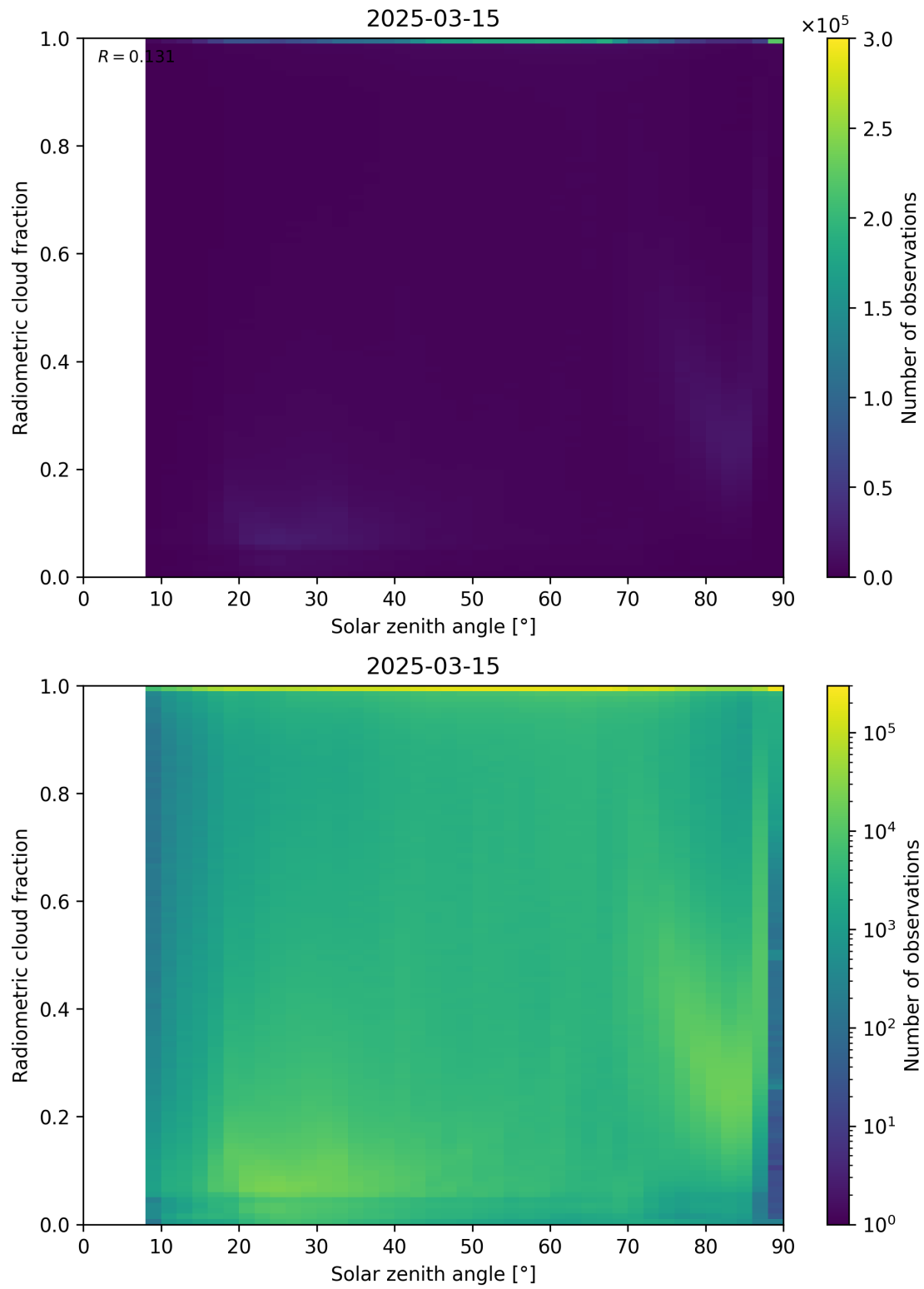
Figure 99: Scatter density plot of “Solar zenith angle” against “Radiometric cloud fraction” for 2025-03-14 to 2025-03-16.
