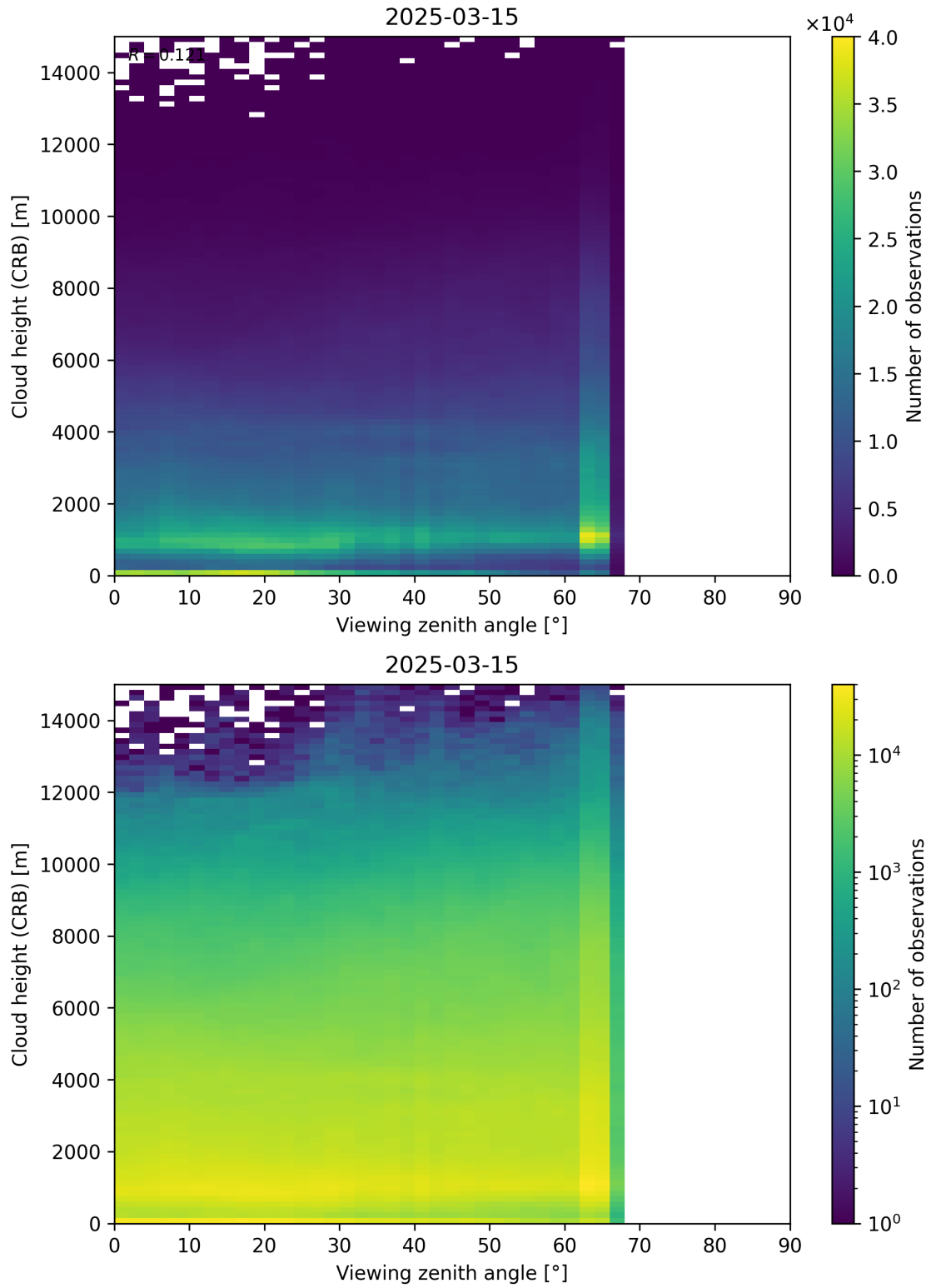
Figure 110: Scatter density plot of “Viewing zenith angle” against “Cloud height (CRB)” for 2025-03-14 to 2025-03-16.
