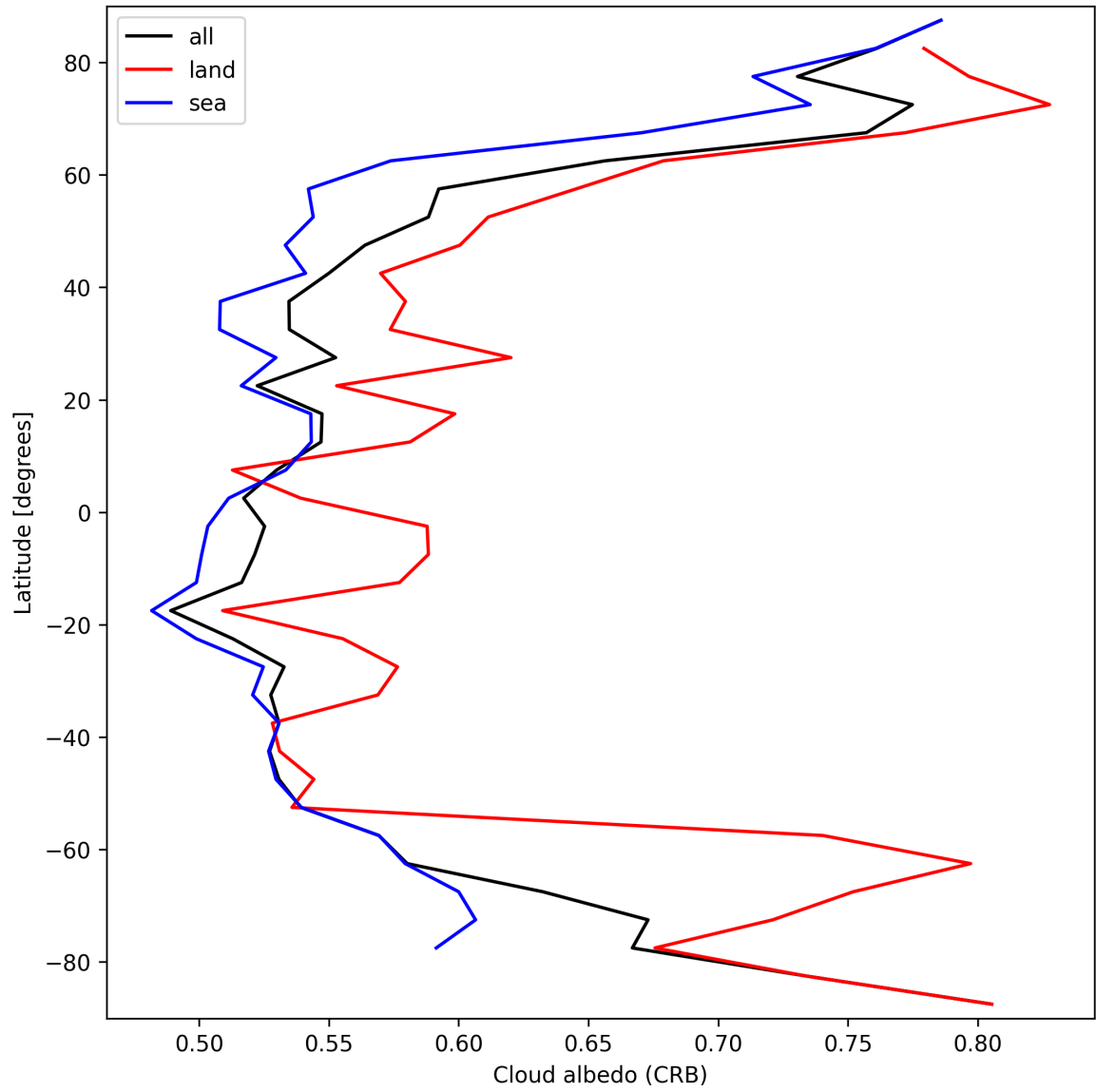
Figure 28: Zonal average of “Cloud albedo (CRB)” for 2025-03-14 to 2025-03-16.
