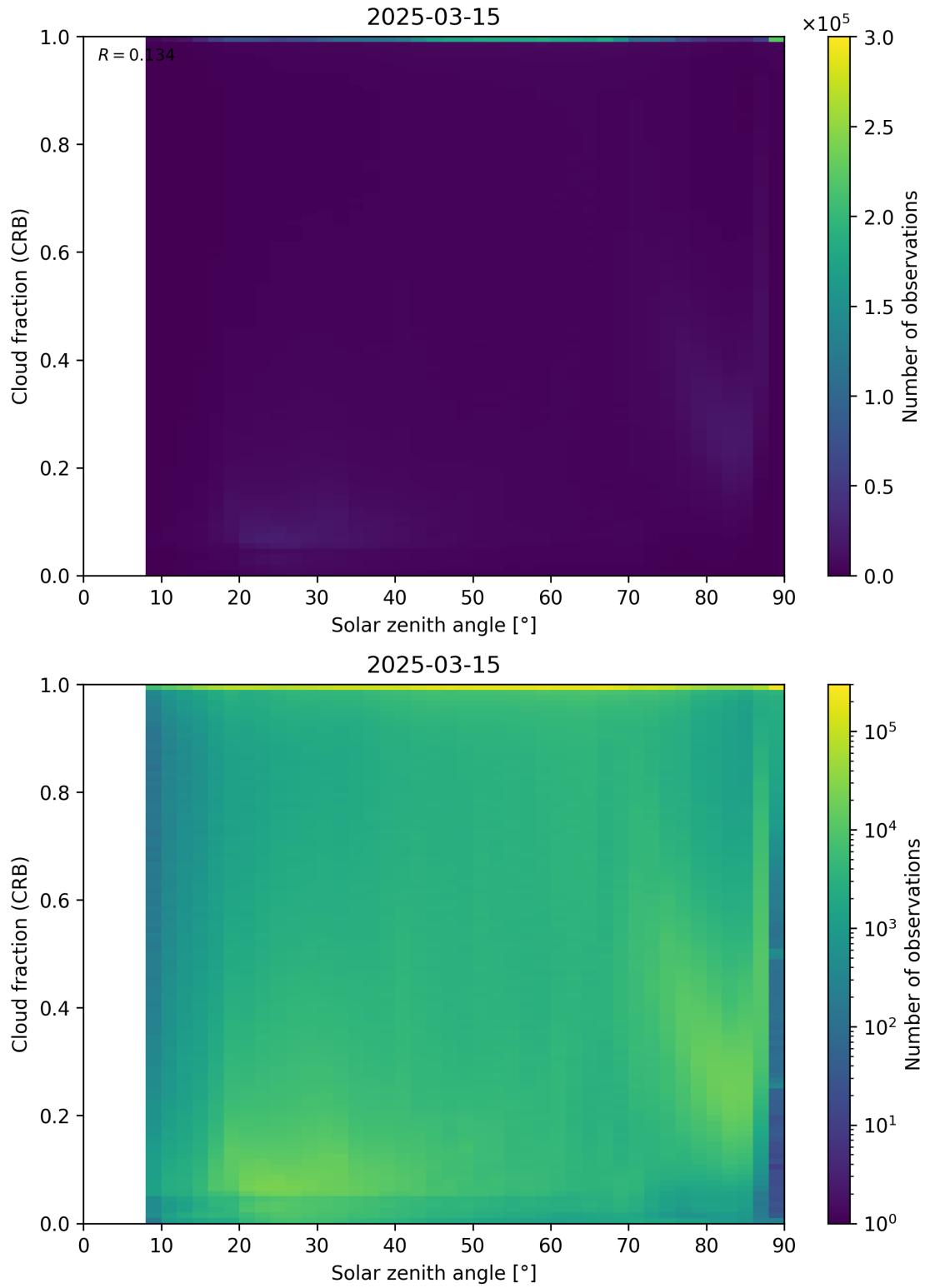
Figure 101: Scatter density plot of “Solar zenith angle” against “Cloud fraction (CRB)” for 2025-03-14 to 2025-03-16.
