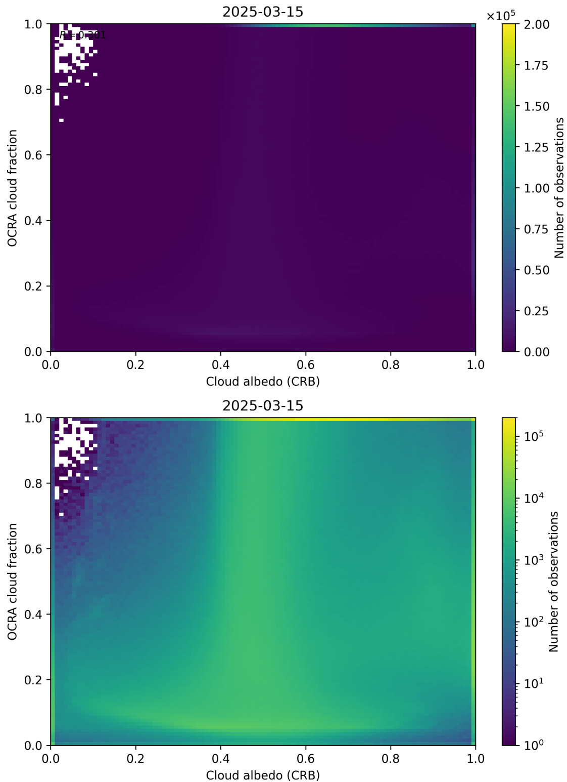
Figure 70: Scatter density plot of “Cloud albedo (CRB)” against “OCRA cloud fraction” for 2025-03-14 to 2025-03-16.
