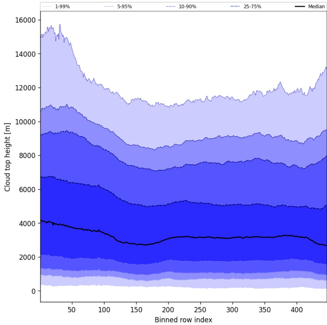
Figure 56: Along track statistics of “Cloud top height” for 2025-03-14 to 2025-03-16
