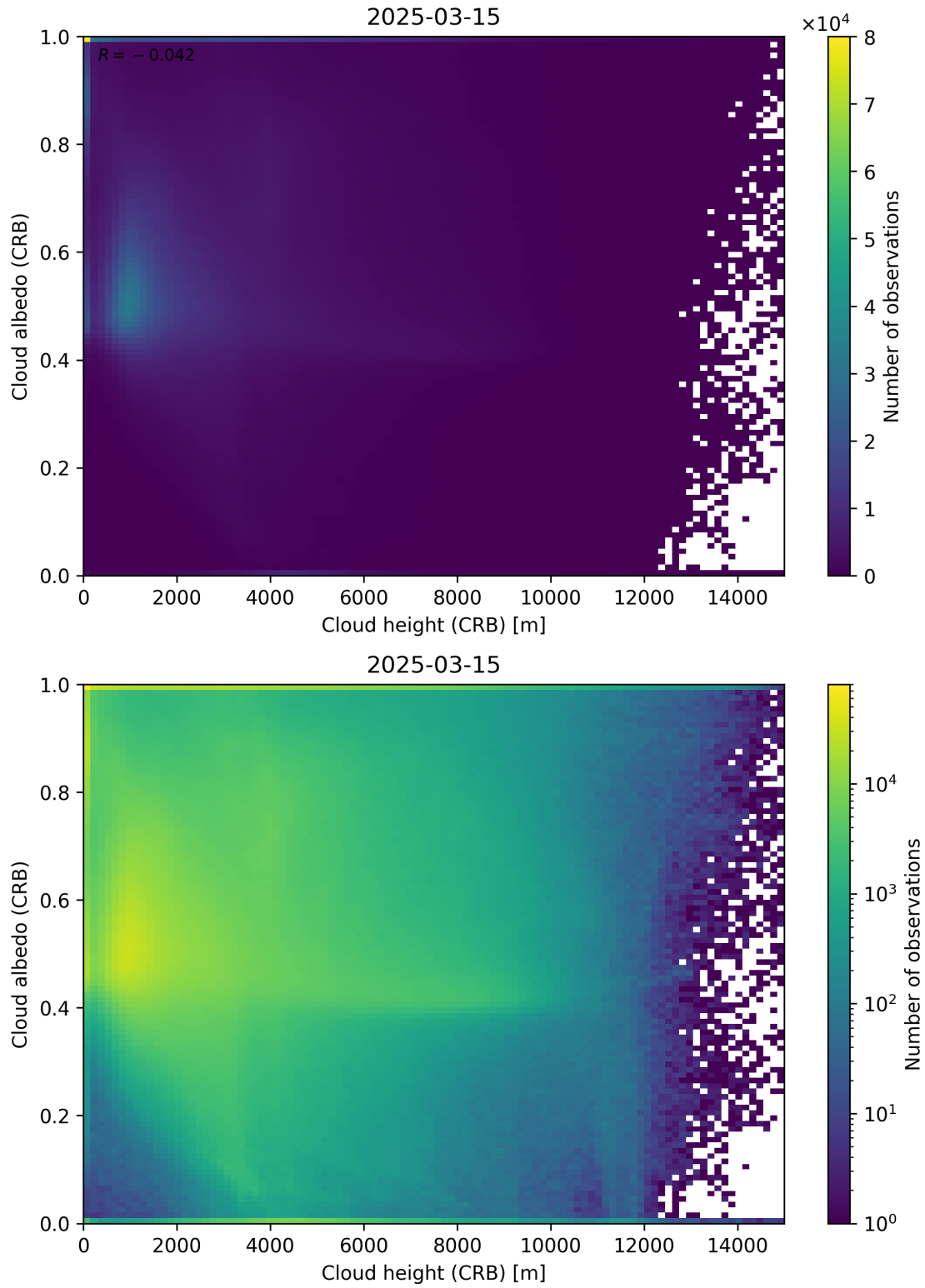
Figure 80: Scatter density plot of “Cloud height (CRB)” against “Cloud albedo (CRB)” for 2025-03-14 to 2025-03-16.
