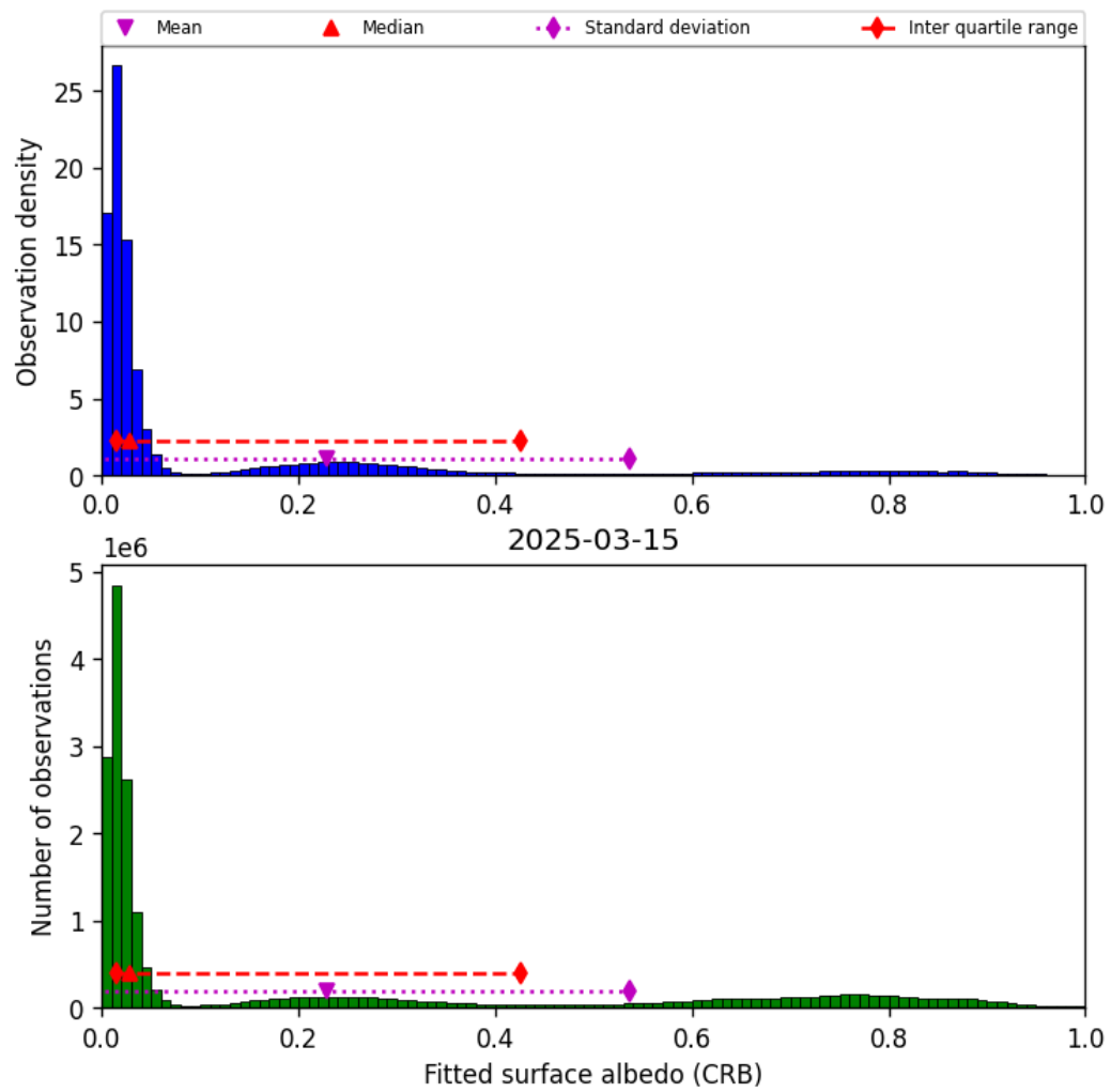
Figure 46: Histogram of “Fitted surface albedo (CRB)” for 2025-03-14 to 2025-03-16
