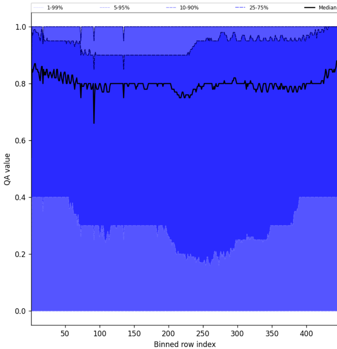
Figure 54: Along track statistics of “QA value” for 2025-03-14 to 2025-03-16
