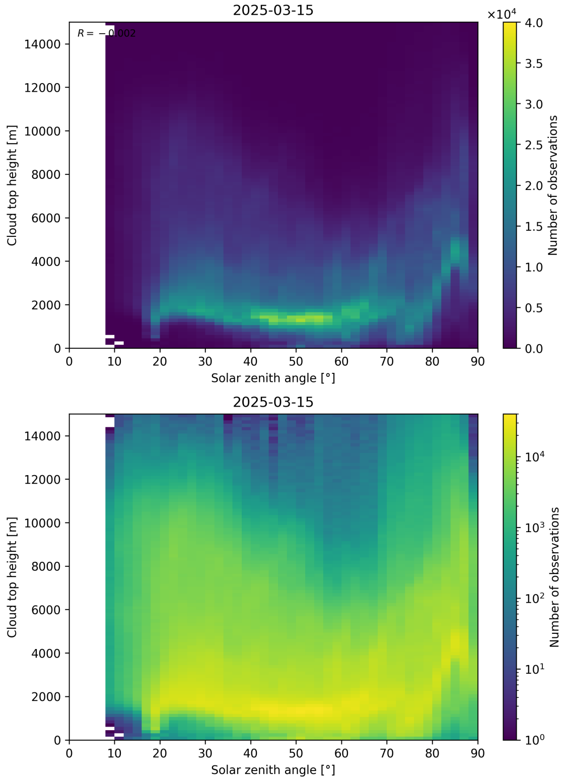
Figure 104: Scatter density plot of “Solar zenith angle” against “Cloud top height” for 2025-03-14 to 2025-03-16.
