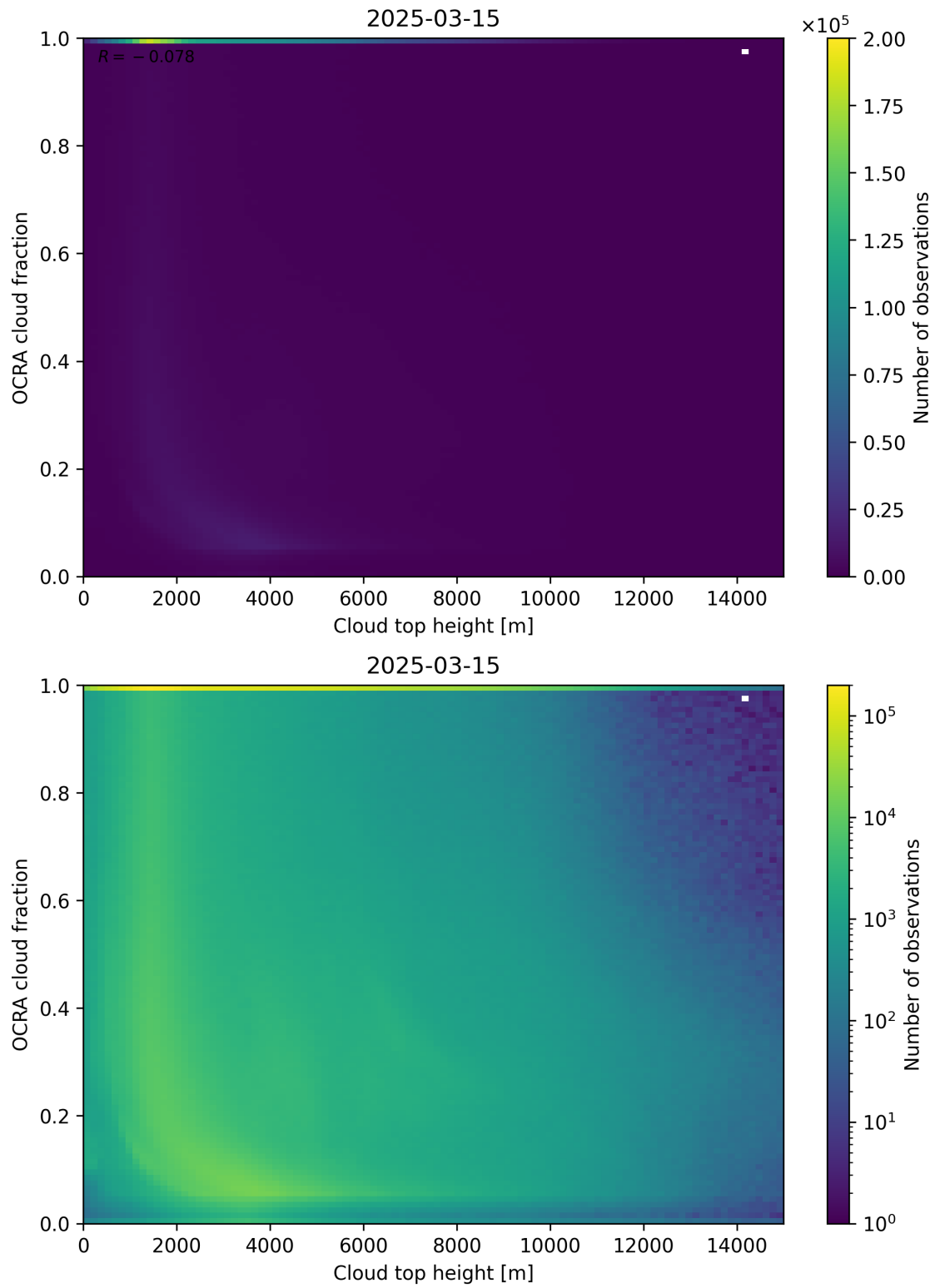
Figure 87: Scatter density plot of “Cloud top height” against “OCRA cloud fraction” for 2025-03-14 to 2025-03-16.
