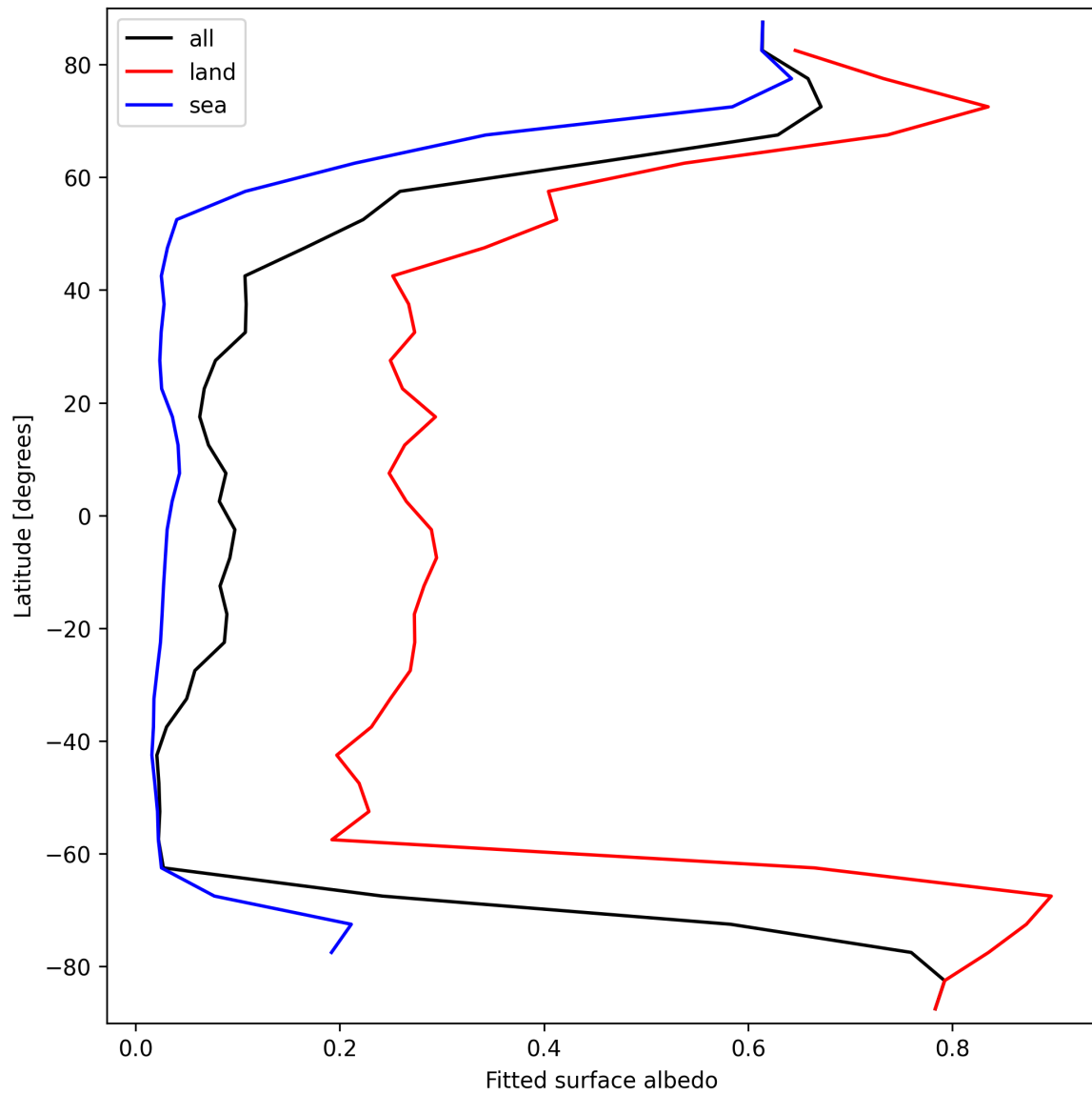
Figure 29: Zonal average of “Fitted surface albedo” for 2025-03-14 to 2025-03-16.
