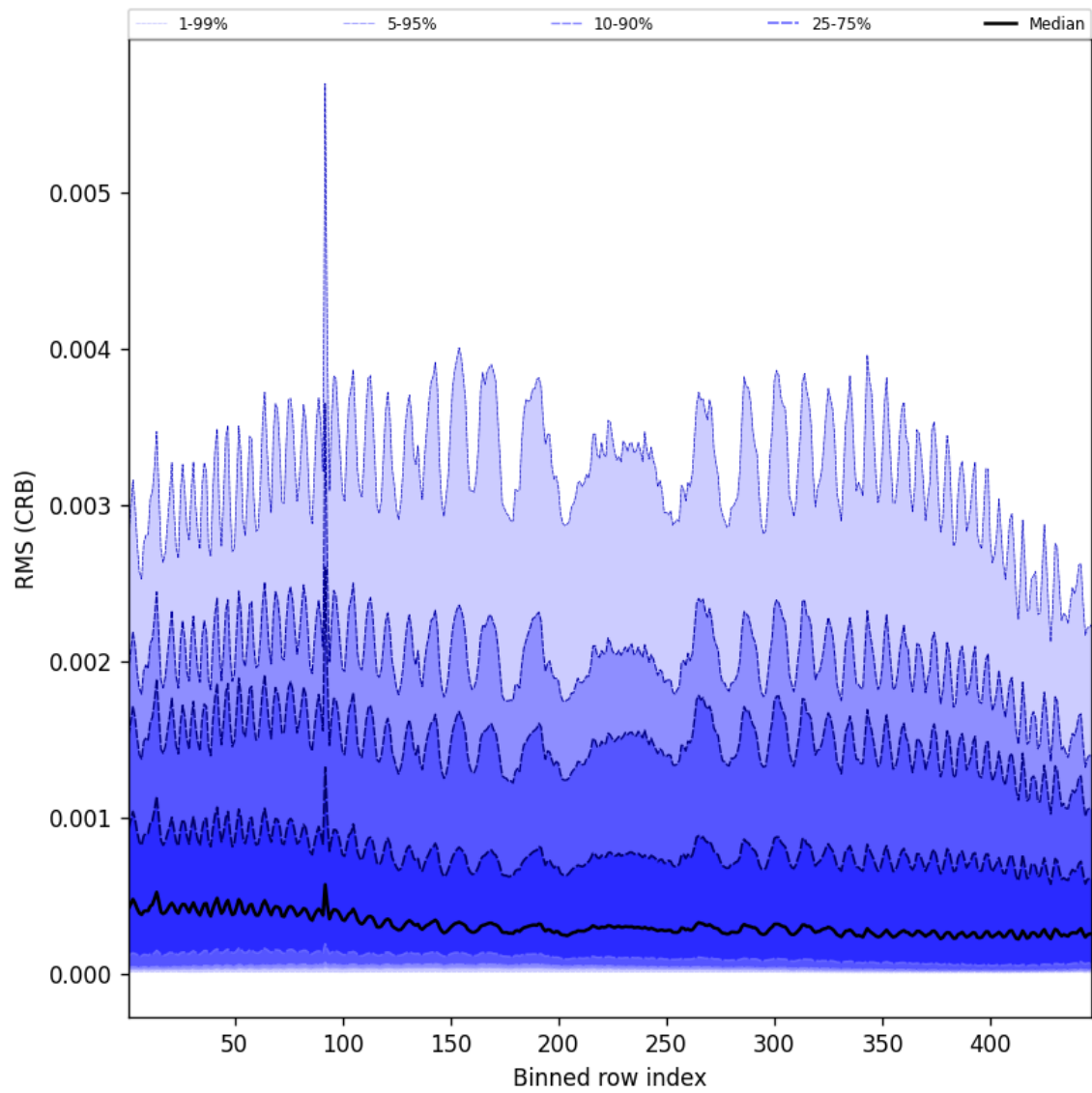
Figure 64: Along track statistics of “RMS (CRB)” for 2025-03-14 to 2025-03-16
