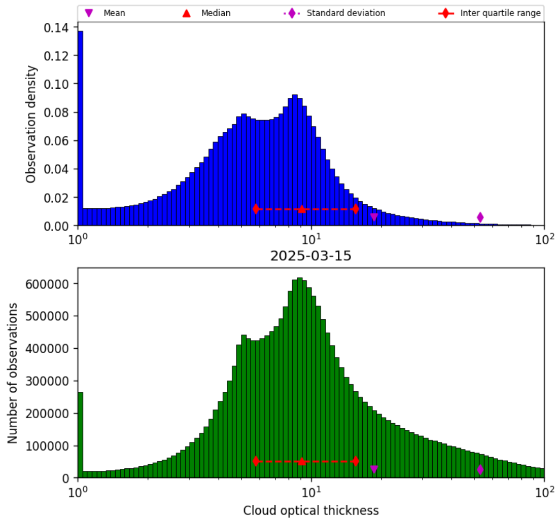
Figure 41: Histogram of “Cloud optical thickness” for 2025-03-14 to 2025-03-16
