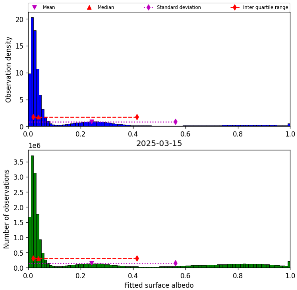
Figure 45: Histogram of “Fitted surface albedo” for 2025-03-14 to 2025-03-16
