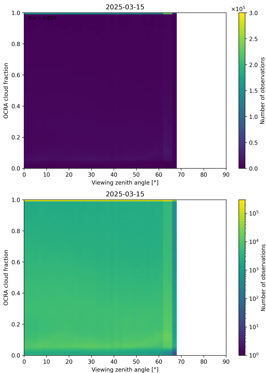
Figure 108: Scatter density plot of “Viewing zenith angle” against “OCRA cloud fraction” for 2025-03-14 to 2025-03-16.
