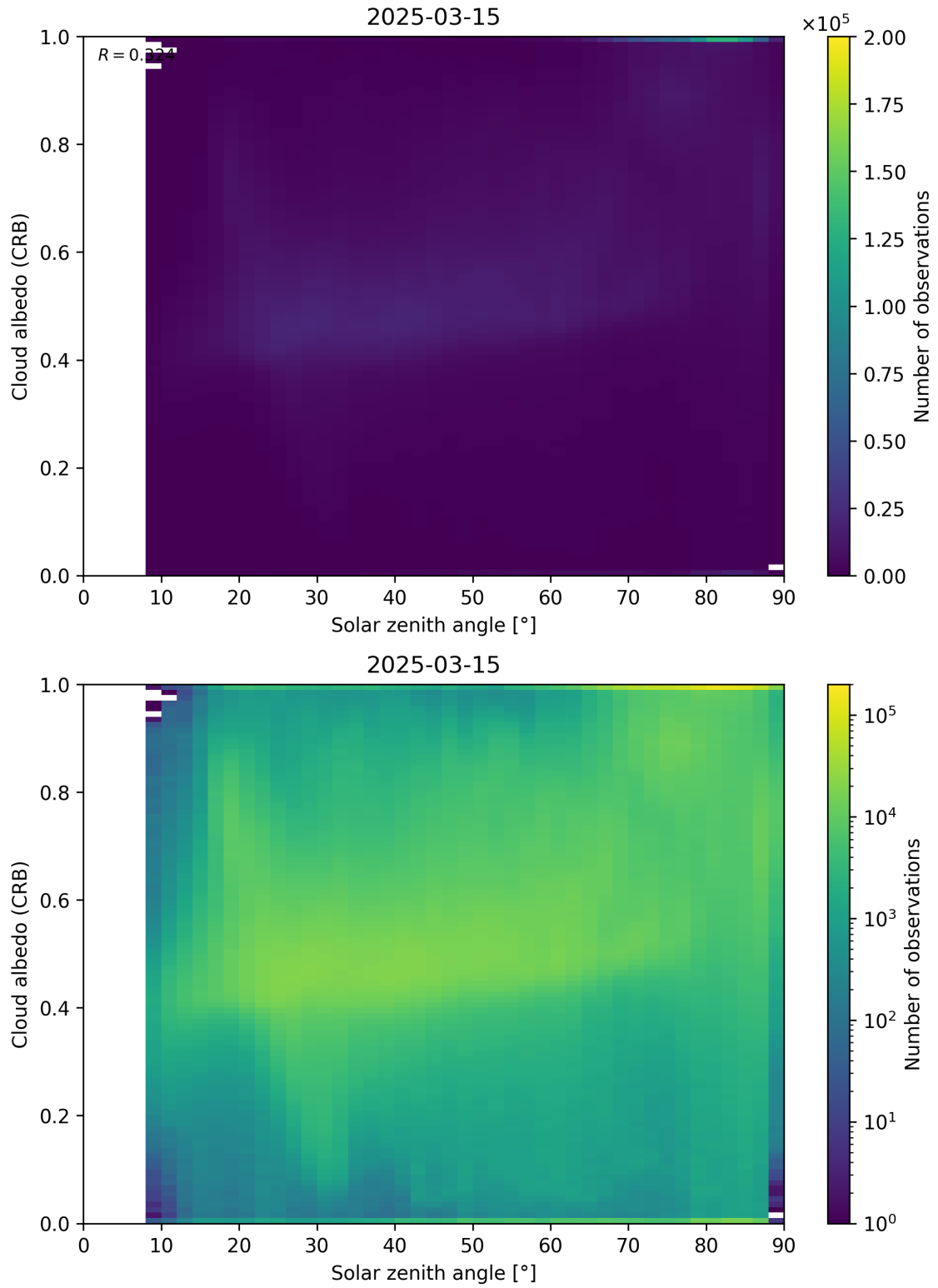
Figure 98: Scatter density plot of “Solar zenith angle” against “Cloud albedo (CRB)” for 2025-03-14 to 2025-03-16.
