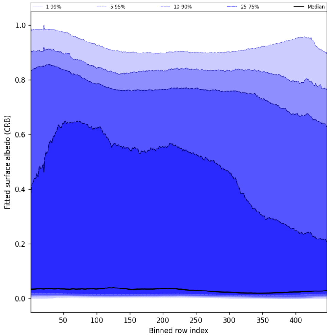
Figure 62: Along track statistics of “Fitted surface albedo (CRB)” for 2025-03-14 to 2025-03-16
