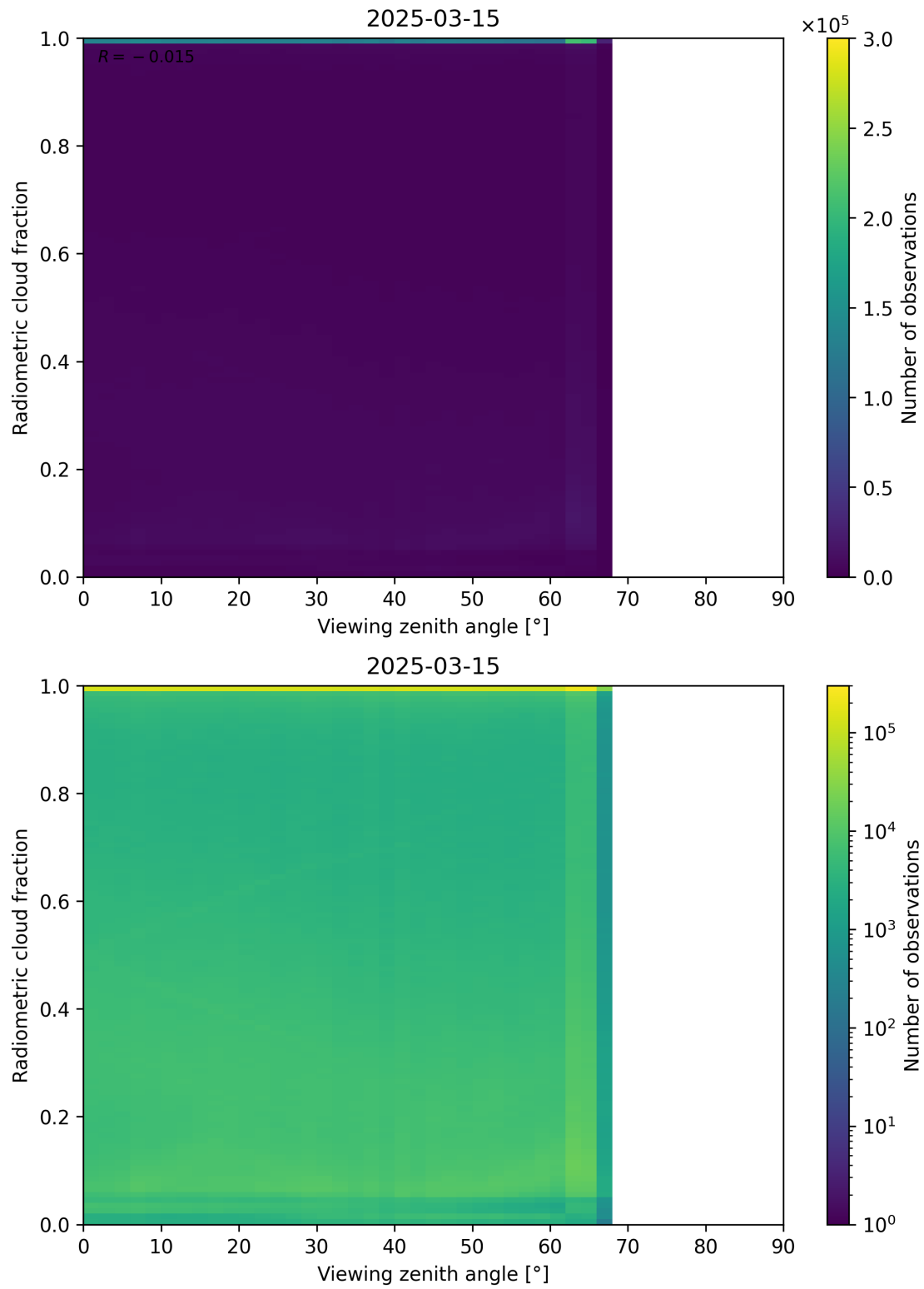
Figure 107: Scatter density plot of “Viewing zenith angle” against “Radiometric cloud fraction” for 2025-03-14 to 2025-03-16.
