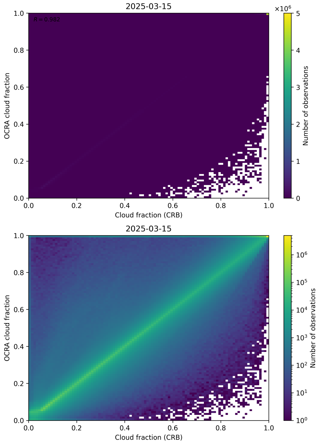
Figure 78: Scatter density plot of “Cloud fraction (CRB)” against “OCRA cloud fraction” for 2025-03-14 to 2025-03-16.
