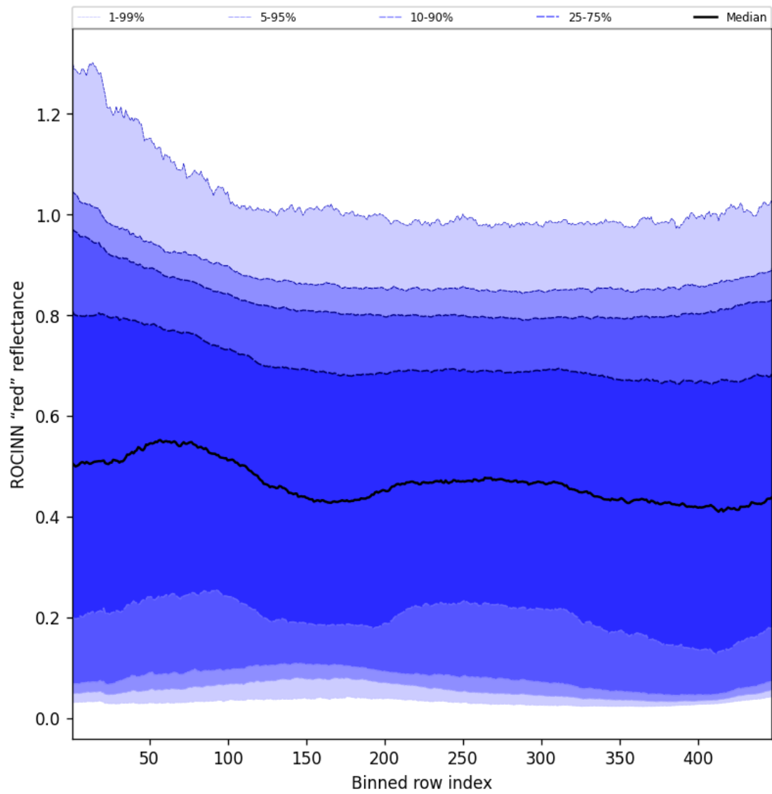
Figure 69: Along track statistics of “ROCINN “red” reflectance” for 2025-03-14 to 2025-03-16
