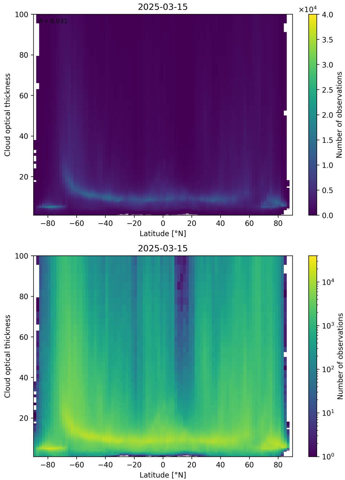
Figure 96: Scatter density plot of “Latitude” against “Cloud optical thickness” for 2025-03-14 to 2025-03-16.
