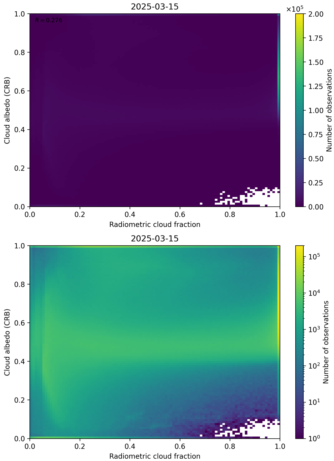
Figure 71: Scatter density plot of “Radiometric cloud fraction” against “Cloud albedo (CRB)” for 2025-03-14 to 2025-03-16.
