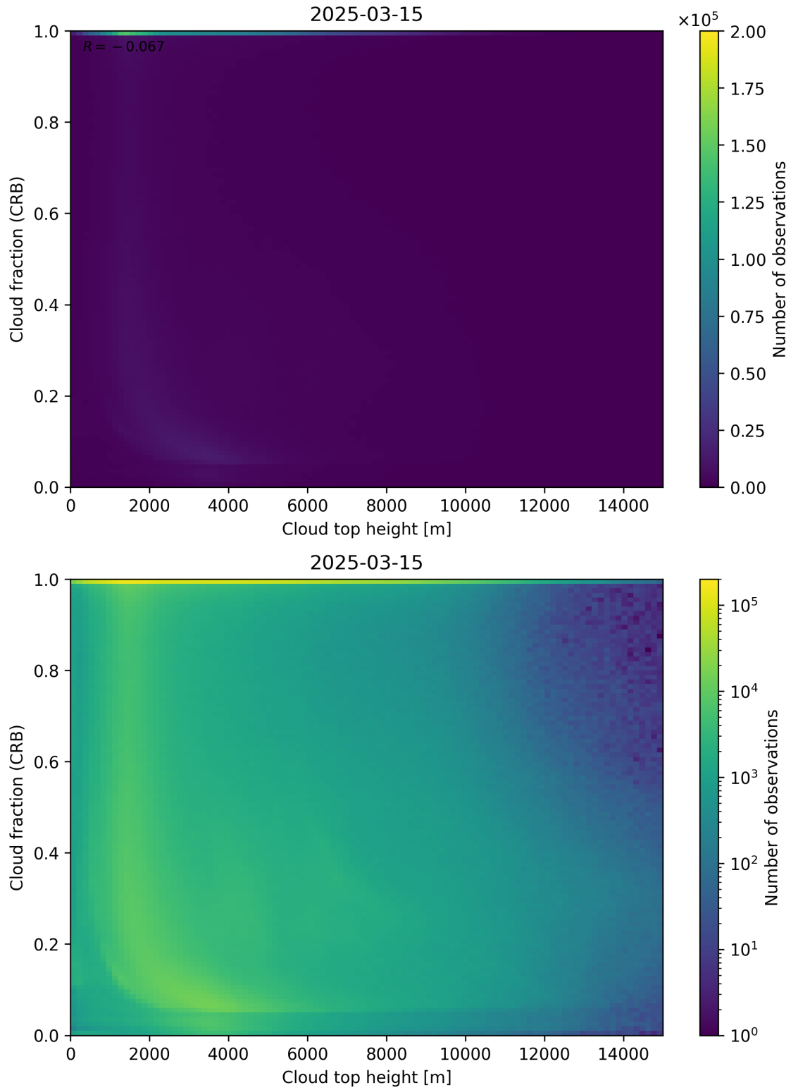
Figure 88: Scatter density plot of “Cloud top height” against “Cloud fraction (CRB)” for 2025-03-14 to 2025-03-16.
