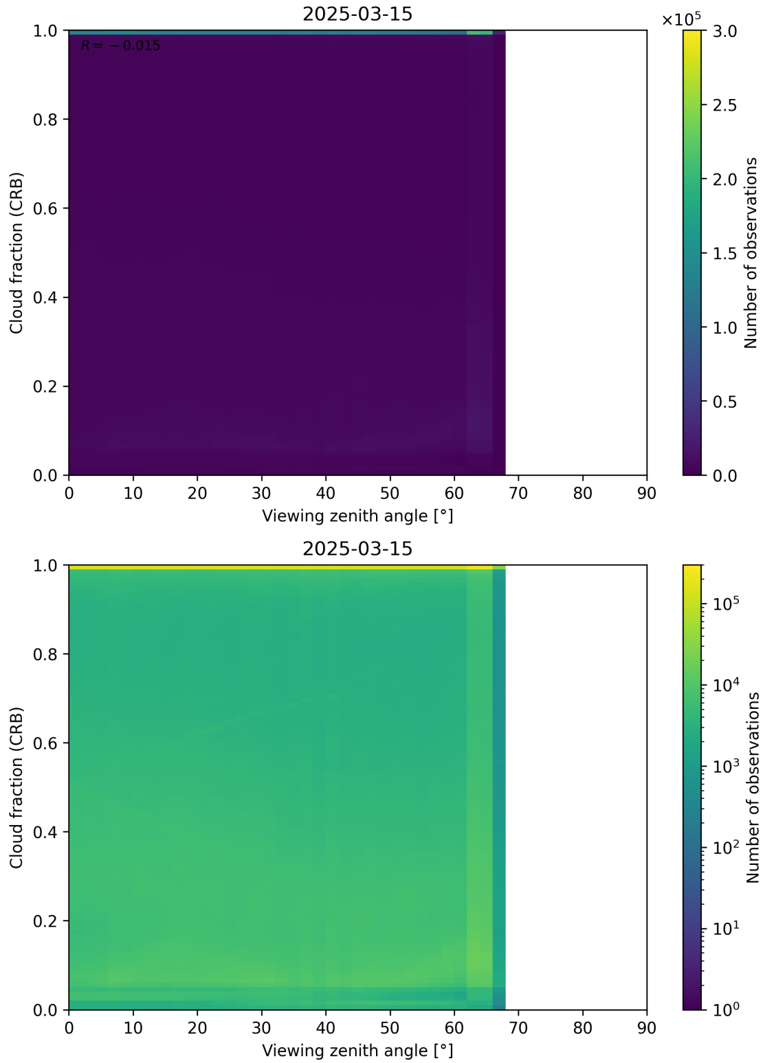
Figure 109: Scatter density plot of “Viewing zenith angle” against “Cloud fraction (CRB)” for 2025-03-14 to 2025-03-16.
