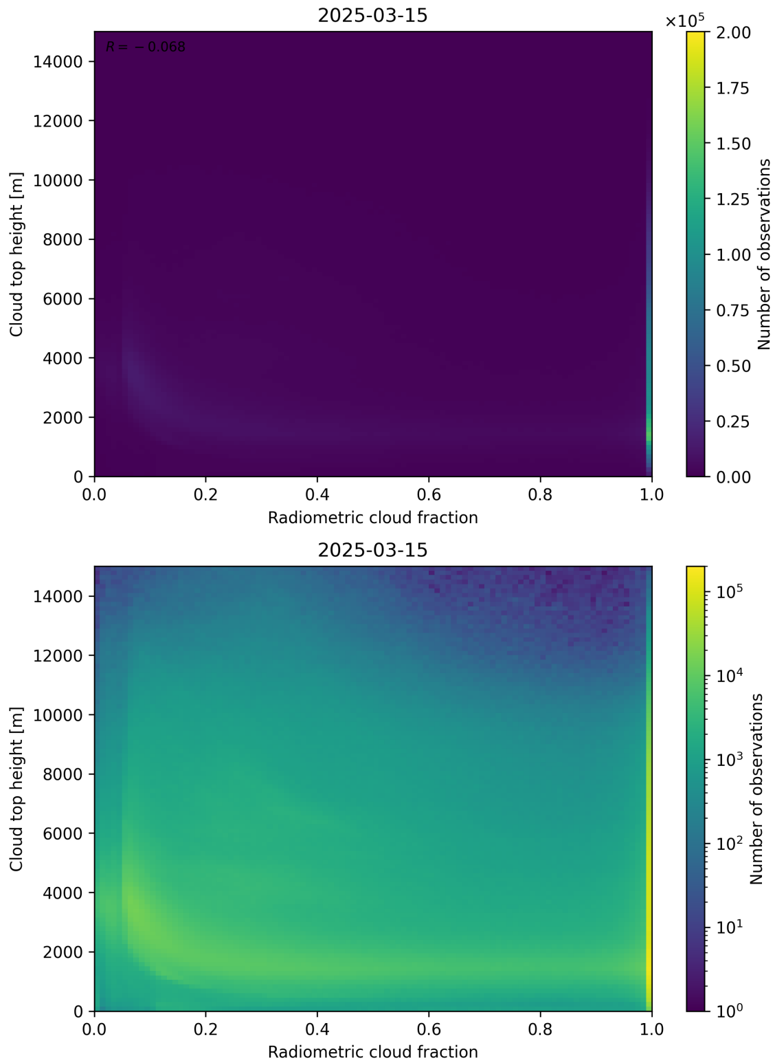
Figure 76: Scatter density plot of “Radiometric cloud fraction” against “Cloud top height” for 2025-03-14 to 2025-03-16.
