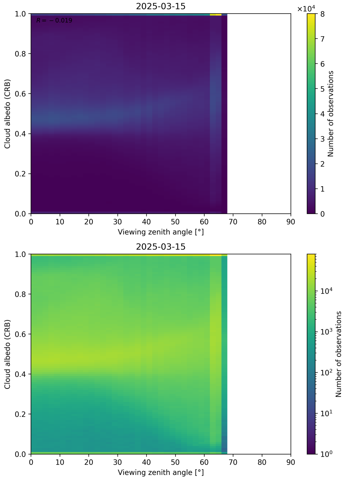
Figure 106: Scatter density plot of “Viewing zenith angle” against “Cloud albedo (CRB)” for 2025-03-14 to 2025-03-16.
