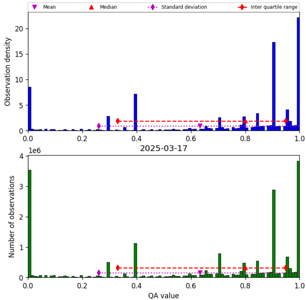
Figure 38: Histogram of “QA value” for 2025-03-17 to 2025-03-18
