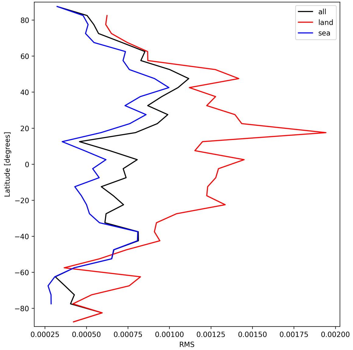
Figure 31: Zonal average of “RMS” for 2025-03-17 to 2025-03-18.
