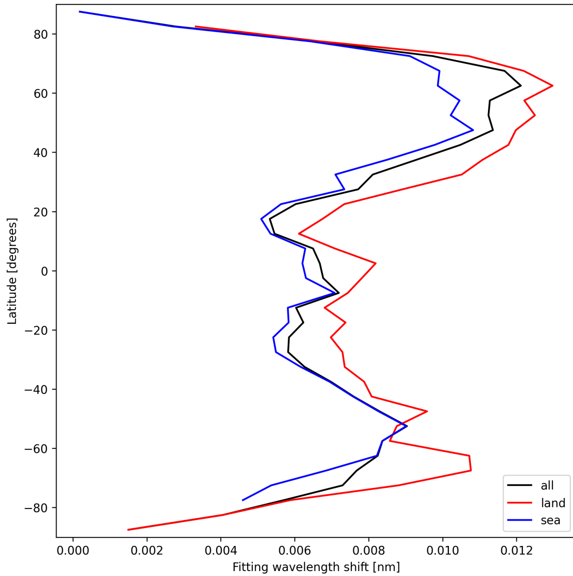
Figure 33: Zonal average of “Fitting wavelength shift” for 2025-03-17 to 2025-03-18.
