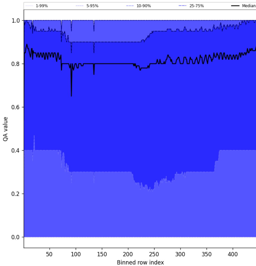
Figure 54: Along track statistics of “QA value” for 2025-03-17 to 2025-03-18
