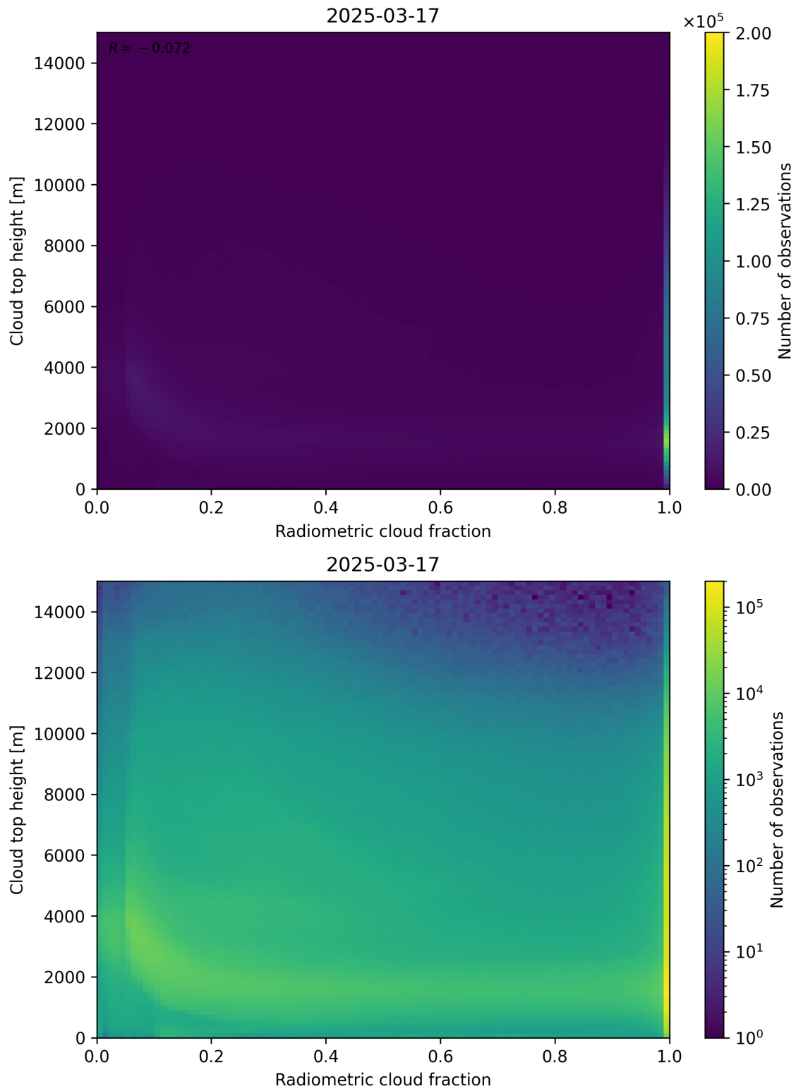
Figure 76: Scatter density plot of “Radiometric cloud fraction” against “Cloud top height” for 2025-03-17 to 2025-03-18.
