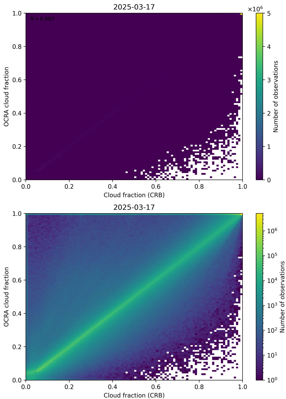
Figure 78: Scatter density plot of “Cloud fraction (CRB)” against “OCRA cloud fraction” for 2025-03-17 to 2025-03-18.
