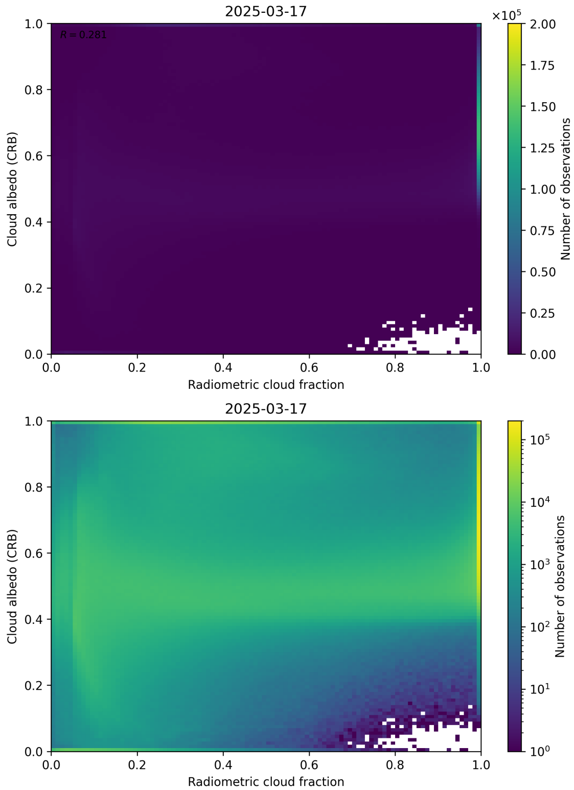
Figure 71: Scatter density plot of “Radiometric cloud fraction” against “Cloud albedo (CRB)” for 2025-03-17 to 2025-03-18.
