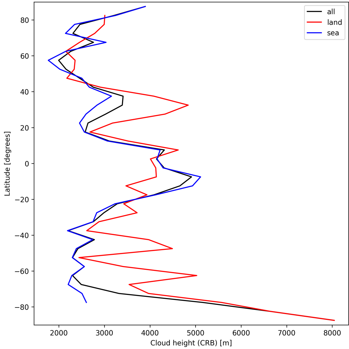
Figure 27: Zonal average of “Cloud height (CRB)” for 2025-03-17 to 2025-03-18.
