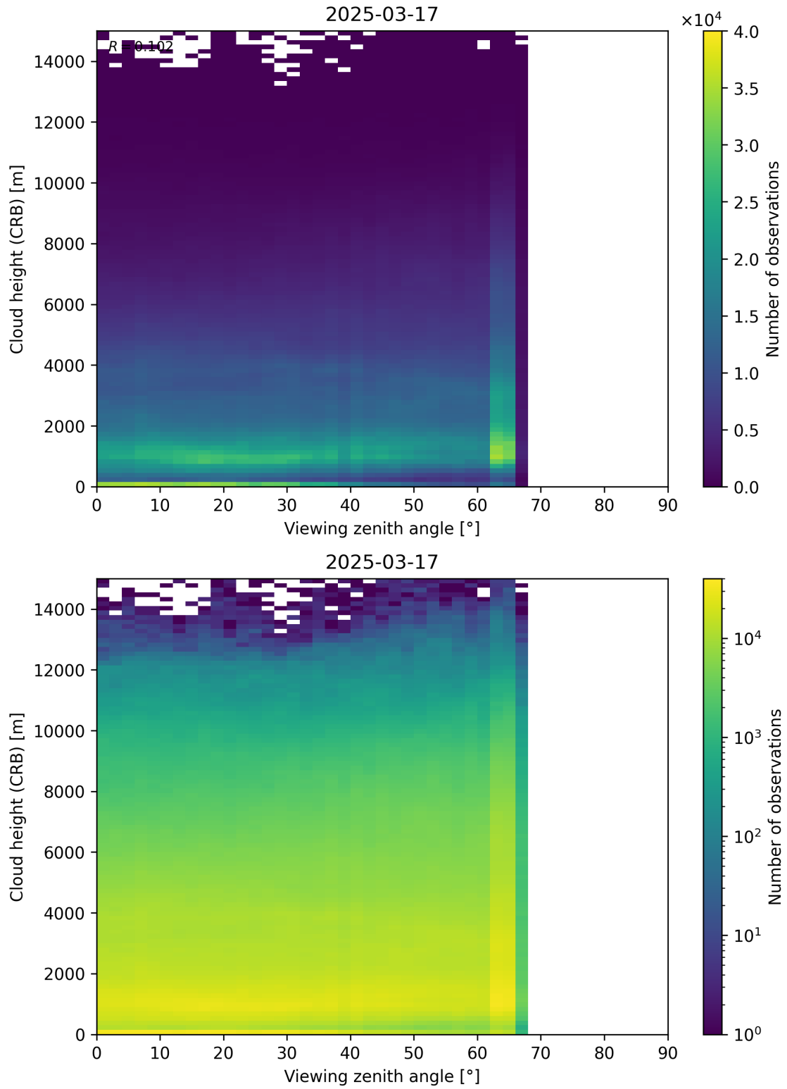
Figure 110: Scatter density plot of “Viewing zenith angle” against “Cloud height (CRB)” for 2025-03-17 to 2025-03-18.
