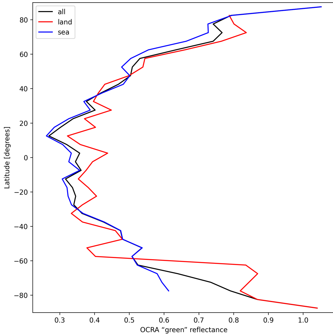
Figure 36: Zonal average of “OCRA “green” reflectance” for 2025-03-17 to 2025-03-18.
