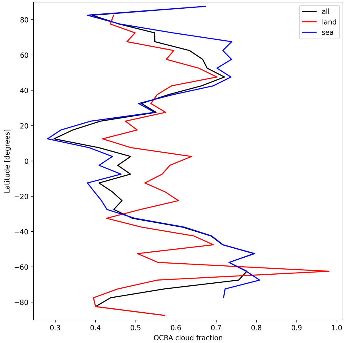
Figure 34: Zonal average of “OCRA cloud fraction” for 2025-03-17 to 2025-03-18.
