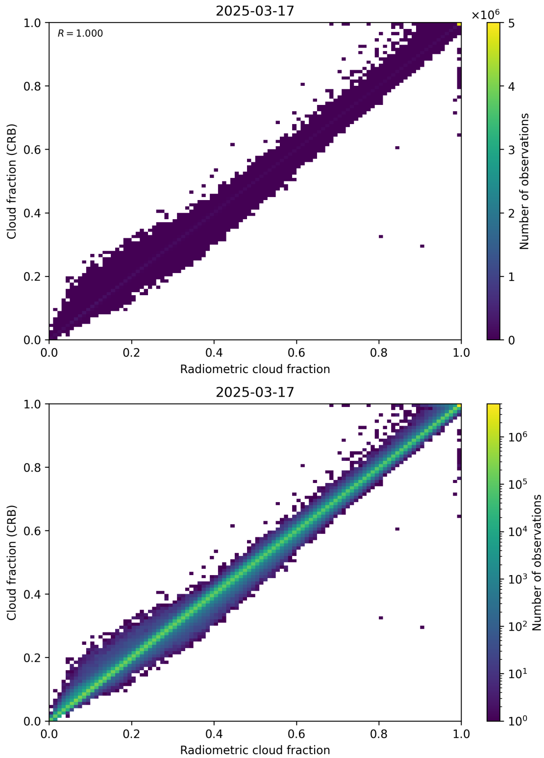
Figure 73: Scatter density plot of “Radiometric cloud fraction” against “Cloud fraction (CRB)” for 2025-03-17 to 2025-03-18.
