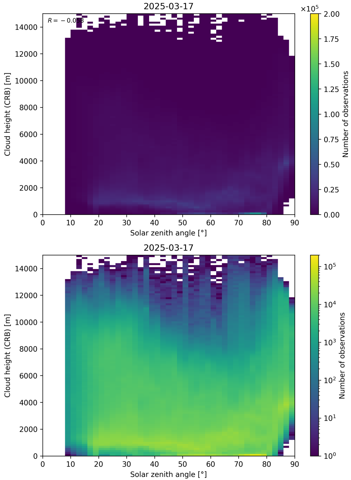
Figure 102: Scatter density plot of “Solar zenith angle” against “Cloud height (CRB)” for 2025-03-17 to 2025-03-18.
