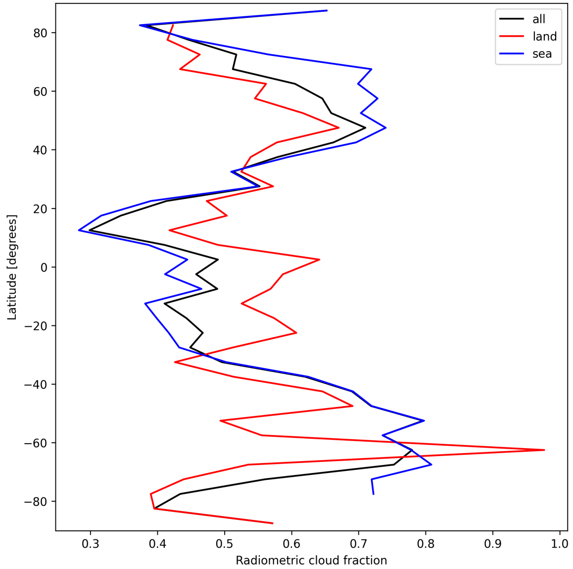
Figure 23: Zonal average of “Radiometric cloud fraction” for 2025-03-17 to 2025-03-18.
