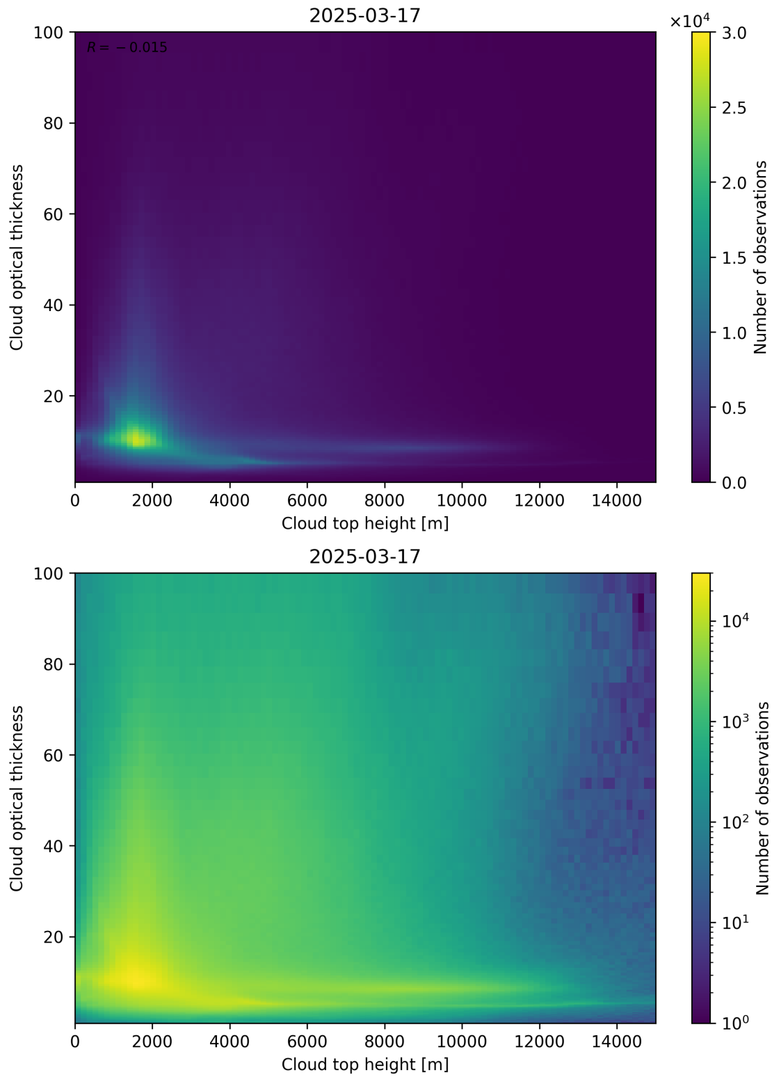
Figure 90: Scatter density plot of “Cloud top height” against “Cloud optical thickness” for 2025-03-17 to 2025-03-18.
