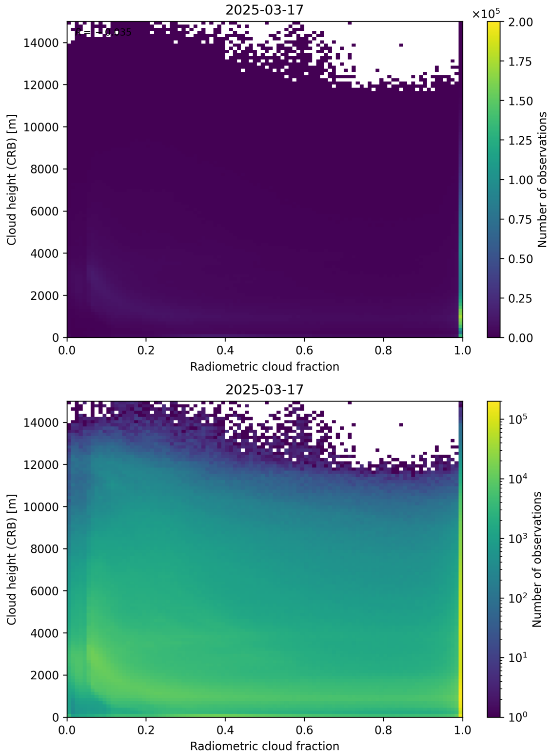
Figure 74: Scatter density plot of “Radiometric cloud fraction” against “Cloud height (CRB)” for 2025-03-17 to 2025-03-18.
