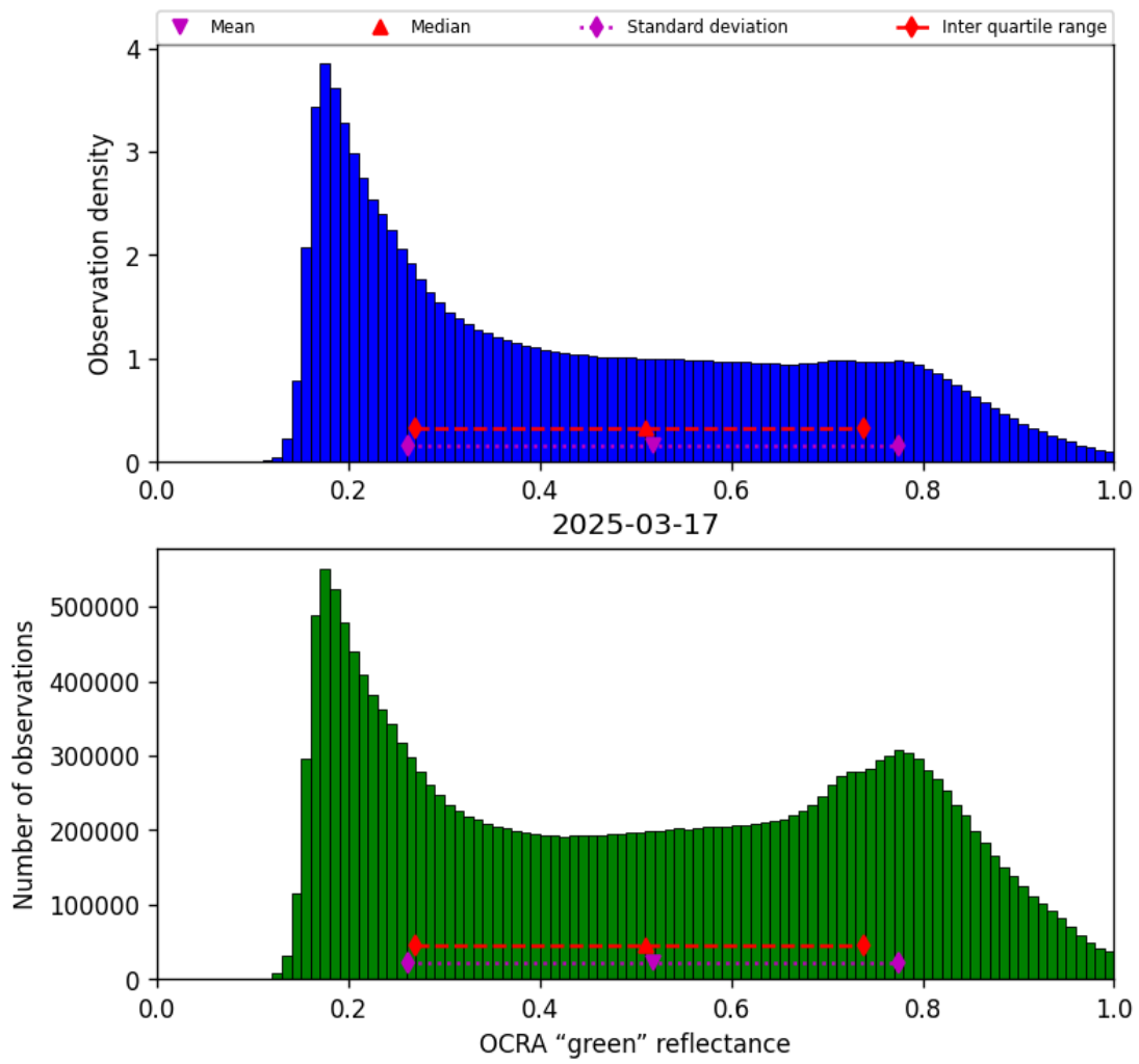
Figure 52: Histogram of “OCRA “green” reflectance” for 2025-03-17 to 2025-03-18
