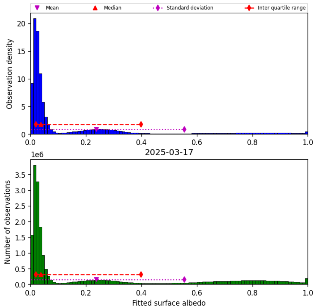
Figure 45: Histogram of “Fitted surface albedo” for 2025-03-17 to 2025-03-18
