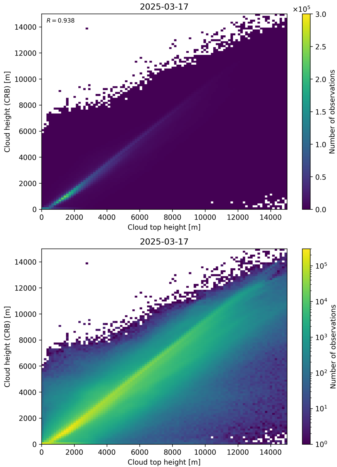
Figure 89: Scatter density plot of “Cloud top height” against “Cloud height (CRB)” for 2025-03-17 to 2025-03-18.
