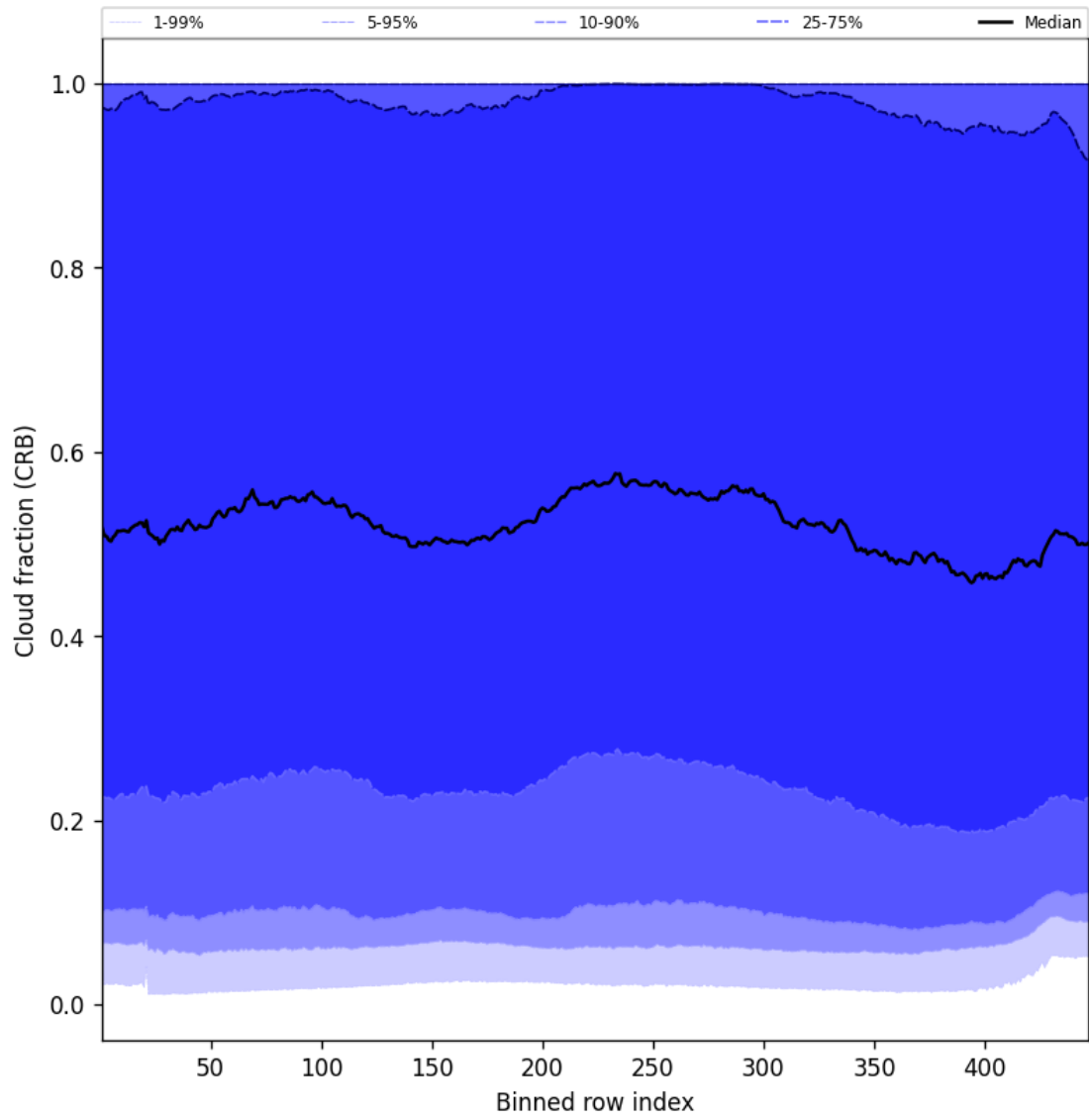
Figure 58: Along track statistics of “Cloud fraction (CRB)” for 2025-03-17 to 2025-03-18
