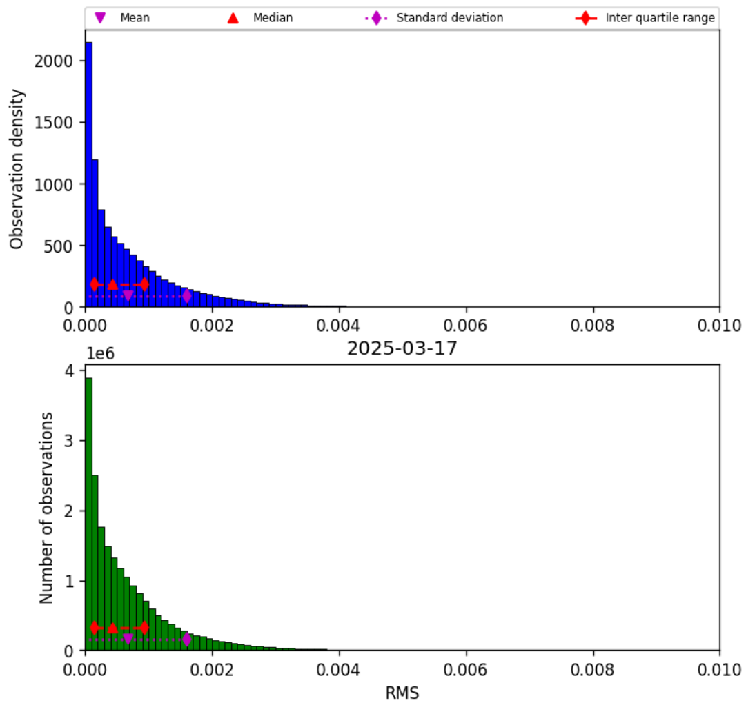
Figure 47: Histogram of “RMS” for 2025-03-17 to 2025-03-18
