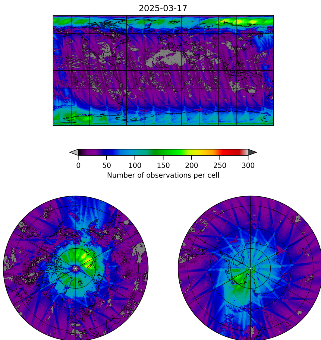
Figure 21: Map of the number of observations for 2025-03-17 to 2025-03-18
