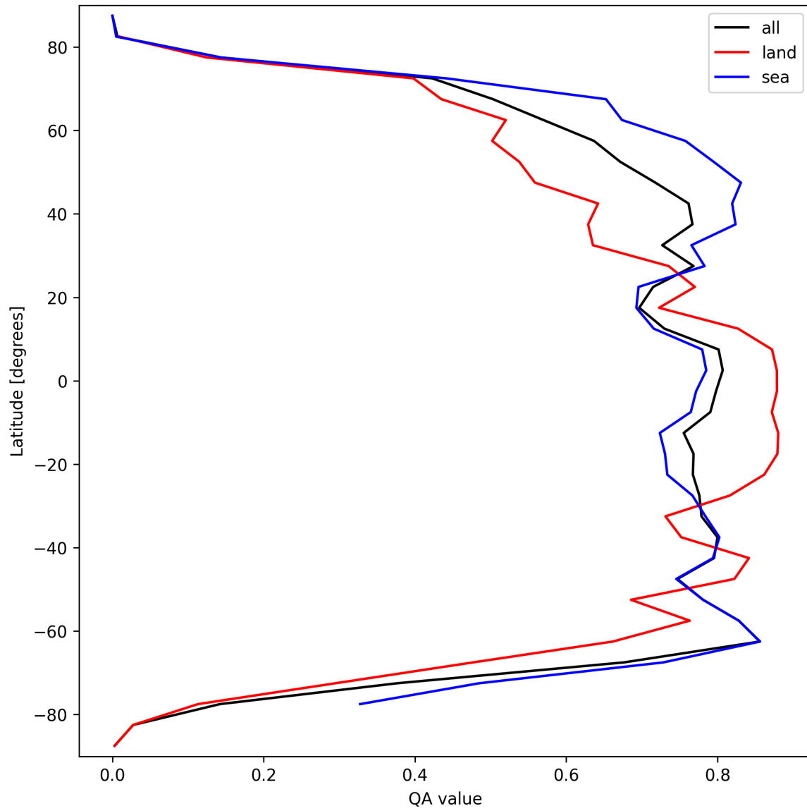
Figure 22: Zonal average of “QA value” for 2025-03-17 to 2025-03-18.
