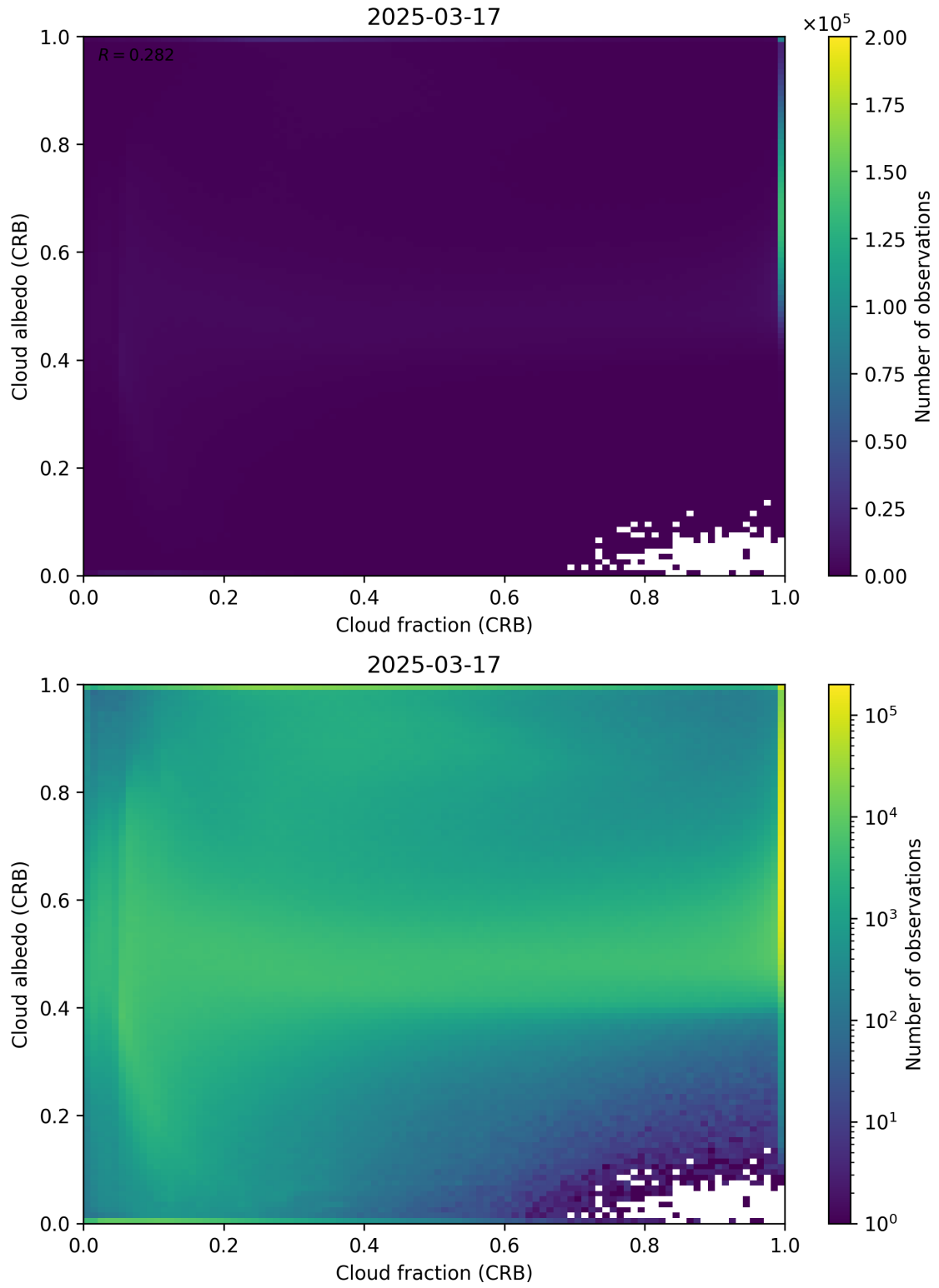
Figure 77: Scatter density plot of “Cloud fraction (CRB)” against “Cloud albedo (CRB)” for 2025-03-17 to 2025-03-18.
