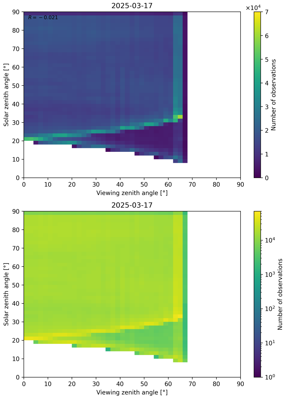
Figure 114: Scatter density plot of “Viewing zenith angle” against “Solar zenith angle” for 2025-03-17 to 2025-03-18.
