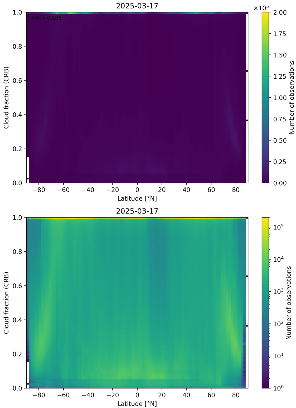
Figure 94: Scatter density plot of “Latitude” against “Cloud fraction (CRB)” for 2025-03-17 to 2025-03-18.
