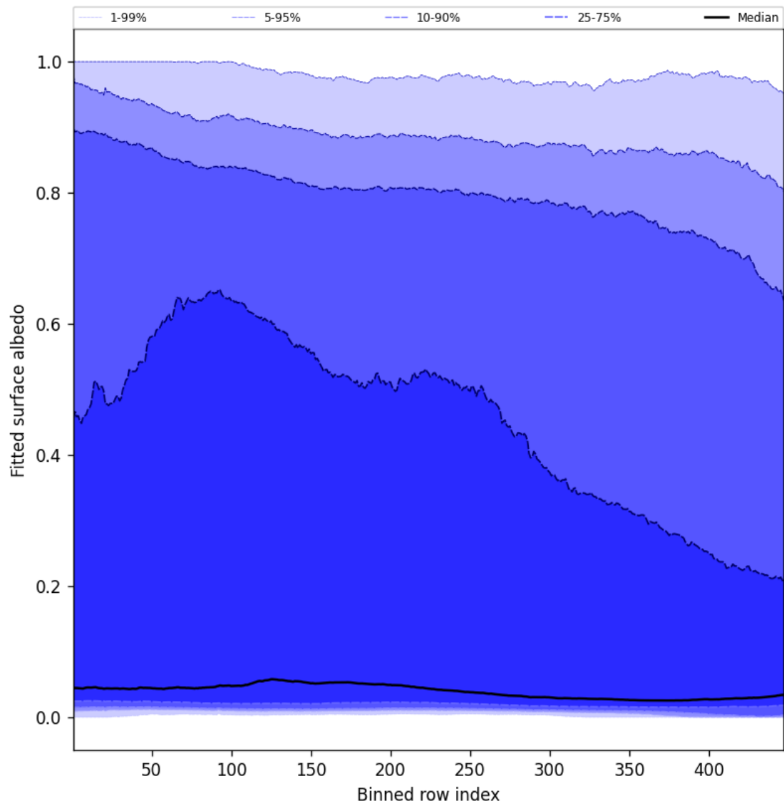
Figure 61: Along track statistics of “Fitted surface albedo” for 2025-03-17 to 2025-03-18
