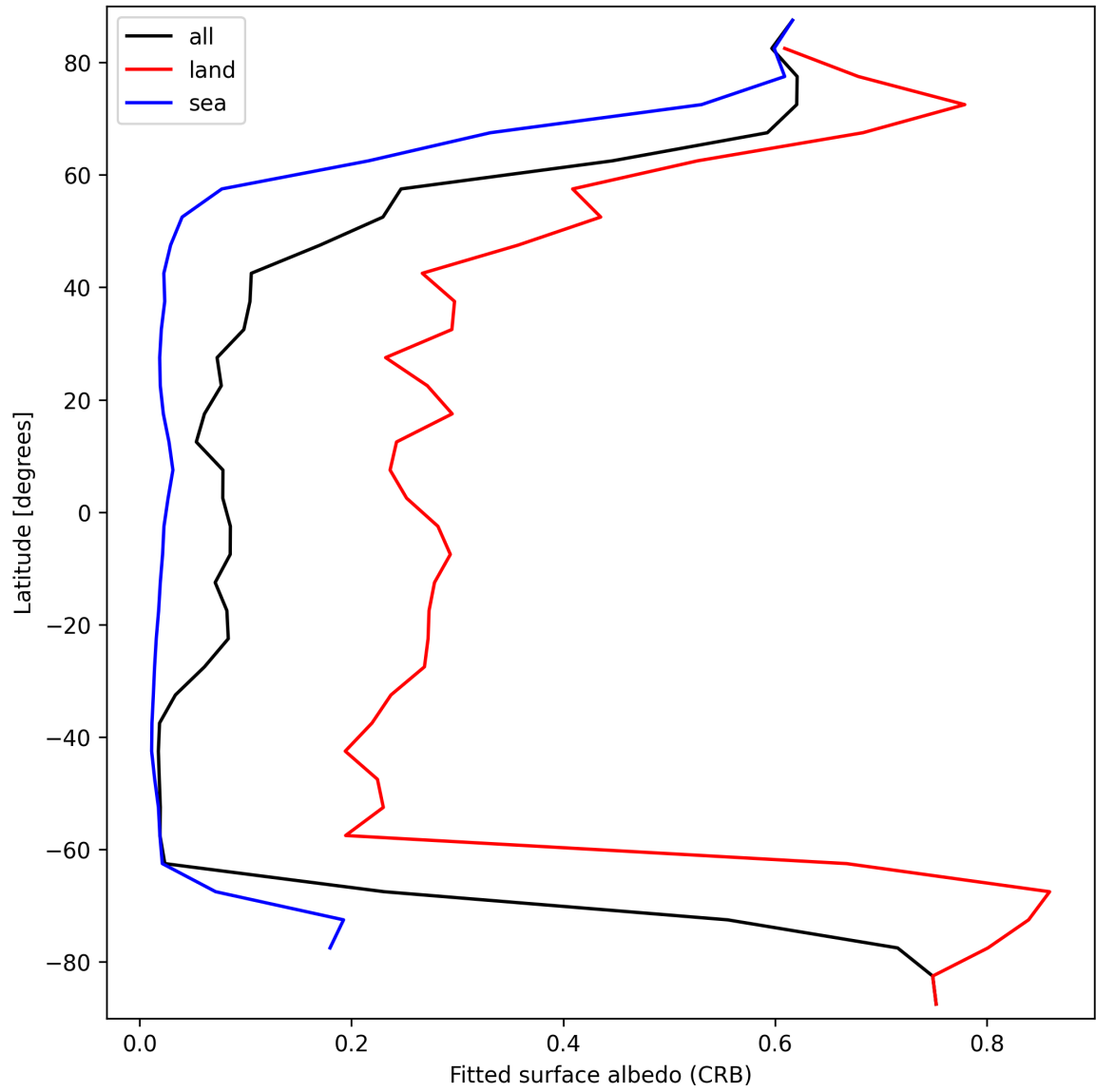
Figure 30: Zonal average of “Fitted surface albedo (CRB)” for 2025-03-17 to 2025-03-18.
