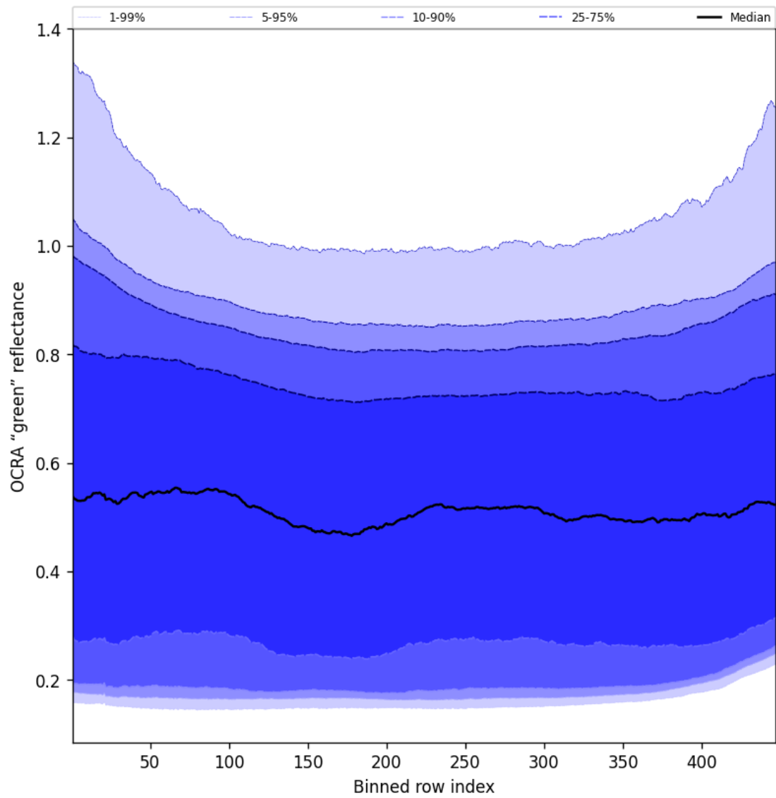
Figure 68: Along track statistics of “OCRA “green” reflectance” for 2025-03-17 to 2025-03-18
