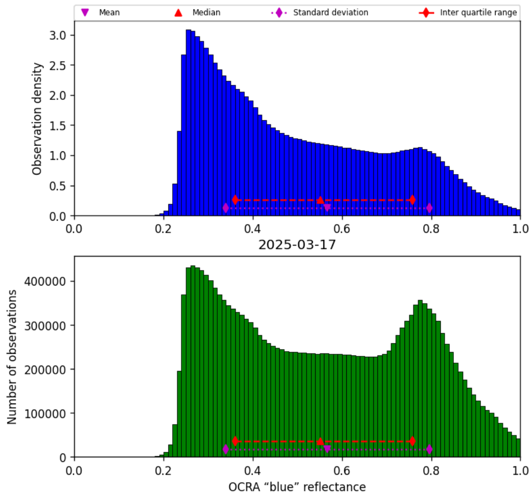
Figure 51: Histogram of “OCRA “blue” reflectance” for 2025-03-17 to 2025-03-18
