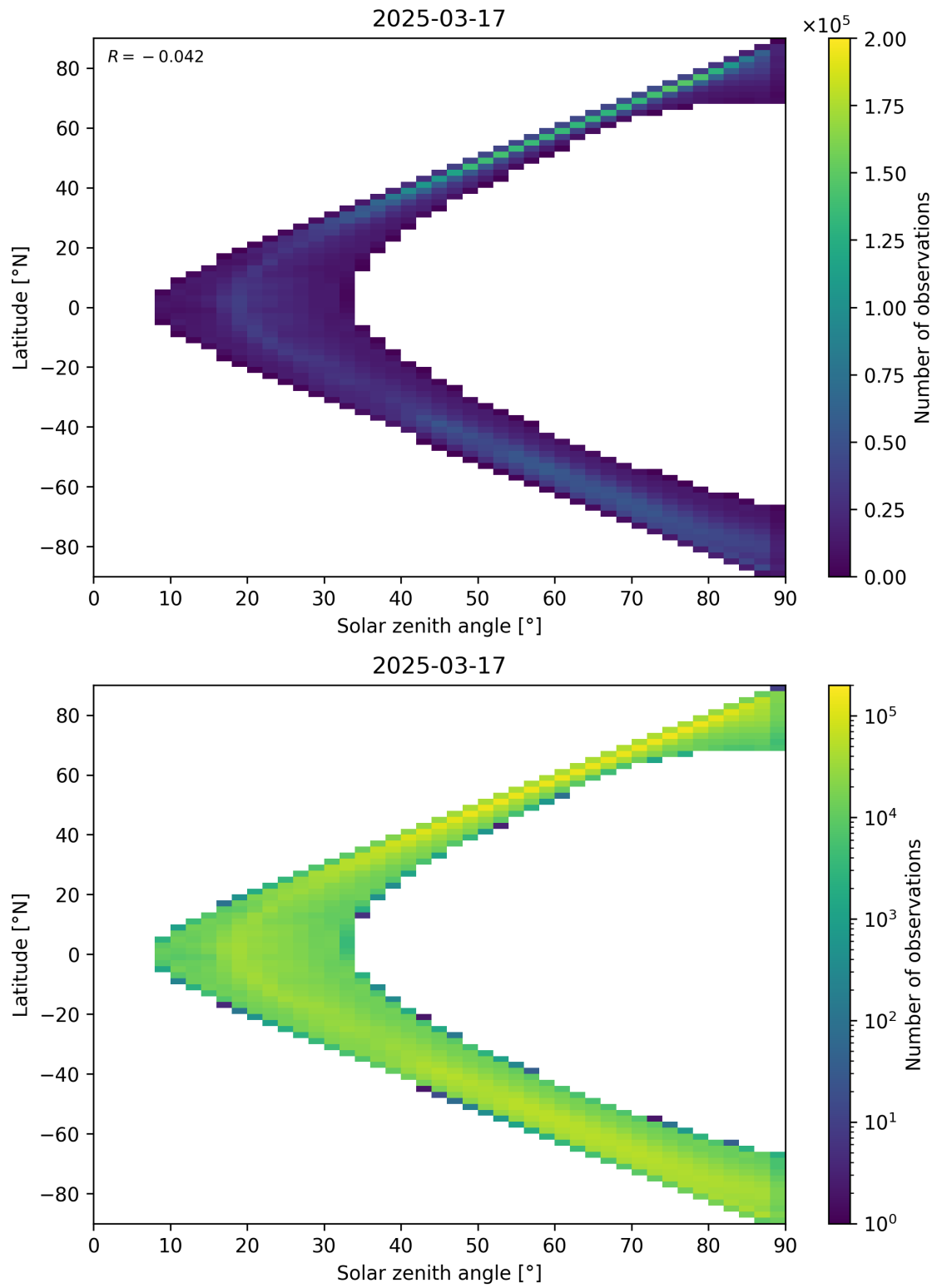
Figure 105: Scatter density plot of “Solar zenith angle” against “Latitude” for 2025-03-17 to 2025-03-18.
