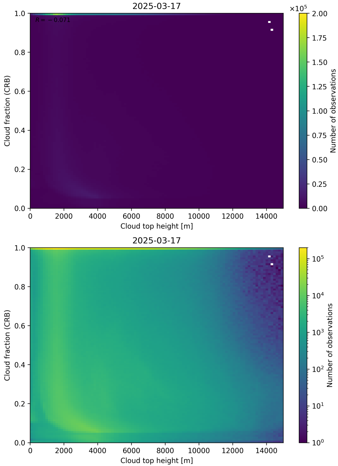
Figure 88: Scatter density plot of “Cloud top height” against “Cloud fraction (CRB)” for 2025-03-17 to 2025-03-18.
