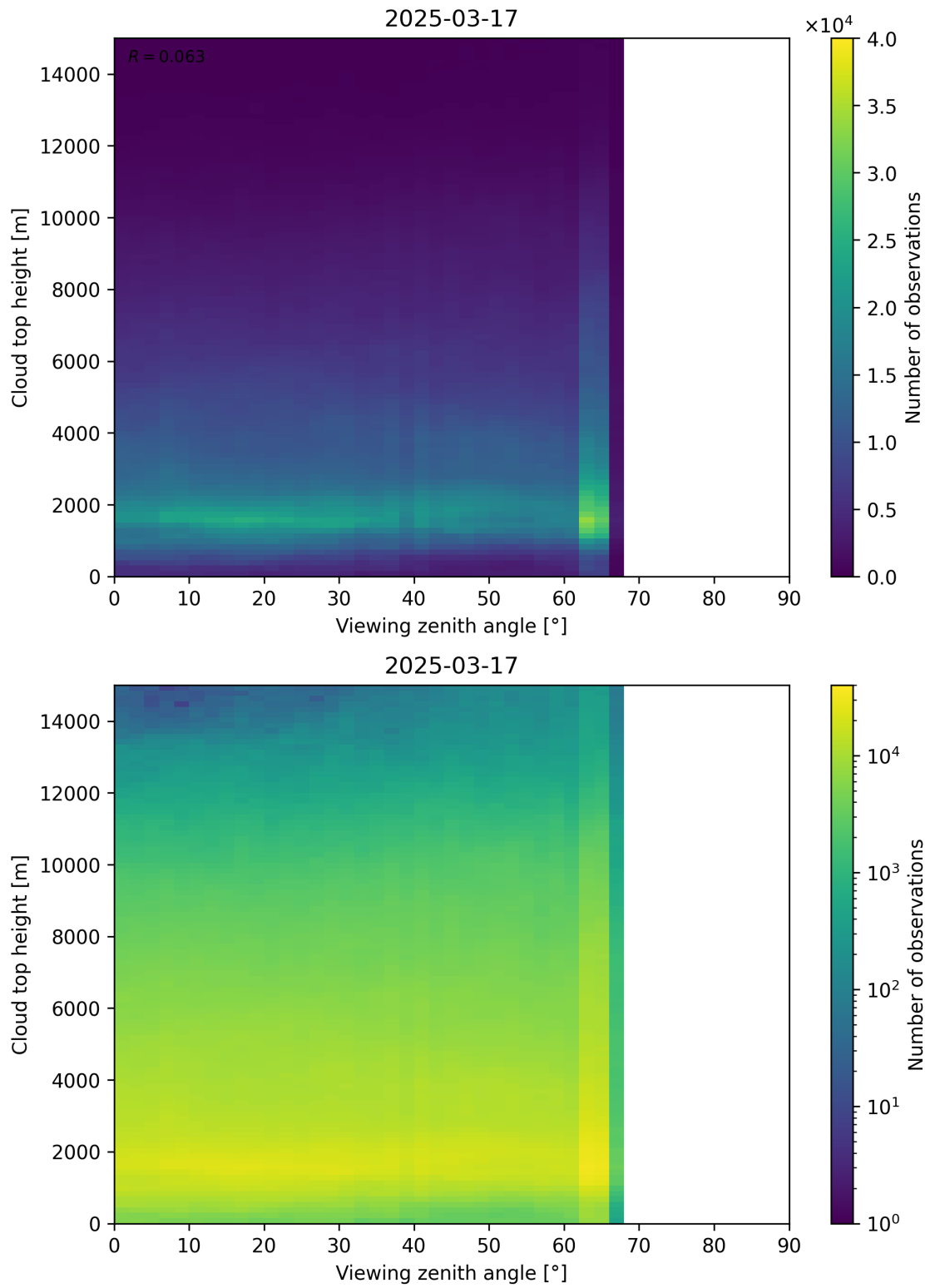
Figure 112: Scatter density plot of “Viewing zenith angle” against “Cloud top height” for 2025-03-17 to 2025-03-18.
