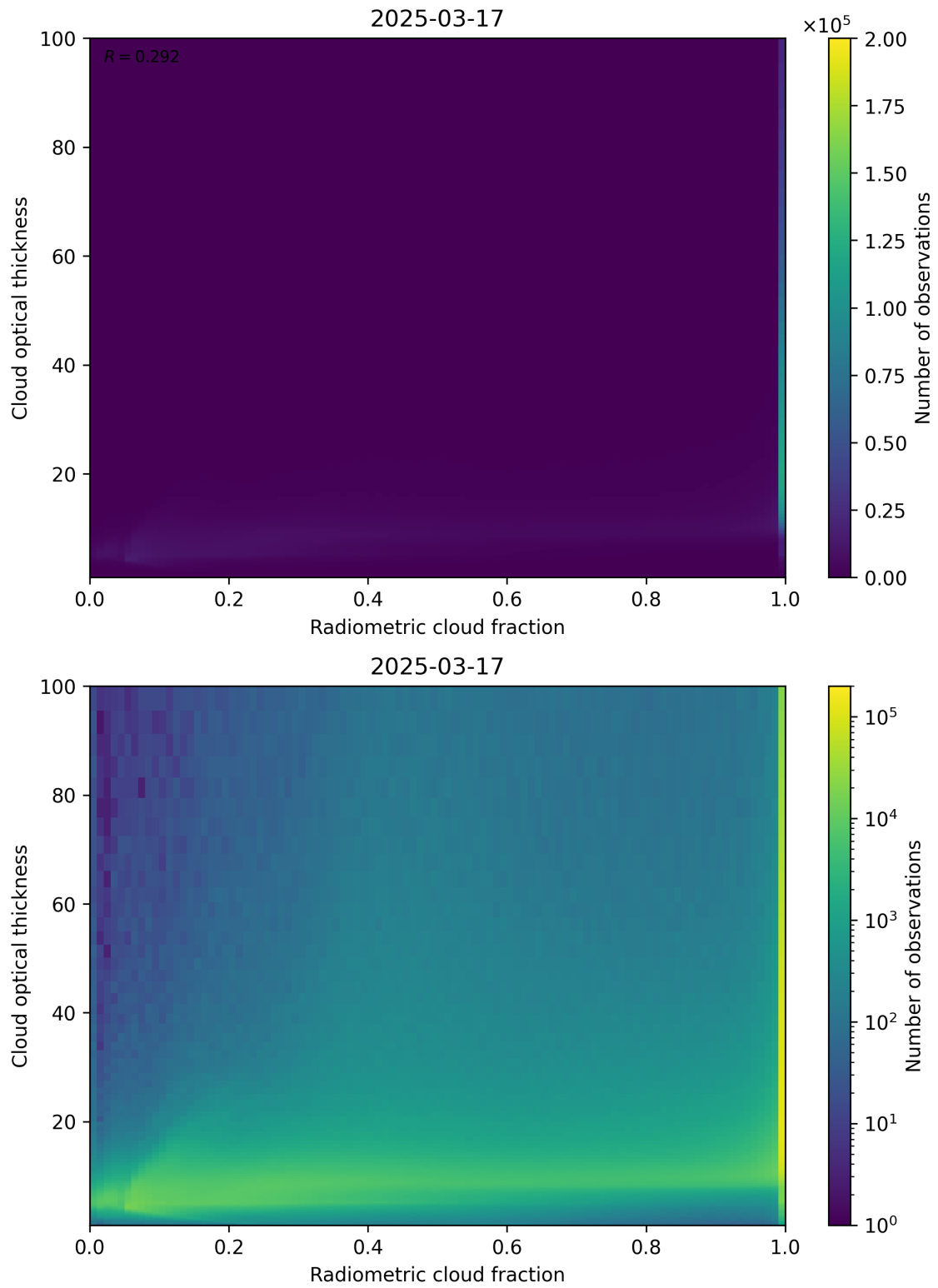
Figure 75: Scatter density plot of “Radiometric cloud fraction” against “Cloud optical thickness” for 2025-03-17 to 2025-03-18.
