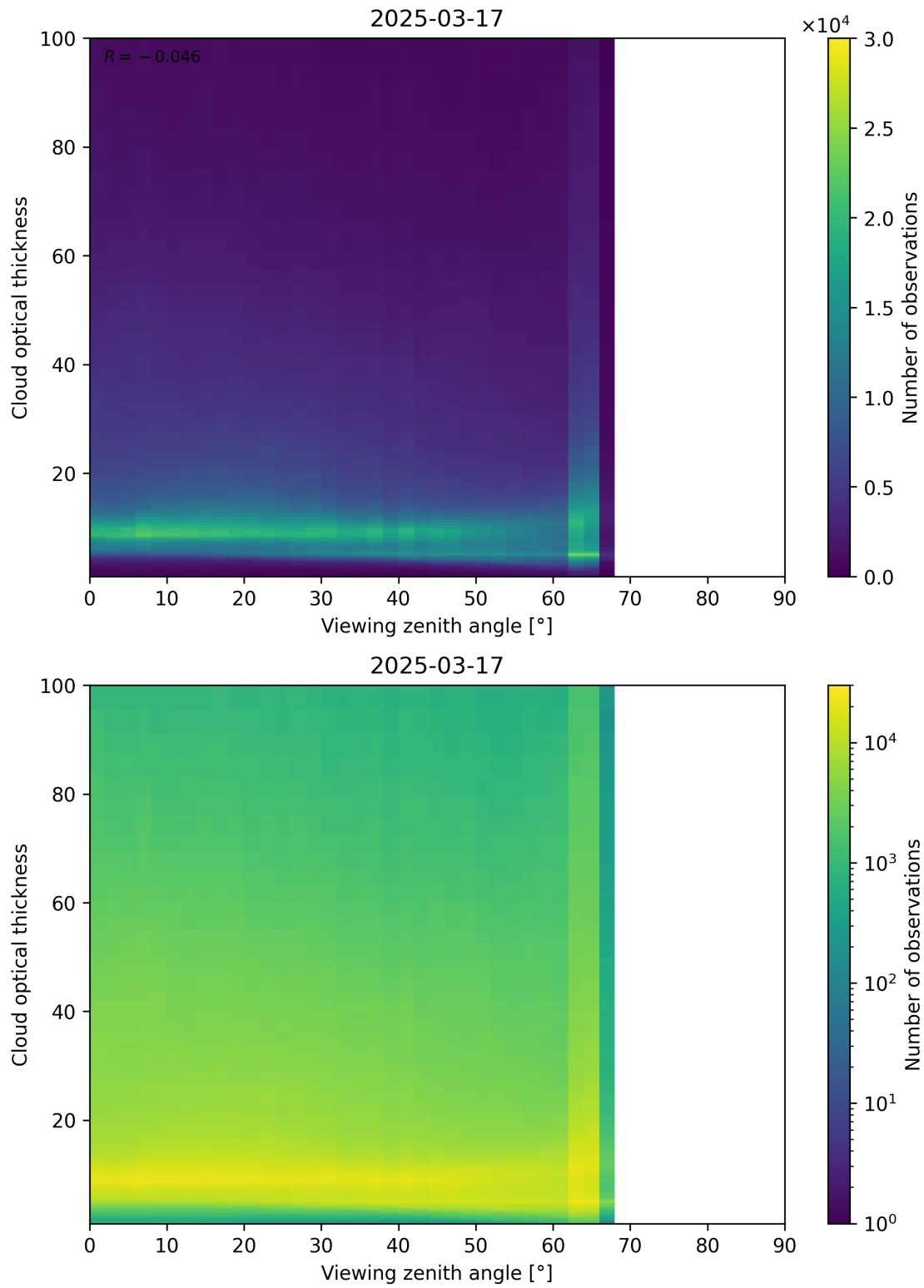
Figure 111: Scatter density plot of “Viewing zenith angle” against “Cloud optical thickness” for 2025-03-17 to 2025-03-18.
