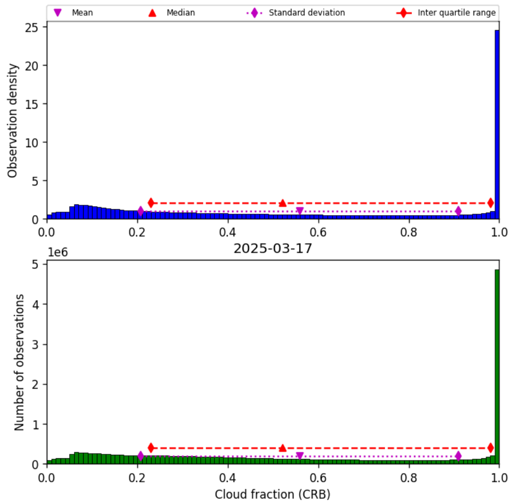
Figure 42: Histogram of “Cloud fraction (CRB)” for 2025-03-17 to 2025-03-18
