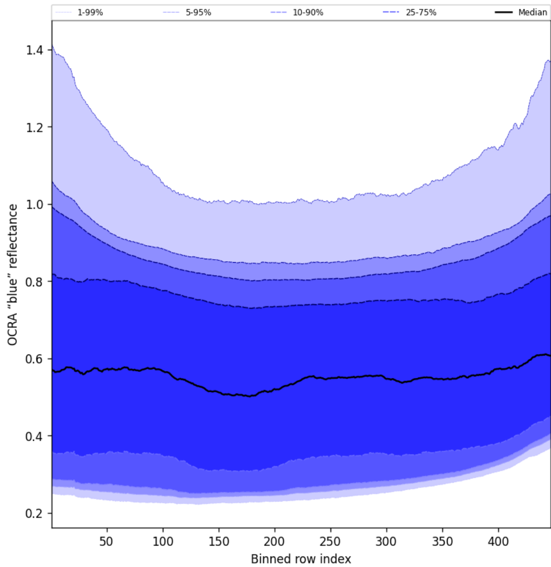
Figure 67: Along track statistics of “OCRA “blue” reflectance” for 2025-03-17 to 2025-03-18
