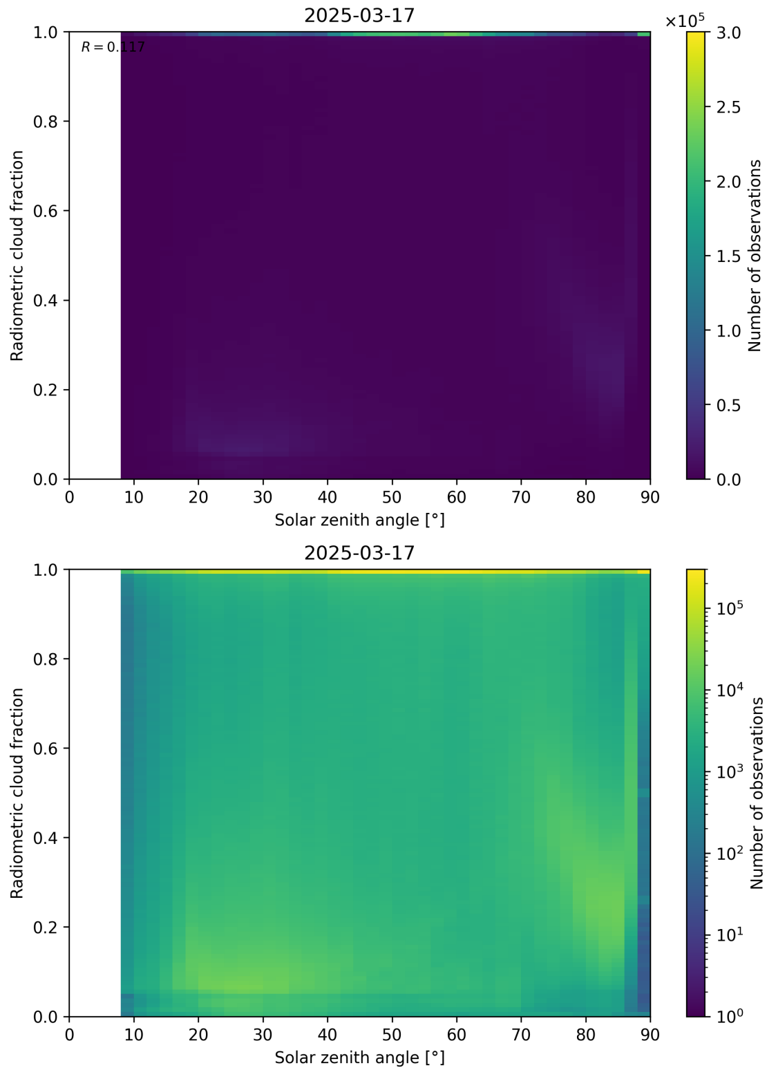
Figure 99: Scatter density plot of “Solar zenith angle” against “Radiometric cloud fraction” for 2025-03-17 to 2025-03-18.
