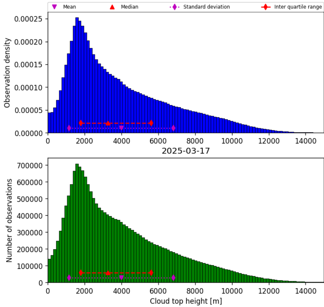
Figure 40: Histogram of “Cloud top height” for 2025-03-17 to 2025-03-18
