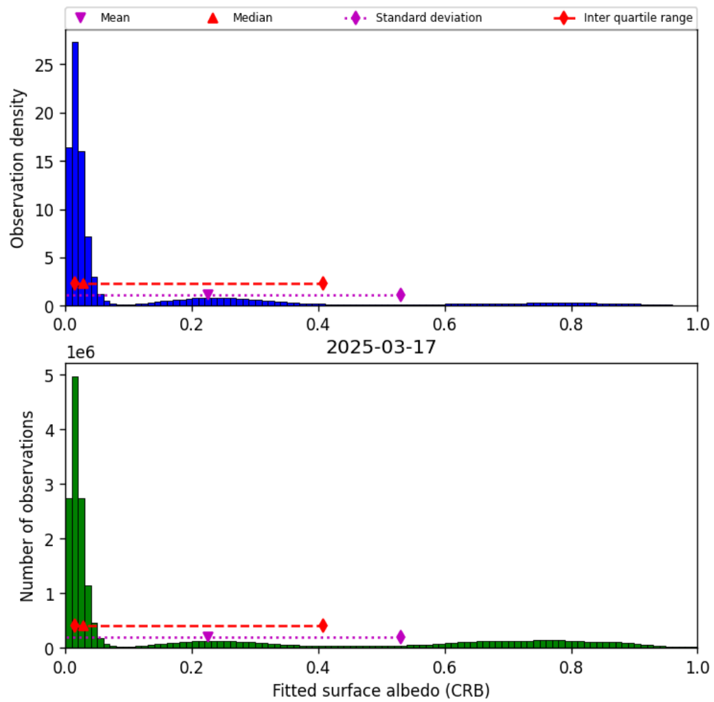
Figure 46: Histogram of “Fitted surface albedo (CRB)” for 2025-03-17 to 2025-03-18
