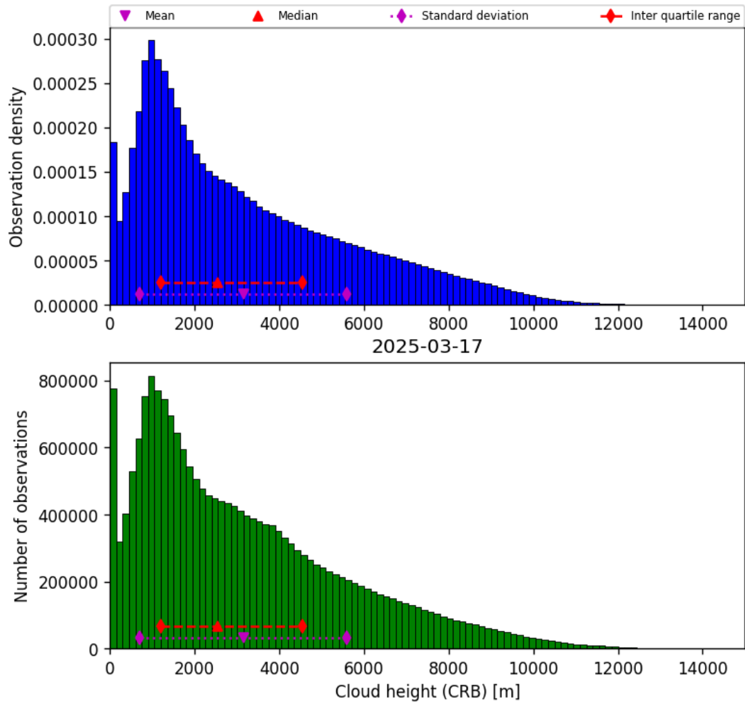
Figure 43: Histogram of “Cloud height (CRB)” for 2025-03-17 to 2025-03-18
