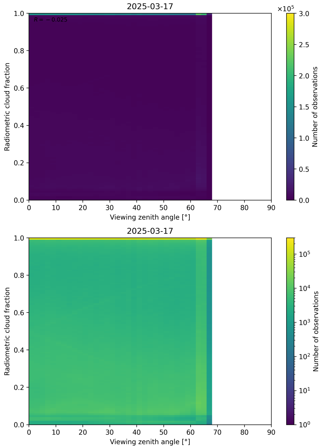
Figure 107: Scatter density plot of “Viewing zenith angle” against “Radiometric cloud fraction” for 2025-03-17 to 2025-03-18.
