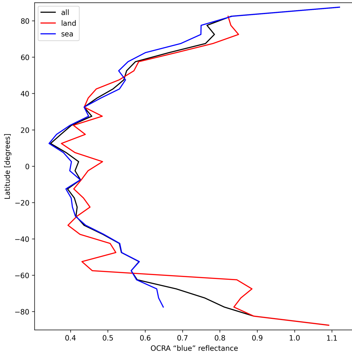
Figure 35: Zonal average of “OCRA “blue” reflectance” for 2025-03-17 to 2025-03-18.
