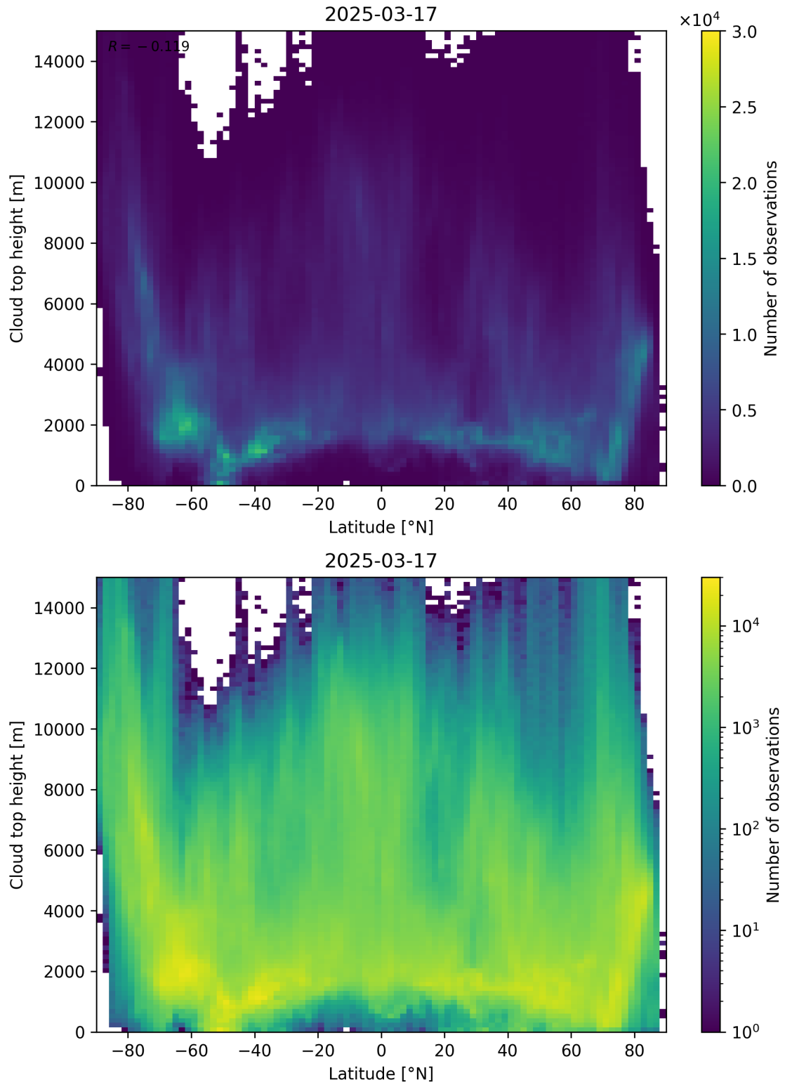
Figure 97: Scatter density plot of “Latitude” against “Cloud top height” for 2025-03-17 to 2025-03-18.
