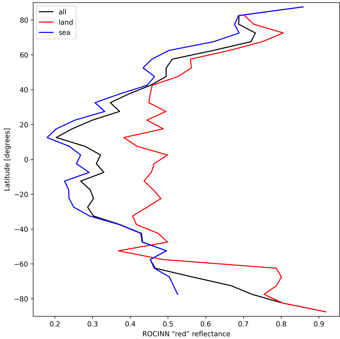
Figure 37: Zonal average of “ROCINN “red” reflectance” for 2025-03-17 to 2025-03-18.
