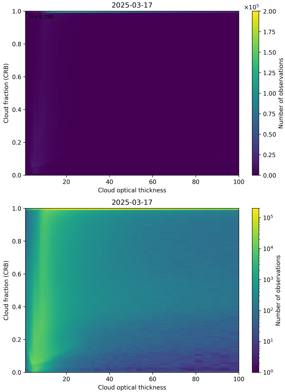
Figure 84: Scatter density plot of “Cloud optical thickness” against “Cloud fraction (CRB)” for 2025-03-17 to 2025-03-18.
