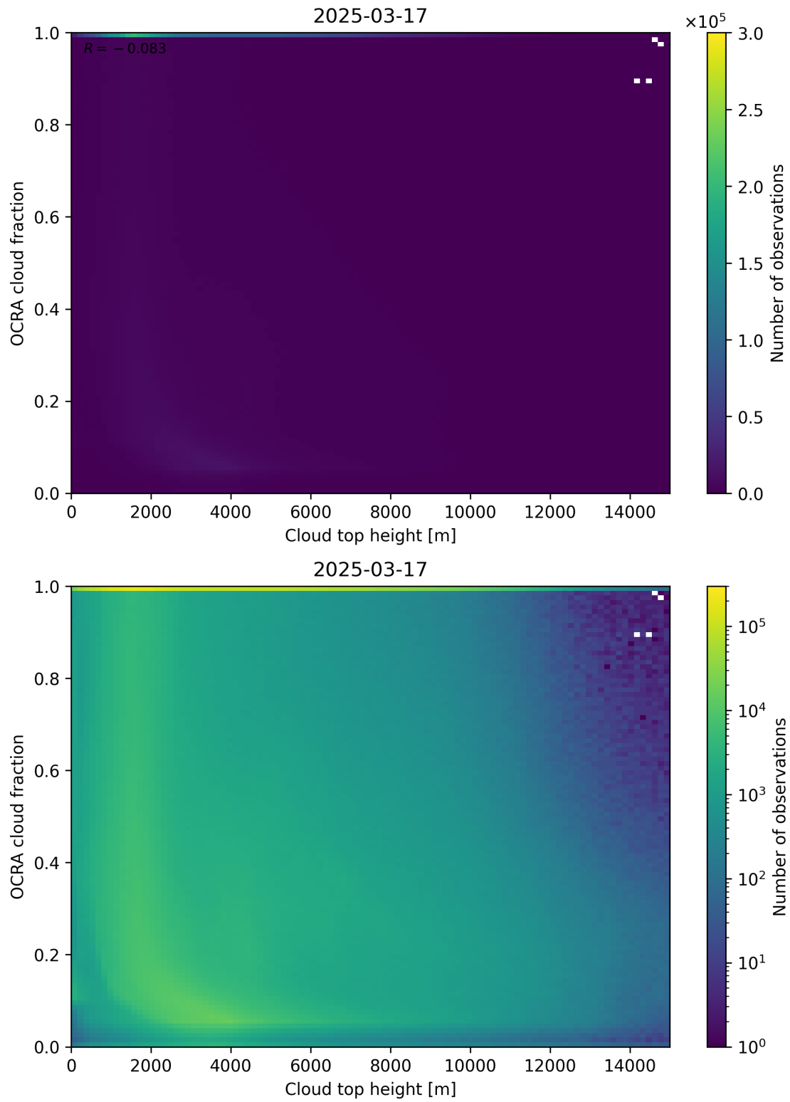
Figure 87: Scatter density plot of “Cloud top height” against “OCRA cloud fraction” for 2025-03-17 to 2025-03-18.
