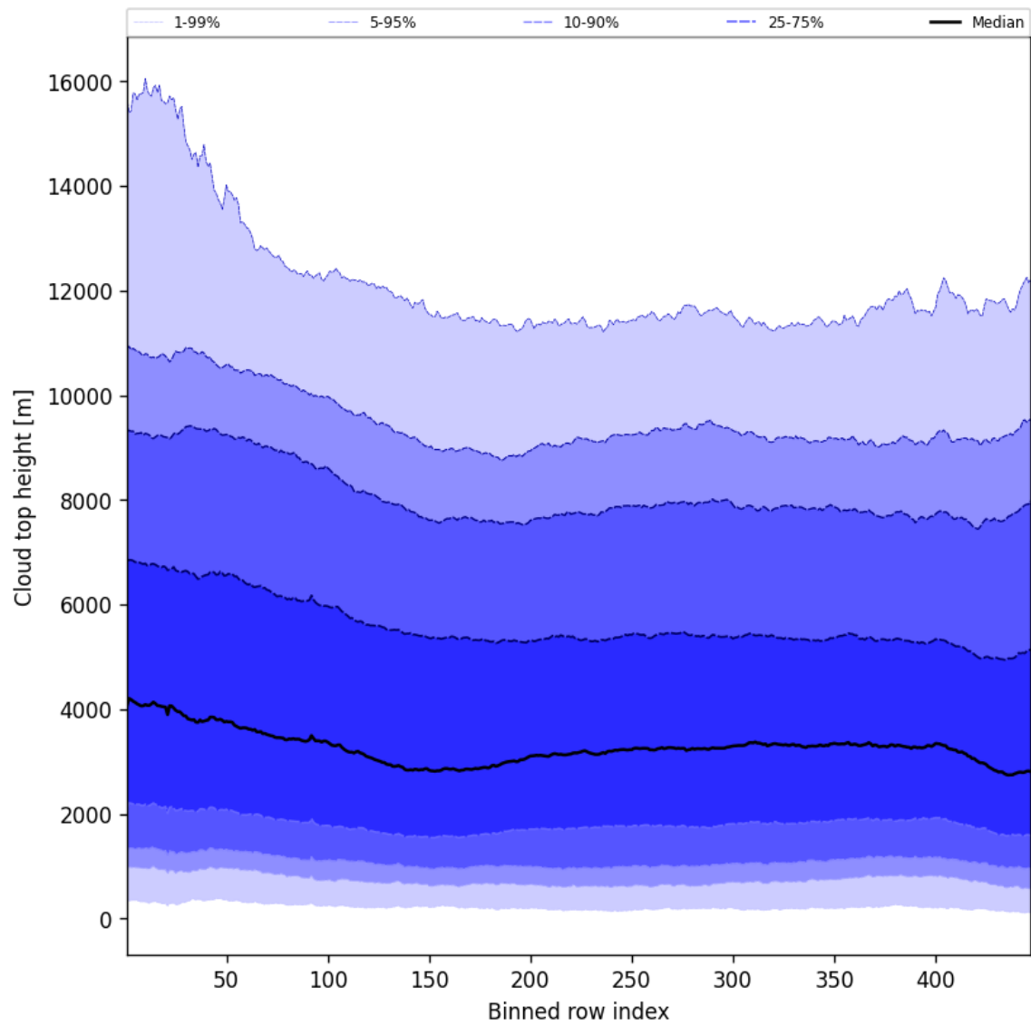
Figure 56: Along track statistics of “Cloud top height” for 2025-03-17 to 2025-03-18
