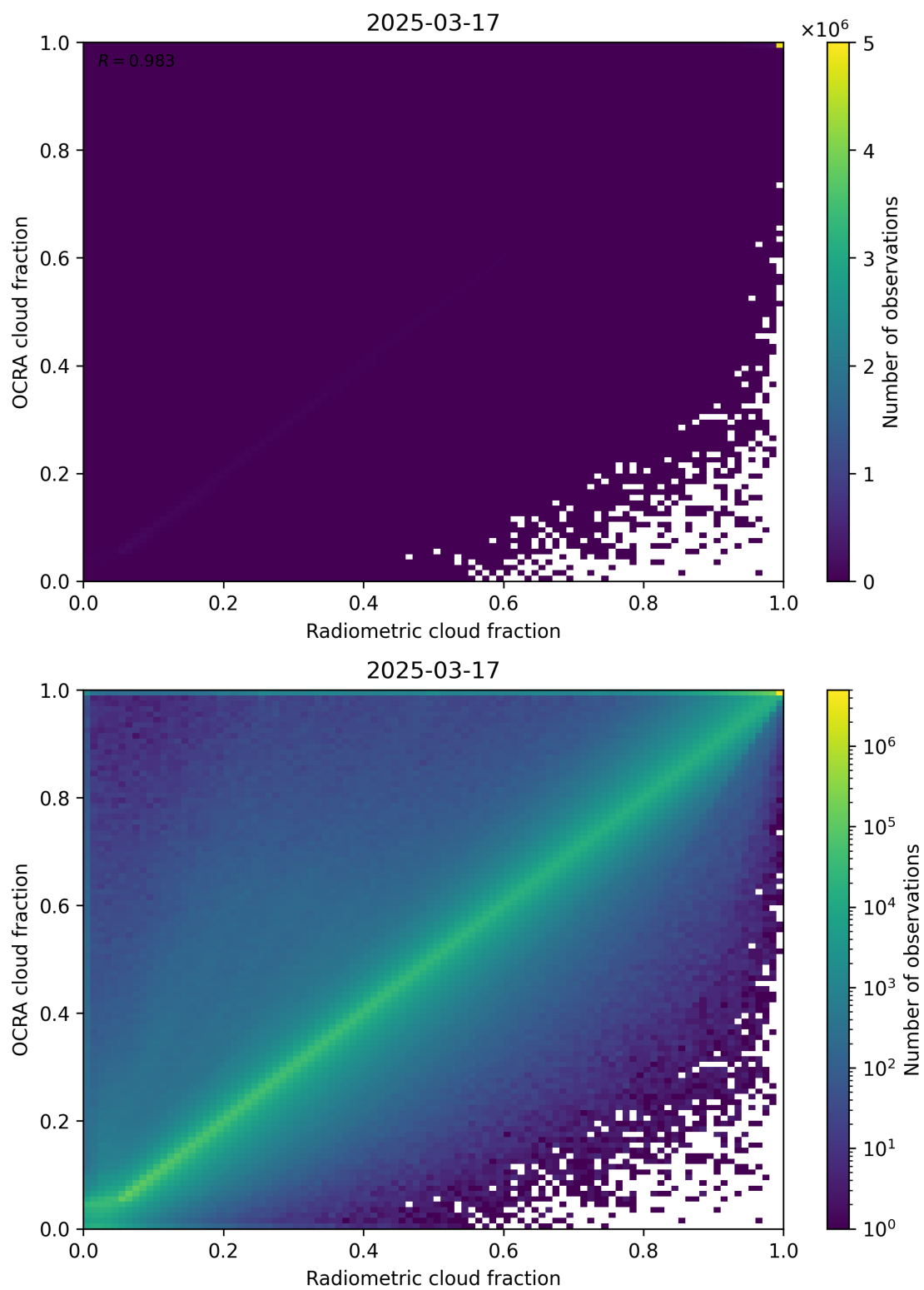
Figure 72: Scatter density plot of “Radiometric cloud fraction” against “OCRA cloud fraction” for 2025-03-17 to 2025-03-18.
