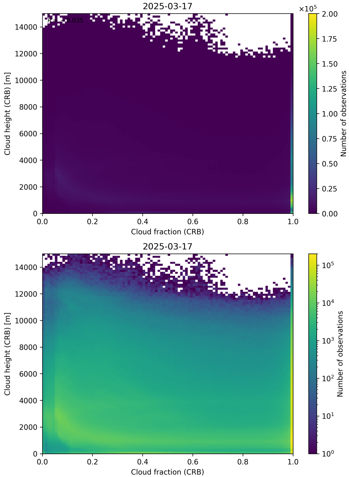
Figure 79: Scatter density plot of “Cloud fraction (CRB)” against “Cloud height (CRB)” for 2025-03-17 to 2025-03-18.
