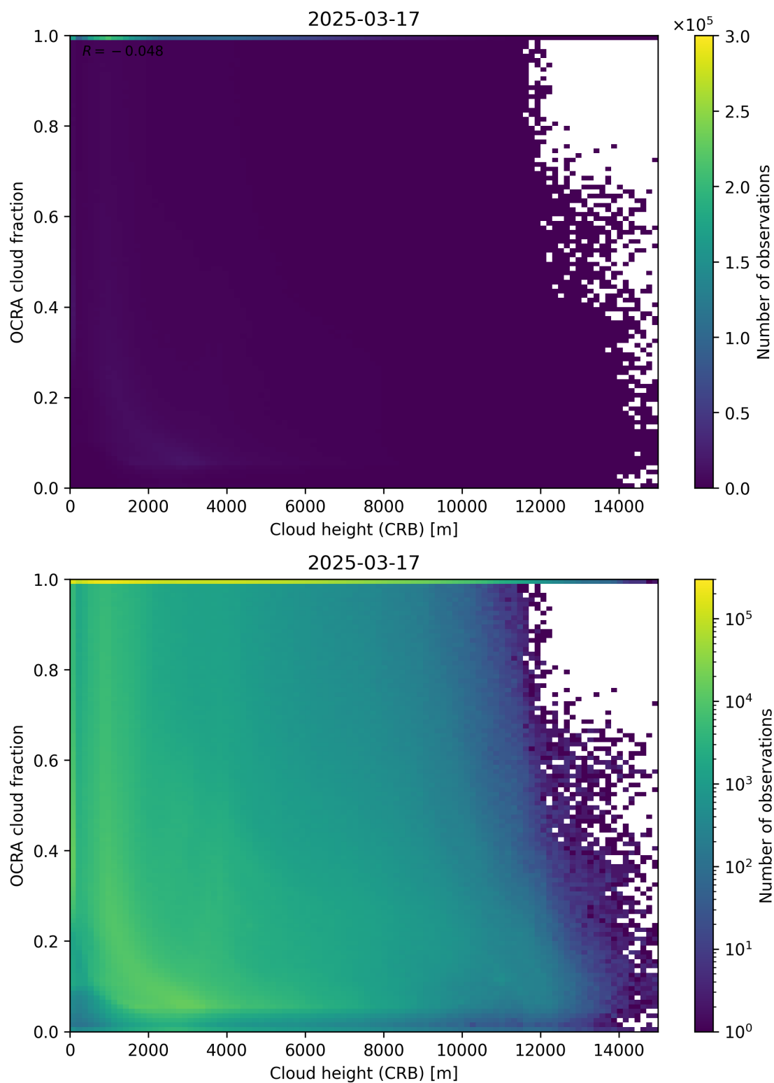
Figure 81: Scatter density plot of “Cloud height (CRB)” against “OCRA cloud fraction” for 2025-03-17 to 2025-03-18.
