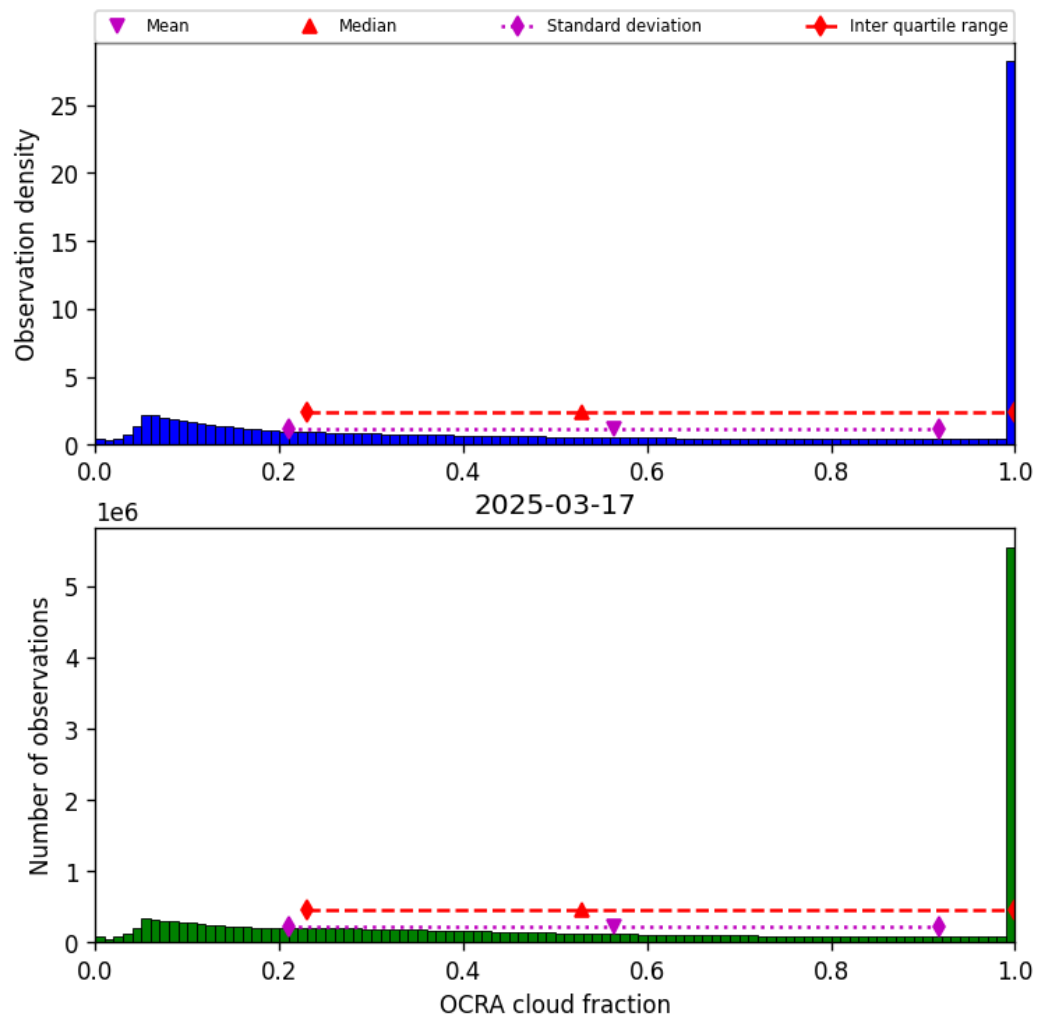
Figure 50: Histogram of “OCRA cloud fraction” for 2025-03-17 to 2025-03-18
