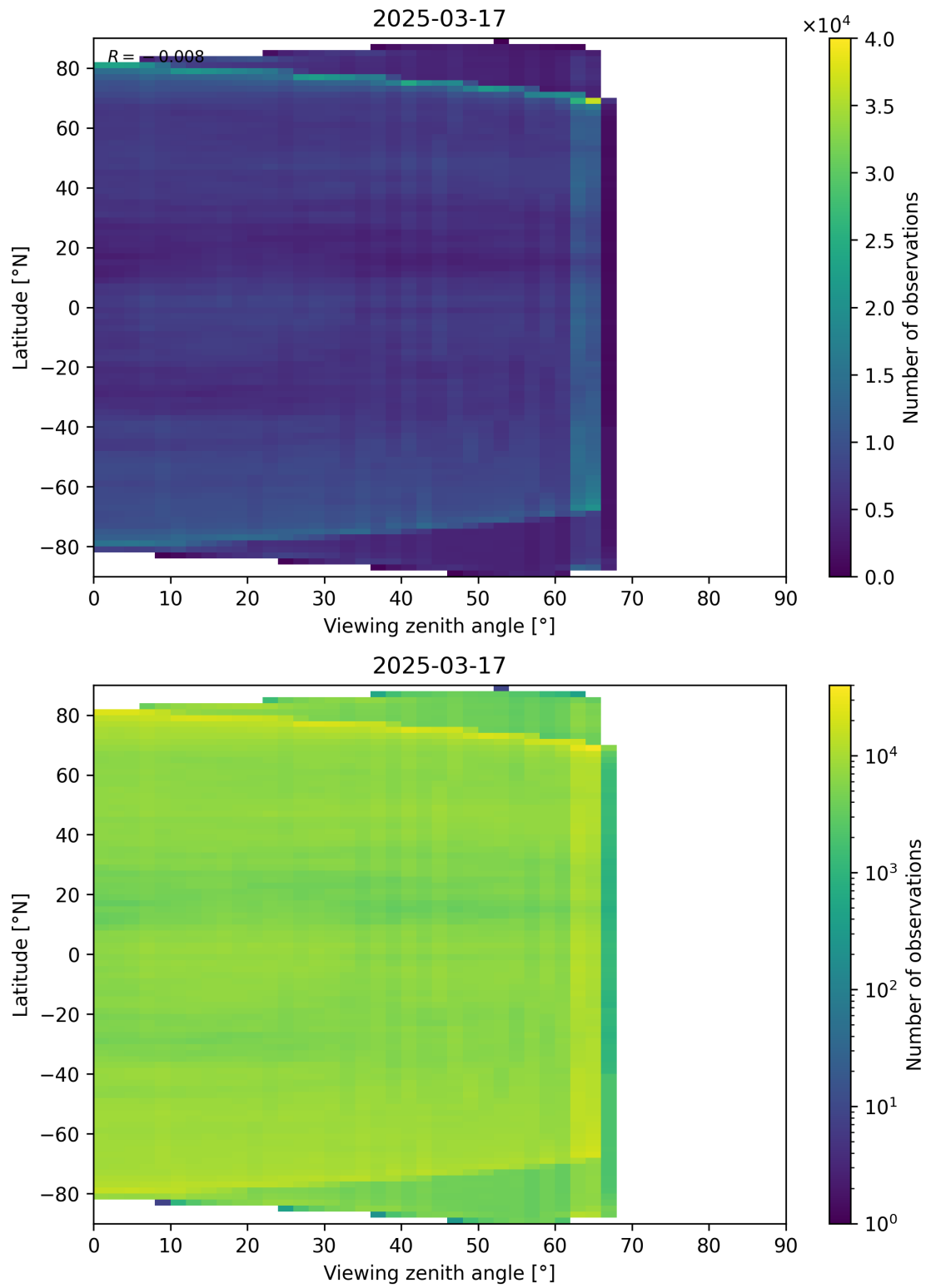
Figure 113: Scatter density plot of “Viewing zenith angle” against “Latitude” for 2025-03-17 to 2025-03-18.
