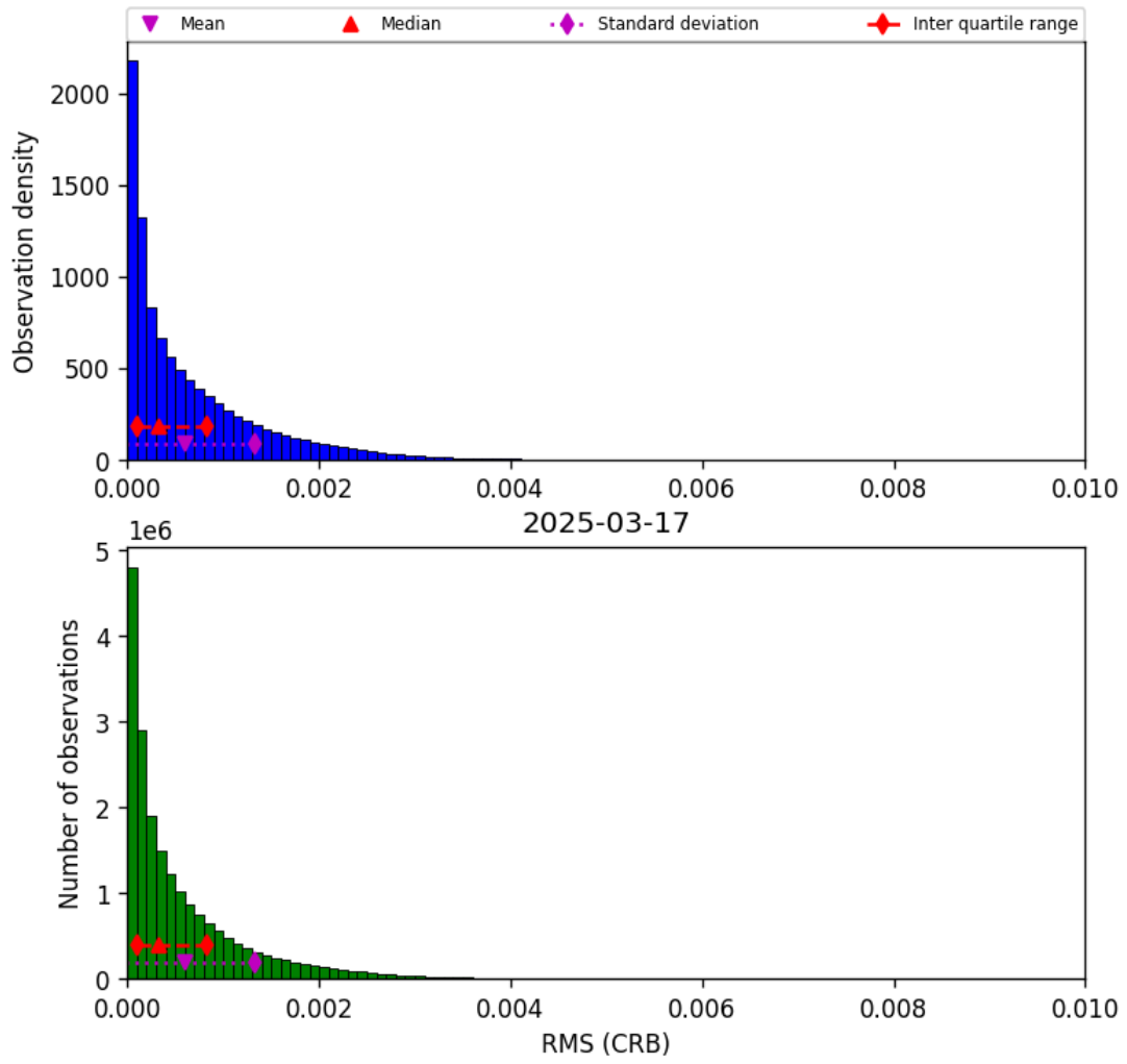
Figure 48: Histogram of “RMS (CRB)” for 2025-03-17 to 2025-03-18
