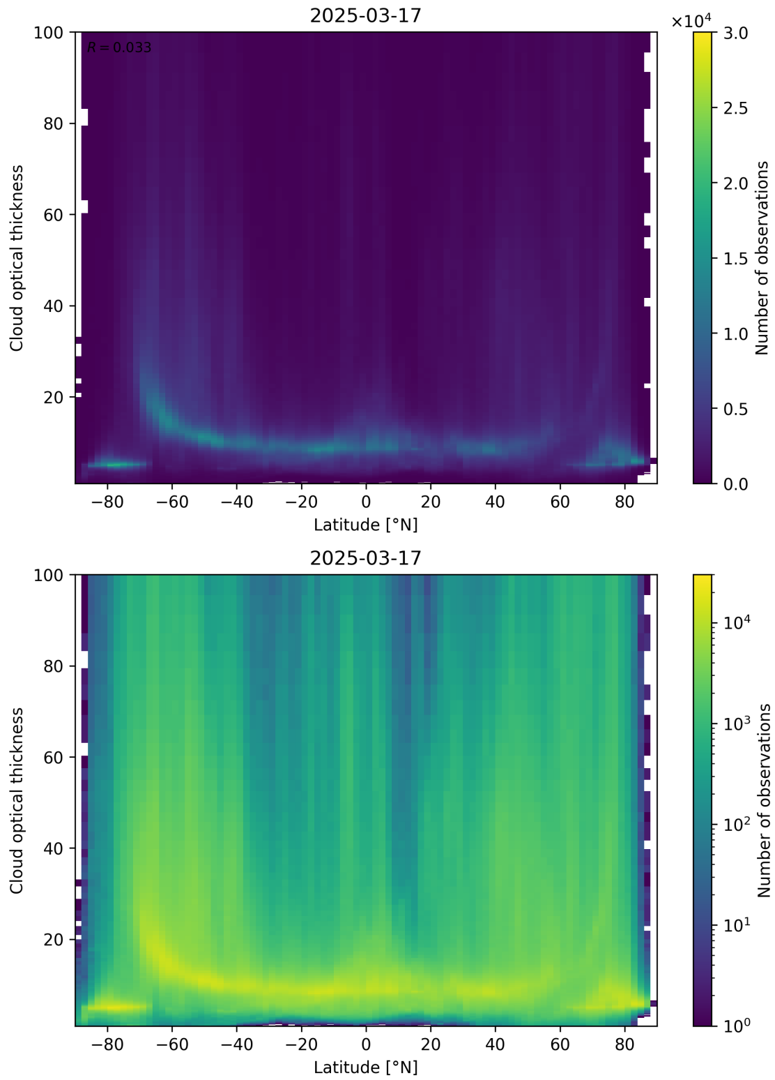
Figure 96: Scatter density plot of “Latitude” against “Cloud optical thickness” for 2025-03-17 to 2025-03-18.
