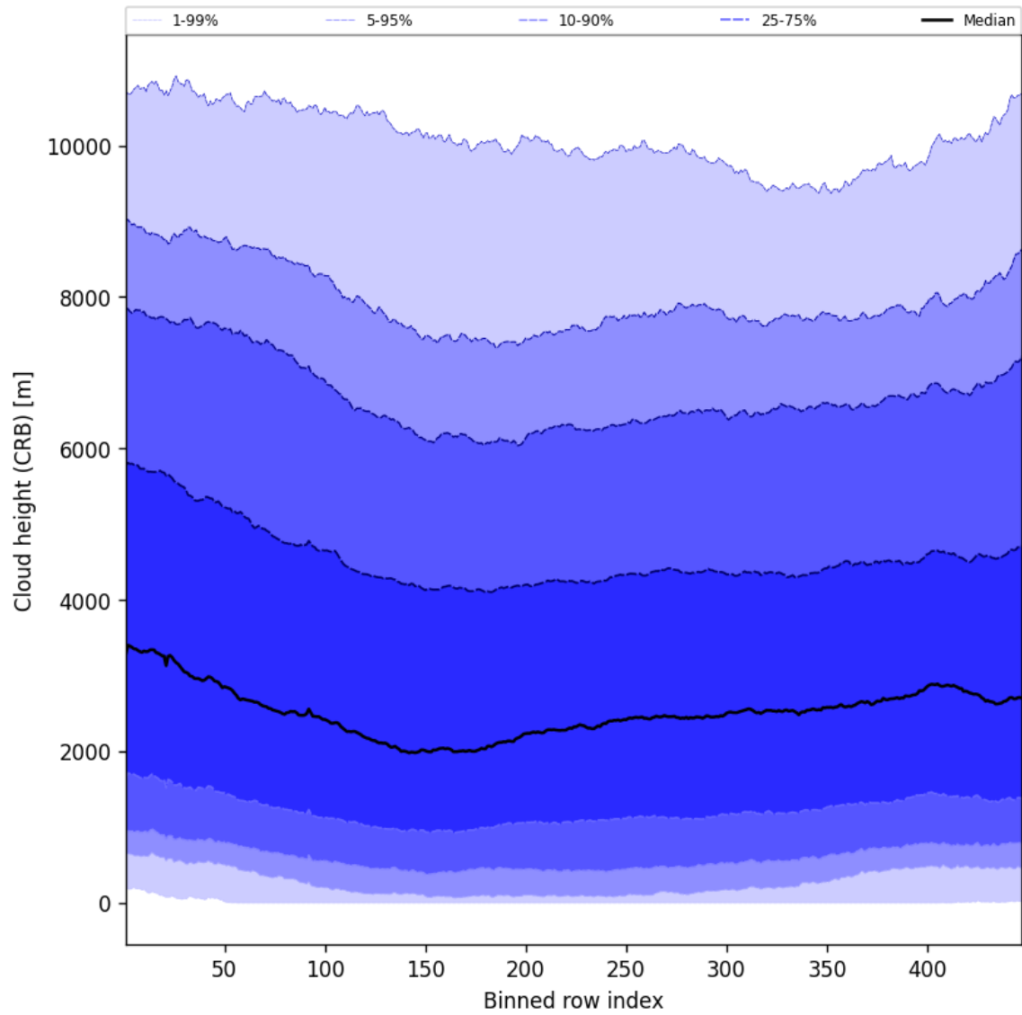
Figure 59: Along track statistics of “Cloud height (CRB)” for 2025-03-17 to 2025-03-18
