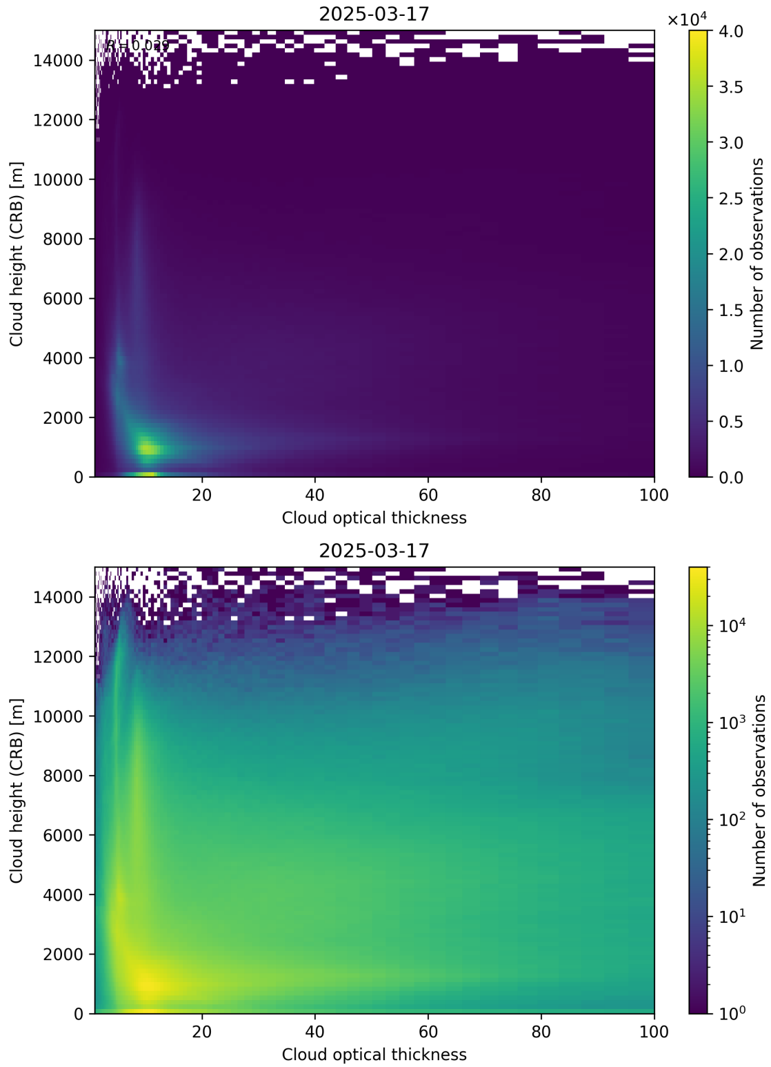
Figure 85: Scatter density plot of “Cloud optical thickness” against “Cloud height (CRB)” for 2025-03-17 to 2025-03-18.
