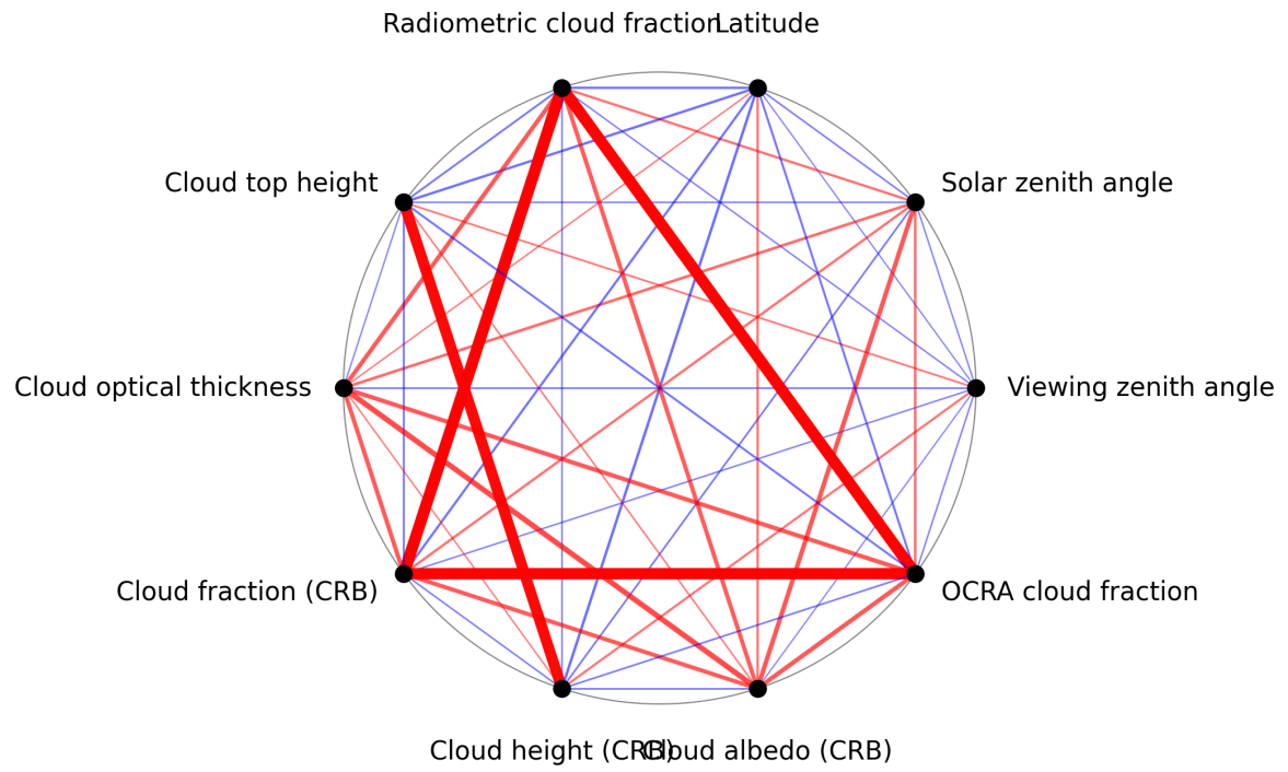
Figure 1: Map of correlation graph for 2025-03-17 to 2025-03-18.
