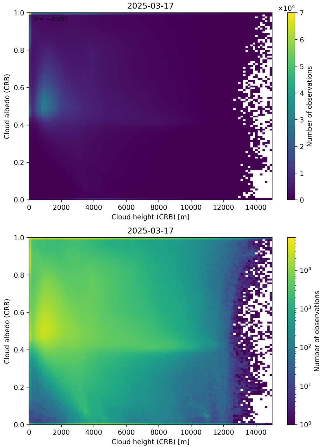
Figure 80: Scatter density plot of “Cloud height (CRB)” against “Cloud albedo (CRB)” for 2025-03-17 to 2025-03-18.
