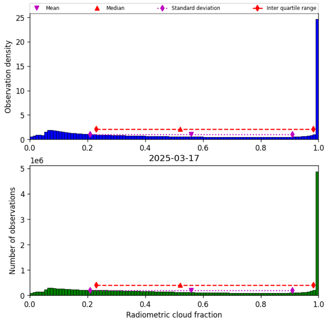
Figure 39: Histogram of “Radiometric cloud fraction” for 2025-03-17 to 2025-03-18
