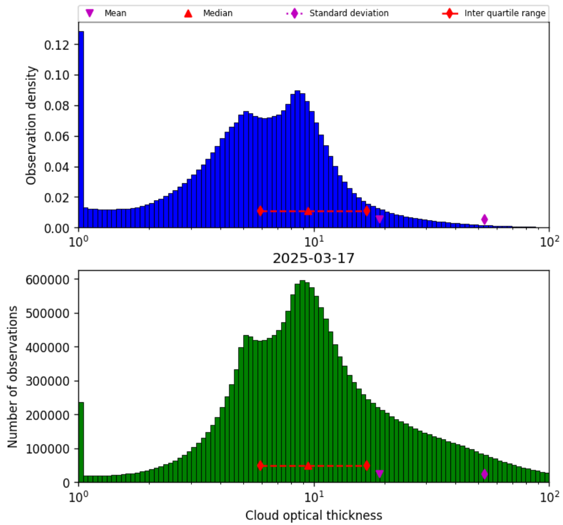
Figure 41: Histogram of “Cloud optical thickness” for 2025-03-17 to 2025-03-18
