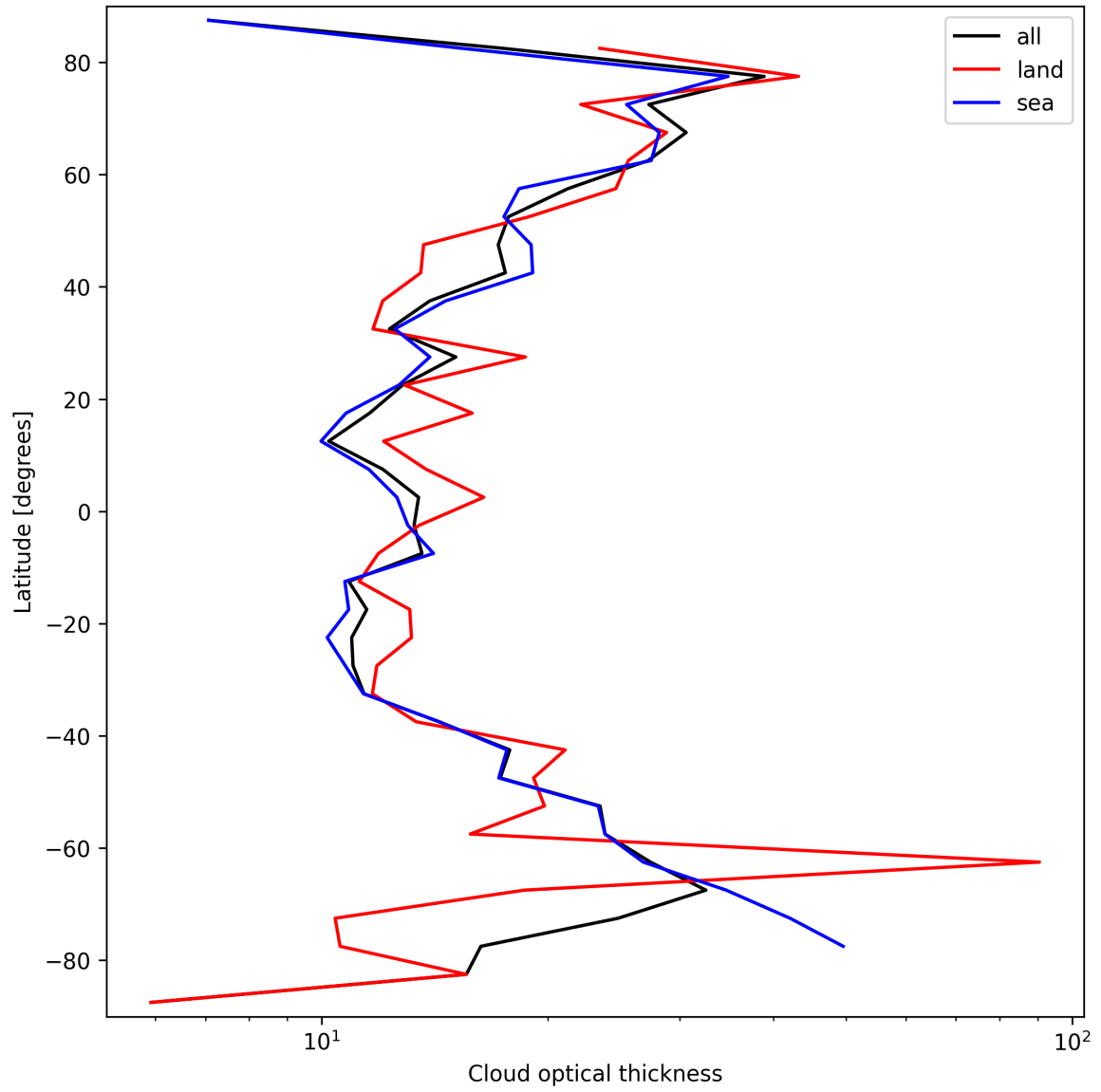
Figure 25: Zonal average of “Cloud optical thickness” for 2025-03-17 to 2025-03-18.
