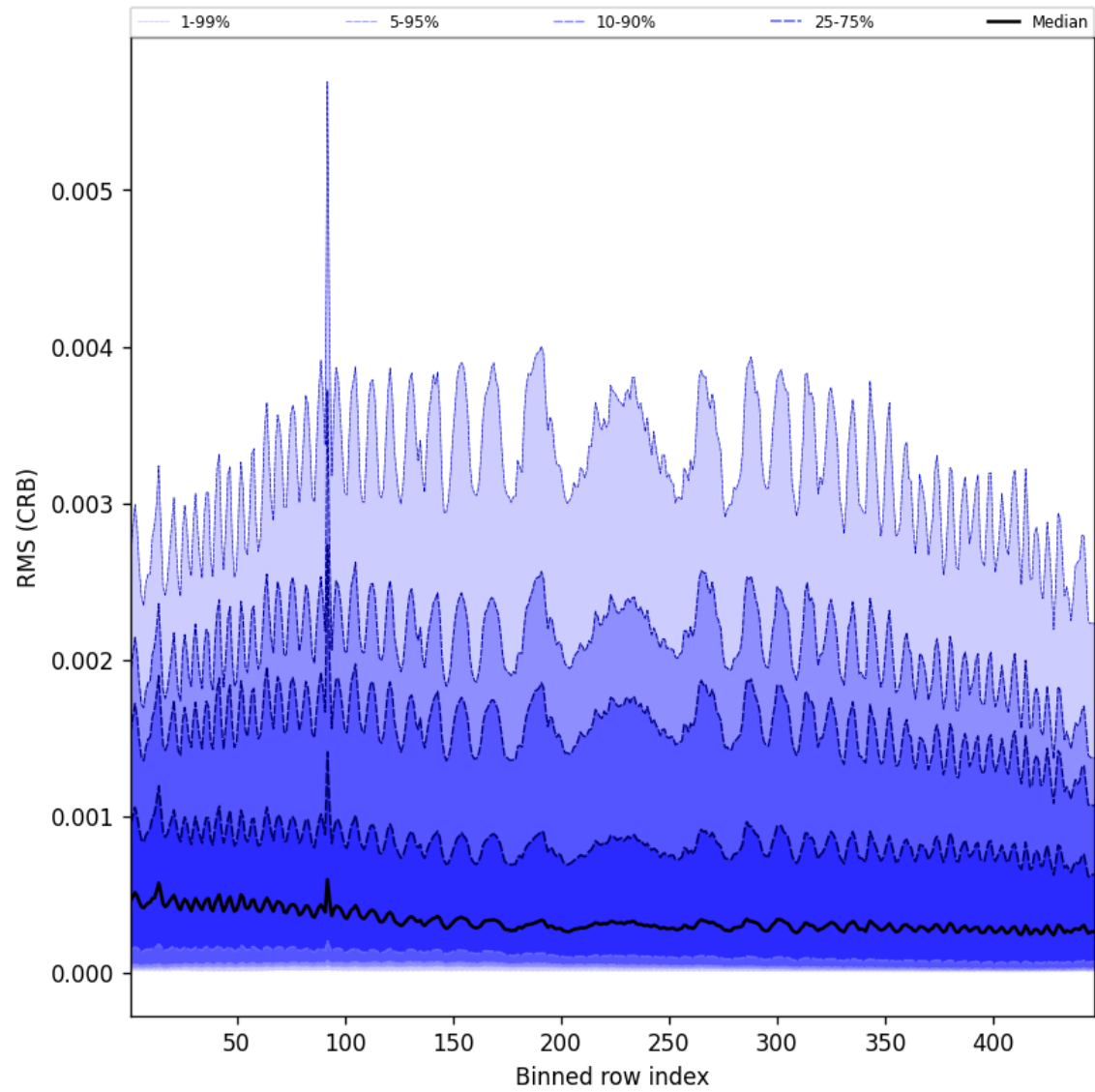
Figure 64: Along track statistics of “RMS (CRB)” for 2025-03-17 to 2025-03-18
