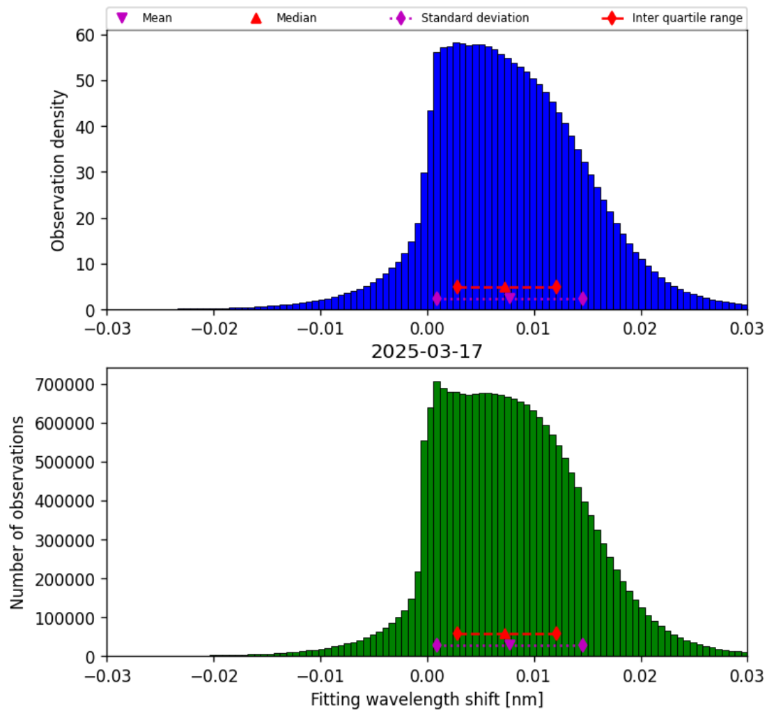
Figure 49: Histogram of “Fitting wavelength shift” for 2025-03-17 to 2025-03-18
