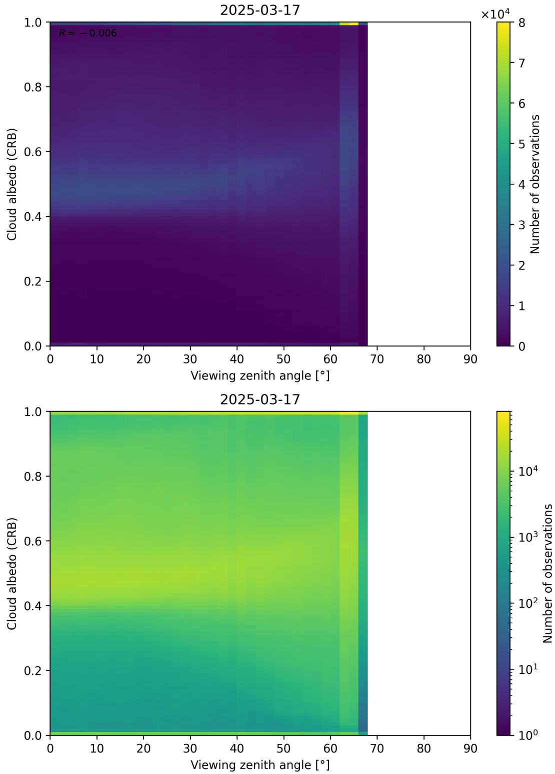
Figure 106: Scatter density plot of “Viewing zenith angle” against “Cloud albedo (CRB)” for 2025-03-17 to 2025-03-18.
