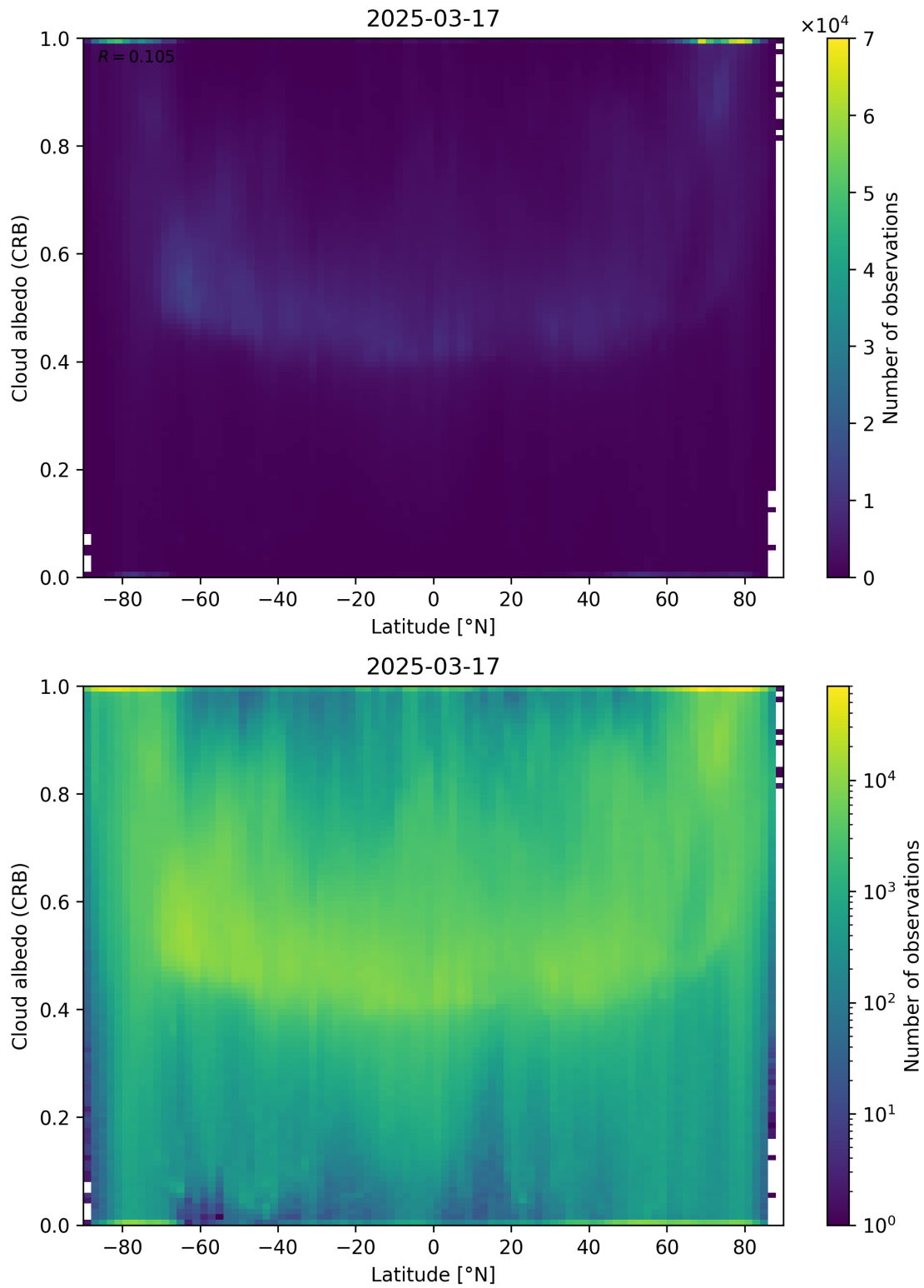
Figure 91: Scatter density plot of “Latitude” against “Cloud albedo (CRB)” for 2025-03-17 to 2025-03-18.
