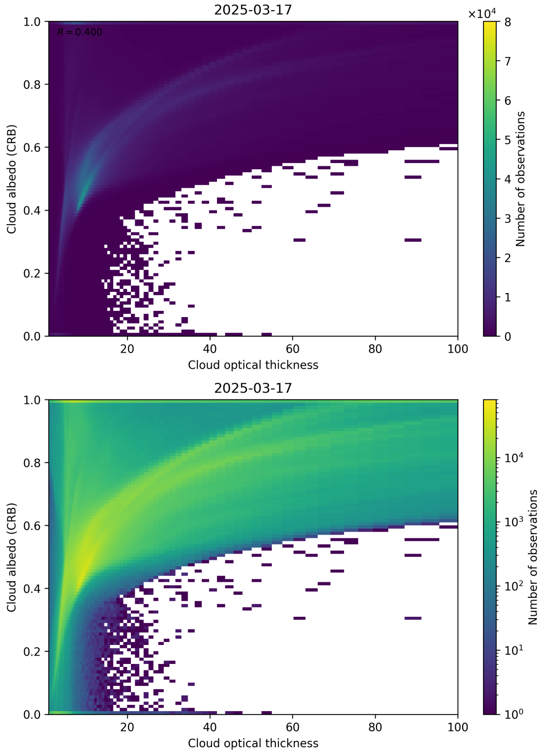
Figure 82: Scatter density plot of “Cloud optical thickness” against “Cloud albedo (CRB)” for 2025-03-17 to 2025-03-18.
