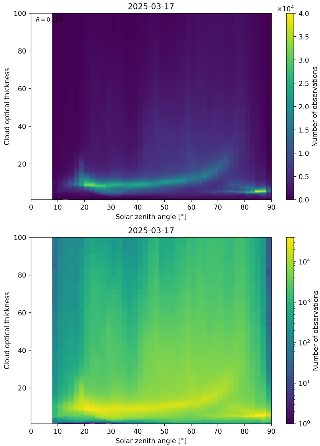
Figure 103: Scatter density plot of “Solar zenith angle” against “Cloud optical thickness” for 2025-03-17 to 2025-03-18.
