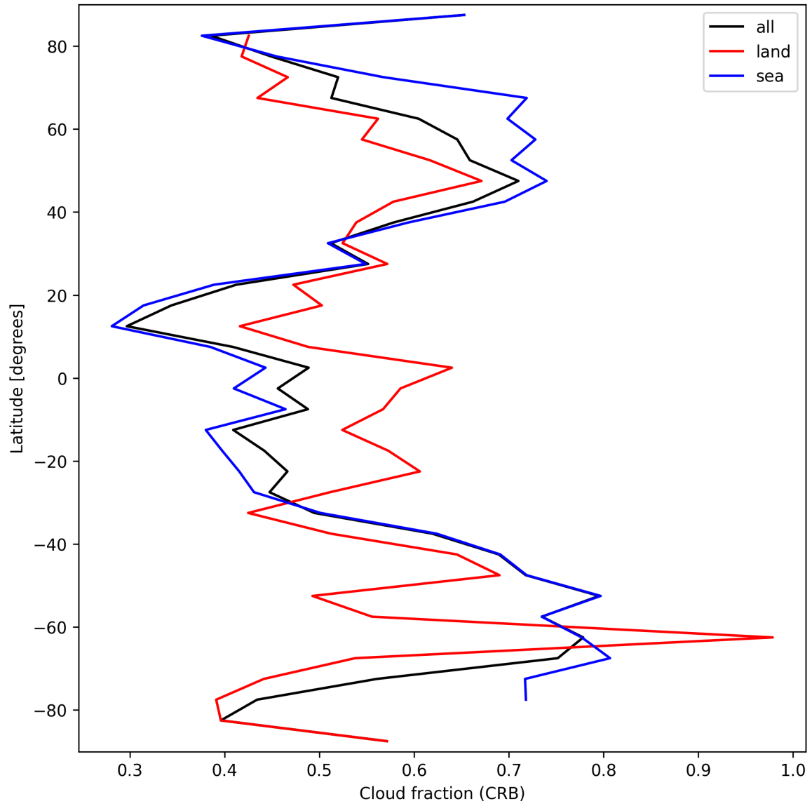
Figure 26: Zonal average of “Cloud fraction (CRB)” for 2025-03-17 to 2025-03-18.
