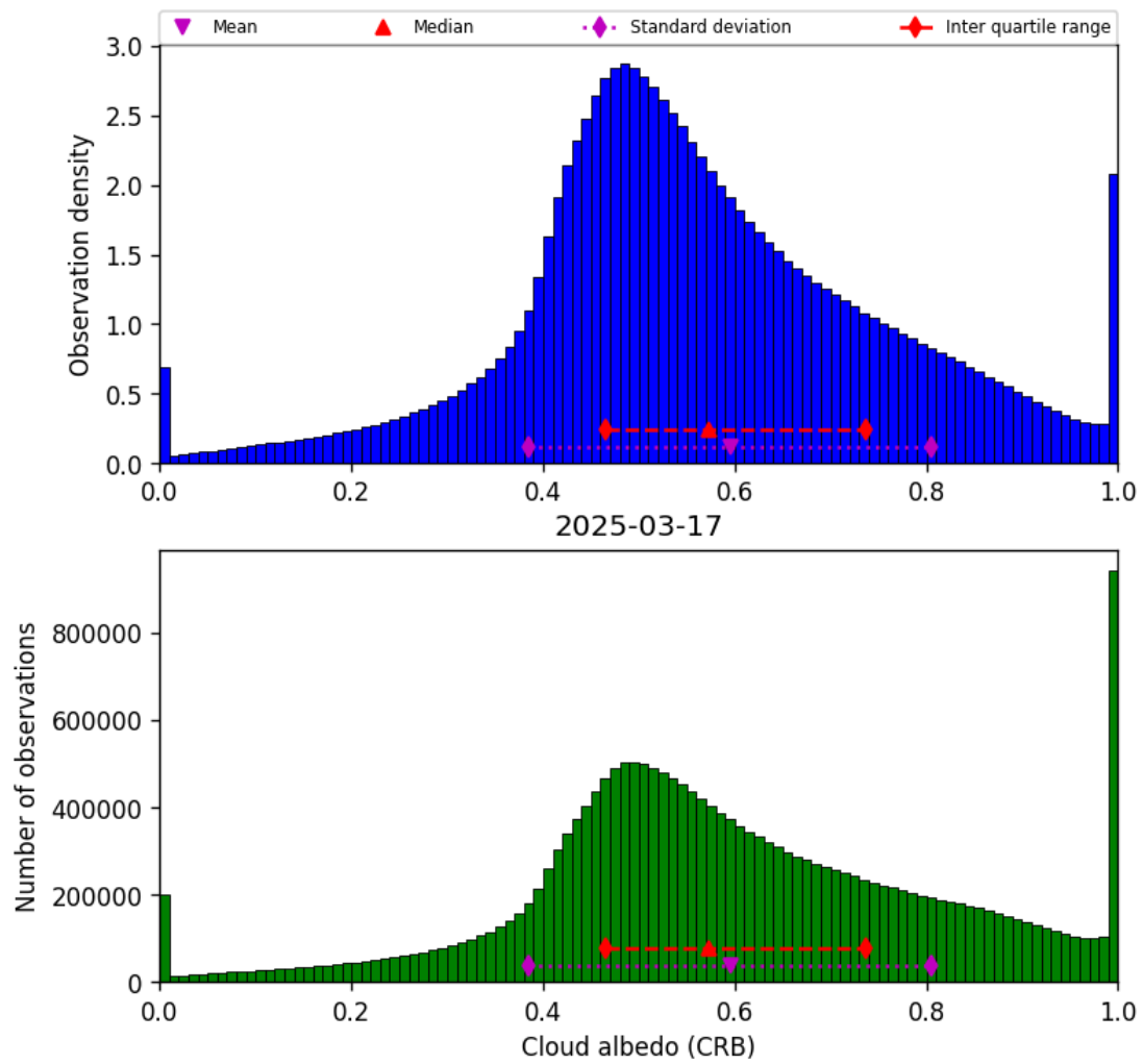
Figure 44: Histogram of “Cloud albedo (CRB)” for 2025-03-17 to 2025-03-18
