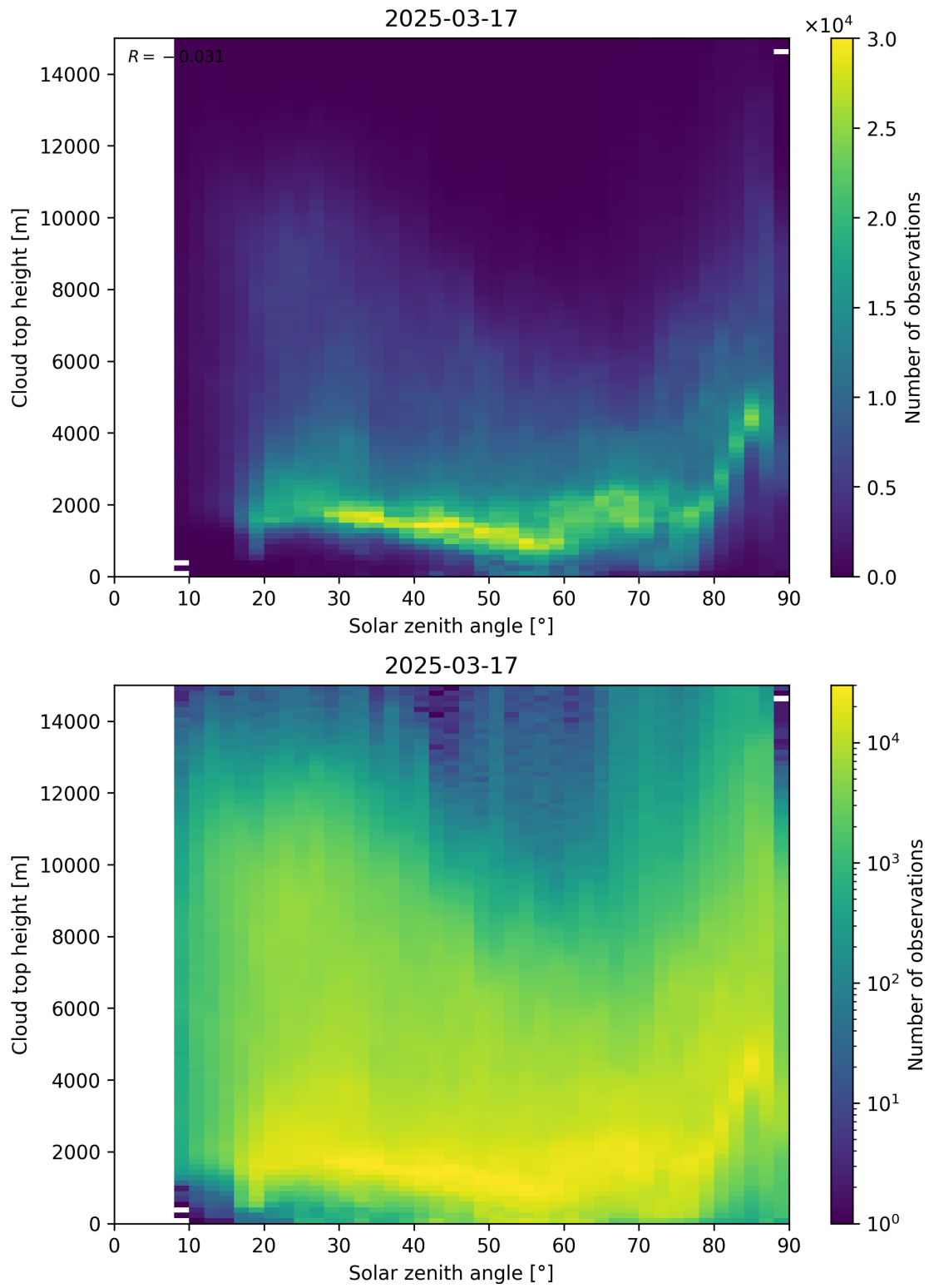
Figure 104: Scatter density plot of “Solar zenith angle” against “Cloud top height” for 2025-03-17 to 2025-03-18.
