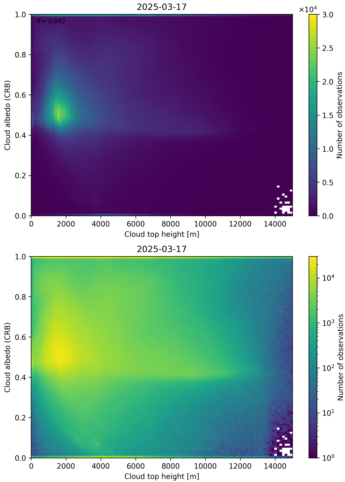
Figure 86: Scatter density plot of “Cloud top height” against “Cloud albedo (CRB)” for 2025-03-17 to 2025-03-18.
