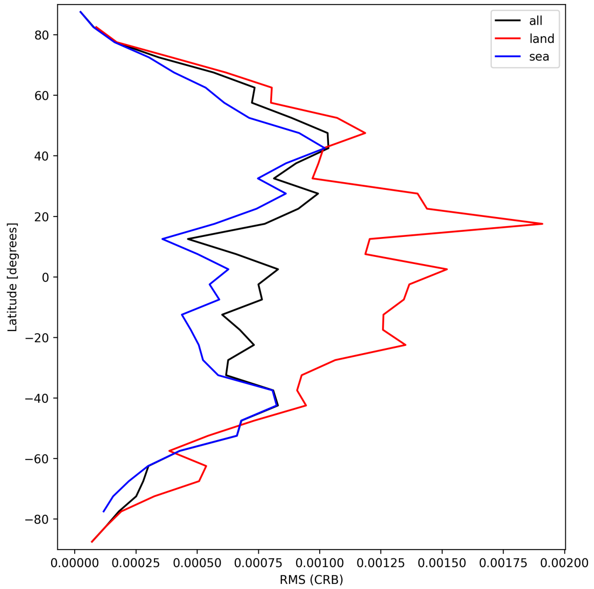
Figure 32: Zonal average of “RMS (CRB)” for 2025-03-17 to 2025-03-18.
