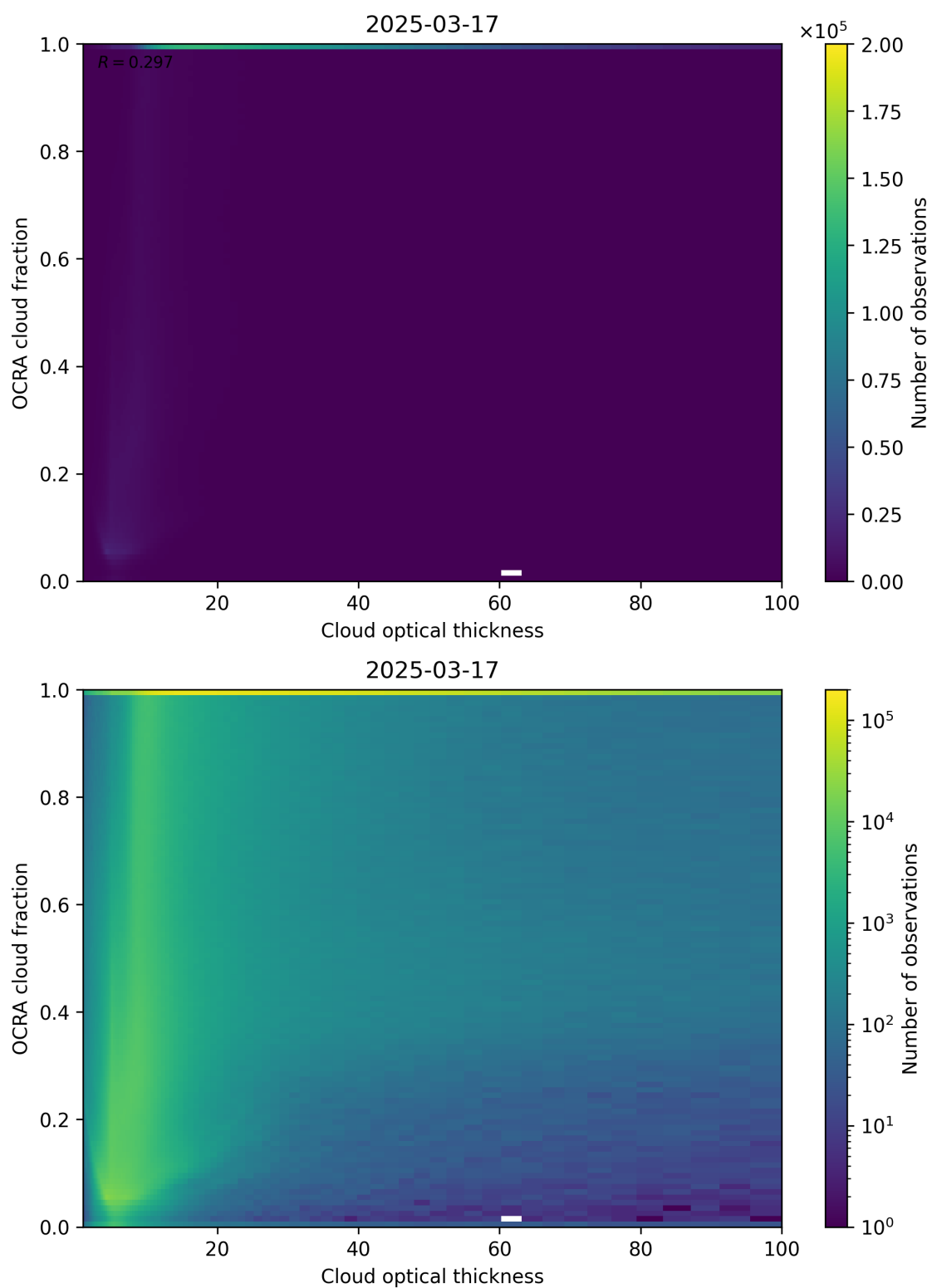
Figure 83: Scatter density plot of “Cloud optical thickness” against “OCRA cloud fraction” for 2025-03-17 to 2025-03-18.
