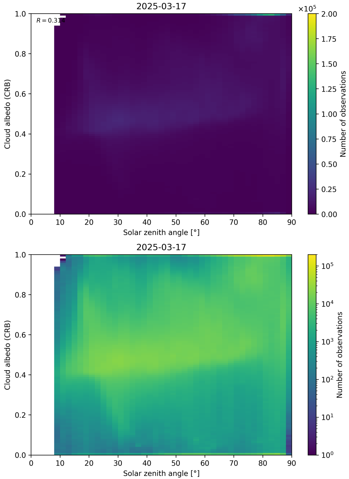
Figure 98: Scatter density plot of “Solar zenith angle” against “Cloud albedo (CRB)” for 2025-03-17 to 2025-03-18.
