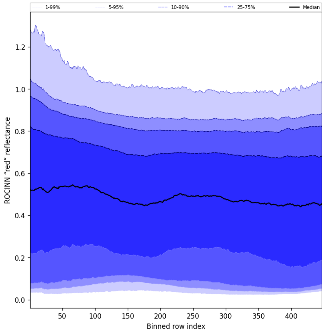
Figure 69: Along track statistics of “ROCINN “red” reflectance” for 2025-03-17 to 2025-03-18
