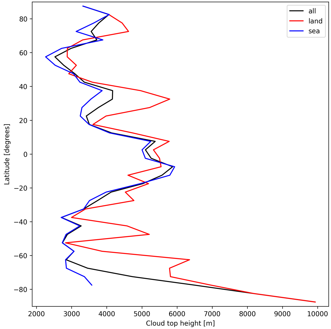
Figure 24: Zonal average of “Cloud top height” for 2025-03-17 to 2025-03-18.
