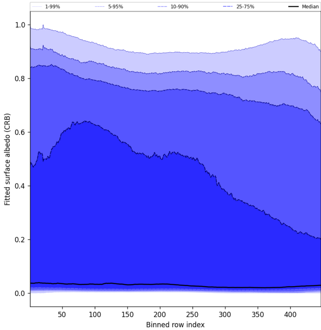
Figure 62: Along track statistics of “Fitted surface albedo (CRB)” for 2025-03-17 to 2025-03-18
