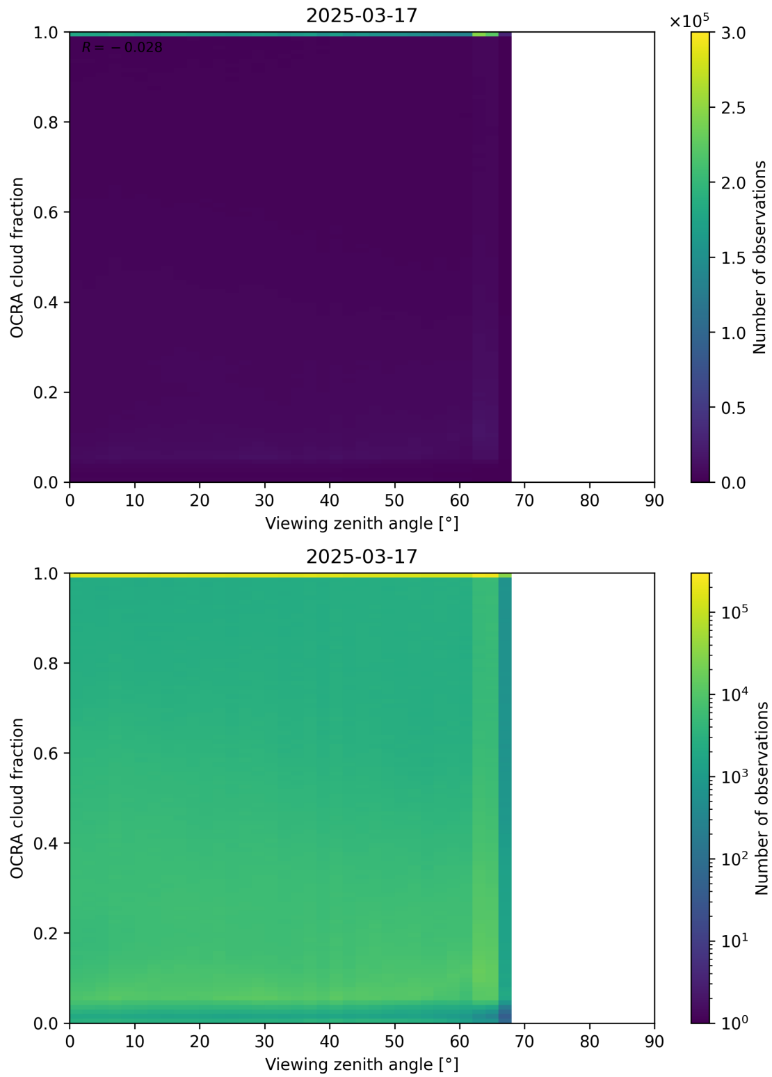
Figure 108: Scatter density plot of “Viewing zenith angle” against “OCRA cloud fraction” for 2025-03-17 to 2025-03-18.
