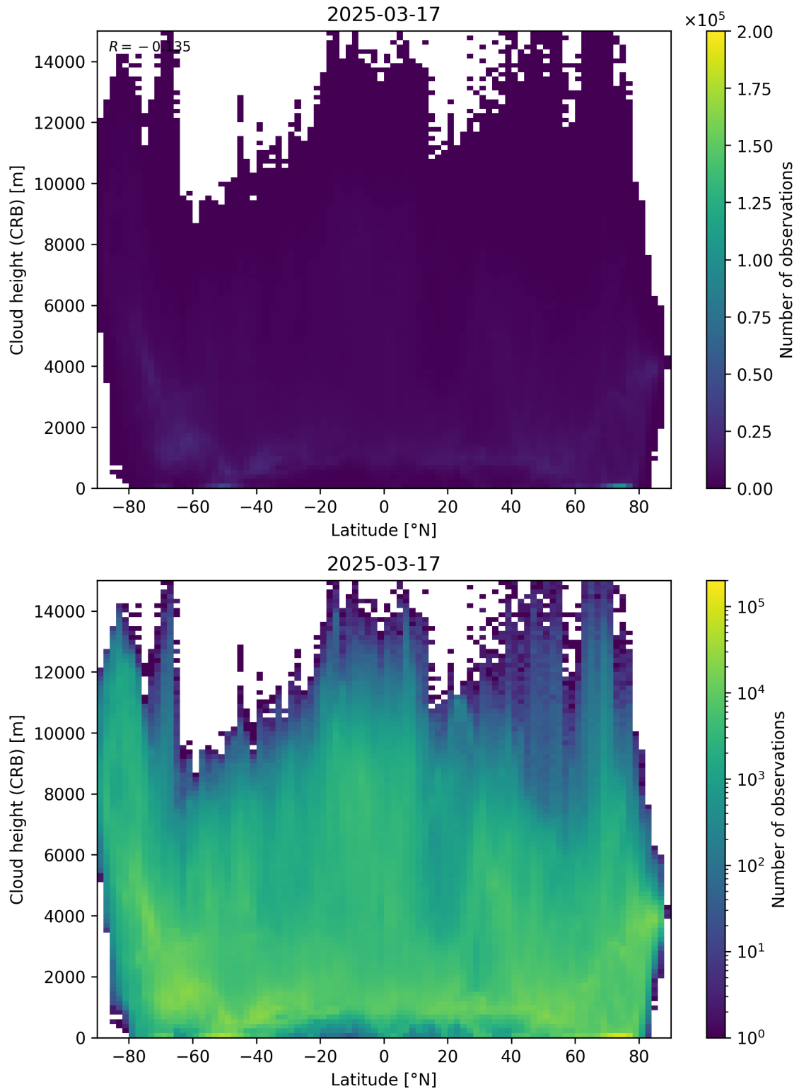
Figure 95: Scatter density plot of “Latitude” against “Cloud height (CRB)” for 2025-03-17 to 2025-03-18.
