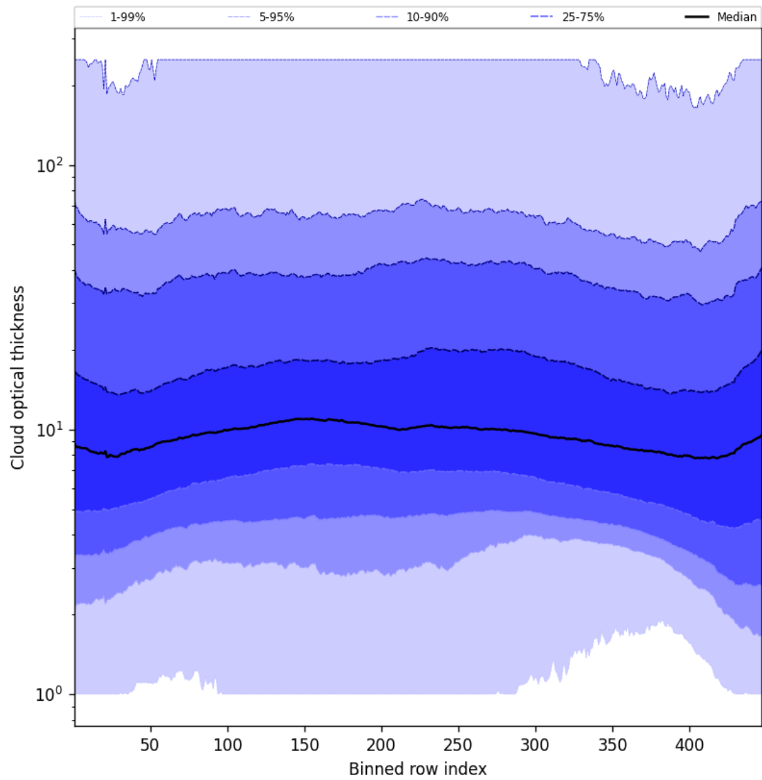
Figure 57: Along track statistics of “Cloud optical thickness” for 2025-03-17 to 2025-03-18
