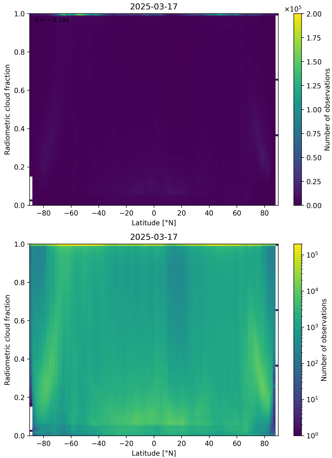
Figure 92: Scatter density plot of “Latitude” against “Radiometric cloud fraction” for 2025-03-17 to 2025-03-18.
