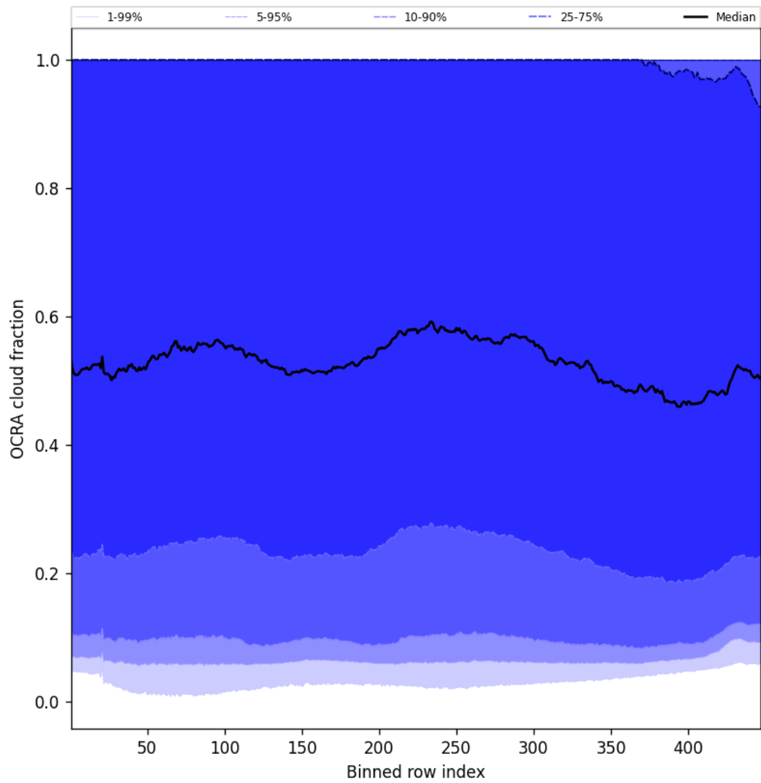
Figure 66: Along track statistics of “OCRA cloud fraction” for 2025-03-17 to 2025-03-18
