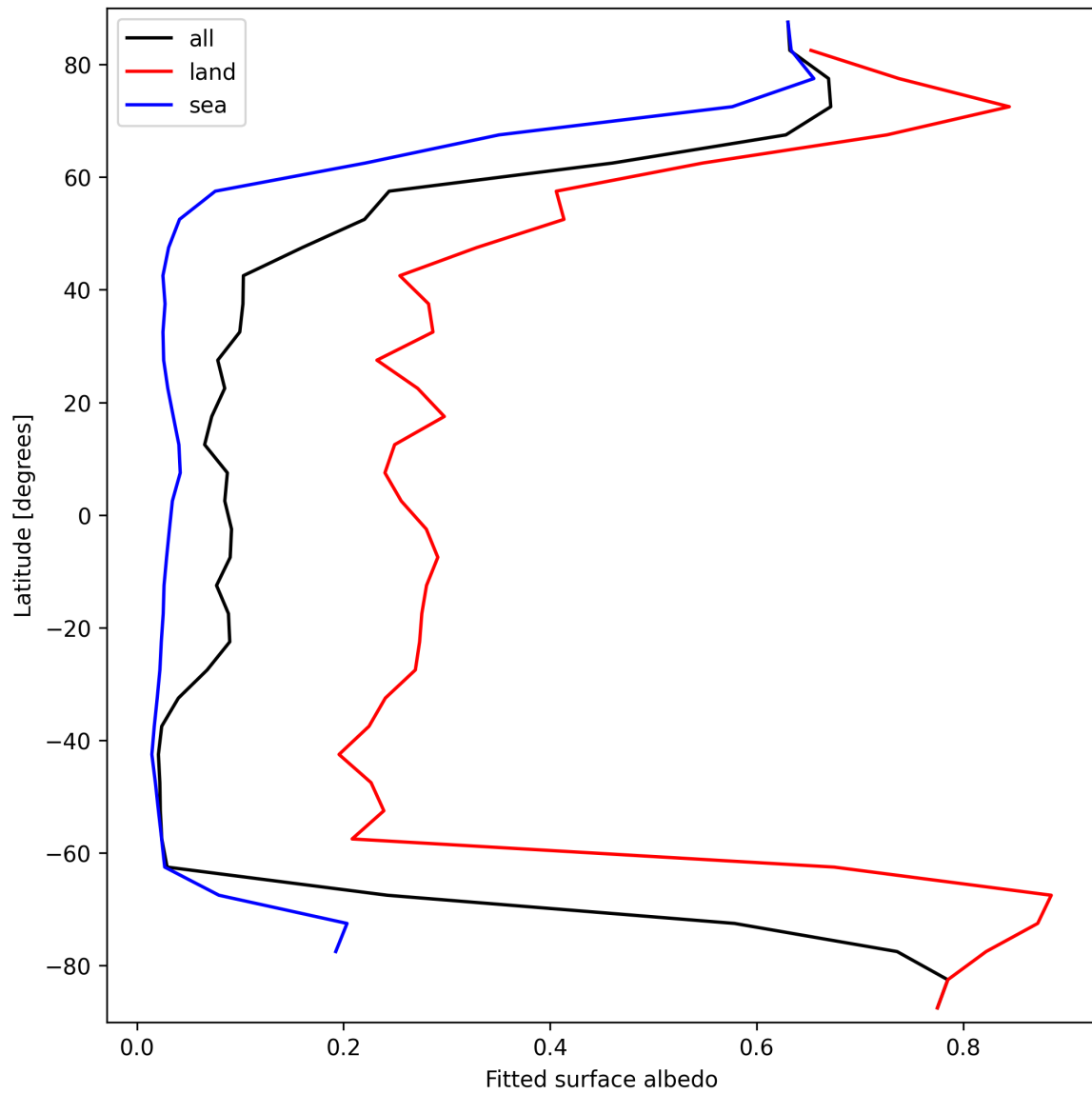
Figure 29: Zonal average of “Fitted surface albedo” for 2025-03-17 to 2025-03-18.
