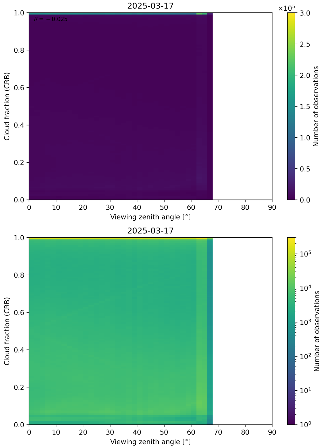
Figure 109: Scatter density plot of “Viewing zenith angle” against “Cloud fraction (CRB)” for 2025-03-17 to 2025-03-18.
