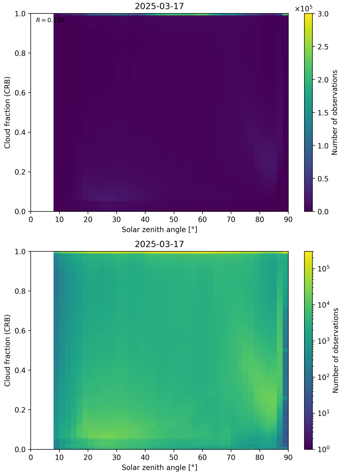
Figure 101: Scatter density plot of “Solar zenith angle” against “Cloud fraction (CRB)” for 2025-03-17 to 2025-03-18.
