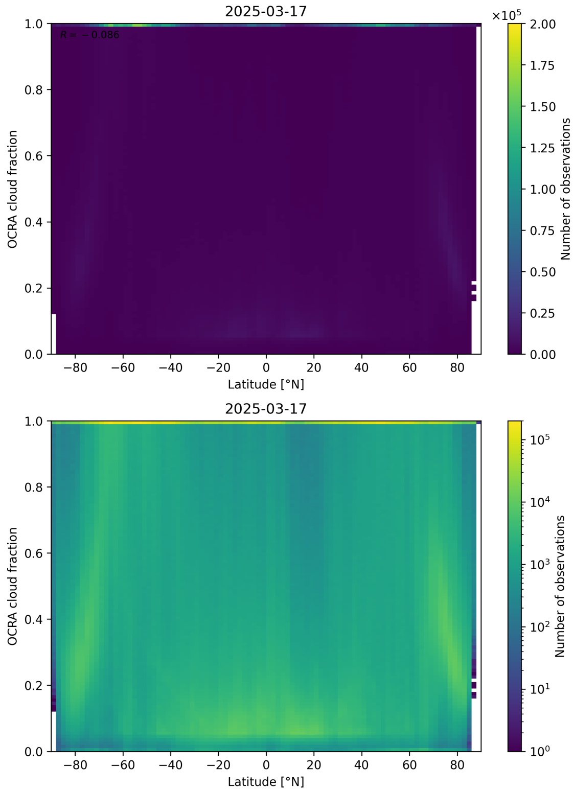
Figure 93: Scatter density plot of “Latitude” against “OCRA cloud fraction” for 2025-03-17 to 2025-03-18.
