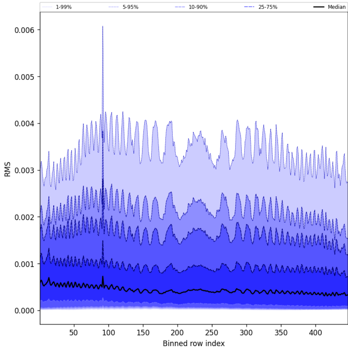
Figure 63: Along track statistics of “RMS” for 2025-03-17 to 2025-03-18
