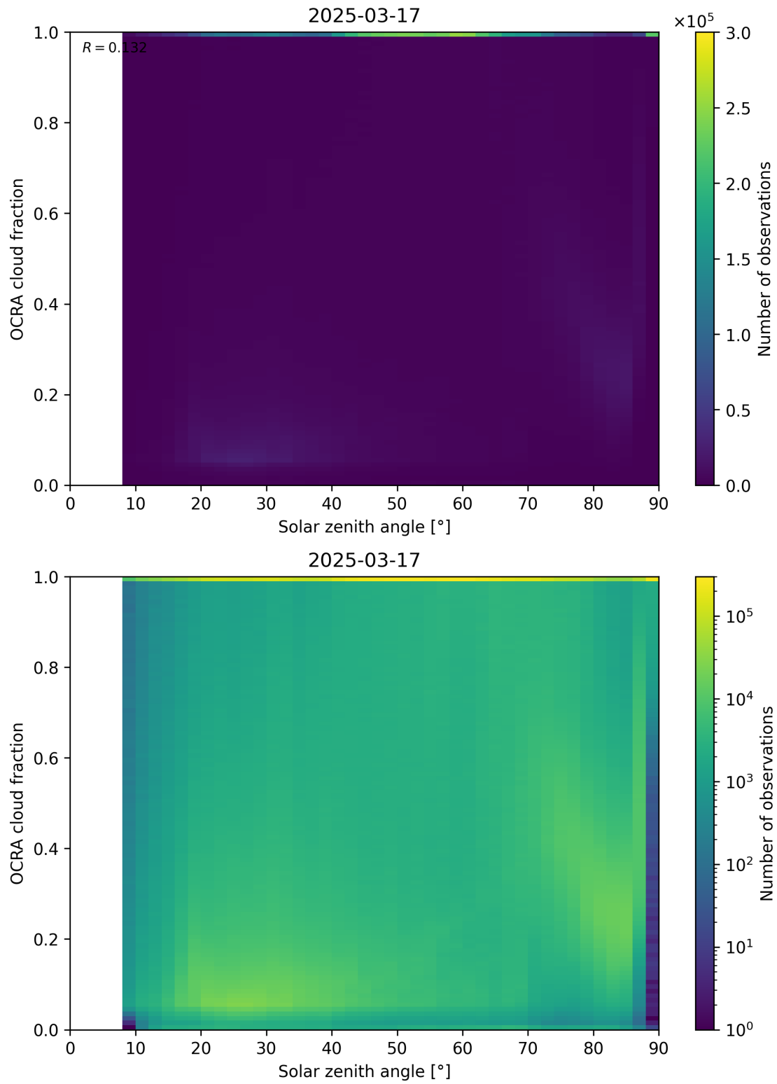
Figure 100: Scatter density plot of “Solar zenith angle” against “OCRA cloud fraction” for 2025-03-17 to 2025-03-18.
