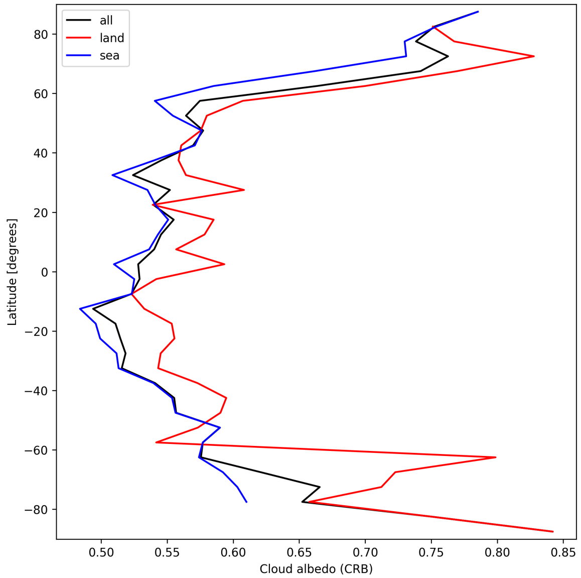
Figure 28: Zonal average of “Cloud albedo (CRB)” for 2025-03-17 to 2025-03-18.
