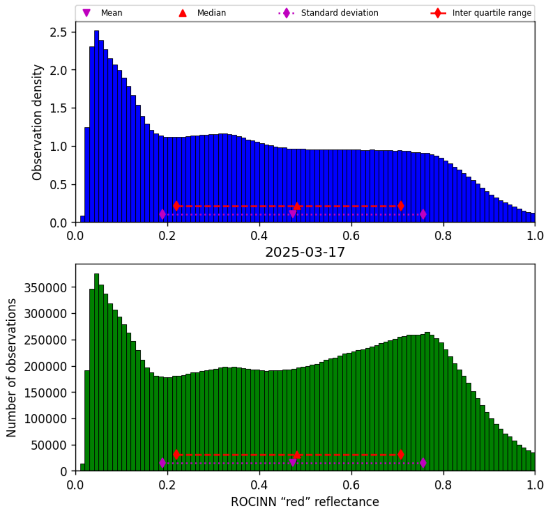
Figure 53: Histogram of “ROCINN “red” reflectance” for 2025-03-17 to 2025-03-18
