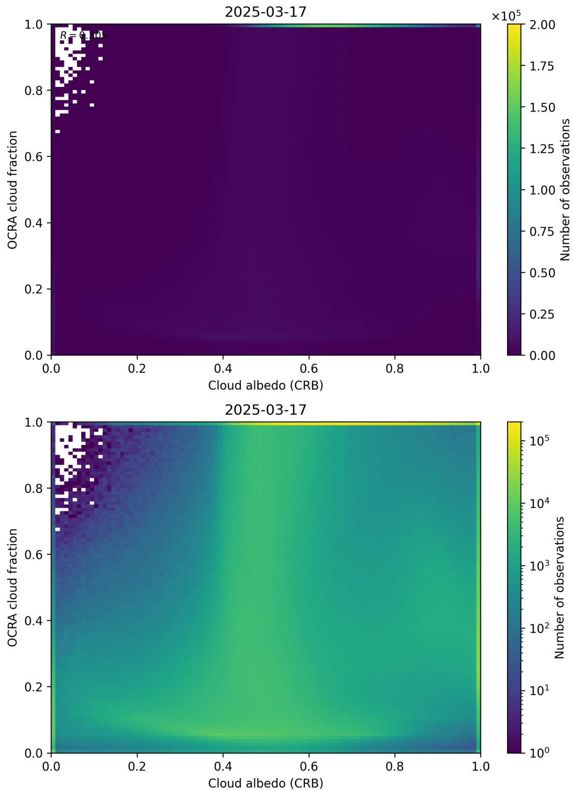
Figure 70: Scatter density plot of “Cloud albedo (CRB)” against “OCRA cloud fraction” for 2025-03-17 to 2025-03-18.
