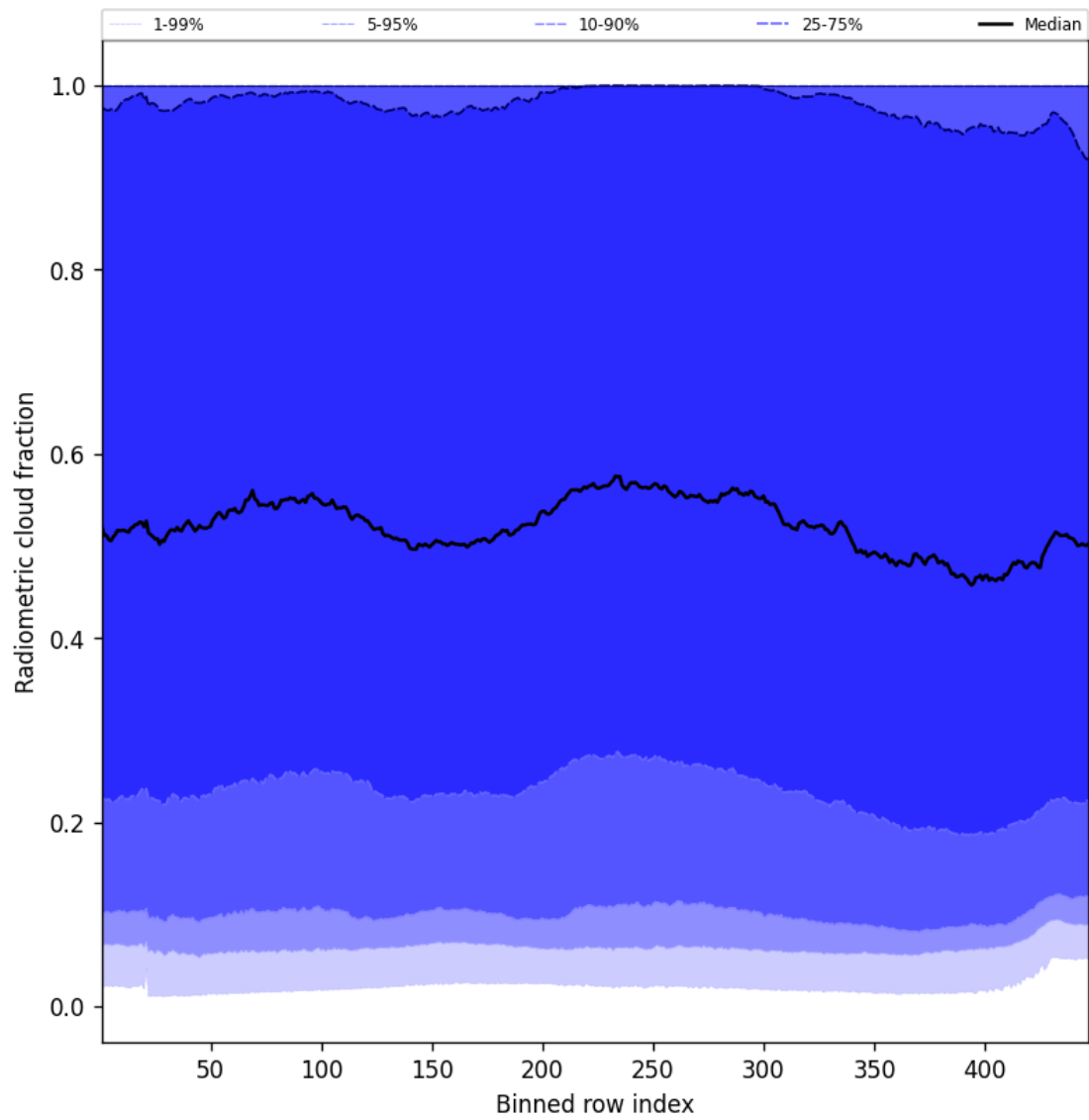
Figure 55: Along track statistics of “Radiometric cloud fraction” for 2025-03-17 to 2025-03-18
