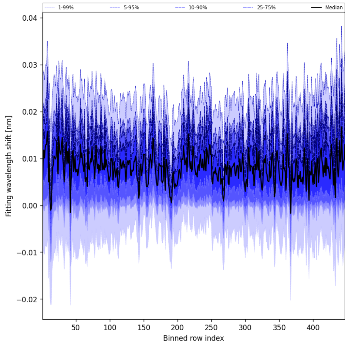
Figure 65: Along track statistics of “Fitting wavelength shift” for 2025-03-17 to 2025-03-18
