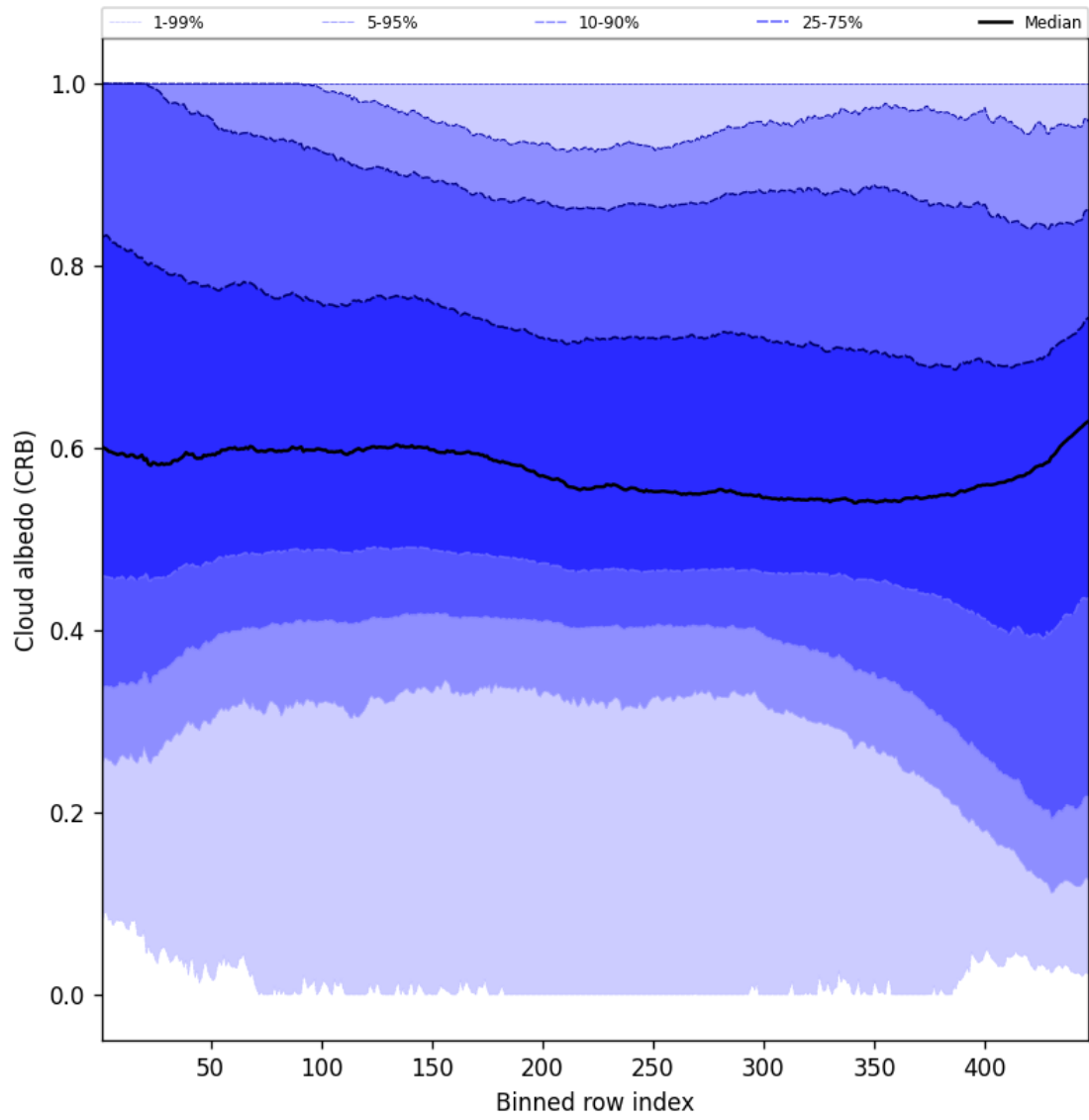
Figure 60: Along track statistics of “Cloud albedo (CRB)” for 2025-03-17 to 2025-03-18
