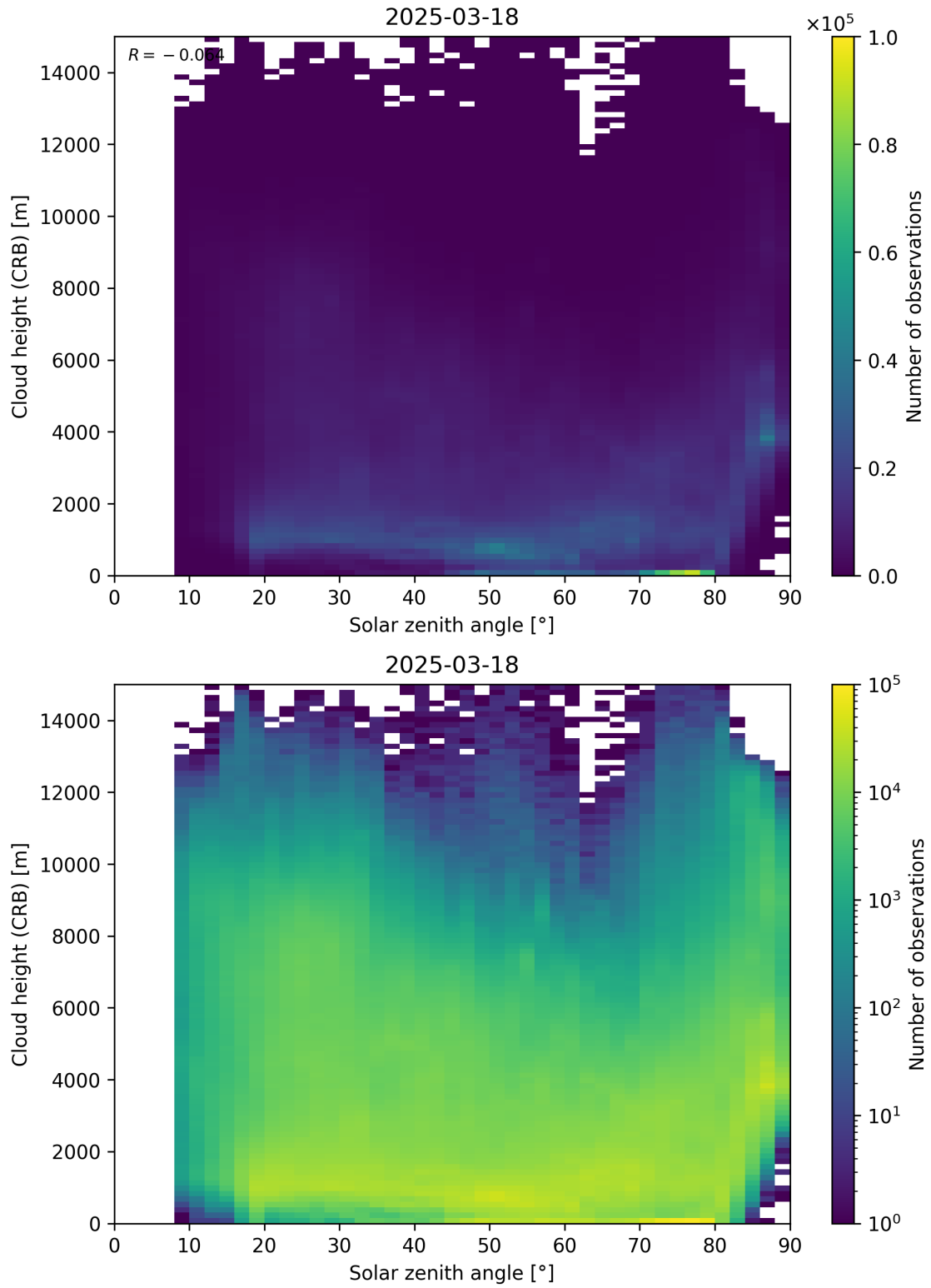
Figure 102: Scatter density plot of “Solar zenith angle” against “Cloud height (CRB)” for 2025-03-17 to 2025-03-19.
