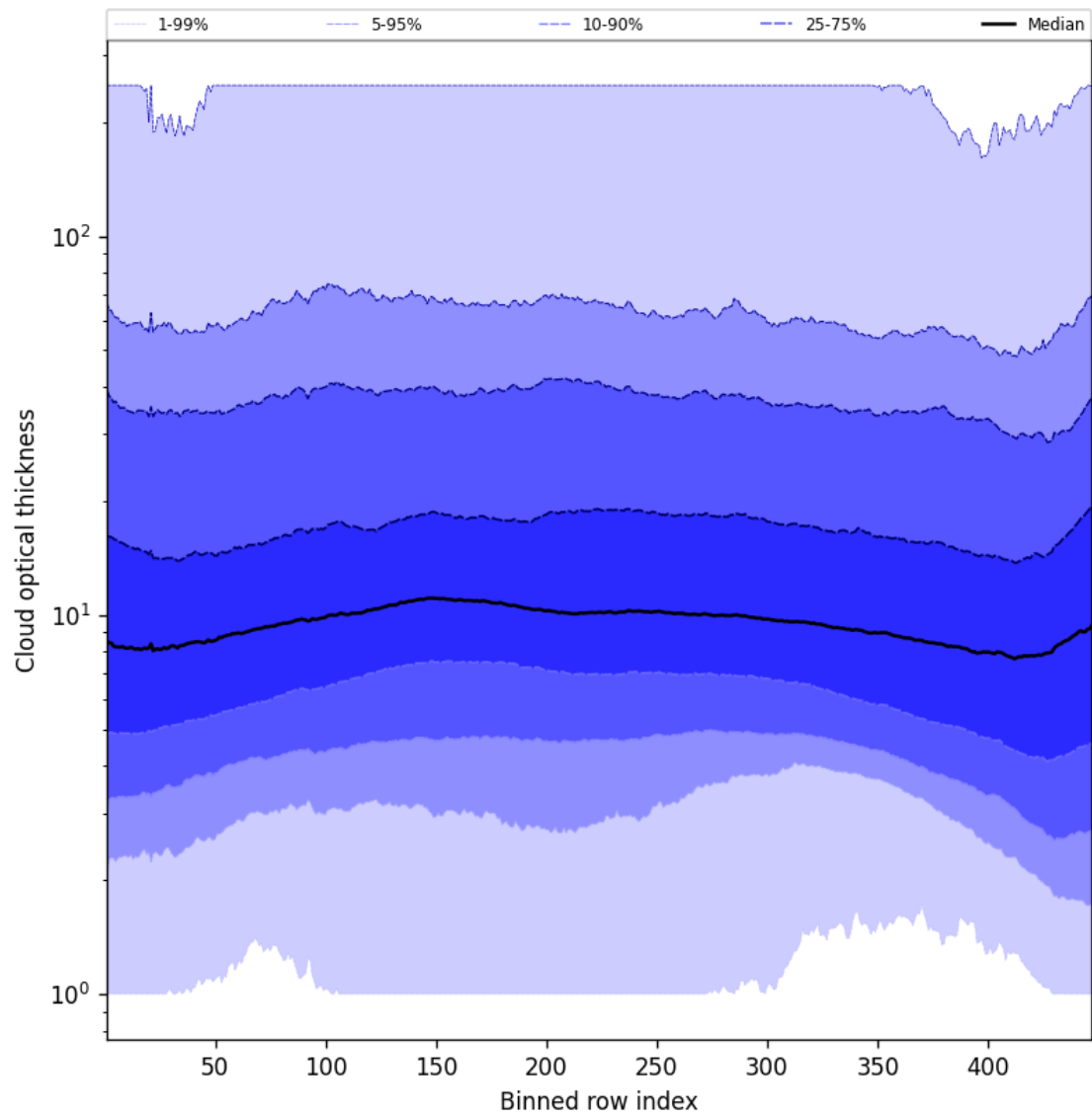
Figure 57: Along track statistics of “Cloud optical thickness” for 2025-03-17 to 2025-03-19
