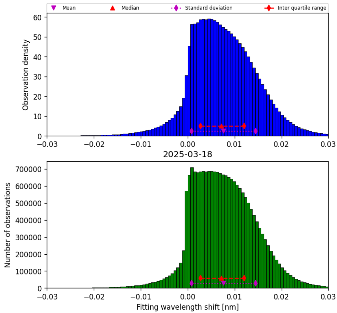
Figure 49: Histogram of “Fitting wavelength shift” for 2025-03-17 to 2025-03-19
