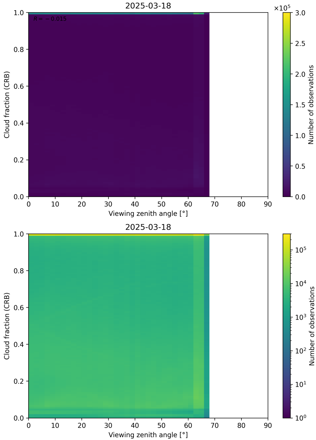
Figure 109: Scatter density plot of “Viewing zenith angle” against “Cloud fraction (CRB)” for 2025-03-17 to 2025-03-19.
