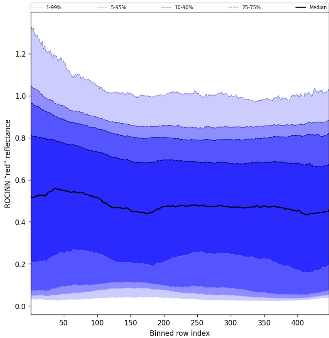
Figure 69: Along track statistics of “ROCINN “red” reflectance” for 2025-03-17 to 2025-03-19
