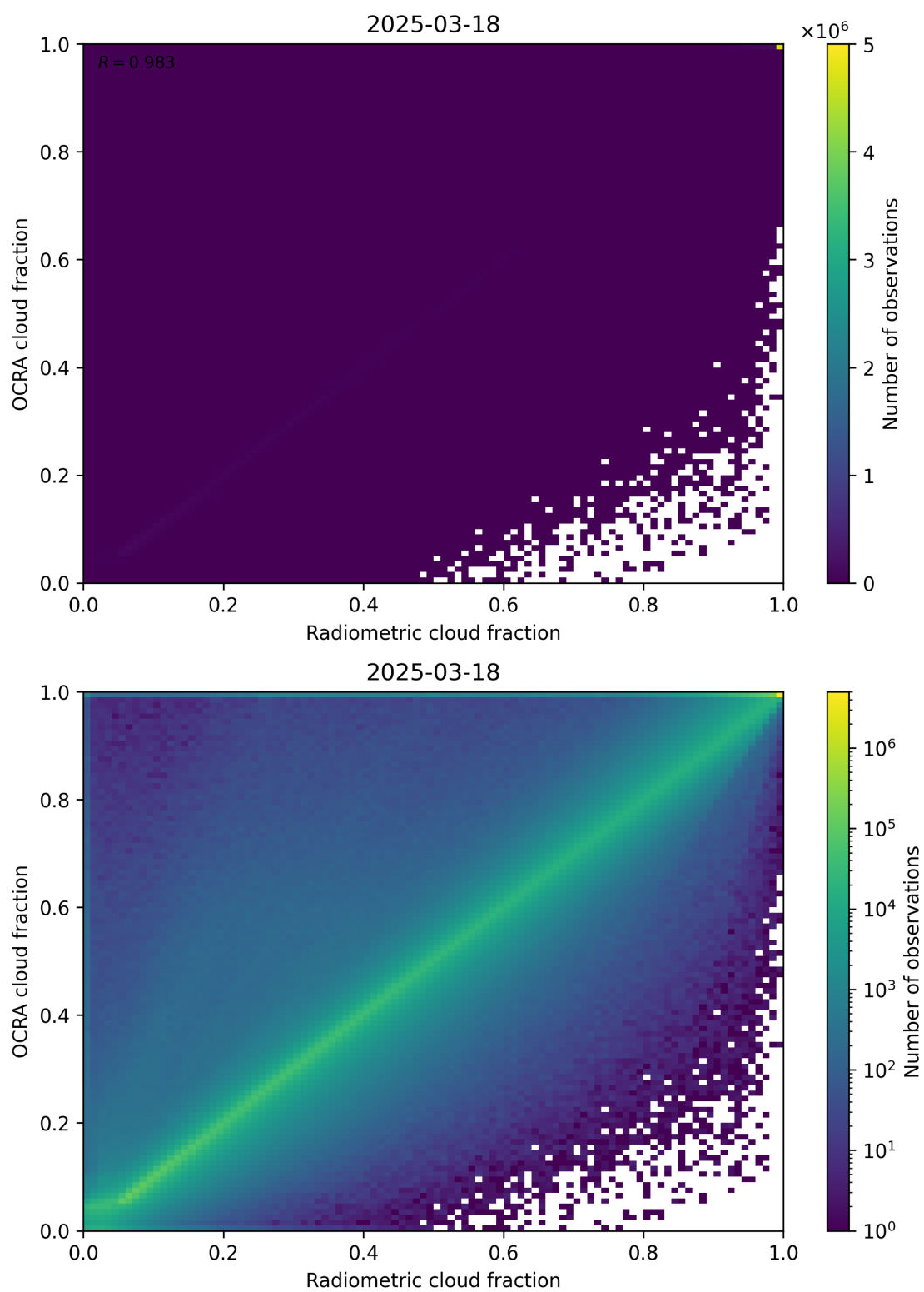
Figure 72: Scatter density plot of “Radiometric cloud fraction” against “OCRA cloud fraction” for 2025-03-17 to 2025-03-19.
