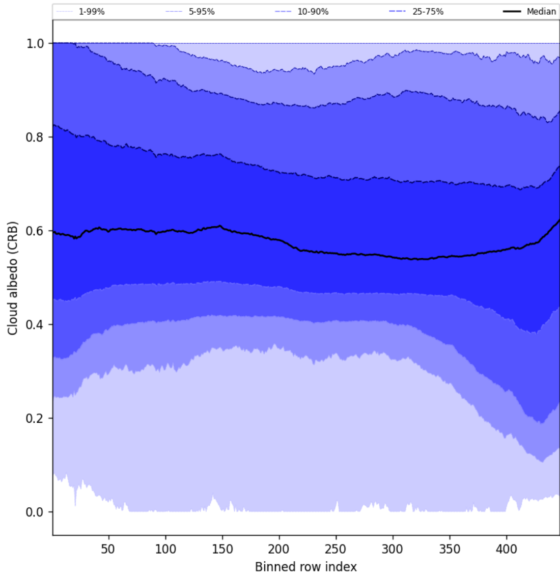
Figure 60: Along track statistics of “Cloud albedo (CRB)” for 2025-03-17 to 2025-03-19
