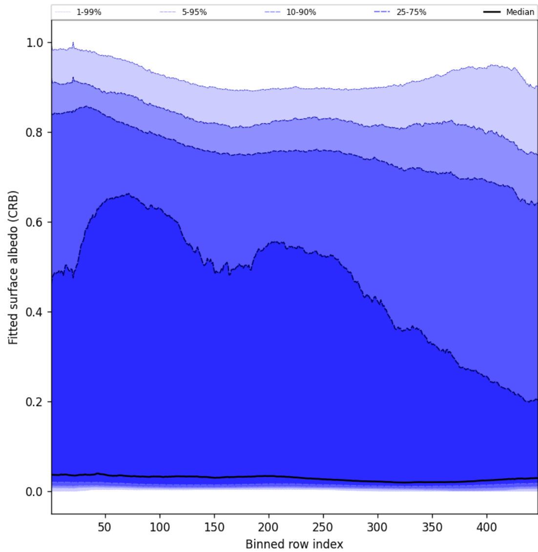
Figure 62: Along track statistics of “Fitted surface albedo (CRB)” for 2025-03-17 to 2025-03-19
