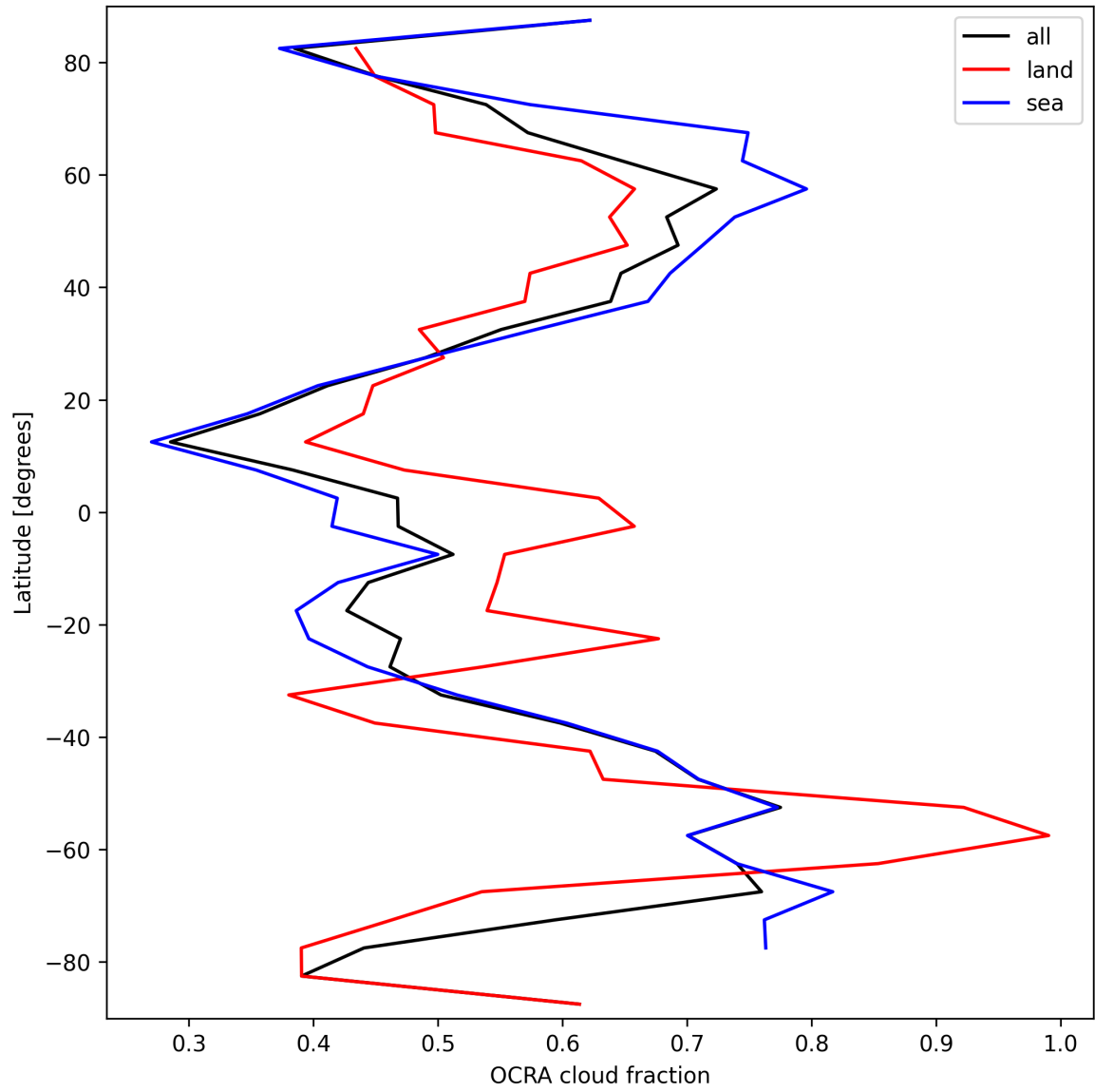
Figure 34: Zonal average of “OCRA cloud fraction” for 2025-03-17 to 2025-03-19.
