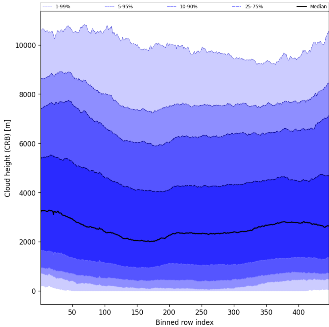
Figure 59: Along track statistics of “Cloud height (CRB)” for 2025-03-17 to 2025-03-19
