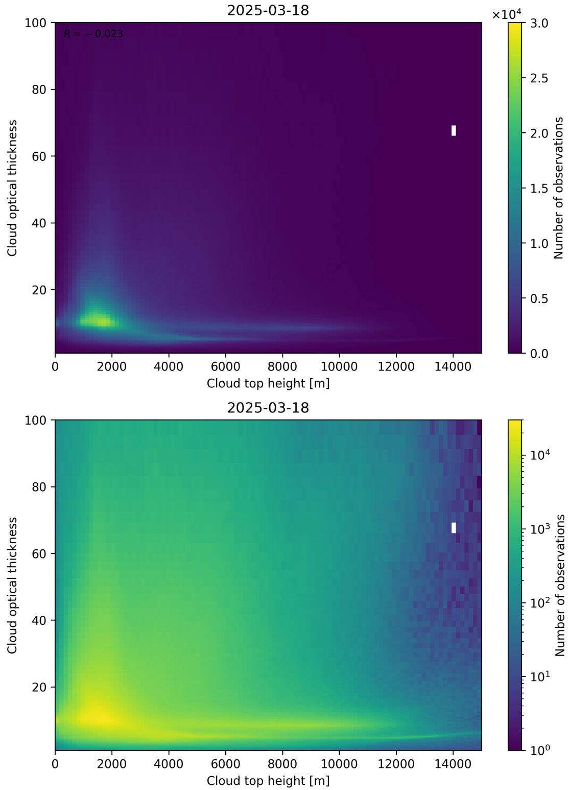
Figure 90: Scatter density plot of “Cloud top height” against “Cloud optical thickness” for 2025-03-17 to 2025-03-19.
