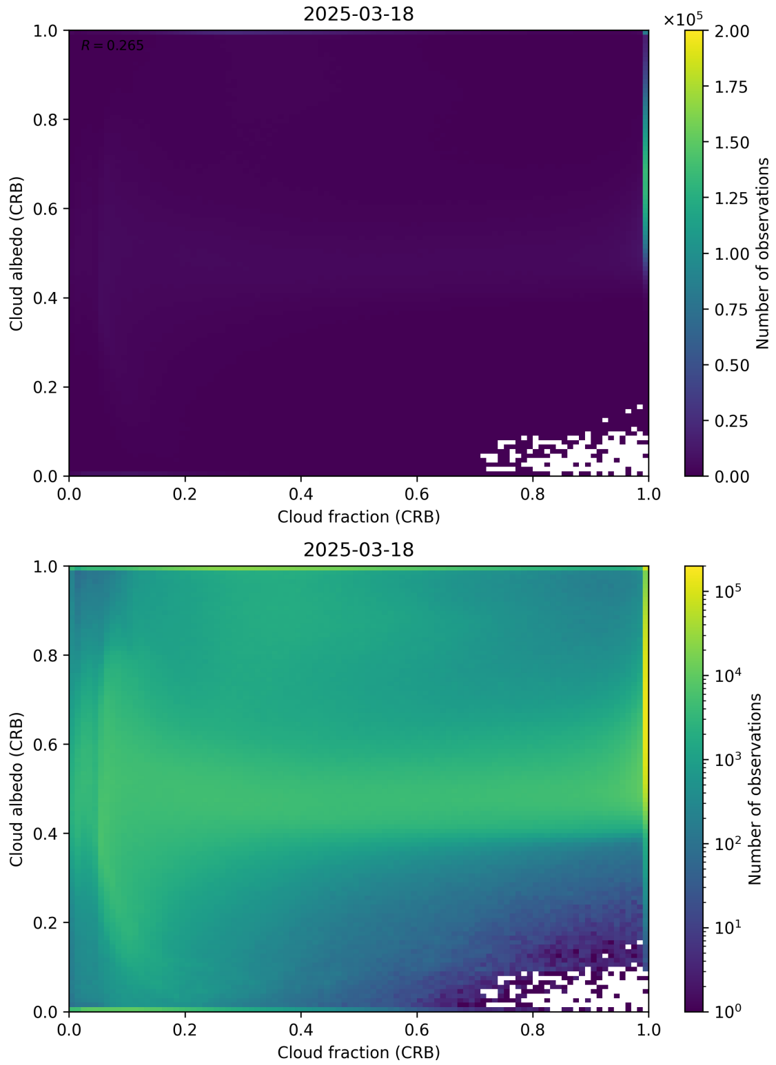
Figure 77: Scatter density plot of “Cloud fraction (CRB)” against “Cloud albedo (CRB)” for 2025-03-17 to 2025-03-19.
