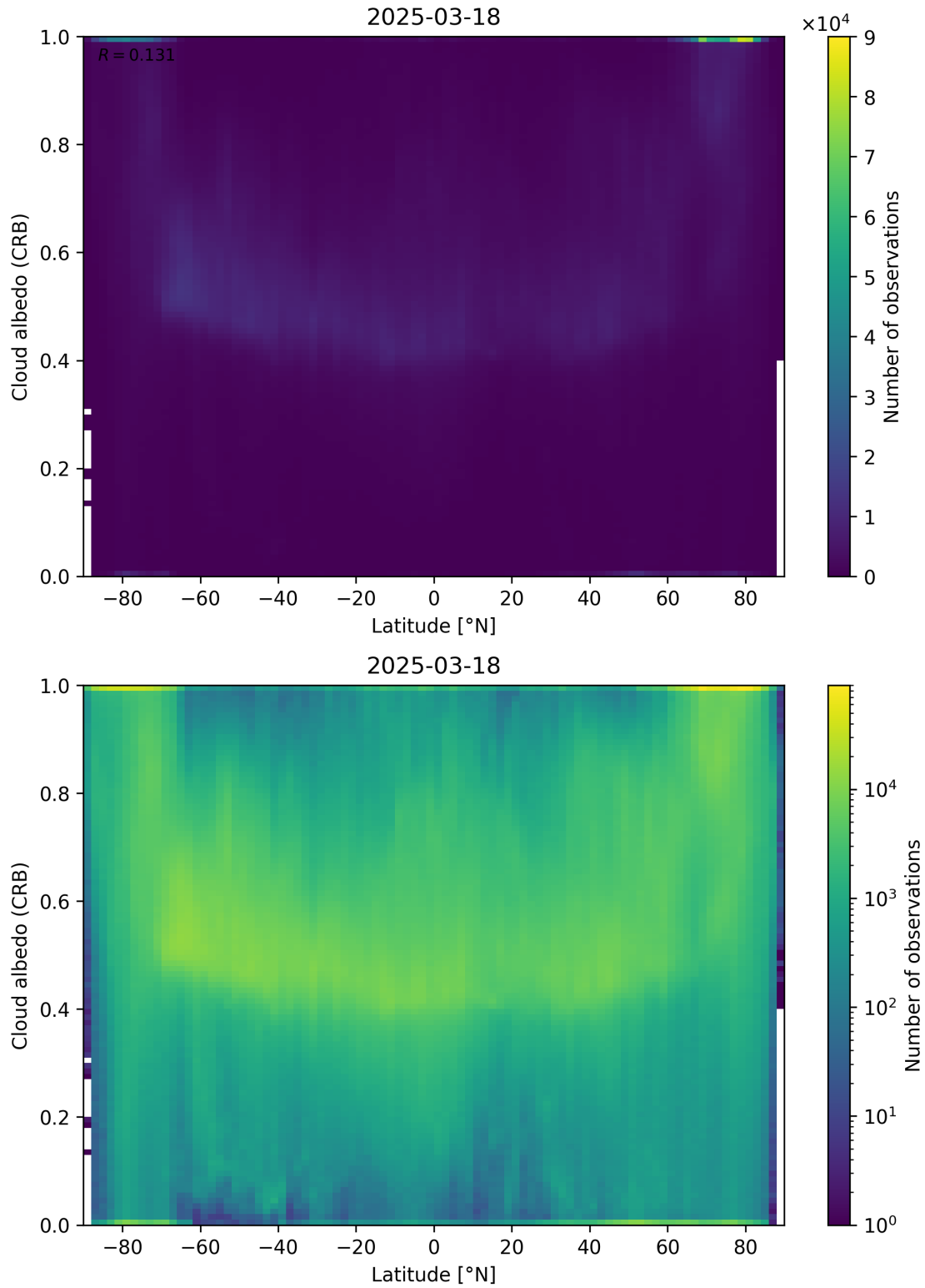
Figure 91: Scatter density plot of “Latitude” against “Cloud albedo (CRB)” for 2025-03-17 to 2025-03-19.
