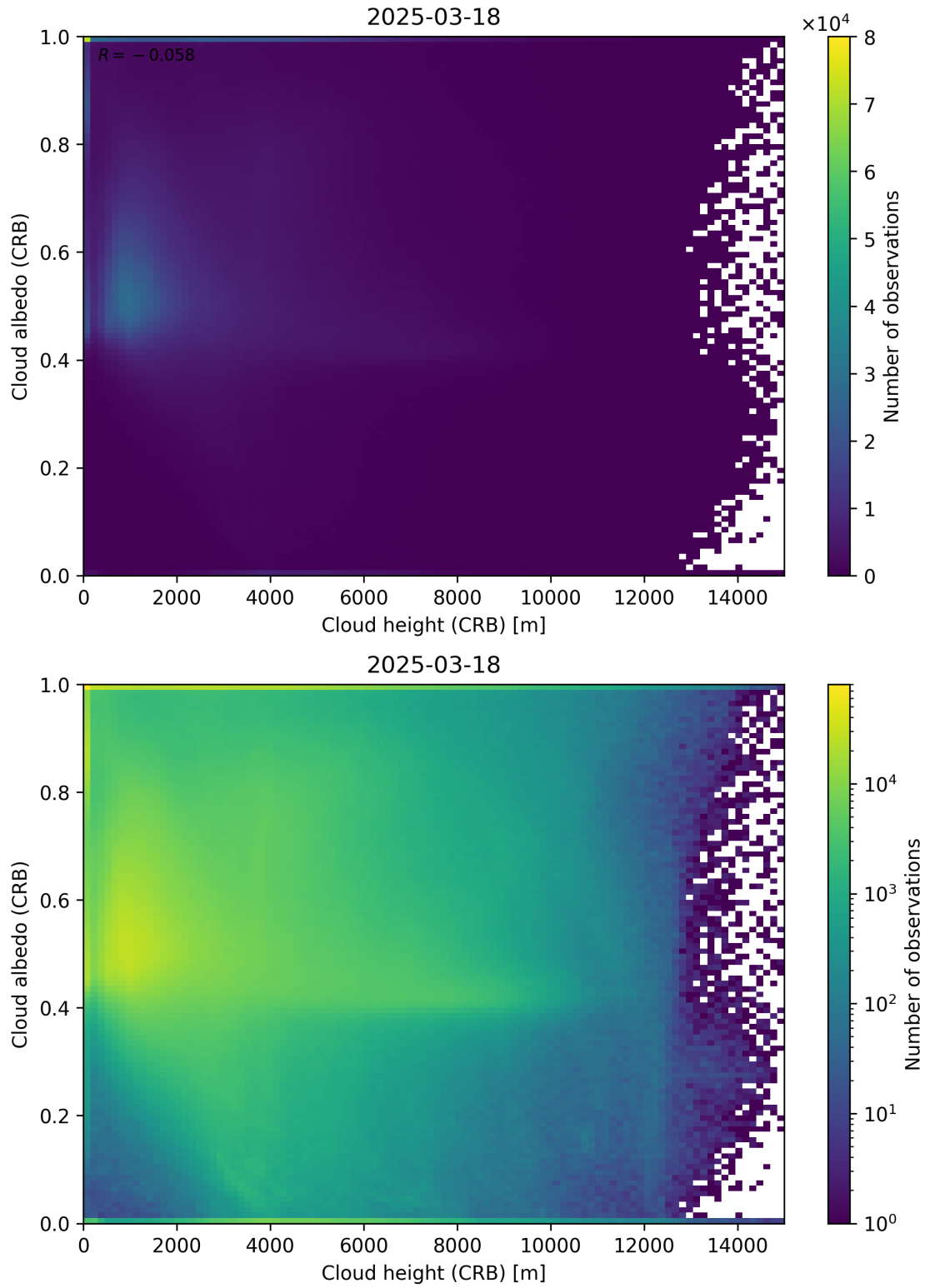
Figure 80: Scatter density plot of “Cloud height (CRB)” against “Cloud albedo (CRB)” for 2025-03-17 to 2025-03-19.
