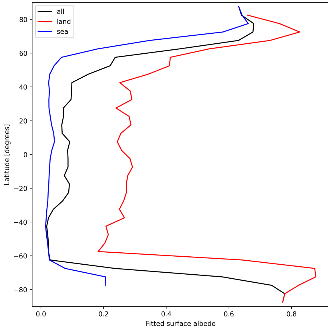
Figure 29: Zonal average of “Fitted surface albedo” for 2025-03-17 to 2025-03-19.
