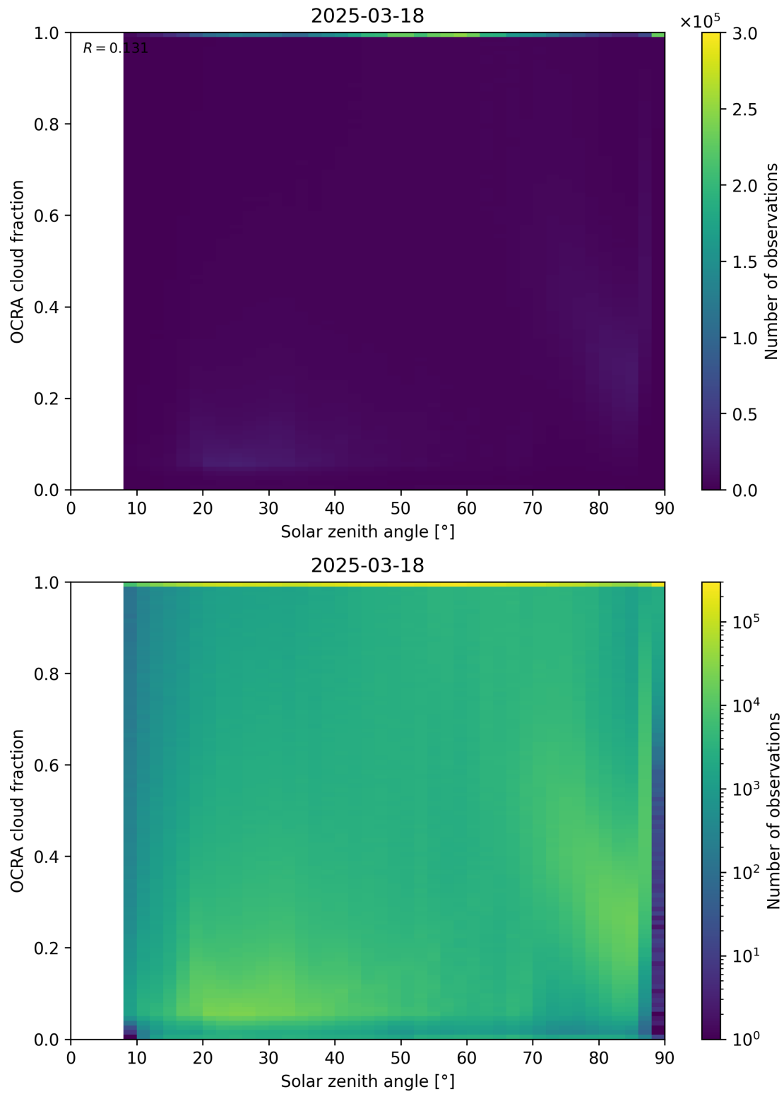
Figure 100: Scatter density plot of “Solar zenith angle” against “OCRA cloud fraction” for 2025-03-17 to 2025-03-19.
