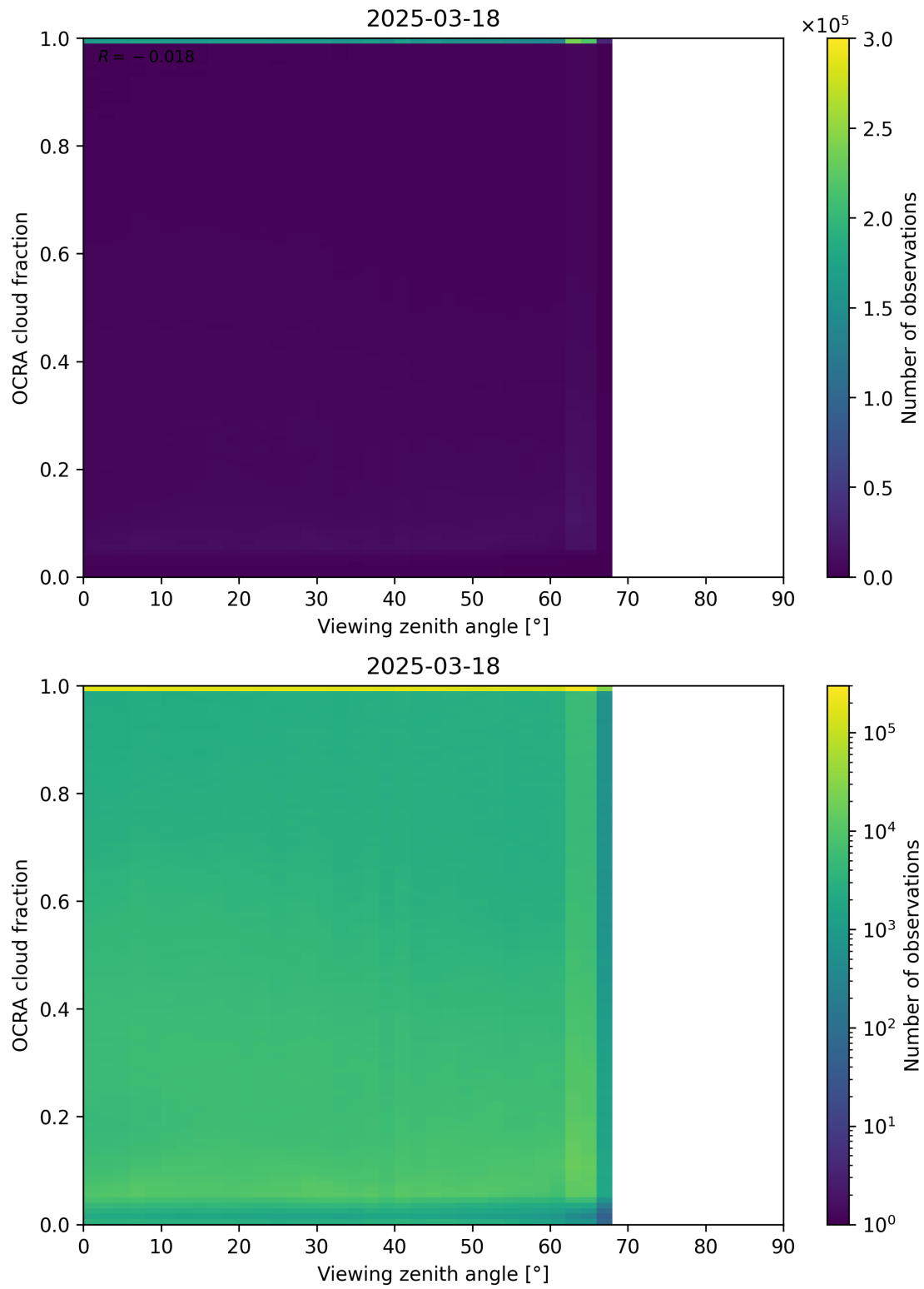
Figure 108: Scatter density plot of “Viewing zenith angle” against “OCRA cloud fraction” for 2025-03-17 to 2025-03-19.
