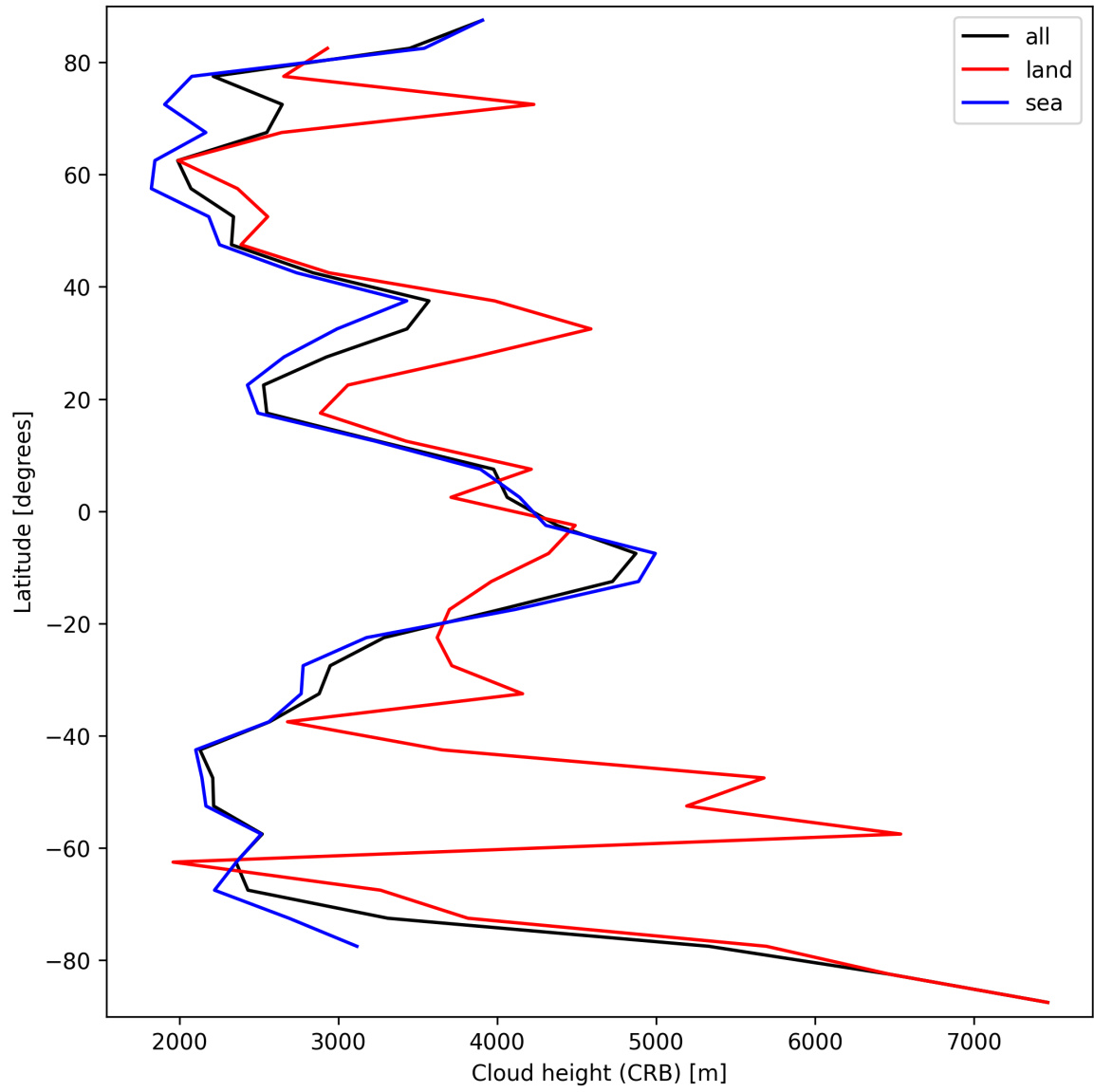
Figure 27: Zonal average of “Cloud height (CRB)” for 2025-03-17 to 2025-03-19.
