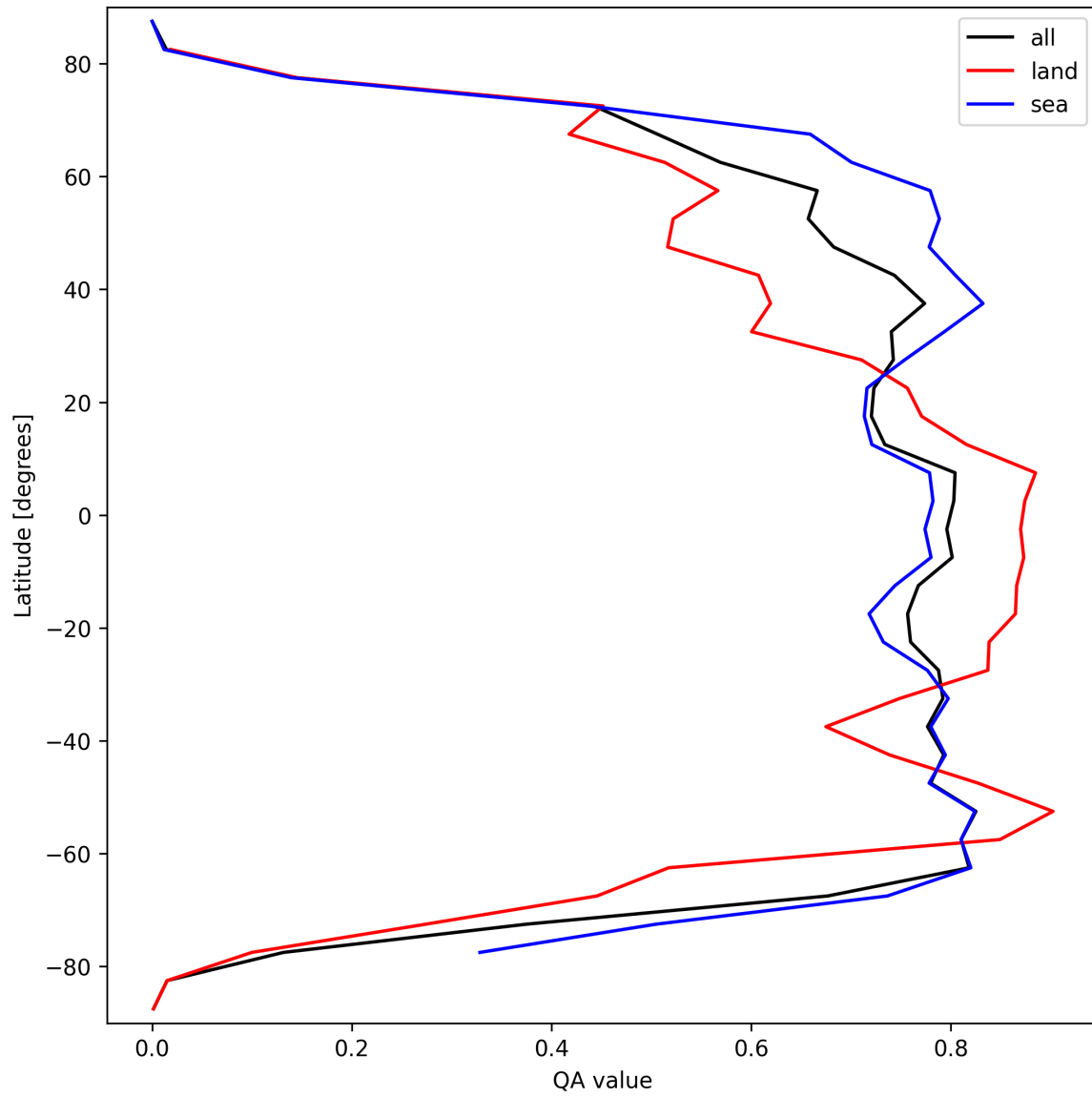
Figure 22: Zonal average of “QA value” for 2025-03-17 to 2025-03-19.
