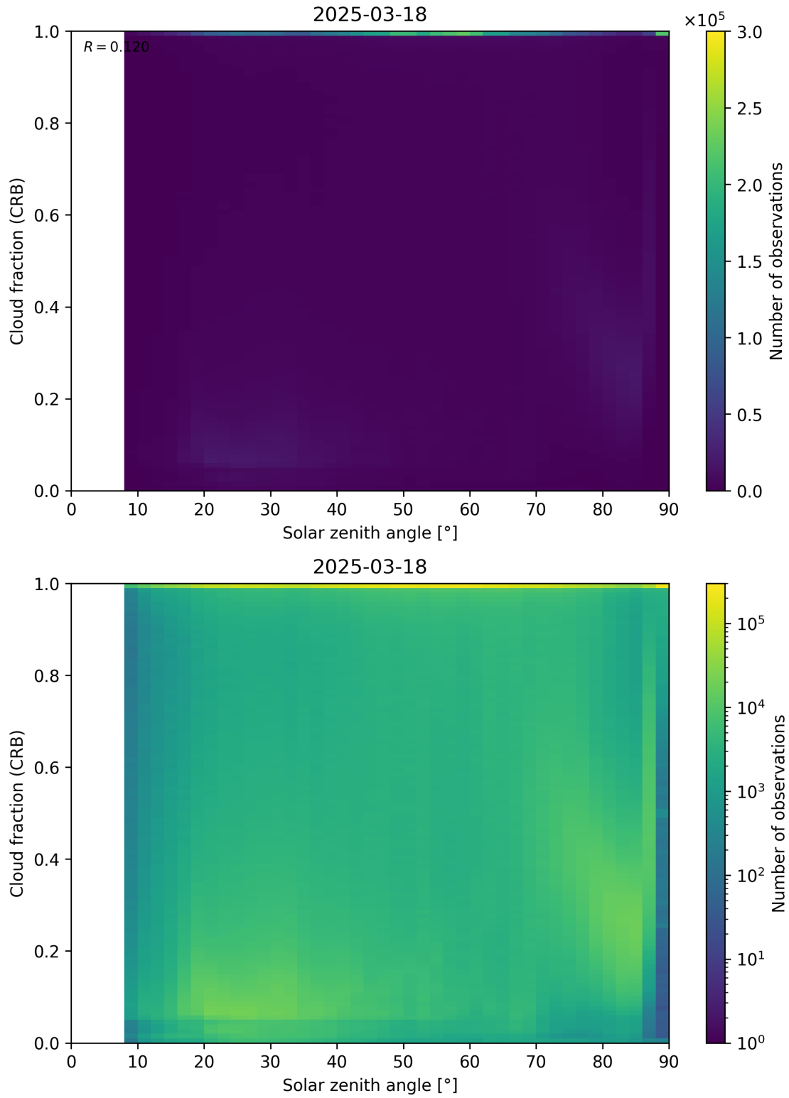
Figure 101: Scatter density plot of “Solar zenith angle” against “Cloud fraction (CRB)” for 2025-03-17 to 2025-03-19.
