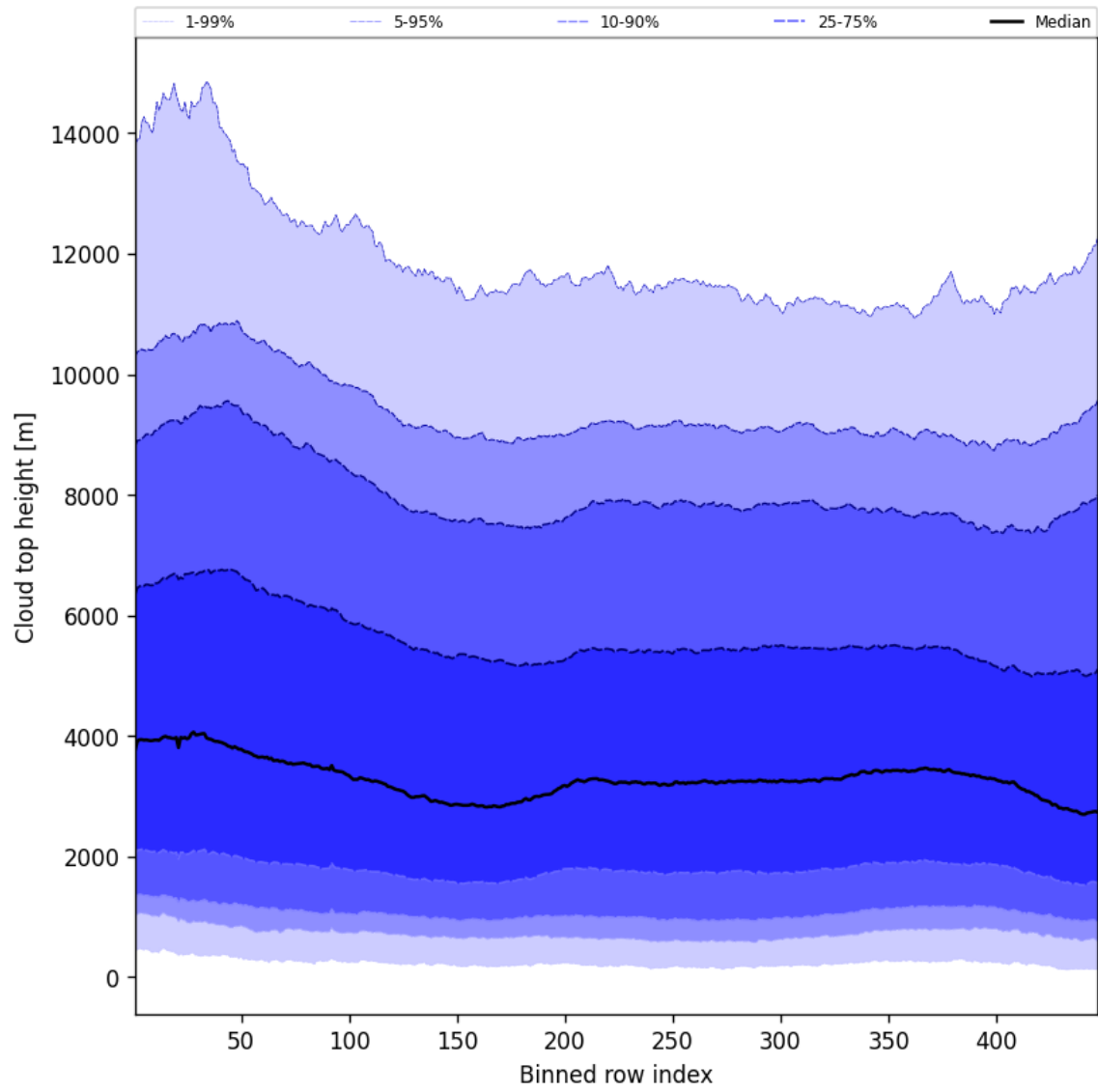
Figure 56: Along track statistics of “Cloud top height” for 2025-03-17 to 2025-03-19
