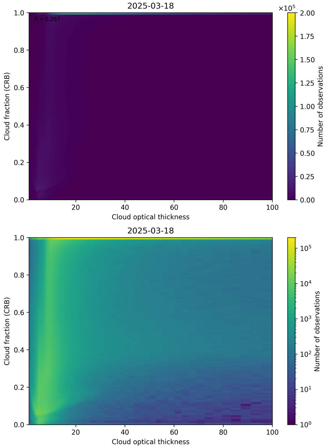
Figure 84: Scatter density plot of “Cloud optical thickness” against “Cloud fraction (CRB)” for 2025-03-17 to 2025-03-19.
