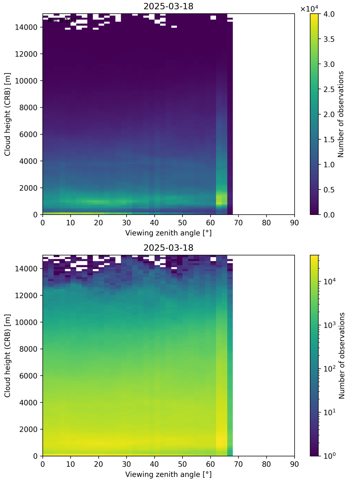
Figure 110: Scatter density plot of “Viewing zenith angle” against “Cloud height (CRB)” for 2025-03-17 to 2025-03-19.
