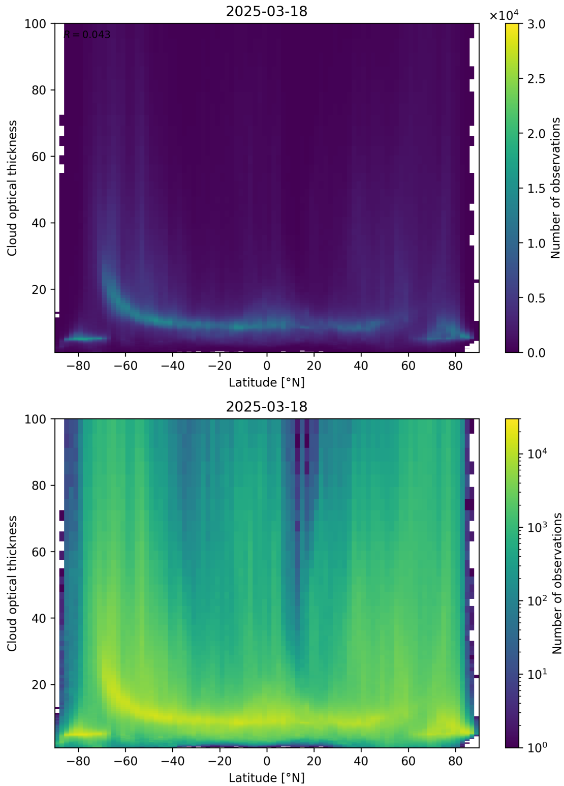
Figure 96: Scatter density plot of “Latitude” against “Cloud optical thickness” for 2025-03-17 to 2025-03-19.
