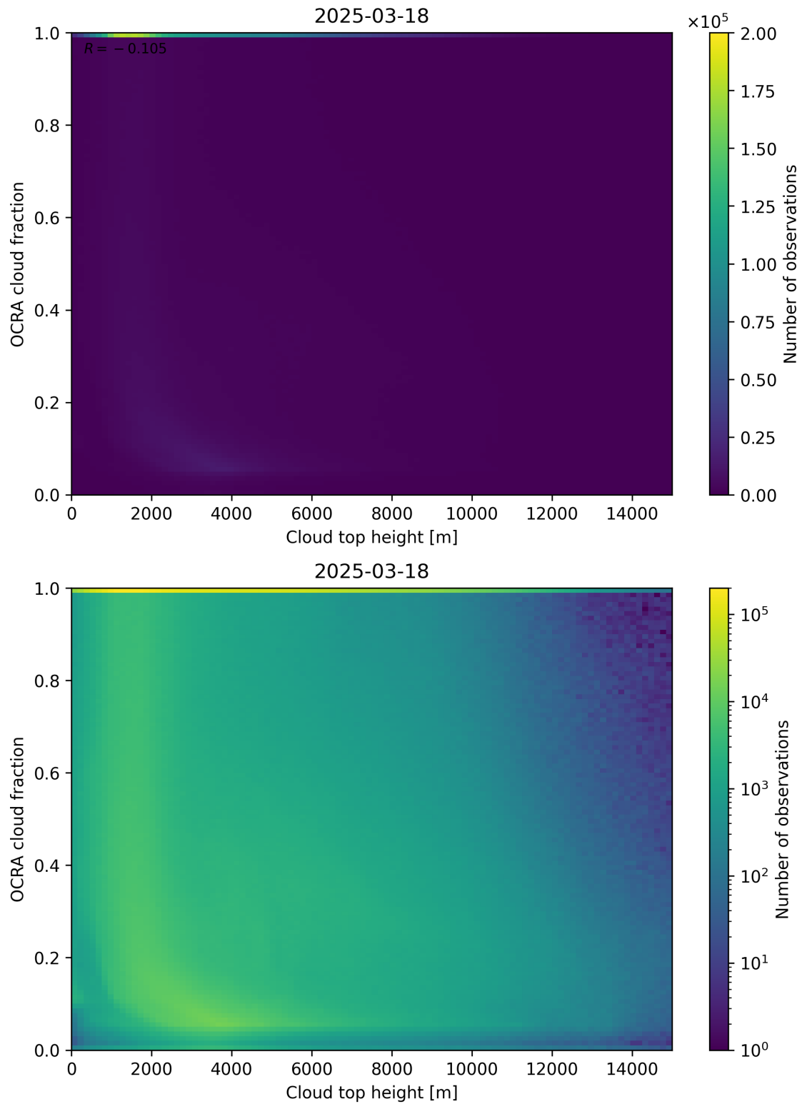
Figure 87: Scatter density plot of “Cloud top height” against “OCRA cloud fraction” for 2025-03-17 to 2025-03-19.
