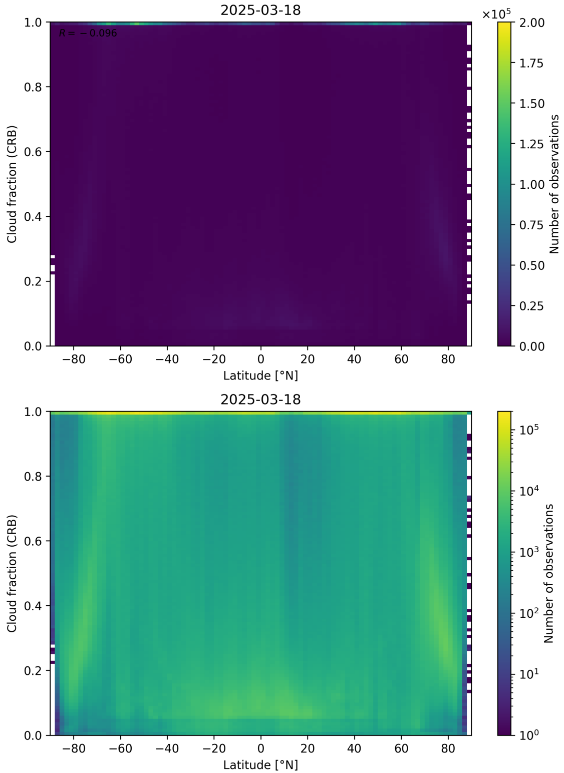
Figure 94: Scatter density plot of “Latitude” against “Cloud fraction (CRB)” for 2025-03-17 to 2025-03-19.
