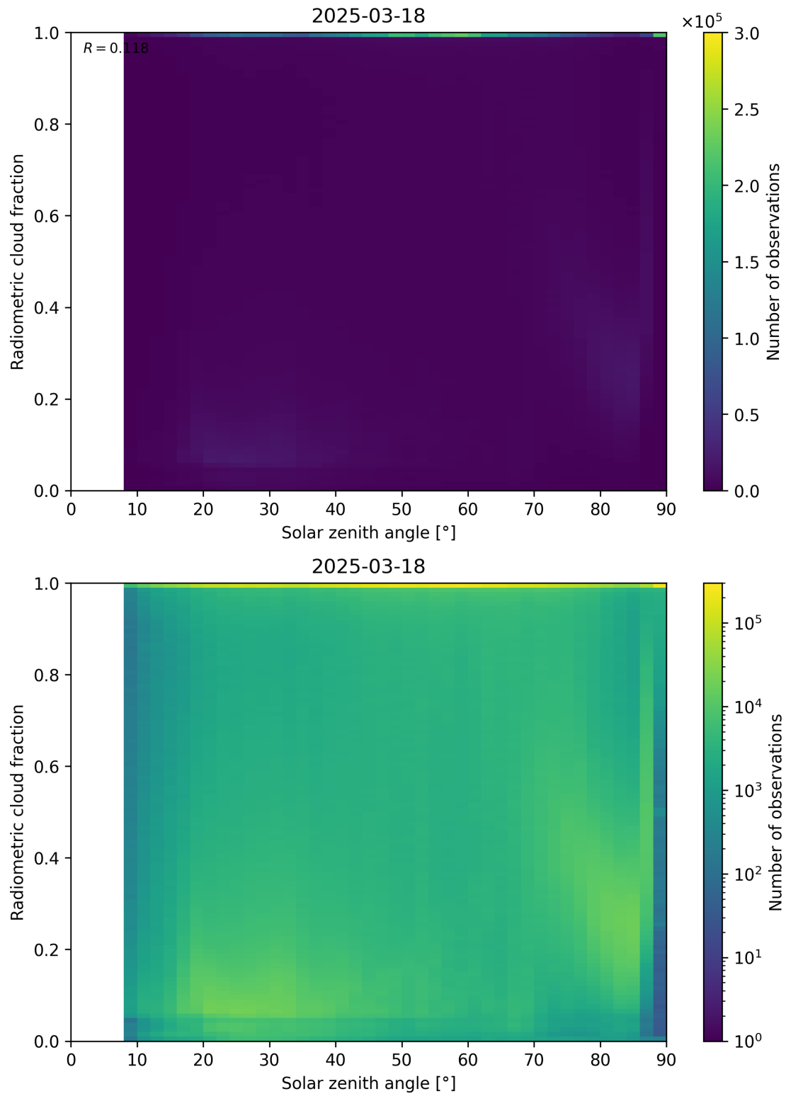
Figure 99: Scatter density plot of “Solar zenith angle” against “Radiometric cloud fraction” for 2025-03-17 to 2025-03-19.
