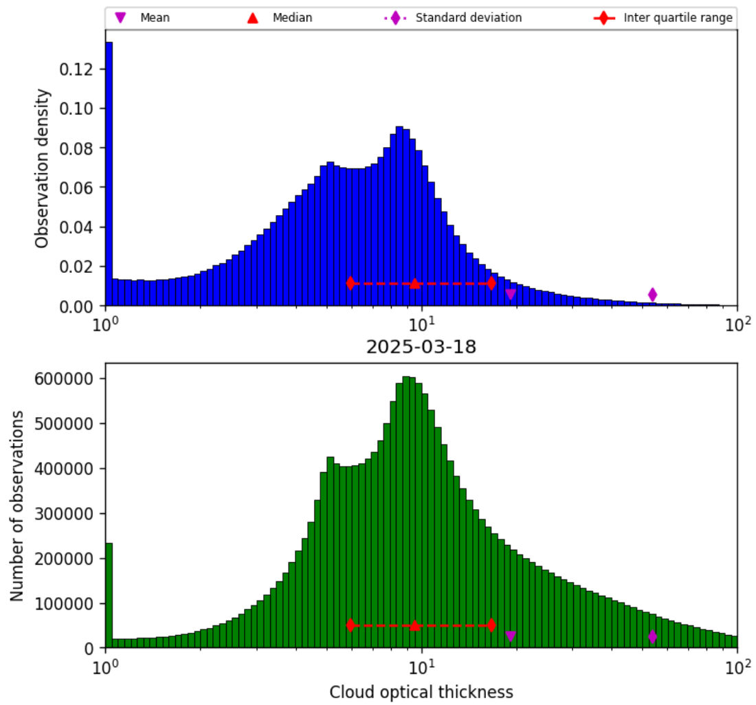
Figure 41: Histogram of “Cloud optical thickness” for 2025-03-17 to 2025-03-19
