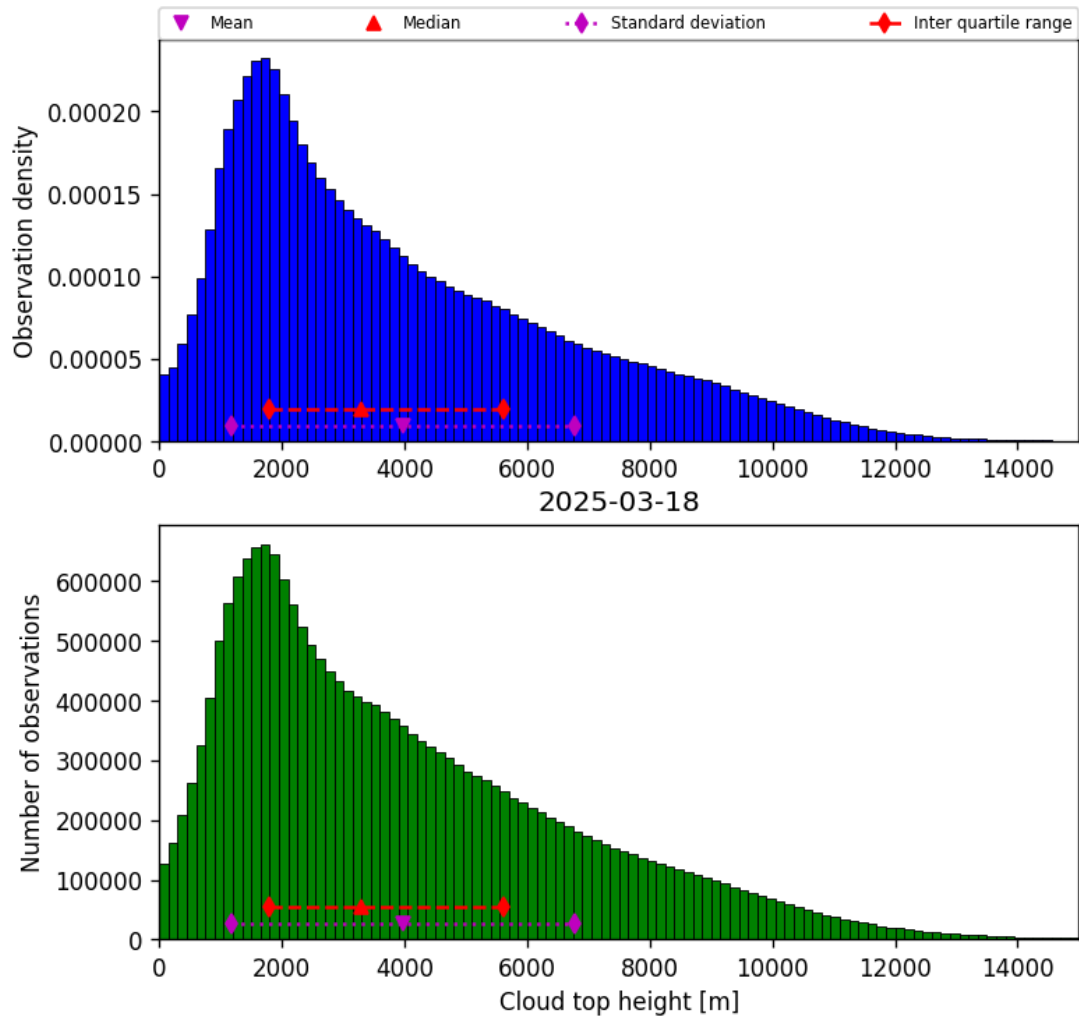
Figure 40: Histogram of “Cloud top height” for 2025-03-17 to 2025-03-19
