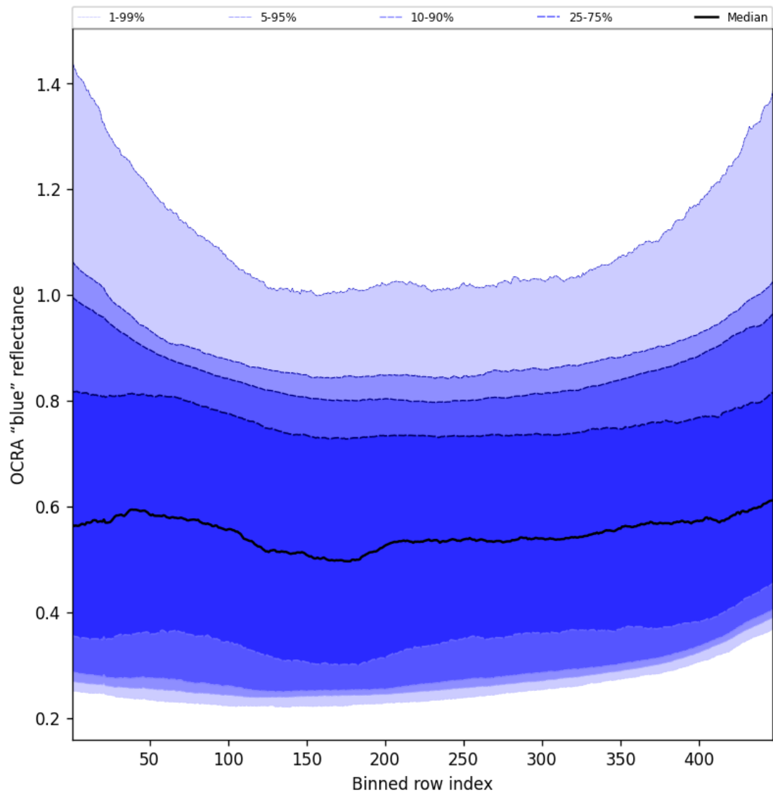
Figure 67: Along track statistics of “OCRA “blue” reflectance” for 2025-03-17 to 2025-03-19
