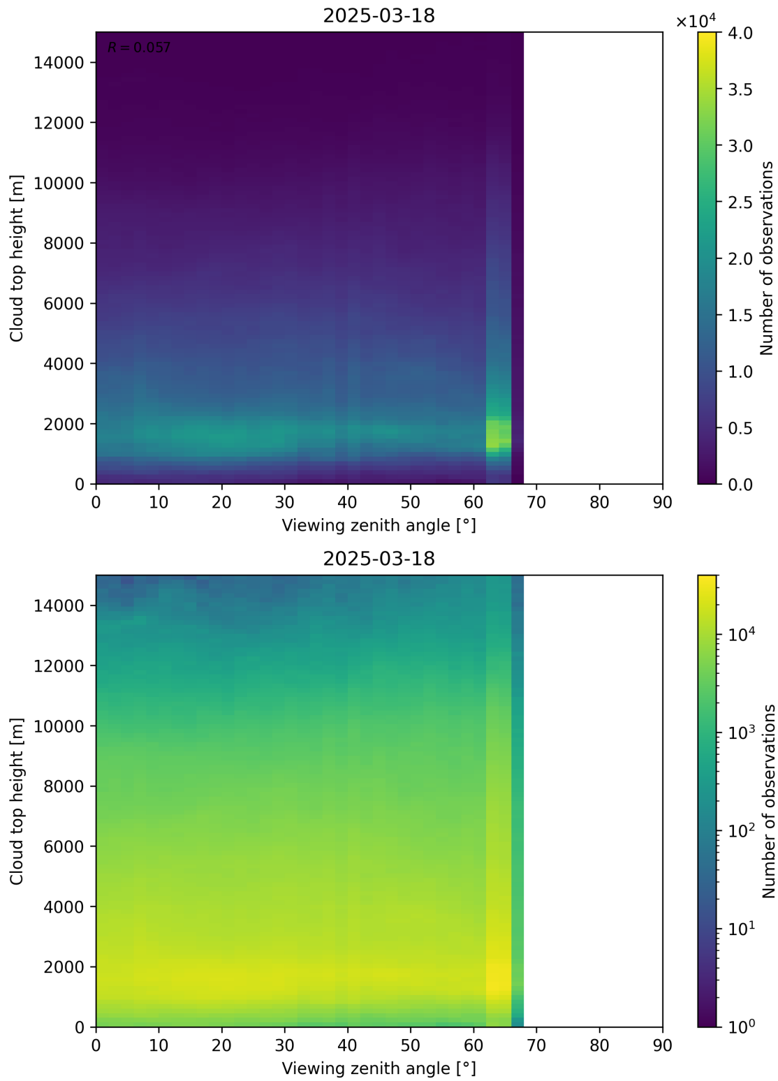
Figure 112: Scatter density plot of “Viewing zenith angle” against “Cloud top height” for 2025-03-17 to 2025-03-19.
