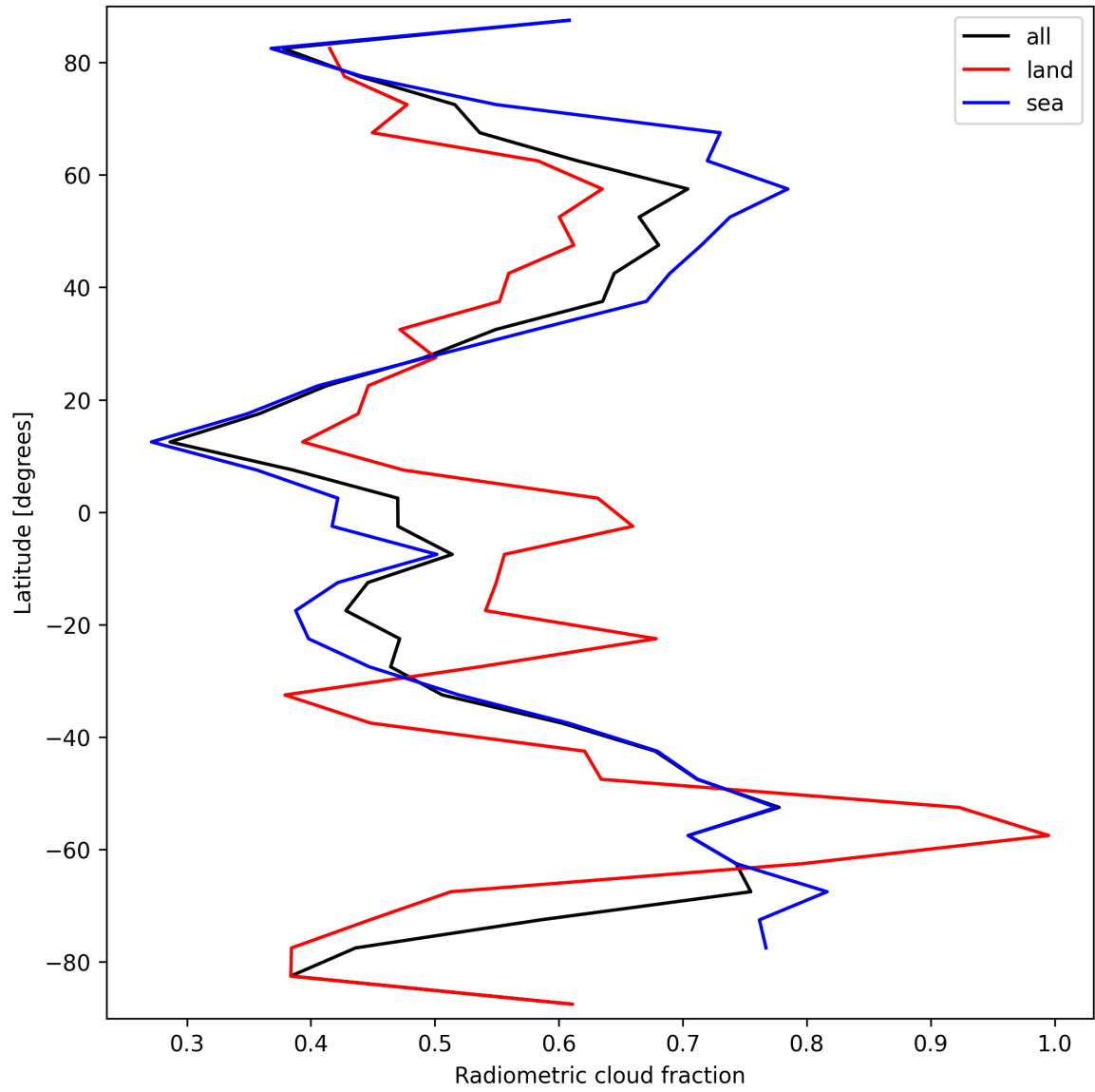
Figure 23: Zonal average of “Radiometric cloud fraction” for 2025-03-17 to 2025-03-19.
