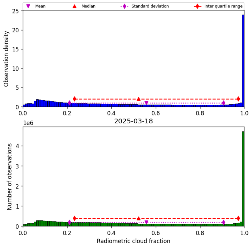
Figure 39: Histogram of “Radiometric cloud fraction” for 2025-03-17 to 2025-03-19
