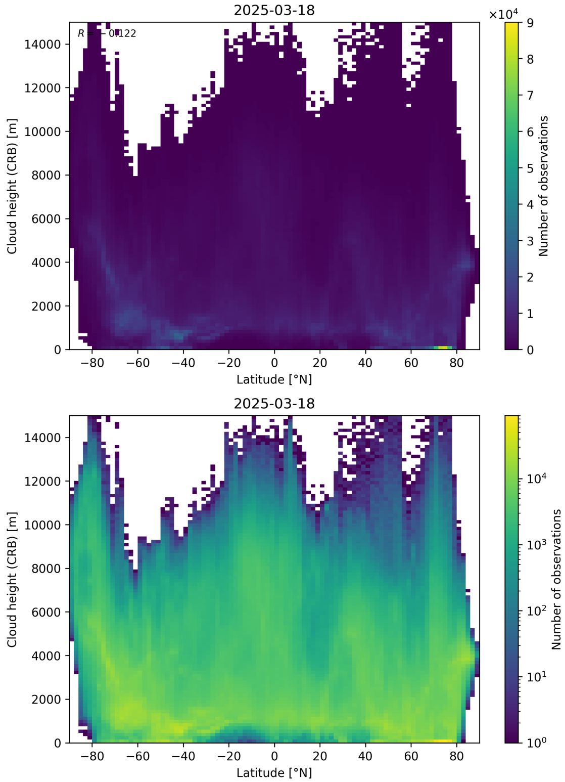
Figure 95: Scatter density plot of “Latitude” against “Cloud height (CRB)” for 2025-03-17 to 2025-03-19.
