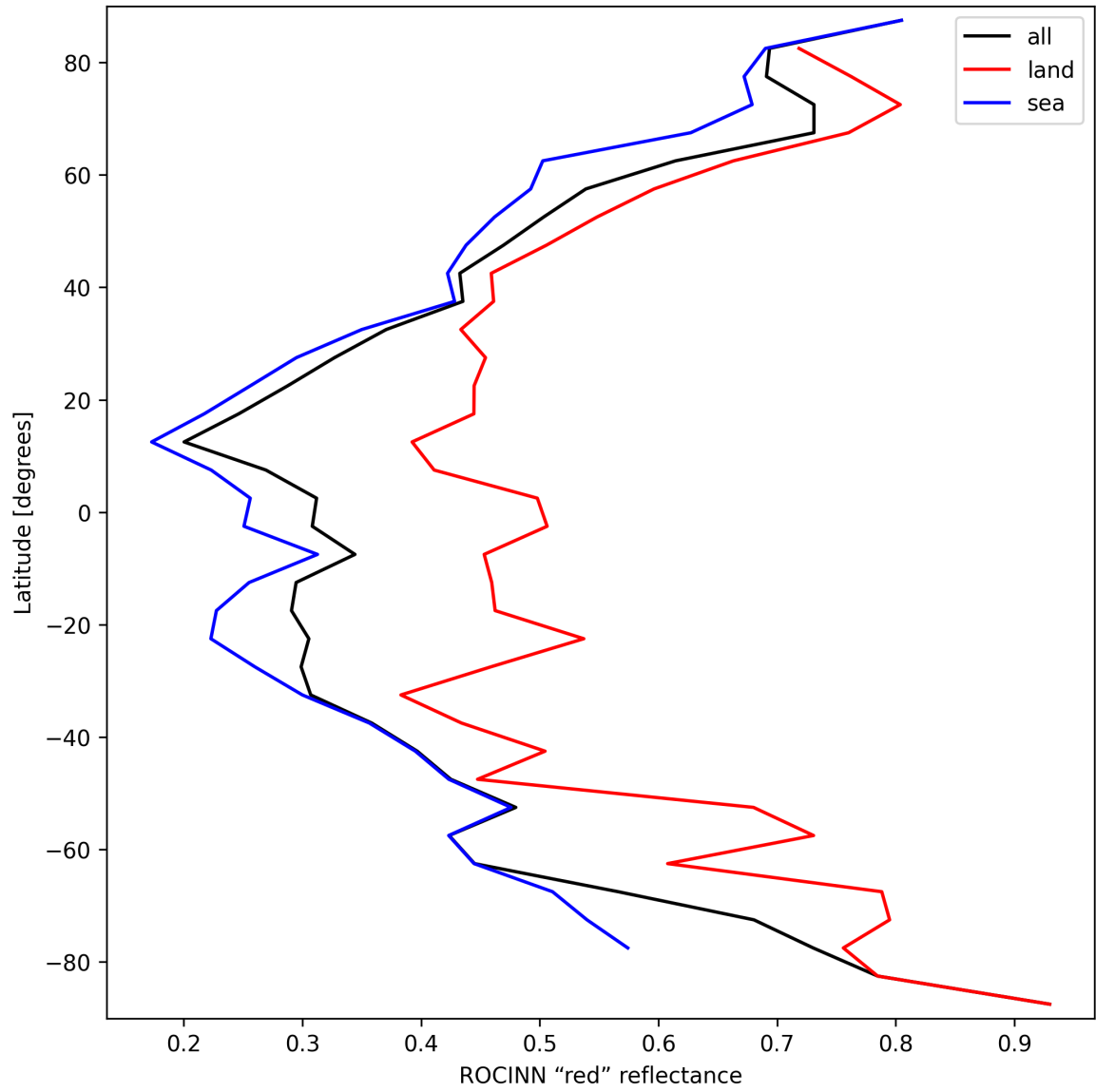
Figure 37: Zonal average of “ROCINN “red” reflectance” for 2025-03-17 to 2025-03-19.
