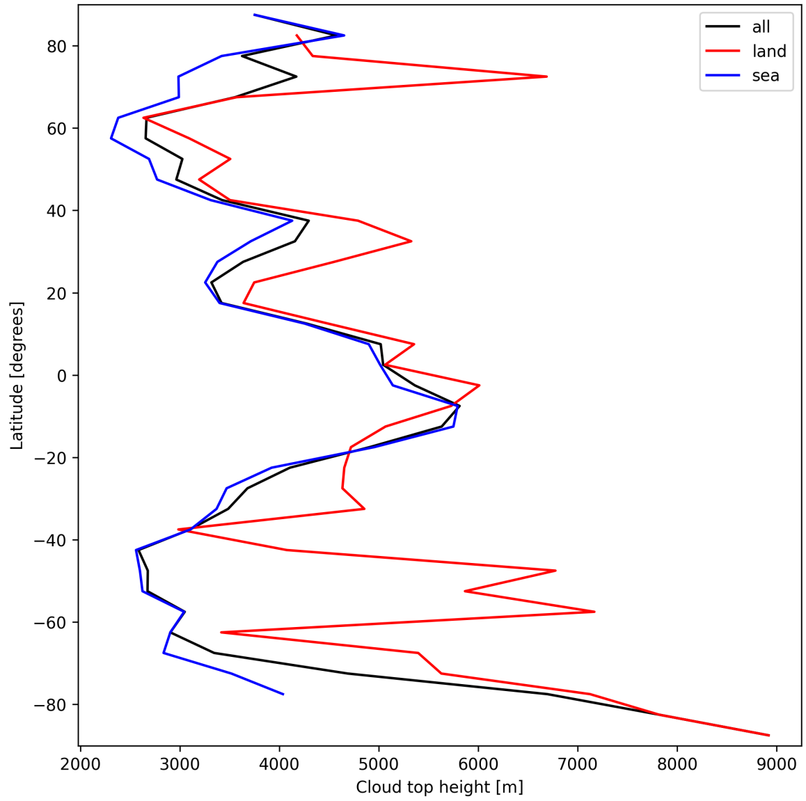
Figure 24: Zonal average of “Cloud top height” for 2025-03-17 to 2025-03-19.
