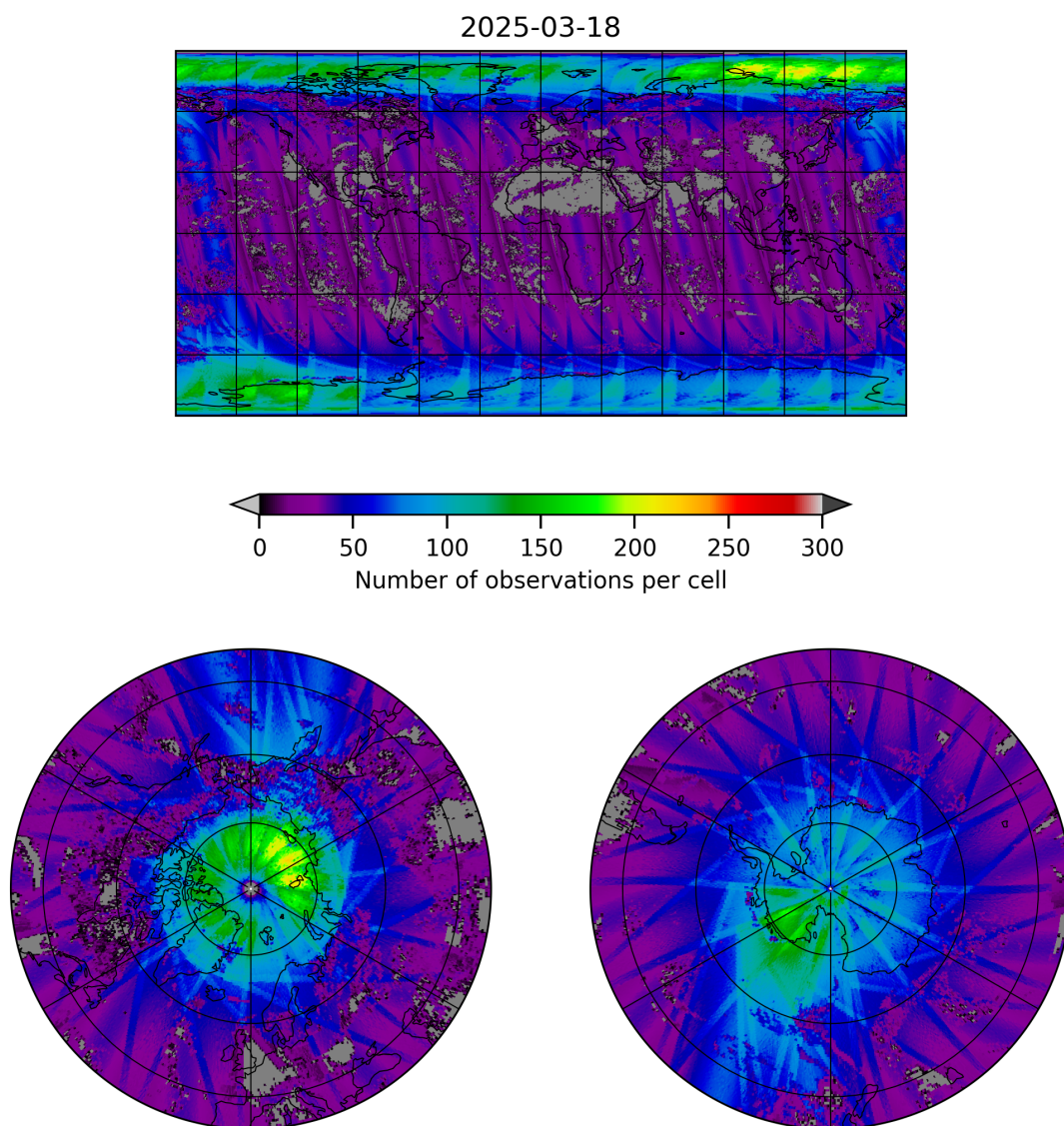
Figure 21: Map of the number of observations for 2025-03-17 to 2025-03-19
