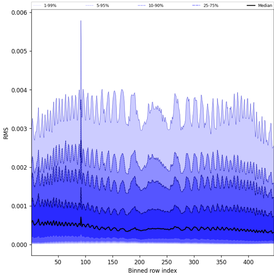
Figure 63: Along track statistics of “RMS” for 2025-03-17 to 2025-03-19
