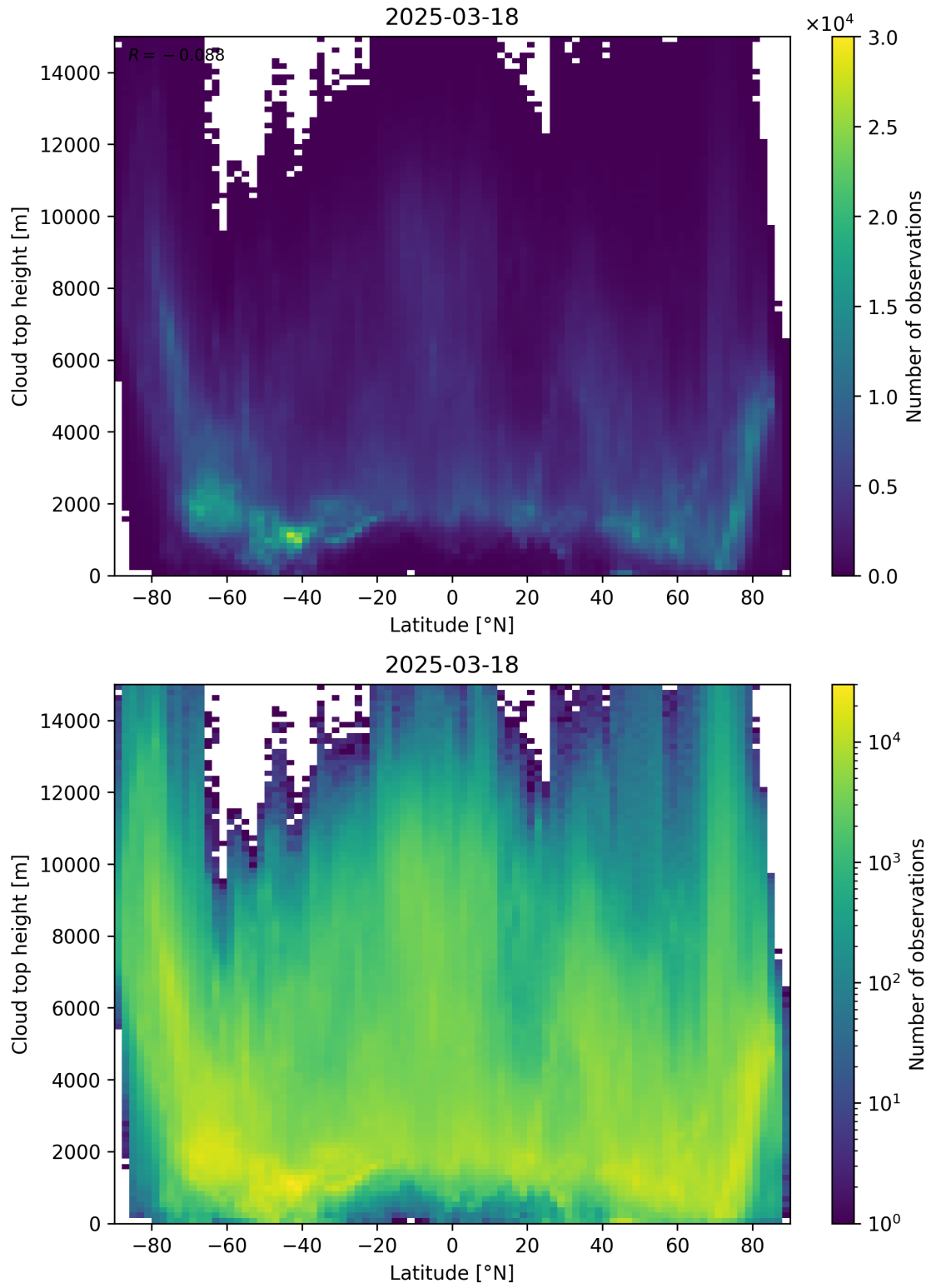
Figure 97: Scatter density plot of “Latitude” against “Cloud top height” for 2025-03-17 to 2025-03-19.
