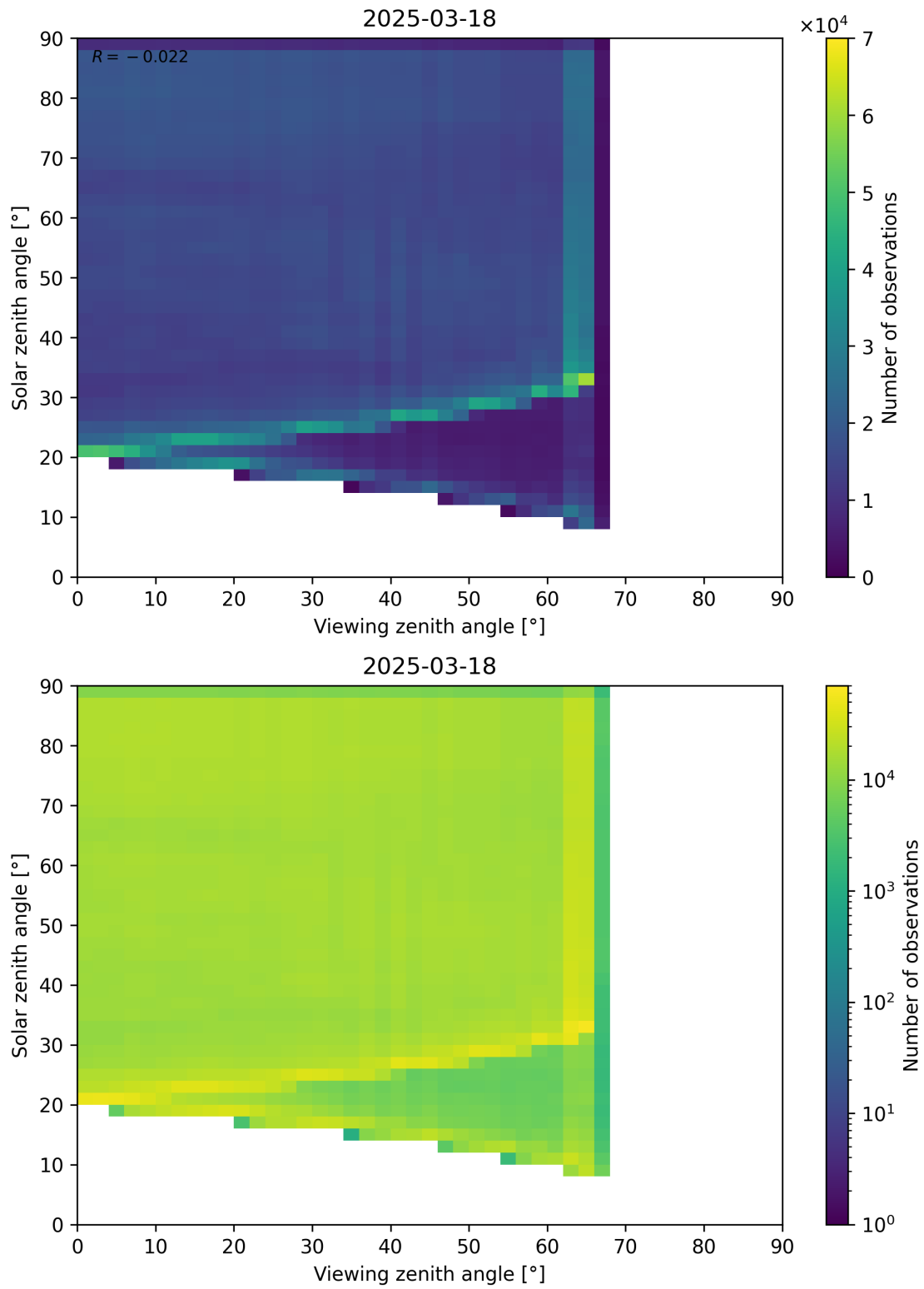
Figure 114: Scatter density plot of “Viewing zenith angle” against “Solar zenith angle” for 2025-03-17 to 2025-03-19.
