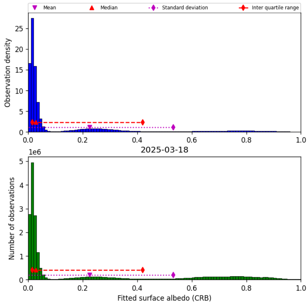
Figure 46: Histogram of “Fitted surface albedo (CRB)” for 2025-03-17 to 2025-03-19
