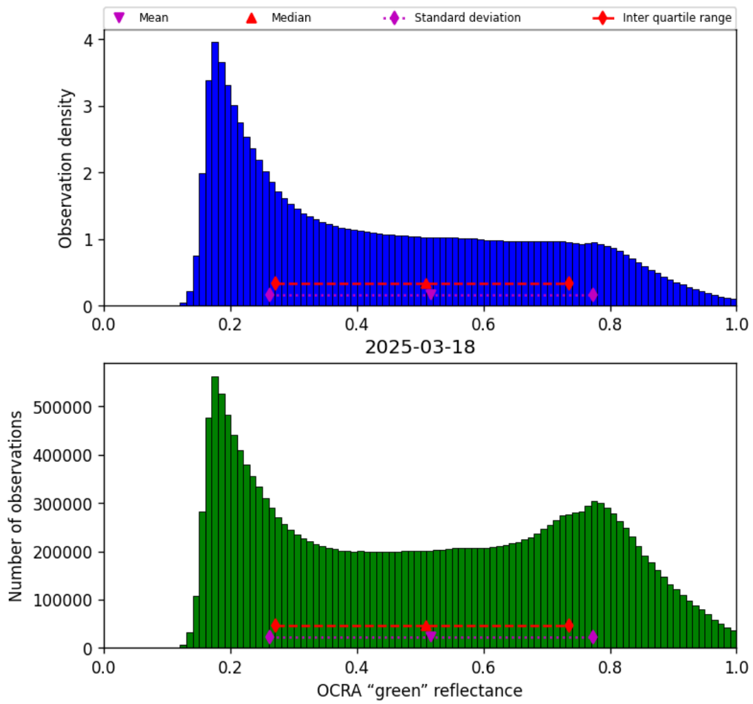
Figure 52: Histogram of “OCRA “green” reflectance” for 2025-03-17 to 2025-03-19
