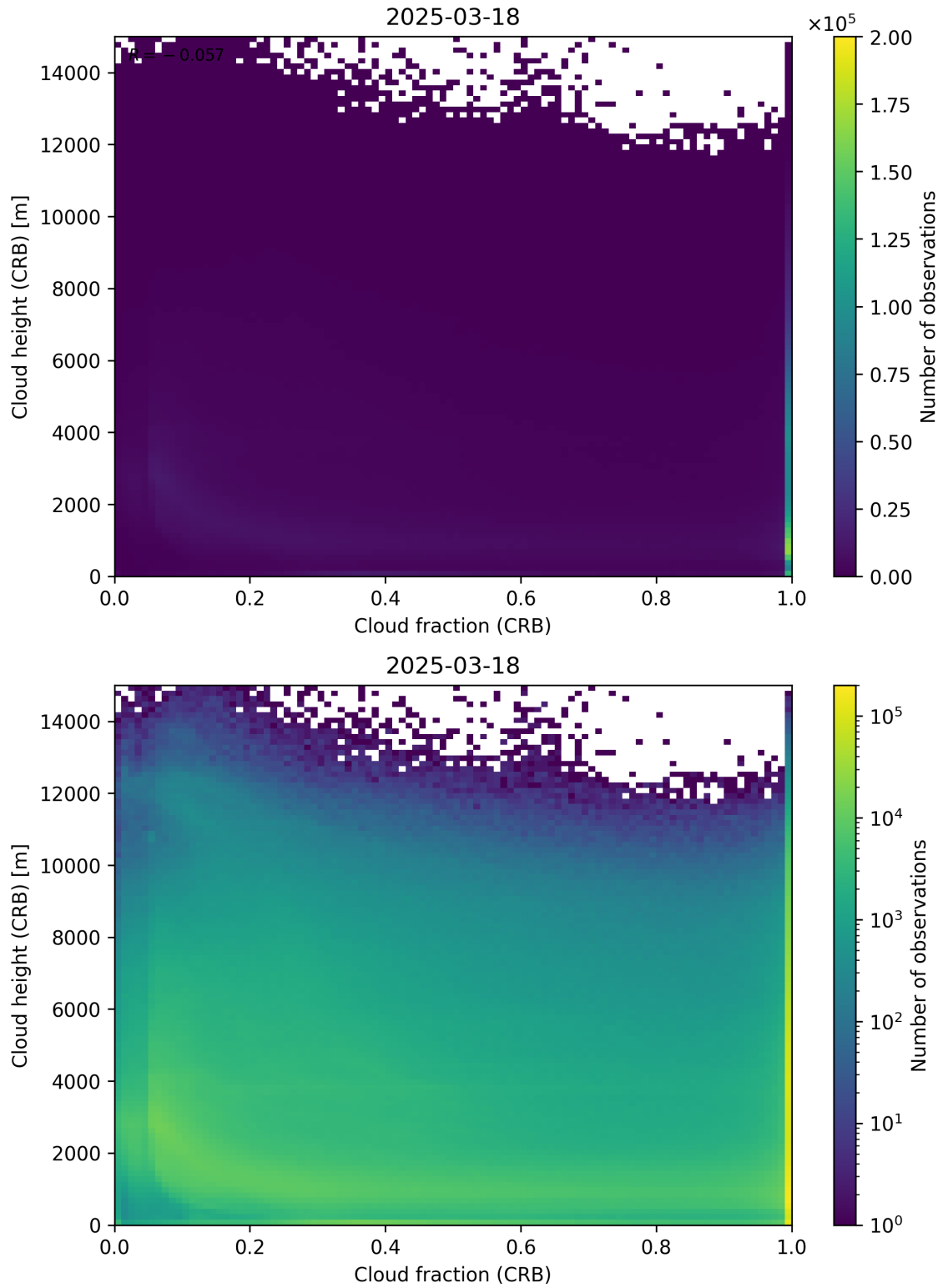
Figure 79: Scatter density plot of “Cloud fraction (CRB)” against “Cloud height (CRB)” for 2025-03-17 to 2025-03-19.
