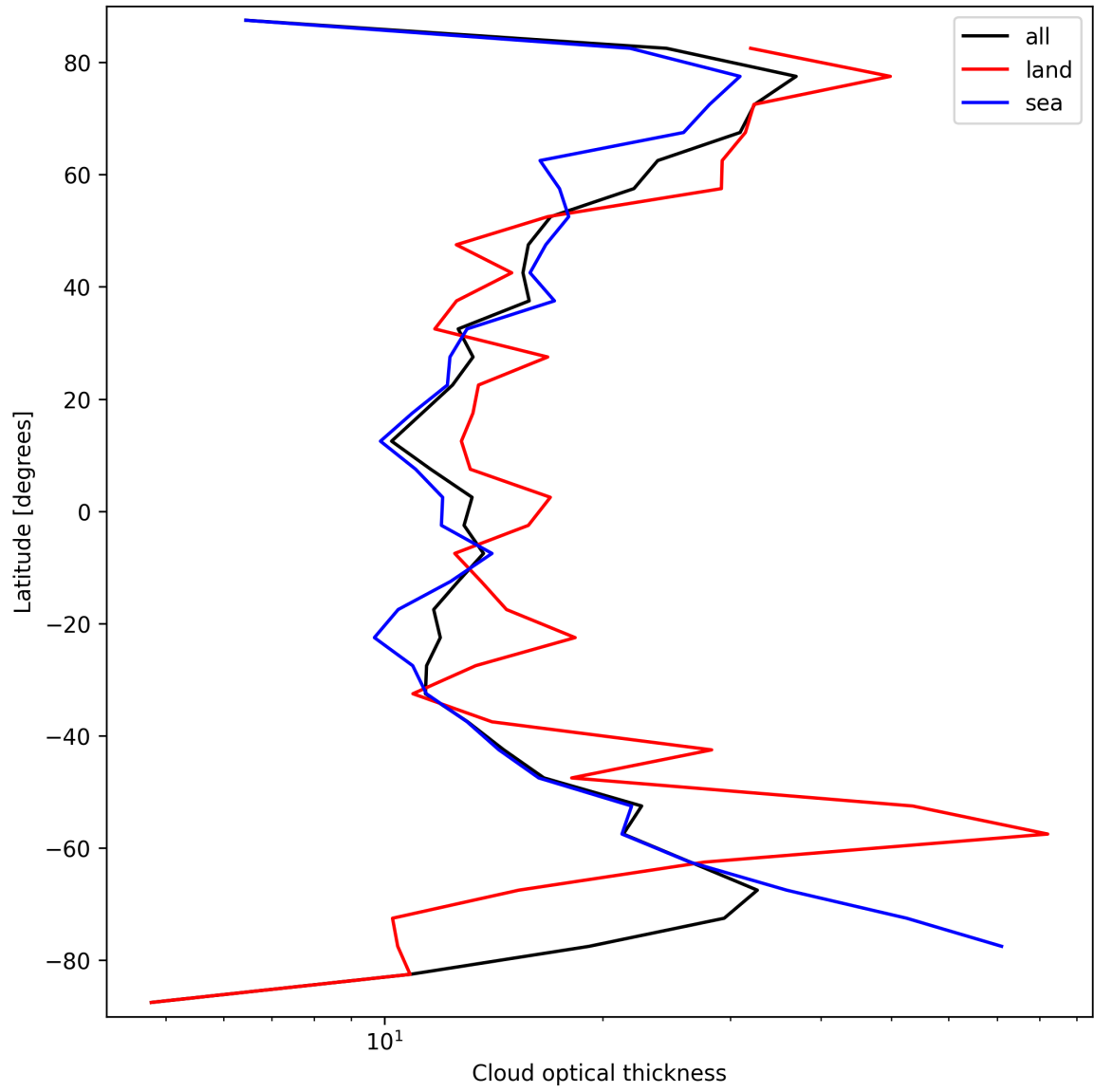
Figure 25: Zonal average of “Cloud optical thickness” for 2025-03-17 to 2025-03-19.
