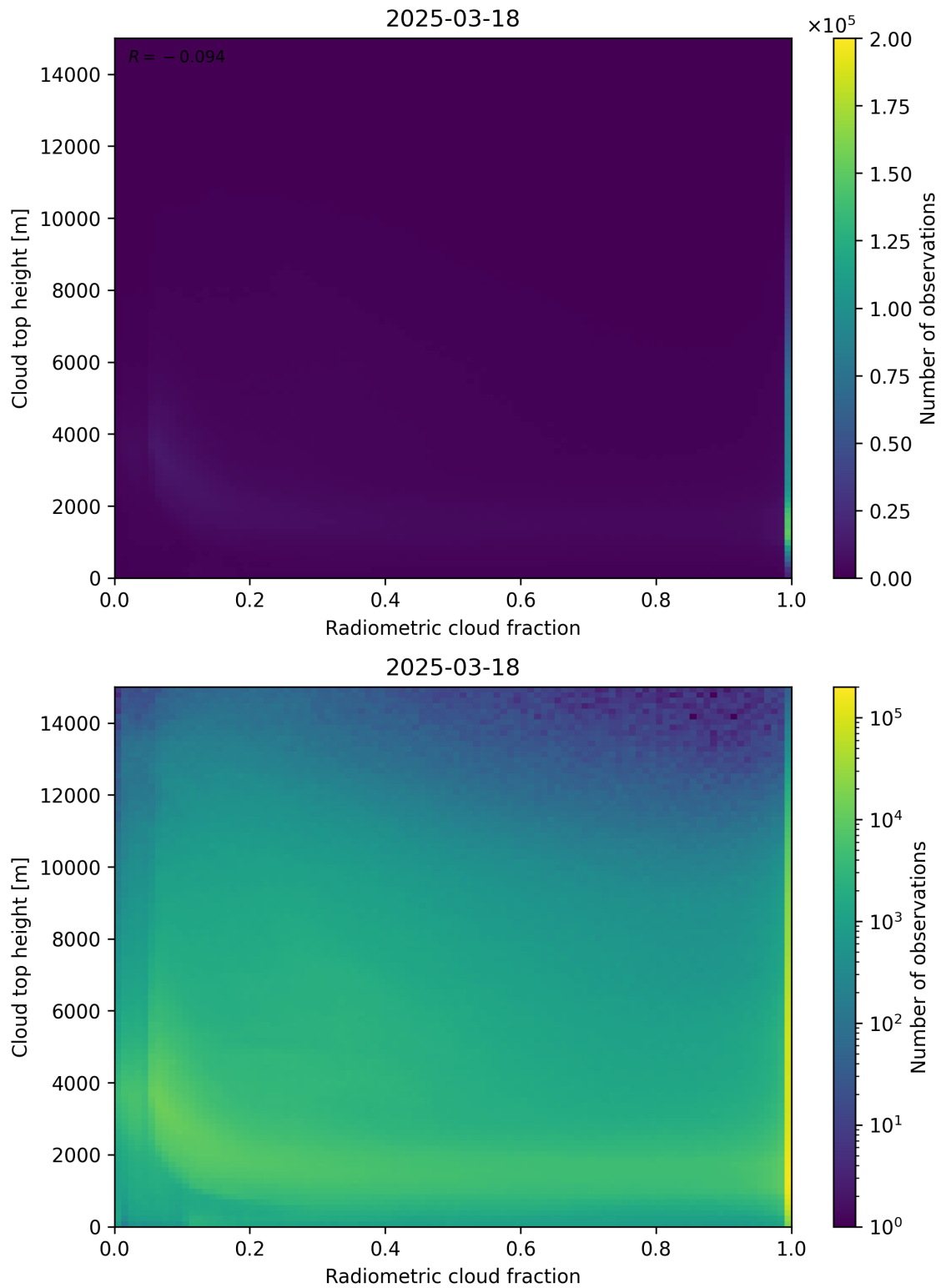
Figure 76: Scatter density plot of “Radiometric cloud fraction” against “Cloud top height” for 2025-03-17 to 2025-03-19.
