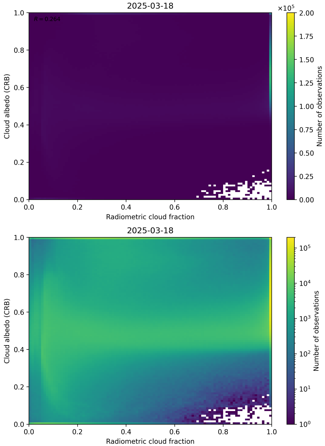
Figure 71: Scatter density plot of “Radiometric cloud fraction” against “Cloud albedo (CRB)” for 2025-03-17 to 2025-03-19.
