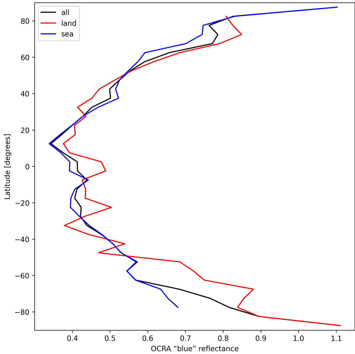
Figure 35: Zonal average of “OCRA “blue” reflectance” for 2025-03-17 to 2025-03-19.
