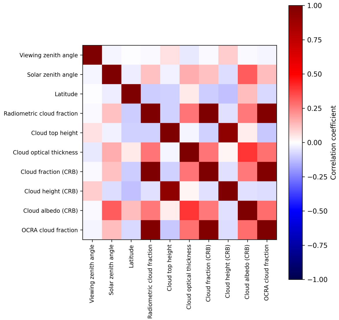
Figure 2: Map of correlation matrix for 2025-03-17 to 2025-03-19.
