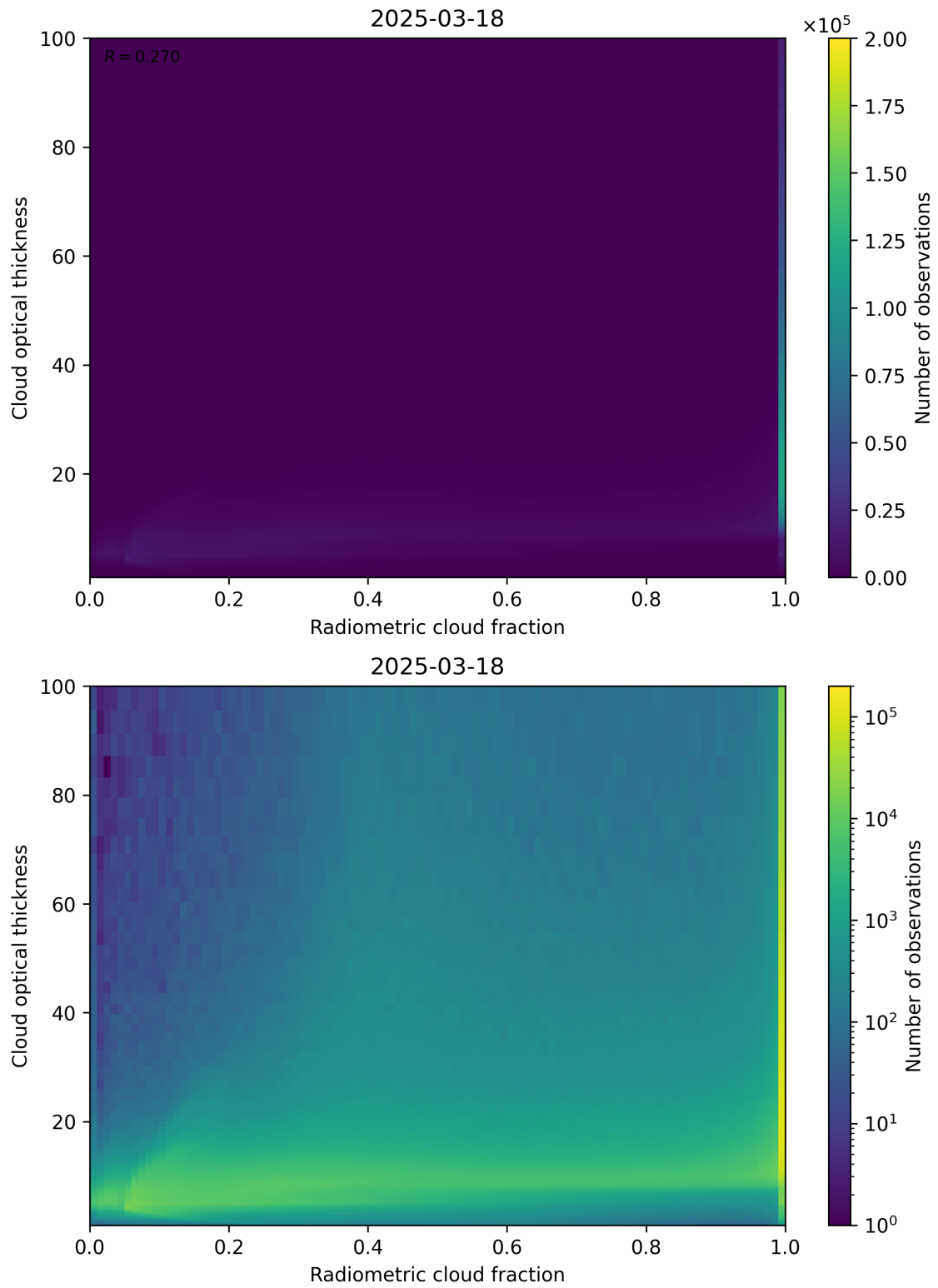
Figure 75: Scatter density plot of “Radiometric cloud fraction” against “Cloud optical thickness” for 2025-03-17 to 2025-03-19.
