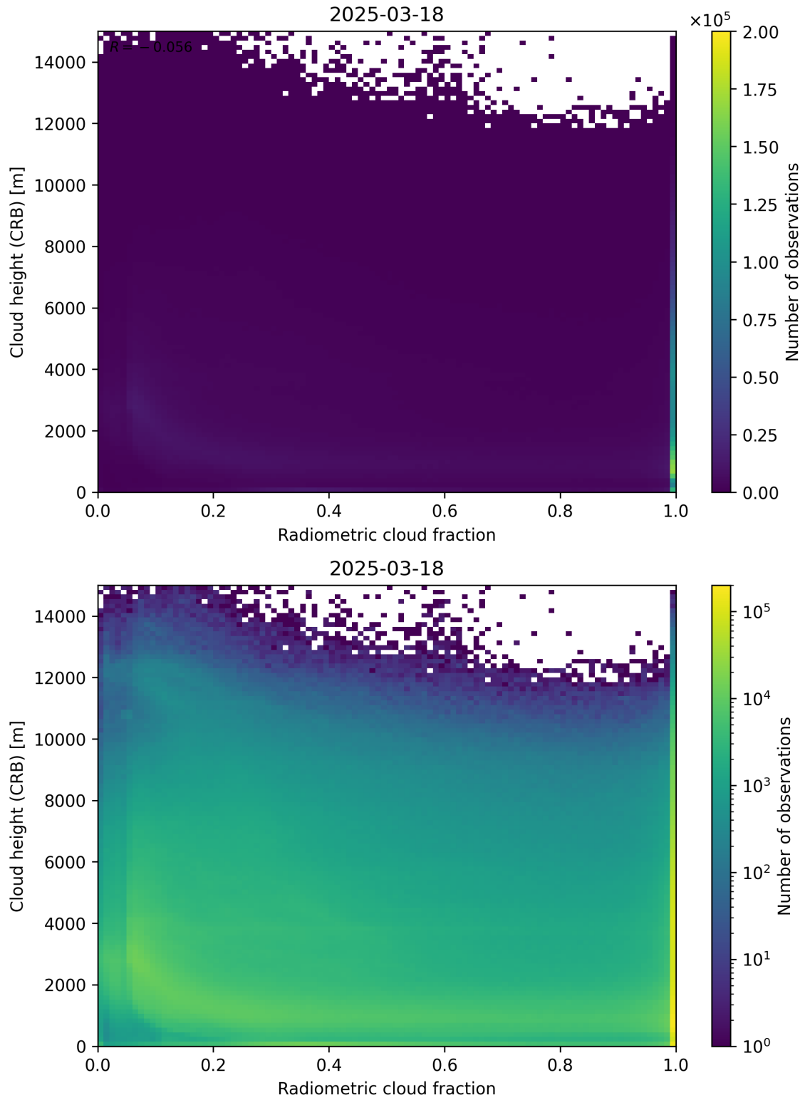
Figure 74: Scatter density plot of “Radiometric cloud fraction” against “Cloud height (CRB)” for 2025-03-17 to 2025-03-19.
