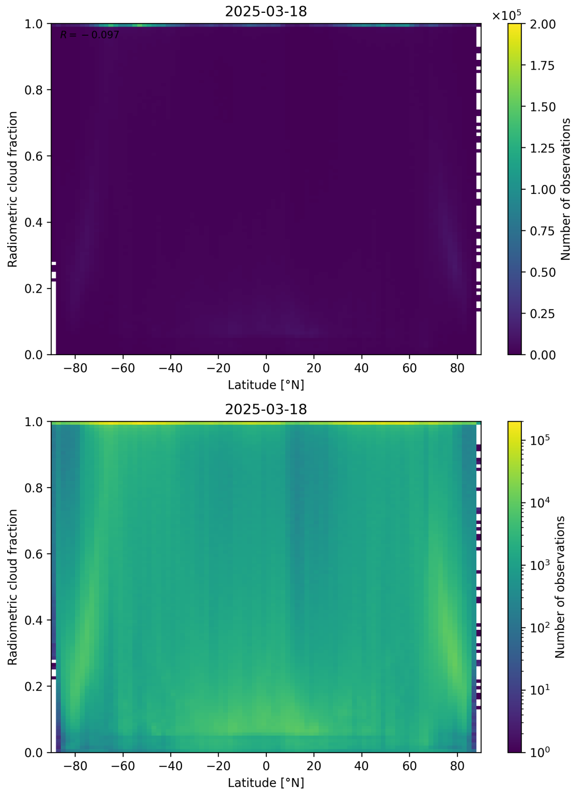
Figure 92: Scatter density plot of “Latitude” against “Radiometric cloud fraction” for 2025-03-17 to 2025-03-19.
