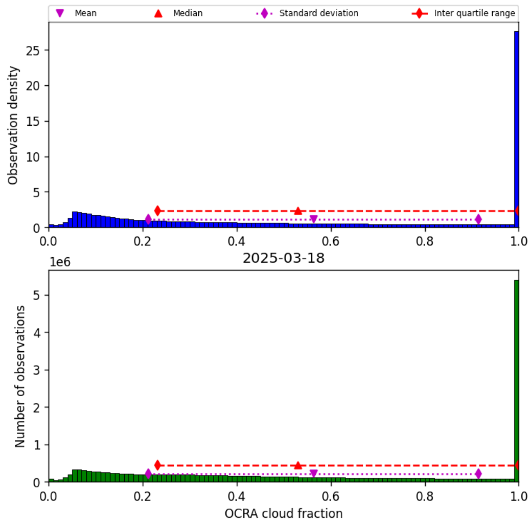
Figure 50: Histogram of “OCRA cloud fraction” for 2025-03-17 to 2025-03-19
