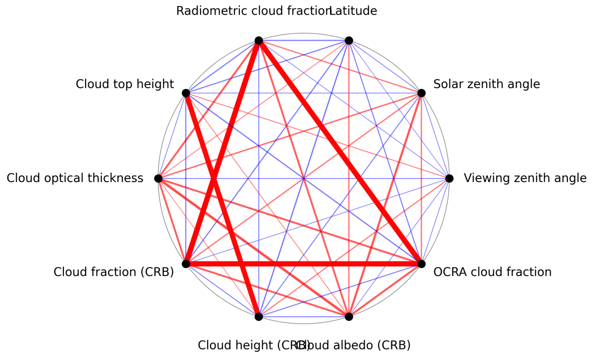
Figure 1: Map of correlation graph for 2025-03-17 to 2025-03-19.
