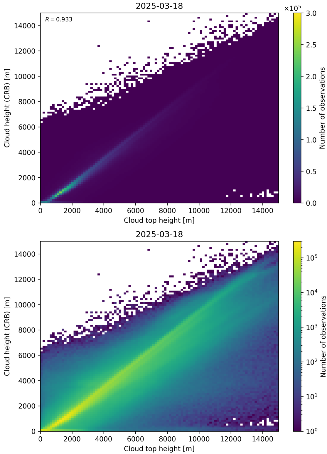
Figure 89: Scatter density plot of “Cloud top height” against “Cloud height (CRB)” for 2025-03-17 to 2025-03-19.
