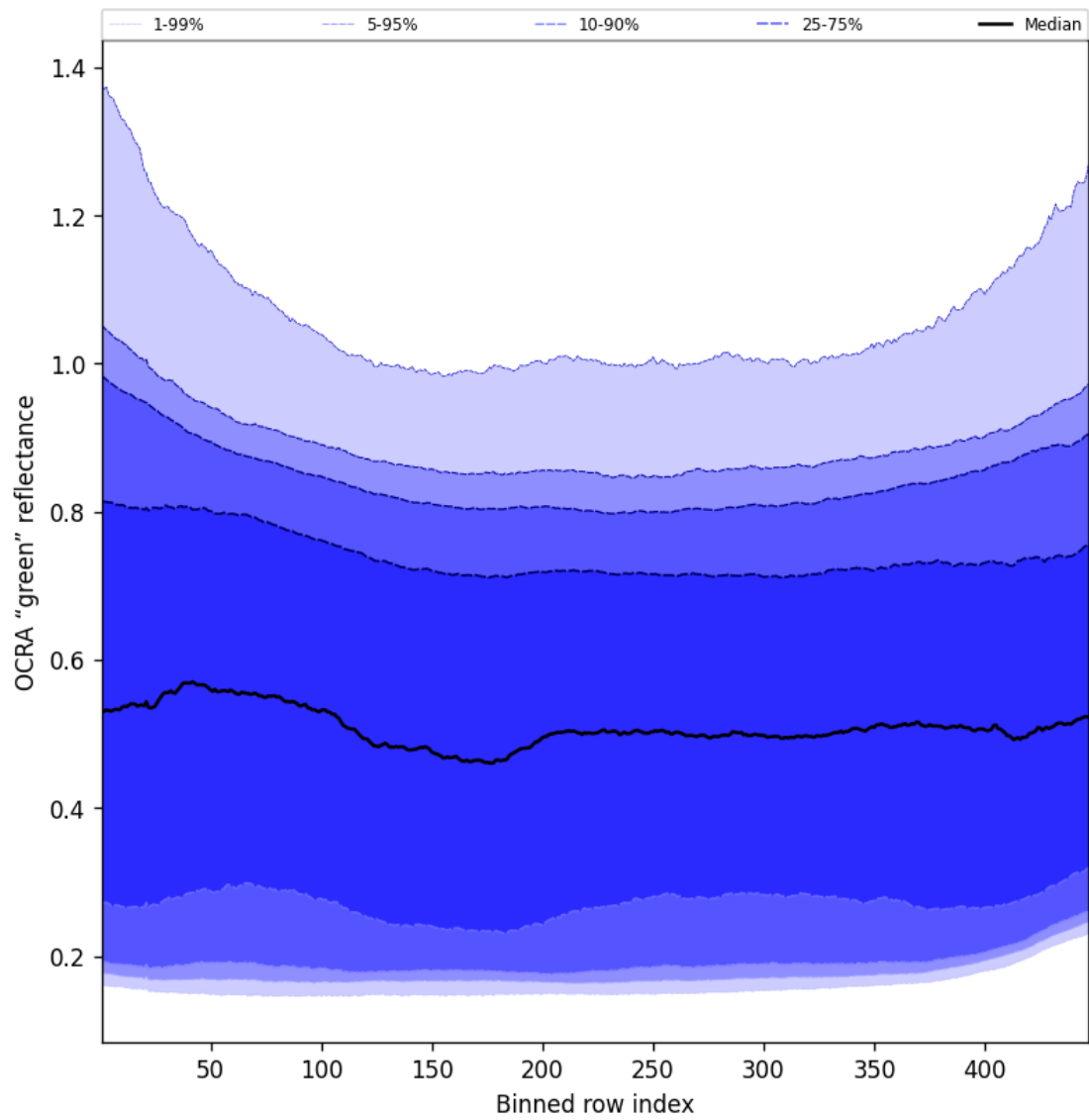
Figure 68: Along track statistics of “OCRA “green” reflectance” for 2025-03-17 to 2025-03-19
