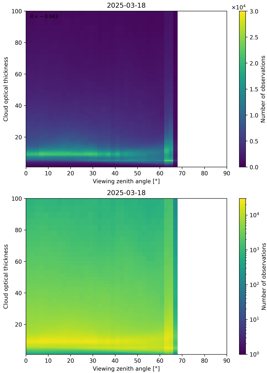
Figure 111: Scatter density plot of “Viewing zenith angle” against “Cloud optical thickness” for 2025-03-17 to 2025-03-19.
