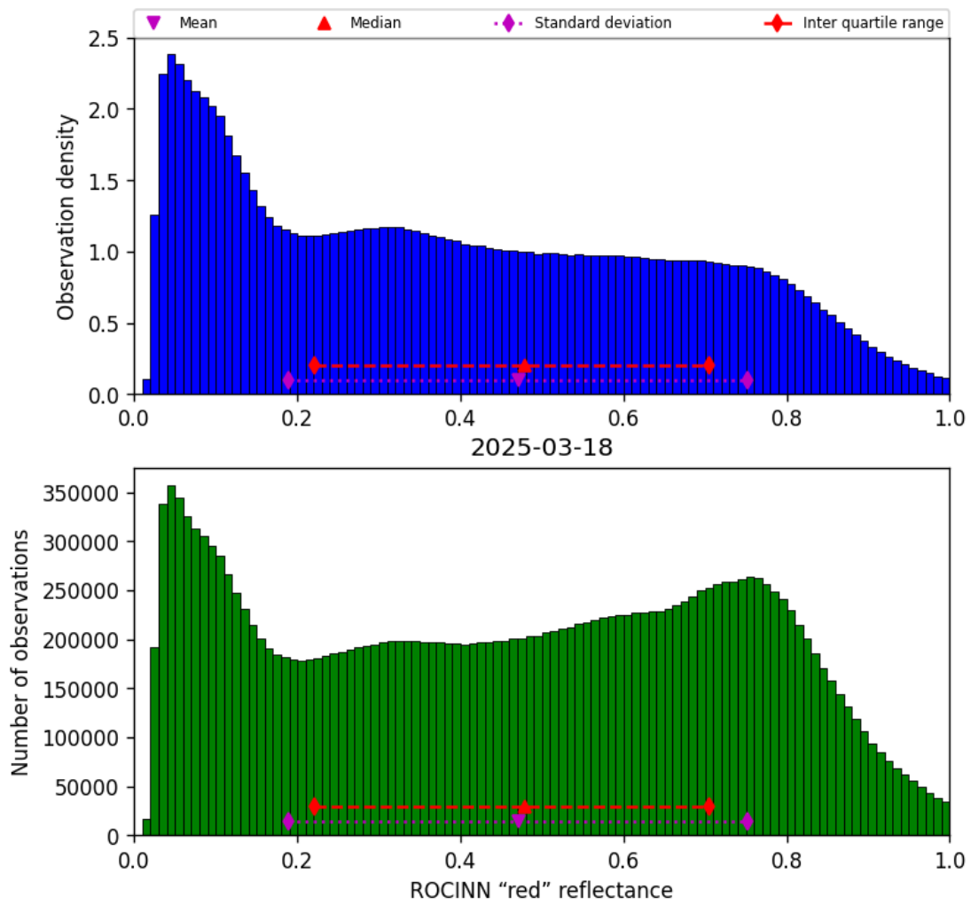
Figure 53: Histogram of “ROCINN “red” reflectance” for 2025-03-17 to 2025-03-19
