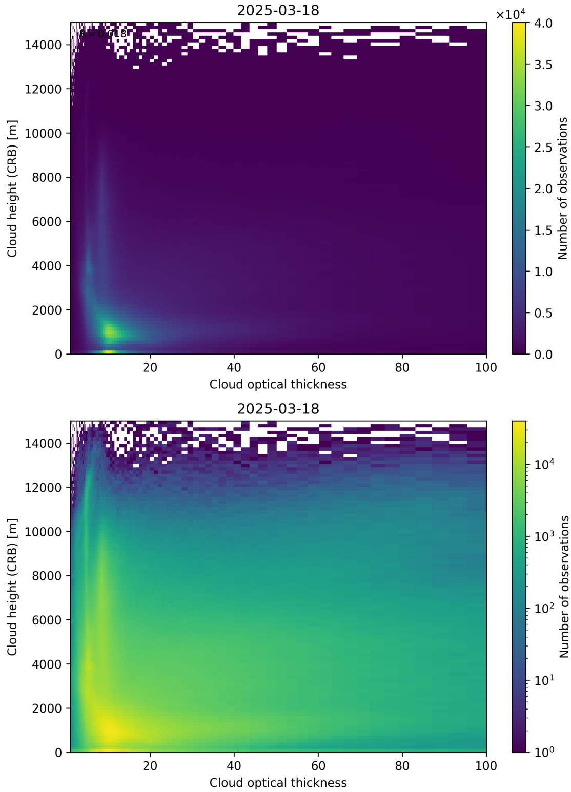
Figure 85: Scatter density plot of “Cloud optical thickness” against “Cloud height (CRB)” for 2025-03-17 to 2025-03-19.
