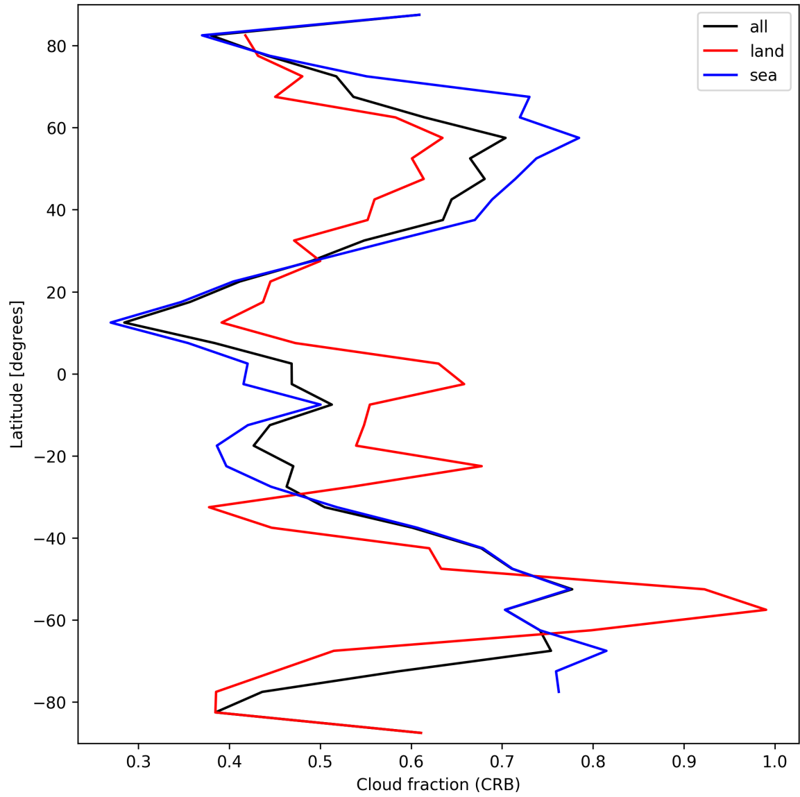
Figure 26: Zonal average of “Cloud fraction (CRB)” for 2025-03-17 to 2025-03-19.
