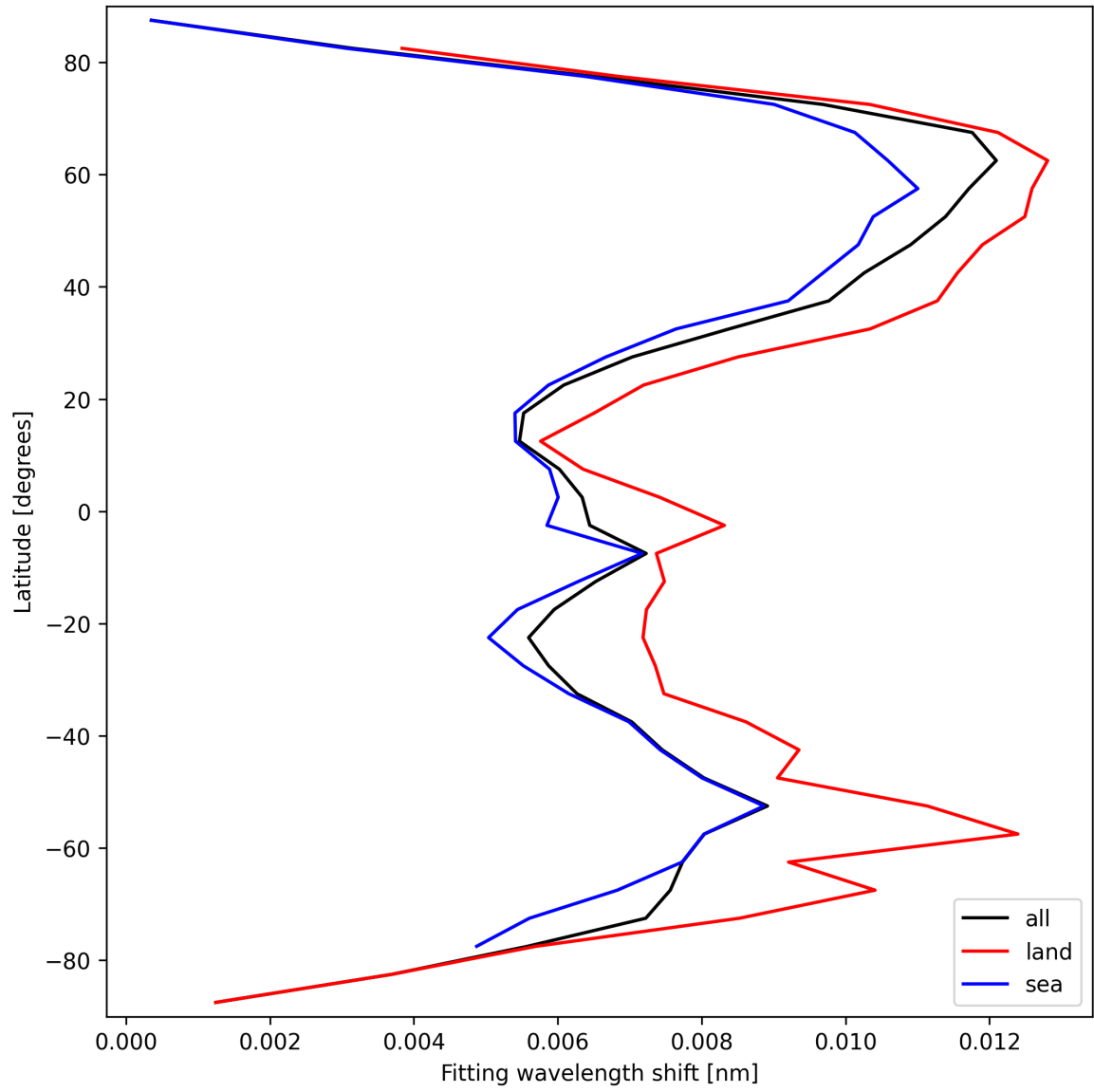
Figure 33: Zonal average of “Fitting wavelength shift” for 2025-03-17 to 2025-03-19.
