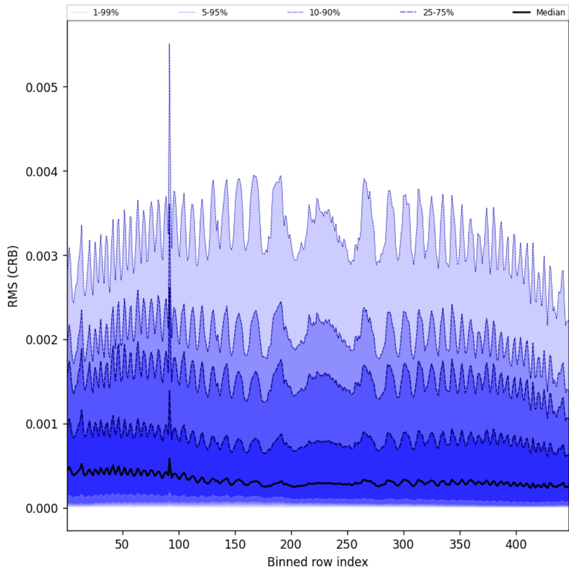
Figure 64: Along track statistics of “RMS (CRB)” for 2025-03-17 to 2025-03-19
