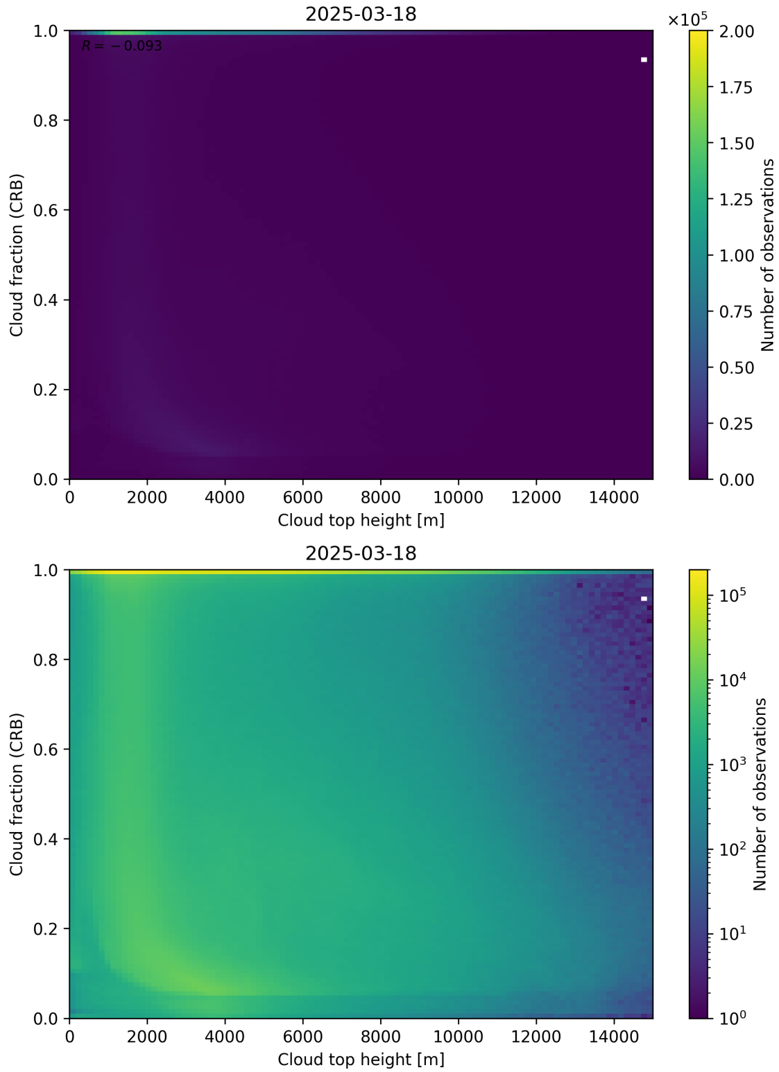
Figure 88: Scatter density plot of “Cloud top height” against “Cloud fraction (CRB)” for 2025-03-17 to 2025-03-19.
