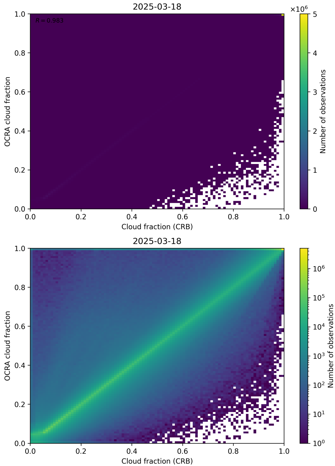
Figure 78: Scatter density plot of “Cloud fraction (CRB)” against “OCRA cloud fraction” for 2025-03-17 to 2025-03-19.
