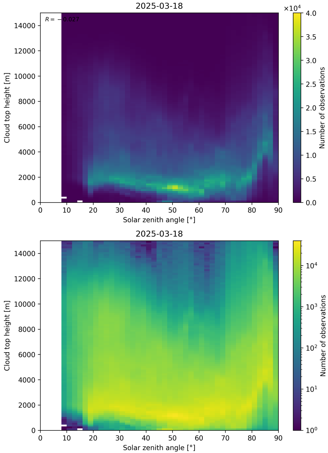
Figure 104: Scatter density plot of “Solar zenith angle” against “Cloud top height” for 2025-03-17 to 2025-03-19.
