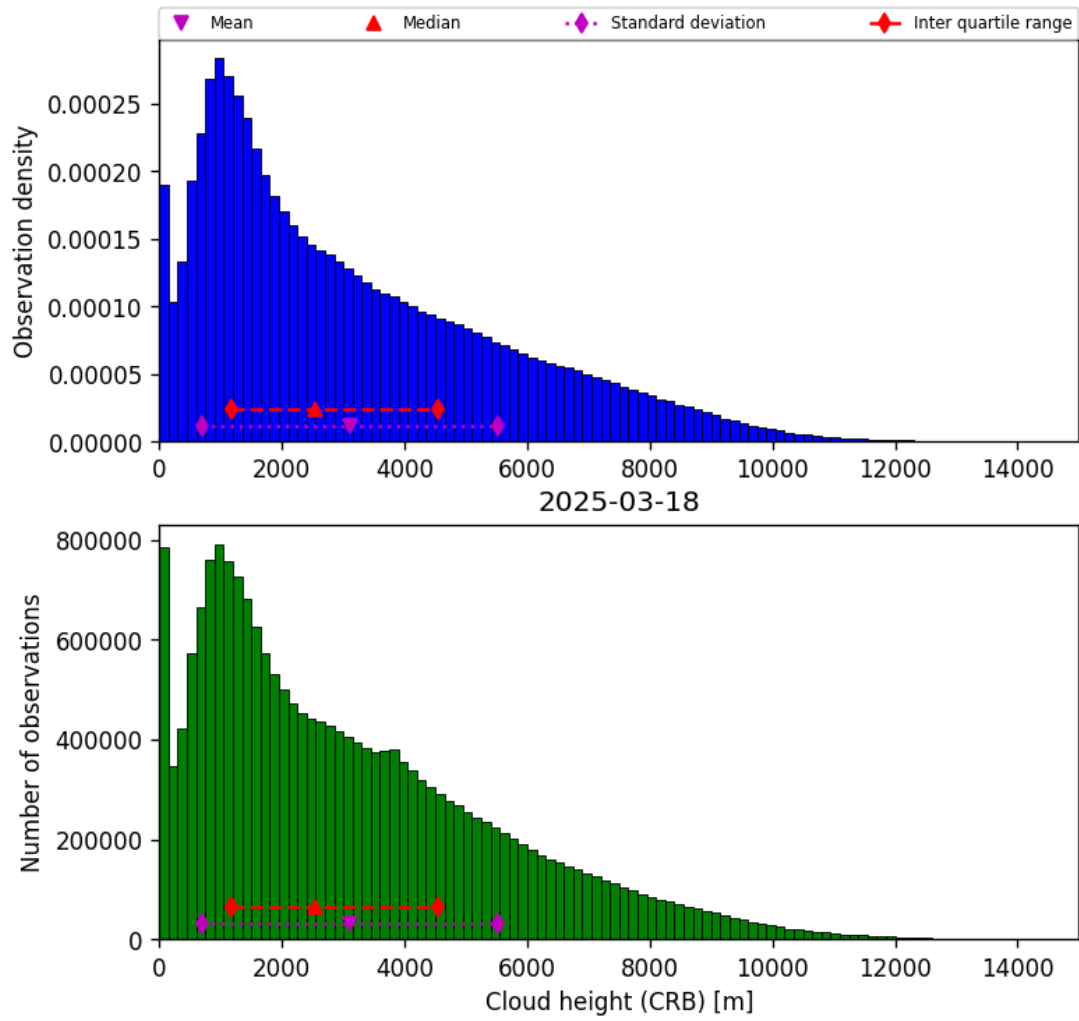
Figure 43: Histogram of “Cloud height (CRB)” for 2025-03-17 to 2025-03-19
