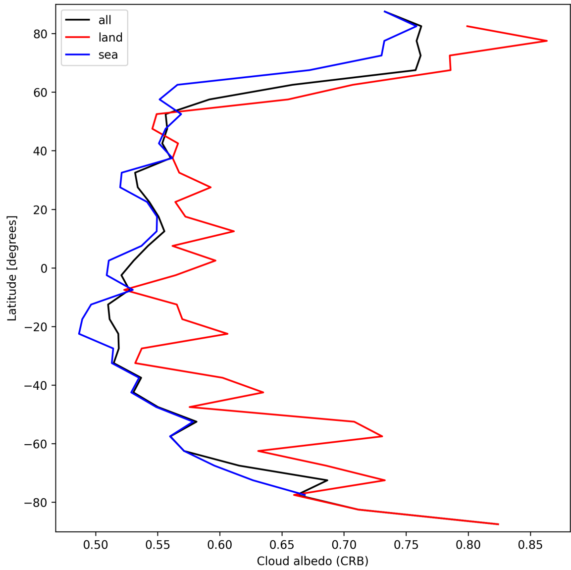
Figure 28: Zonal average of “Cloud albedo (CRB)” for 2025-03-17 to 2025-03-19.
