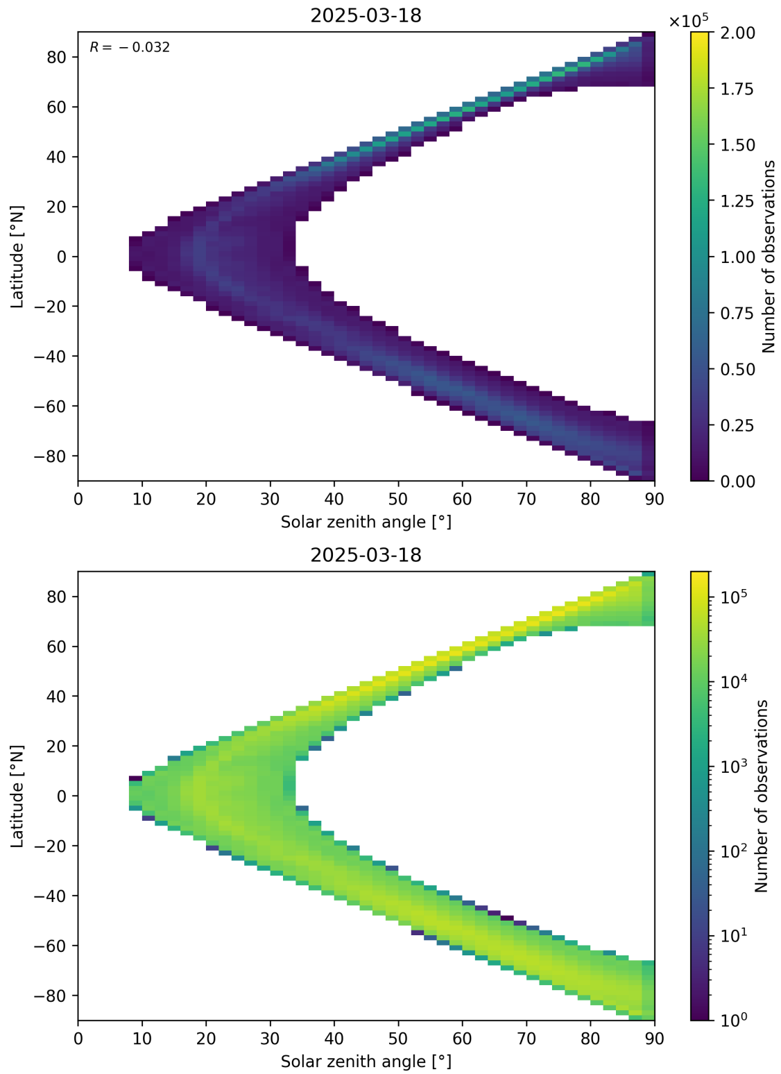
Figure 105: Scatter density plot of “Solar zenith angle” against “Latitude” for 2025-03-17 to 2025-03-19.
