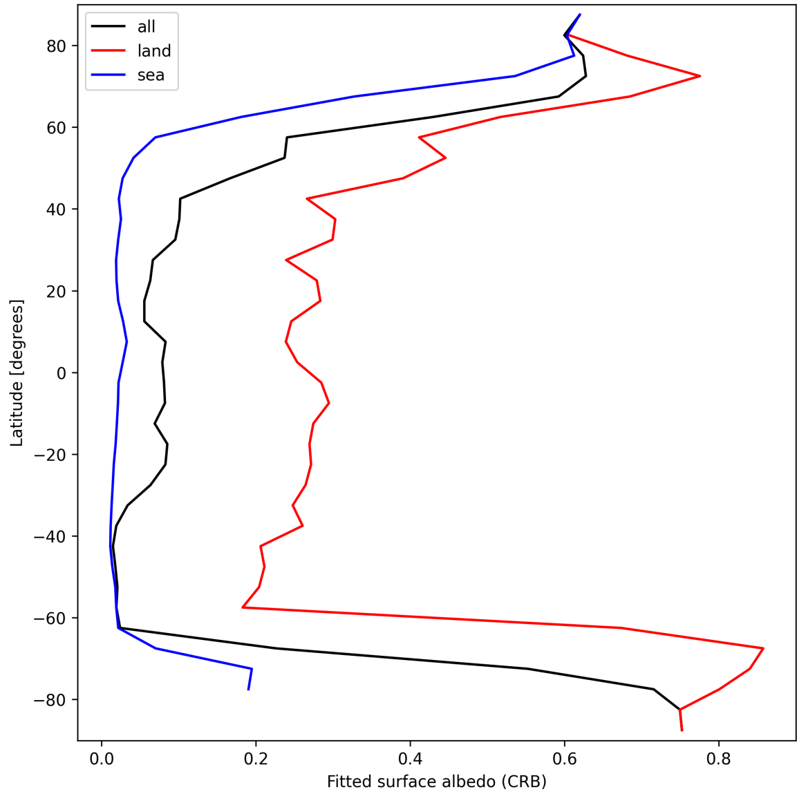
Figure 30: Zonal average of “Fitted surface albedo (CRB)” for 2025-03-17 to 2025-03-19.
