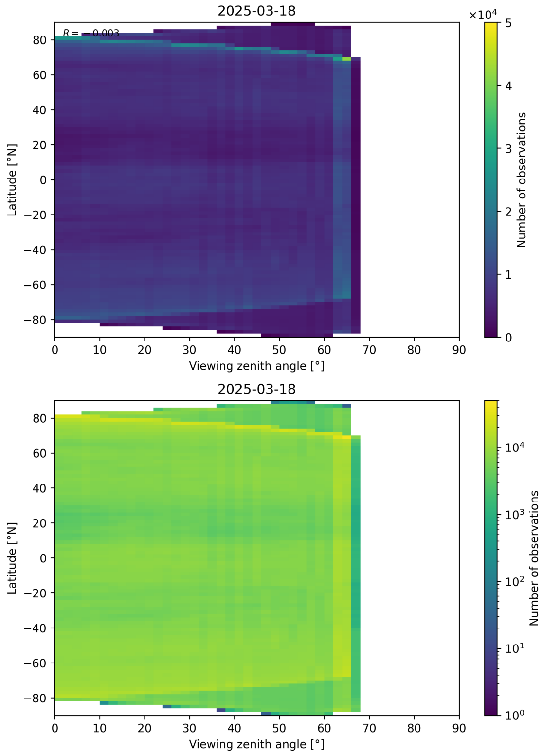
Figure 113: Scatter density plot of “Viewing zenith angle” against “Latitude” for 2025-03-17 to 2025-03-19.
