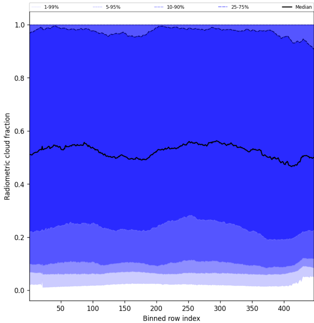
Figure 55: Along track statistics of “Radiometric cloud fraction” for 2025-03-17 to 2025-03-19
