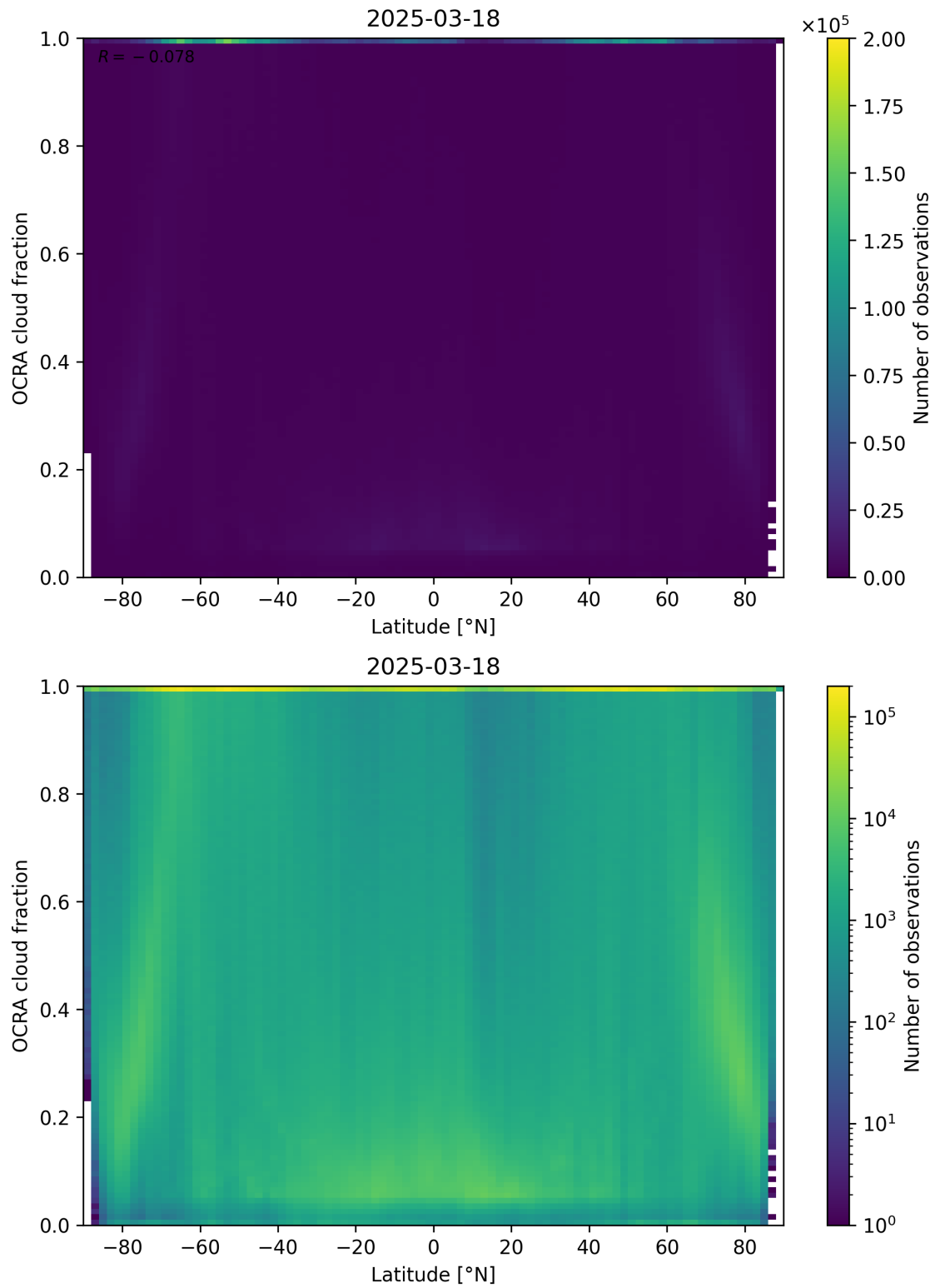
Figure 93: Scatter density plot of “Latitude” against “OCRA cloud fraction” for 2025-03-17 to 2025-03-19.
