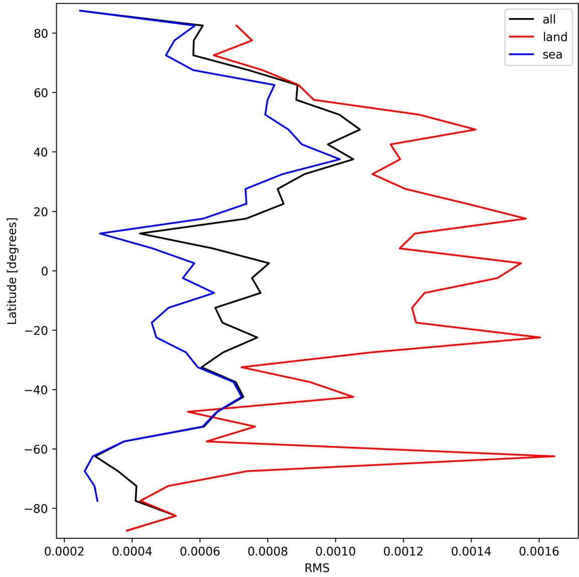
Figure 31: Zonal average of “RMS” for 2025-03-17 to 2025-03-19.
