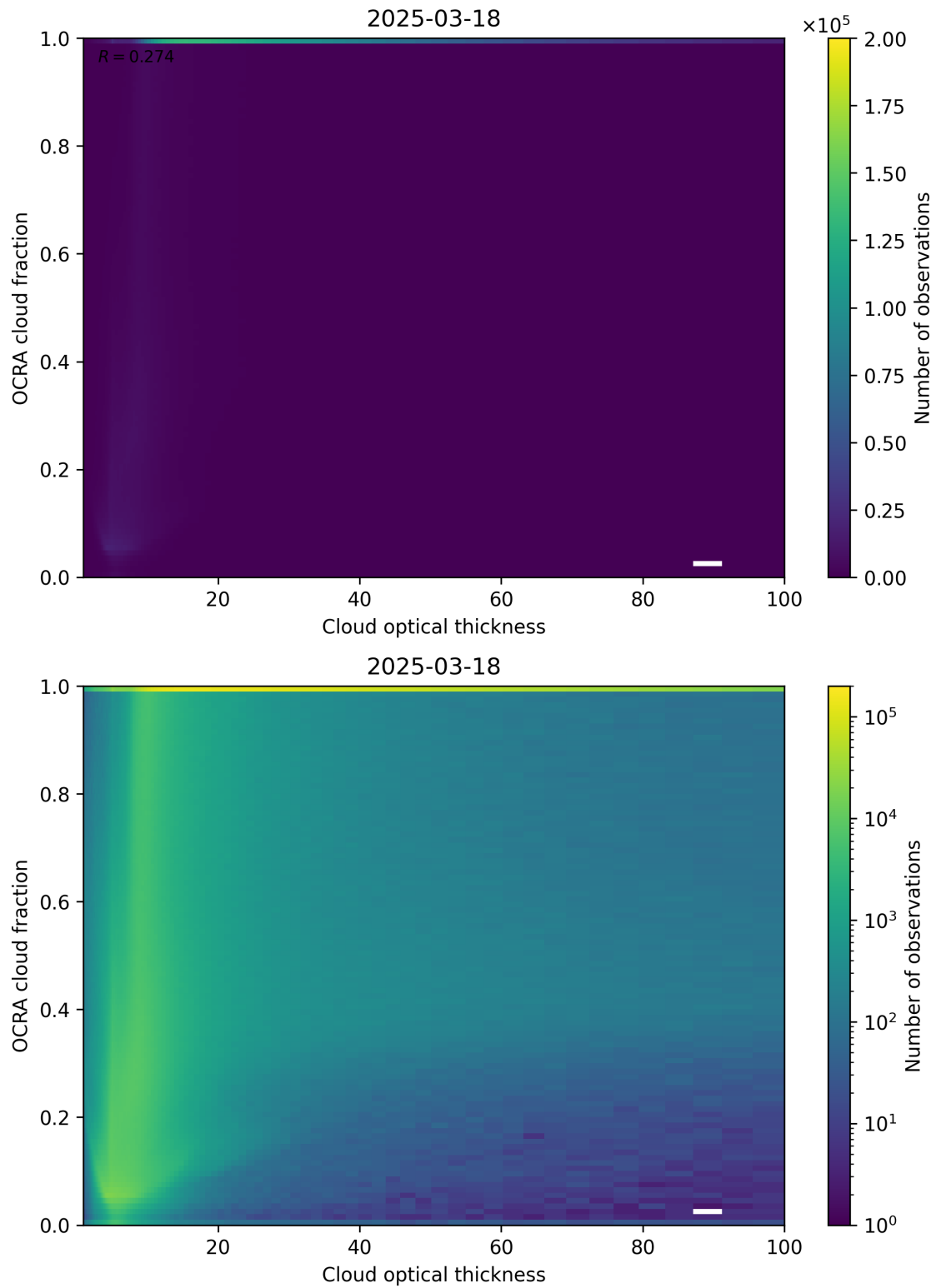
Figure 83: Scatter density plot of “Cloud optical thickness” against “OCRA cloud fraction” for 2025-03-17 to 2025-03-19.
