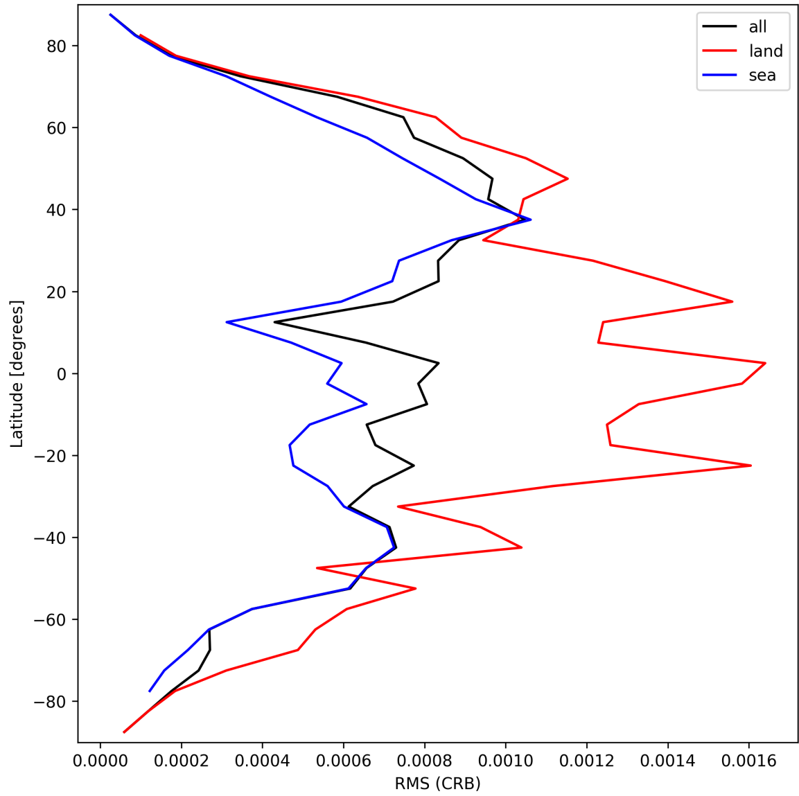
Figure 32: Zonal average of “RMS (CRB)” for 2025-03-17 to 2025-03-19.
