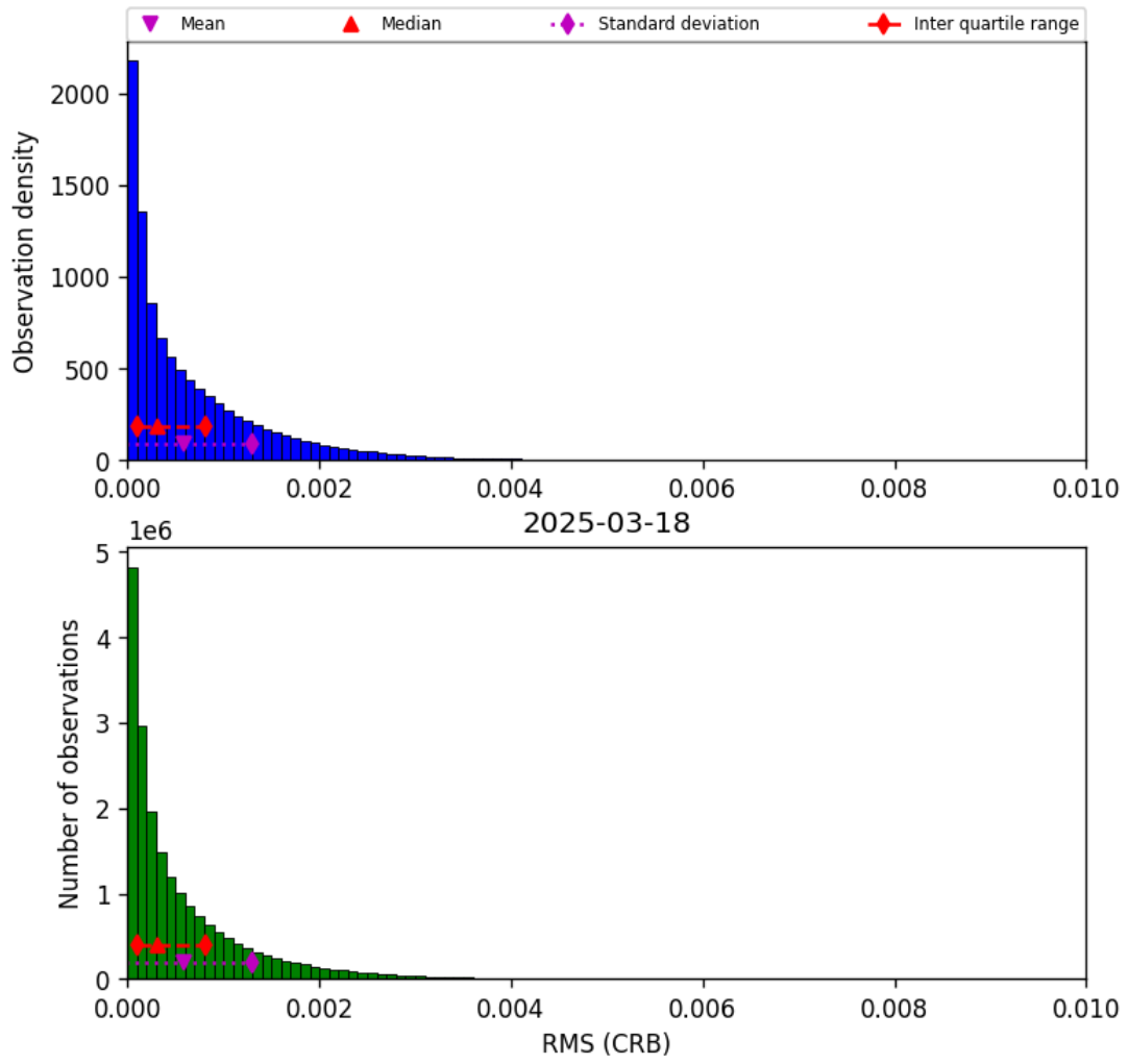
Figure 48: Histogram of “RMS (CRB)” for 2025-03-17 to 2025-03-19
