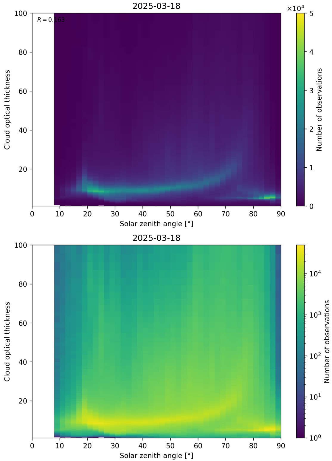
Figure 103: Scatter density plot of “Solar zenith angle” against “Cloud optical thickness” for 2025-03-17 to 2025-03-19.
