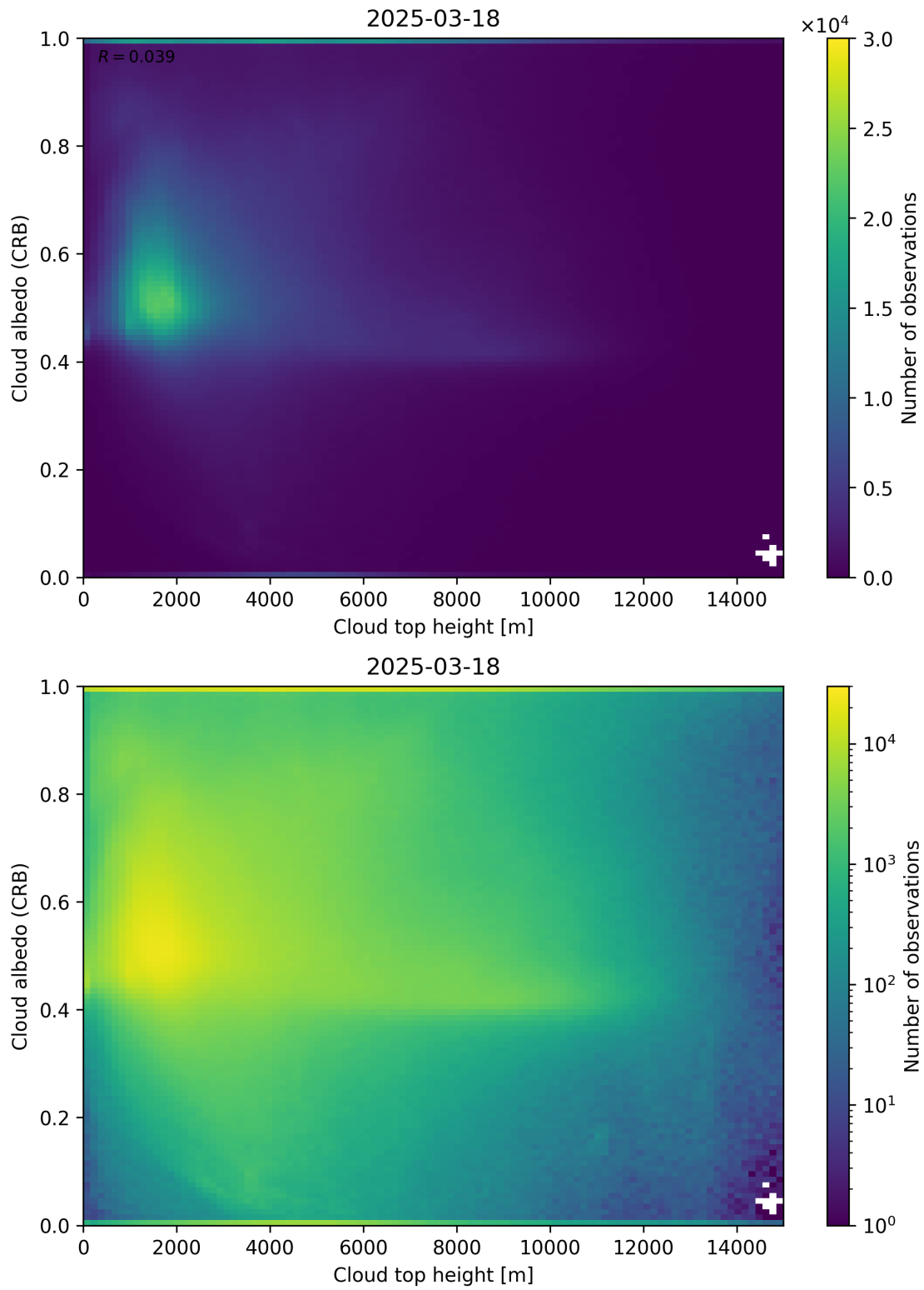
Figure 86: Scatter density plot of “Cloud top height” against “Cloud albedo (CRB)” for 2025-03-17 to 2025-03-19.
