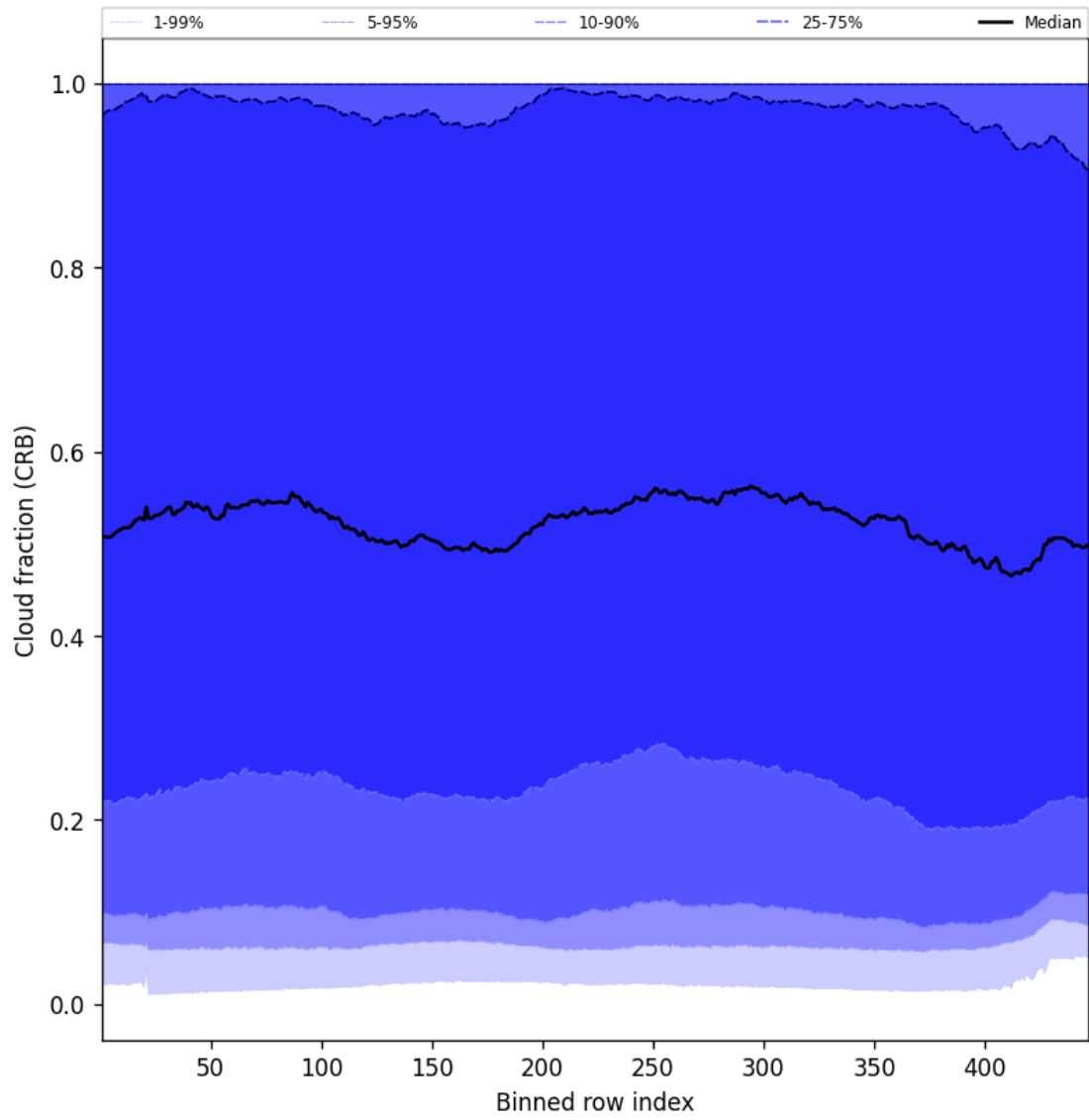
Figure 58: Along track statistics of “Cloud fraction (CRB)” for 2025-03-17 to 2025-03-19
