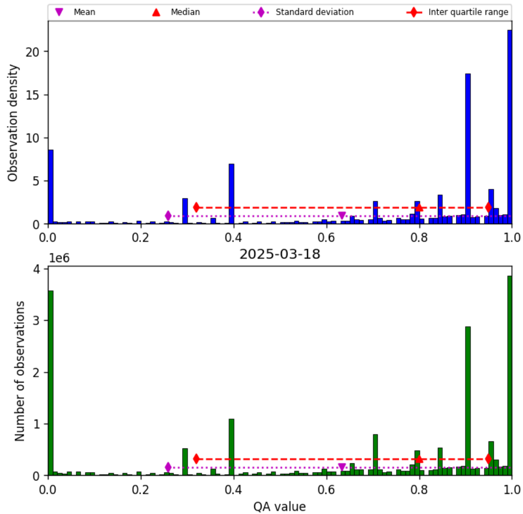
Figure 38: Histogram of “QA value” for 2025-03-17 to 2025-03-19
