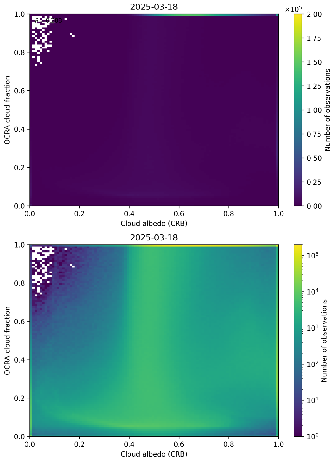
Figure 70: Scatter density plot of “Cloud albedo (CRB)” against “OCRA cloud fraction” for 2025-03-17 to 2025-03-19.
