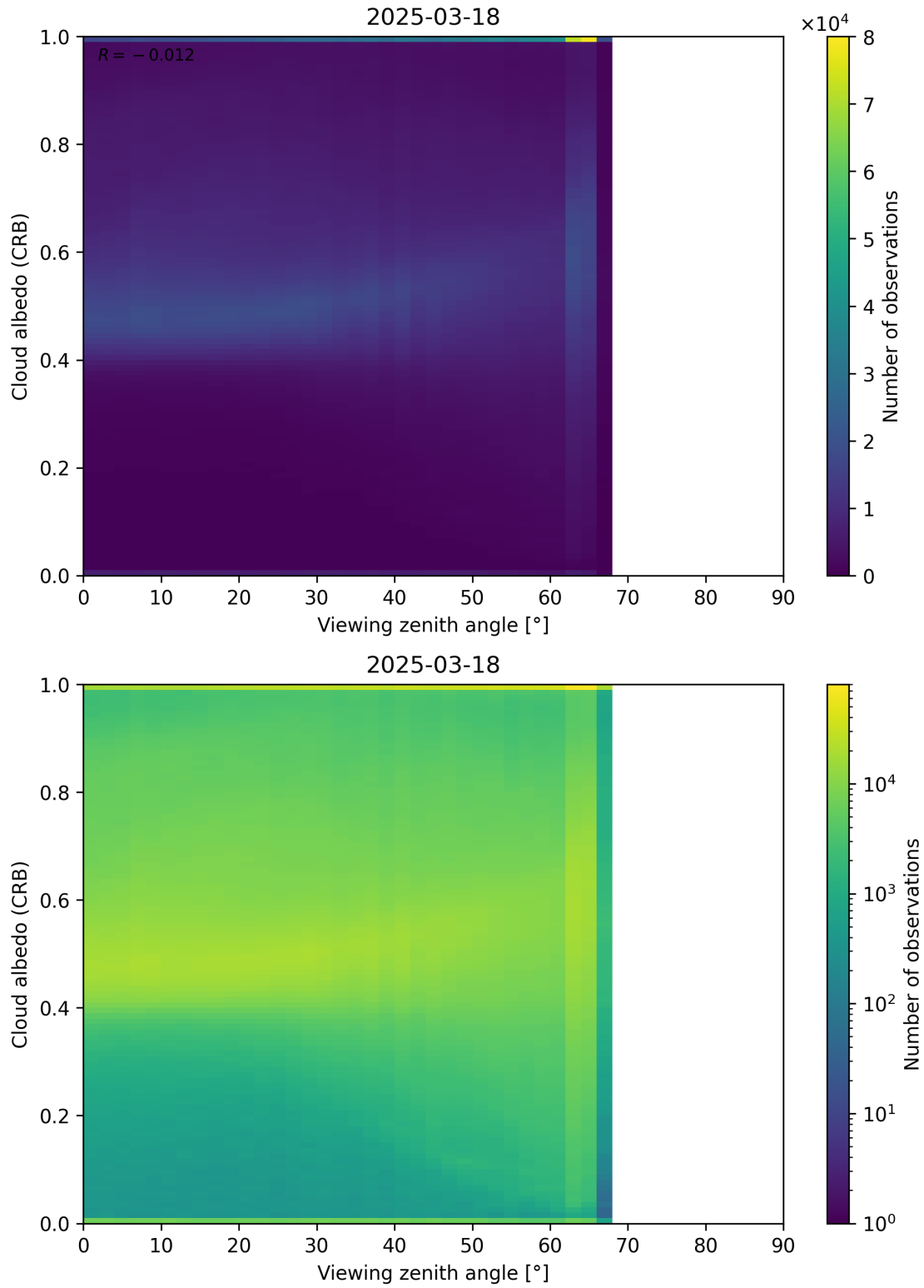
Figure 106: Scatter density plot of “Viewing zenith angle” against “Cloud albedo (CRB)” for 2025-03-17 to 2025-03-19.
