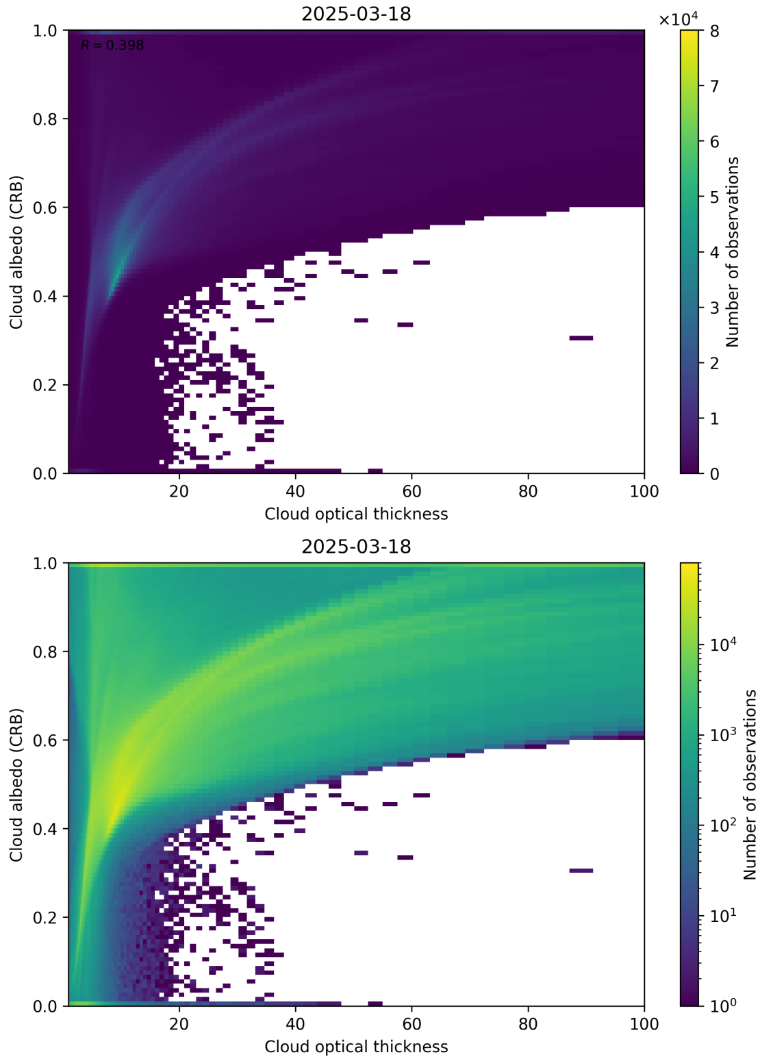
Figure 82: Scatter density plot of “Cloud optical thickness” against “Cloud albedo (CRB)” for 2025-03-17 to 2025-03-19.
