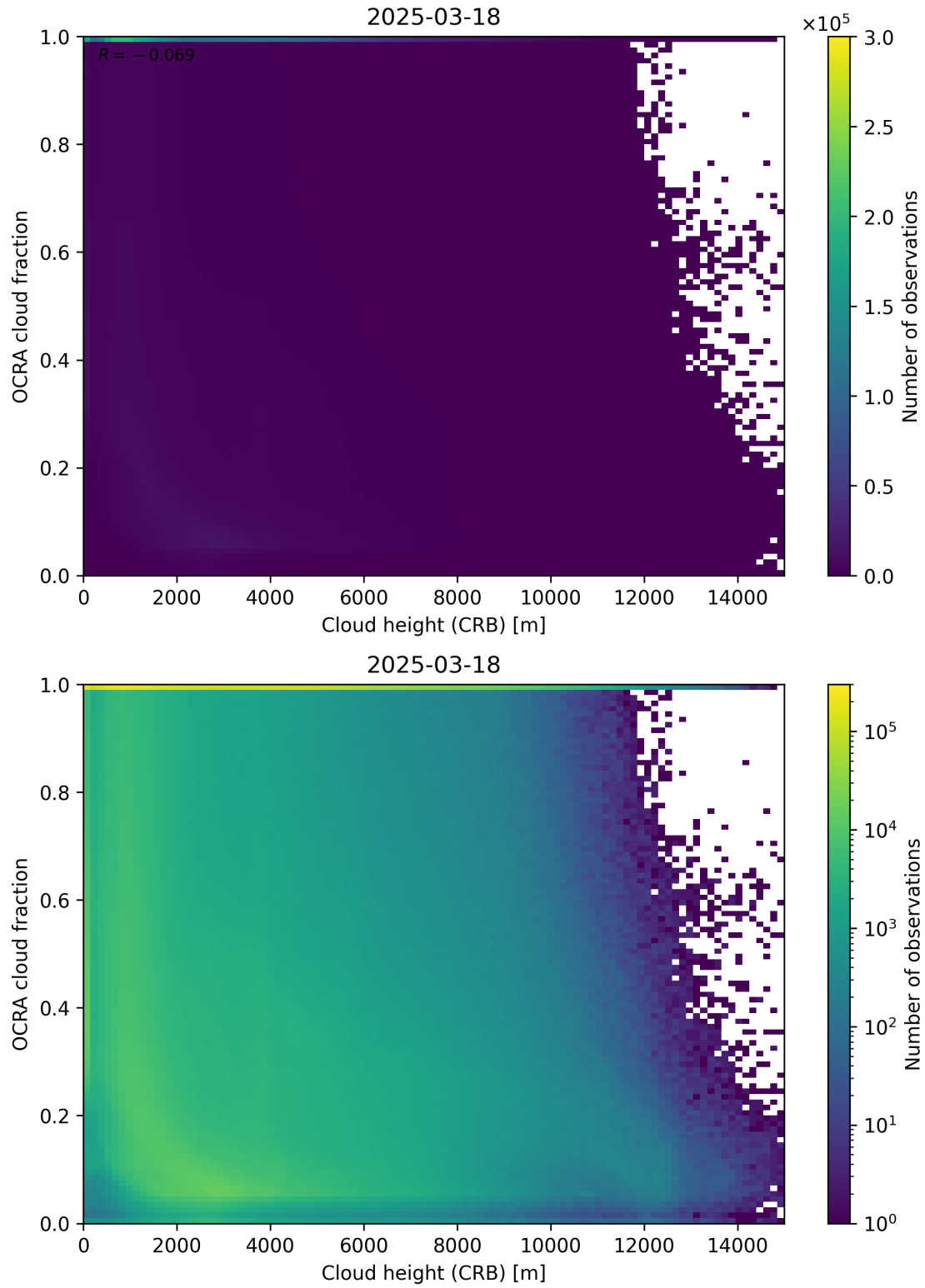
Figure 81: Scatter density plot of “Cloud height (CRB)” against “OCRA cloud fraction” for 2025-03-17 to 2025-03-19.
