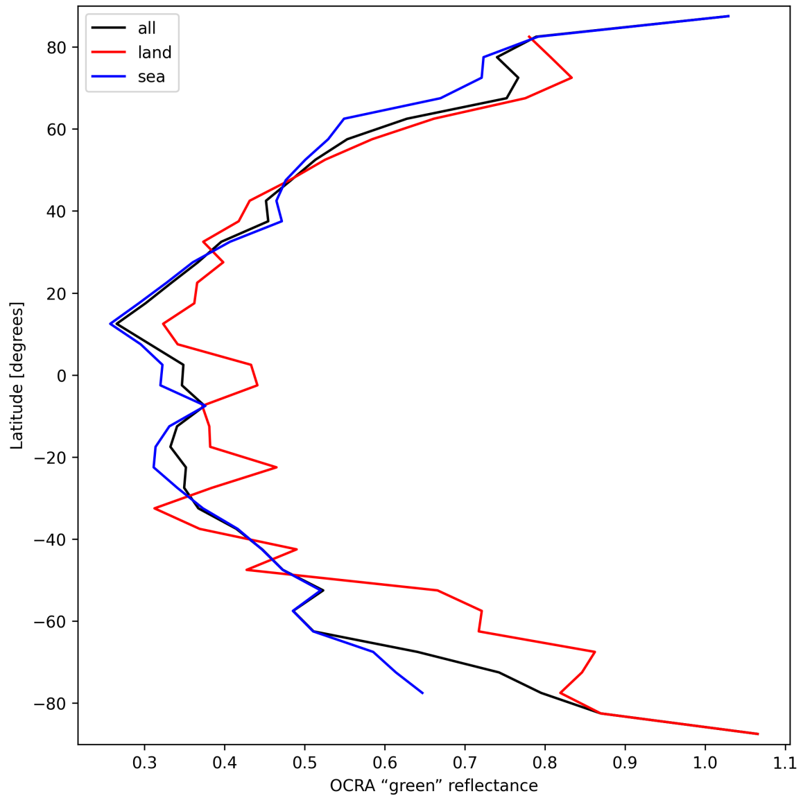
Figure 36: Zonal average of “OCRA “green” reflectance” for 2025-03-17 to 2025-03-19.
