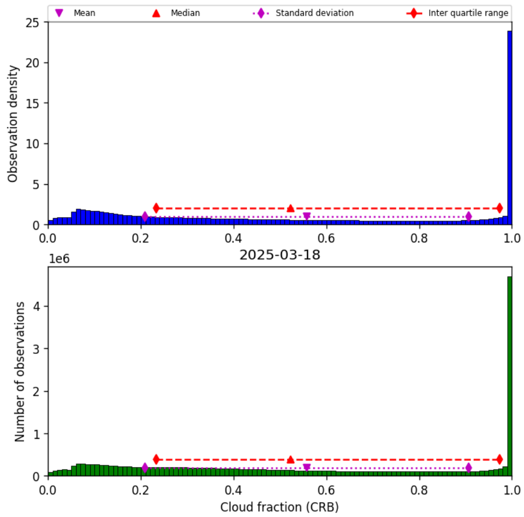
Figure 42: Histogram of “Cloud fraction (CRB)” for 2025-03-17 to 2025-03-19
