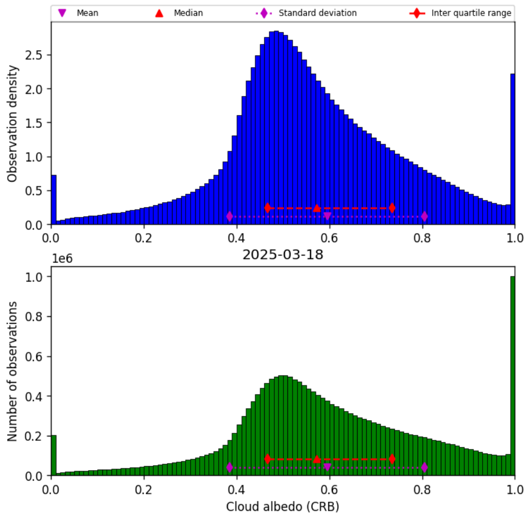
Figure 44: Histogram of “Cloud albedo (CRB)” for 2025-03-17 to 2025-03-19
