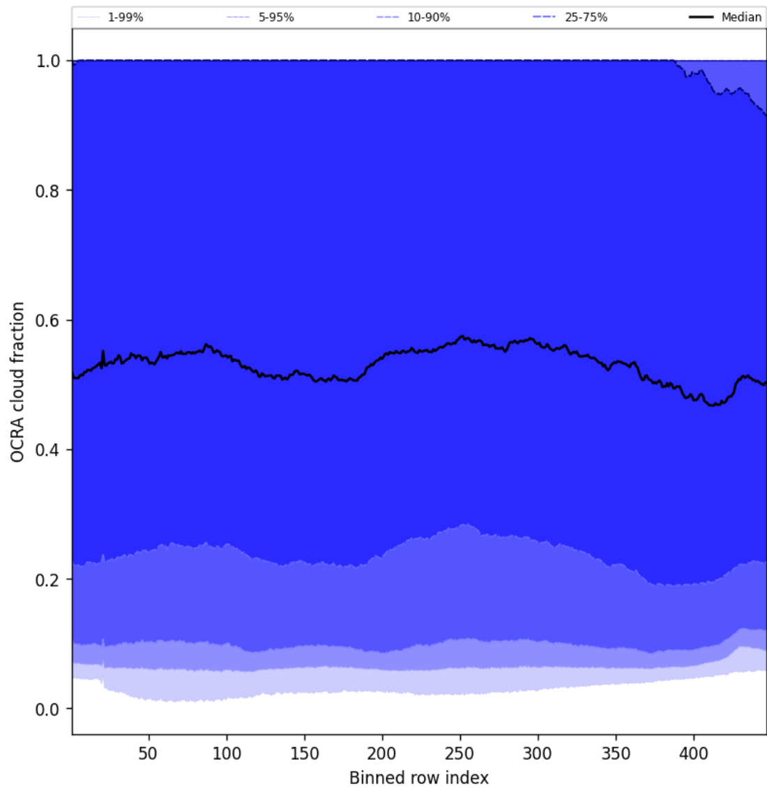
Figure 66: Along track statistics of “OCRA cloud fraction” for 2025-03-17 to 2025-03-19
