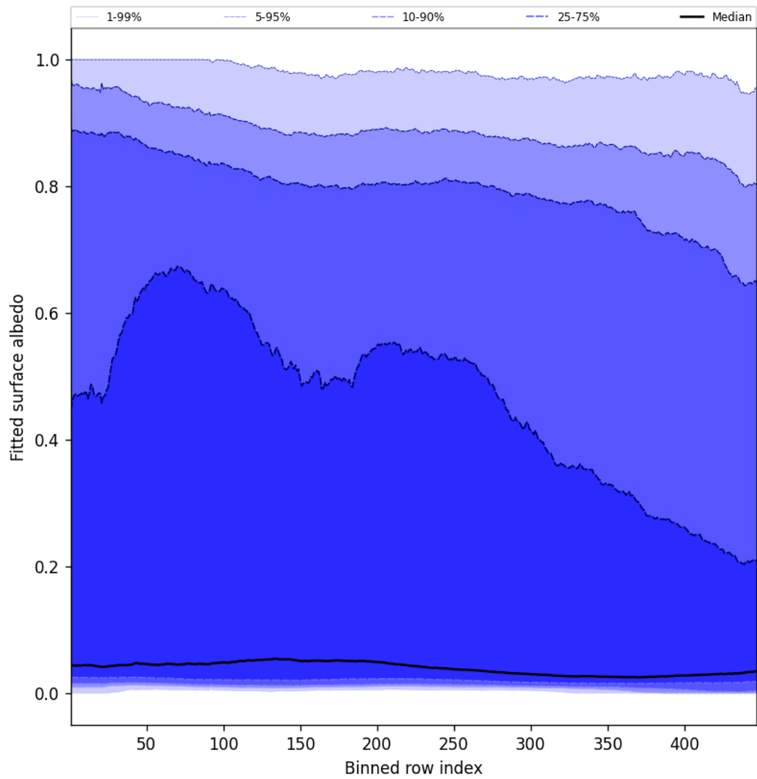
Figure 61: Along track statistics of “Fitted surface albedo” for 2025-03-17 to 2025-03-19
