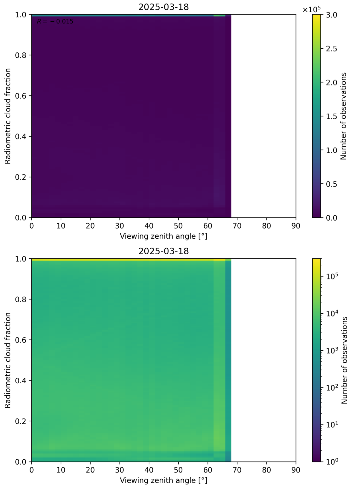
Figure 107: Scatter density plot of “Viewing zenith angle” against “Radiometric cloud fraction” for 2025-03-17 to 2025-03-19.
