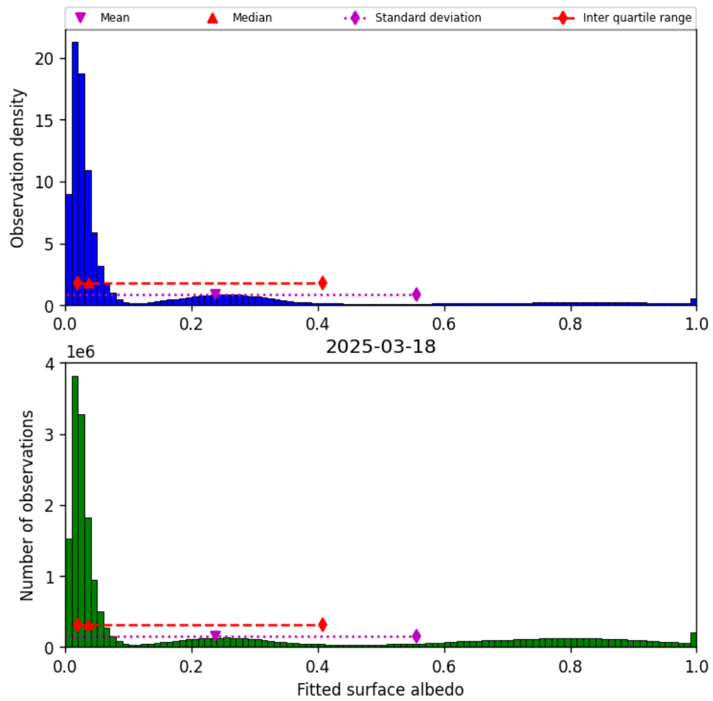
Figure 45: Histogram of “Fitted surface albedo” for 2025-03-17 to 2025-03-19
