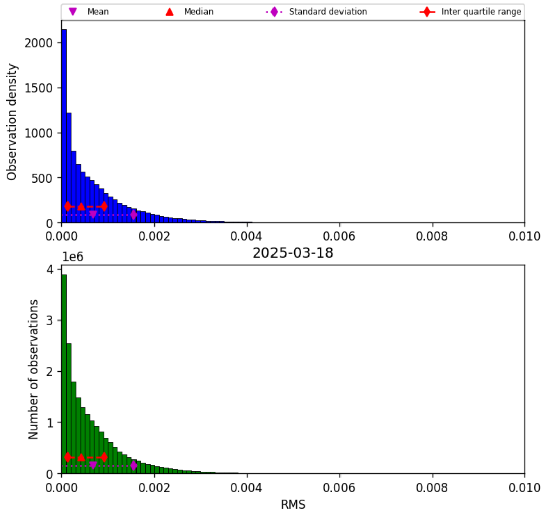
Figure 47: Histogram of “RMS” for 2025-03-17 to 2025-03-19
