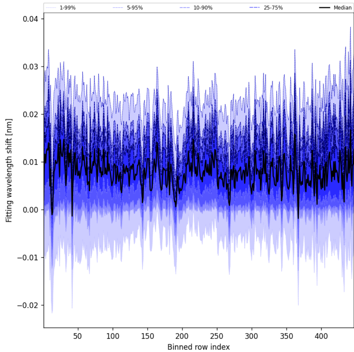
Figure 65: Along track statistics of “Fitting wavelength shift” for 2025-03-17 to 2025-03-19
