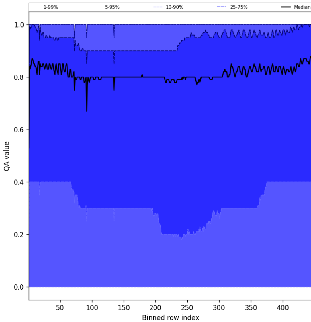
Figure 54: Along track statistics of “QA value” for 2025-03-17 to 2025-03-19
