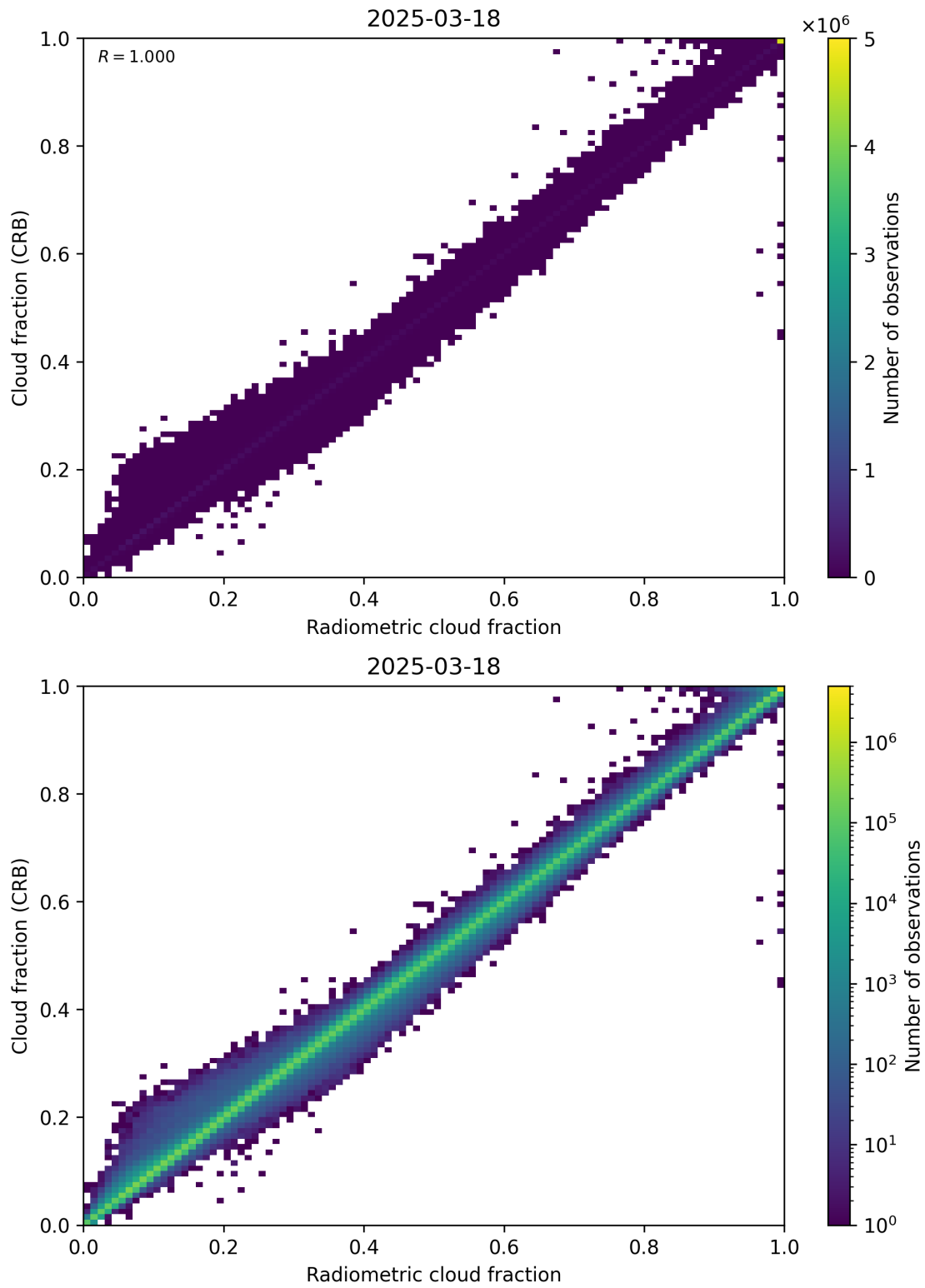
Figure 73: Scatter density plot of “Radiometric cloud fraction” against “Cloud fraction (CRB)” for 2025-03-17 to 2025-03-19.
