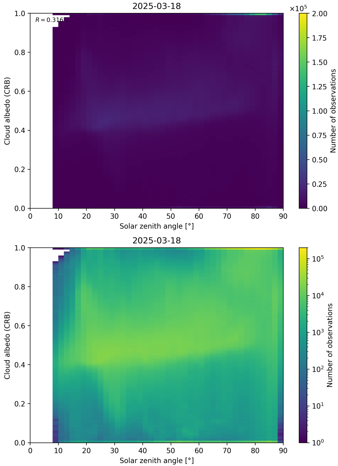
Figure 98: Scatter density plot of “Solar zenith angle” against “Cloud albedo (CRB)” for 2025-03-17 to 2025-03-19.
