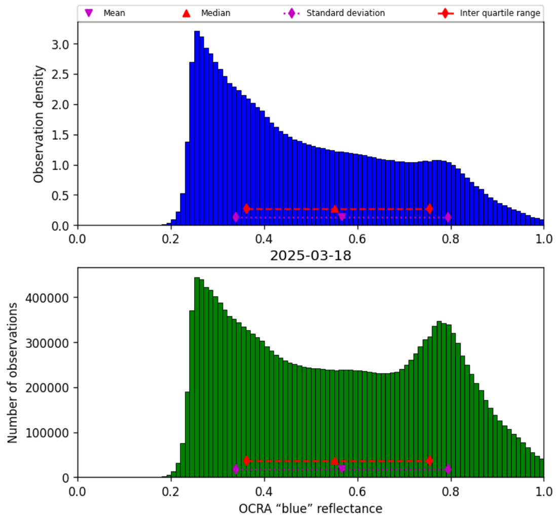
Figure 51: Histogram of “OCRA “blue” reflectance” for 2025-03-17 to 2025-03-19
