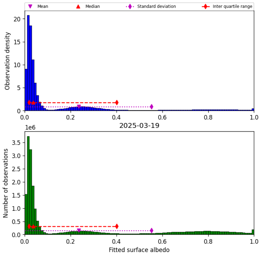
Figure 45: Histogram of “Fitted surface albedo” for 2025-03-18 to 2025-03-20
