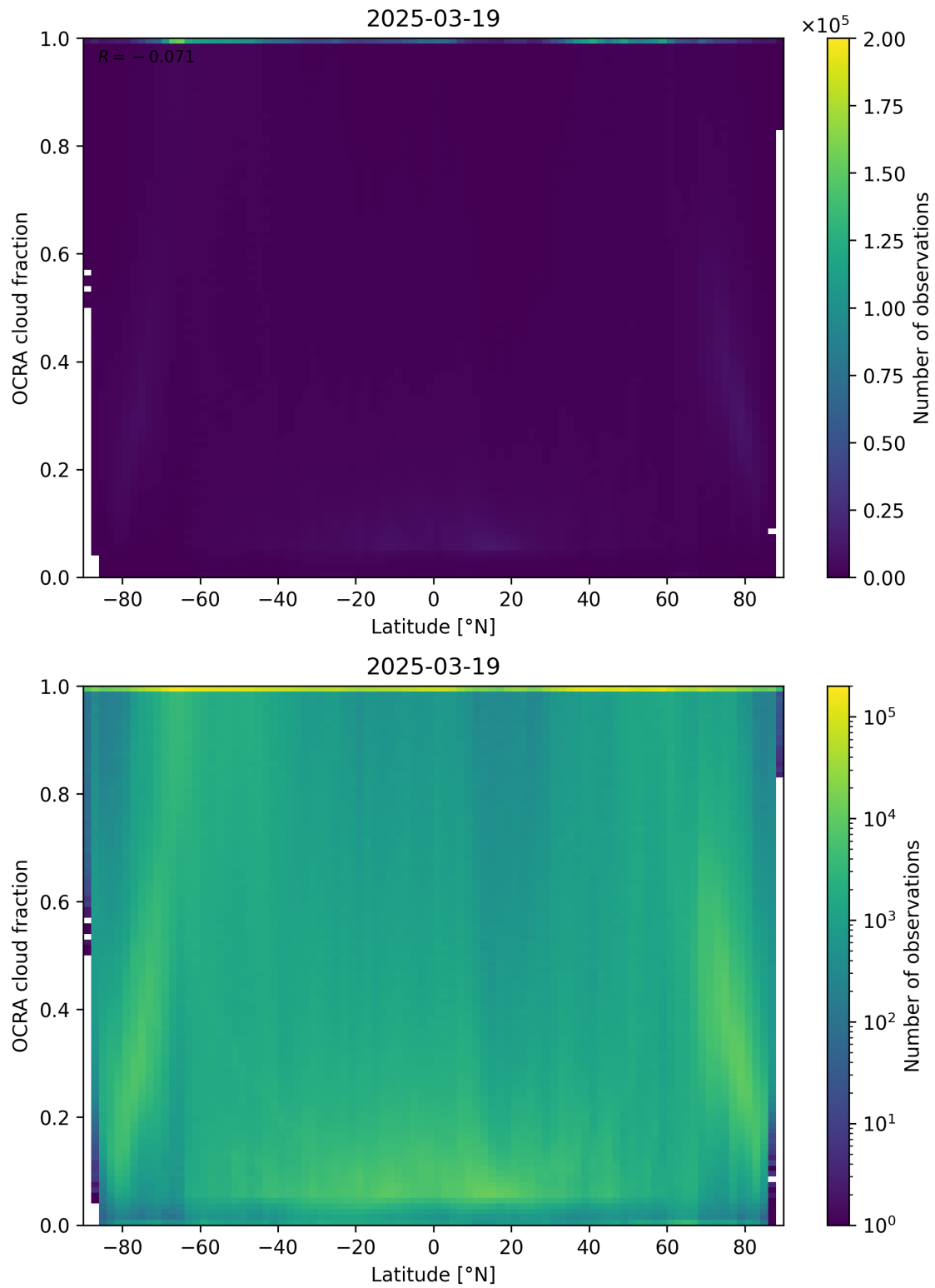
Figure 93: Scatter density plot of “Latitude” against “OCRA cloud fraction” for 2025-03-18 to 2025-03-20.
