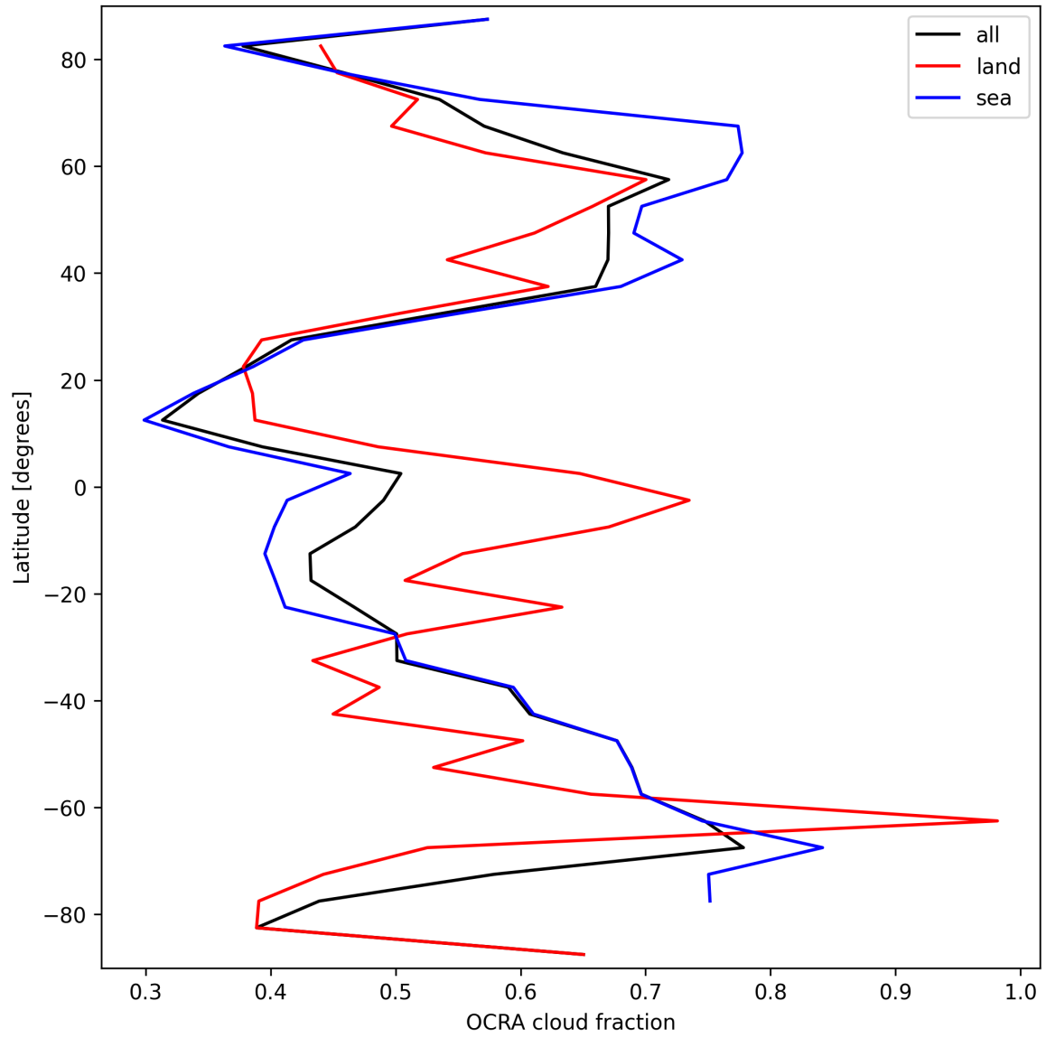
Figure 34: Zonal average of “OCRA cloud fraction” for 2025-03-18 to 2025-03-20.
