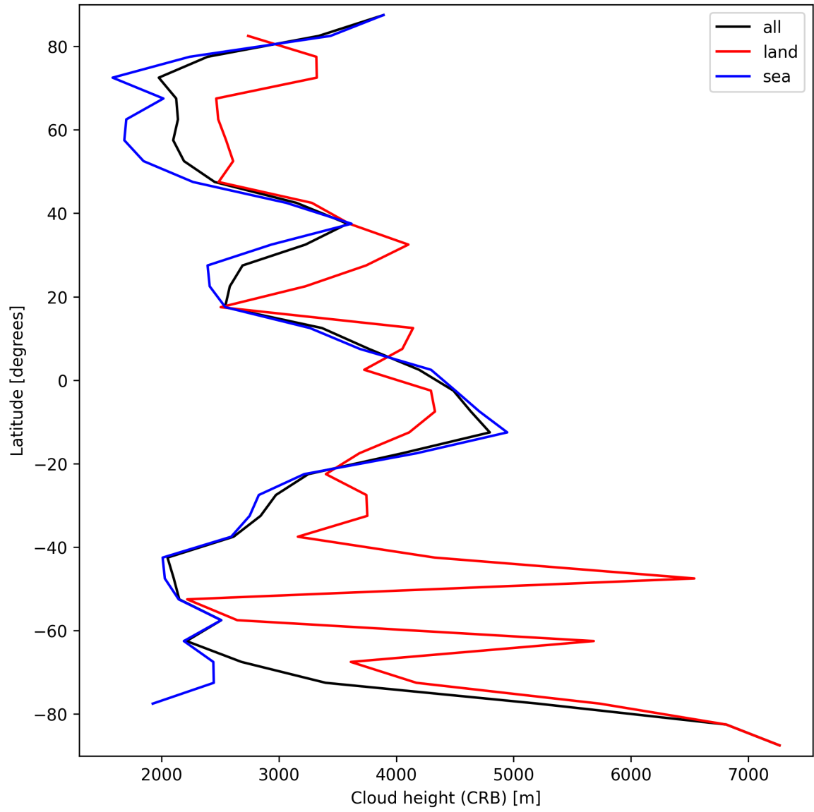
Figure 27: Zonal average of “Cloud height (CRB)” for 2025-03-18 to 2025-03-20.
