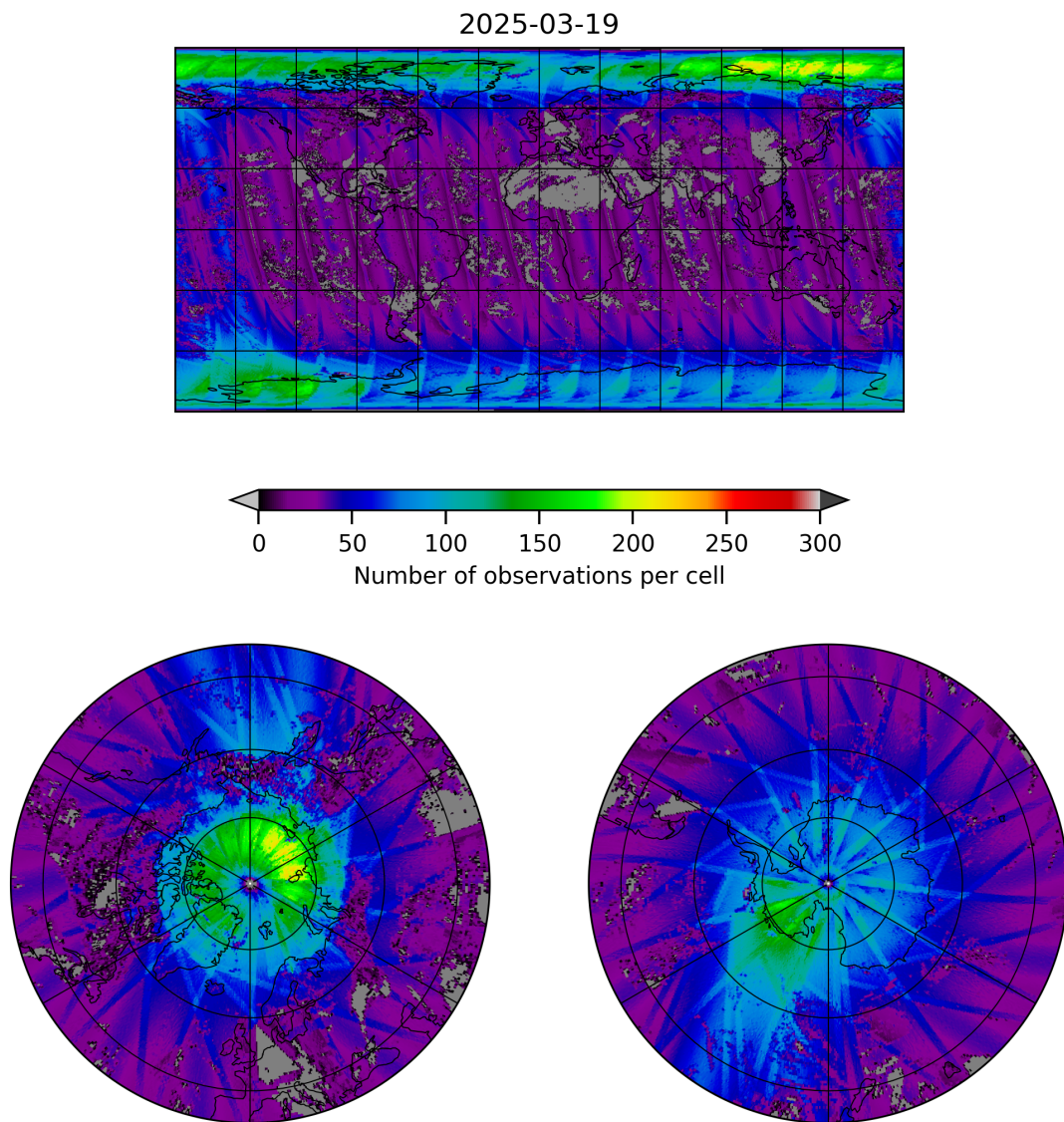
Figure 21: Map of the number of observations for 2025-03-18 to 2025-03-20
