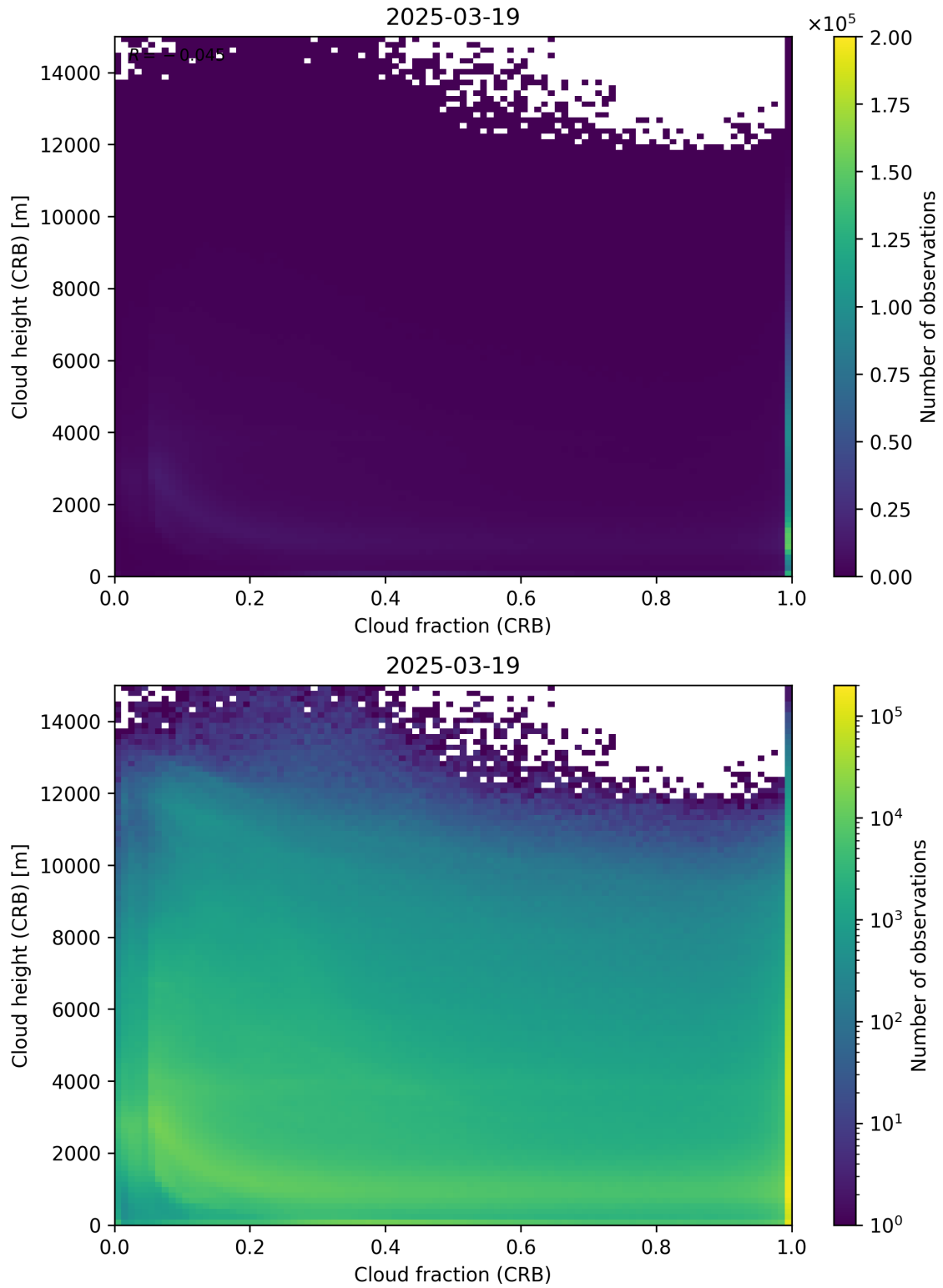
Figure 79: Scatter density plot of “Cloud fraction (CRB)” against “Cloud height (CRB)” for 2025-03-18 to 2025-03-20.
