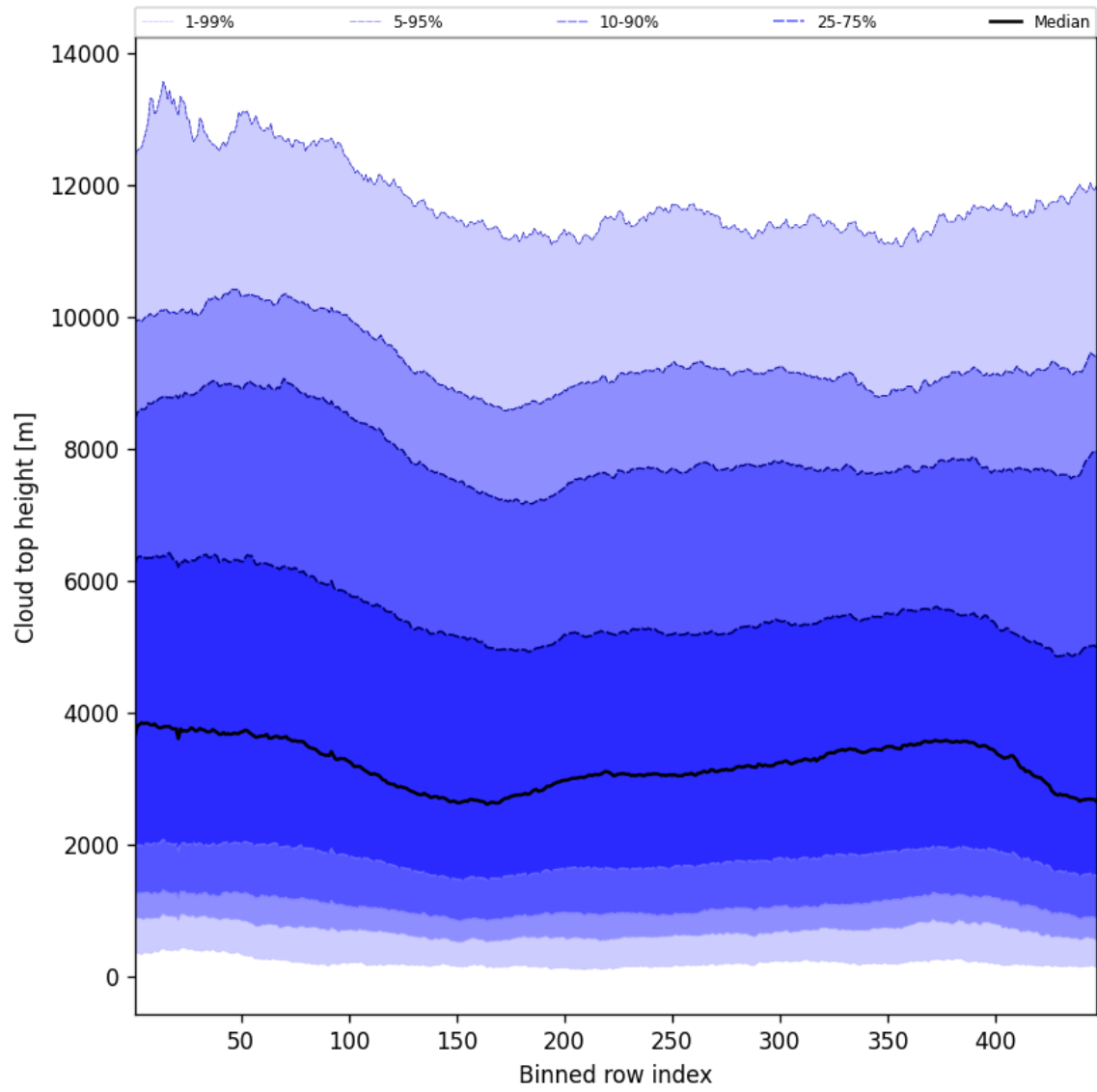
Figure 56: Along track statistics of “Cloud top height” for 2025-03-18 to 2025-03-20
