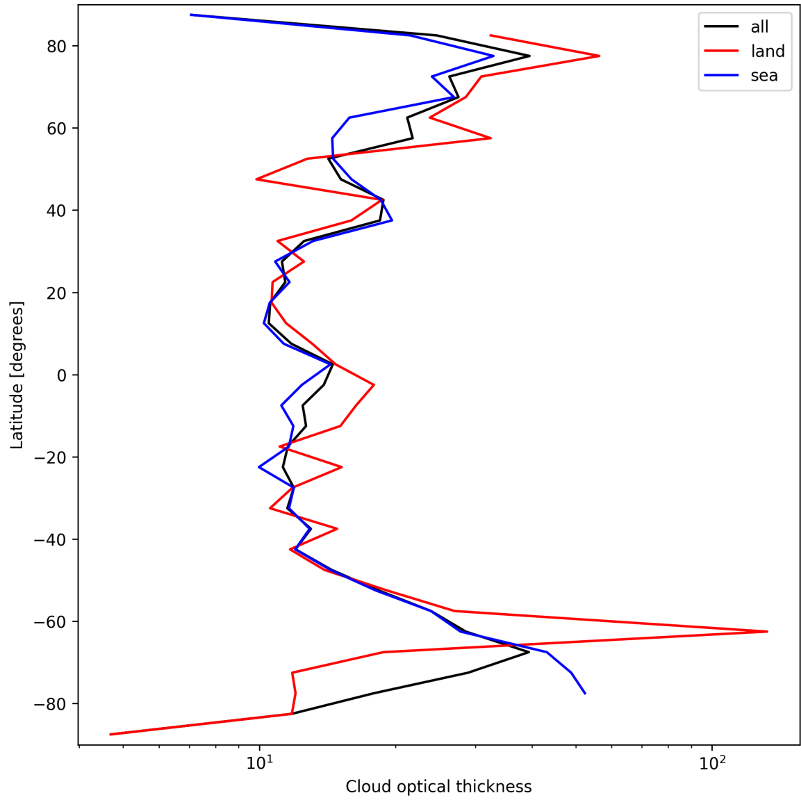
Figure 25: Zonal average of “Cloud optical thickness” for 2025-03-18 to 2025-03-20.
