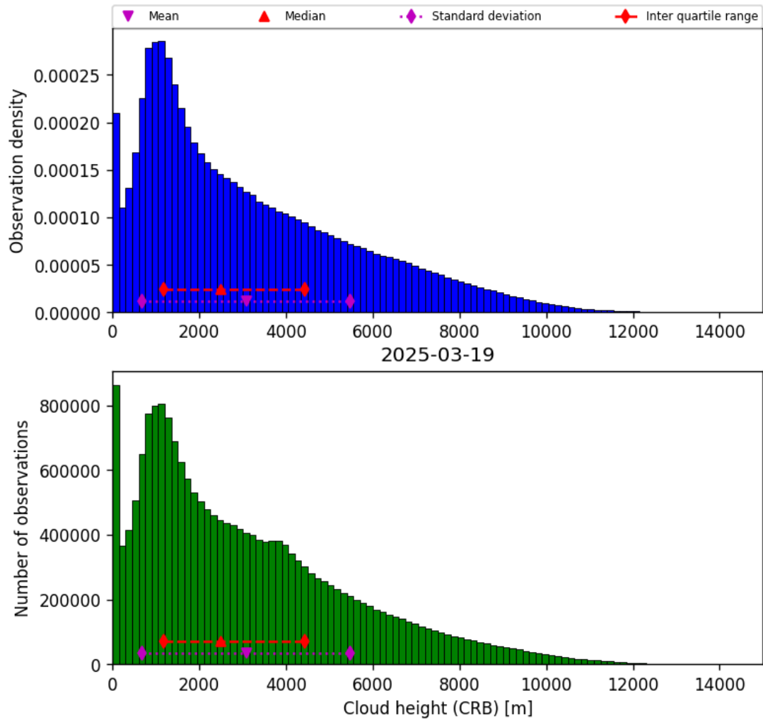
Figure 43: Histogram of “Cloud height (CRB)” for 2025-03-18 to 2025-03-20
