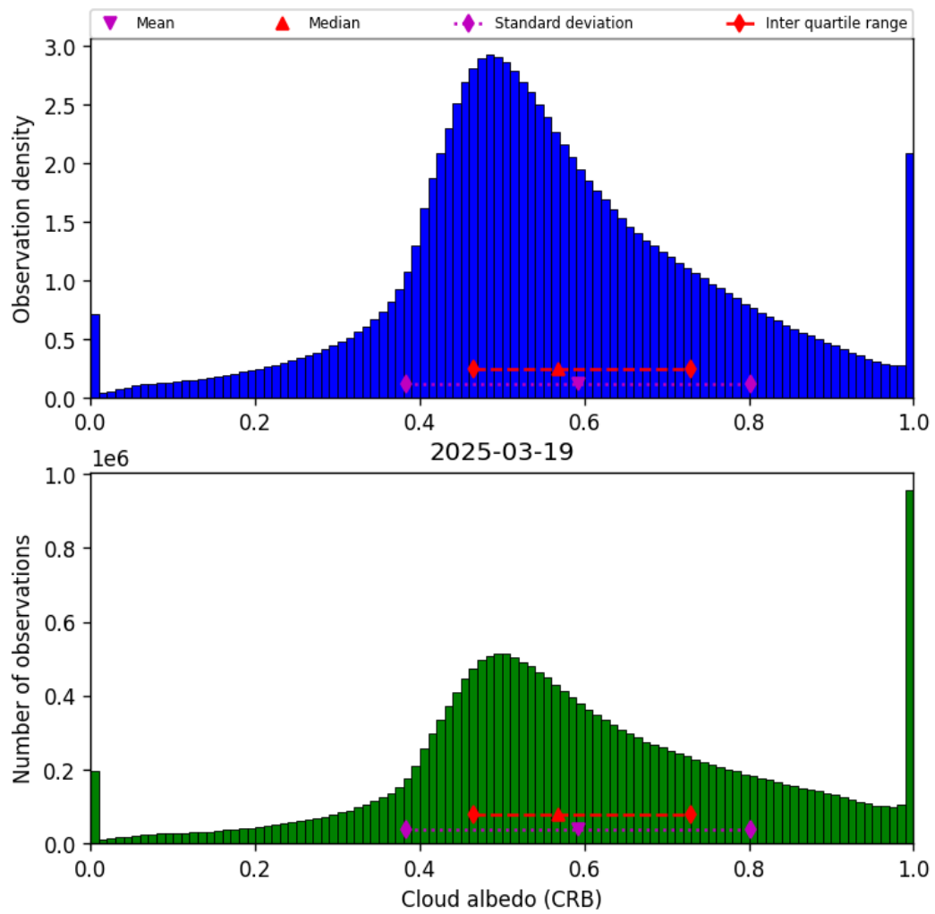
Figure 44: Histogram of “Cloud albedo (CRB)” for 2025-03-18 to 2025-03-20
