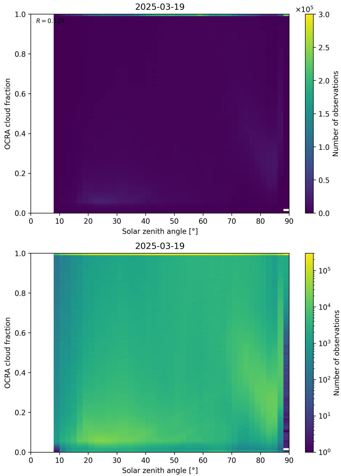
Figure 100: Scatter density plot of “Solar zenith angle” against “OCRA cloud fraction” for 2025-03-18 to 2025-03-20.
