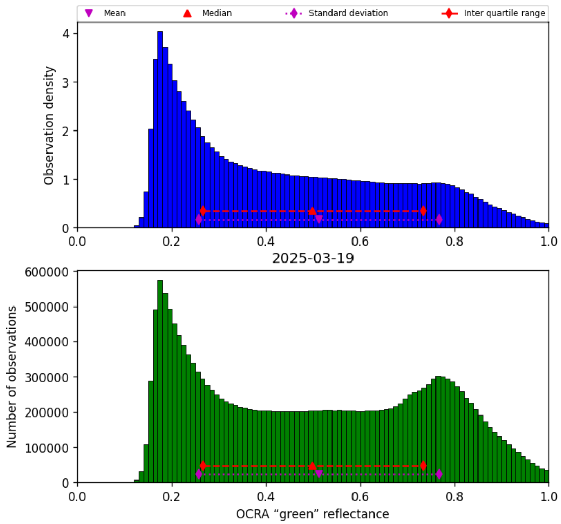
Figure 52: Histogram of “OCRA “green” reflectance” for 2025-03-18 to 2025-03-20
