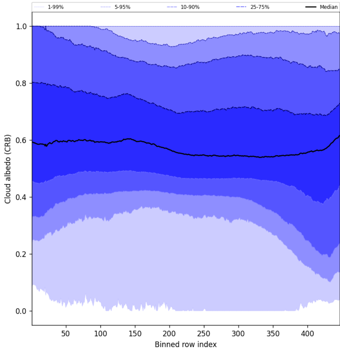
Figure 60: Along track statistics of “Cloud albedo (CRB)” for 2025-03-18 to 2025-03-20
