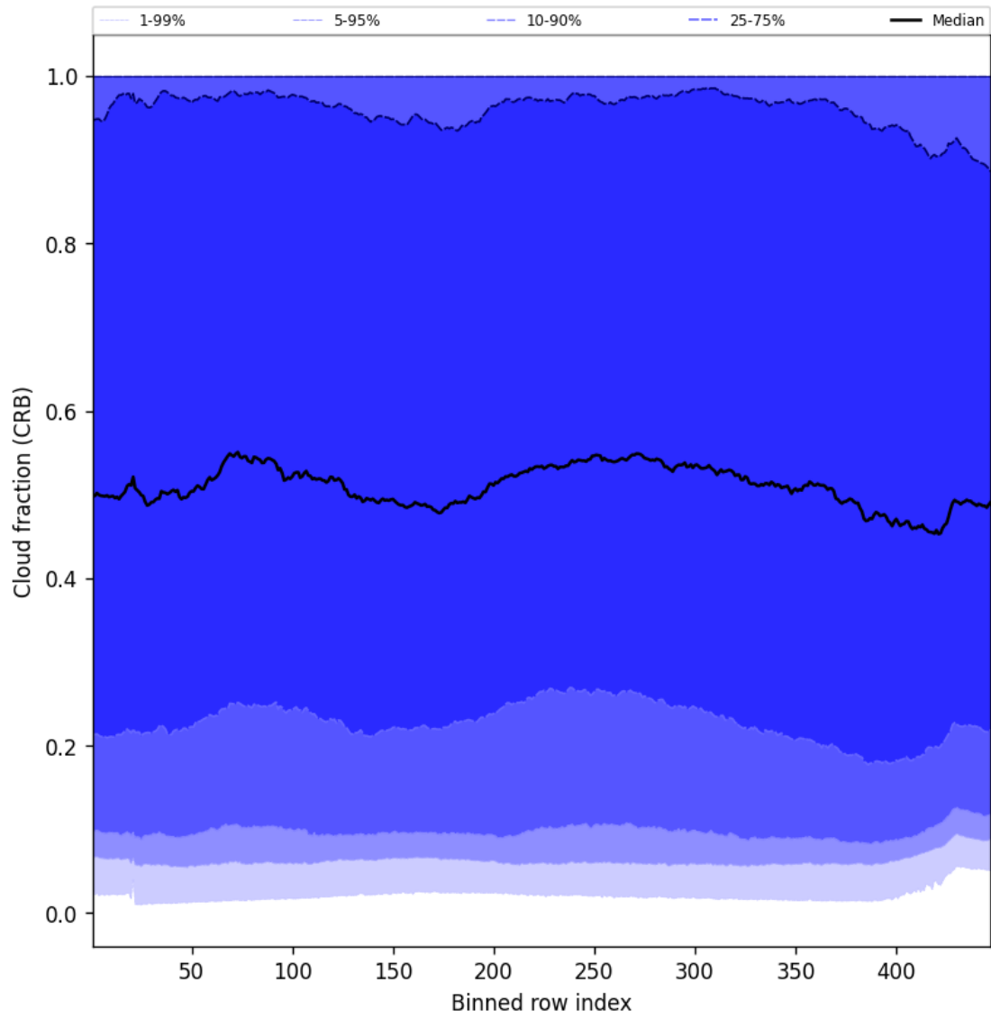
Figure 58: Along track statistics of “Cloud fraction (CRB)” for 2025-03-18 to 2025-03-20
