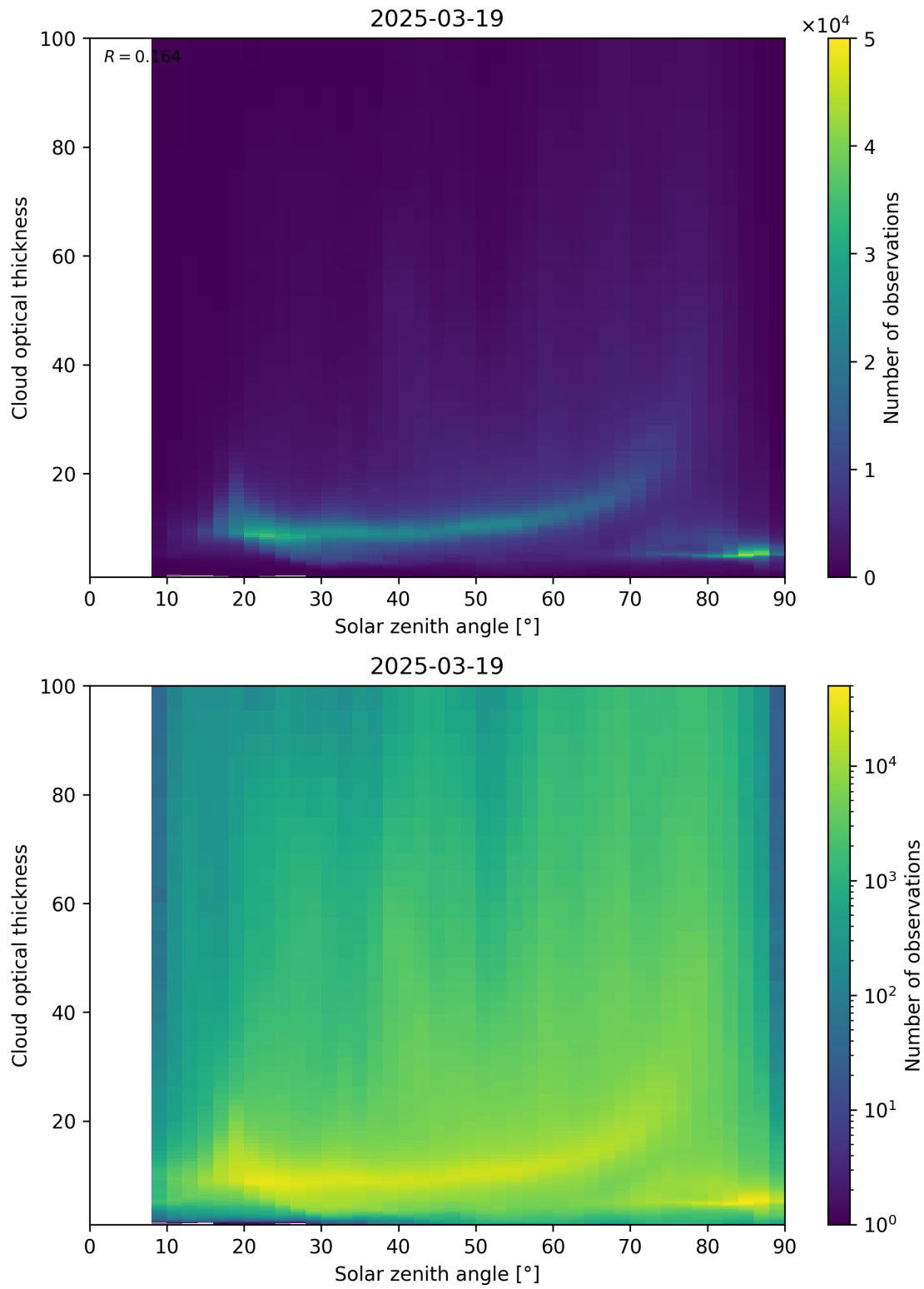
Figure 103: Scatter density plot of “Solar zenith angle” against “Cloud optical thickness” for 2025-03-18 to 2025-03-20.
