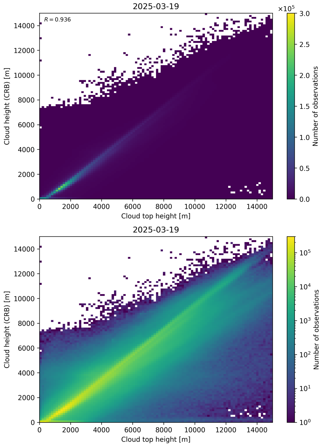
Figure 89: Scatter density plot of “Cloud top height” against “Cloud height (CRB)” for 2025-03-18 to 2025-03-20.
