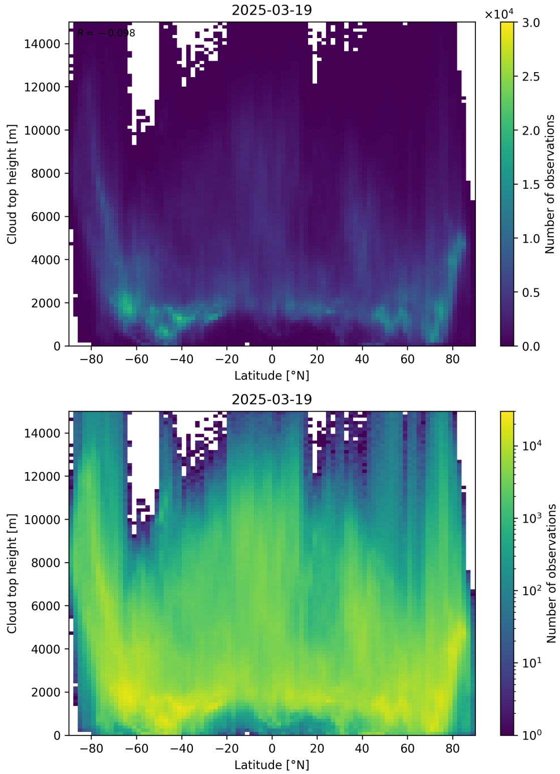
Figure 97: Scatter density plot of “Latitude” against “Cloud top height” for 2025-03-18 to 2025-03-20.
