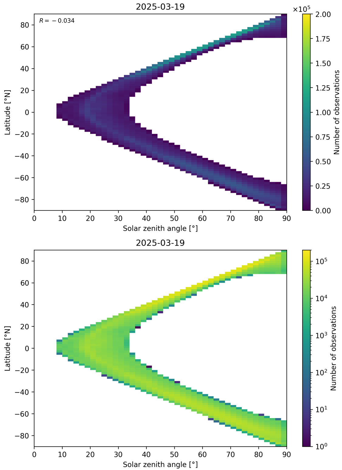
Figure 105: Scatter density plot of “Solar zenith angle” against “Latitude” for 2025-03-18 to 2025-03-20.
