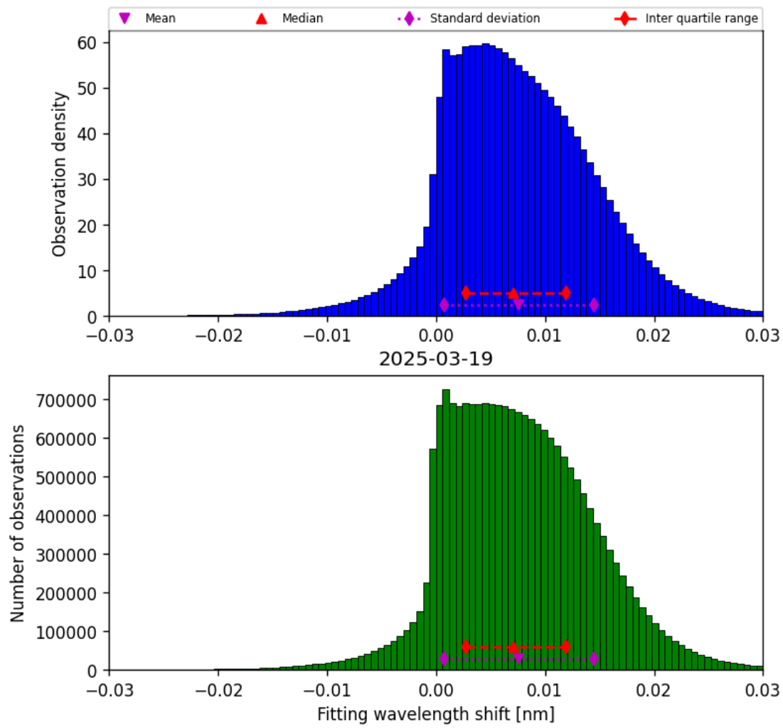
Figure 49: Histogram of “Fitting wavelength shift” for 2025-03-18 to 2025-03-20
