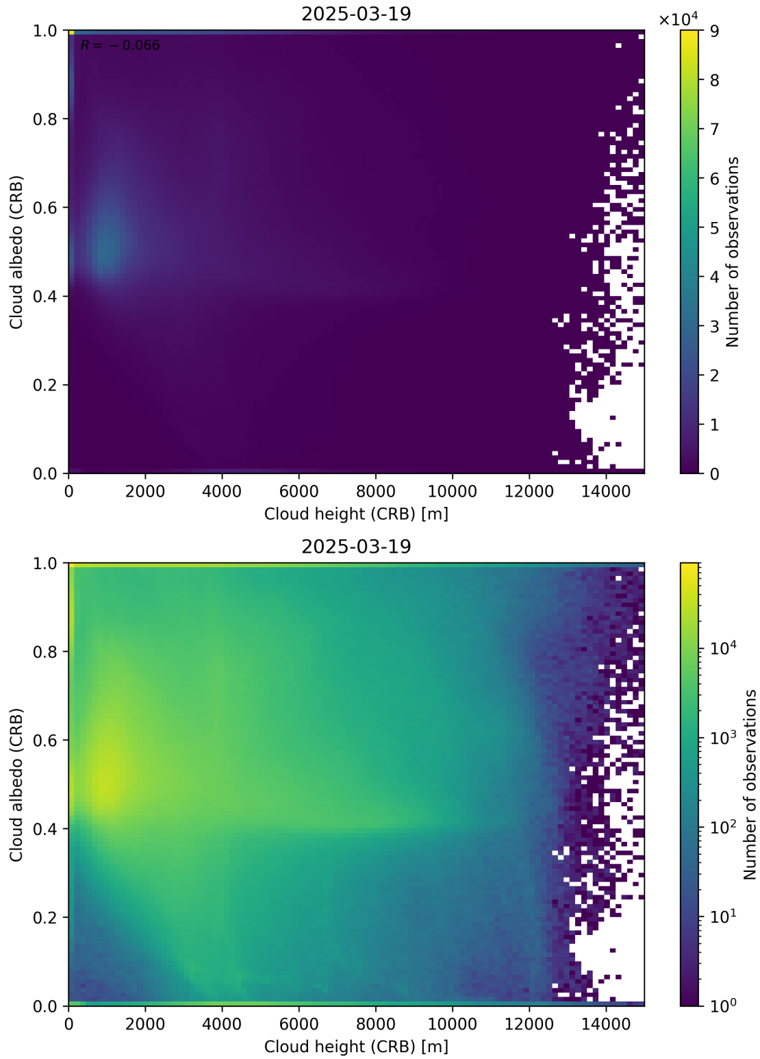
Figure 80: Scatter density plot of “Cloud height (CRB)” against “Cloud albedo (CRB)” for 2025-03-18 to 2025-03-20.
