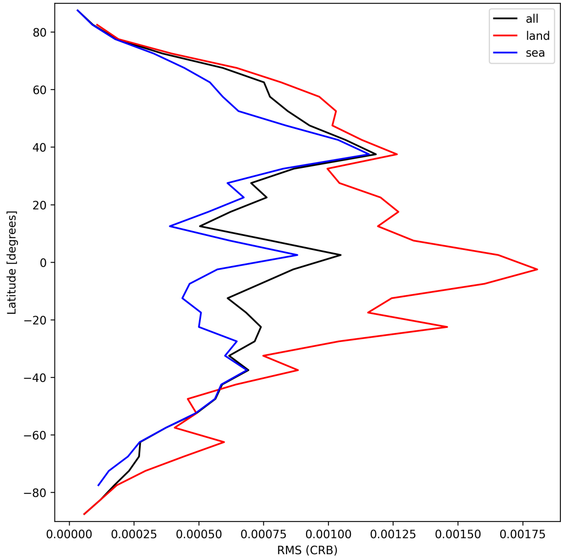
Figure 32: Zonal average of “RMS (CRB)” for 2025-03-18 to 2025-03-20.
