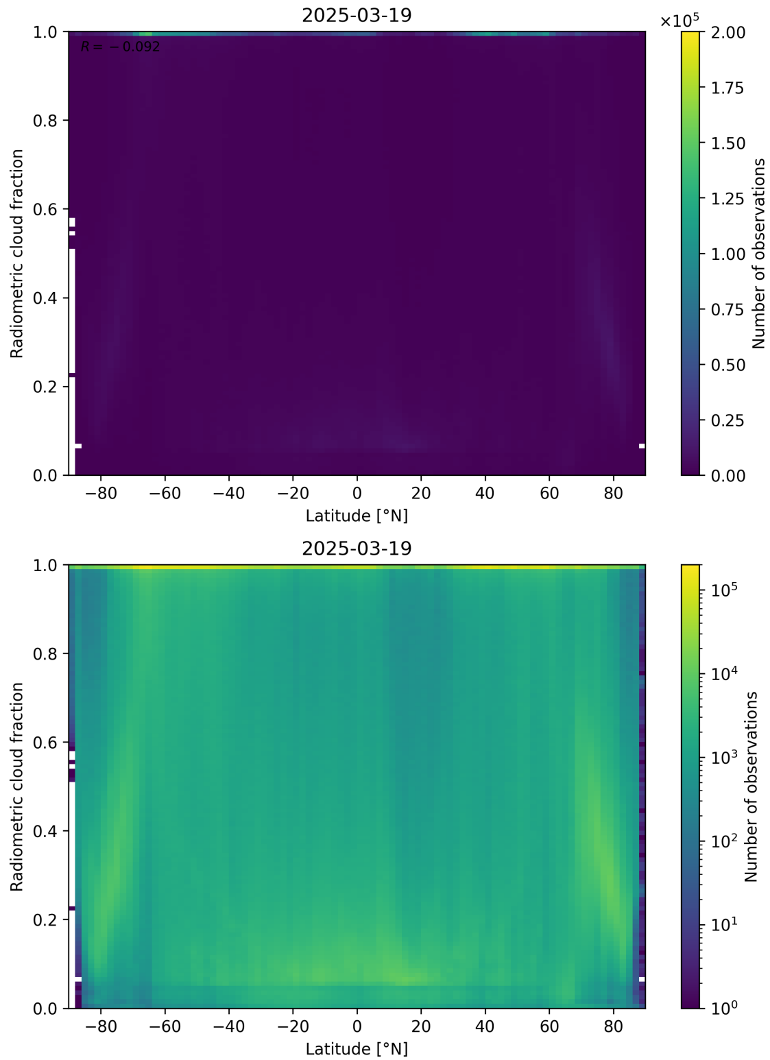
Figure 92: Scatter density plot of “Latitude” against “Radiometric cloud fraction” for 2025-03-18 to 2025-03-20.
