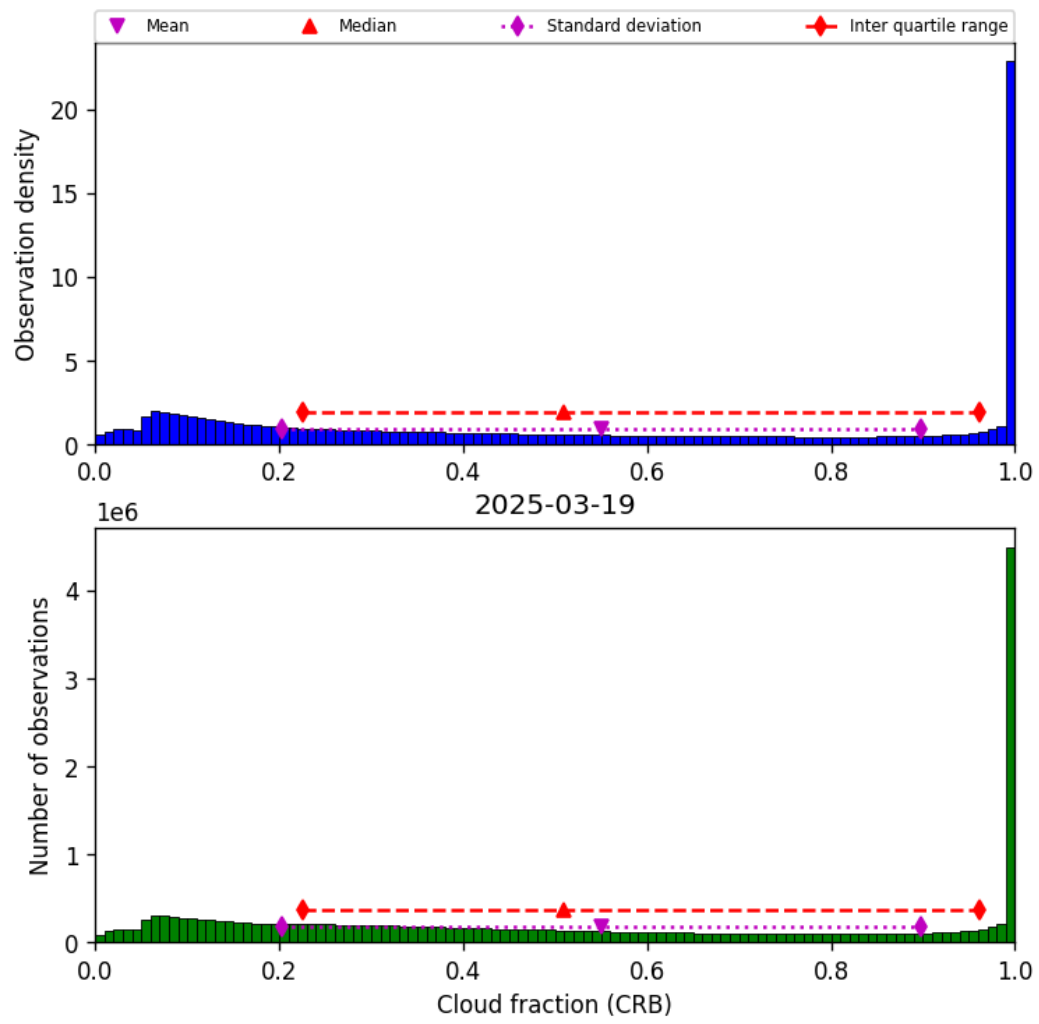
Figure 42: Histogram of “Cloud fraction (CRB)” for 2025-03-18 to 2025-03-20
