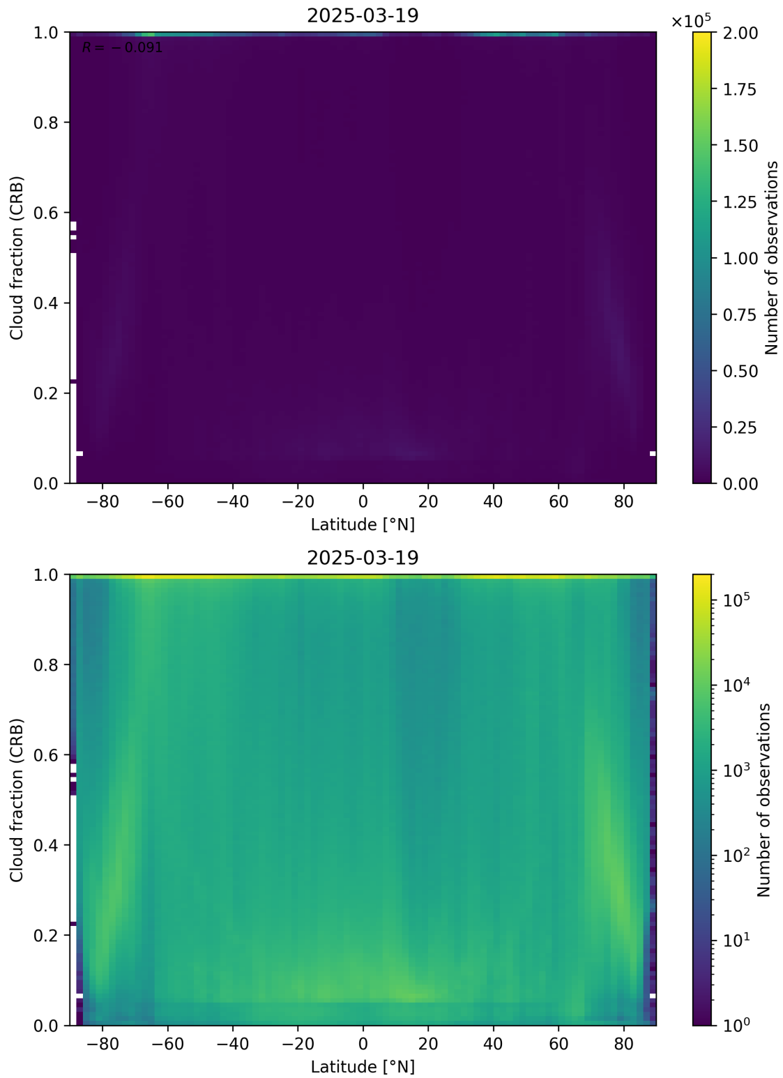
Figure 94: Scatter density plot of “Latitude” against “Cloud fraction (CRB)” for 2025-03-18 to 2025-03-20.
