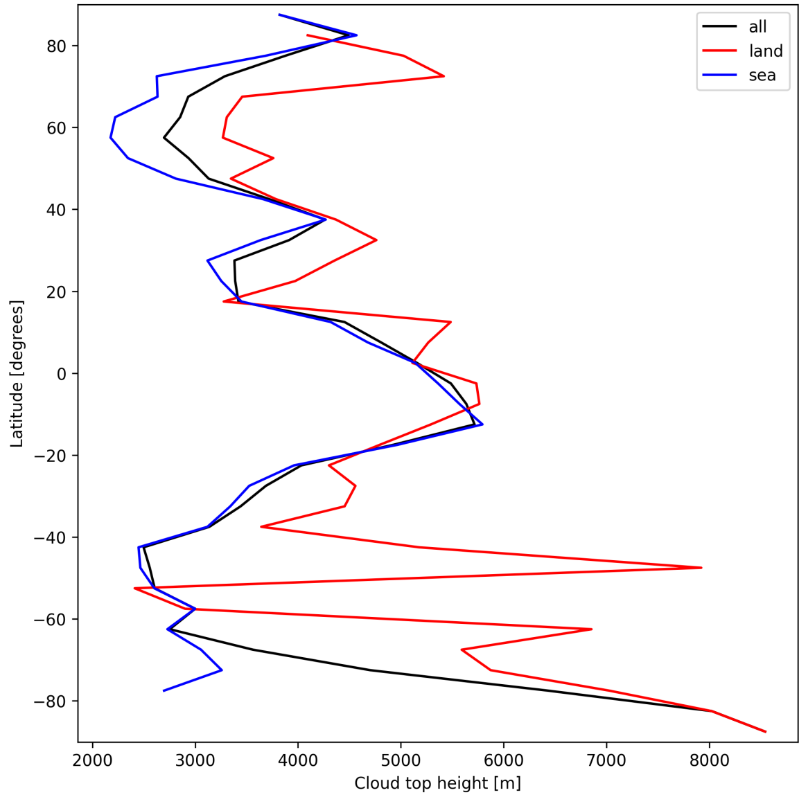
Figure 24: Zonal average of “Cloud top height” for 2025-03-18 to 2025-03-20.
