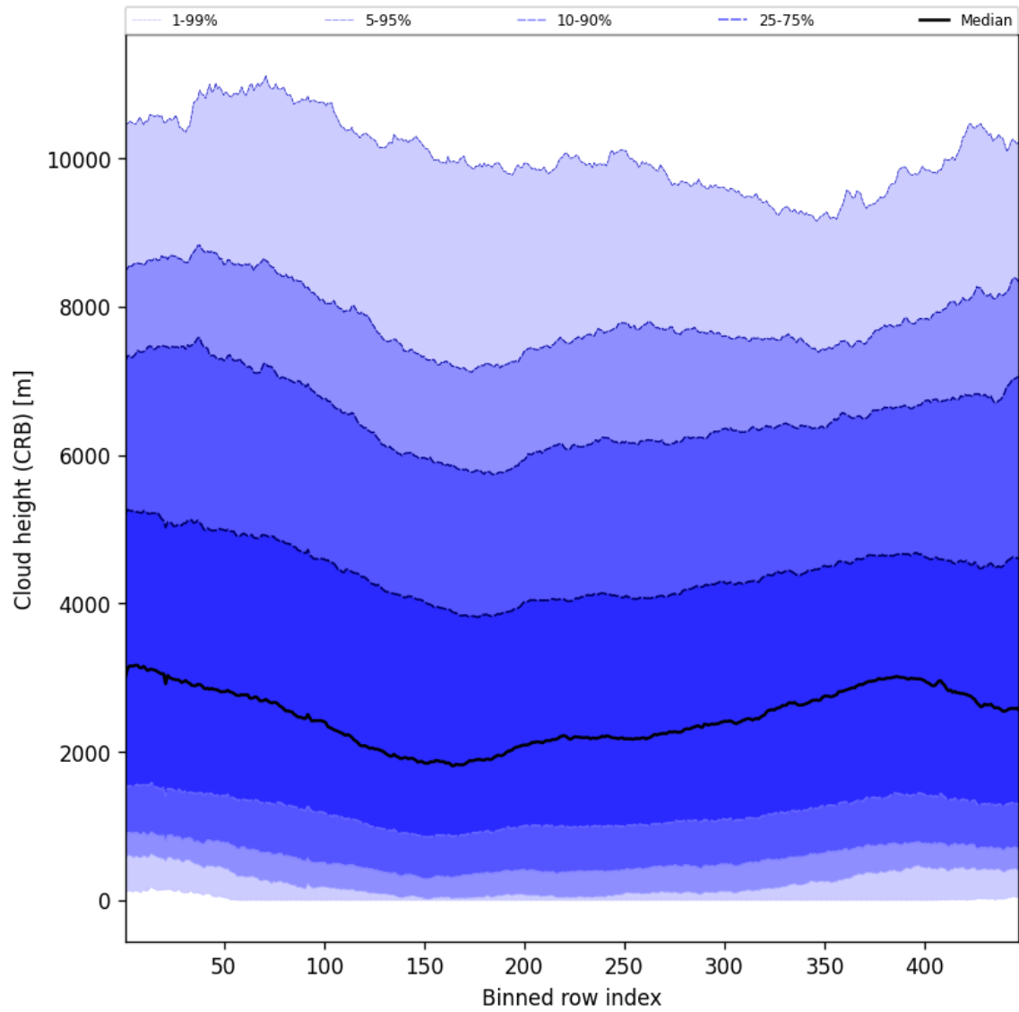
Figure 59: Along track statistics of “Cloud height (CRB)” for 2025-03-18 to 2025-03-20
