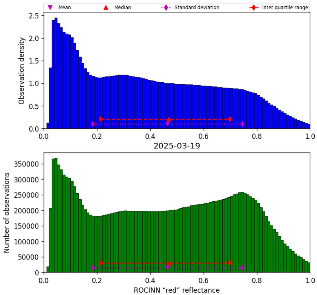
Figure 53: Histogram of “ROCINN “red” reflectance” for 2025-03-18 to 2025-03-20
