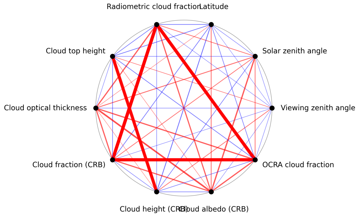
Figure 1: Map of correlation graph for 2025-03-18 to 2025-03-20.
