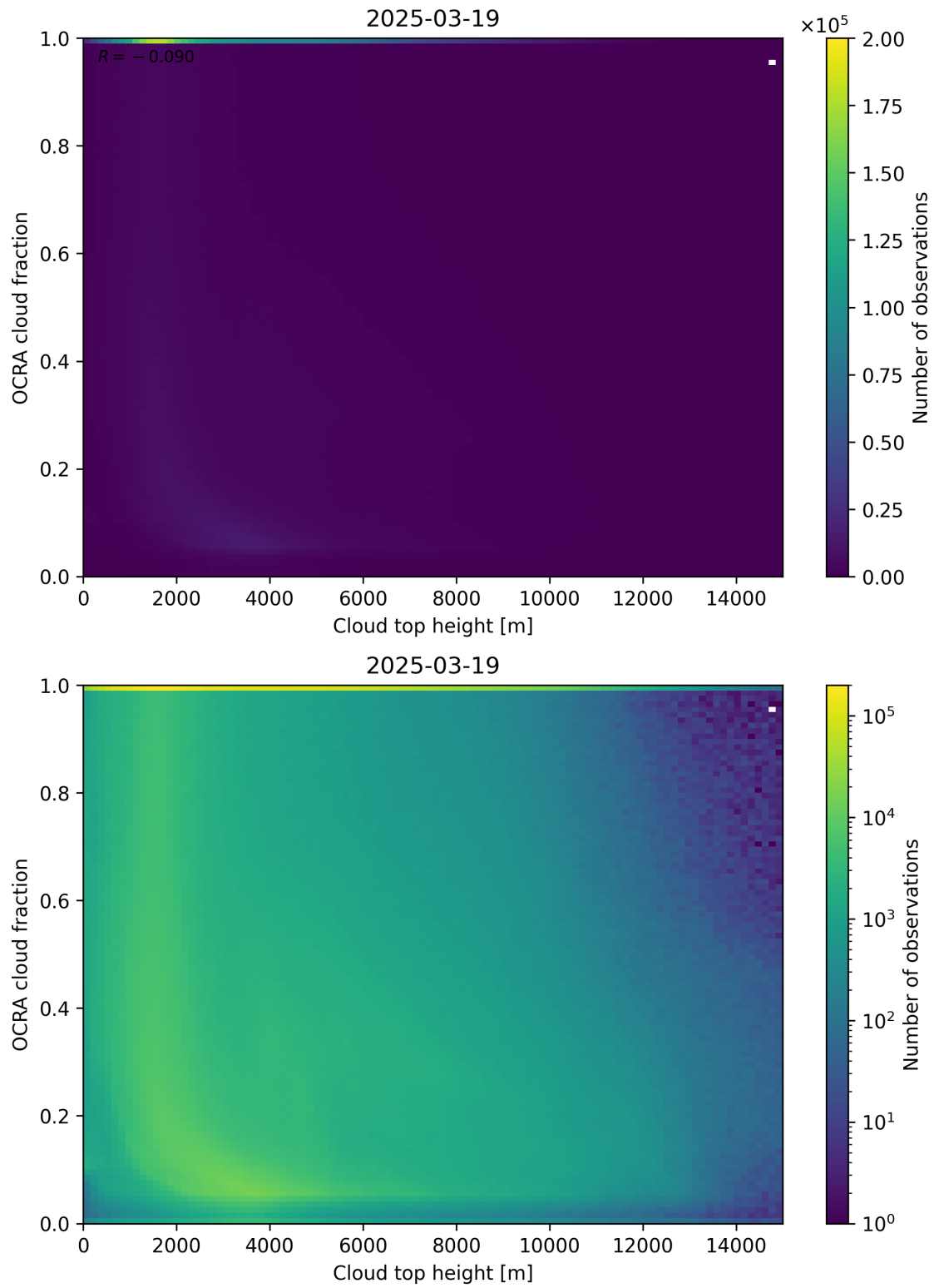
Figure 87: Scatter density plot of “Cloud top height” against “OCRA cloud fraction” for 2025-03-18 to 2025-03-20.
