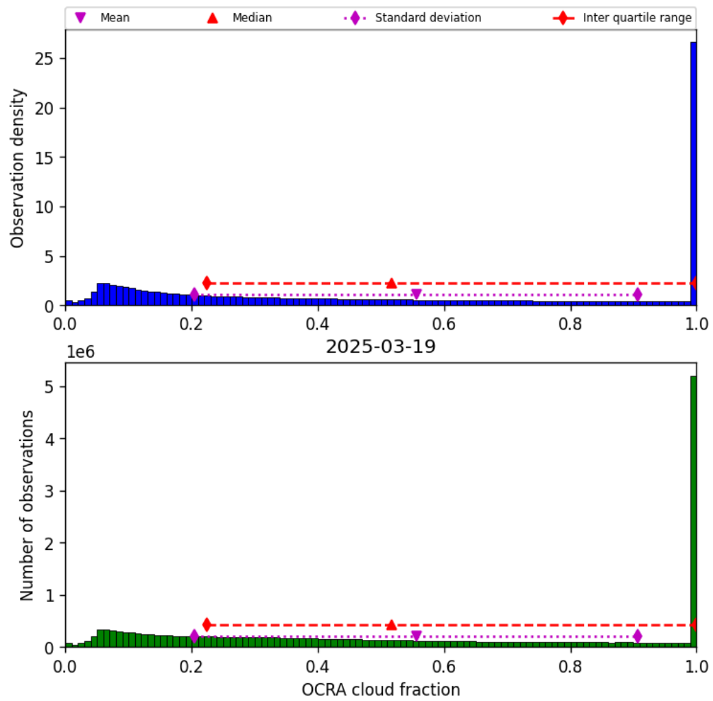
Figure 50: Histogram of “OCRA cloud fraction” for 2025-03-18 to 2025-03-20
