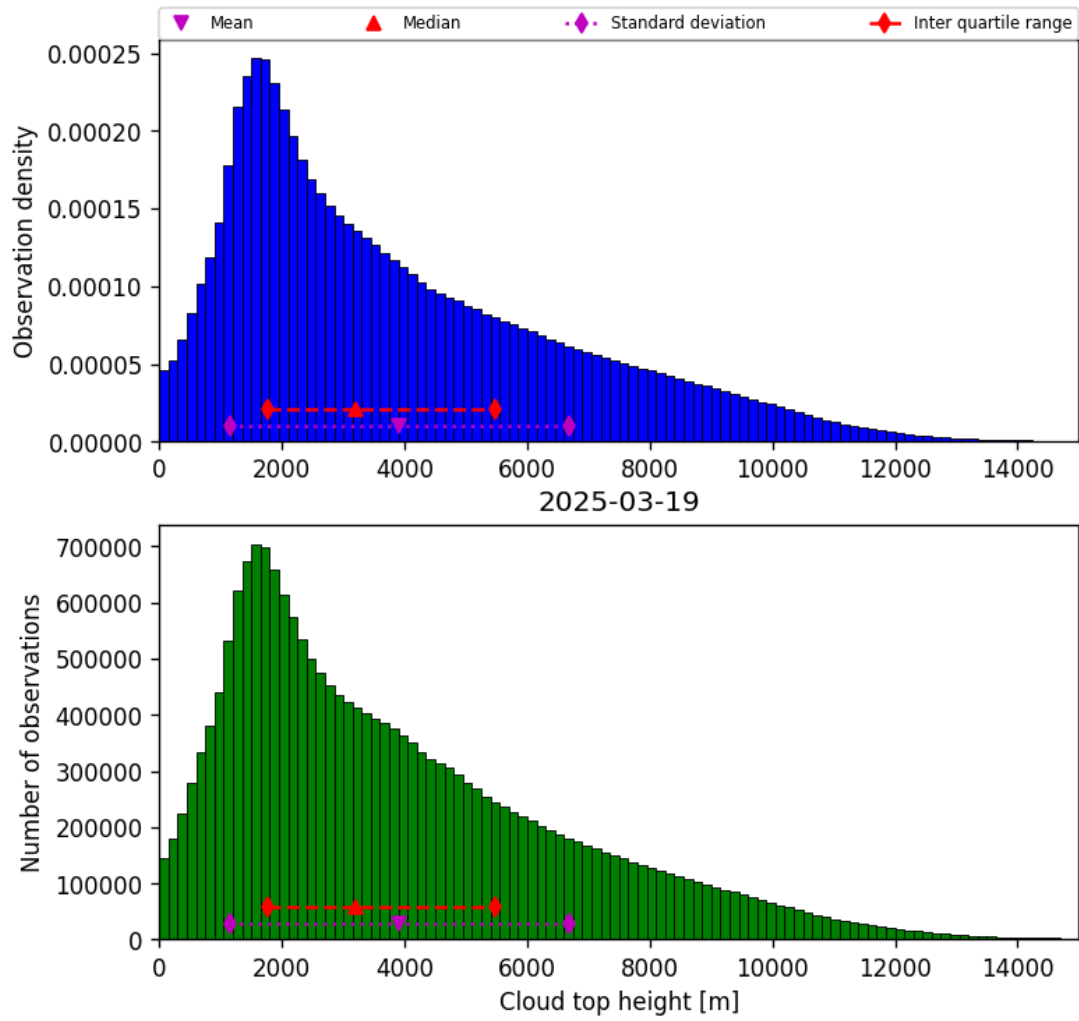
Figure 40: Histogram of “Cloud top height” for 2025-03-18 to 2025-03-20
