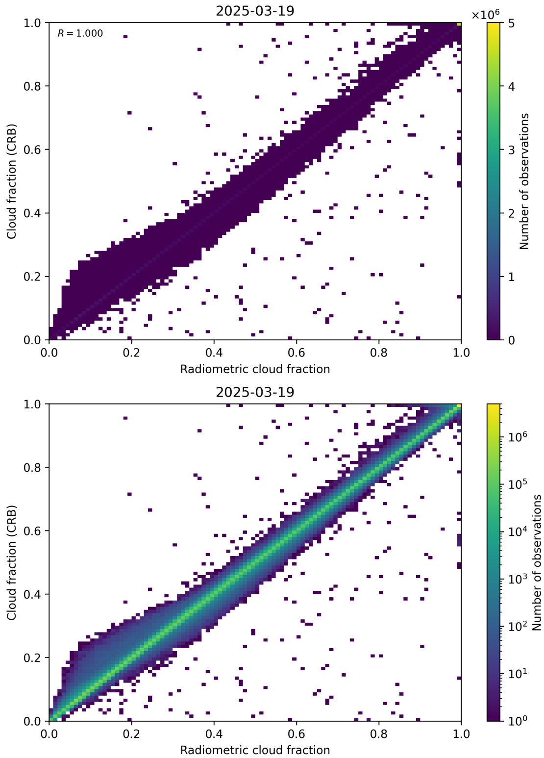
Figure 73: Scatter density plot of “Radiometric cloud fraction” against “Cloud fraction (CRB)” for 2025-03-18 to 2025-03-20.
