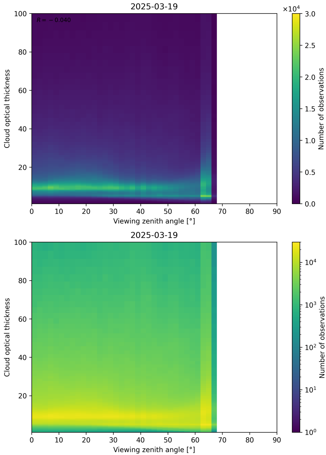
Figure 111: Scatter density plot of “Viewing zenith angle” against “Cloud optical thickness” for 2025-03-18 to 2025-03-20.
