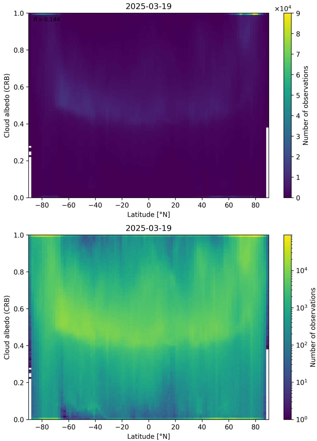
Figure 91: Scatter density plot of “Latitude” against “Cloud albedo (CRB)” for 2025-03-18 to 2025-03-20.
