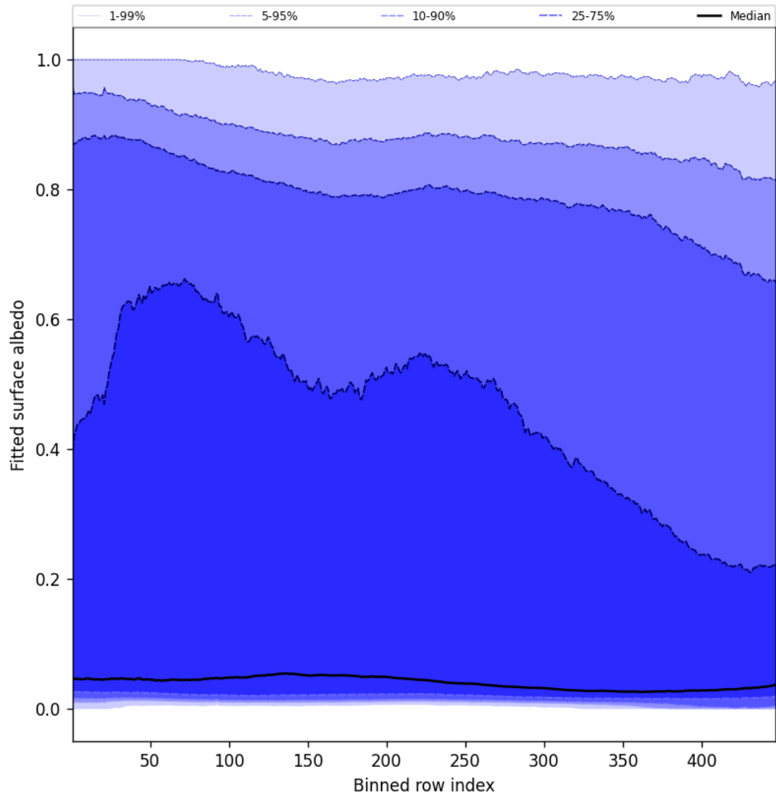
Figure 61: Along track statistics of “Fitted surface albedo” for 2025-03-18 to 2025-03-20
