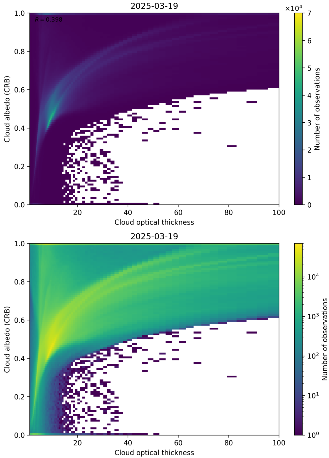
Figure 82: Scatter density plot of “Cloud optical thickness” against “Cloud albedo (CRB)” for 2025-03-18 to 2025-03-20.
