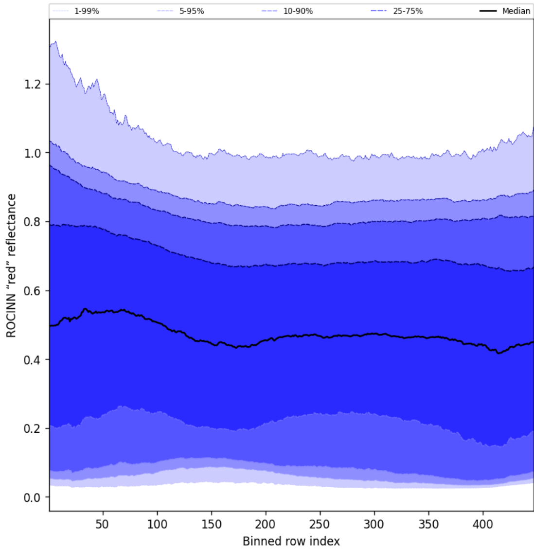
Figure 69: Along track statistics of "ROCINN "red" reflectance" for 2025-03-18 to 2025-03-20
