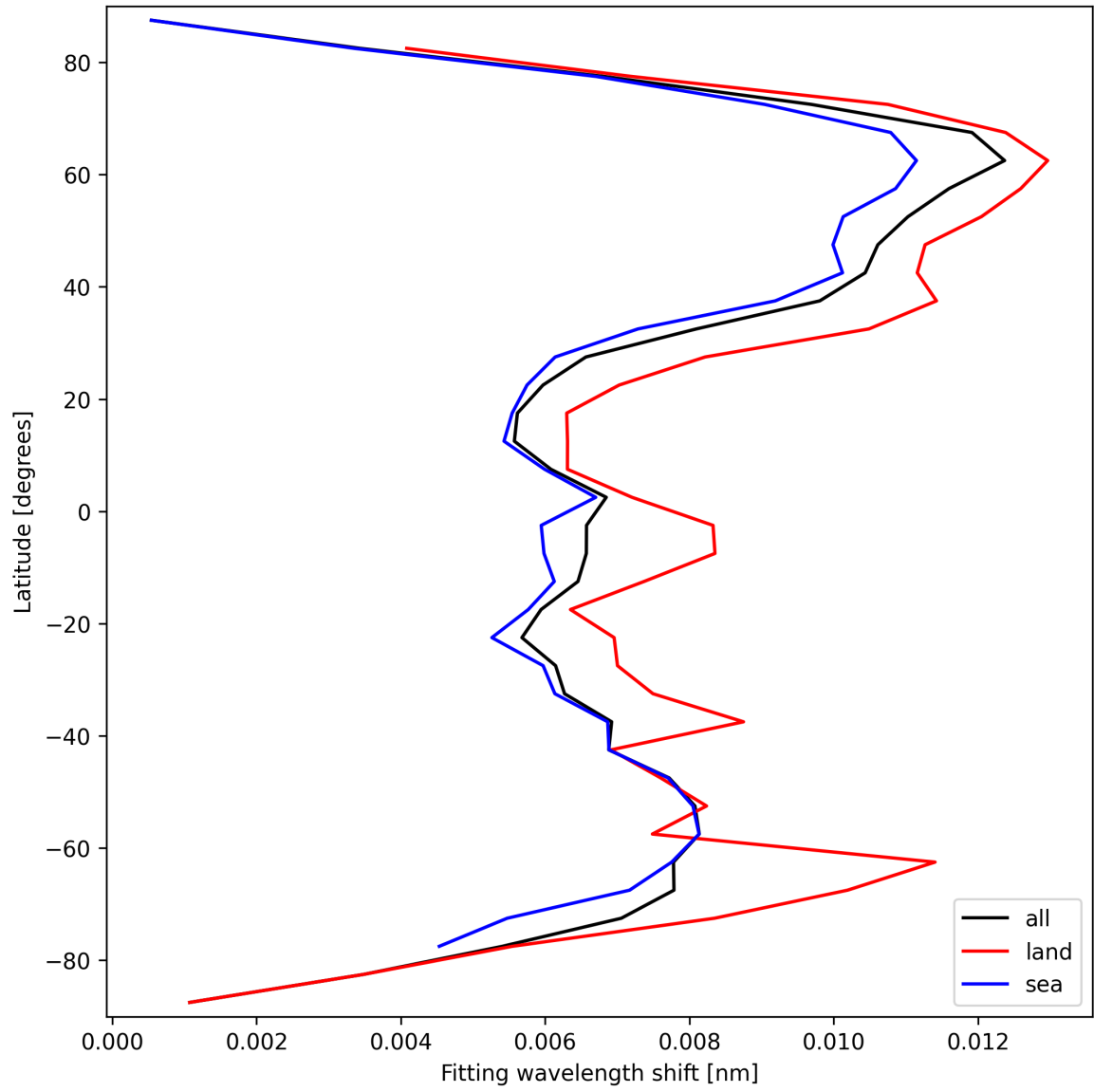
Figure 33: Zonal average of “Fitting wavelength shift” for 2025-03-18 to 2025-03-20.
