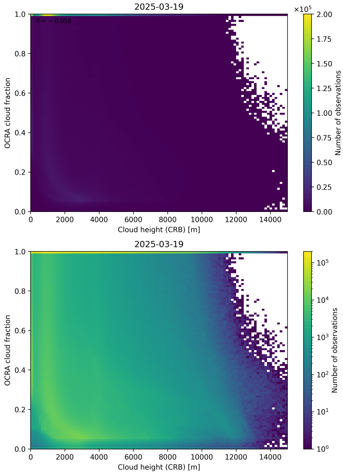
Figure 81: Scatter density plot of “Cloud height (CRB)” against “OCRA cloud fraction” for 2025-03-18 to 2025-03-20.
