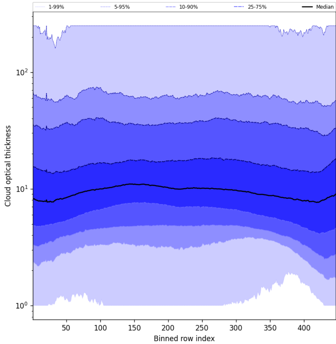
Figure 57: Along track statistics of “Cloud optical thickness” for 2025-03-18 to 2025-03-20
