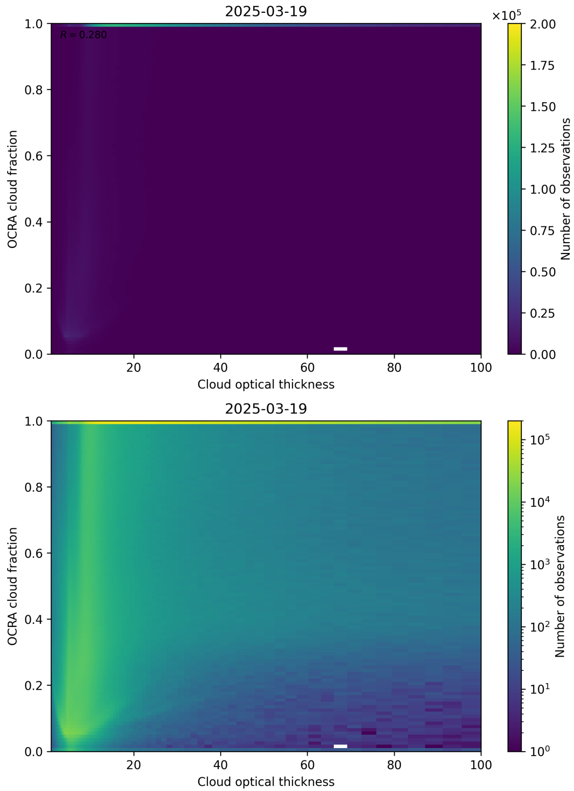
Figure 83: Scatter density plot of “Cloud optical thickness” against “OCRA cloud fraction” for 2025-03-18 to 2025-03-20.
