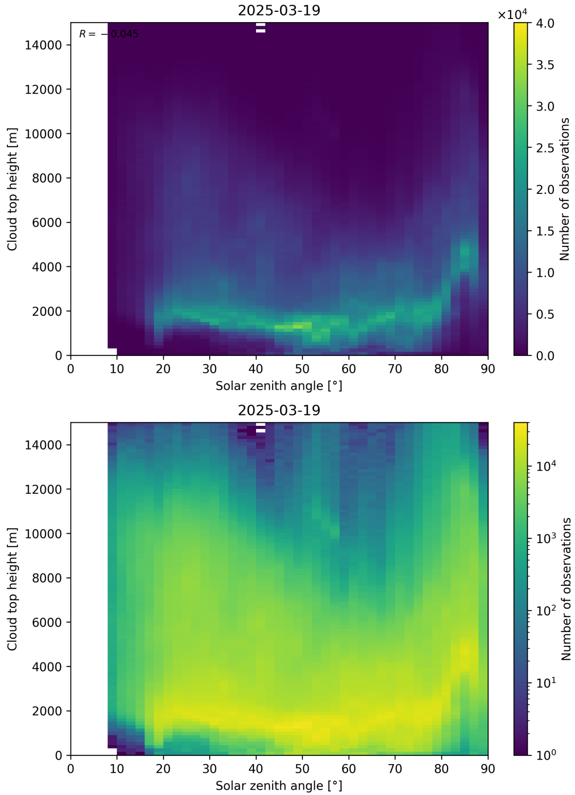
Figure 104: Scatter density plot of “Solar zenith angle” against “Cloud top height” for 2025-03-18 to 2025-03-20.
