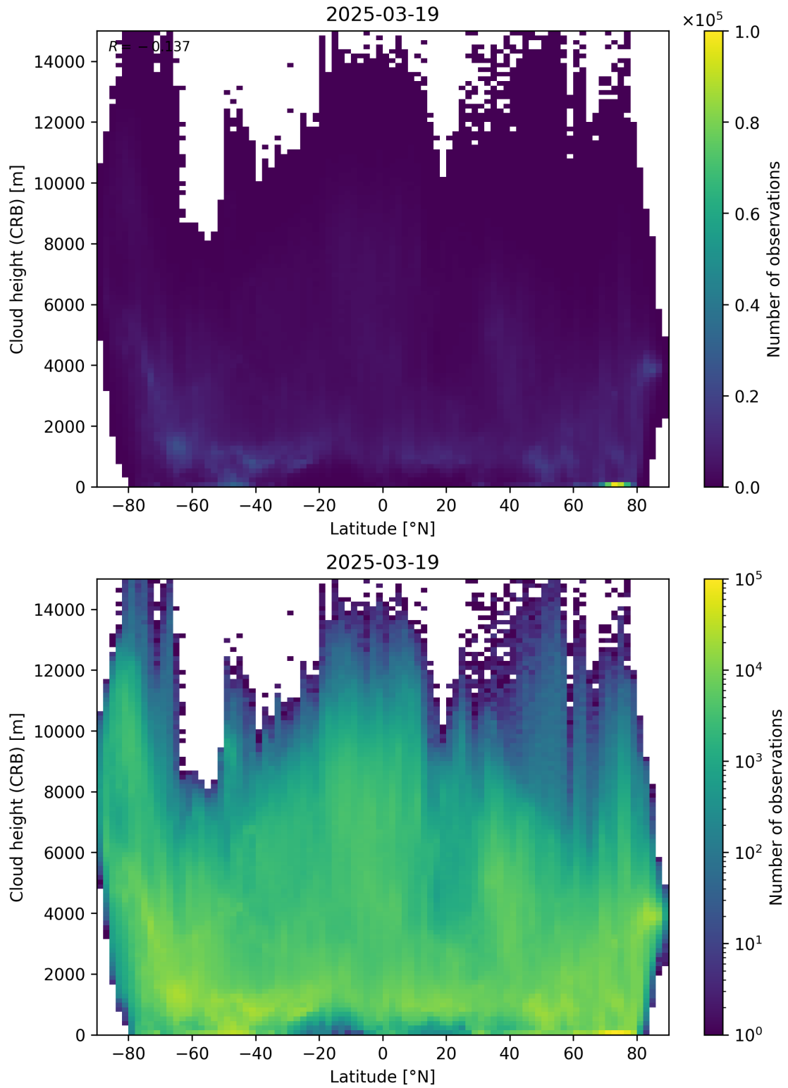
Figure 95: Scatter density plot of “Latitude” against “Cloud height (CRB)” for 2025-03-18 to 2025-03-20.
