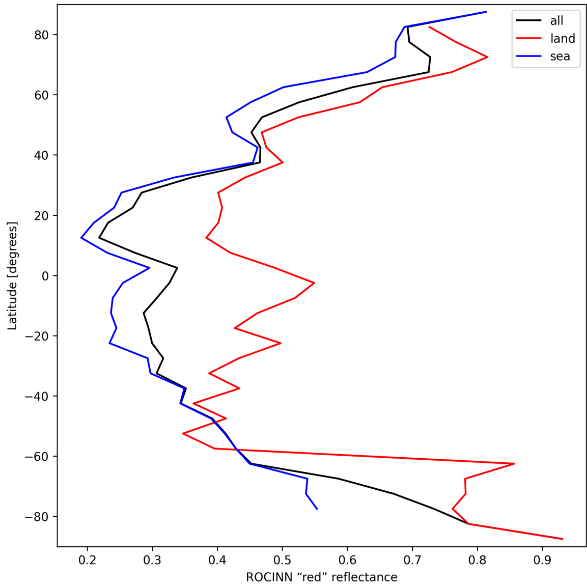
Figure 37: Zonal average of “ROCINN “red” reflectance” for 2025-03-18 to 2025-03-20.
