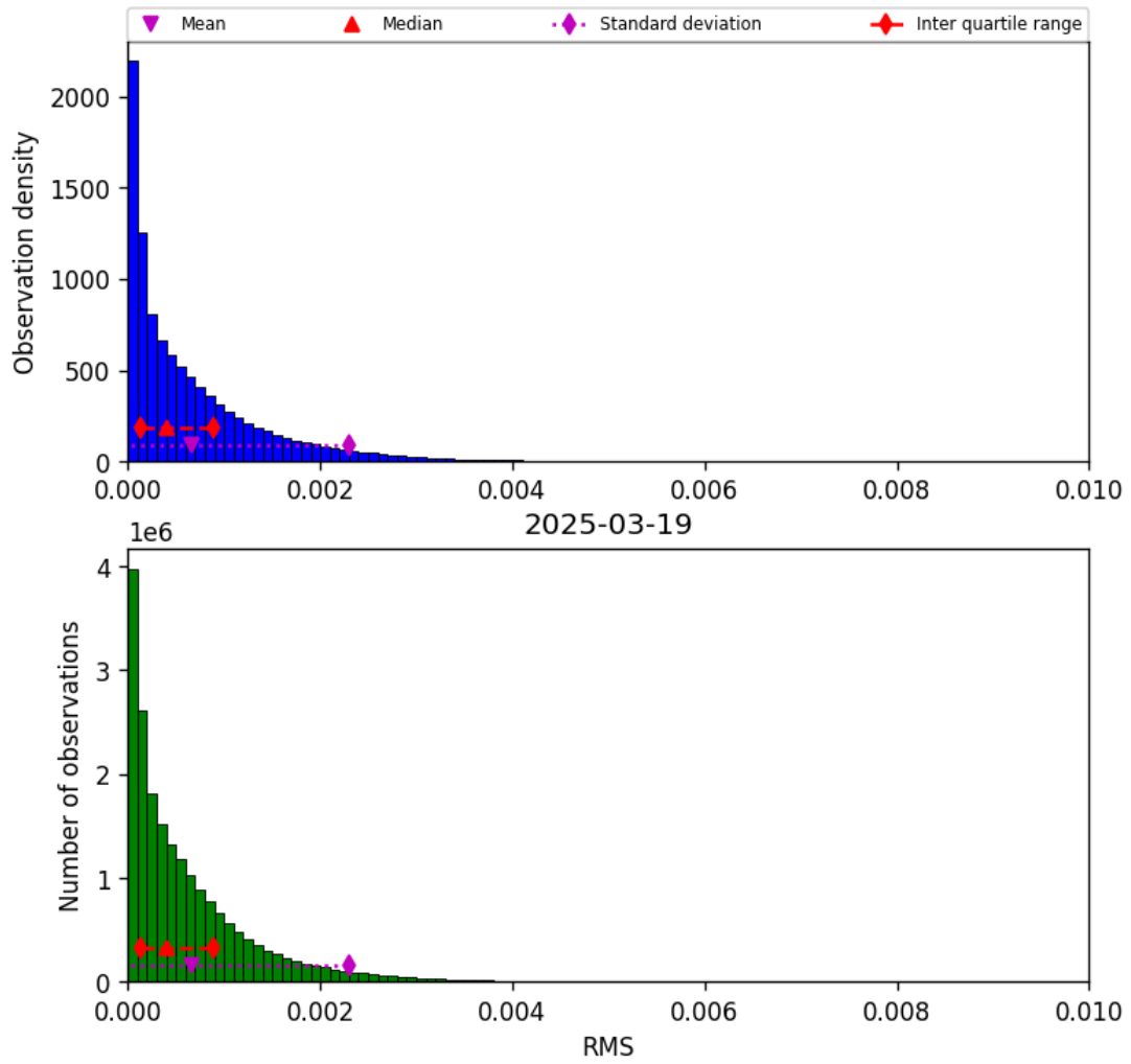
Figure 47: Histogram of “RMS” for 2025-03-18 to 2025-03-20
