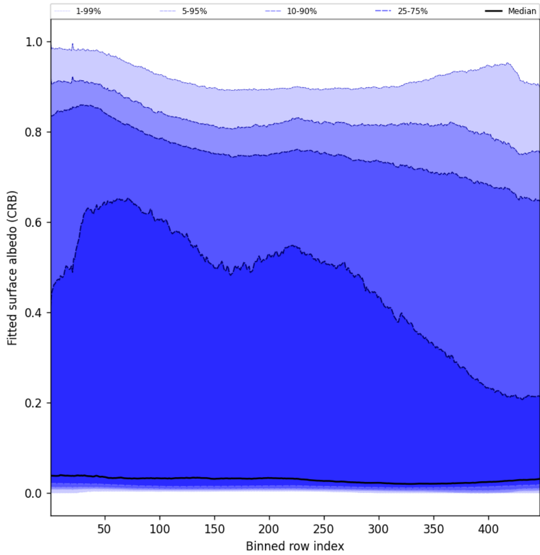
Figure 62: Along track statistics of “Fitted surface albedo (CRB)” for 2025-03-18 to 2025-03-20
