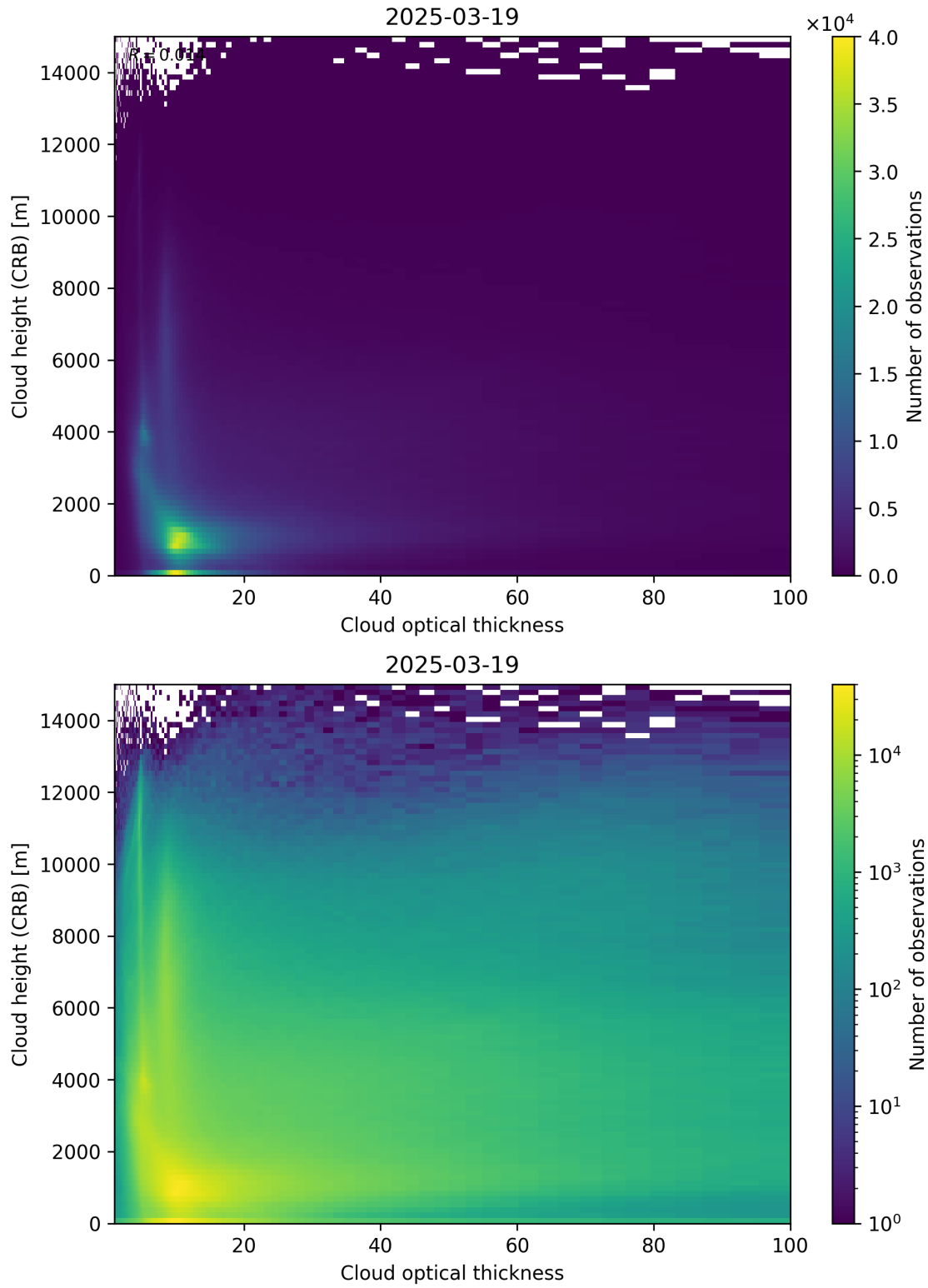
Figure 85: Scatter density plot of “Cloud optical thickness” against “Cloud height (CRB)” for 2025-03-18 to 2025-03-20.
