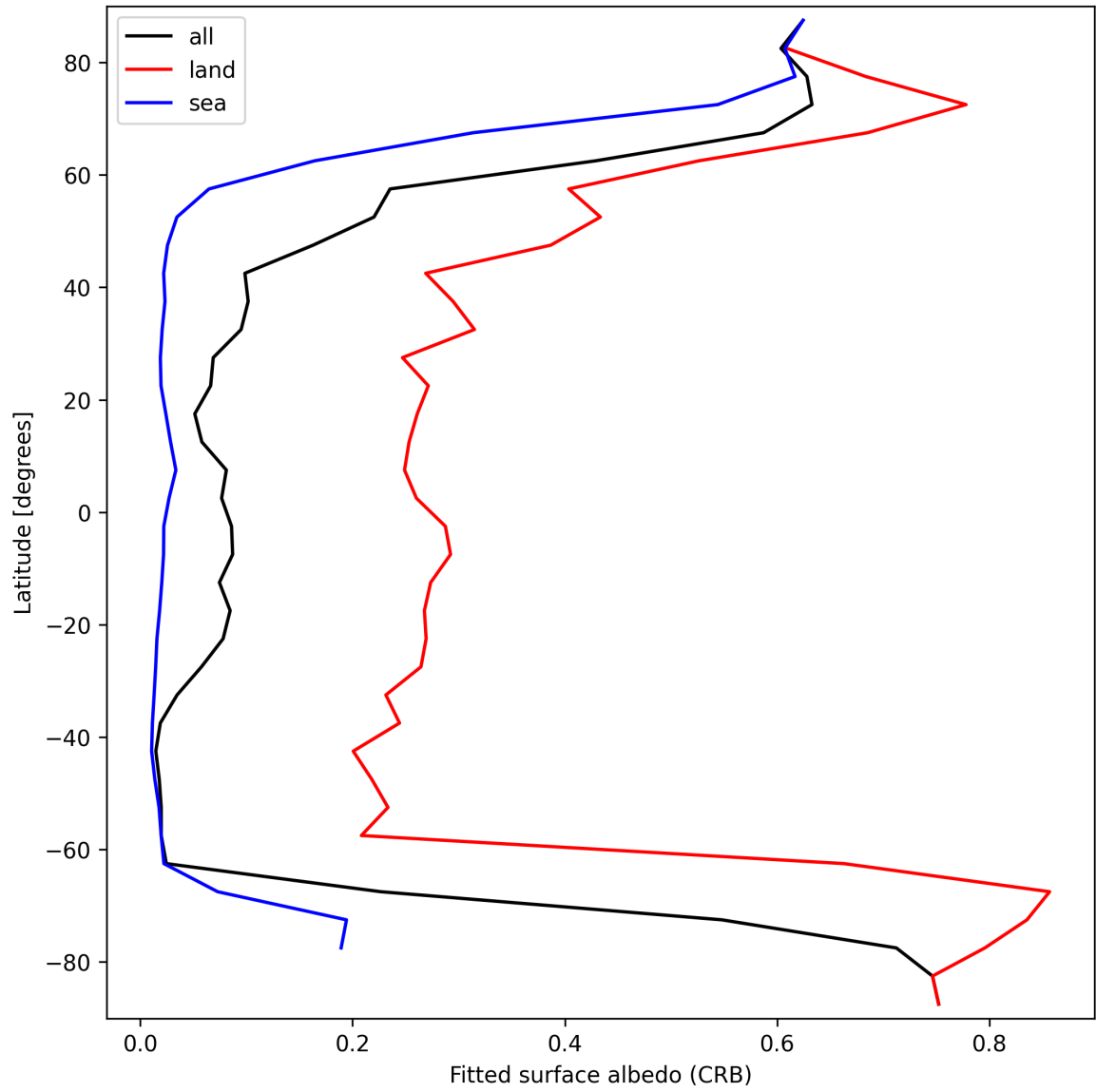
Figure 30: Zonal average of “Fitted surface albedo (CRB)” for 2025-03-18 to 2025-03-20.
