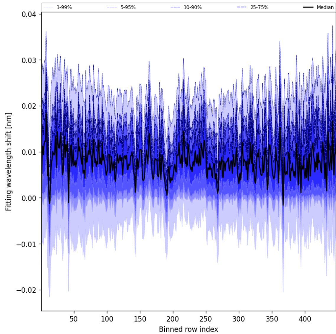
Figure 65: Along track statistics of “Fitting wavelength shift” for 2025-03-18 to 2025-03-20
