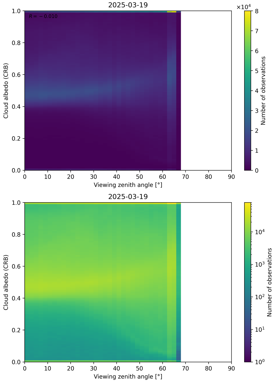
Figure 106: Scatter density plot of “Viewing zenith angle” against “Cloud albedo (CRB)” for 2025-03-18 to 2025-03-20.
