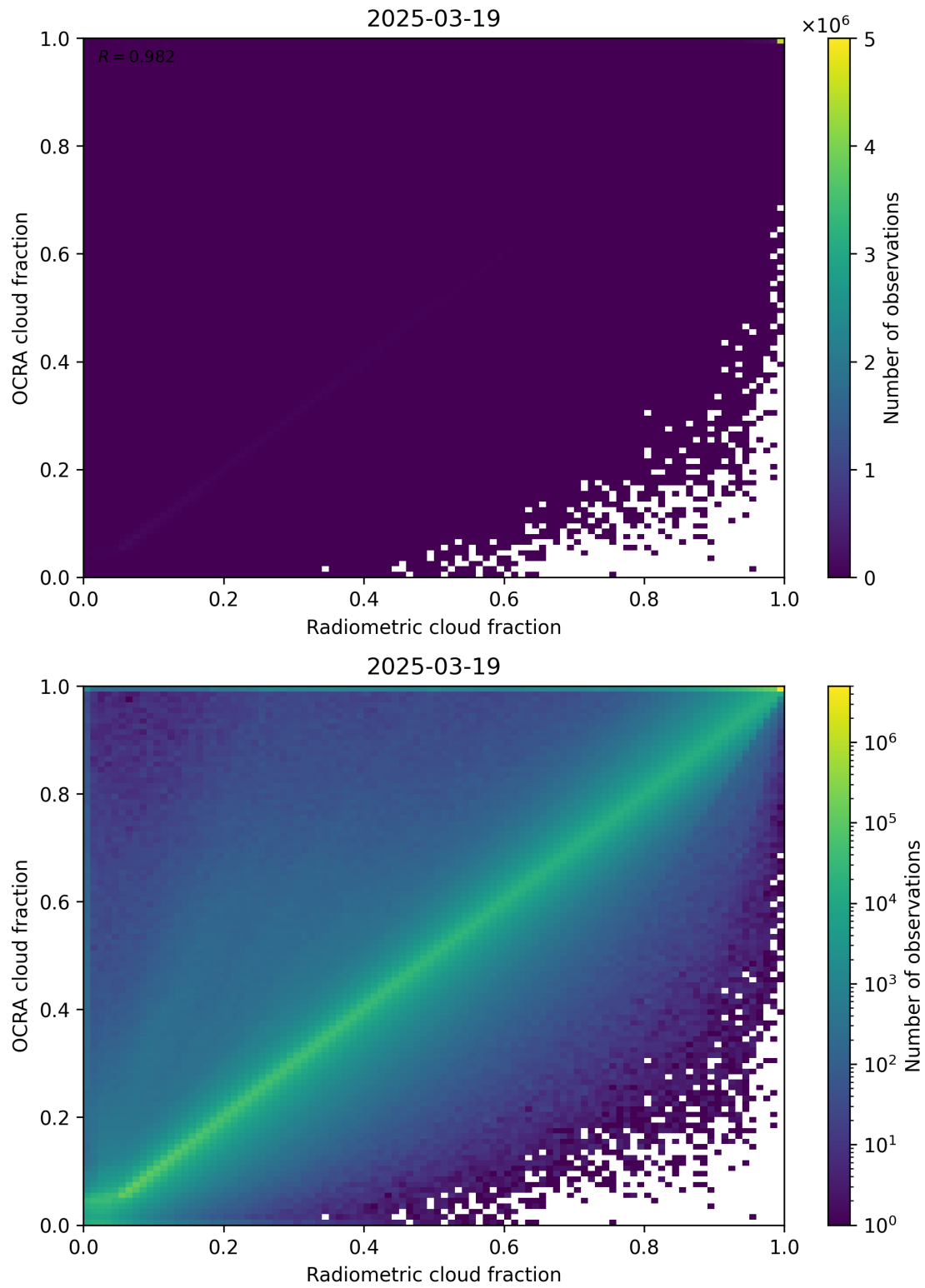
Figure 72: Scatter density plot of “Radiometric cloud fraction” against “OCRA cloud fraction” for 2025-03-18 to 2025-03-20.
