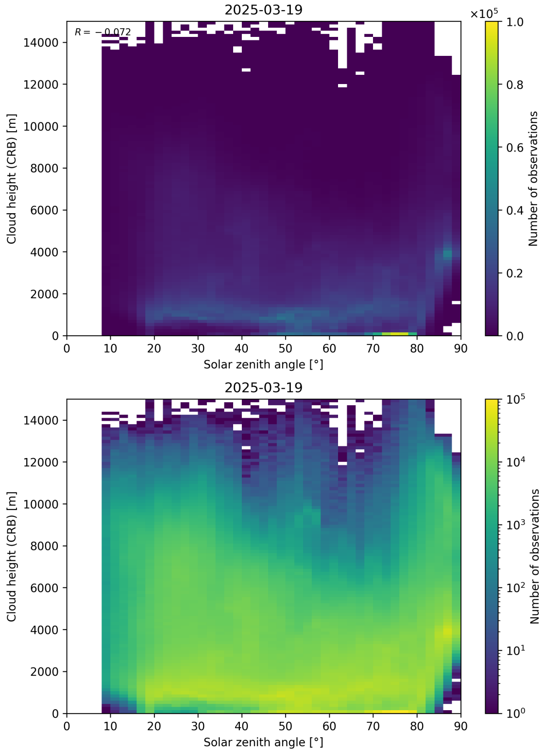
Figure 102: Scatter density plot of “Solar zenith angle” against “Cloud height (CRB)” for 2025-03-18 to 2025-03-20.
