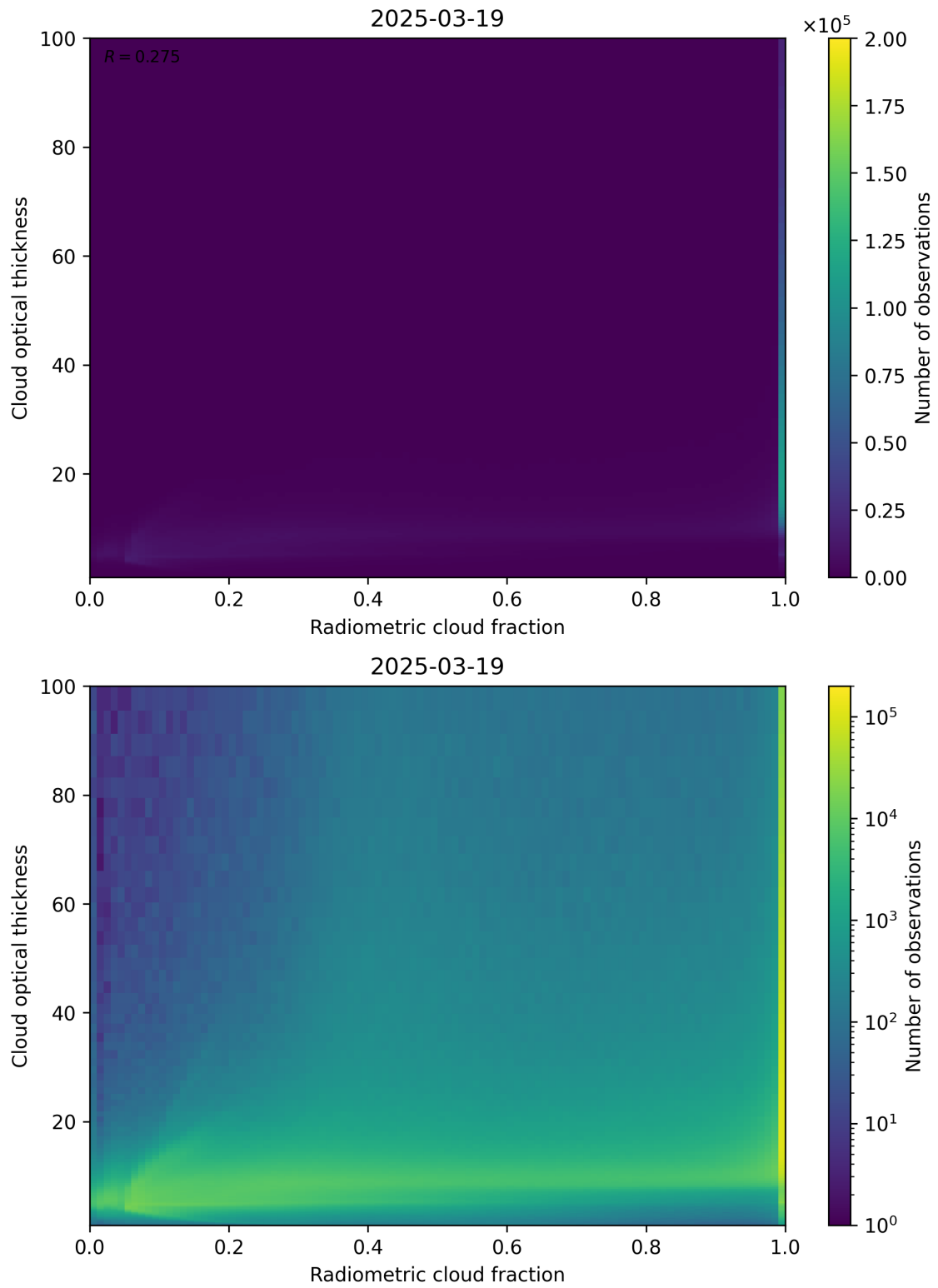
Figure 75: Scatter density plot of “Radiometric cloud fraction” against “Cloud optical thickness” for 2025-03-18 to 2025-03-20.
