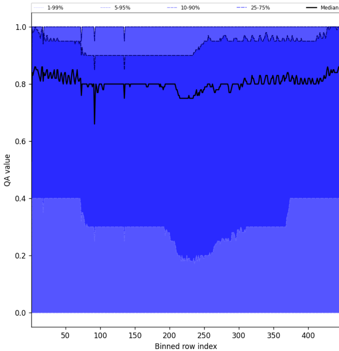
Figure 54: Along track statistics of “QA value” for 2025-03-18 to 2025-03-20
