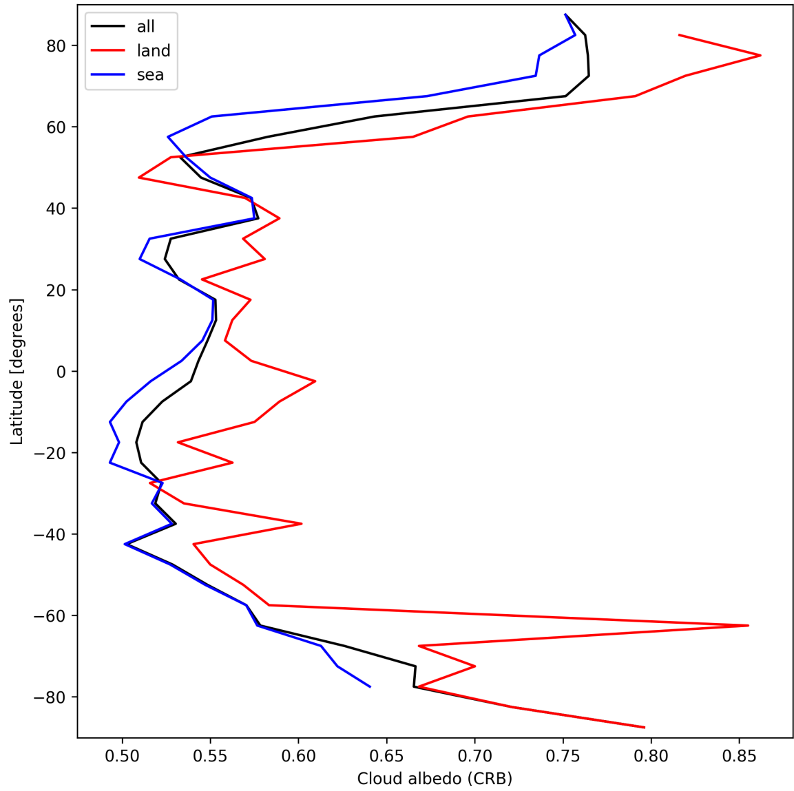
Figure 28: Zonal average of “Cloud albedo (CRB)” for 2025-03-18 to 2025-03-20.
