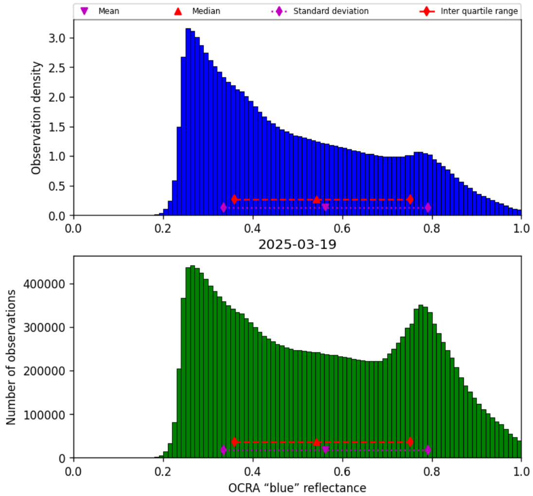
Figure 51: Histogram of “OCRA “blue” reflectance” for 2025-03-18 to 2025-03-20
