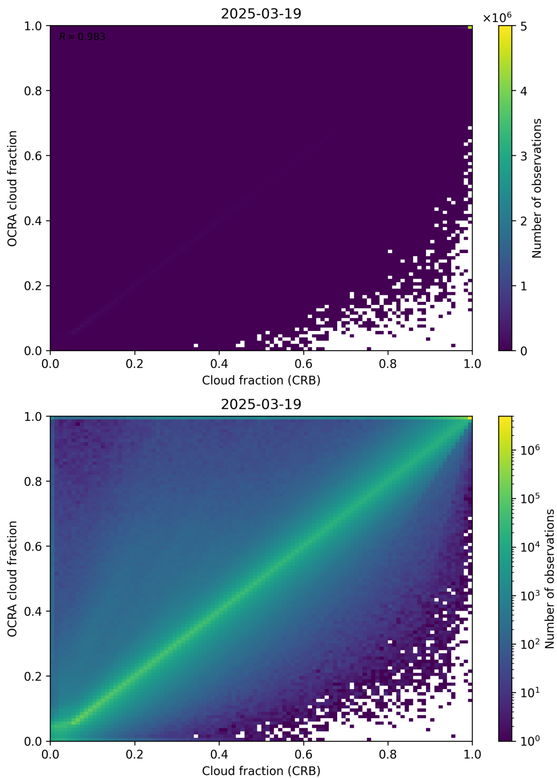
Figure 78: Scatter density plot of “Cloud fraction (CRB)” against “OCRA cloud fraction” for 2025-03-18 to 2025-03-20.
