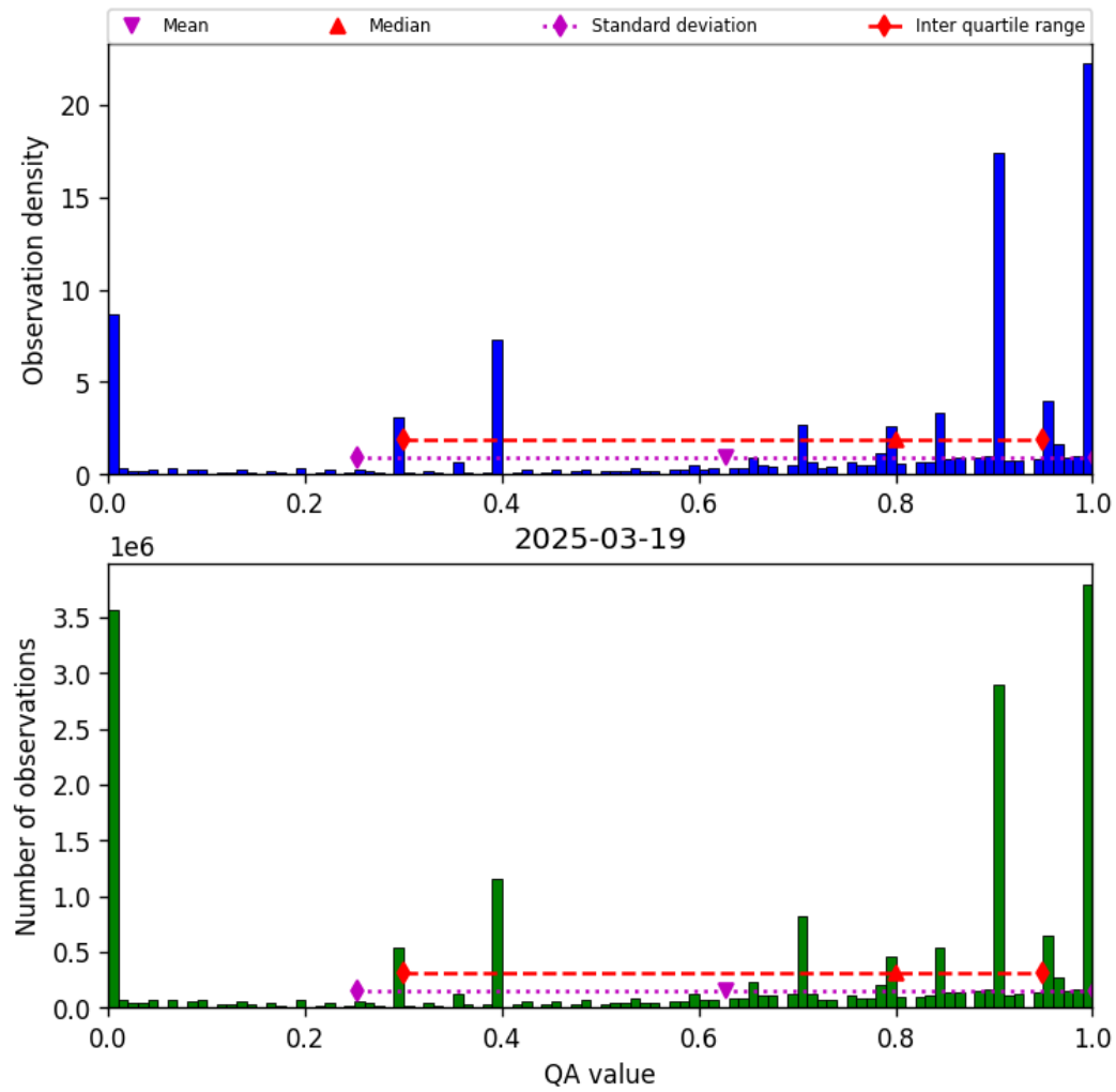
Figure 38: Histogram of “QA value” for 2025-03-18 to 2025-03-20
