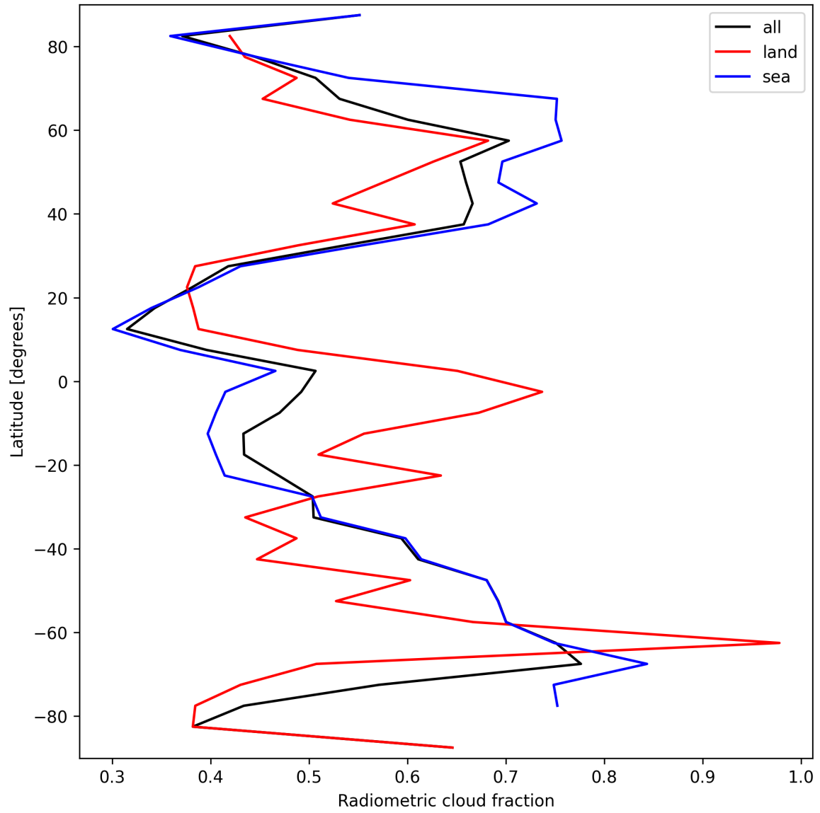
Figure 23: Zonal average of “Radiometric cloud fraction” for 2025-03-18 to 2025-03-20.
