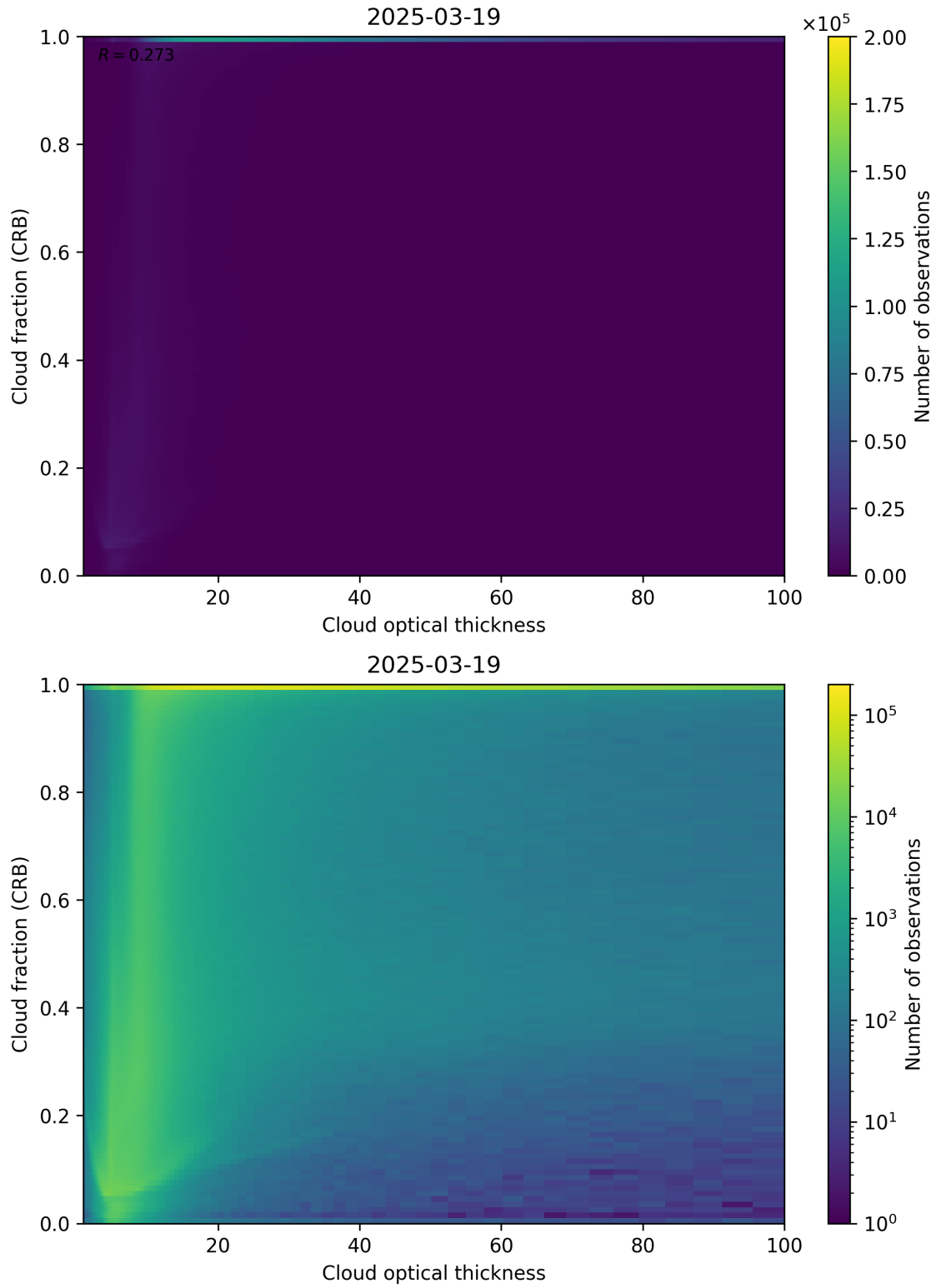
Figure 84: Scatter density plot of “Cloud optical thickness” against “Cloud fraction (CRB)” for 2025-03-18 to 2025-03-20.
