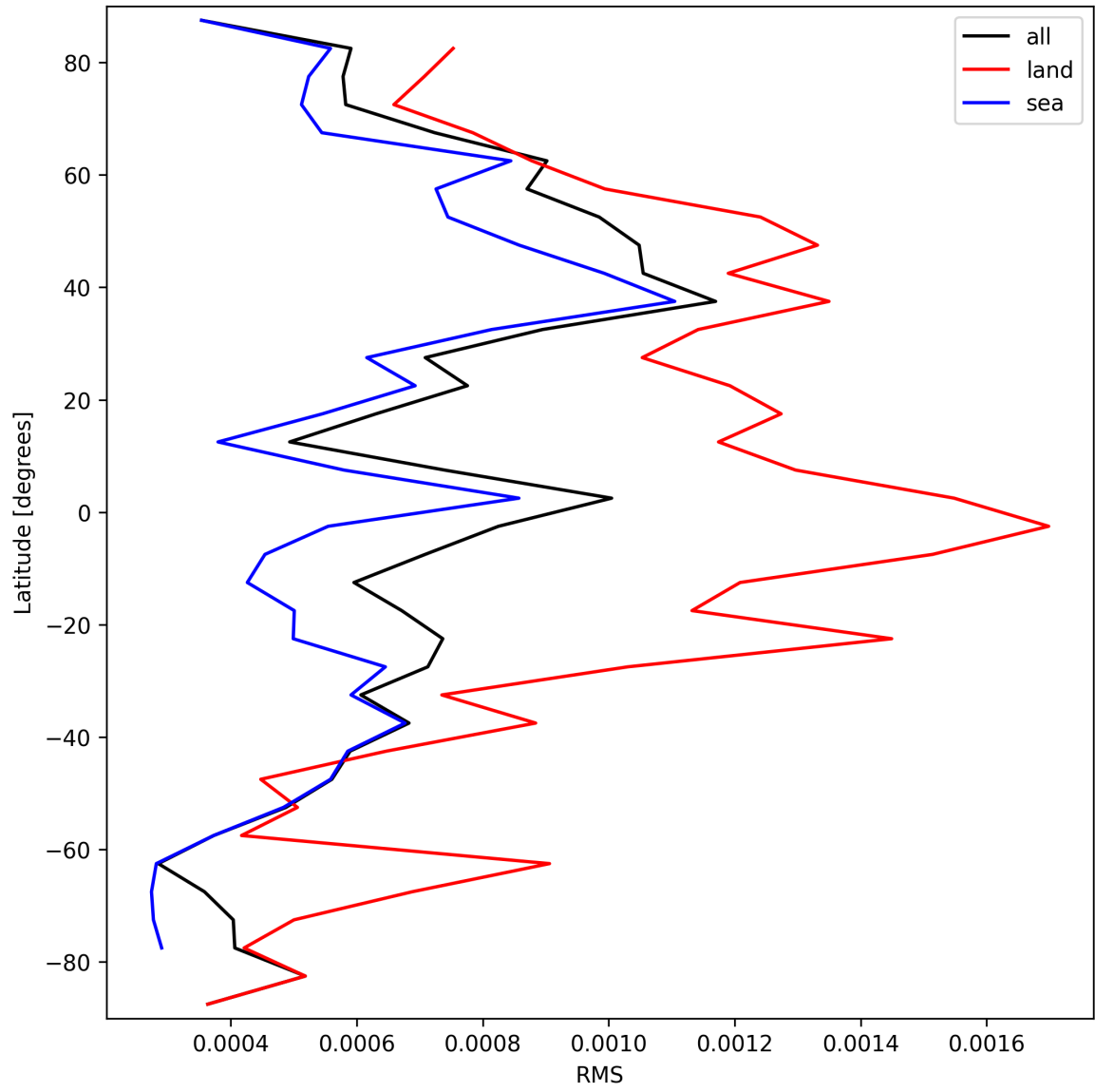
Figure 31: Zonal average of “RMS” for 2025-03-18 to 2025-03-20.
