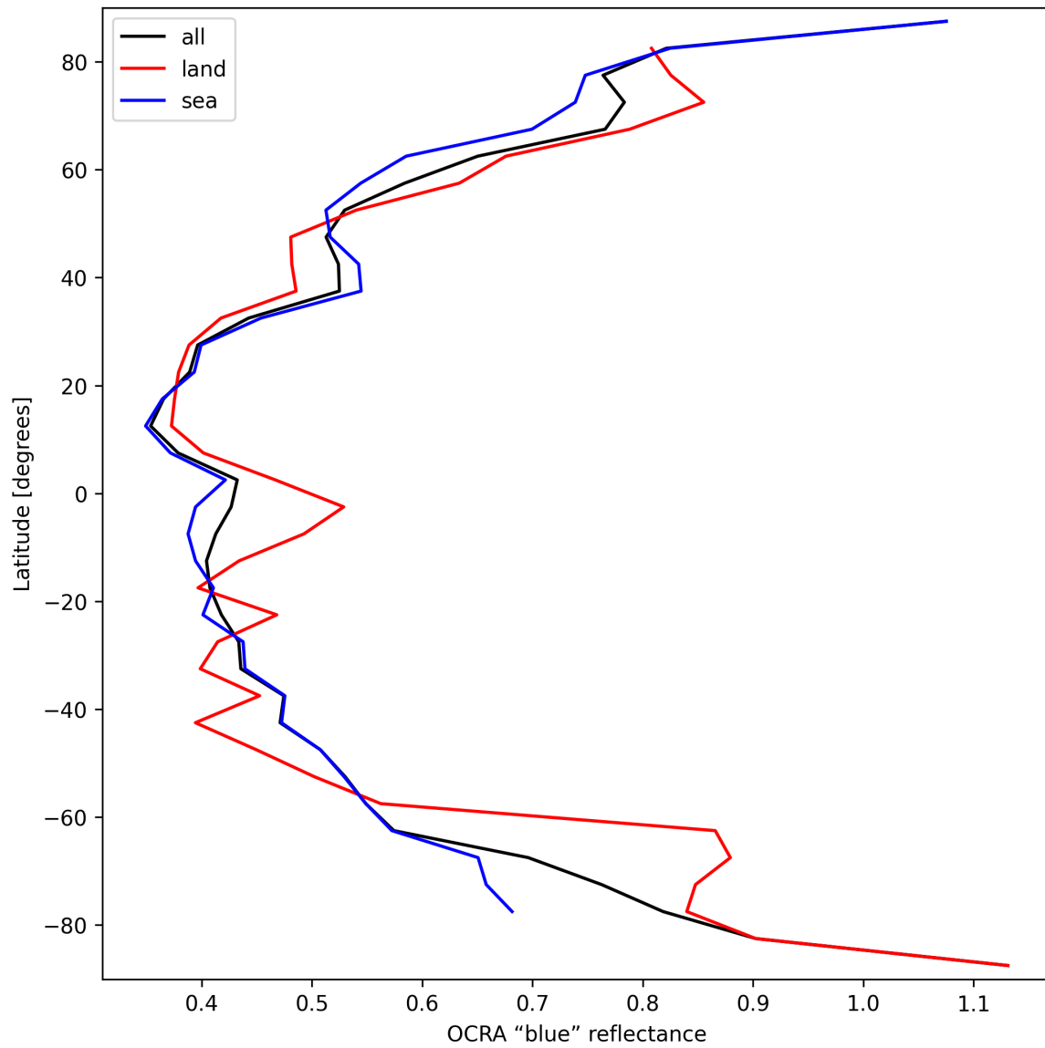
Figure 35: Zonal average of “OCRA “blue” reflectance” for 2025-03-18 to 2025-03-20.
