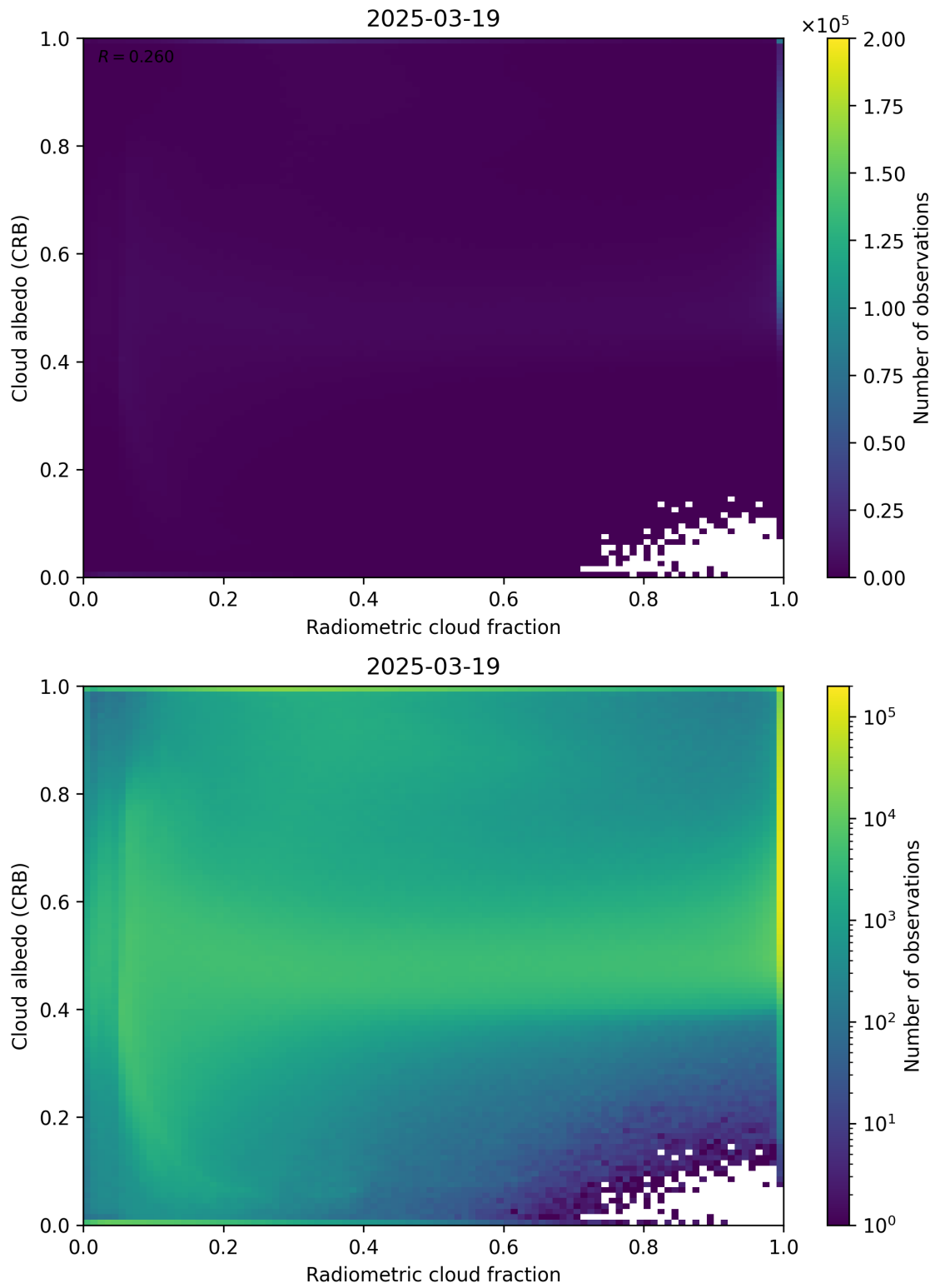
Figure 71: Scatter density plot of “Radiometric cloud fraction” against “Cloud albedo (CRB)” for 2025-03-18 to 2025-03-20.
