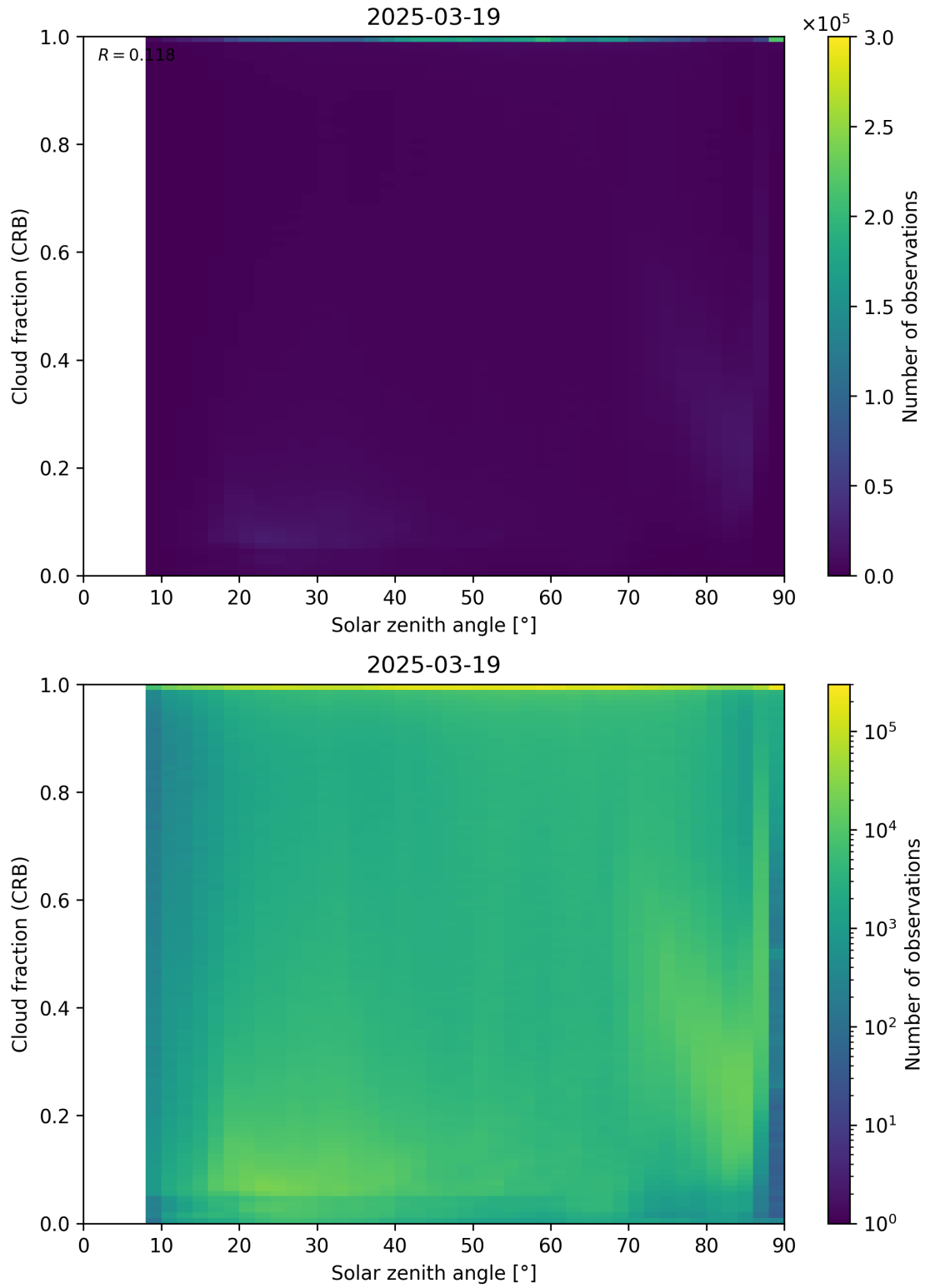
Figure 101: Scatter density plot of “Solar zenith angle” against “Cloud fraction (CRB)” for 2025-03-18 to 2025-03-20.
