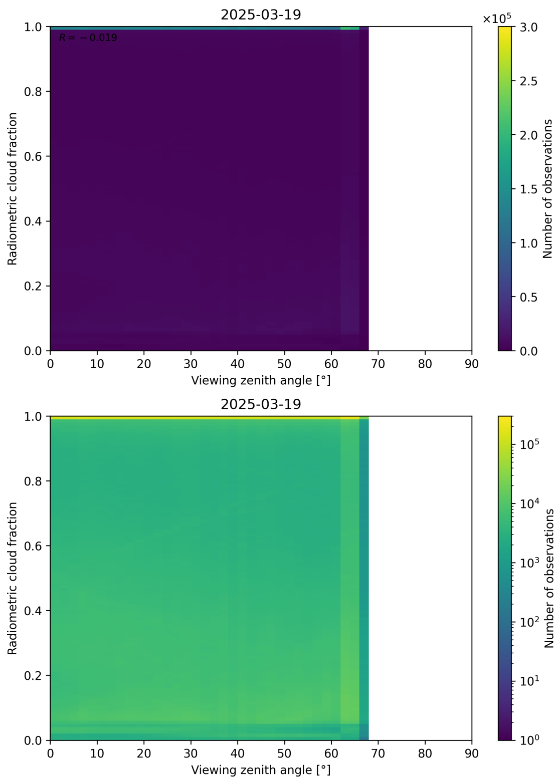
Figure 107: Scatter density plot of “Viewing zenith angle” against “Radiometric cloud fraction” for 2025-03-18 to 2025-03-20.
