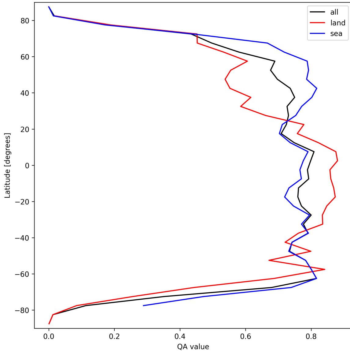
Figure 22: Zonal average of “QA value” for 2025-03-18 to 2025-03-20.
