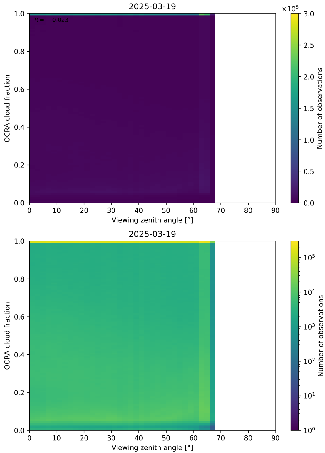
Figure 108: Scatter density plot of “Viewing zenith angle” against “OCRA cloud fraction” for 2025-03-18 to 2025-03-20.
