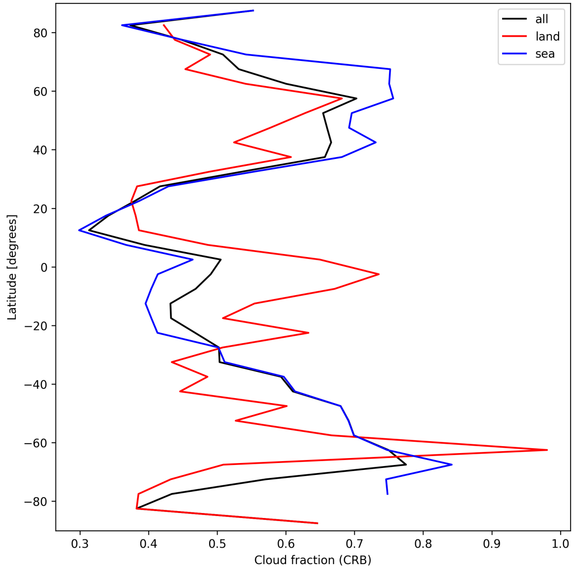
Figure 26: Zonal average of “Cloud fraction (CRB)” for 2025-03-18 to 2025-03-20.
