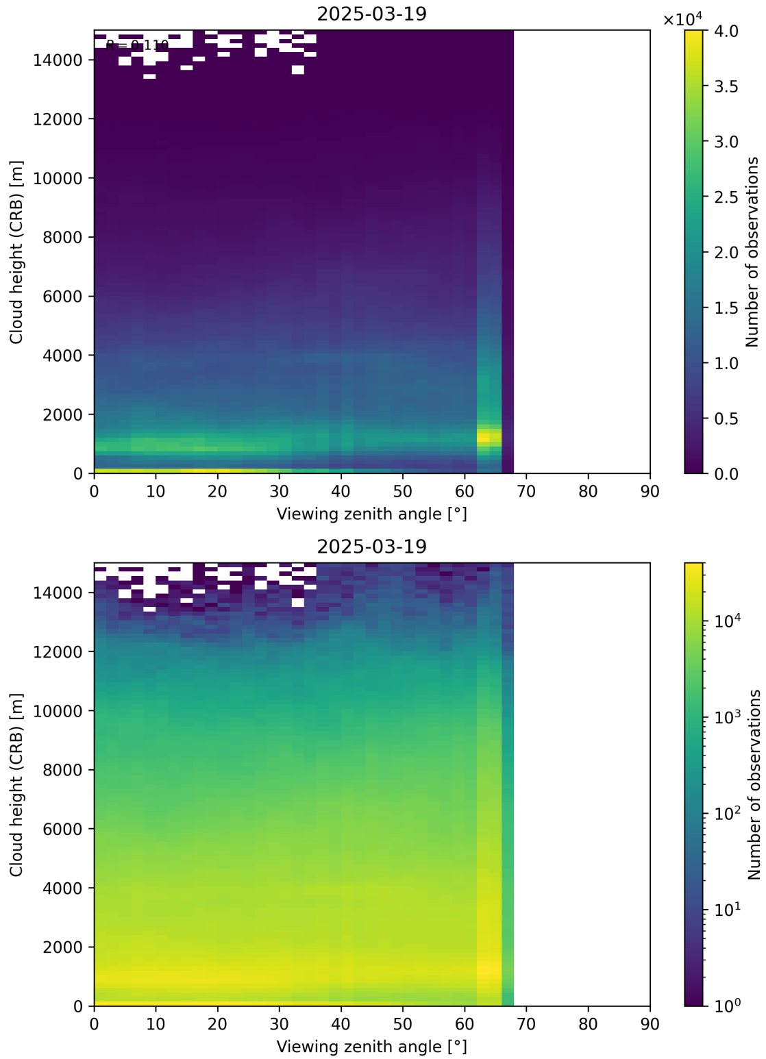
Figure 110: Scatter density plot of “Viewing zenith angle” against “Cloud height (CRB)” for 2025-03-18 to 2025-03-20.
