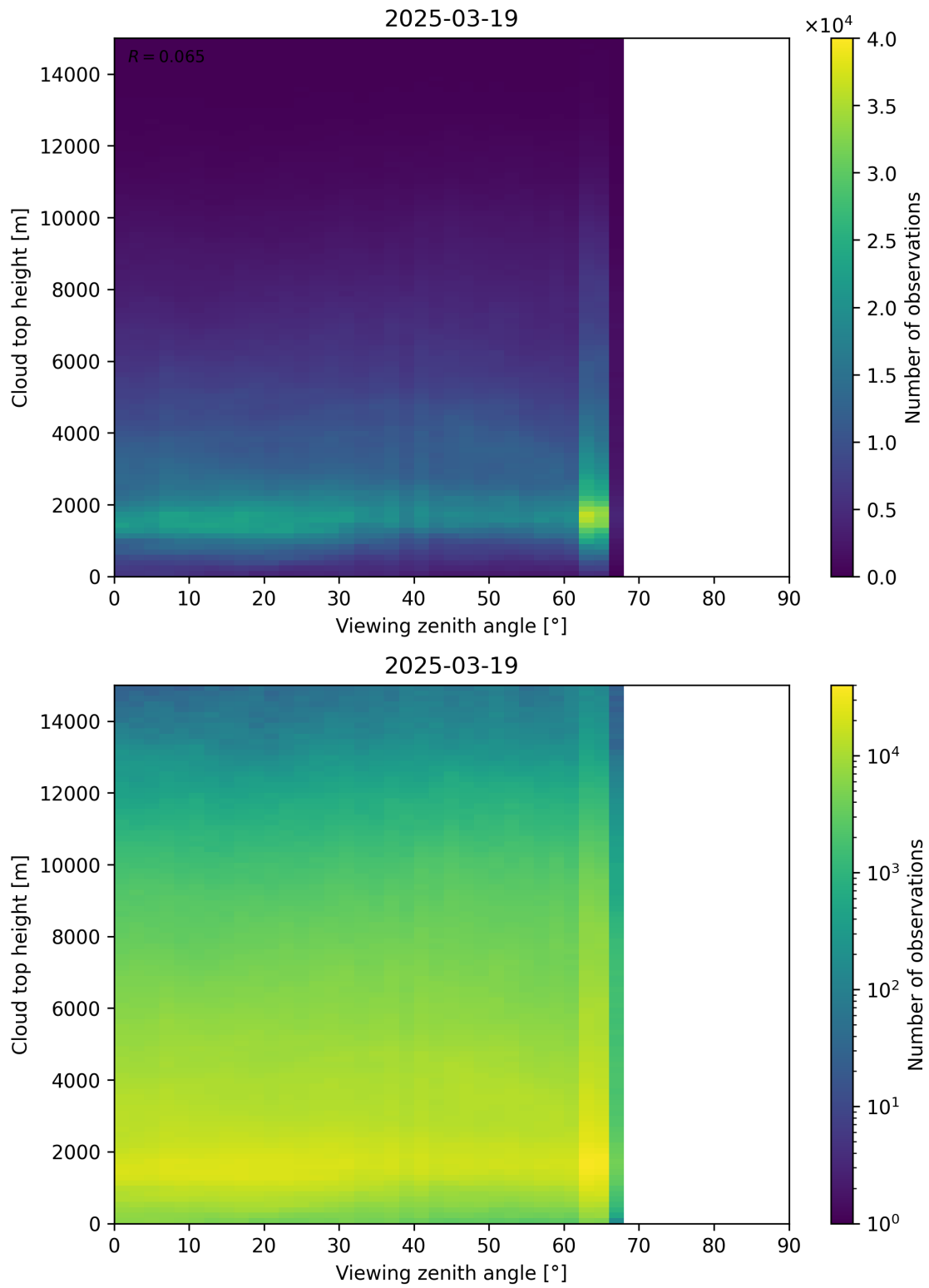
Figure 112: Scatter density plot of “Viewing zenith angle” against “Cloud top height” for 2025-03-18 to 2025-03-20.
