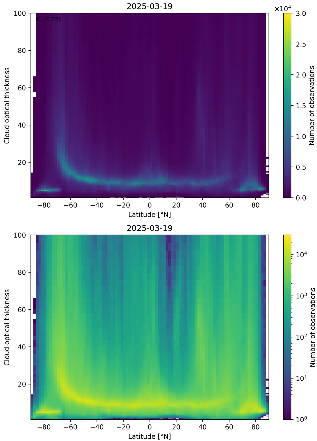
Figure 96: Scatter density plot of “Latitude” against “Cloud optical thickness” for 2025-03-18 to 2025-03-20.
