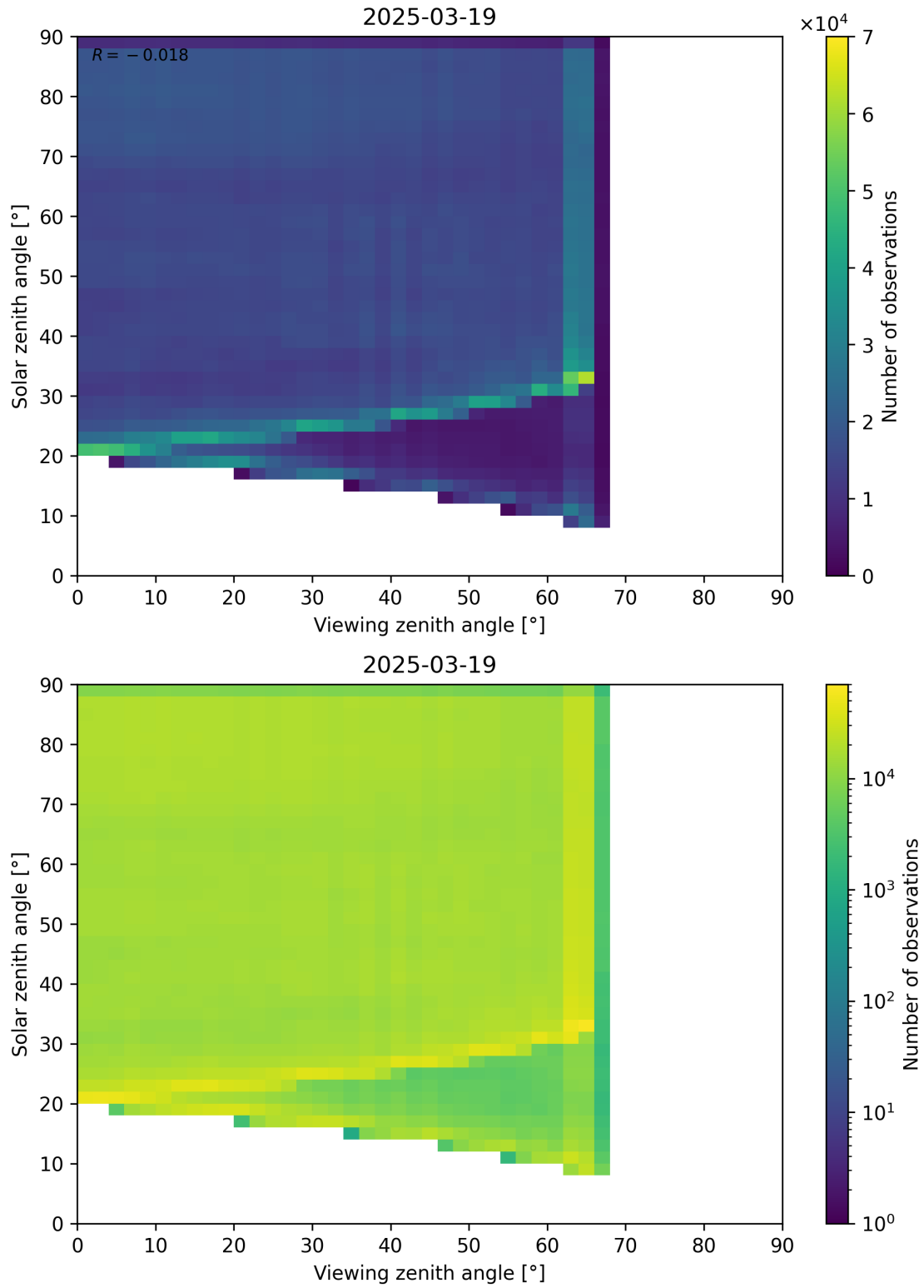
Figure 114: Scatter density plot of “Viewing zenith angle” against “Solar zenith angle” for 2025-03-18 to 2025-03-20.
