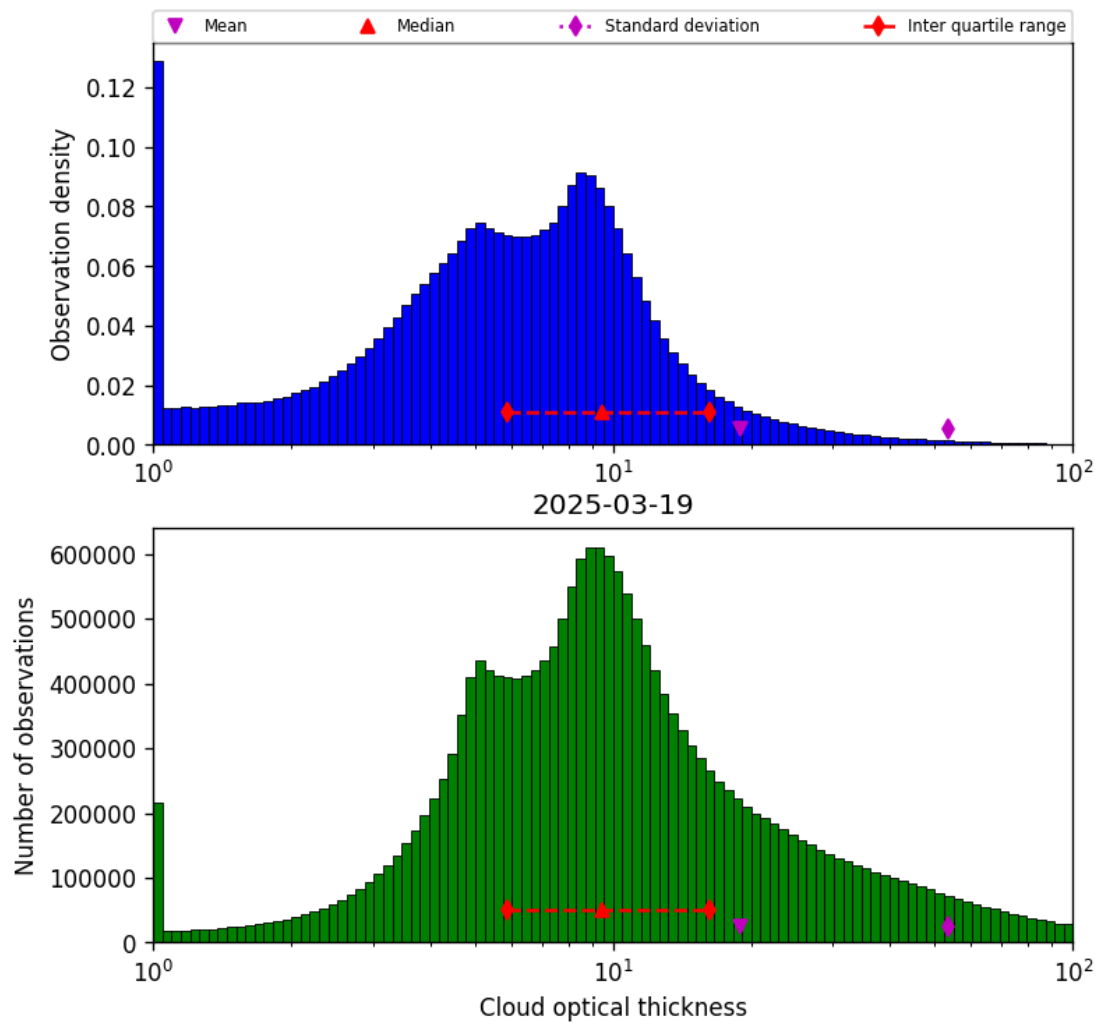
Figure 41: Histogram of “Cloud optical thickness” for 2025-03-18 to 2025-03-20
