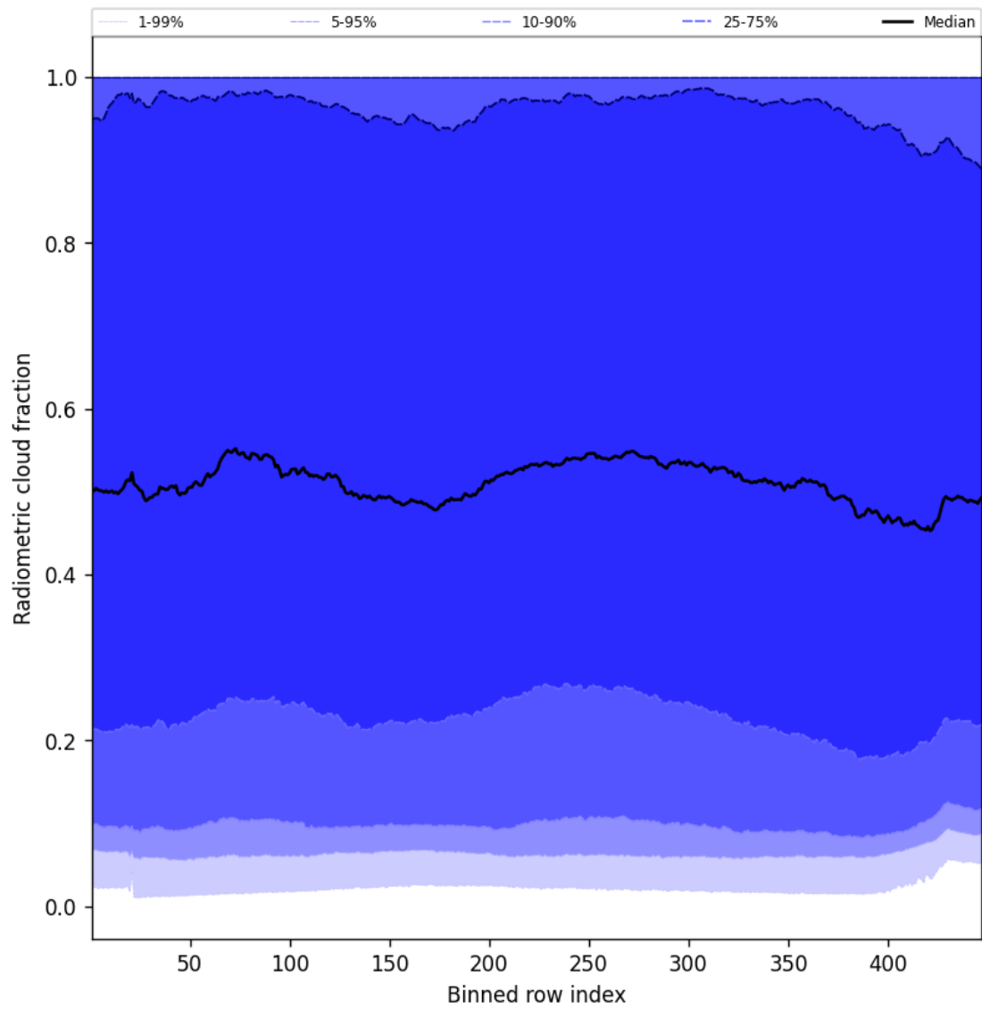
Figure 55: Along track statistics of “Radiometric cloud fraction” for 2025-03-18 to 2025-03-20
