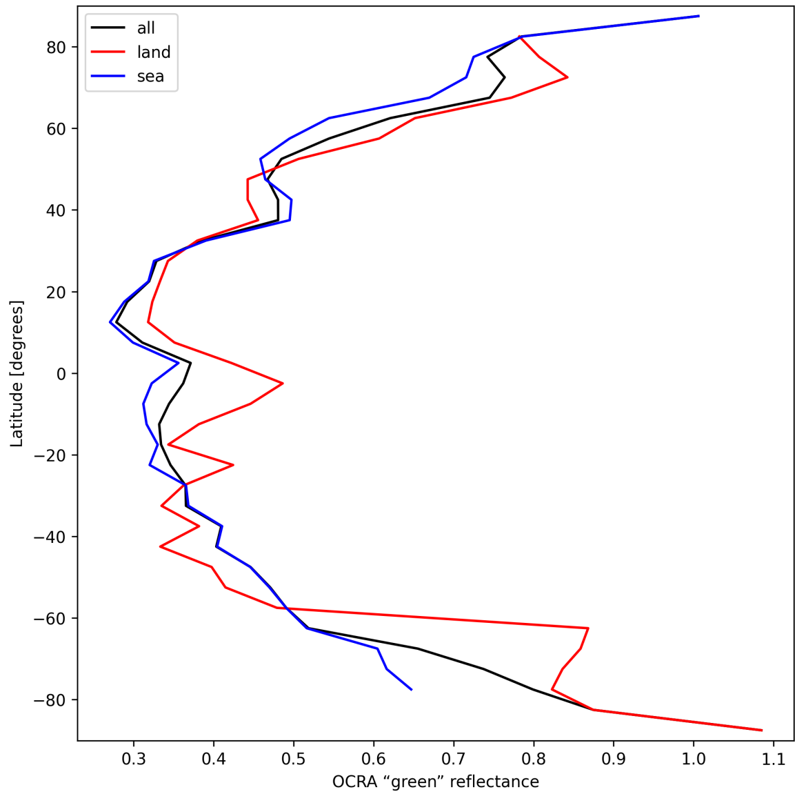
Figure 36: Zonal average of “OCRA “green” reflectance” for 2025-03-18 to 2025-03-20.
