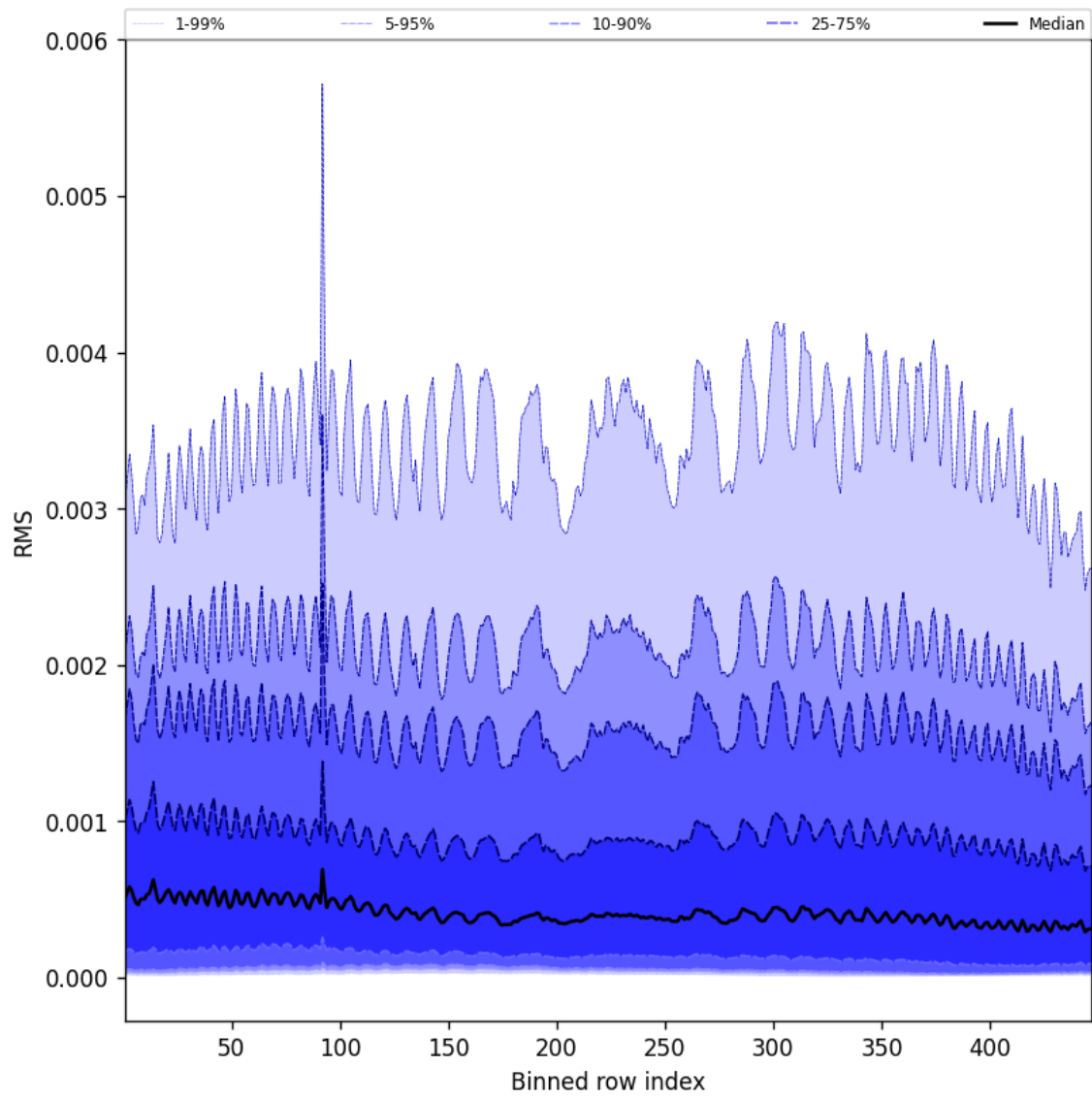
Figure 63: Along track statistics of “RMS” for 2025-03-18 to 2025-03-20
