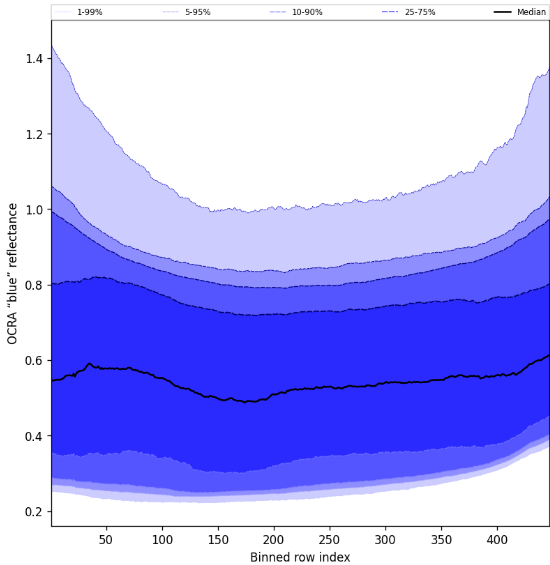
Figure 67: Along track statistics of “OCRA “blue” reflectance” for 2025-03-18 to 2025-03-20
