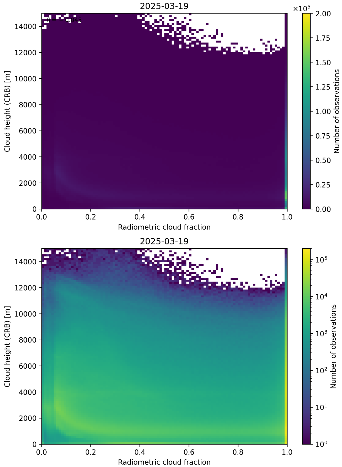
Figure 74: Scatter density plot of “Radiometric cloud fraction” against “Cloud height (CRB)” for 2025-03-18 to 2025-03-20.
