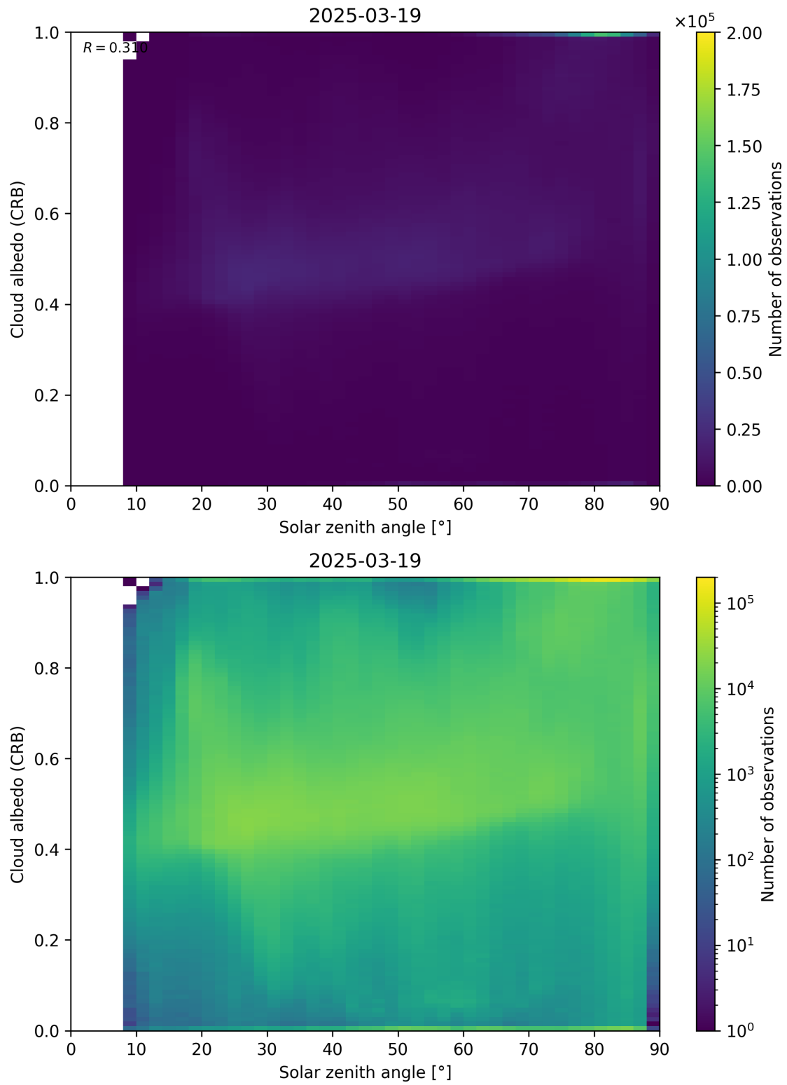
Figure 98: Scatter density plot of “Solar zenith angle” against “Cloud albedo (CRB)” for 2025-03-18 to 2025-03-20.
