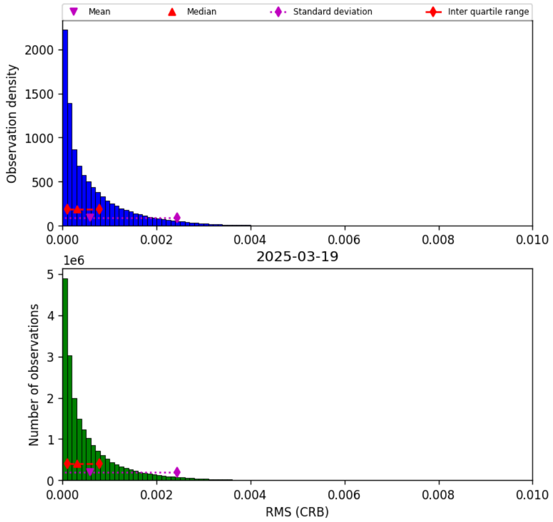
Figure 48: Histogram of “RMS (CRB)” for 2025-03-18 to 2025-03-20
