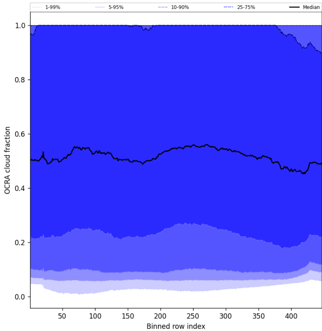
Figure 66: Along track statistics of “OCRA cloud fraction” for 2025-03-18 to 2025-03-20
