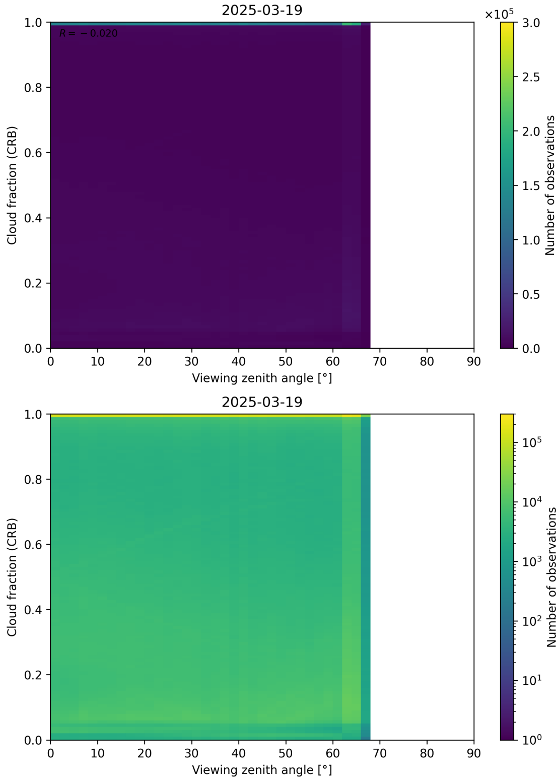
Figure 109: Scatter density plot of “Viewing zenith angle” against “Cloud fraction (CRB)” for 2025-03-18 to 2025-03-20.
