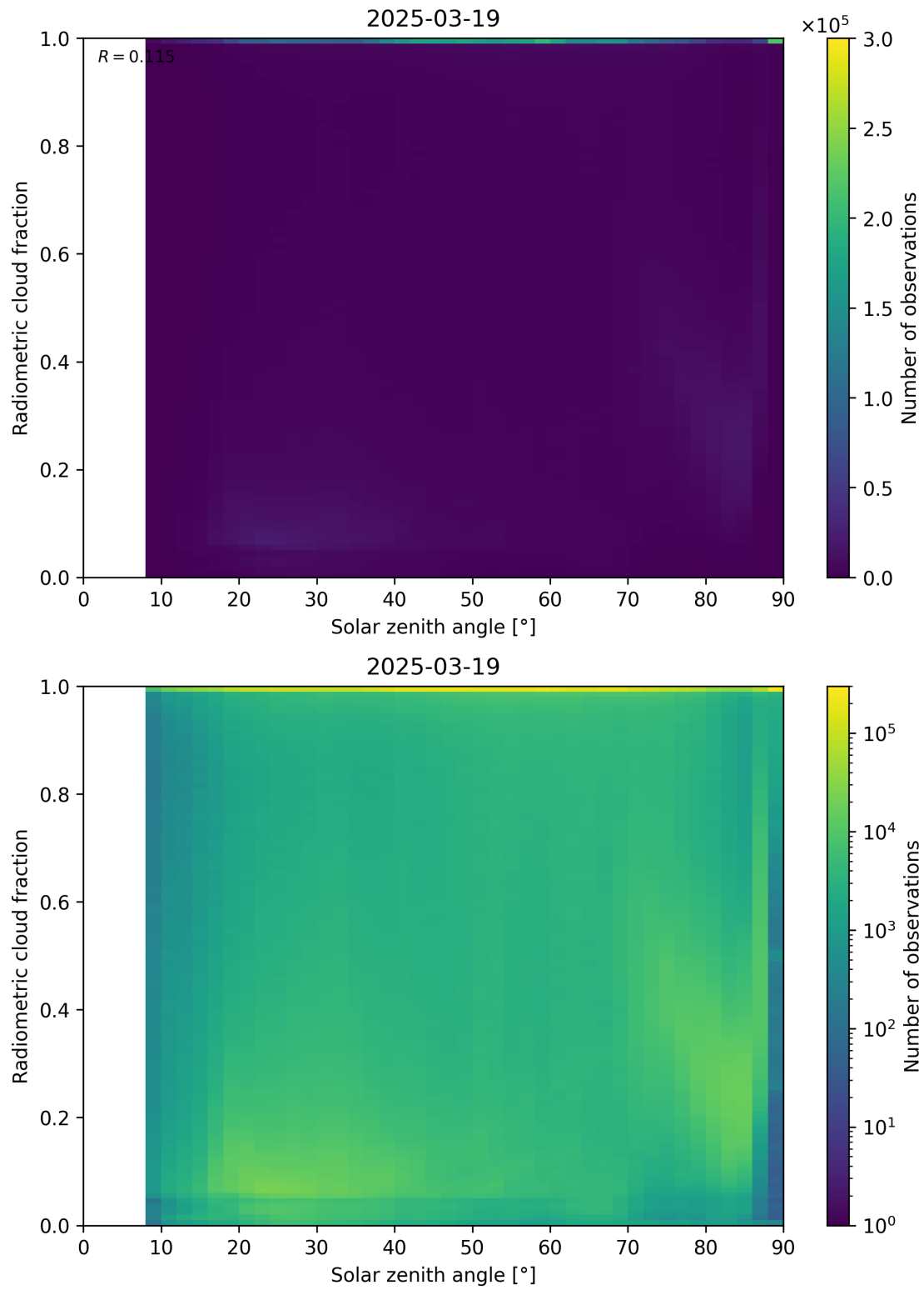
Figure 99: Scatter density plot of “Solar zenith angle” against “Radiometric cloud fraction” for 2025-03-18 to 2025-03-20.
