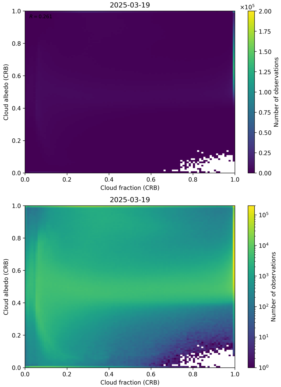
Figure 77: Scatter density plot of “Cloud fraction (CRB)” against “Cloud albedo (CRB)” for 2025-03-18 to 2025-03-20.
