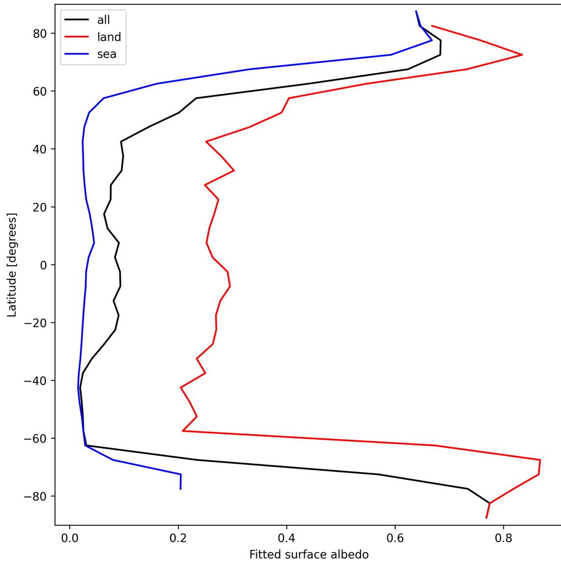
Figure 29: Zonal average of “Fitted surface albedo” for 2025-03-18 to 2025-03-20.
