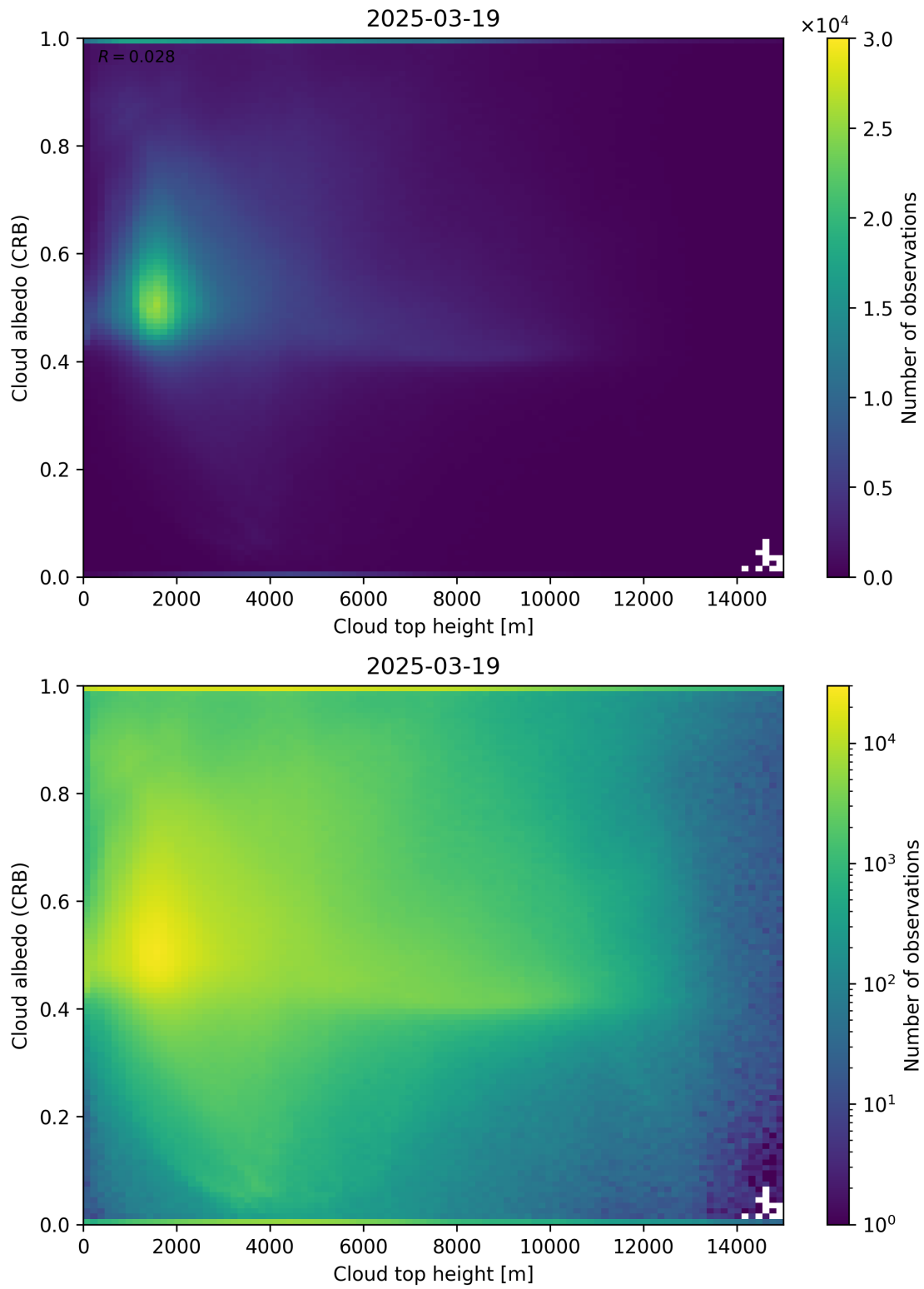
Figure 86: Scatter density plot of “Cloud top height” against “Cloud albedo (CRB)” for 2025-03-18 to 2025-03-20.
