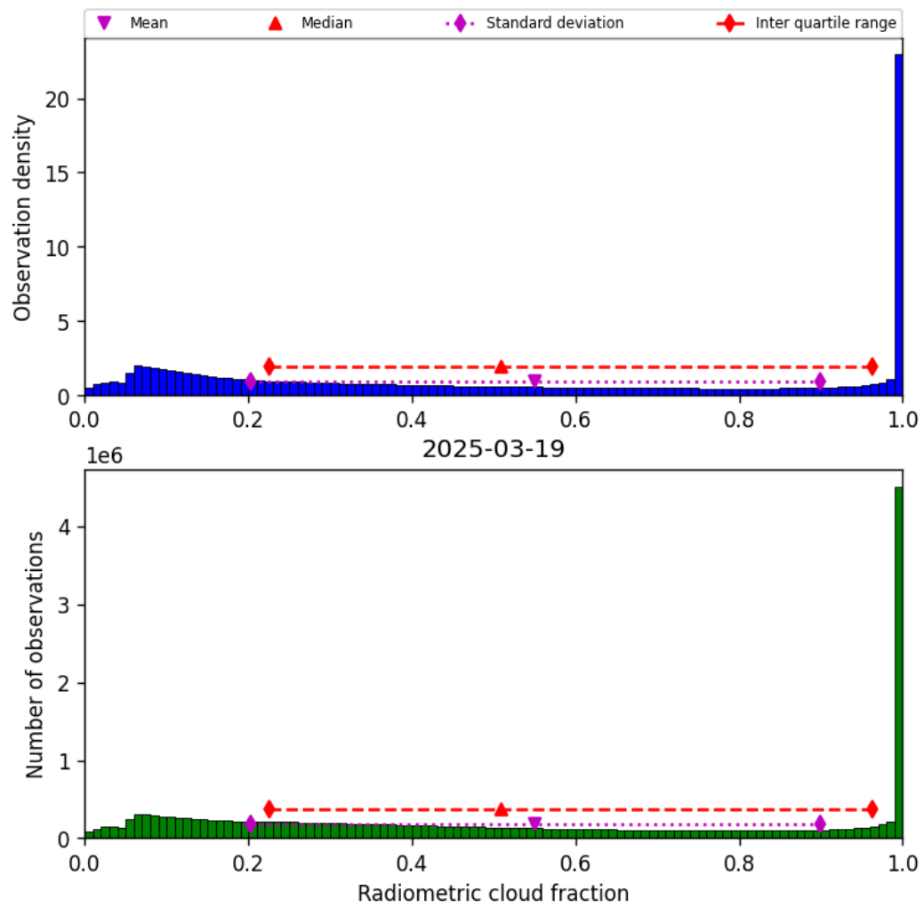
Figure 39: Histogram of “Radiometric cloud fraction” for 2025-03-18 to 2025-03-20
