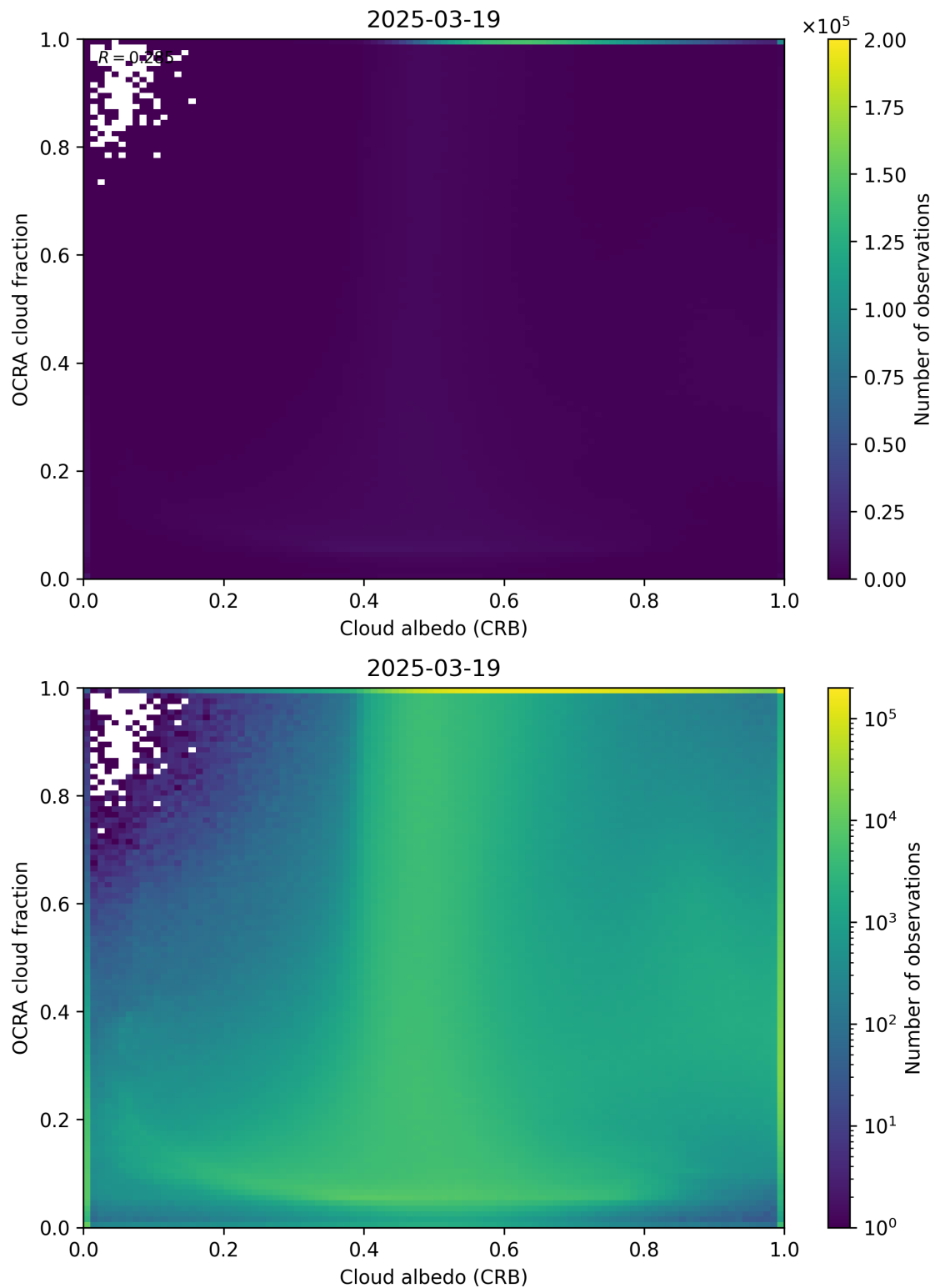
Figure 70: Scatter density plot of “Cloud albedo (CRB)” against “OCRA cloud fraction” for 2025-03-18 to 2025-03-20.
