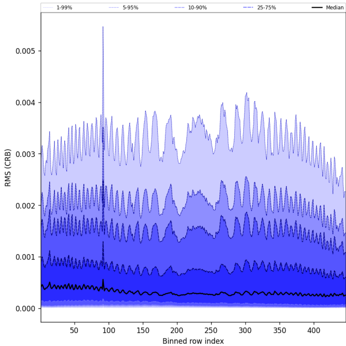
Figure 64: Along track statistics of “RMS (CRB)” for 2025-03-18 to 2025-03-20
