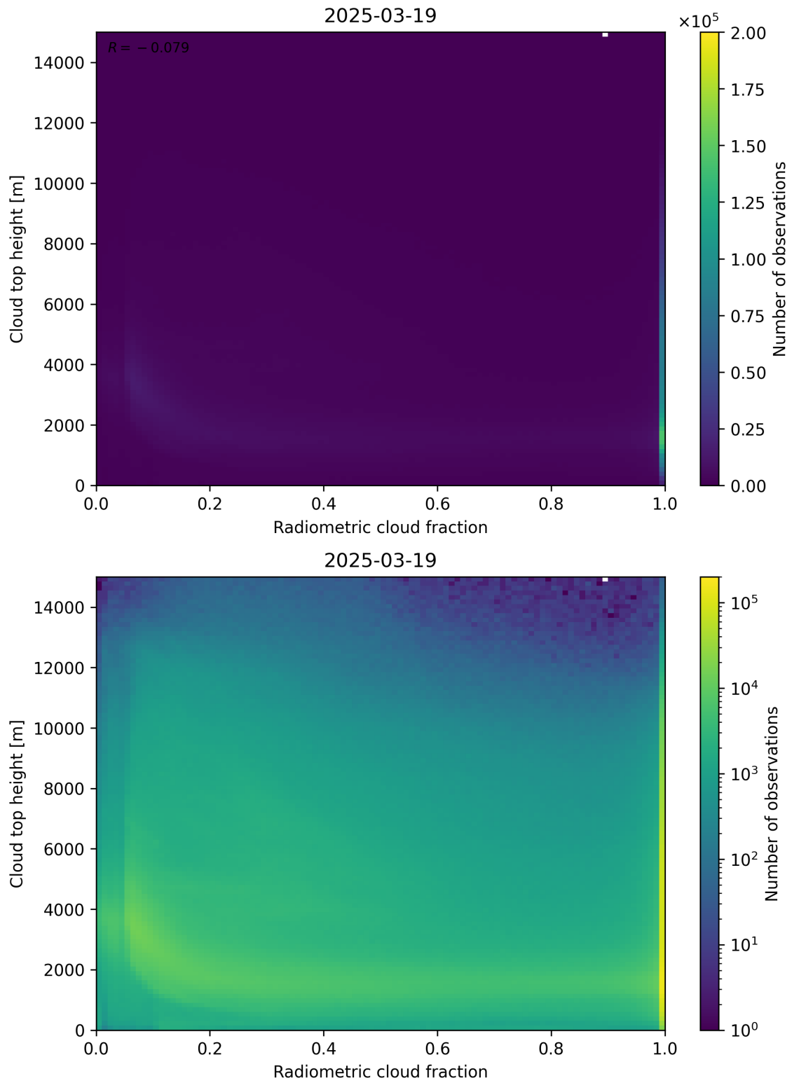
Figure 76: Scatter density plot of “Radiometric cloud fraction” against “Cloud top height” for 2025-03-18 to 2025-03-20.
