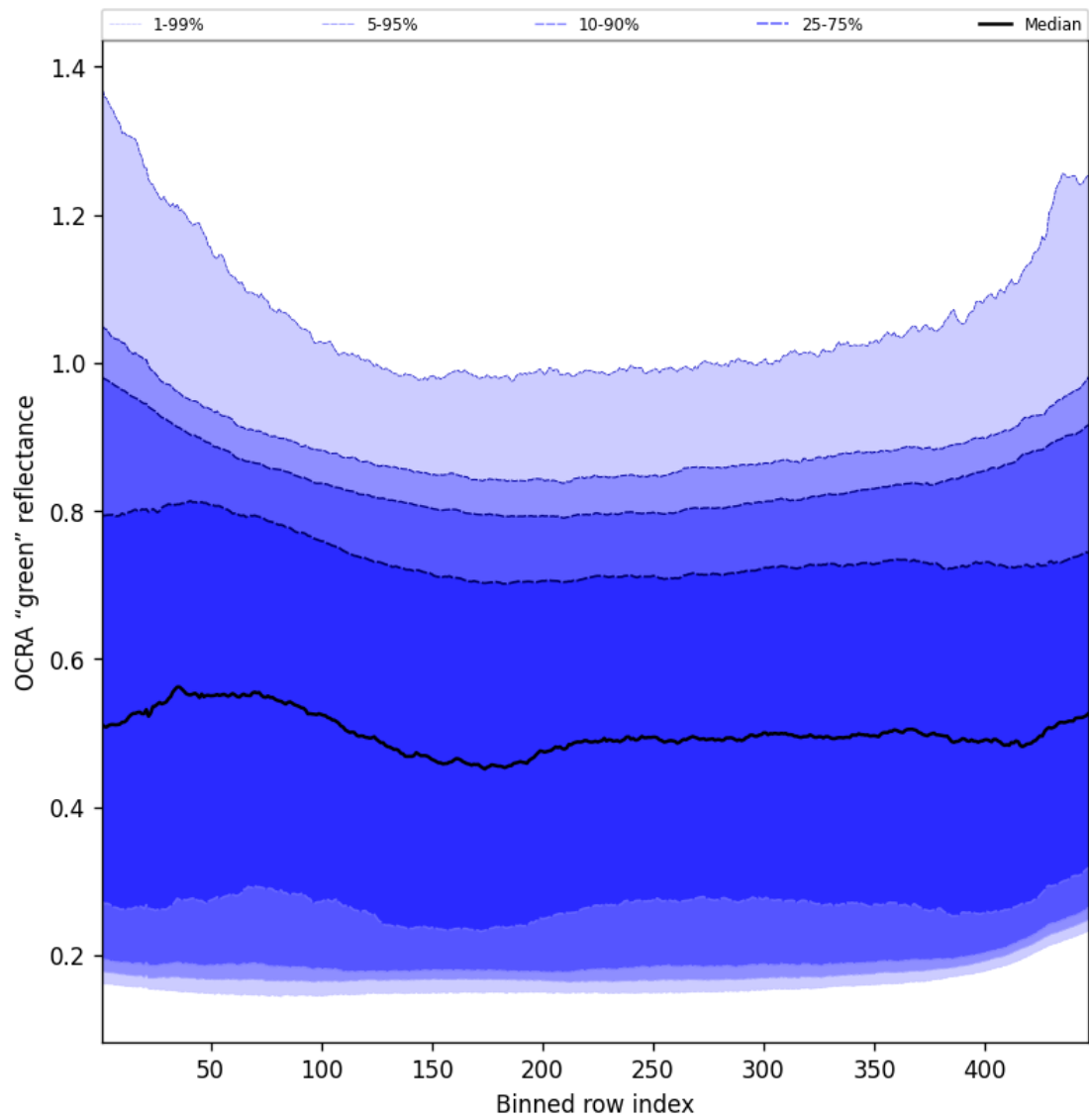
Figure 68: Along track statistics of "OCRA "green" reflectance" for 2025-03-18 to 2025-03-20
