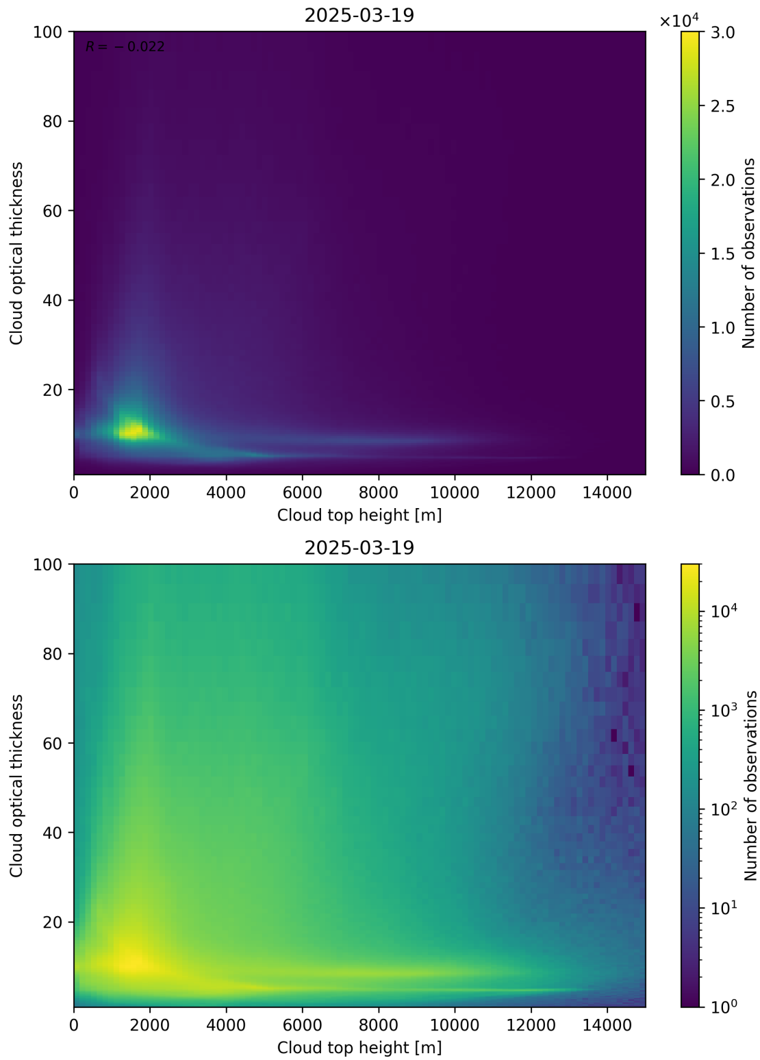
Figure 90: Scatter density plot of “Cloud top height” against “Cloud optical thickness” for 2025-03-18 to 2025-03-20.
