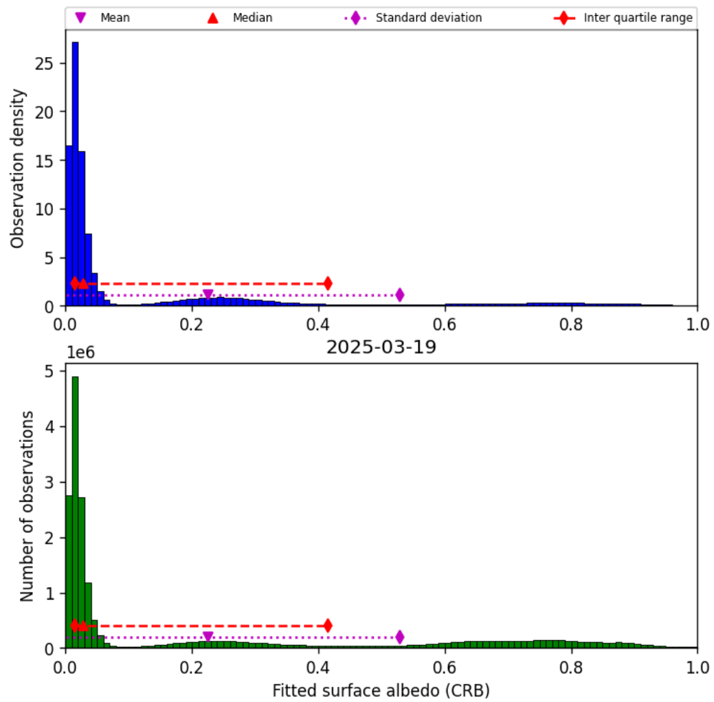
Figure 46: Histogram of “Fitted surface albedo (CRB)” for 2025-03-18 to 2025-03-20
