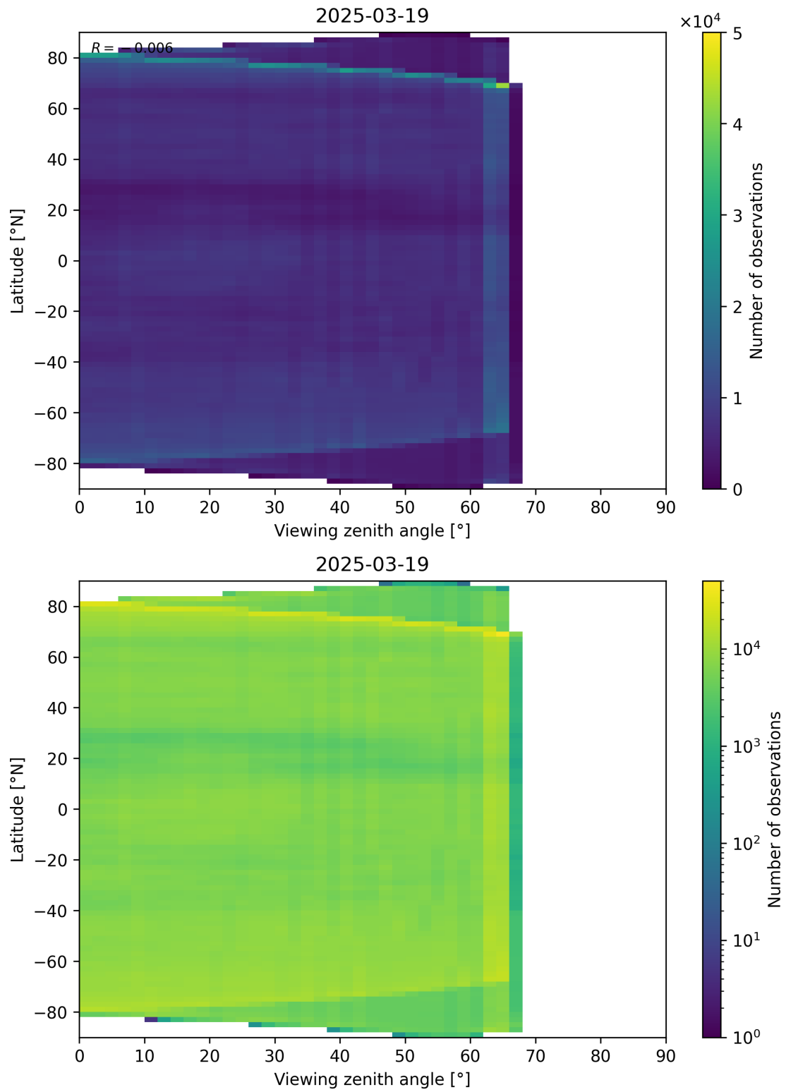
Figure 113: Scatter density plot of “Viewing zenith angle” against “Latitude” for 2025-03-18 to 2025-03-20.
