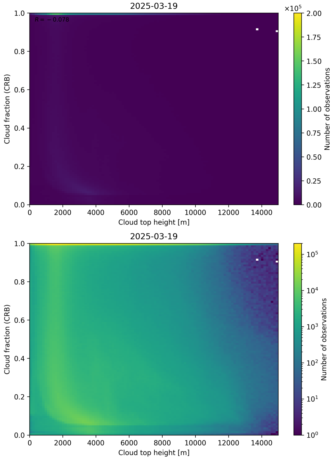
Figure 88: Scatter density plot of “Cloud top height” against “Cloud fraction (CRB)” for 2025-03-18 to 2025-03-20.
