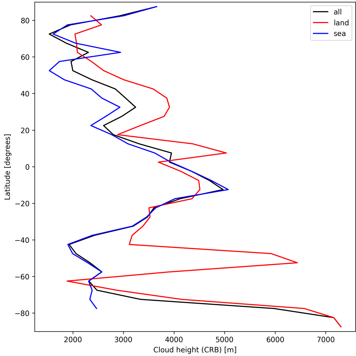
Figure 27: Zonal average of “Cloud height (CRB)” for 2025-03-23 to 2025-03-24.
