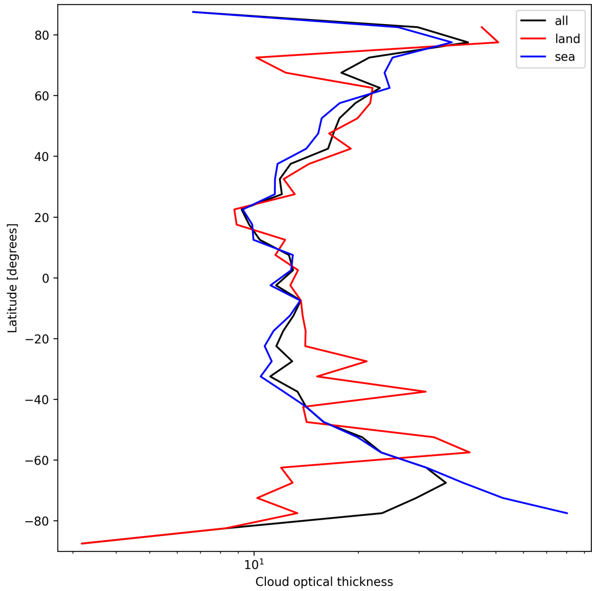
Figure 25: Zonal average of “Cloud optical thickness” for 2025-03-23 to 2025-03-24.
