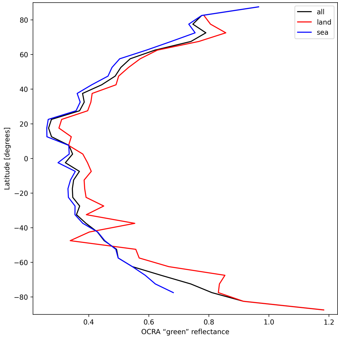
Figure 36: Zonal average of “OCRA “green” reflectance” for 2025-03-23 to 2025-03-24.
