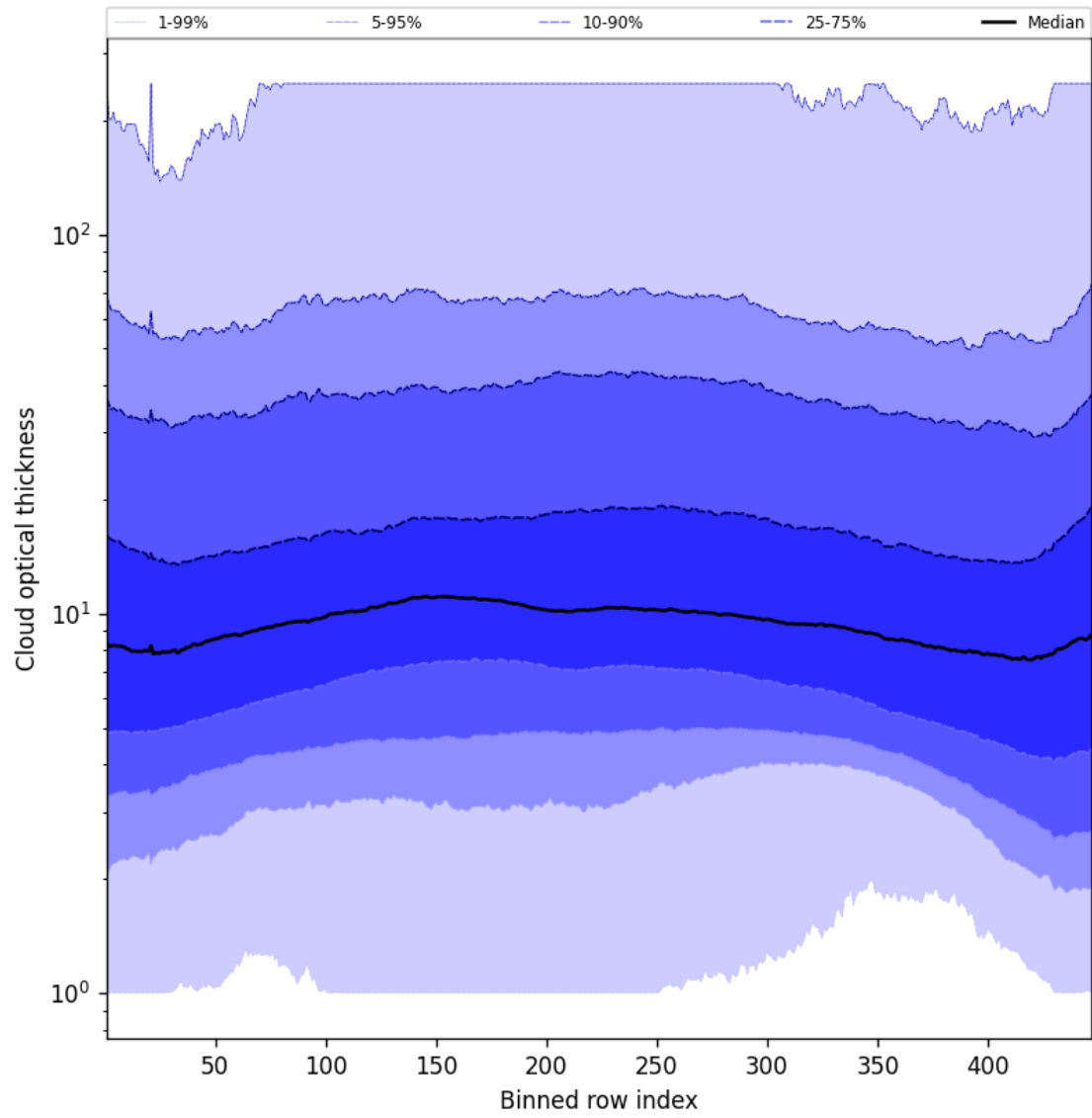
Figure 57: Along track statistics of “Cloud optical thickness” for 2025-03-23 to 2025-03-24
