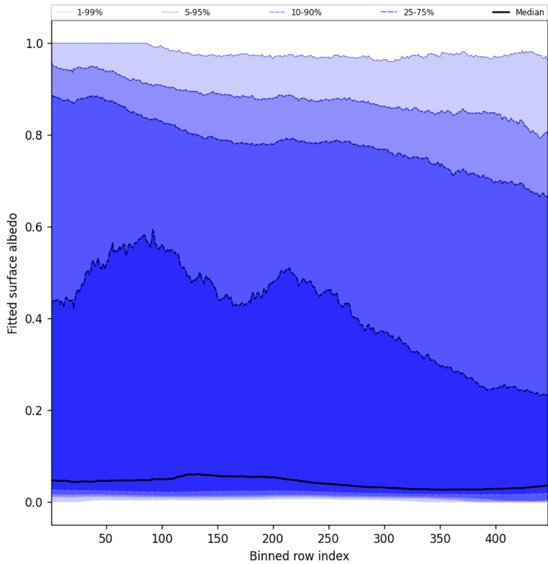
Figure 61: Along track statistics of “Fitted surface albedo” for 2025-03-23 to 2025-03-24
