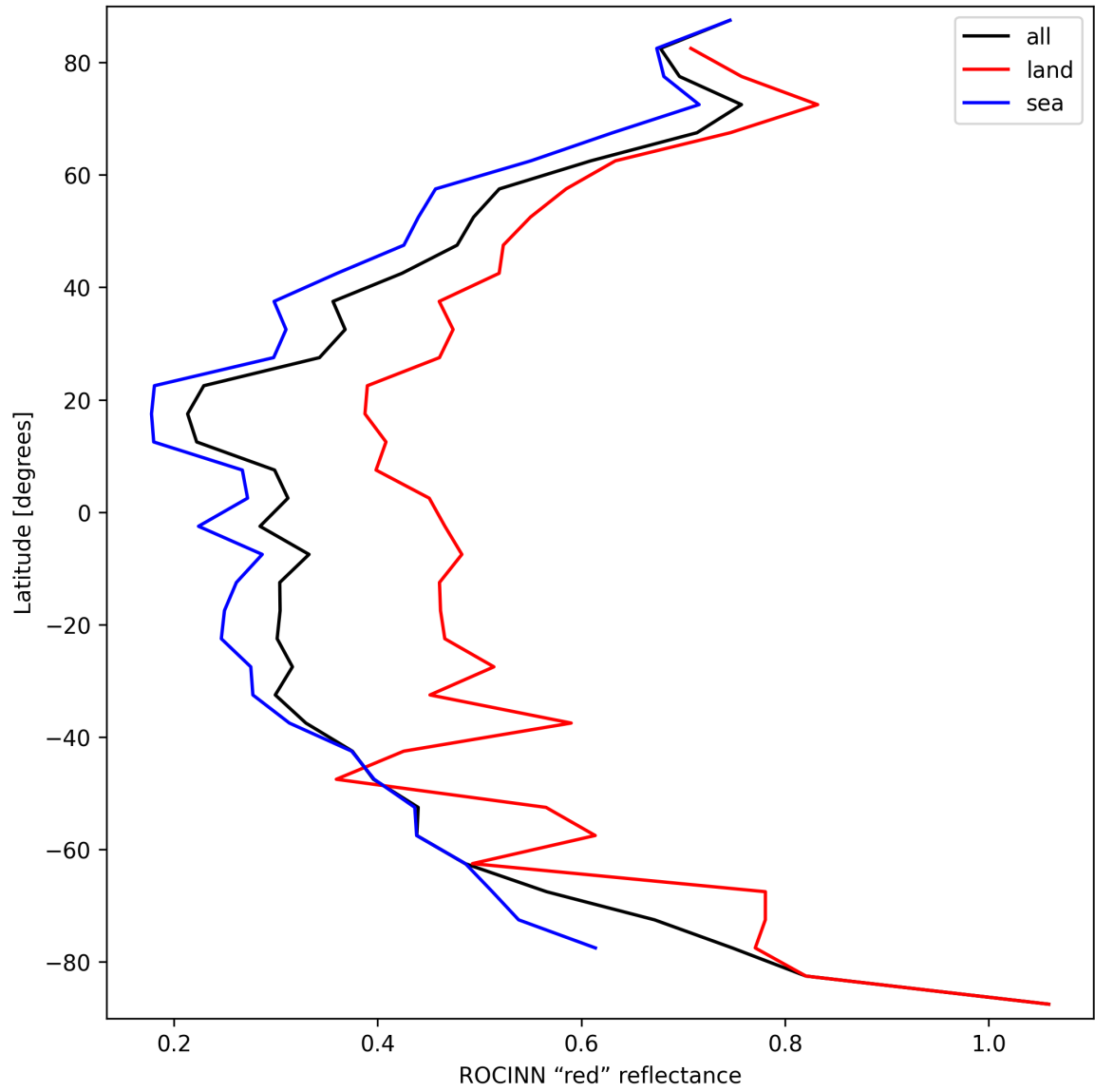
Figure 37: Zonal average of “ROCINN “red” reflectance” for 2025-03-23 to 2025-03-24.
