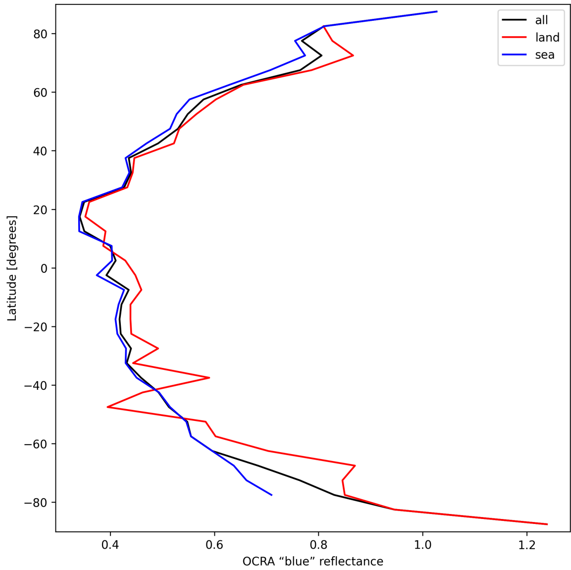
Figure 35: Zonal average of “OCRA “blue” reflectance” for 2025-03-23 to 2025-03-24.
