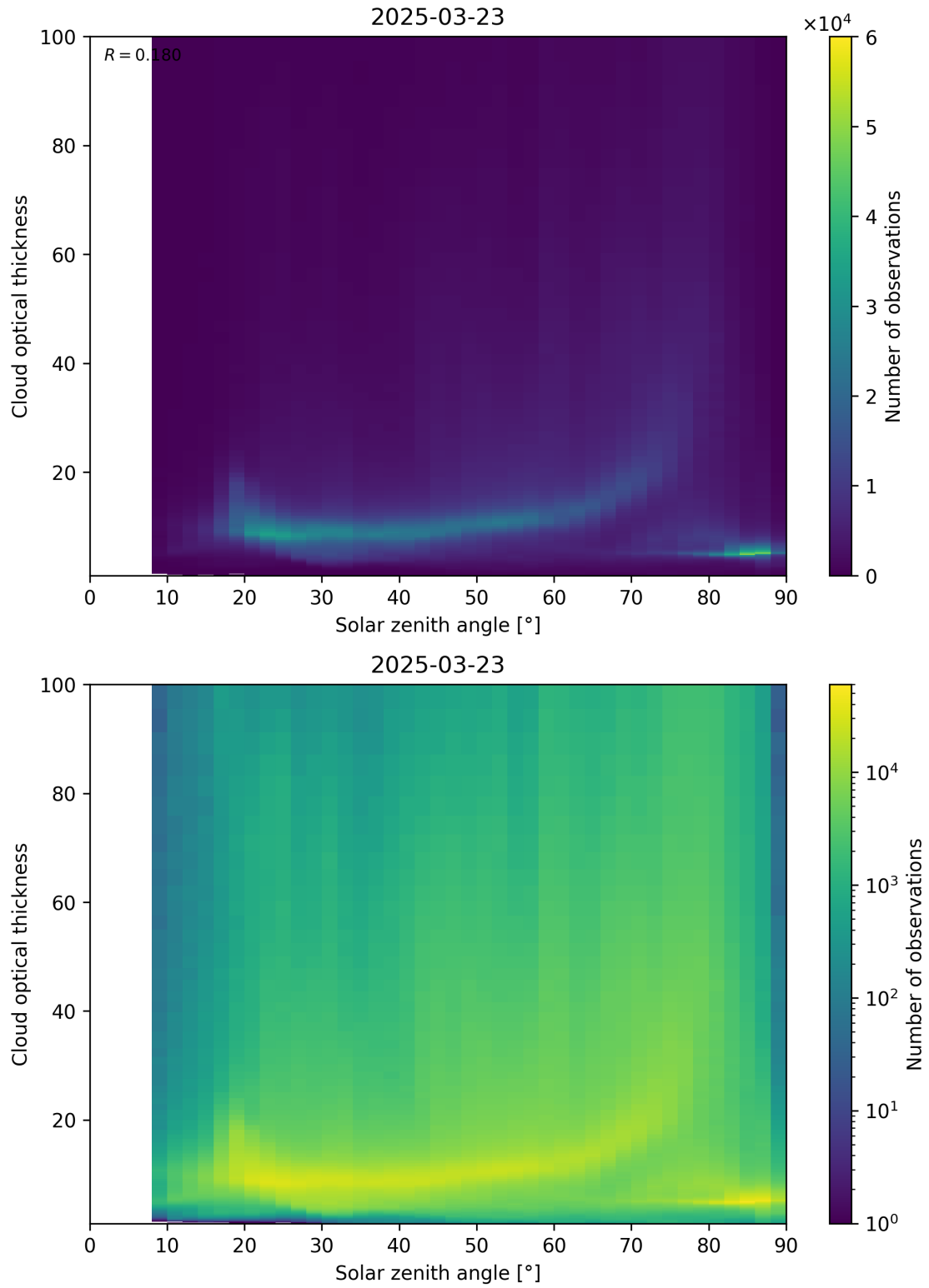
Figure 103: Scatter density plot of “Solar zenith angle” against “Cloud optical thickness” for 2025-03-23 to 2025-03-24.
