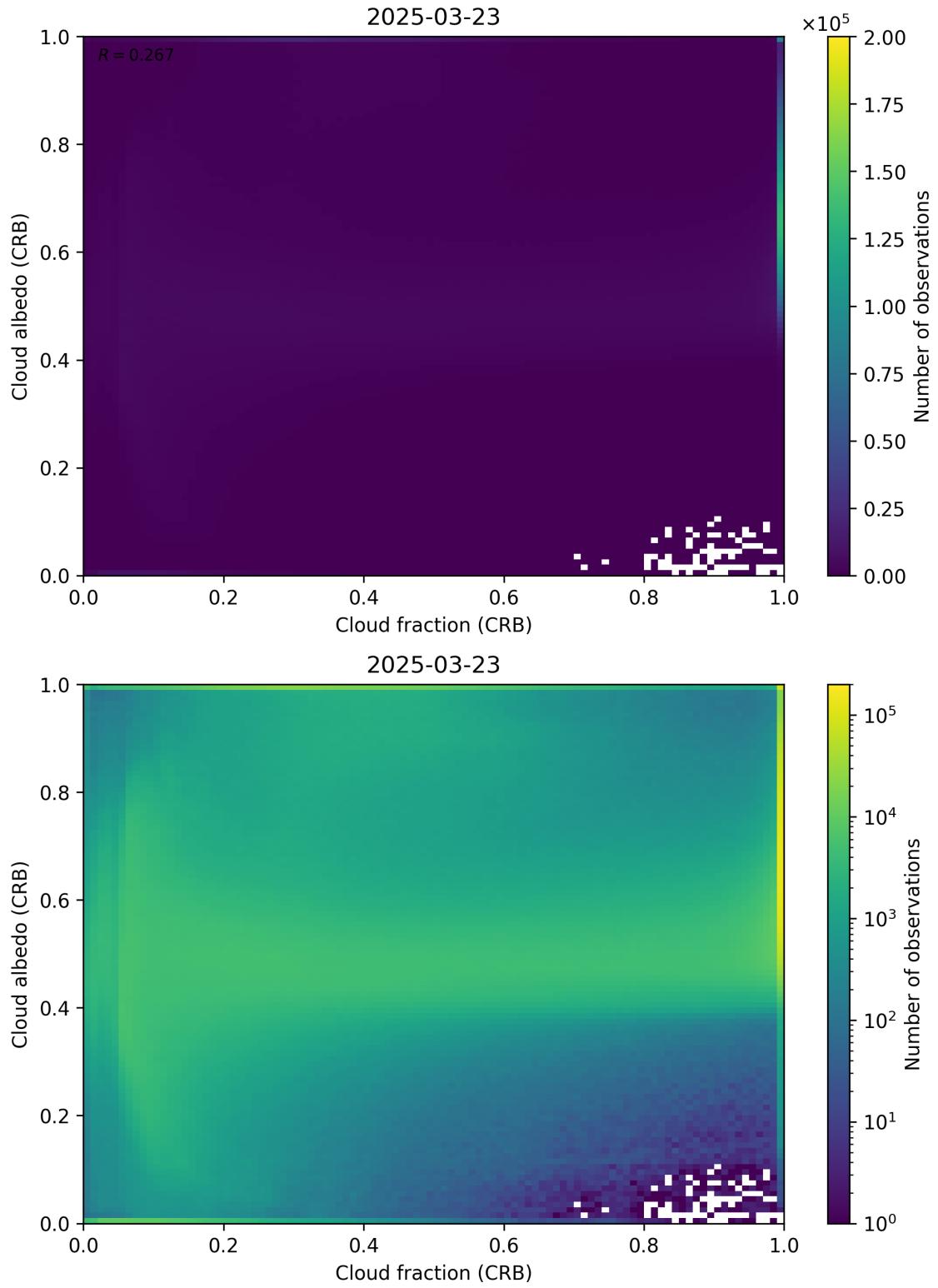
Figure 77: Scatter density plot of “Cloud fraction (CRB)” against “Cloud albedo (CRB)” for 2025-03-23 to 2025-03-24.
