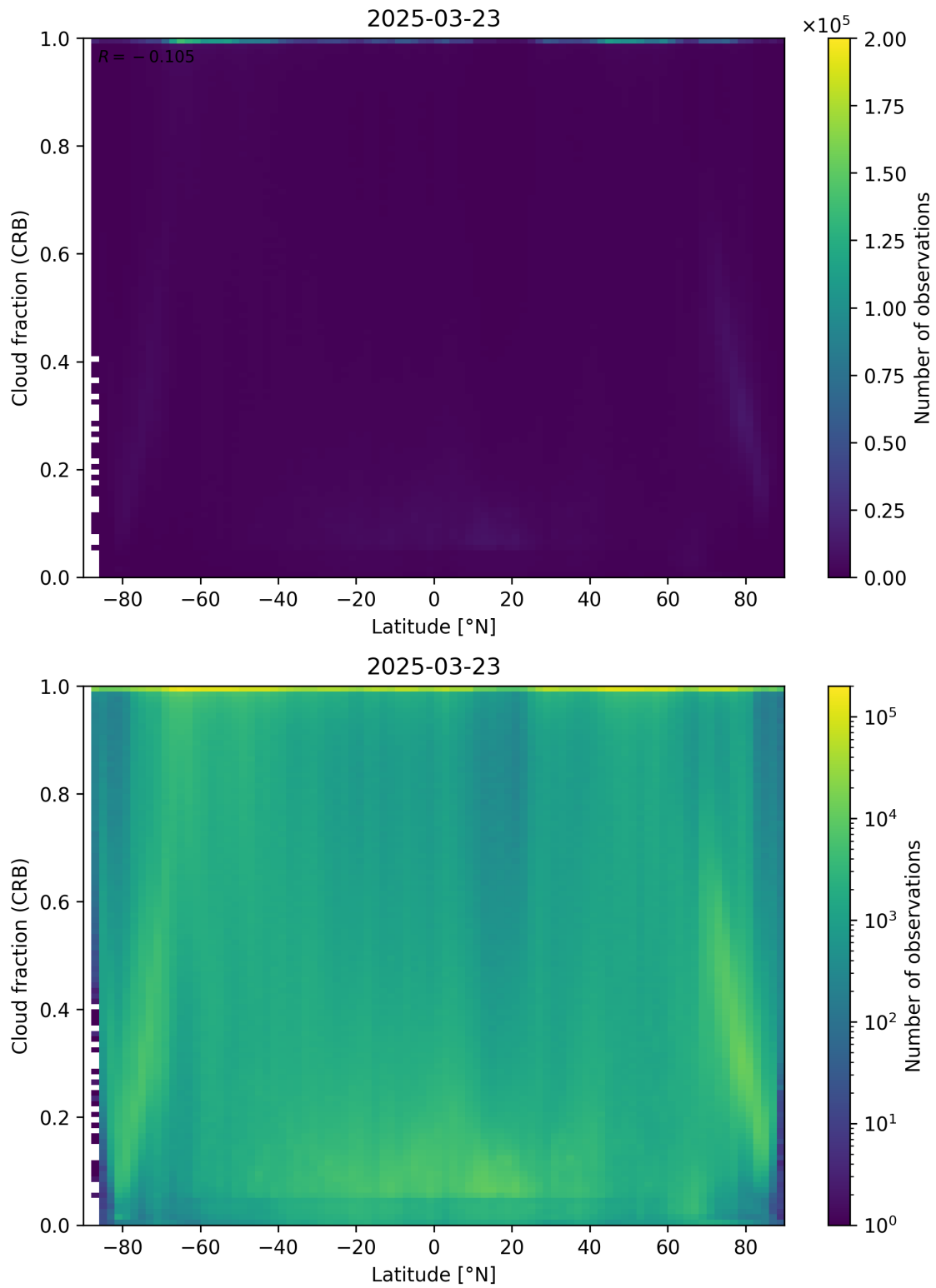
Figure 94: Scatter density plot of “Latitude” against “Cloud fraction (CRB)” for 2025-03-23 to 2025-03-24.
