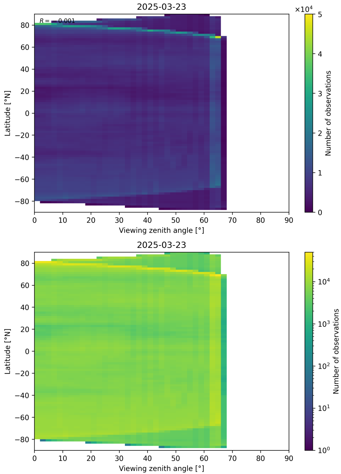
Figure 113: Scatter density plot of “Viewing zenith angle” against “Latitude” for 2025-03-23 to 2025-03-24.
