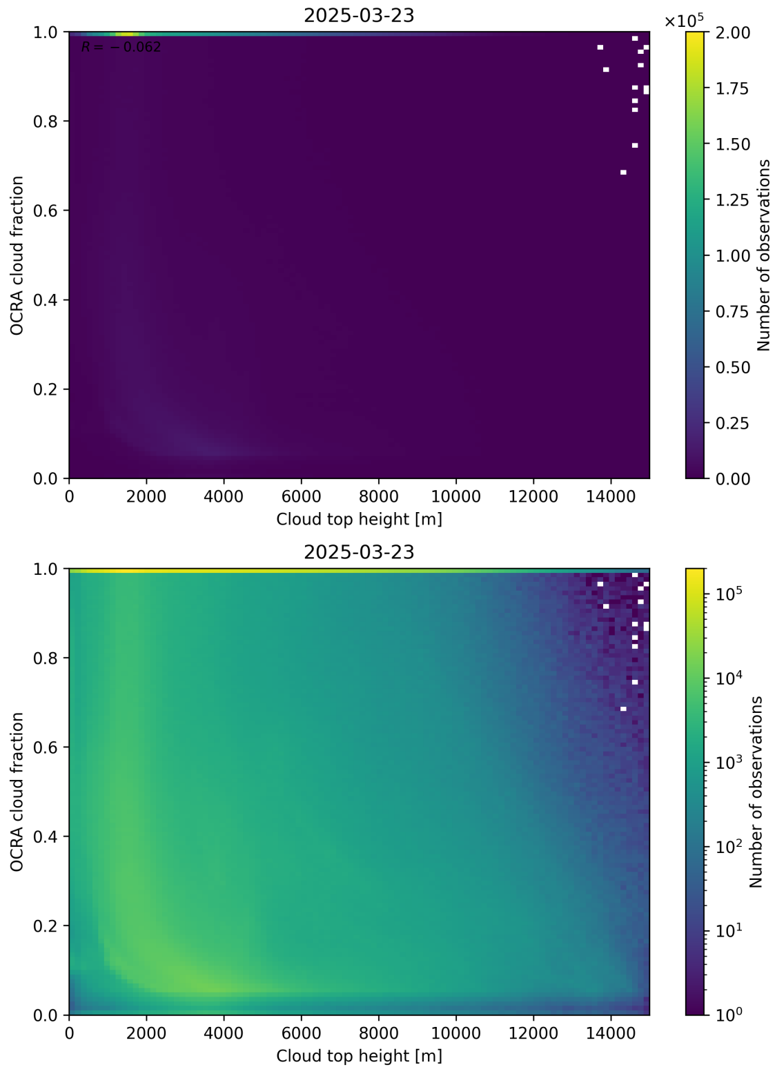
Figure 87: Scatter density plot of “Cloud top height” against “OCRA cloud fraction” for 2025-03-23 to 2025-03-24.
