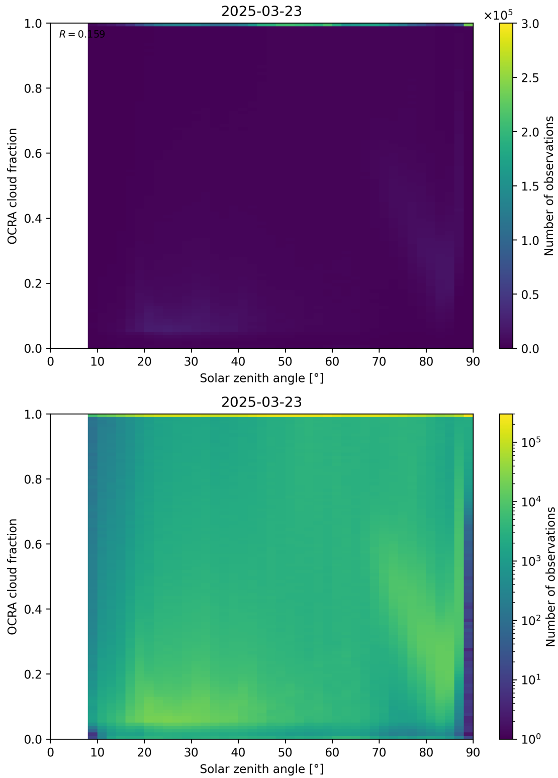
Figure 100: Scatter density plot of “Solar zenith angle” against “OCRA cloud fraction” for 2025-03-23 to 2025-03-24.
