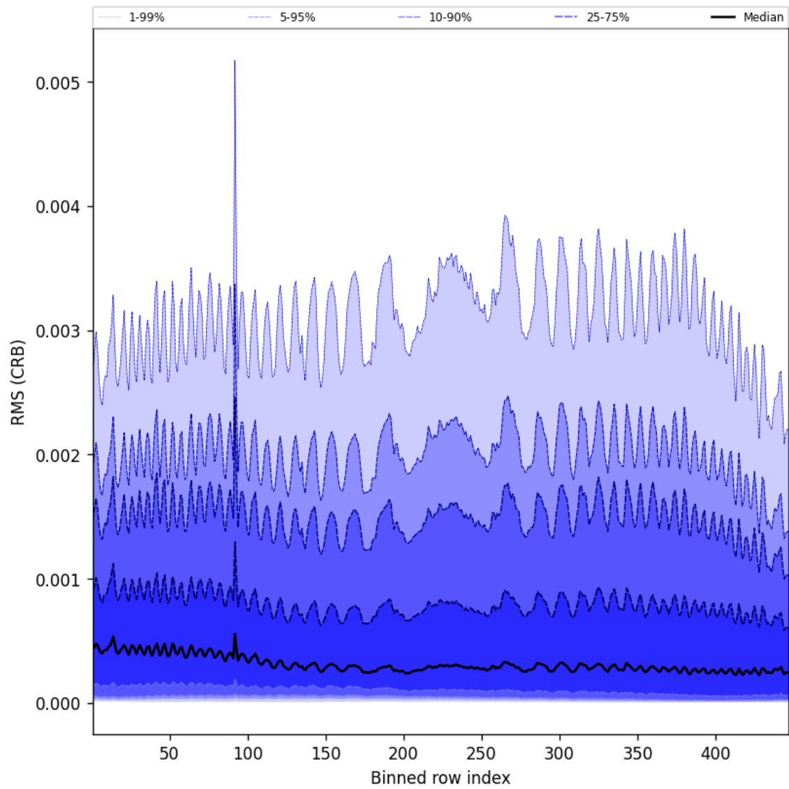
Figure 64: Along track statistics of “RMS (CRB)” for 2025-03-23 to 2025-03-24
