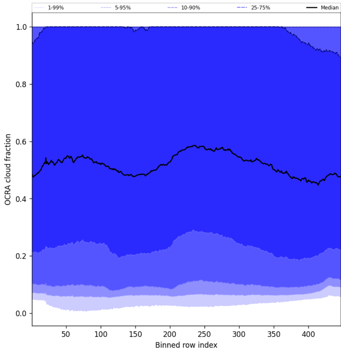
Figure 66: Along track statistics of “OCRA cloud fraction” for 2025-03-23 to 2025-03-24
