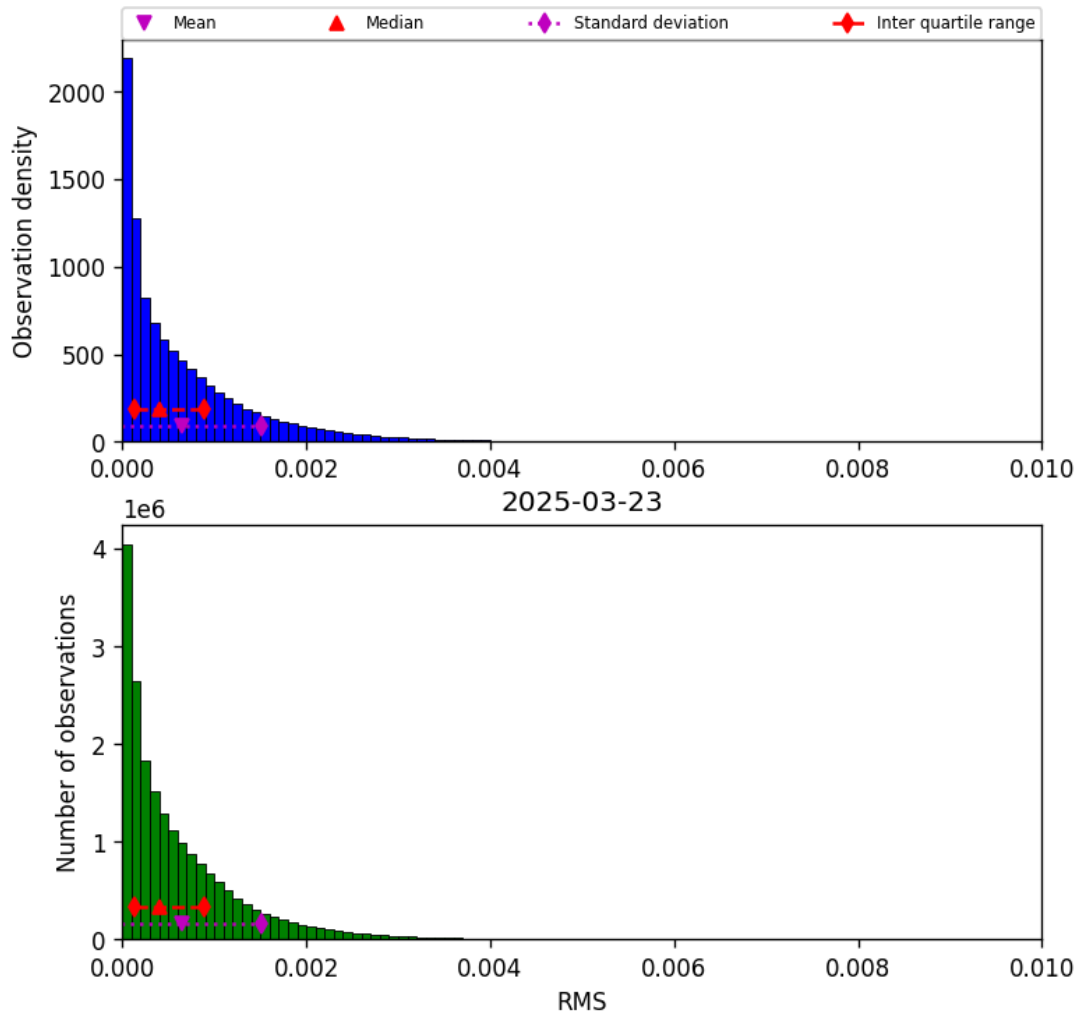
Figure 47: Histogram of “RMS” for 2025-03-23 to 2025-03-24
