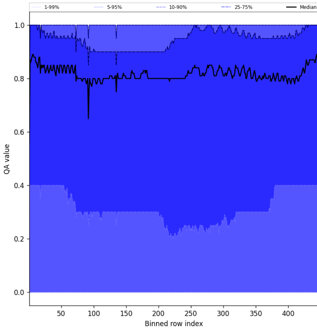
Figure 54: Along track statistics of “QA value” for 2025-03-23 to 2025-03-24
