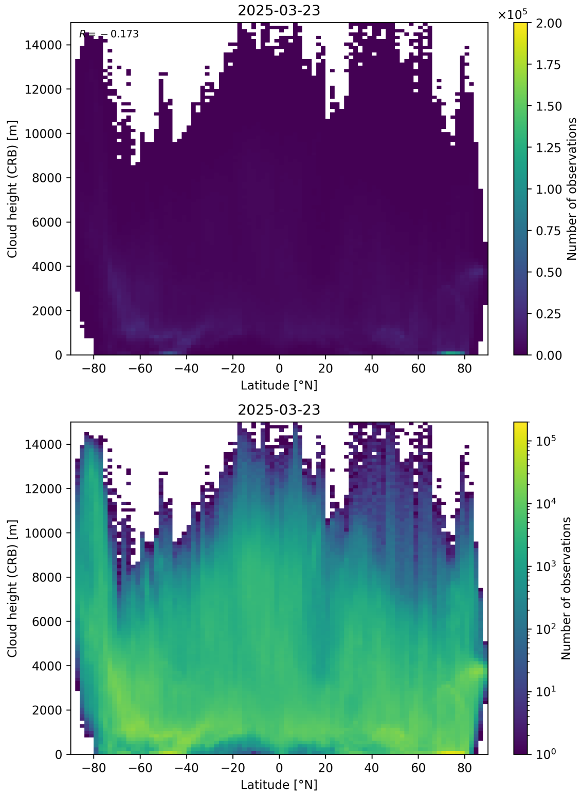
Figure 95: Scatter density plot of “Latitude” against “Cloud height (CRB)” for 2025-03-23 to 2025-03-24.
