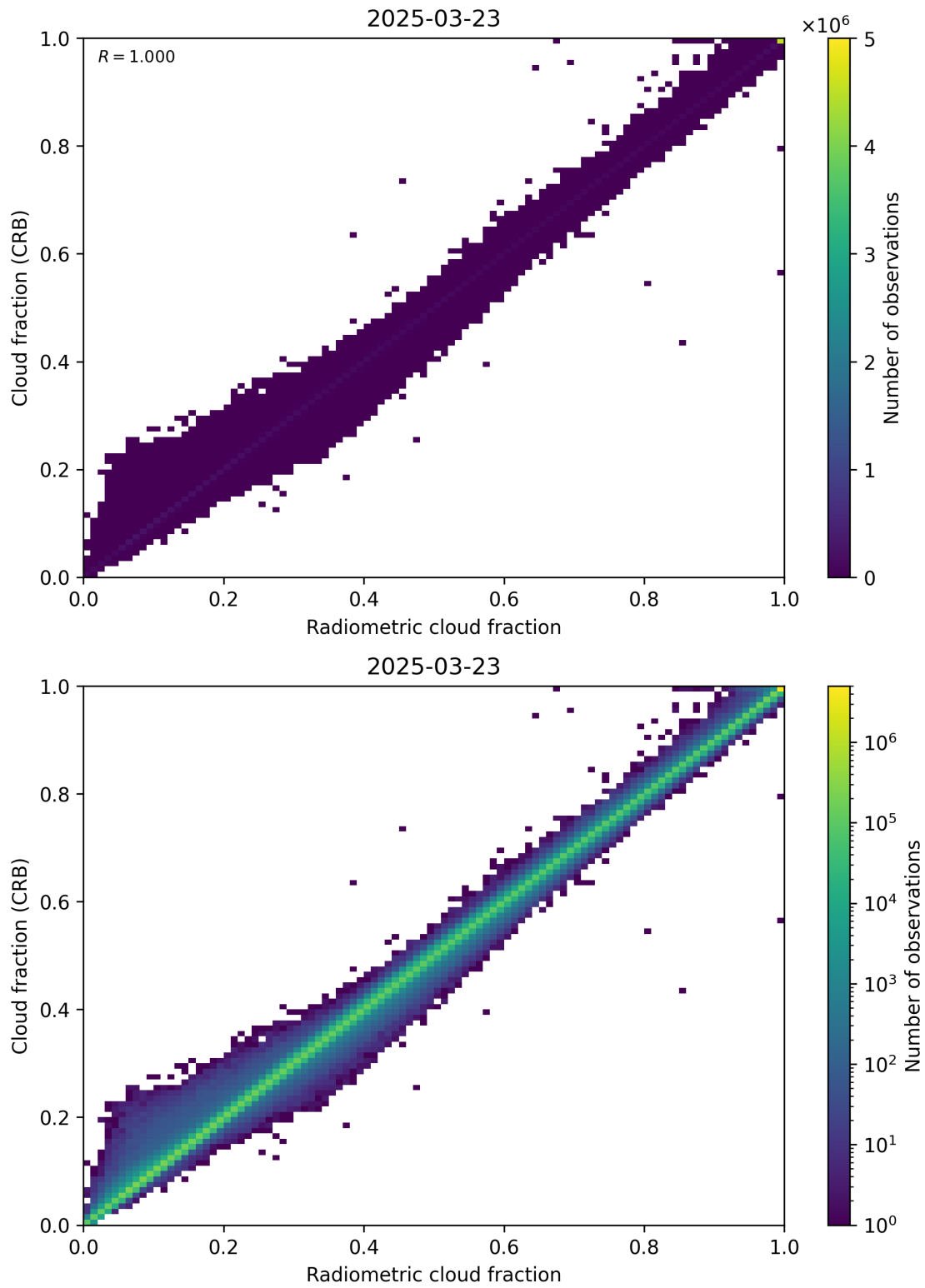
Figure 73: Scatter density plot of “Radiometric cloud fraction” against “Cloud fraction (CRB)” for 2025-03-23 to 2025-03-24.
