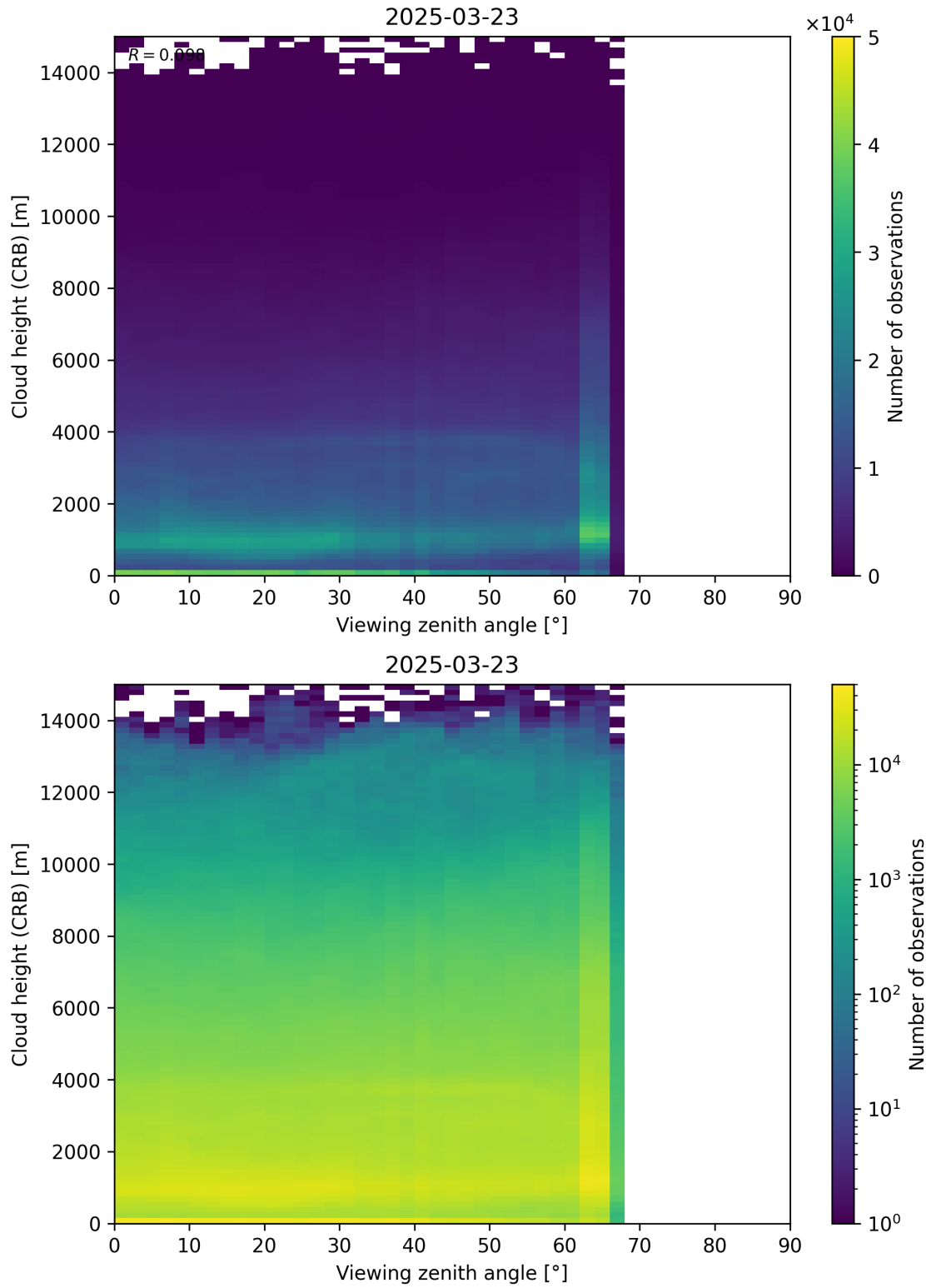
Figure 110: Scatter density plot of “Viewing zenith angle” against “Cloud height (CRB)” for 2025-03-23 to 2025-03-24.
