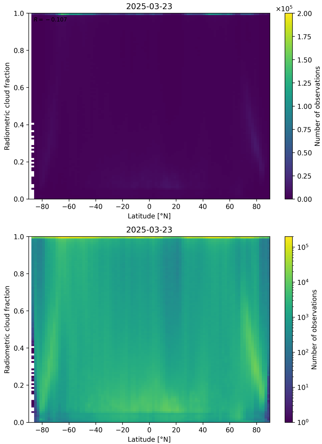
Figure 92: Scatter density plot of “Latitude” against “Radiometric cloud fraction” for 2025-03-23 to 2025-03-24.
