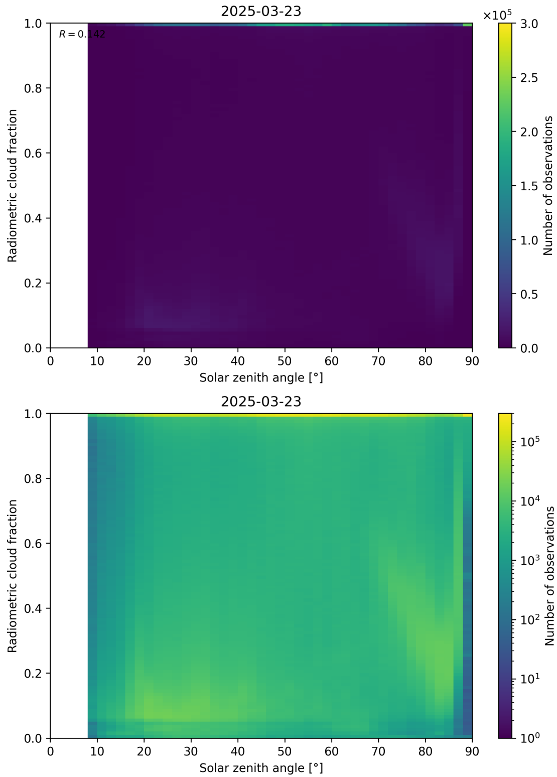
Figure 99: Scatter density plot of “Solar zenith angle” against “Radiometric cloud fraction” for 2025-03-23 to 2025-03-24.
