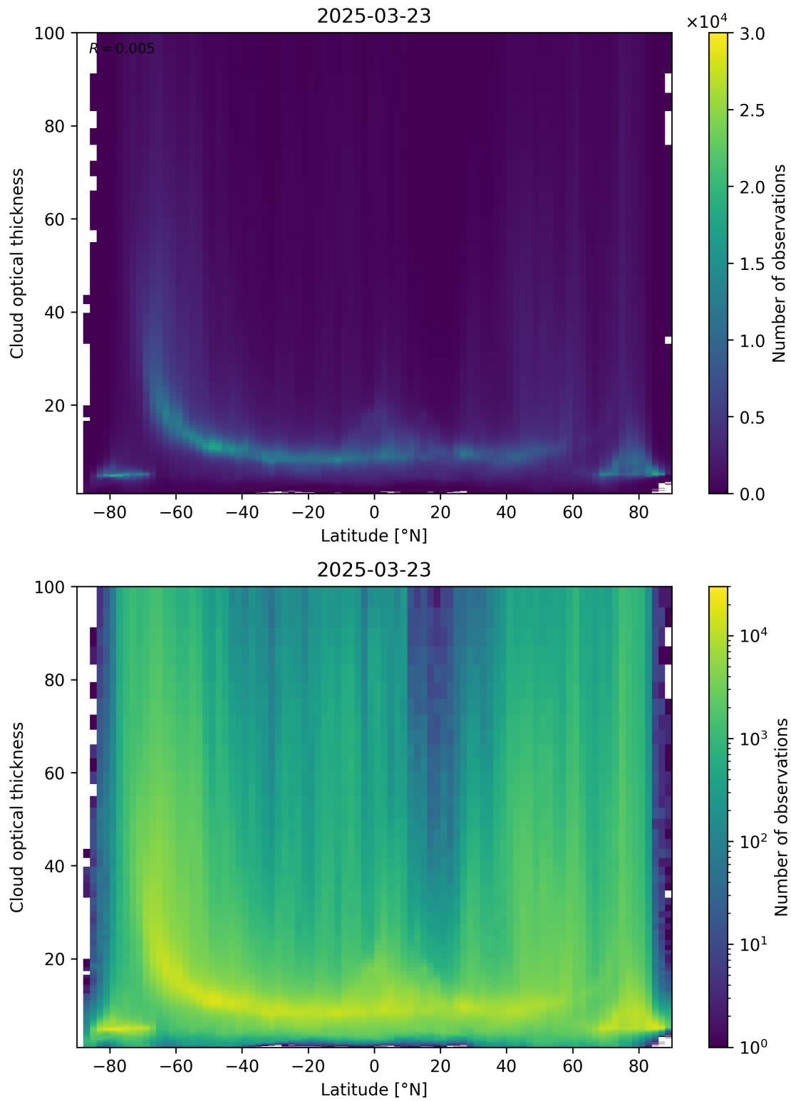
Figure 96: Scatter density plot of “Latitude” against “Cloud optical thickness” for 2025-03-23 to 2025-03-24.
