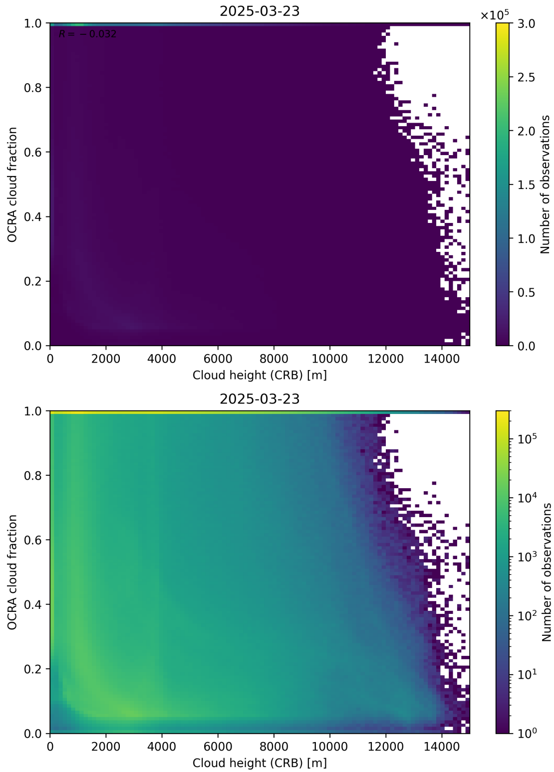
Figure 81: Scatter density plot of “Cloud height (CRB)” against “OCRA cloud fraction” for 2025-03-23 to 2025-03-24.
