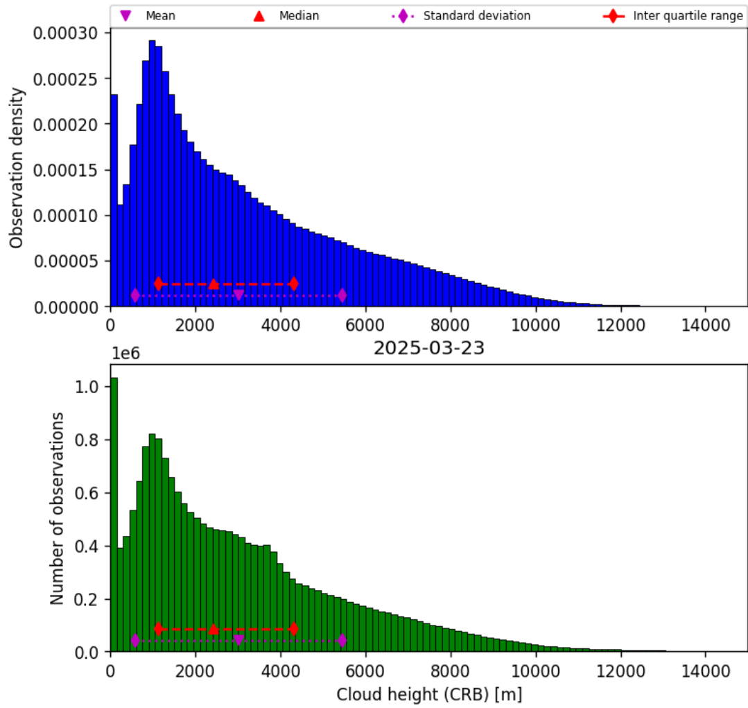
Figure 43: Histogram of “Cloud height (CRB)” for 2025-03-23 to 2025-03-24
