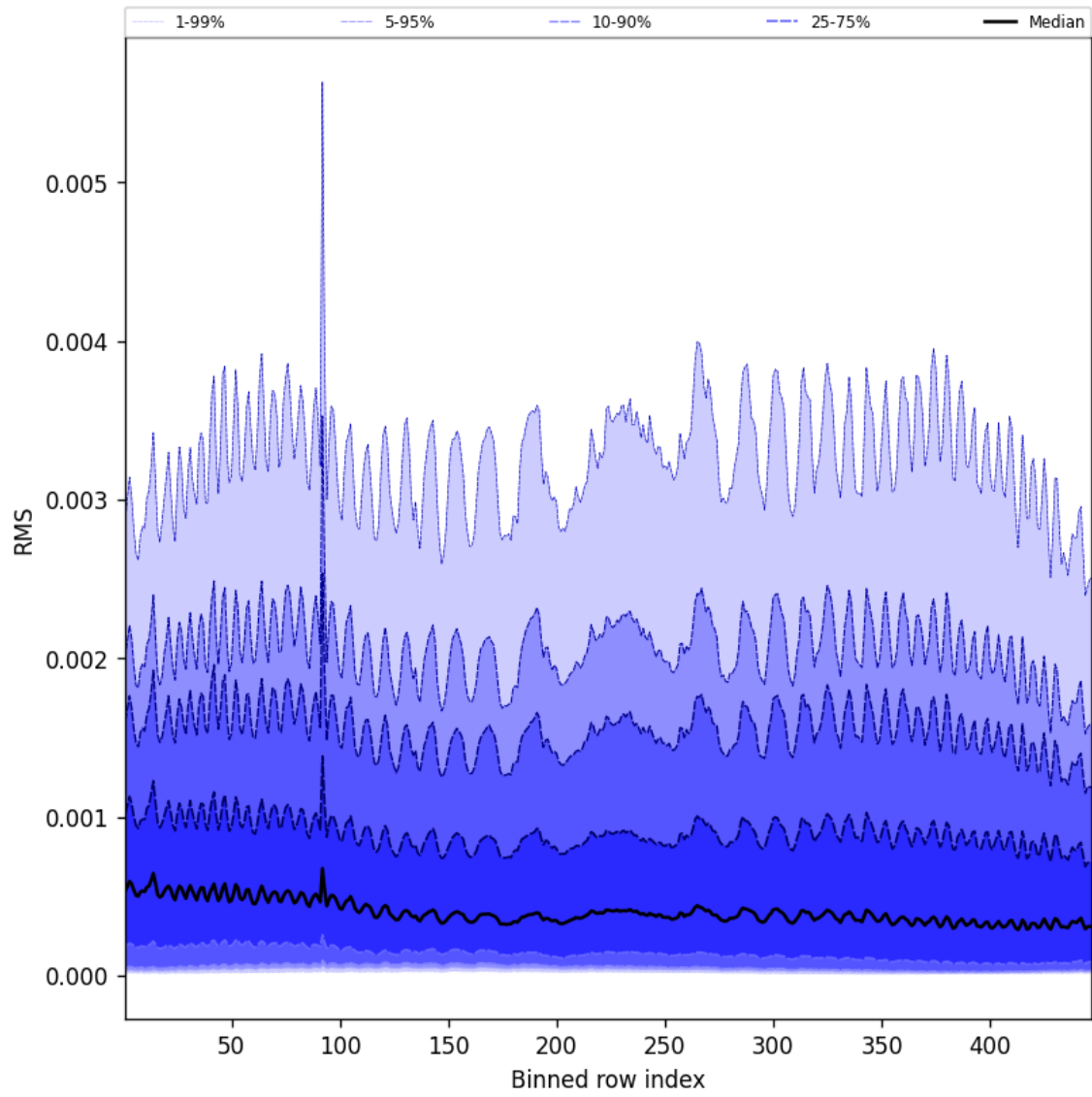
Figure 63: Along track statistics of “RMS” for 2025-03-23 to 2025-03-24
