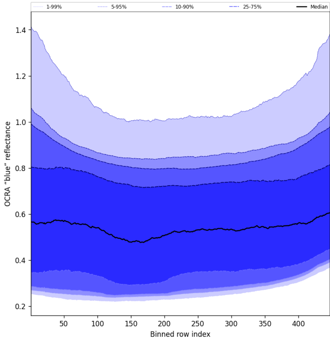
Figure 67: Along track statistics of “OCRA “blue” reflectance” for 2025-03-23 to 2025-03-24
