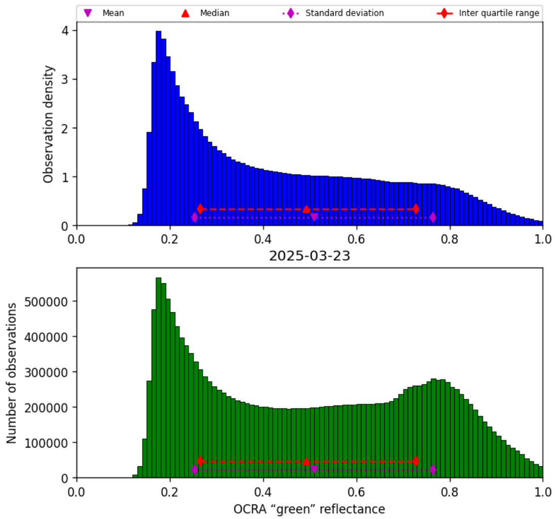
Figure 52: Histogram of “OCRA “green” reflectance” for 2025-03-23 to 2025-03-24
