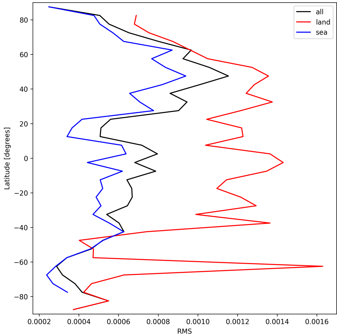
Figure 31: Zonal average of “RMS” for 2025-03-23 to 2025-03-24.
