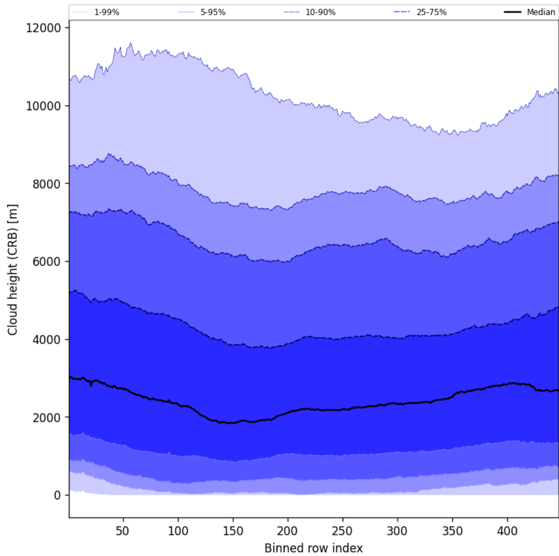
Figure 59: Along track statistics of “Cloud height (CRB)” for 2025-03-23 to 2025-03-24
