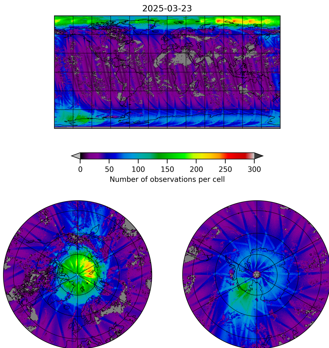
Figure 21: Map of the number of observations for 2025-03-23 to 2025-03-24
