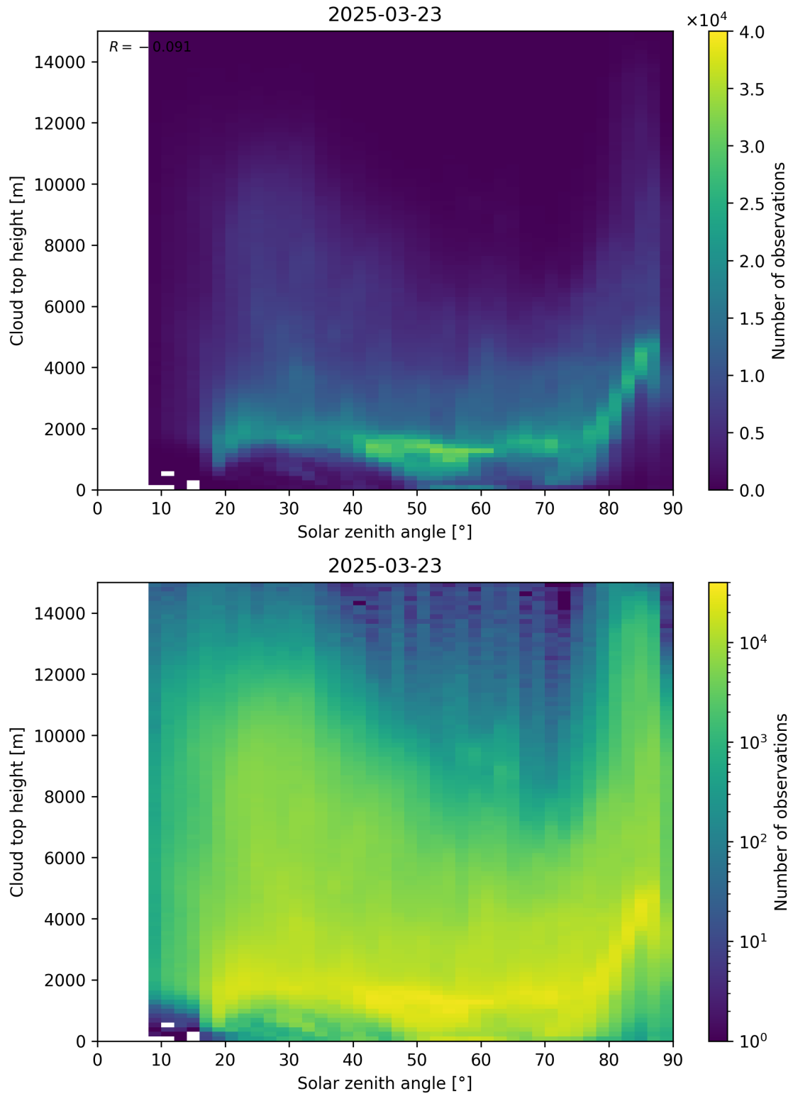
Figure 104: Scatter density plot of “Solar zenith angle” against “Cloud top height” for 2025-03-23 to 2025-03-24.
