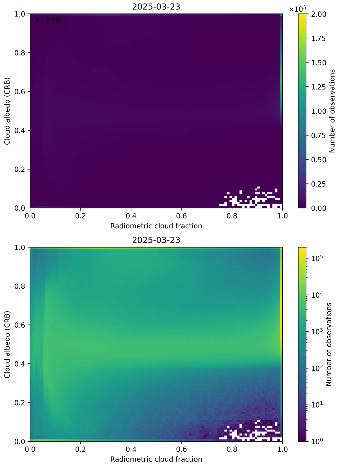
Figure 71: Scatter density plot of “Radiometric cloud fraction” against “Cloud albedo (CRB)” for 2025-03-23 to 2025-03-24.
