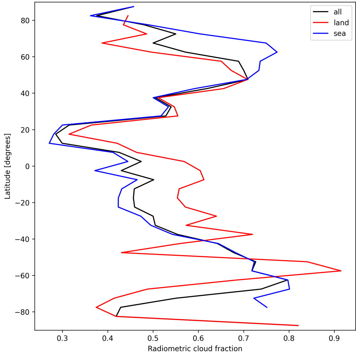
Figure 23: Zonal average of “Radiometric cloud fraction” for 2025-03-23 to 2025-03-24.
