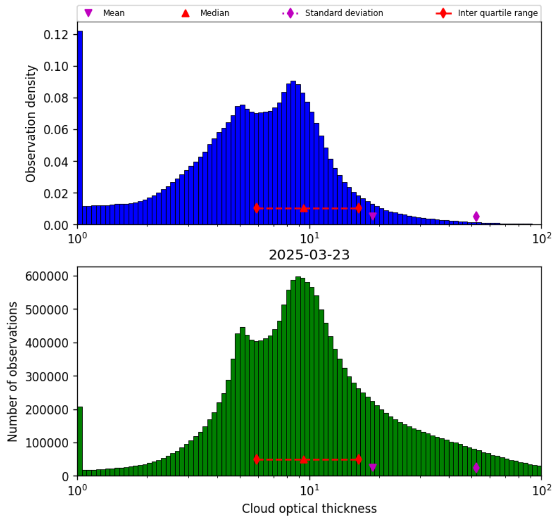
Figure 41: Histogram of “Cloud optical thickness” for 2025-03-23 to 2025-03-24
