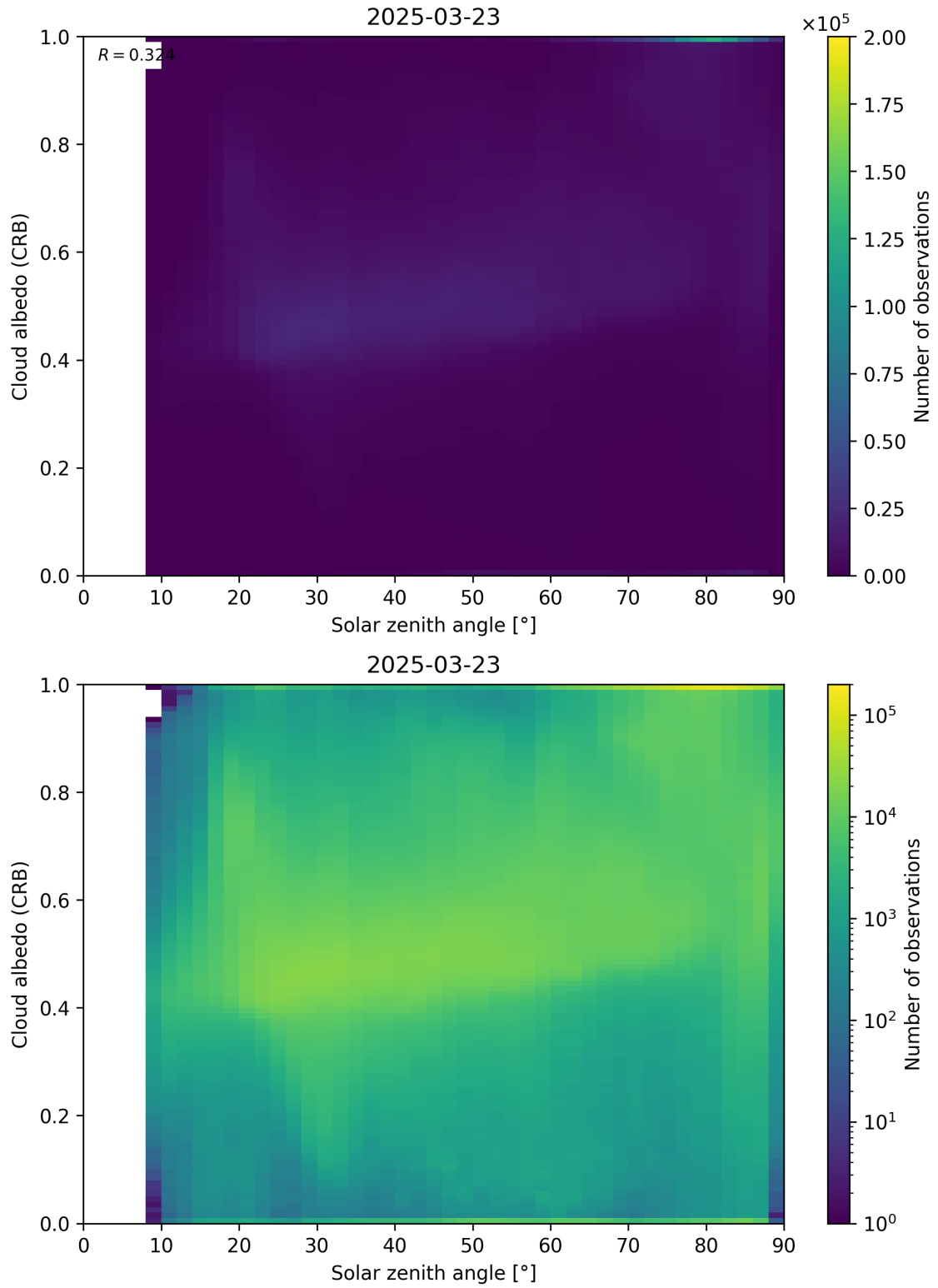
Figure 98: Scatter density plot of “Solar zenith angle” against “Cloud albedo (CRB)” for 2025-03-23 to 2025-03-24.
