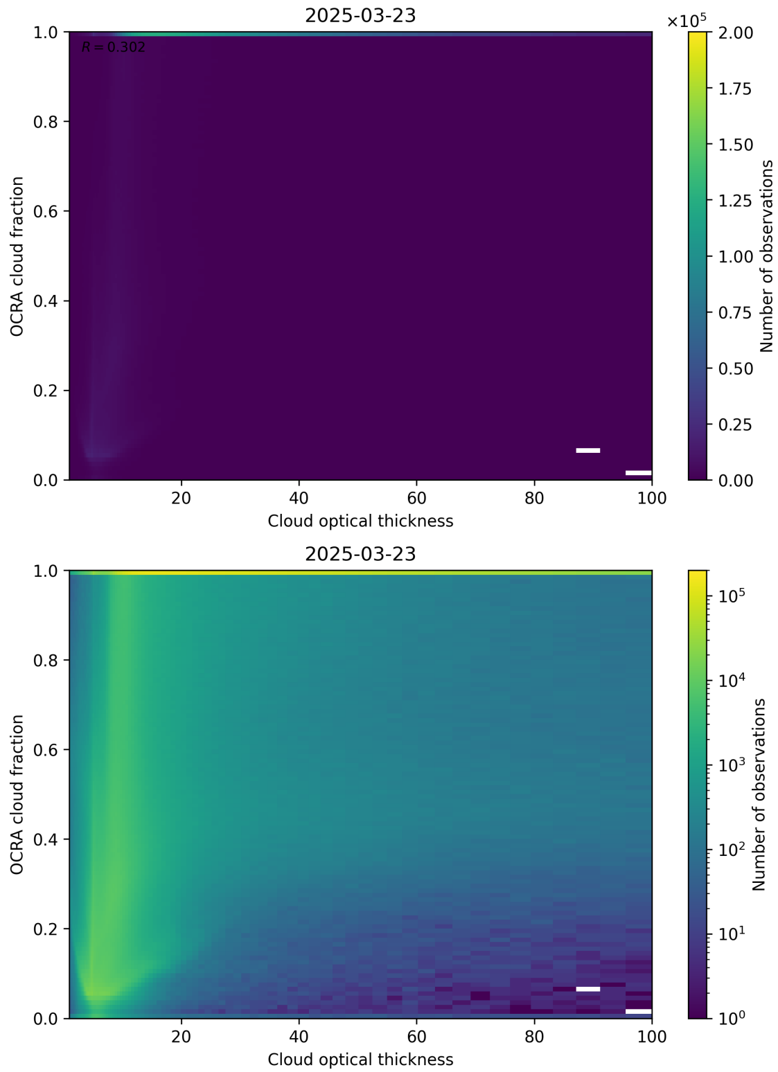
Figure 83: Scatter density plot of “Cloud optical thickness” against “OCRA cloud fraction” for 2025-03-23 to 2025-03-24.
