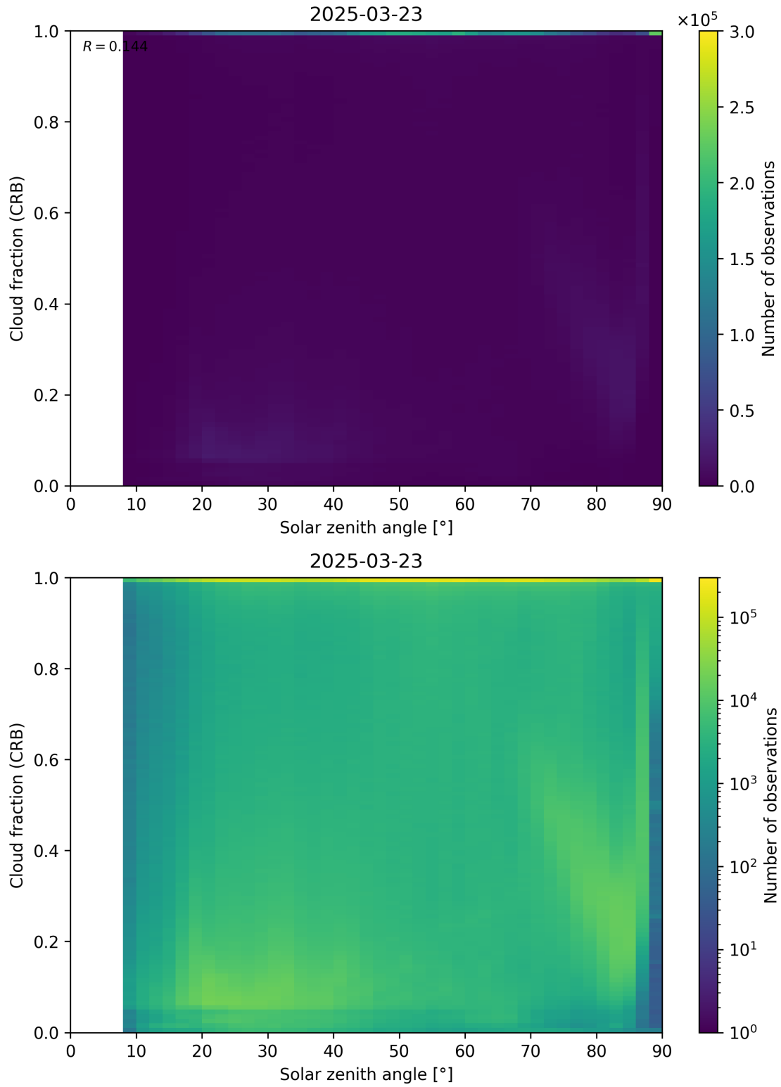
Figure 101: Scatter density plot of “Solar zenith angle” against “Cloud fraction (CRB)” for 2025-03-23 to 2025-03-24.
