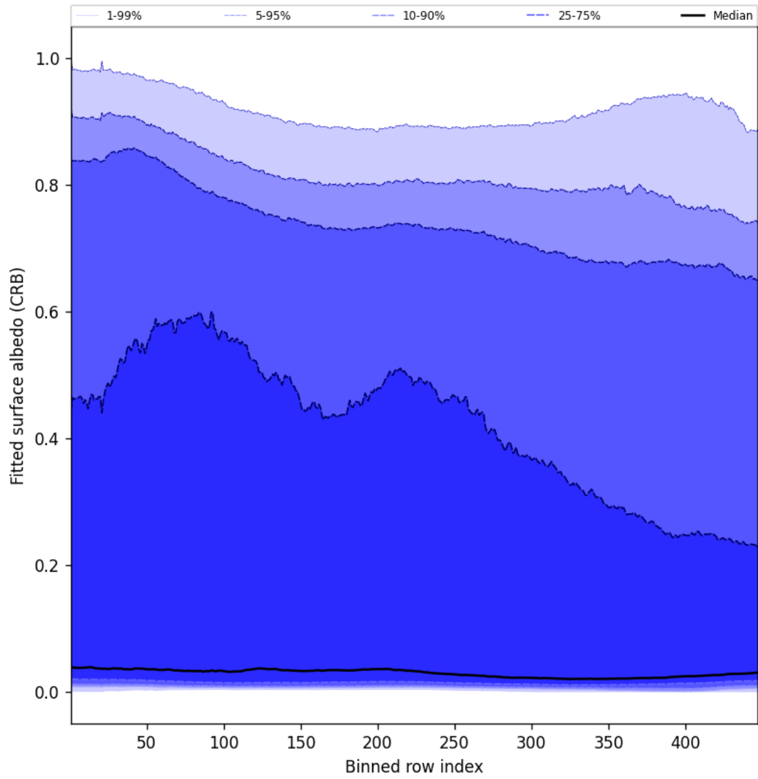
Figure 62: Along track statistics of “Fitted surface albedo (CRB)” for 2025-03-23 to 2025-03-24
