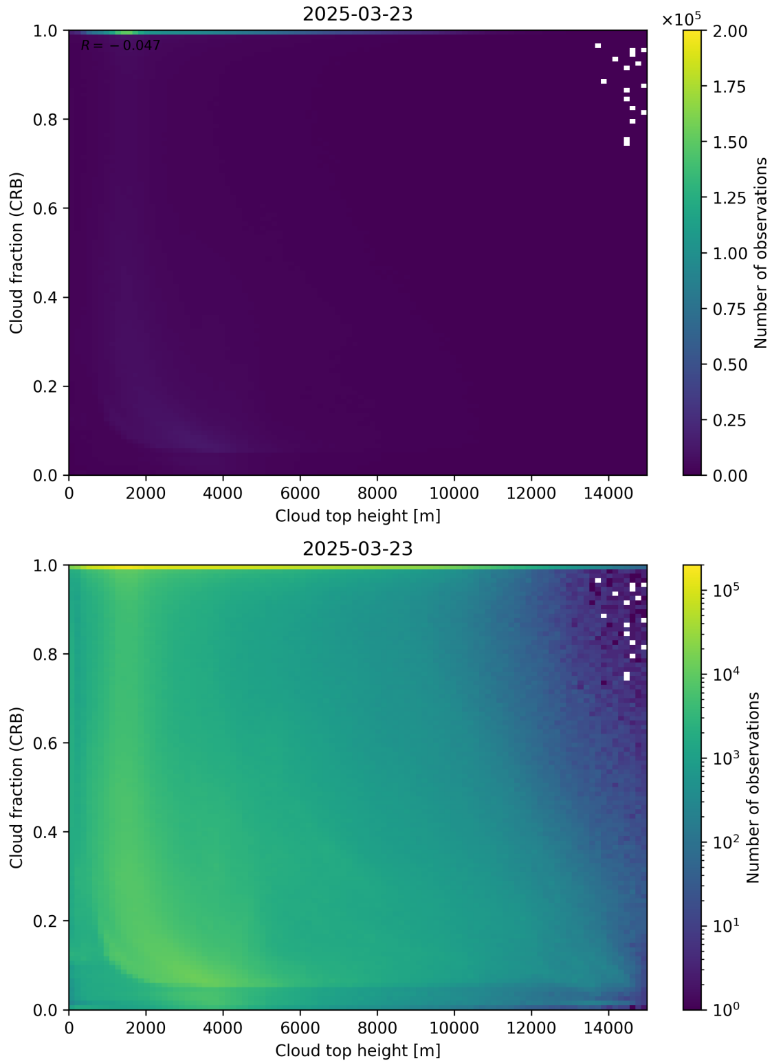
Figure 88: Scatter density plot of “Cloud top height” against “Cloud fraction (CRB)” for 2025-03-23 to 2025-03-24.
