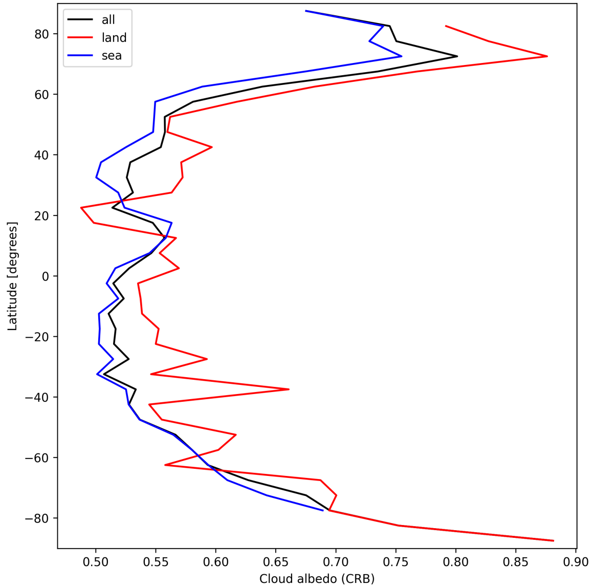
Figure 28: Zonal average of “Cloud albedo (CRB)” for 2025-03-23 to 2025-03-24.
