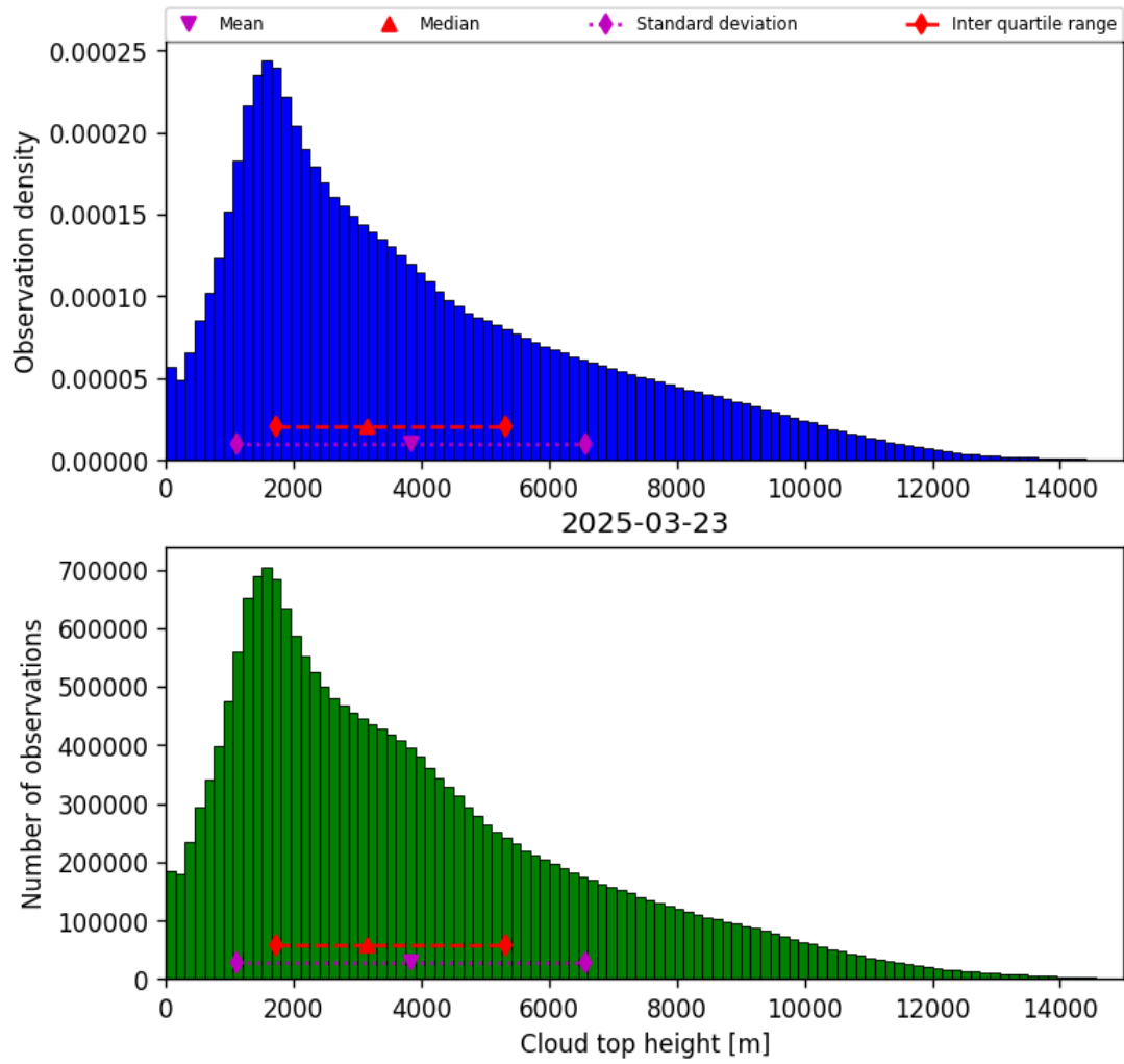
Figure 40: Histogram of “Cloud top height” for 2025-03-23 to 2025-03-24
