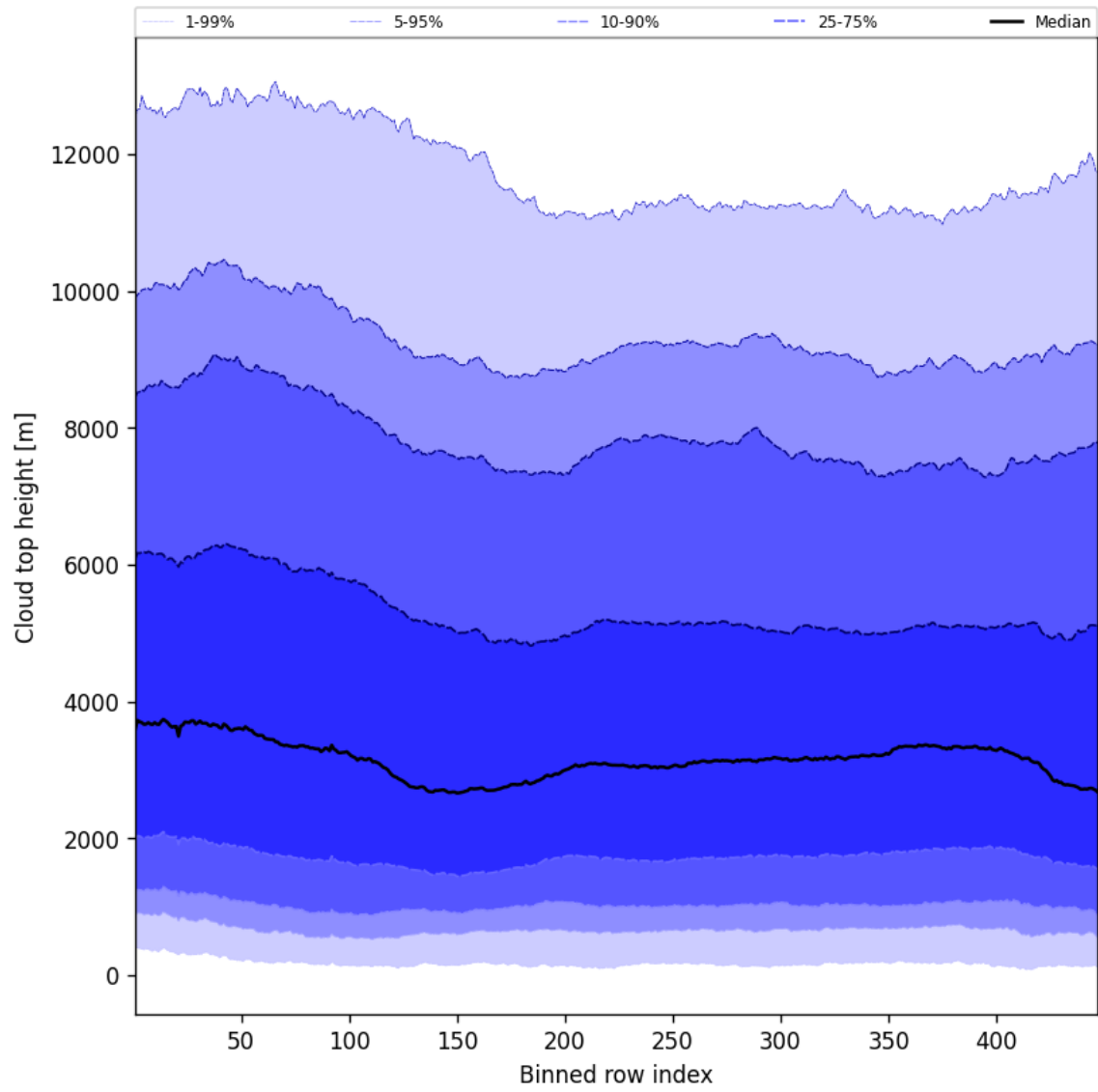
Figure 56: Along track statistics of “Cloud top height” for 2025-03-23 to 2025-03-24
