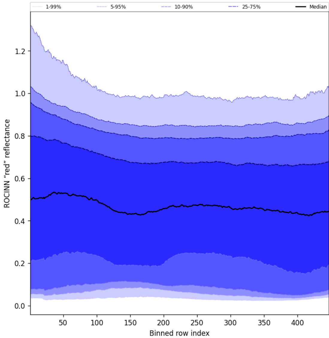
Figure 69: Along track statistics of "ROCINN "red" reflectance" for 2025-03-23 to 2025-03-24
