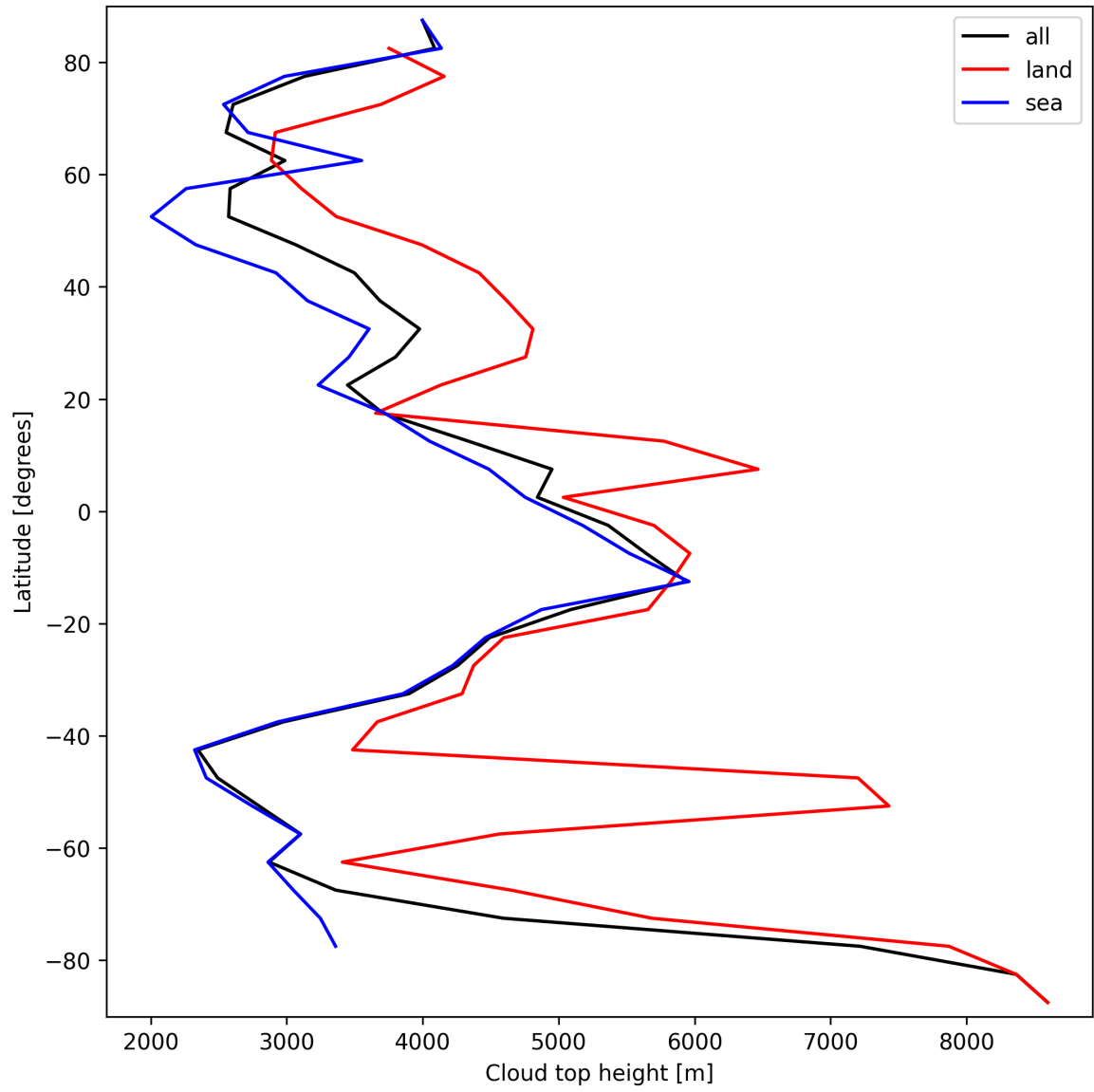
Figure 24: Zonal average of “Cloud top height” for 2025-03-23 to 2025-03-24.
