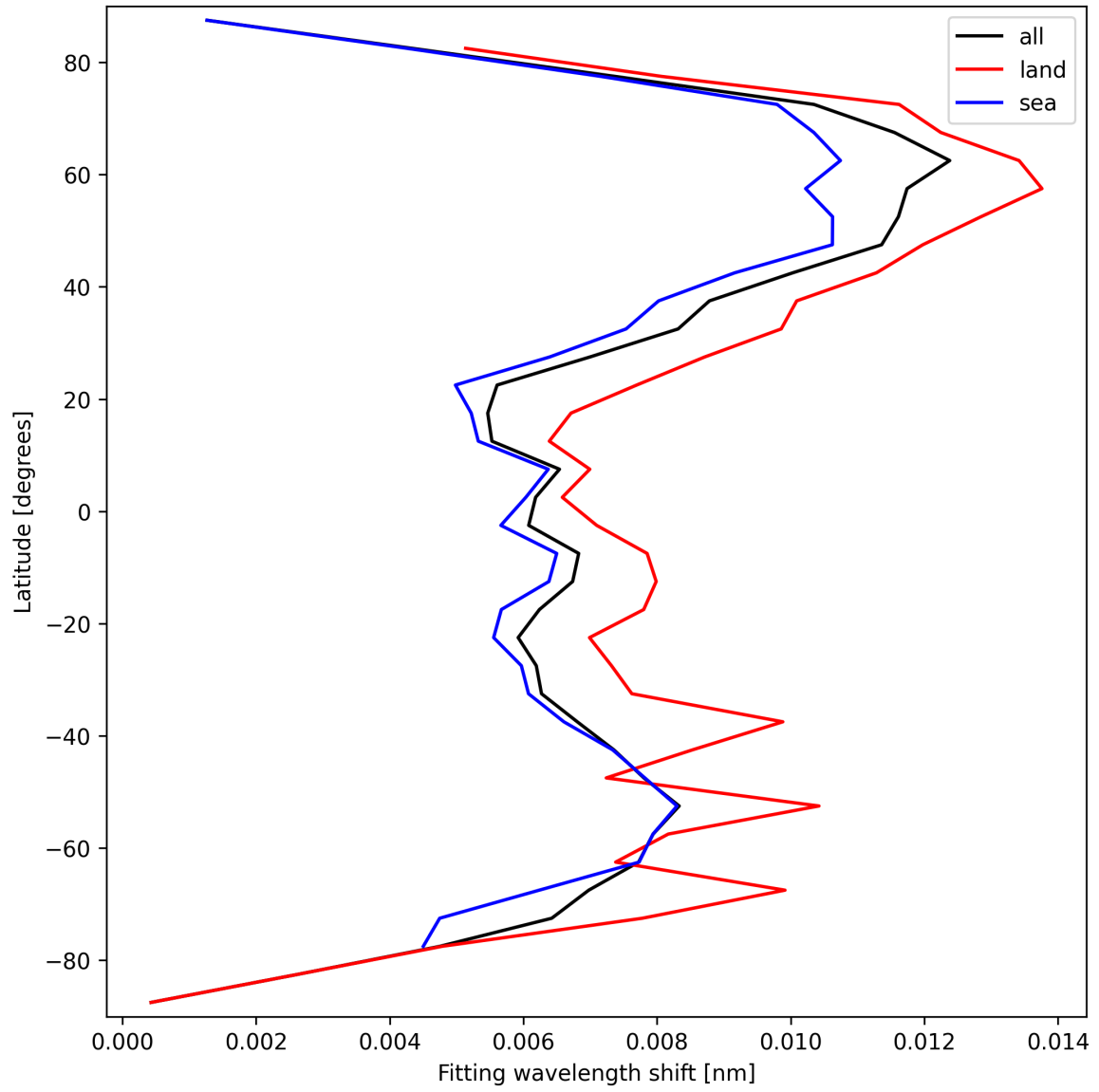
Figure 33: Zonal average of “Fitting wavelength shift” for 2025-03-23 to 2025-03-24.
