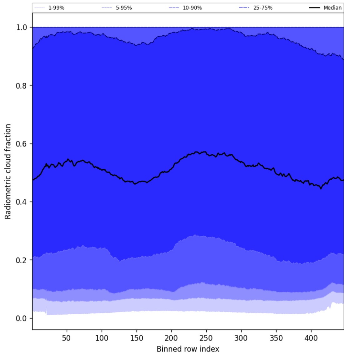
Figure 55: Along track statistics of “Radiometric cloud fraction” for 2025-03-23 to 2025-03-24
