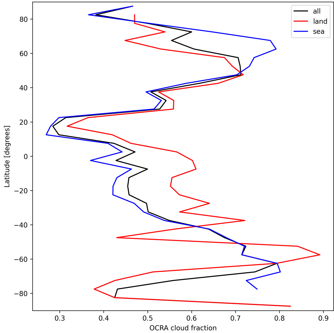
Figure 34: Zonal average of “OCRA cloud fraction” for 2025-03-23 to 2025-03-24.
