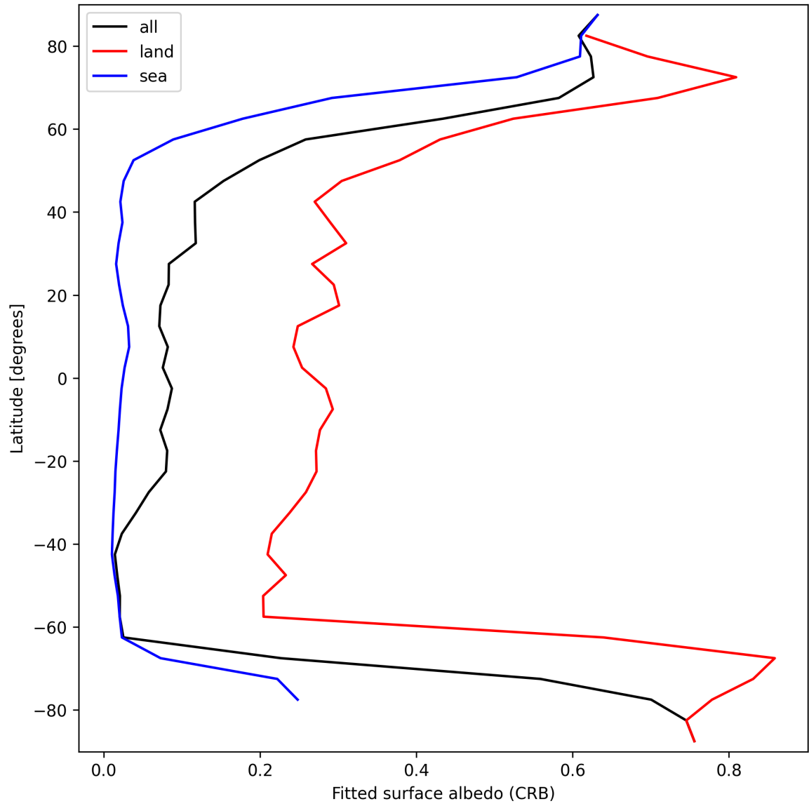
Figure 30: Zonal average of “Fitted surface albedo (CRB)” for 2025-03-23 to 2025-03-24.
