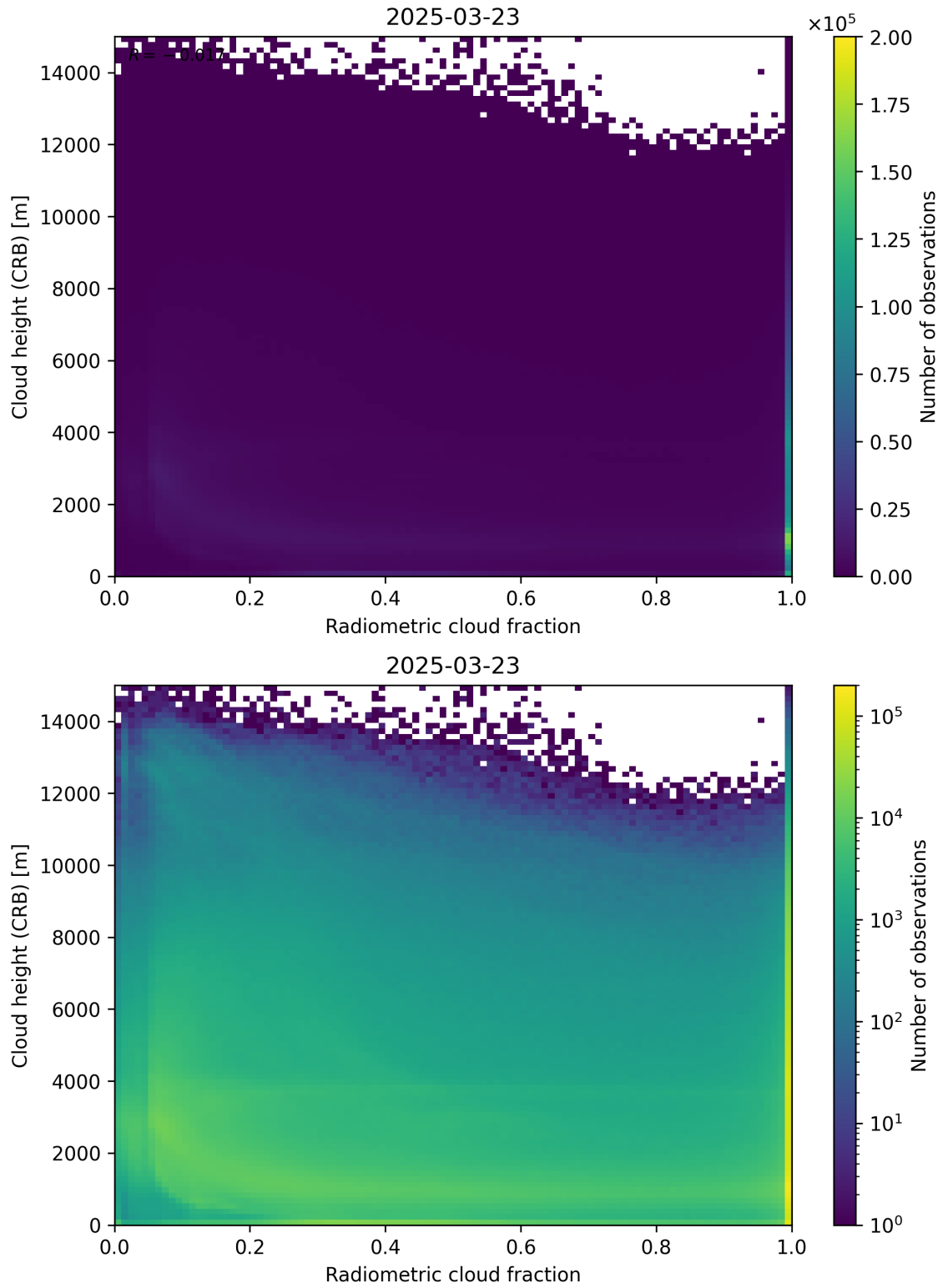
Figure 74: Scatter density plot of “Radiometric cloud fraction” against “Cloud height (CRB)” for 2025-03-23 to 2025-03-24.
