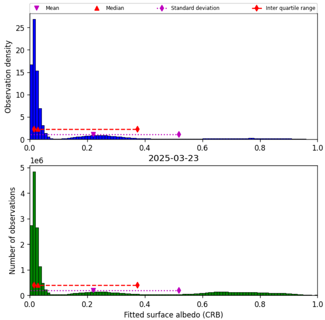
Figure 46: Histogram of “Fitted surface albedo (CRB)” for 2025-03-23 to 2025-03-24
