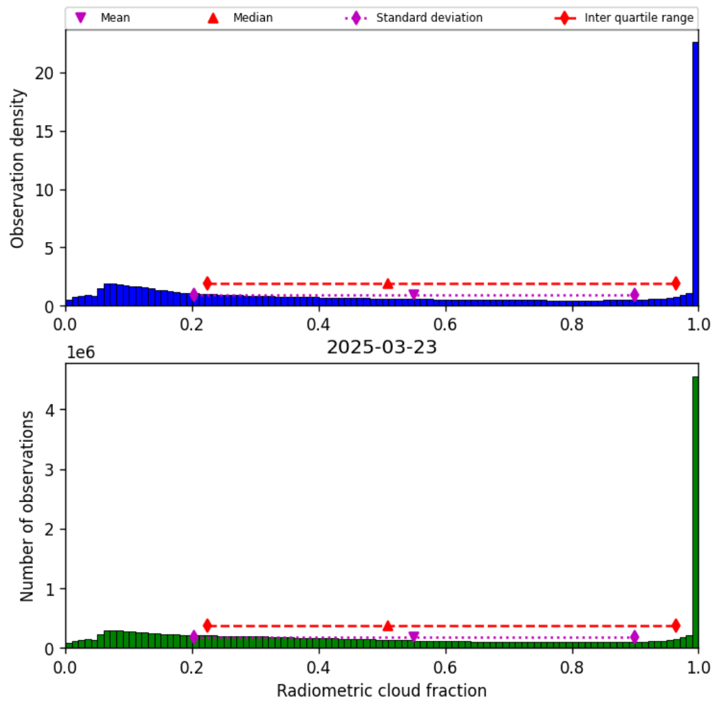
Figure 39: Histogram of “Radiometric cloud fraction” for 2025-03-23 to 2025-03-24
