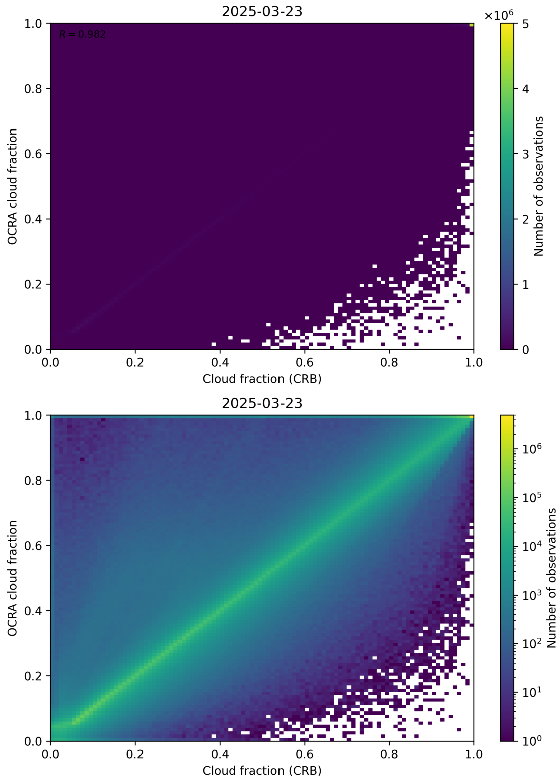
Figure 78: Scatter density plot of “Cloud fraction (CRB)” against “OCRA cloud fraction” for 2025-03-23 to 2025-03-24.
