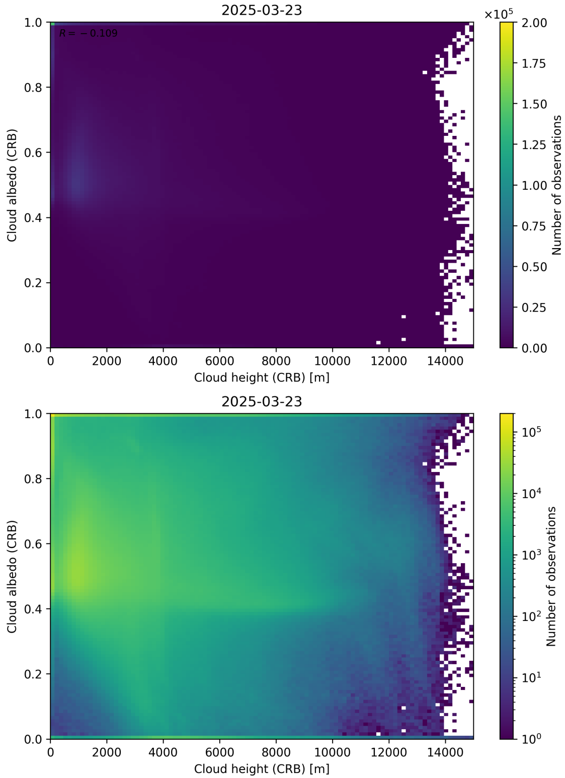
Figure 80: Scatter density plot of “Cloud height (CRB)” against “Cloud albedo (CRB)” for 2025-03-23 to 2025-03-24.
