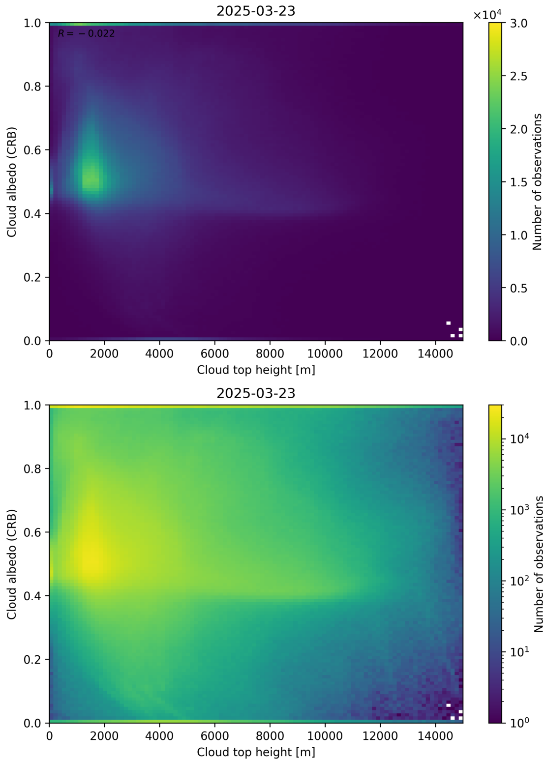
Figure 86: Scatter density plot of “Cloud top height” against “Cloud albedo (CRB)” for 2025-03-23 to 2025-03-24.
