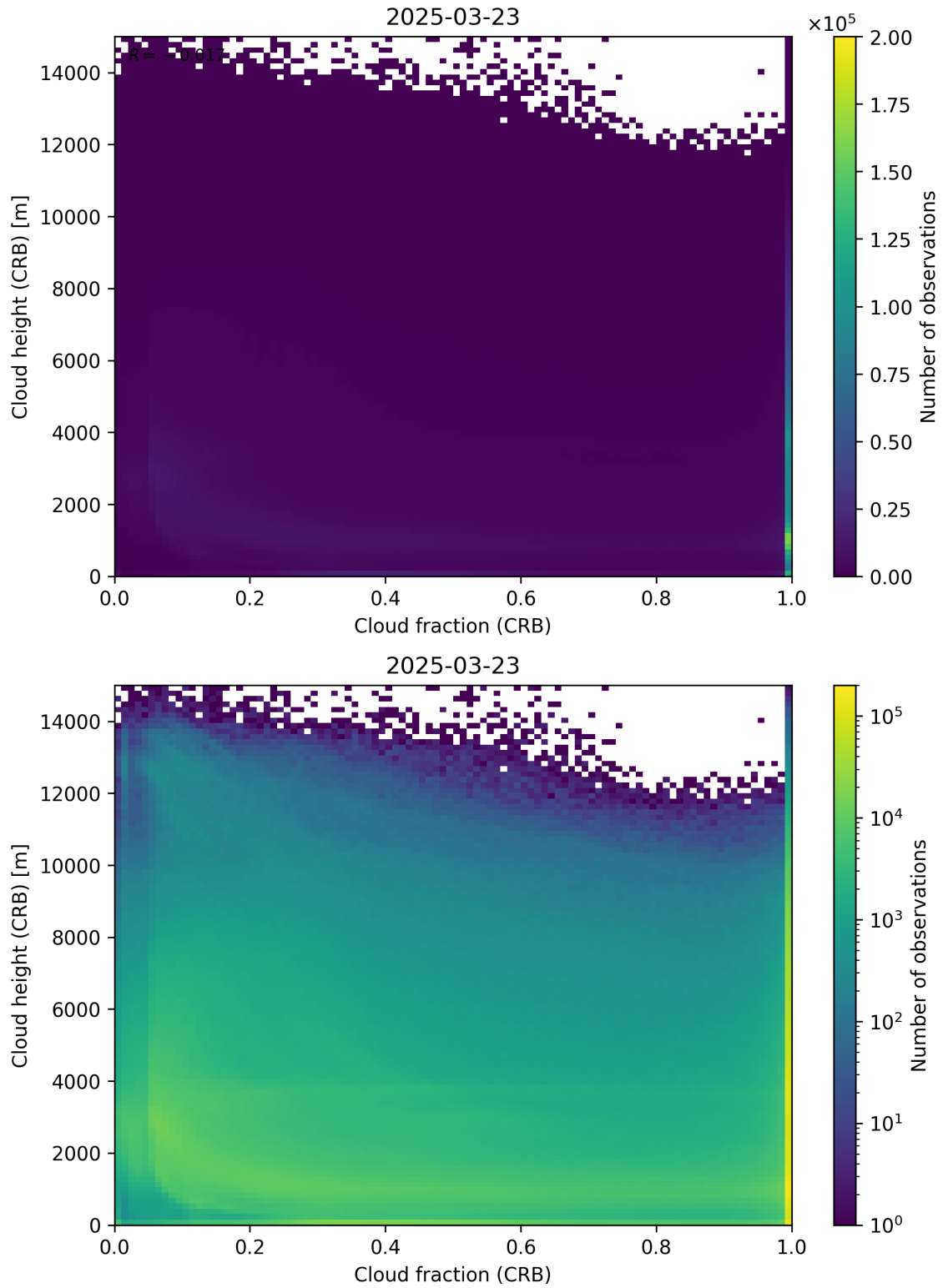
Figure 79: Scatter density plot of “Cloud fraction (CRB)” against “Cloud height (CRB)” for 2025-03-23 to 2025-03-24.
