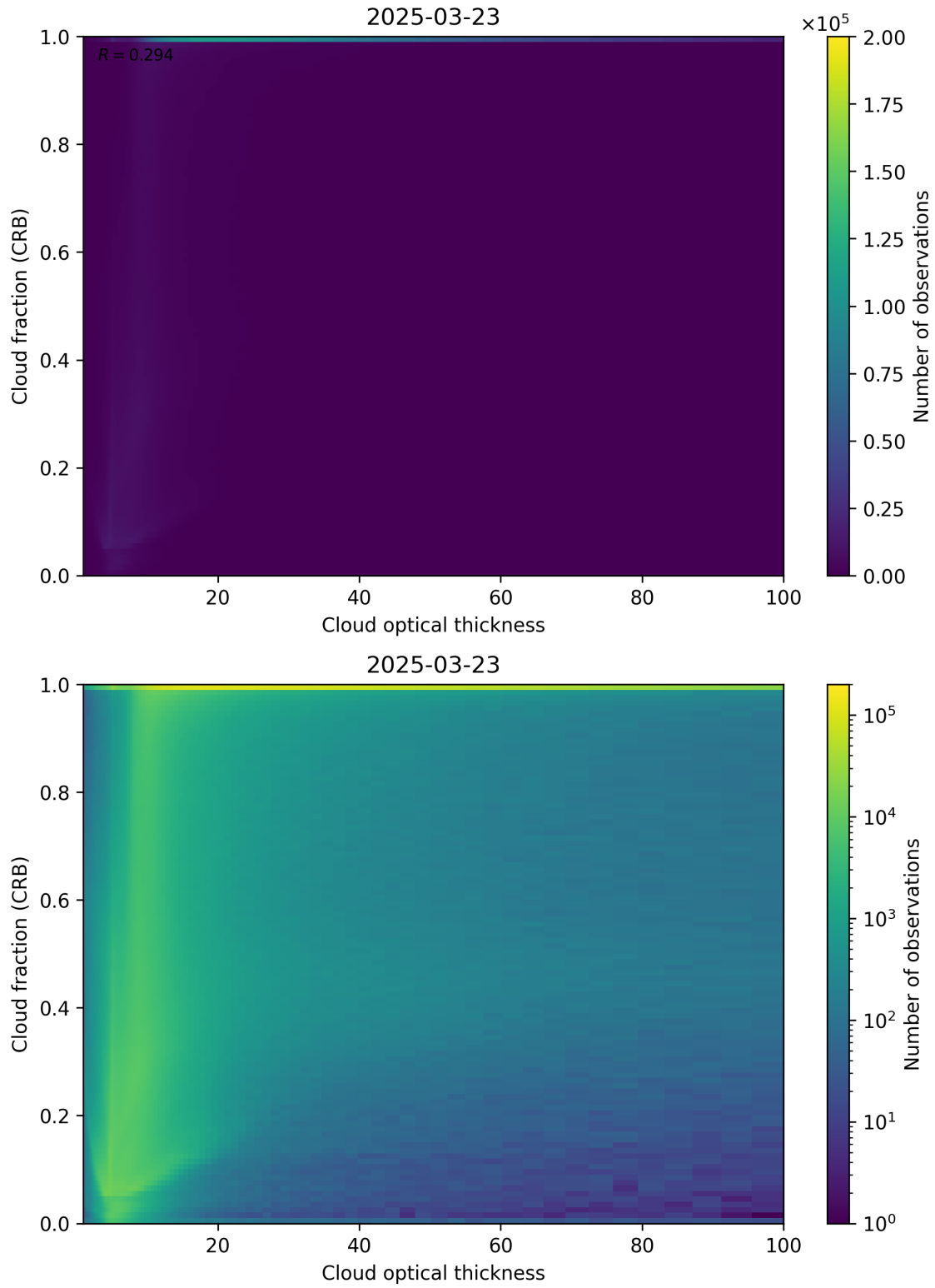
Figure 84: Scatter density plot of “Cloud optical thickness” against “Cloud fraction (CRB)” for 2025-03-23 to 2025-03-24.
