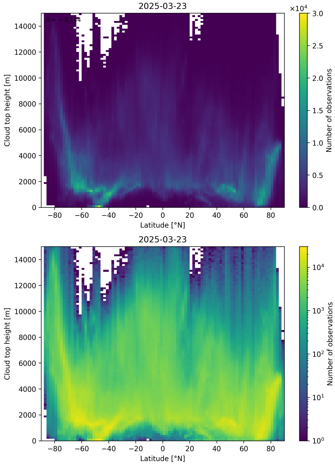
Figure 97: Scatter density plot of “Latitude” against “Cloud top height” for 2025-03-23 to 2025-03-24.
