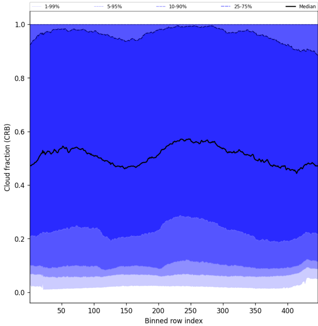
Figure 58: Along track statistics of “Cloud fraction (CRB)” for 2025-03-23 to 2025-03-24
