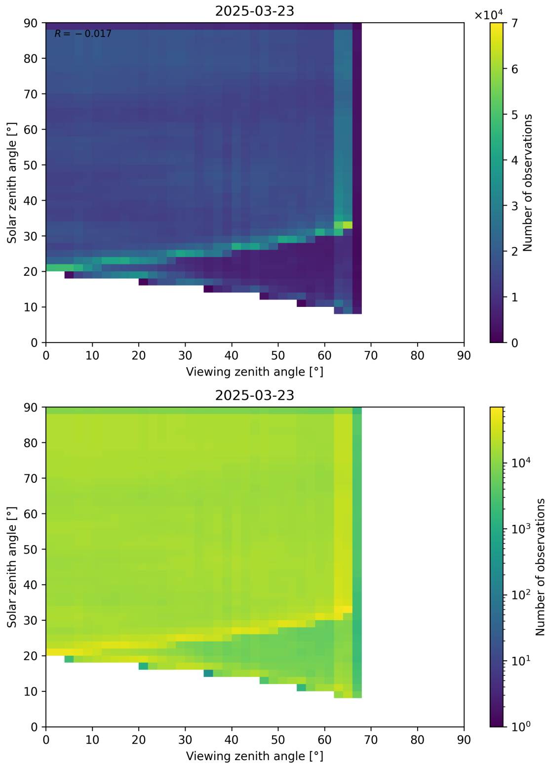
Figure 114: Scatter density plot of “Viewing zenith angle” against “Solar zenith angle” for 2025-03-23 to 2025-03-24.
