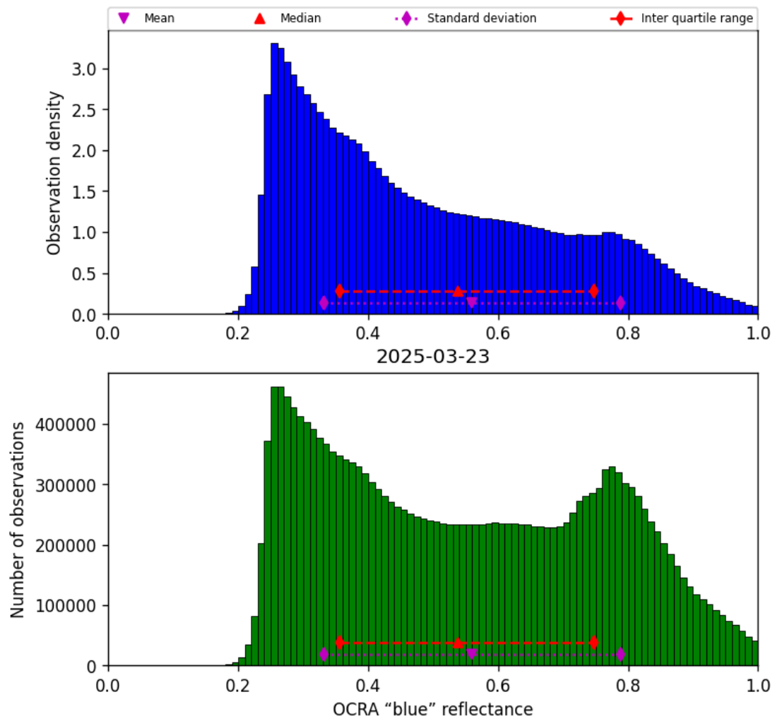
Figure 51: Histogram of “OCRA “blue” reflectance” for 2025-03-23 to 2025-03-24
