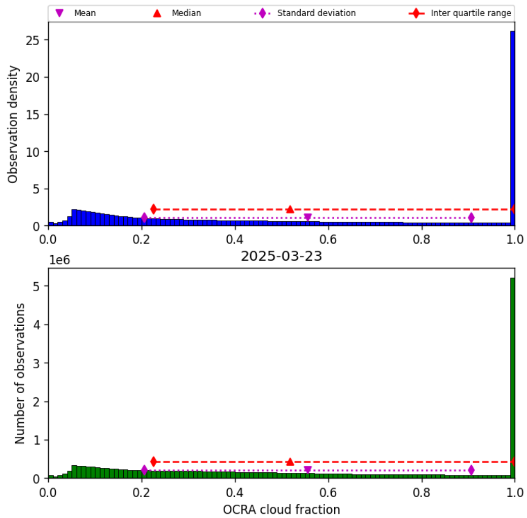
Figure 50: Histogram of “OCRA cloud fraction” for 2025-03-23 to 2025-03-24
