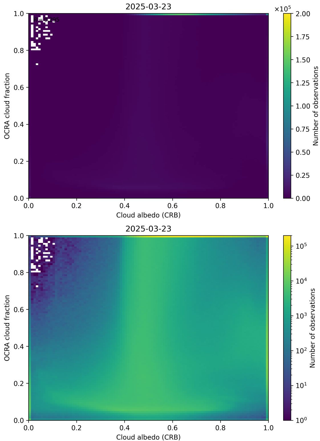
Figure 70: Scatter density plot of “Cloud albedo (CRB)” against “OCRA cloud fraction” for 2025-03-23 to 2025-03-24.
