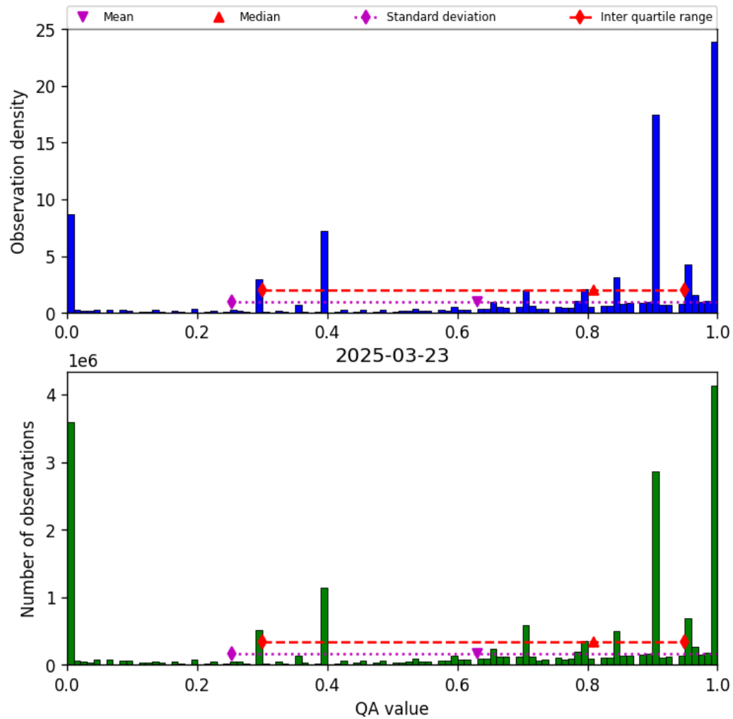
Figure 38: Histogram of “QA value” for 2025-03-23 to 2025-03-24
