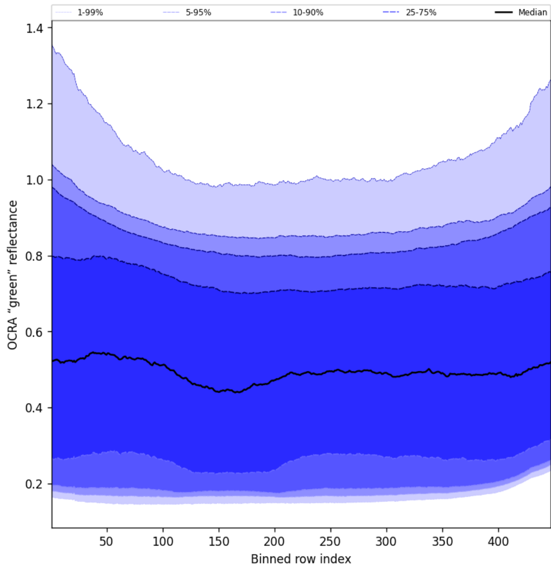
Figure 68: Along track statistics of "OCRA "green" reflectance" for 2025-03-23 to 2025-03-24
