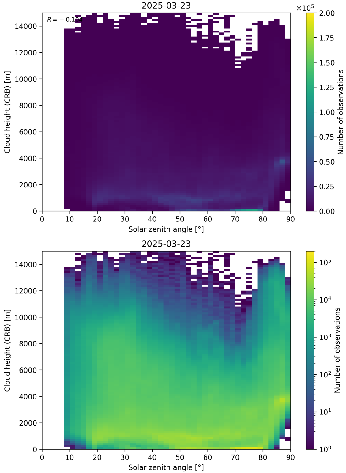
Figure 102: Scatter density plot of “Solar zenith angle” against “Cloud height (CRB)” for 2025-03-23 to 2025-03-24.
