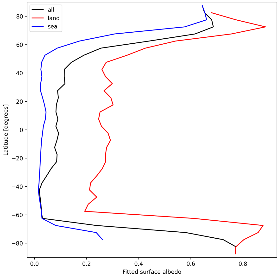
Figure 29: Zonal average of “Fitted surface albedo” for 2025-03-23 to 2025-03-24.
