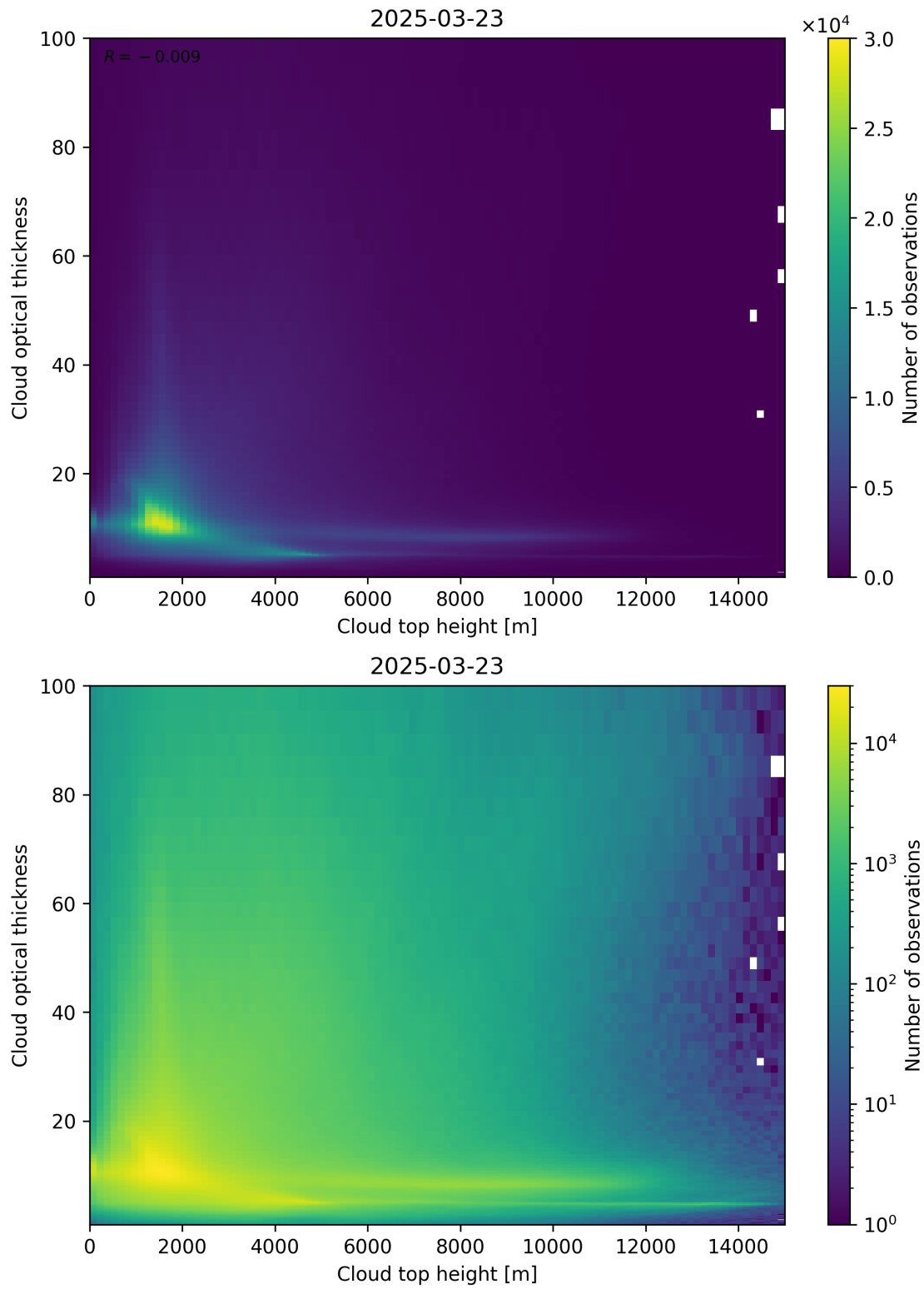
Figure 90: Scatter density plot of “Cloud top height” against “Cloud optical thickness” for 2025-03-23 to 2025-03-24.
