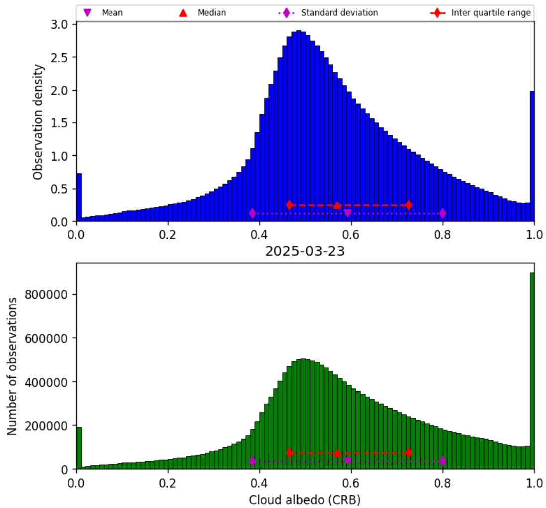
Figure 44: Histogram of “Cloud albedo (CRB)” for 2025-03-23 to 2025-03-24
