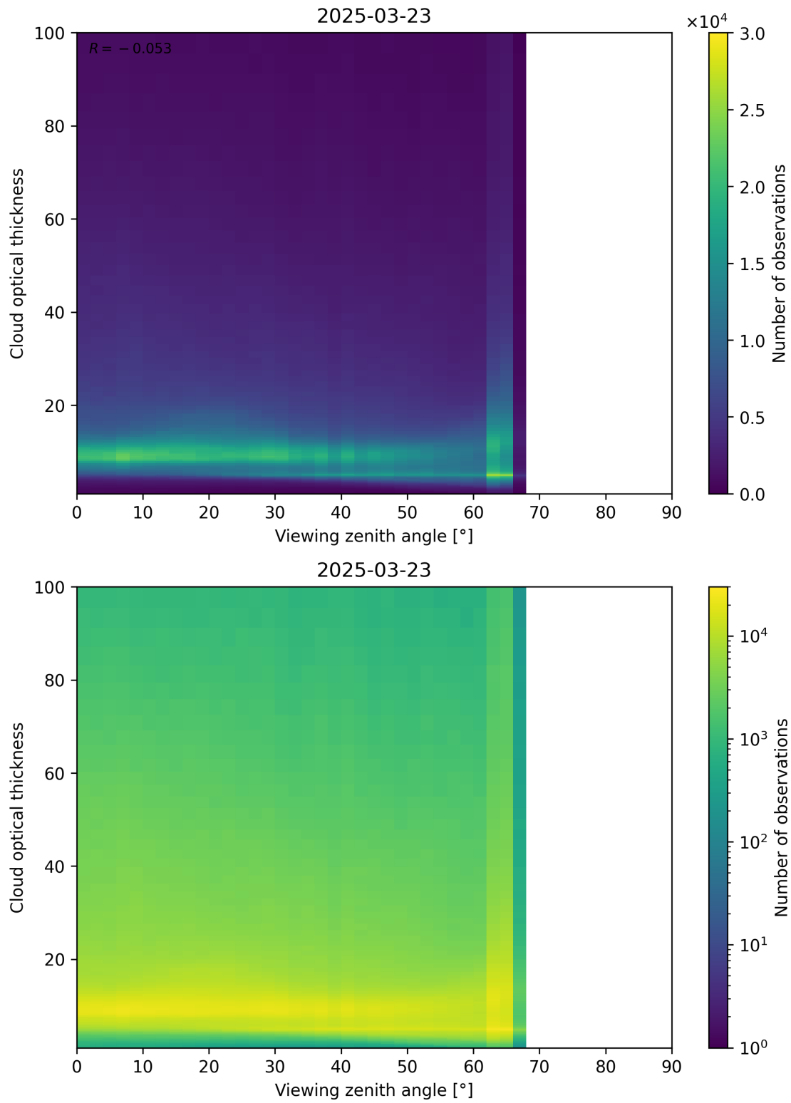
Figure 111: Scatter density plot of “Viewing zenith angle” against “Cloud optical thickness” for 2025-03-23 to 2025-03-24.
