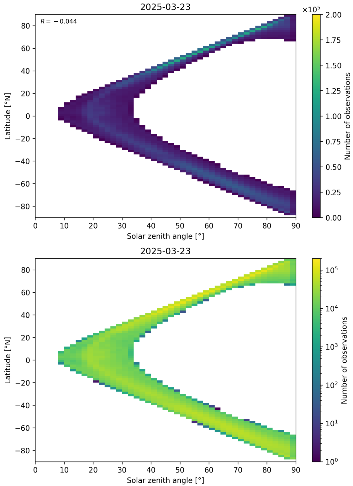
Figure 105: Scatter density plot of “Solar zenith angle” against “Latitude” for 2025-03-23 to 2025-03-24.
