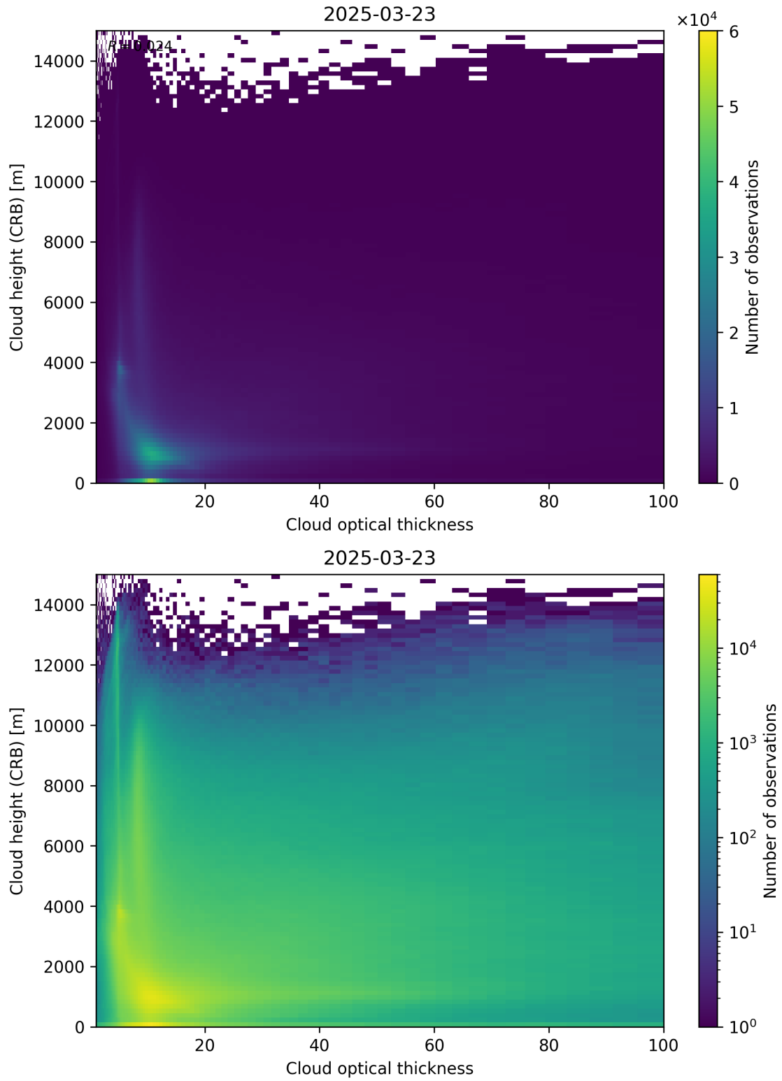
Figure 85: Scatter density plot of “Cloud optical thickness” against “Cloud height (CRB)” for 2025-03-23 to 2025-03-24.
