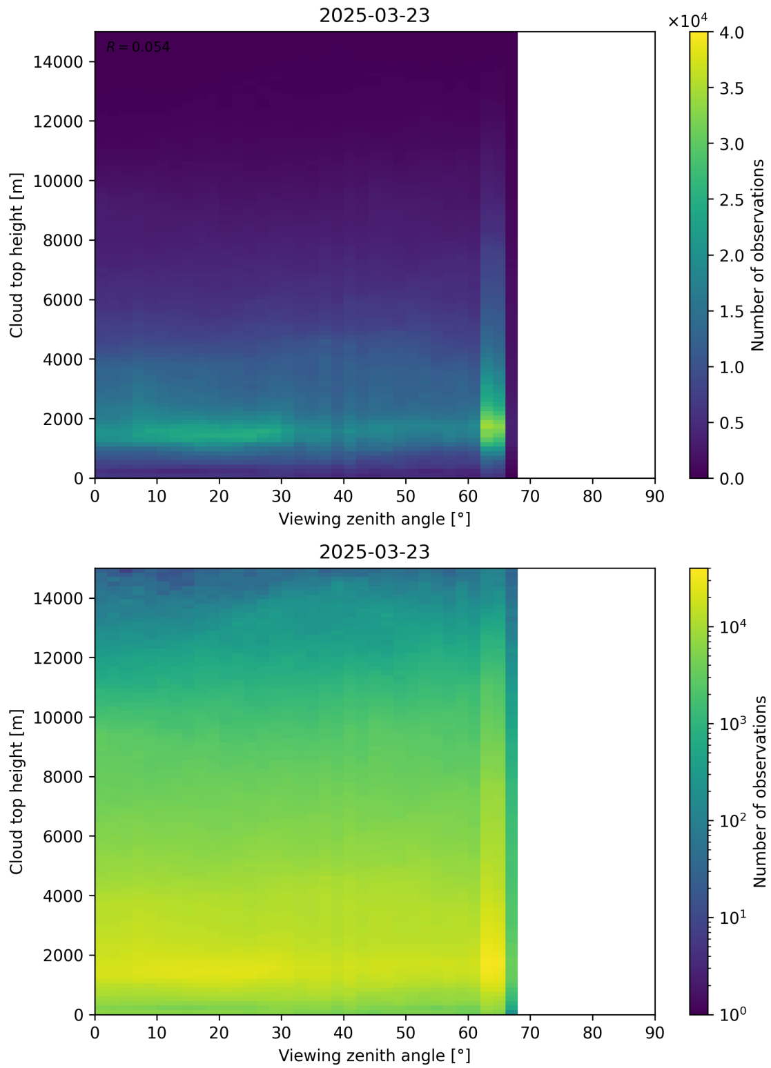
Figure 112: Scatter density plot of “Viewing zenith angle” against “Cloud top height” for 2025-03-23 to 2025-03-24.
