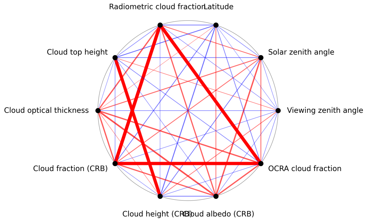
Figure 1: Map of correlation graph for 2025-03-23 to 2025-03-24.
