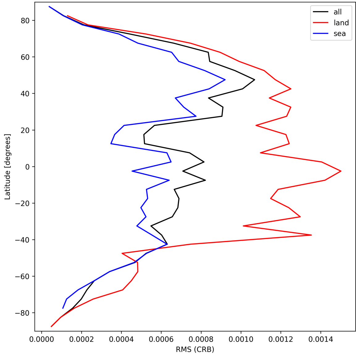
Figure 32: Zonal average of “RMS (CRB)” for 2025-03-23 to 2025-03-24.
