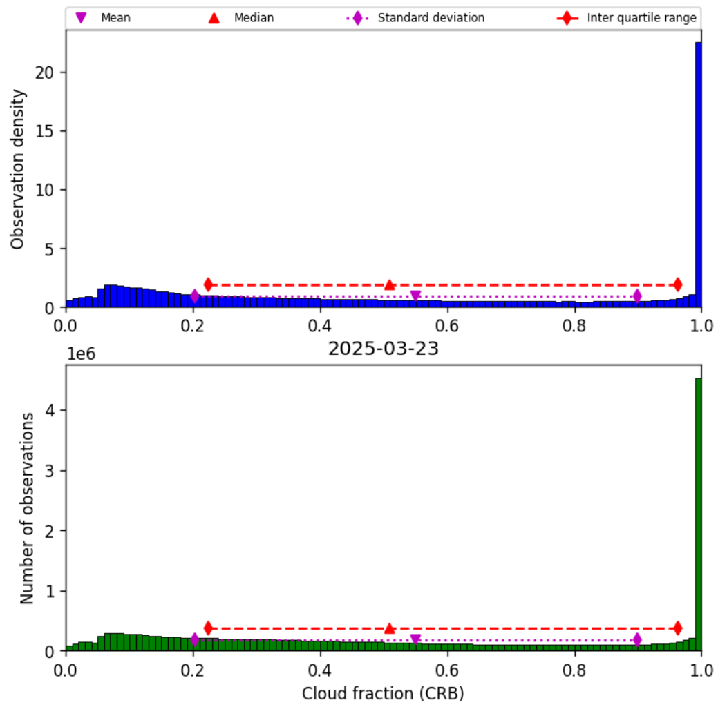
Figure 42: Histogram of “Cloud fraction (CRB)” for 2025-03-23 to 2025-03-24
