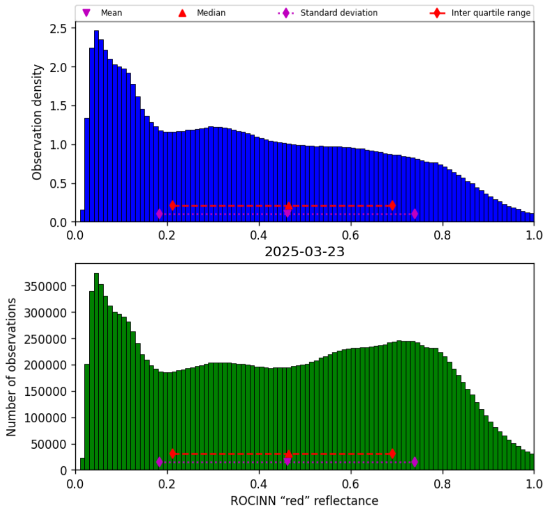
Figure 53: Histogram of “ROCINN “red” reflectance” for 2025-03-23 to 2025-03-24
