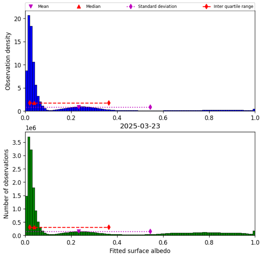
Figure 45: Histogram of “Fitted surface albedo” for 2025-03-23 to 2025-03-24
