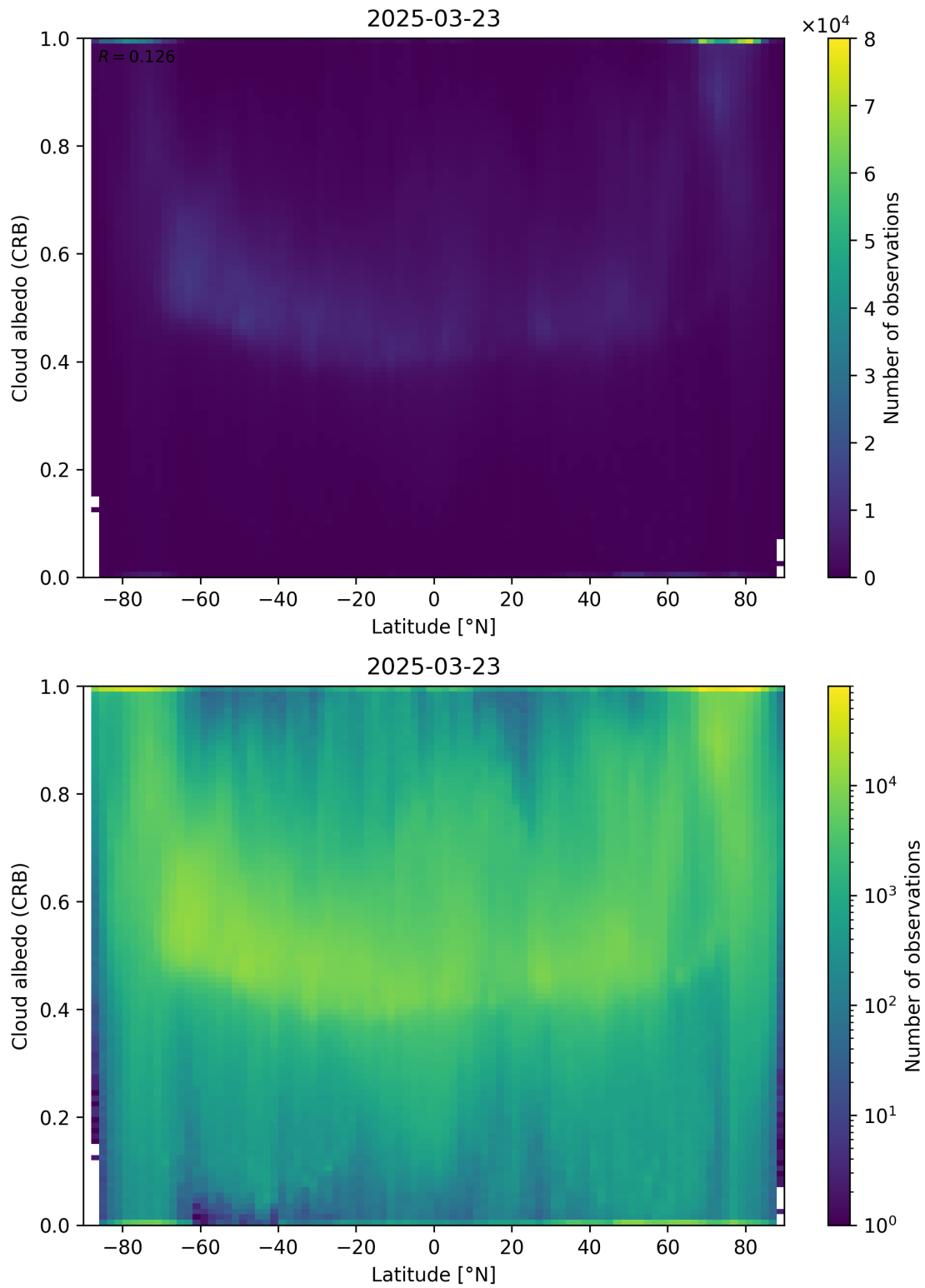
Figure 91: Scatter density plot of “Latitude” against “Cloud albedo (CRB)” for 2025-03-23 to 2025-03-24.
