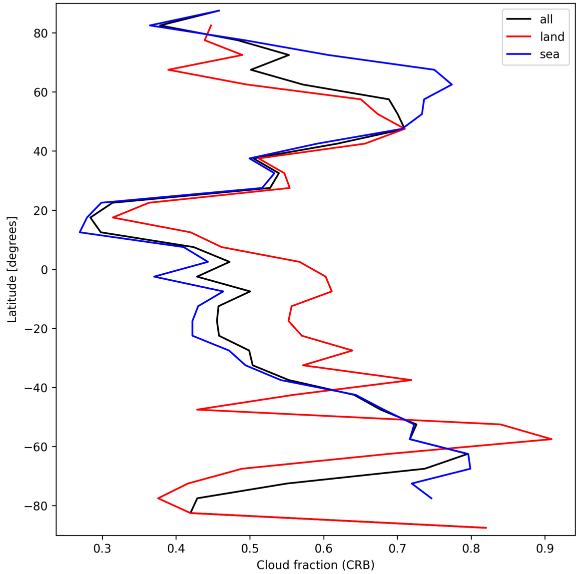
Figure 26: Zonal average of “Cloud fraction (CRB)” for 2025-03-23 to 2025-03-24.
