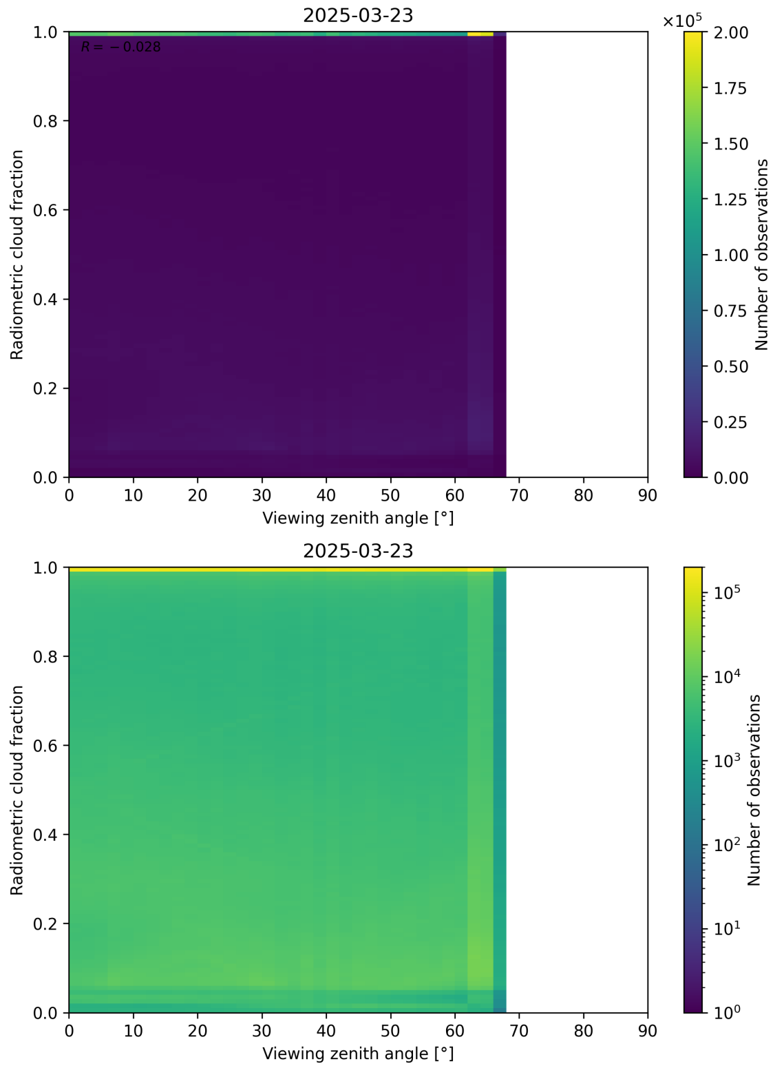
Figure 107: Scatter density plot of “Viewing zenith angle” against “Radiometric cloud fraction” for 2025-03-23 to 2025-03-24.
