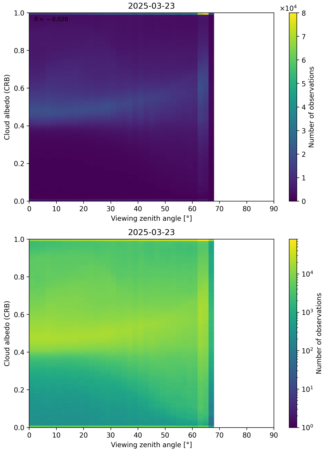
Figure 106: Scatter density plot of “Viewing zenith angle” against “Cloud albedo (CRB)” for 2025-03-23 to 2025-03-24.
