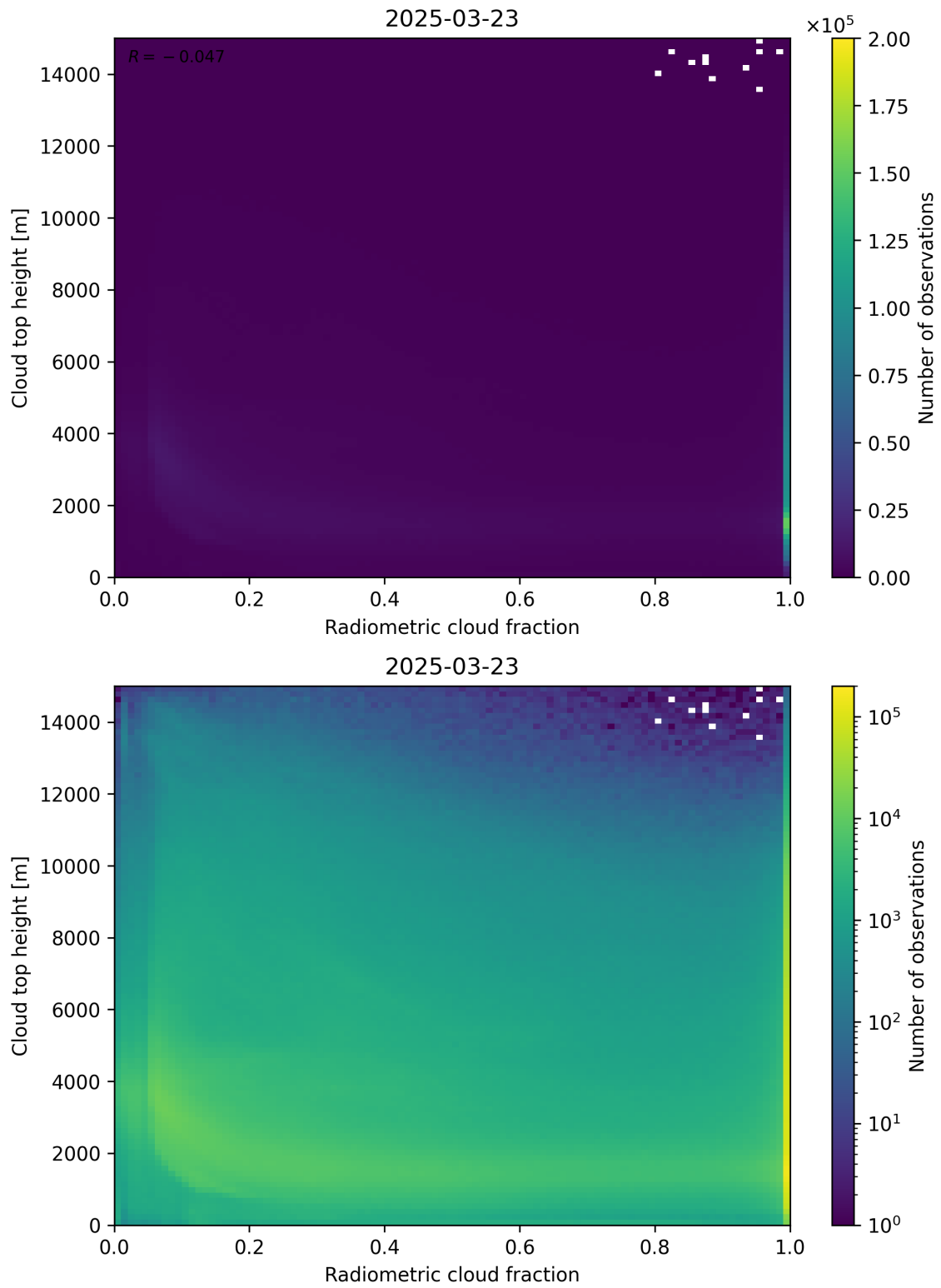
Figure 76: Scatter density plot of “Radiometric cloud fraction” against “Cloud top height” for 2025-03-23 to 2025-03-24.
