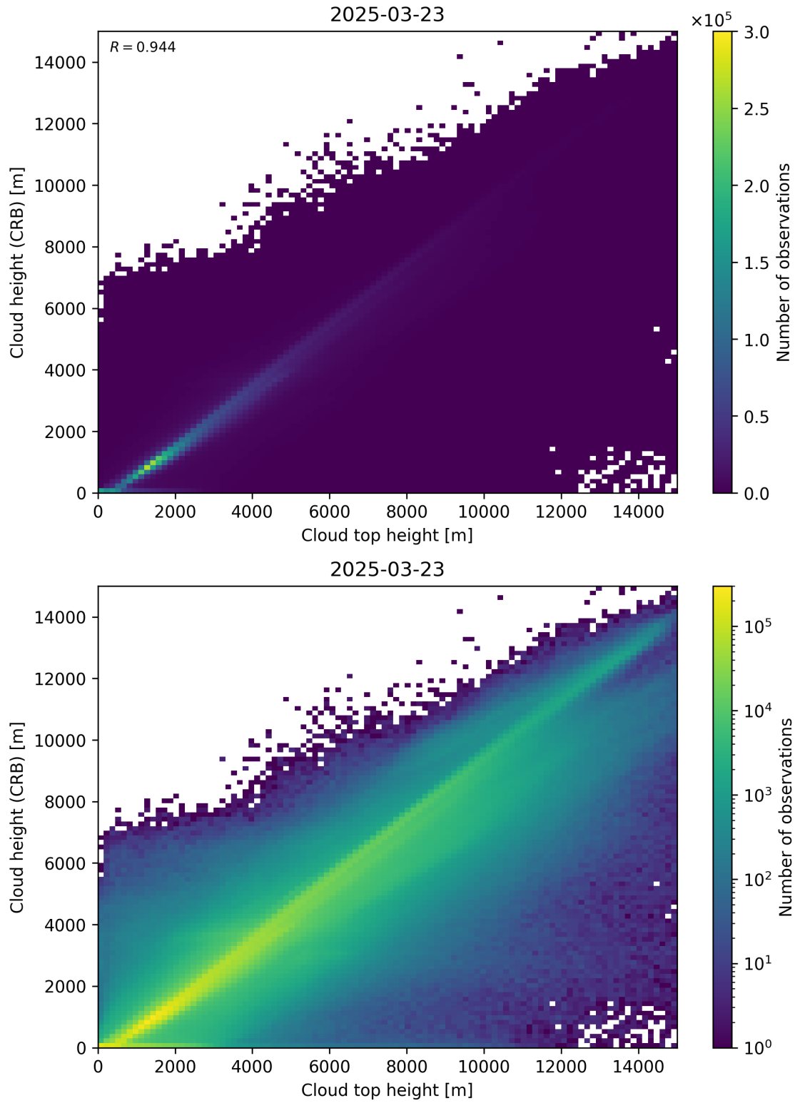
Figure 89: Scatter density plot of “Cloud top height” against “Cloud height (CRB)” for 2025-03-23 to 2025-03-24.
