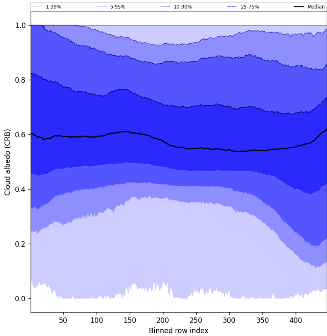
Figure 60: Along track statistics of “Cloud albedo (CRB)” for 2025-03-23 to 2025-03-24
