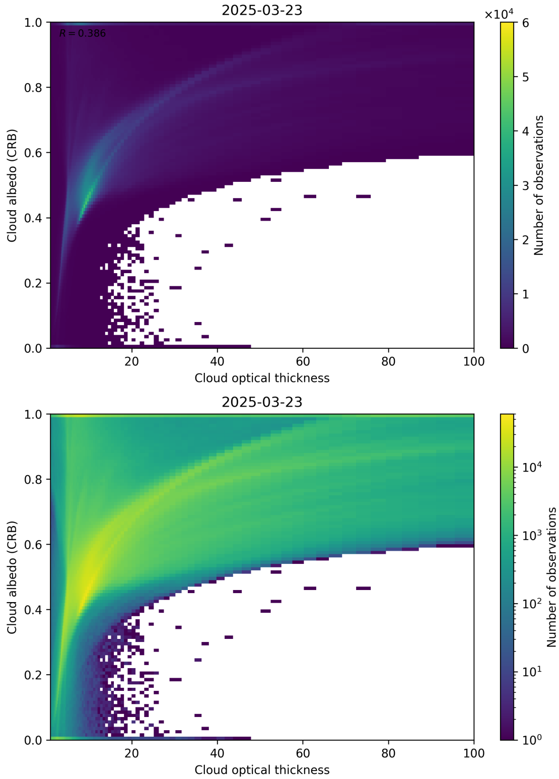
Figure 82: Scatter density plot of “Cloud optical thickness” against “Cloud albedo (CRB)” for 2025-03-23 to 2025-03-24.
