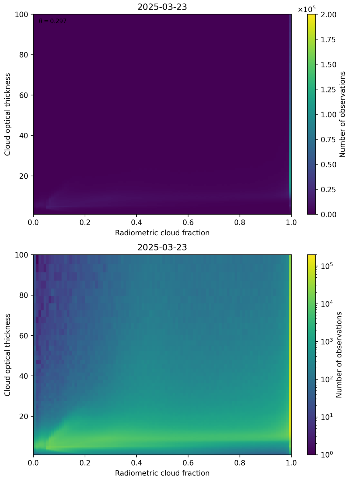
Figure 75: Scatter density plot of “Radiometric cloud fraction” against “Cloud optical thickness” for 2025-03-23 to 2025-03-24.
