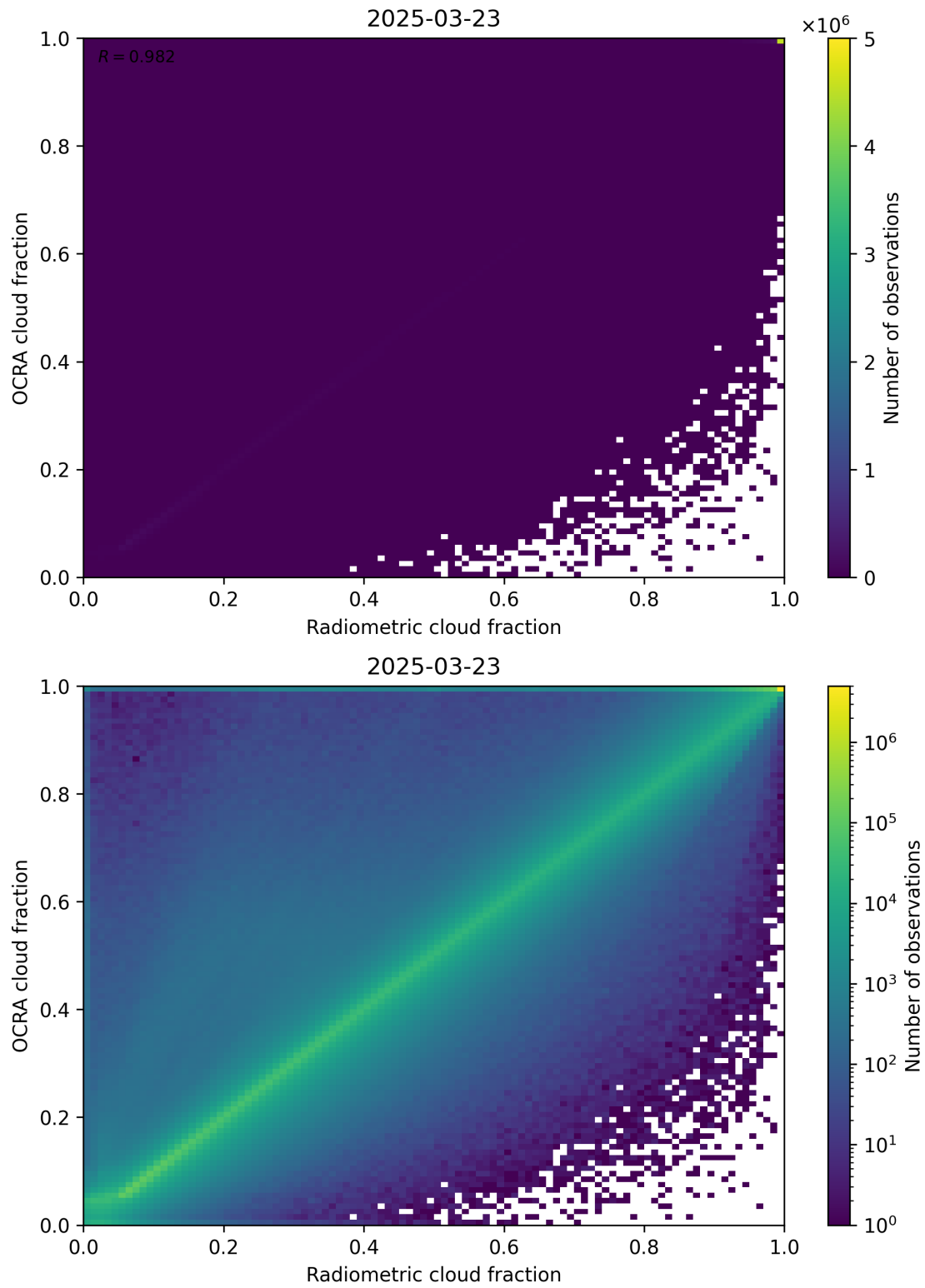
Figure 72: Scatter density plot of “Radiometric cloud fraction” against “OCRA cloud fraction” for 2025-03-23 to 2025-03-24.
