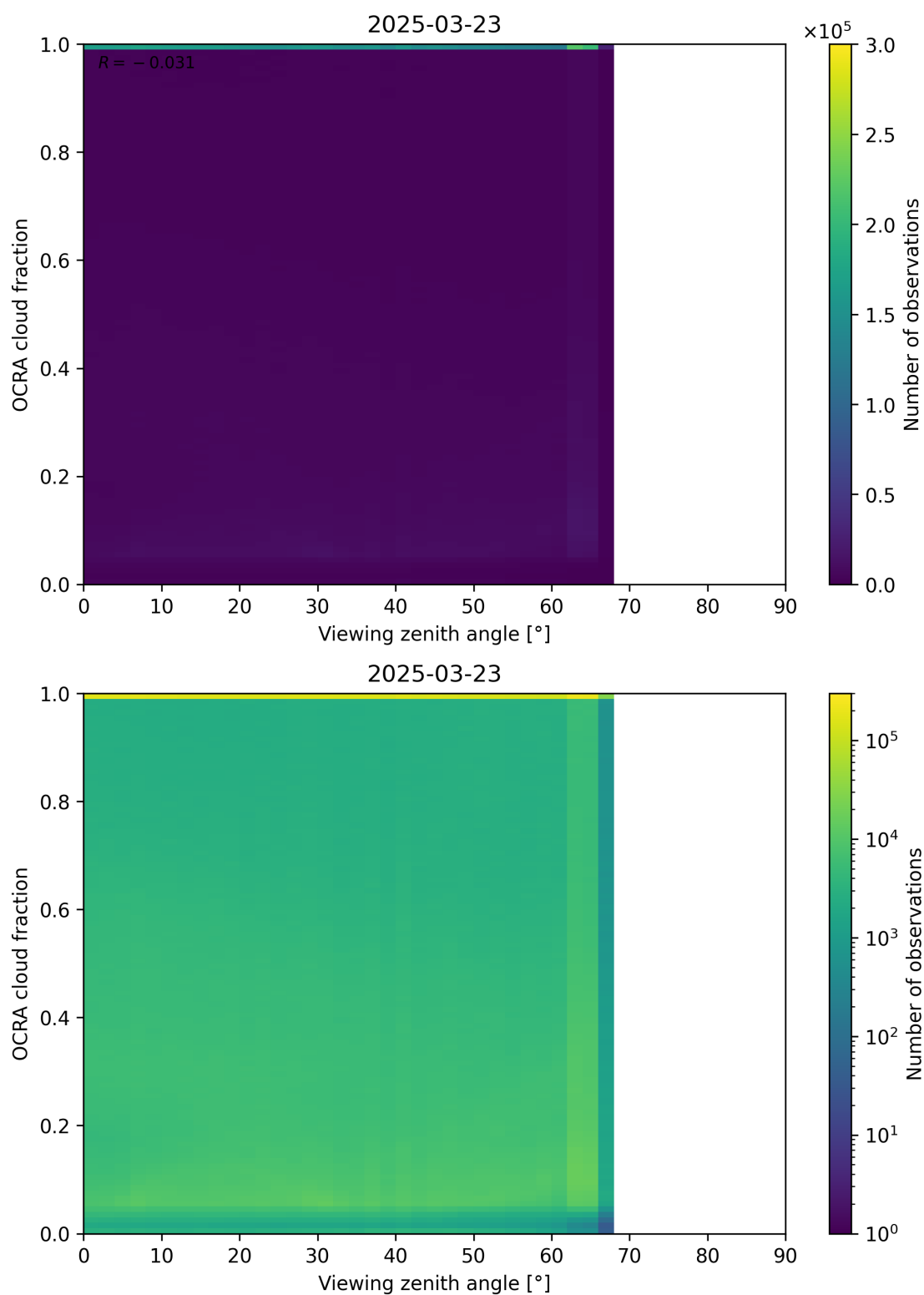
Figure 108: Scatter density plot of “Viewing zenith angle” against “OCRA cloud fraction” for 2025-03-23 to 2025-03-24.
