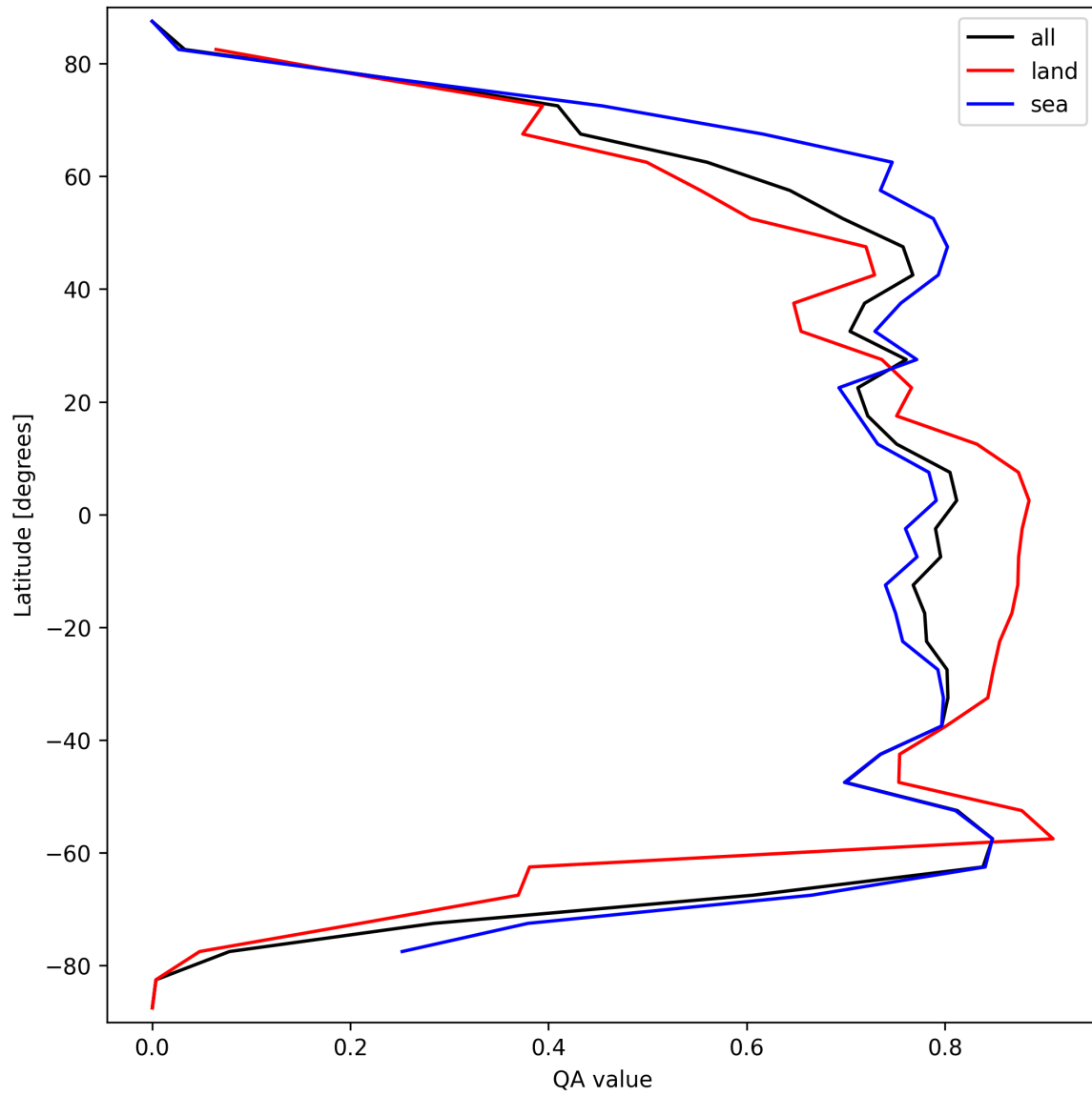
Figure 22: Zonal average of “QA value” for 2025-03-23 to 2025-03-24.
