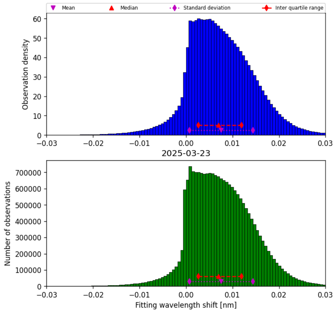
Figure 49: Histogram of “Fitting wavelength shift” for 2025-03-23 to 2025-03-24
