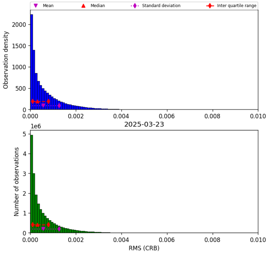
Figure 48: Histogram of "RMS (CRB)" for 2025-03-23 to 2025-03-24
