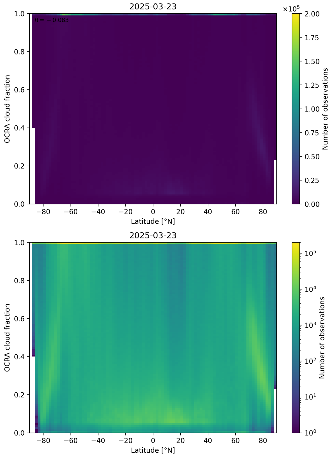
Figure 93: Scatter density plot of “Latitude” against “OCRA cloud fraction” for 2025-03-23 to 2025-03-24.
