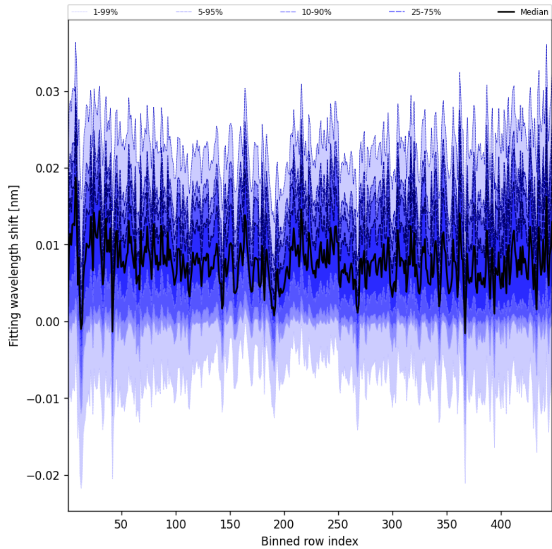
Figure 65: Along track statistics of “Fitting wavelength shift” for 2025-03-23 to 2025-03-24
