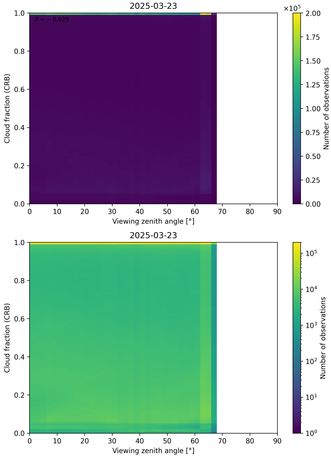
Figure 109: Scatter density plot of “Viewing zenith angle” against “Cloud fraction (CRB)” for 2025-03-23 to 2025-03-24.
