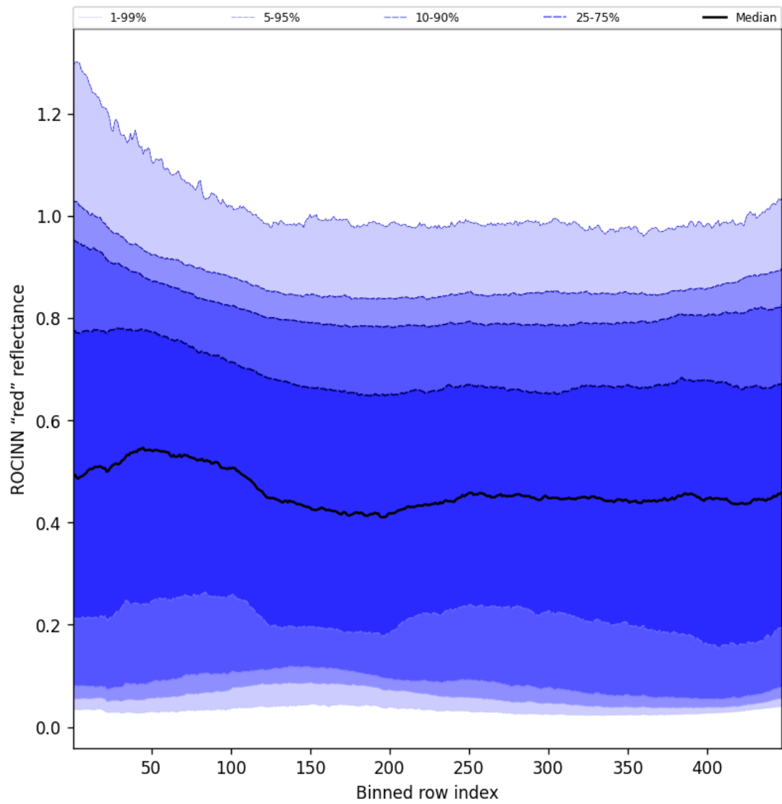
Figure 69: Along track statistics of “ROCINN “red” reflectance” for 2025-03-24 to 2025-03-26
