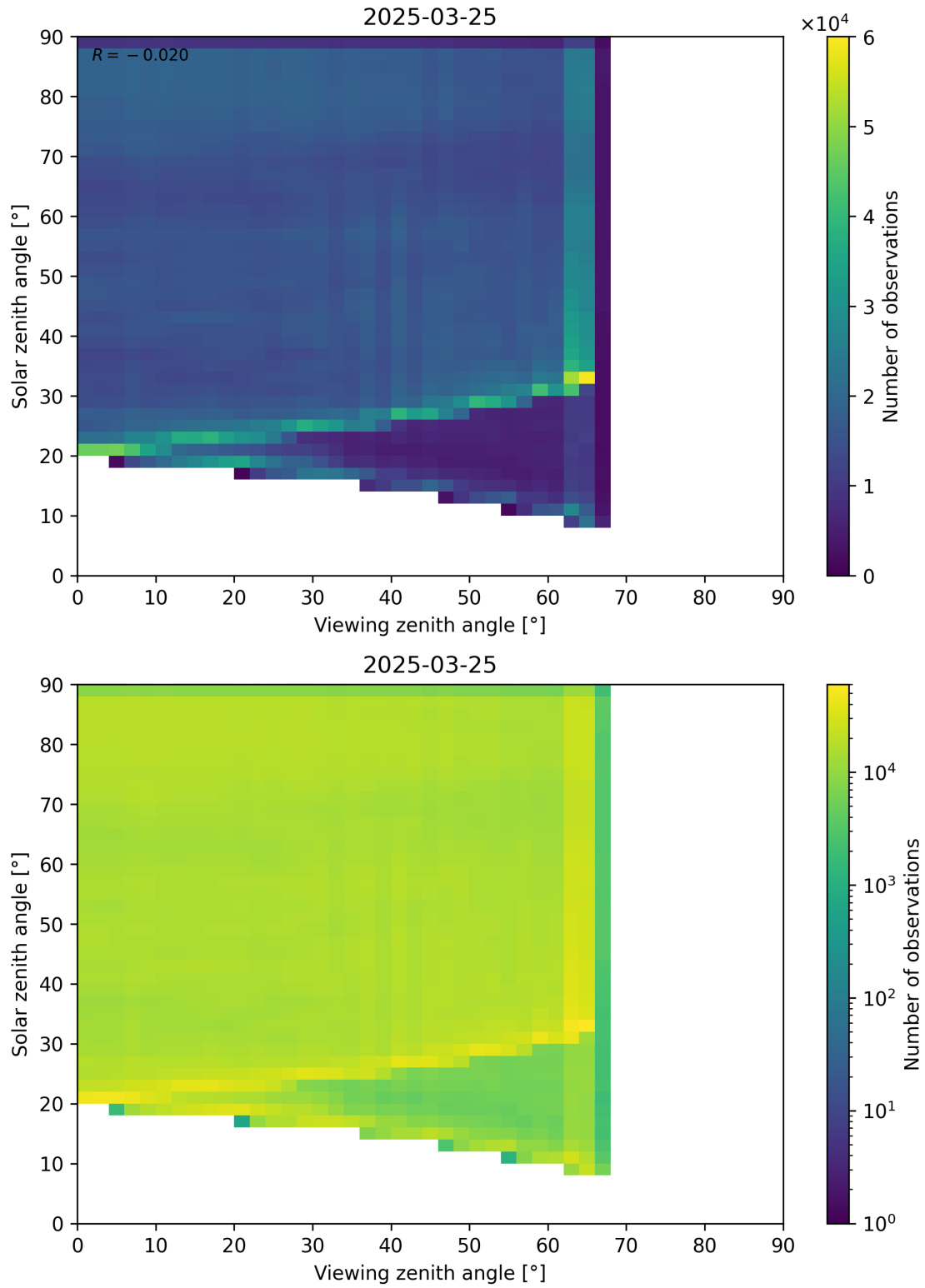
Figure 114: Scatter density plot of “Viewing zenith angle” against “Solar zenith angle” for 2025-03-24 to 2025-03-26.
