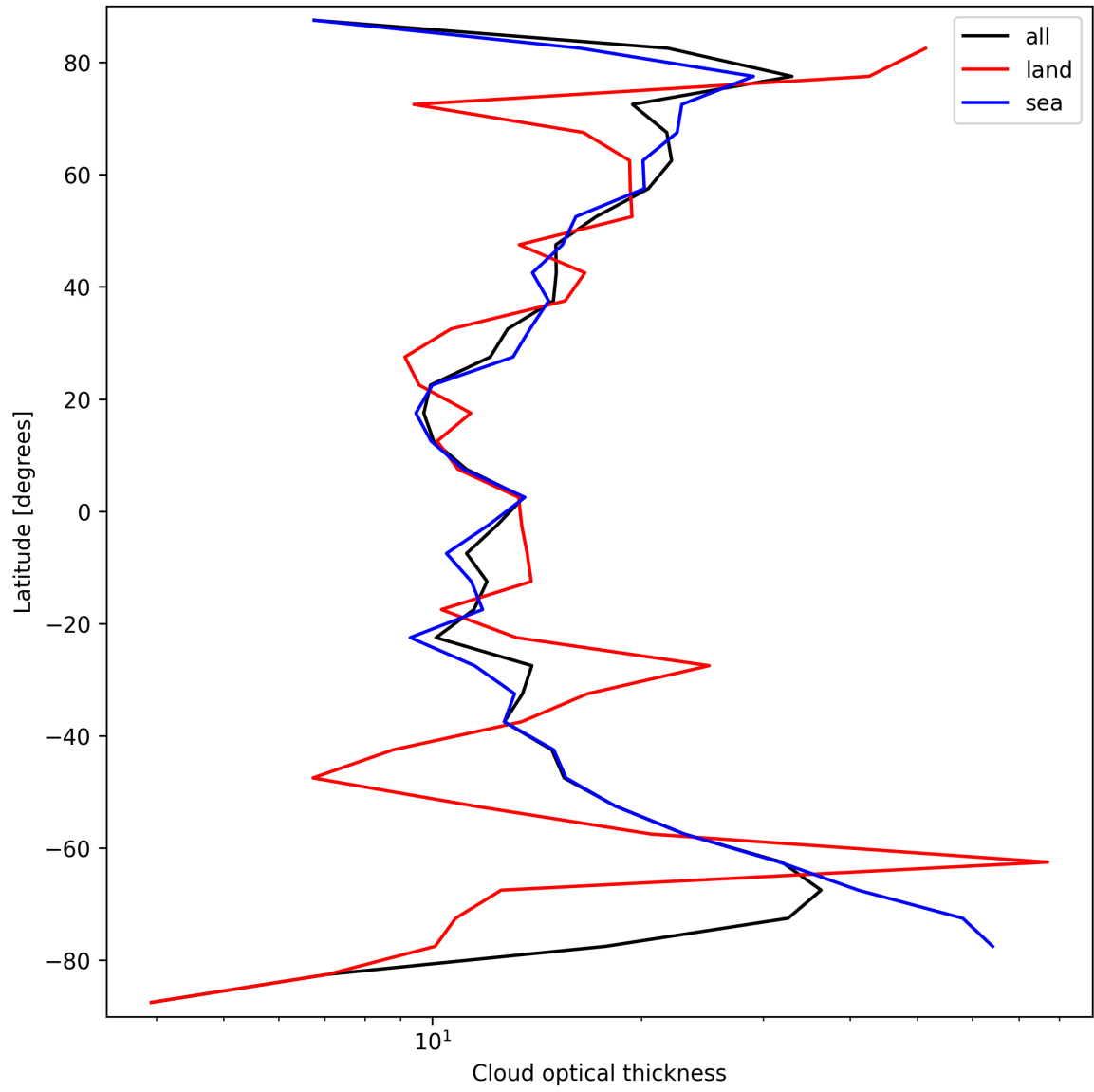
Figure 25: Zonal average of “Cloud optical thickness” for 2025-03-24 to 2025-03-26.
