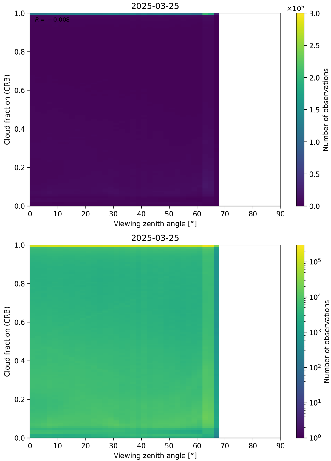
Figure 109: Scatter density plot of “Viewing zenith angle” against “Cloud fraction (CRB)” for 2025-03-24 to 2025-03-26.
