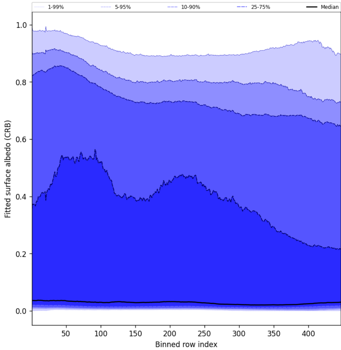
Figure 62: Along track statistics of “Fitted surface albedo (CRB)” for 2025-03-24 to 2025-03-26
