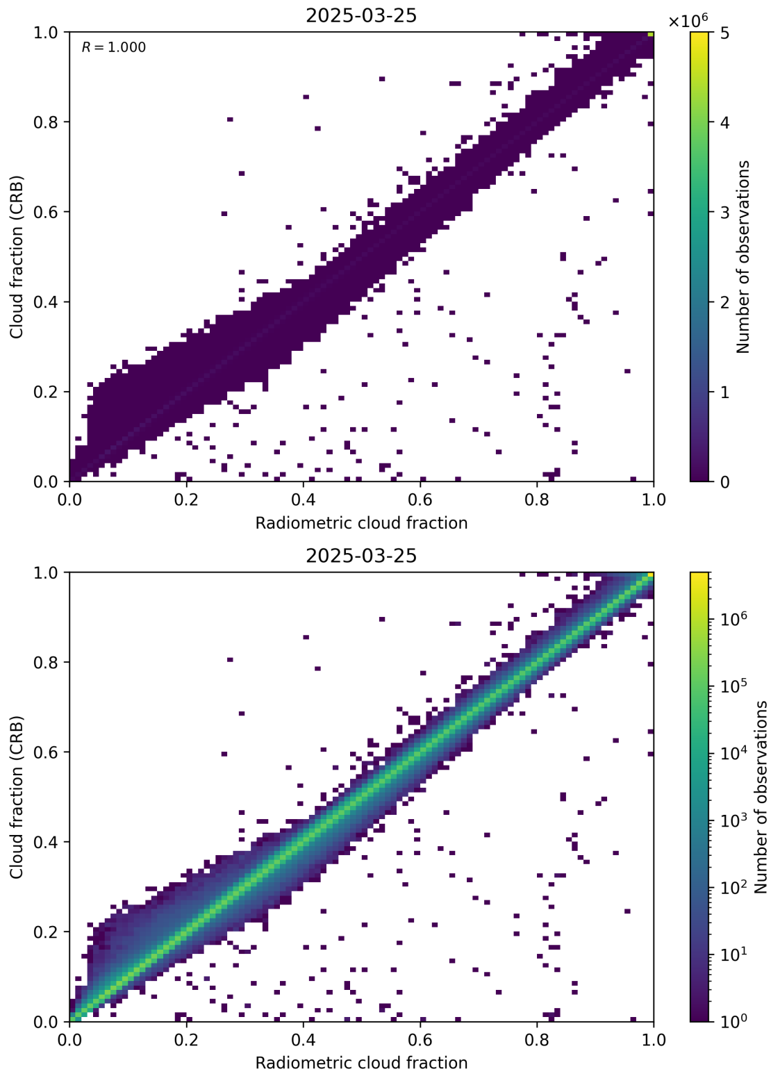
Figure 73: Scatter density plot of “Radiometric cloud fraction” against “Cloud fraction (CRB)” for 2025-03-24 to 2025-03-26.
