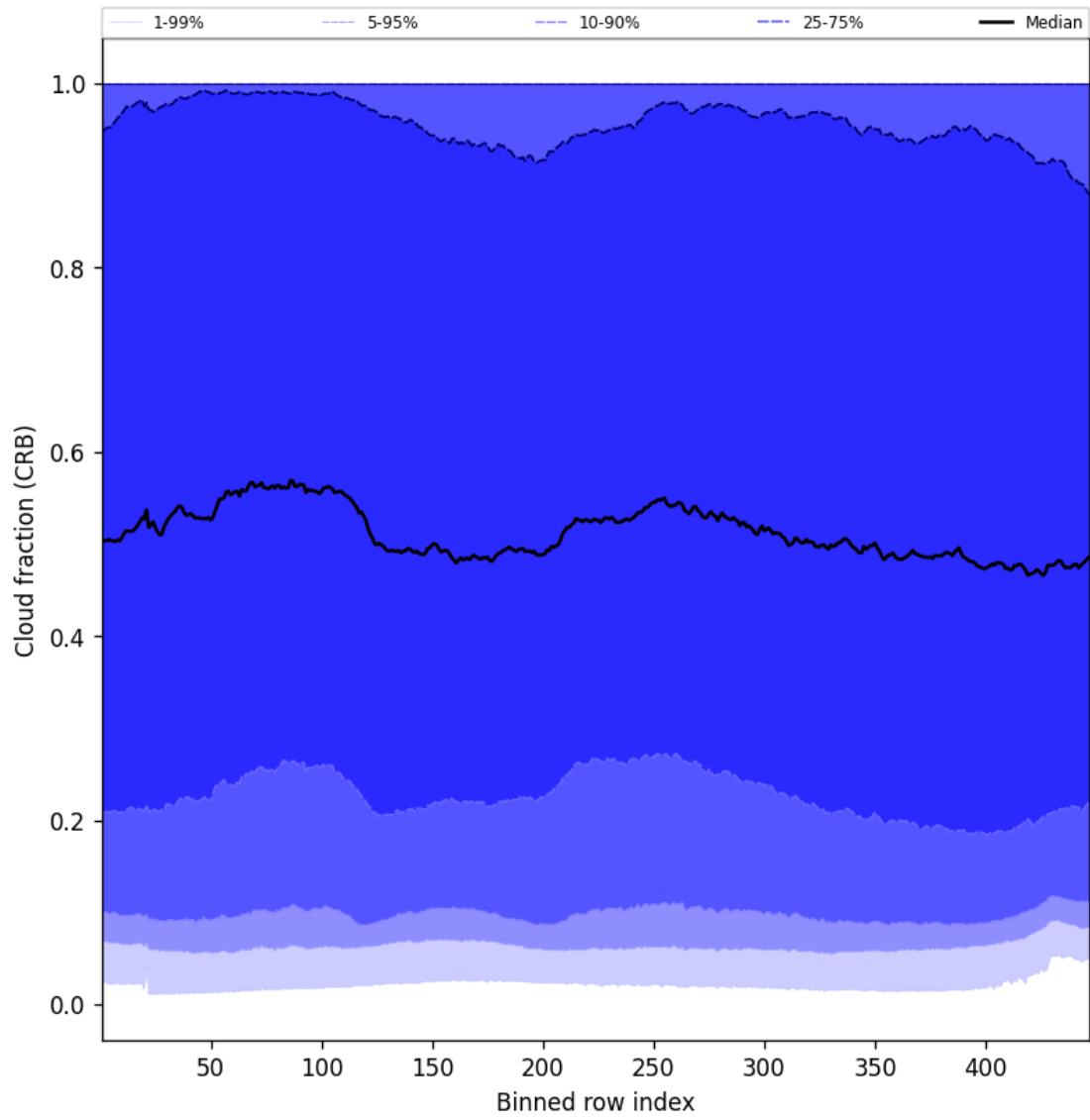
Figure 58: Along track statistics of “Cloud fraction (CRB)” for 2025-03-24 to 2025-03-26
