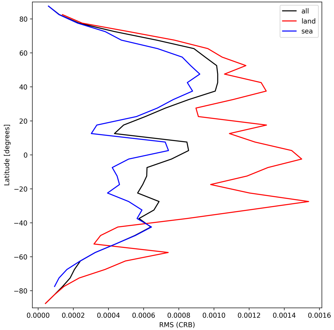
Figure 32: Zonal average of “RMS (CRB)” for 2025-03-24 to 2025-03-26.
