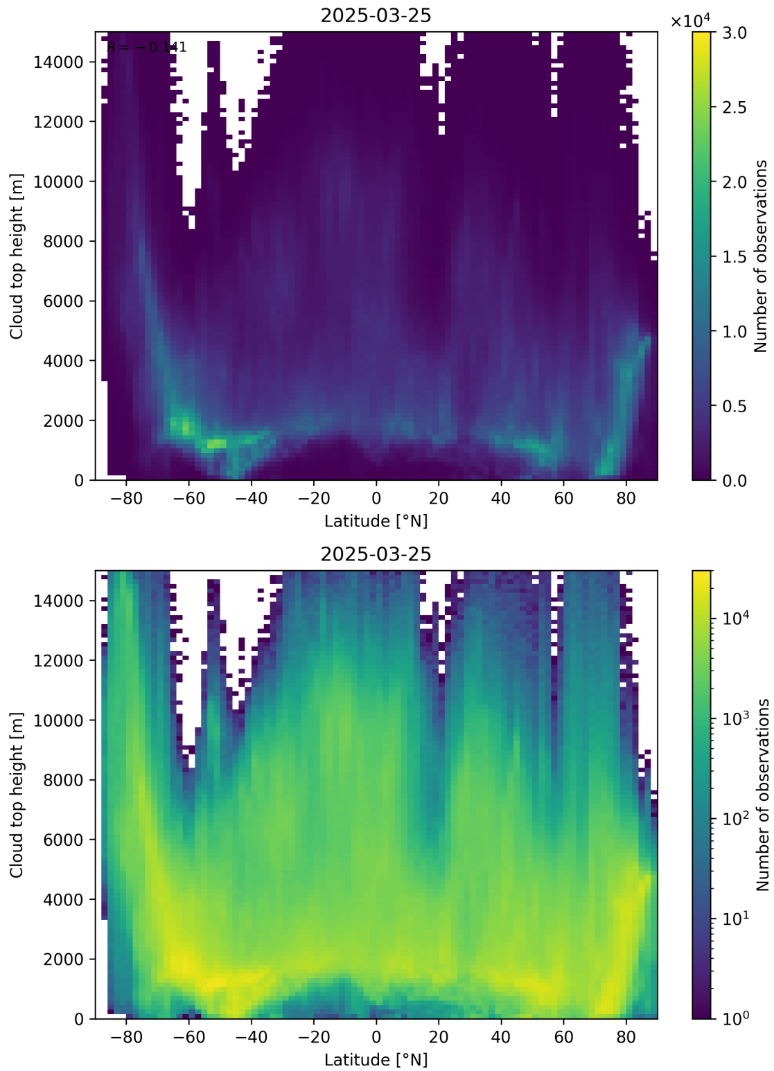
Figure 97: Scatter density plot of “Latitude” against “Cloud top height” for 2025-03-24 to 2025-03-26.
