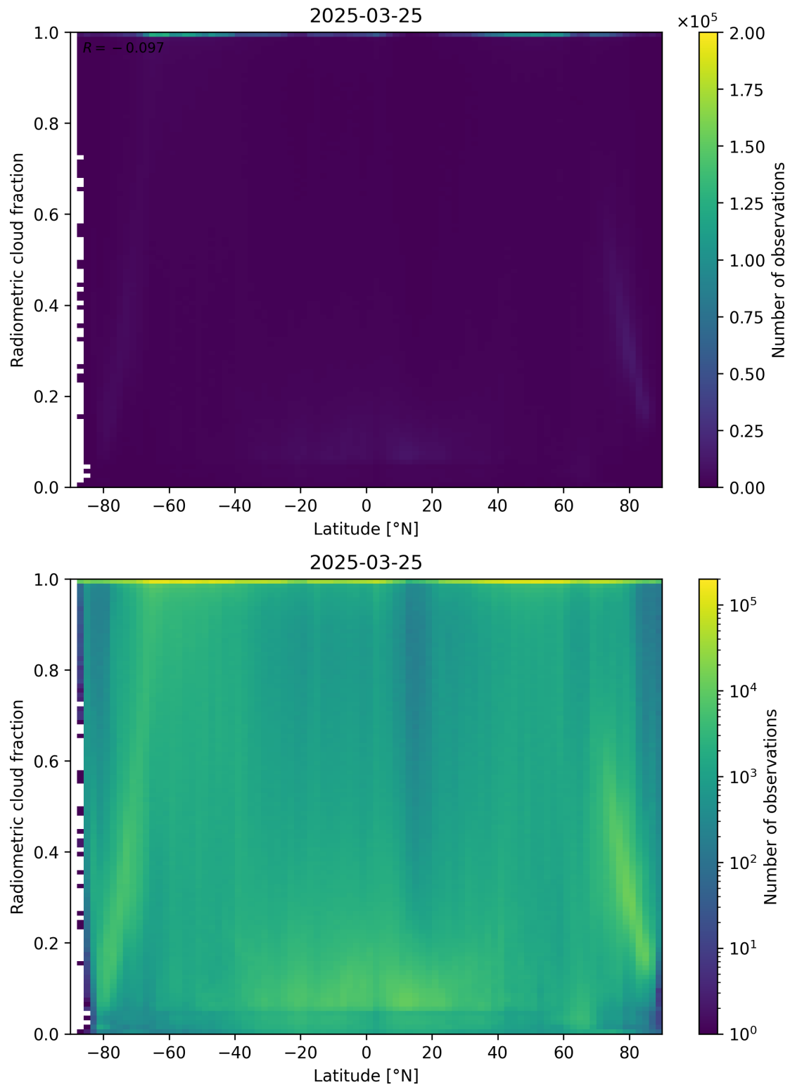
Figure 92: Scatter density plot of “Latitude” against “Radiometric cloud fraction” for 2025-03-24 to 2025-03-26.
