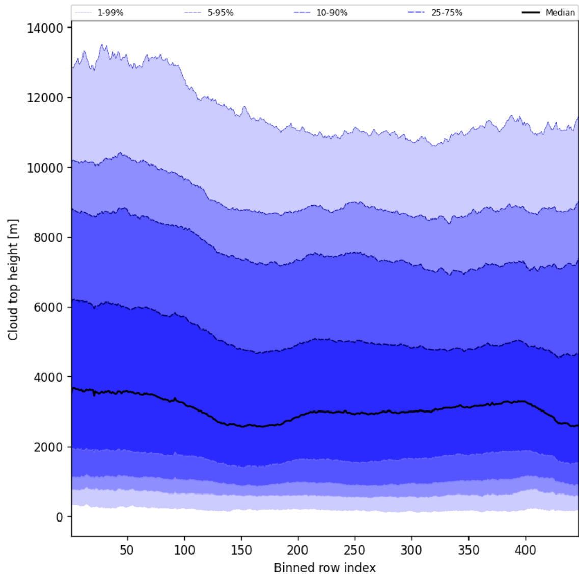
Figure 56: Along track statistics of “Cloud top height” for 2025-03-24 to 2025-03-26
