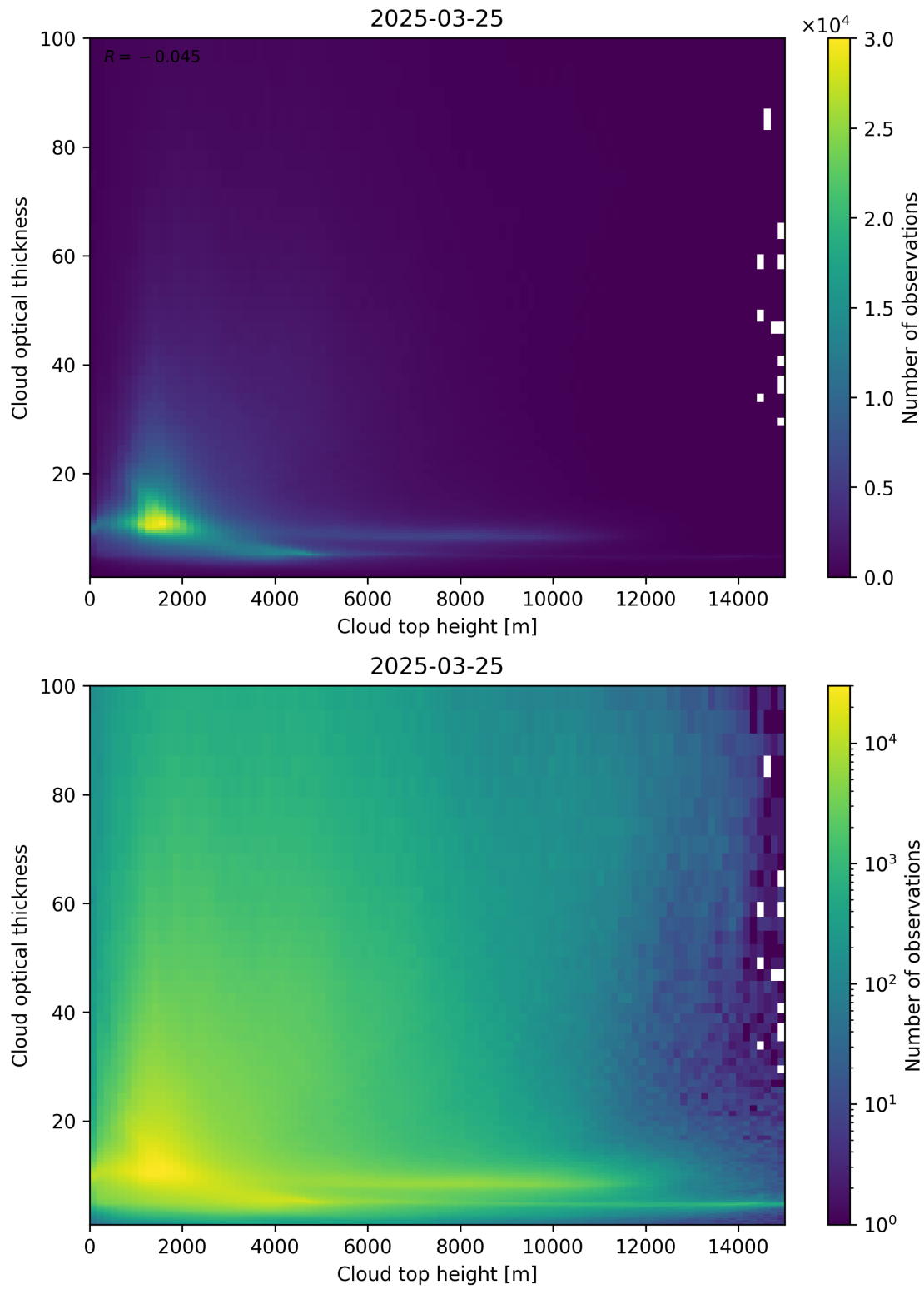
Figure 90: Scatter density plot of “Cloud top height” against “Cloud optical thickness” for 2025-03-24 to 2025-03-26.
