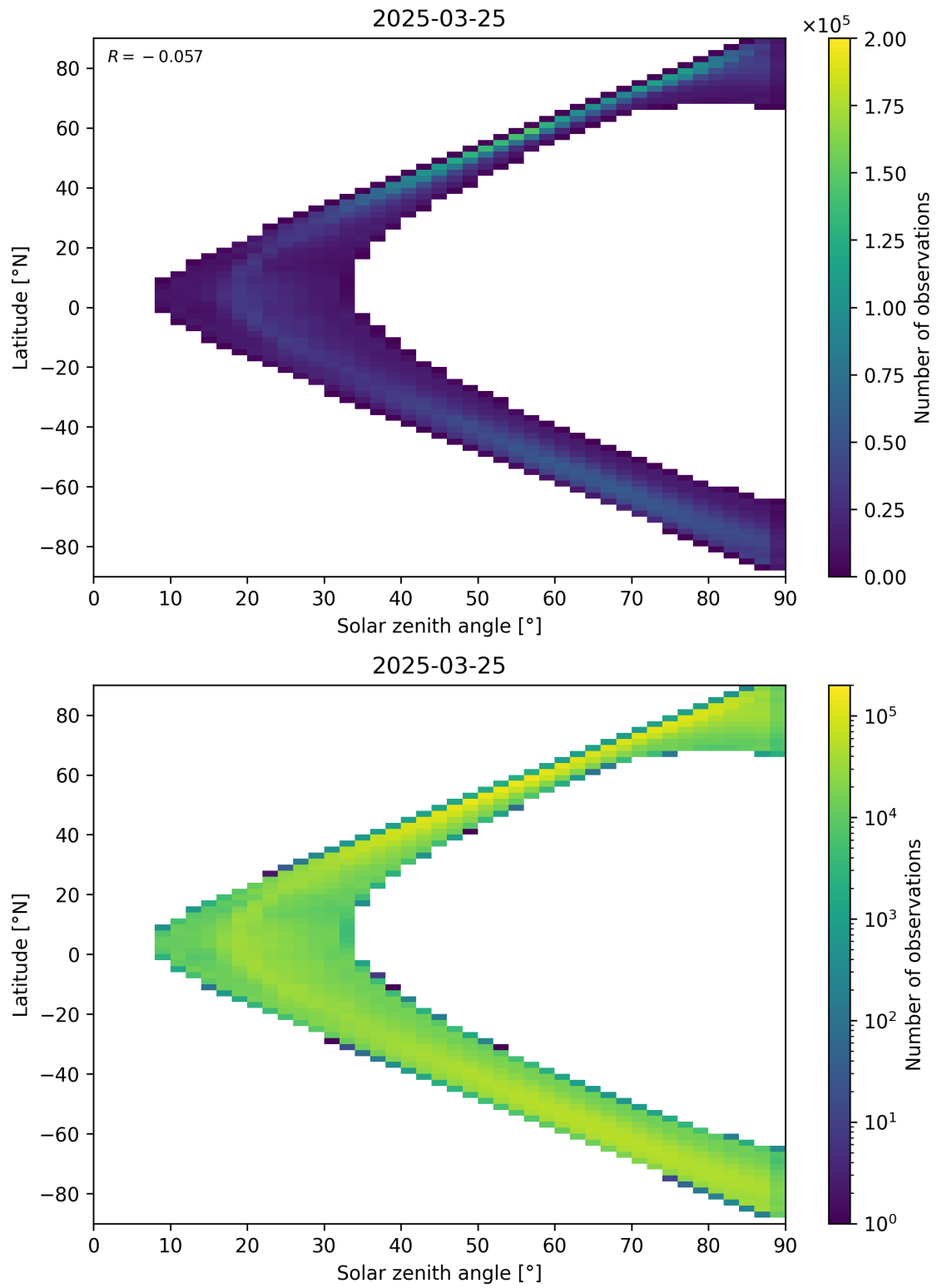
Figure 105: Scatter density plot of “Solar zenith angle” against “Latitude” for 2025-03-24 to 2025-03-26.
