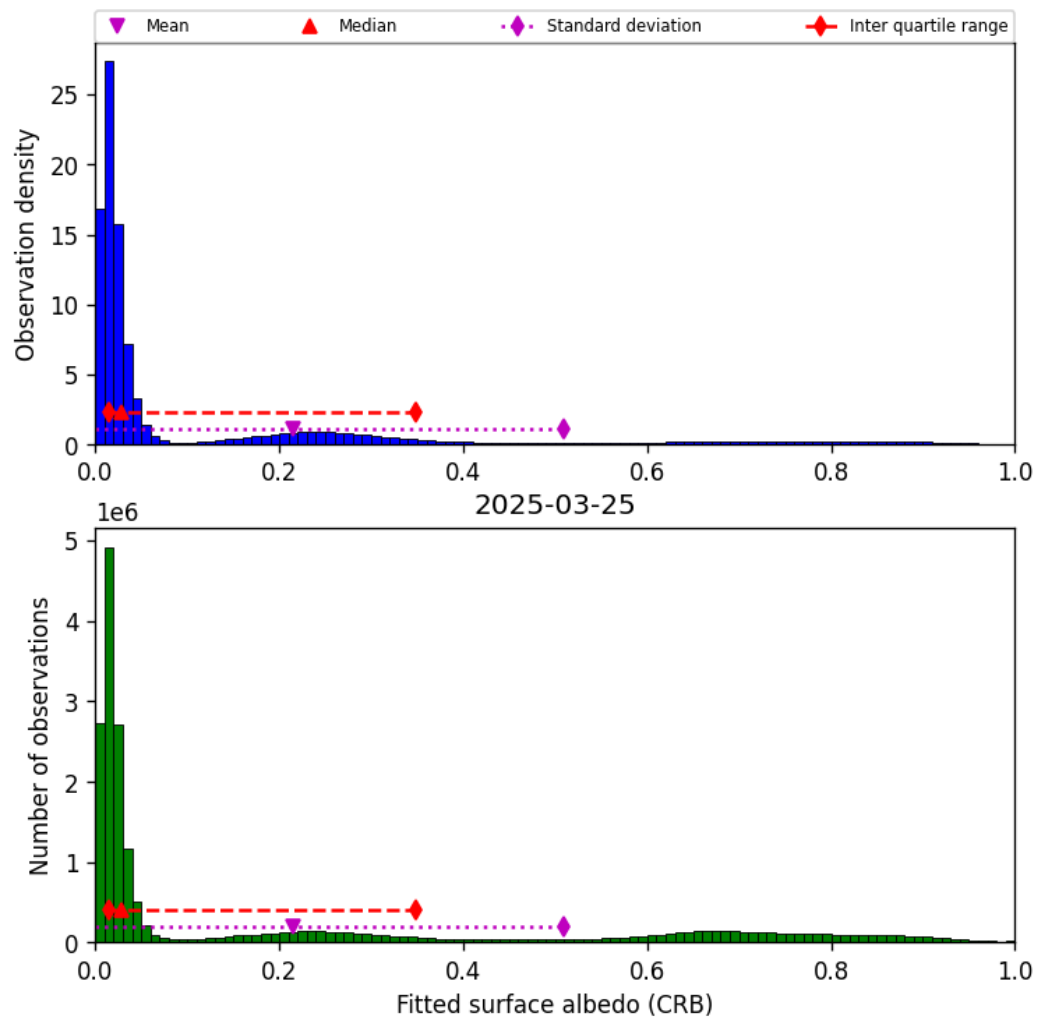
Figure 46: Histogram of “Fitted surface albedo (CRB)” for 2025-03-24 to 2025-03-26
