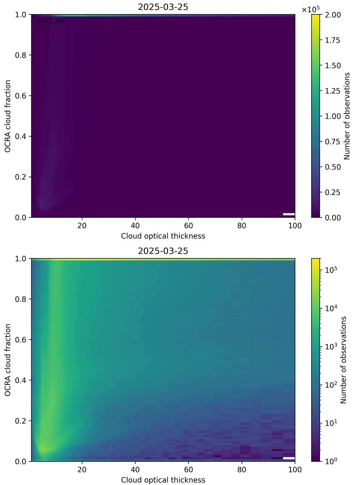
Figure 83: Scatter density plot of “Cloud optical thickness” against “OCRA cloud fraction” for 2025-03-24 to 2025-03-26.
