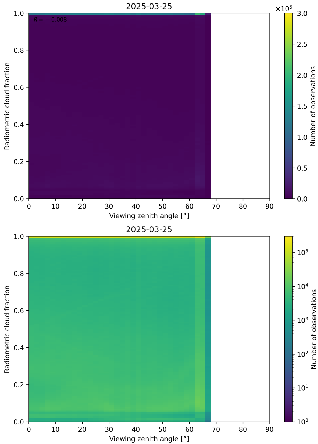
Figure 107: Scatter density plot of “Viewing zenith angle” against “Radiometric cloud fraction” for 2025-03-24 to 2025-03-26.
