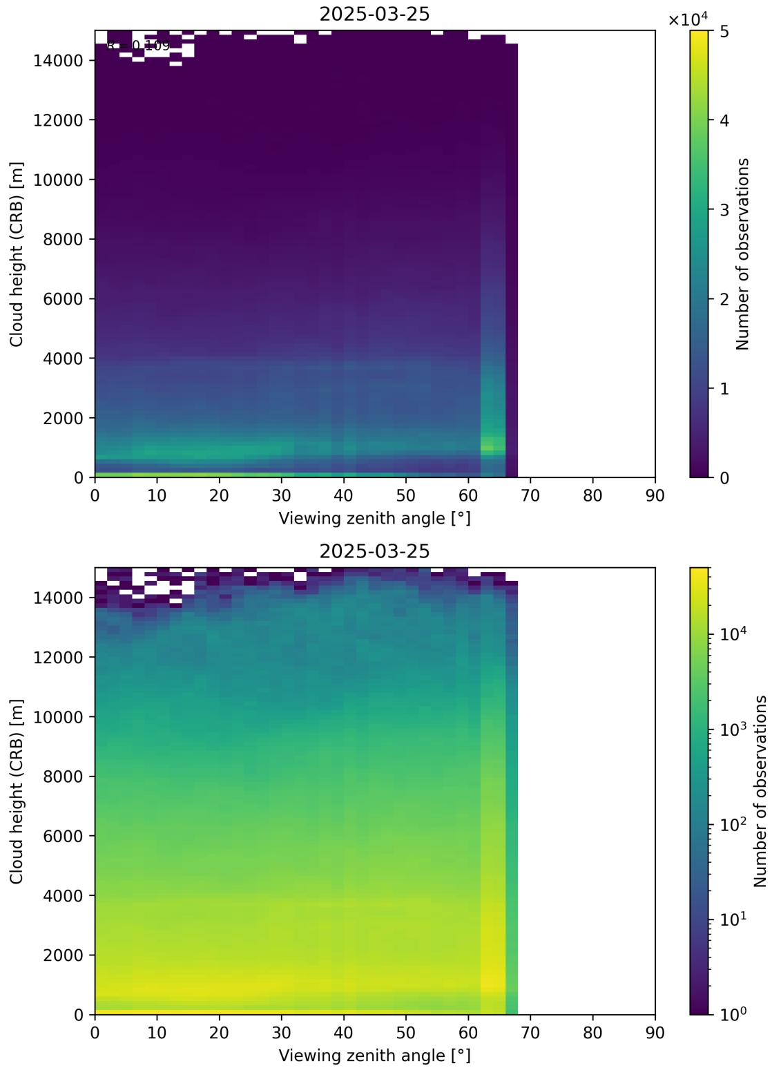
Figure 110: Scatter density plot of “Viewing zenith angle” against “Cloud height (CRB)” for 2025-03-24 to 2025-03-26.
