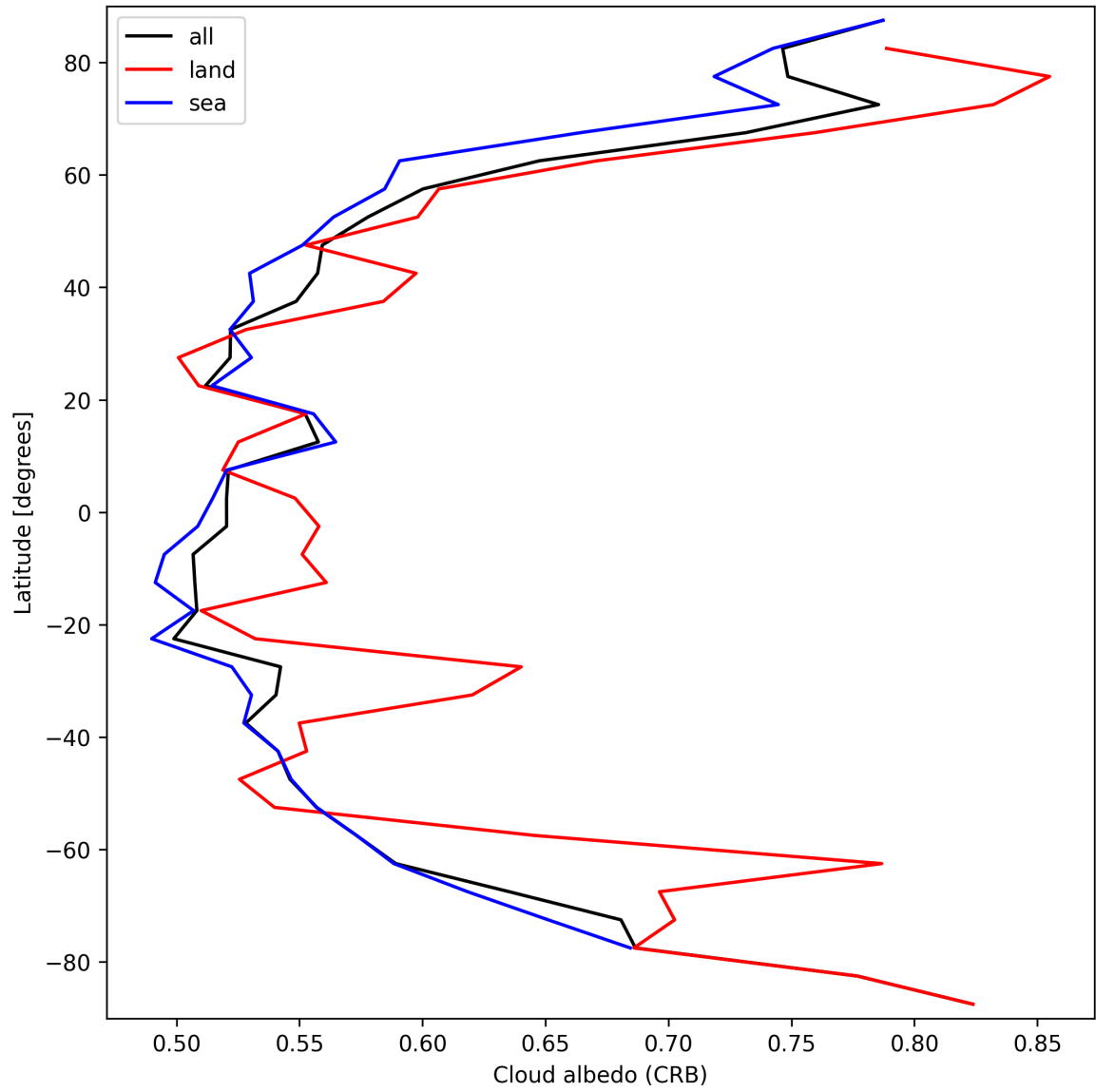
Figure 28: Zonal average of “Cloud albedo (CRB)” for 2025-03-24 to 2025-03-26.
