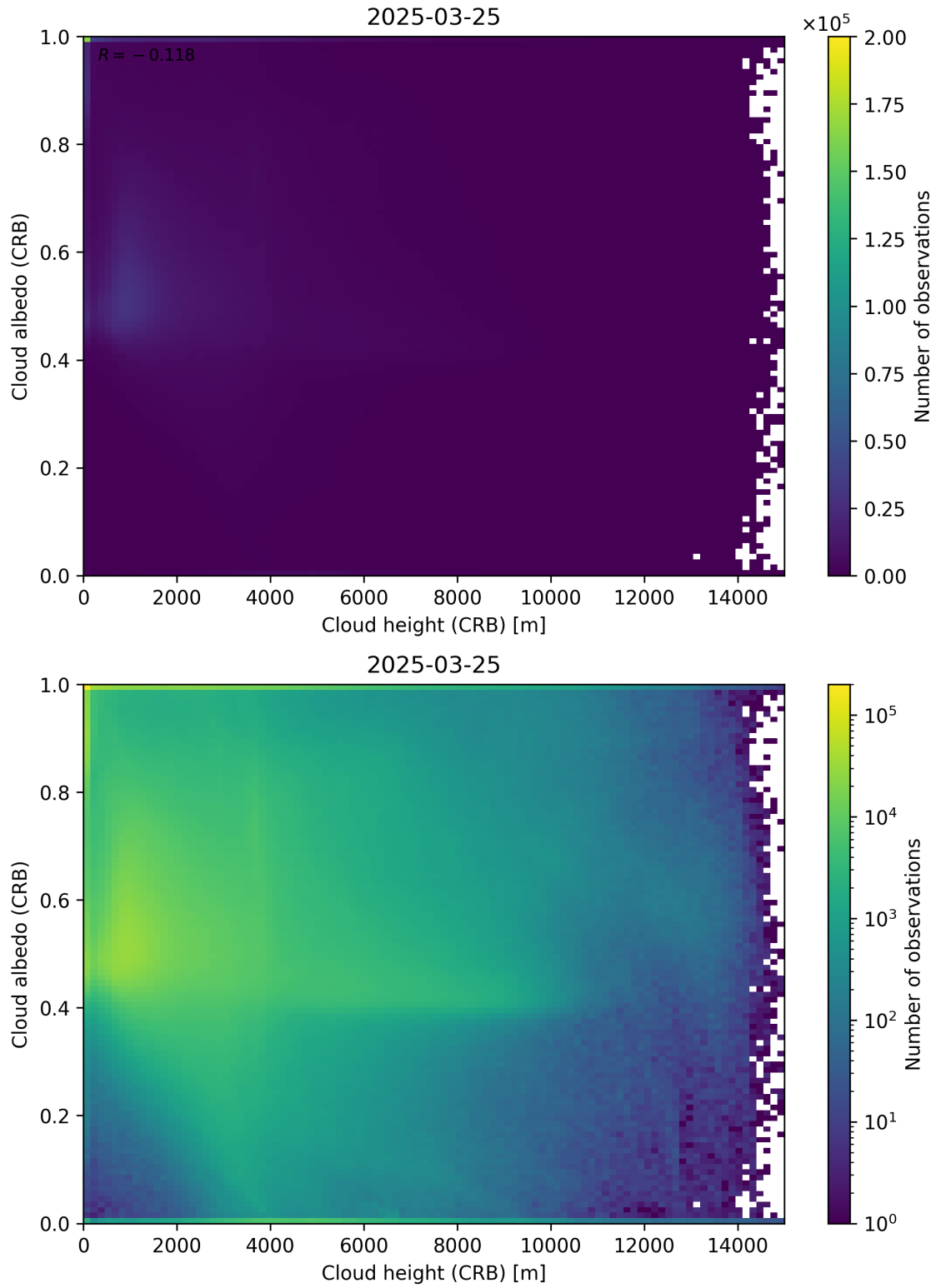
Figure 80: Scatter density plot of “Cloud height (CRB)” against “Cloud albedo (CRB)” for 2025-03-24 to 2025-03-26.
