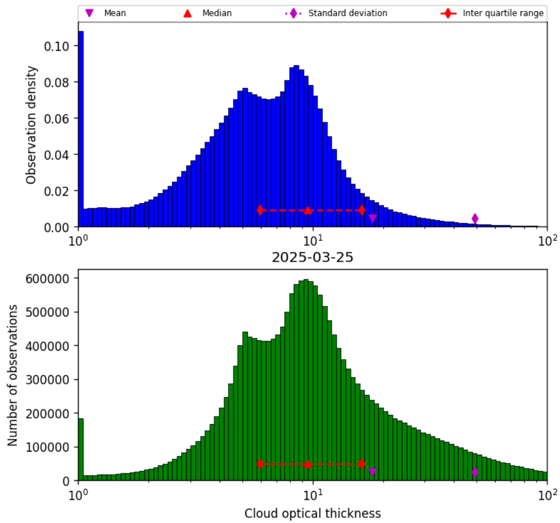
Figure 41: Histogram of “Cloud optical thickness” for 2025-03-24 to 2025-03-26
