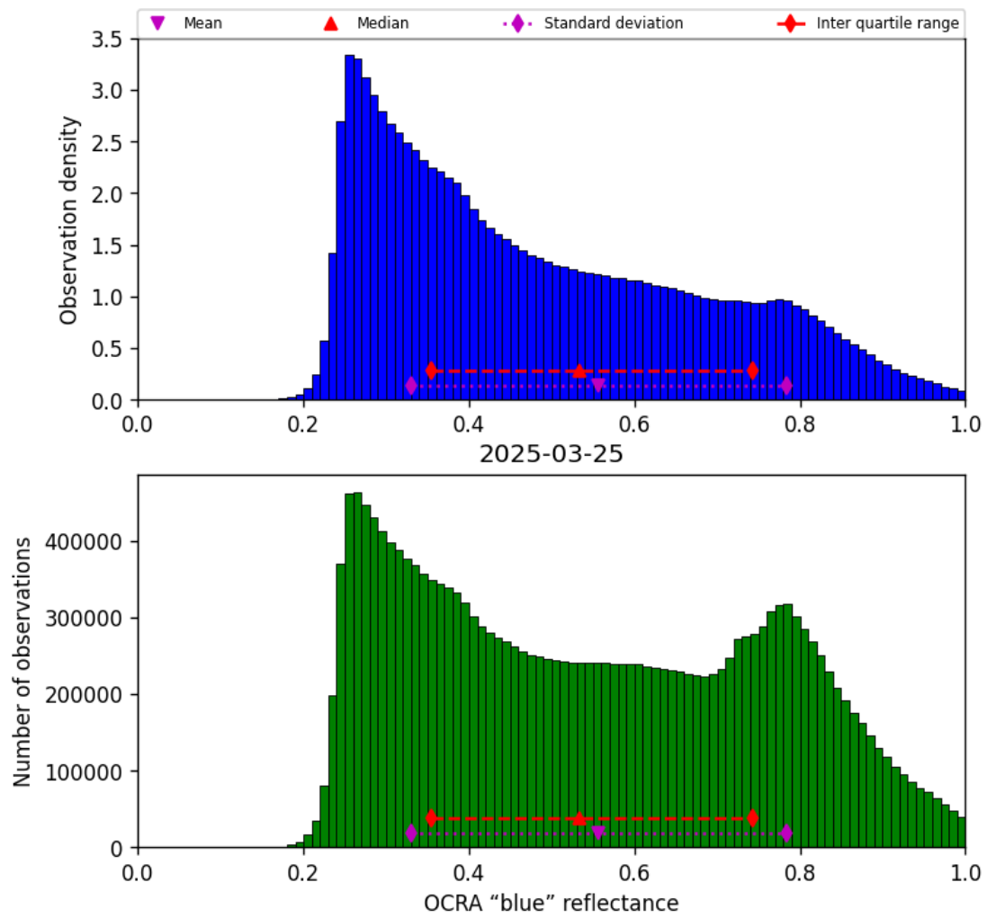
Figure 51: Histogram of “OCRA “blue” reflectance” for 2025-03-24 to 2025-03-26
