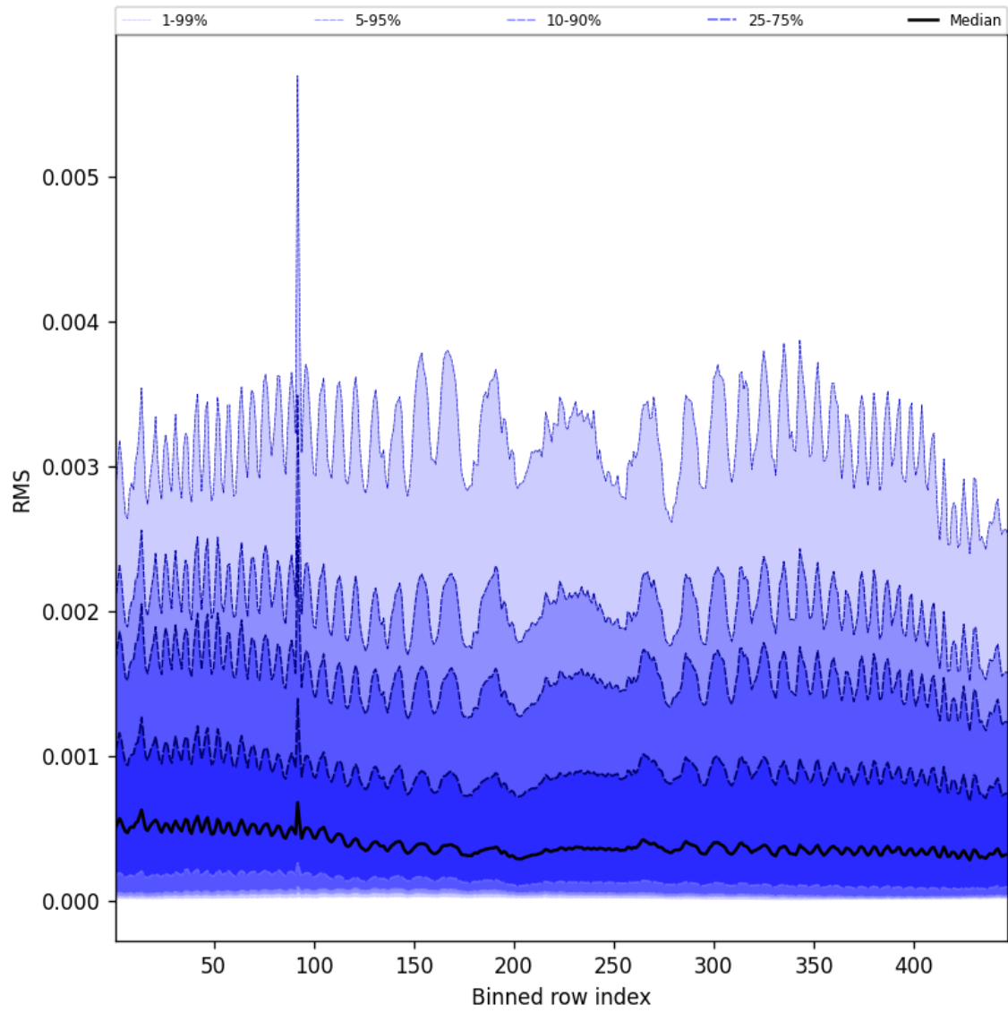
Figure 63: Along track statistics of “RMS” for 2025-03-24 to 2025-03-26
