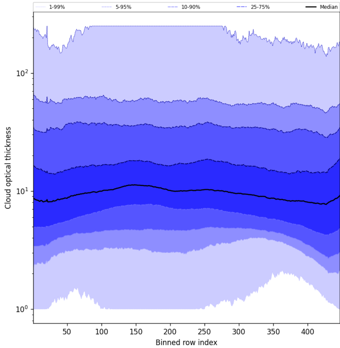
Figure 57: Along track statistics of “Cloud optical thickness” for 2025-03-24 to 2025-03-26
