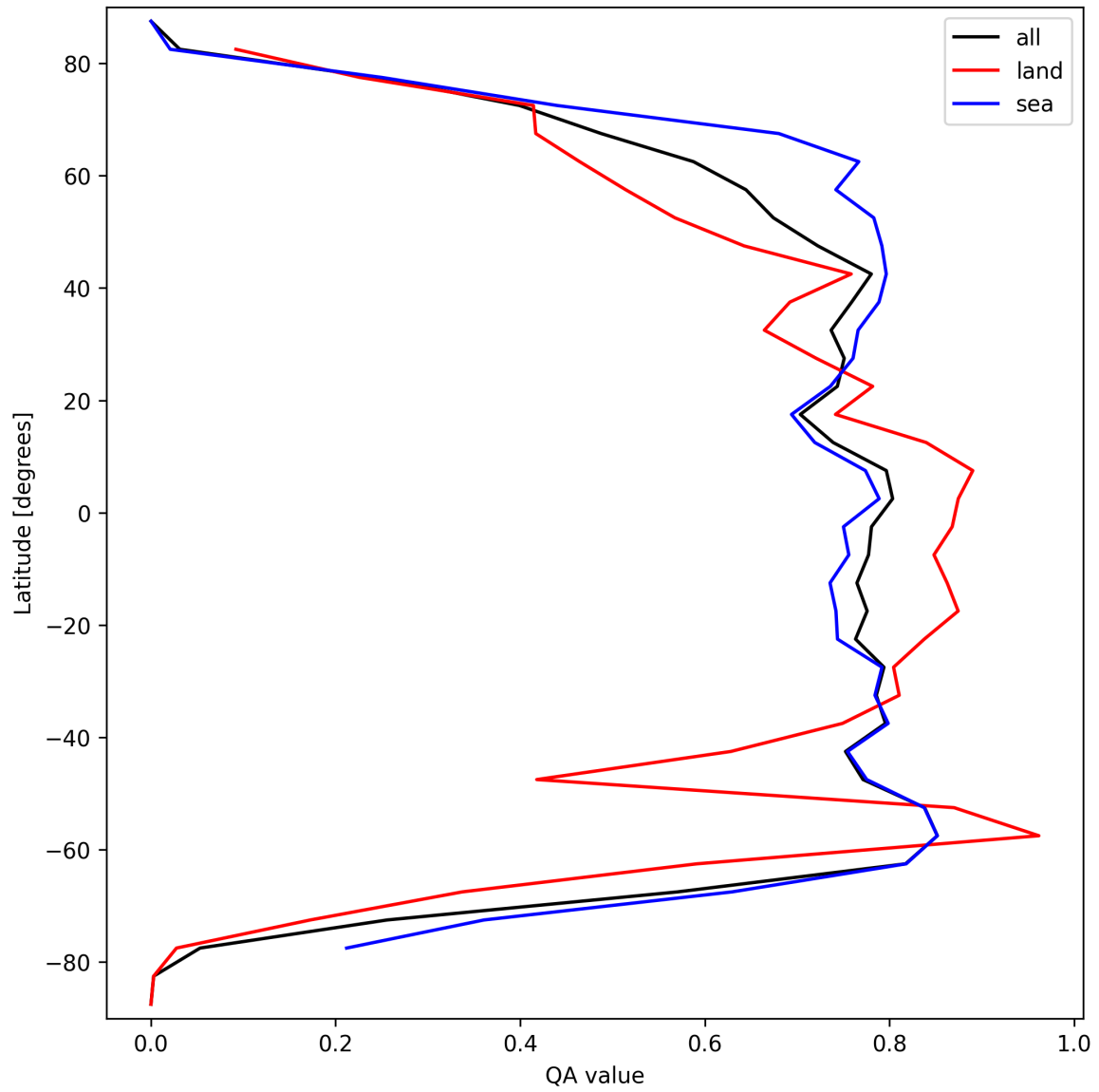
Figure 22: Zonal average of “QA value” for 2025-03-24 to 2025-03-26.
