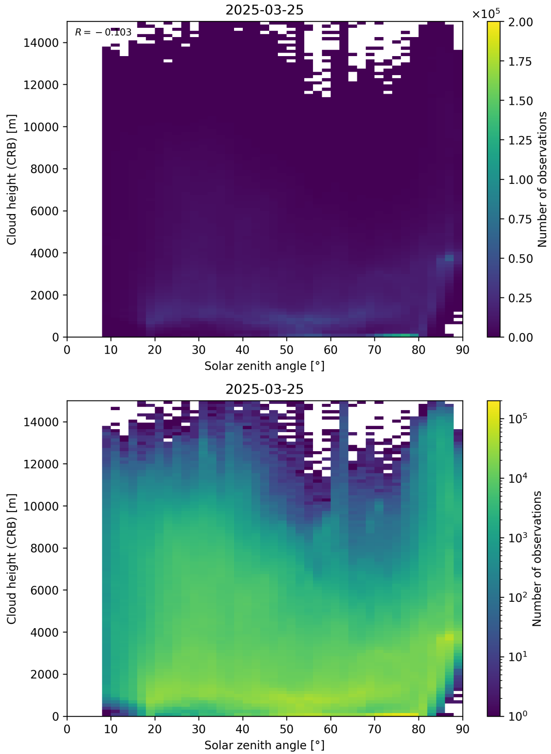
Figure 102: Scatter density plot of “Solar zenith angle” against “Cloud height (CRB)” for 2025-03-24 to 2025-03-26.
