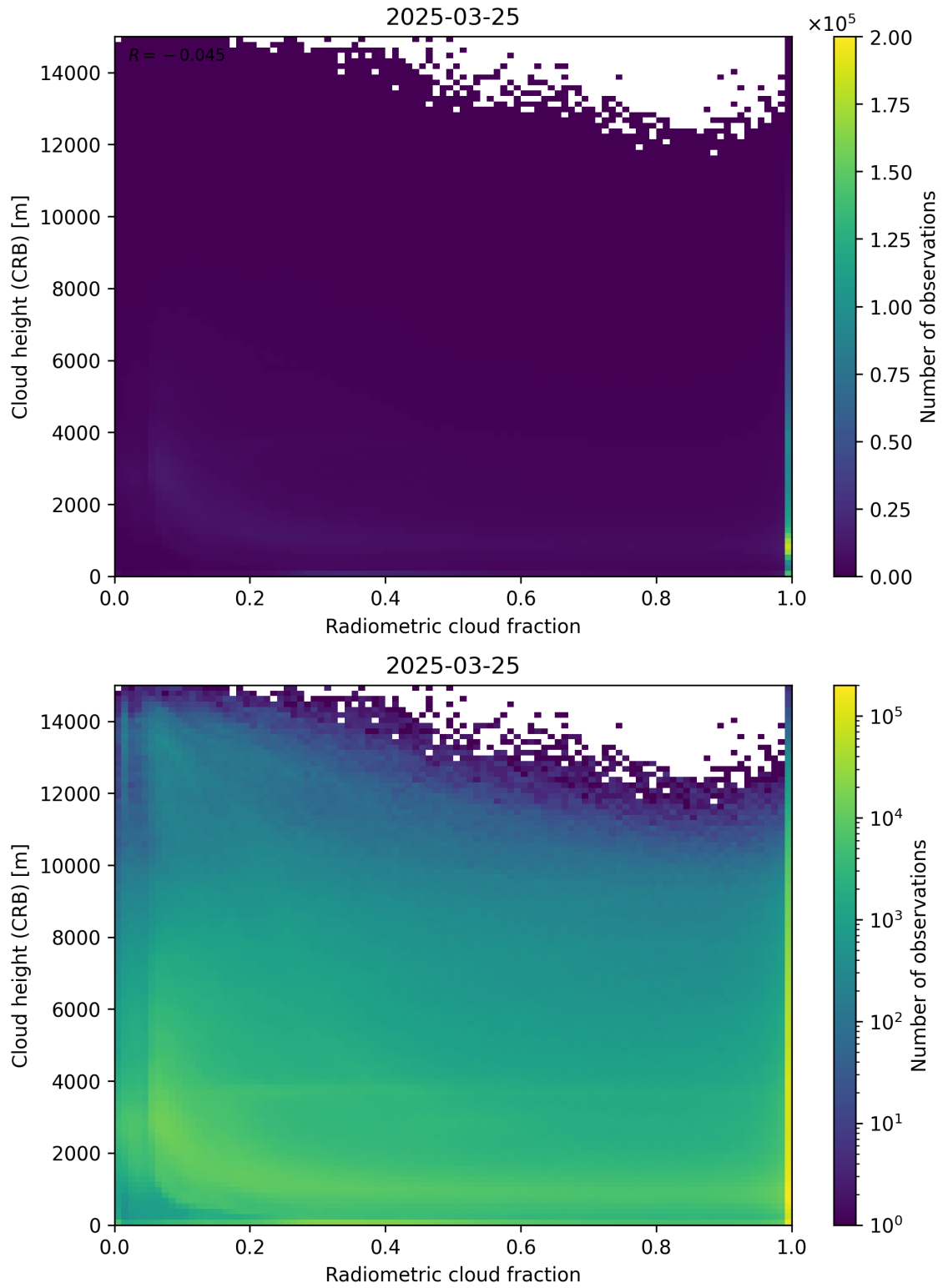
Figure 74: Scatter density plot of “Radiometric cloud fraction” against “Cloud height (CRB)” for 2025-03-24 to 2025-03-26.
