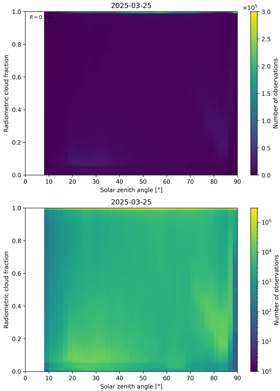
Figure 99: Scatter density plot of “Solar zenith angle” against “Radiometric cloud fraction” for 2025-03-24 to 2025-03-26.
