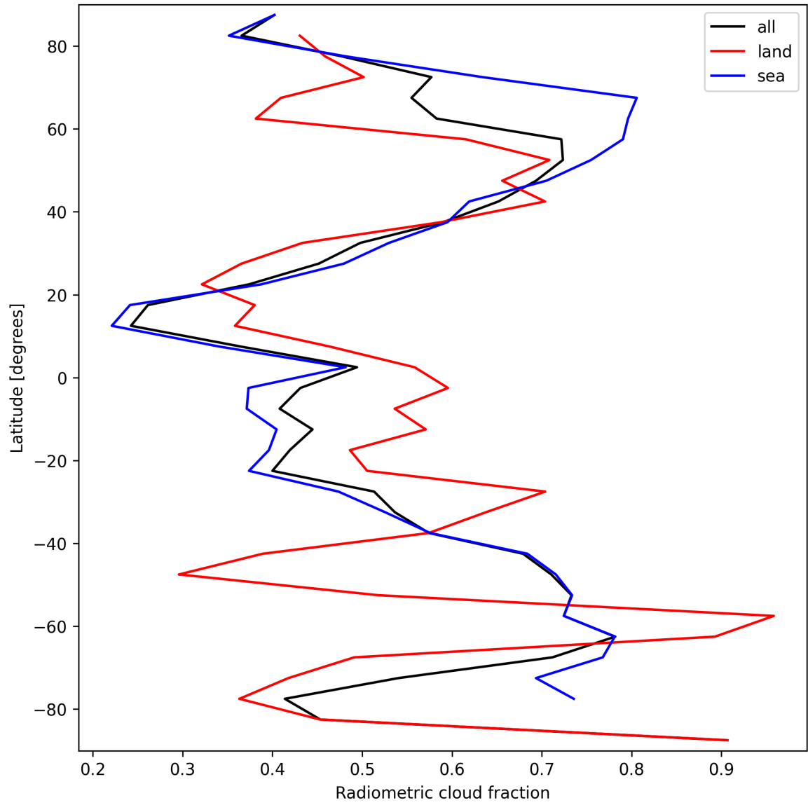
Figure 23: Zonal average of “Radiometric cloud fraction” for 2025-03-24 to 2025-03-26.
