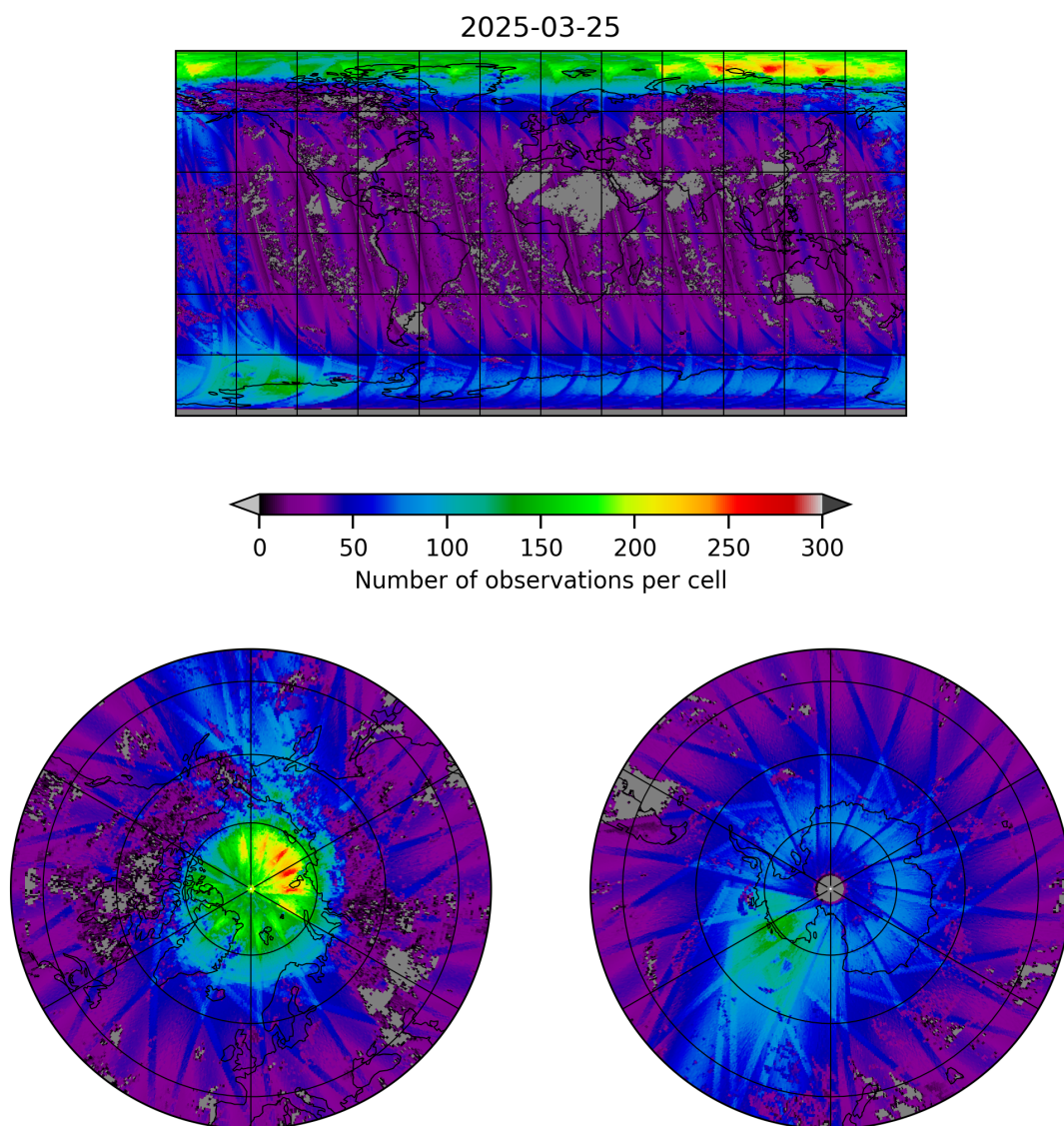
Figure 21: Map of the number of observations for 2025-03-24 to 2025-03-26
