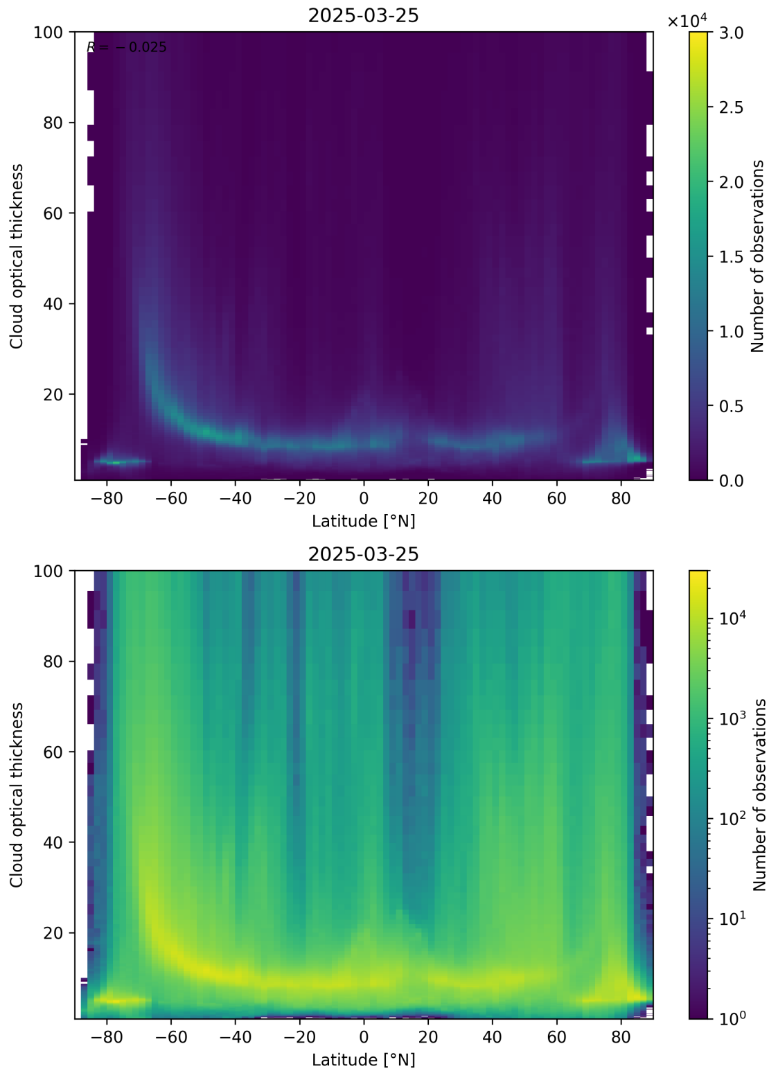
Figure 96: Scatter density plot of “Latitude” against “Cloud optical thickness” for 2025-03-24 to 2025-03-26.
