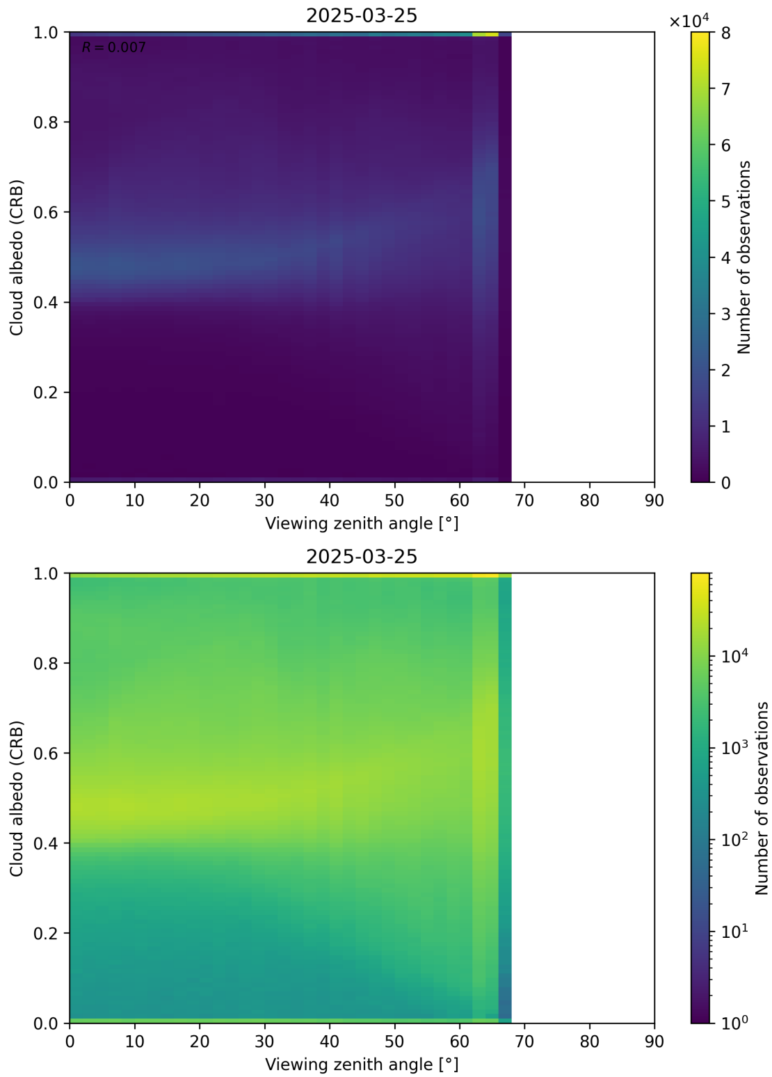
Figure 106: Scatter density plot of “Viewing zenith angle” against “Cloud albedo (CRB)” for 2025-03-24 to 2025-03-26.
