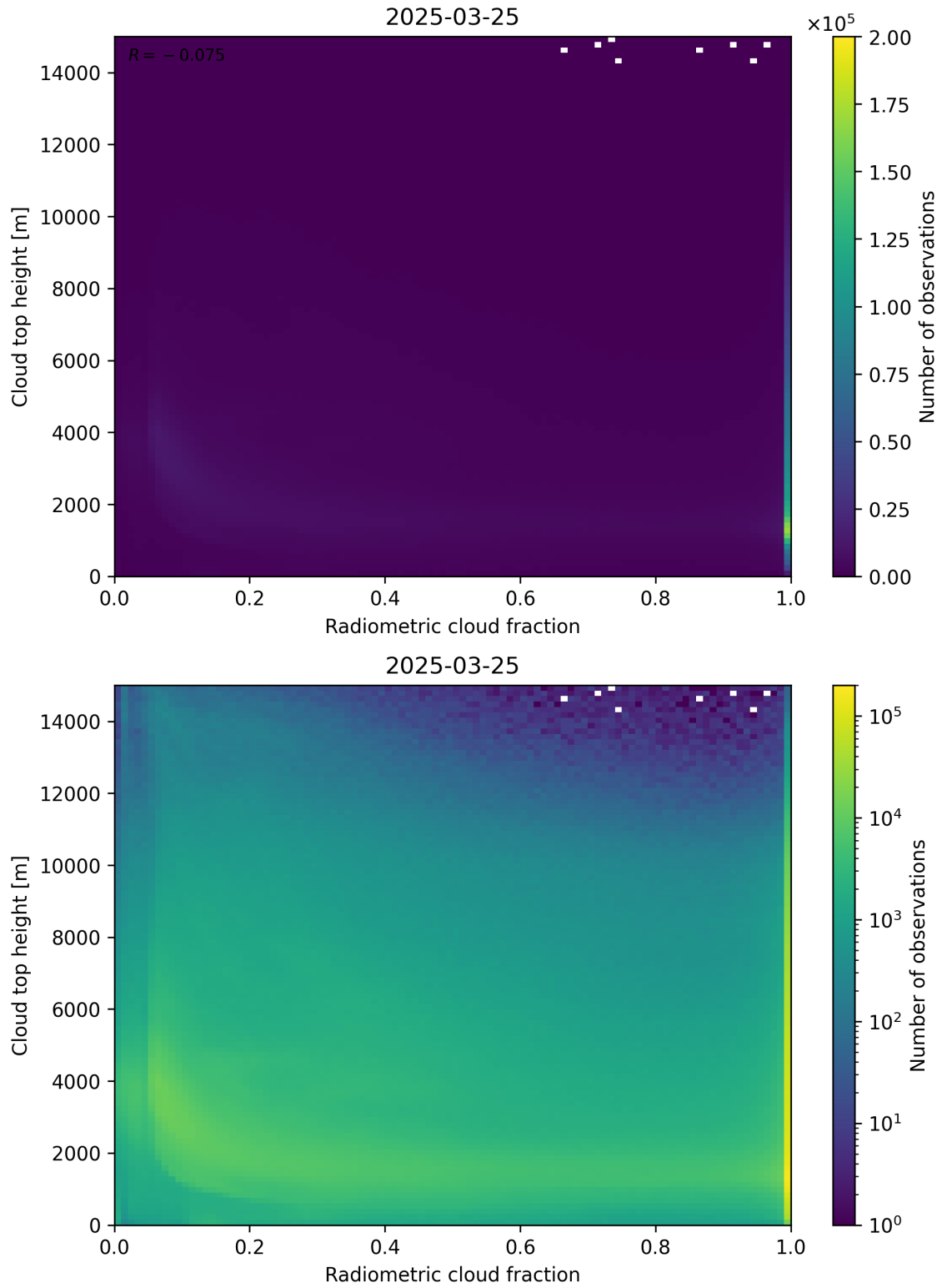
Figure 76: Scatter density plot of “Radiometric cloud fraction” against “Cloud top height” for 2025-03-24 to 2025-03-26.
