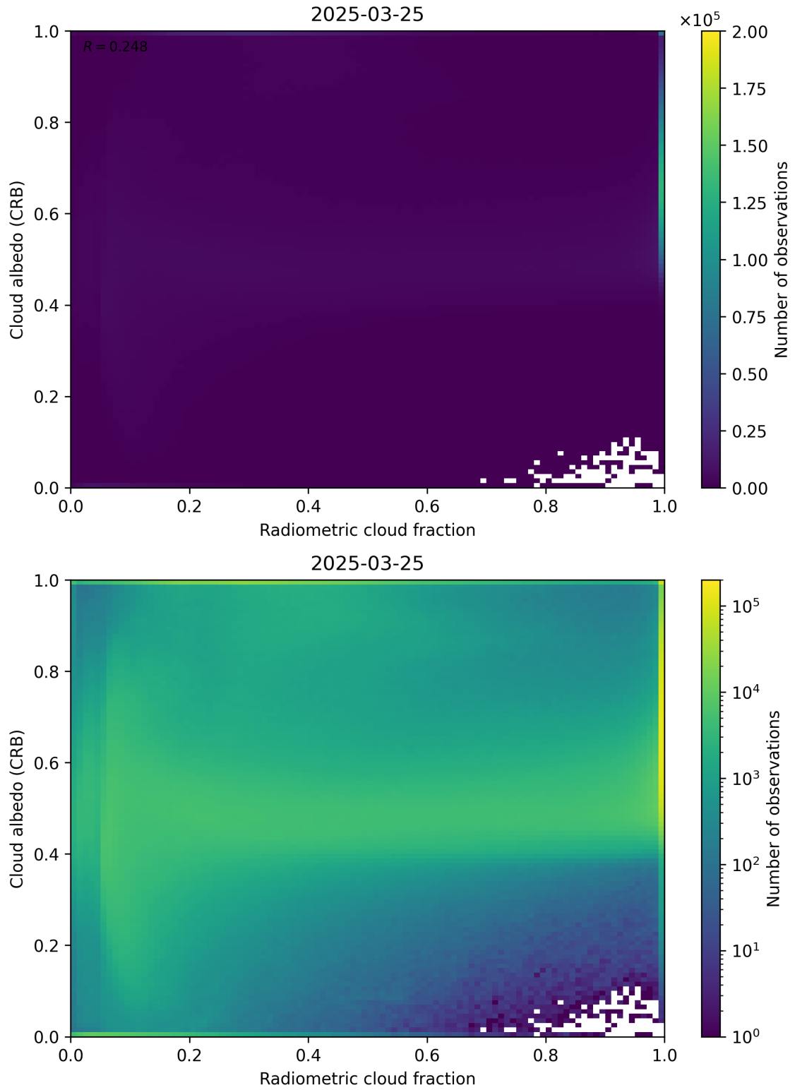
Figure 71: Scatter density plot of “Radiometric cloud fraction” against “Cloud albedo (CRB)” for 2025-03-24 to 2025-03-26.
