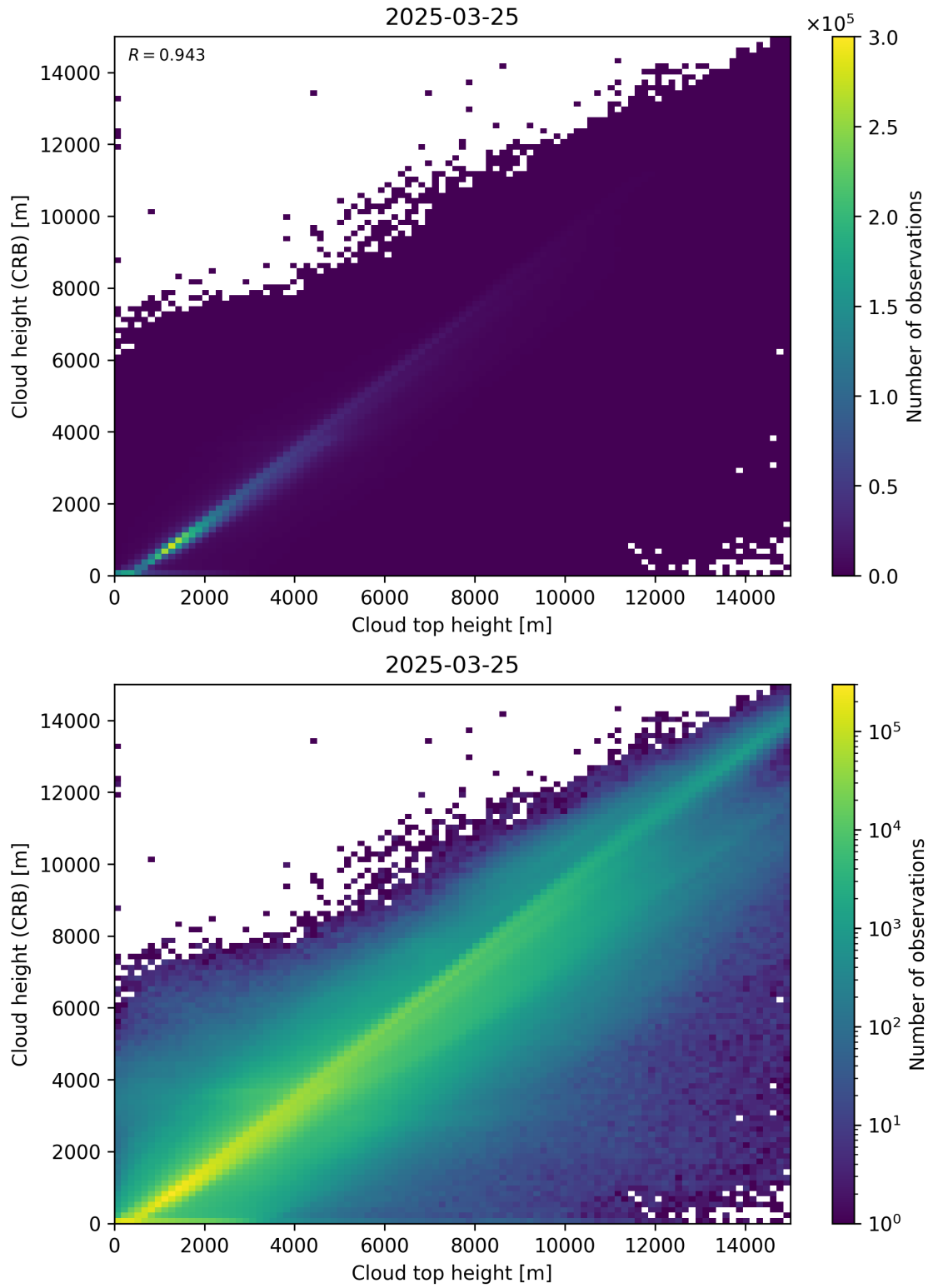
Figure 89: Scatter density plot of “Cloud top height” against “Cloud height (CRB)” for 2025-03-24 to 2025-03-26.
