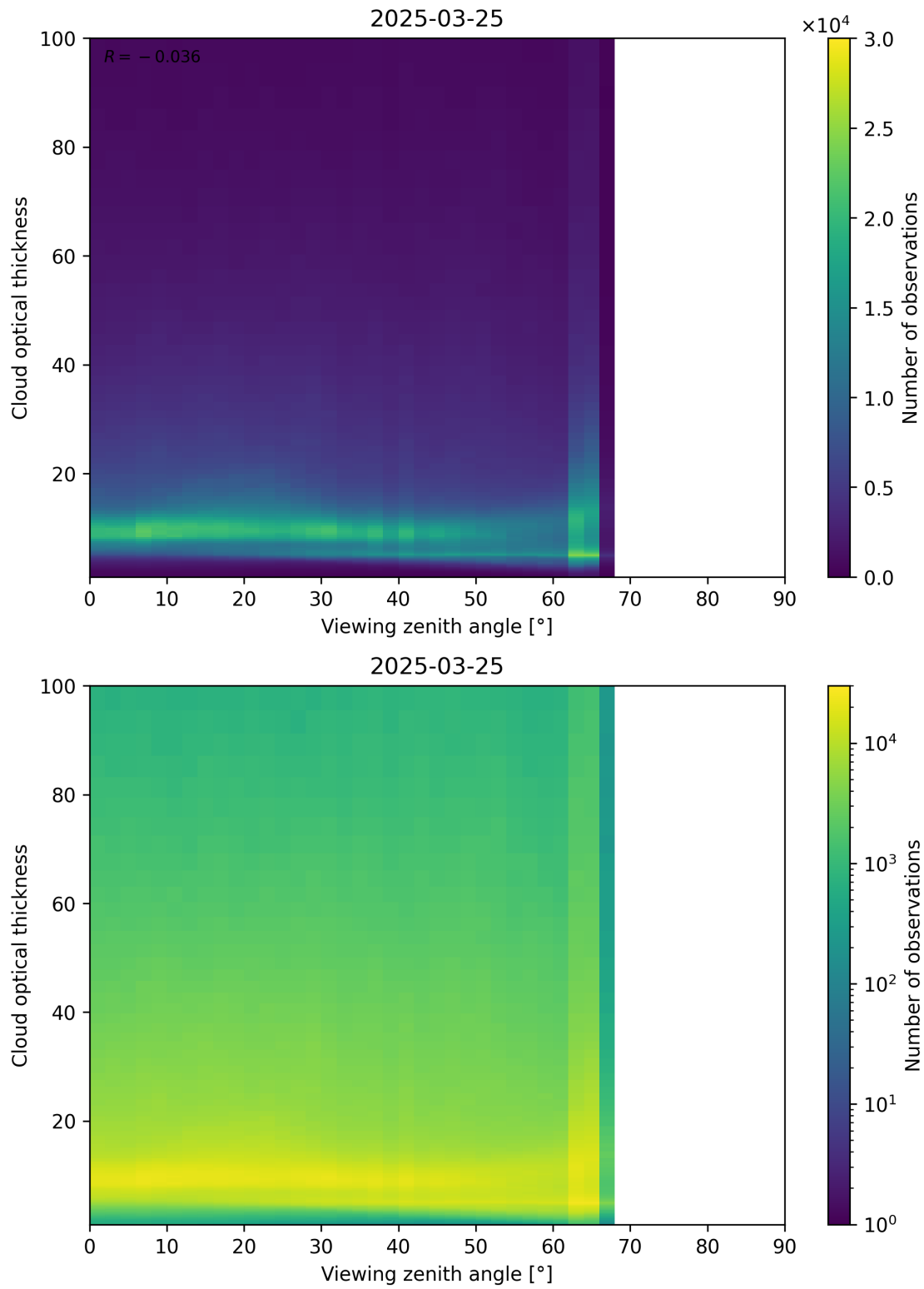
Figure 111: Scatter density plot of “Viewing zenith angle” against “Cloud optical thickness” for 2025-03-24 to 2025-03-26.
