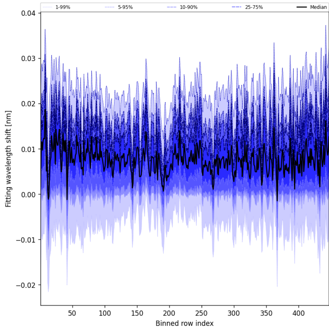
Figure 65: Along track statistics of “Fitting wavelength shift” for 2025-03-24 to 2025-03-26
