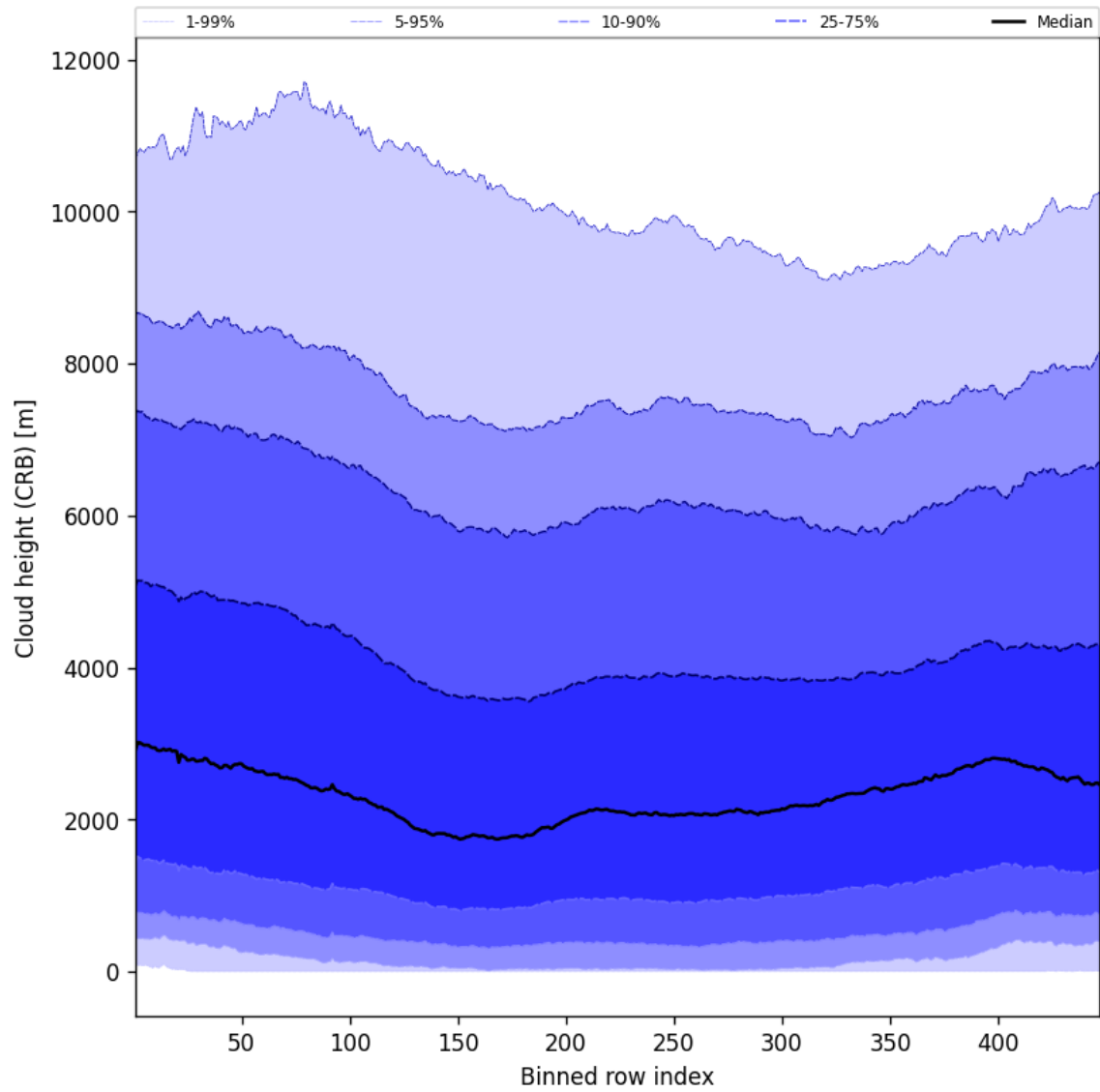
Figure 59: Along track statistics of “Cloud height (CRB)” for 2025-03-24 to 2025-03-26
