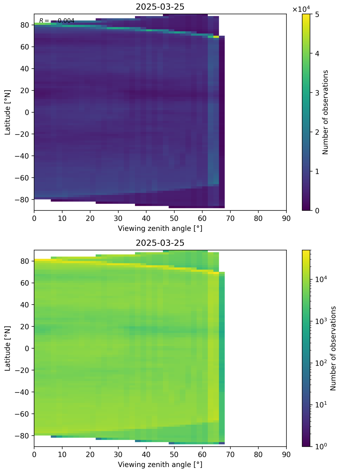
Figure 113: Scatter density plot of “Viewing zenith angle” against “Latitude” for 2025-03-24 to 2025-03-26.
