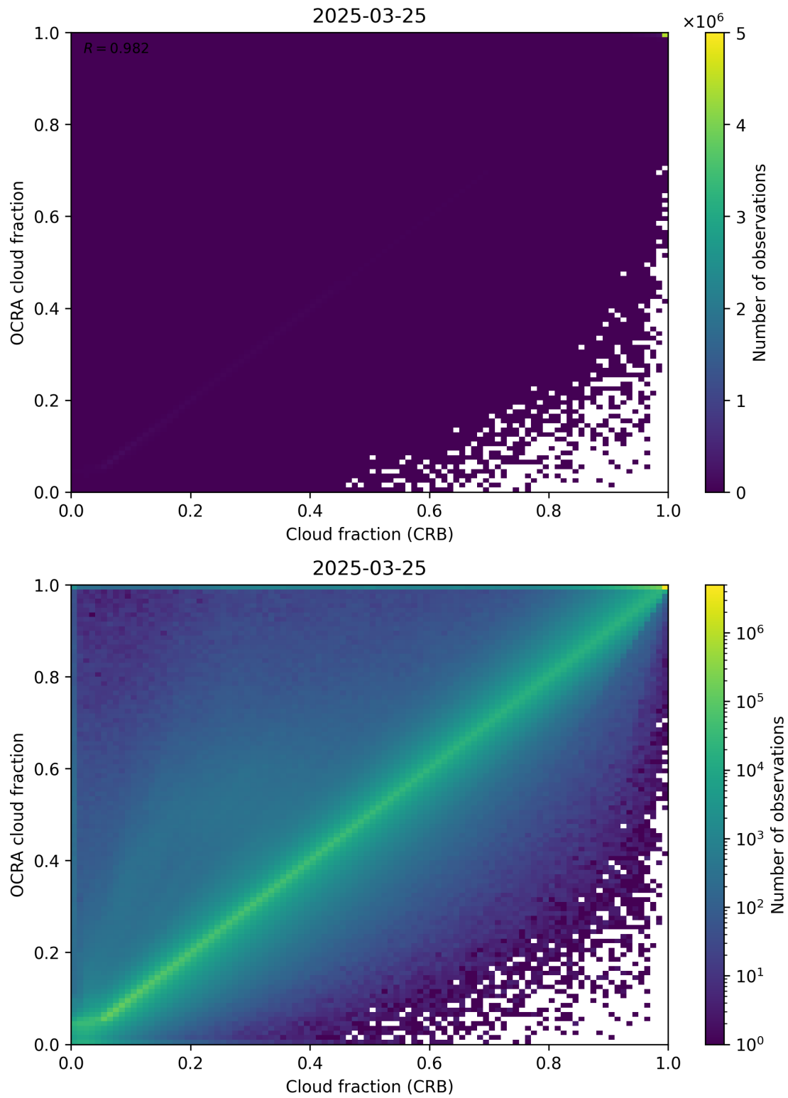
Figure 78: Scatter density plot of “Cloud fraction (CRB)” against “OCRA cloud fraction” for 2025-03-24 to 2025-03-26.
