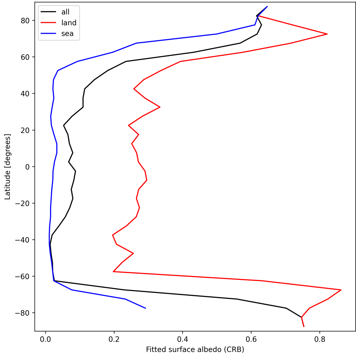
Figure 30: Zonal average of “Fitted surface albedo (CRB)” for 2025-03-24 to 2025-03-26.
