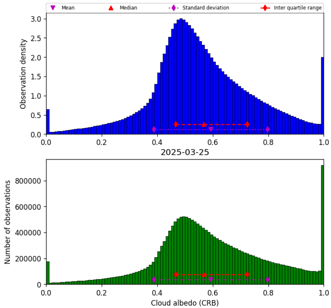
Figure 44: Histogram of “Cloud albedo (CRB)” for 2025-03-24 to 2025-03-26
