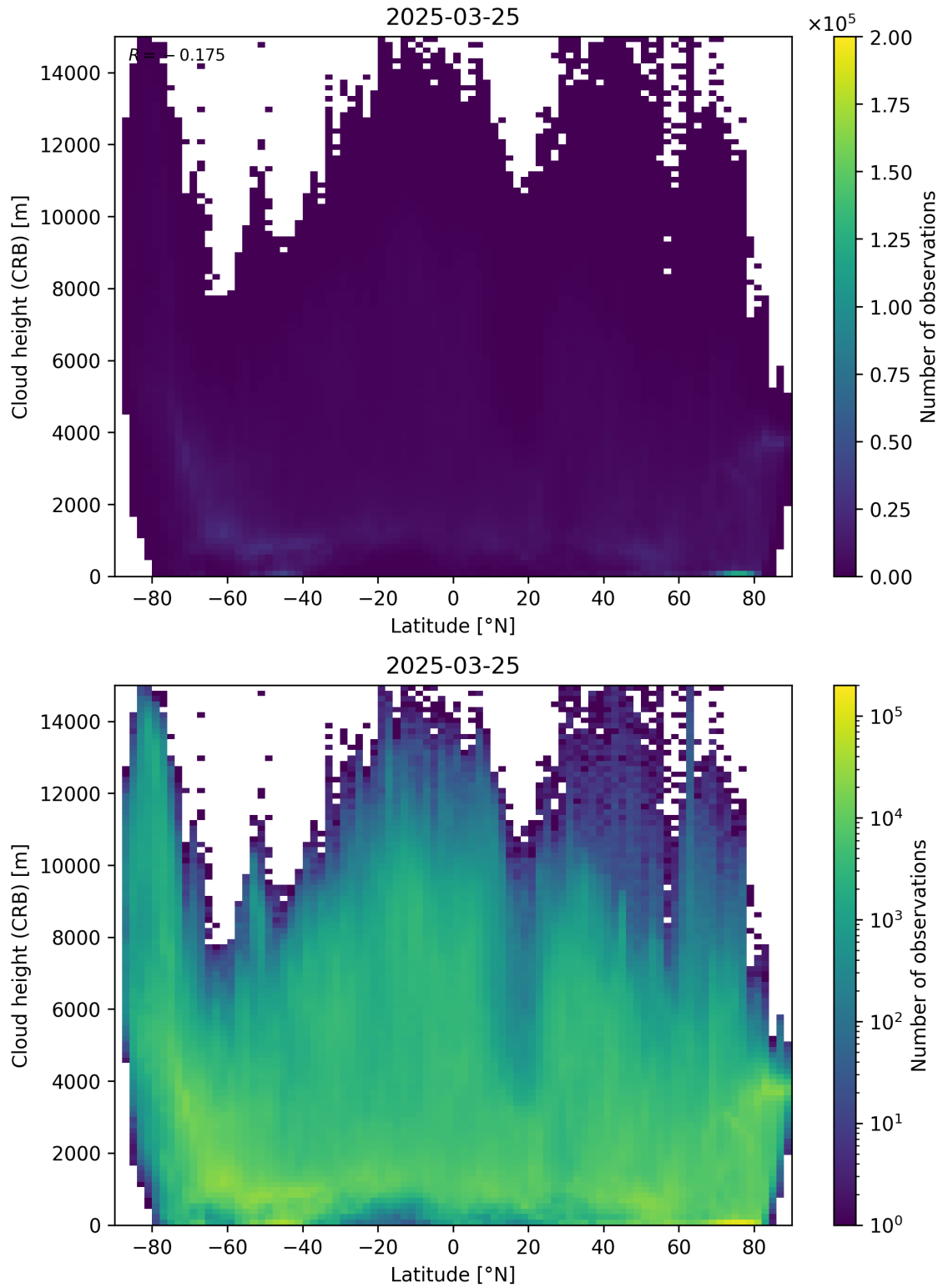
Figure 95: Scatter density plot of “Latitude” against “Cloud height (CRB)” for 2025-03-24 to 2025-03-26.
