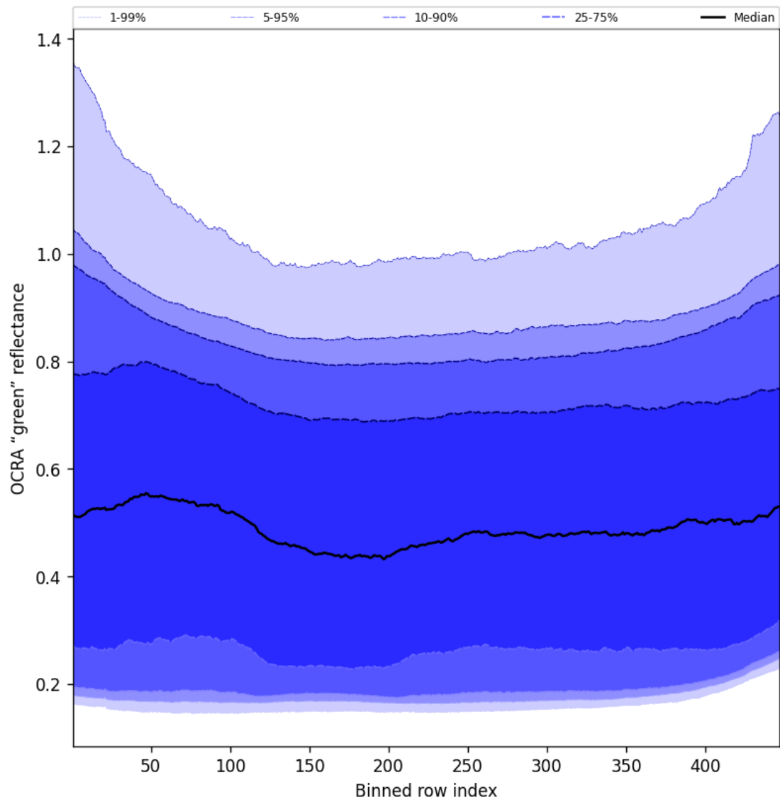
Figure 68: Along track statistics of “OCRA “green” reflectance” for 2025-03-24 to 2025-03-26
