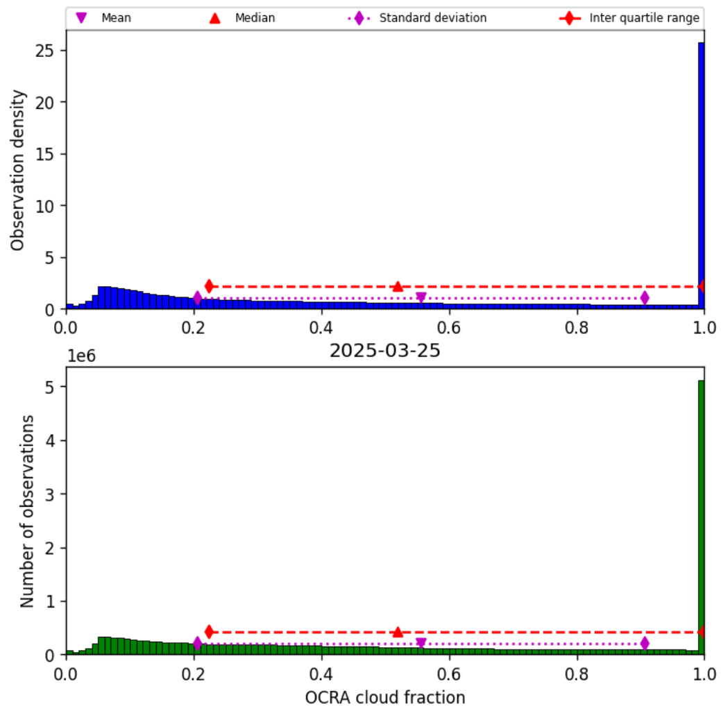
Figure 50: Histogram of “OCRA cloud fraction” for 2025-03-24 to 2025-03-26
