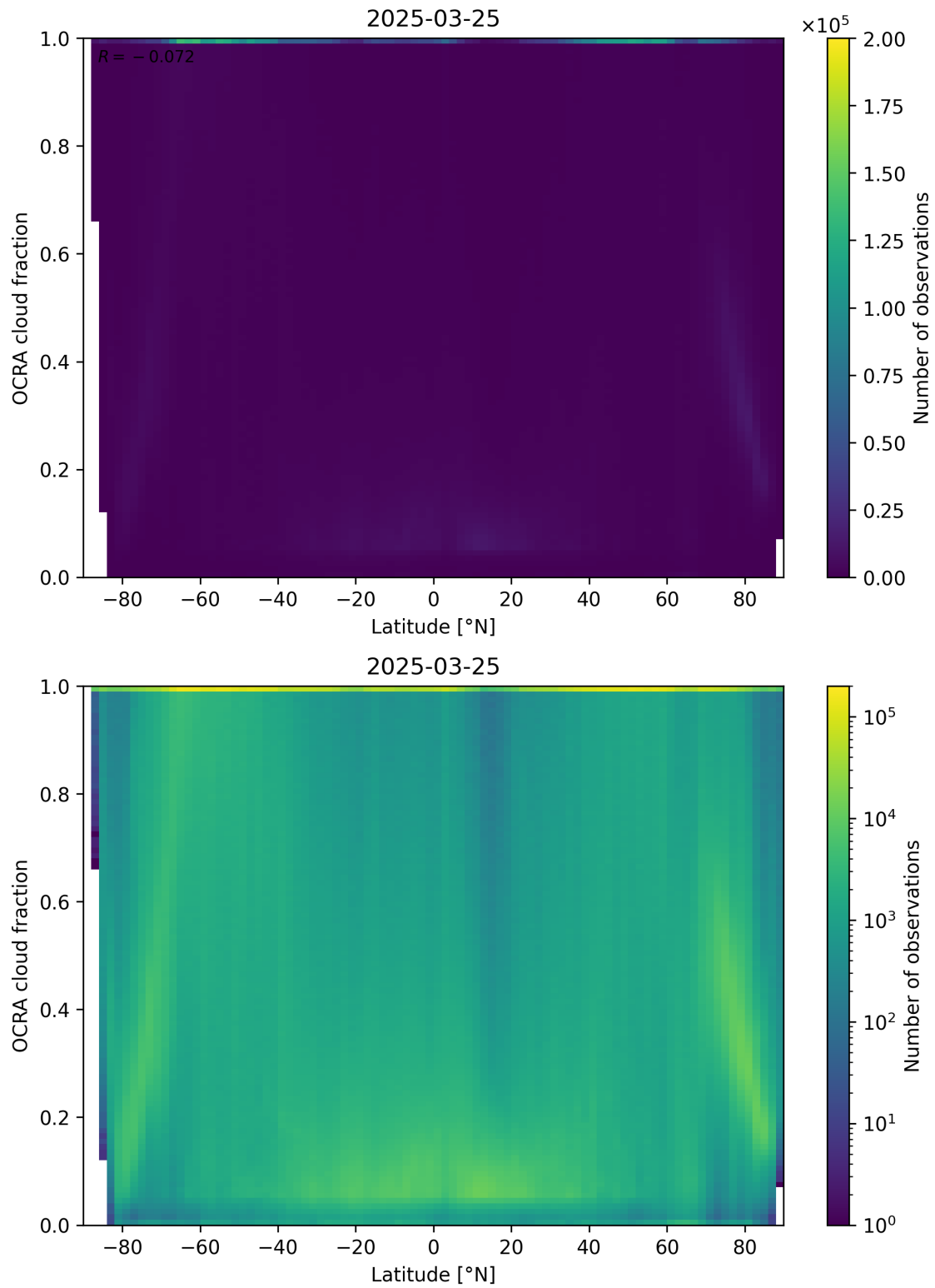
Figure 93: Scatter density plot of “Latitude” against “OCRA cloud fraction” for 2025-03-24 to 2025-03-26.
