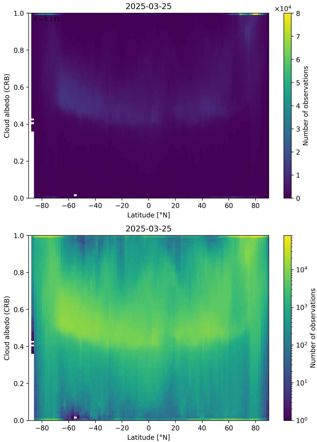
Figure 91: Scatter density plot of “Latitude” against “Cloud albedo (CRB)” for 2025-03-24 to 2025-03-26.
