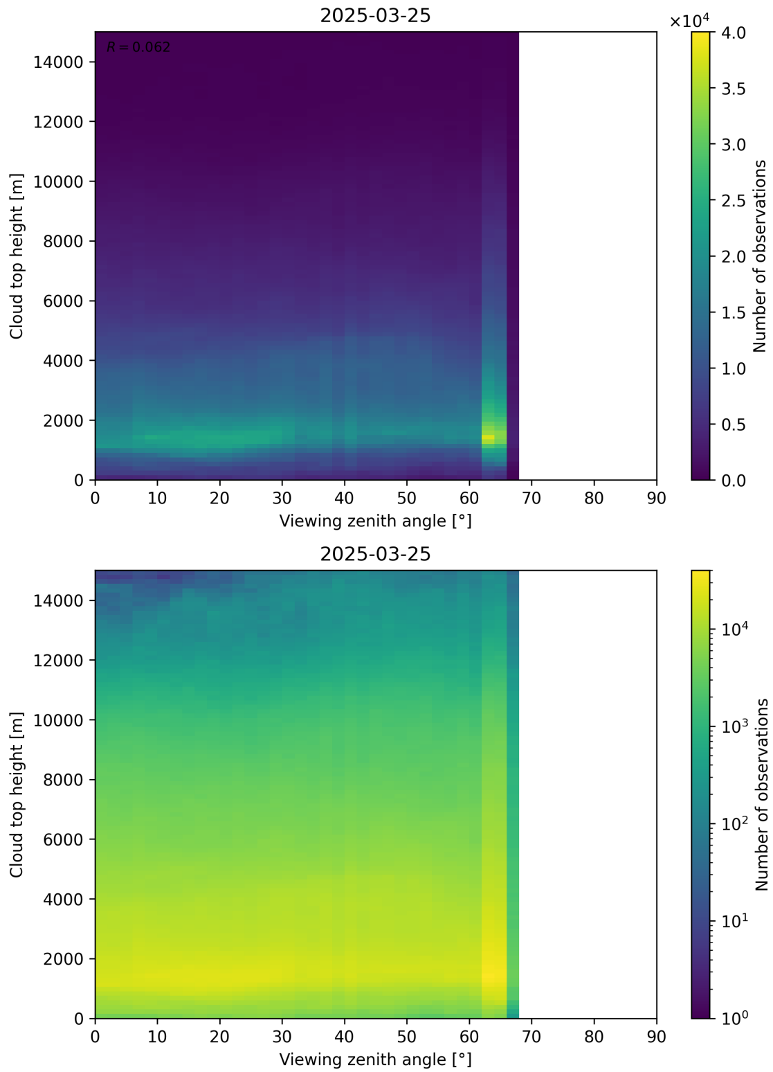
Figure 112: Scatter density plot of “Viewing zenith angle” against “Cloud top height” for 2025-03-24 to 2025-03-26.
