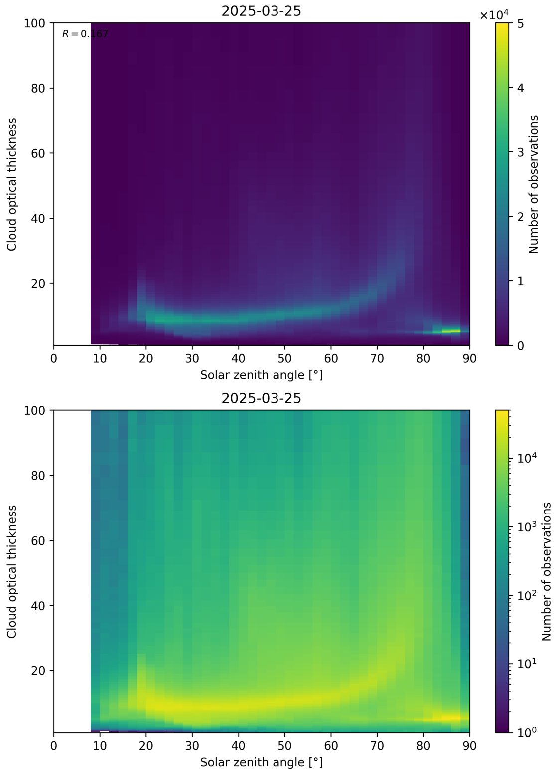
Figure 103: Scatter density plot of “Solar zenith angle” against “Cloud optical thickness” for 2025-03-24 to 2025-03-26.
