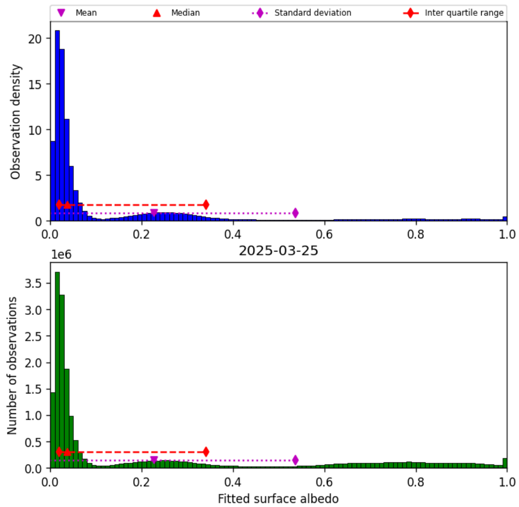
Figure 45: Histogram of “Fitted surface albedo” for 2025-03-24 to 2025-03-26
