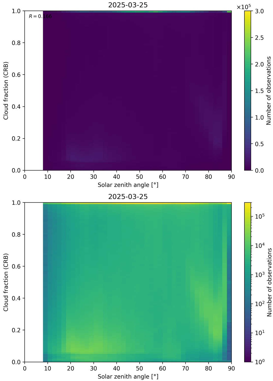
Figure 101: Scatter density plot of “Solar zenith angle” against “Cloud fraction (CRB)” for 2025-03-24 to 2025-03-26.
