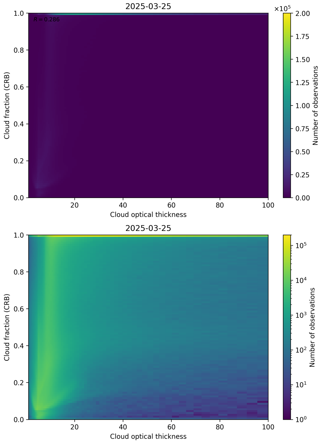
Figure 84: Scatter density plot of “Cloud optical thickness” against “Cloud fraction (CRB)” for 2025-03-24 to 2025-03-26.
