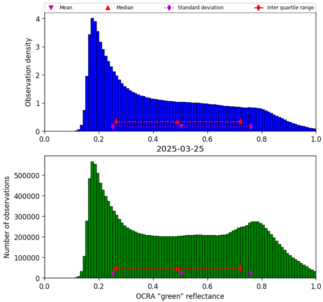
Figure 52: Histogram of “OCRA “green” reflectance” for 2025-03-24 to 2025-03-26
