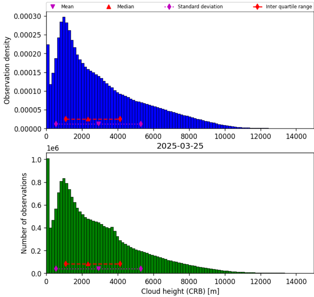
Figure 43: Histogram of “Cloud height (CRB)” for 2025-03-24 to 2025-03-26
