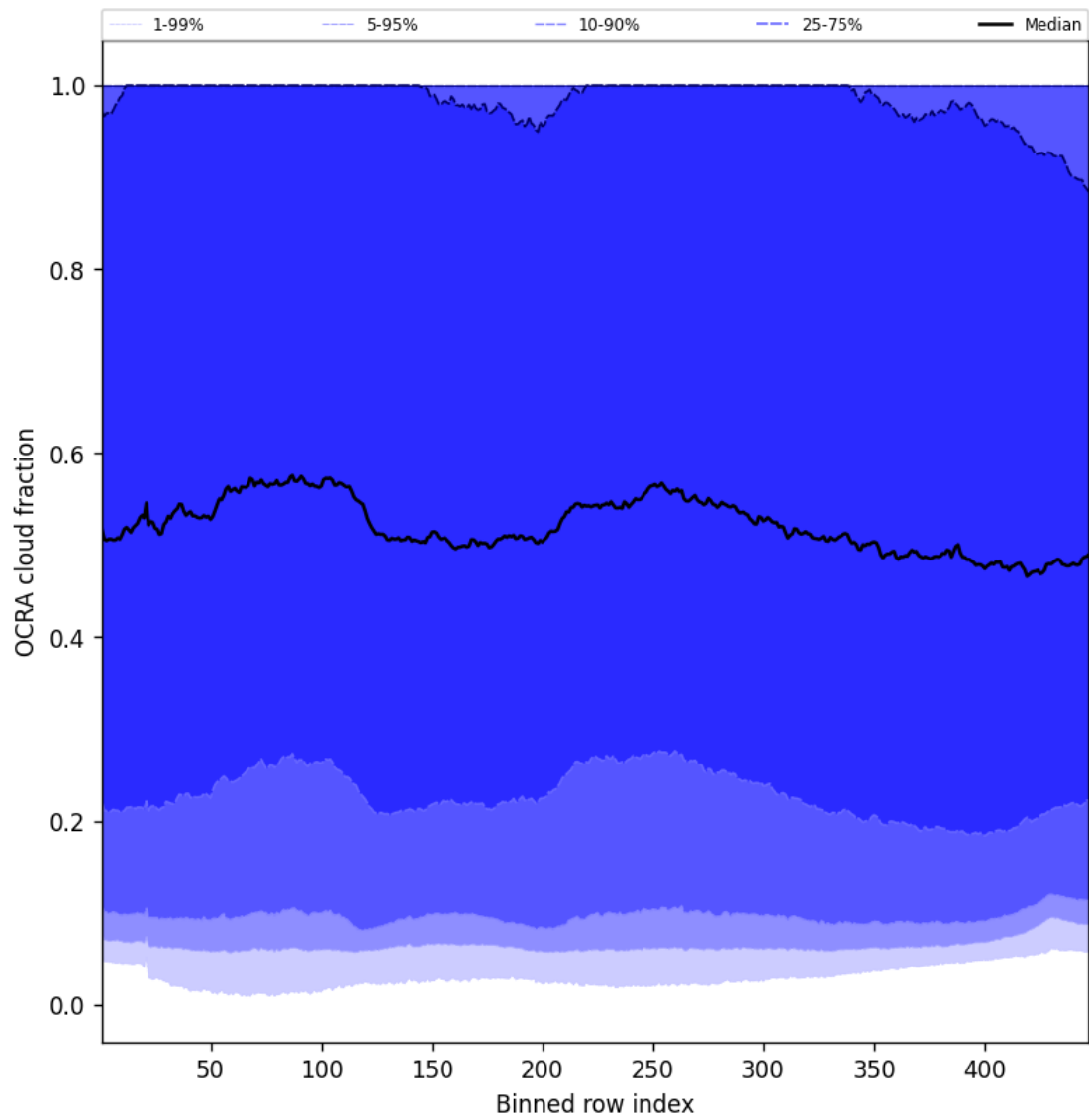
Figure 66: Along track statistics of “OCRA cloud fraction” for 2025-03-24 to 2025-03-26
