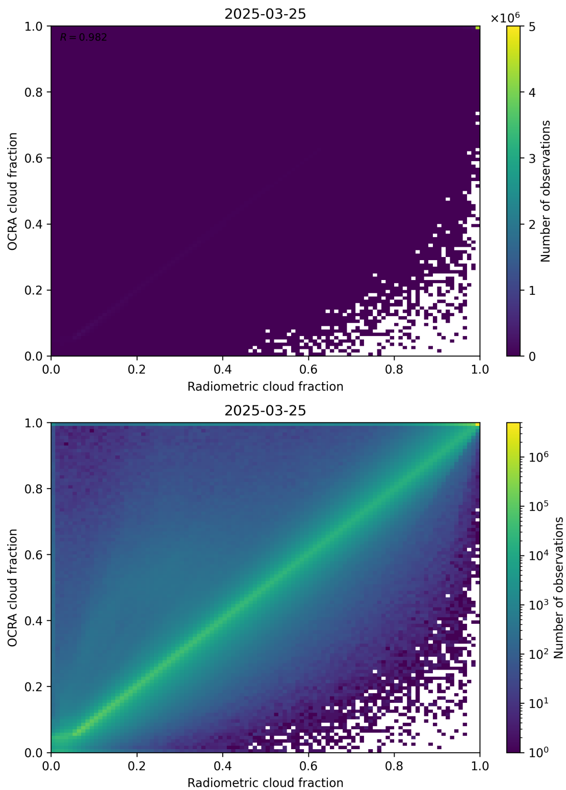
Figure 72: Scatter density plot of “Radiometric cloud fraction” against “OCRA cloud fraction” for 2025-03-24 to 2025-03-26.
