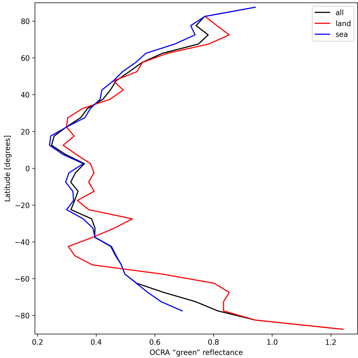
Figure 36: Zonal average of “OCRA “green” reflectance” for 2025-03-24 to 2025-03-26.
