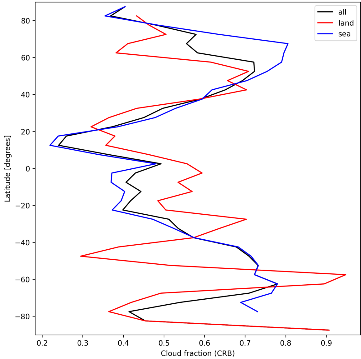
Figure 26: Zonal average of “Cloud fraction (CRB)” for 2025-03-24 to 2025-03-26.
