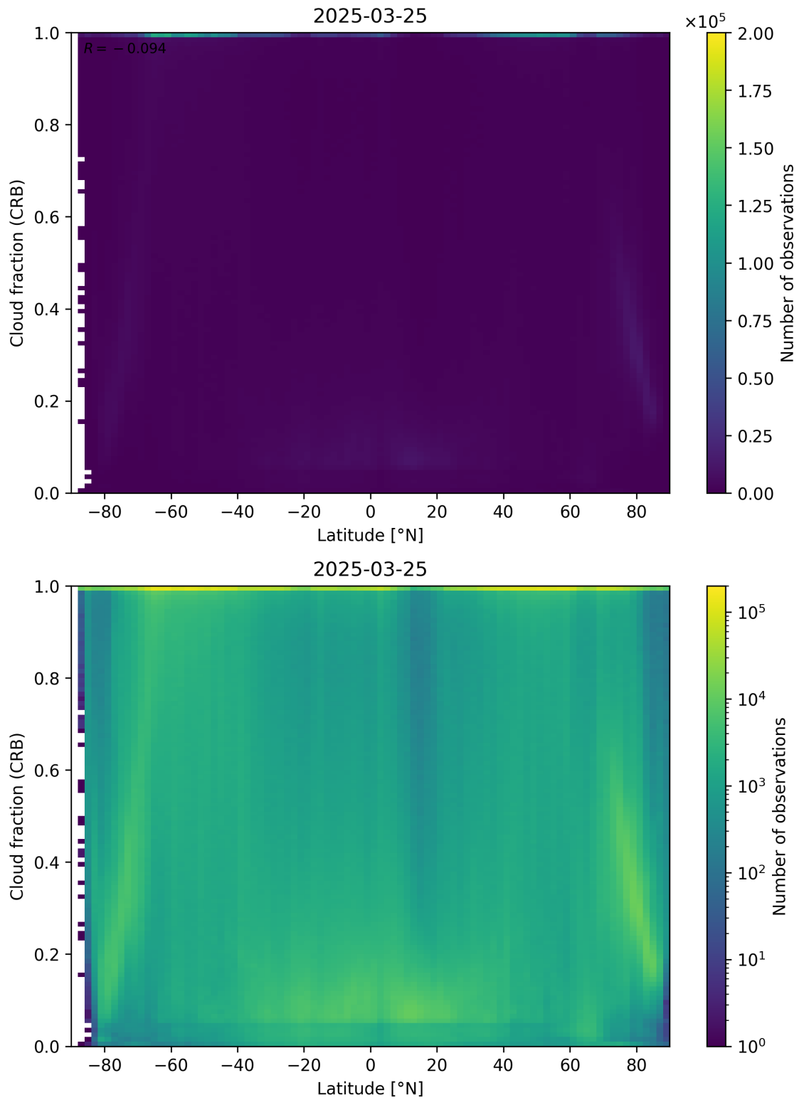
Figure 94: Scatter density plot of “Latitude” against “Cloud fraction (CRB)” for 2025-03-24 to 2025-03-26.
