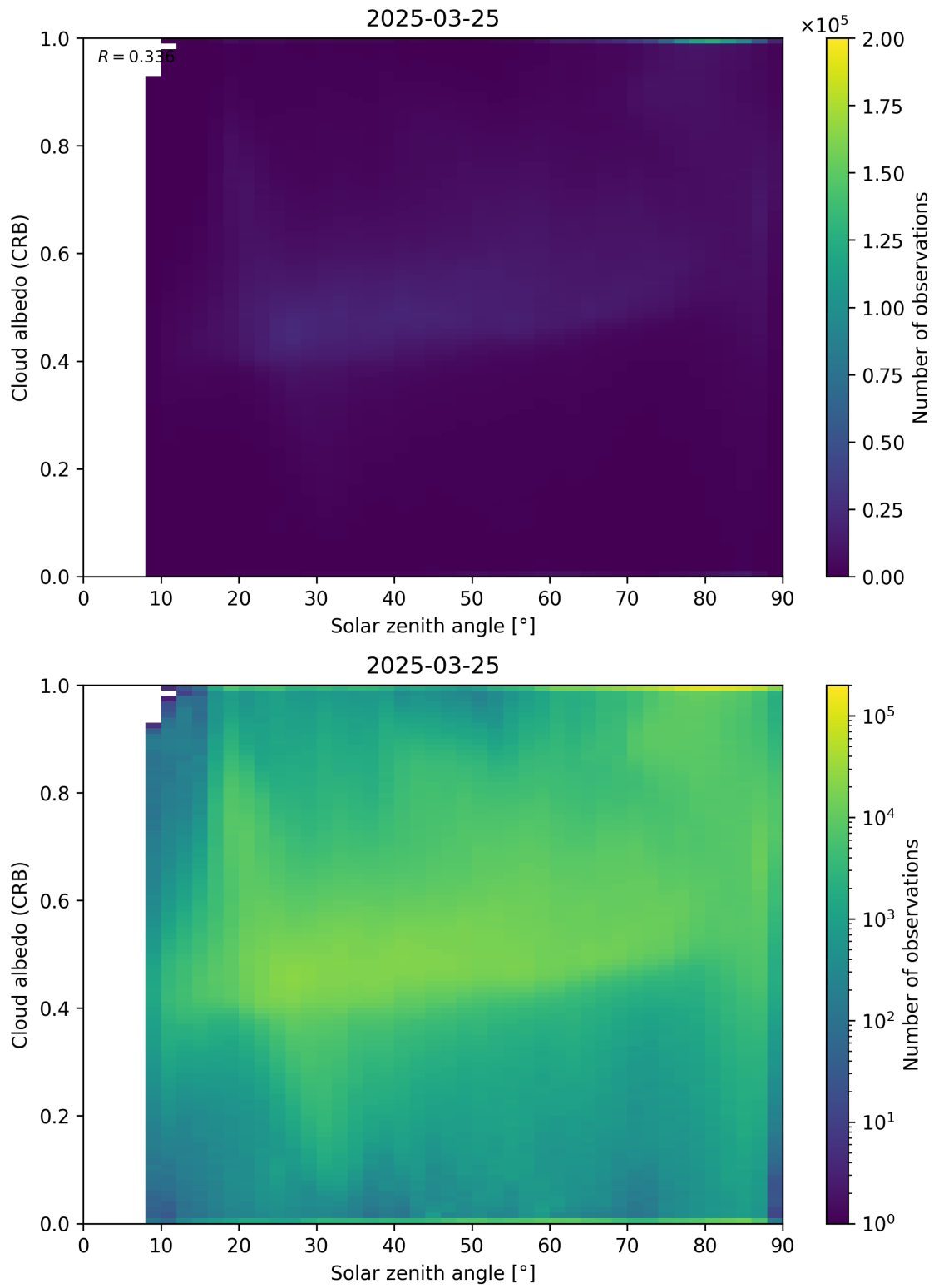
Figure 98: Scatter density plot of “Solar zenith angle” against “Cloud albedo (CRB)” for 2025-03-24 to 2025-03-26.
