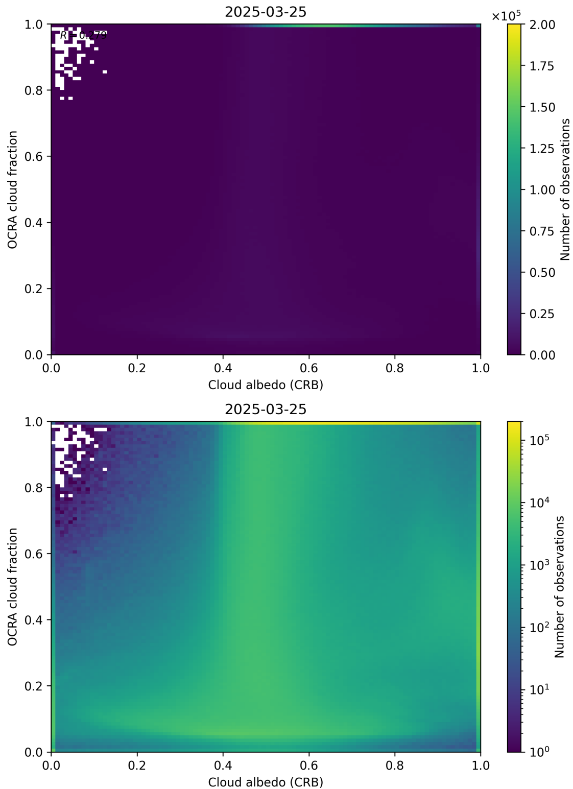
Figure 70: Scatter density plot of “Cloud albedo (CRB)” against “OCRA cloud fraction” for 2025-03-24 to 2025-03-26.
