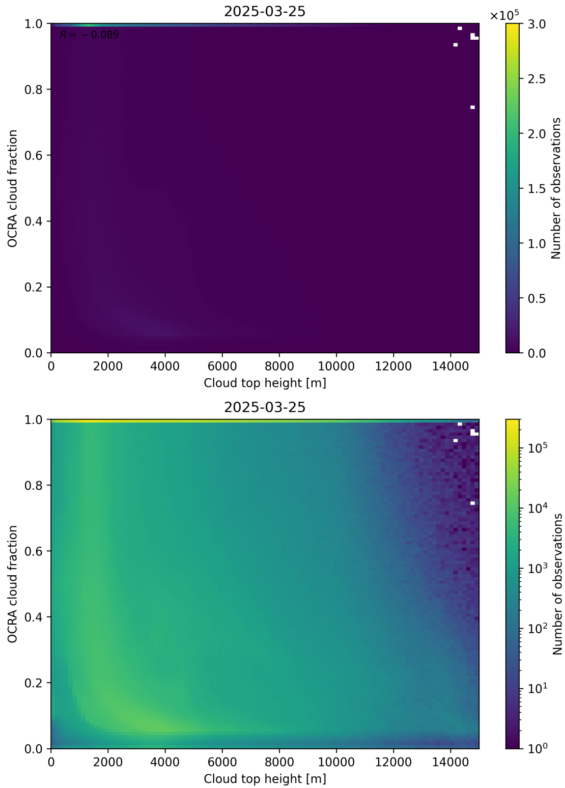
Figure 87: Scatter density plot of “Cloud top height” against “OCRA cloud fraction” for 2025-03-24 to 2025-03-26.
