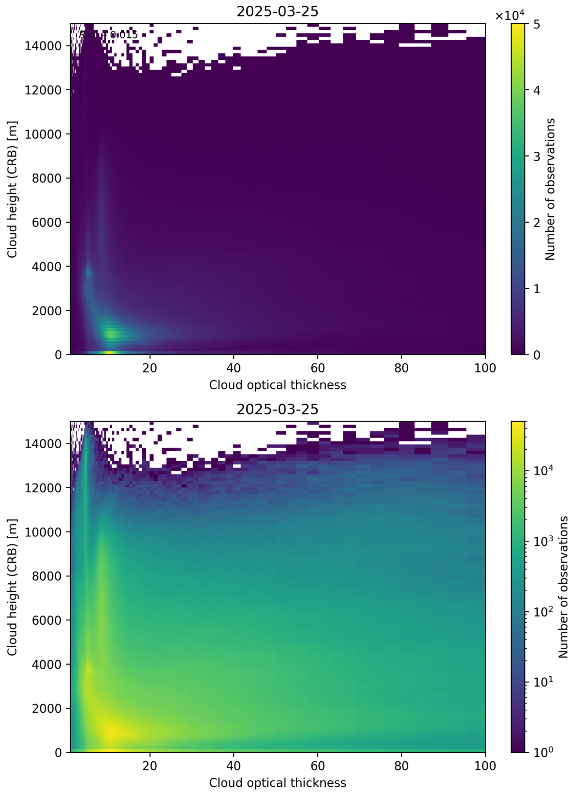
Figure 85: Scatter density plot of “Cloud optical thickness” against “Cloud height (CRB)” for 2025-03-24 to 2025-03-26.
