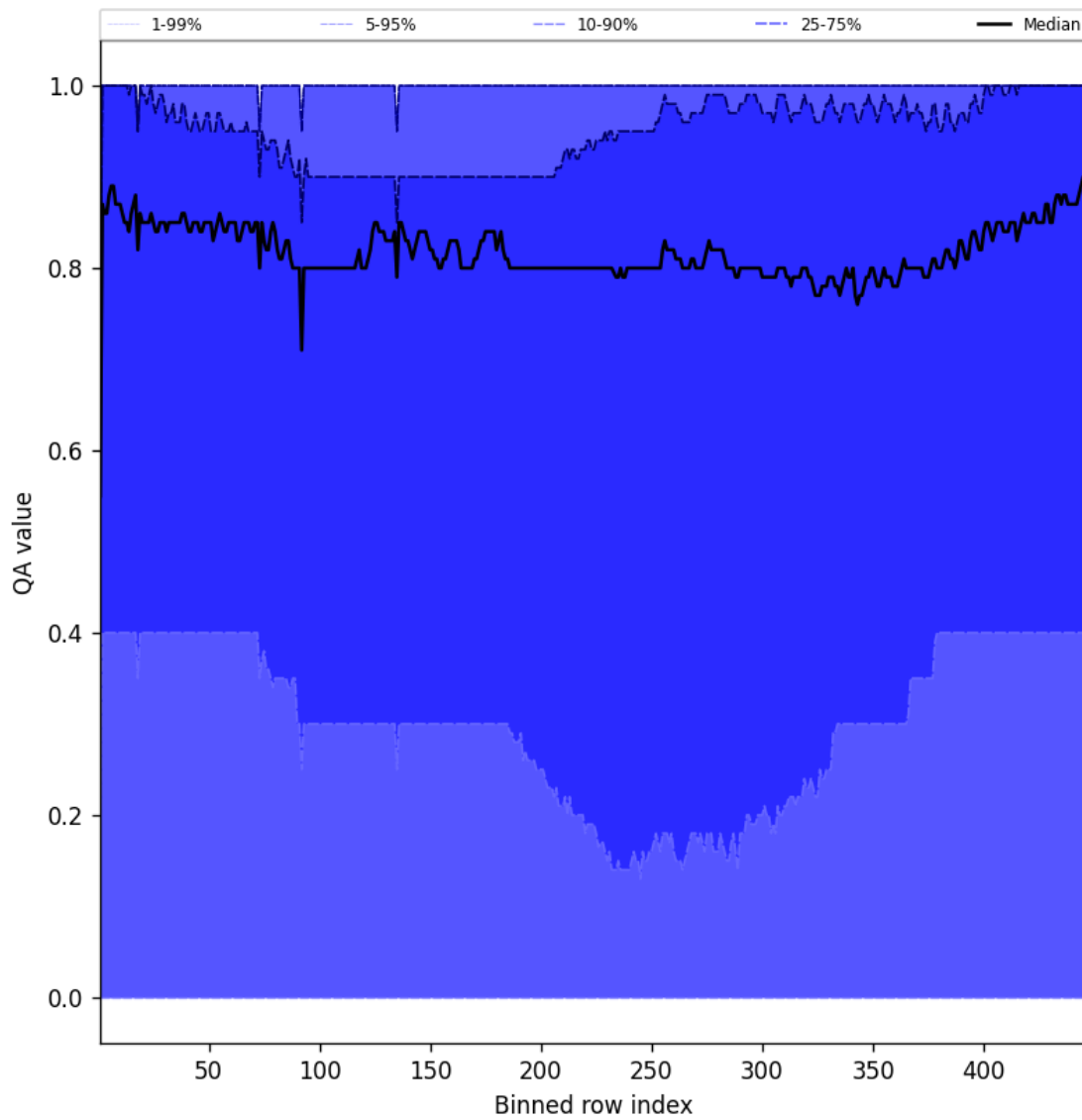
Figure 54: Along track statistics of "QA value" for 2025-03-24 to 2025-03-26
