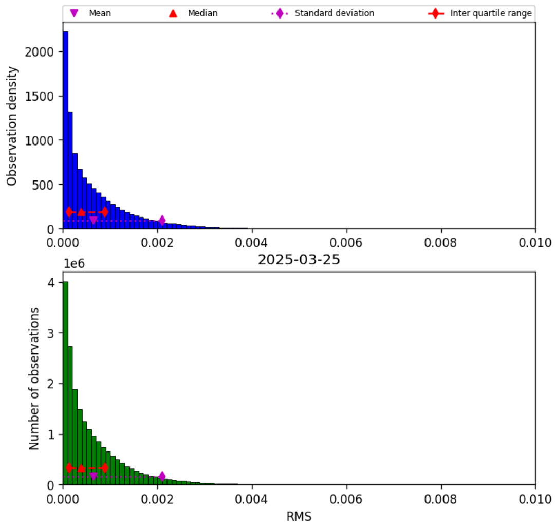
Figure 47: Histogram of “RMS” for 2025-03-24 to 2025-03-26
