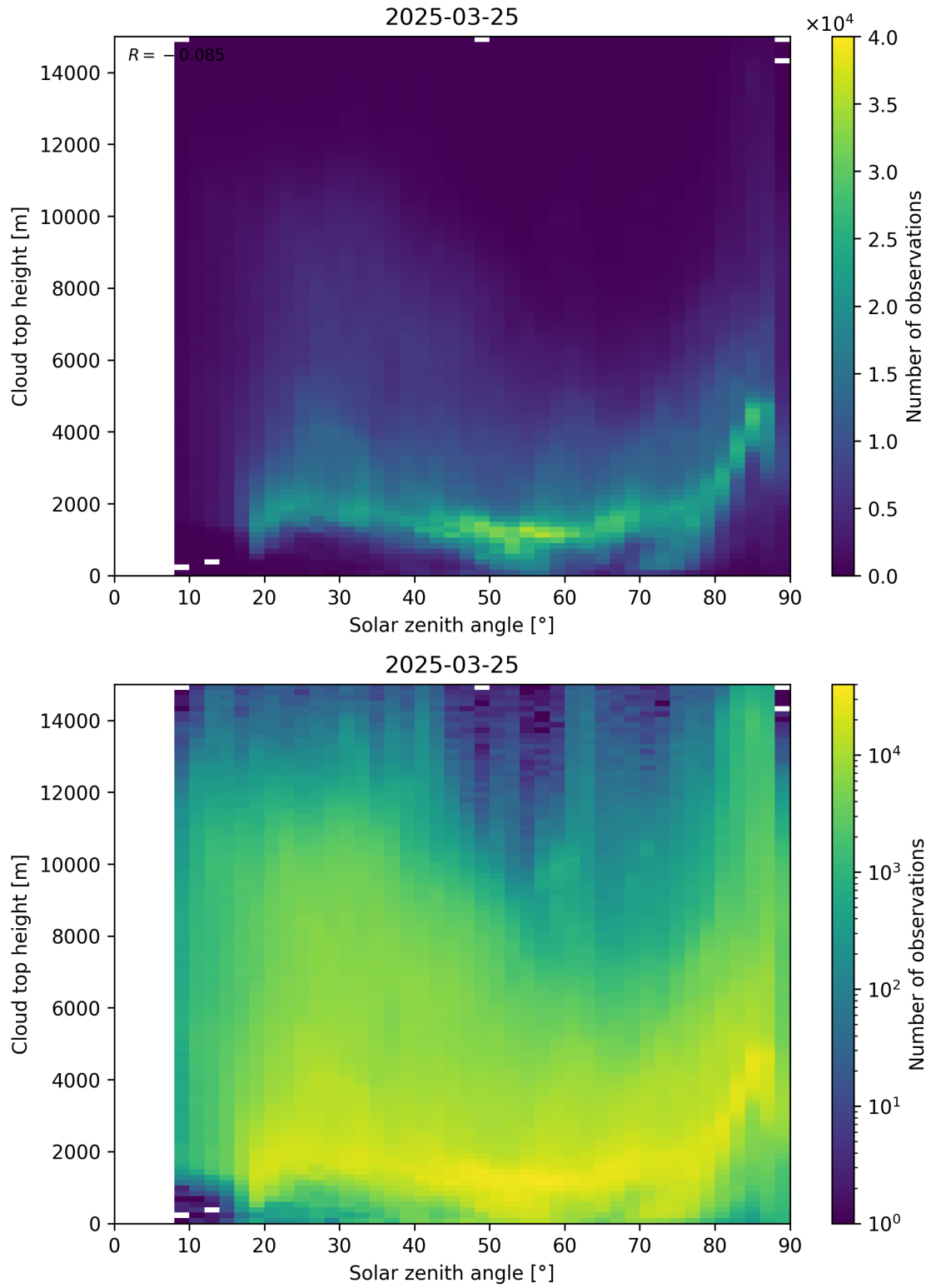
Figure 104: Scatter density plot of “Solar zenith angle” against “Cloud top height” for 2025-03-24 to 2025-03-26.
