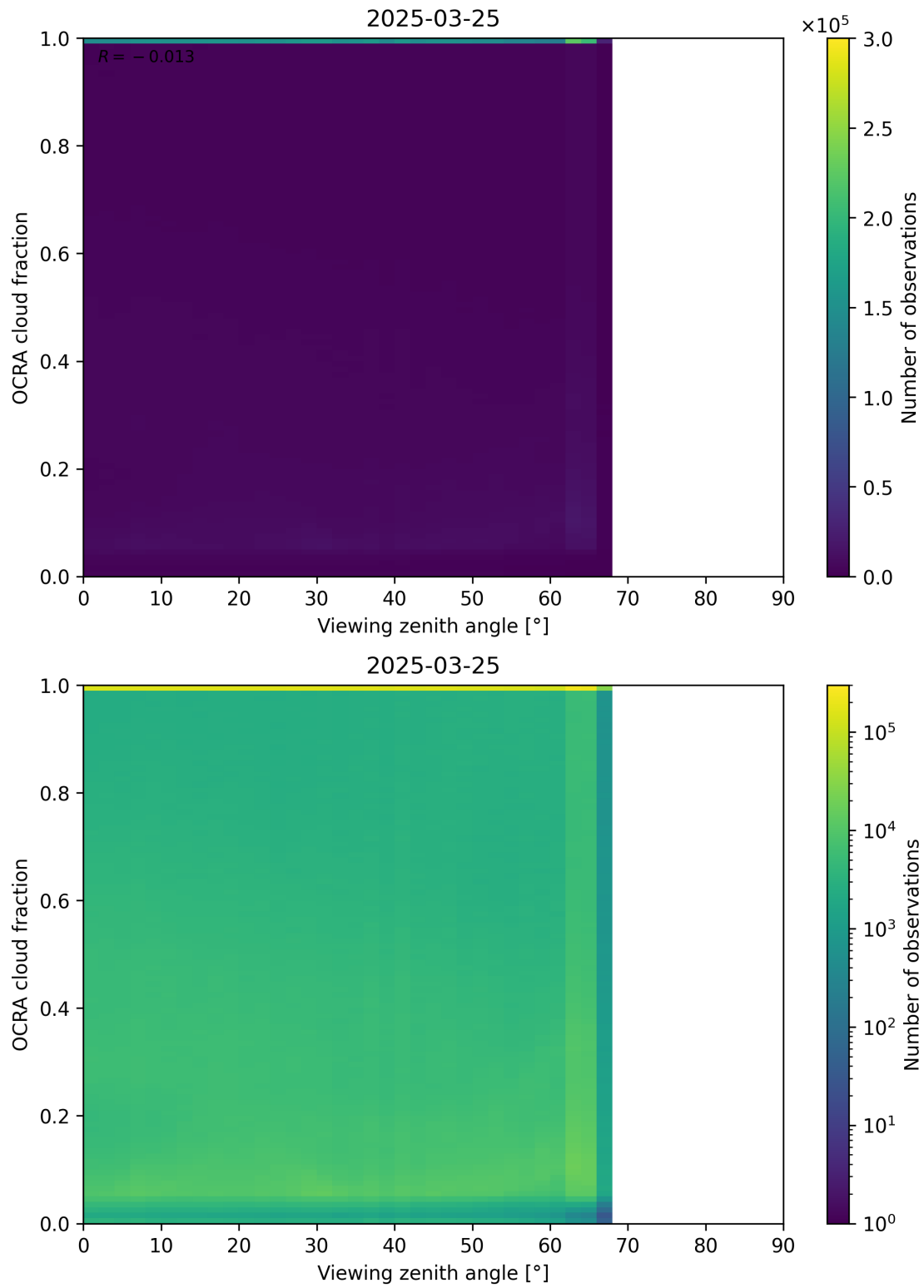
Figure 108: Scatter density plot of “Viewing zenith angle” against “OCRA cloud fraction” for 2025-03-24 to 2025-03-26.
