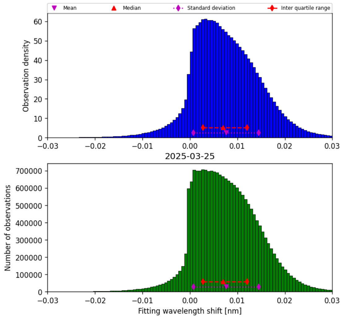
Figure 49: Histogram of “Fitting wavelength shift” for 2025-03-24 to 2025-03-26
