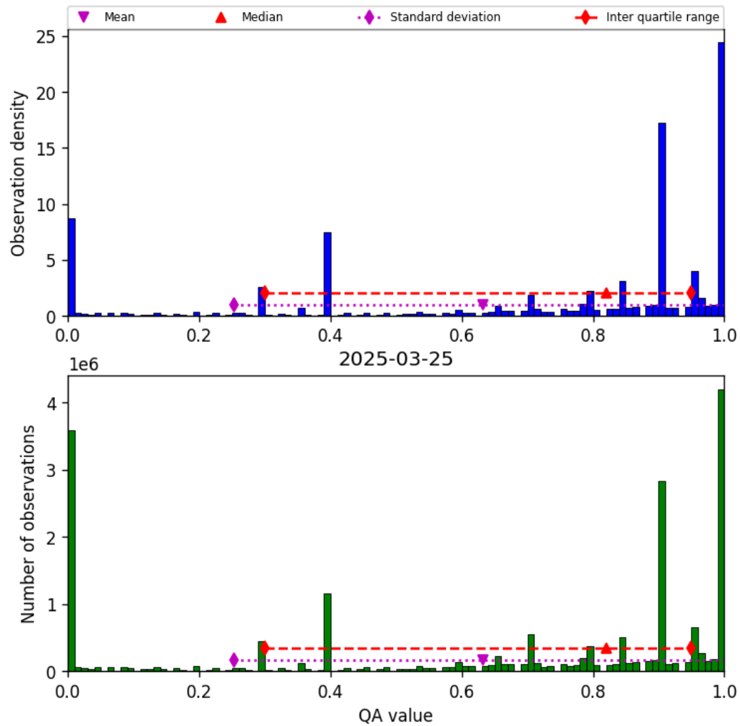
Figure 38: Histogram of “QA value” for 2025-03-24 to 2025-03-26
