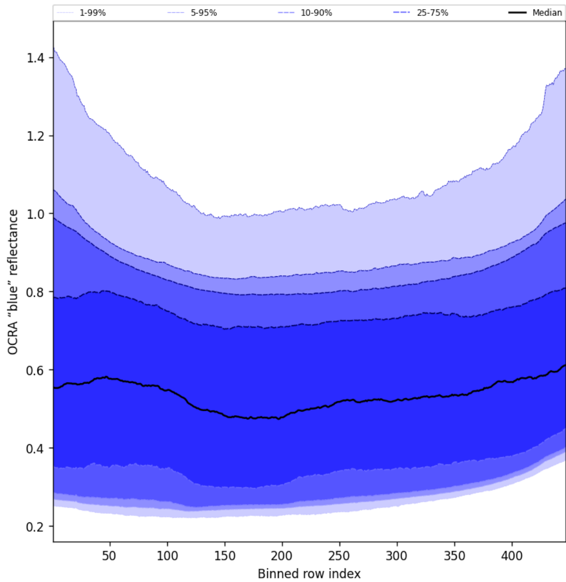
Figure 67: Along track statistics of “OCRA “blue” reflectance” for 2025-03-24 to 2025-03-26
