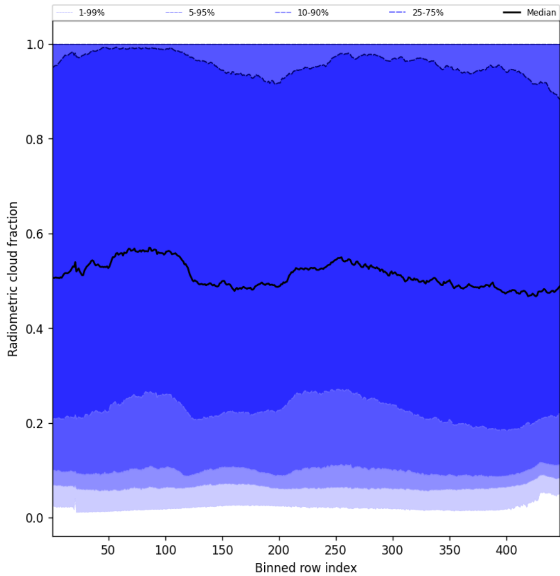
Figure 55: Along track statistics of “Radiometric cloud fraction” for 2025-03-24 to 2025-03-26
