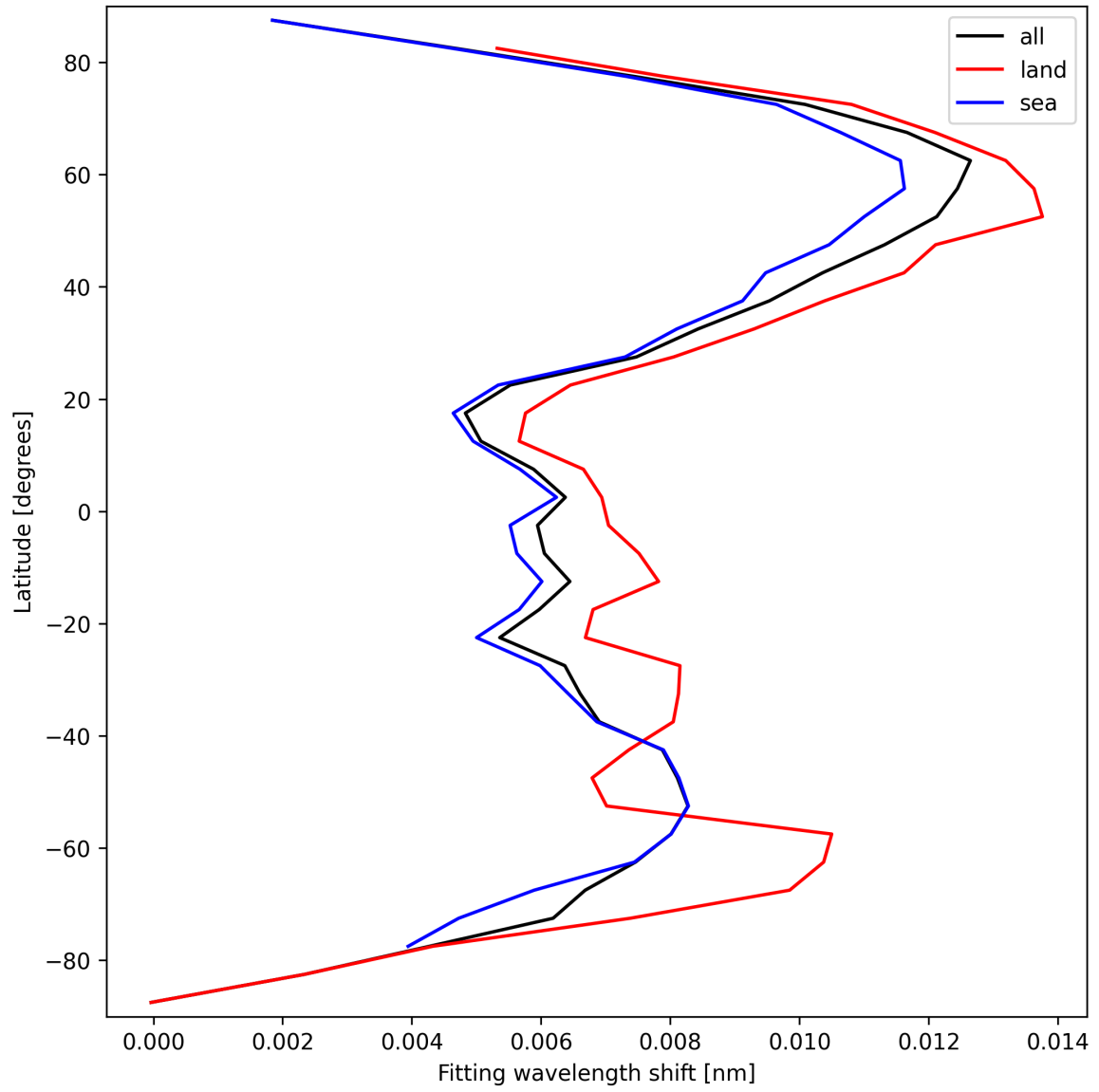
Figure 33: Zonal average of “Fitting wavelength shift” for 2025-03-24 to 2025-03-26.
