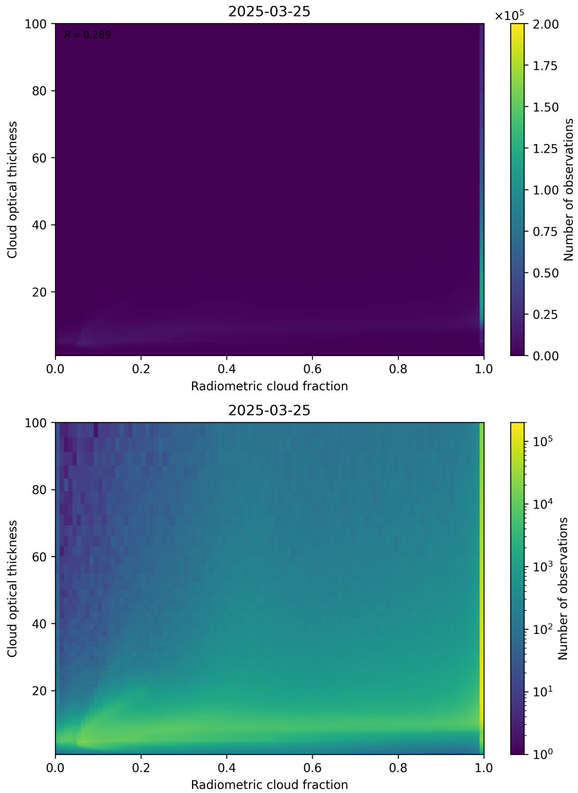
Figure 75: Scatter density plot of “Radiometric cloud fraction” against “Cloud optical thickness” for 2025-03-24 to 2025-03-26.
