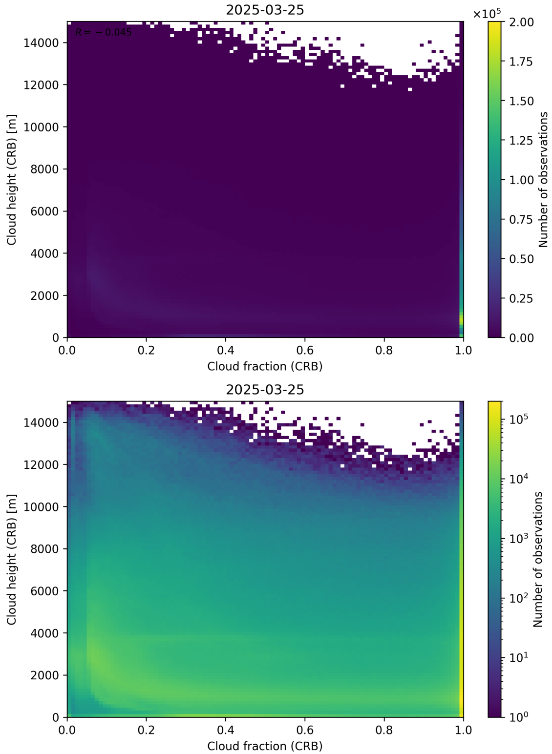
Figure 79: Scatter density plot of “Cloud fraction (CRB)” against “Cloud height (CRB)” for 2025-03-24 to 2025-03-26.
