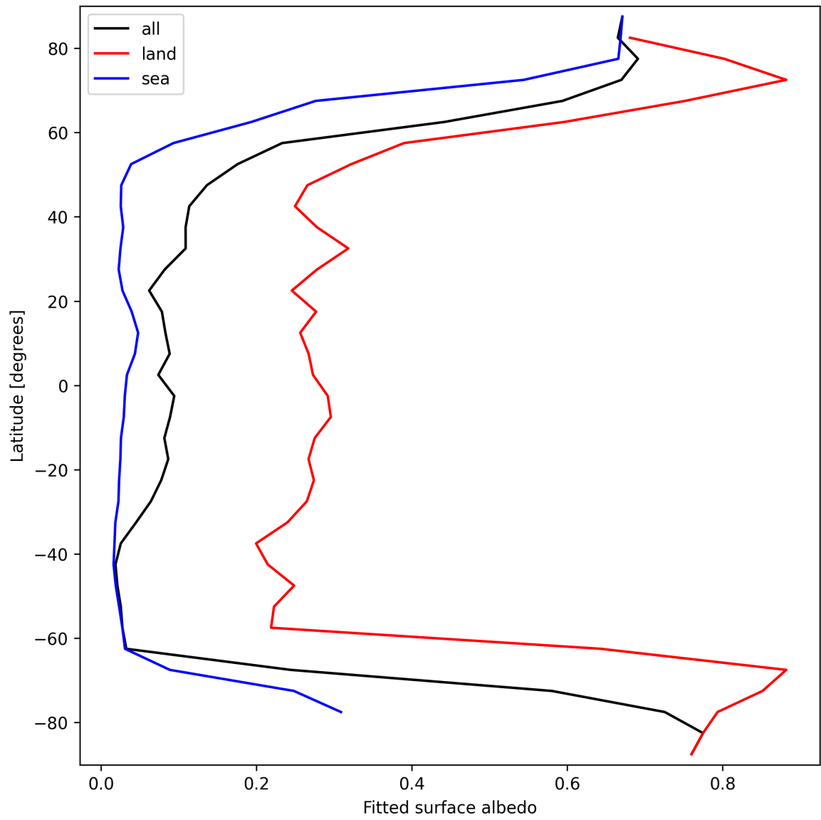
Figure 29: Zonal average of “Fitted surface albedo” for 2025-03-24 to 2025-03-26.
