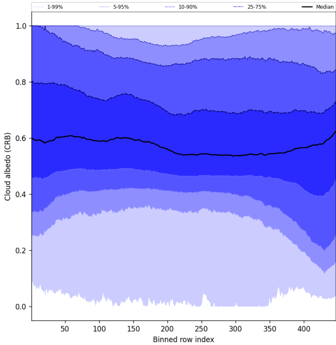
Figure 60: Along track statistics of “Cloud albedo (CRB)” for 2025-03-24 to 2025-03-26
