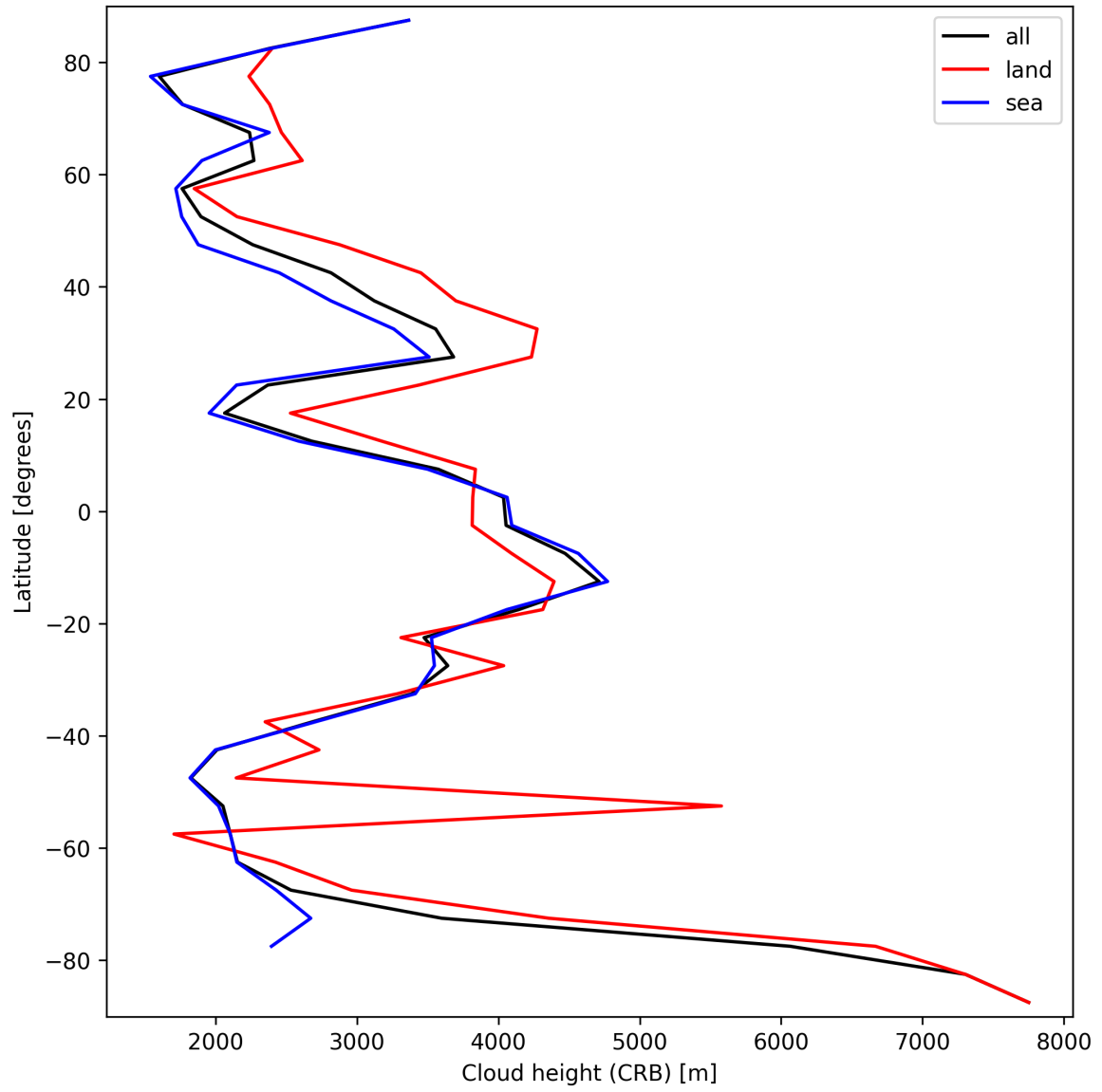
Figure 27: Zonal average of “Cloud height (CRB)” for 2025-03-24 to 2025-03-26.
