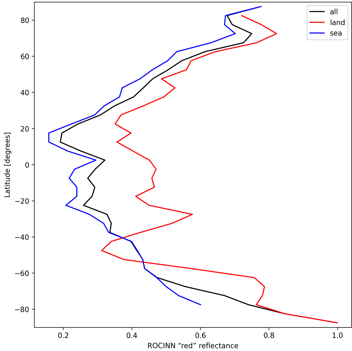
Figure 37: Zonal average of "ROCINN "red" reflectance" for 2025-03-24 to 2025-03-26.
