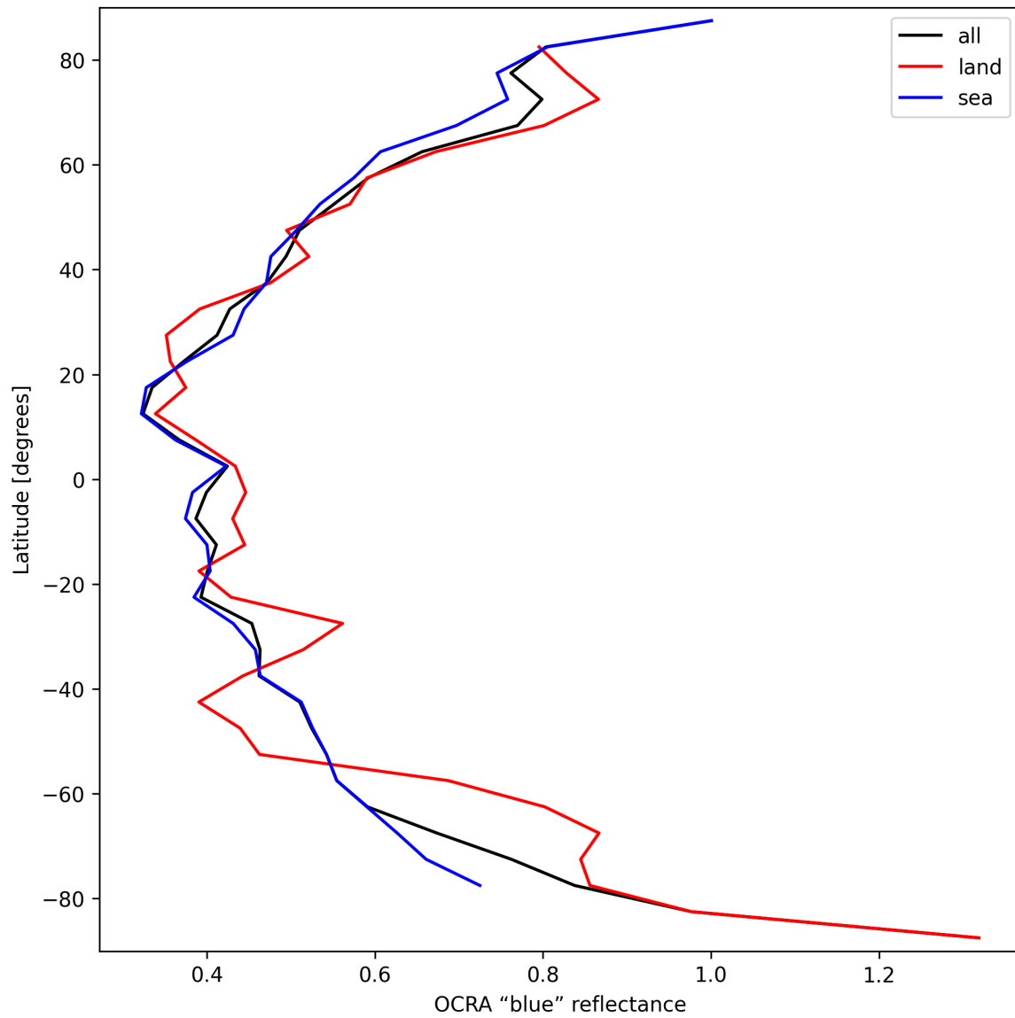
Figure 35: Zonal average of "OCRA "blue" reflectance" for 2025-03-24 to 2025-03-26.
