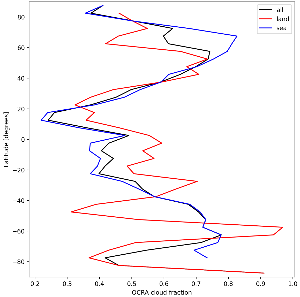
Figure 34: Zonal average of “OCRA cloud fraction” for 2025-03-24 to 2025-03-26.
