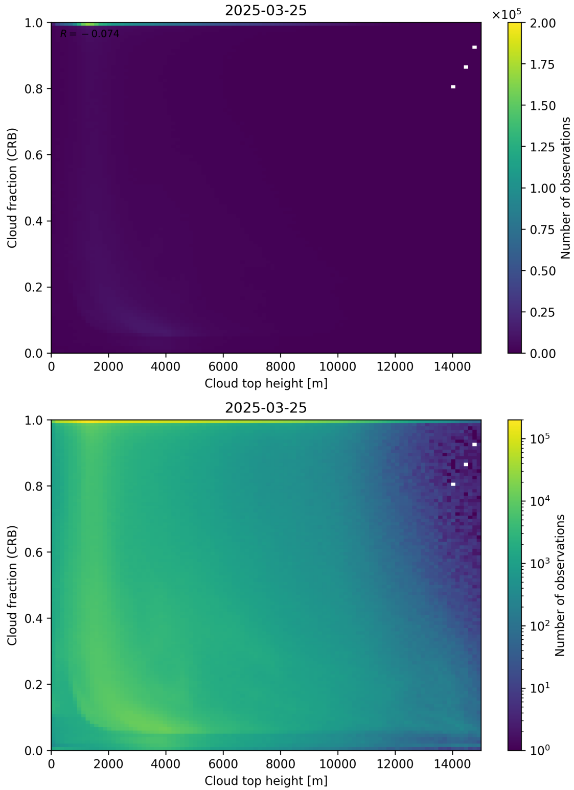
Figure 88: Scatter density plot of “Cloud top height” against “Cloud fraction (CRB)” for 2025-03-24 to 2025-03-26.
