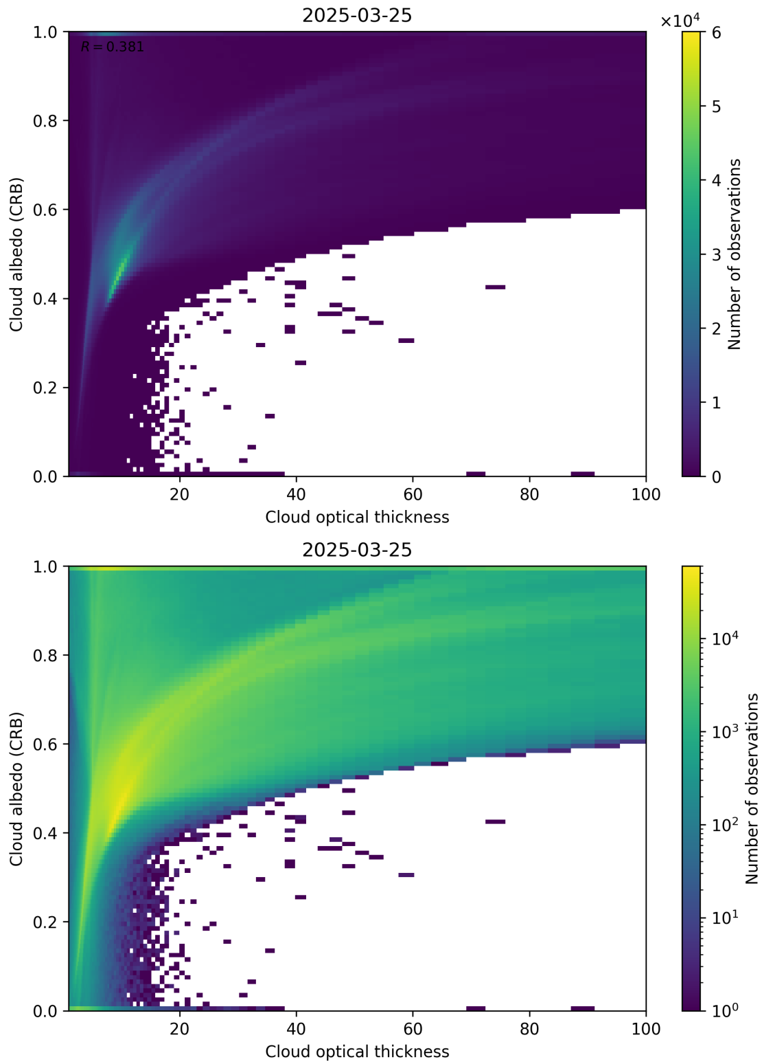
Figure 82: Scatter density plot of “Cloud optical thickness” against “Cloud albedo (CRB)” for 2025-03-24 to 2025-03-26.
