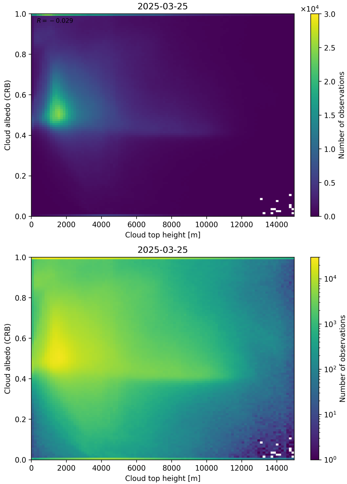
Figure 86: Scatter density plot of “Cloud top height” against “Cloud albedo (CRB)” for 2025-03-24 to 2025-03-26.
