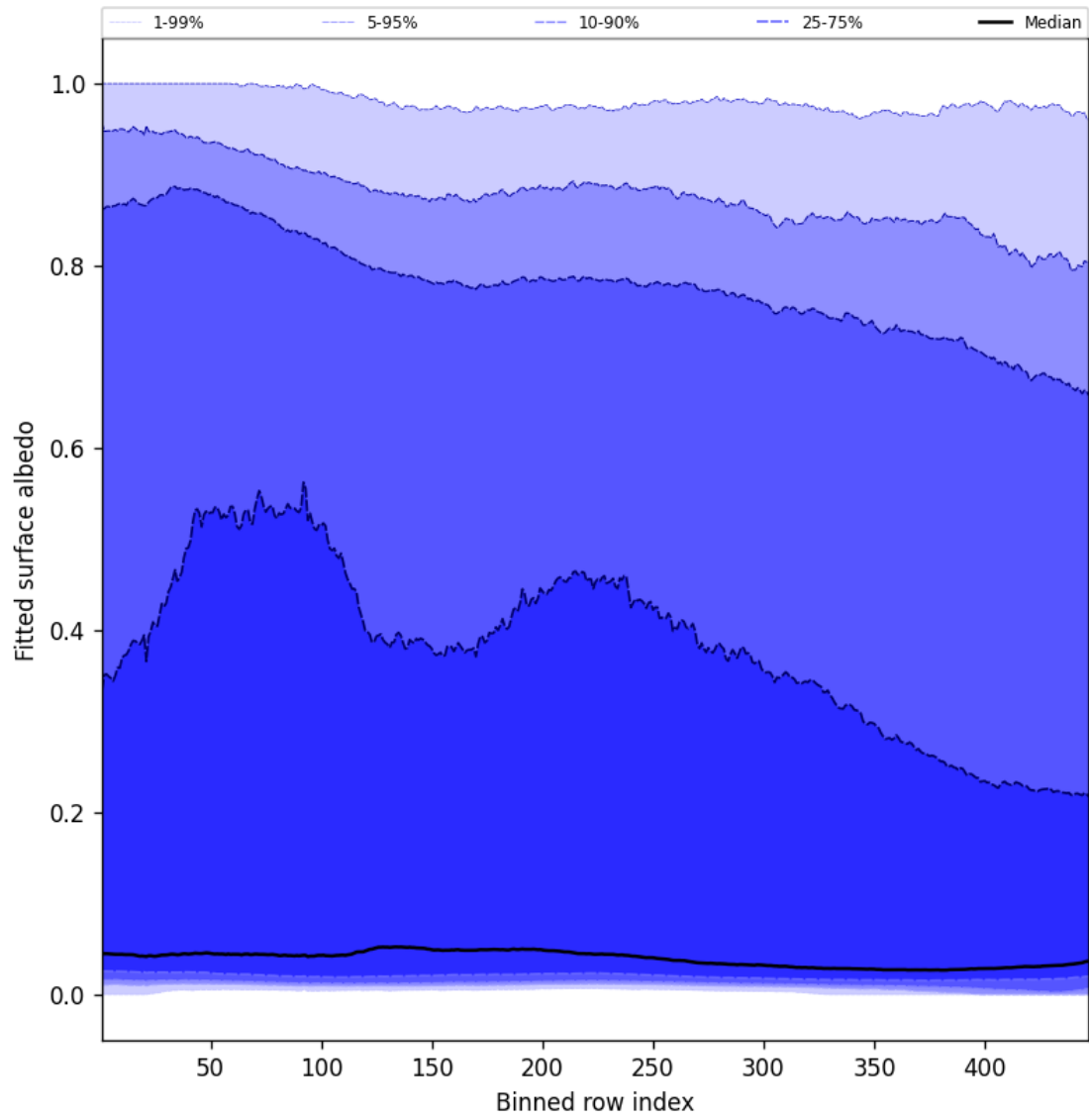
Figure 61: Along track statistics of “Fitted surface albedo” for 2025-03-24 to 2025-03-26
