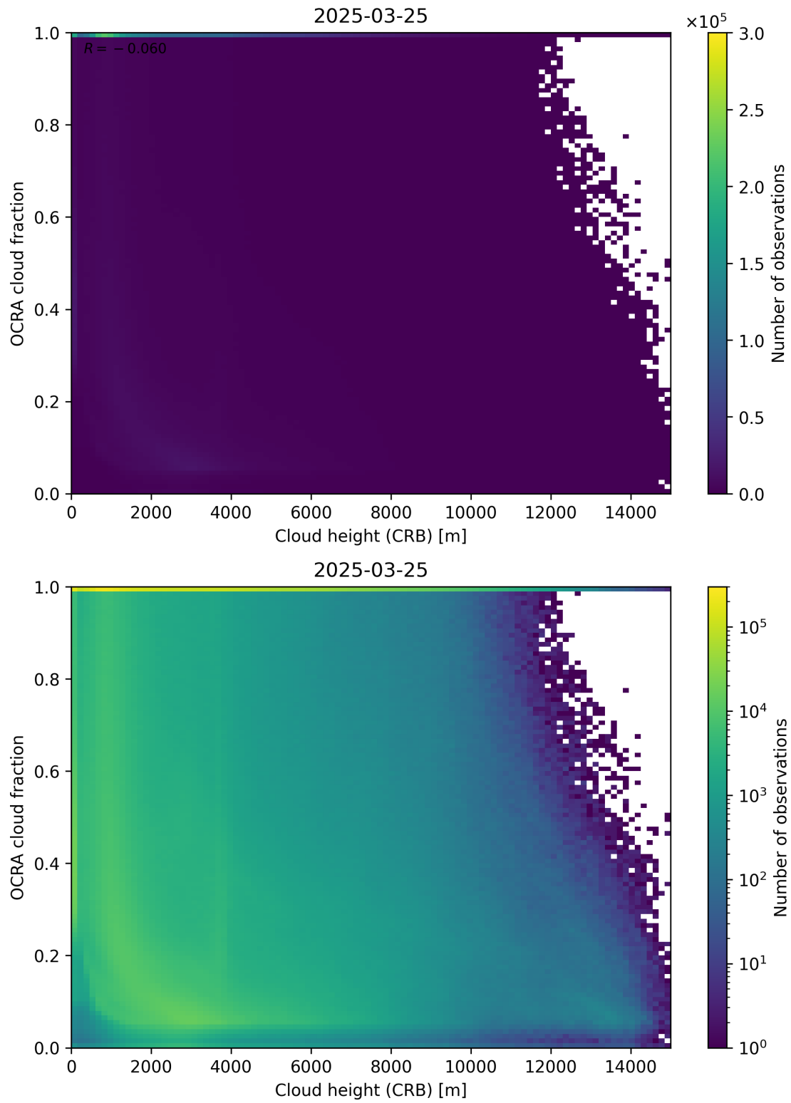
Figure 81: Scatter density plot of “Cloud height (CRB)” against “OCRA cloud fraction” for 2025-03-24 to 2025-03-26.
