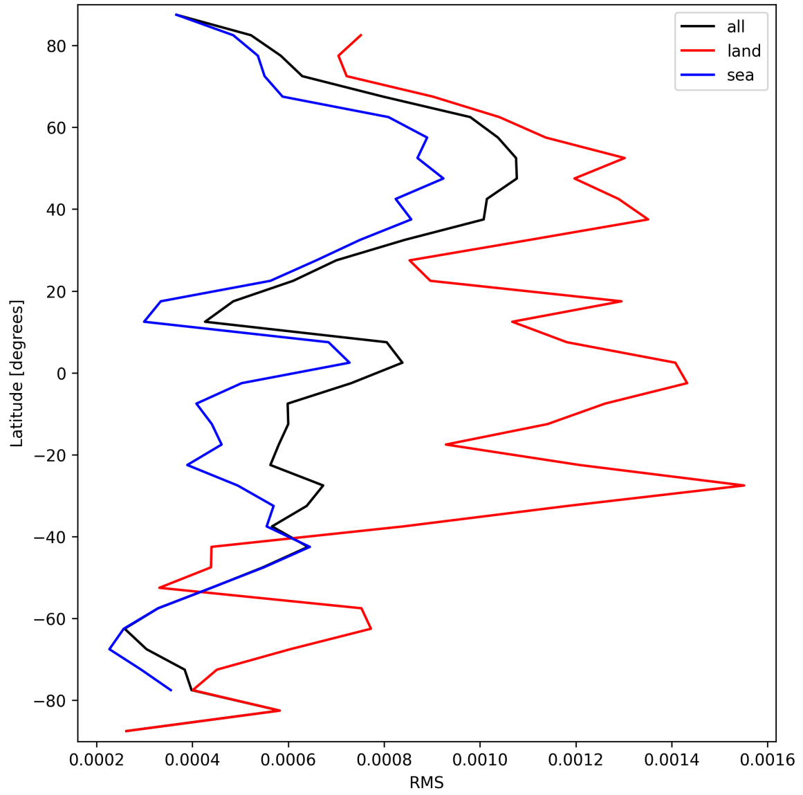
Figure 31: Zonal average of “RMS” for 2025-03-24 to 2025-03-26.
