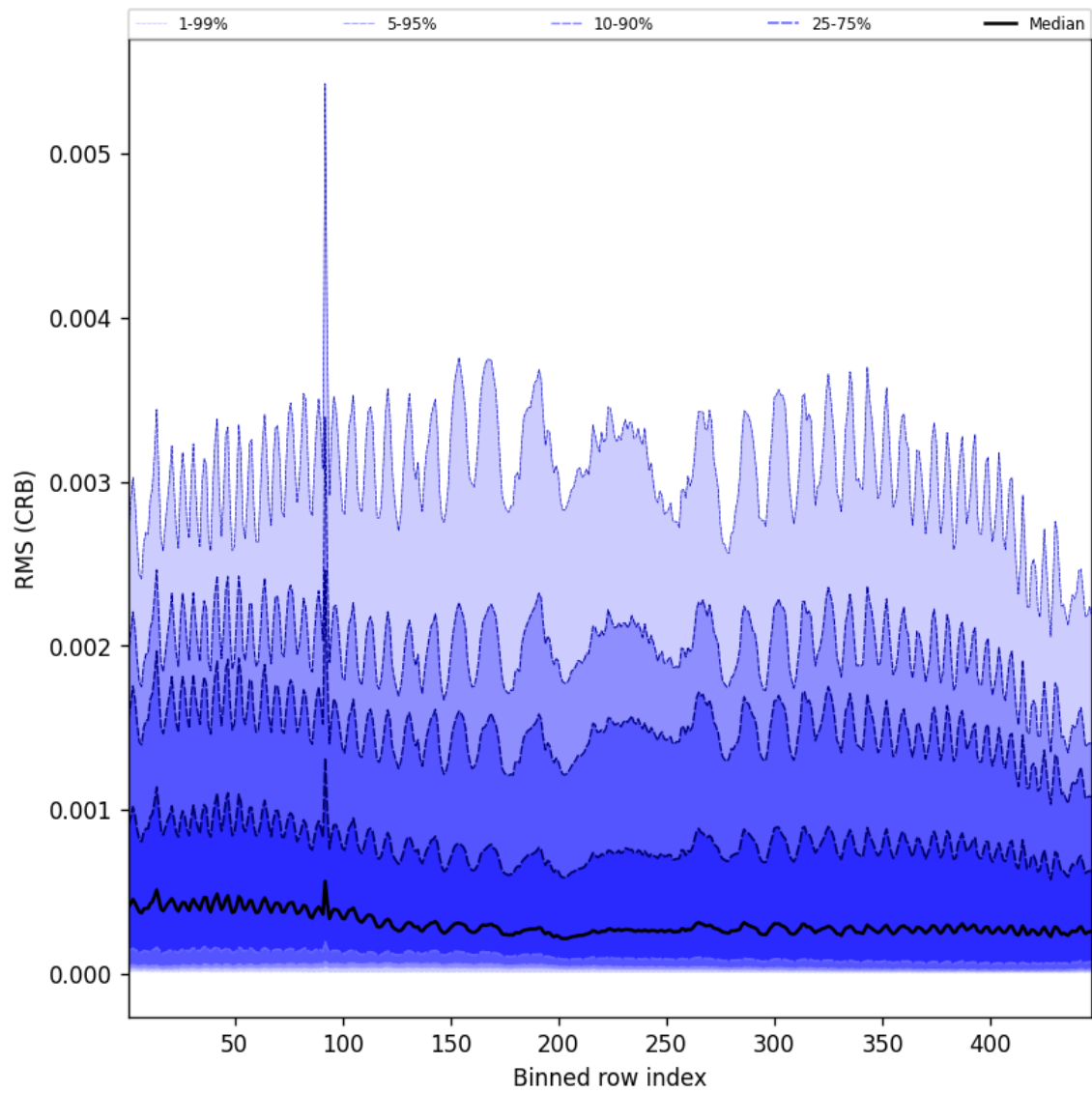
Figure 64: Along track statistics of “RMS (CRB)” for 2025-03-24 to 2025-03-26
