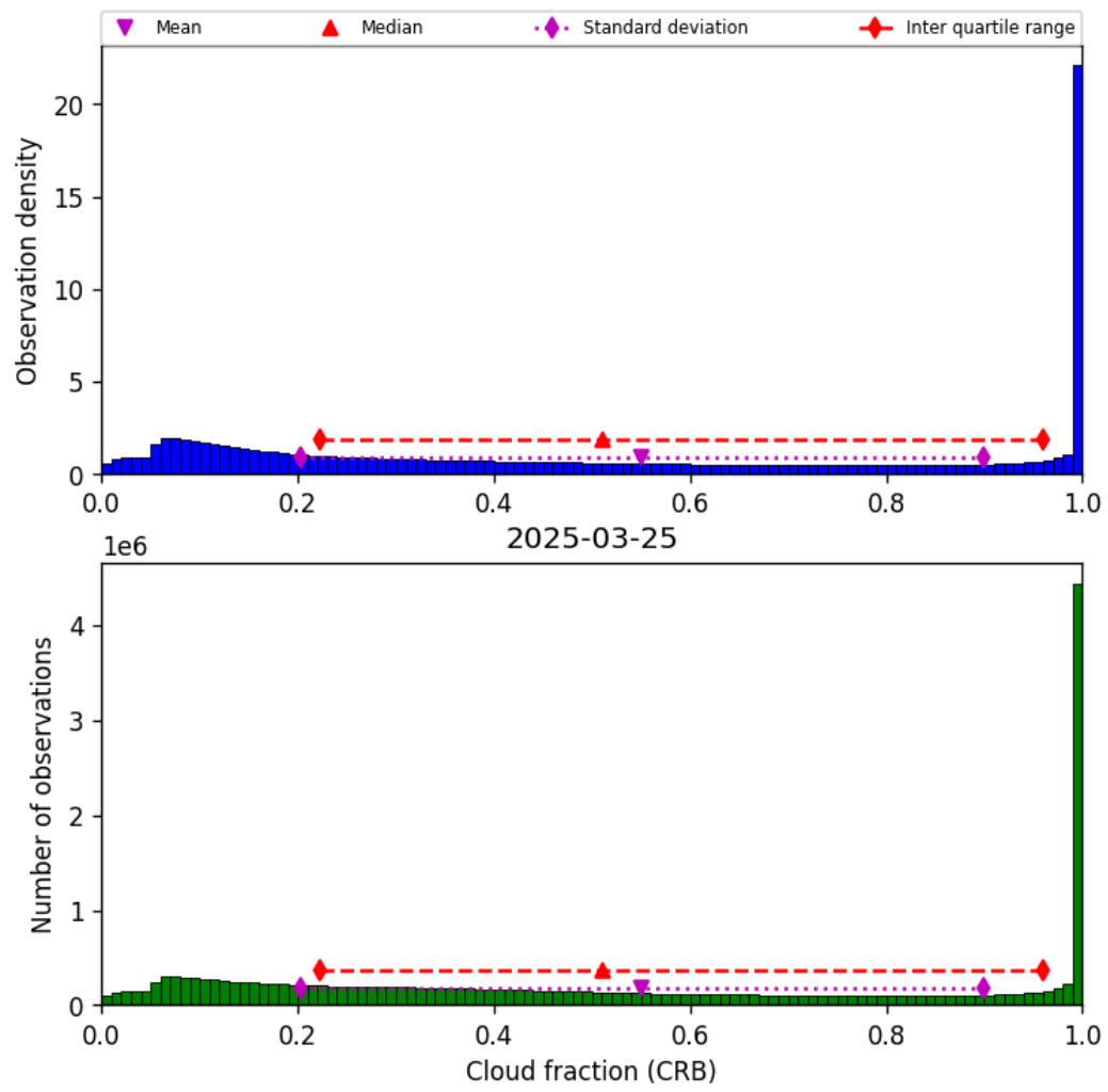
Figure 42: Histogram of “Cloud fraction (CRB)” for 2025-03-24 to 2025-03-26
