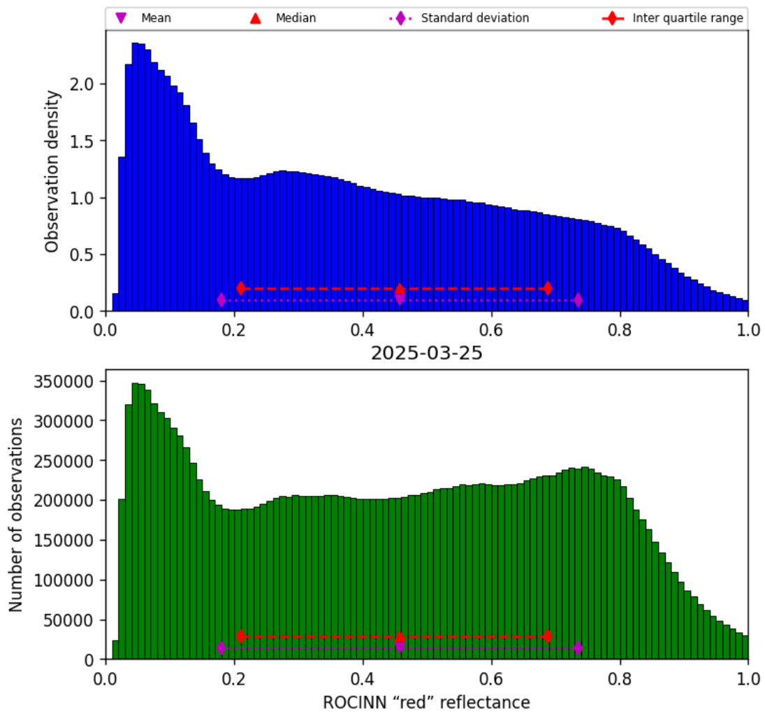
Figure 53: Histogram of “ROCINN “red” reflectance” for 2025-03-24 to 2025-03-26
