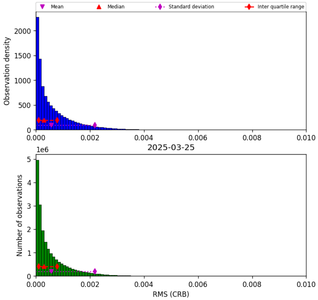
Figure 48: Histogram of “RMS (CRB)” for 2025-03-24 to 2025-03-26
