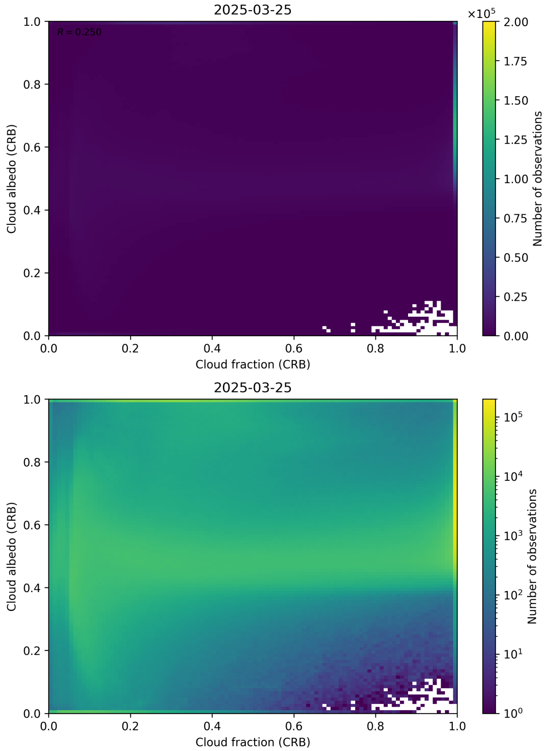
Figure 77: Scatter density plot of “Cloud fraction (CRB)” against “Cloud albedo (CRB)” for 2025-03-24 to 2025-03-26.
