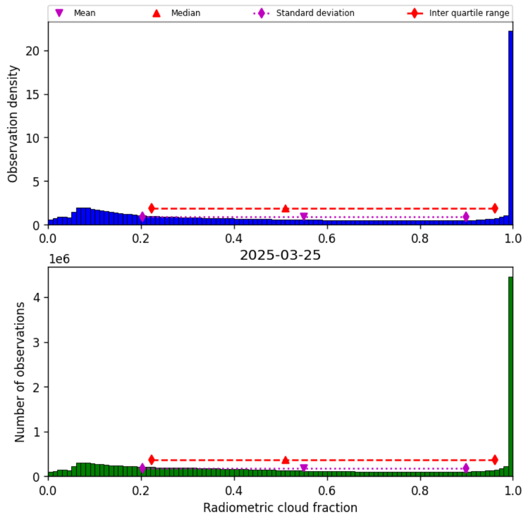
Figure 39: Histogram of “Radiometric cloud fraction” for 2025-03-24 to 2025-03-26
