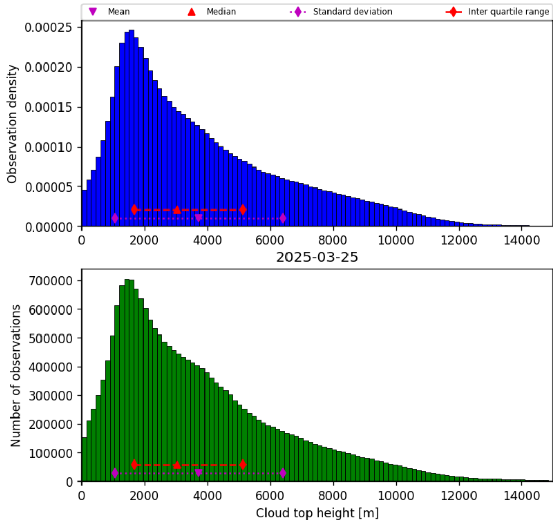
Figure 40: Histogram of “Cloud top height” for 2025-03-24 to 2025-03-26
