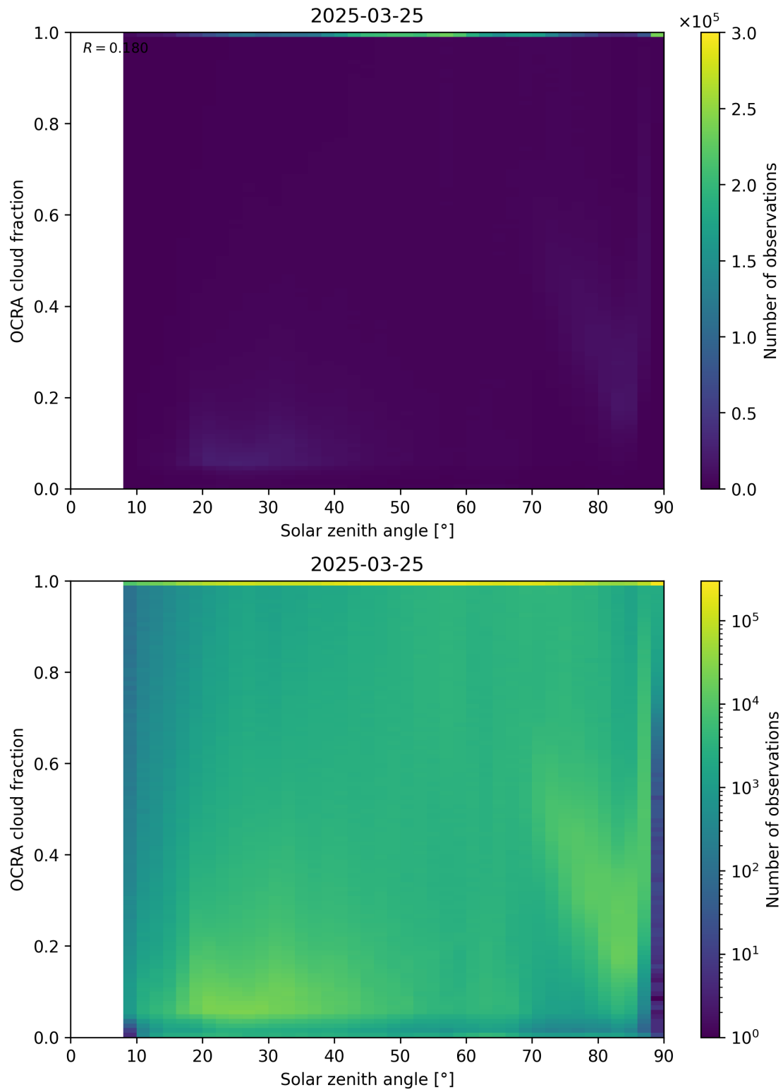
Figure 100: Scatter density plot of “Solar zenith angle” against “OCRA cloud fraction” for 2025-03-24 to 2025-03-26.
