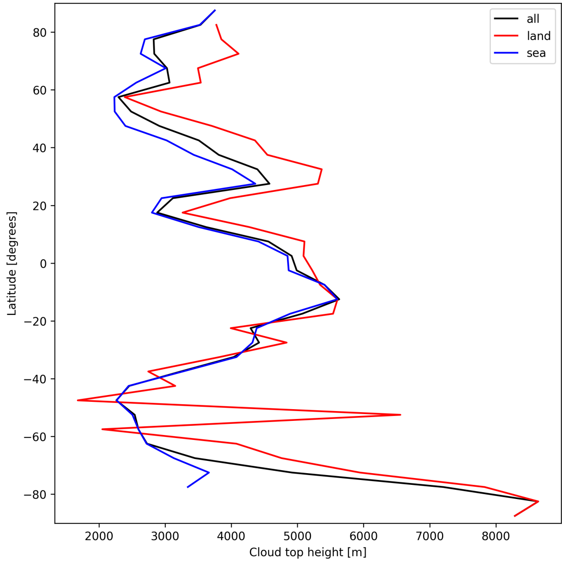
Figure 24: Zonal average of “Cloud top height” for 2025-03-24 to 2025-03-26.
